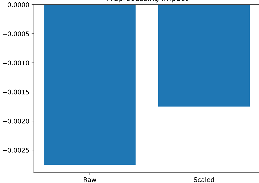
Preprocessing Impact
