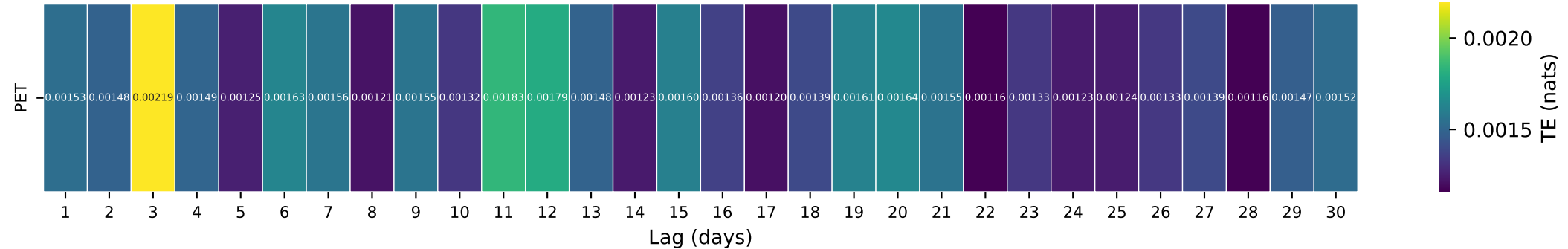
Gauge ID: 01187300 | HUBBARD RIVER NR. WEST HARTLAND, CT. | PET(t-\tau) \rightarrow Q(t)
