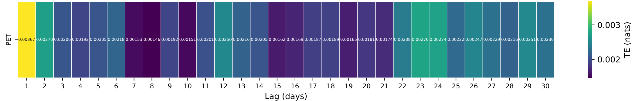
Gauge ID: 04122200 | WHITE RIVER NEAR WHITEHALL, MI | PET(t-\tau) \rightarrow Q(t)
