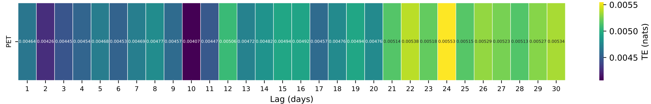
Gauge ID: 11476600 | BULL C NR WEOTT CA | PET(t- \tau ) \rightarrow Q(t)
