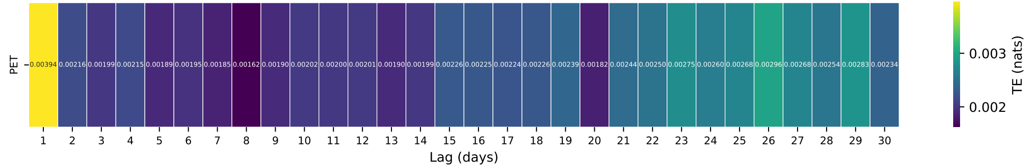
Gauge ID: 02479560 | ESCATAWPA RIVER NEAR AGRICOLA MS | PET(t-\tau) \rightarrow Q(t)
