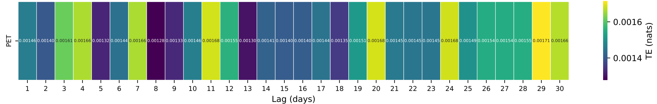
Gauge ID: 09497800 | CIBECUE CREEK NEAR CHYSOTILE, AZ. | PET(t-\tau) \rightarrow Q(t)
