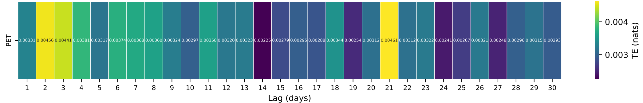
Gauge ID: 08324000 | JEMEZ RIVER NEAR JEMEZ, NM | PET(t-\tau) \rightarrow Q(t)
