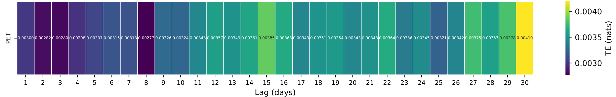
Gauge ID: 11141280 | LOPEZ C NR ARROYO GRANDE CA | PET(t- \tau ) \rightarrow Q(t)
