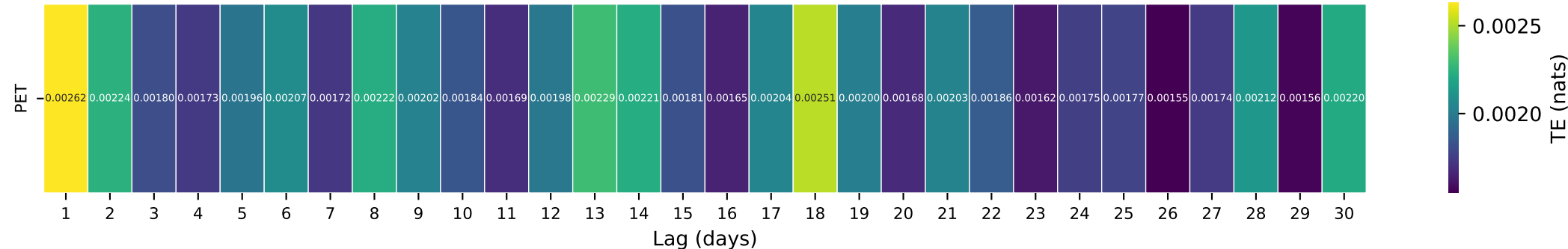
Gauge ID: 04256000 | INDEPENDENCE RIVER AT DONNATTSBURG NY | PET(t-τ) → Q(t)
