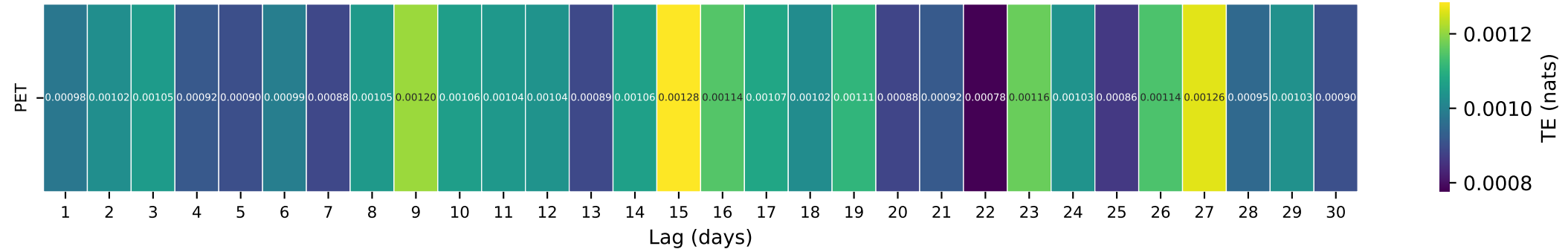
Gauge ID: 06803510 | LITTLE SALT CREEK NEAR LINCOLN, NEBR. | PET(t-\tau) \rightarrow Q(t)
