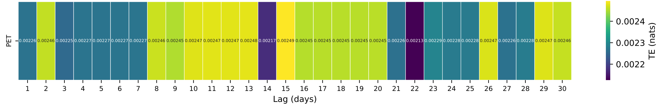
Gauge ID: 14182500 | LITTLE NORTH SANTIAM RIVER NEAR MEHAMA, OR | PET(t-\tau) \rightarrow Q(t)
