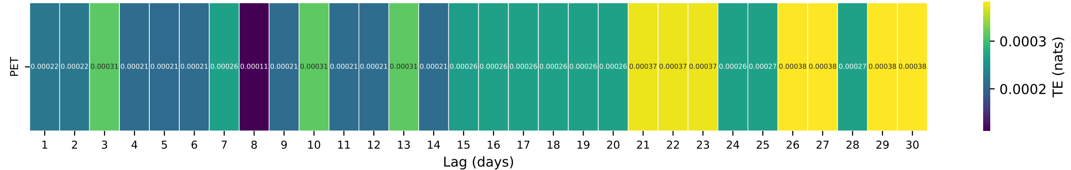
Gauge ID: 01605500 | SOUTH BRANCH POTOMAC RIVER AT FRANKLIN, WV | PET(t-\tau) \rightarrow Q(t)
