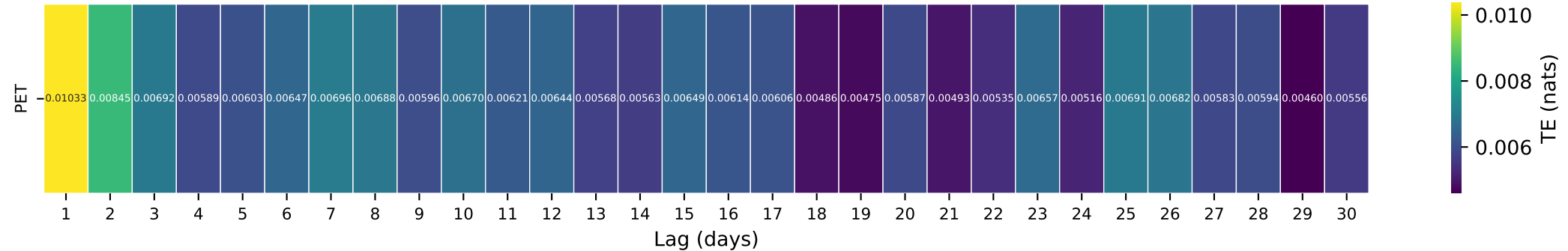
Gauge ID: 13023000 | GREYS RIVER AB RESERVOIR NR ALPINE WY | PET(t-\tau) \rightarrow Q(t)
