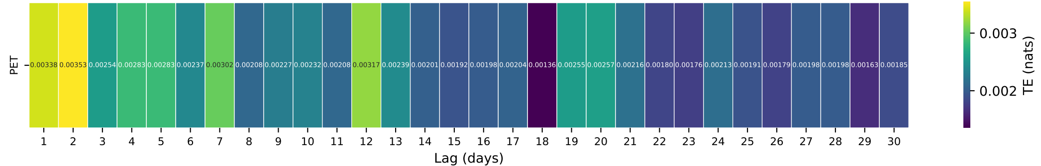
Gauge ID: 01142500 | AYERS BROOK AT RANDOLPH, VT | PET(t-\tau) \rightarrow Q(t)
