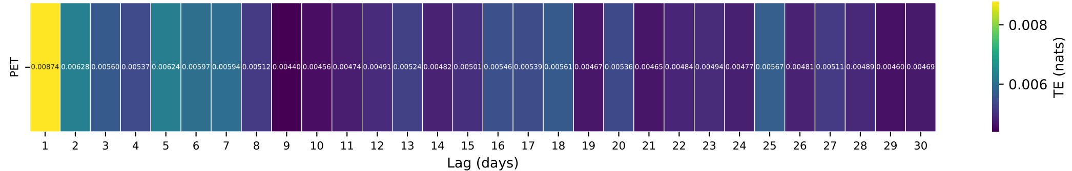
Gauge ID: 06622700 | NORTH BRUSH CREEK NEAR SARATOGA, WY | PET(t-\tau) \rightarrow Q(t)
