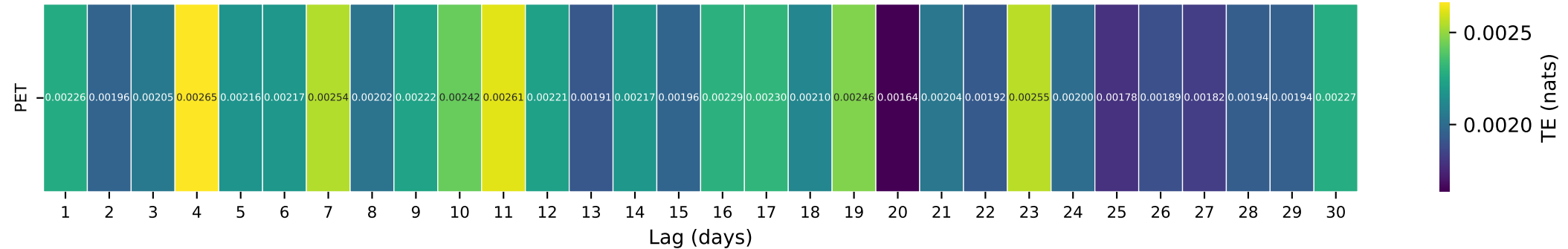
Gauge ID: 06784000 | SOUTH LOUP R AT ST. MICHAEL, NEBR. | PET(t-\tau) \rightarrow Q(t)
