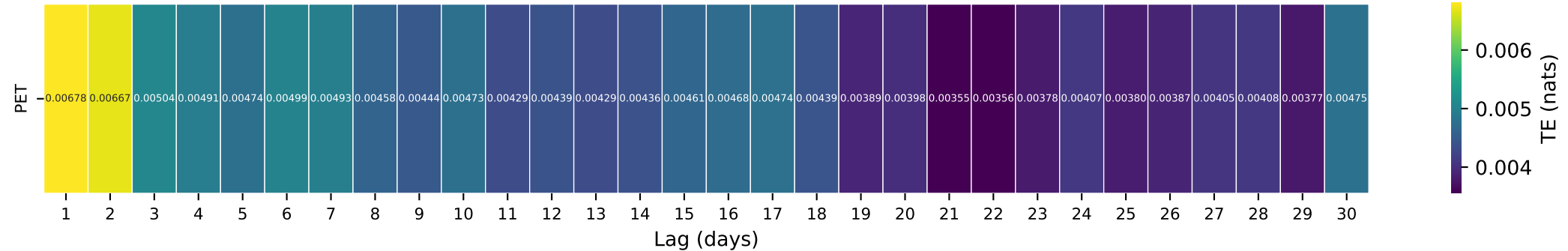
Gauge ID: 12048000 | DUNGENESS RIVER NEAR SEQUIM, WA | PET(t-\tau) \rightarrow Q(t)
