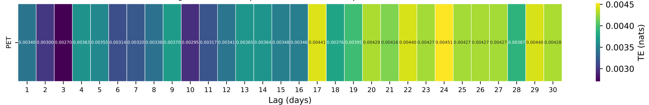
Gauge ID: 04197170 | Rock Creek at Tiffin OH | PET(t-\tau) \rightarrow Q(t)
