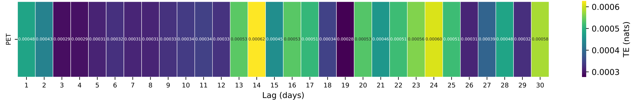
Gauge ID: 08104900 | S Fk San Gabriel Rv at Georgetown, TX | PET(t-\tau) \rightarrow Q(t)
