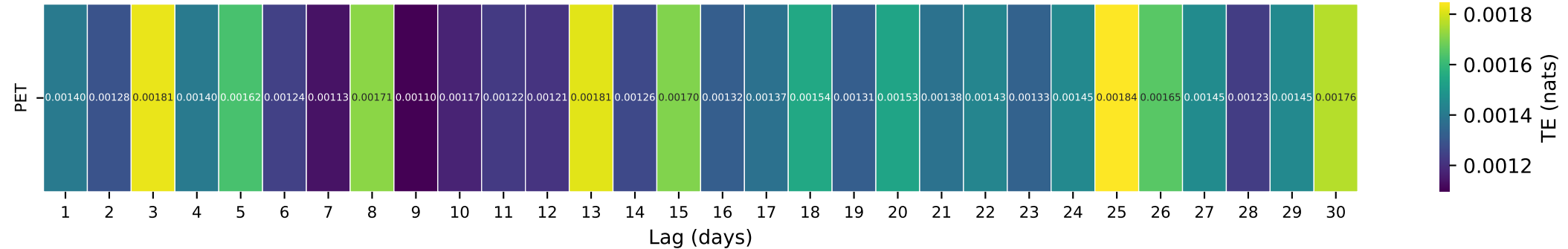
Gauge ID: 01638480 | CATOCTIN CREEK AT TAYLORSTOWN, VA | PET(t-\tau) \rightarrow Q(t)
