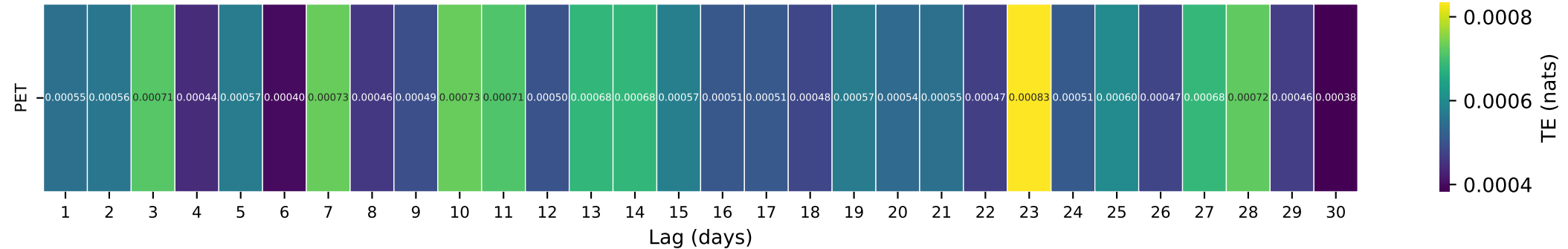
Gauge ID: 02369800 | BLACKWATER RIVER NEAR BRADLEY AL | PET(t- \tau ) \rightarrow Q(t)
