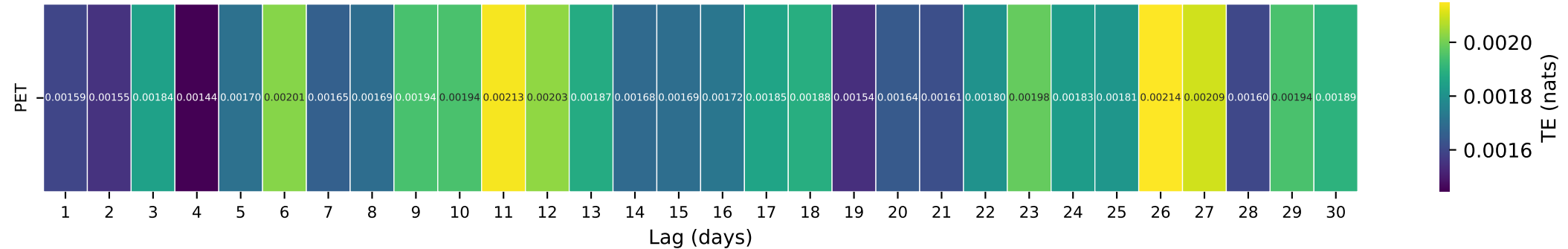
Gauge ID: 09484000 | SABINO CREEK NEAR TUCSON, AZ. | PET(t-\tau) \rightarrow Q(t)
