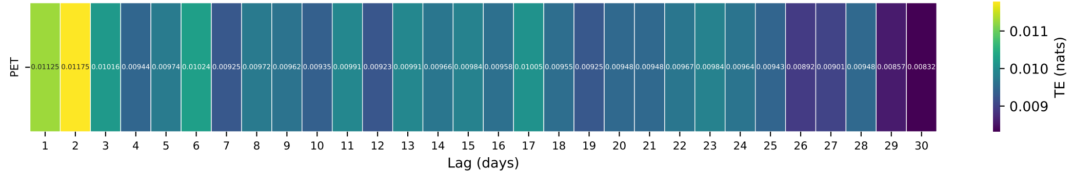
Gauge ID: 12040500 | QUEETS RIVER NEAR CLEARWATER, WA | PET(t-\tau) \rightarrow Q(t)
