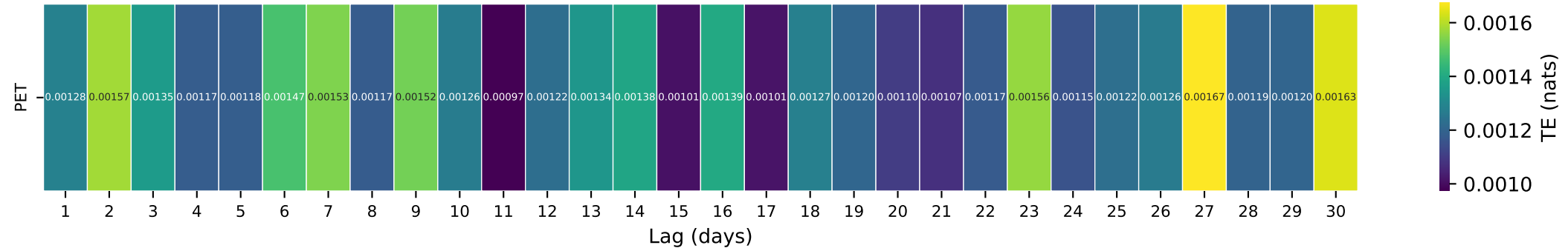
Gauge ID: 08155200 | Barton Ck at SH 71 nr Oak Hill, TX | PET(t-\tau) \rightarrow Q(t)
