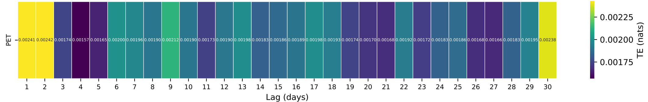
Gauge ID: 07362100 | SMACKOVER CREEK NEAR SMACKOVER, ARK. | PET(t-\tau) \rightarrow Q(t)
