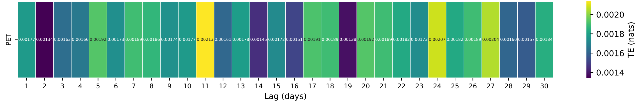
Gauge ID: 07066000 | Jacks Fork at Eminence, MO | PET(t-\tau) \rightarrow Q(t)
