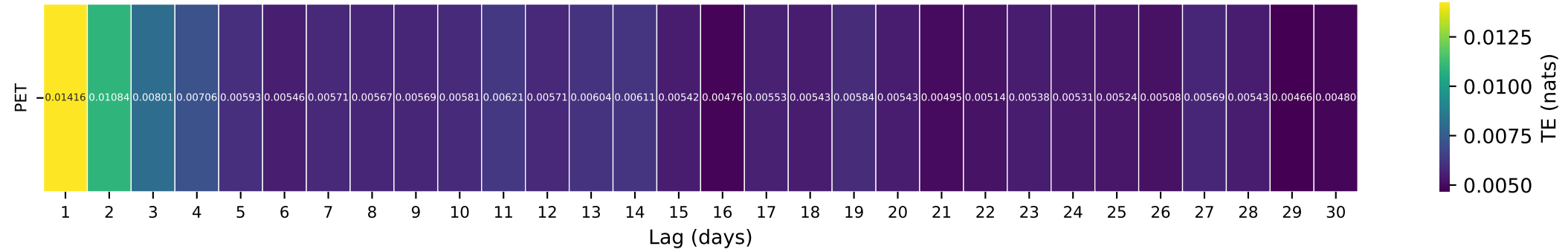
Gauge ID: 09081600 | CRYSTAL RIVER AB AVALANCHE C, NEAR REDSTONE, CO. | PET(t-\tau) \rightarrow Q(t)
