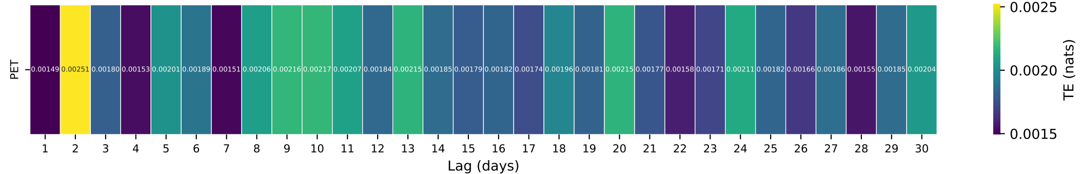
Gauge ID: 05495500 | BEAR CREEK NEAR MARCELLINE, IL | PET(t-\tau) \rightarrow Q(t)
