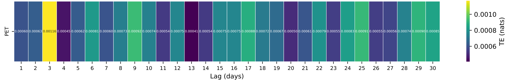
Gauge ID: 07315200 | E Fk Little Wichita Rv nr Henrietta, TX | PET(t-\tau) \rightarrow Q(t)
