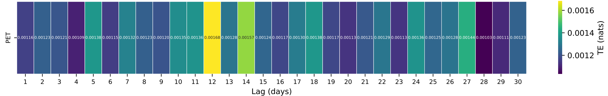
Gauge ID: 02198100 | BEAVERDAM CREEK NEAR SARDIS, GA | PET(t- \tau ) \rightarrow Q(t)
