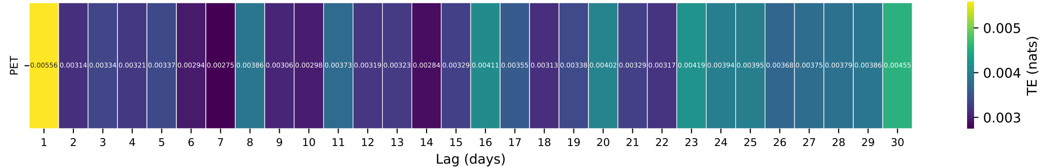
Gauge ID: 02051500 | MEHERRIN RIVER NEAR LAWRENCEVILLE, VA | PET(t-\tau) \rightarrow Q(t)
