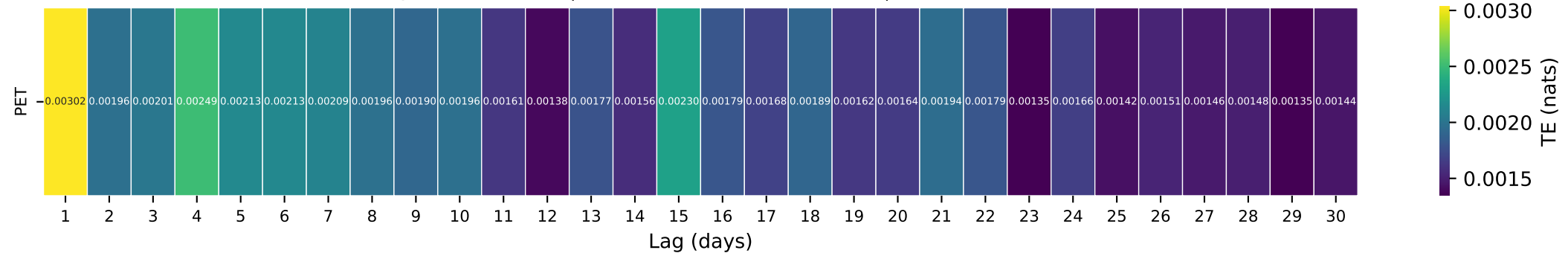
Gauge ID: 11237500 | PITMAN C BL TAMARACK C CA | PET(t- \tau ) \rightarrow Q(t)
