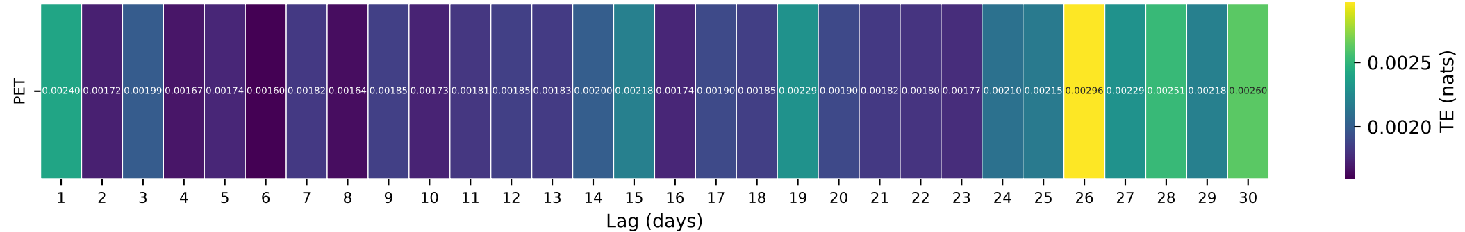
Gauge ID: 02216180 | TURNPIKE CREEK NEAR MCRAE, GA | PET(t-\tau) \rightarrow Q(t)
