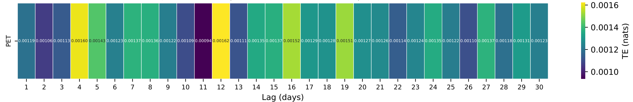
Gauge ID: 05585000 | LA MOINE RIVER AT RIPLEY, IL | PET(t-\tau) \rightarrow Q(t)
