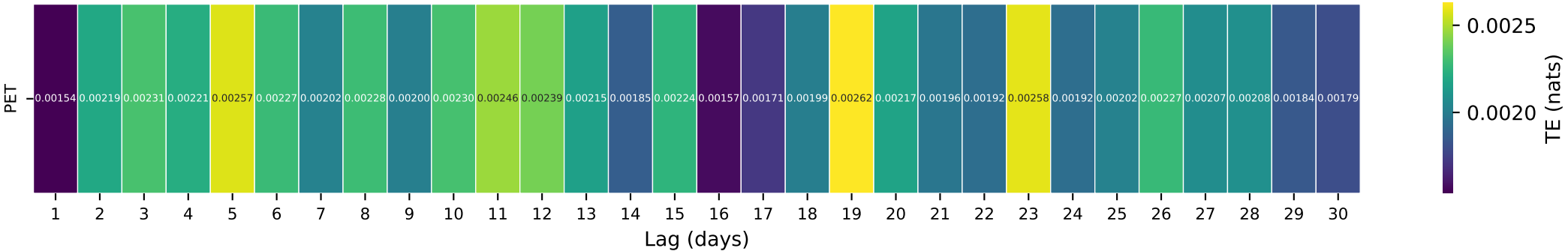
Gauge ID: 02112360 | MITCHELL RIVER NEAR STATE ROAD, NC | PET(t-\tau) \rightarrow Q(t)
