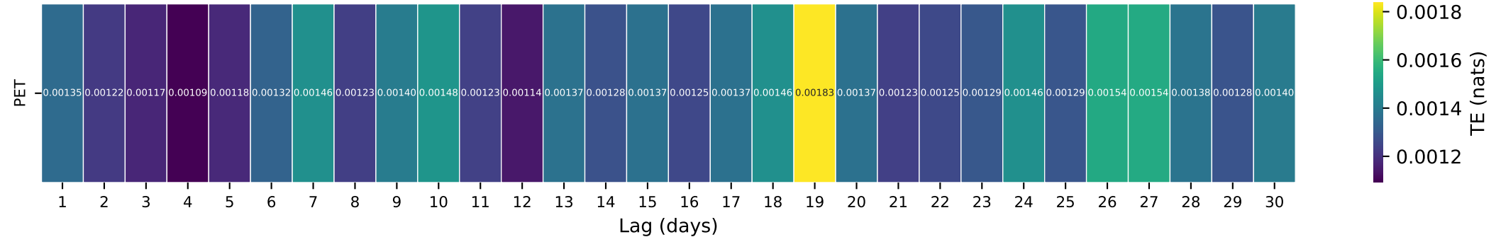
Gauge ID: 03456500 | EAST FORK PIGEON RIVER NEAR CANTON, NC | PET(t-\tau) \rightarrow Q(t)
