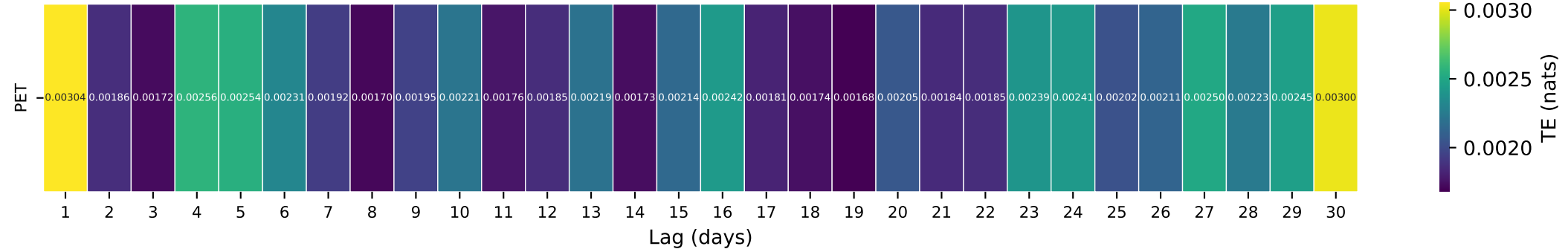
Gauge ID: 02427250 | PINE BARREN CREEK NEAR SNOW HILL, AL. | PET(t-\tau) \rightarrow Q(t)
