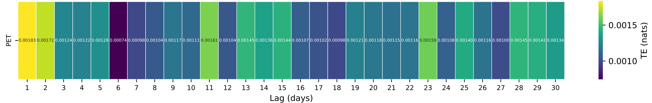
Gauge ID: 02374500 | MURDER CREEK NEAR EVERGREEN AL | PET(t- \tau ) \rightarrow Q(t)
