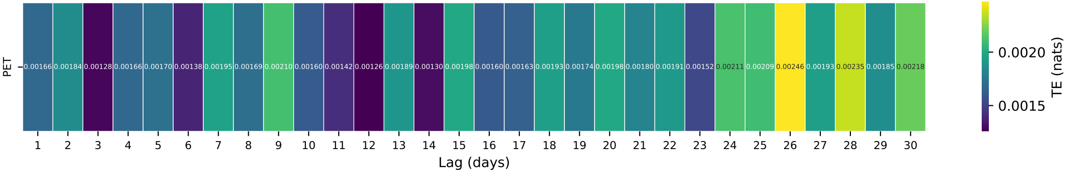
Gauge ID: 07263295 | Maumelle River at Williams Junction, AR | PET(t-\tau) \rightarrow Q(t)
