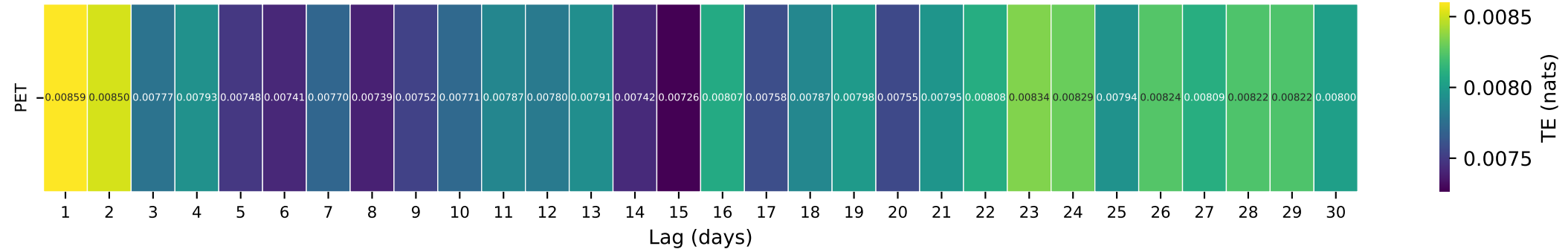
Gauge ID: 14185900 | QUARTZVILLE CREEK NEAR CASCADIA, OREG. | PET(t-\tau) \rightarrow Q(t)
