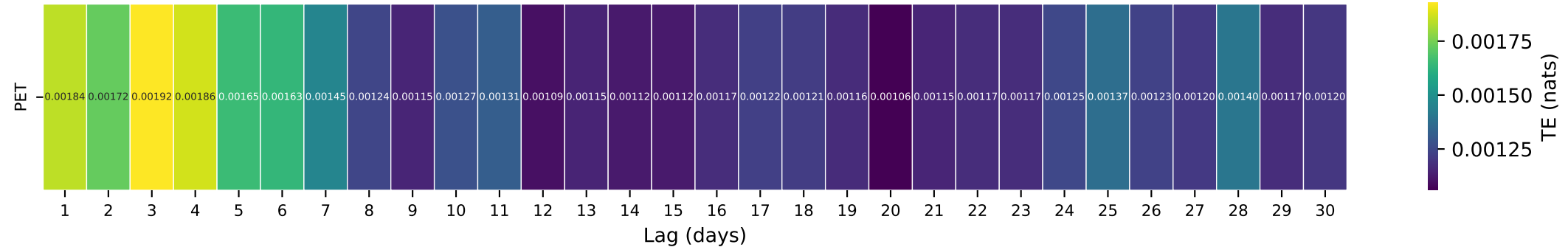
Gauge ID: 06354000 | CANNONBALL RIVER AT BREIEN, ND | PET(t-\tau) \rightarrow Q(t)
