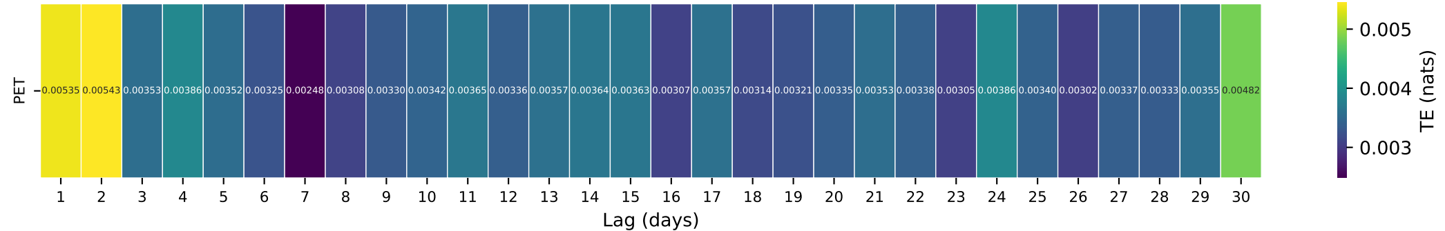
Gauge ID: 09223000 | HAMS FORK BELOW POLE CREEK, NEAR FRONTIER, WY | PET(t-\tau) \rightarrow Q(t)
