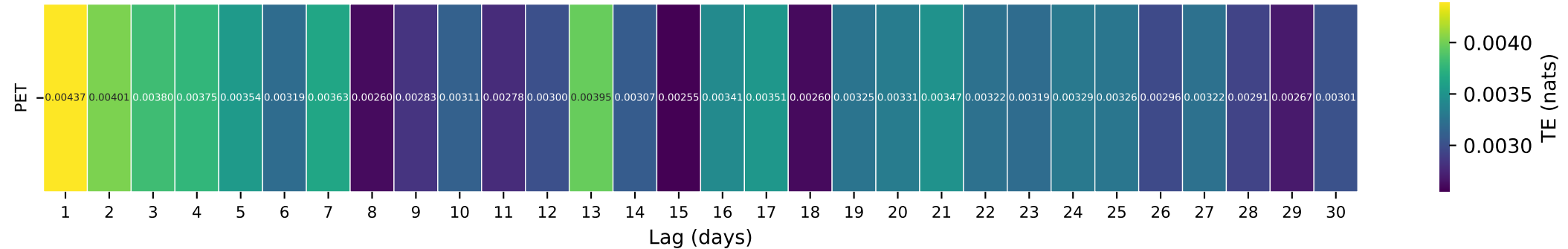
Gauge ID: 03010655 | Oswayo Creek at Shinglehouse, PA | PET(t-\tau) \rightarrow Q(t)
