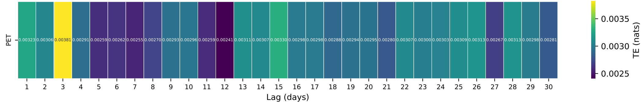
Gauge ID: 02481000 | BILOXI RIVER AT WORTHAM, MS | PET(t-\tau) \rightarrow Q(t)
