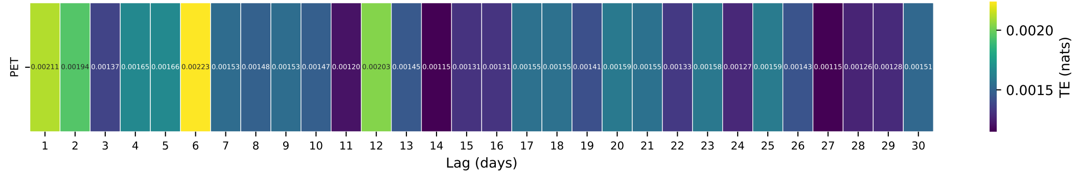
Gauge ID: 01350080 | MANOR KILL AT WEST CONESVILLE NEAR GILBOA NY | PET(t-\tau) \rightarrow Q(t)
