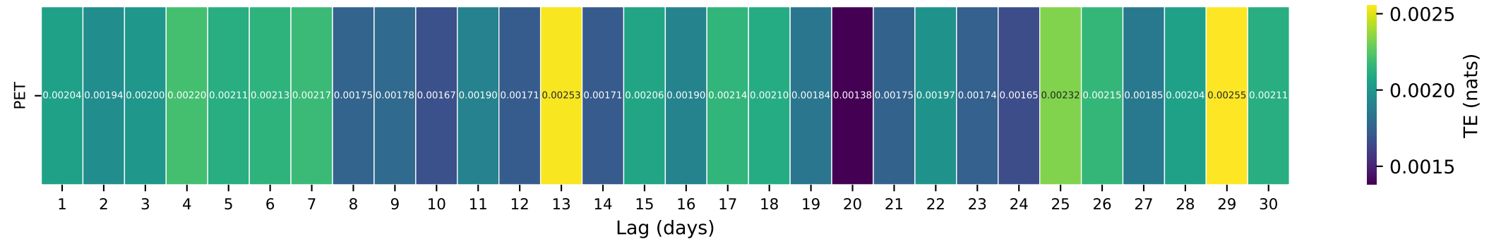
Gauge ID: 03237280 | Upper Twin Creek at McGaw OH | PET(t-\tau) \rightarrow Q(t)
