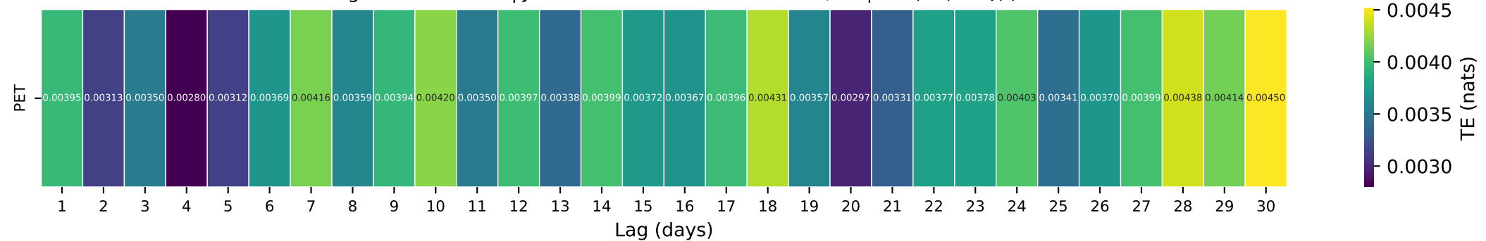
Gauge ID: 01451800 | Jordan Creek near Schnecksville, PA | PET(t-\tau) \rightarrow Q(t)
