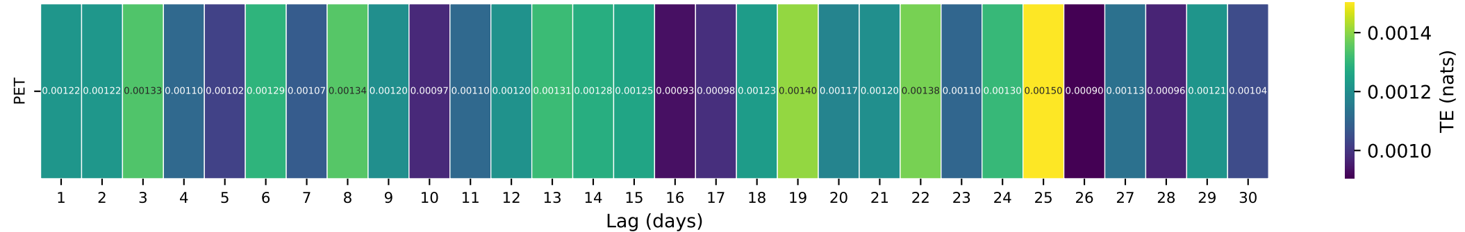
Gauge ID: 06447500 | LITTLE WHITE R NEAR MARTIN SD | PET(t- \tau ) \rightarrow Q(t)
