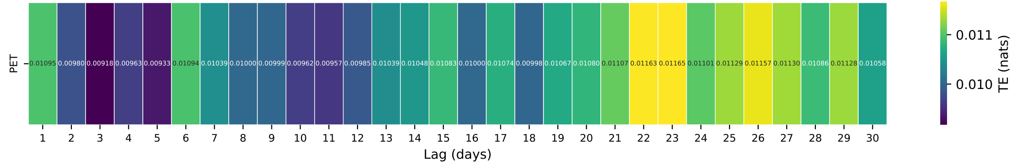
Gauge ID: 14325000 | SOUTH FORK COQUILLE RIVER AT POWERS, OR | PET(t-\tau) \rightarrow Q(t)
