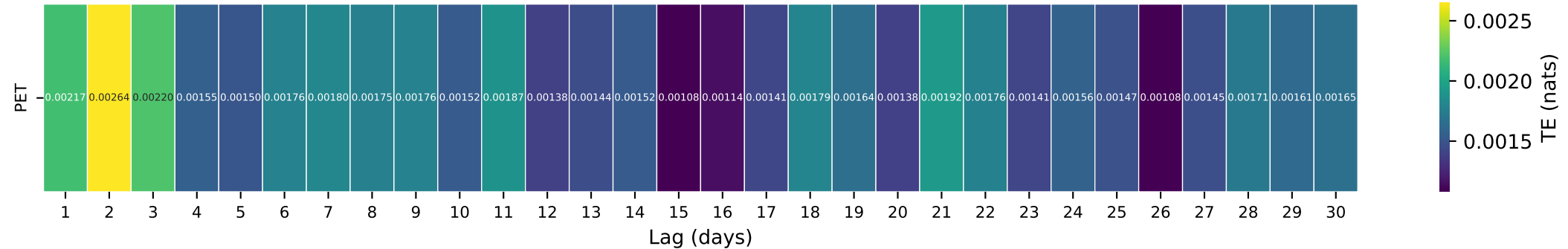
Gauge ID: 02314500 | SUWANNEE RIVER AT US 441, AT FARGO, GA | PET(t-\tau) \rightarrow Q(t)
