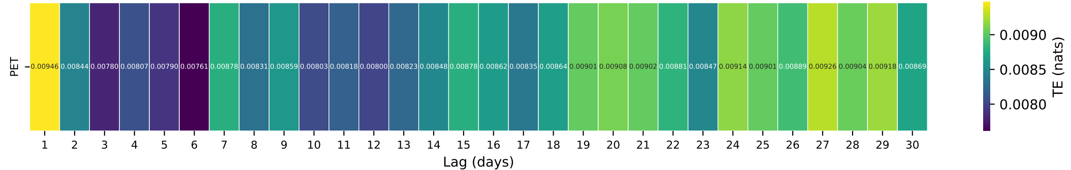
Gauge ID: 11532500 | SMITH R NR CRESCENT CITY CA | PET(t-\tau) \rightarrow Q(t)
