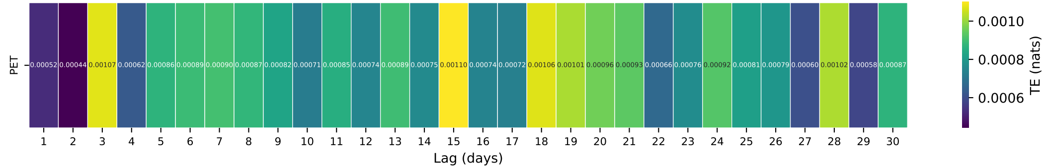
Gauge ID: 01532000 | Towanda Creek near Monroeton, PA | PET(t-\tau) \rightarrow Q(t)
