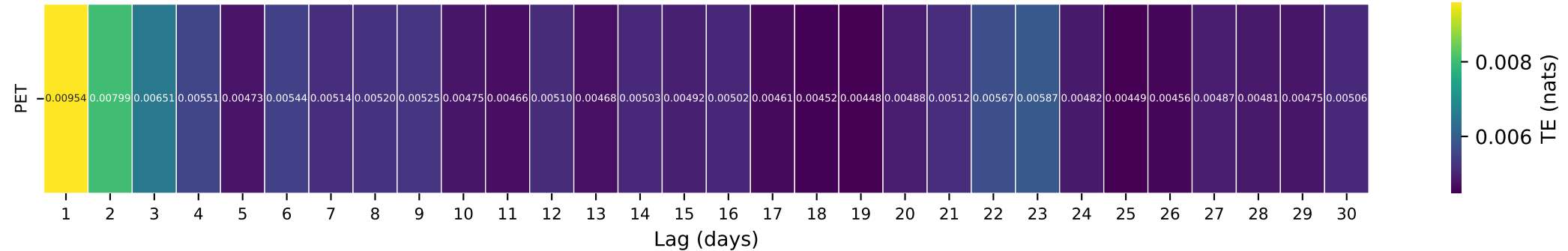
Gauge ID: 12488500 | AMERICAN RIVER NEAR NILE, WA | PET(t-\tau) \rightarrow Q(t)
