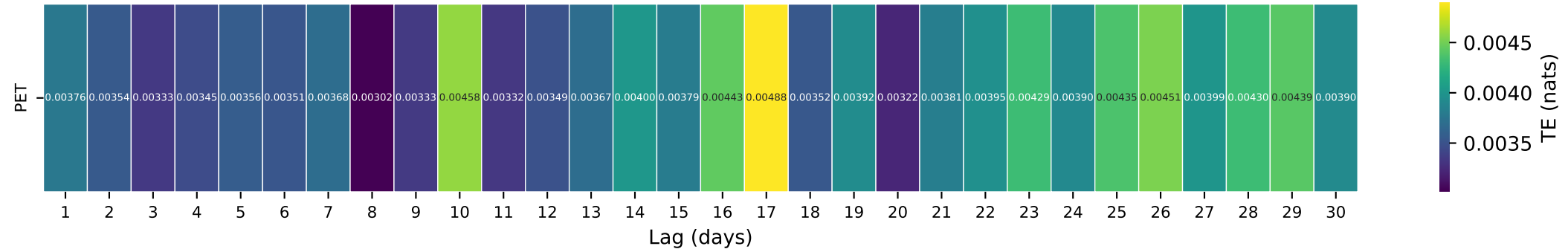
Gauge ID: 02196000 | STEVENS CREEK NEAR MODOC, SC | PET(t-\tau) \rightarrow Q(t)
