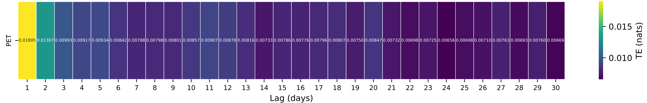
Gauge ID: 06280300 | SOUTH FORK SHOSHONE RIVER NEAR VALLEY, WY | PET(t-\tau) \rightarrow Q(t)
