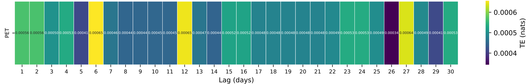
Gauge ID: 08029500 | Big Cow Ck nr Newton, TX | PET(t- \tau ) \rightarrow Q(t)
