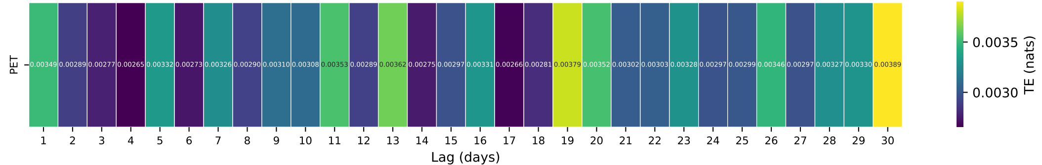
Gauge ID: 08023080 | Bayou Grand Cane near Stanley, LA | PET(t- \tau ) \rightarrow Q(t)
