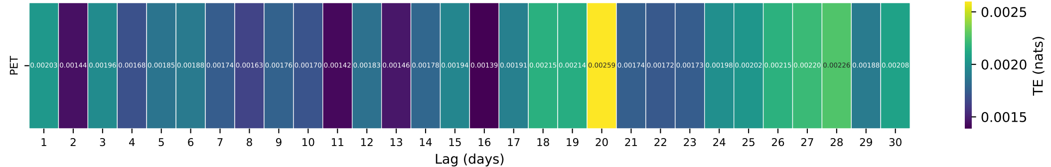
Gauge ID: 07291000 | HOMOCHITTO RIVER AT EDDICETON, MS | PET(t-\tau) \rightarrow Q(t)
