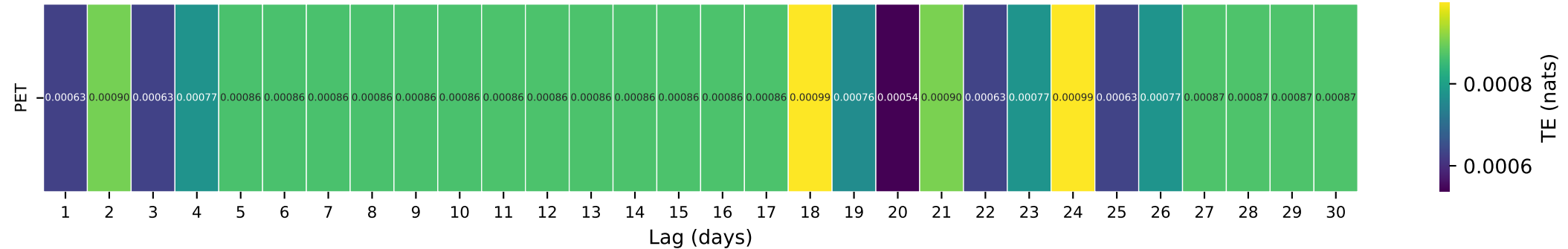
Gauge ID: 10258000 | TAHQUITZ C NR PALM SPRINGS CA | PET(t- \tau ) \rightarrow Q(t)
