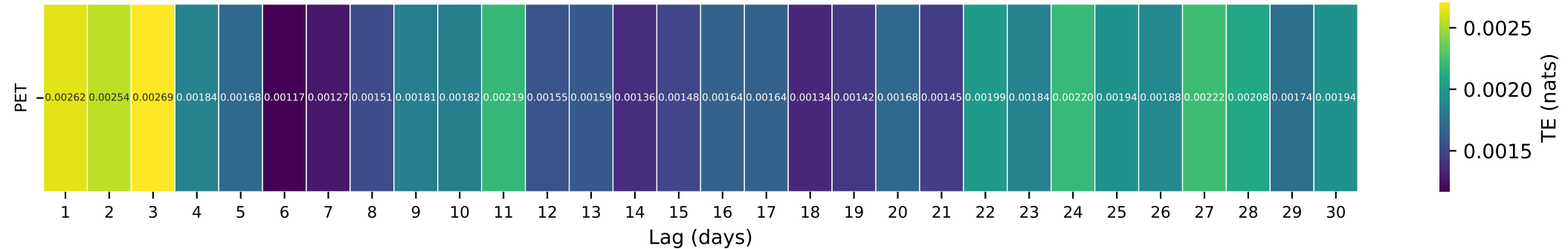
Gauge ID: 01123000 | LITTLE RIVER NEAR HANOVER, CT. | PET(t-\tau) \rightarrow Q(t)
