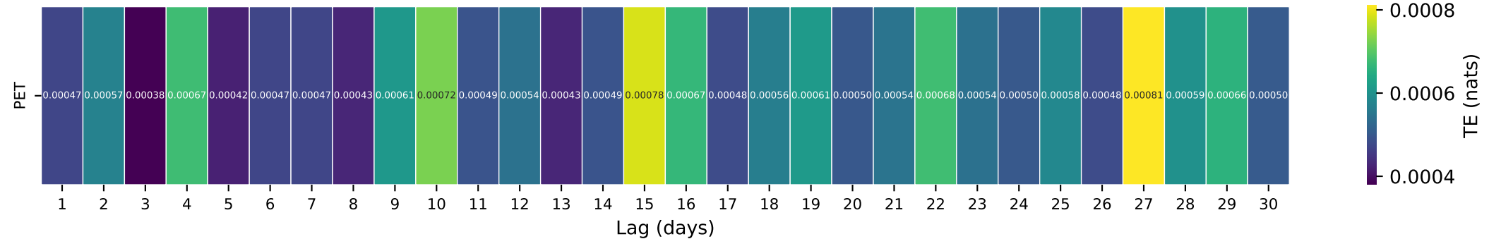
Gauge ID: 08196000 | Dry Frio Rv nr Reagan Wells, TX | PET(t-\tau) \rightarrow Q(t)
