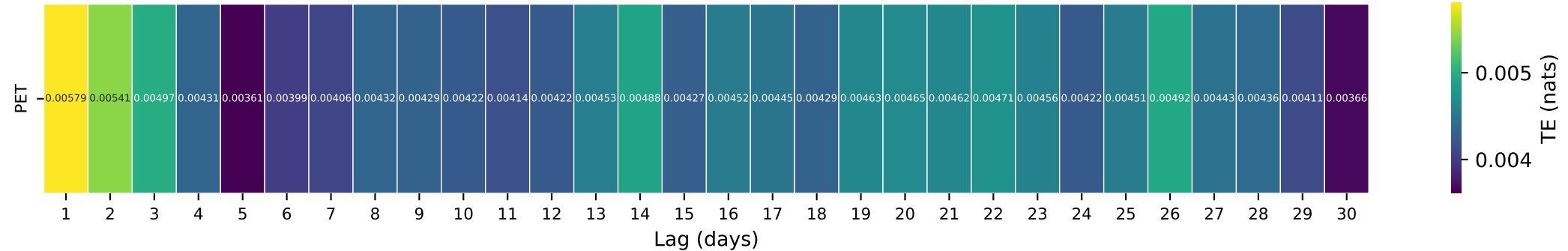
Gauge ID: 12141300 | MIDDLE FORK SNOQUALMIE RIVER NEAR TANNER, WA | PET(t-\tau) \rightarrow Q(t)
