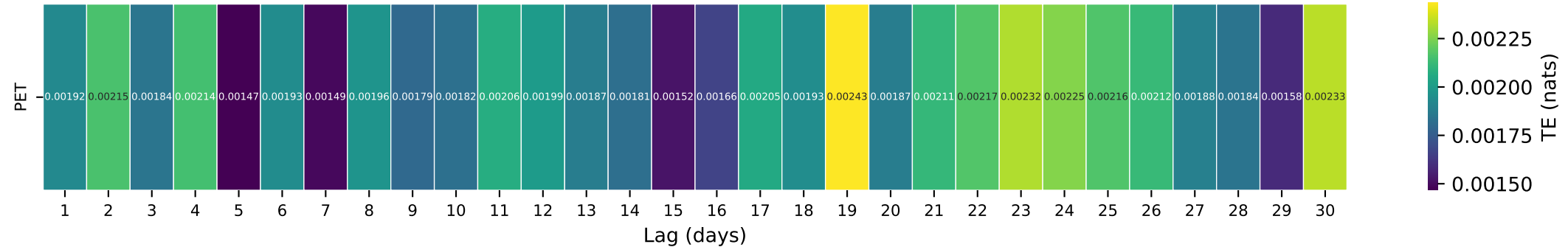
Gauge ID: 06154410 | Little Peoples Creek near Hays MT | PET(t- \tau ) \rightarrow Q(t)
