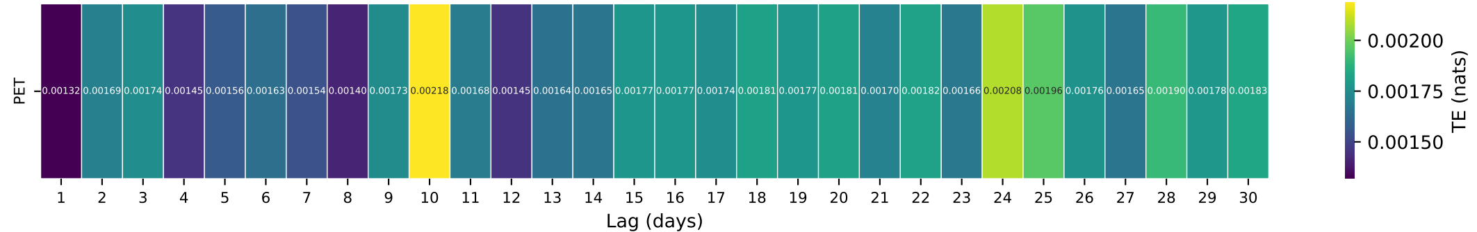
Gauge ID: 09494000 | WHITE RIVER NEAR FORT APACHE, AZ. | PET(t-\tau) \rightarrow Q(t)
