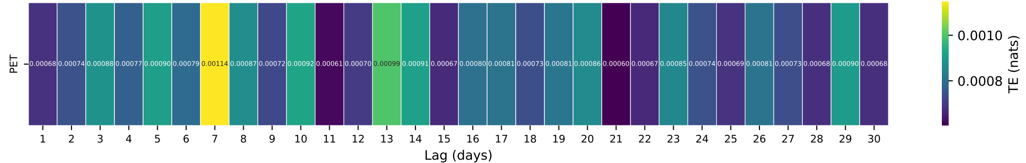
Gauge ID: 01547700 | Marsh Creek at Blanchard, PA | PET(t-\tau) \rightarrow Q(t)
