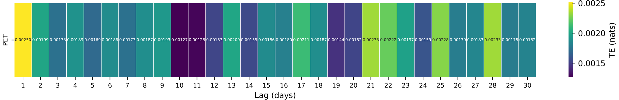
Gauge ID: 01440000 | FLAT BROOK NEAR FLATBROOKVILLE NJ | PET(t-τ) → Q(t)
