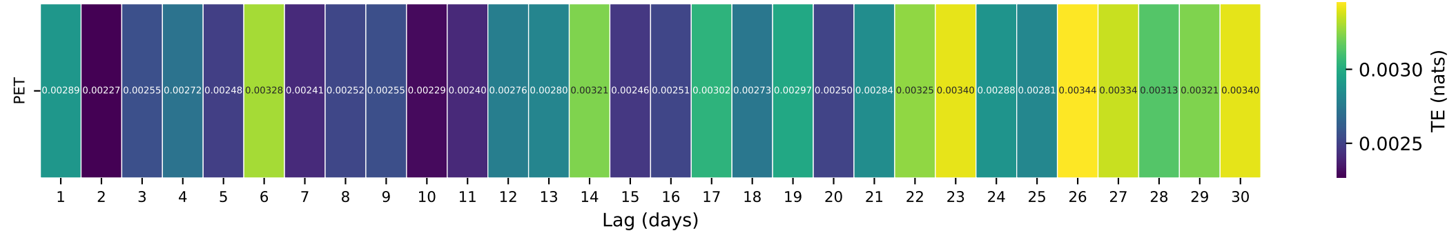
Gauge ID: 03076600 | BEAR CREEK AT FRIENDSVILLE, MD | PET(t-\tau) \rightarrow Q(t)
