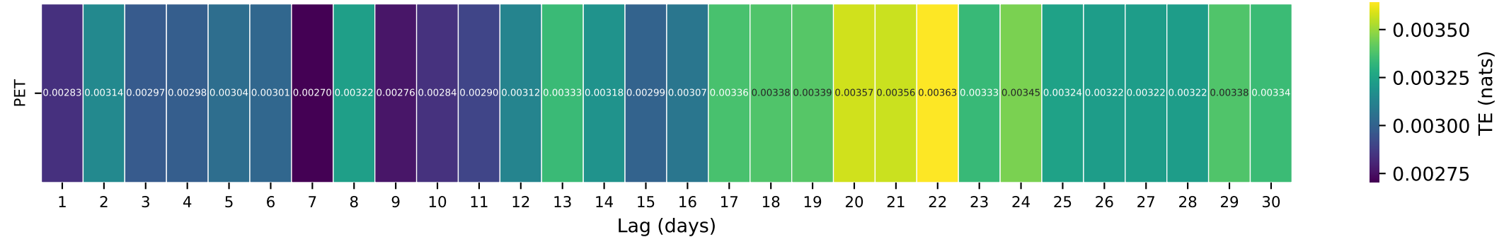
Gauge ID: 11299600 | BLACK C NR COPPEROPOLIS CA | PET(t- \tau ) \rightarrow Q(t)
