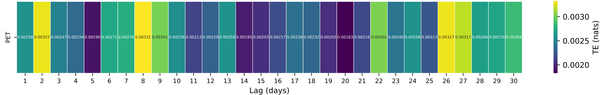
Gauge ID: 09312600 | WHITE RIVER BL TABBYUNE C NEAR SOLDIER SUMMIT, UT | PET(t-\tau) \rightarrow Q(t)
