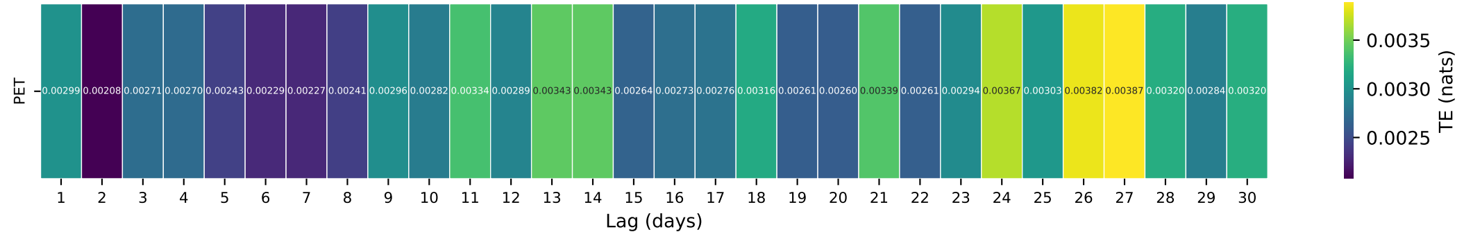
Gauge ID: 03050000 | TYGART VALLEY RIVER NEAR DAILEY, WV | PET(t-\tau) \rightarrow Q(t)
