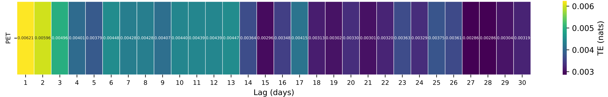
Gauge ID: 09066300 | MIDDLE CREEK NEAR MINTURN, CO. | PET(t-\tau) \rightarrow Q(t)
