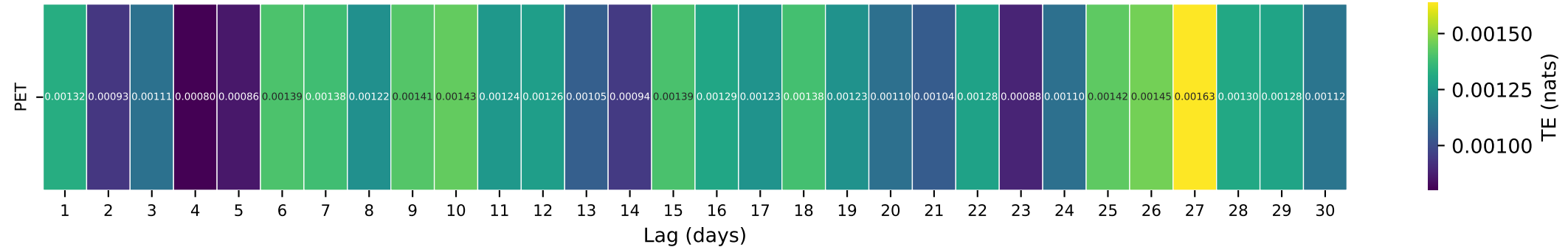
Gauge ID: 01491000 | CHOPTANK RIVER NEAR GREENSBORO, MD | PET(t-\tau) \rightarrow Q(t)
