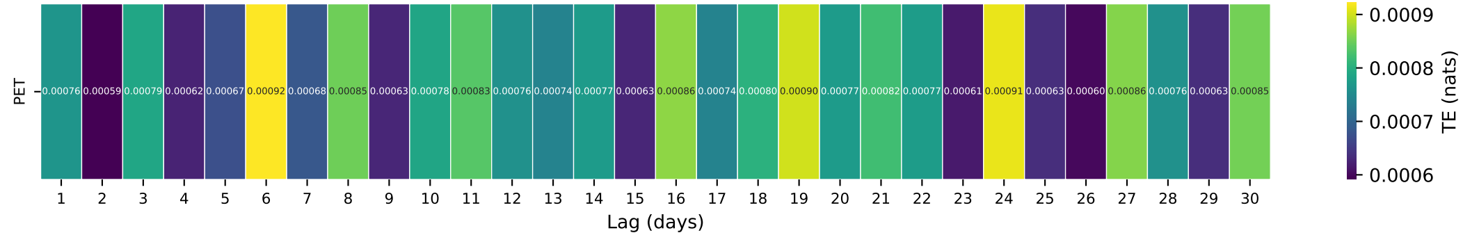
Gauge ID: 08198500 | Sabinal Rv at Sabinal, TX | PET(t-\tau) \rightarrow Q(t)
