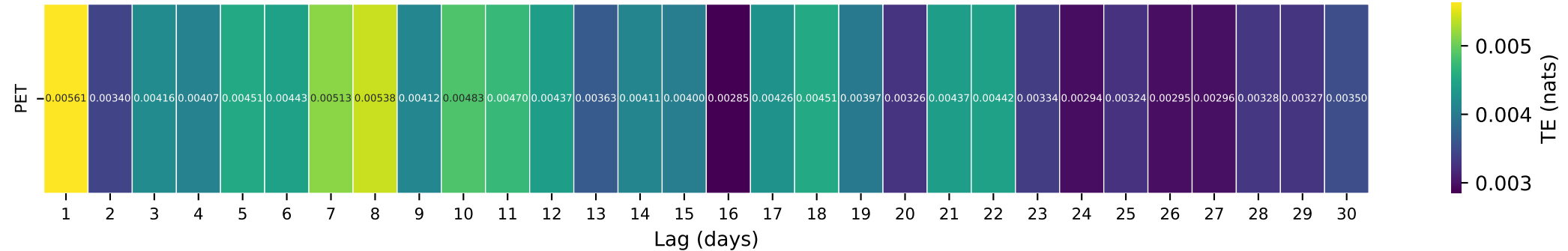
Gauge ID: 05362000 | JUMP RIVER AT SHELDON, WI | PET(t-\tau) \rightarrow Q(t)
