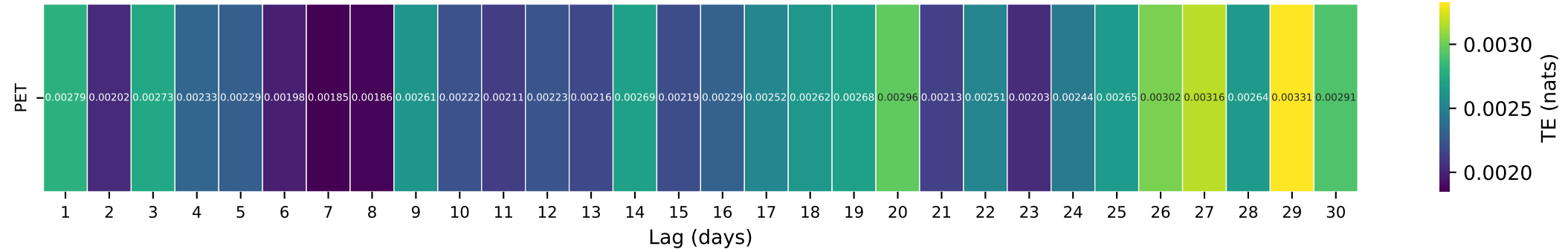
Gauge ID: 01596500 | SAVAGE RIVER NEAR BARTON, MD | PET(t-\tau) \rightarrow Q(t)
