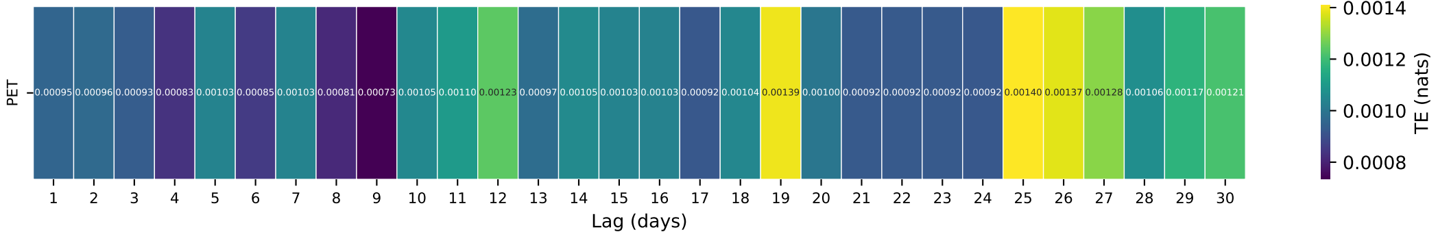
Gauge ID: 03604000 | BUFFALO RIVER NEAR FLAT WOODS, TN | PET(t-\tau) \rightarrow Q(t)
