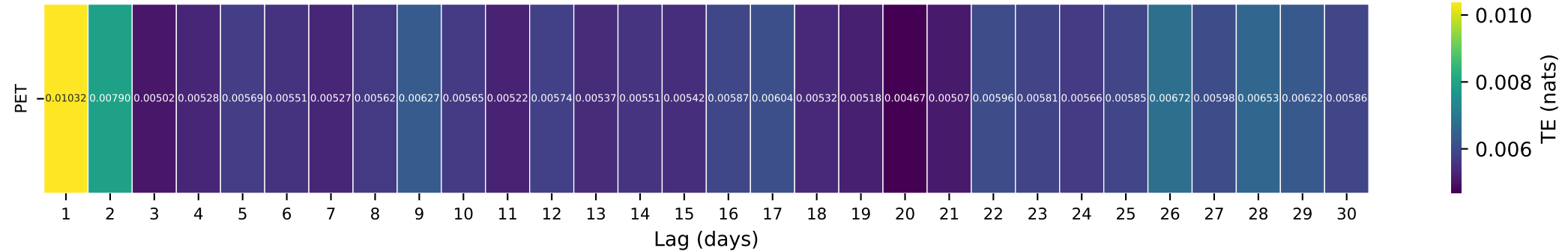
Gauge ID: 13011500 | PACIFIC CREEK AT MORAN WY | PET(t-\tau) \rightarrow Q(t)
