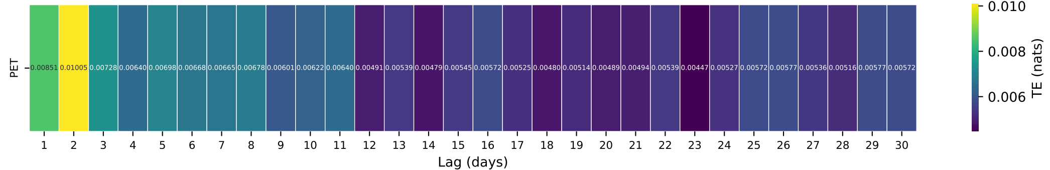
Gauge ID: 13340000 | CLEARWATER RIVER AT OROFINO ID | PET(t-\tau) \rightarrow Q(t)
