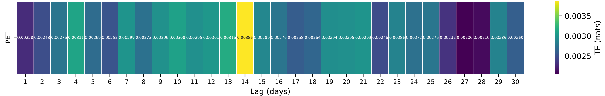
Gauge ID: 07148400 | Salt Fork Arkansas River nr Alva, OK | PET(t-\tau) \rightarrow Q(t)
