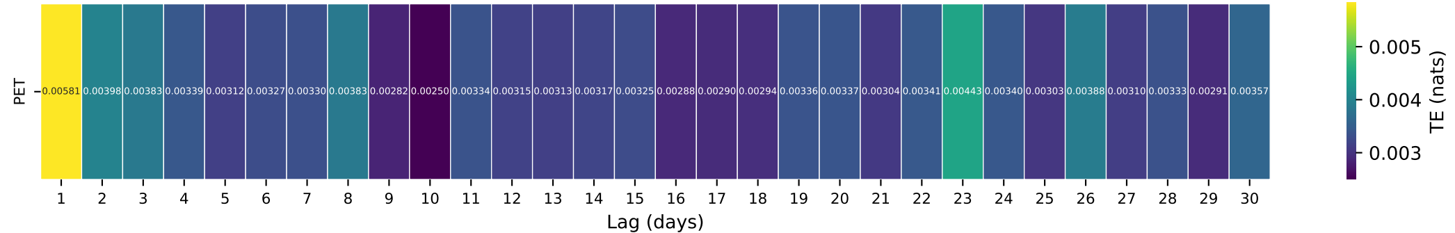
Gauge ID: 10242000 | COAL CREEK NEAR CEDAR CITY, UT | PET(t-\tau) \rightarrow Q(t)
