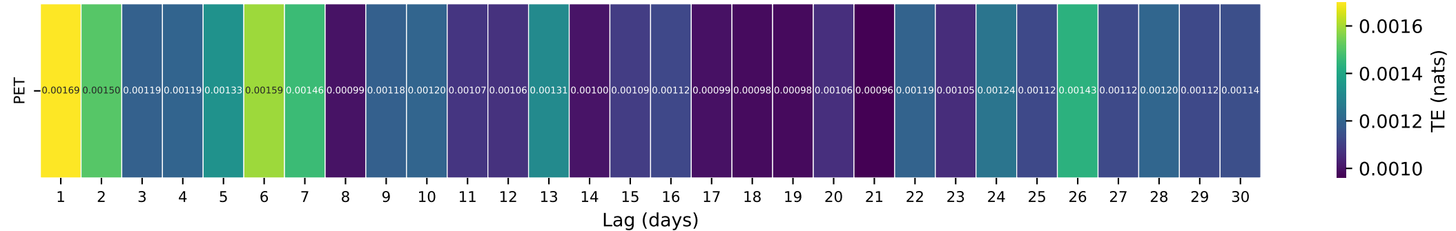
Gauge ID: 14092750 | SHITIKE CR, AT PETERS PASTURE, NR WARM SPRINGS, OR | PET(t-\tau) \rightarrow Q(t)
