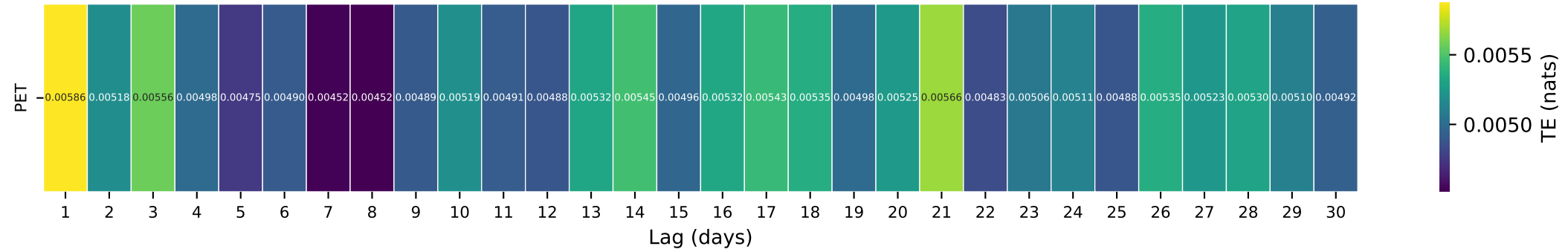
Gauge ID: 14138800 | BLAZED ALDER CREEK NEAR RHODODENDRON, OREG. | PET(t-\tau) \rightarrow Q(t)
