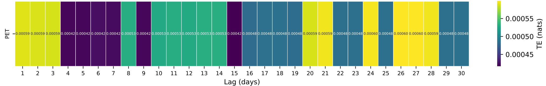
Gauge ID: 01606500 | SO. BRANCH POTOMAC RIVER NR PETERSBURG, WV | PET(t-\tau) \rightarrow Q(t)
