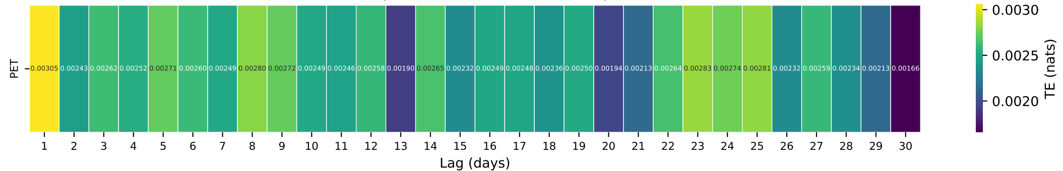
Gauge ID: 07068000 | Current River at Doniphan, MO | PET(t-\tau) \rightarrow Q(t)
