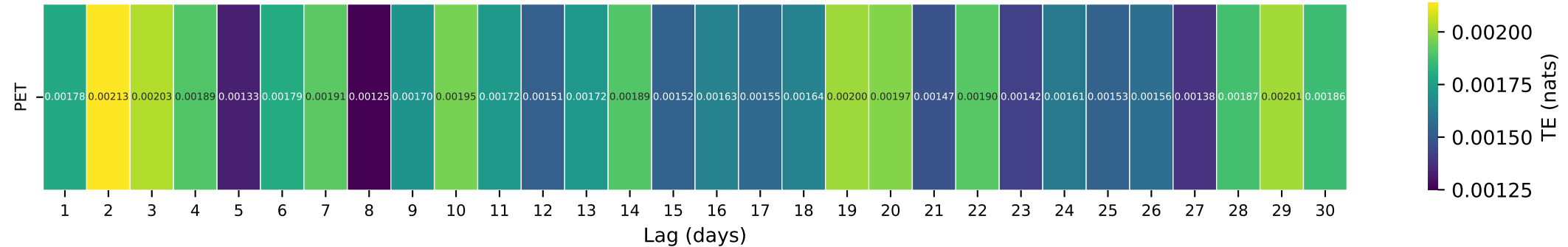
Gauge ID: 05503800 | Crooked Creek near Paris, MO | PET(t-\tau) \rightarrow Q(t)
