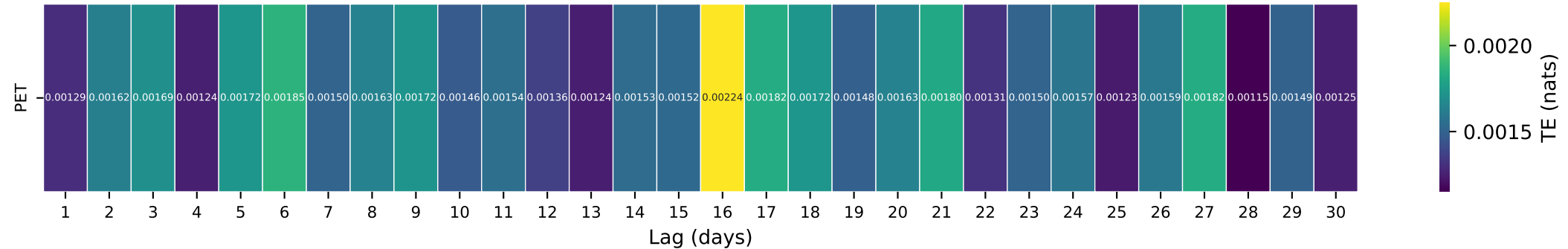
Gauge ID: 06879650 | KINGS C NR MANHATTAN, KS | PET(t- \tau ) \rightarrow Q(t)
