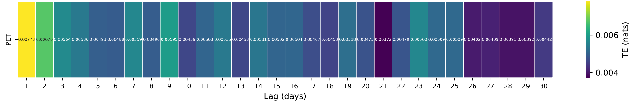
Gauge ID: 06311000 | NORTH FORK POWDER RIVER NEAR HAZELTON, WY | PET(t-\tau) \rightarrow Q(t)
