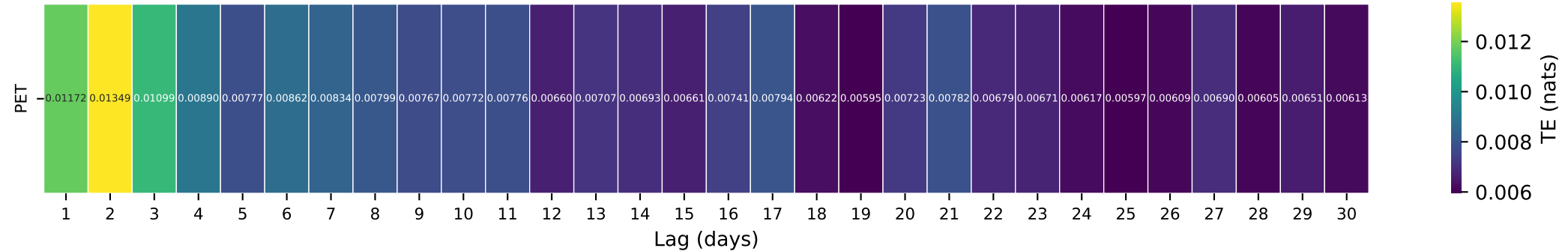
Gauge ID: 12358500 | Middle Fork Flathead River nr West Glacier MT | PET(t-\tau) \rightarrow Q(t)
