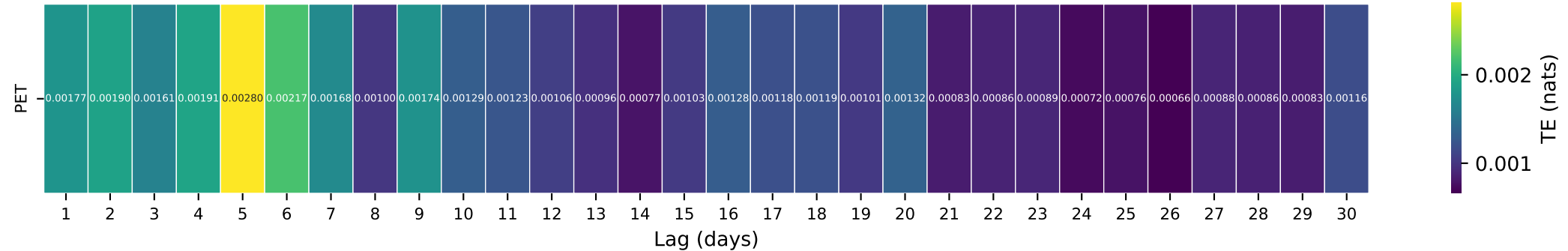
Gauge ID: 06468250 | JAMES RIVER ABOVE ARROWWOOD LAKE NR KENSAL, ND | PET(t-\tau) \rightarrow Q(t)
