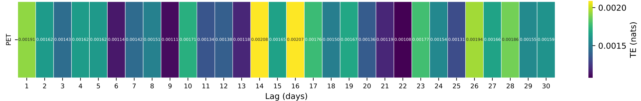
Gauge ID: 05495000 | Fox River at Wayland, MO | PET(t-\tau) \rightarrow Q(t)
