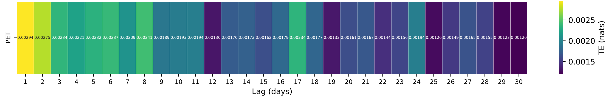
Gauge ID: 05291000 | WHETSTONE RIVER NEAR BIG STONE CITY, SD | PET(t-\tau) \rightarrow Q(t)
