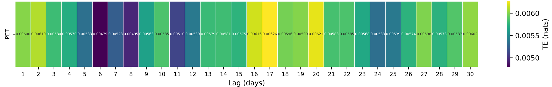
Gauge ID: 14138900 | NORTH FORK BULL RUN RIVER NEAR MULTNOMAH FALLS, OR | PET(t-\tau) \rightarrow Q(t)
