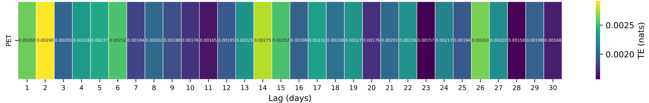
Gauge ID: 06477500 | FIRESTEEL CR NEAR MOUNT VERNON SD | PET(t-\tau) \rightarrow Q(t)
