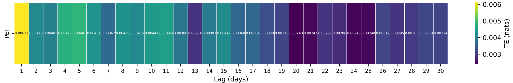
Gauge ID: 04127918 | PINE RIVER NEAR RUDYARD, MI | PET(t-\tau) \rightarrow Q(t)
