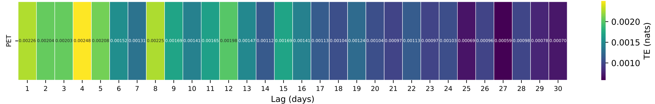
Gauge ID: 05057000 | SHEYENNE RIVER NR COOPERSTOWN, ND | PET(t-\tau) \rightarrow Q(t)
