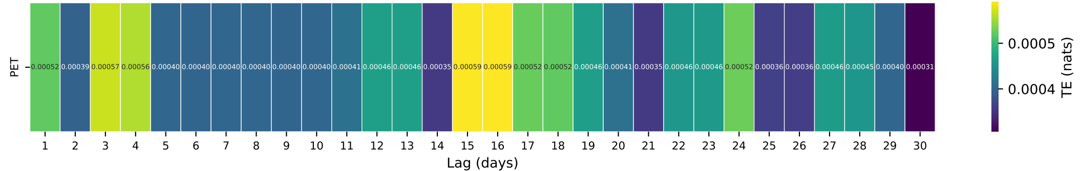
Gauge ID: 02064000 | FALLING RIVER NEAR NARUNA, VA | PET(t-\tau) \rightarrow Q(t)
