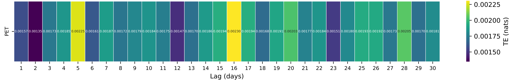
Gauge ID: 02028500 | ROCKFISH RIVER NEAR GREENFIELD, VA | PET(t-\tau) \rightarrow Q(t)
