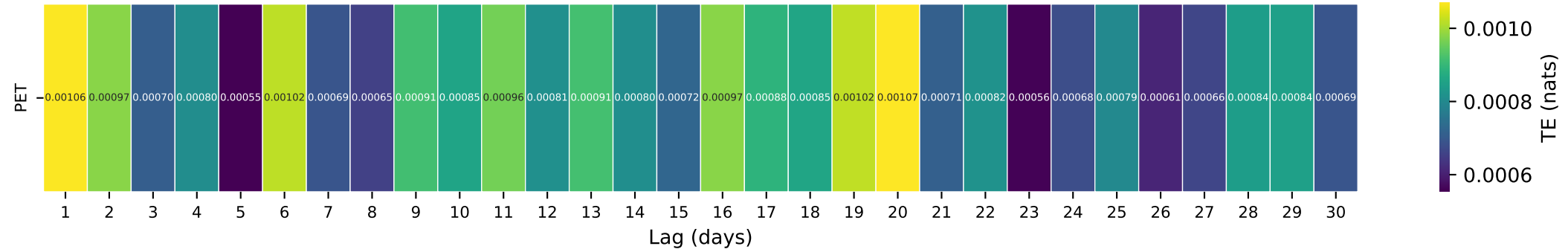
Gauge ID: 01350000 | SCHOHARIE CREEK AT PRATTSVILLE NY | PET(t-\tau) \rightarrow Q(t)
