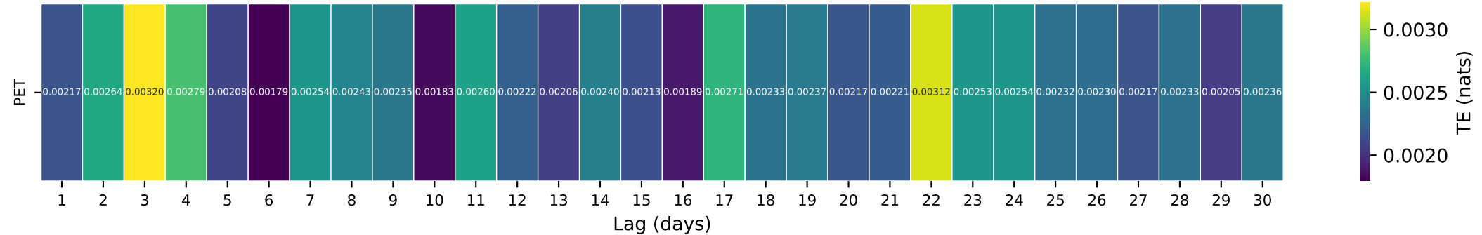
Gauge ID: 01557500 | Bald Eagle Creek at Tyrone, PA | PET(t-\tau) \rightarrow Q(t)
