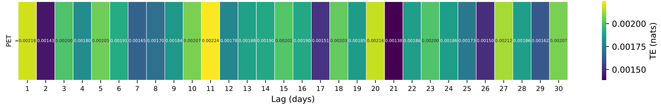
Gauge ID: 03346000 | NORTH FORK EMBARRAS RIVER NEAR OBLONG, IL | PET(t-\tau) \rightarrow Q(t)
