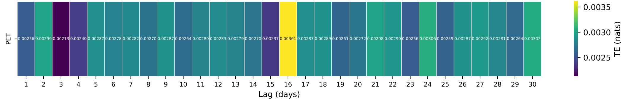
Gauge ID: 01350140 | MINE KILL NEAR NORTH BLENHEIM NY | PET(t-\tau) \rightarrow Q(t)
