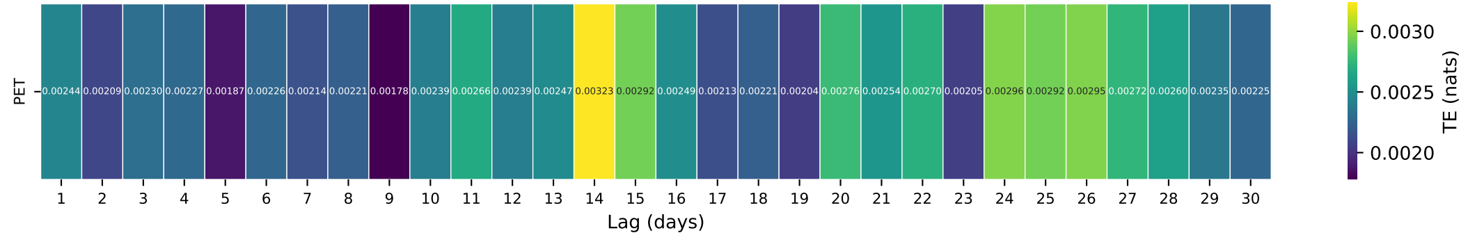
Gauge ID: 03300400 | BEECH FORK AT MAUD, KY | PET(t-\tau) \rightarrow Q(t)
