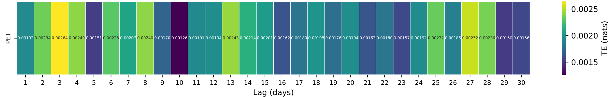
Gauge ID: 01548500 | Pine Creek at Cedar Run, PA | PET(t-\tau) \rightarrow Q(t)
