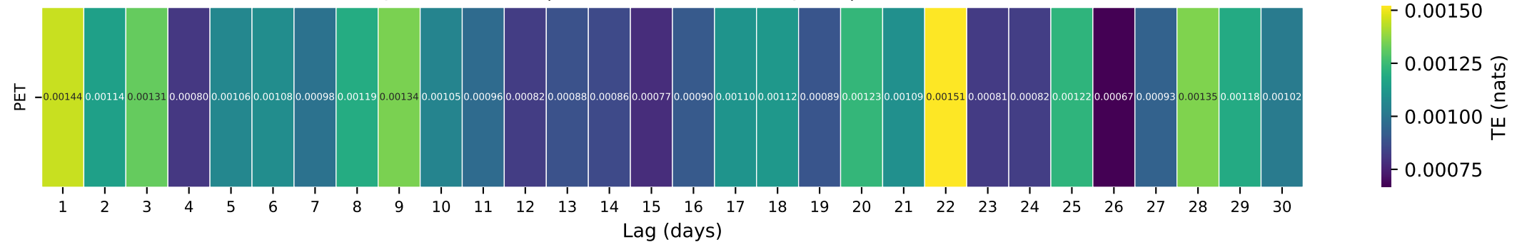
Gauge ID: 07315700 | Mud Creek near Courtney, OK | PET(t-\tau) \rightarrow Q(t)
