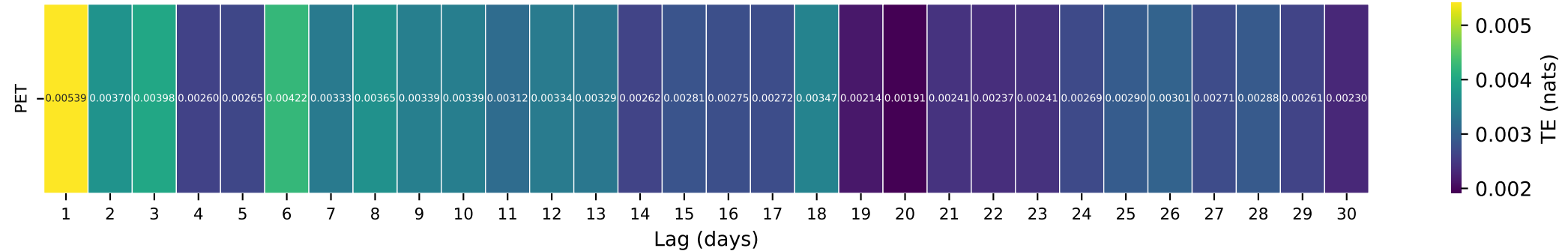
Gauge ID: 01052500 | Diamond River near Wentworth Location, NH | PET(t-\tau) \rightarrow Q(t)
