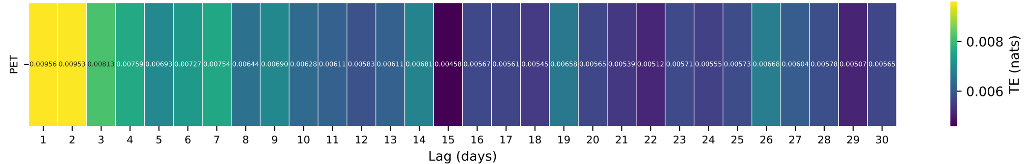
Gauge ID: 13340600 | NF CLEARWATER RIVER NR CANYON RANGER STATION ID | PET(t-\tau) \rightarrow Q(t)
