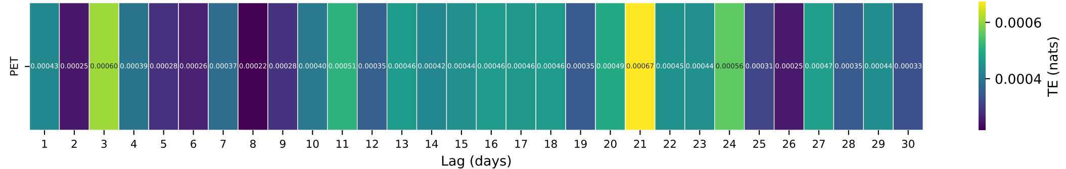
Gauge ID: 02082950 | LITTLE FISHING CREEK NEAR WHITE OAK, NC | PET(t-\tau) \rightarrow Q(t)
