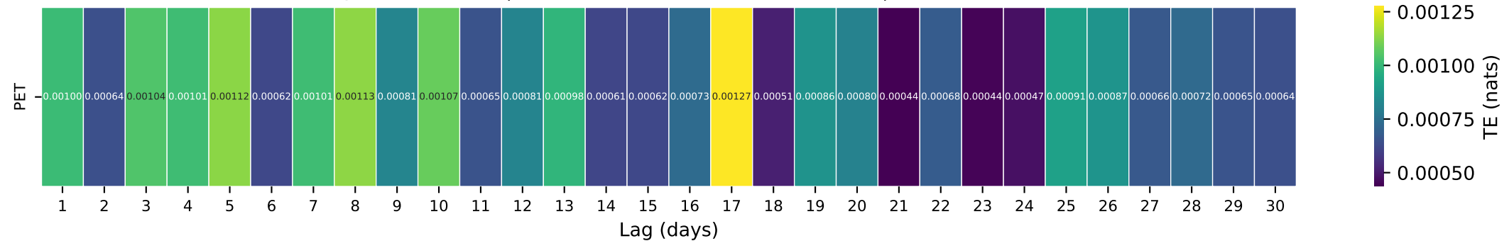
Gauge ID: 06918460 | Turnback Creek above Greenfield, MO | PET(t-\tau) \rightarrow Q(t)
