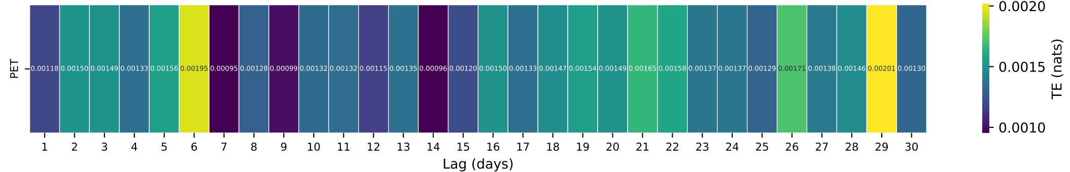
Gauge ID: 02381600 | FAUSETT CREEK NEAR TALKING ROCK, GA | PET(t-\tau) \rightarrow Q(t)
