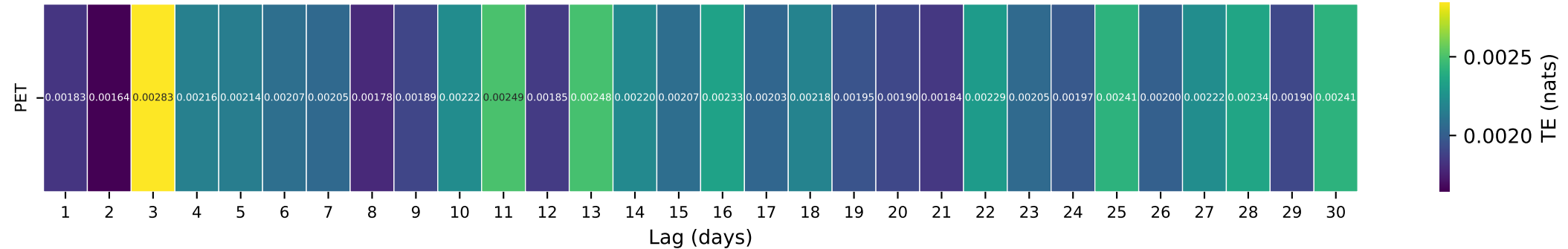
Gauge ID: 03500240 | CARTOOGECHAYE CREEK NEAR FRANKLIN, NC | PET(t-\tau) \rightarrow Q(t)
