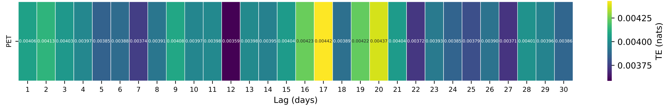
Gauge ID: 14138870 | FIR CREEK NEAR BRIGHTWOOD, OR | PET(t-\tau) \rightarrow Q(t)
