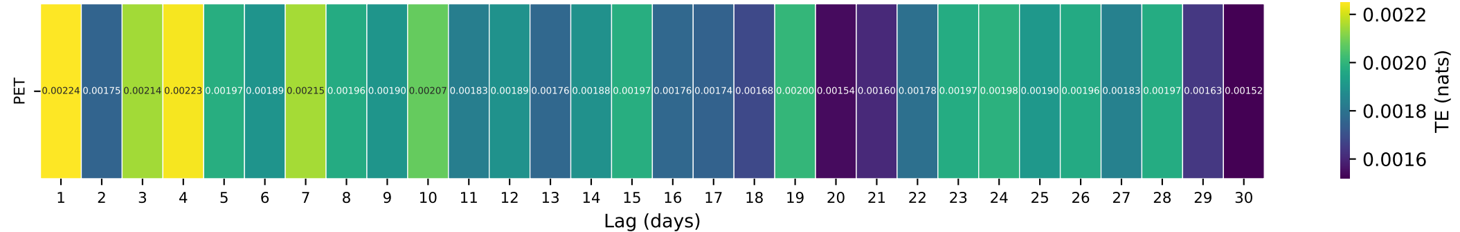
Gauge ID: 05584500 | LA MOINE RIVER AT COLMAR, IL | PET(t-\tau) \rightarrow Q(t)
