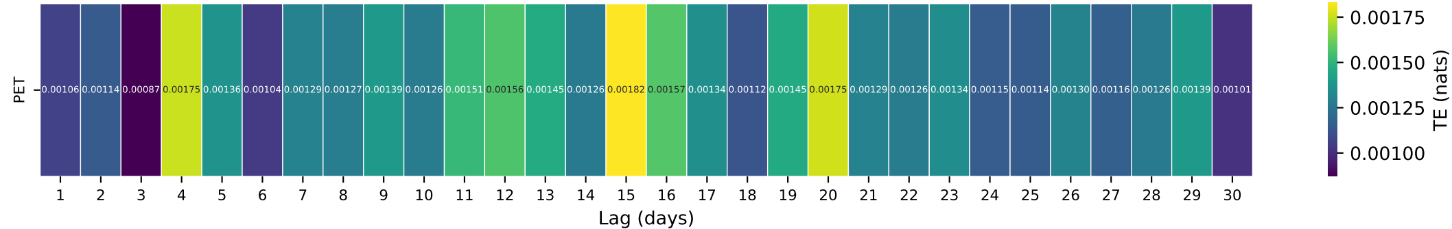
Gauge ID: 08171300 | Blanco Rv nr Kyle, TX | PET(t- \tau ) \rightarrow Q(t)
