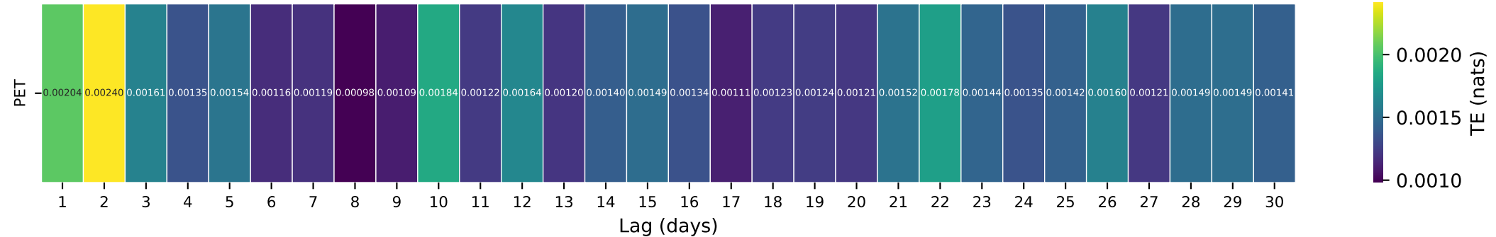
Gauge ID: 07376000 | Tickfaw River at Holden, LA | PET(t-\tau) \rightarrow Q(t)
