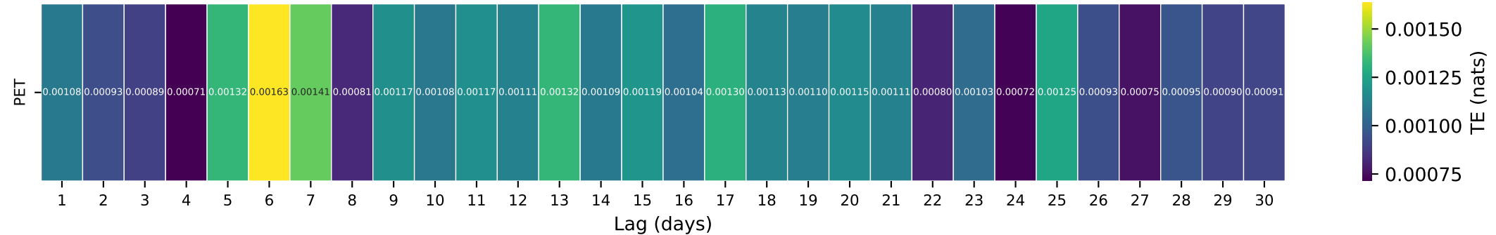
Gauge ID: 06450500 | LITTLE WHITE R BELOW WHITE RIVER SD | PET(t- \tau ) \rightarrow Q(t)
