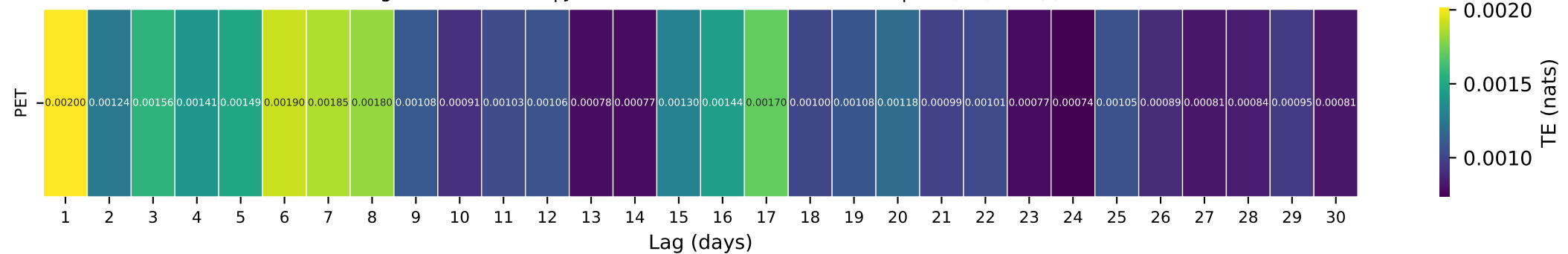
Gauge ID: 06468170 | JAMES RIVER NR GRACE CITY, ND | PET(t-\tau) \rightarrow Q(t)
