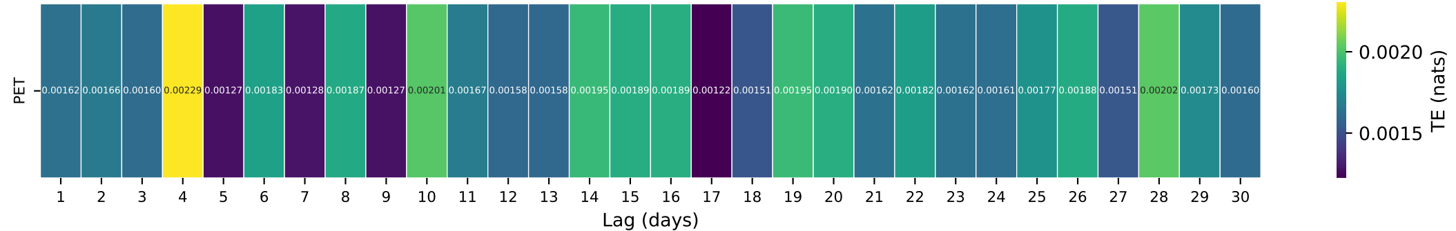
Gauge ID: 02111500 | REDDIES RIVER AT NORTH WILKESBORO, NC | PET(t-\tau) \rightarrow Q(t)
