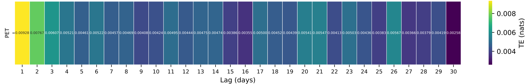
Gauge ID: 08271000 | RIO LUCERO NEAR ARROYO SECO, NM | PET(t- \tau ) \rightarrow Q(t)
