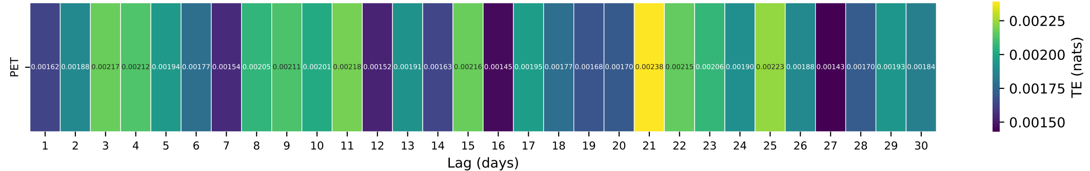
Gauge ID: 07145700 | SLATE C AT WELLINGTON, KS | PET(t- \tau ) \rightarrow Q(t)
