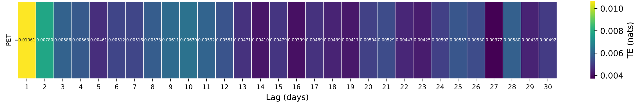
Gauge ID: 10316500 | LAMOILLE C NR LAMOILLE, NV | PET(t- \tau ) \rightarrow Q(t)
