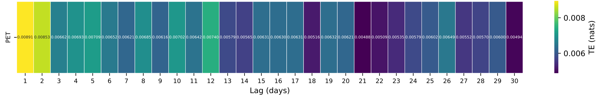
Gauge ID: 06746095 | JOE WRIGHT CREEK ABOVE JOE WRIGHT RESERVOIR, CO. | PET(t-\tau) \rightarrow Q(t)
