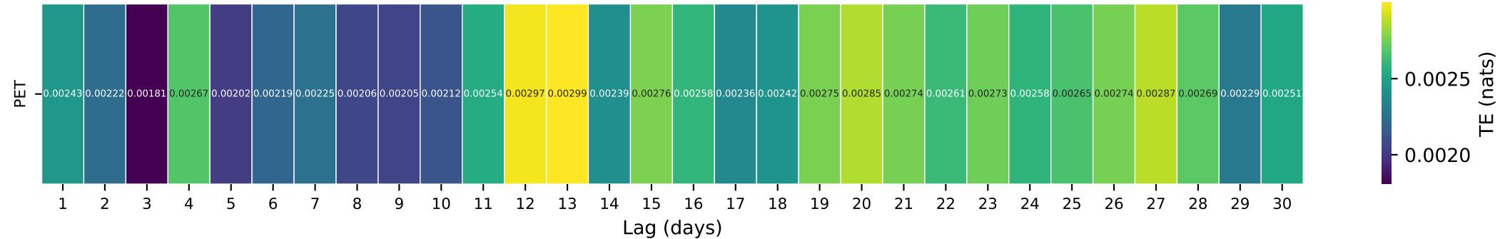
Gauge ID: 07295000 | BUFFALO RIVER NR WOODVILLE, MS | PET(t-\tau) \rightarrow Q(t)
