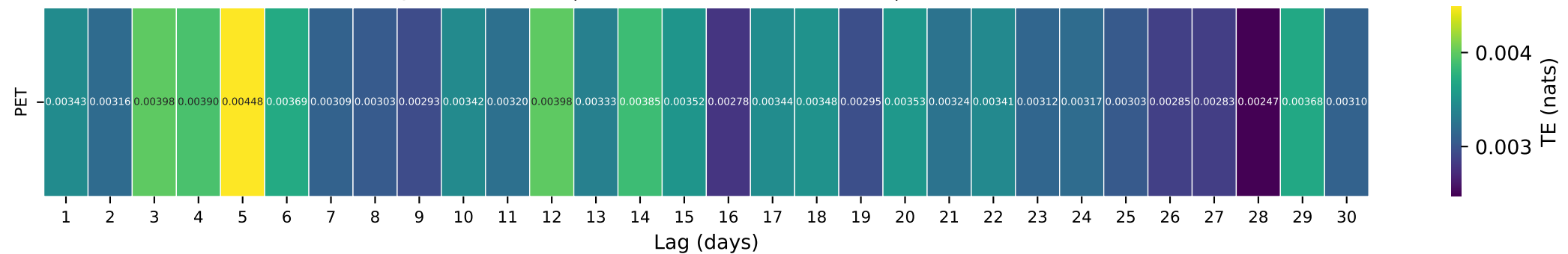
Gauge ID: 06878000 | CHAPMAN C NR CHAPMAN, KS | PET(t- \tau ) \rightarrow Q(t)
