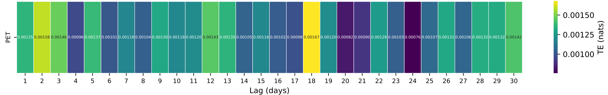
Gauge ID: 09404450 | EAST FORK VIRGIN RIVER NEAR GLENDALE, UT | PET(t-\tau) \rightarrow Q(t)
