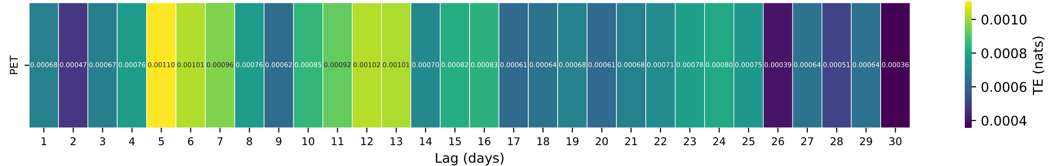
Gauge ID: 06889200 | SOLDIER C NR DELIA, KS | PET(t-\tau) \rightarrow Q(t)
