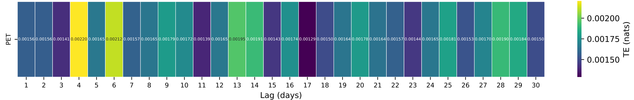
Gauge ID: 05412500 | Turkey River at Garber, IA | PET(t-\tau) \rightarrow Q(t)
