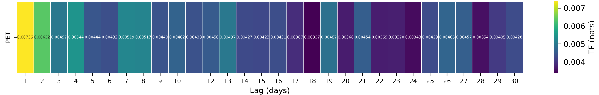
Gauge ID: 09035800 | DARLING CREEK NEAR LEAL, CO. | PET(t- \tau ) \rightarrow Q(t)
