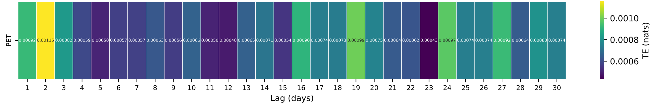
Gauge ID: 03066000 | BLACKWATER R AT DAVIS, WV | PET(t- \tau ) \rightarrow Q(t)
