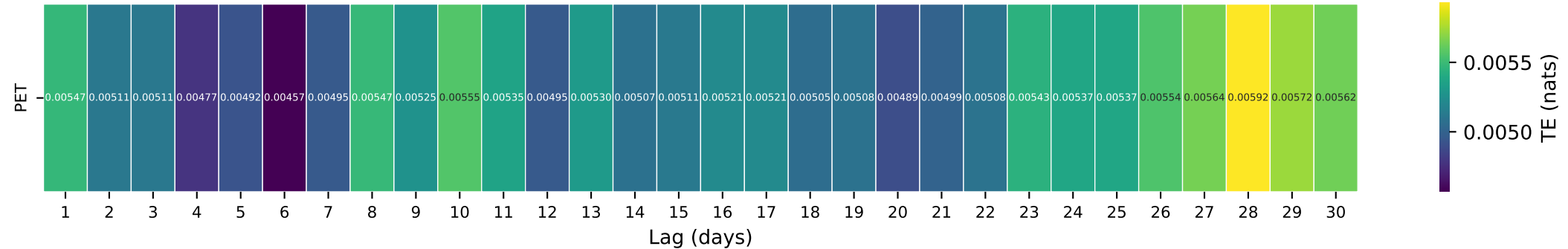
Gauge ID: 12025700 | SKOOKUMCHUCK RIVER NEAR VAIL, WA | PET(t-\tau) \rightarrow Q(t)
