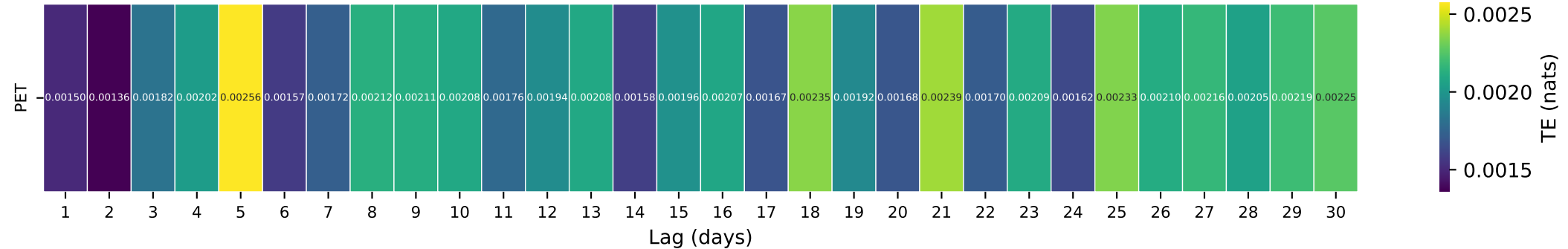
Gauge ID: 02053800 | S F ROANOKE RIVER NEAR SHAWSVILLE, VA | PET(t-\tau) \rightarrow Q(t)
