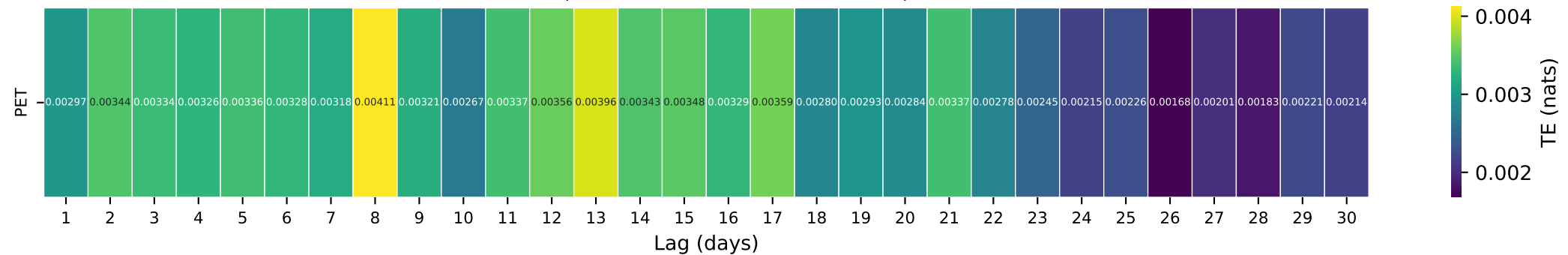
Gauge ID: 01013500 | Fish River near Fort Kent, Maine | PET(t-\tau) \rightarrow Q(t)
