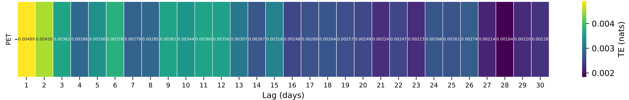
Gauge ID: 04059500 | FORD RIVER NEAR HYDE, MI | PET(t- \tau ) \rightarrow Q(t)
