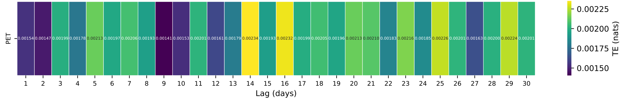
Gauge ID: 05595730 | RAYSE CREEK NEAR WALTONVILLE, IL | PET(t-\tau) \rightarrow Q(t)
