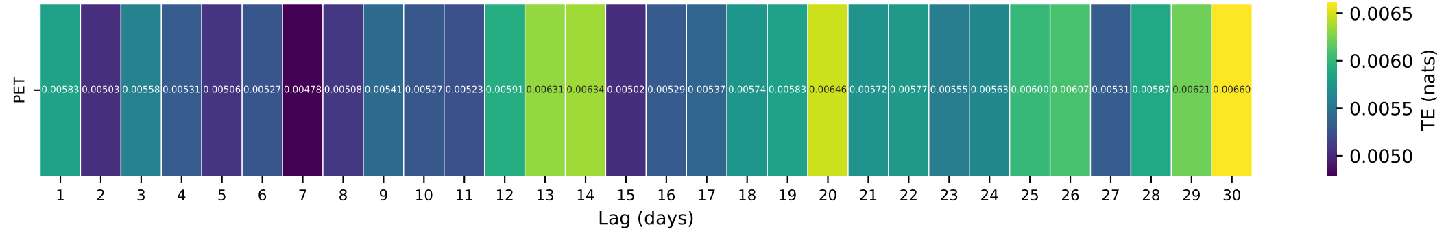
Gauge ID: 14158500 | MCKENZIE RIVER AT OUTLET OF CLEAR LAKE, OR | PET(t-\tau) \rightarrow Q(t)
