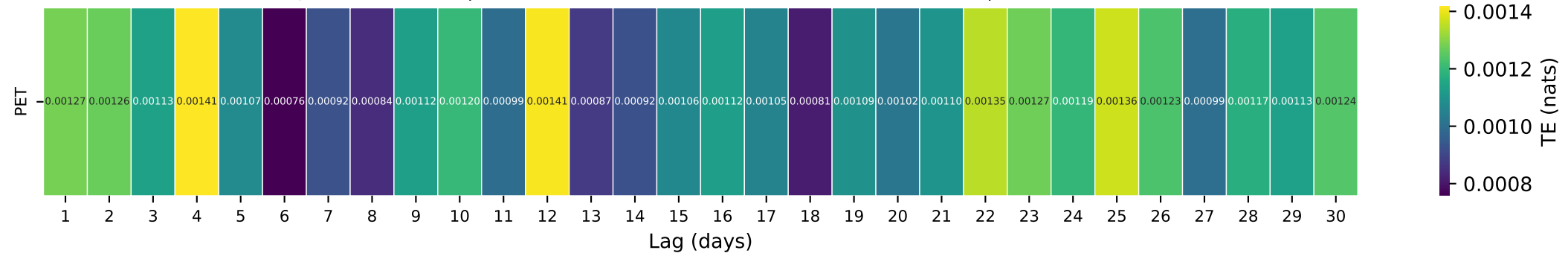
Gauge ID: 01118300 | PENDLETON HILL BROOK NEAR CLARKS FALLS, CT. | PET(t-\tau) \rightarrow Q(t)
