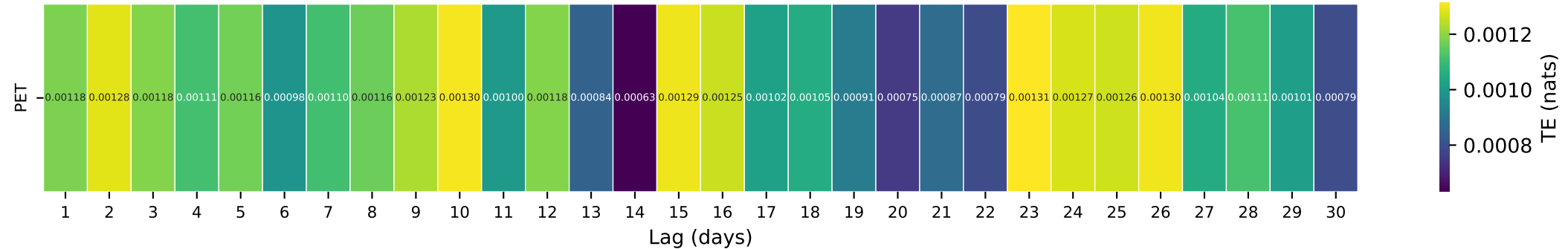
Gauge ID: 02363000 | PEA RIVER NEAR ARITON AL | PET(t- \tau ) \rightarrow Q(t)
