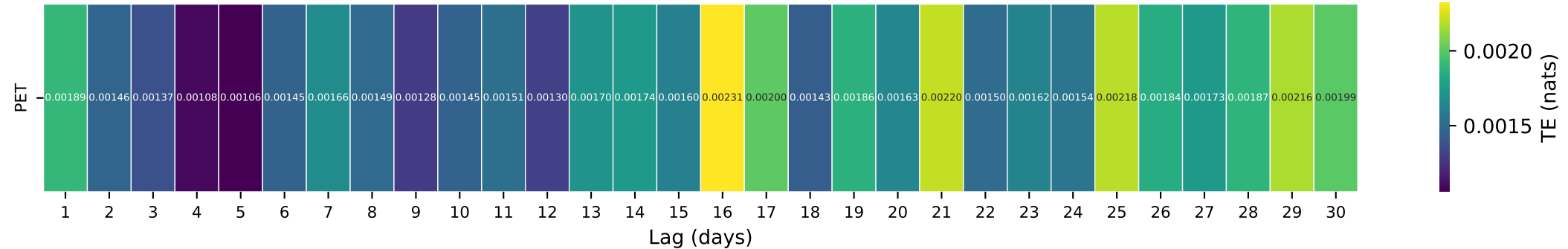
Gauge ID: 02013000 | DUNLAP CREEK NEAR COVINGTON, VA | PET(t-\tau) \rightarrow Q(t)
