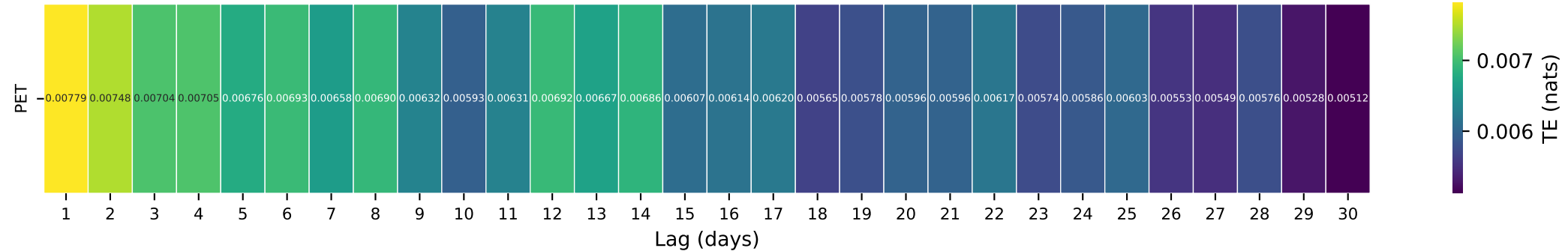
Gauge ID: 12054000 | DUCKABUSH RIVER NEAR BRINNON, WA | PET(t-\tau) \rightarrow Q(t)
