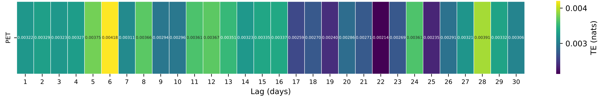
Gauge ID: 07208500 | RAYADO CREEK NEAR CIMARRON, NM | PET(t-\tau) \rightarrow Q(t)
