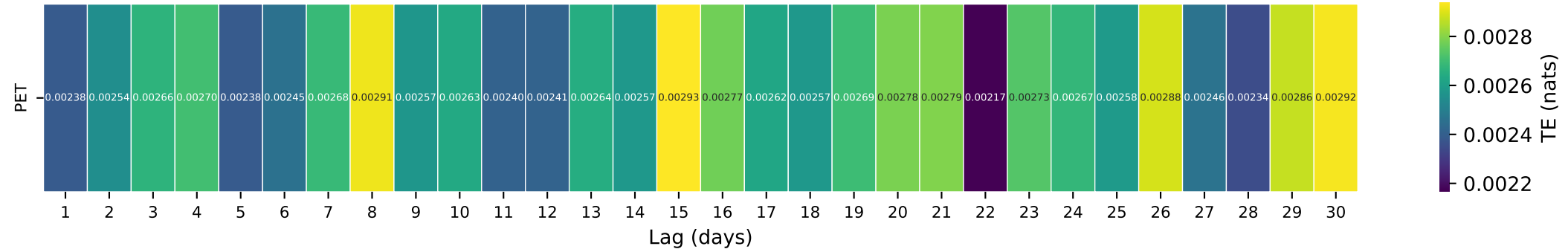
Gauge ID: 05591550 | WHITLEY CREEK NEAR ALLENVILLE, IL | PET(t-\tau) \rightarrow Q(t)
