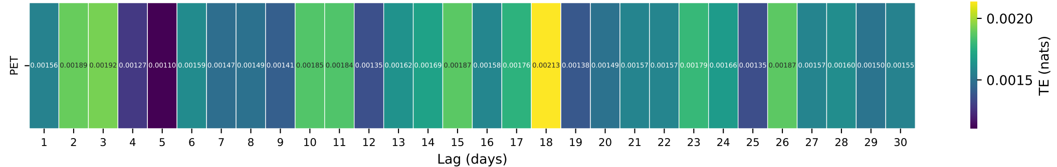
Gauge ID: 02202600 | BLACK CREEK NEAR BLITCHTON, GA | PET(t-\tau) \rightarrow Q(t)
