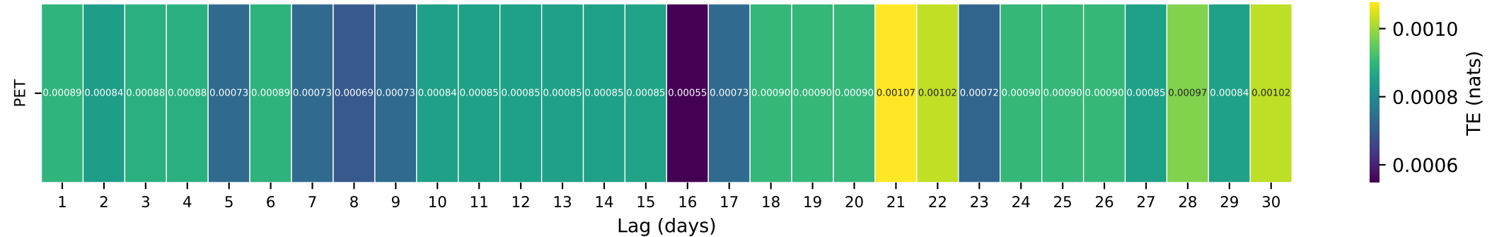
Gauge ID: 09505800 | WEST CLEAR CREEK NEAR CAMP VERDE, AZ. | PET(t-\tau) \rightarrow Q(t)
