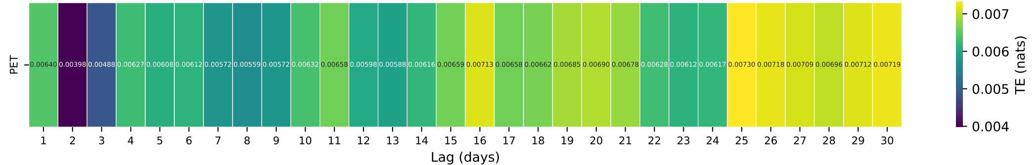
Gauge ID: 04127997 | STURGEON RIVER AT WOLVERINE, MI | PET(t-\tau) \rightarrow Q(t)
