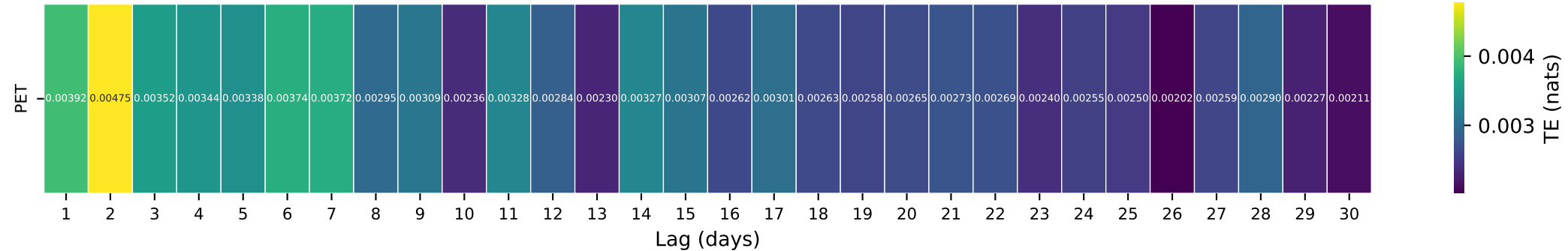
Gauge ID: 12390700 | Prospect Creek at Thompson Falls MT | PET(t-\tau) \rightarrow Q(t)
