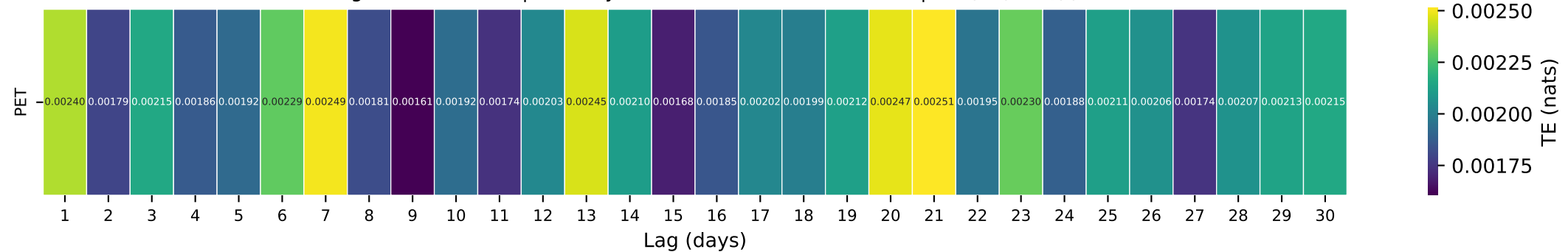
Gauge ID: 08014500 | Whiskey Chitto Creek Near Oberlin, LA | PET(t-\tau) \rightarrow Q(t)
