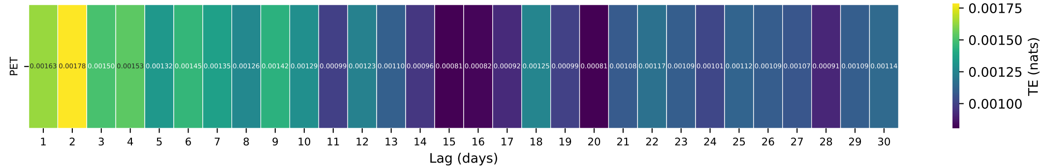
Gauge ID: 12178100 | NEWHALEM CREEK NEAR NEWHALEM, WA | PET(t-\tau) \rightarrow Q(t)
