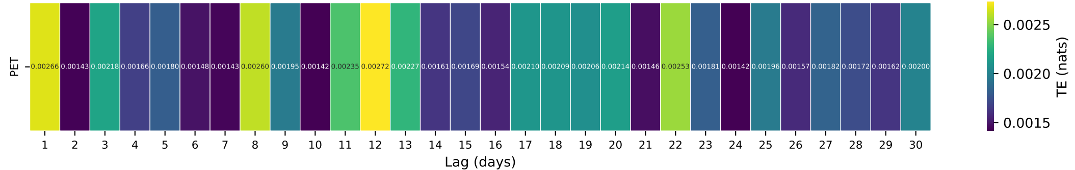
Gauge ID: 01055000 | Swift River near Roxbury, Maine | PET(t-\tau) \rightarrow Q(t)
