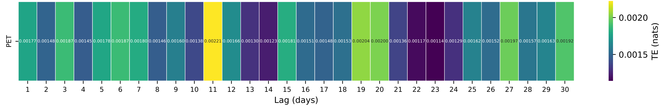
Gauge ID: 06404000 | BATTLE CR NEAR KEYSTONE SD | PET(t- \tau ) \rightarrow Q(t)
