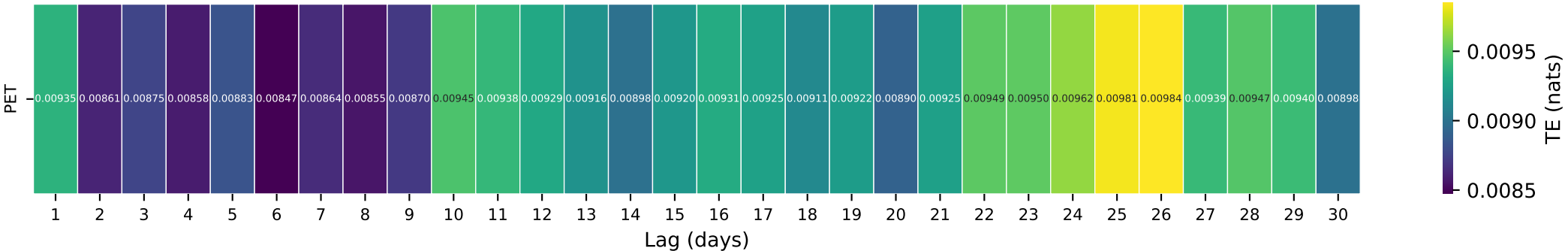
Gauge ID: 12025000 | NEWAUKUM RIVER NEAR CHEHALIS, WA | PET(t-τ) → Q(t)
