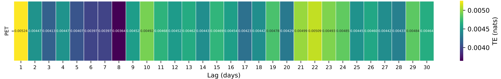
Gauge ID: 12147500 | NORTH FORK TOLT RIVER NEAR CARNATION, WA | PET(t-\tau) \rightarrow Q(t)
