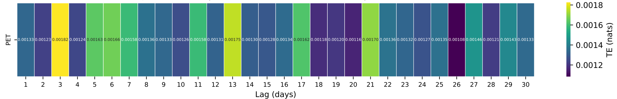
Gauge ID: 02118500 | HUNTING CREEK NEAR HARMONY, NC | PET(t-\tau) \rightarrow Q(t)
