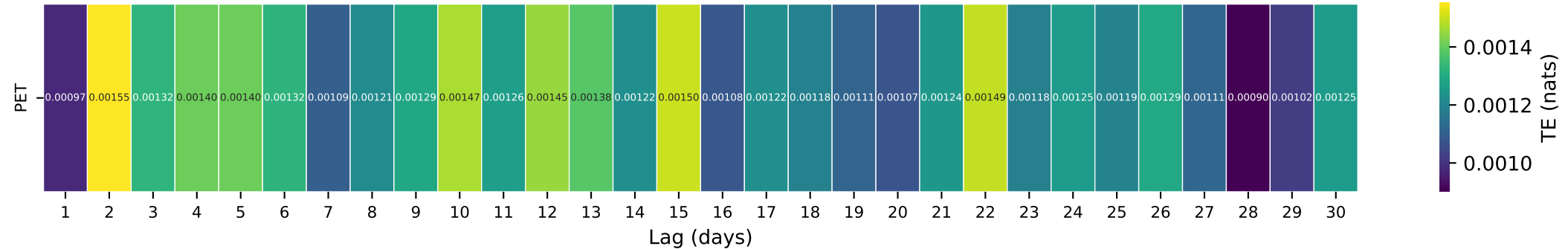
Gauge ID: 07167500 | OTTER C AT CLIMAX, KS | PET(t-\tau) \rightarrow Q(t)
