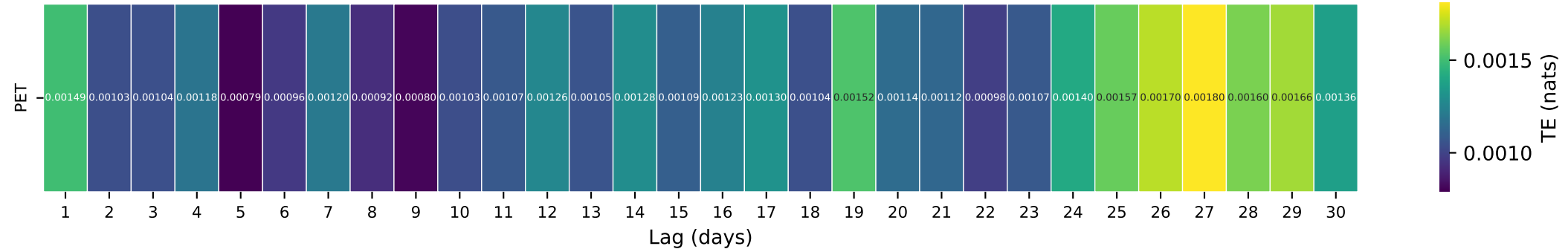
Gauge ID: 03574500 | PAINT ROCK RIVER NEAR WOODVILLE AL | PET(t-\tau) \rightarrow Q(t)
