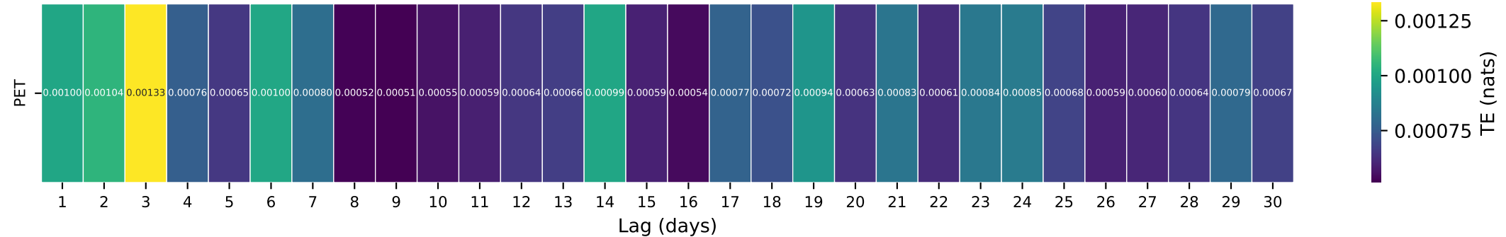
Gauge ID: 02053200 | POTECASI CREEK NEAR UNION, NC | PET(t-\tau) \rightarrow Q(t)
