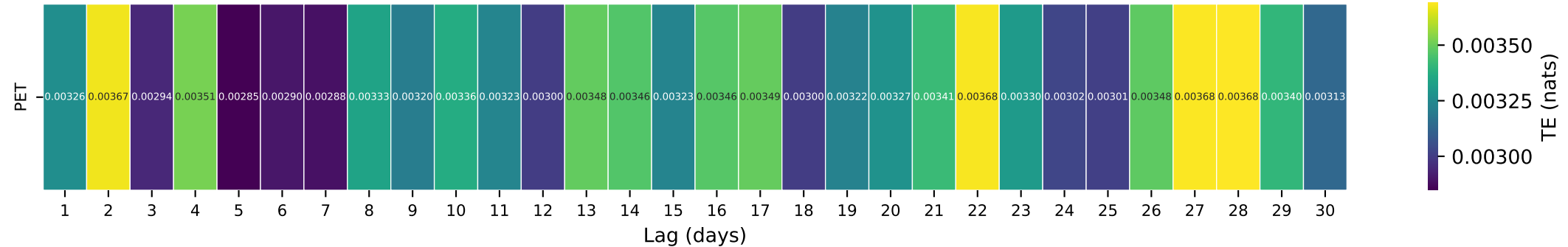
Gauge ID: 12143600 | SF SNOQUALMIE RIVER AT EDGEWICK, WA | PET(t-\tau) \rightarrow Q(t)
