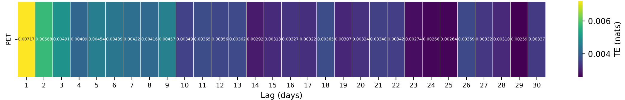
Gauge ID: 11230500 | BEAR C NR LAKE THOMAS A EDISON CA | PET(t-\tau) \rightarrow Q(t)
