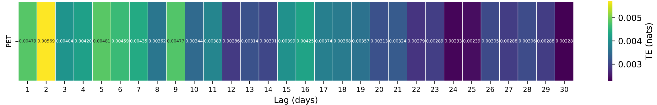
Gauge ID: 06409000 | CASTLE CR ABOVE DEERFIELD RES NEAR HILL CITY SD | PET(t-\tau) \rightarrow Q(t)
