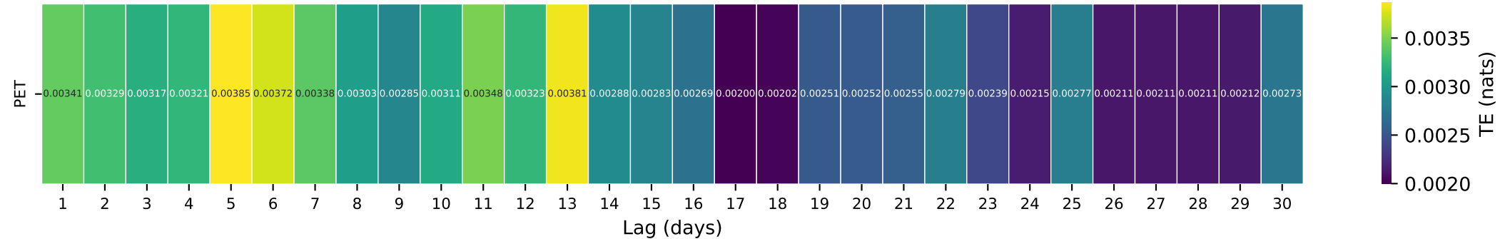
Gauge ID: 13161500 | BRUNEAU RIVER AT ROWLAND NV | PET(t-\tau) \rightarrow Q(t)
