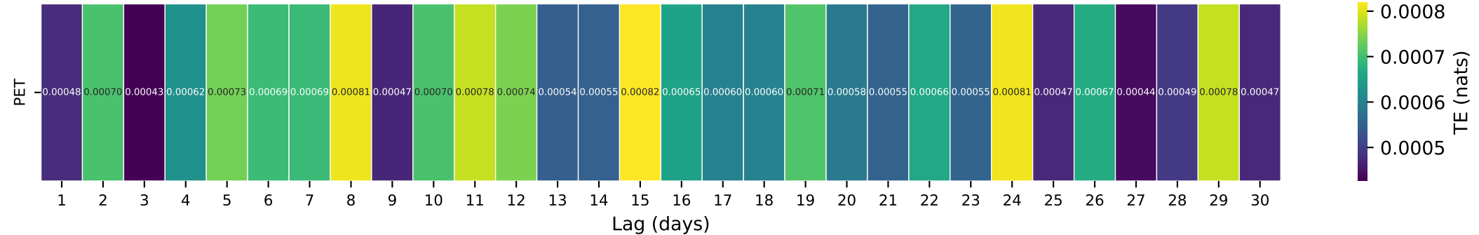
Gauge ID: 02361000 | CHOCTAWHATCHEE RIVER NEAR NEWTON, AL. | PET(t-\tau) \rightarrow Q(t)
