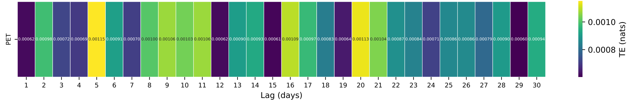
Gauge ID: 07142300 | RATTLESNAKE C NR MACKSVILLE, KS | PET(t- \tau ) \rightarrow Q(t)
