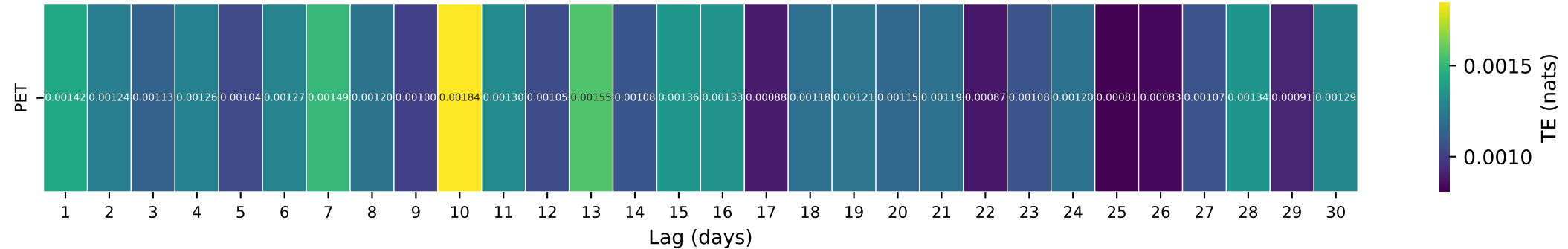
Gauge ID: 02384540 | MILL CREEK NEAR CRANDALL, GA | PET(t-\tau) \rightarrow Q(t)
