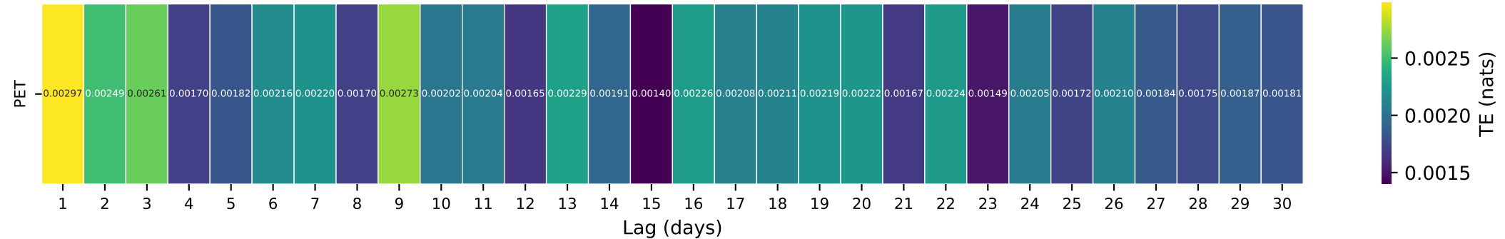
Gauge ID: 06906800 | Lamine River near Otterville, MO | PET(t- \tau ) \rightarrow Q(t)
