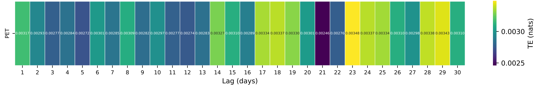
Gauge ID: 07261000 | Cadron Creek near Guy, AR | PET(t-\tau) \rightarrow Q(t)
