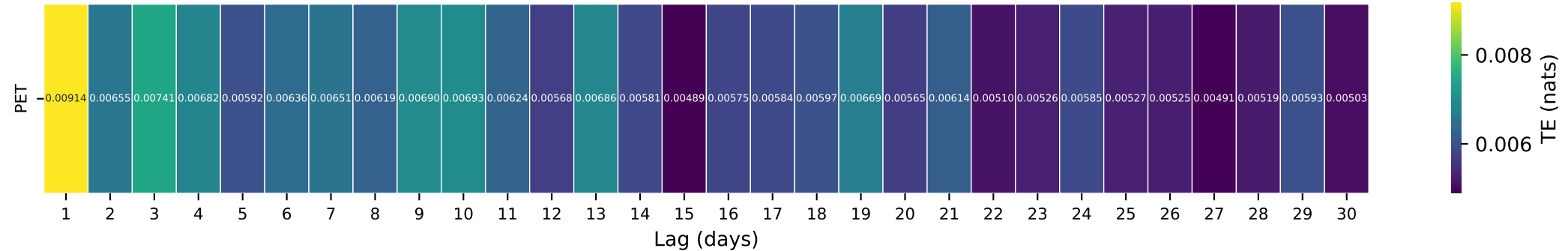
Gauge ID: 09034900 | BOBTAIL CREEK NEAR JONES PASS, CO. | PET(t-\tau) \rightarrow Q(t)
