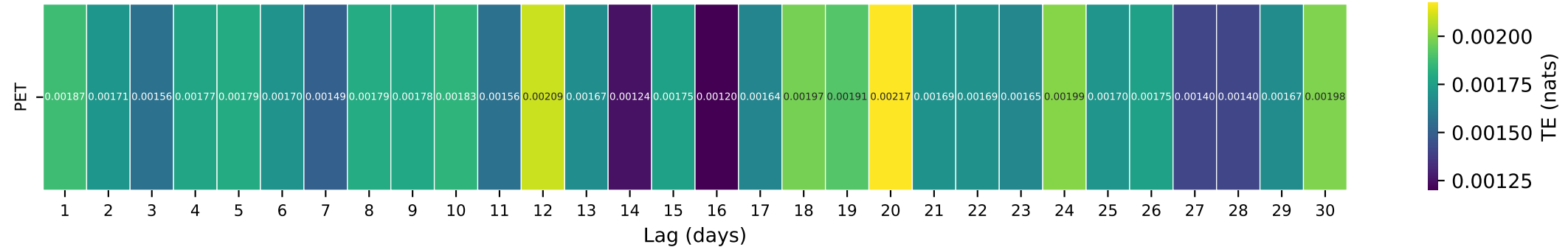
Gauge ID: 06921070 | Pomme de Terre River near Polk, MO | PET(t-\tau) \rightarrow Q(t)
