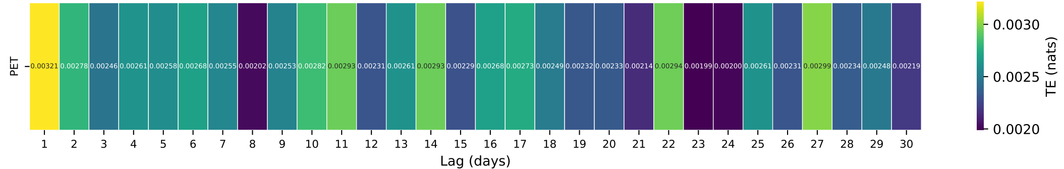
Gauge ID: 05501000 | North River at Palmyra, MO | PET(t-\tau) \rightarrow Q(t)
