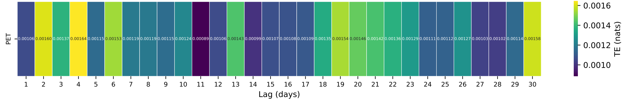
Gauge ID: 02102908 | FLAT CREEK NEAR INVERNESS, NC | PET(t- \tau ) \rightarrow Q(t)
