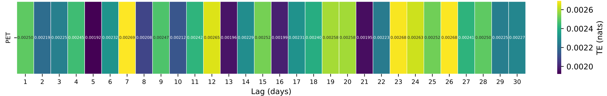
Gauge ID: 02193340 | KETTLE CREEK NEAR WASHINGTON, GA | PET(t-\tau) \rightarrow Q(t)
