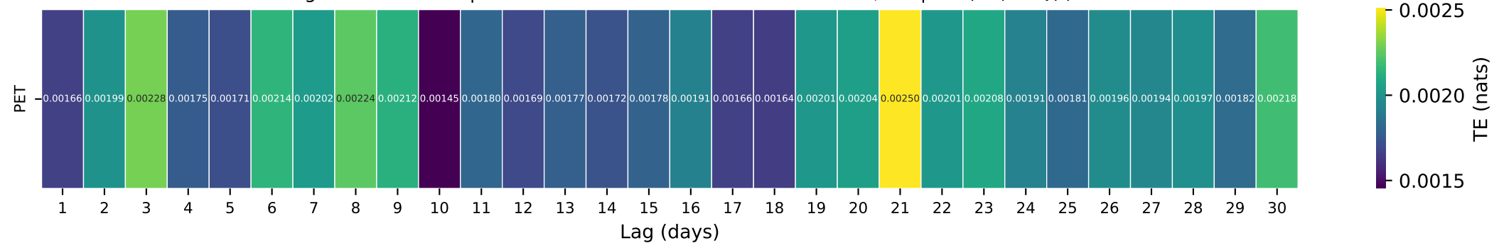
Gauge ID: 01121000 | MOUNT HOPE RIVER NEAR WARRENVILLE, CT. | PET(t-\tau) \rightarrow Q(t)
