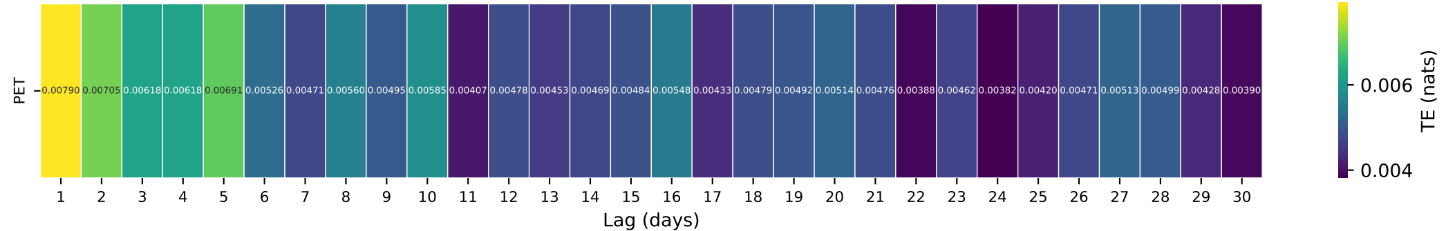
Gauge ID: 09035900 | SOUTH FORK OF WILLIAMS FORK NEAR LEAL, CO. | PET(t- \tau ) \rightarrow Q(t)
