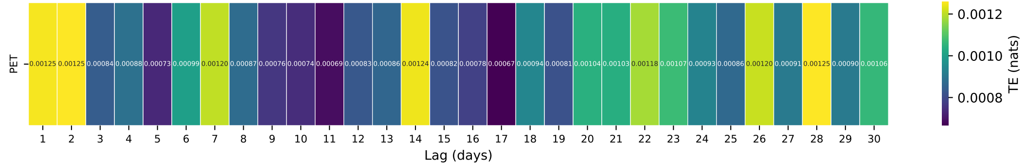
Gauge ID: 03161000 | SOUTH FORK NEW RIVER NEAR JEFFERSON, NC | PET(t-\tau) \rightarrow Q(t)
