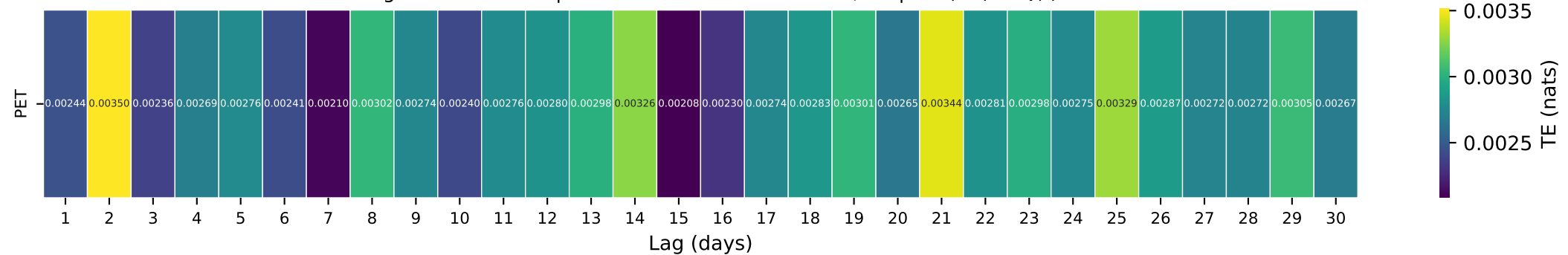
Gauge ID: 10023000 | BIG CREEK NEAR RANDOLPH, UT | PET(t-\tau) \rightarrow Q(t)
