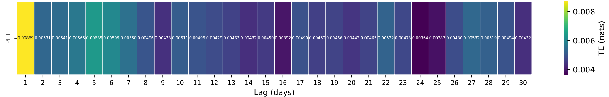
Gauge ID: 06623800 | ENCAMPMENT RIVER AB HOG PARK CR, NR ENCAMPMENT, WY | PET(t-\tau) \rightarrow Q(t)
