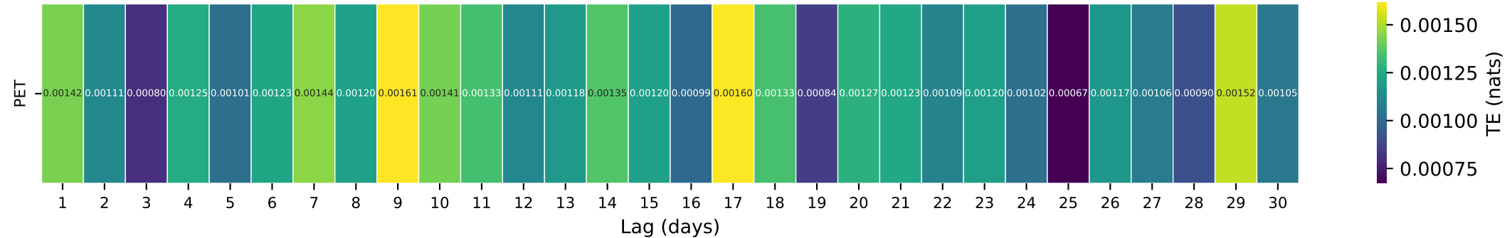
Gauge ID: 03340800 | BIG RACCOON CREEK NEAR FINCASTLE IND | PET(t-\tau) \rightarrow Q(t)
