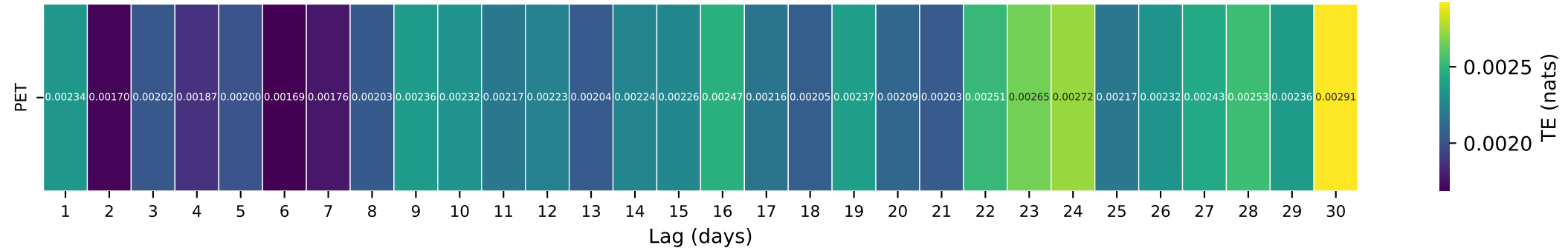
Gauge ID: 02125000 | BIG BEAR CR NR RICHFIELD, NC | PET( t-\tau ) \rightarrow Q( t )
