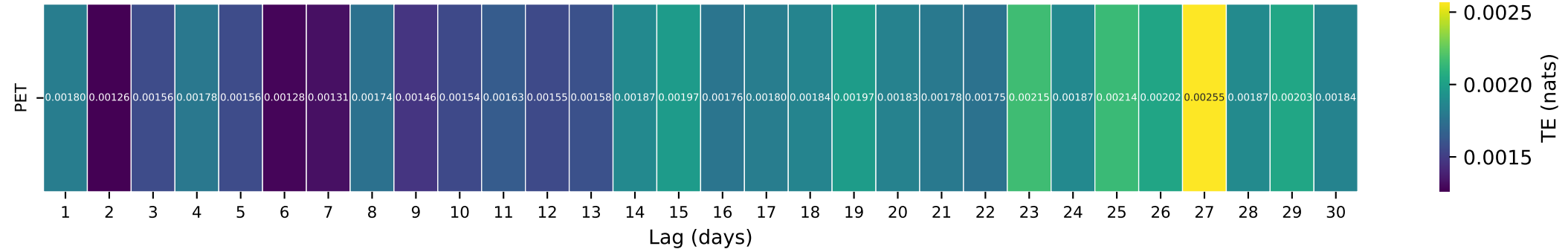
Gauge ID: 03159540 | Shade River near Chester OH | PET(t-\tau) \rightarrow Q(t)
