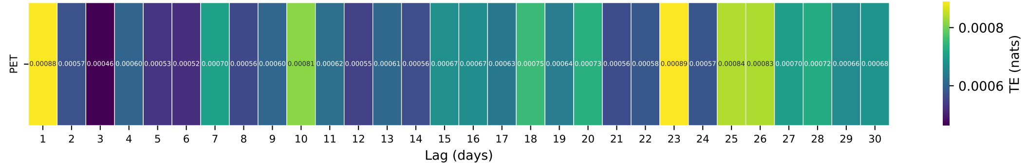
Gauge ID: 02038850 | HOLIDAY CREEK NEAR ANDERSONVILLE, VA | PET(t-\tau) \rightarrow Q(t)
