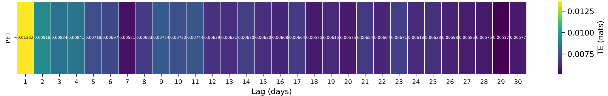
Gauge ID: 09065500 | GORE CREEK AT UPPER STATION, NEAR MINTURN, CO. | PET(t-\tau) \rightarrow Q(t)
