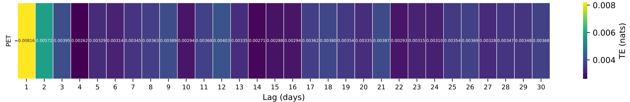
Gauge ID: 04124000 | MANISTEE RIVER NEAR SHERMAN, MI | PET(t-\tau) \rightarrow Q(t)
