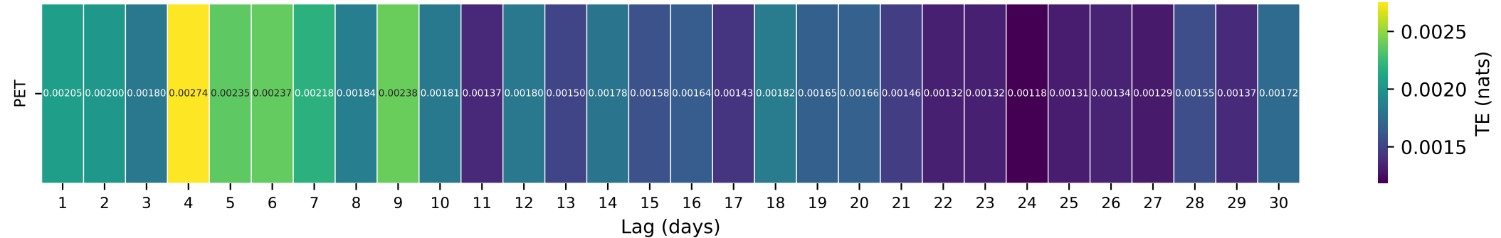
Gauge ID: 05087500 | MIDDLE RIVER AT ARGYLE, MN | PET(t- \tau ) \rightarrow Q(t)
