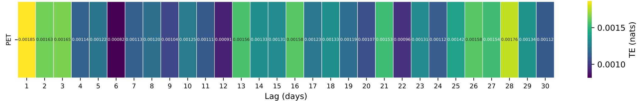
Gauge ID: 01485500 | NASSAWANGO CREEK NEAR SNOW HILL, MD | PET(t-\tau) \rightarrow Q(t)
