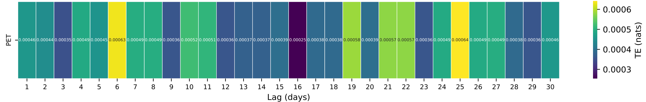
Gauge ID: 08086290 | Big Sandy Ck abv Breckenridge, TX | PET(t-\tau) \rightarrow Q(t)
