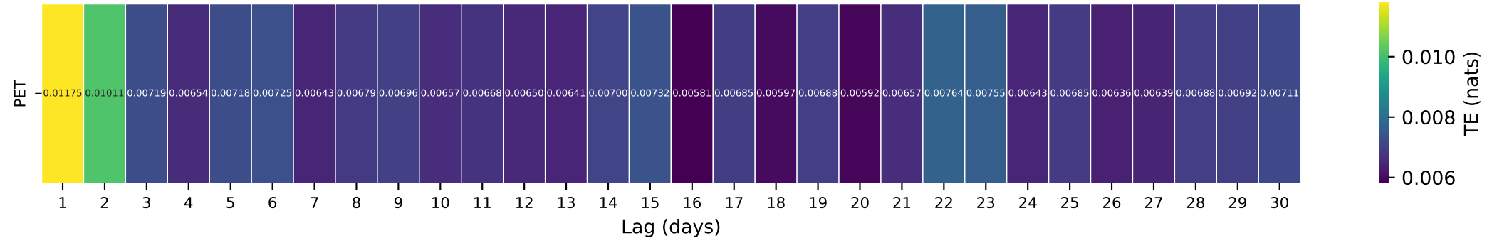
Gauge ID: 06191500 | Yellowstone River at Corwin Springs MT | PET(t-\tau) \rightarrow Q(t)
