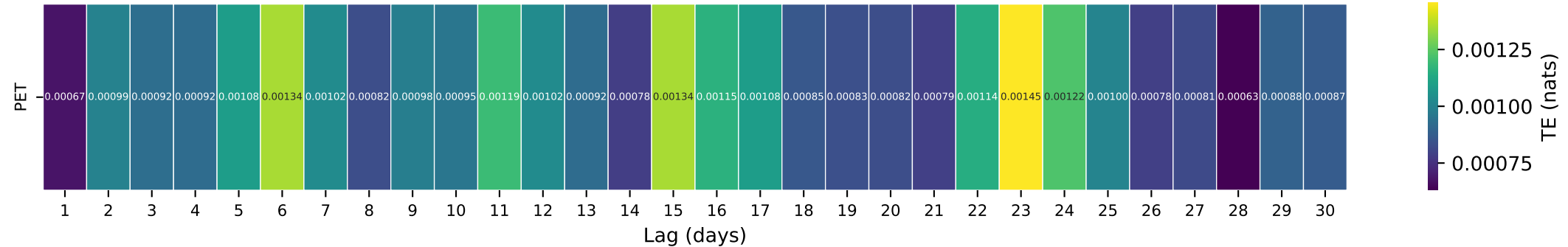
Gauge ID: 05556500 | BIG BUREAU CREEK AT PRINCETON, IL | PET(t-\tau) \rightarrow Q(t)
