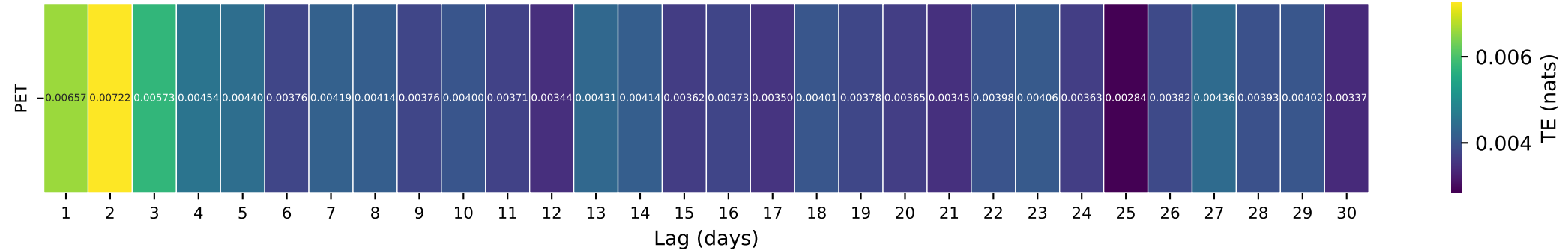
Gauge ID: 13240000 | LAKE FORK PAYETTE RIVER AB JUMBO CR NR MCCALL ID | PET(t-\tau) \rightarrow Q(t)
