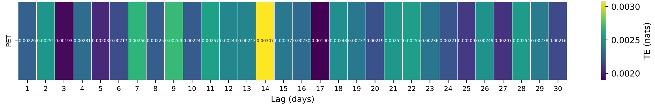
Gauge ID: 05508805 | Spencer Cr. bl Plum Cr. nr Frankford, MO | PET(t- \tau ) \rightarrow Q(t)
