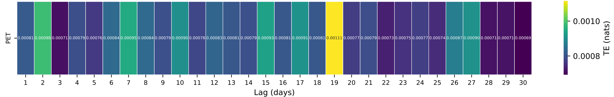
Gauge ID: 08202700 | Seco Ck at Rowe Ranch nr D'Hanis, TX | PET(t- \tau ) \rightarrow Q(t)
