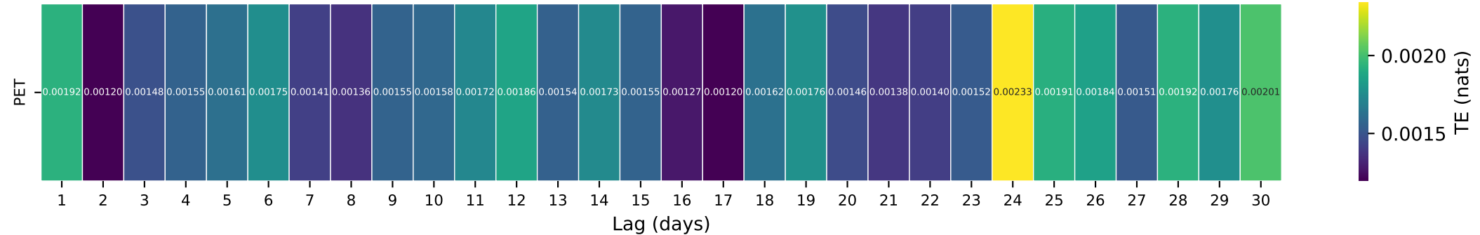
Gauge ID: 01586610 | MORGAN RUN NEAR LOUISVILLE, MD | PET(t-\tau) \rightarrow Q(t)
