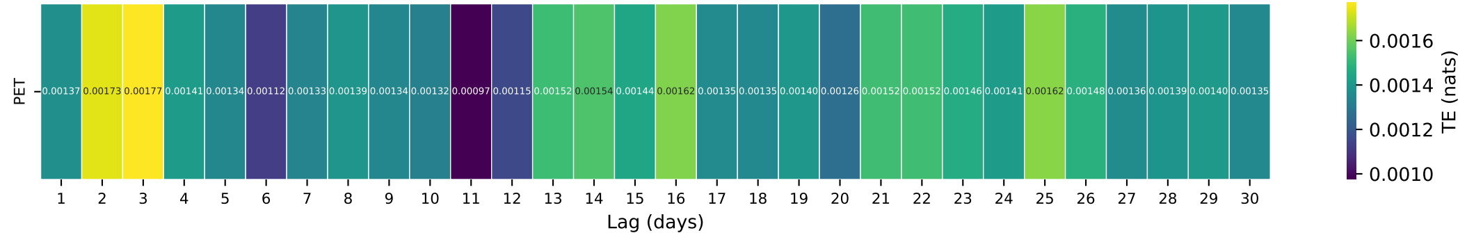
Gauge ID: 01632900 | SMITH CREEK NEAR NEW MARKET, VA | PET(t-\tau) \rightarrow Q(t)
