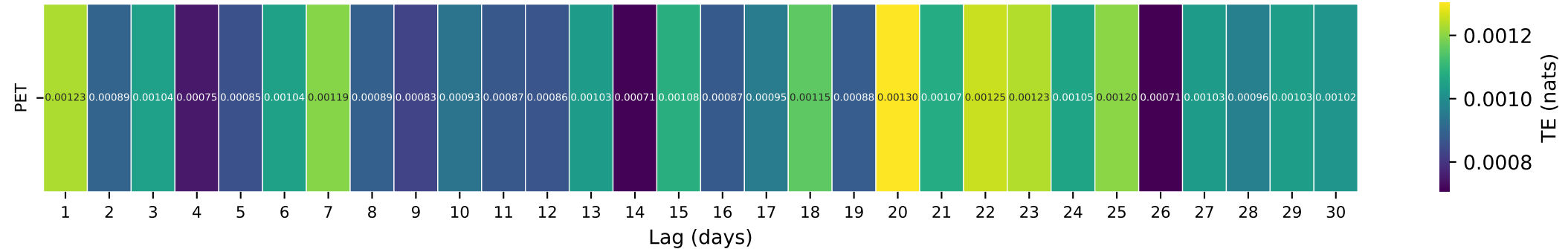
Gauge ID: 03463300 | SOUTH TOE RIVER NEAR CELO, NC | PET(t-\tau) \rightarrow Q(t)
