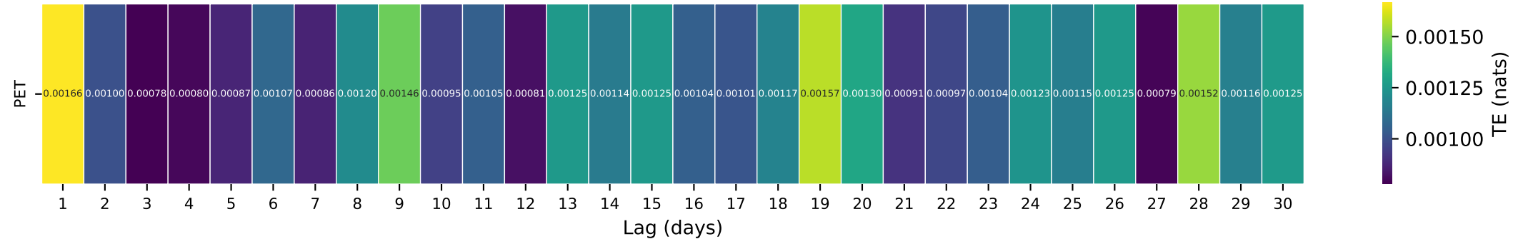
Gauge ID: 03164000 | NEW RIVER NEAR GALAX, VA | PET(t- \tau ) \rightarrow Q(t)
