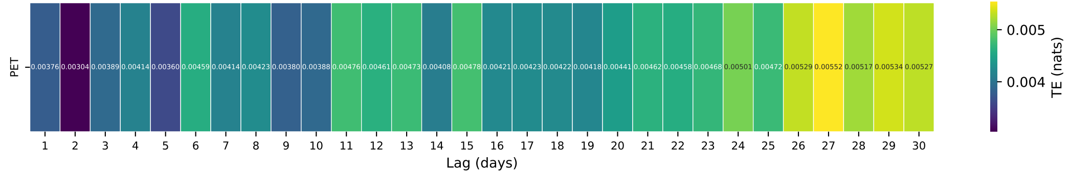
Gauge ID: 01333000 | GREEN RIVER AT WILLIAMSTOWN, MA | PET(t-\tau) \rightarrow Q(t)
