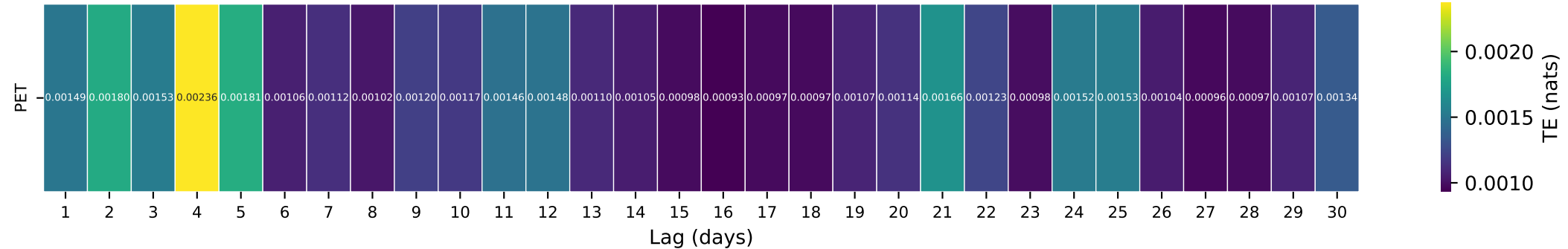
Gauge ID: 09386900 | RIO NUTRIA NEAR RAMAH, NM | PET(t- \tau ) \rightarrow Q(t)
