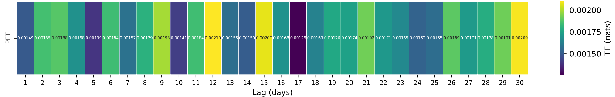
Gauge ID: 01435000 | NEVERSINK RIVER NEAR CLARYVILLE NY | PET(t-\tau) \rightarrow Q(t)
