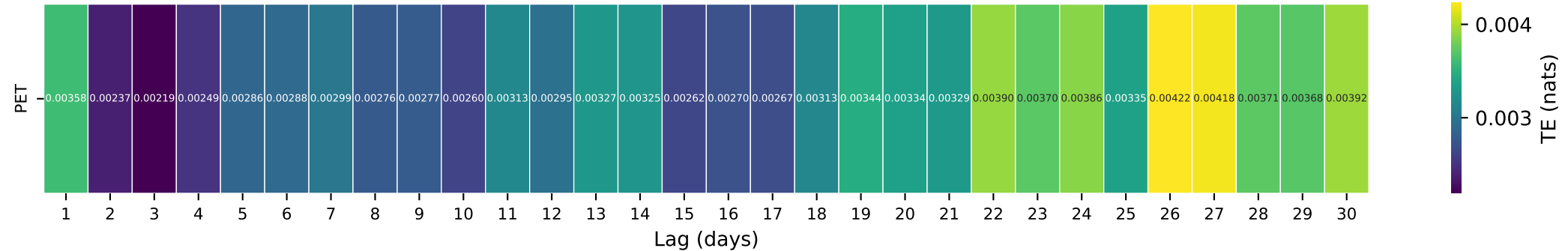
Gauge ID: 03070500 | BIG SANDY CREEK AT ROCKVILLE, WV | PET(t-\tau) \rightarrow Q(t)
