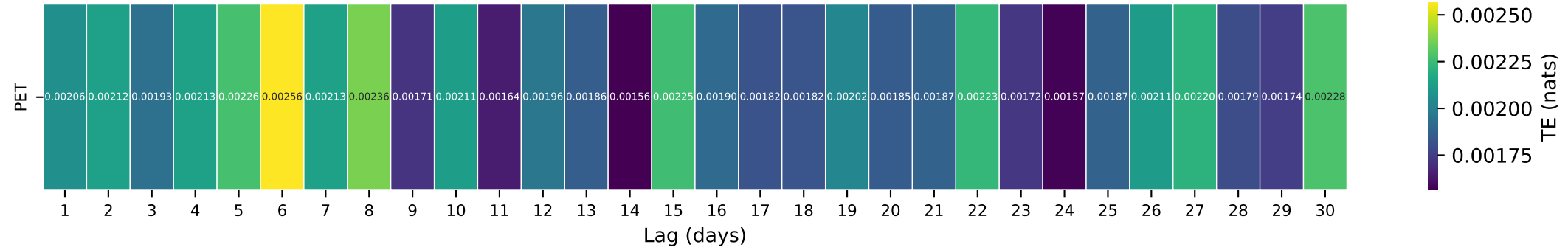
Gauge ID: 05454000 | Rapid Creek near Iowa City, IA | PET(t-\tau) \rightarrow Q(t)
