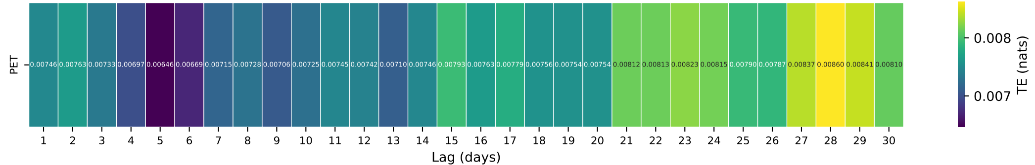
Gauge ID: 14166500 | LONG TOM RIVER NEAR NOTI, OREG. | PET(t-\tau) \rightarrow Q(t)
