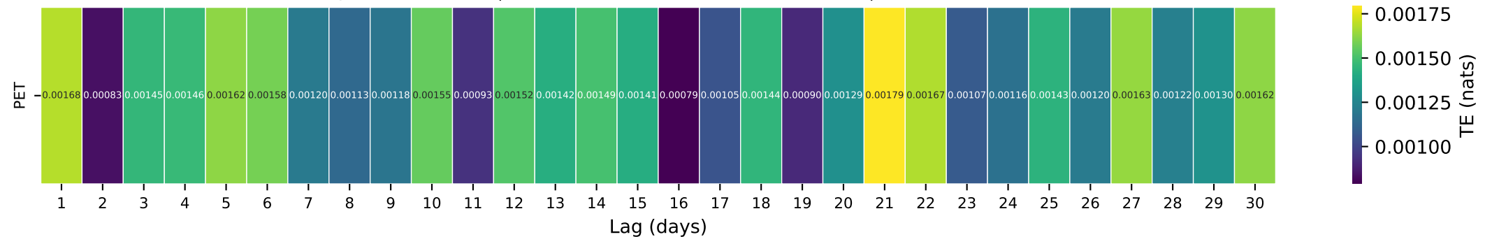
Gauge ID: 02300700 | BULLFROG CREEK NEAR WIMAUMA FL | PET(t- \tau ) \rightarrow Q(t)
