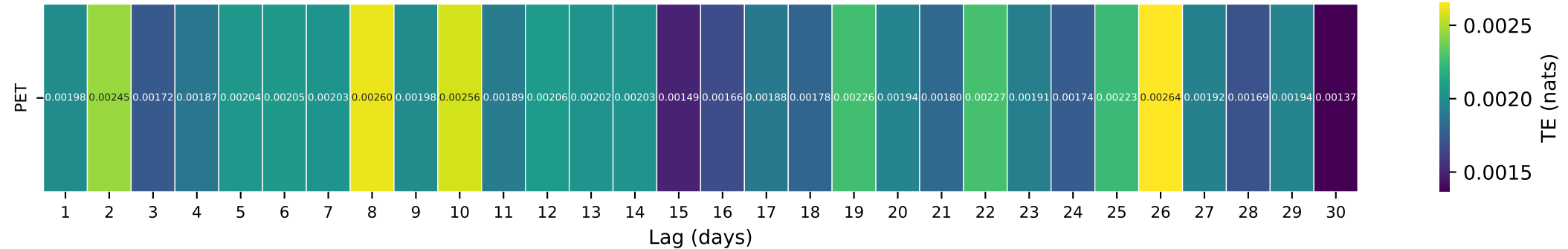
Gauge ID: 06431500 | SPEARFISH CR AT SPEARFISH SD | PET(t- \tau ) \rightarrow Q(t)
