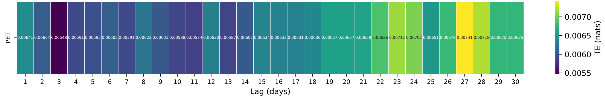
Gauge ID: 14154500 | ROW RIVER ABOVE PITCHER CREEK NEAR, DORENA, OREG | PET(t-\tau) \rightarrow Q(t)
