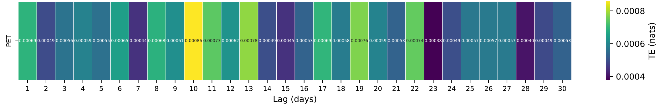
Gauge ID: 04015330 | KNIFE RIVER NEAR TWO HARBORS, MN | PET(t-\tau) \rightarrow Q(t)
