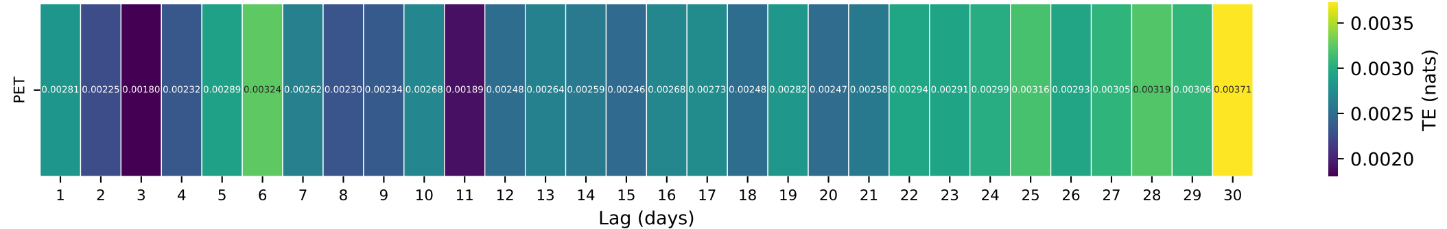
Gauge ID: 02081500 | TAR RIVER NEAR TAR RIVER, NC | PET(t-\tau) \rightarrow Q(t)
