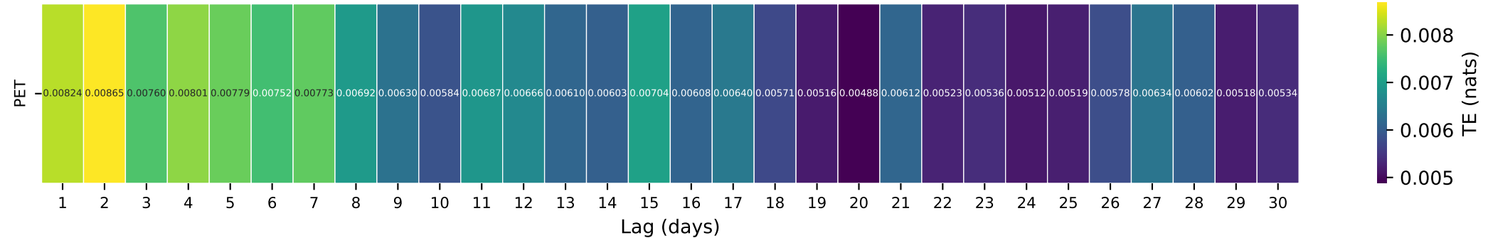
Gauge ID: 12414500 | ST JOE RIVER AT CALDER ID | PET(t-\tau) \rightarrow Q(t)
