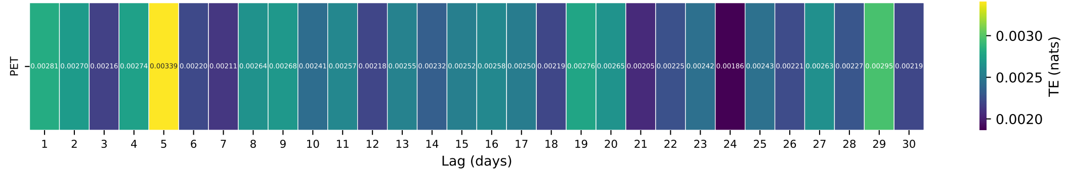
Gauge ID: 03338780 | NORTH FORK VERMILION RIVER NEAR BISMARCK, IL | PET(t-\tau) \rightarrow Q(t)
