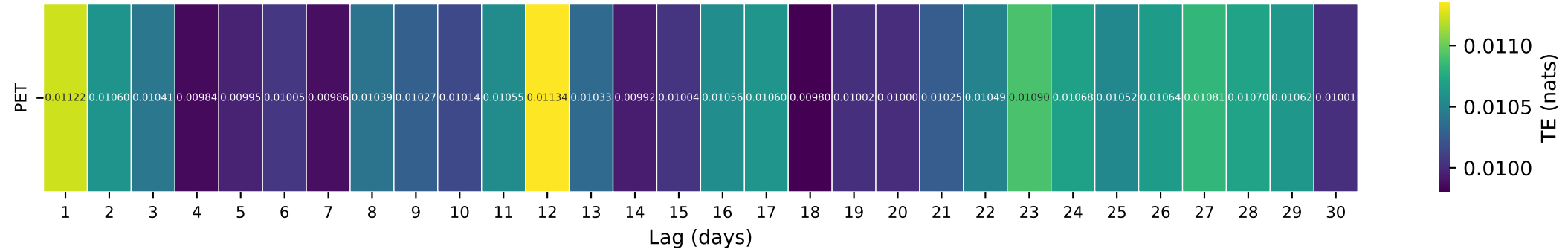
Gauge ID: 12013500 | WILLAPA RIVER NEAR WILLAPA, WA | PET(t-\tau) \rightarrow Q(t)
