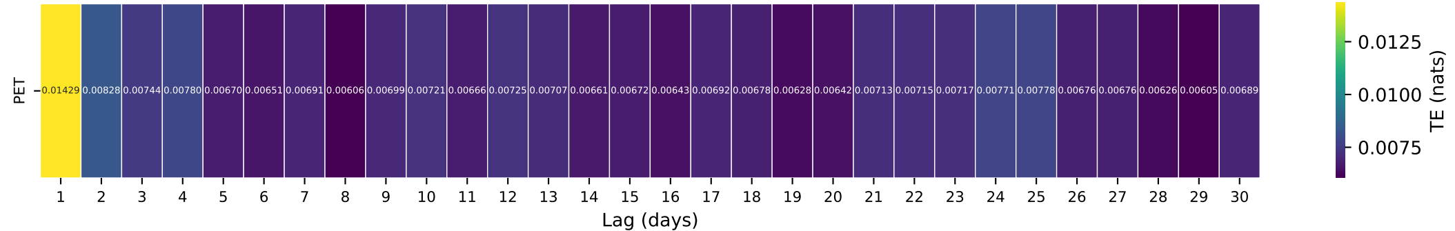
Gauge ID: 06188000 | LAMAR RIVER NR TOWER FALLS RANGER STATION, YNP | PET(t-\tau) \rightarrow Q(t)
