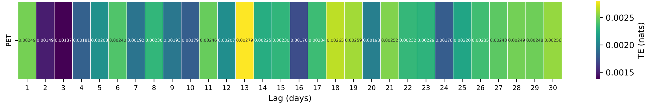
Gauge ID: 05592575 | HICKORY CREEK NEAR BROWNSTOWN, IL | PET(t-\tau) \rightarrow Q(t)
