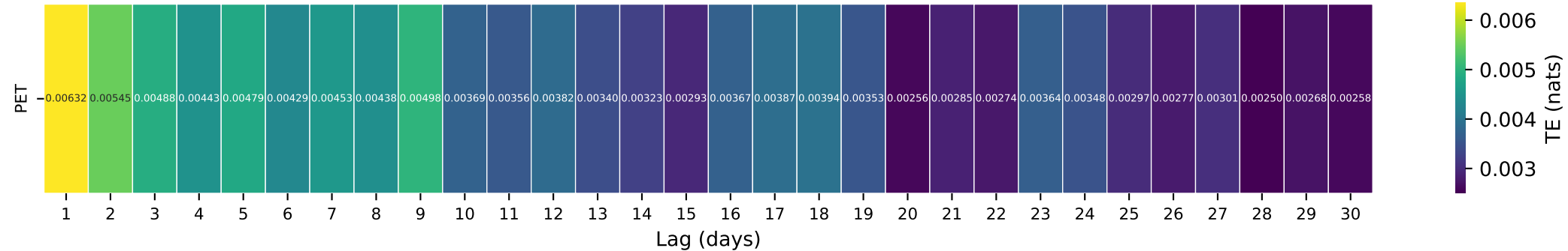
Gauge ID: 05131500 | LITTLE FORK RIVER AT LITTLEFORK, MN | PET(t-\tau) \rightarrow Q(t)
