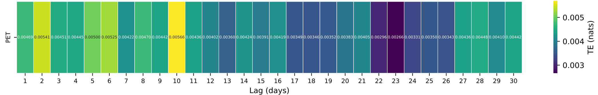
Gauge ID: 12411000 | NF COEUR D ALENE R AB SHOSHONE CK NR PRICHARD ID | PET(t- \tau ) \rightarrow Q(t)
