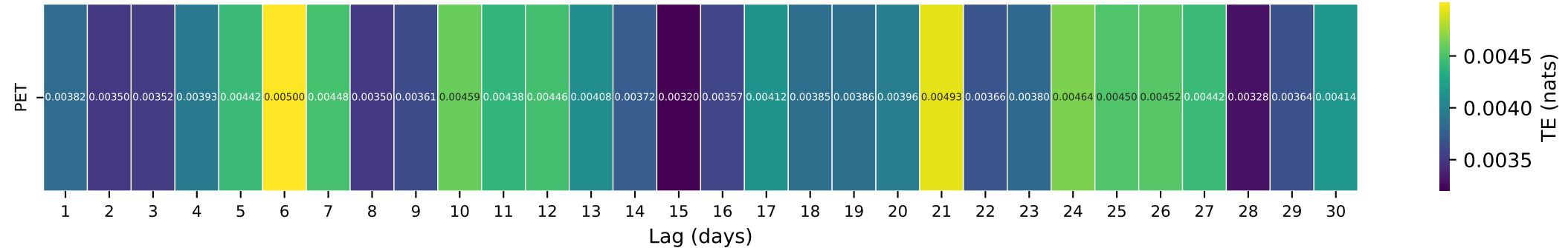
Gauge ID: 10166430 | WEST CANYON CREEK NEAR CEDAR FORT, UT | PET(t-\tau) \rightarrow Q(t)
