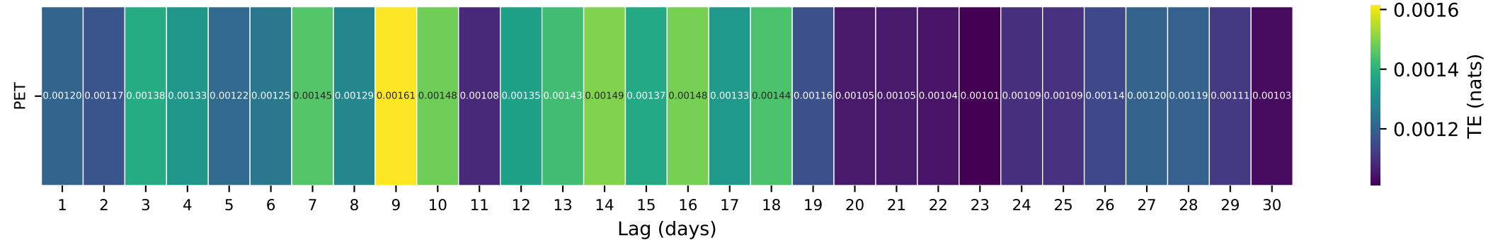
Gauge ID: 10258500 | PALM CYN C NR PALM SPRINGS CA | PET(t- \tau ) \rightarrow Q(t)
