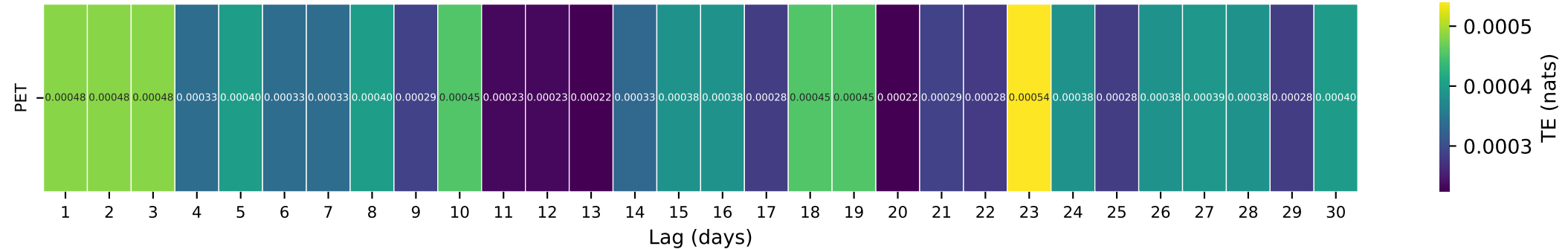
Gauge ID: 02055100 | TINKER CREEK NEAR DALEVILLE, VA | PET(t-\tau) \rightarrow Q(t)
