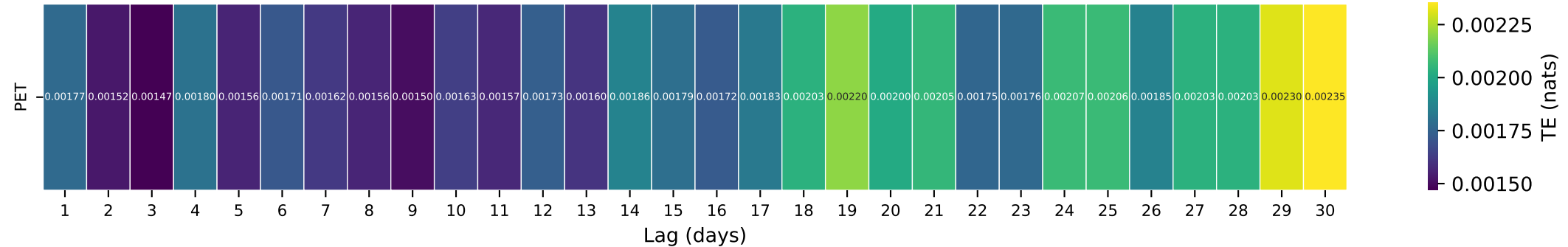
Gauge ID: 11522500 | SALMON R A SOMES BAR CA | PET(t- \tau ) \rightarrow Q(t)
