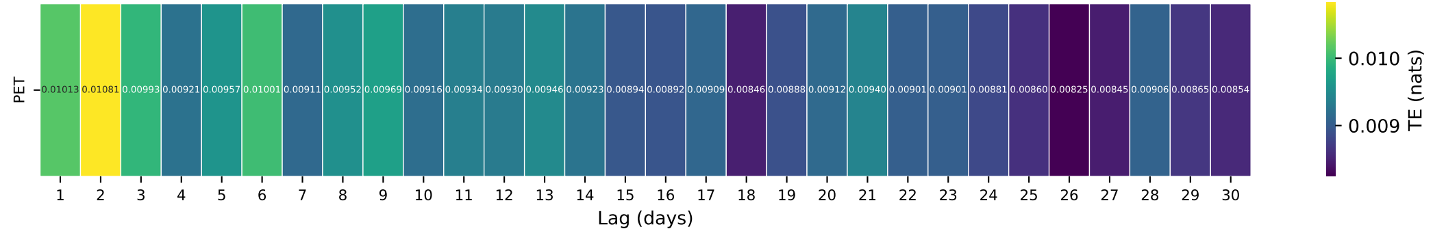
Gauge ID: 12043000 | CALAWAH RIVER NEAR FORKS, WA | PET(t-\tau) \rightarrow Q(t)
