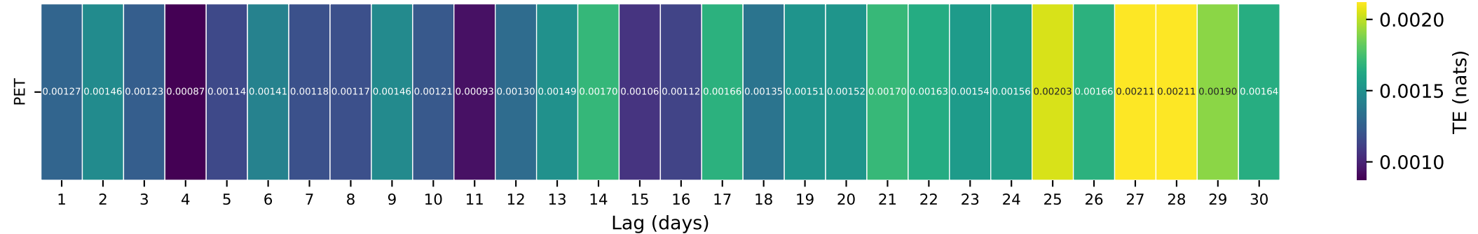
Gauge ID: 03069500 | CHEAT RIVER NEAR PARSONS, WV | PET(t-\tau) \rightarrow Q(t)
