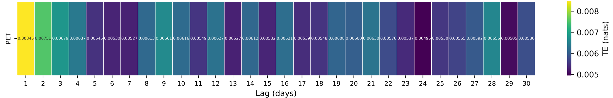
Gauge ID: 06614800 | MICHIGAN RIVER NEAR CAMERON PASS, CO. | PET(t-\tau) \rightarrow Q(t)
