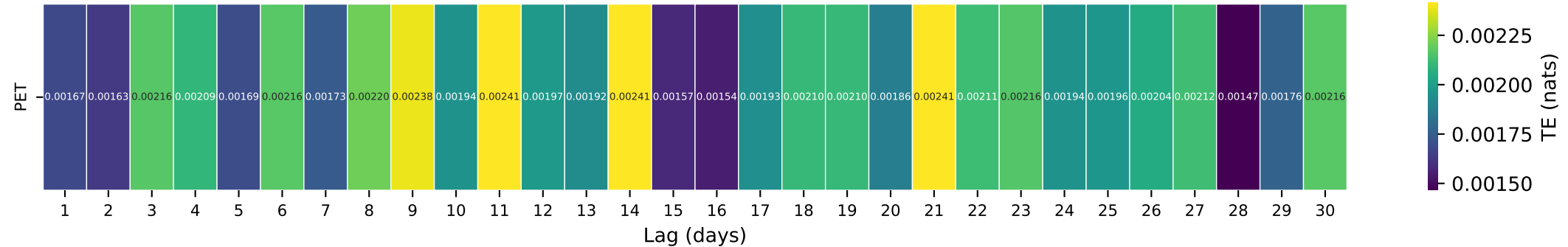
Gauge ID: 03165000 | CHESTNUT CREEK AT GALAX, VA | PET(t-\tau) \rightarrow Q(t)
