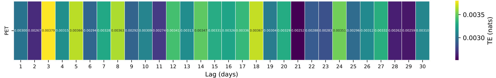
Gauge ID: 06447000 | WHITE R NEAR KADOKA SD | PET(t- \tau ) \rightarrow Q(t)
