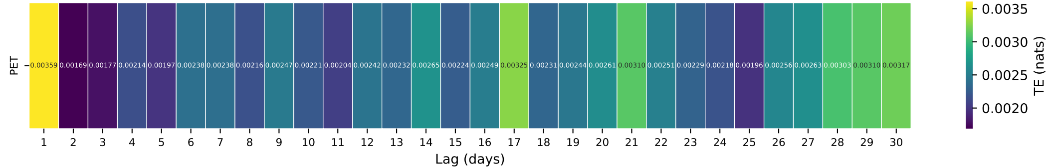
Gauge ID: 01439500 | Bush Kill at Shoemakers, PA | PET(t- \tau ) \rightarrow Q(t)
