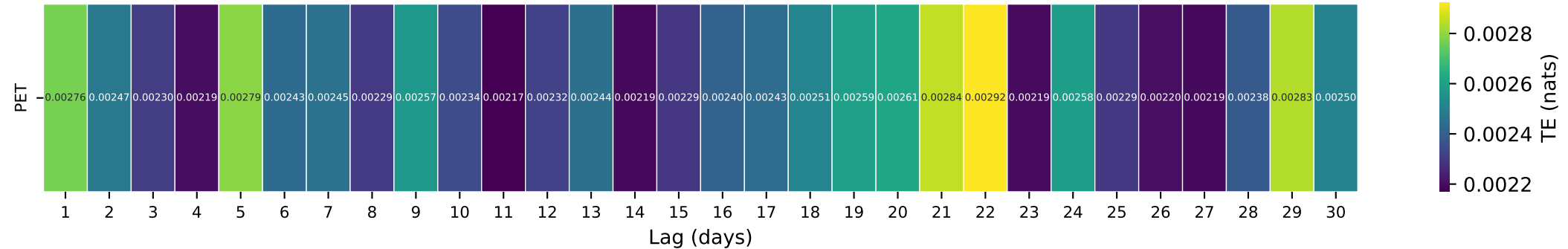
Gauge ID: 01568000 | Sherman Creek at Shermans Dale, PA | PET(t-\tau) \rightarrow Q(t)
