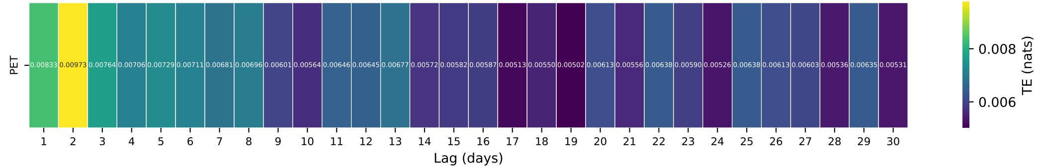
Gauge ID: 12388400 | Revais Cr bl West Fork nr Dixon MT | PET(t- \tau ) \rightarrow Q(t)
