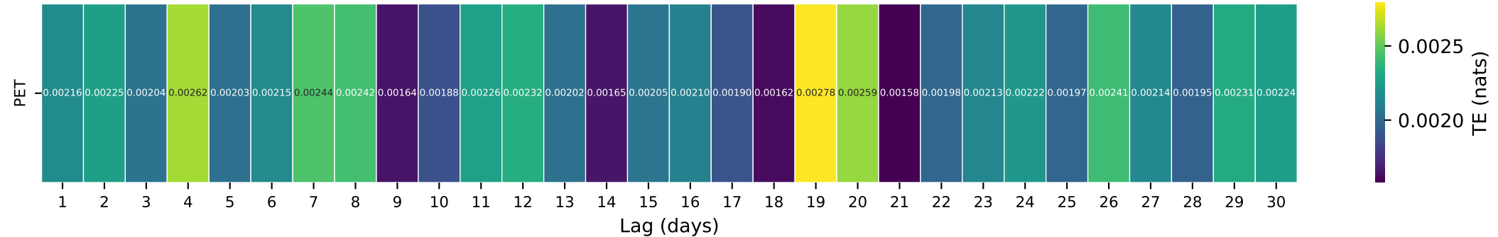
Gauge ID: 01170100 | GREEN RIVER NEAR COLRAIN, MA | PET(t- \tau ) \rightarrow Q(t)
