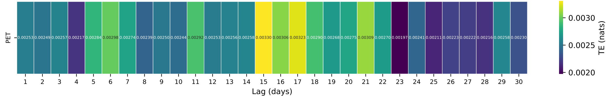
Gauge ID: 04024430 | NEMADJI RIVER NEAR SOUTH SUPERIOR, WI | PET(t-\tau) \rightarrow Q(t)
