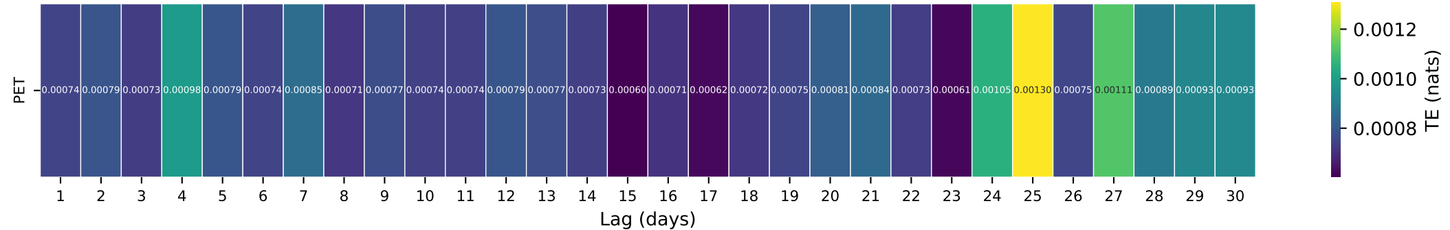
Gauge ID: 03592718 | LITTLE YELLOW CREEK EAST NR BURNSVILLE, MS | PET(t-\tau) \rightarrow Q(t)
