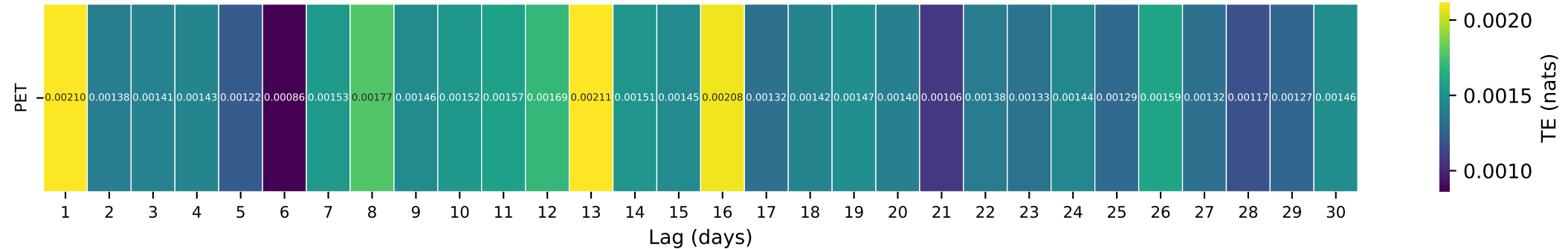
Gauge ID: 01440400 | Brodhead Creek near Analomink, PA | PET(t- \tau ) \rightarrow Q(t)
