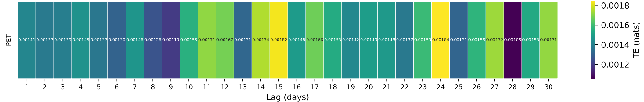
Gauge ID: 07071500 | Eleven Point River near Bardley, MO | PET(t-\tau) \rightarrow Q(t)
