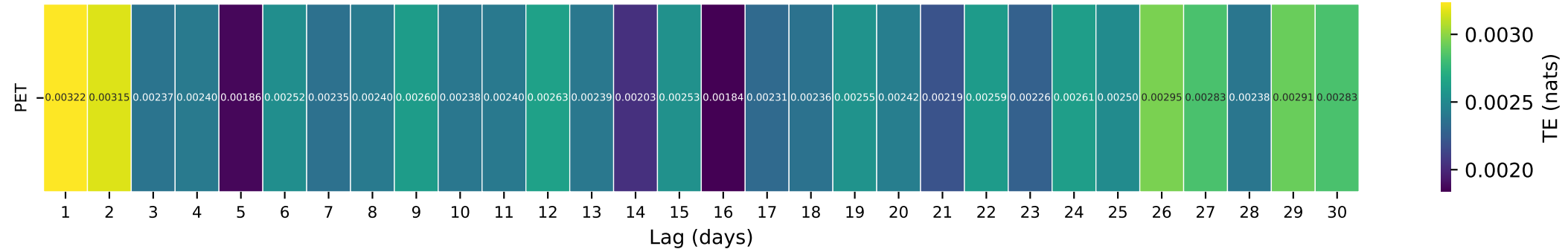
Gauge ID: 04185000 | Tiffin River at Stryker OH | PET(t-\tau) \rightarrow Q(t)
