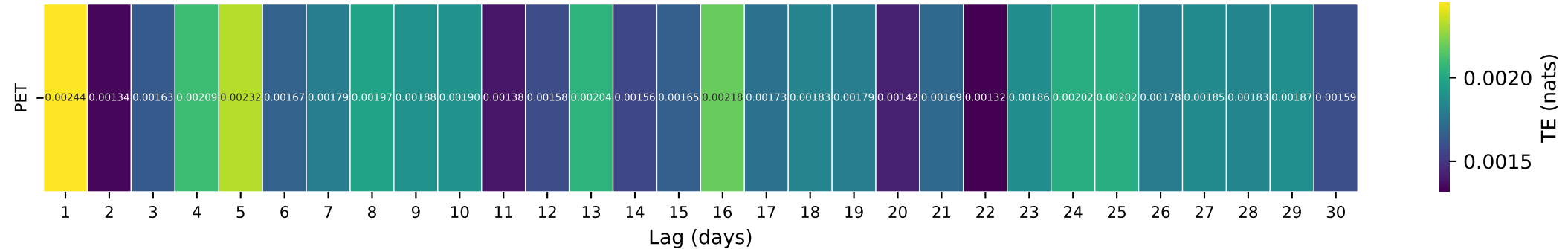
Gauge ID: 01073000 | OYSTER RIVER NEAR DURHAM, NH | PET(t-\tau) \rightarrow Q(t)
