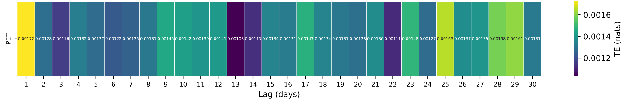
Gauge ID: 07359610 | Caddo River near Caddo Gap, AR | PET(t-\tau) \rightarrow Q(t)
