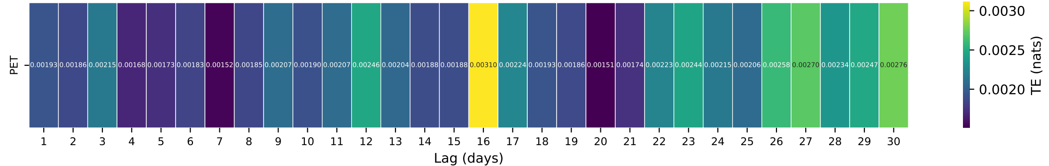
Gauge ID: 03368000 | BRUSH CREEK NEAR NEBRASKA, IN | PET(t-\tau) \rightarrow Q(t)
