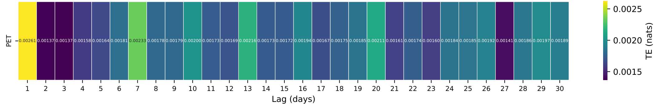
Gauge ID: 01580000 | DEER CREEK AT ROCKS, MD | PET(t-\tau) \rightarrow Q(t)
