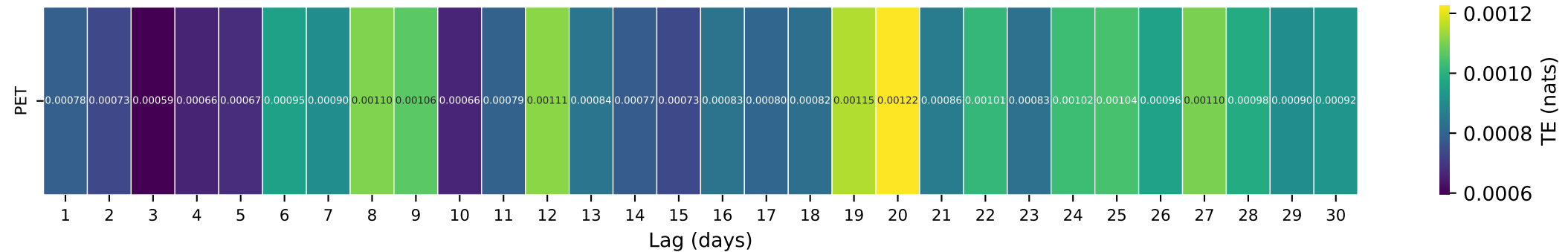
Gauge ID: 08079600 | DMF Brazos Rv at Justiceburg, TX | PET(t-\tau) \rightarrow Q(t)
