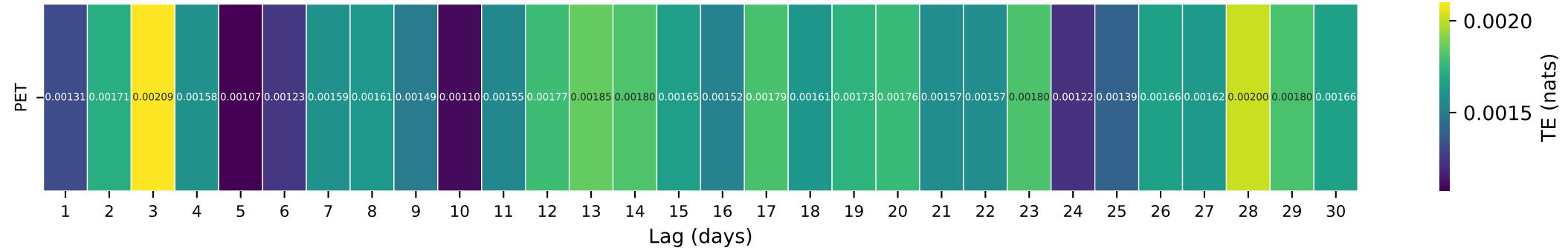
Gauge ID: 01516500 | Corey Creek near Mainesburg, PA | PET(t-\tau) \rightarrow Q(t)
