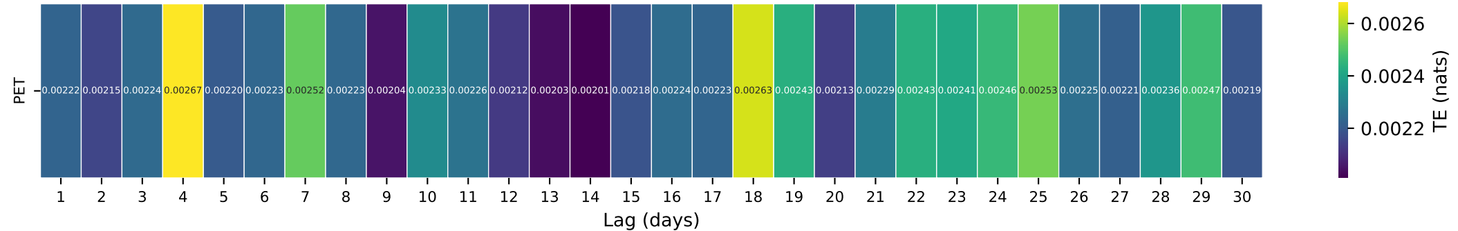
Gauge ID: 05444000 | ELKHORN CREEK NEAR PENROSE, IL | PET(t- \tau ) \rightarrow Q(t)
