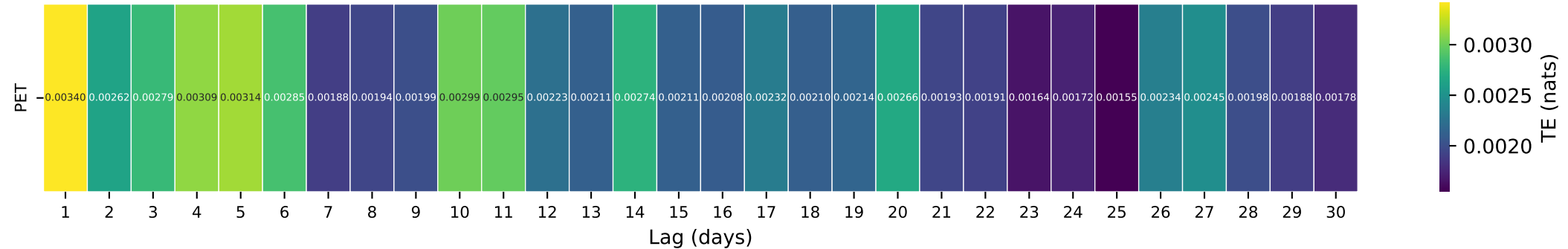
Gauge ID: 10172700 | VERNON CREEK NEAR VERNON, UT | PET(t-\tau) \rightarrow Q(t)
