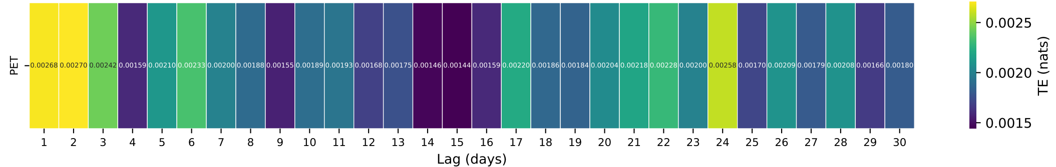
Gauge ID: 06360500 | MOREAU R NEAR WHITEHORSE SD | PET(t- \tau ) \rightarrow Q(t)
