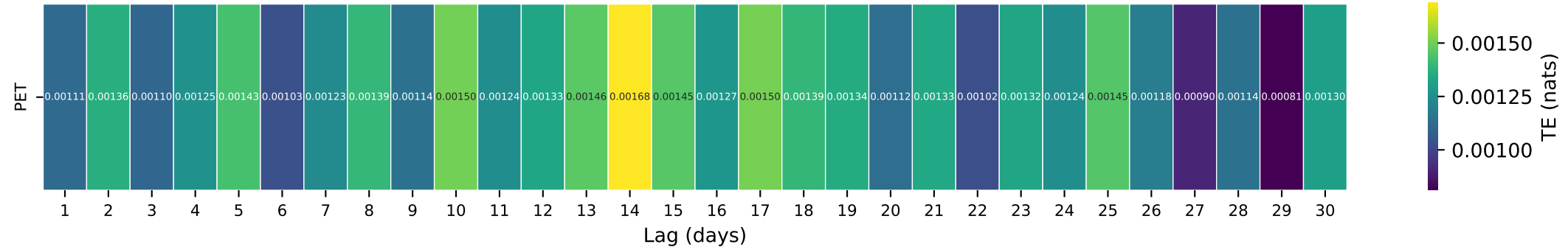
Gauge ID: 01666500 | ROBINSON RIVER NEAR LOCUST DALE, VA | PET(t-\tau) \rightarrow Q(t)
