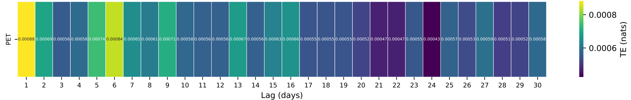
Gauge ID: 08150800 | Beaver Ck nr Mason, TX | PET(t- \tau ) \rightarrow Q(t)
