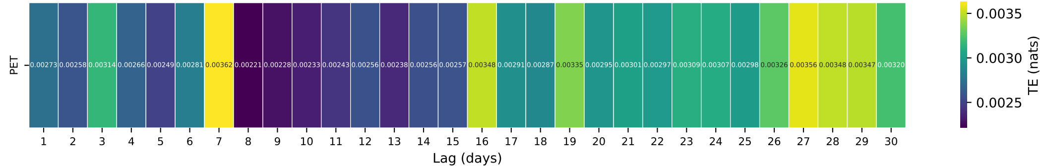
Gauge ID: 04161580 | STONY CREEK NEAR ROMEO, MI | PET(t-\tau) \rightarrow Q(t)
