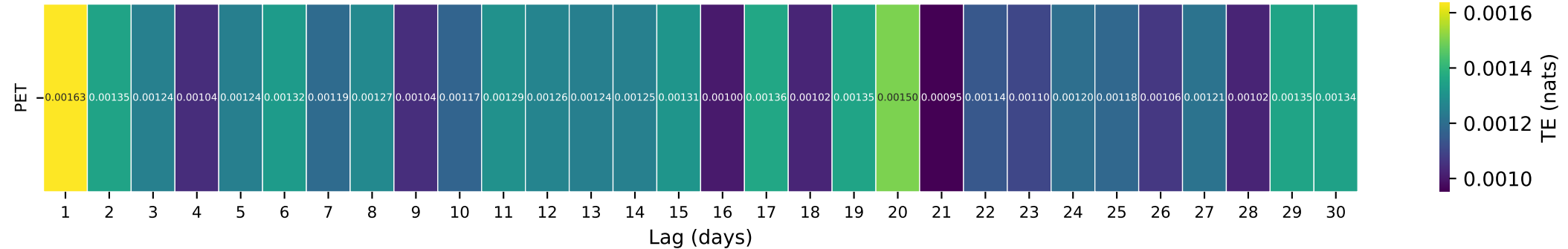
Gauge ID: 01583500 | WESTERN RUN AT WESTERN RUN, MD | PET(t-\tau) \rightarrow Q(t)
