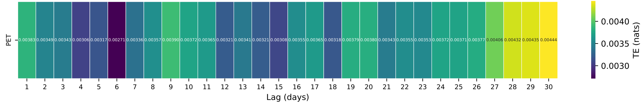
Gauge ID: 04216418 | TONAWANDA CREEK AT ATTICA NY | PET(t-\tau) \rightarrow Q(t)
