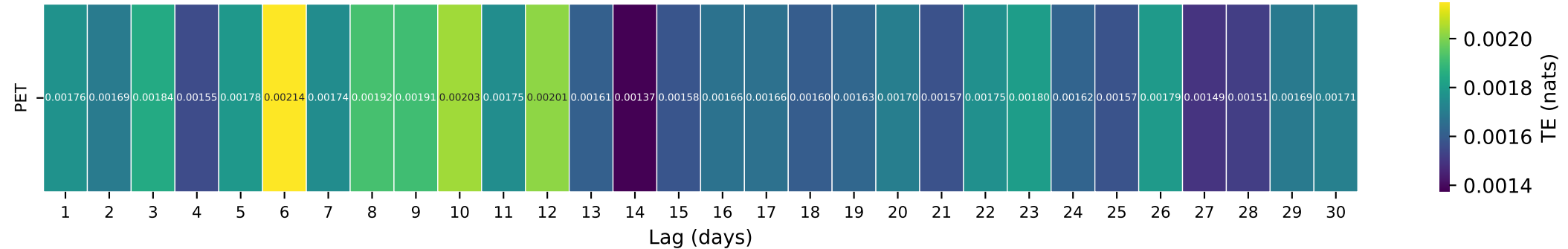
Gauge ID: 05413500 | GRANT RIVER AT BURTON, WI | PET(t-\tau) \rightarrow Q(t)
