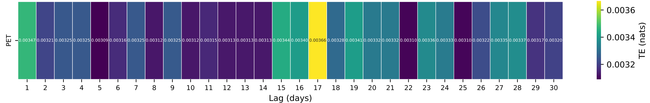
Gauge ID: 14137000 | SANDY RIVER NEAR MARMOT, OR | PET(t-\tau) \rightarrow Q(t)
