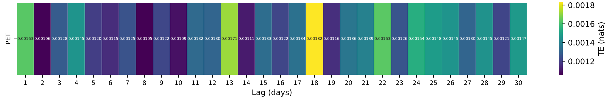
Gauge ID: 03028000 | West Branch Clarion River at Wilcox, PA | PET(t-\tau) \rightarrow Q(t)
