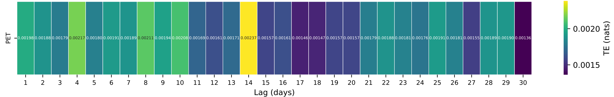
Gauge ID: 05489000 | Cedar Creek near Bussey, IA | PET(t- \tau ) \rightarrow Q(t)
