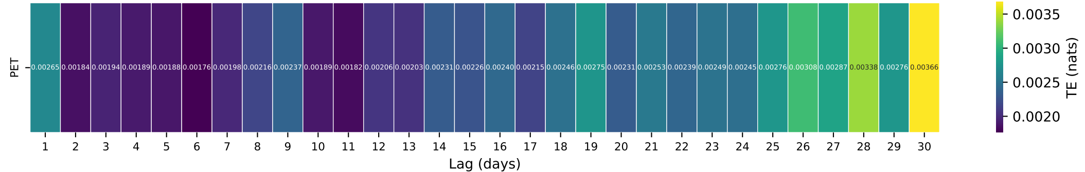
Gauge ID: 03281100 | GOOSE CREEK AT MANCHESTER, KY | PET(t-\tau) \rightarrow Q(t)
