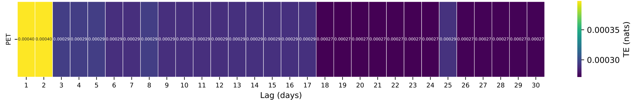
Gauge ID: 09447800 | BONITA CREEK NEAR MORENCI, AZ. | PET(t-\tau) \rightarrow Q(t)
