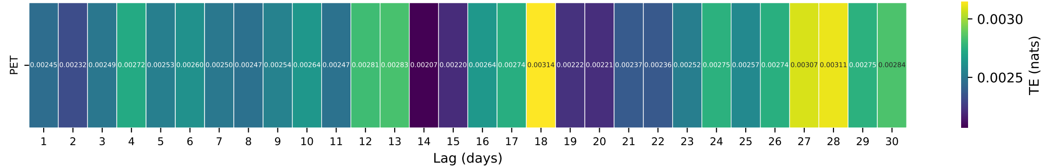
Gauge ID: 03241500 | Massies Creek at Wilberforce OH | PET(t- \tau ) \rightarrow Q(t)
