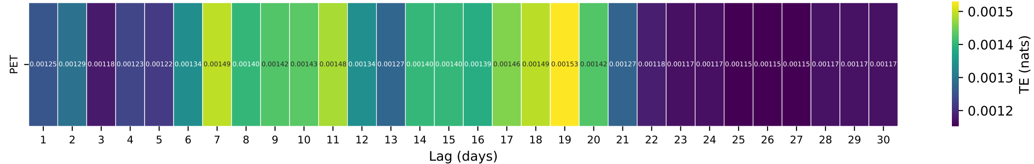
Gauge ID: 10259200 | DEEP C NR PALM DESERT CA | PET( t-\tau ) \rightarrow Q( t )
