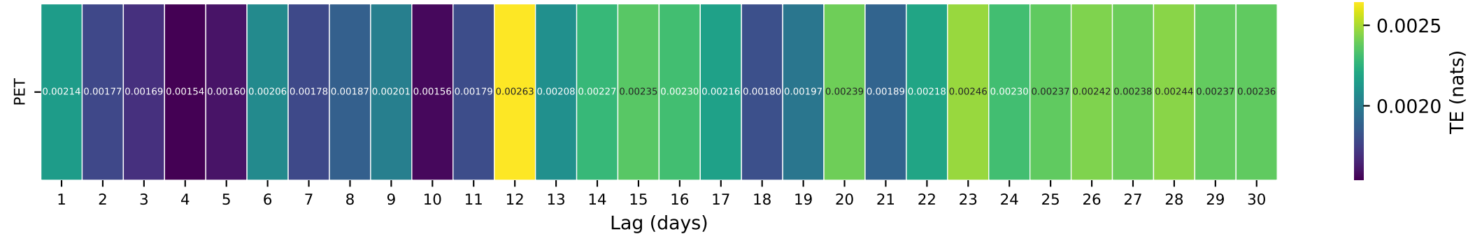
Gauge ID: 01486000 | MANOKIN BRANCH NEAR PRINCESS ANNE, MD | PET(t-\tau) \rightarrow Q(t)
