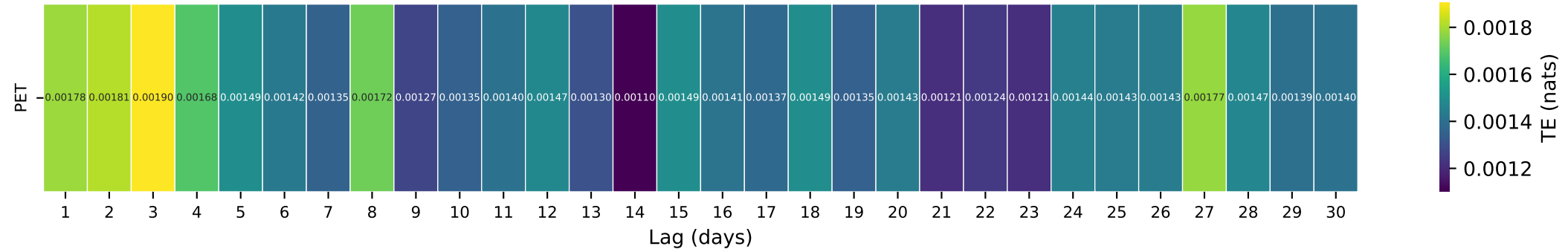
Gauge ID: 03173000 | WALKER CREEK AT BANE, VA | PET(t-\tau) \rightarrow Q(t)
