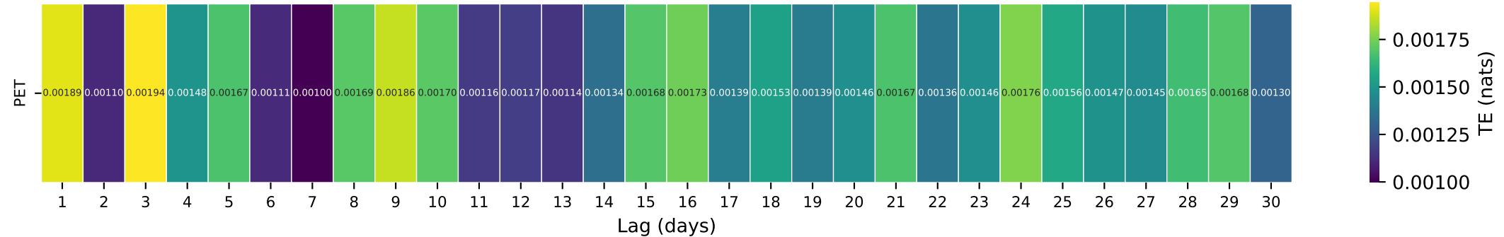
Gauge ID: 02056900 | BLACKWATER RIVER NEAR ROCKY MOUNT, VA | PET(t-\tau) \rightarrow Q(t)
