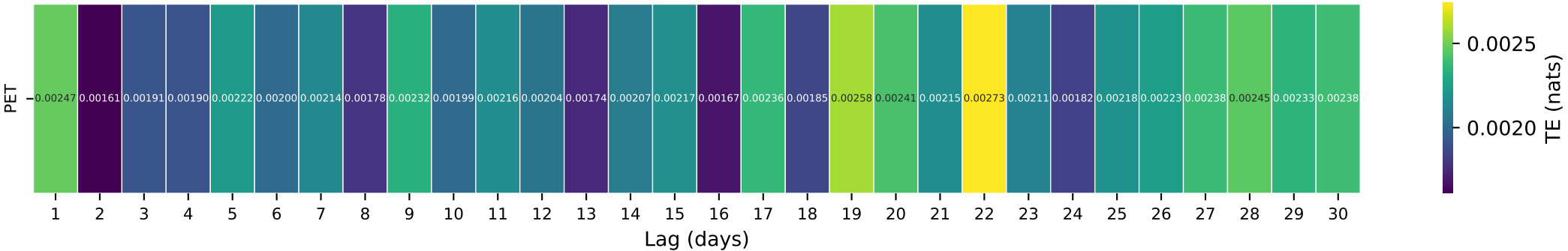
Gauge ID: 06919500 | Cedar Creek near Pleasant View, MO | PET(t-\tau) \rightarrow Q(t)
