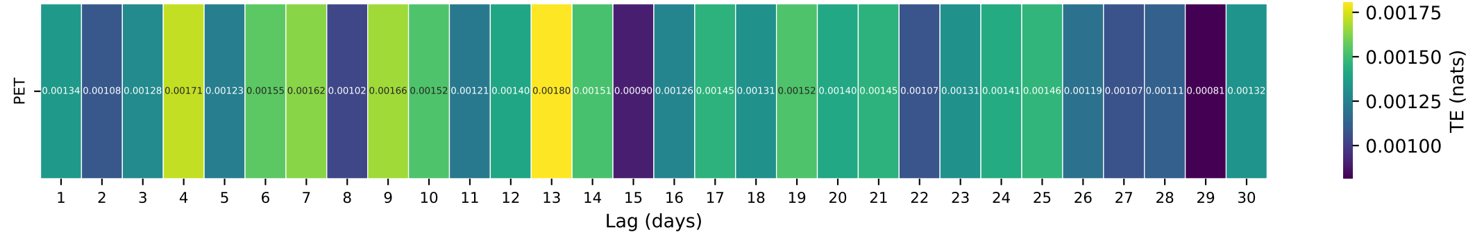
Gauge ID: 01552000 | Loyalsock Creek at Loyalsockville, PA | PET(t-\tau) \rightarrow Q(t)
