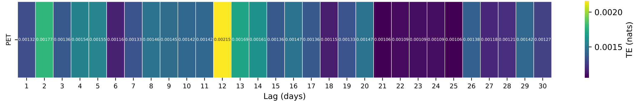
Gauge ID: 05062500 | WILD RICE RIVER AT TWIN VALLEY, MN | PET(t-\tau) \rightarrow Q(t)
