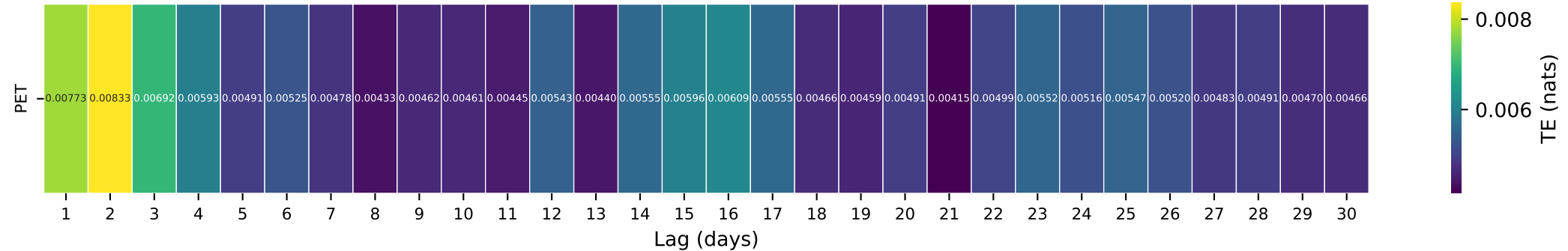
Gauge ID: 06043500 | Gallatin River near Gallatin Gateway MT | PET(t- \tau ) \rightarrow Q(t)
