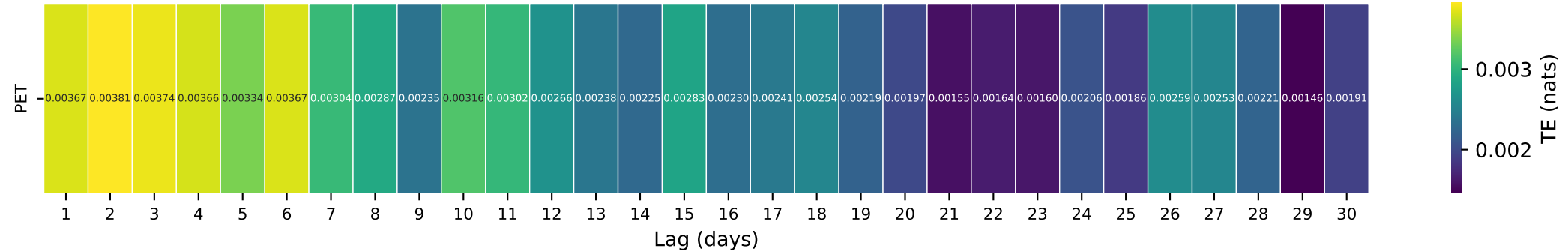
Gauge ID: 12374250 | Mill Cr ab Bassoo Cr nr Niarada MT | PET(t- \tau ) \rightarrow Q(t)
