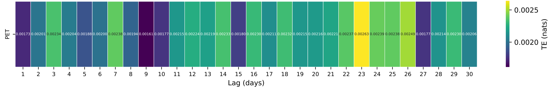
Gauge ID: 05593575 | LITTLE CROOKED CREEK NEAR NEW MINDEN, IL | PET(t-\tau) \rightarrow Q(t)
