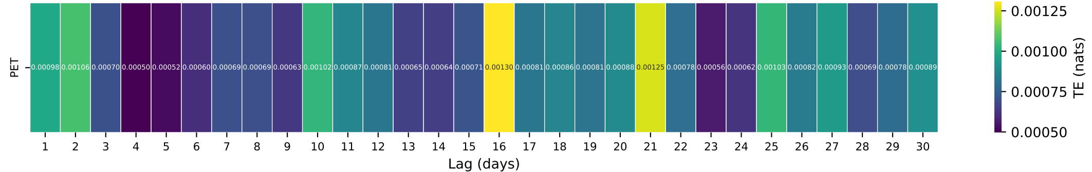
Gauge ID: 02011400 | JACKSON RIVER NEAR BACOVA, VA | PET(t-\tau) \rightarrow Q(t)
