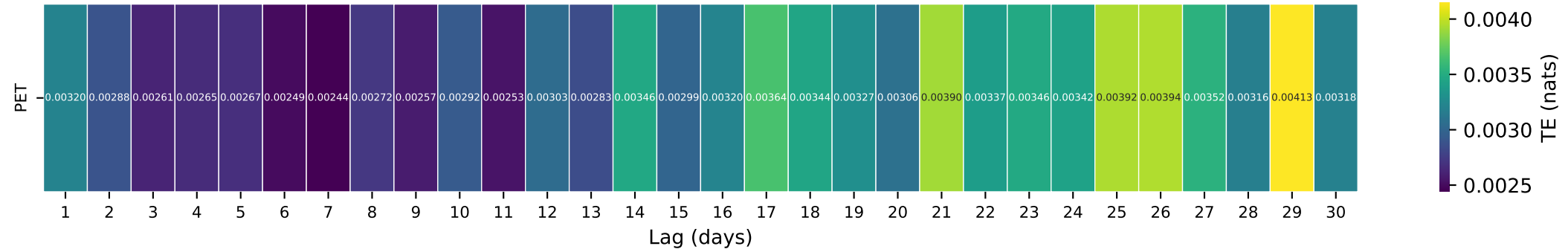
Gauge ID: 04197100 | Honey Creek at Melmore OH | PET( t-\tau ) \rightarrow Q( t )
