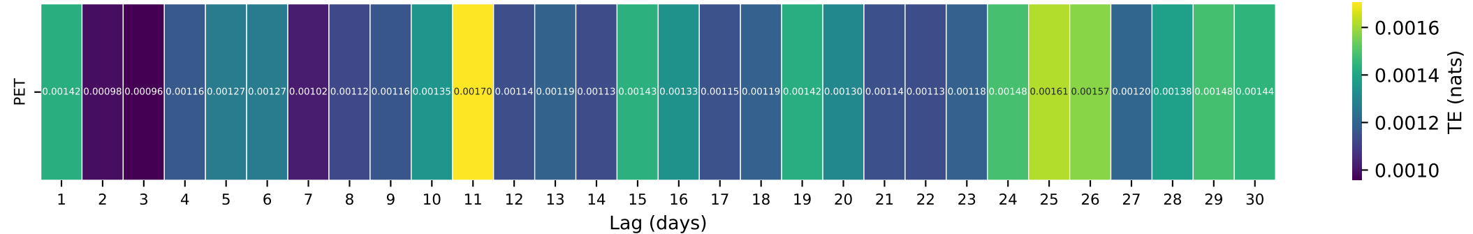
Gauge ID: 02143000 | HENRY FORK NEAR HENRY RIVER, NC | PET(t-\tau) \rightarrow Q(t)
