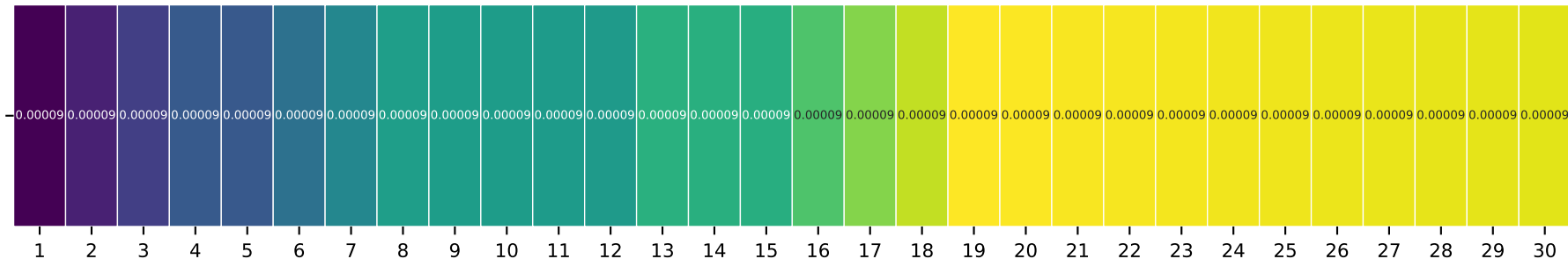
Gauge ID: 10348850 | GALENA C AT GALENA C STATE PARK | PET(t-\tau) \rightarrow Q(t)
