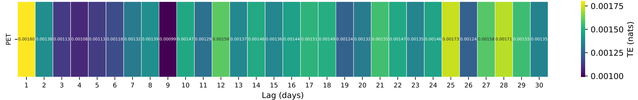
Gauge ID: 02479155 | CYPRESS CREEK NR JANICE, MS | PET(t- \tau ) \rightarrow Q(t)
