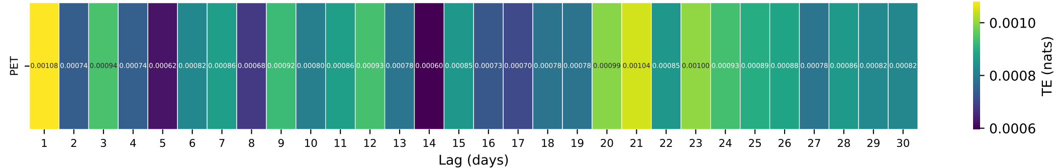
Gauge ID: 02149000 | COVE CREEK NEAR LAKE LURE, NC | PET(t-\tau) \rightarrow Q(t)
