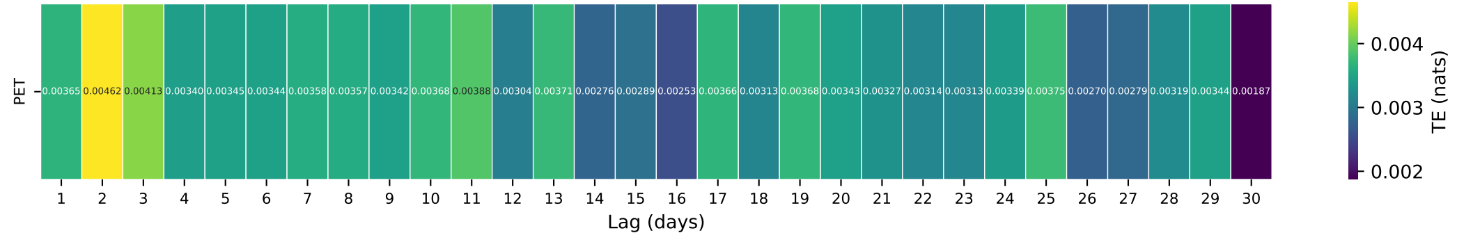
Gauge ID: 08378500 | PECOS RIVER NEAR PECOS, NM | PET(t- \tau ) \rightarrow Q(t)
