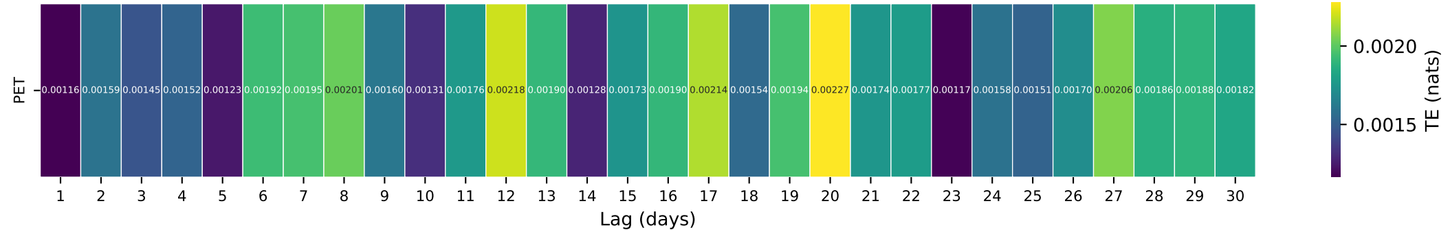
Gauge ID: 01169000 | NORTH RIVER AT SHATTUCKVILLE, MA | PET(t-\tau) \rightarrow Q(t)
