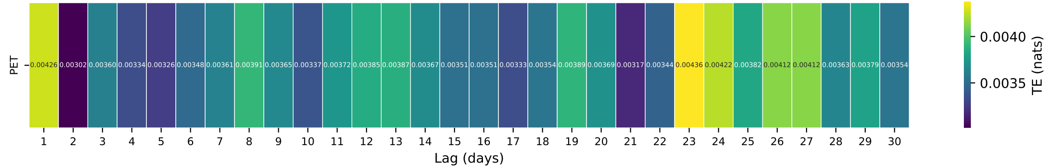
Gauge ID: 04213000 | Conneaut Creek at Conneaut OH | PET(t- \tau ) \rightarrow Q(t)
