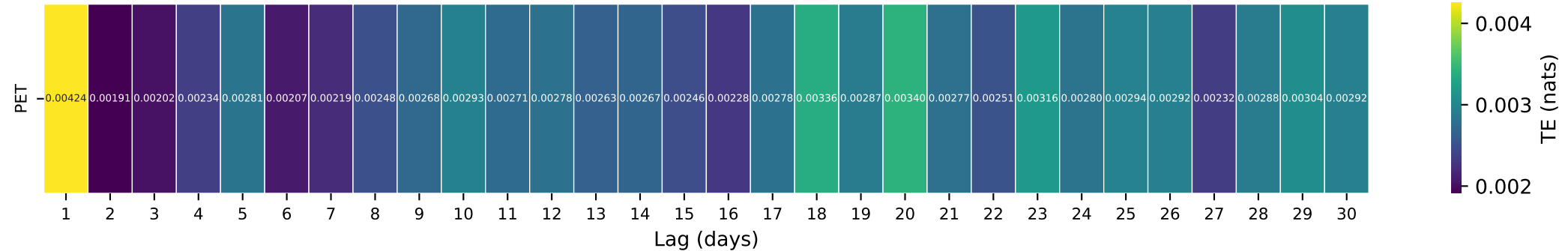
Gauge ID: 04105700 | AUGUSTA CREEK NEAR AUGUSTA, MI | PET(t-\tau) \rightarrow Q(t)
