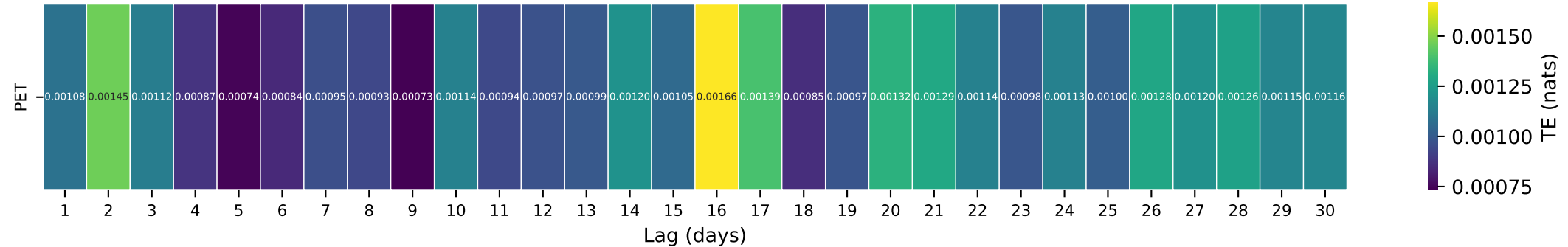
Gauge ID: 02015700 | BULLPASTURE RIVER AT WILLIAMSVILLE, VA | PET(t-\tau) \rightarrow Q(t)
