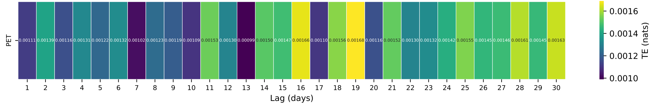
Gauge ID: 03479000 | WATAUGA RIVER NEAR SUGAR GROVE, NC | PET(t-\tau) \rightarrow Q(t)
