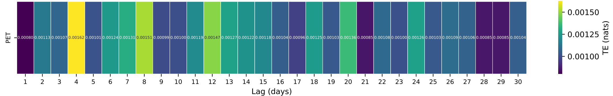
Gauge ID: 01181000 | WEST BRANCH WESTFIELD RIVER AT HUNTINGTON, MA | PET(t-\tau) \rightarrow Q(t)
