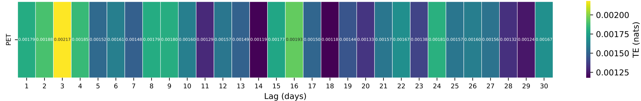
Gauge ID: 08066300 | Menard Ck nr Rye, TX | PET(t- \tau ) \rightarrow Q(t)
