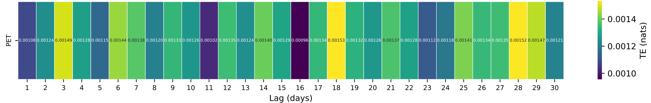
Gauge ID: 02074500 | SANDY RIVER NEAR DANVILLE, VA | PET(t-\tau) \rightarrow Q(t)
