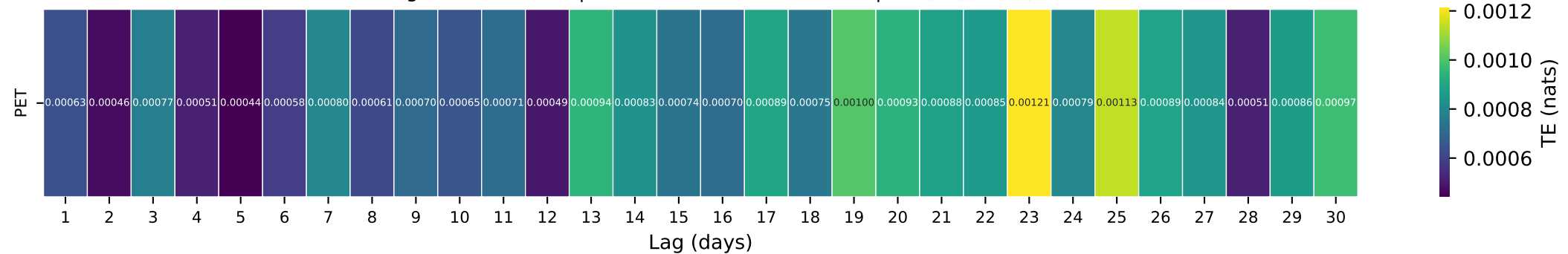
Gauge ID: 02111180 | ELK CREEK AT ELKVILLE, NC | PET(t-\tau) \rightarrow Q(t)
