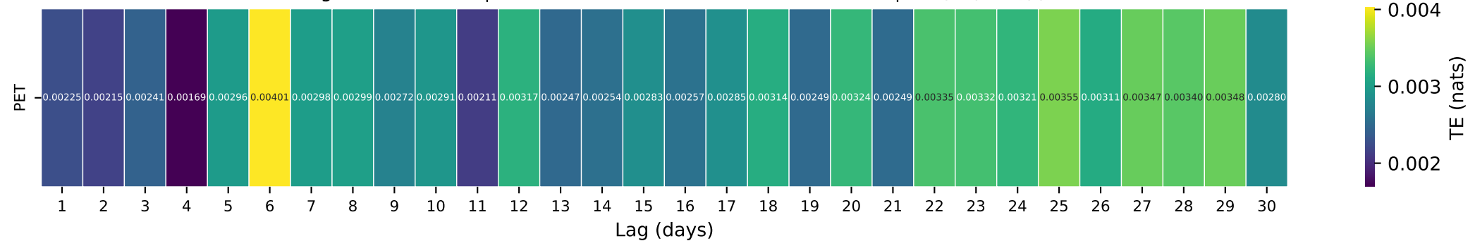
Gauge ID: 01594950 | MCMILLAN F NEAR FORT PENDLETON, MD | PET(t- \tau ) \rightarrow Q(t)
