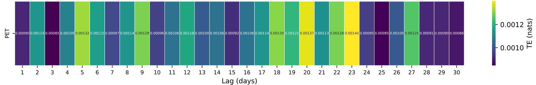
Gauge ID: 07184000 | LIGHTNING C NR MCCUNE, KS | PET(t- \tau ) \rightarrow Q(t)
