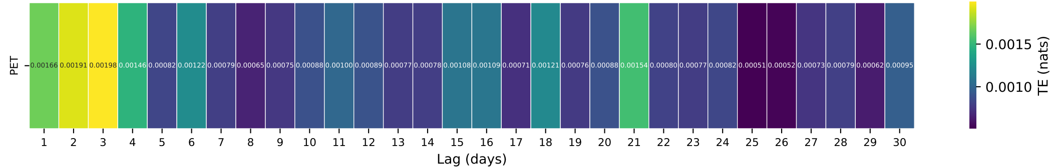
Gauge ID: 06479438 | BIG SIOUX R NEAR WATERTOWN SD | PET( t-\tau ) \rightarrow Q( t )
