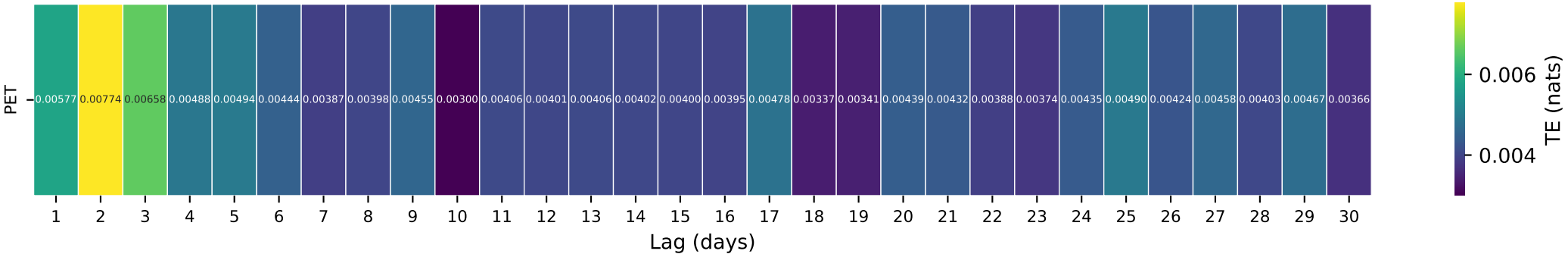
Gauge ID: 12381400 | South Fork Jocko River near Arlee MT | PET(t-τ) → Q(t)
