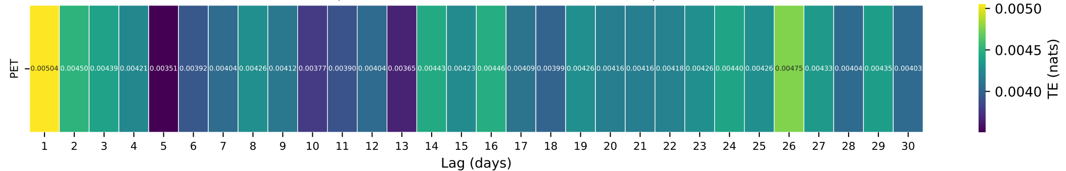
Gauge ID: 12144000 | SF SNOQUALMIE RIVER AT NORTH BEND, WA | PET(t-\tau) \rightarrow Q(t)
