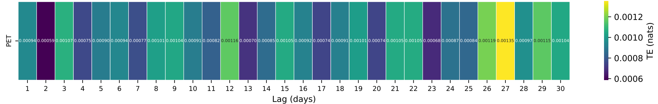
Gauge ID: 01484100 | BEAVERDAM BRANCH AT HOUSTON, DE | PET(t-\tau) \rightarrow Q(t)
