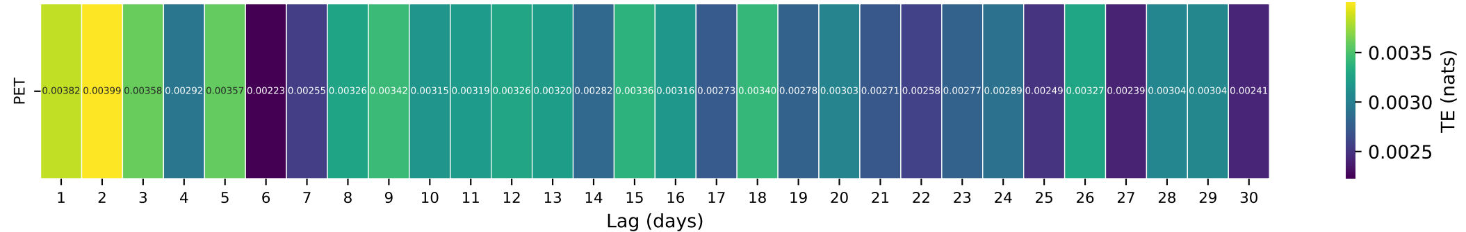
Gauge ID: 08377900 | RIO MORA NEAR TERRERO, NM | PET(t-\tau) \rightarrow Q(t)
