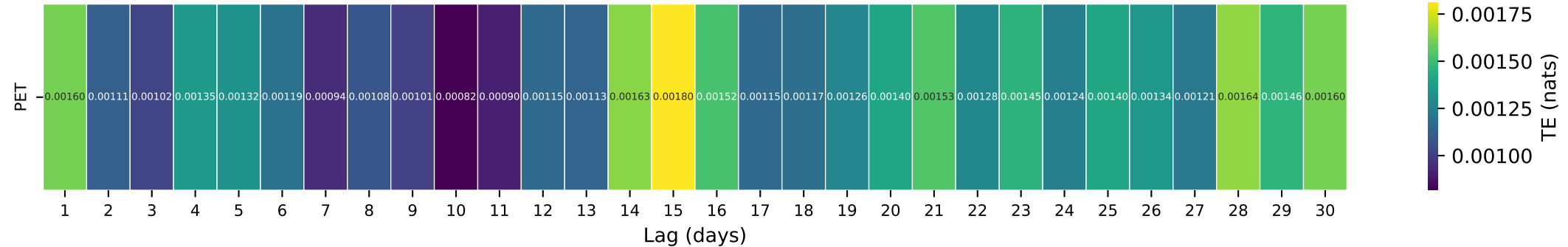
Gauge ID: 02422500 | MULBERRY CREEK AT JONES AL | PET(t- \tau ) \rightarrow Q(t)
