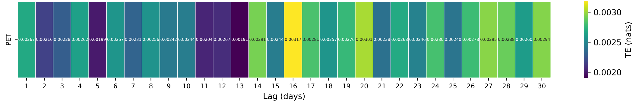
Gauge ID: 03473000 | S F HOLSTON RIVER NEAR DAMASCUS, VA | PET(t-\tau) \rightarrow Q(t)
