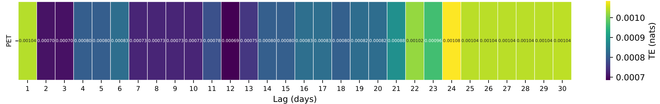
Gauge ID: 09513780 | NEW RIVER NEAR ROCK SPRINGS, AZ. | PET(t-\tau) \rightarrow Q(t)
