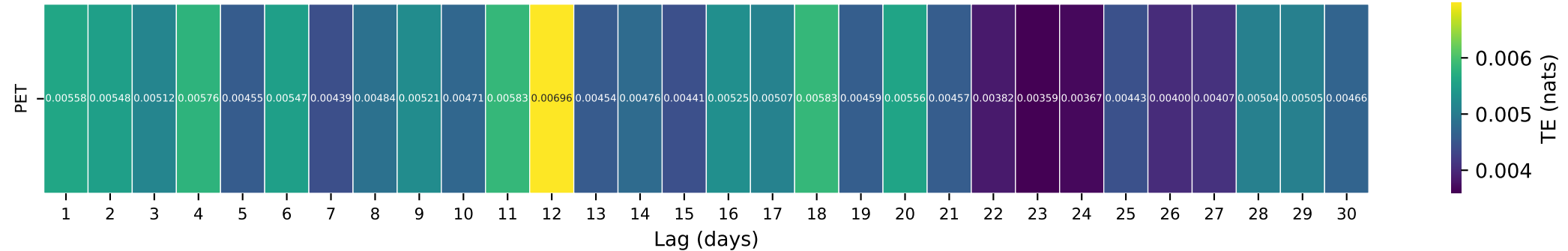
Gauge ID: 01139800 | EAST ORANGE BRANCH AT EAST ORANGE, VT | PET(t-\tau) \rightarrow Q(t)
