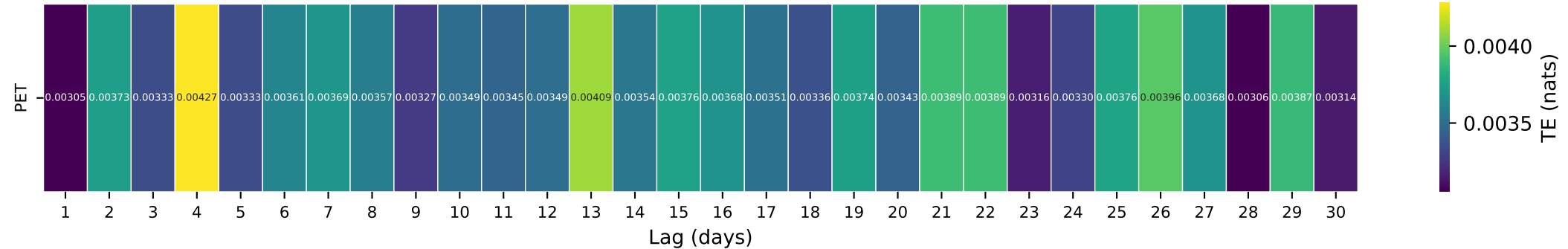
Gauge ID: 06885500 | BLACK VERMILLION R NR FRANKFORT, KS | PET(t- \tau ) \rightarrow Q(t)
