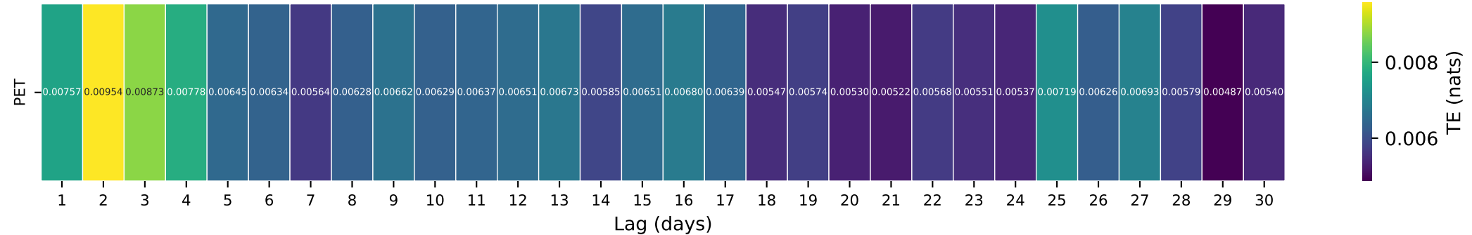
Gauge ID: 06037500 | Madison River near West Yellowstone MT | PET(t-\tau) \rightarrow Q(t)
