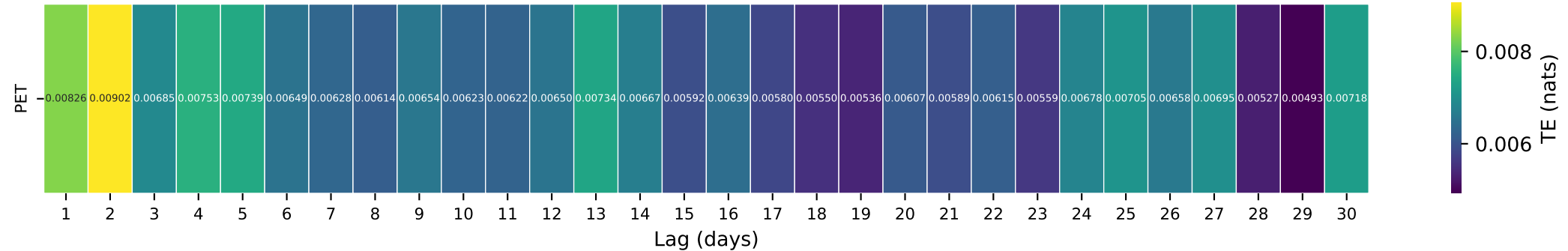
Gauge ID: 13310700 | SF SALMON RIVER NR KRASSEL RANGER STATION ID | PET(t-\tau) \rightarrow Q(t)
