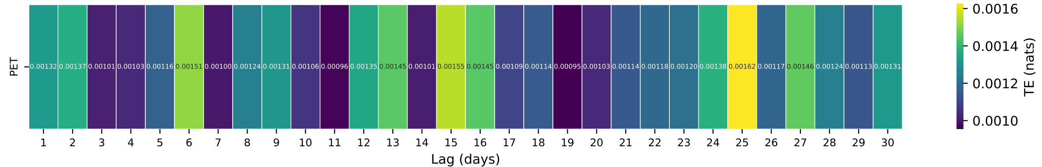
Gauge ID: 04233000 | CAYUGA INLET NEAR ITHACA NY | PET(t- \tau ) \rightarrow Q(t)
