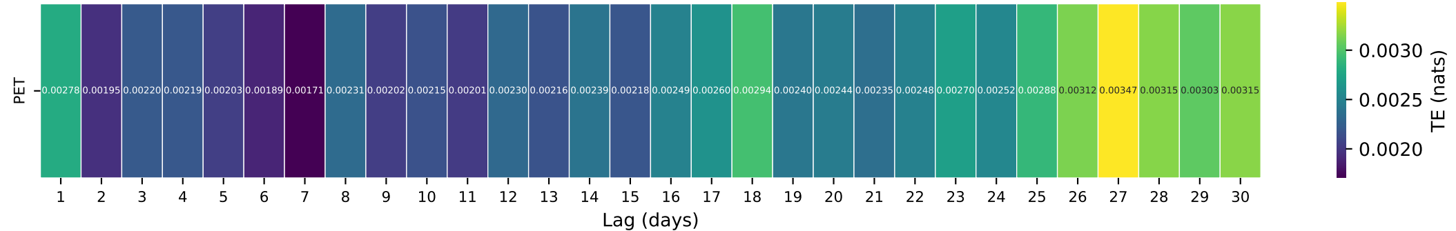
Gauge ID: 03281500 | SOUTH FORK KENTUCKY RIVER AT BOONEVILLE, KY | PET(t-\tau) \rightarrow Q(t)
