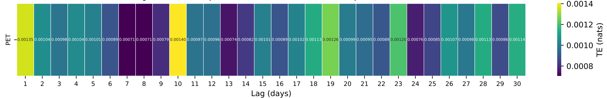
Gauge ID: 06344600 | GREEN RIVER NR NEW HRADEC, ND | PET(t- \tau ) \rightarrow Q(t)
