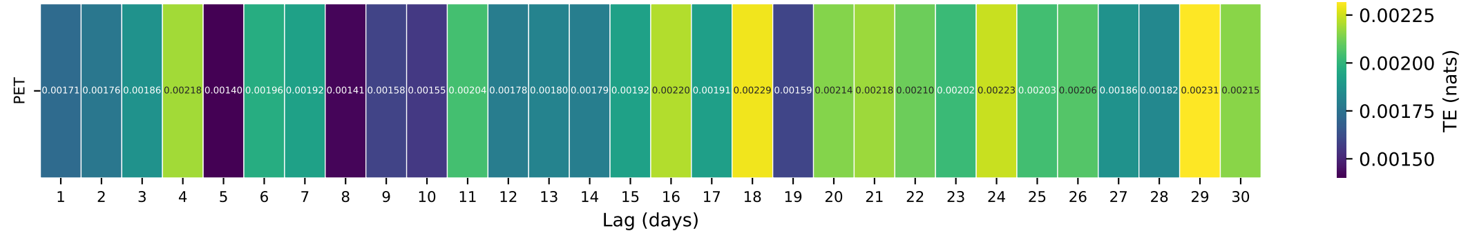
Gauge ID: 01414500 | MILL BROOK NEAR DUNRAVEN NY | PET(t-\tau) \rightarrow Q(t)
