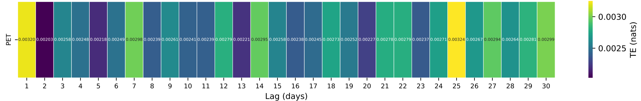
Gauge ID: 03213700 | TUG FORK AT WILLIAMSON, WV | PET(t-\tau) \rightarrow Q(t)
