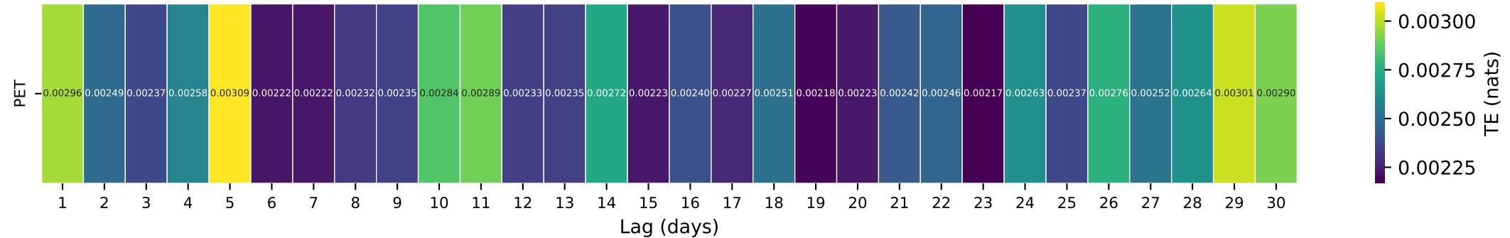
Gauge ID: 03170000 | LITTLE RIVER AT GRAYSONTOWN, VA | PET(t-\tau) \rightarrow Q(t)
