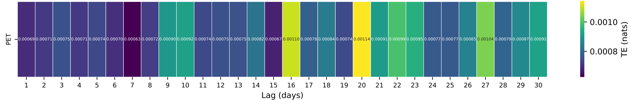
Gauge ID: 01667500 | RAPIDAN RIVER NEAR CULPEPER, VA | PET(t-\tau) \rightarrow Q(t)
