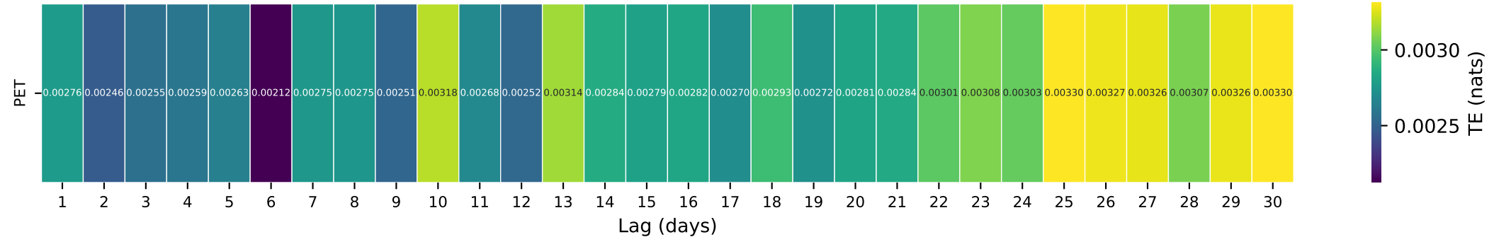
Gauge ID: 11176400 | ARROYO VALLE BL LANG CN NR LIVERMORE CA | PET(t- \tau ) \rightarrow Q(t)
