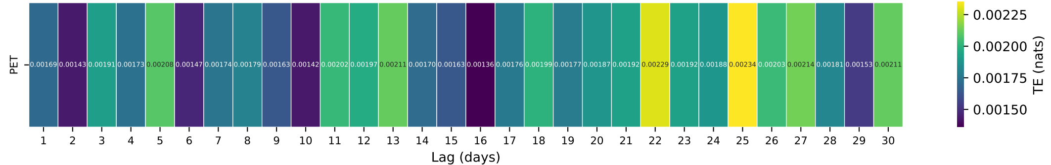
Gauge ID: 07196900 | Baron Fork at Dutch Mills, AR | PET(t-\tau) \rightarrow Q(t)
