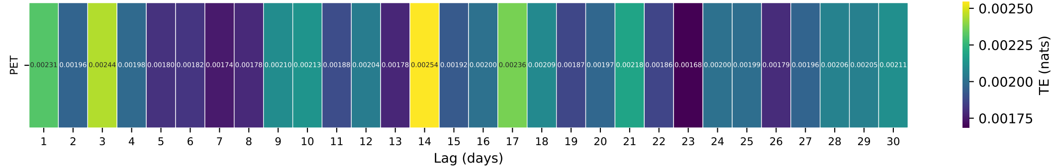
Gauge ID: 07335700 | Kiamichi River near Big Cedar, OK | PET(t-\tau) \rightarrow Q(t)
