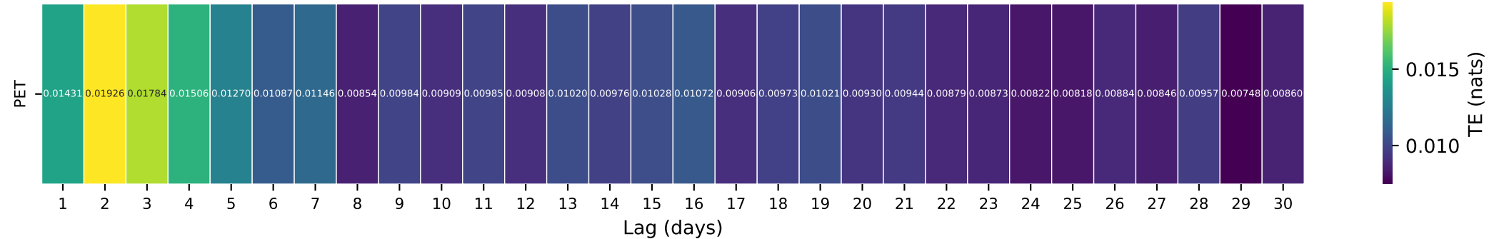
Gauge ID: 06224000 | BULL LAKE CREEK ABOVE BULL LAKE, WY | PET(t-\tau) \rightarrow Q(t)
