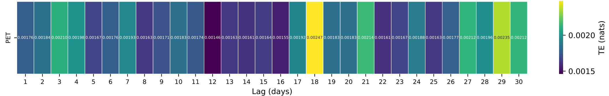
Gauge ID: 06921200 | Lindley Creek near Polk, MO | PET(t-\tau) \rightarrow Q(t)
