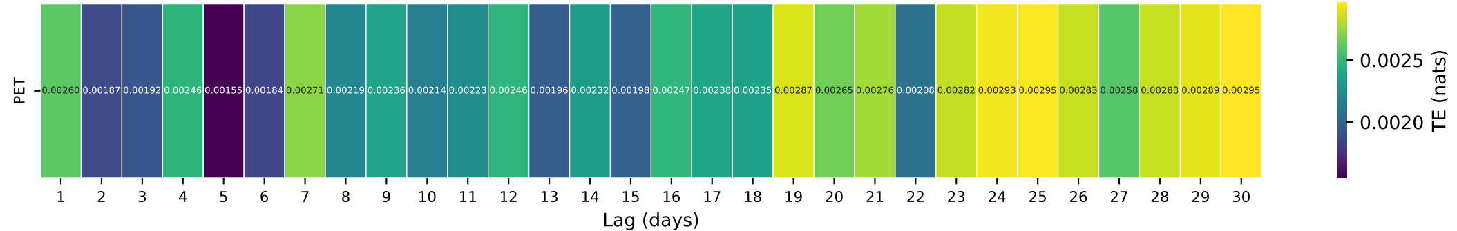
Gauge ID: 03187500 | CRANBERRY RIVER NEAR RICHWOOD, WV | PET(t-\tau) \rightarrow Q(t)
