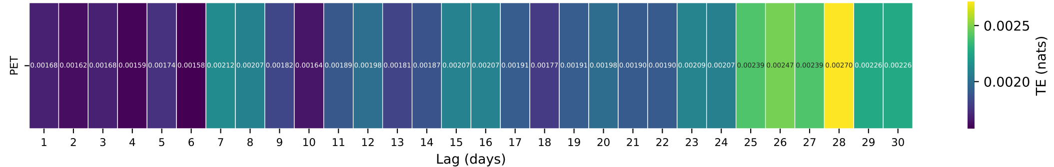
Gauge ID: 12095000 | SOUTH PRAIRIE CREEK AT SOUTH PRAIRIE, WA | PET(t-\tau) \rightarrow Q(t)
