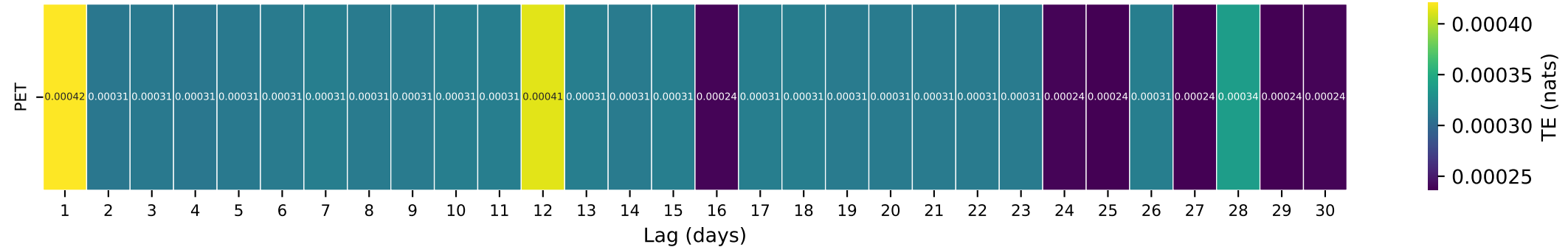
Gauge ID: 05408000 | KICKAPOO RIVER AT LA FARGE, WI | PET(t-\tau) \rightarrow Q(t)
