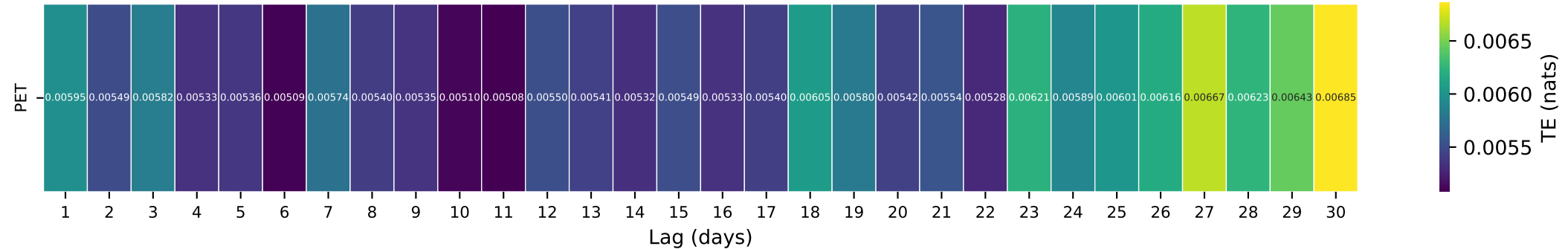
Gauge ID: 14187000 | WILEY CREEK NEAR FOSTER, OR | PET(t-\tau) \rightarrow Q(t)
