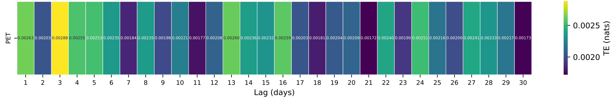
Gauge ID: 01544500 | Kettle Creek at Cross Fork, PA | PET(t-\tau) \rightarrow Q(t)
