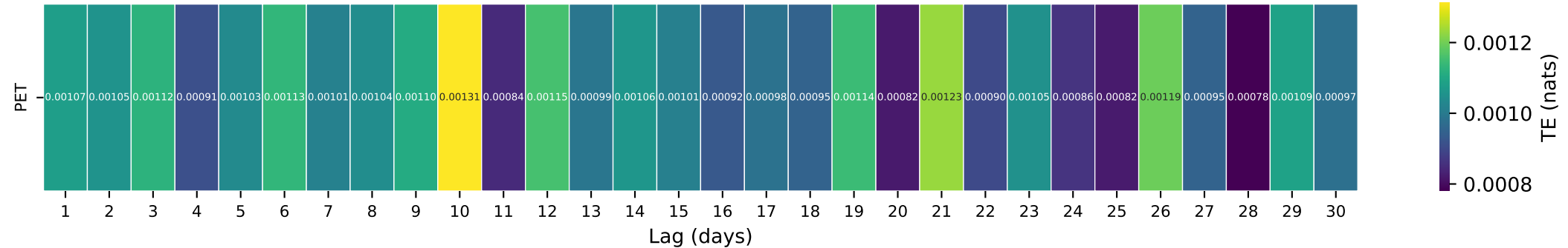
Gauge ID: 05458000 | Little Cedar River near Ionia, IA | PET(t-\tau) \rightarrow Q(t)
