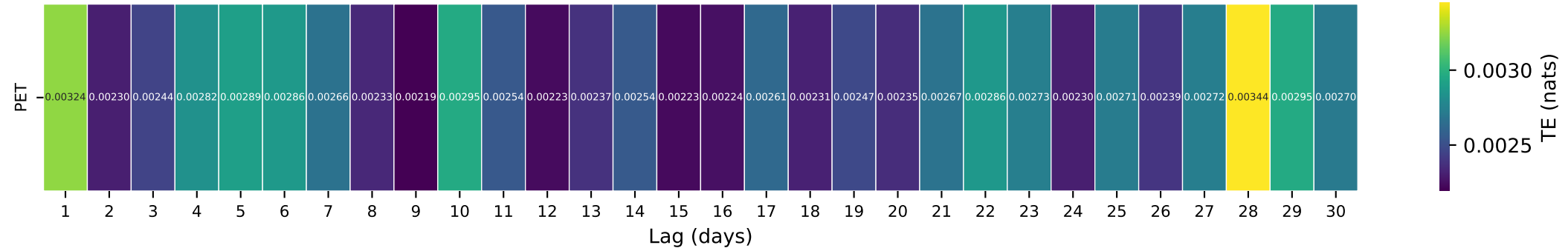
Gauge ID: 04115265 | FISH CREEK NEAR CRYSTAL, MI | PET(t-\tau) \rightarrow Q(t)
