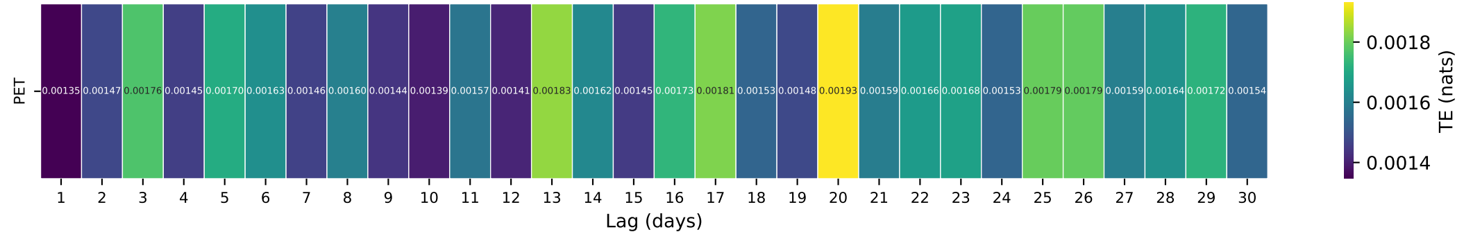
Gauge ID: 07226500 | UTE CREEK NEAR LOGAN, NM | PET(t-\tau) \rightarrow Q(t)
