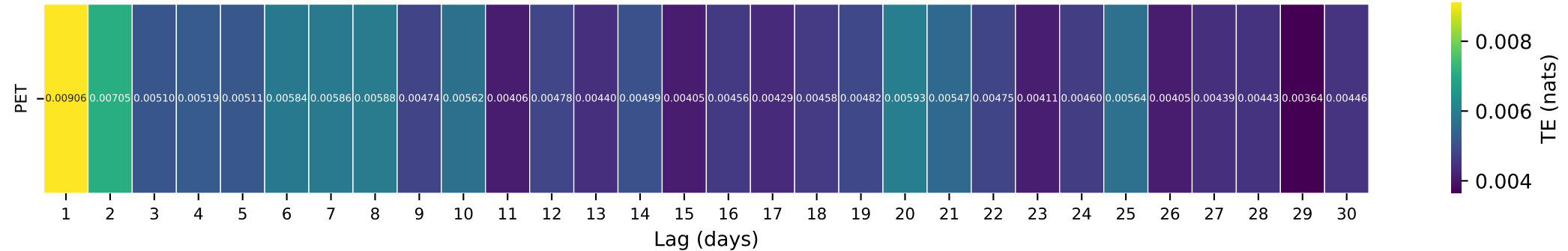
Gauge ID: 12447390 | ANDREWS CREEK NEAR MAZAMA, WA | PET(t-\tau) \rightarrow Q(t)
