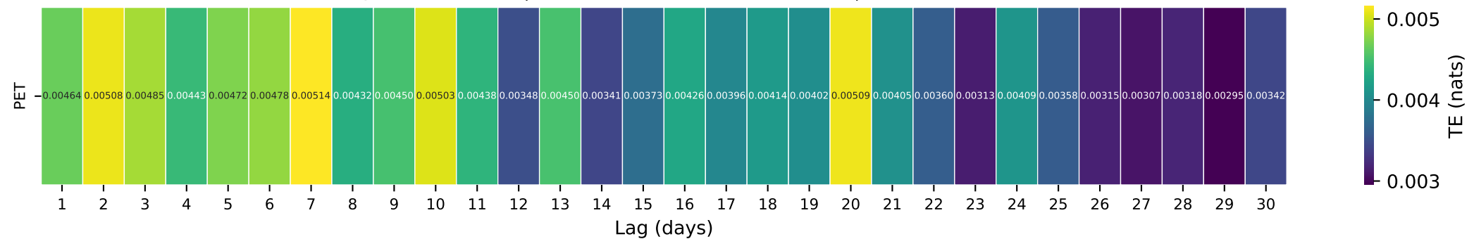
Gauge ID: 05393500 | SPIRIT RIVER AT SPIRIT FALLS, WI | PET(t-\tau) \rightarrow Q(t)
