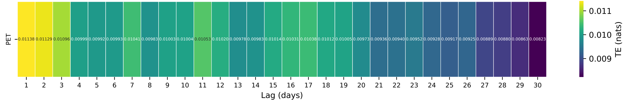
Gauge ID: 12041200 | HOH RIVER AT US HIGHWAY 101 NEAR FORKS, WA | PET(t-\tau) \rightarrow Q(t)
