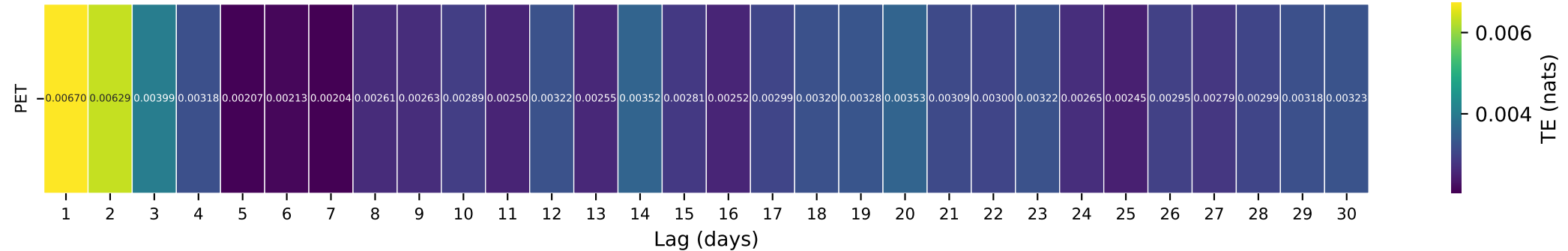
Gauge ID: 01030500 | Mattawamkeag River near Mattawamkeag, Maine | PET(t-\tau) \rightarrow Q(t)
