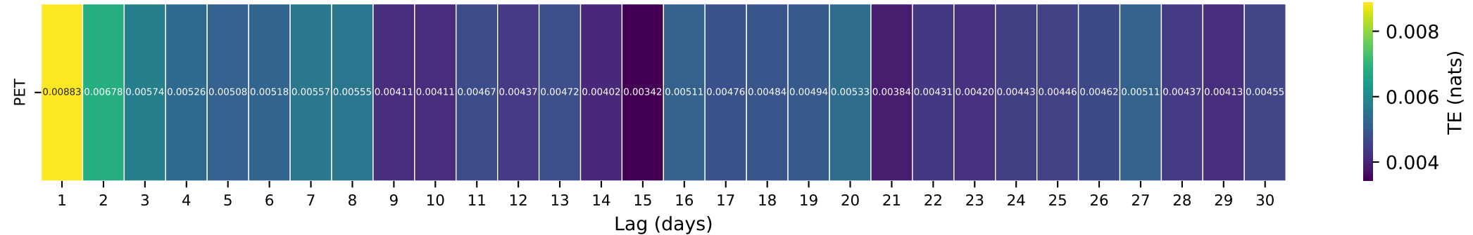
Gauge ID: 06632400 | ROCK CREEK AB KING CANYON CANAL, NR ARLINGTON, WY | PET(t-\tau) \rightarrow Q(t)
