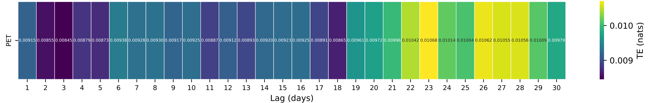
Gauge ID: 14309500 | WEST FORK COW CREEK NEAR GLENDALE, OR | PET(t-\tau) \rightarrow Q(t)
