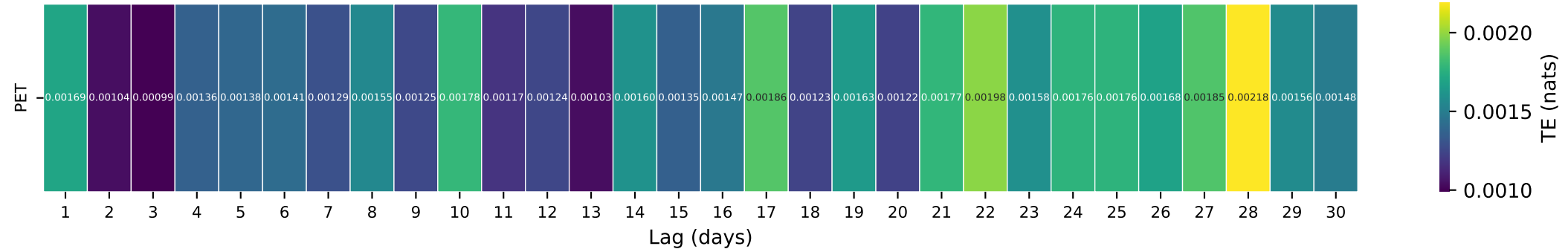
Gauge ID: 02016000 | COWPASTURE RIVER NEAR CLIFTON FORGE, VA | PET(t-\tau) \rightarrow Q(t)
