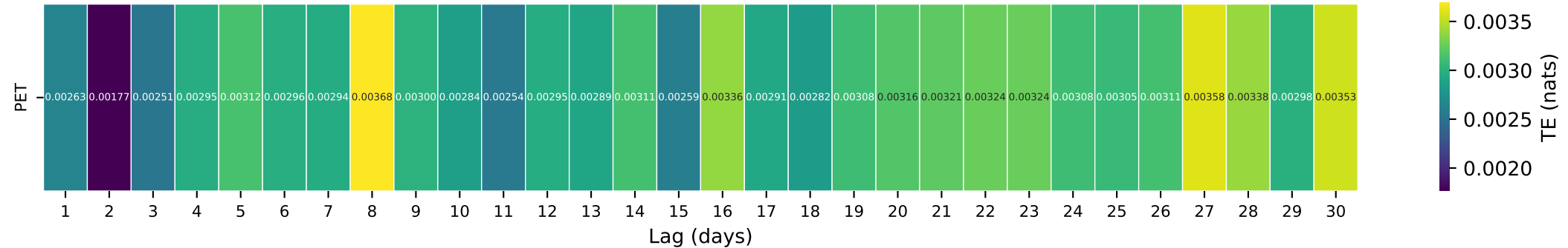
Gauge ID: 01195100 | INDIAN RIVER NEAR CLINTON, CT. | PET(t-\tau) \rightarrow Q(t)
