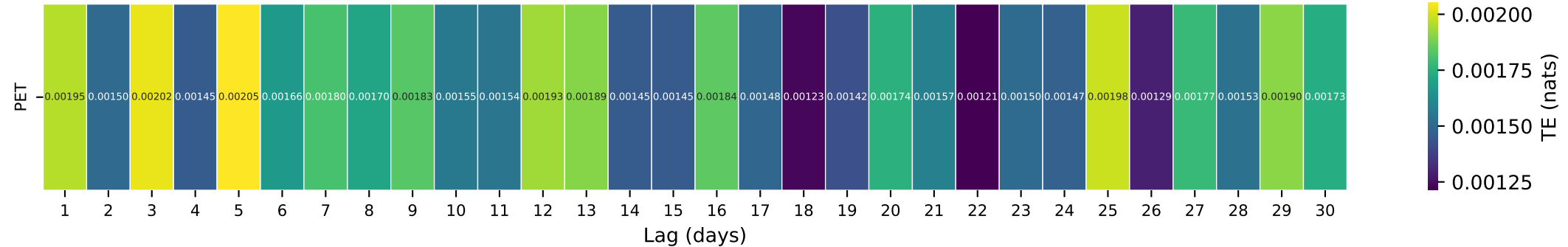
Gauge ID: 01545600 | Young Womans Creek near Renovo, PA | PET( t-\tau ) \rightarrow Q( t )
