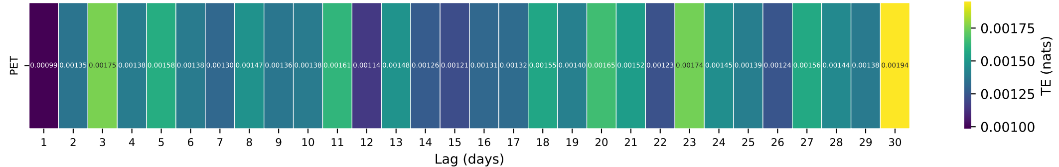
Gauge ID: 07299670 | Groesbeck Ck at SH 6 nr Quannah, TX | PET(t-\tau) \rightarrow Q(t)
