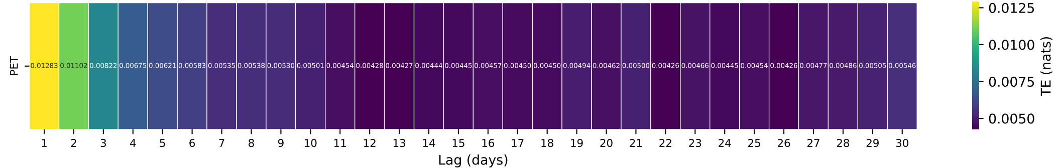
Gauge ID: 12175500 | THUNDER CREEK NEAR NEWHALEM, WA | PET(t-\tau) \rightarrow Q(t)
