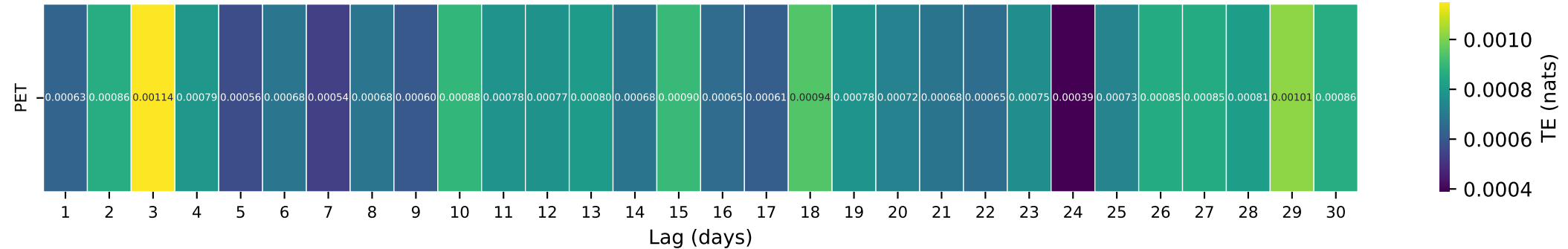
Gauge ID: 03237500 | Ohio Brush Creek near West Union OH | PET(t-\tau) \rightarrow Q(t)
