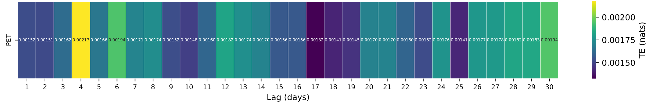
Gauge ID: 01552500 | Muncy Creek near Sonestown, PA | PET(t-\tau) \rightarrow Q(t)
