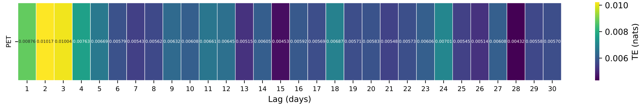
Gauge ID: 12375900 | South Crow Creek near Ronan MT | PET(t-\tau) \rightarrow Q(t)
