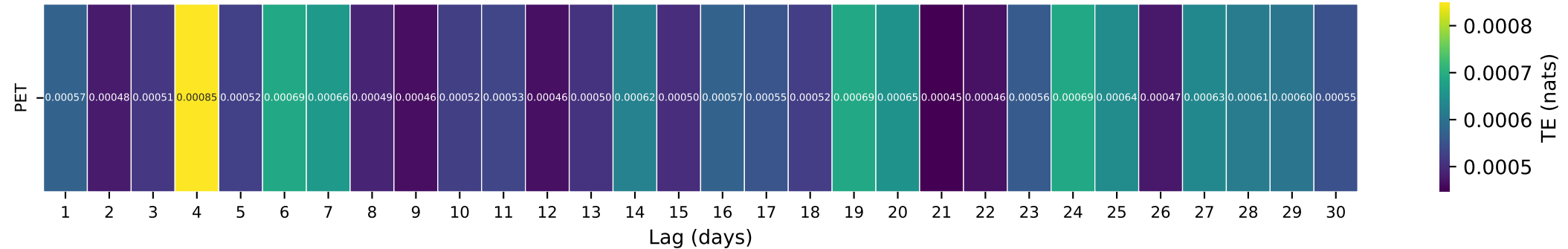
Gauge ID: 02465493 | ELLIOTTS CREEK AT MOUNDVILLE AL | PET(t-\tau) \rightarrow Q(t)
