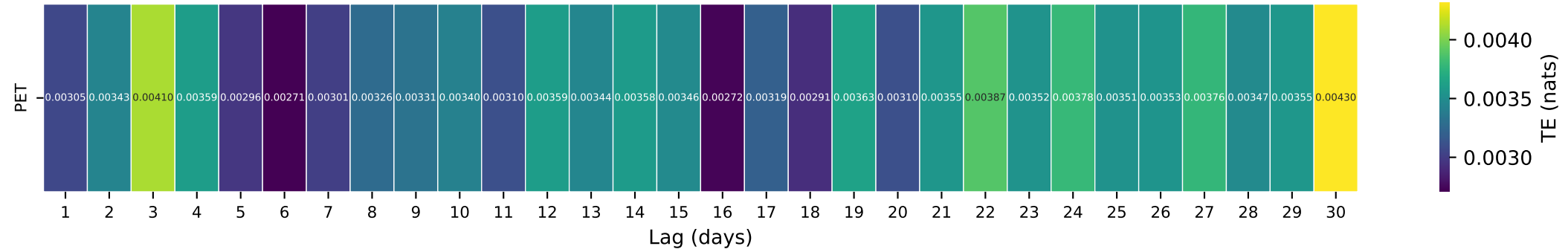
Gauge ID: 02415000 | HILLABEE CREEK NEAR HACKNEYVILLE AL | PET(t-\tau) \rightarrow Q(t)
