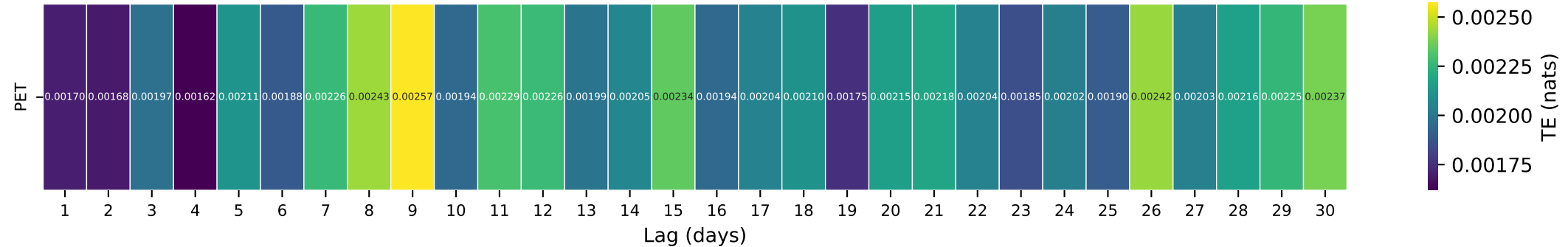
Gauge ID: 01423000 | WEST BRANCH DELAWARE RIVER AT WALTON NY | PET(t-\tau) \rightarrow Q(t)
