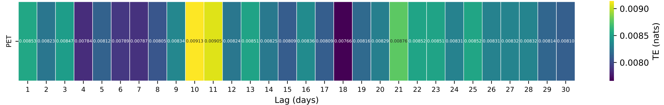
Gauge ID: 12035000 | SATSOP RIVER NEAR SATSOP, WA | PET(t-\tau) \rightarrow Q(t)
