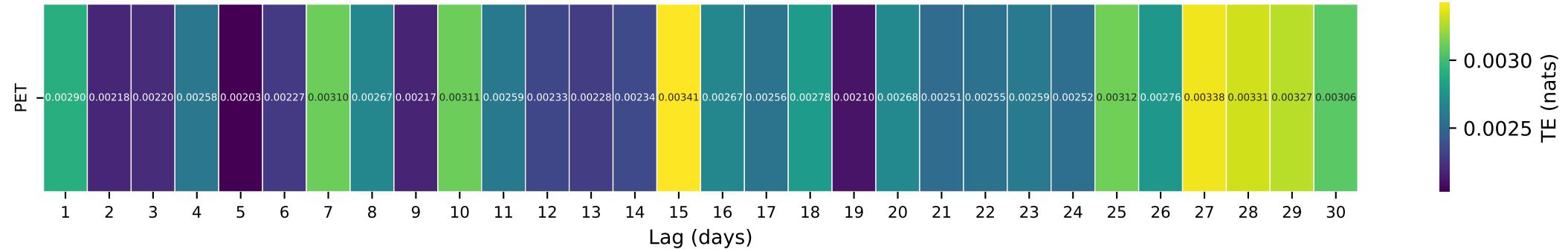
Gauge ID: 02450250 | SIPSEY FORK NEAR GRAYSON AL | PET(t- \tau ) \rightarrow Q(t)
