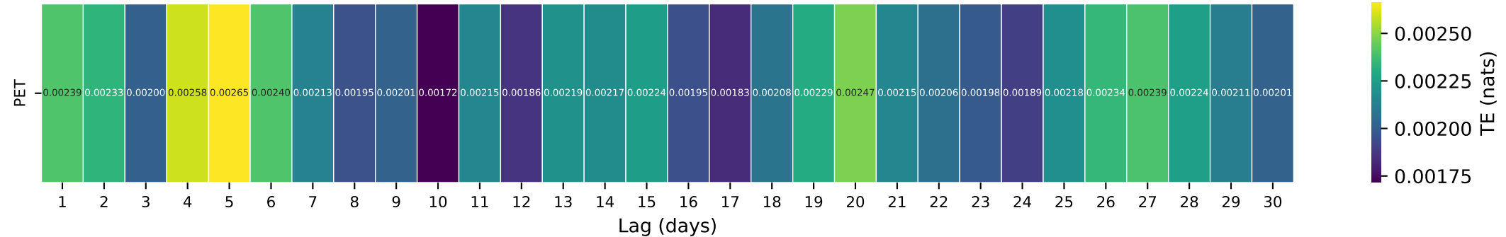
Gauge ID: 02212600 | FALLING CREEK NEAR JULIETTE, GA | PET(t-\tau) \rightarrow Q(t)
