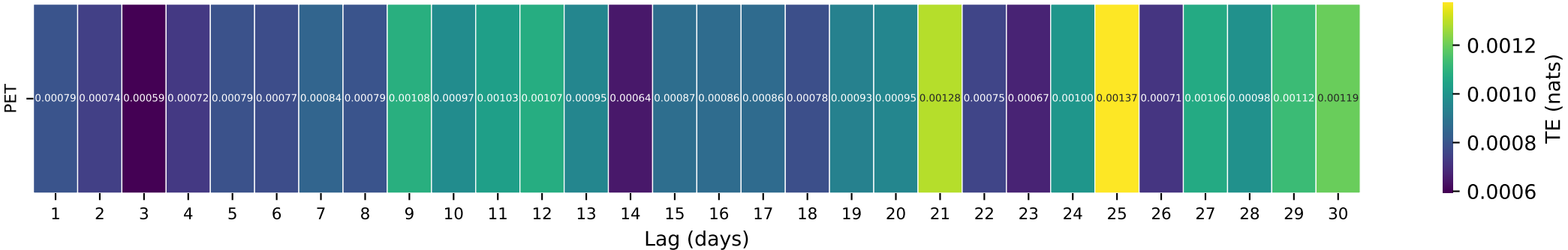
Gauge ID: 02070000 | NORTH MAYO RIVER NEAR SPENCER, VA | PET(t-τ) → Q(t)
