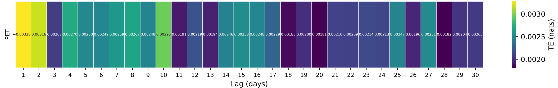
Gauge ID: 05466500 | EDWARDS RIVER NEAR NEW BOSTON, IL | PET(t-\tau) \rightarrow Q(t)
