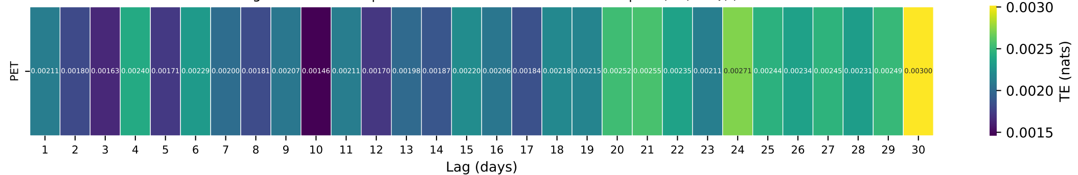
Gauge ID: 01510000 | OTSELIC RIVER AT CINCINNATUS NY | PET(t-\tau) \rightarrow Q(t)
