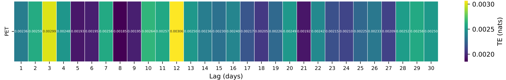
Gauge ID: 06406000 | BATTLE CR AT HERMOSA SD | PET(t- \tau ) \rightarrow Q(t)
