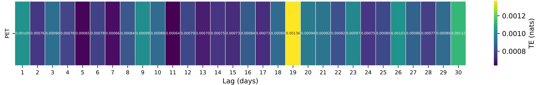
Gauge ID: 08195000 | Frio Rv at Concan, TX | PET(t-\tau) \rightarrow Q(t)
