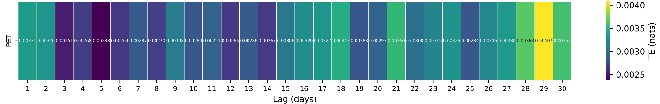
Gauge ID: 04196800 | Tymochtee Creek at Crawford OH | PET(t-\tau) \rightarrow Q(t)
