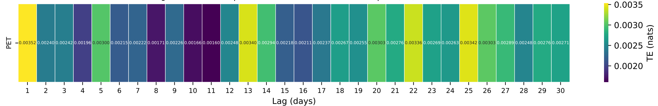
Gauge ID: 01078000 | SMITH RIVER NEAR BRISTOL, NH | PET(t-\tau) \rightarrow Q(t)
