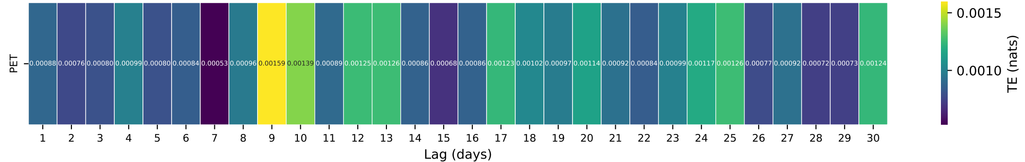
Gauge ID: 01047000 | Carrabassett River near North Anson, Maine | PET(t-\tau) \rightarrow Q(t)
