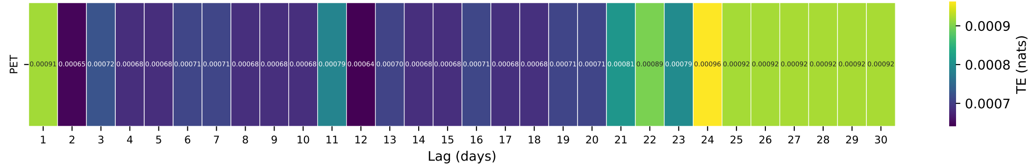
Gauge ID: 09512280 | CAVE CREEK BLW COTTONWOOD CR NEAR CAVE CREEK, AZ. | PET(t-\tau) \rightarrow Q(t)
