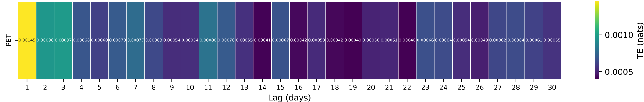
Gauge ID: 06339100 | KNIFE RIVER AT MANNING, ND | PET(t-\tau) \rightarrow Q(t)
