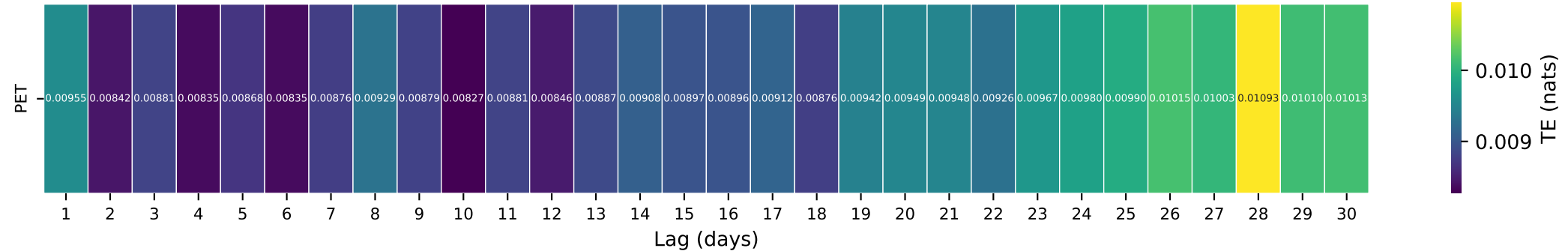
Gauge ID: 14316700 | STEAMBOAT CREEK NEAR GLIDE, OR | PET(t-\tau) \rightarrow Q(t)
