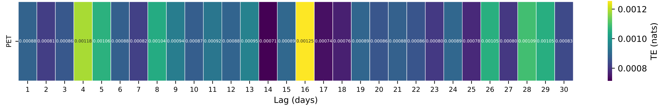
Gauge ID: 02350900 | KINCHAFOONEE CREEK NEAR DAWSON, GA | PET(t-\tau) \rightarrow Q(t)
