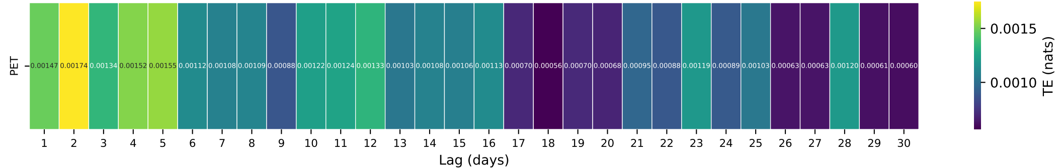
Gauge ID: 09492400 | EAST FORK WHITE RIVER NEAR FORT APACHE, AZ. | PET(t-\tau) \rightarrow Q(t)
