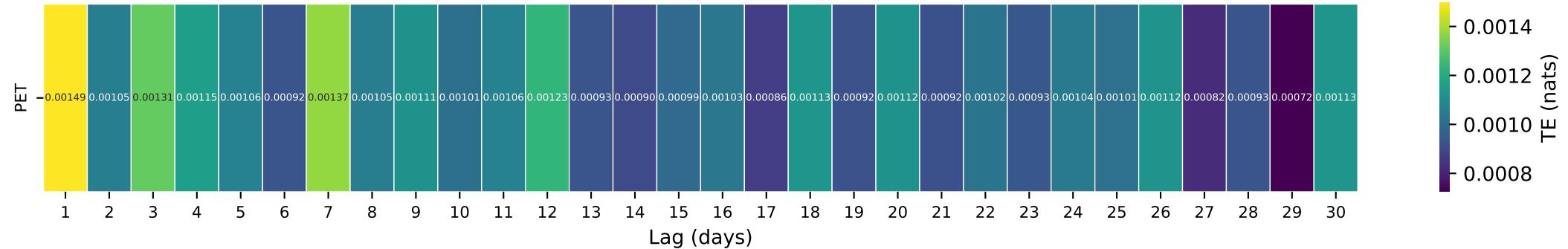
Gauge ID: 01669000 | PISCATAWAY CREEK NEAR TAPPAHANNOCK, VA | PET(t-\tau) \rightarrow Q(t)
