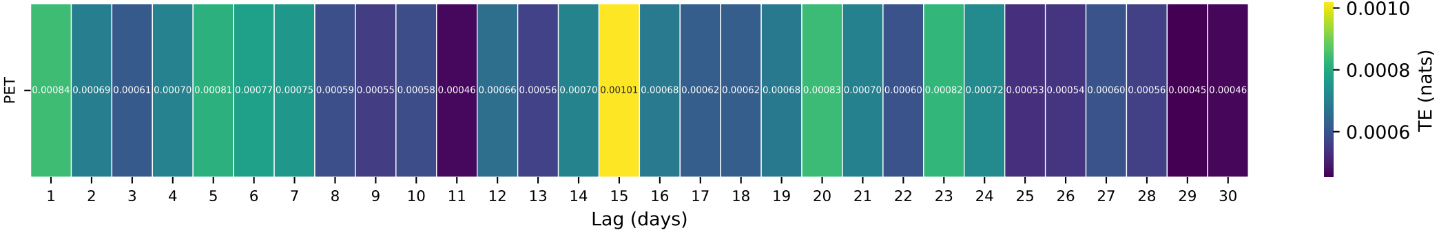
Gauge ID: 07060710 | North Sylamore Creek near Fifty Six, AR | PET(t-\tau) \rightarrow Q(t)
