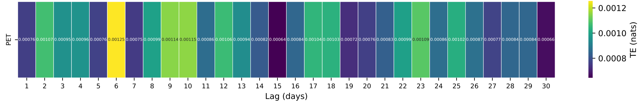
Gauge ID: 06917000 | L OSAGE R AT FULTON, KS | PET(t- \tau ) \rightarrow Q(t)
