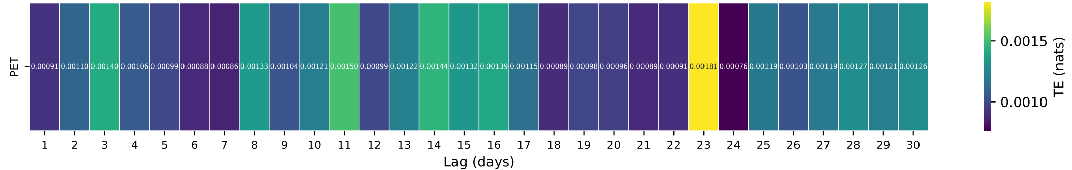
Gauge ID: 08189500 | Mission Rv at Refugio, TX | PET(t- \tau ) \rightarrow Q(t)
