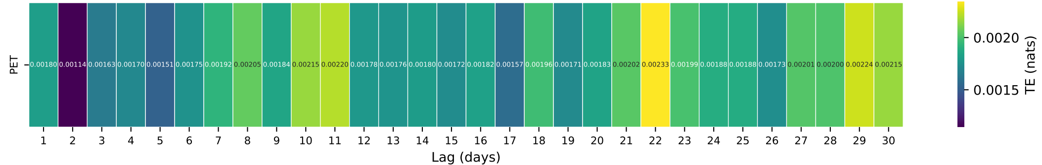
Gauge ID: 08025500 | Bayou Toro near Toro, LA | PET(t- \tau ) \rightarrow Q(t)
