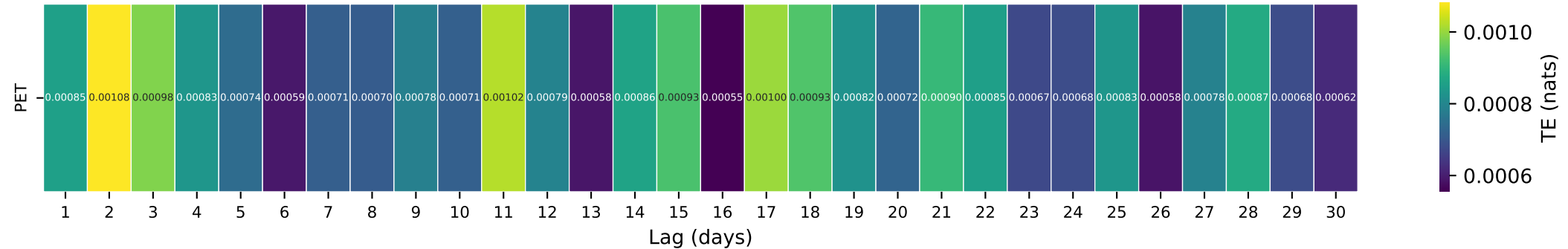
Gauge ID: 01632000 | N F SHENANDOAH RIVER AT COOTES STORE, VA | PET(t-\tau) \rightarrow Q(t)
