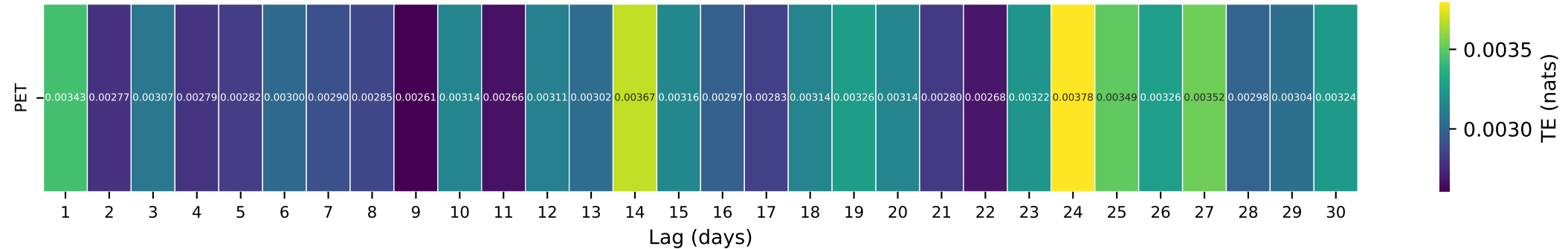
Gauge ID: 07292500 | HOMOCHITTO RIVER AT ROSETTA, MS | PET(t-\tau) \rightarrow Q(t)
