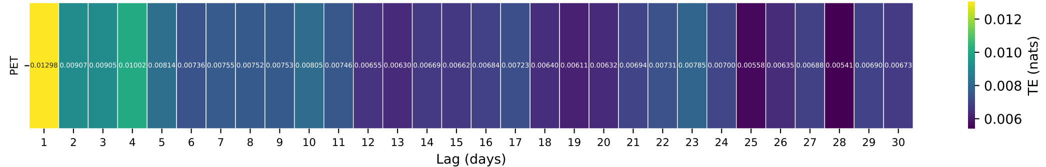
Gauge ID: 09066200 | BOOTH CREEK NEAR MINTURN, CO. | PET(t-\tau) \rightarrow Q(t)
