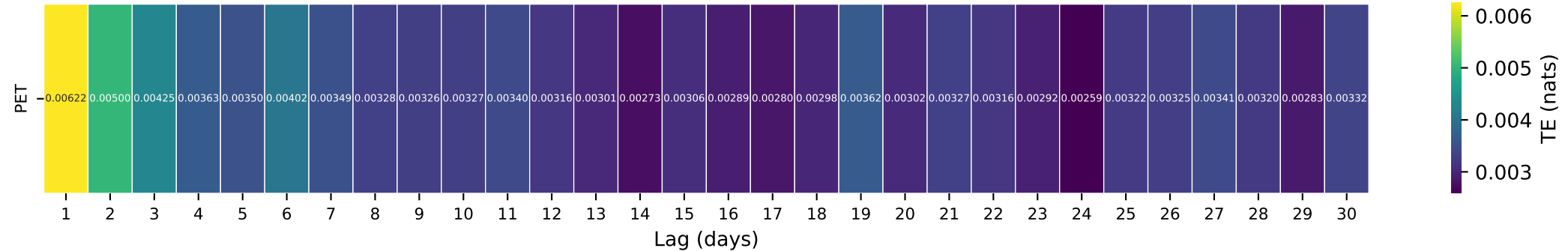
Gauge ID: 10336645 | GENERAL C NR MEEKS BAY CA | PET(t- \tau ) \rightarrow Q(t)
