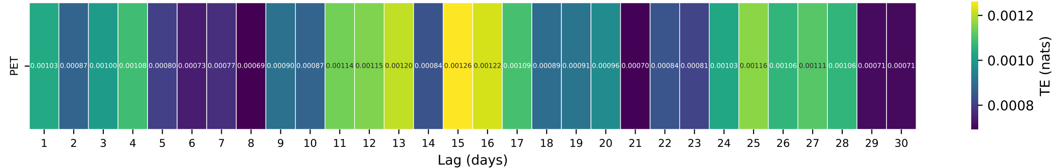
Gauge ID: 02143040 | JACOB FORK AT RAMSEY, NC | PET(t-\tau) \rightarrow Q(t)
