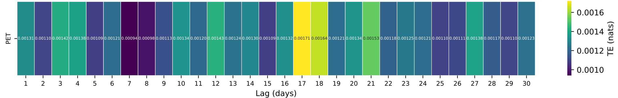
Gauge ID: 06601000 | OMAHA CR AT HOMER, NEBR | PET(t- \tau ) \rightarrow Q(t)
