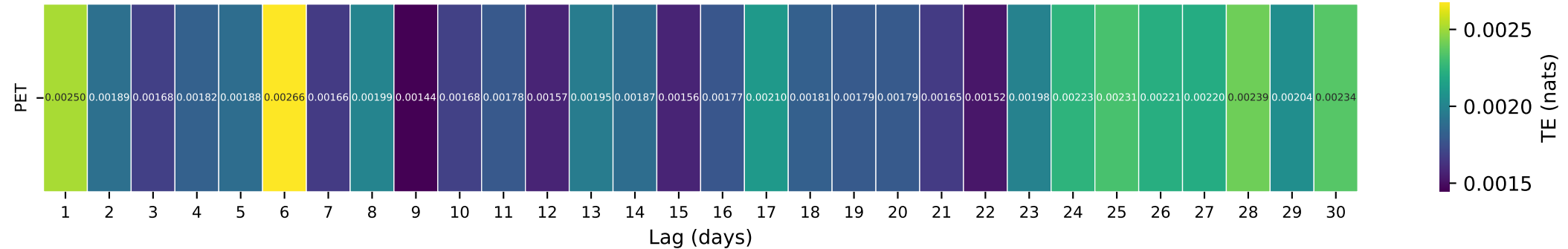
Gauge ID: 02017500 | JOHNS CREEK AT NEW CASTLE, VA | PET(t-\tau) \rightarrow Q(t)
