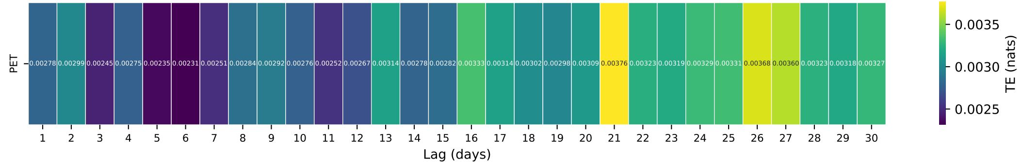
Gauge ID: 12115000 | CEDAR RIVER NEAR CEDAR FALLS, WA | PET(t-\tau) \rightarrow Q(t)
