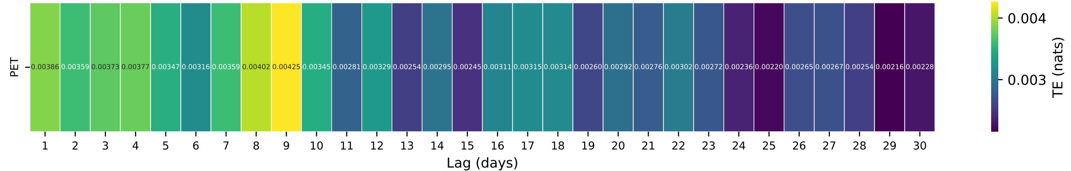
Gauge ID: 09378170 | SOUTH CREEK ABOVE RESERVOIR NEAR MONTICELLO, UT | PET(t-\tau) \rightarrow Q(t)
