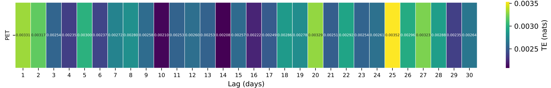
Gauge ID: 01137500 | AMMONOOSUC RIVER AT BETHLEHEM JUNCTION, NH | PET(t-\tau) \rightarrow Q(t)
