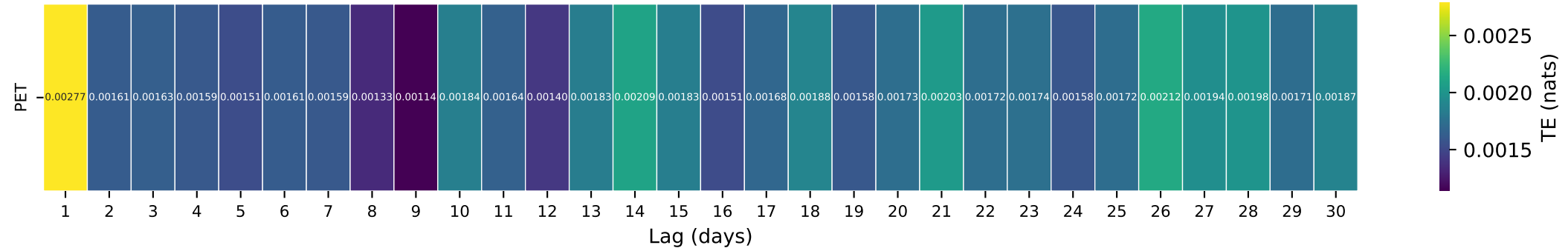
Gauge ID: 03500000 | LITTLE TENNESSEE RIVER NEAR PRENTISS, NC | PET(t-\tau) \rightarrow Q(t)
