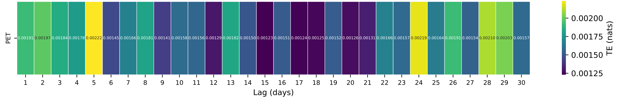
Gauge ID: 01518862 | Cowanesque River at Westfield, PA | PET(t-\tau) \rightarrow Q(t)
