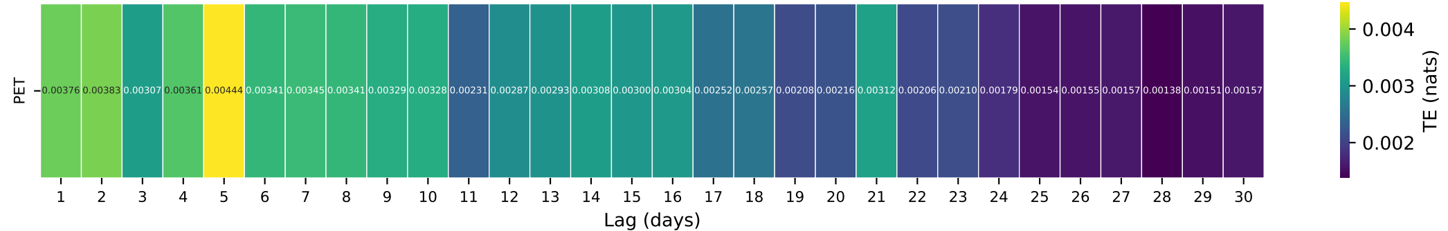
Gauge ID: 04040500 | STURGEON RIVER NEAR SIDNAW, MI | PET(t-\tau) \rightarrow Q(t)
