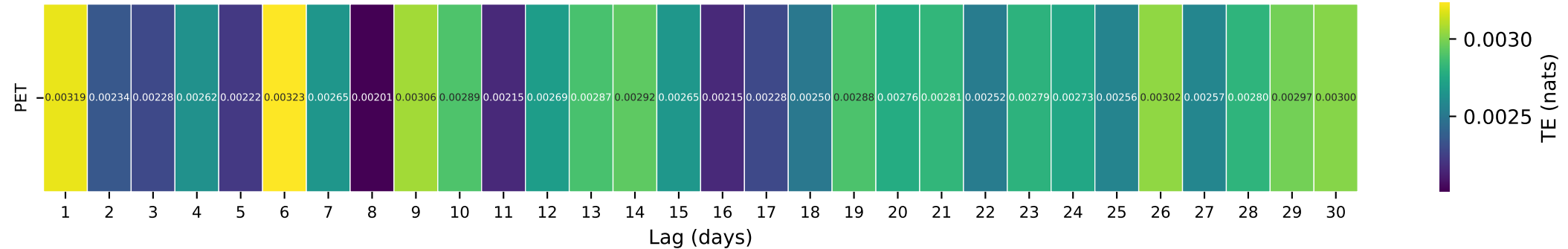
Gauge ID: 02464360 | BINION CREEK BELOW GIN CREEK NEAR SAMANTHA AL | PET(t-\tau) \rightarrow Q(t)
