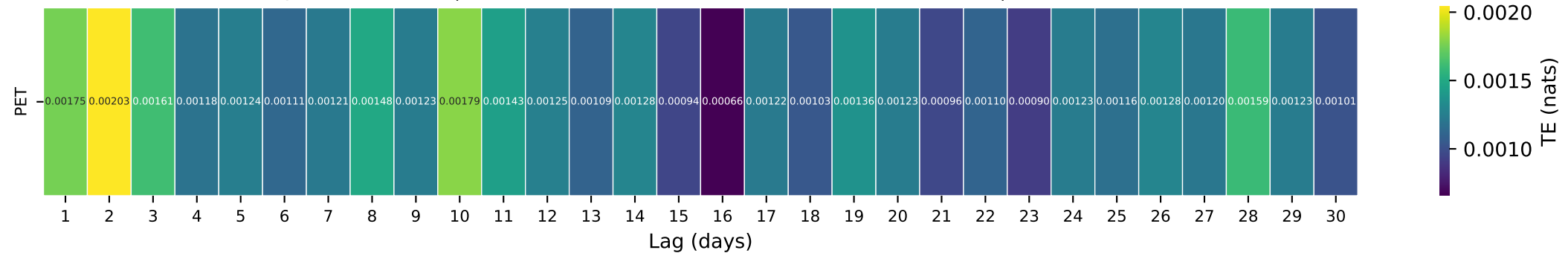
Gauge ID: 01466500 | MCDONALDS BRANCH IN LEBANON STATE FOREST NJ | PET(t-\tau) \rightarrow Q(t)
