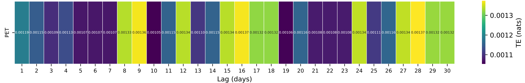
Gauge ID: 14096850 | BEAVER CREEK, BLW QUARTZ CR, NR SIMNASHO, OR. | PET(t-\tau) \rightarrow Q(t)
