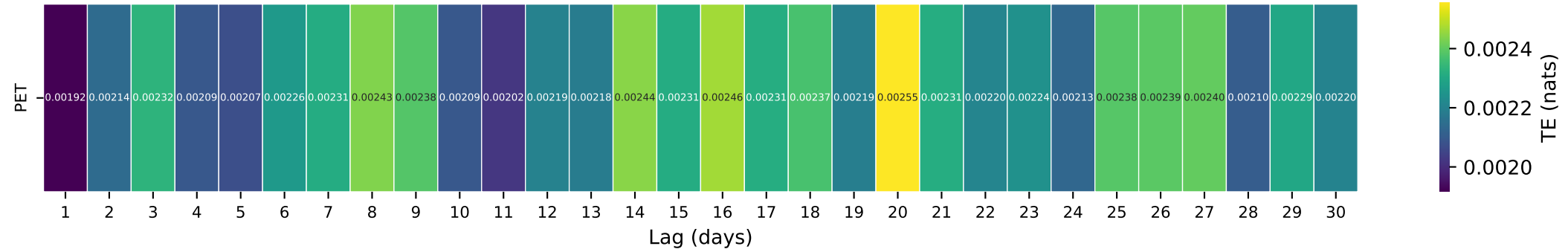
Gauge ID: 03498500 | LITTLE RIVER NEAR MARYVILLE, TN | PET(t-\tau) \rightarrow Q(t)
