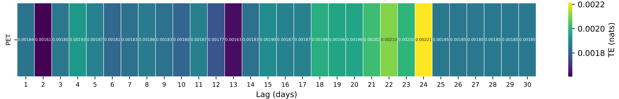
Gauge ID: 09510200 | SYCAMORE CREEK NEAR FORT MCDOWELL, AZ. | PET(t-\tau) \rightarrow Q(t)
