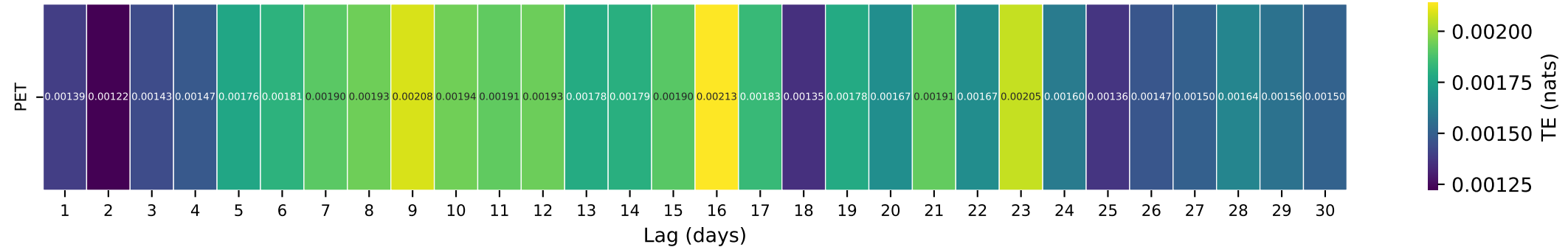
Gauge ID: 02027000 | TYE RIVER NEAR LOVINGSTON, VA | PET(t-\tau) \rightarrow Q(t)
