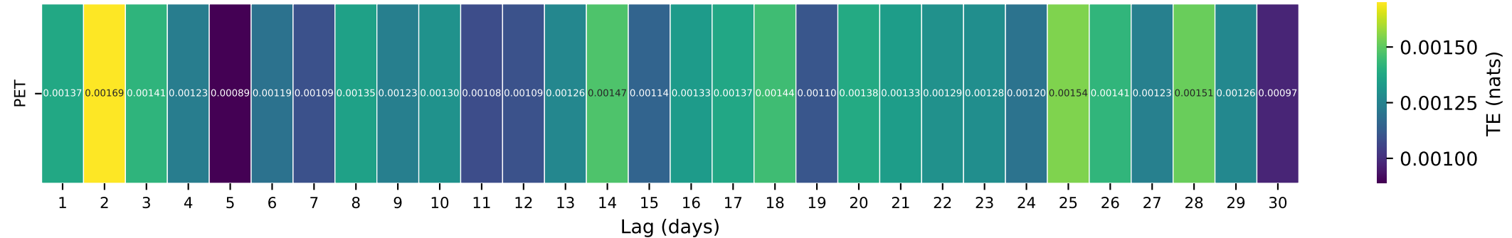
Gauge ID: 02140991 | JOHNS RIVER AT ARNEYS STORE, NC | PET(t-\tau) \rightarrow Q(t)
