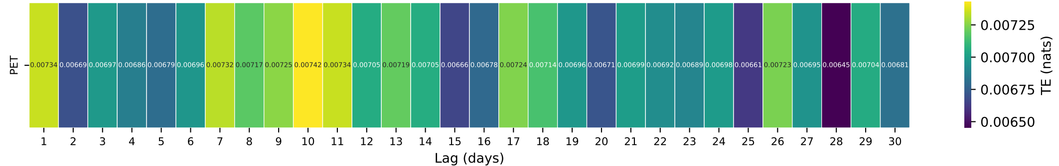
Gauge ID: 14303200 | TUCCA CREEK NEAR BLAINE, OR. | PET(t-\tau) \rightarrow Q(t)
