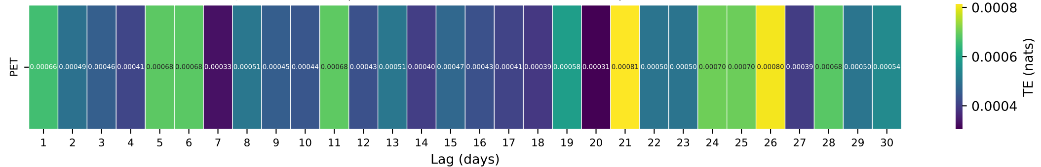
Gauge ID: 02059500 | GOOSE CREEK NEAR HUDDLESTON, VA | PET(t-\tau) \rightarrow Q(t)
