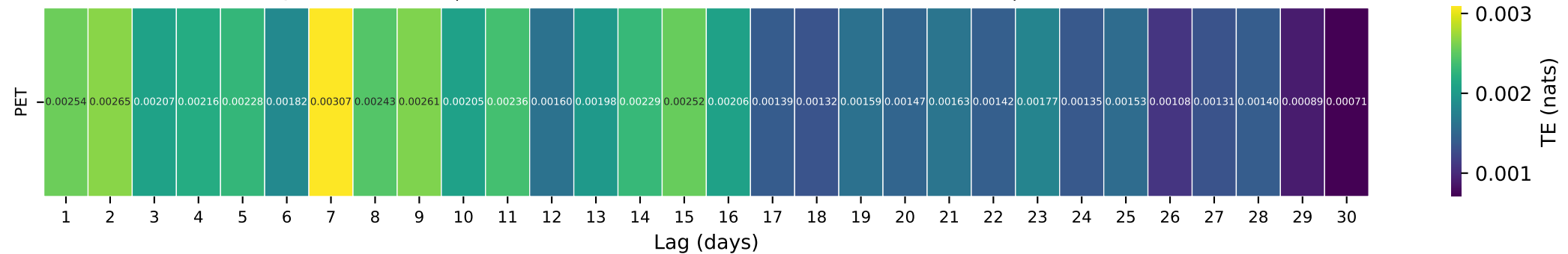
Gauge ID: 04057800 | MIDDLE BRANCH ESCANABA RIVER AT HUMBOLDT, MI | PET(t-\tau) \rightarrow Q(t)
