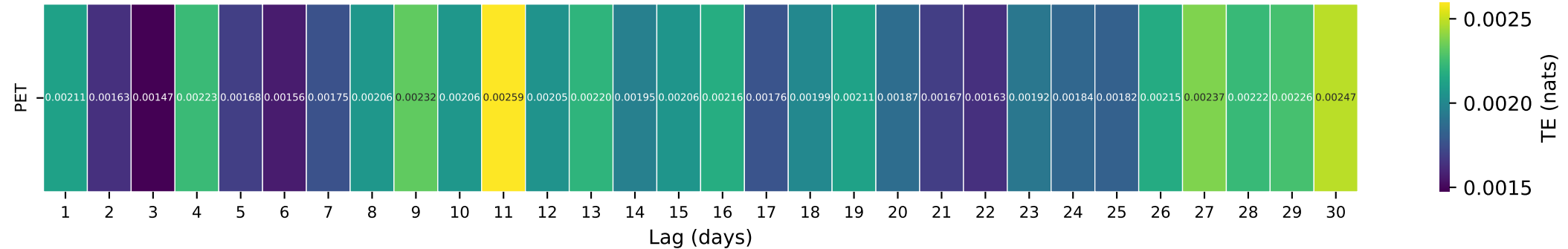
Gauge ID: 05514500 | CUIVRE RIVER NEAR TROY, MO | PET(t-\tau) \rightarrow Q(t)
