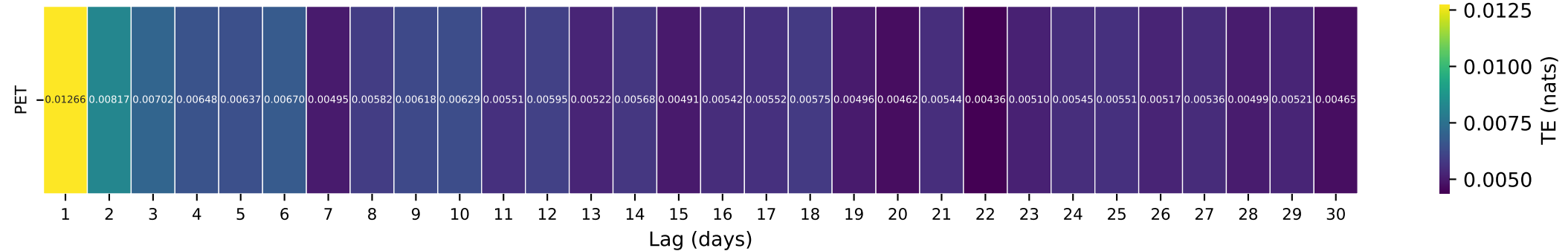
Gauge ID: 09107000 | TAYLOR RIVER AT TAYLOR PARK, CO. | PET(t-\tau) \rightarrow Q(t)
