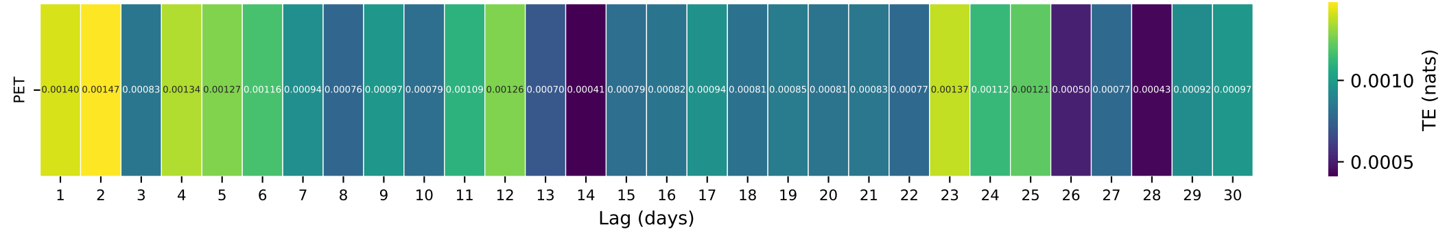
Gauge ID: 01669520 | DRAGON SWAMP AT MASCOT, VA | PET(t-\tau) \rightarrow Q(t)
