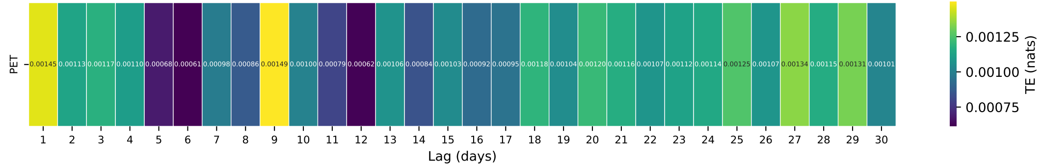
Gauge ID: 02128000 | LITTLE RIVER NEAR STAR, NC | PET(t- \tau ) \rightarrow Q(t)
