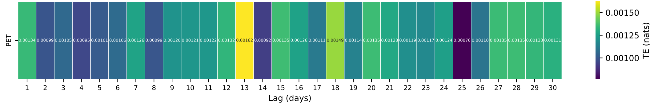
Gauge ID: 05414000 | PLATTE RIVER NEAR ROCKVILLE, WI | PET(t-\tau) \rightarrow Q(t)
