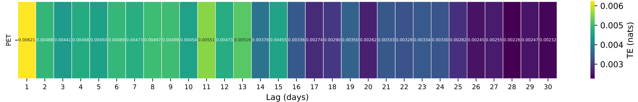
Gauge ID: 05129115 | VERMILION RIVER NR CRANE LAKE, MN | PET(t-\tau) \rightarrow Q(t)
