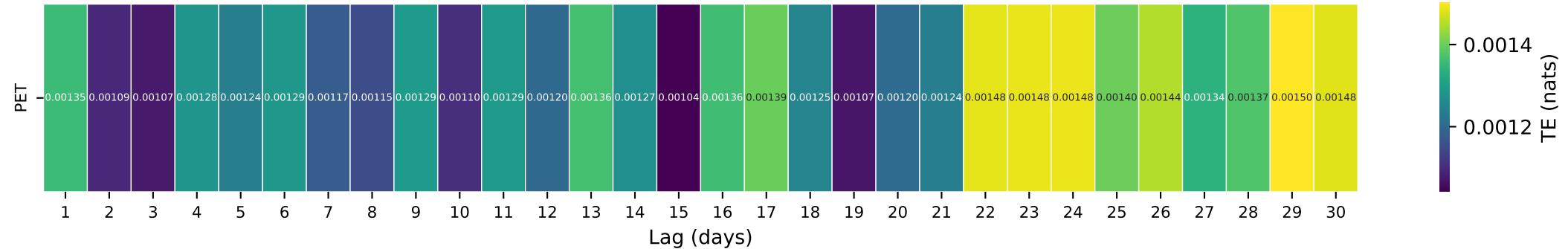
Gauge ID: 07197000 | Baron Fork at Eldon, OK | PET(t-\tau) \rightarrow Q(t)
