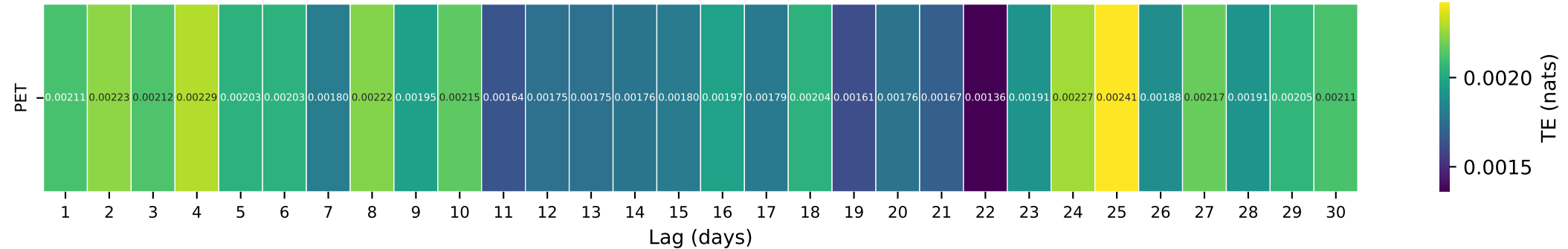
Gauge ID: 02014000 | POTTS CREEK NEAR COVINGTON, VA | PET(t-\tau) \rightarrow Q(t)
