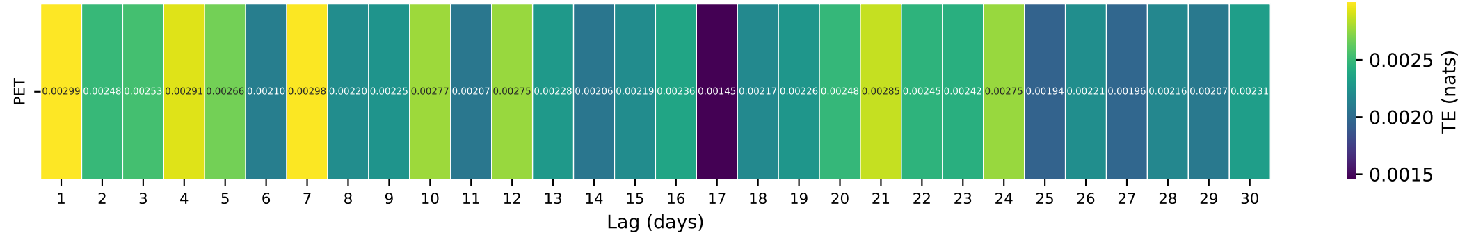
Gauge ID: 07014500 | Meramec River near Sullivan, MO | PET(t-\tau) \rightarrow Q(t)
