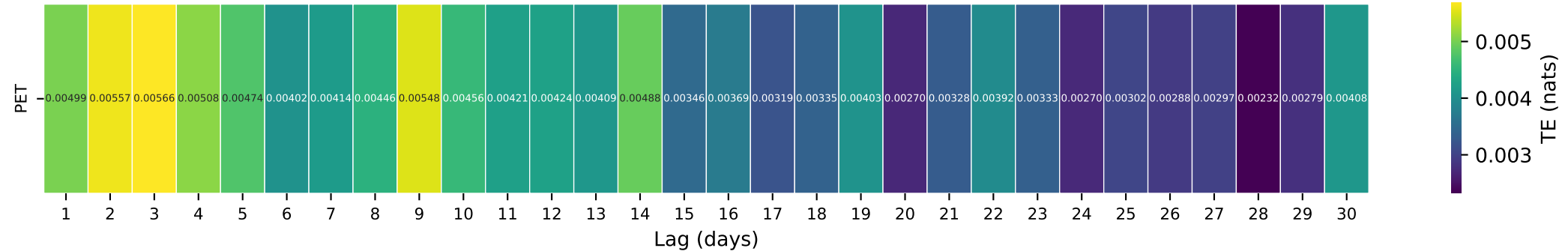
Gauge ID: 04045500 | TAHQUAMENON RIVER NEAR PARADISE, MI | PET(t-\tau) \rightarrow Q(t)
