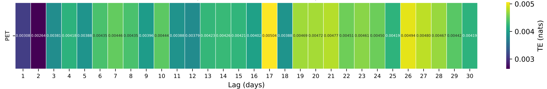
Gauge ID: 09484600 | PANTANO WASH NEAR VAIL, AZ. | PET(t-\tau) \rightarrow Q(t)
