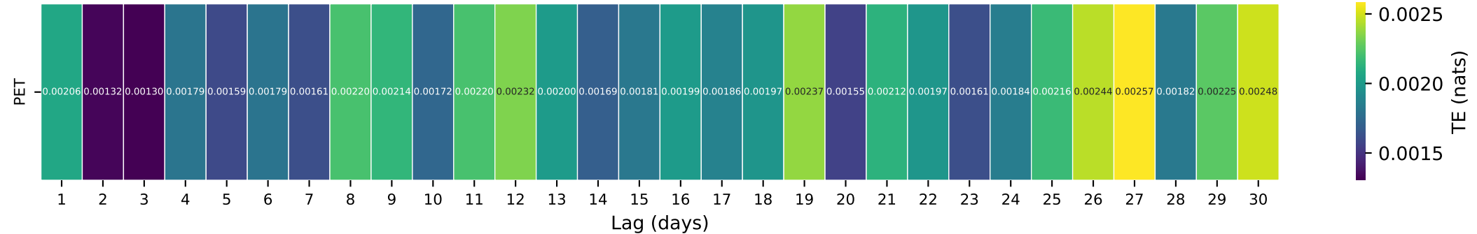
Gauge ID: 02297155 | HORSE CREEK NEAR MYAKKA HEAD FL | PET(t- \tau ) \rightarrow Q(t)
