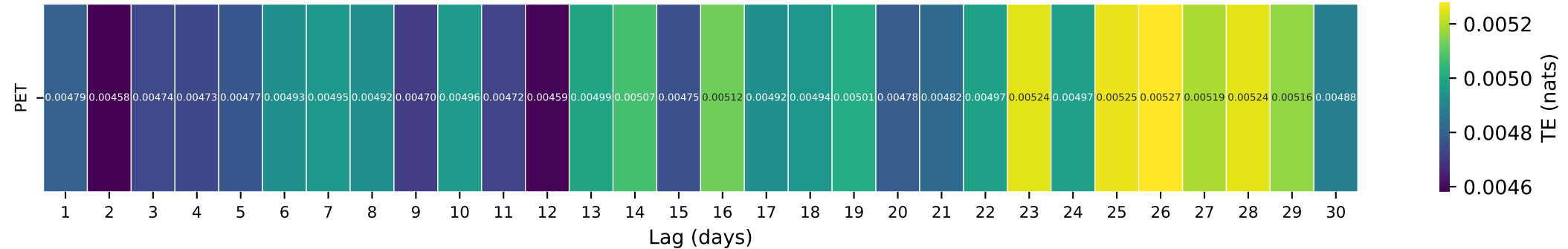
Gauge ID: 14236200 | TILTON RIVER AB BEAR CANYON CREEK NEAR CINEBAR, WA | PET(t-\tau) \rightarrow Q(t)
