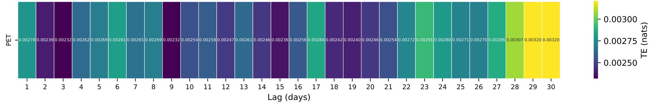
Gauge ID: 11468500 | NOYO R NR FORT BRAGG CA | PET(t- \tau ) \rightarrow Q(t)
