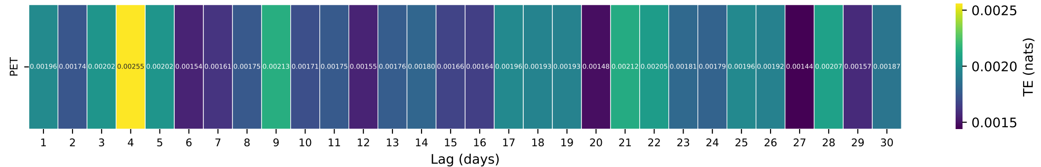
Gauge ID: 06876700 | SALT C NR ADA, KS | PET(t- \tau ) \rightarrow Q(t)
