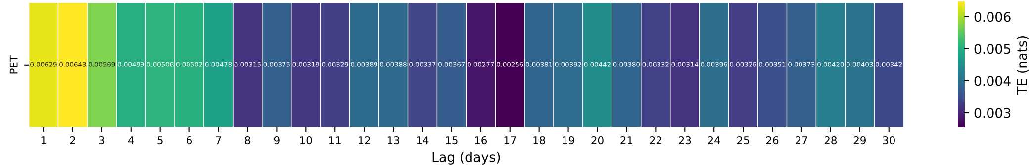
Gauge ID: 08267500 | RIO HONDO NEAR VALDEZ, NM | PET(t-\tau) \rightarrow Q(t)
