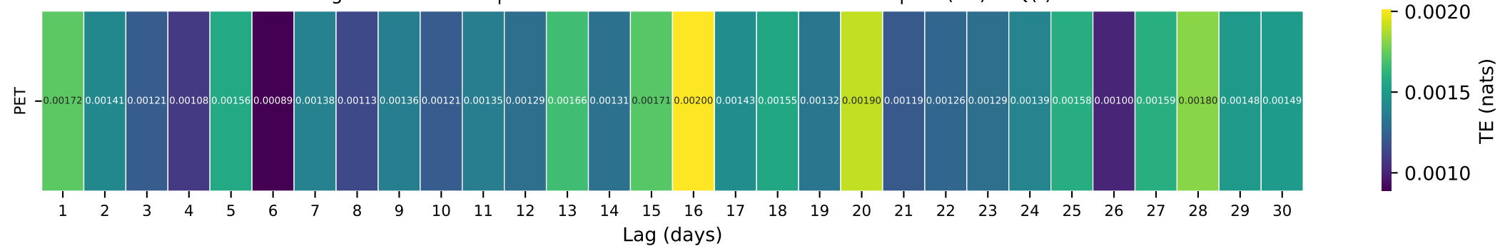
Gauge ID: 02299950 | MANATEE RIVER NEAR MYAKKA HEAD FL | PET(t- \tau ) \rightarrow Q(t)
