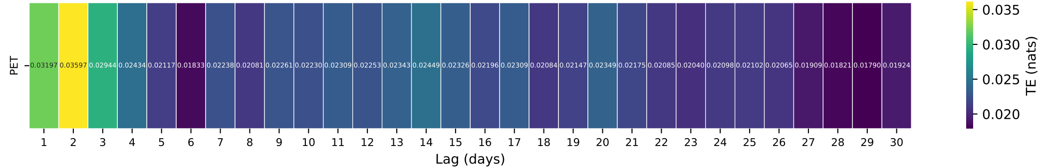
Gauge ID: 06221400 | DINWOODY CREEK ABOVE LAKES, NEAR BURRIS, WYO. | PET(t-\tau) \rightarrow Q(t)
