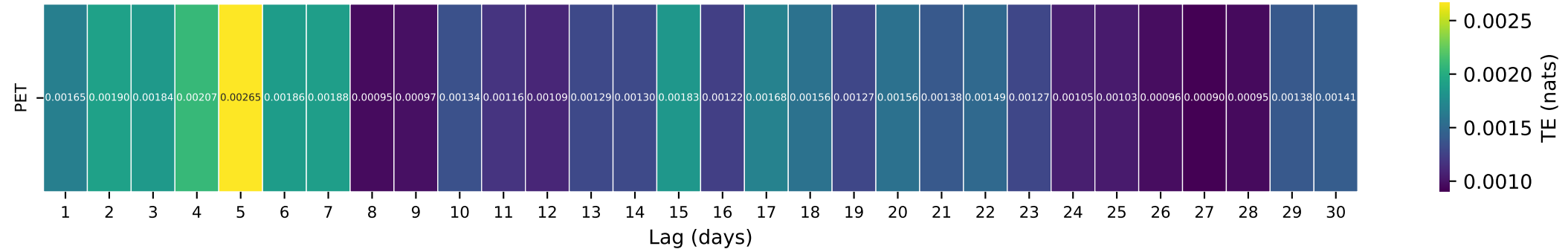
Gauge ID: 06470800 | BEAR CREEK NR OAKES, ND | PET(t- \tau ) \rightarrow Q(t)
