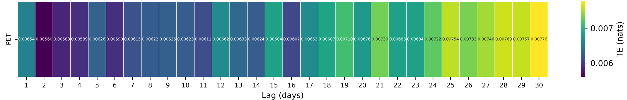
Gauge ID: 11482500 | REDWOOD C A ORICK CA | PET(t- \tau ) \rightarrow Q(t)
