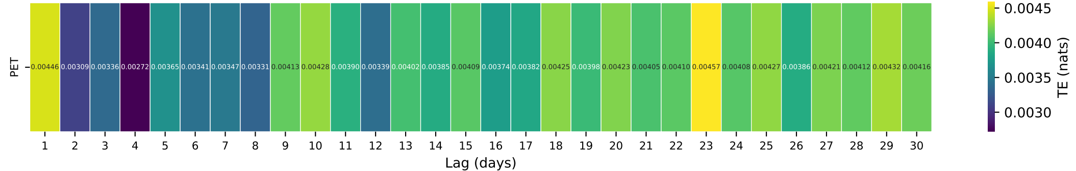
Gauge ID: 01022500 | Narraguagus River at Cherryfield, Maine | PET(t-\tau) \rightarrow Q(t)
