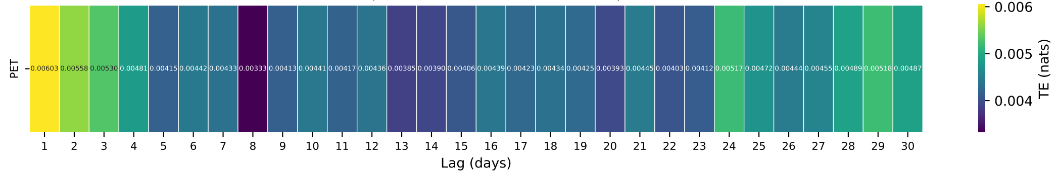
Gauge ID: 13018300 | CACHE CREEK NEAR JACKSON, WY | PET(t-\tau) \rightarrow Q(t)
