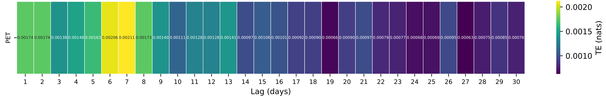
Gauge ID: 05056000 | SHEYENNE RIVER NR WARWICK, ND | PET(t-\tau) \rightarrow Q(t)
