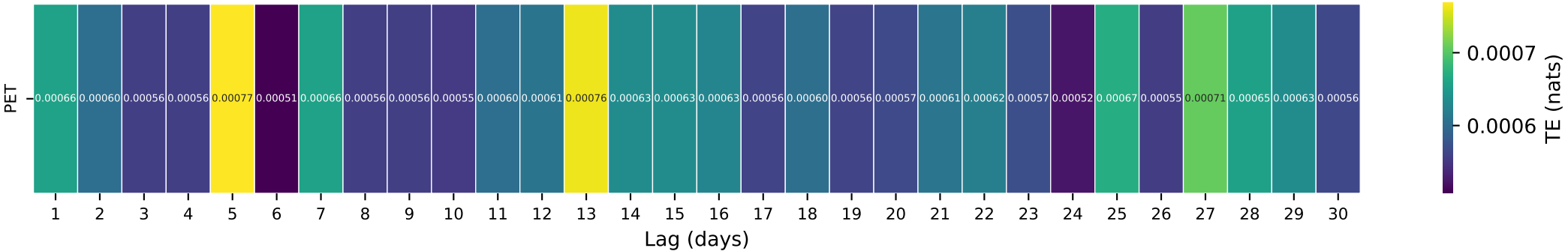
Gauge ID: 03049800 | Little Pine Creek near Etna, PA | PET(t-τ) → Q(t)
