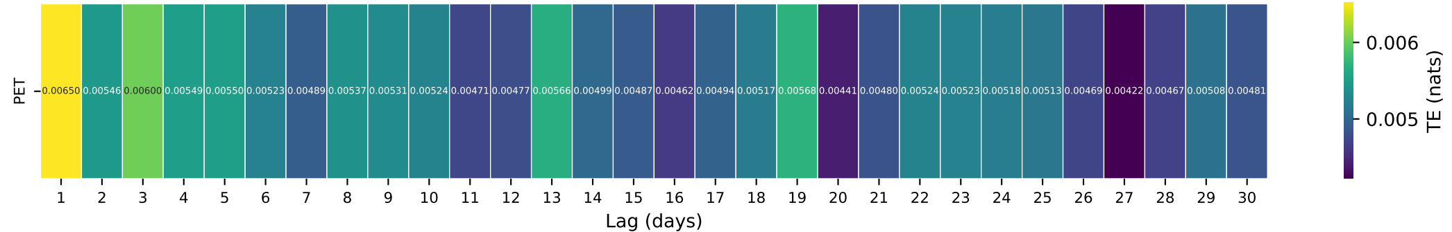
Gauge ID: 01139000 | WELLS RIVER AT WELLS RIVER, VT | PET(t-\tau) \rightarrow Q(t)
