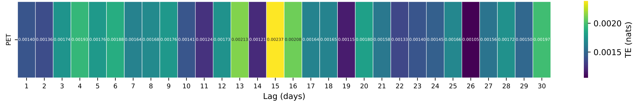
Gauge ID: 01365000 | RONDOUT CREEK NEAR LOWES CORNERS NY | PET(t-\tau) \rightarrow Q(t)
