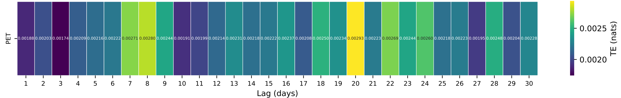
Gauge ID: 03439000 | FRENCH BROAD RIVER AT ROSMAN, NC | PET(t-\tau) \rightarrow Q(t)
