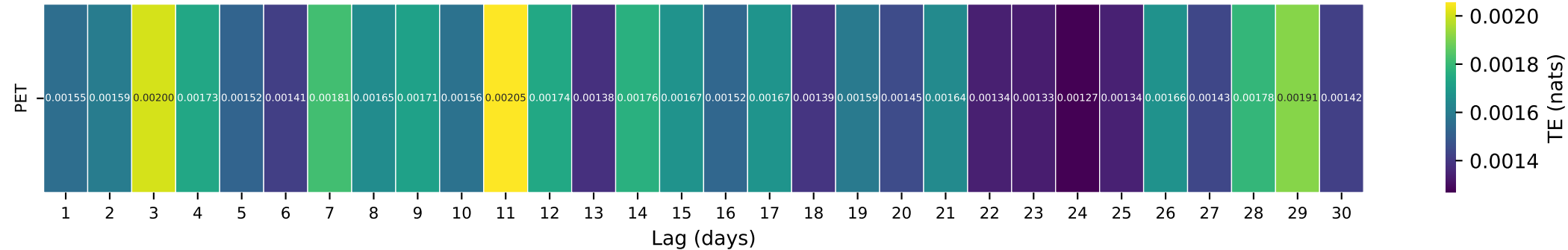
Gauge ID: 05507600 | Lick Creek at Perry, MO | PET(t-\tau) \rightarrow Q(t)
