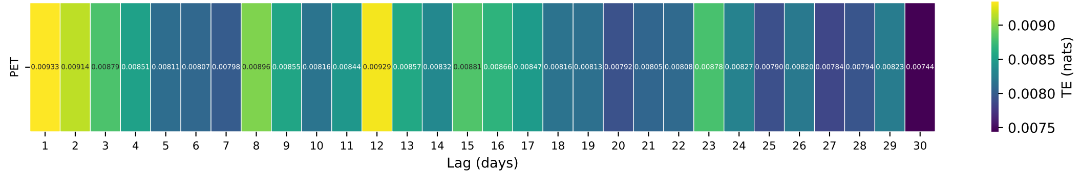
Gauge ID: 12010000 | NASELLE RIVER NEAR NASELLE, WA | PET(t-\tau) \rightarrow Q(t)
