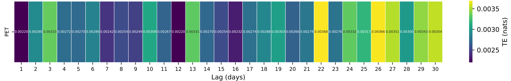
Gauge ID: 03238500 | White Oak Creek near Georgetown OH | PET(t- \tau ) \rightarrow Q(t)
