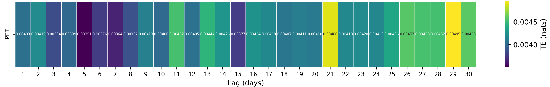
Gauge ID: 12115500 | REX RIVER NEAR CEDAR FALLS, WA | PET(t-\tau) \rightarrow Q(t)
