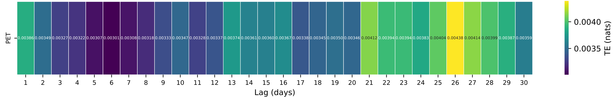
Gauge ID: 12082500 | NISQUALLY RIVER NEAR NATIONAL, WA | PET(t-\tau) \rightarrow Q(t)
