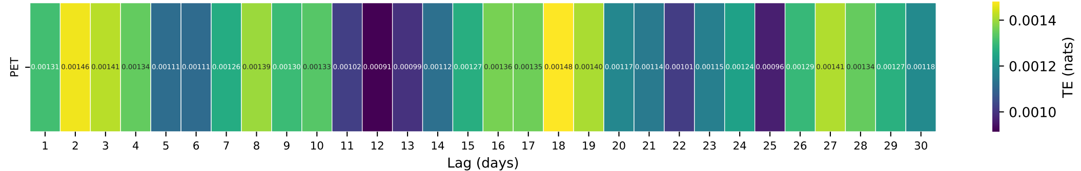
Gauge ID: 06803530 | ROCK CREEK NEAR CERESCO, NEBR. | PET(t-\tau) \rightarrow Q(t)
