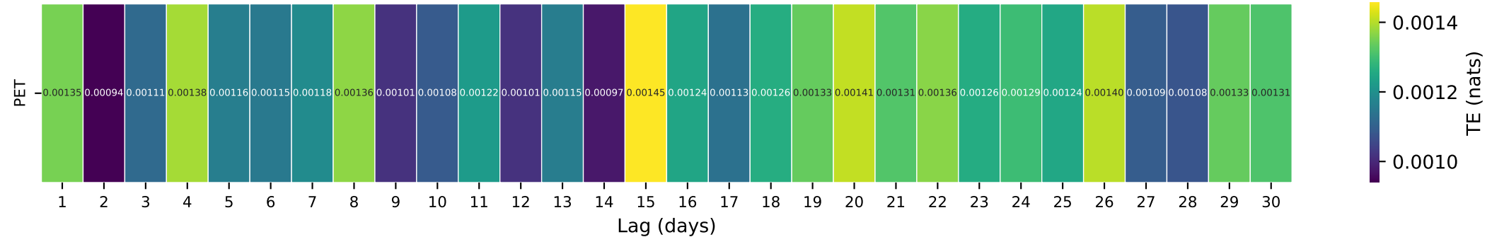
Gauge ID: 02349900 | TURKEY CREEK AT BYROMVILLE, GA | PET(t-\tau) \rightarrow Q(t)
