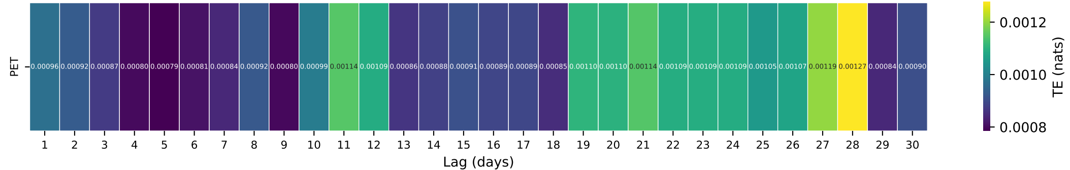
Gauge ID: 02342933 | SOUTH FORK COWIKEE CREEK NEAR BATESVILLE AL | PET(t-\tau) \rightarrow Q(t)
