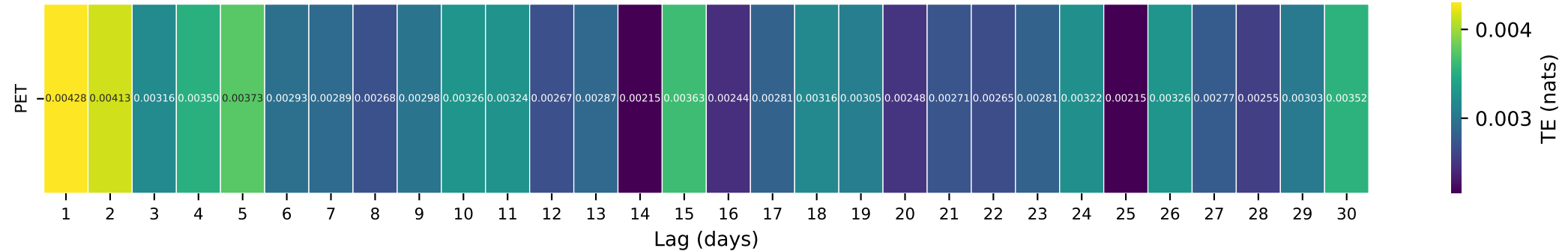
Gauge ID: 10173450 | MAMMOTH CREEK ABV WEST HATCH DITCH, NEAR HATCH, UT | PET(t-\tau) \rightarrow Q(t)
