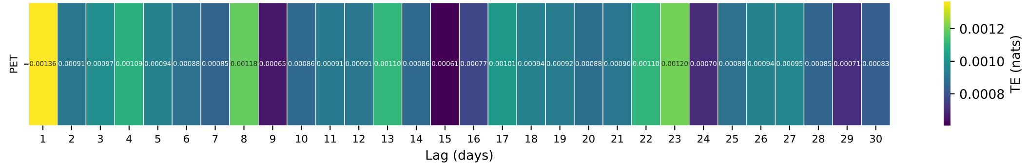
Gauge ID: 01057000 | Little Androscoggin River near South Paris, Maine | PET(t- \tau ) \rightarrow Q(t)
