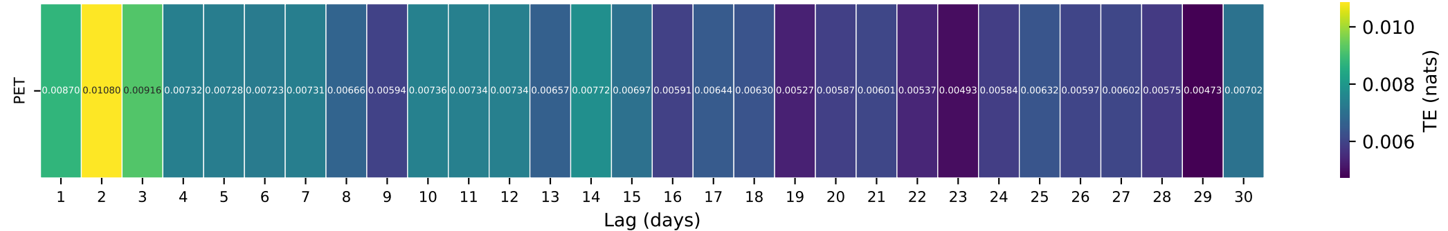
Gauge ID: 13235000 | SF PAYETTE RIVER AT LOWMAN ID | PET(t-\tau) \rightarrow Q(t)
