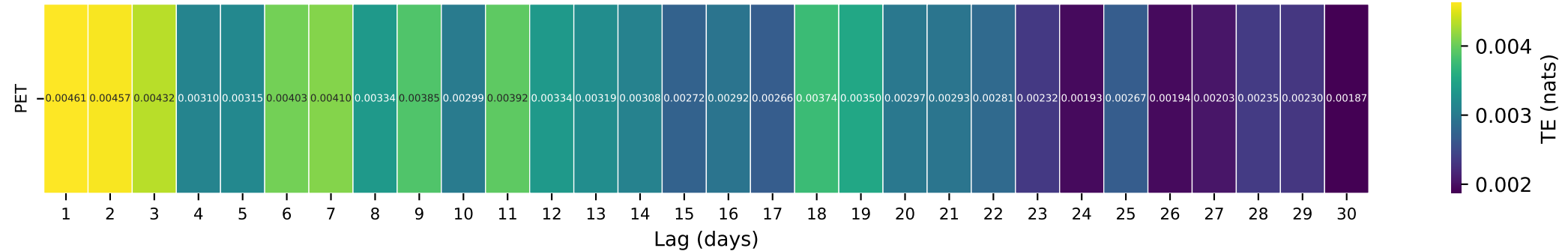
Gauge ID: 04063700 | POPPLE RIVER NEAR FENCE, WI | PET(t-\tau) \rightarrow Q(t)
