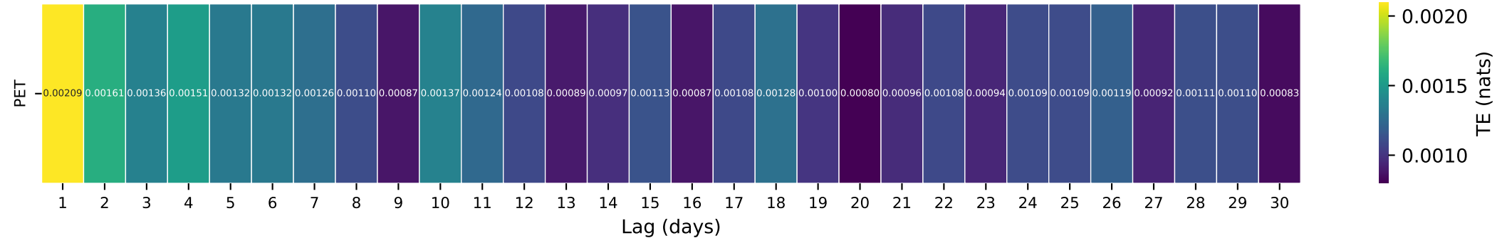
Gauge ID: 01613050 | Tonoloway Creek near Needmore, PA | PET(t-\tau) \rightarrow Q(t)
