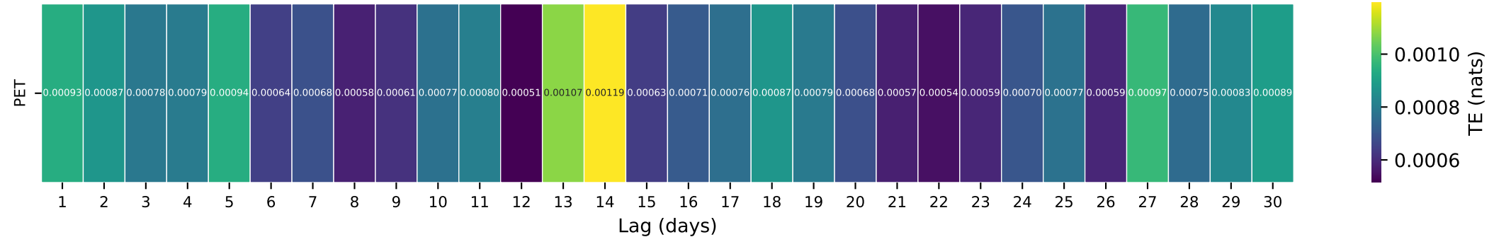
Gauge ID: 02092500 | TRENT RIVER NEAR TRENTON, NC | PET(t-\tau) \rightarrow Q(t)
