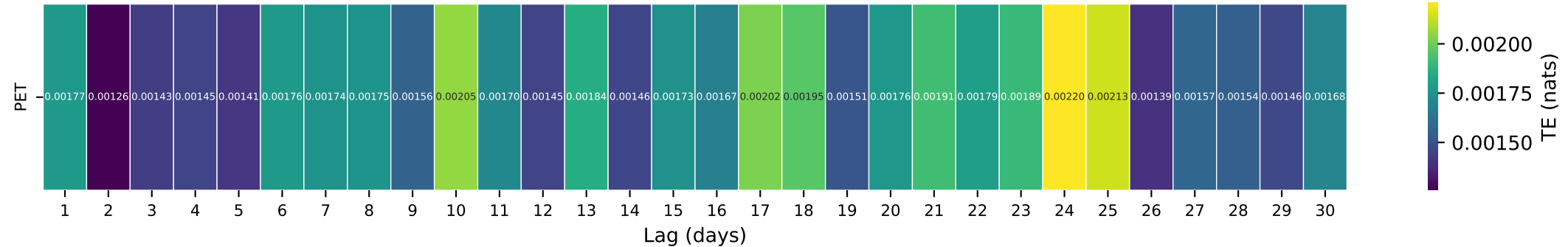
Gauge ID: 01658500 | S F QUANTICO CREEK NEAR INDEPENDENT HILL, VA | PET(t-\tau) \rightarrow Q(t)
