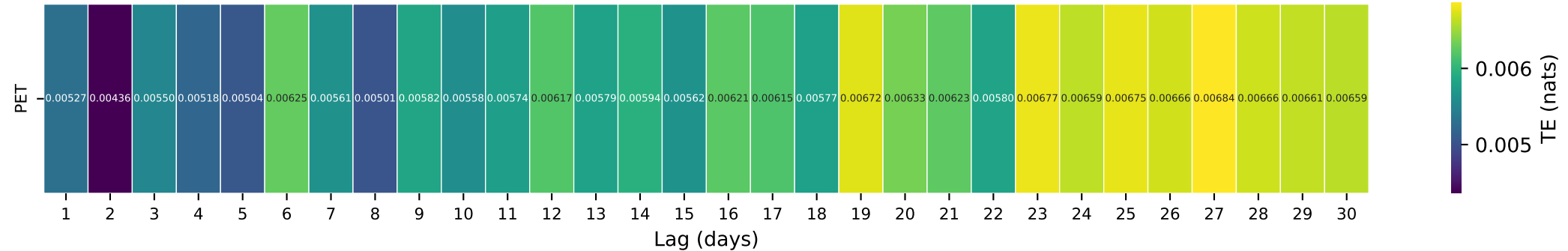
Gauge ID: 03021350 | French Creek near Wattsburg, PA | PET(t-\tau) \rightarrow Q(t)
