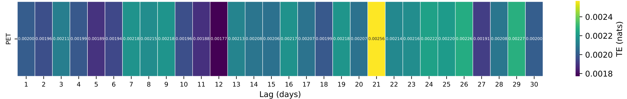
Gauge ID: 09505350 | DRY BEAVER CREEK NEAR RIMROCK, AZ. | PET(t-\tau) \rightarrow Q(t)
