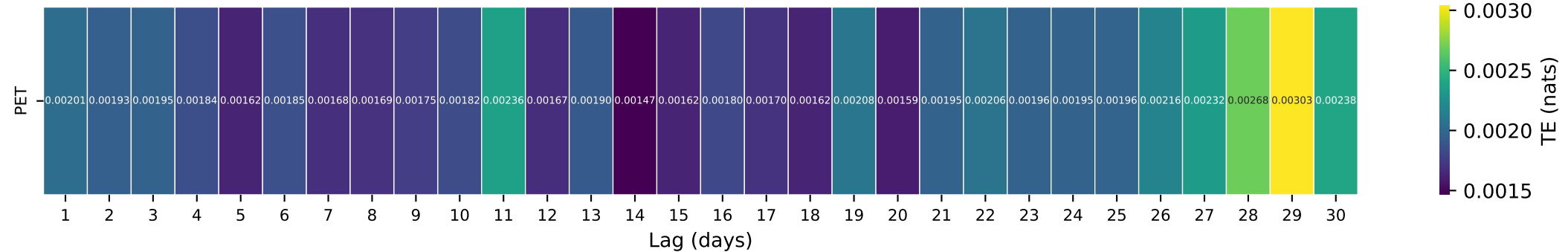
Gauge ID: 02469800 | SATILPA CREEK NEAR COFFEEVILLE AL | PET(t-\tau) \rightarrow Q(t)
