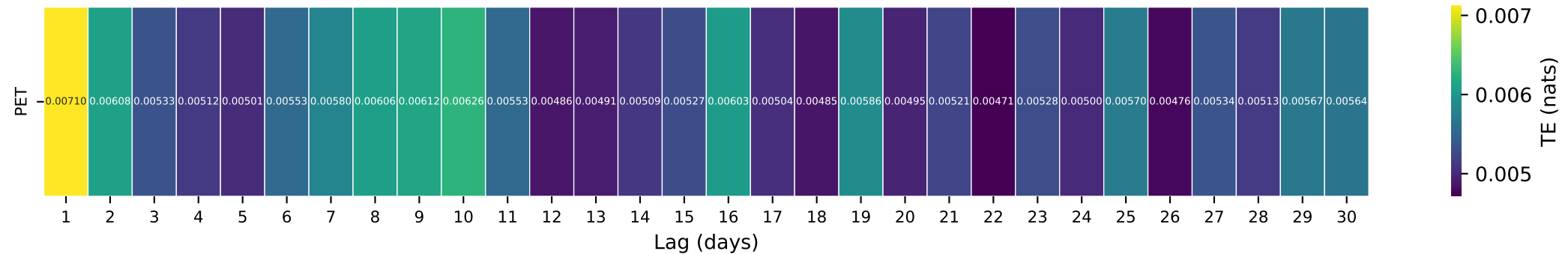
Gauge ID: 06291500 | Lodge Grass Cr ab Willow C Div nr Wyola MT | PET( t-\tau ) \rightarrow Q( t )
