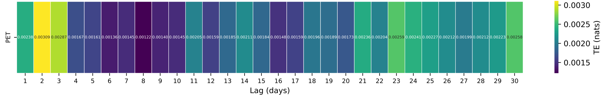
Gauge ID: 04122500 | PERE MARQUETTE RIVER AT SCOTTVILLE, MI | PET(t-\tau) \rightarrow Q(t)
