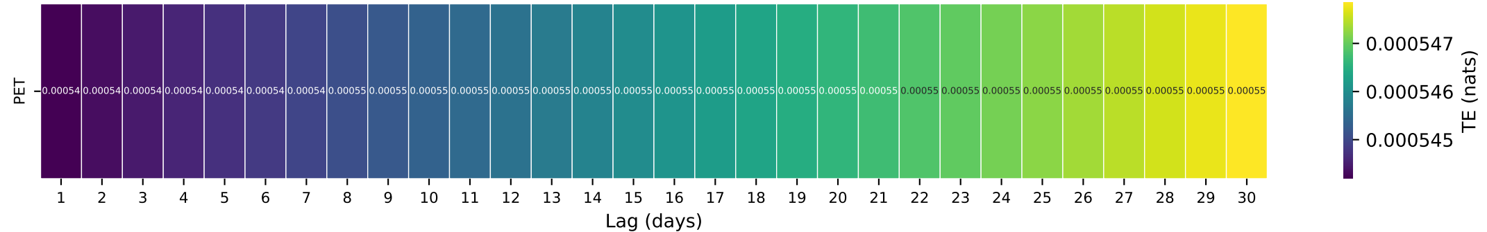
Gauge ID: 14362250 | STAR GULCH NEAR RUCH, OR. | PET(t-\tau) \rightarrow Q(t)
