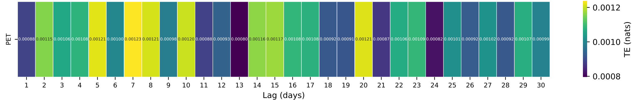
Gauge ID: 09480000 | SANTA CRUZ RIVER NEAR LOCHIEL, AZ. | PET(t-\tau) \rightarrow Q(t)
