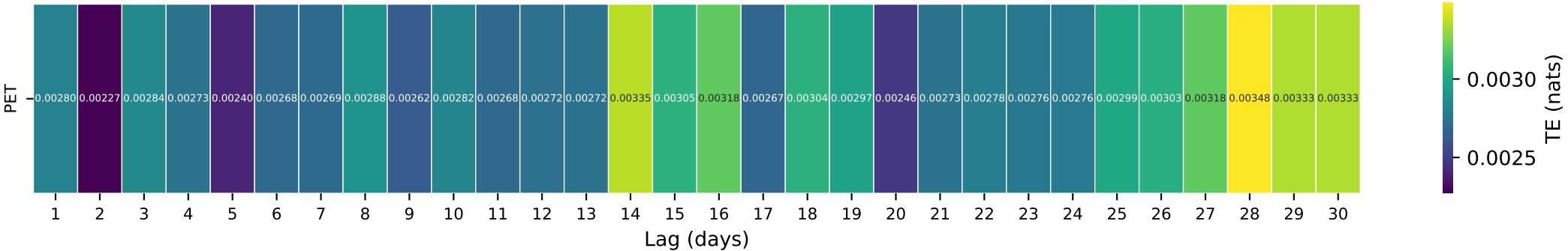
Gauge ID: 11528700 | SF TRINITY R BL HYAMPOM CA | PET(t-τ) → Q(t)
