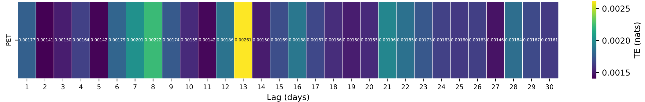
Gauge ID: 01550000 | Lycoming Creek near Trout Run, PA | PET(t-\tau) \rightarrow Q(t)
