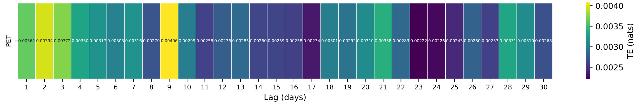
Gauge ID: 09378630 | RECAPTURE CREEK NEAR BLANDING, UT | PET(t-\tau) \rightarrow Q(t)
