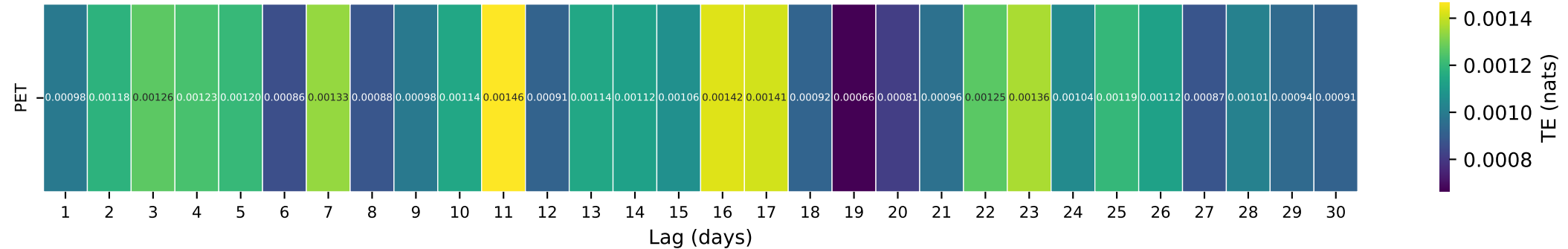
Gauge ID: 02372250 | PATSALIGA CREEK NEAR BRANTLEY AL | PET(t-\tau) \rightarrow Q(t)
