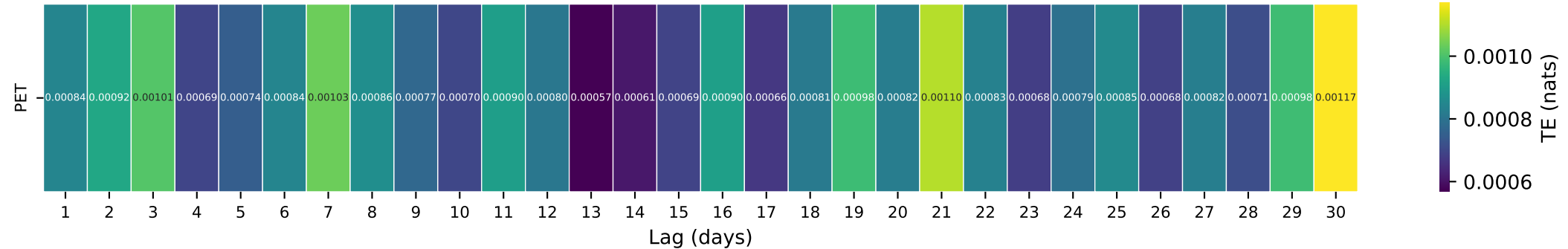
Gauge ID: 08066200 | Long King Ck at Livingston, TX | PET(t- \tau ) \rightarrow Q(t)
