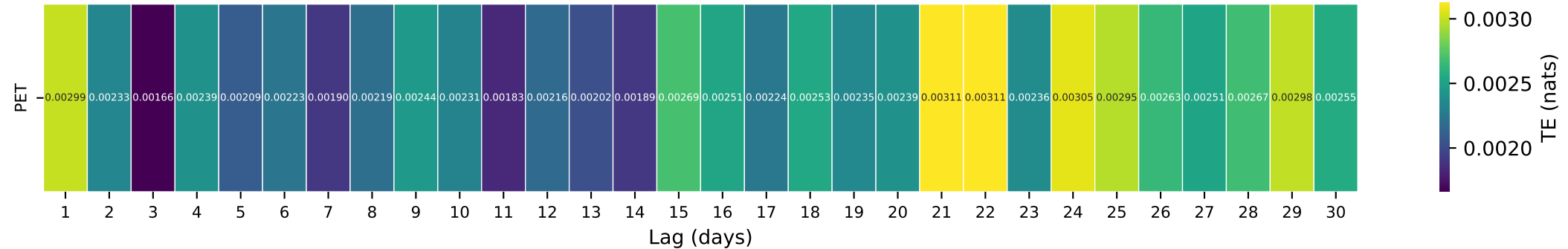
Gauge ID: 02472000 | LEAF RIVER NR COLLINS, MS | PET(t-\tau) \rightarrow Q(t)
