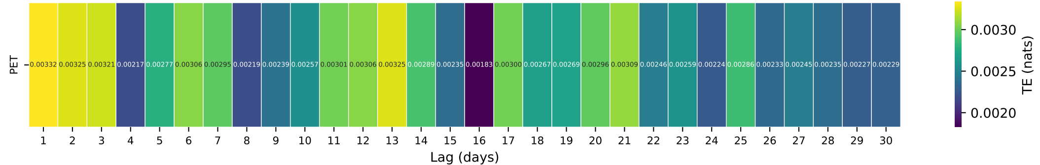
Gauge ID: 01144000 | WHITE RIVER AT WEST HARTFORD, VT | PET(t-\tau) \rightarrow Q(t)
