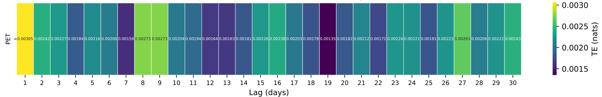
Gauge ID: 02324400 | FENHOLLOWAY RIVER NEAR FOLEY, FLA. | PET(t-\tau) \rightarrow Q(t)
