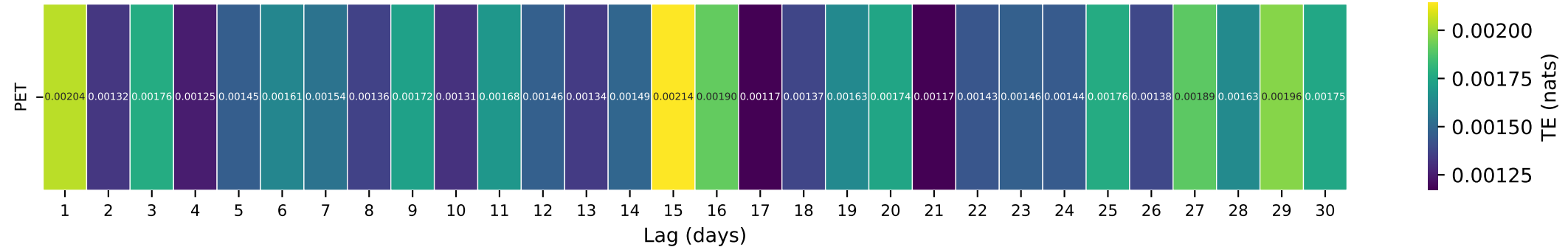
Gauge ID: 05525500 | SUGAR CREEK AT MILFORD, IL | PET(t-\tau) \rightarrow Q(t)
