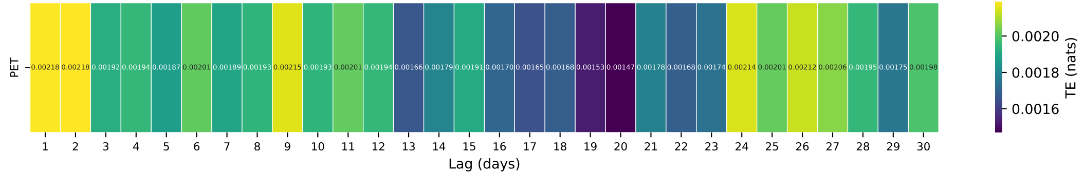
Gauge ID: 11523200 | TRINITY R AB COFFEE C NR TRINITY CTR CA | PET(t- \tau ) \rightarrow Q(t)
