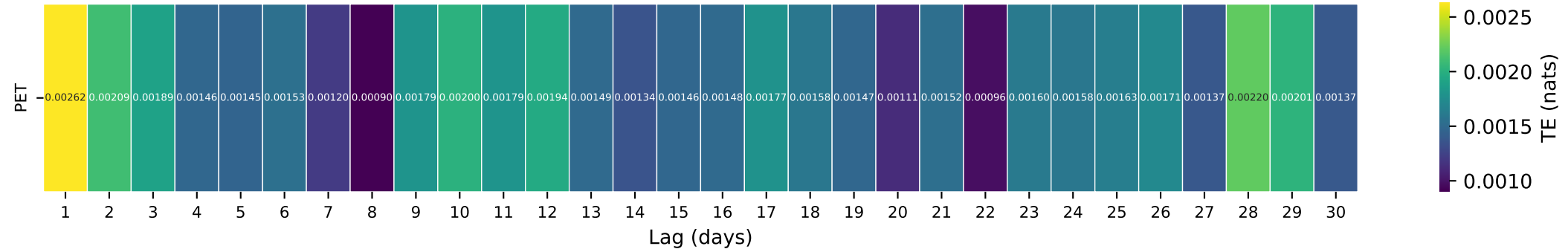
Gauge ID: 02296500 | CHARLIE CREEK NEAR GARDNER FL | PET(t-\tau) \rightarrow Q(t)
