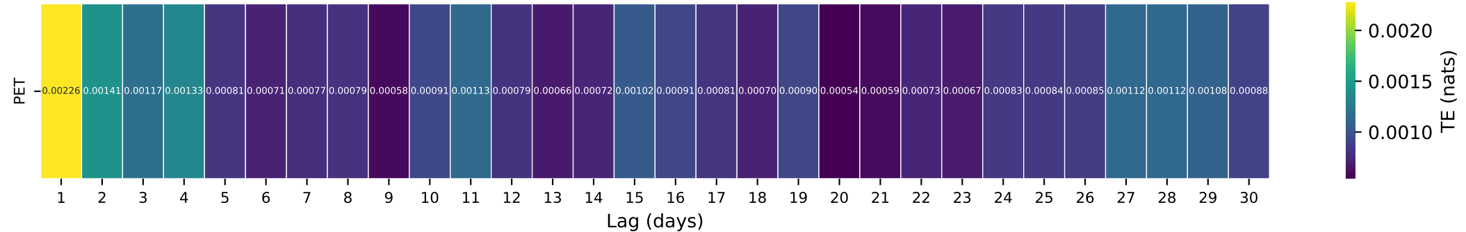
Gauge ID: 06339500 | KNIFE RIVER NR GOLDEN VALLEY, ND | PET(t-\tau) \rightarrow Q(t)
