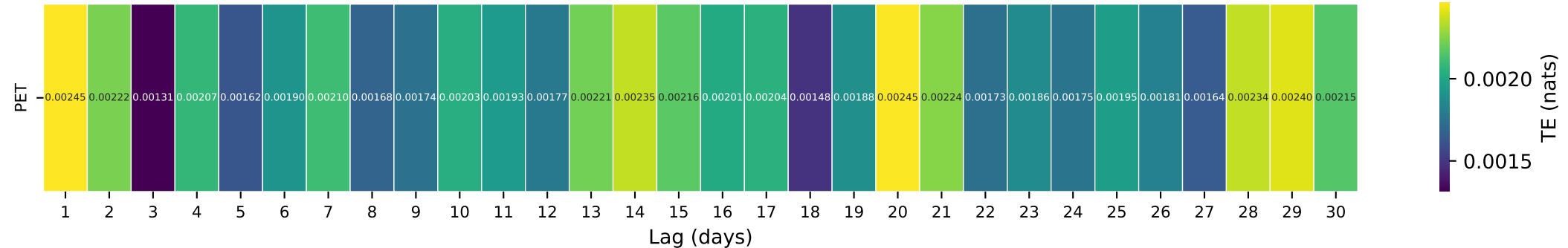
Gauge ID: 02231342 | FT DRUM CREEK AT SUNSHINE ST PKY NEAR FT DRUM, FL | PET(t-\tau) \rightarrow Q(t)
