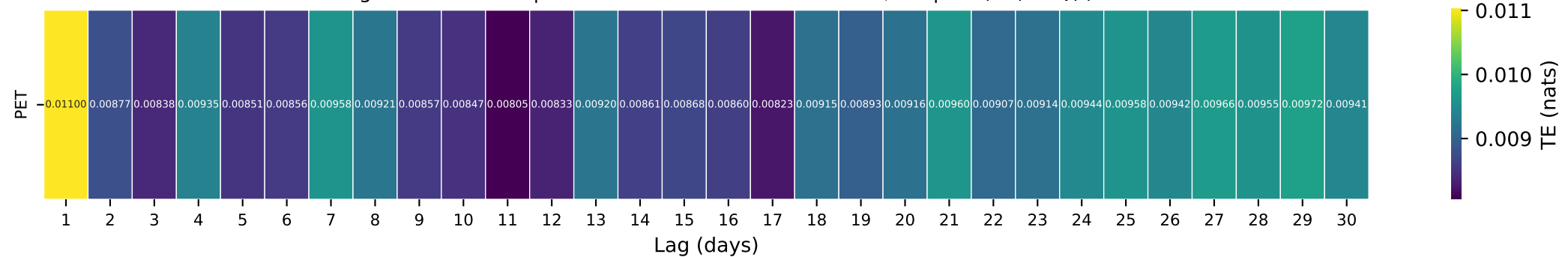
Gauge ID: 14400000 | CHETCO RIVER NEAR BROOKINGS, OR | PET(t-\tau) \rightarrow Q(t)
