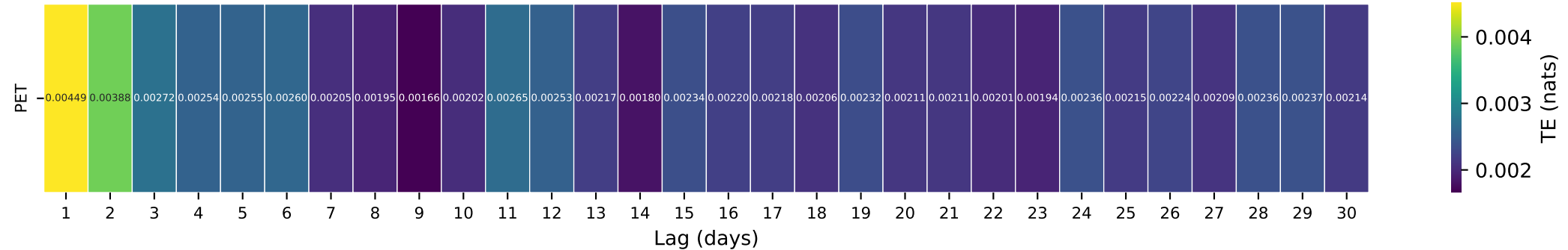
Gauge ID: 06464500 | KEYA PAHA R AT WEWELA SD | PET(t- \tau ) \rightarrow Q(t)
