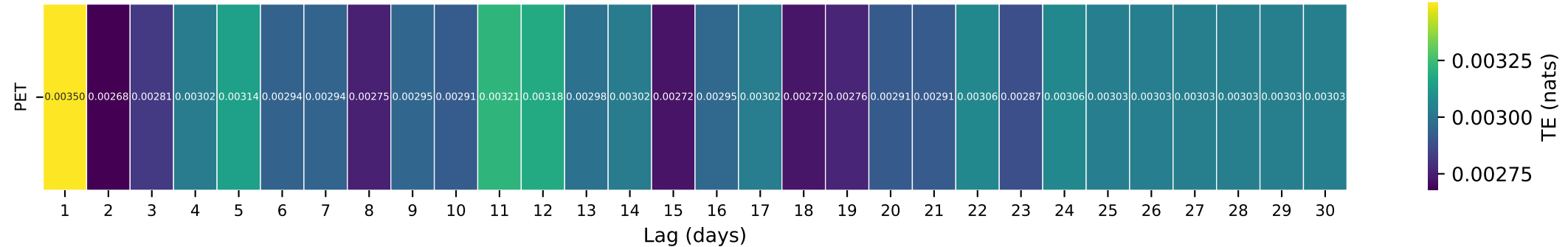
Gauge ID: 12073500 | HUGE CREEK NEAR WAUNA, WA | PET(t-\tau) \rightarrow Q(t)
