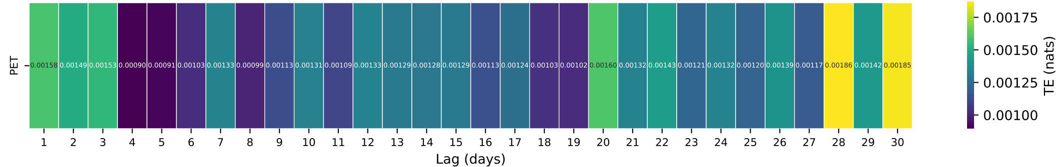
Gauge ID: 08380500 | GALLINAS CREEK NEAR MONTEZUMA, NM | PET(t-\tau) \rightarrow Q(t)
