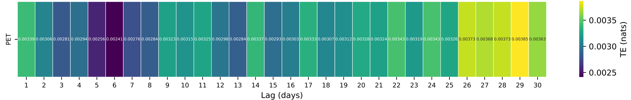
Gauge ID: 12117000 | TAYLOR CREEK NEAR SELLECK, WA | PET(t-\tau) \rightarrow Q(t)
