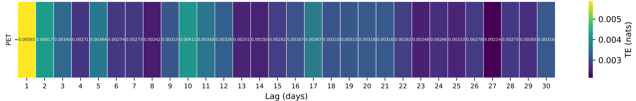
Gauge ID: 10234500 | BEAVER RIVER NEAR BEAVER, UT | PET(t-\tau) \rightarrow Q(t)
