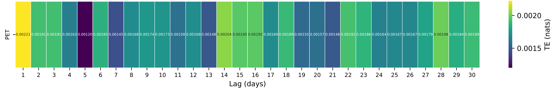
Gauge ID: 05592050 | ROBINSON CREEK NEAR SHELBYVILLE, IL | PET(t-\tau) \rightarrow Q(t)
