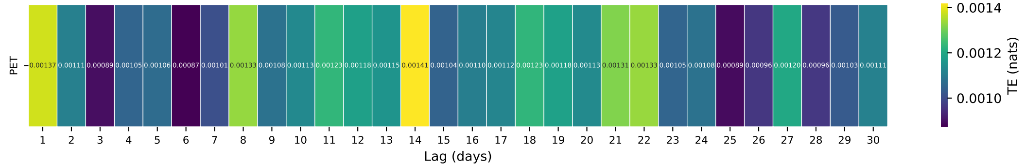
Gauge ID: 01539000 | Fishing Creek near Bloomsburg, PA | PET(t-\tau) \rightarrow Q(t)
