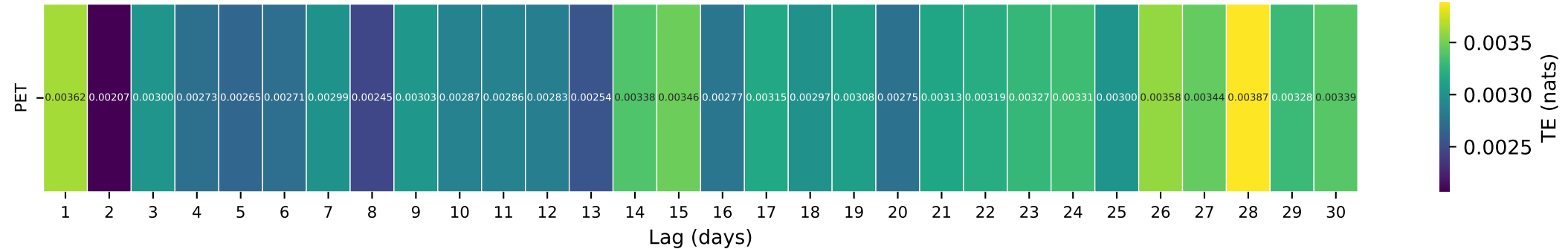
Gauge ID: 01487000 | NANTICOKE RIVER NEAR BRIDGEVILLE, DE | PET(t-\tau) \rightarrow Q(t)
