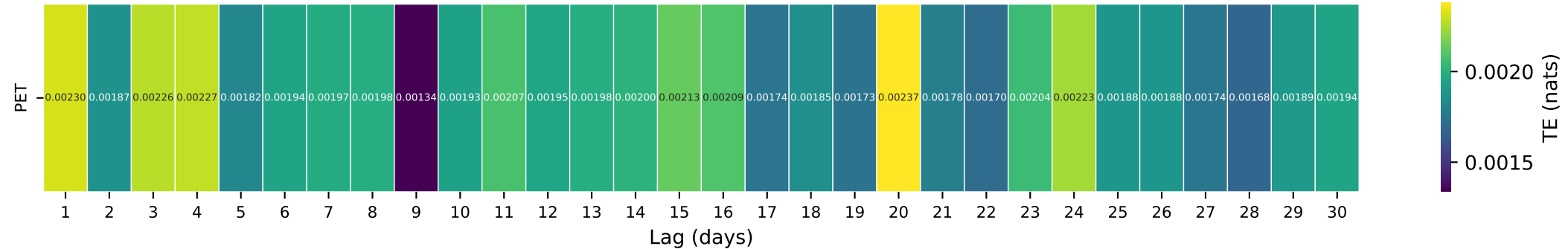
Gauge ID: 03504000 | NANTAHALA RIVER NEAR RAINBOW SPRINGS, NC | PET(t-\tau) \rightarrow Q(t)
