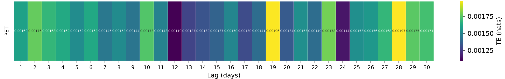
Gauge ID: 01591400 | CATTAIL CREEK NEAR GLENWOOD, MD | PET(t-\tau) \rightarrow Q(t)
