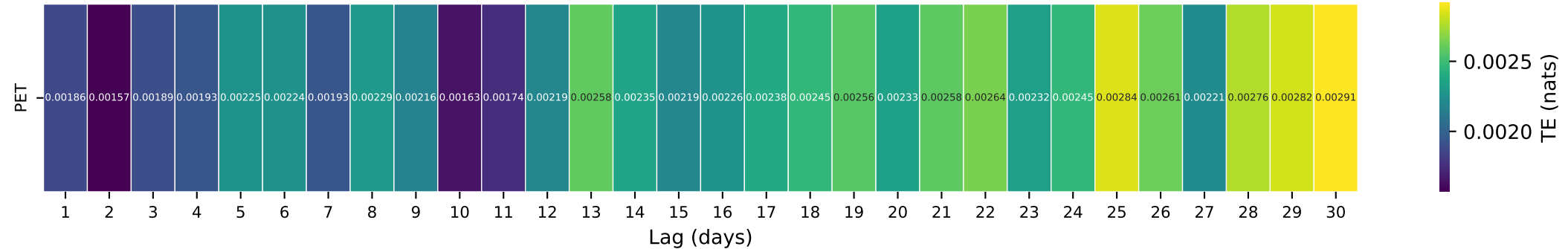
Gauge ID: 01639500 | BIG PIPE CREEK AT BRUCEVILLE, MD | PET(t-\tau) \rightarrow Q(t)
