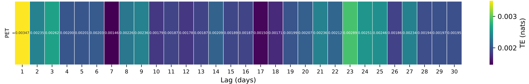
Gauge ID: 02479300 | RED CREEK AT VESTRY, MS | PET(t-\tau) \rightarrow Q(t)
