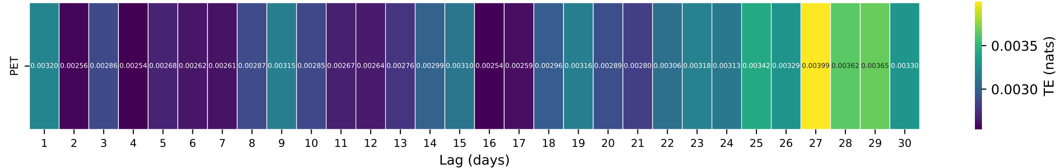
Gauge ID: 02464000 | NORTH RIVER NEAR SAMANTHA AL | PET(t- \tau ) \rightarrow Q(t)
