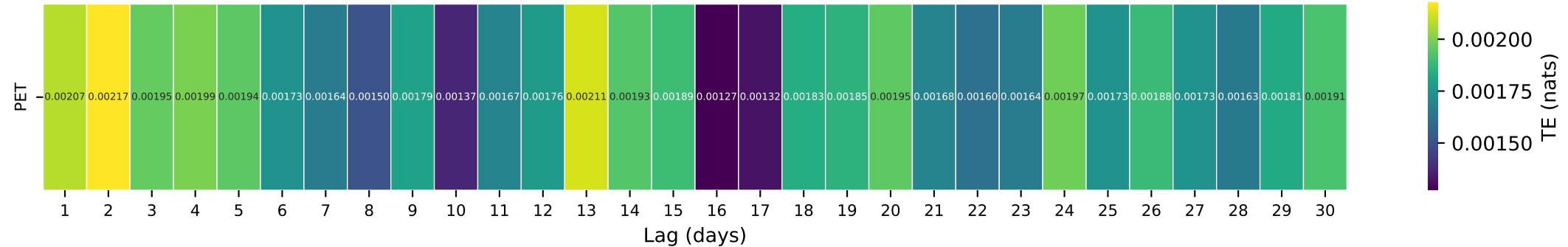
Gauge ID: 08164600 | Garcitas Ck nr Inez, TX | PET(t- \tau ) \rightarrow Q(t)
