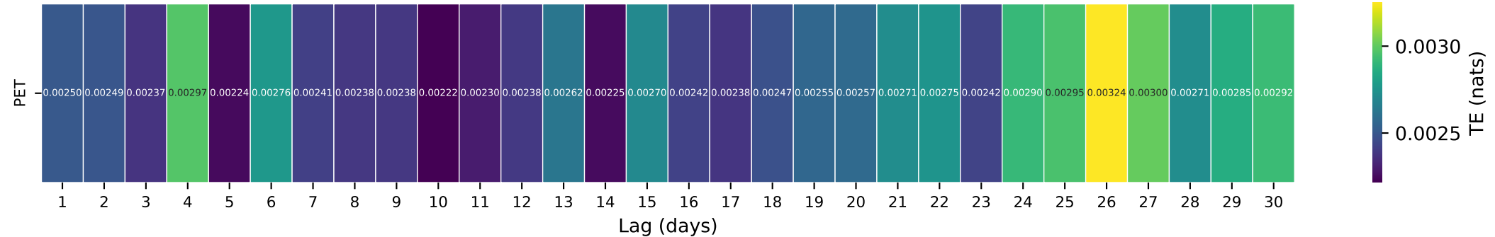
Gauge ID: 14216500 | MUDDY CREEK BELOW CLEAR CREEK NEAR COUGAR, WA | PET(t-\tau) \rightarrow Q(t)
