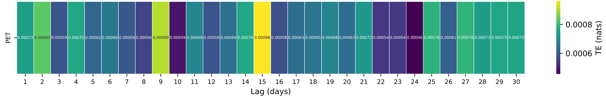
Gauge ID: 06903400 | Chariton River near Chariton, IA | PET(t-\tau) \rightarrow Q(t)
