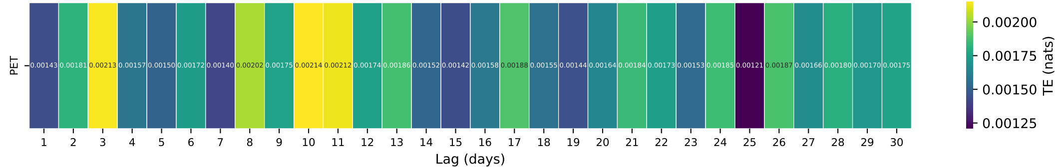
Gauge ID: 01567500 | Bixler Run near Loysville, PA | PET(t- \tau ) \rightarrow Q(t)
