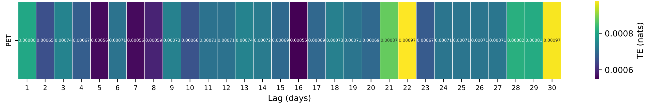
Gauge ID: 09505200 | WET BEAVER CREEK NEAR RIMROCK, AZ. | PET(t-\tau) \rightarrow Q(t)
