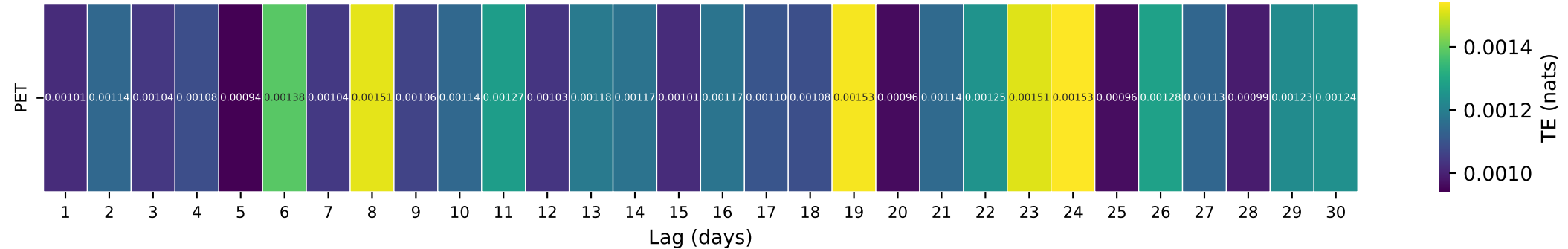
Gauge ID: 08176900 | Coleta Ck at Arnold Rd nr Schroeder, TX | PET(t- \tau ) \rightarrow Q(t)
