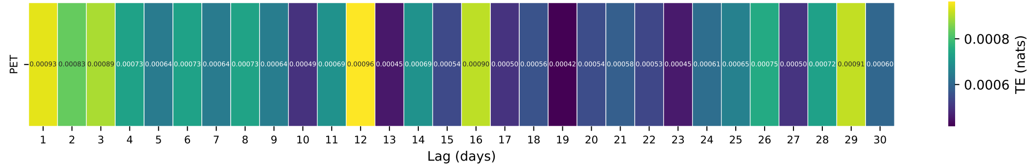
Gauge ID: 02108000 | NORTHEAST CAPE FEAR RIVER NEAR CHINQUAPIN, NC | PET(t-\tau) \rightarrow Q(t)
