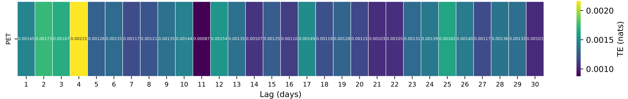
Gauge ID: 02371500 | CONECUH RIVER AT BRANTLEY AL | PET(t-\tau) \rightarrow Q(t)
