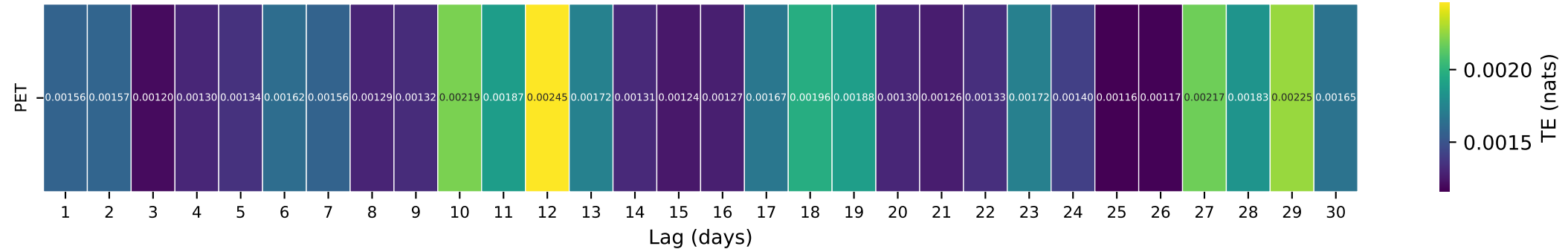
Gauge ID: 10249300 | S TWIN R NR ROUND MOUNTAIN, NV | PET(t-\tau) \rightarrow Q(t)
