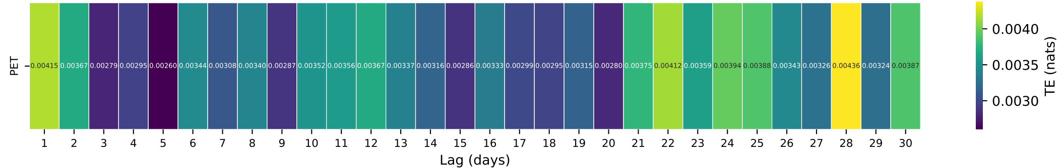
Gauge ID: 06934000 | Gasconade River near Rich Fountain, MO | PET(t-\tau) \rightarrow Q(t)
