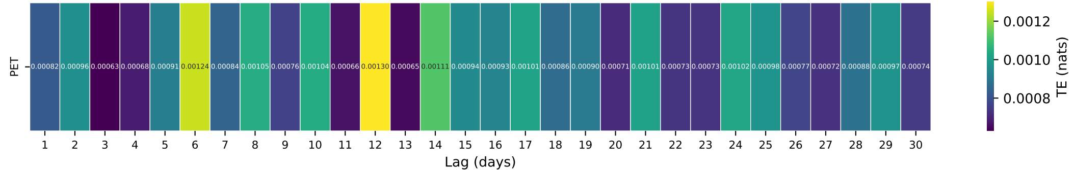
Gauge ID: 01620500 | NORTH RIVER NEAR STOKESVILLE, VA | PET(t-\tau) \rightarrow Q(t)
