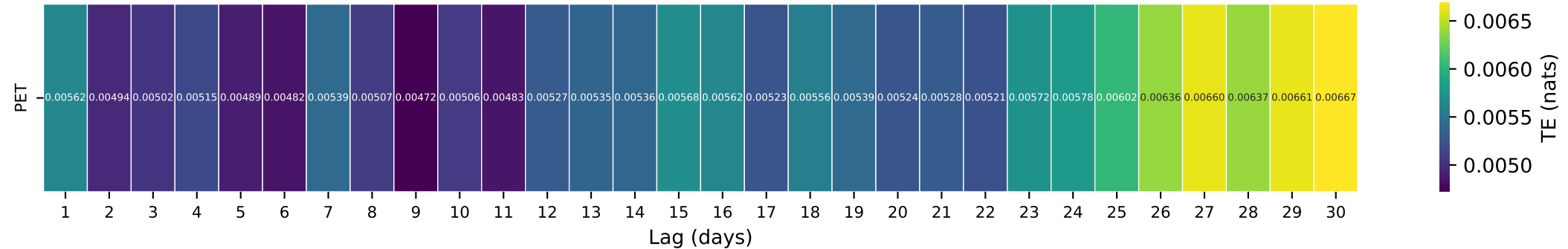
Gauge ID: 11480390 | MAD R AB RUTH RES NR FOREST GLEN CA | PET(t- \tau ) \rightarrow Q(t)
