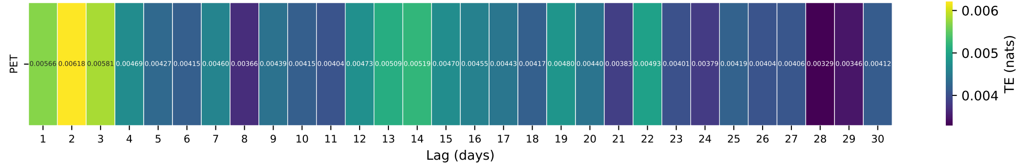
Gauge ID: 10172800 | SOUTH WILLOW CREEK NEAR GRANTSVILLE, UT | PET(t-\tau) \rightarrow Q(t)
