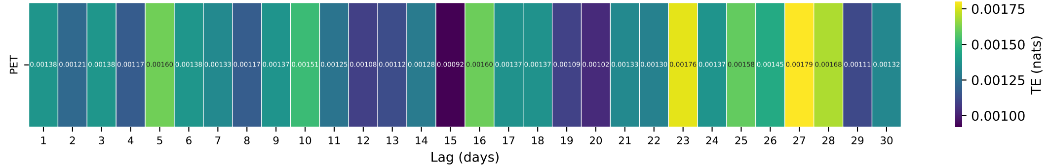
Gauge ID: 03364500 | CLIFTY CREEK AT HARTSVILLE, IN | PET(t-\tau) \rightarrow Q(t)
