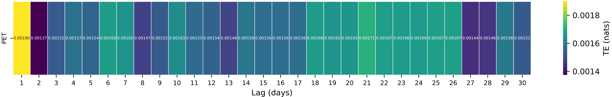
Gauge ID: 09508300 | WET BOTTOM CREEK NEAR CHILDS, AZ. | PET(t-\tau) \rightarrow Q(t)
