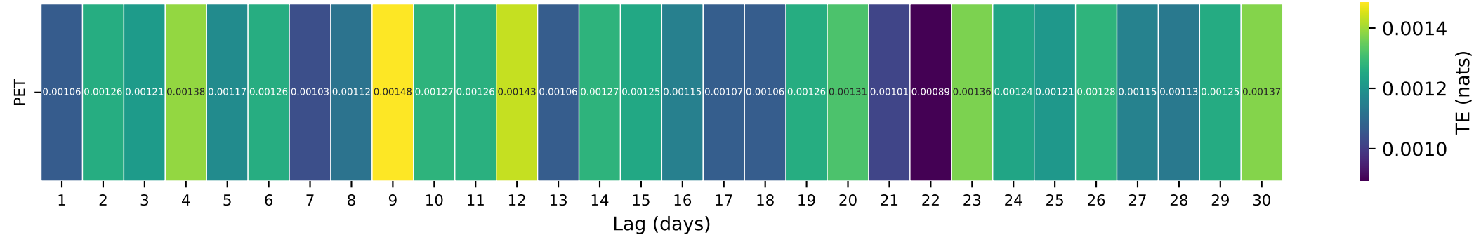
Gauge ID: 08194200 | San Casimiro Ck nr Freer, TX | PET(t- \tau ) \rightarrow Q(t)
