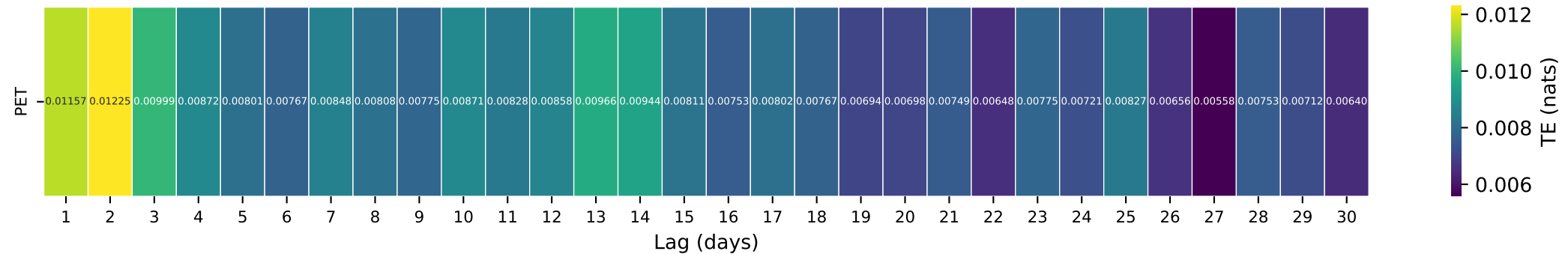
Gauge ID: 12383500 | Big Knife Creek near Arlee MT | PET(t-\tau) \rightarrow Q(t)
