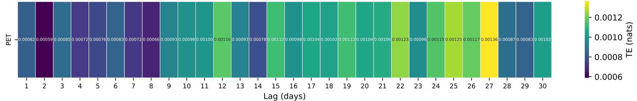
Gauge ID: 02011460 | BACK CREEK NEAR SUNRISE, VA | PET(t-\tau) \rightarrow Q(t)
