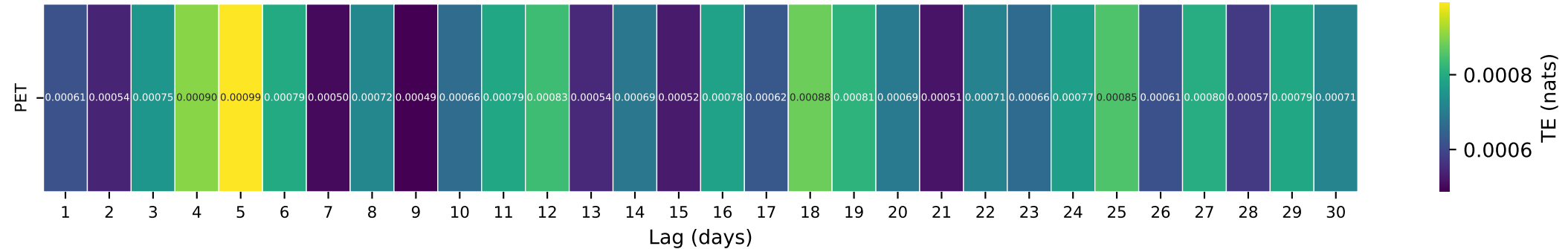
Gauge ID: 08158810 | Bear Ck bl FM 1826 nr Driftwood, TX | PET(t-\tau) \rightarrow Q(t)
