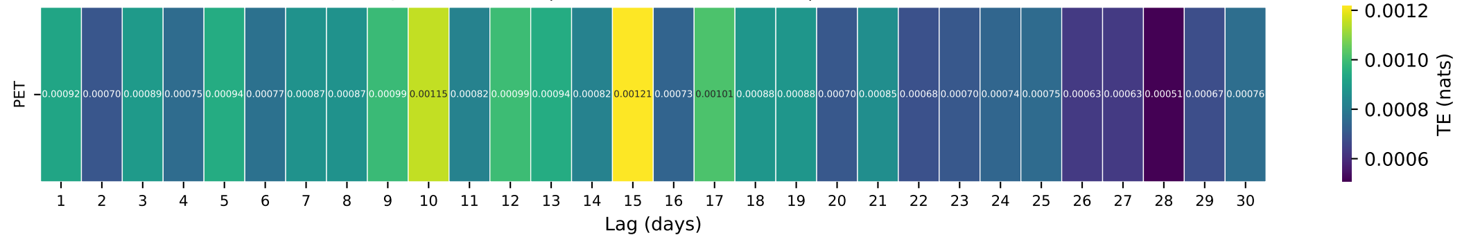
Gauge ID: 08178880 | Medina Rv at Bandera, TX | PET(t-\tau) \rightarrow Q(t)
