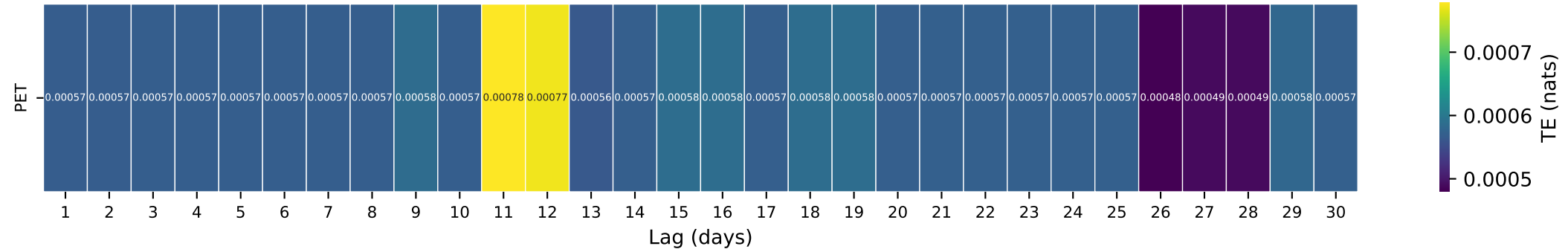
Gauge ID: 12020000 | CHEHALIS RIVER NEAR DOTY, WA | PET(t-\tau) \rightarrow Q(t)
