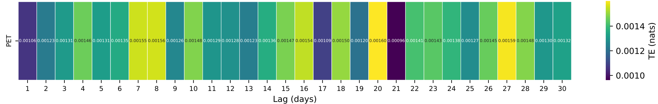
Gauge ID: 04213075 | Brandy Run near Girard, PA | PET(t- \tau ) \rightarrow Q(t)
