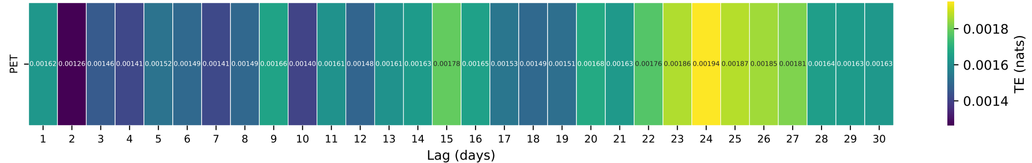
Gauge ID: 11383500 | DEER C NR VINA CA | PET(t- \tau ) \rightarrow Q(t)
