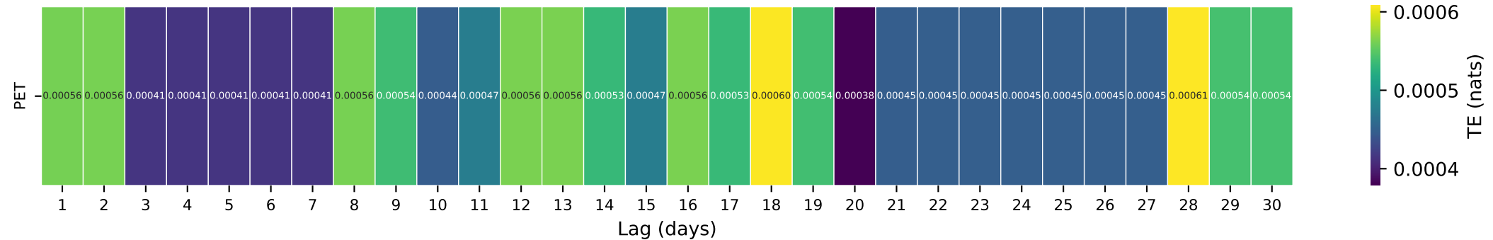
Gauge ID: 10310500 | CLEAR CREEK NEAR CARSON CITY, NV | PET(t-\tau) \rightarrow Q(t)
