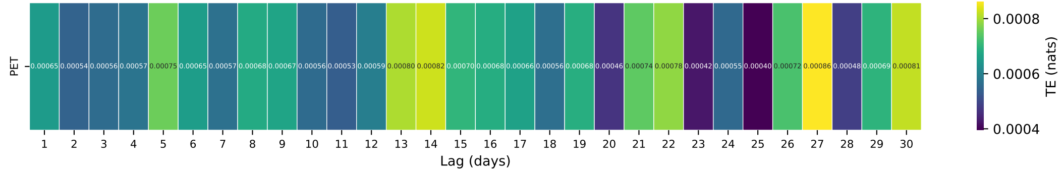
Gauge ID: 02069700 | SOUTH MAYO RIVER NEAR NETTLERIDGE, VA | PET(t-\tau) \rightarrow Q(t)
