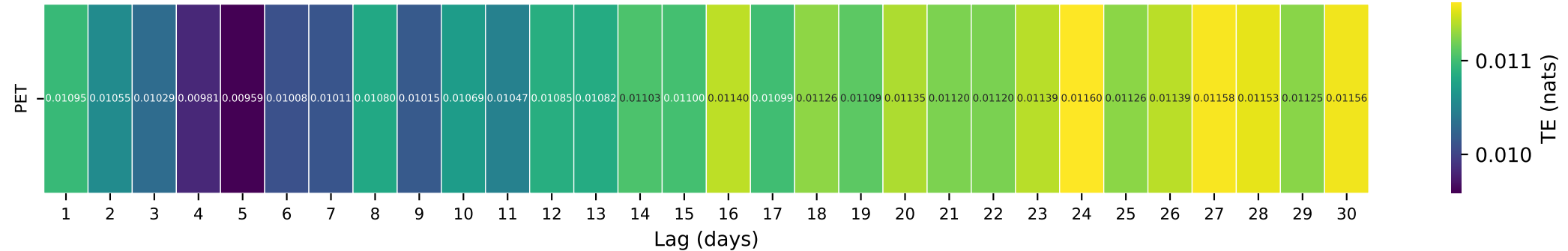
Gauge ID: 14306500 | ALSEA RIVER NEAR TIDEWATER, OR | PET(t-\tau) \rightarrow Q(t)
