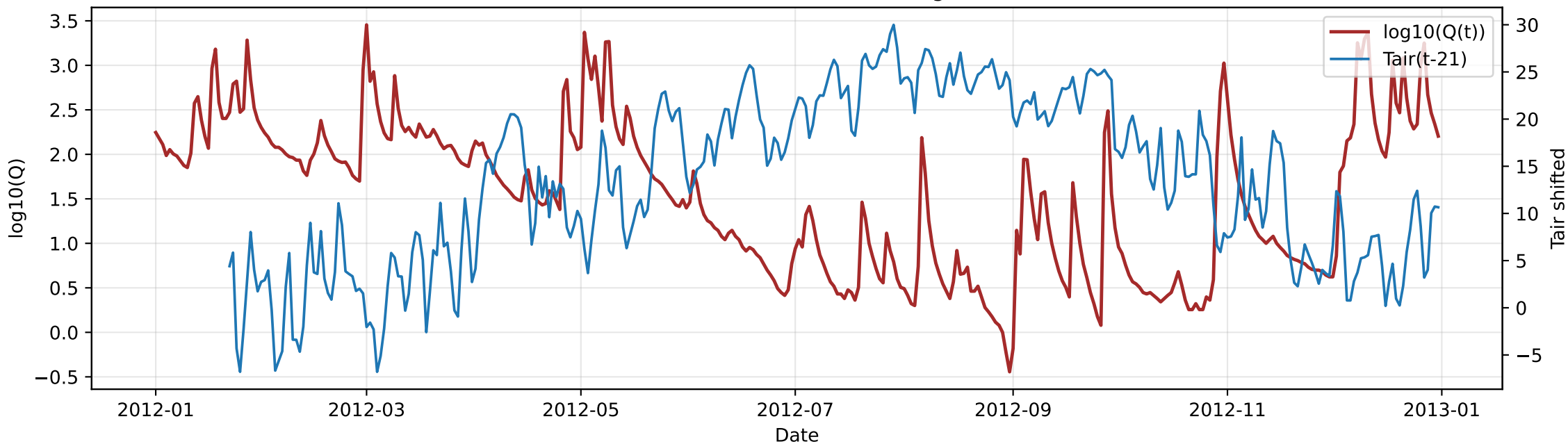
Basin 03159540: Tair(t-21) and log10(Q(t))
