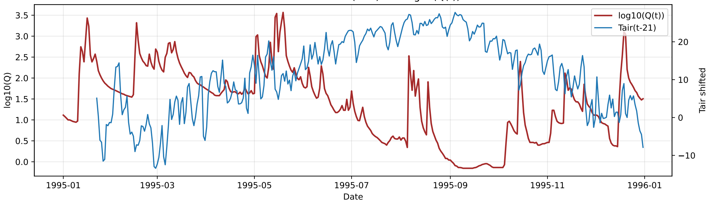
Basin 03159540: Tair(t-21) and log10(Q(t))
