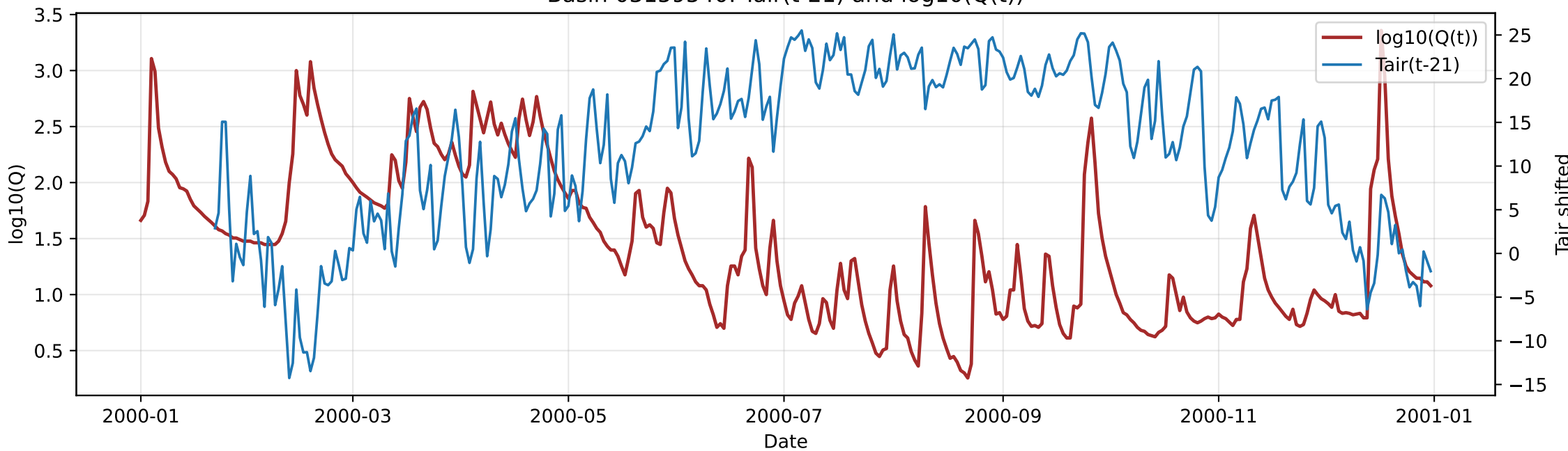
Basin 03159540: Tair(t-21) and log10(Q(t))
