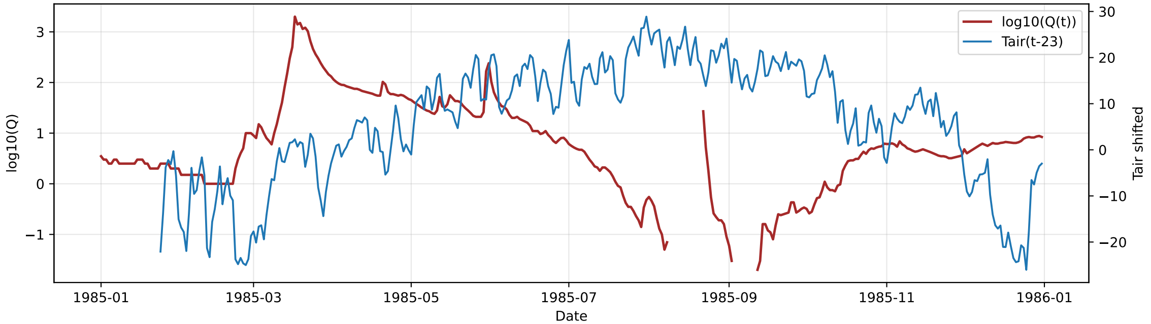
Basin 06353000: Tair(t-23) and log10(Q(t))
