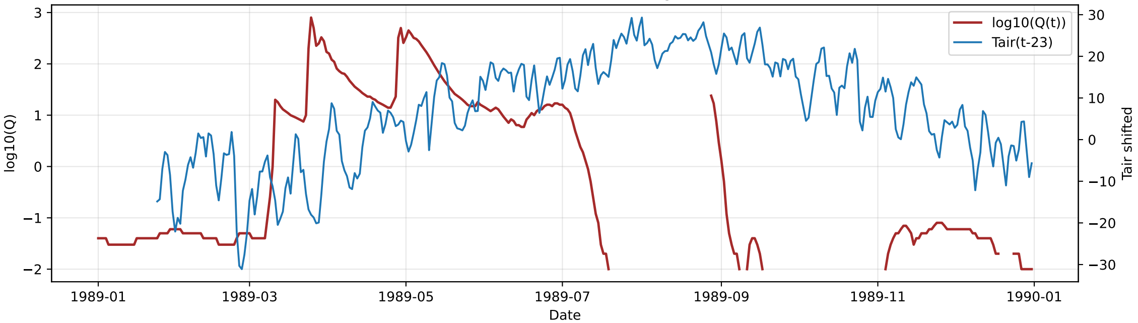
Basin 06353000: Tair(t-23) and log10(Q(t))
