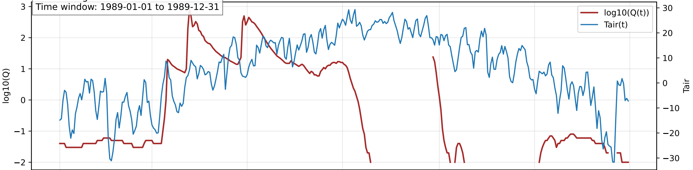
Basin 06353000: Tair(t) and log10(Q(t))
