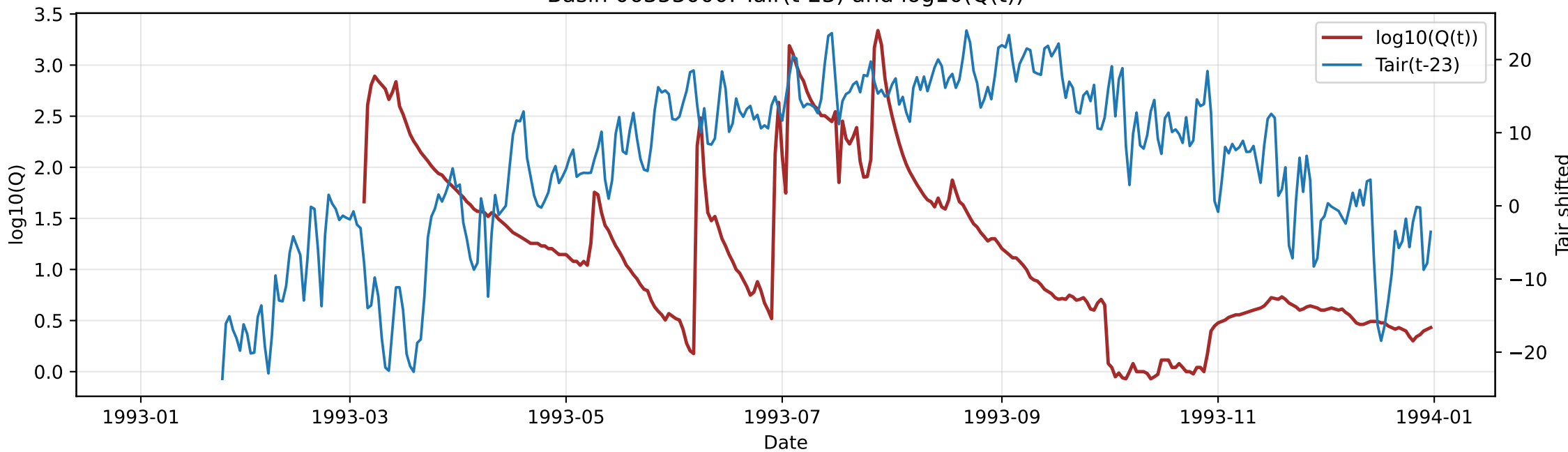
Basin 06353000: Tair(t-23) and log10(Q(t))
