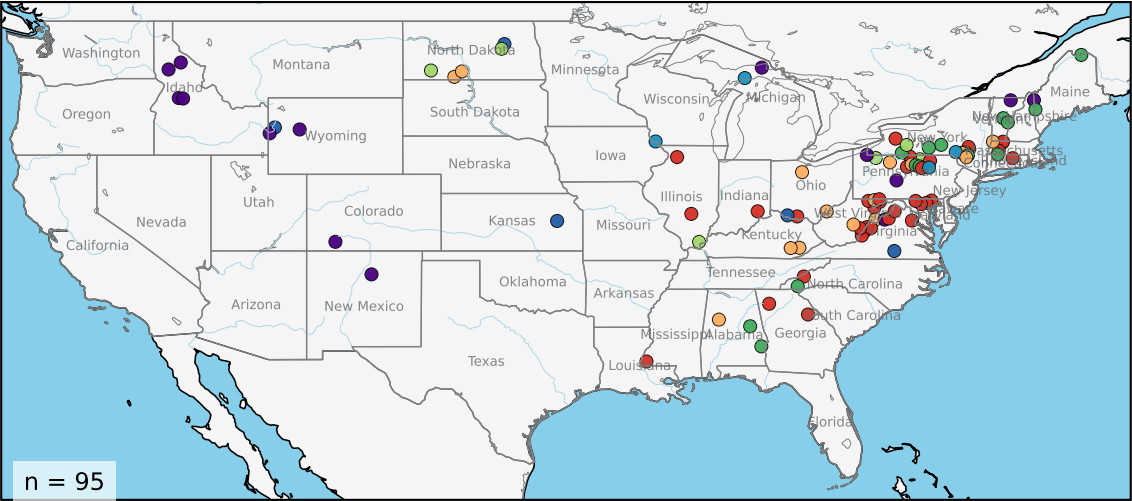
Tair-dominant basins: Peak Lag
