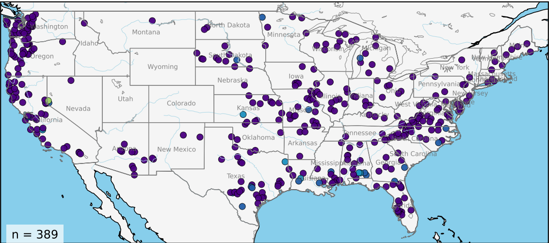
PRCP-dominant basins: Peak Lag
