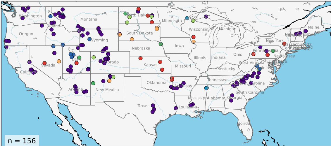
SRAD-dominant basins: Peak Lag
