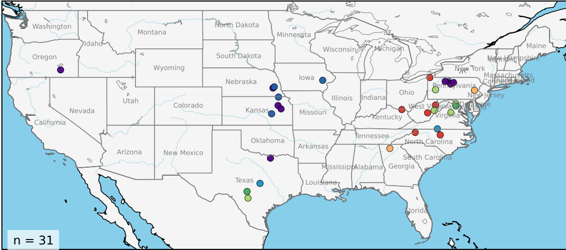
VP-dominant basins
