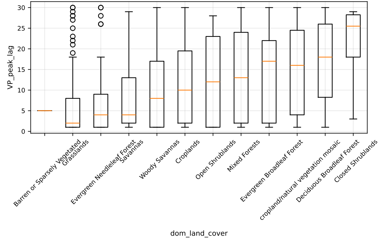
VP_peak_lag by dom_land_cover
