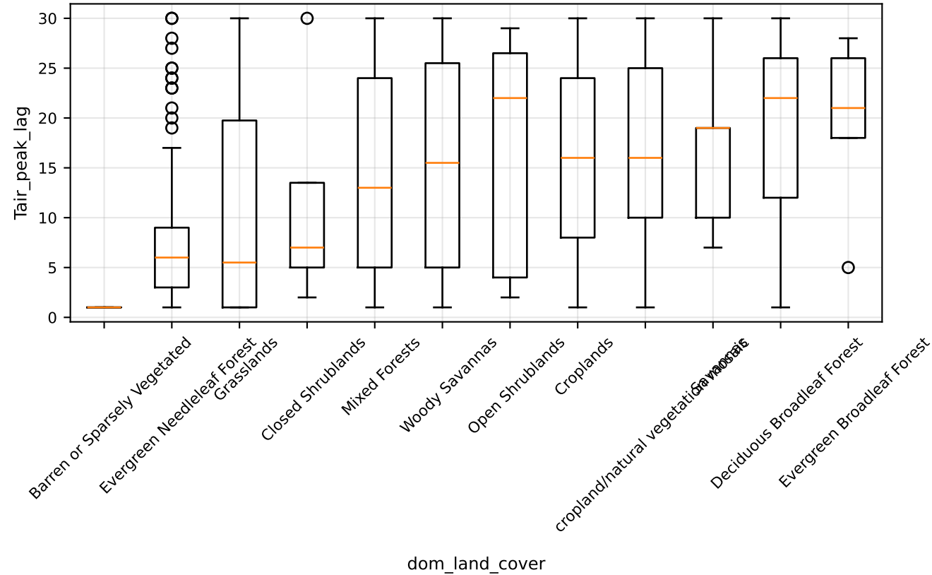
Tair_peak_lag by dom_land_cover
