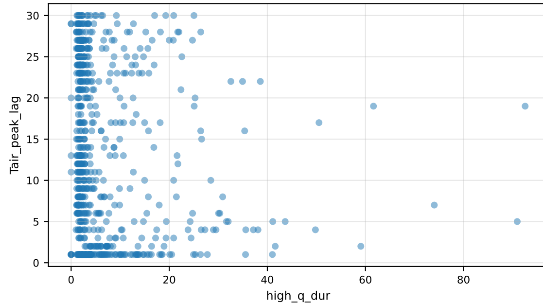
Tair_peak_lag vs high_q_dur
