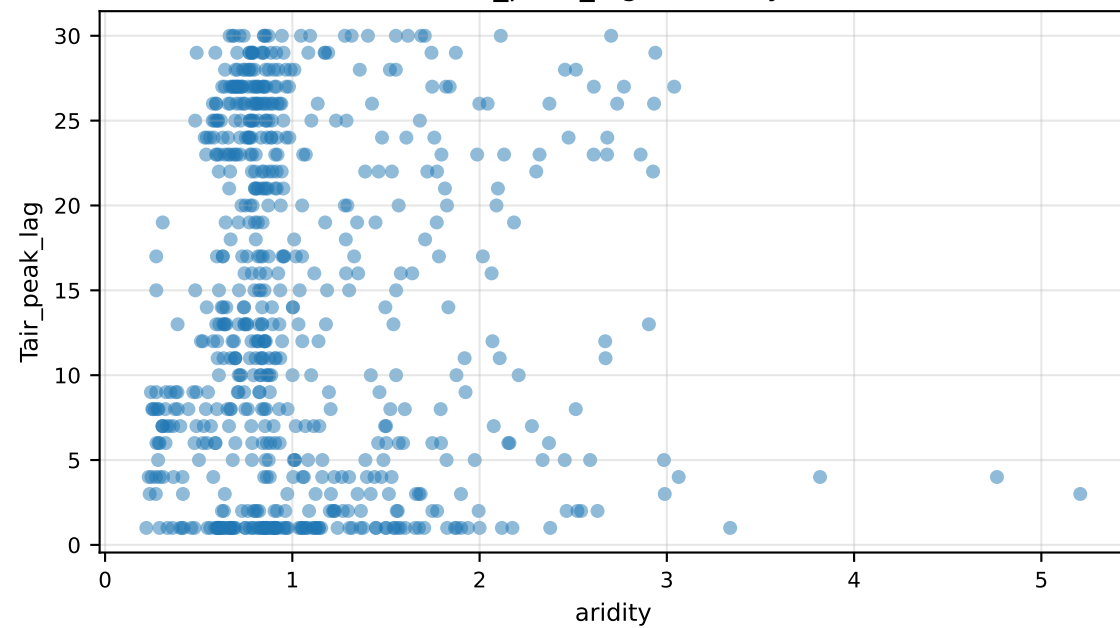
Tair_peak_lag vs aridity
