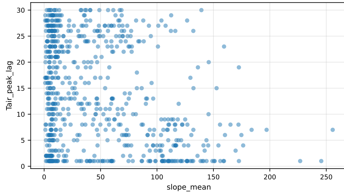
Tair_peak_lag vs slope_mean
