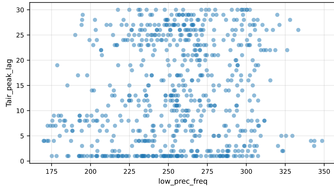
Tair_peak_lag vs low_prec_freq
