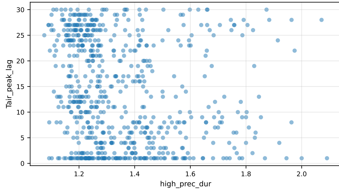
Tair_peak_lag vs high_prec_dur
