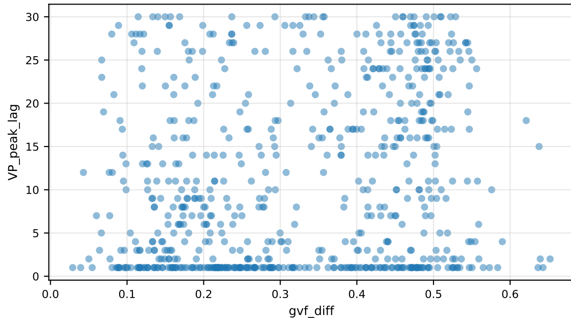
VP_peak_lag vs gvf_diff
