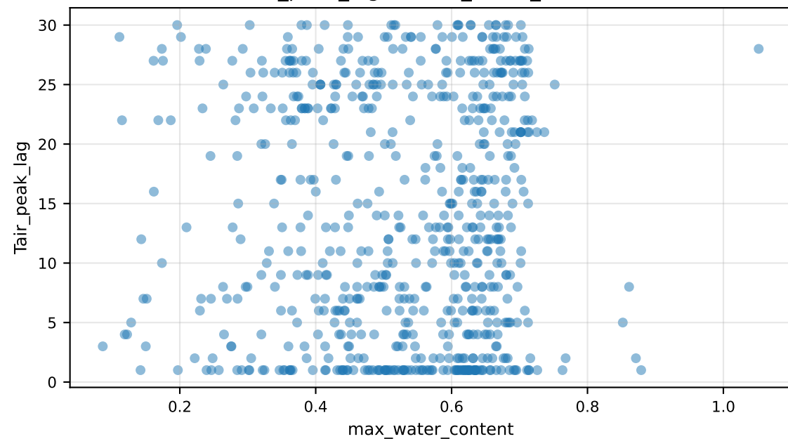
Tair_peak_lag vs max_water_content
