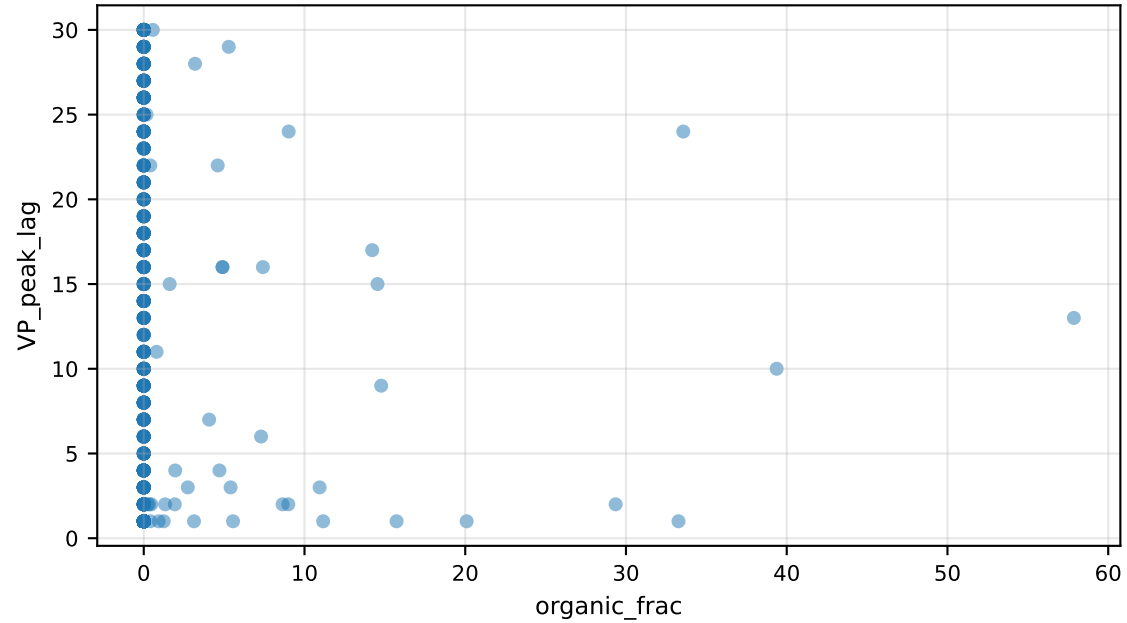
VP_peak_lag vs organic_frac
