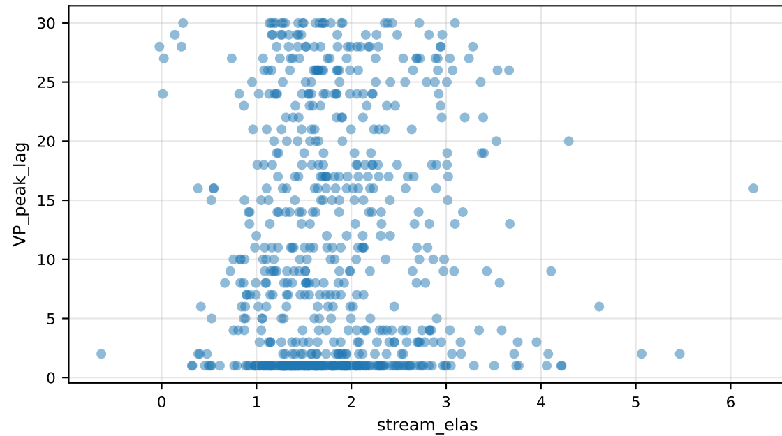
VP_peak_lag vs stream_elas
