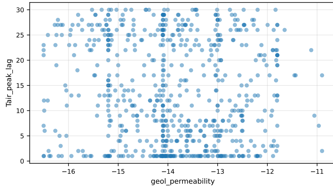
Tair_peak_lag vs geol_permeability
