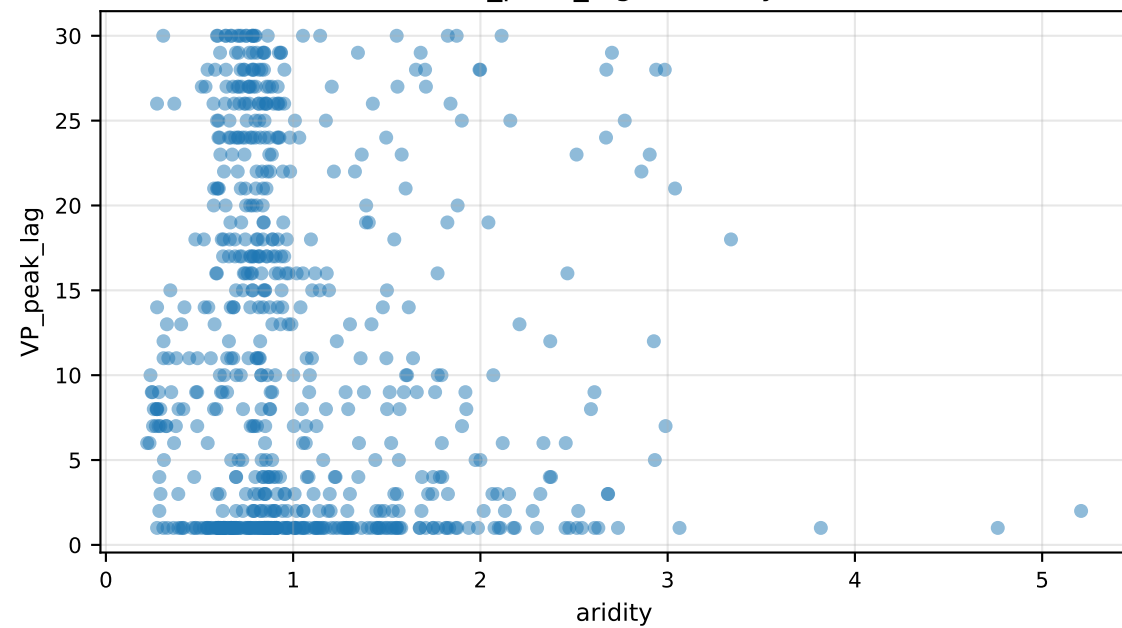
VP_peak_lag vs aridity
