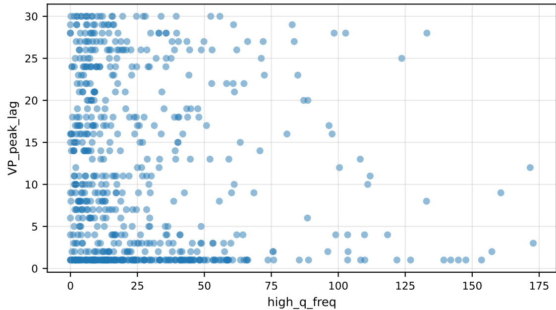
VP_peak_lag vs high_q_freq
