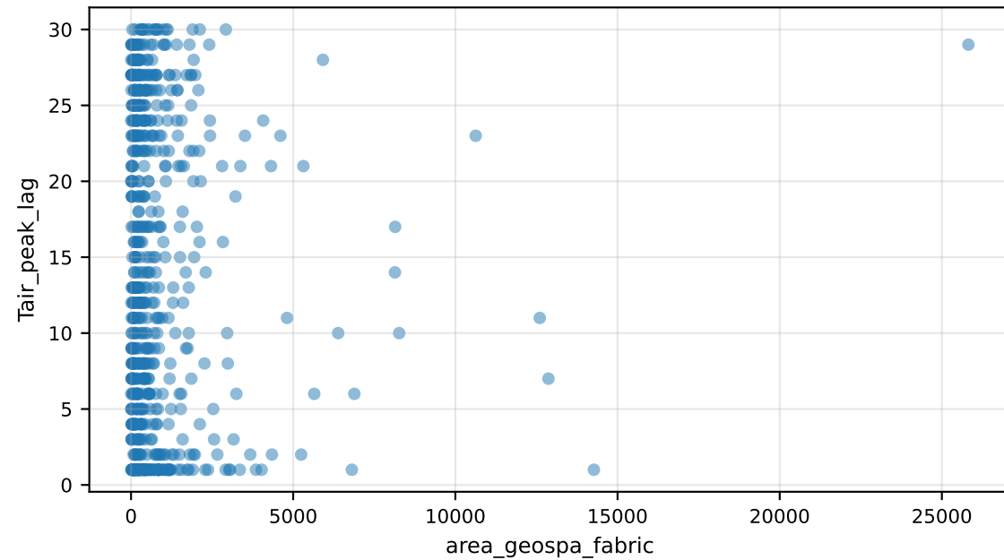
Tair_peak_lag vs area_geospa_fabric
