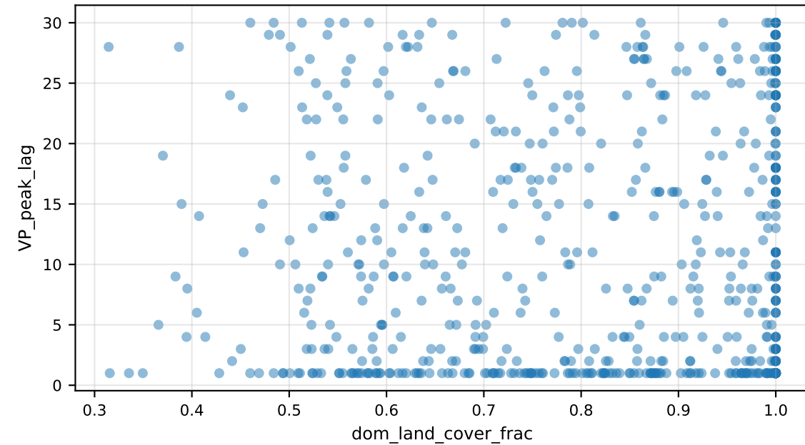
VP_peak_lag vs dom_land_cover_frac
