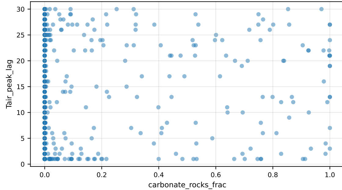
Tair_peak_lag vs carbonate_rocks_frac
