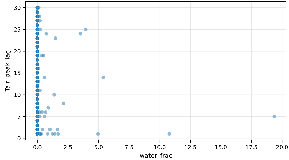
Tair_peak_lag vs water_frac
