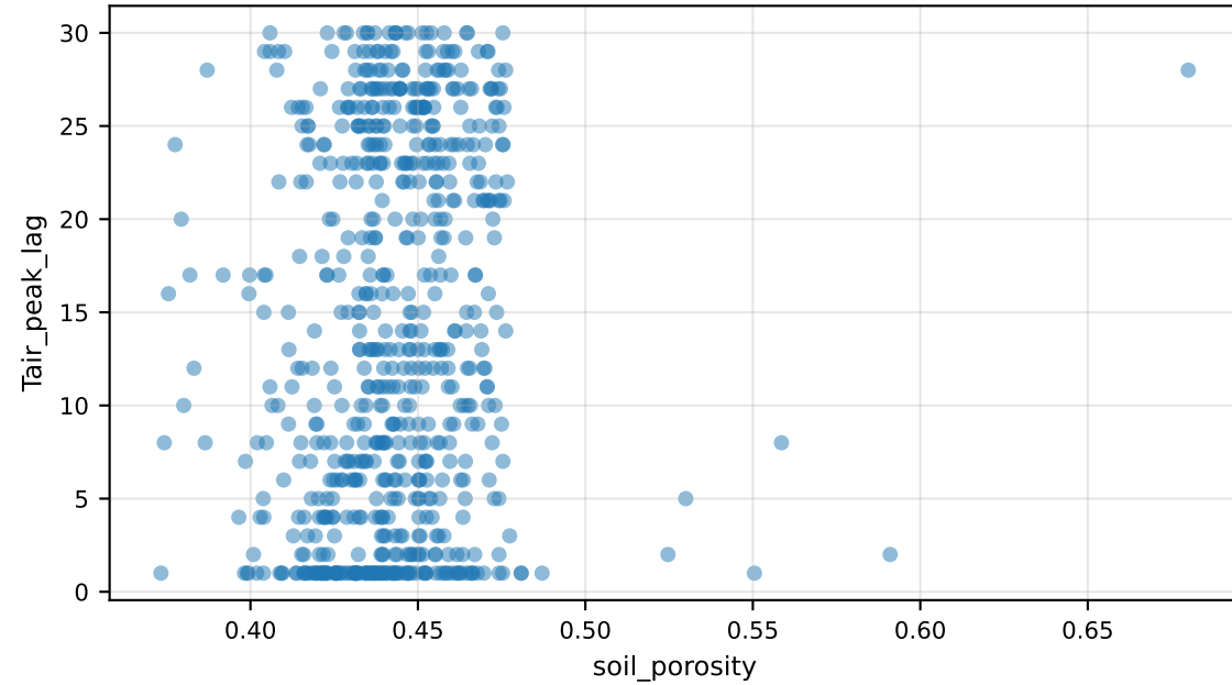
Tair_peak_lag vs soil_porosity
