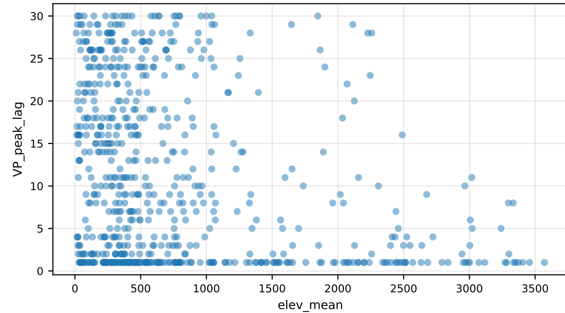
VP_peak_lag vs elev_mean
