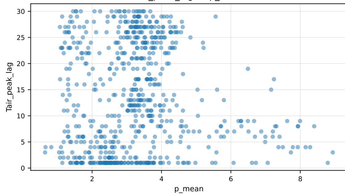
Tair_peak_lag vs p_mean
