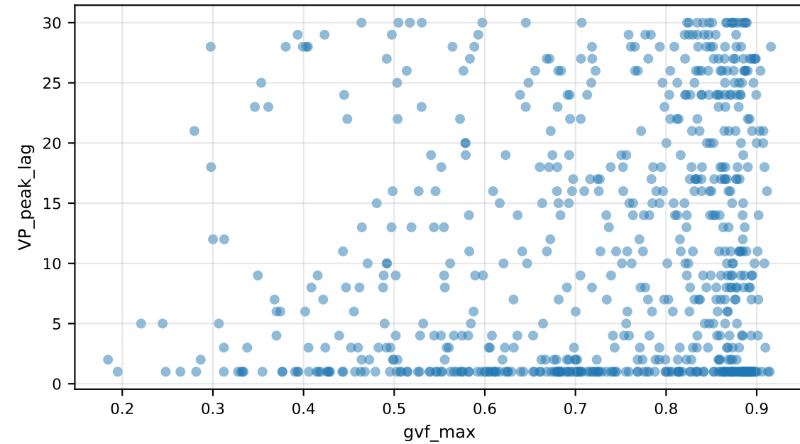
VP_peak_lag vs gvf_max
