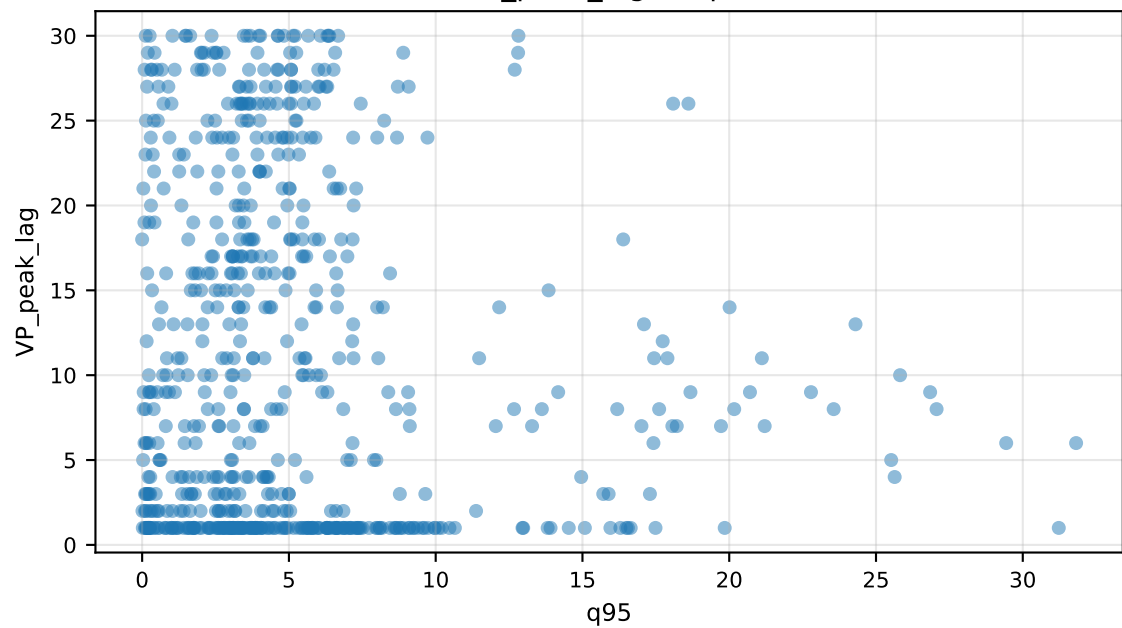
VP_peak_lag vs q95
