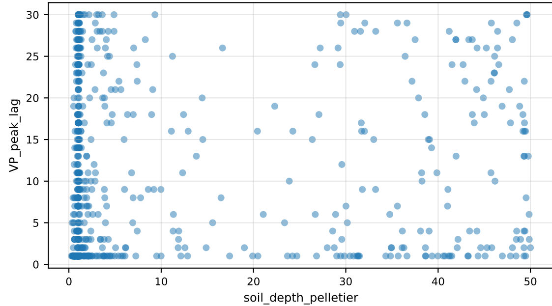
VP_peak_lag vs soil_depth_pelletier
