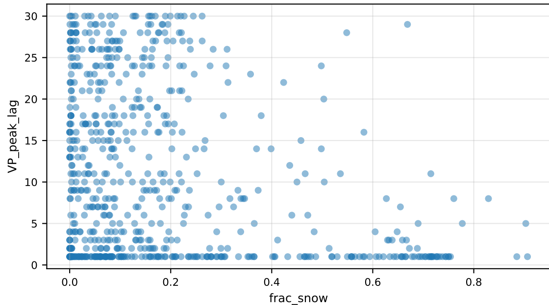
VP_peak_lag vs frac_snow
