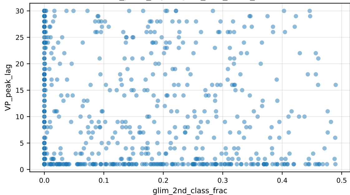
VP_peak_lag vs glim_2nd_class_frac
