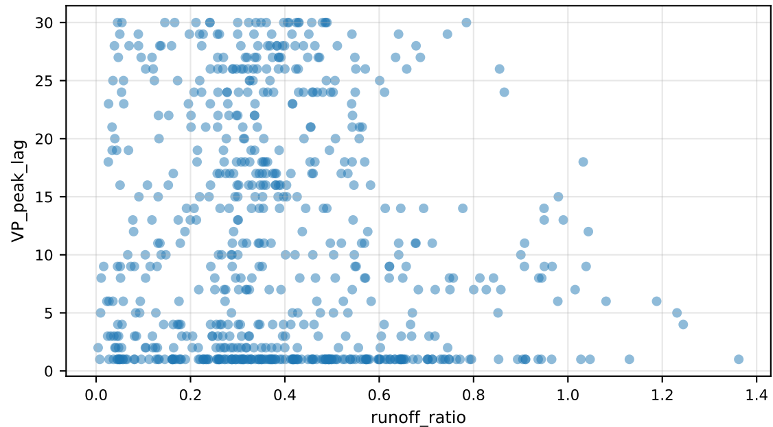
VP_peak_lag vs runoff_ratio
