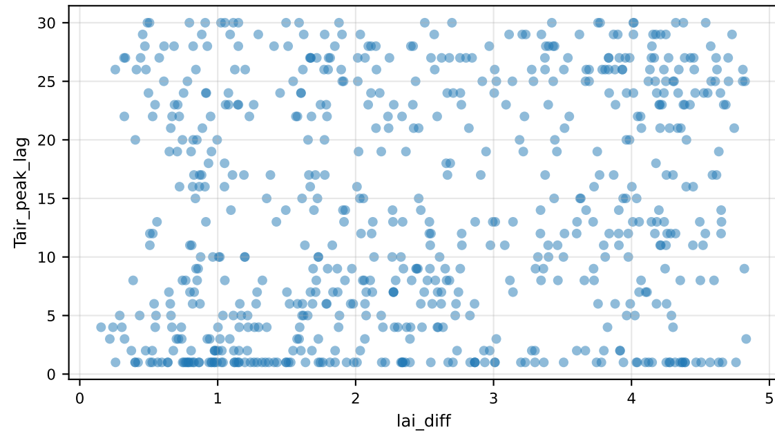
Tair_peak_lag vs lai_diff
