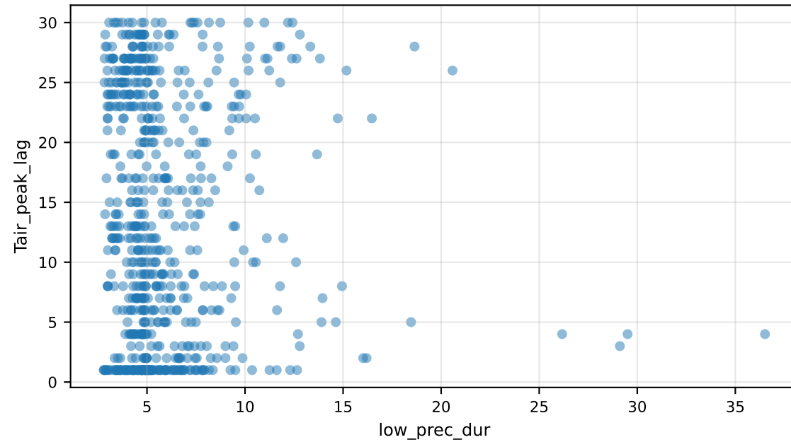
Tair_peak_lag vs low_prec_dur
