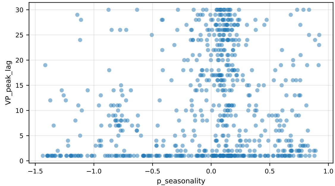
VP_peak_lag vs p_seasonality
