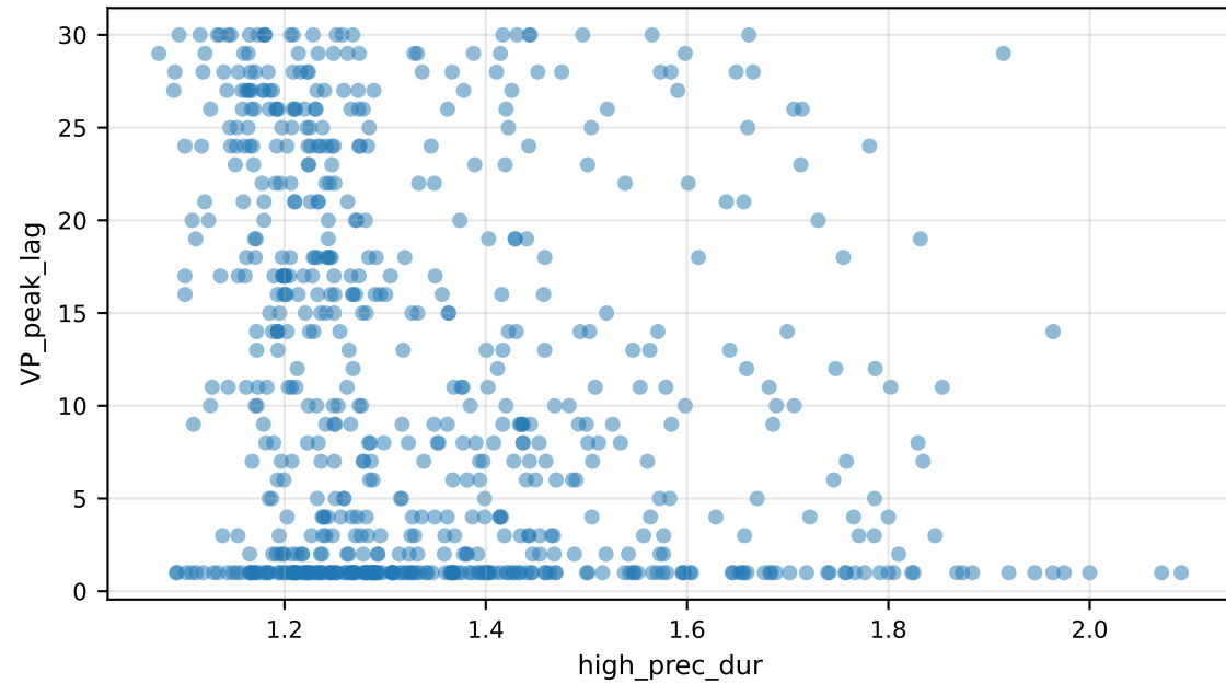
VP_peak_lag vs high_prec_dur
