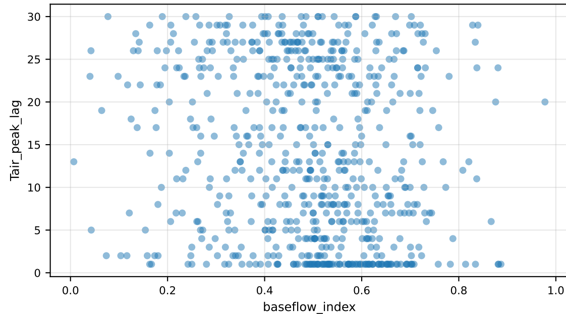
Tair_peak_lag vs baseflow_index
