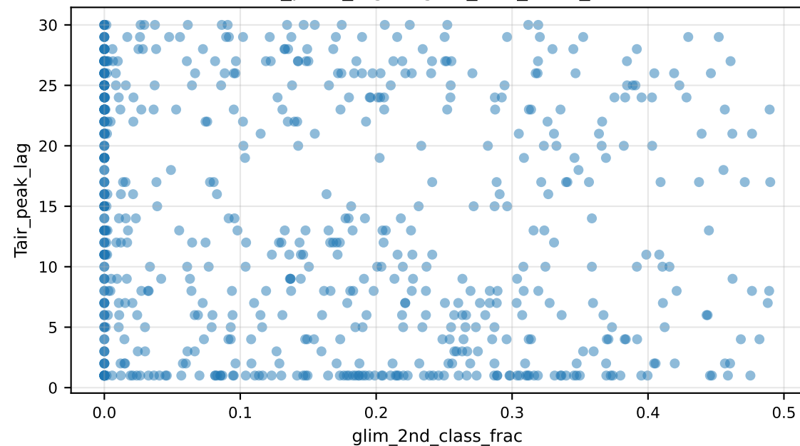
Tair_peak_lag vs glim_2nd_class_frac
