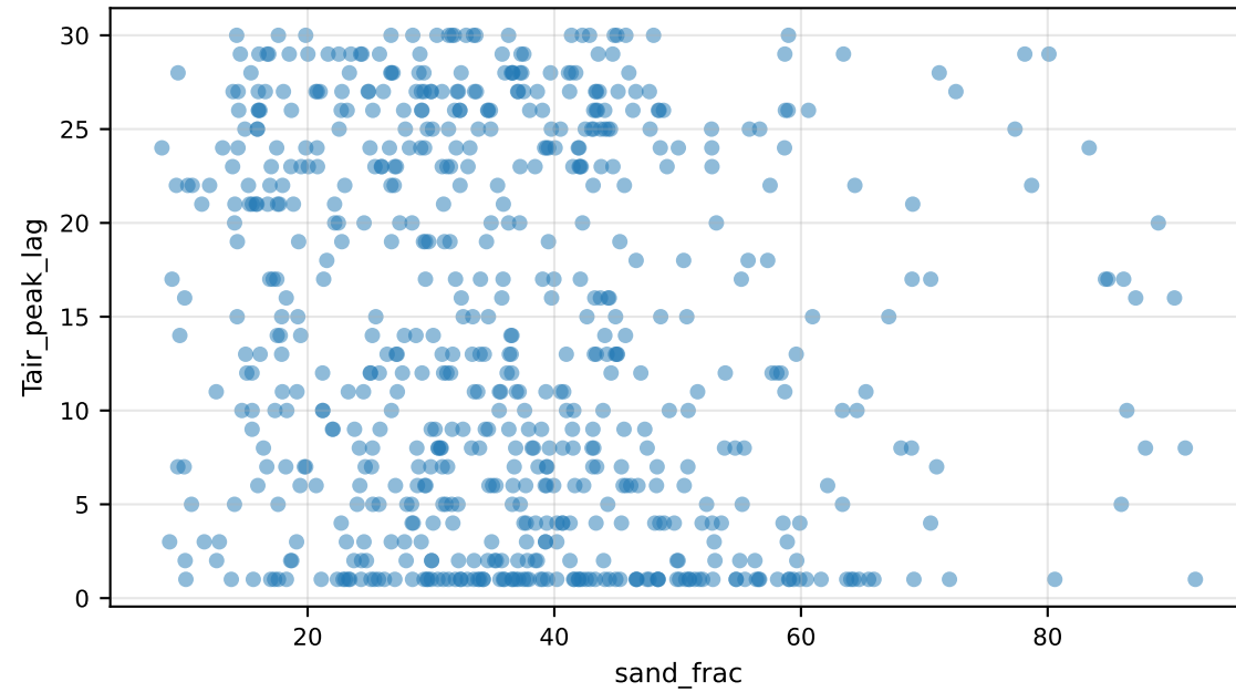
Tair_peak_lag vs sand_frac
