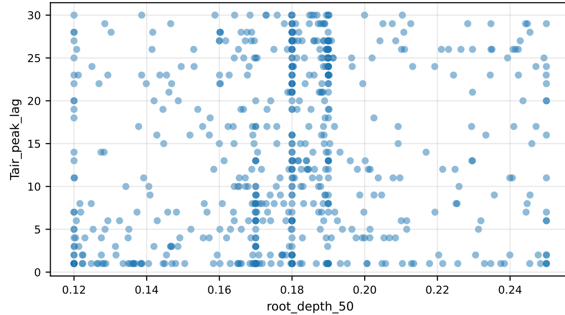
Tair_peak_lag vs root_depth_50
