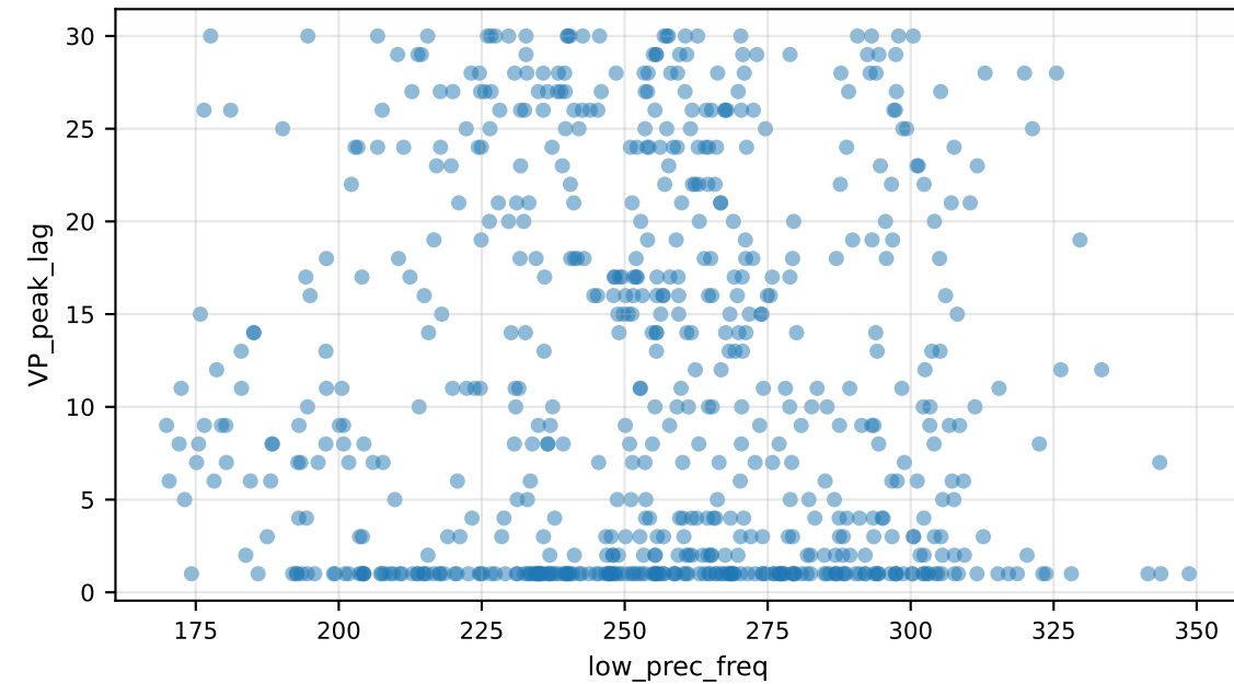
VP_peak_lag vs low_prec_freq
