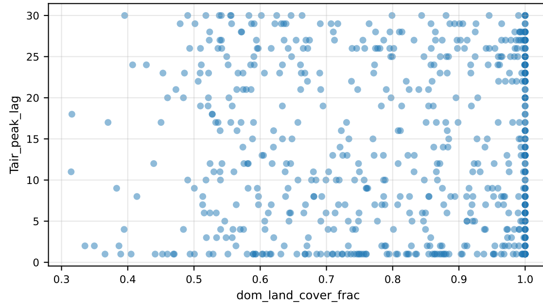
Tair_peak_lag vs dom_land_cover_frac
