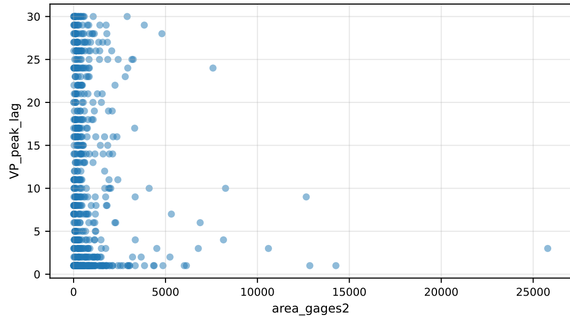
VP_peak_lag vs area_gages2
