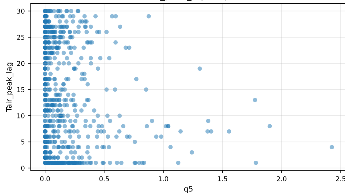
Tair_peak_lag vs q5
