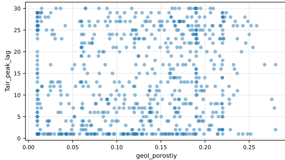
Tair_peak_lag vs geol_porostiy
