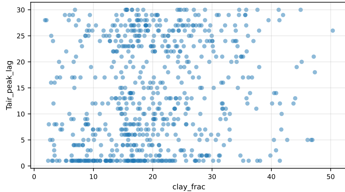
Tair_peak_lag vs clay_frac
