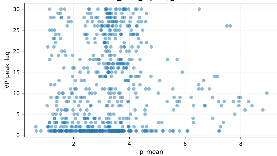
VP_peak_lag vs p_mean
