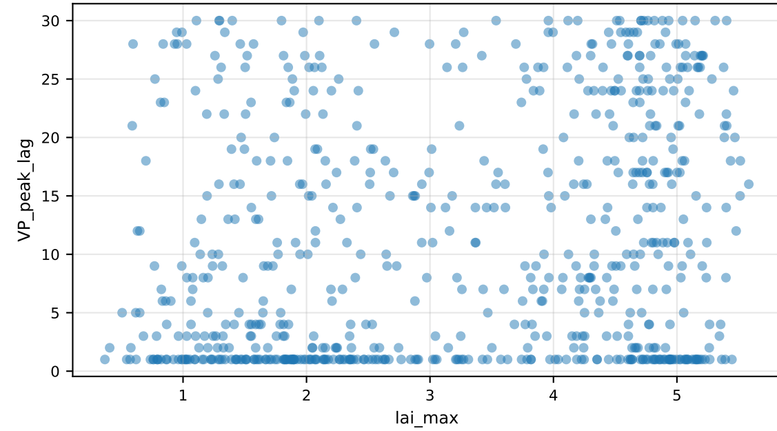
VP_peak_lag vs lai_max
