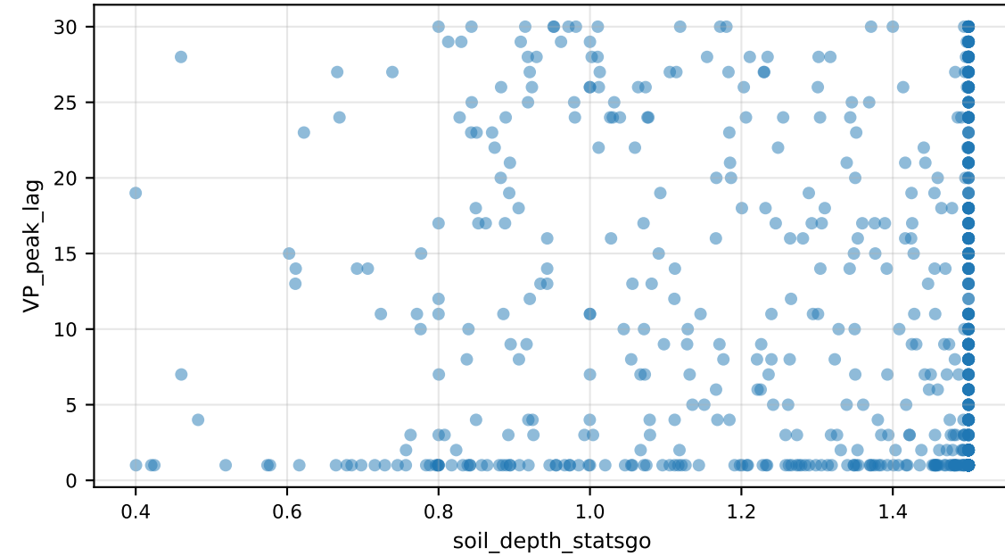
VP_peak_lag vs soil_depth_statsgo
