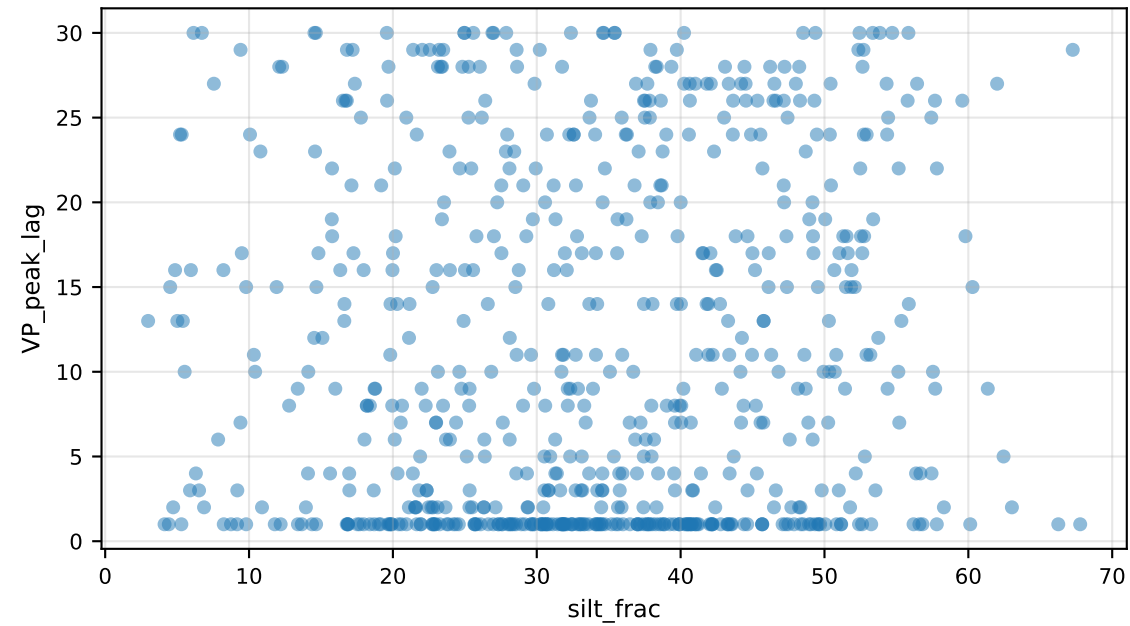
VP_peak_lag vs silt_frac
