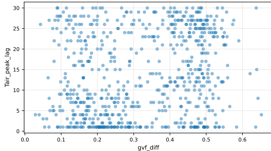
Tair_peak_lag vs gvf_diff
