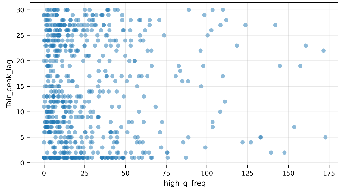
Tair_peak_lag vs high_q_freq
