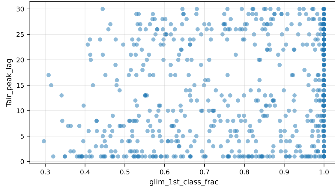
Tair_peak_lag vs glim_1st_class_frac
