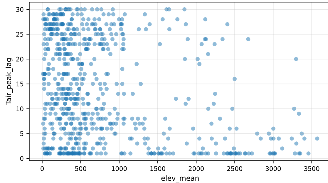
Tair_peak_lag vs elev_mean
