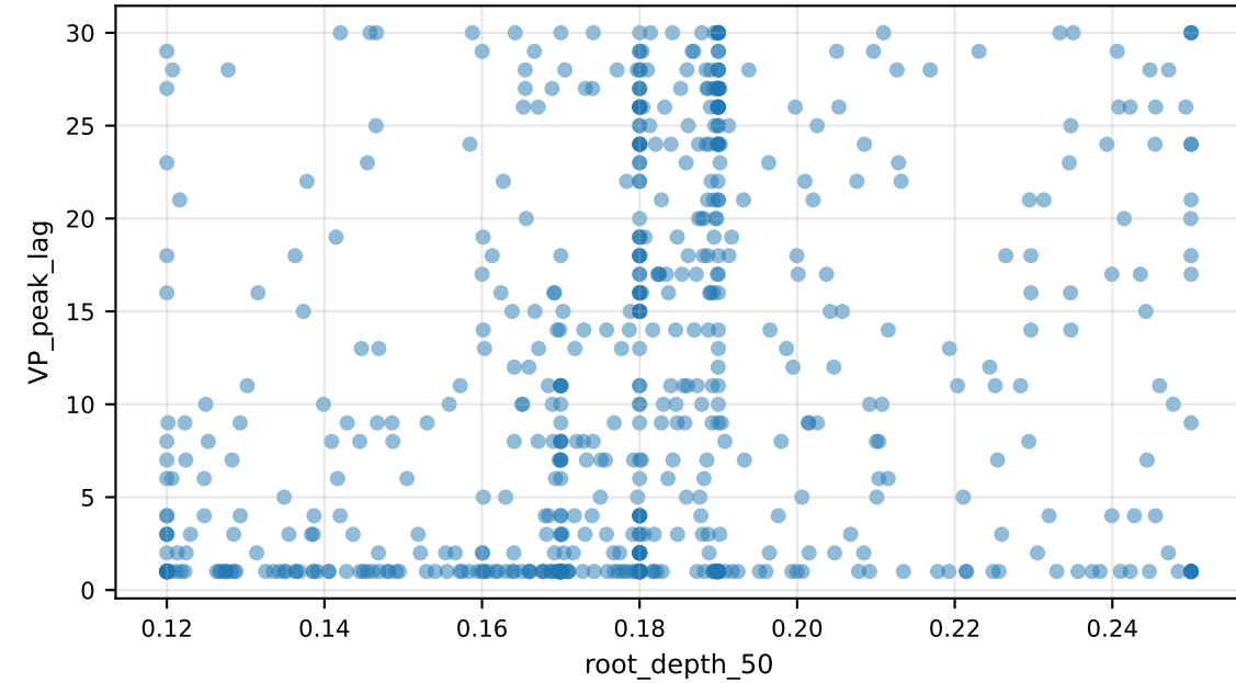
VP_peak_lag vs root_depth_50
