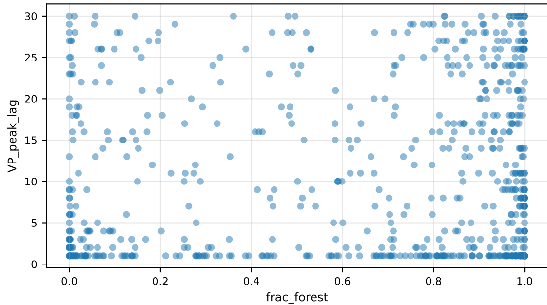
VP_peak_lag vs frac_forest
