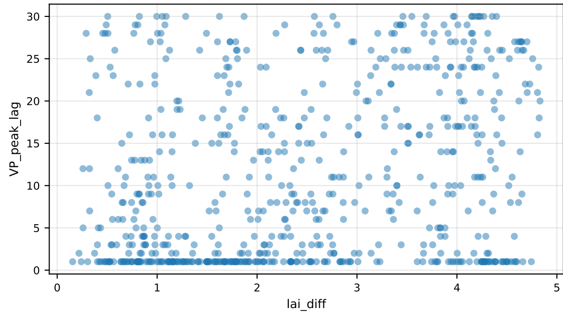
VP_peak_lag vs lai_diff
