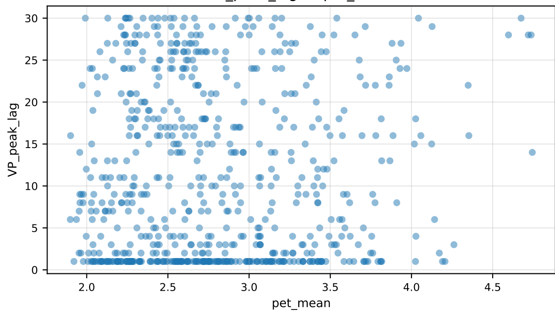
VP_peak_lag vs pet_mean
