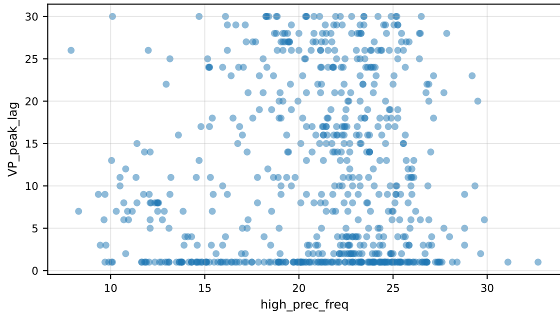
VP_peak_lag vs high_prec_freq
