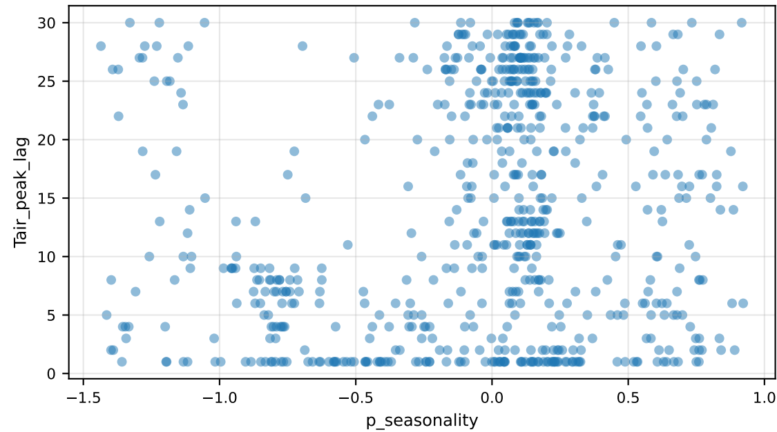
Tair_peak_lag vs p_seasonality
