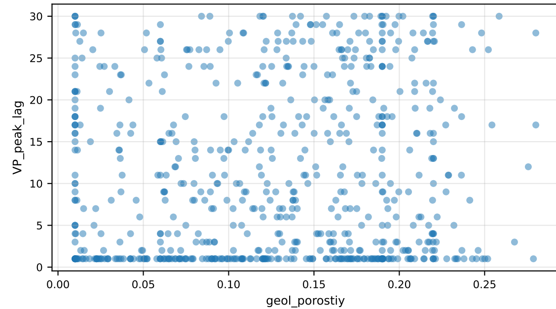
VP_peak_lag vs geol_porostiy
