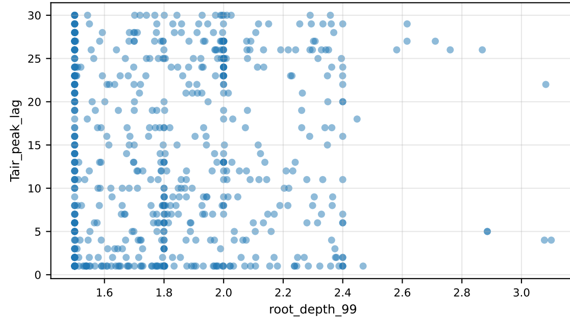
Tair_peak_lag vs root_depth_99
