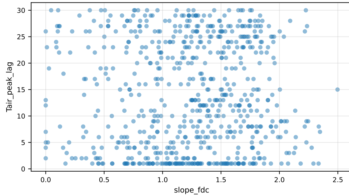
Tair_peak_lag vs slope_fdc
