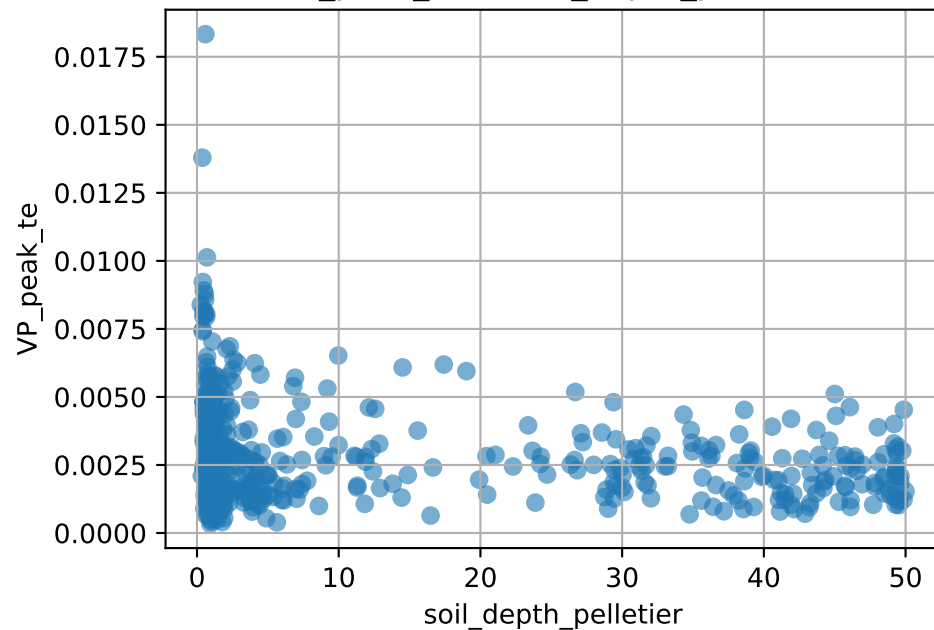
VP_peak_te vs soil_depth_pelletier
