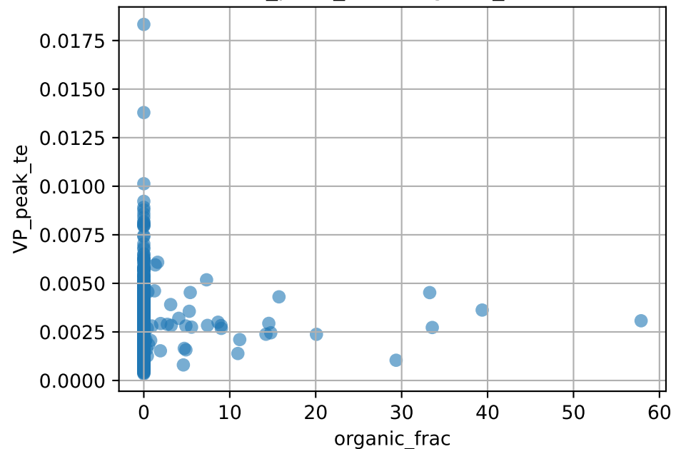
VP_peak_te vs organic_frac
