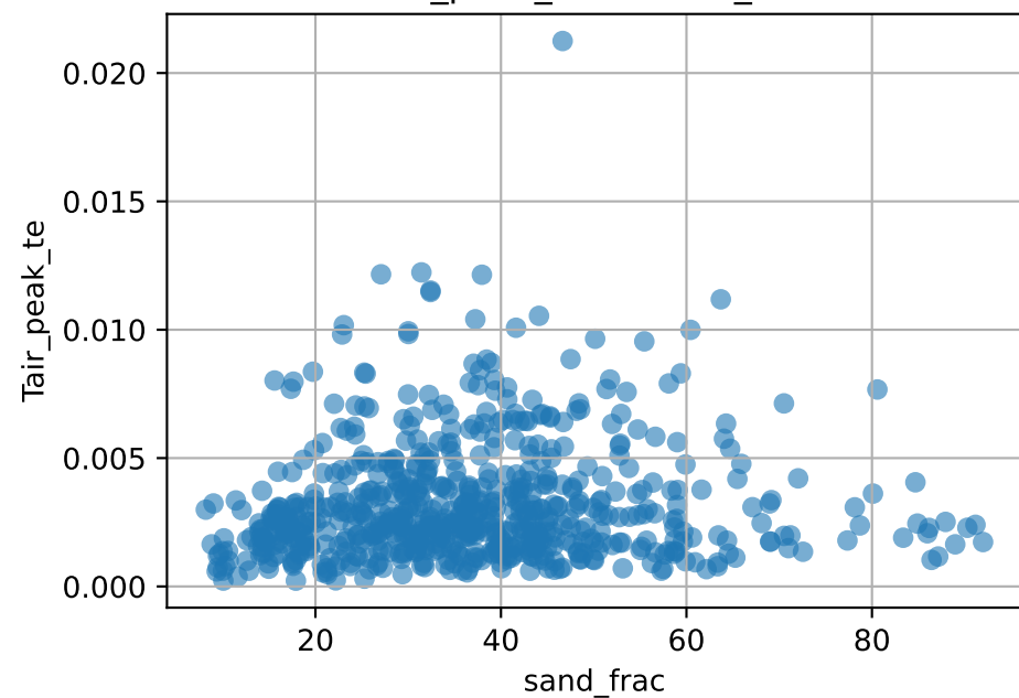
Tair_peak_te vs sand_frac
