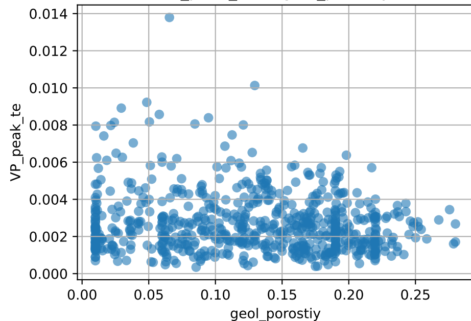
VP_peak_te vs geol_porostiy
