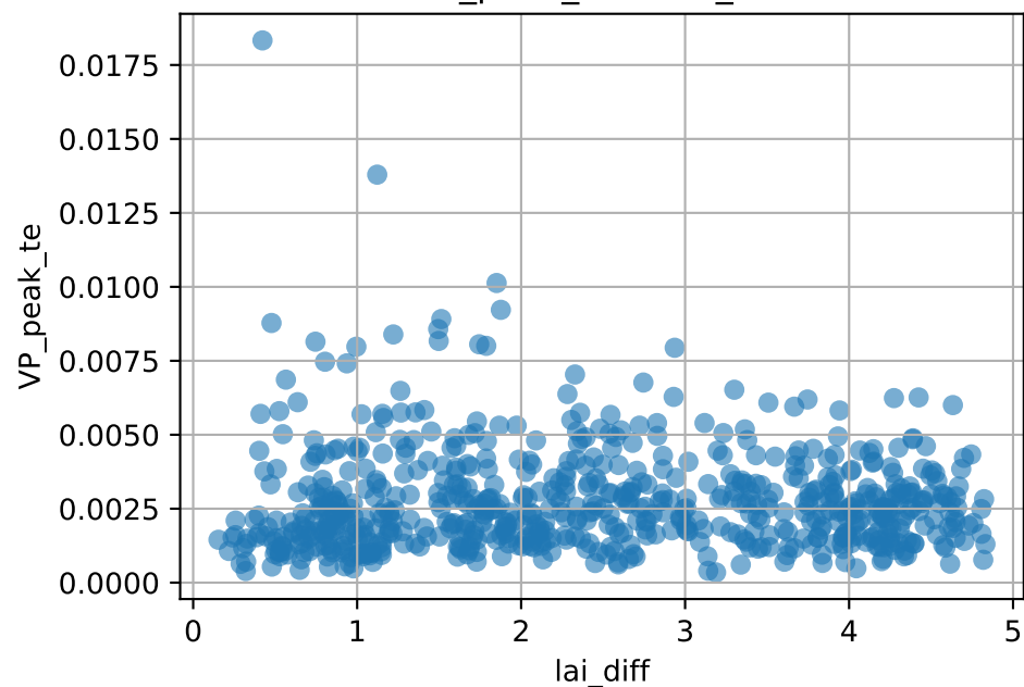
VP_peak_te vs lai_diff
