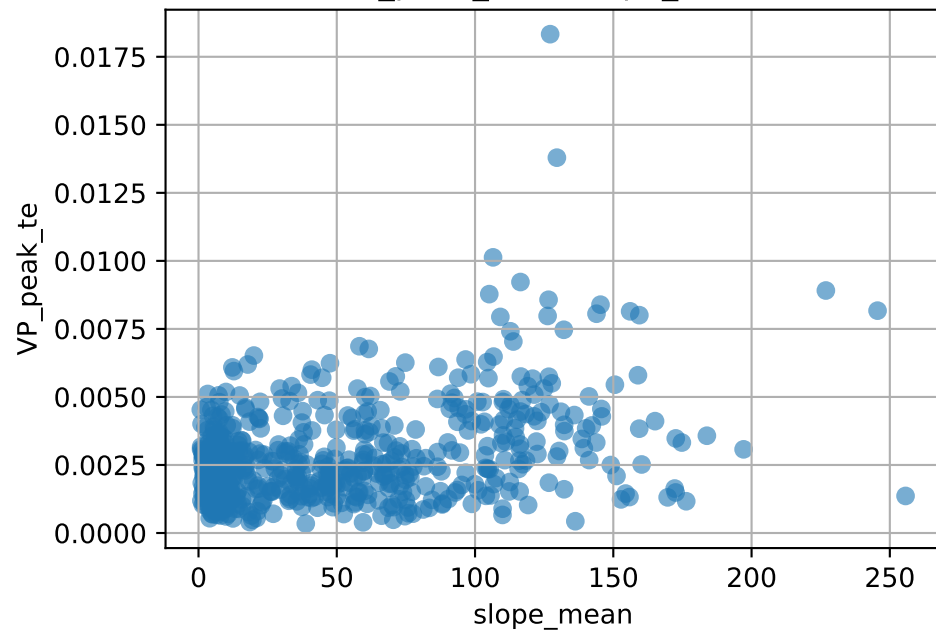
VP_peak_te vs slope_mean
