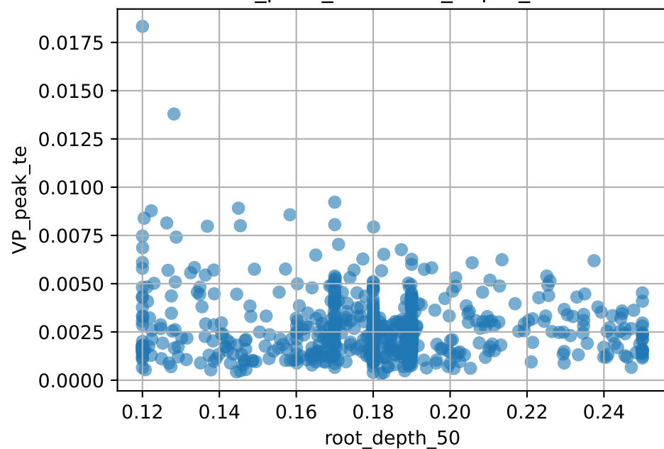
VP_peak_te vs root_depth_50
