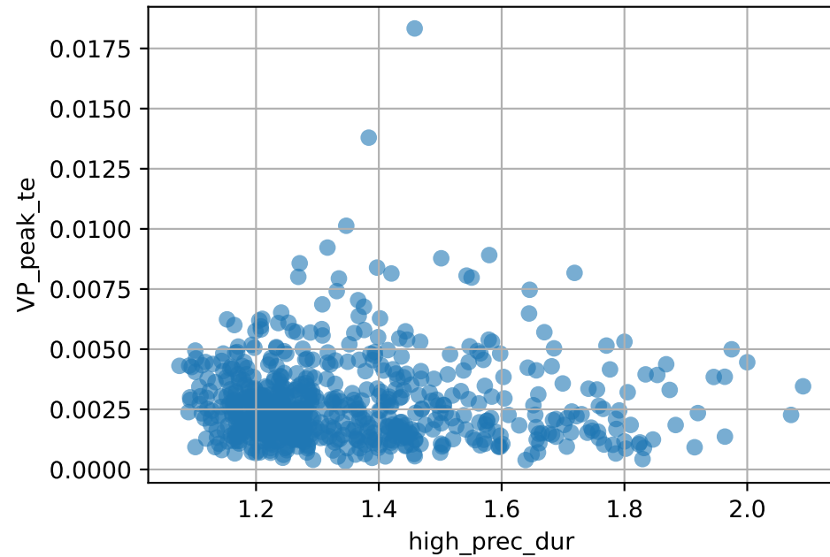
VP_peak_te vs high_prec_dur
