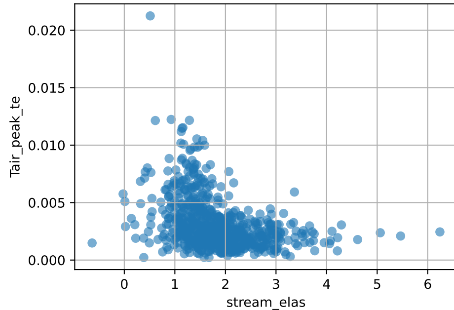
Tair_peak_te vs stream_elas
