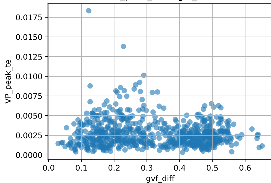
VP_peak_te vs gvf_diff
