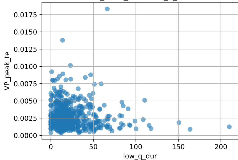
VP_peak_te vs low_q_dur
