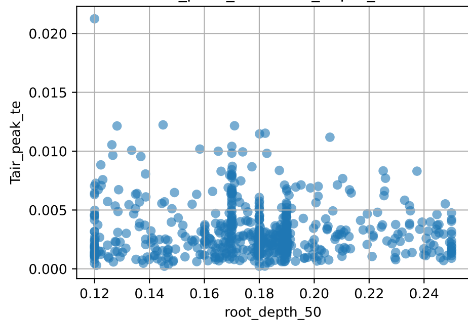
Tair_peak_te vs root_depth_50
