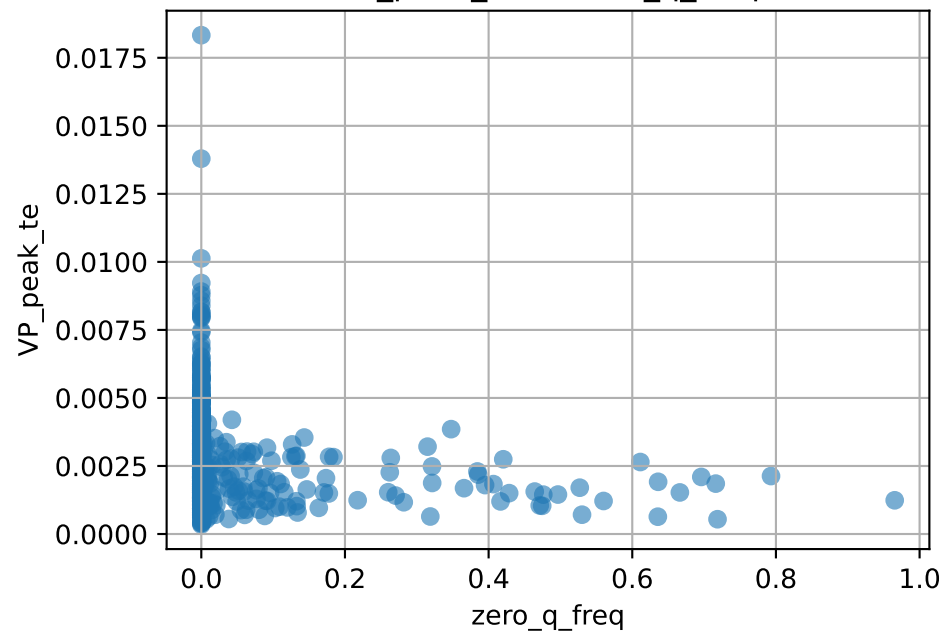
VP_peak_te vs zero_q_freq
