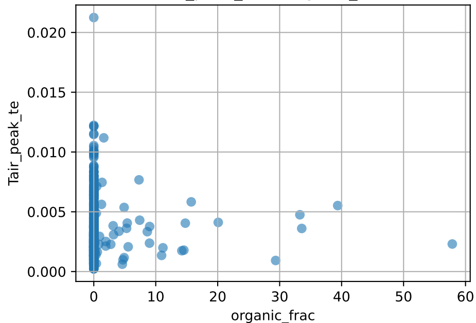
Tair_peak_te vs organic_frac
