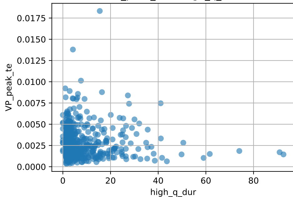
VP_peak_te vs high_q_dur
