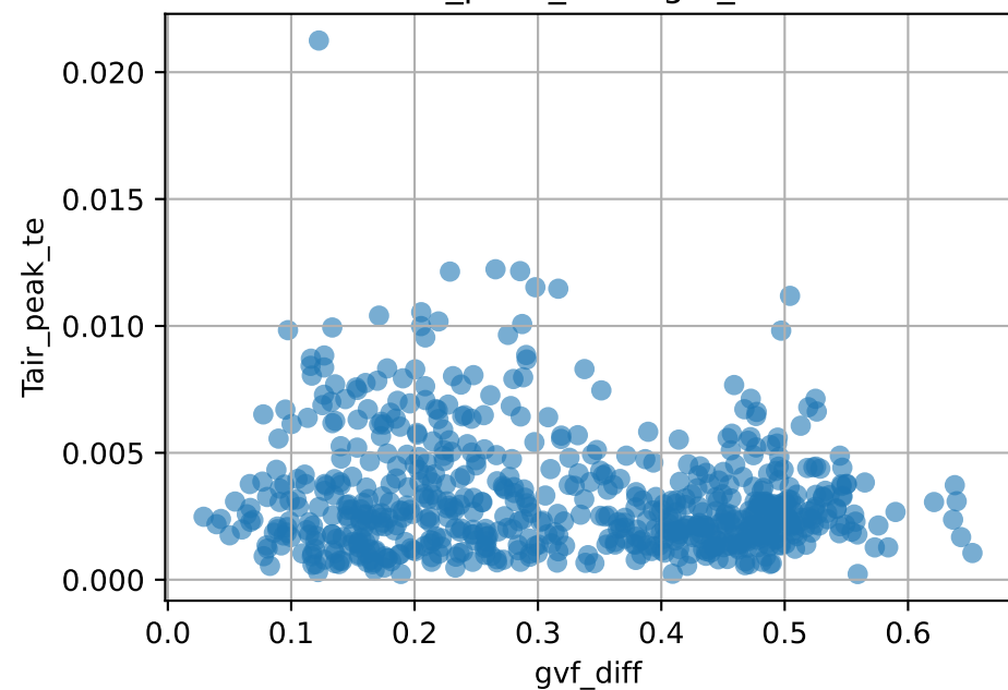
Tair_peak_te vs gvf_diff
