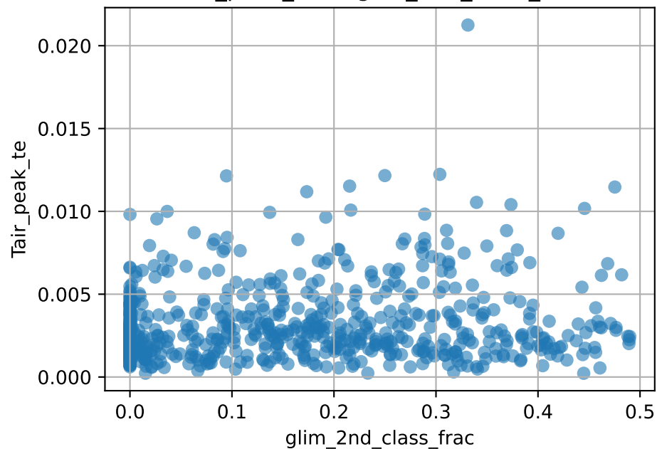
Tair_peak_te vs glim_2nd_class_frac
