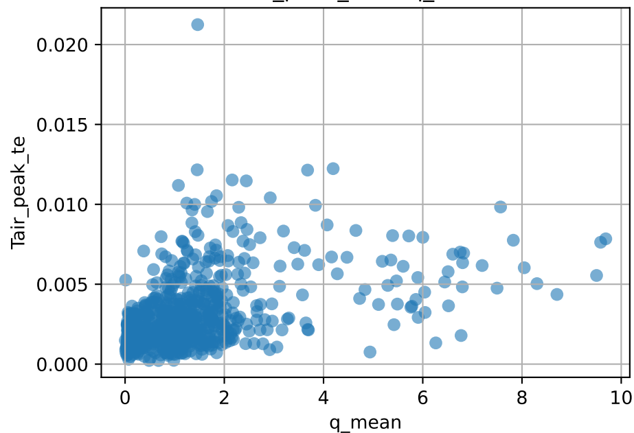
Tair_peak_te vs q_mean
