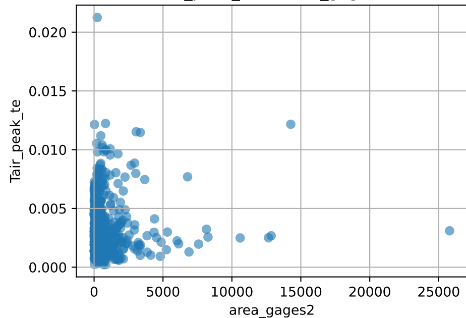
Tair_peak_te vs area_gages2
