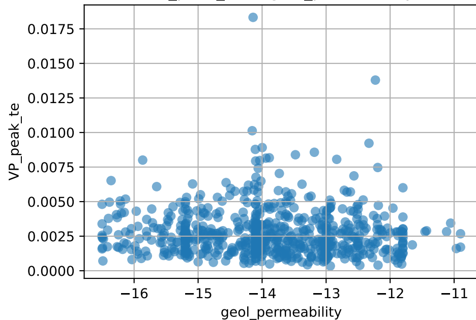
VP_peak_te vs geol_permeability
