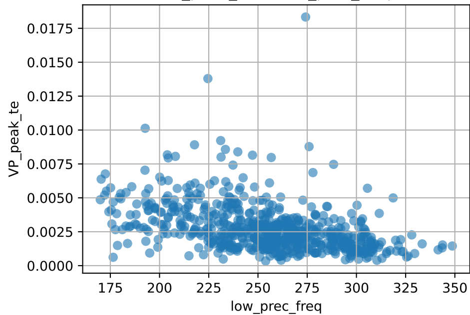
VP_peak_te vs low_prec_freq
