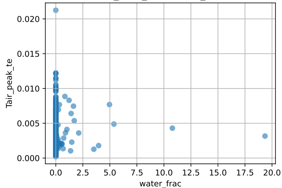
Tair_peak_te vs water_frac
