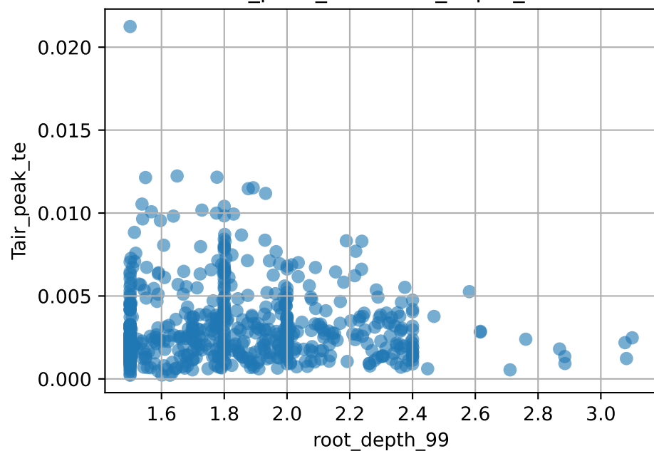
Tair_peak_te vs root_depth_99
