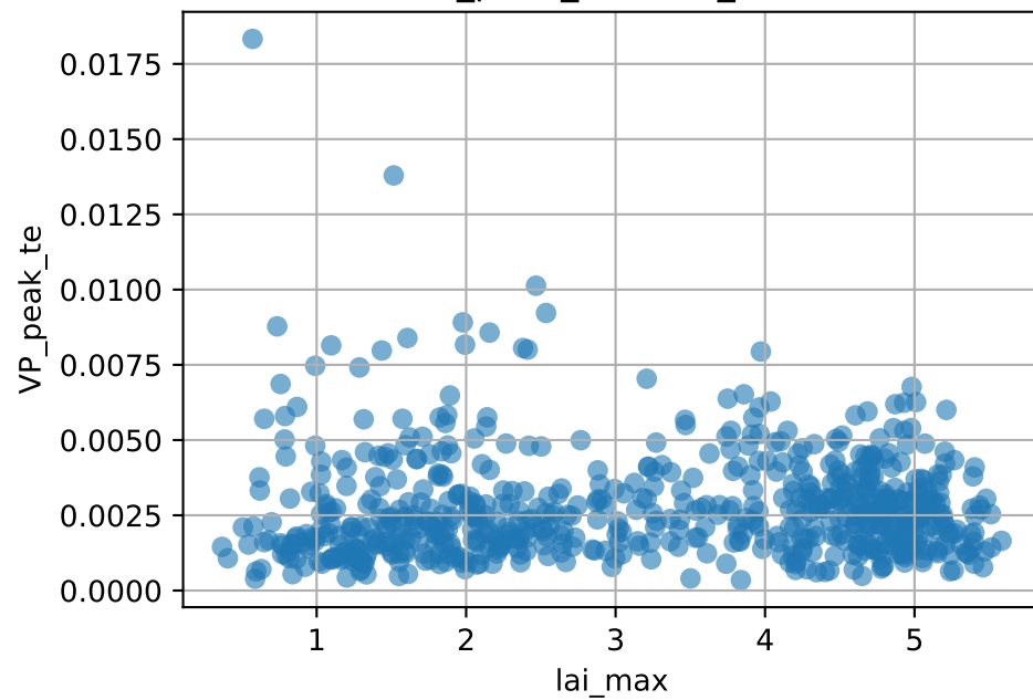
VP_peak_te vs lai_max
