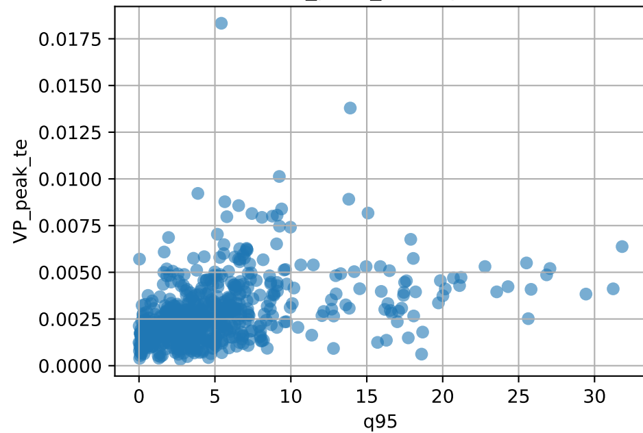
VP_peak_te vs q95
