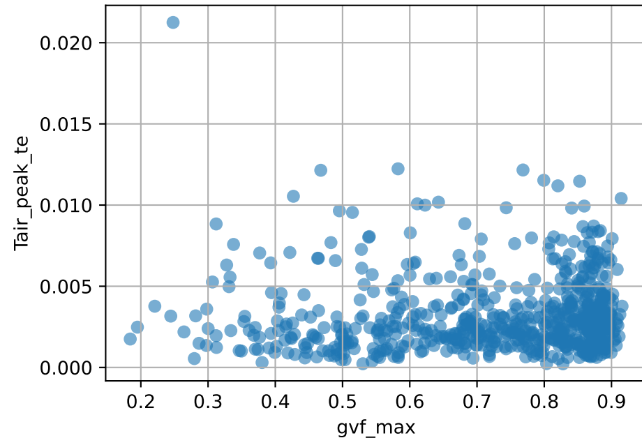
Tair_peak_te vs gvf_max
