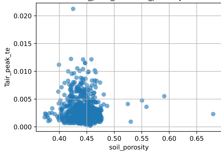
Tair_peak_te vs soil_porosity
