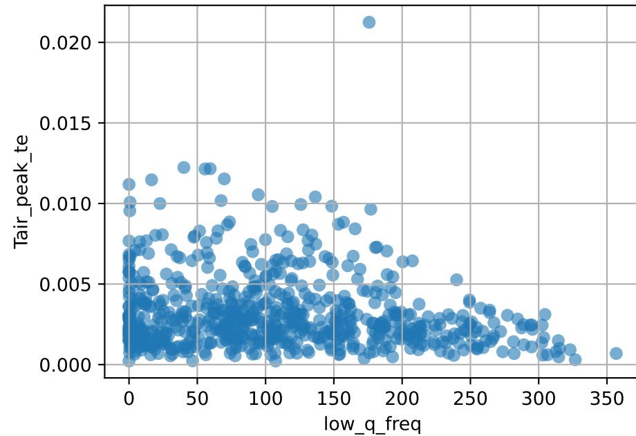
Tair_peak_te vs low_q_freq
