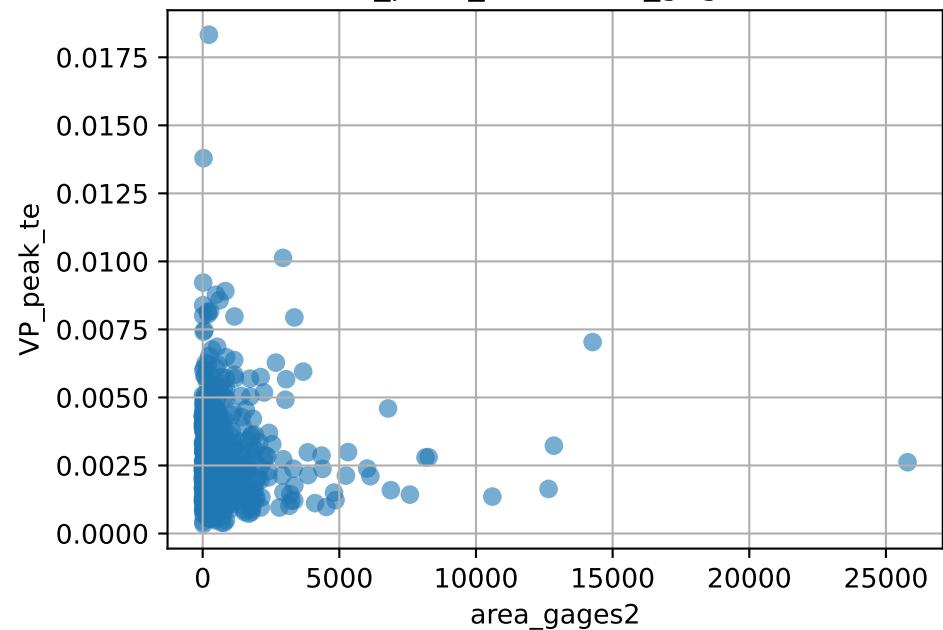
VP_peak_te vs area_gages2
