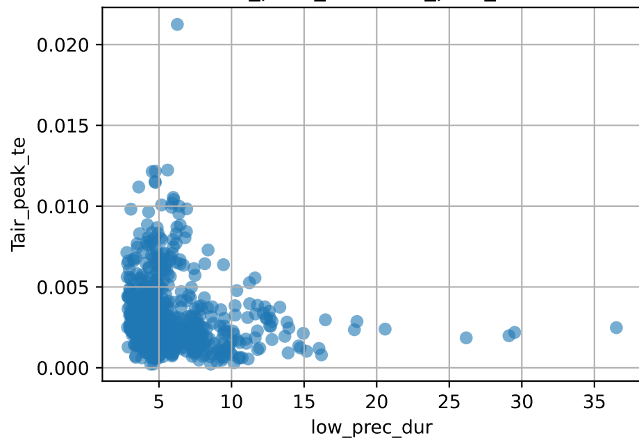
Tair_peak_te vs low_prec_dur
