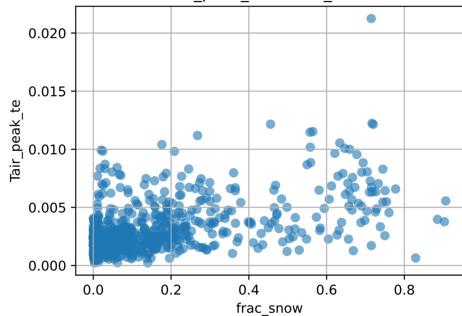
Tair_peak_te vs frac_snow
