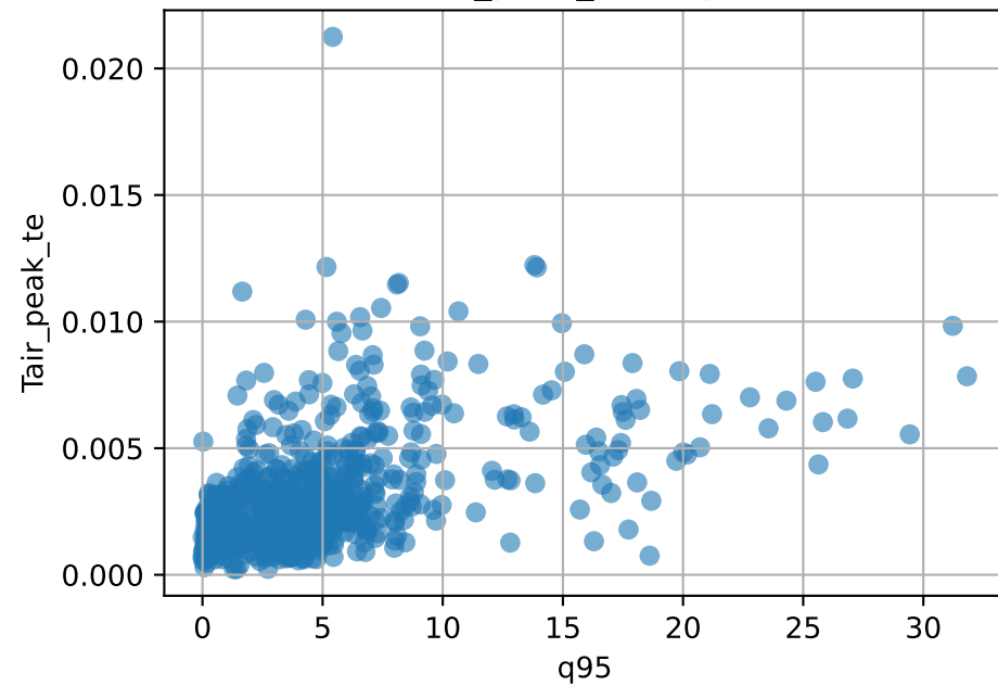
Tair_peak_te vs q95
