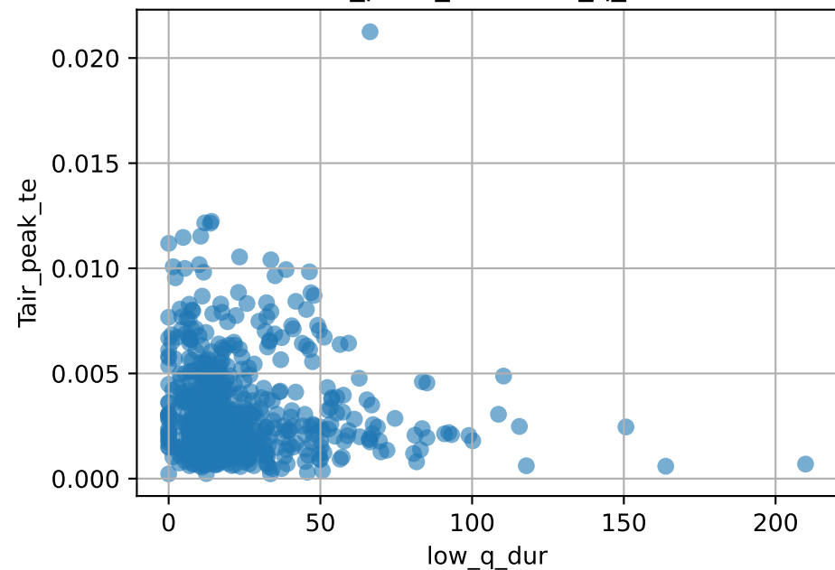
Tair_peak_te vs low_q_dur
