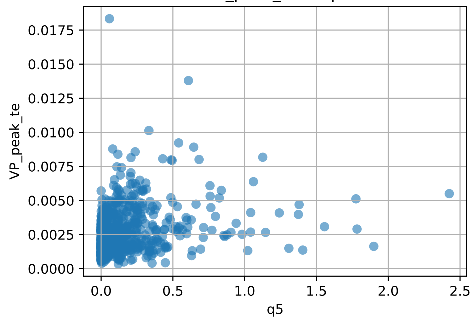
VP_peak_te vs q5
