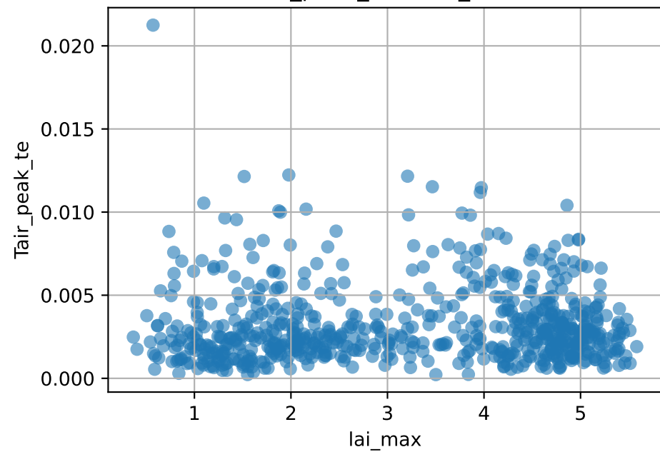
Tair_peak_te vs lai_max
