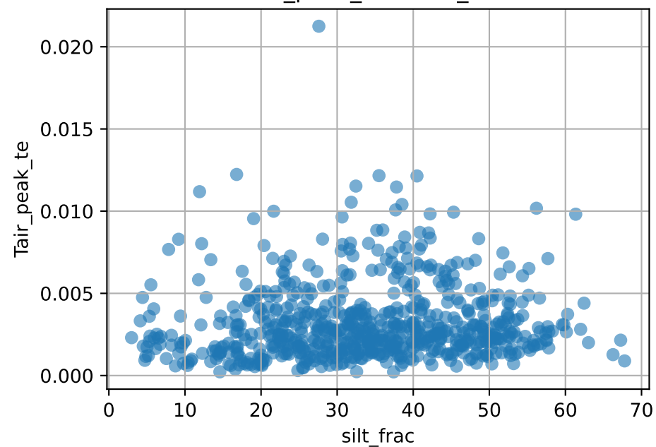
Tair_peak_te vs silt_frac
