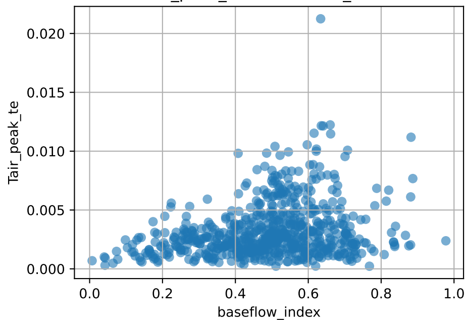
Tair_peak_te vs baseflow_index
