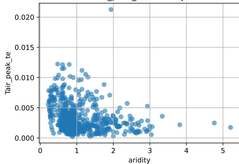
Tair_peak_te vs aridity
