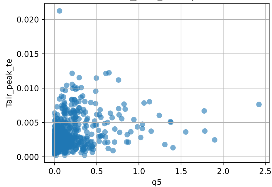
Tair_peak_te vs q5
