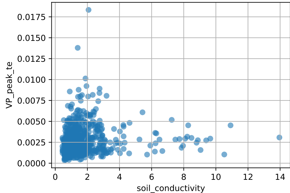
VP_peak_te vs soil_conductivity
