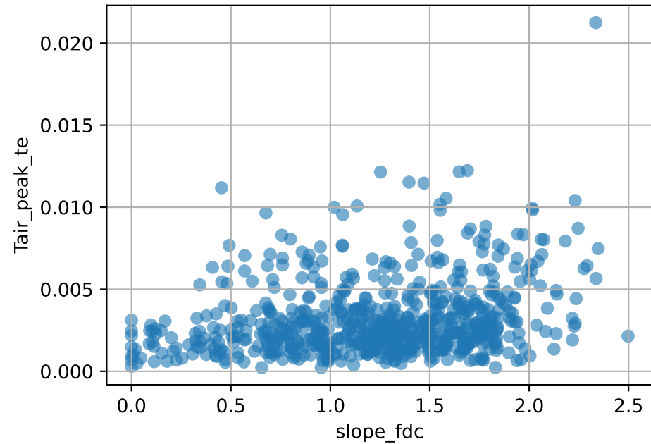
Tair_peak_te vs slope_fdc
