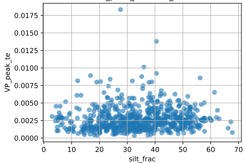
VP_peak_te vs silt_frac
