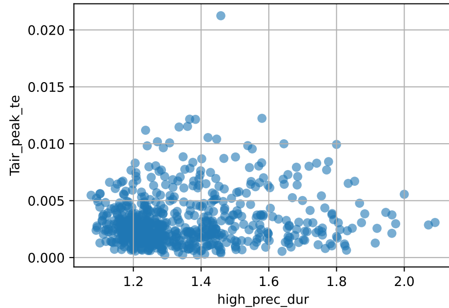
Tair_peak_te vs high_prec_dur
