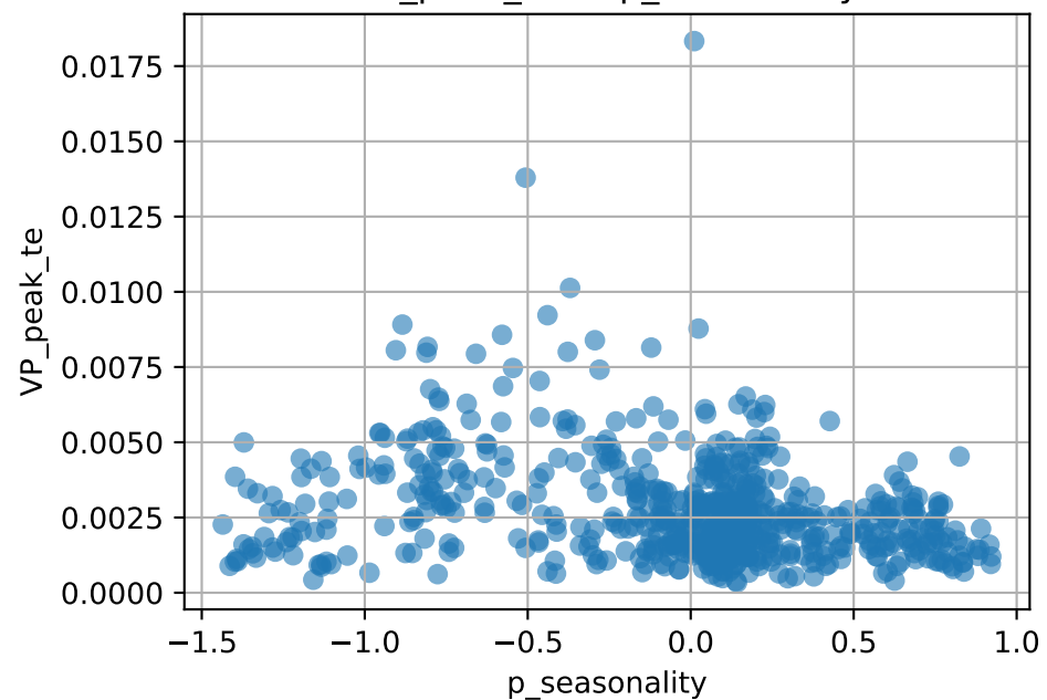
VP_peak_te vs p_seasonality
