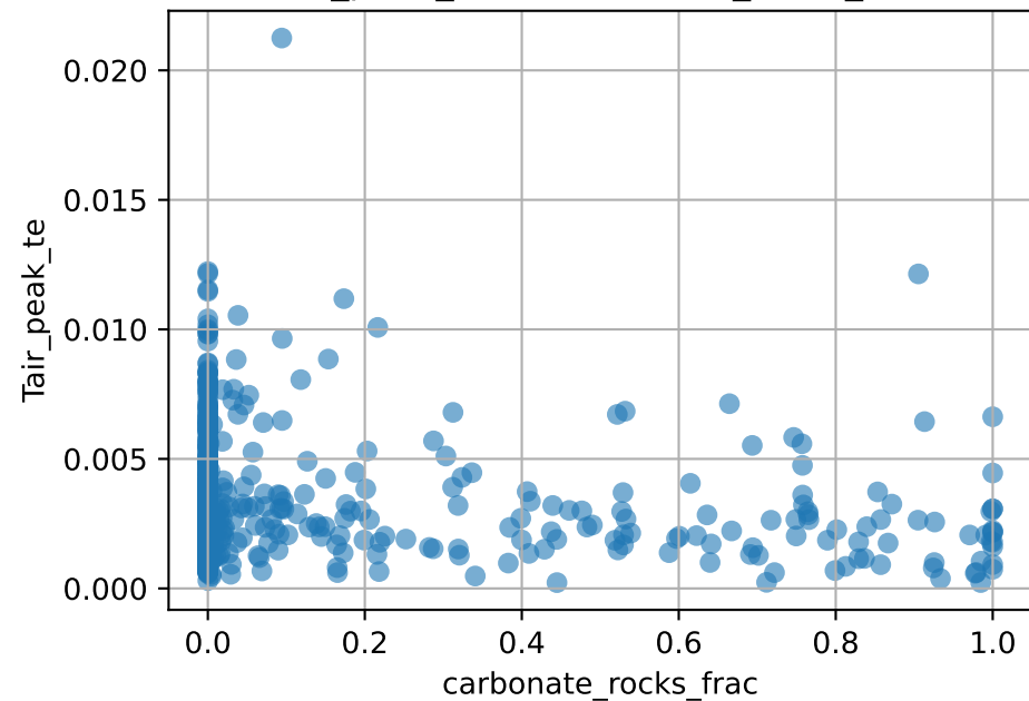
Tair_peak_te vs carbonate_rocks_frac
