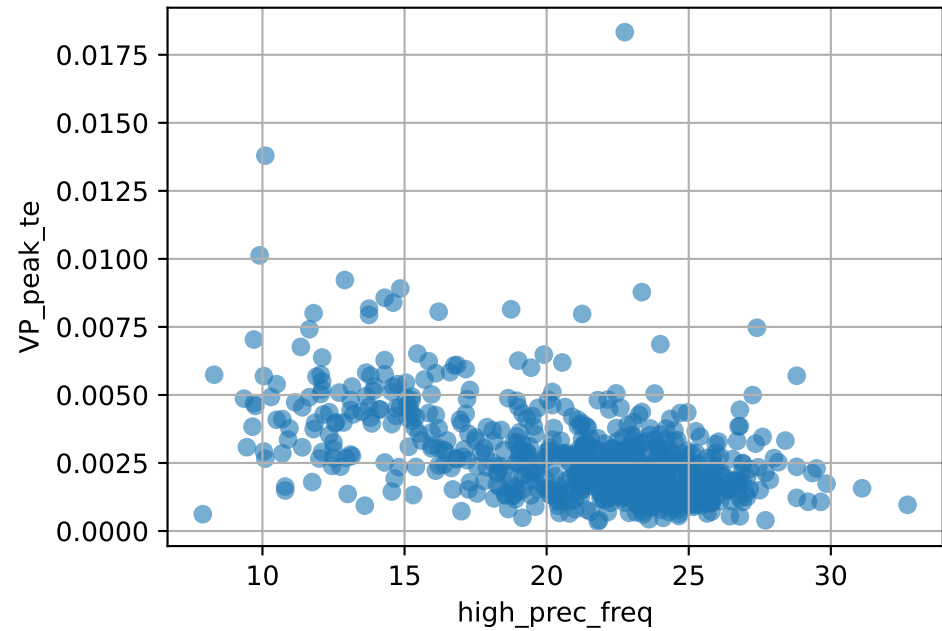
VP_peak_te vs high_prec_freq
