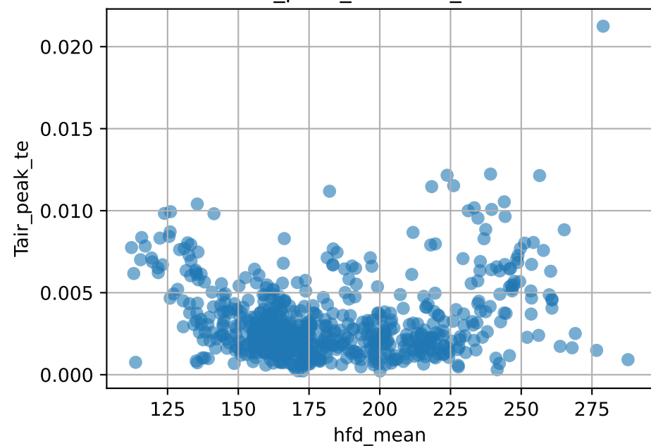
Tair_peak_te vs hfd_mean
