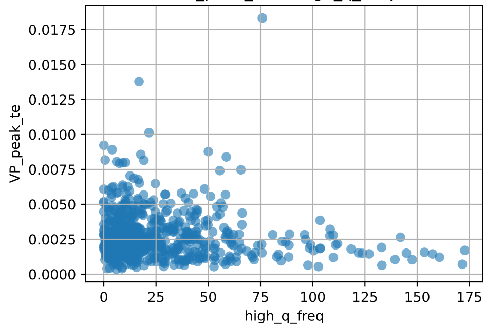
VP_peak_te vs high_q_freq
