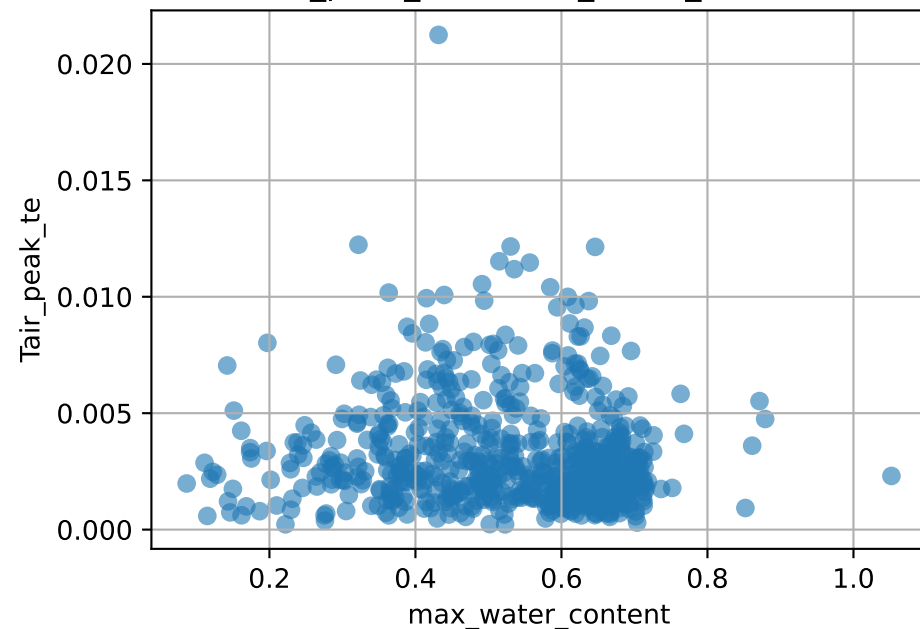
Tair_peak_te vs max_water_content
