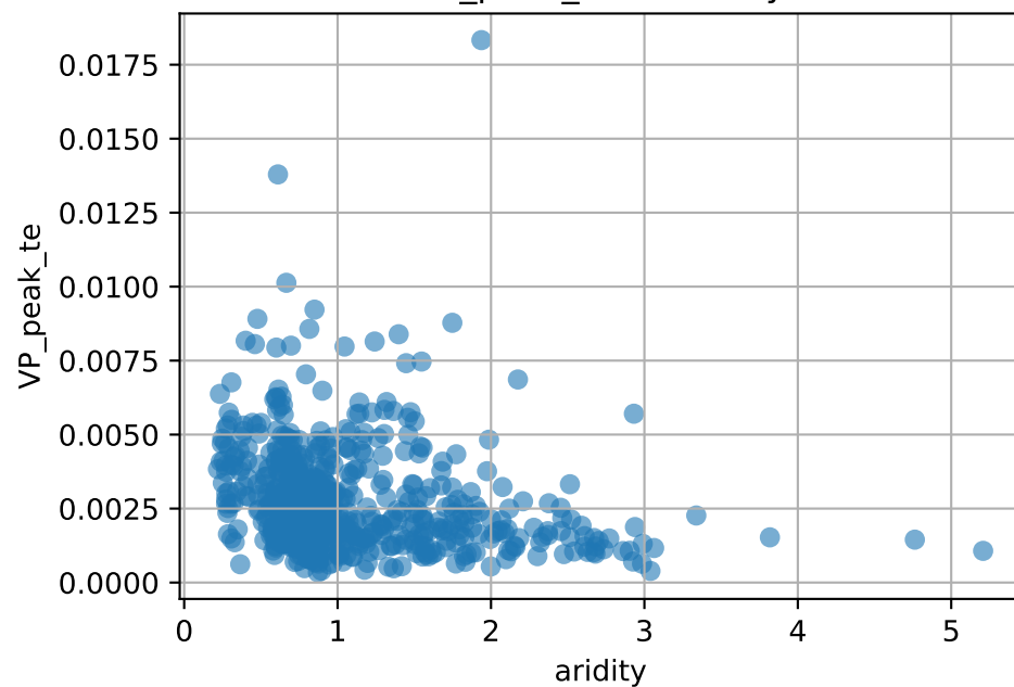
VP_peak_te vs aridity
