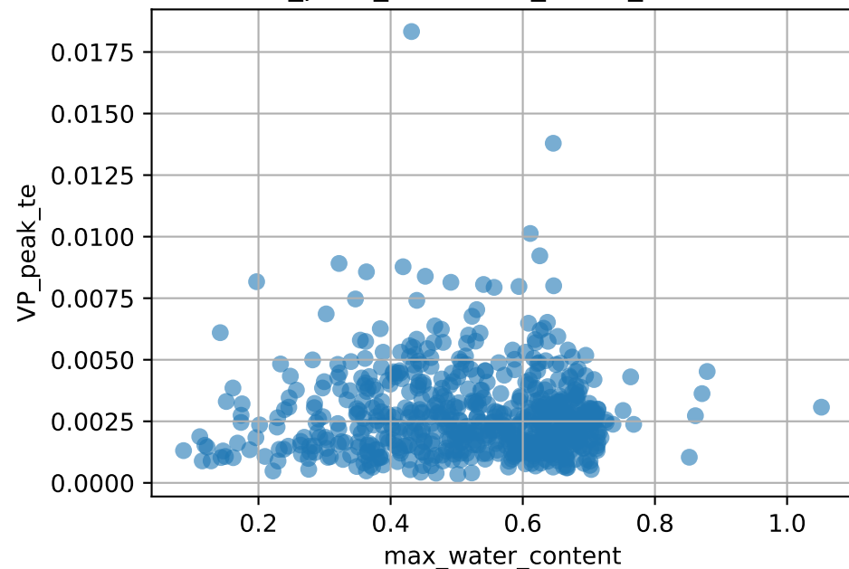
VP_peak_te vs max_water_content
