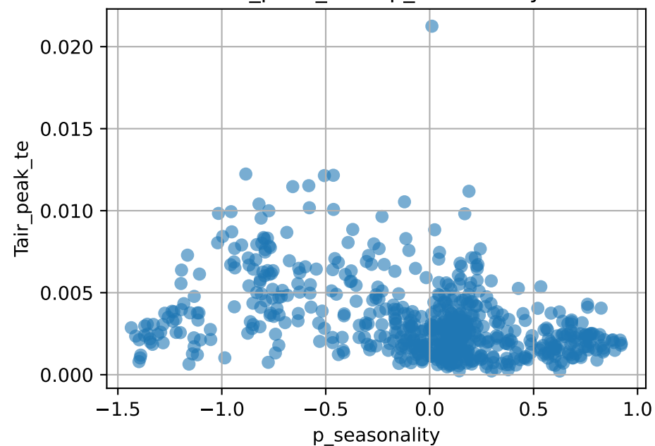
Tair_peak_te vs p_seasonality
