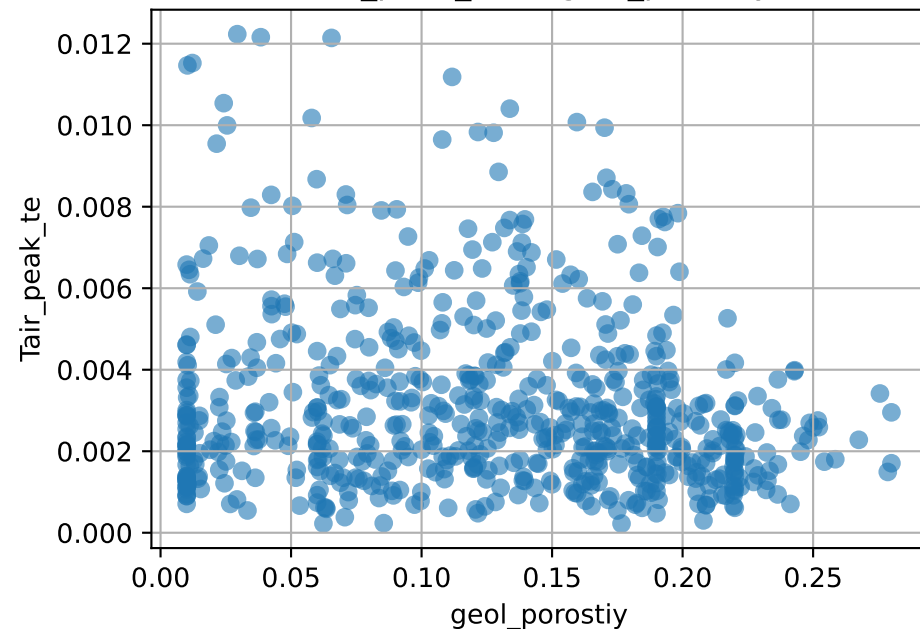
Tair_peak_te vs geol_porostiy
