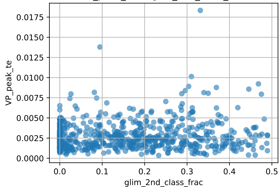
VP_peak_te vs glim_2nd_class_frac
