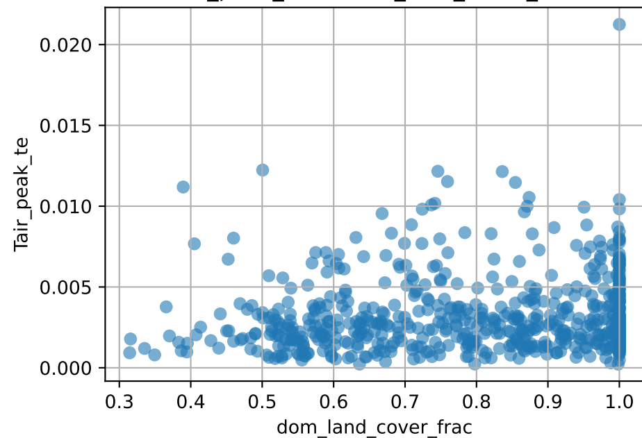
Tair_peak_te vs dom_land_cover_frac
