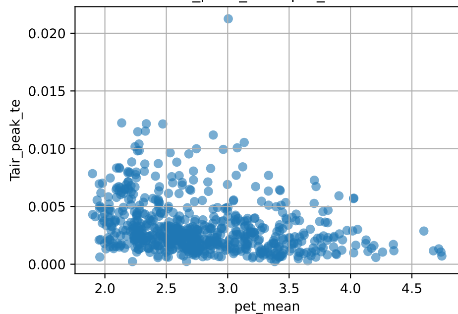
Tair_peak_te vs pet_mean
