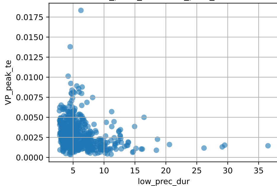
VP_peak_te vs low_prec_dur
