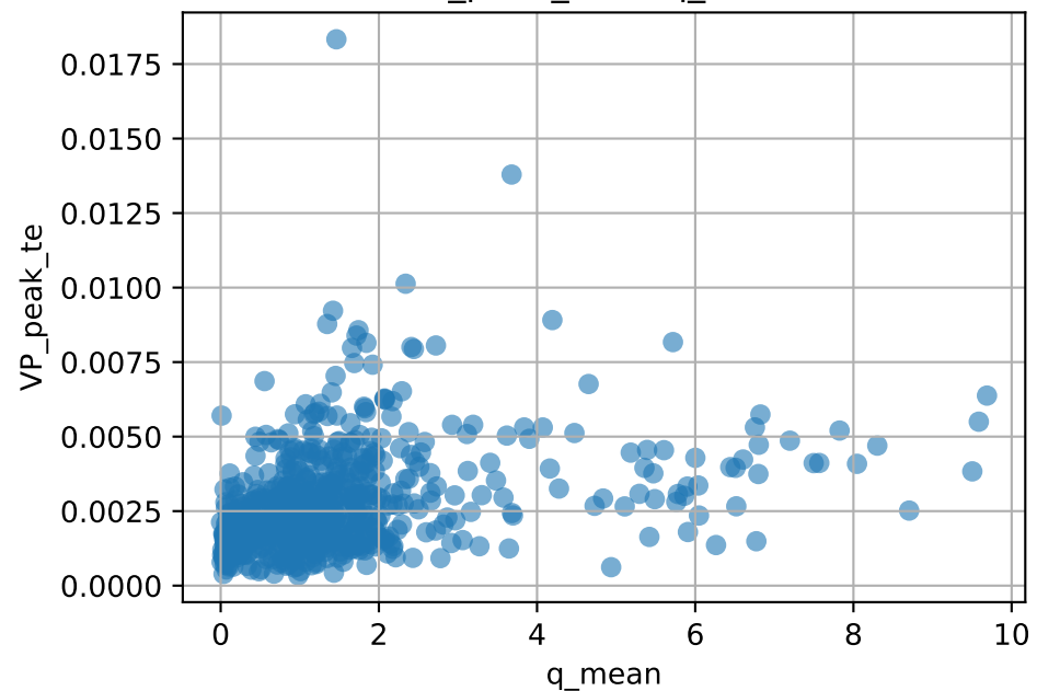
VP_peak_te vs q_mean
