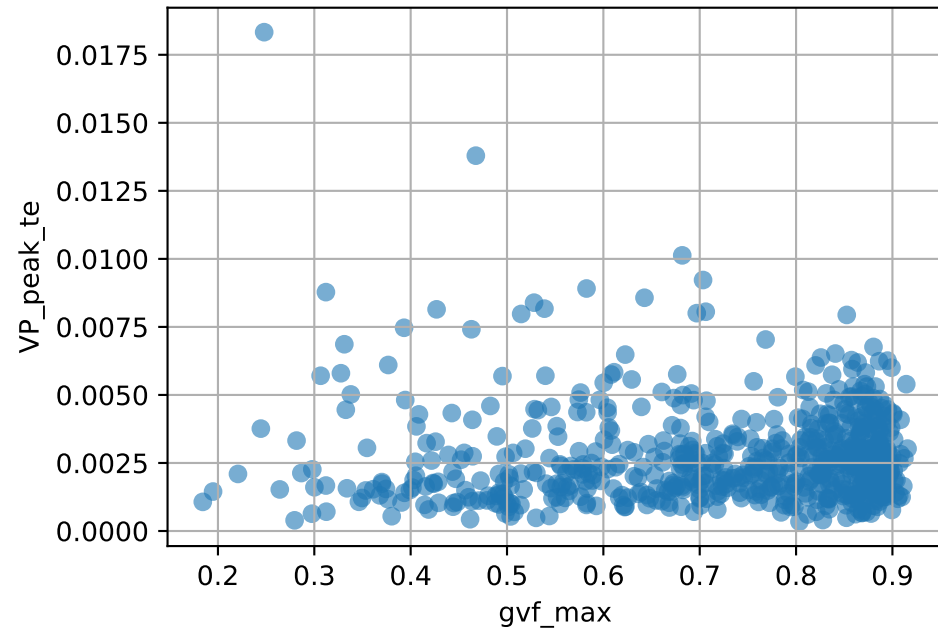
VP_peak_te vs gvf_max
