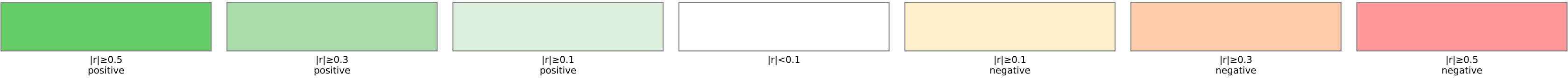
Comparison Table — PRCP (All forcings vs Dominant forcing only)
