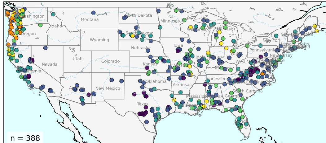
PRCP-dominant basins
