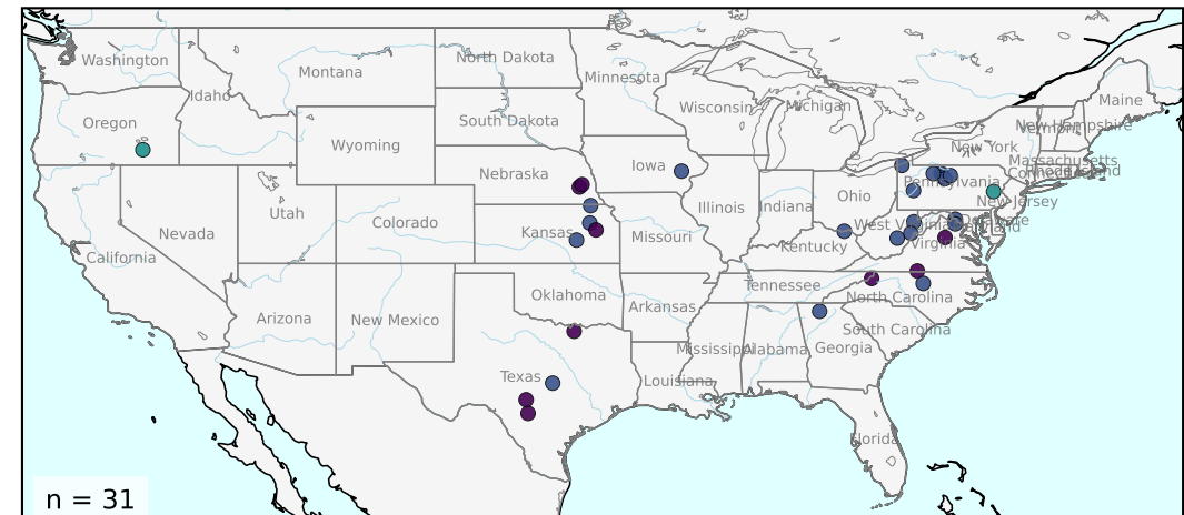
VP-dominant basins
