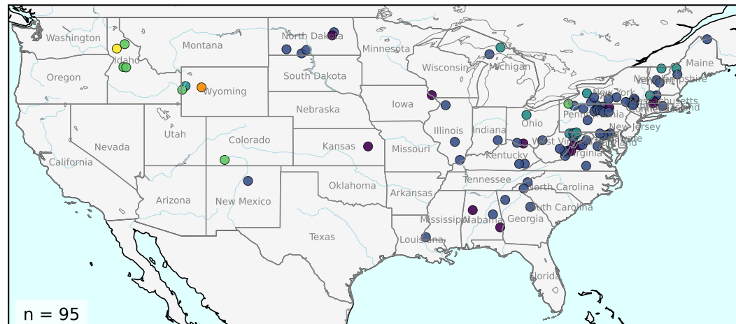
Tair-dominant basins
