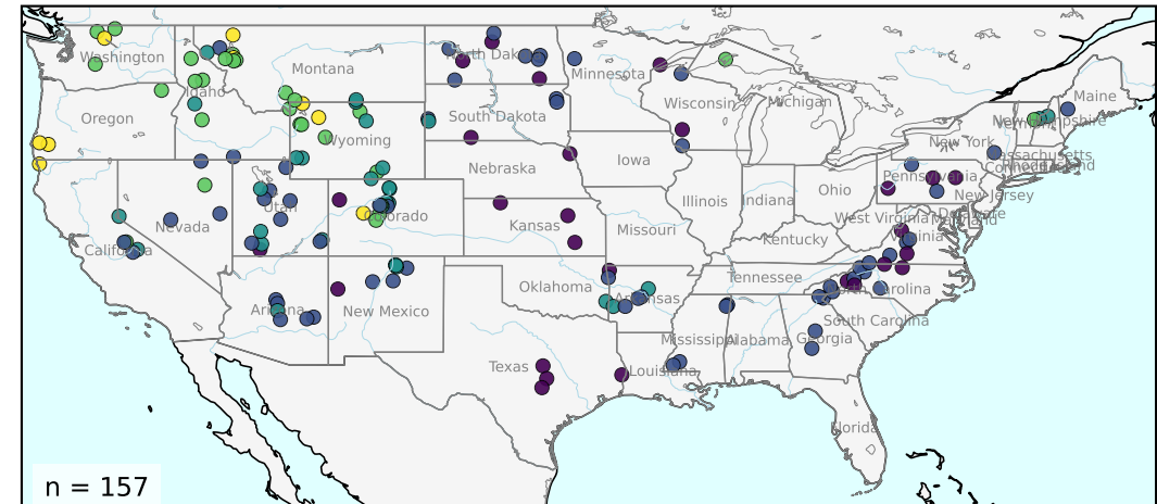
SRAD-dominant basins
