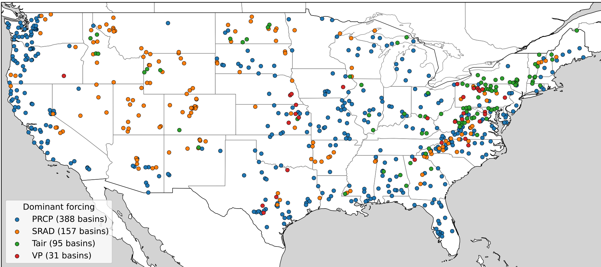
Dominant forcing for each of the 671 CAMELS basins
