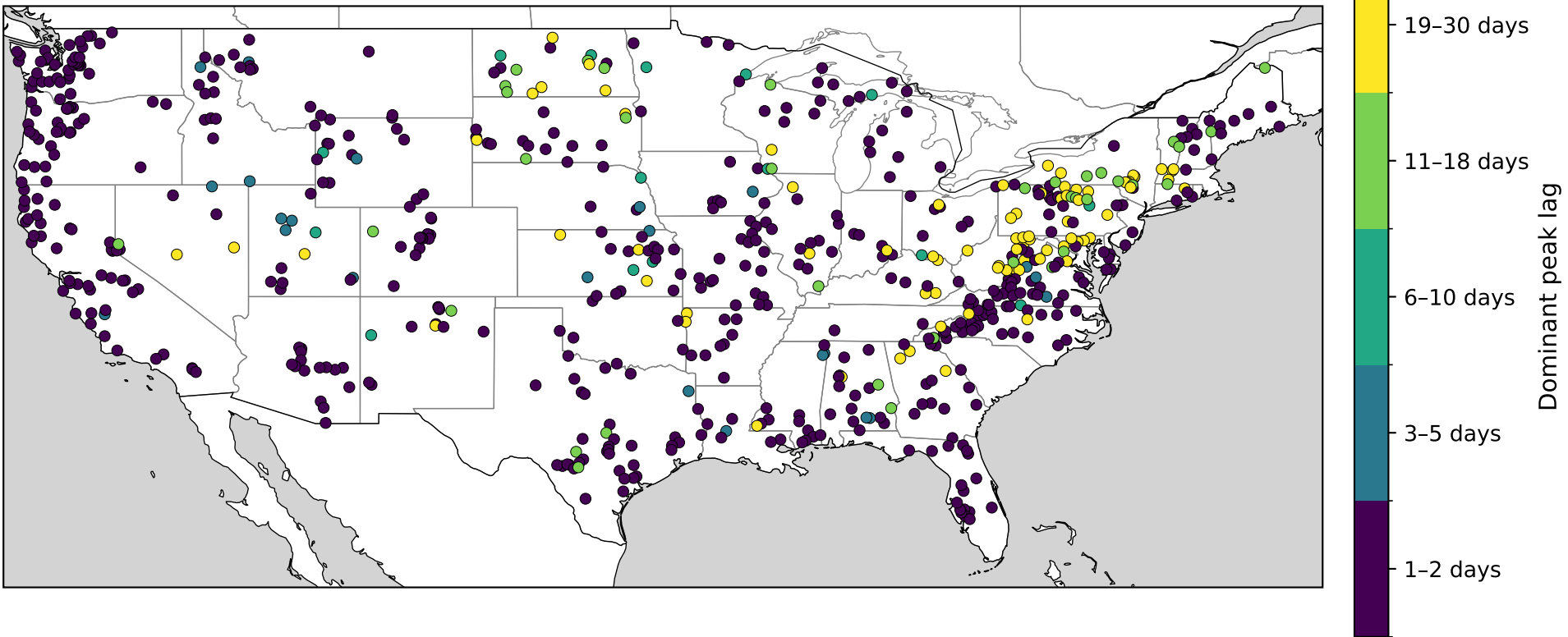
Dominant peak lag for each of the 671 CAMELS basins
