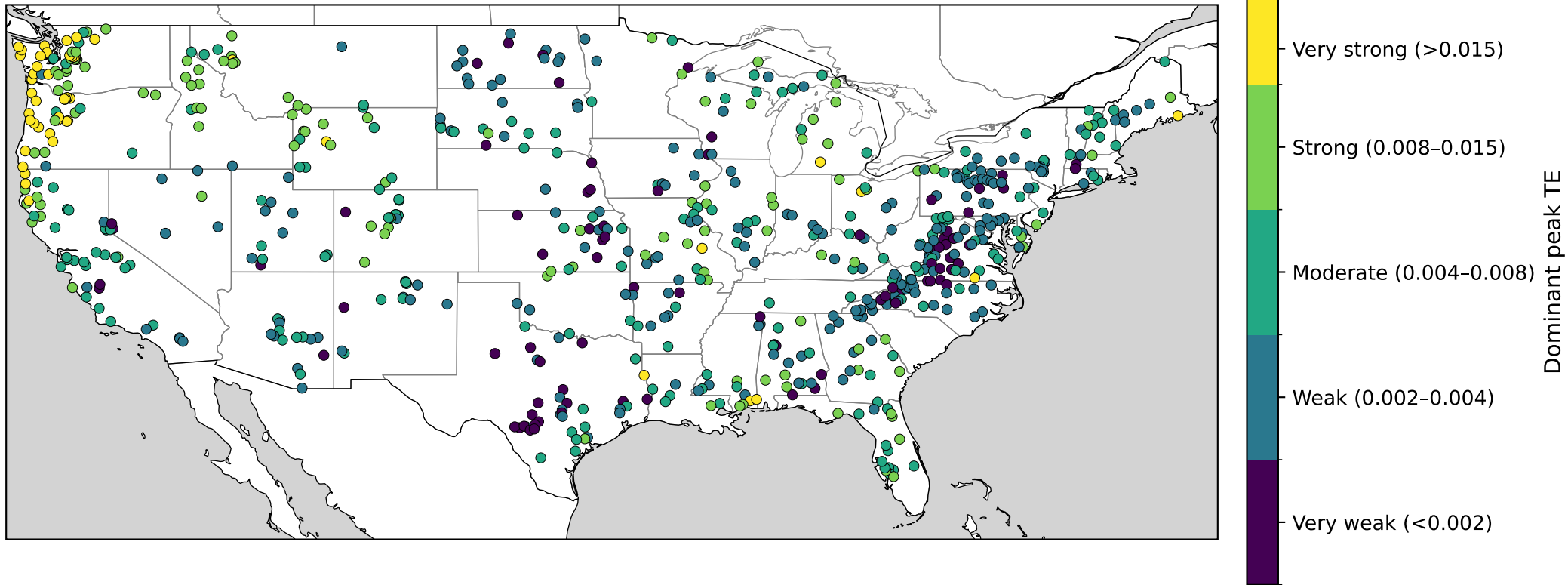
Dominant peak TE strength for each of the 671 CAMELS basins
