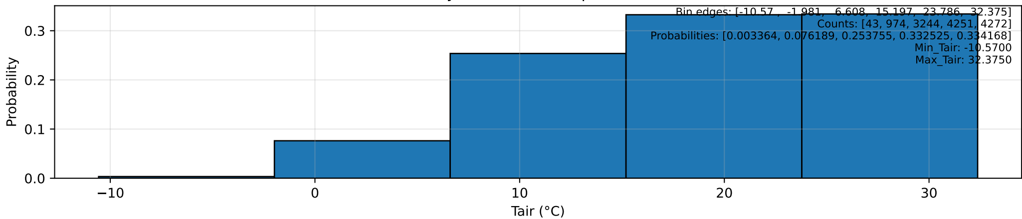
VP Probability Distribution (equal-width bins = 5)
