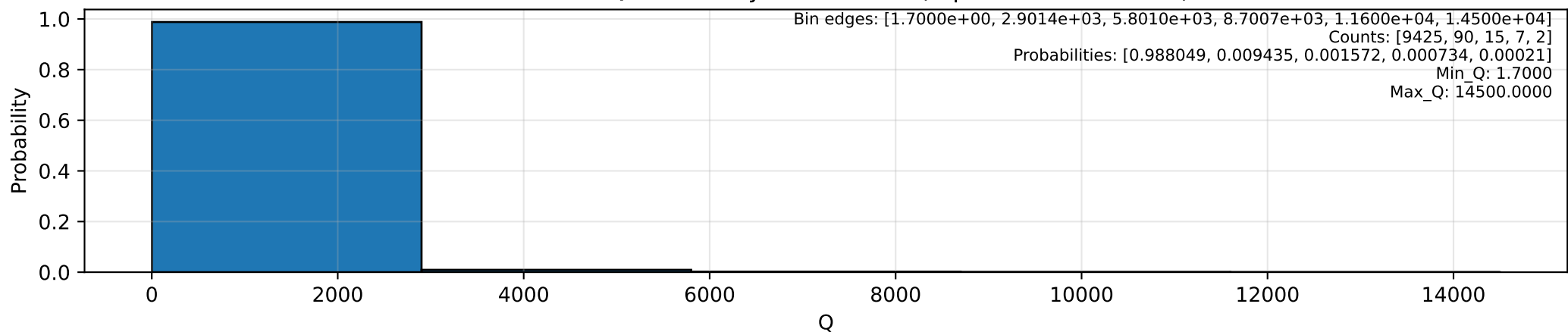
Streamflow Q Probability Distribution (equal-width bins = 5)
