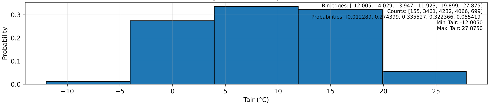
VP Probability Distribution (equal-width bins = 5)
