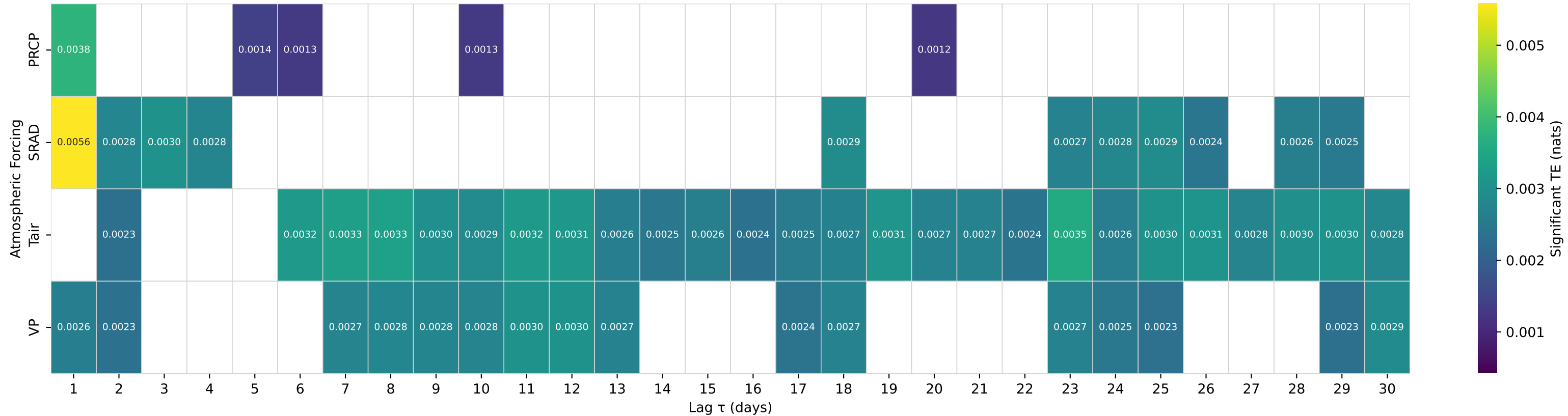
Shuffle-Test Significant TE to Streamflow — Basin 07340300 (HUC 11) — Cossatot River near Vandervoort, AR
