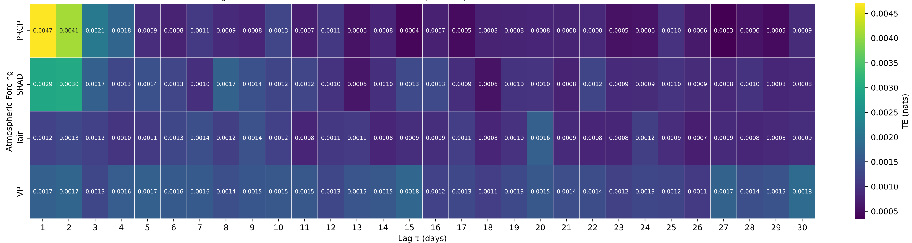
Shuffle-Test Significant TE to Streamflow — Basin 02297310 (HUC 03) — HORSE CREEK NEAR ARCADIA FL
