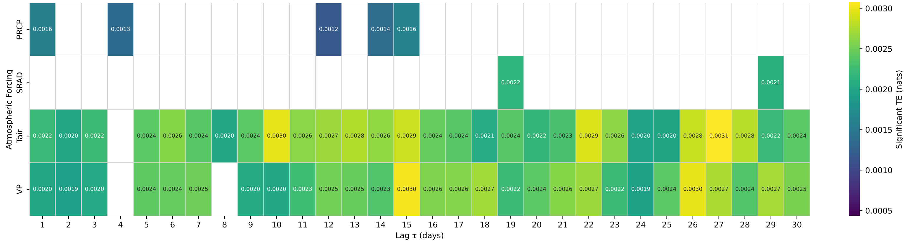
Shuffle-Test Significant TE to Streamflow — Basin 03368000 (HUC 05) — BRUSH CREEK NEAR NEBRASKA, IN
