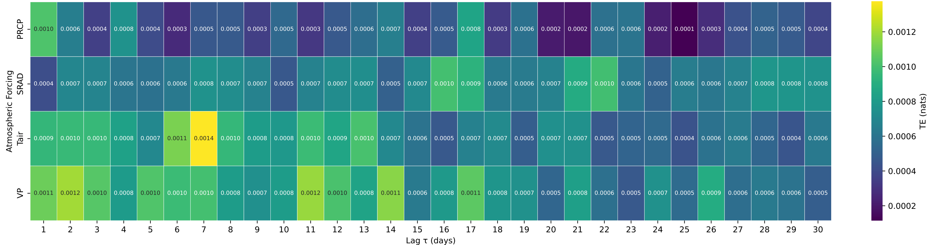
Shuffle-Test Significant TE to Streamflow — Basin 06910800 (HUC 10) — MARAIS DES CYGNES R NR READING, KS
