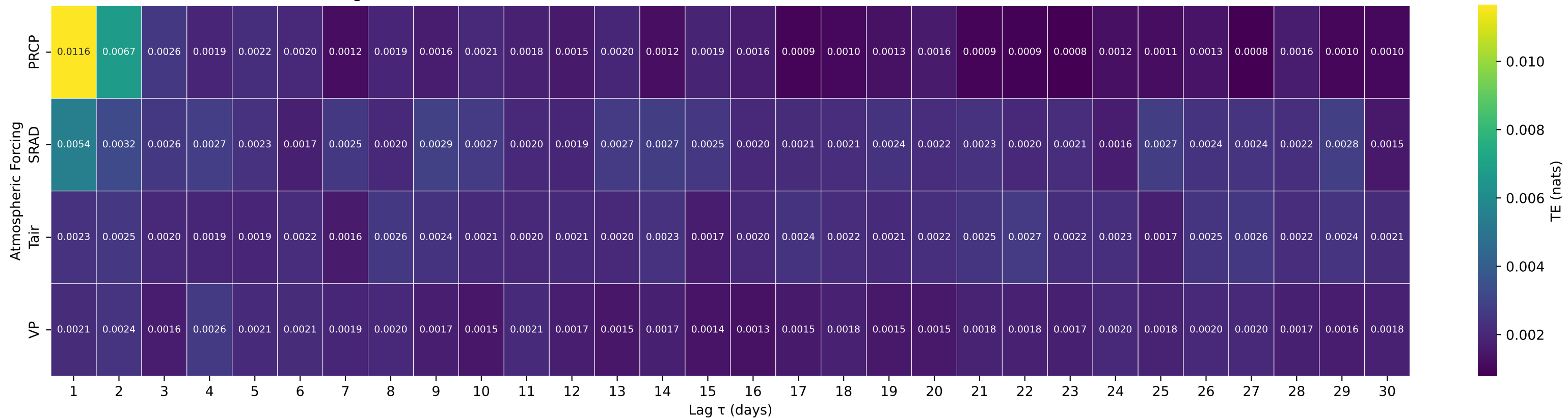
Shuffle-Test Significant TE to Streamflow — Basin 05466500 (HUC 07) — EDWARDS RIVER NEAR NEW BOSTON, IL
