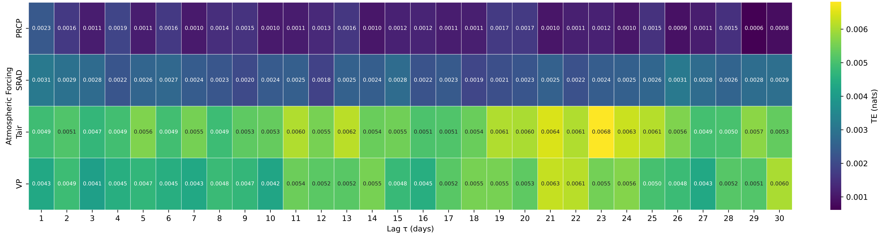
Shuffle-Test Significant TE to Streamflow — Basin 01333000 (HUC 02) — GREEN RIVER AT WILLIAMSTOWN, MA
