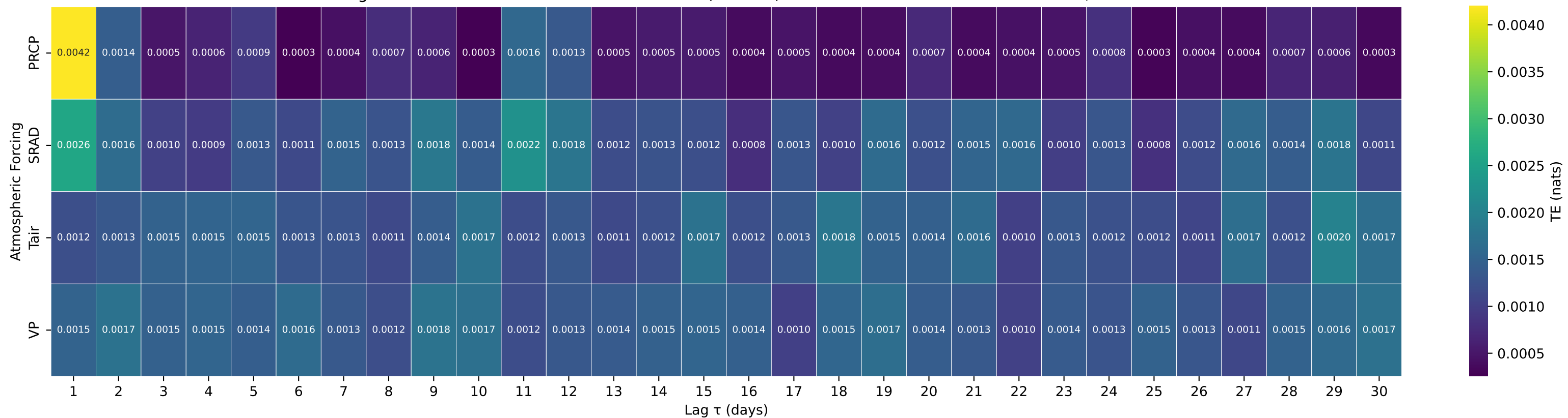
Shuffle-Test Significant TE to Streamflow — Basin 02198100 (HUC 03) — BEAVERDAM CREEK NEAR SARDIS, GA
