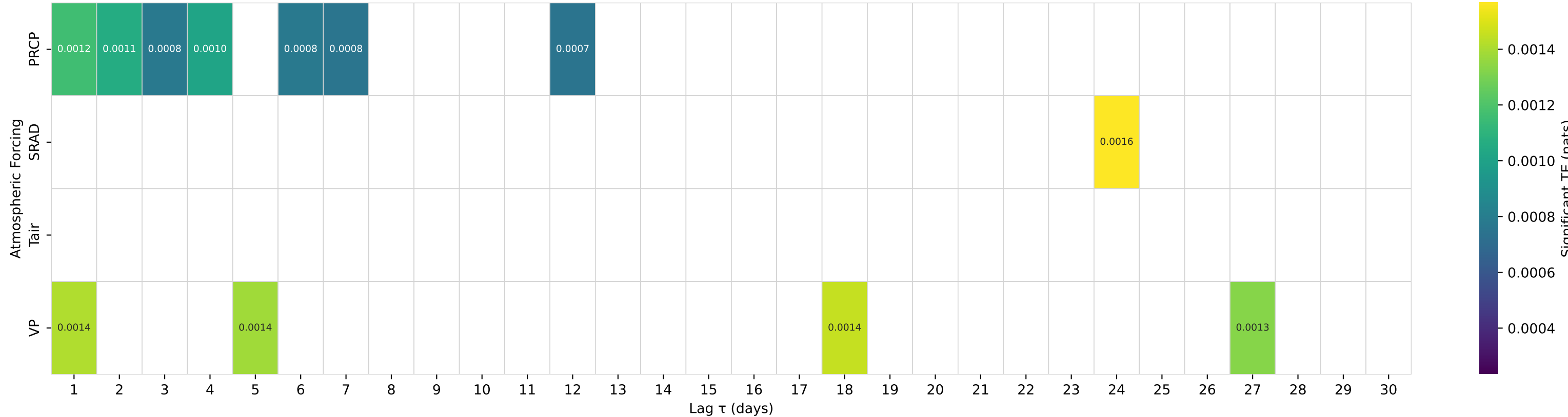
Shuffle-Test Significant TE to Streamflow — Basin 07167500 (HUC 11) — OTTER C AT CLIMAX, KS
