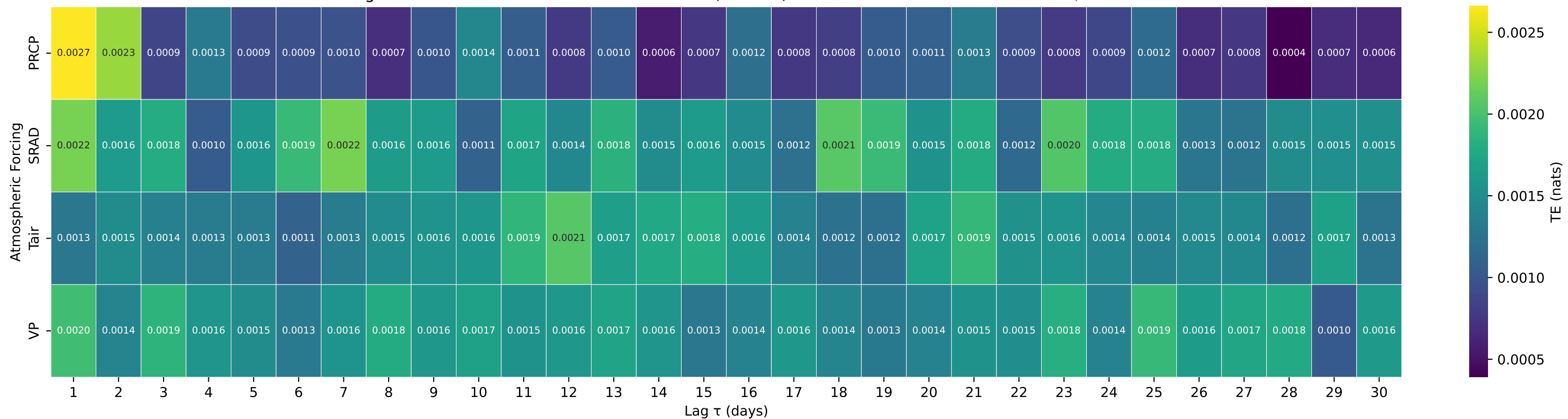
Shuffle-Test Significant TE to Streamflow — Basin 06921070 (HUC 10) — Pomme de Terre River near Polk, MO
