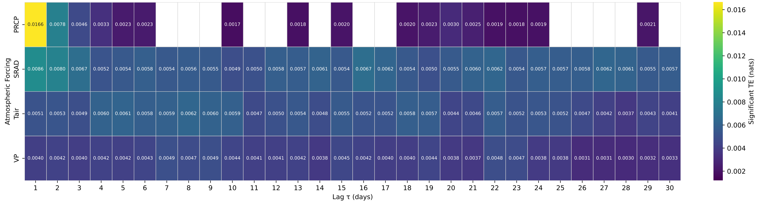
Shuffle-Test Significant TE to Streamflow — Basin 12145500 (HUC 17) — RAGING RIVER NEAR FALL CITY, WA
