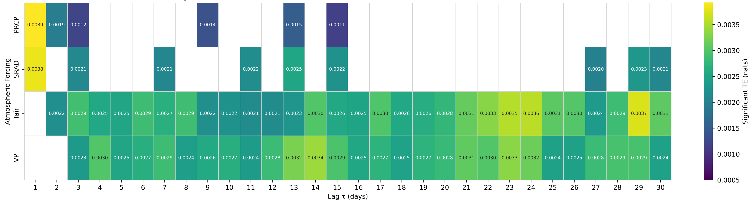
Shuffle-Test Significant TE to Streamflow — Basin 02408540 (HUC 03) — HATCHET CREEK BELOW ROCKFORD AL
