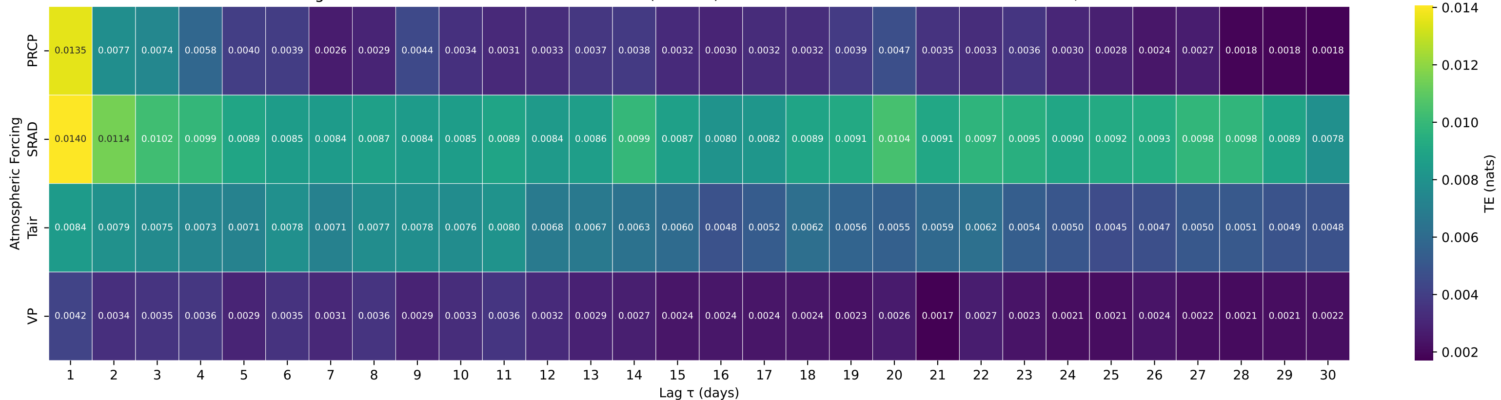
Shuffle-Test Significant TE to Streamflow — Basin 14309500 (HUC 17) — WEST FORK COW CREEK NEAR GLENDALE, OR
