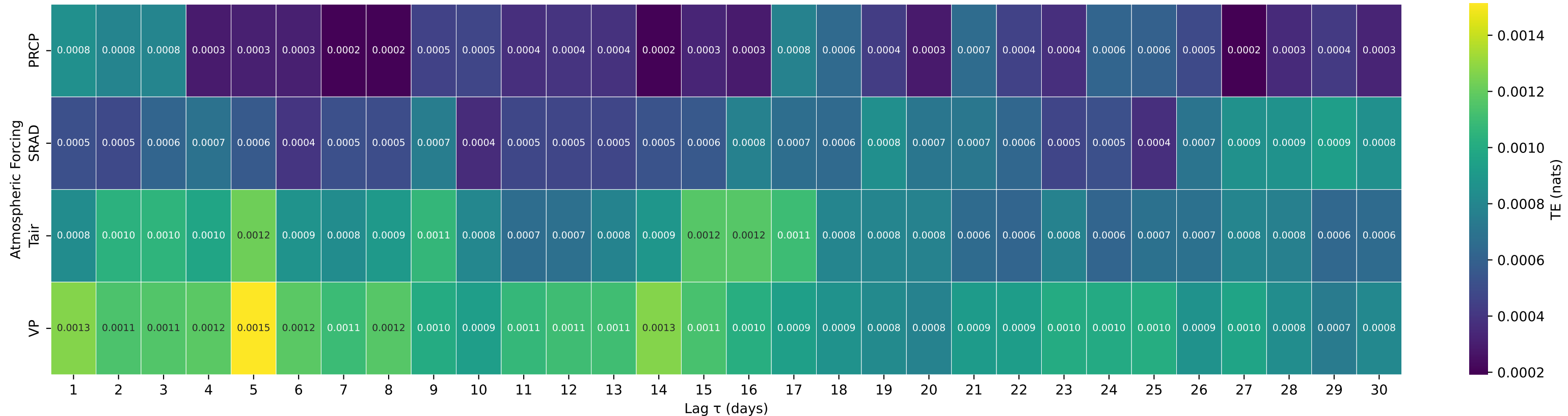
Shuffle-Test Significant TE to Streamflow — Basin 06803530 (HUC 10) — ROCK CREEK NEAR CERESCO, NEBR.
