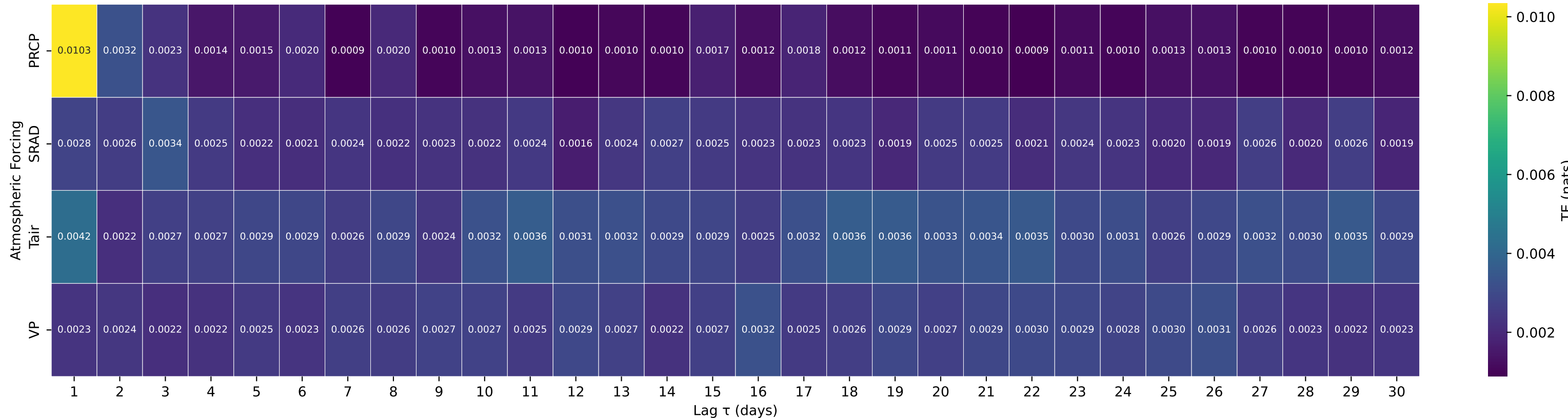
Shuffle-Test Significant TE to Streamflow — Basin 04115265 (HUC 04) — FISH CREEK NEAR CRYSTAL, MI
