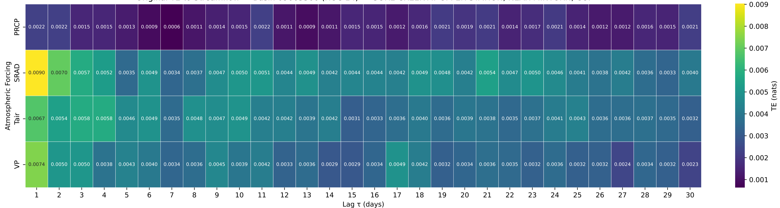
Shuffle-Test Significant TE to Streamflow — Basin 09065500 (HUC 14) — GORE CREEK AT UPPER STATION, NEAR MINTURN, CO.
