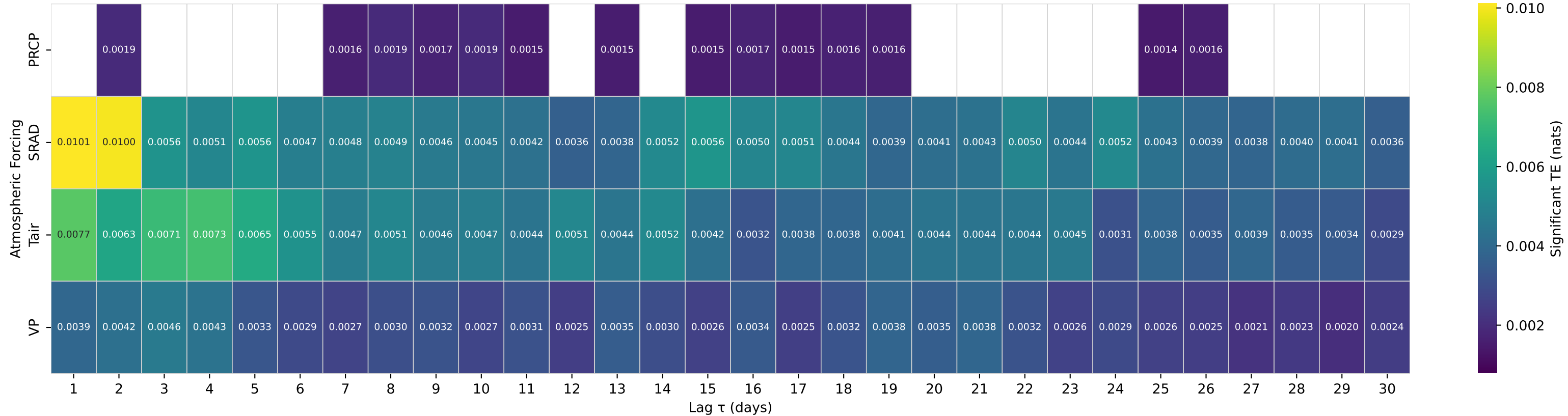
Shuffle-Test Significant TE to Streamflow — Basin 06191500 (HUC 10) — Yellowstone River at Corwin Springs MT
