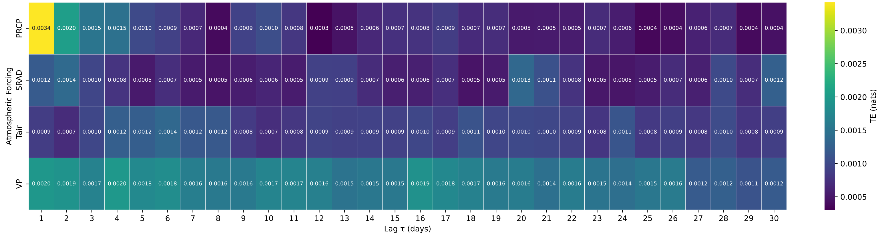
Shuffle-Test Significant TE to Streamflow — Basin 08380500 (HUC 13) — GALLINAS CREEK NEAR MONTEZUMA, NM
