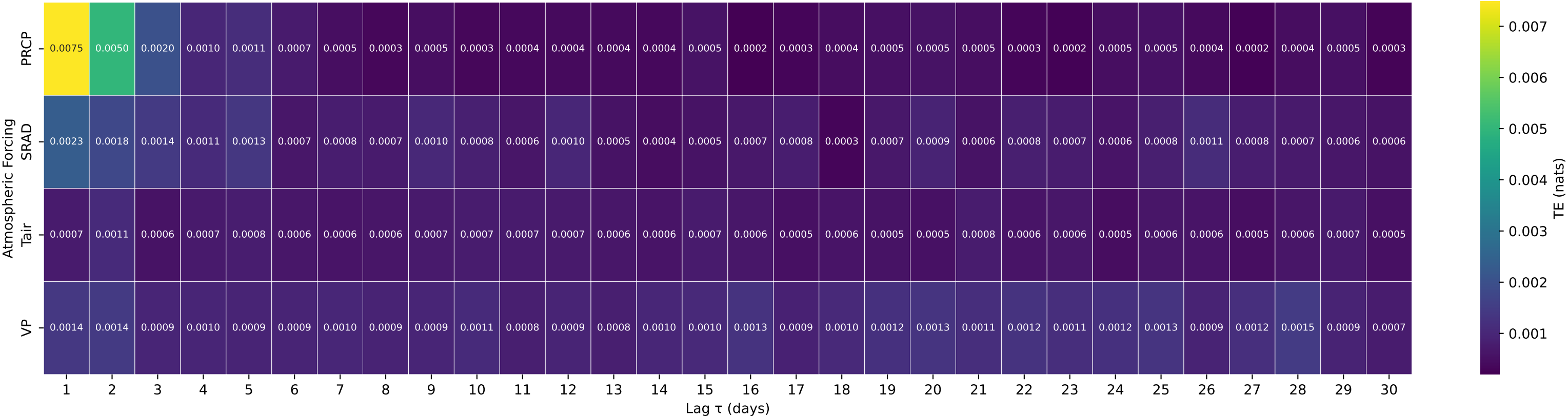
Shuffle-Test Significant TE to Streamflow — Basin 08189500 (HUC 12) — Mission Rv at Refugio, TX
