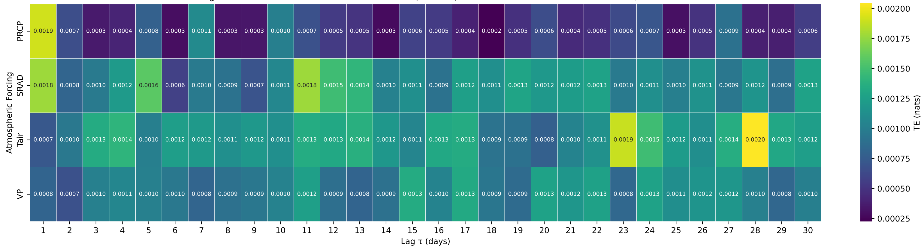
Shuffle-Test Significant TE to Streamflow — Basin 01583500 (HUC 02) — WESTERN RUN AT WESTERN RUN, MD
