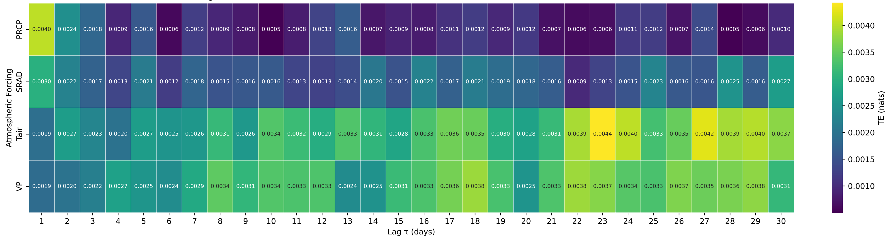
Shuffle-Test Significant TE to Streamflow — Basin 03281100 (HUC 05) — GOOSE CREEK AT MANCHESTER, KY
