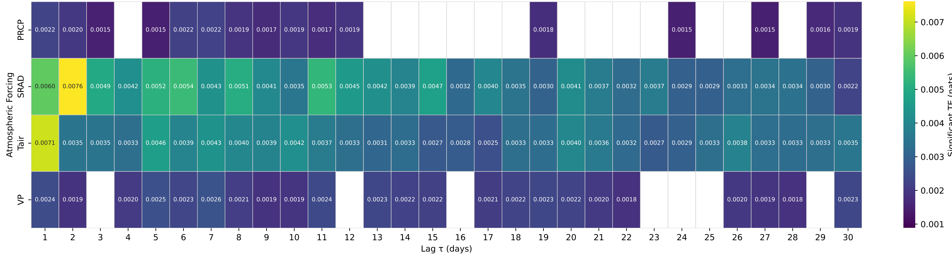
Shuffle-Test Significant TE to Streamflow — Basin 09210500 (HUC 14) — FONTENELLE C NR HERSCHLER RANCH, NR FONTENELLE, WY
