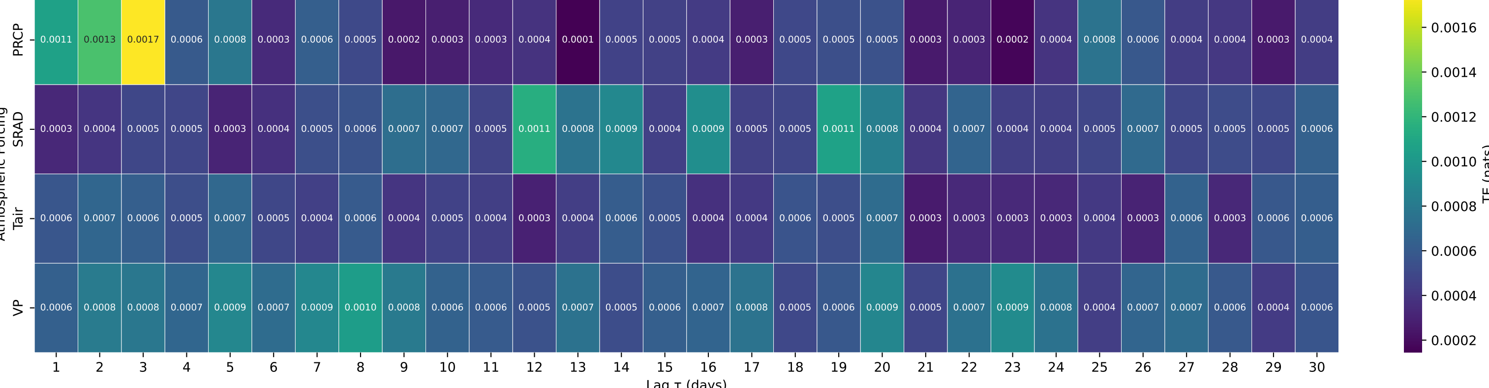
Original TE to Streamflow — Basin 07142300 (HUC 11) — RATTLESNAKE C NR MACKSVILLE, KS
