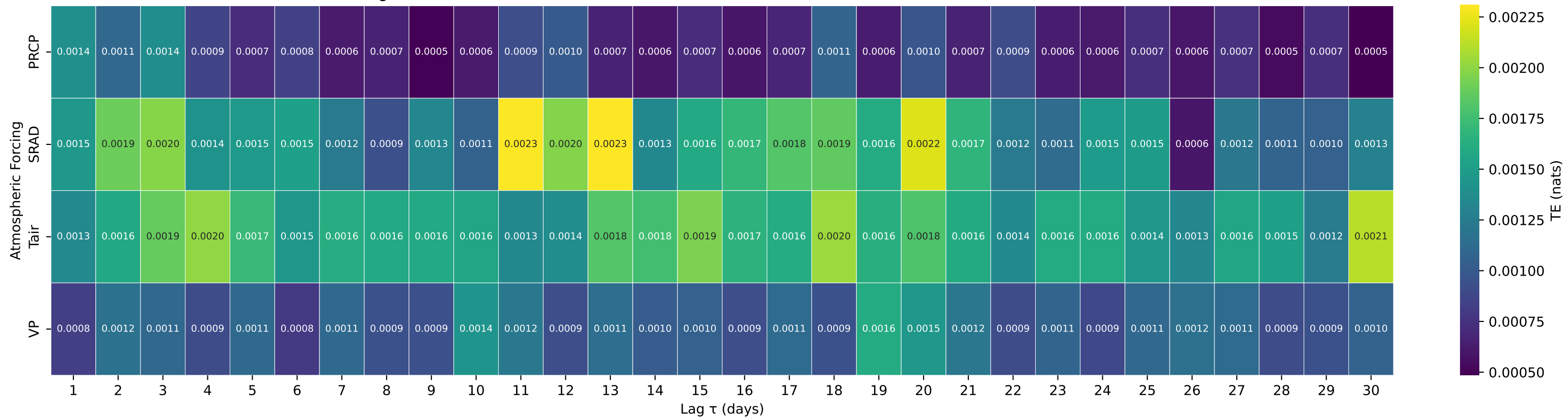
Shuffle-Test Significant TE to Streamflow — Basin 05057200 (HUC 09) — BALDHILL CREEK NR DAZEY, ND
