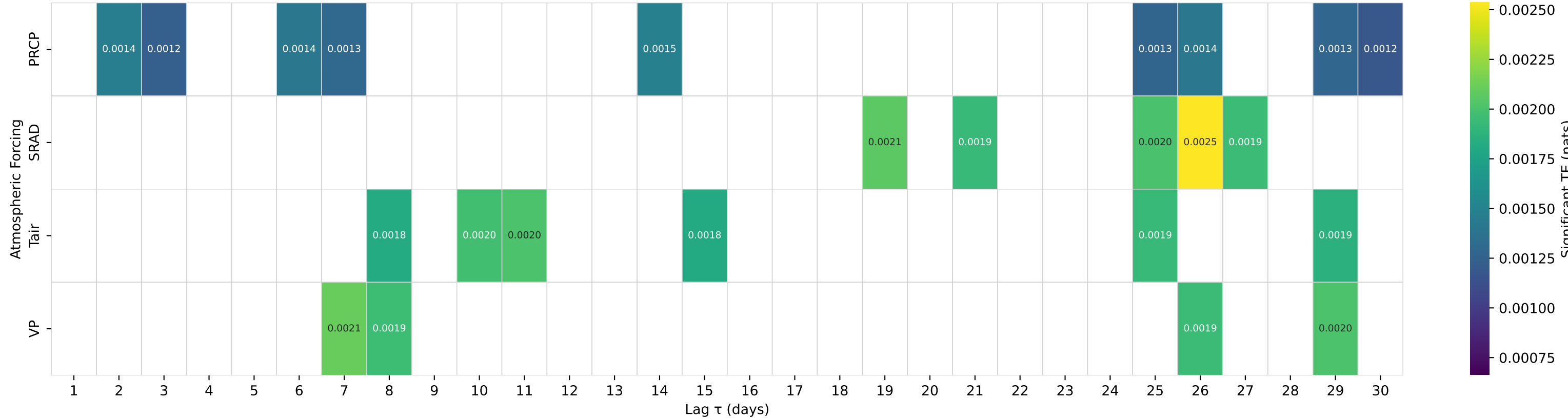
Shuffle-Test Significant TE to Streamflow — Basin 07196900 (HUC 11) — Baron Fork at Dutch Mills, AR
