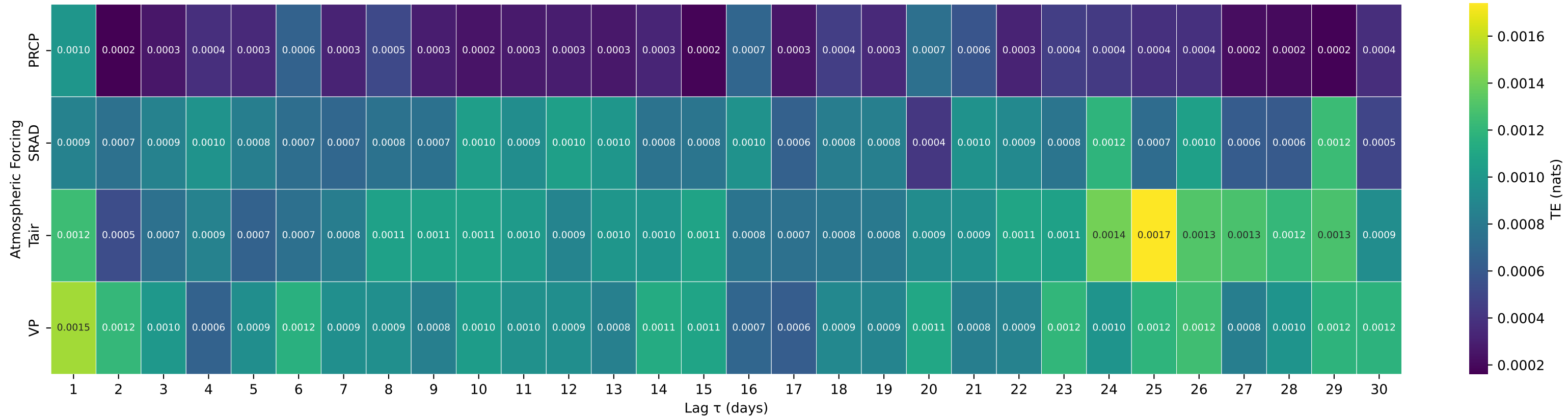
Shuffle-Test Significant TE to Streamflow — Basin 02011400 (HUC 02) — JACKSON RIVER NEAR BACOVA, VA
