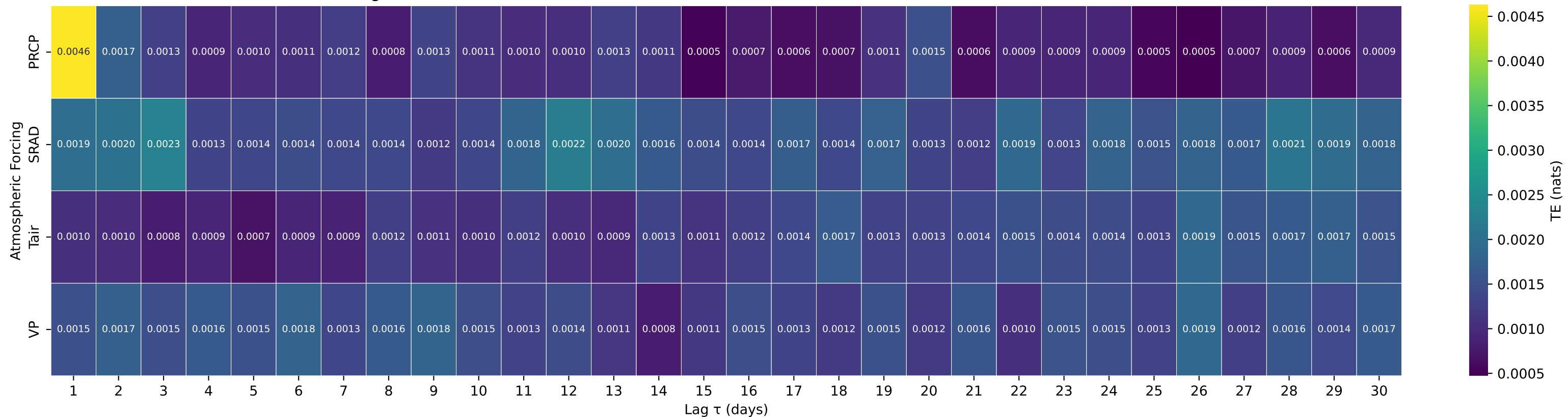
Shuffle-Test Significant TE to Streamflow — Basin 05495500 (HUC 07) — BEAR CREEK NEAR MARCELLINE, IL
