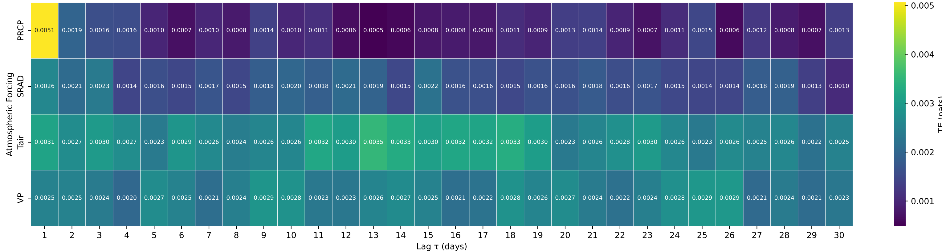
Shuffle-Test Significant TE to Streamflow — Basin 01439500 (HUC 02) — Bush Kill at Shoemakers, PA
