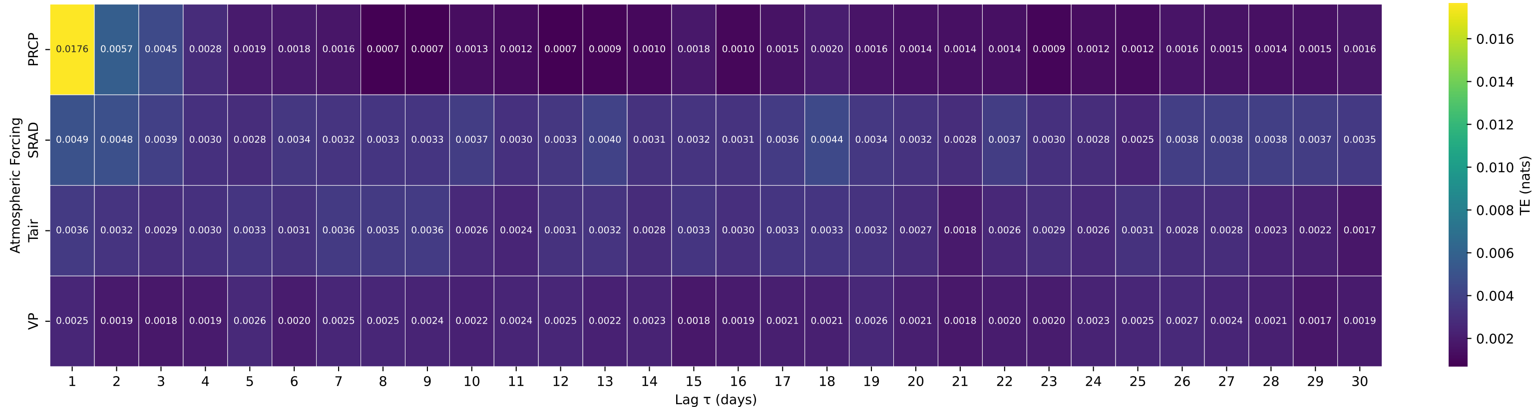
Shuffle-Test Significant TE to Streamflow — Basin 12143600 (HUC 17) — SF SNOQUALMIE RIVER AT EDGEWICK, WA
