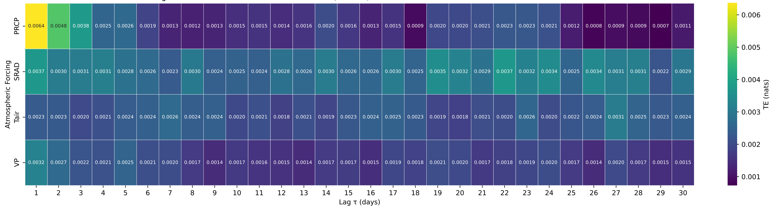
Shuffle-Test Significant TE to Streamflow — Basin 11180960 (HUC 18) — CULL C AB CULL C RES NR CASTRO VALLEY CA
