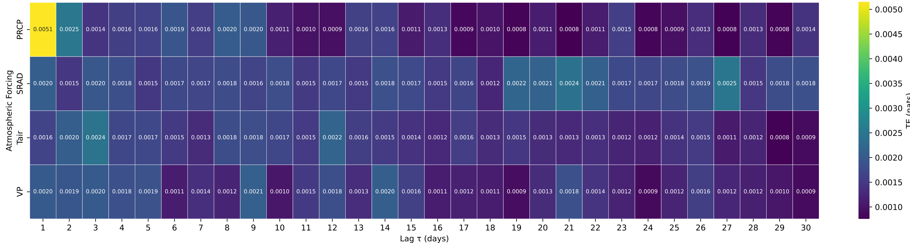
Shuffle-Test Significant TE to Streamflow — Basin 06406000 (HUC 10) — BATTLE CR AT HERMOSA SD
