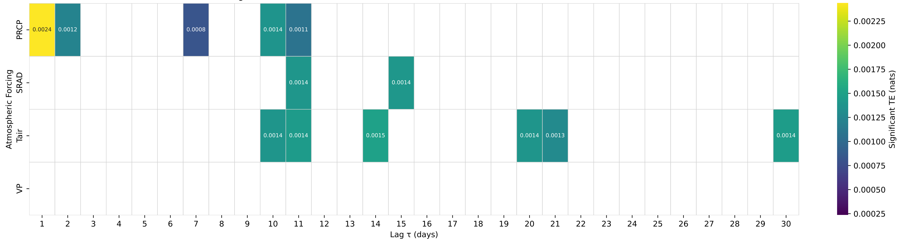
Shuffle-Test Significant TE to Streamflow — Basin 06339100 (HUC 10) — KNIFE RIVER AT MANNING, ND
