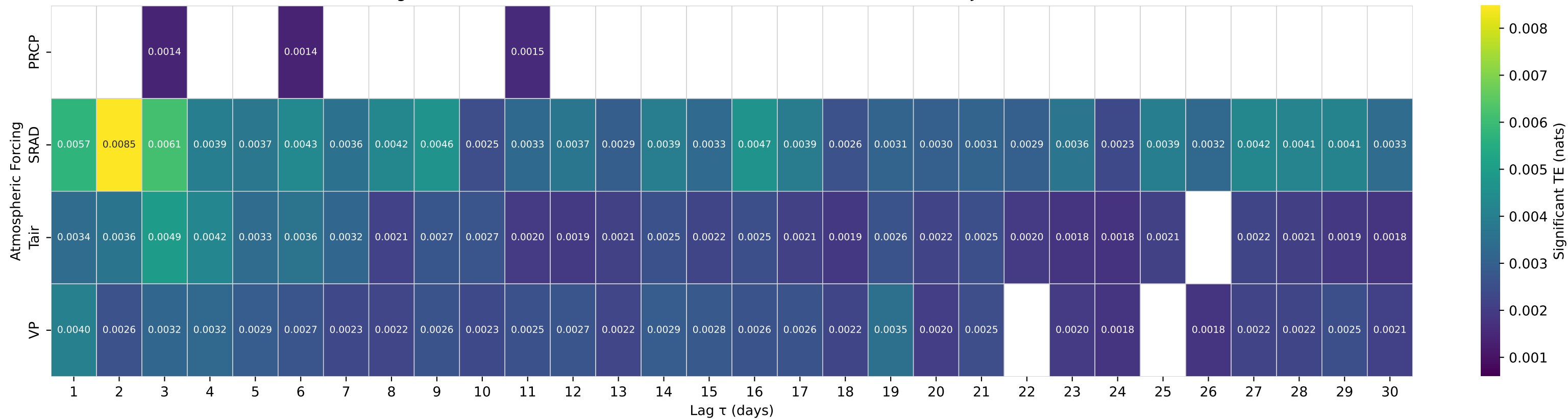
Shuffle-Test Significant TE to Streamflow — Basin 12381400 (HUC 17) — South Fork Jocko River near Arlee MT
