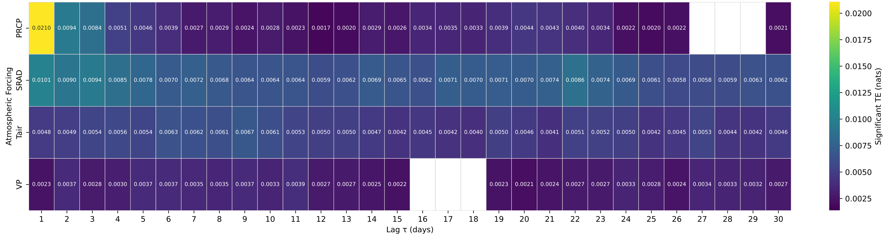
Shuffle-Test Significant TE to Streamflow — Basin 14306340 (HUC 17) — EAST FORK LOBSTER CREEK NEAR ALSEA, OR.
