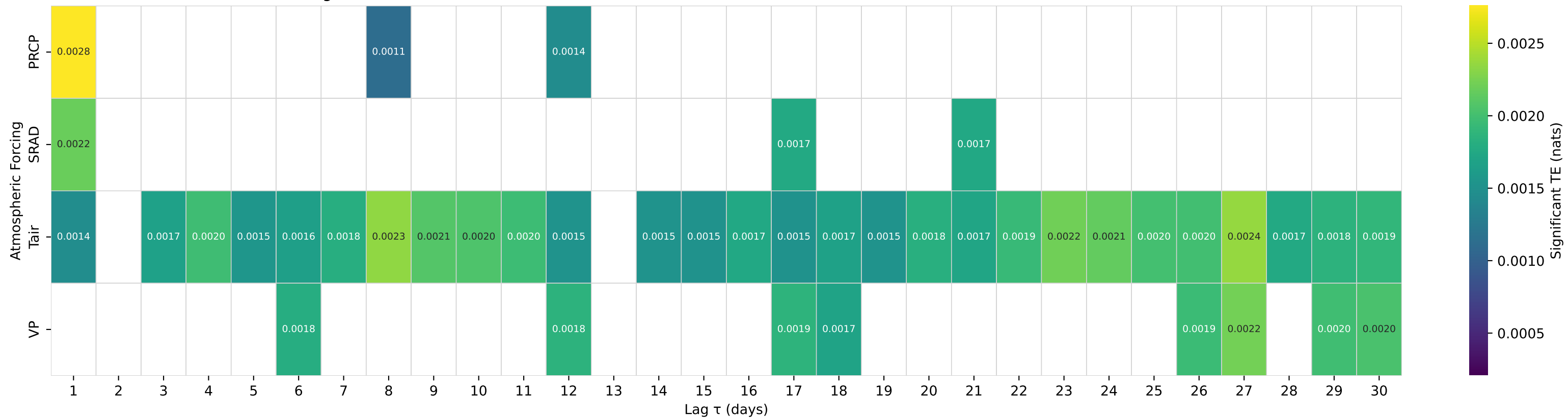
Shuffle-Test Significant TE to Streamflow — Basin 03471500 (HUC 06) — S F HOLSTON RIVER AT RIVERSIDE NR CHILHOWIE, VA
