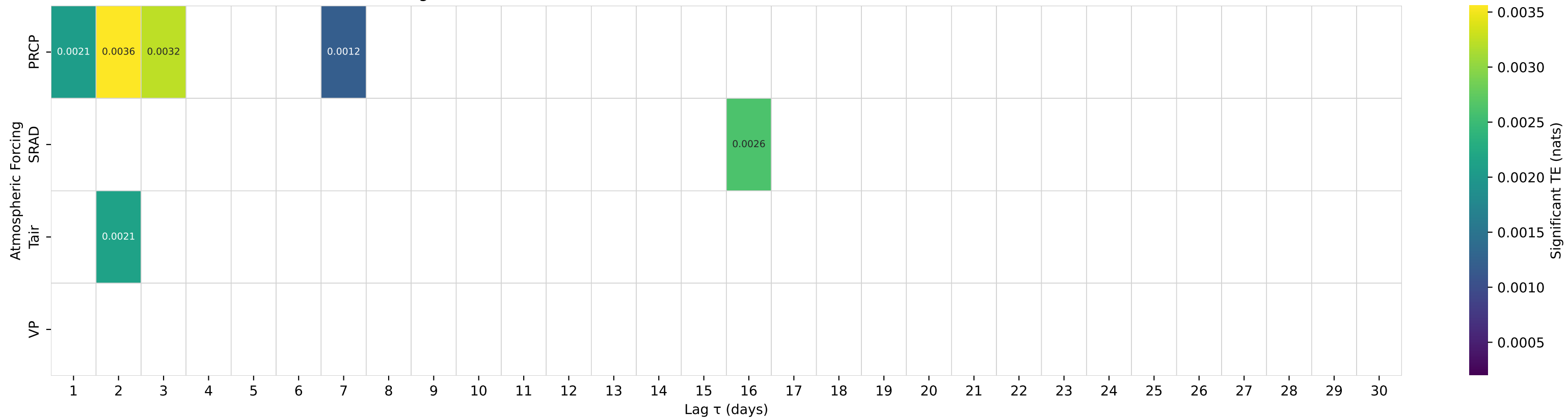
Shuffle-Test Significant TE to Streamflow — Basin 05087500 (HUC 09) — MIDDLE RIVER AT ARGYLE, MN
