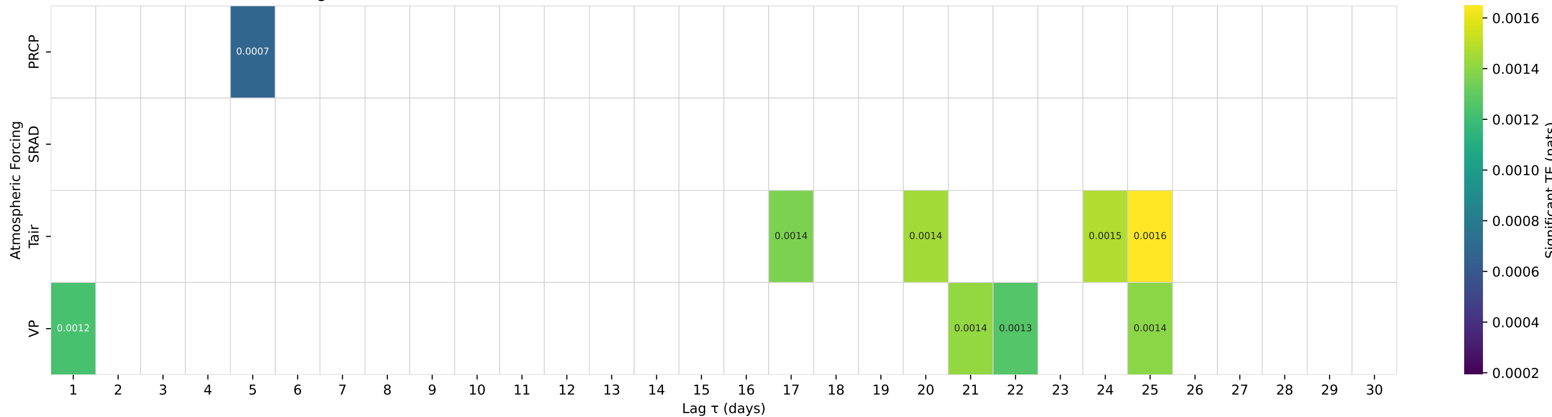
Shuffle-Test Significant TE to Streamflow — Basin 01181000 (HUC 01) — WEST BRANCH WESTFIELD RIVER AT HUNTINGTON, MA
