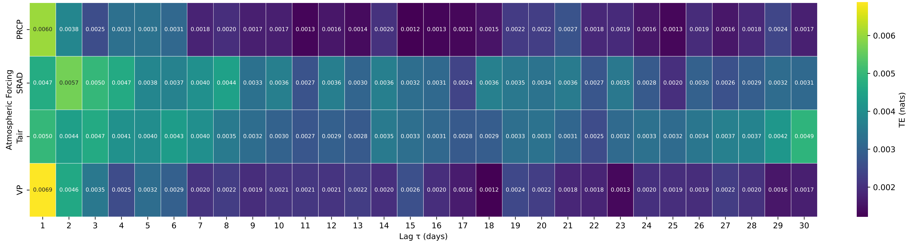
Shuffle-Test Significant TE to Streamflow — Basin 10396000 (HUC 17) — DONNER UND BLITZEN RIVER NR FRENCHGLEN OR
