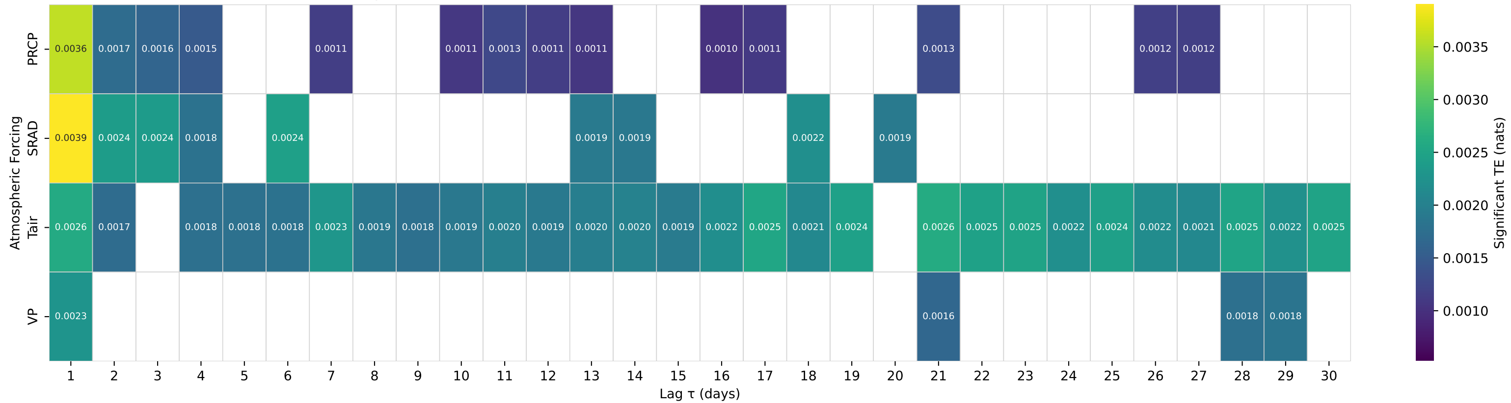
Shuffle-Test Significant TE to Streamflow — Basin 09494000 (HUC 15) — WHITE RIVER NEAR FORT APACHE, AZ.
