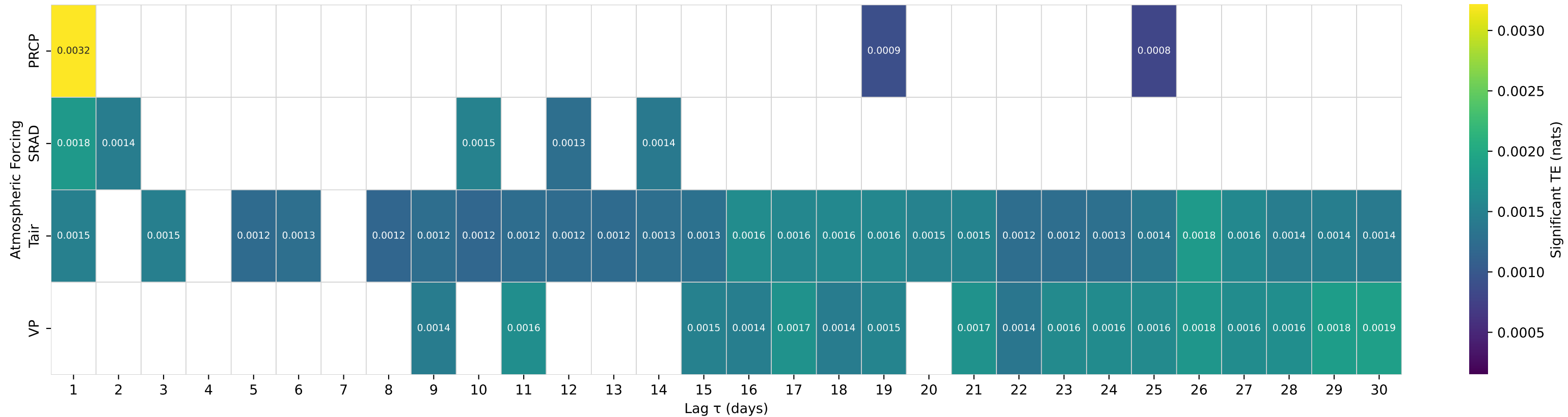
Shuffle-Test Significant TE to Streamflow — Basin 02479155 (HUC 03) — CYPRESS CREEK NR JANICE, MS
