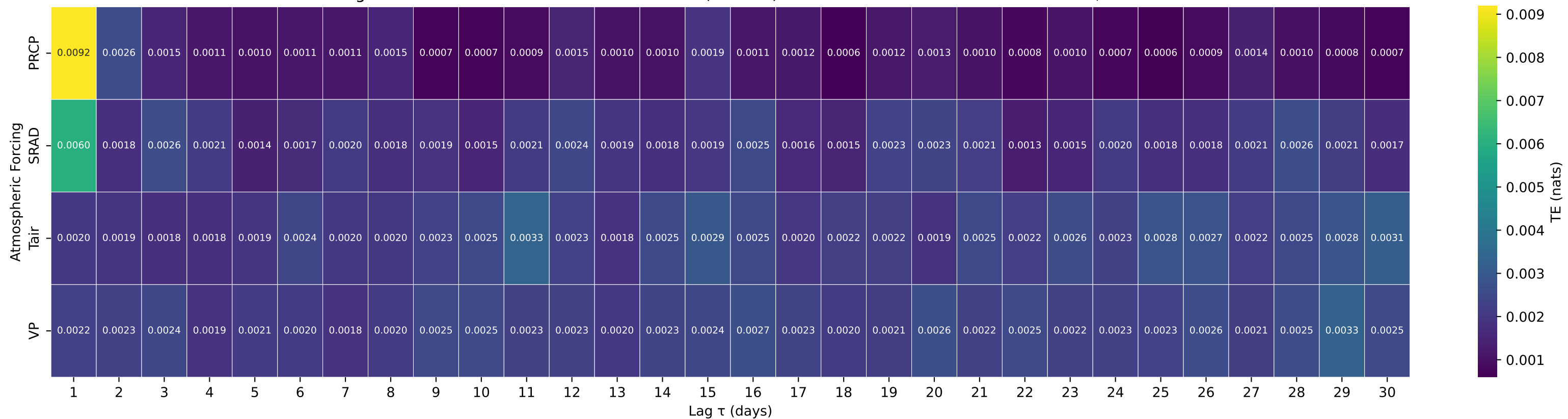
Shuffle-Test Significant TE to Streamflow — Basin 02221525 (HUC 03) — MURDER CREEK BELOW EATONTON, GA
