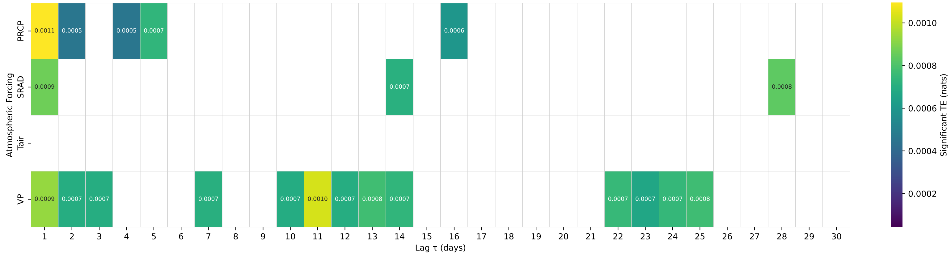
Shuffle-Test Significant TE to Streamflow — Basin 08196000 (HUC 12) — Dry Frio Rv nr Reagan Wells, TX
