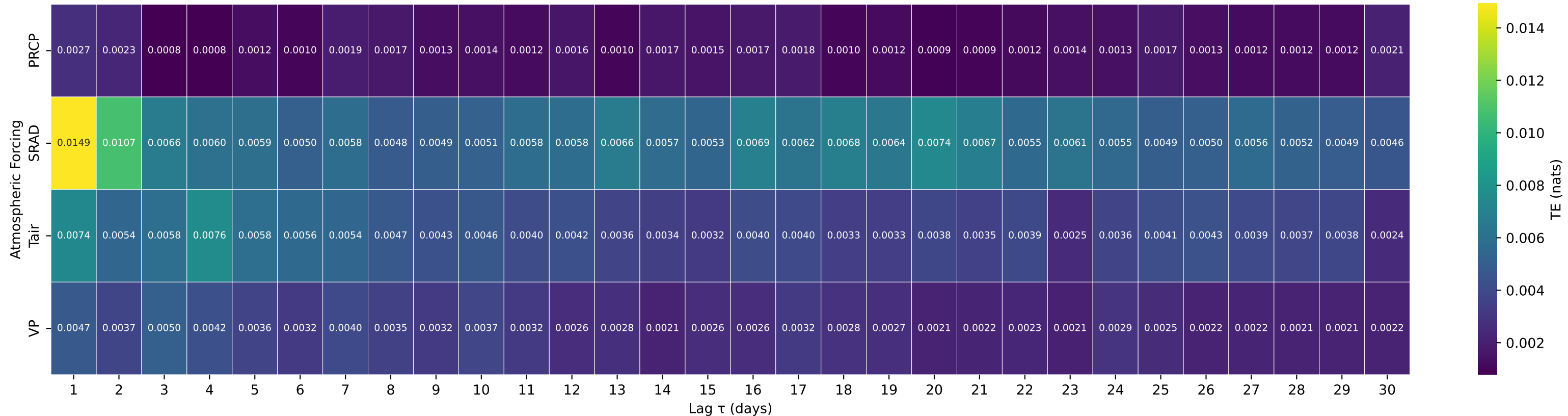
Shuffle-Test Significant TE to Streamflow — Basin 06280300 (HUC 10) — SOUTH FORK SHOSHONE RIVER NEAR VALLEY, WY
