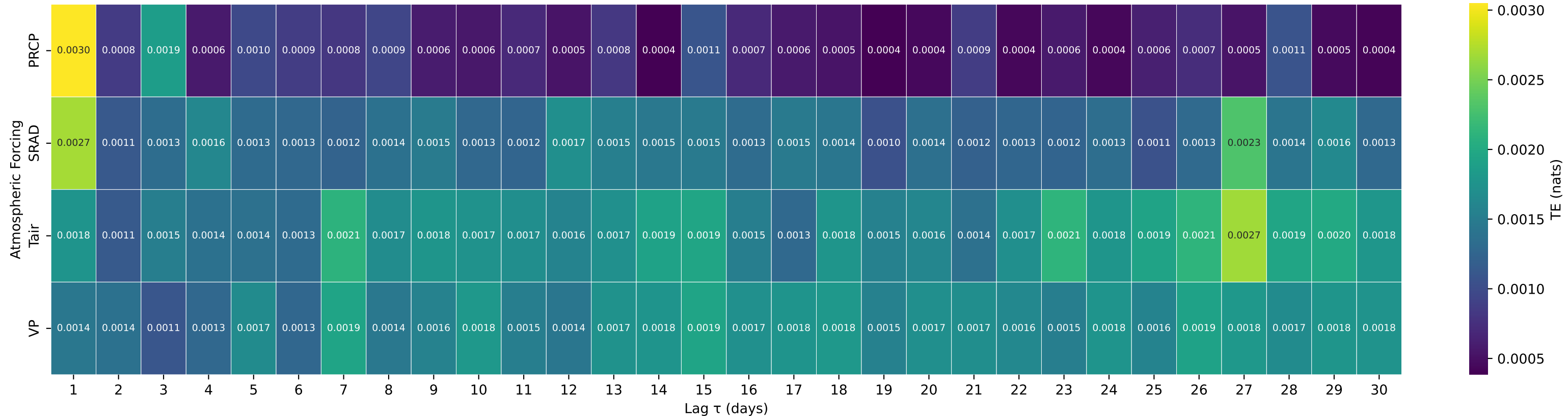
Shuffle-Test Significant TE to Streamflow — Basin 03357350 (HUC 05) — PLUM CREEK NEAR BAINBRIDGE, IND.
