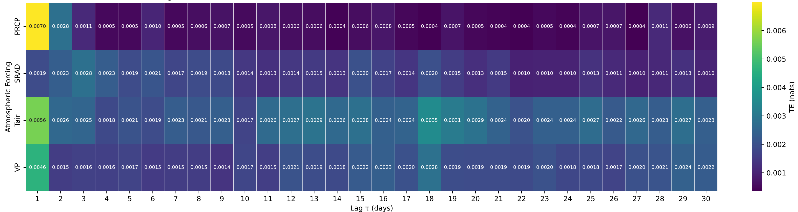
Shuffle-Test Significant TE to Streamflow — Basin 04256000 (HUC 04) — INDEPENDENCE RIVER AT DONNATTSBURG NY
