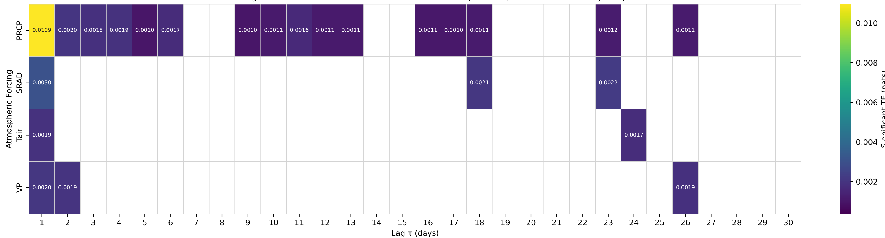
Shuffle-Test Significant TE to Streamflow — Basin 05495000 (HUC 07) — Fox River at Wayland, MO
