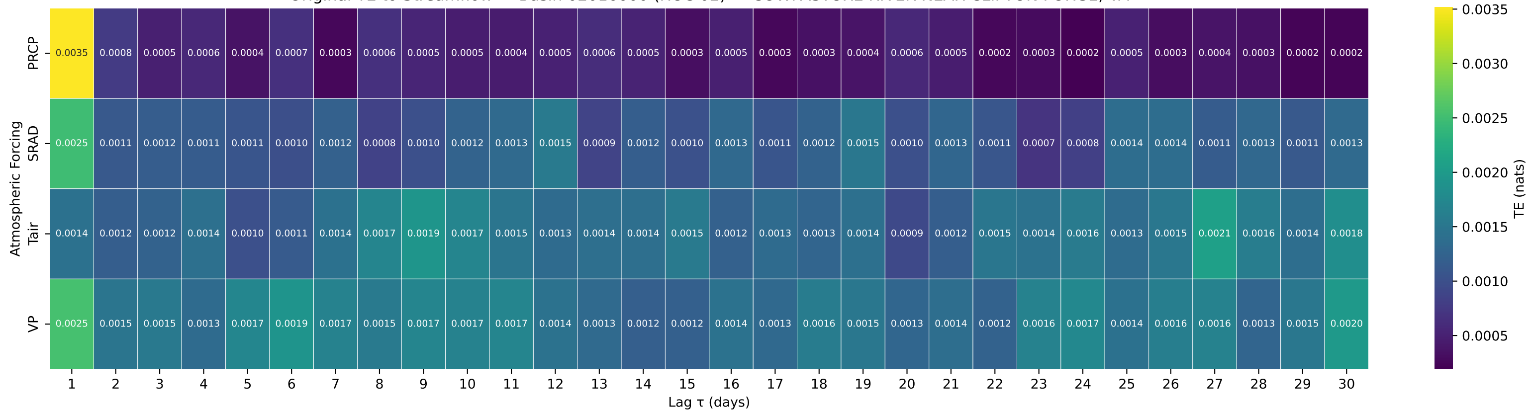
Shuffle-Test Significant TE to Streamflow — Basin 02016000 (HUC 02) — COWPASTURE RIVER NEAR CLIFTON FORGE, VA
