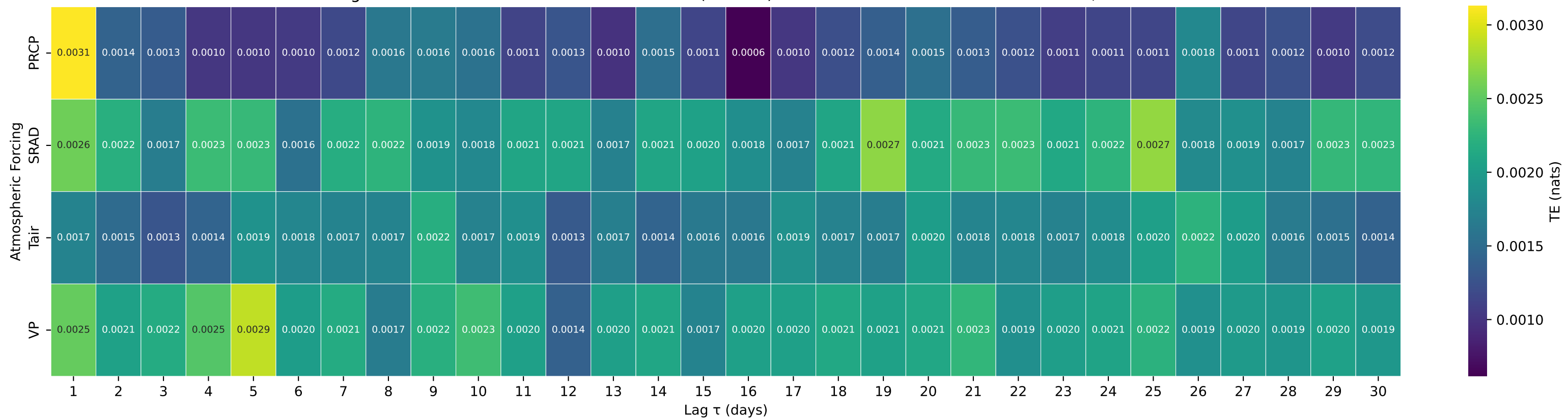
Shuffle-Test Significant TE to Streamflow — Basin 02112360 (HUC 03) — MITCHELL RIVER NEAR STATE ROAD, NC
