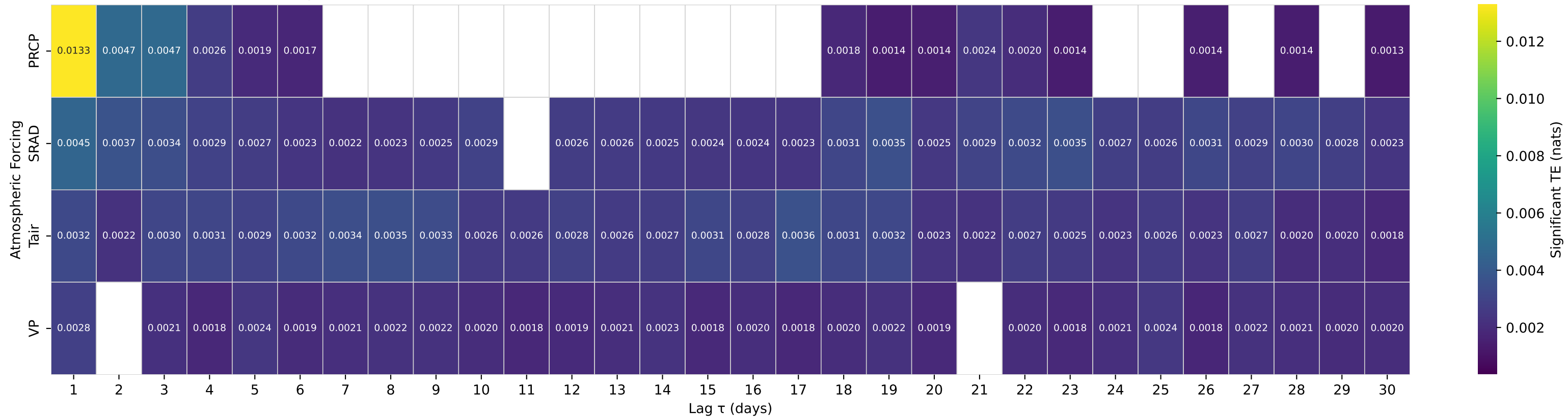
Shuffle-Test Significant TE to Streamflow — Basin 12114500 (HUC 17) — CEDAR RIVER BELOW BEAR CREEK NEAR CEDAR FALLS, WA
