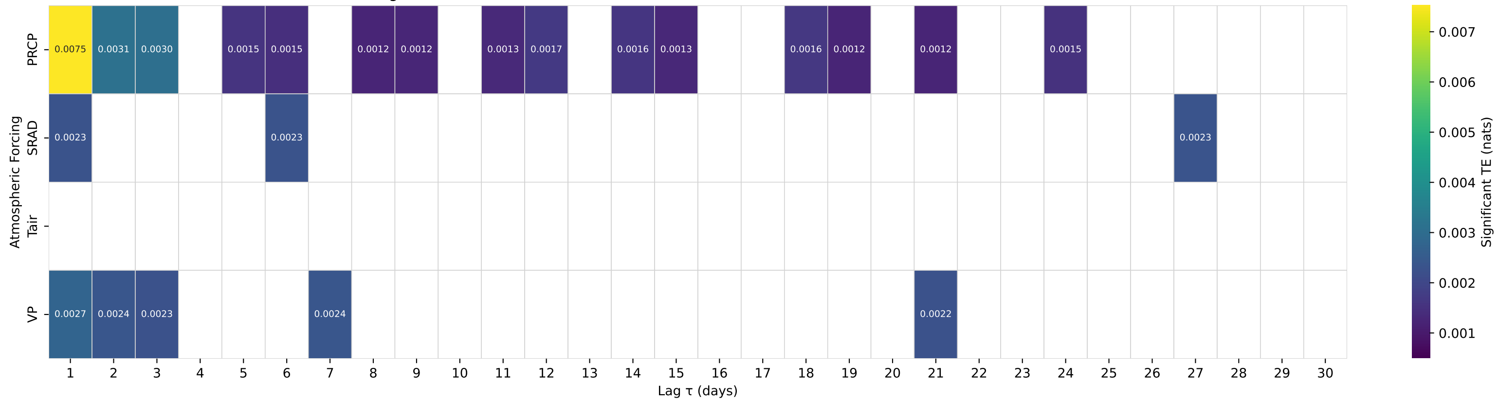
Shuffle-Test Significant TE to Streamflow — Basin 06892000 (HUC 10) — STRANGER C NR TONGANOXIE, KS
