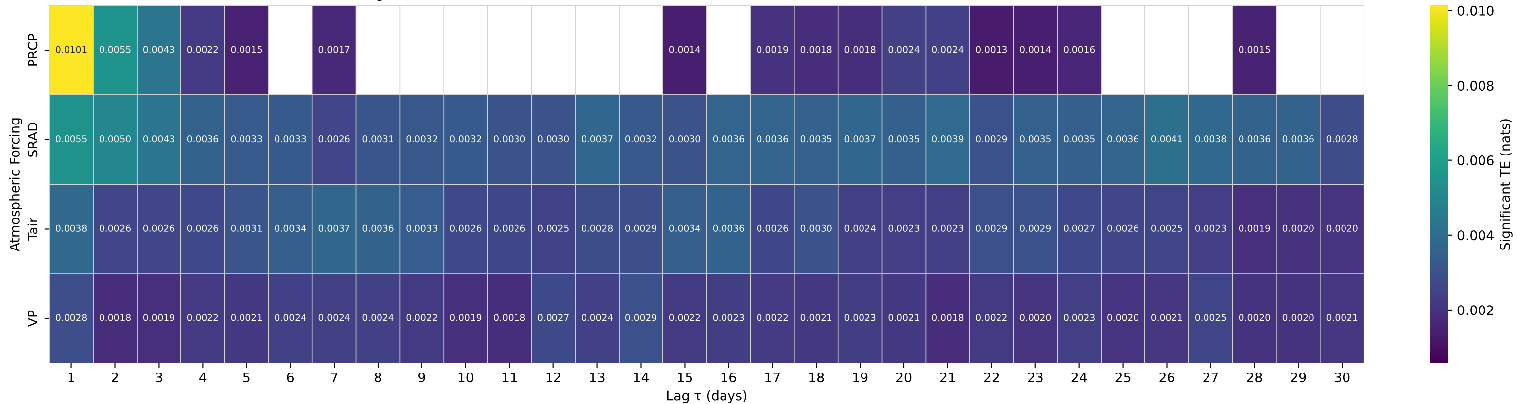
Shuffle-Test Significant TE to Streamflow — Basin 12082500 (HUC 17) — NISQUALLY RIVER NEAR NATIONAL, WA
