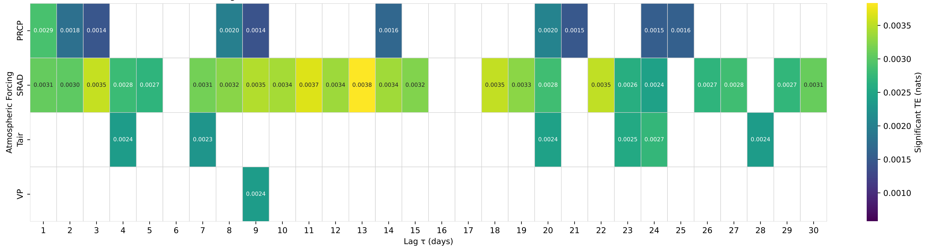
Shuffle-Test Significant TE to Streamflow — Basin 07208500 (HUC 11) — RAYADO CREEK NEAR CIMARRON, NM
