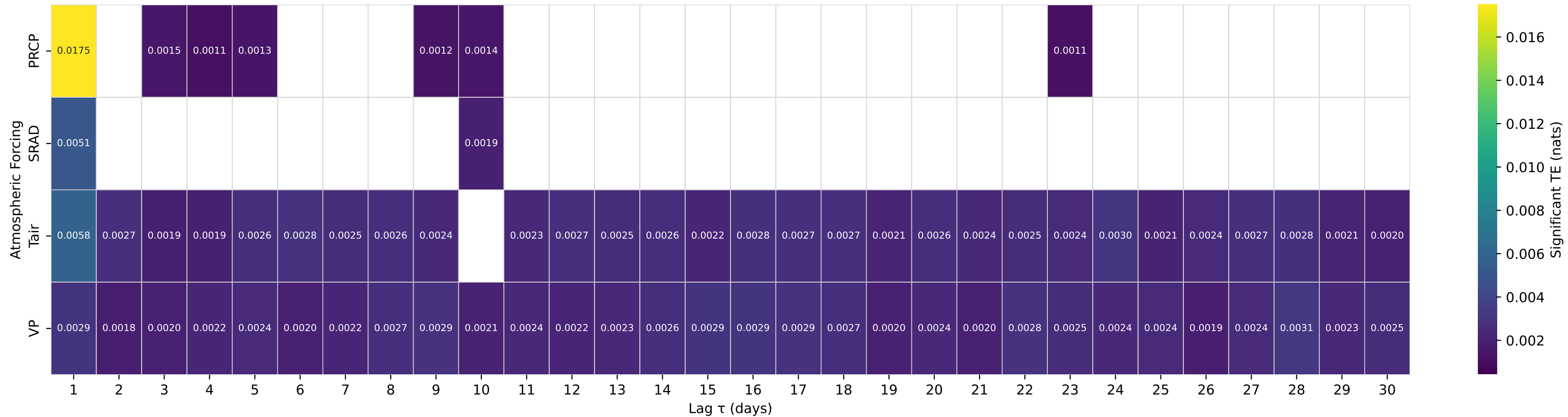
Shuffle-Test Significant TE to Streamflow — Basin 04105700 (HUC 04) — AUGUSTA CREEK NEAR AUGUSTA, MI
