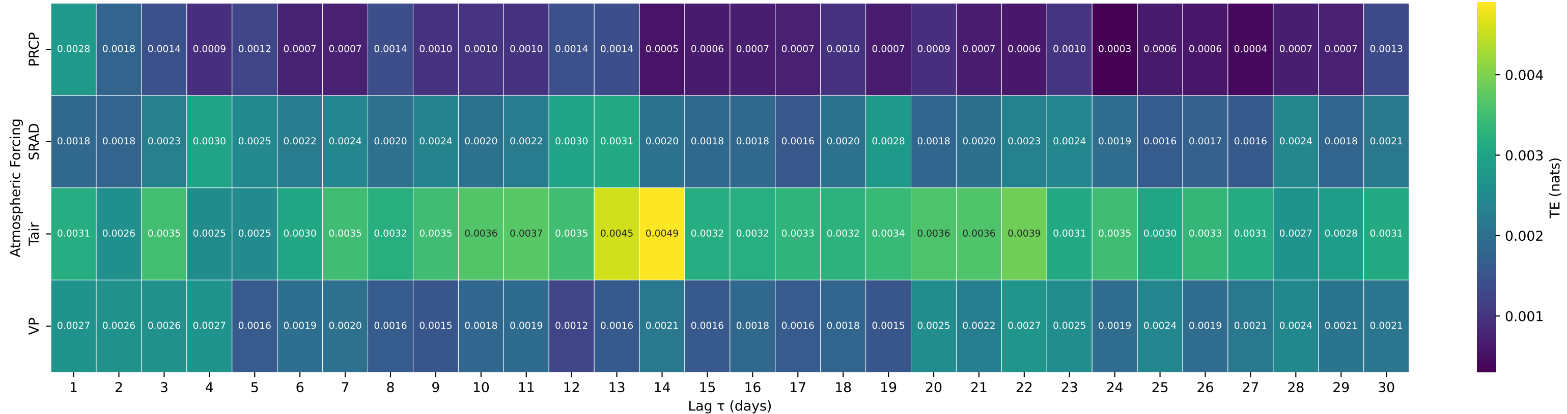
Shuffle-Test Significant TE to Streamflow — Basin 01013500 (HUC 01) — Fish River near Fort Kent, Maine
