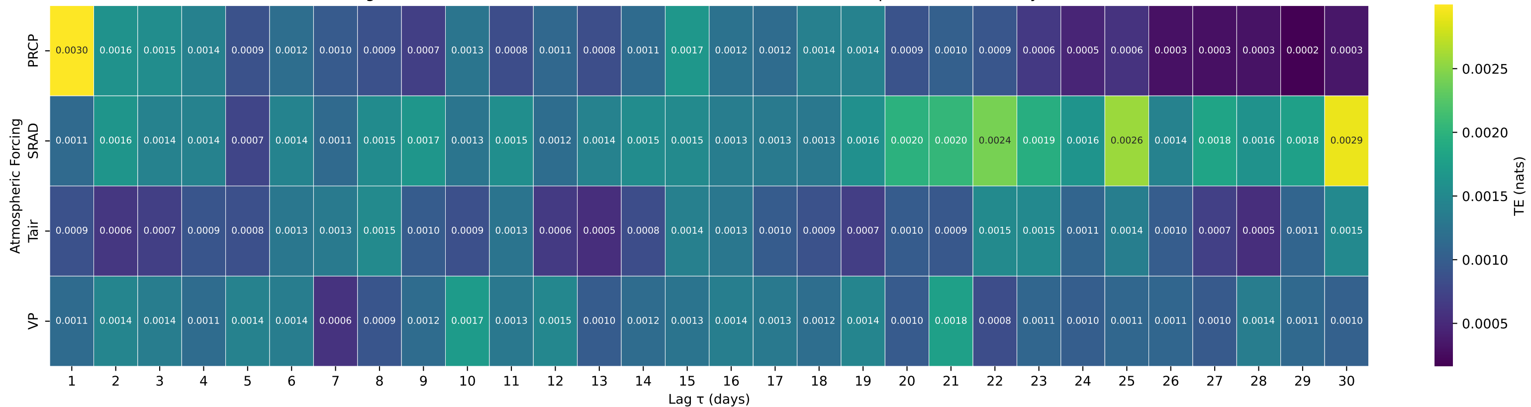
Shuffle-Test Significant TE to Streamflow — Basin 06154410 (HUC 10) — Little Peoples Creek near Hays MT
