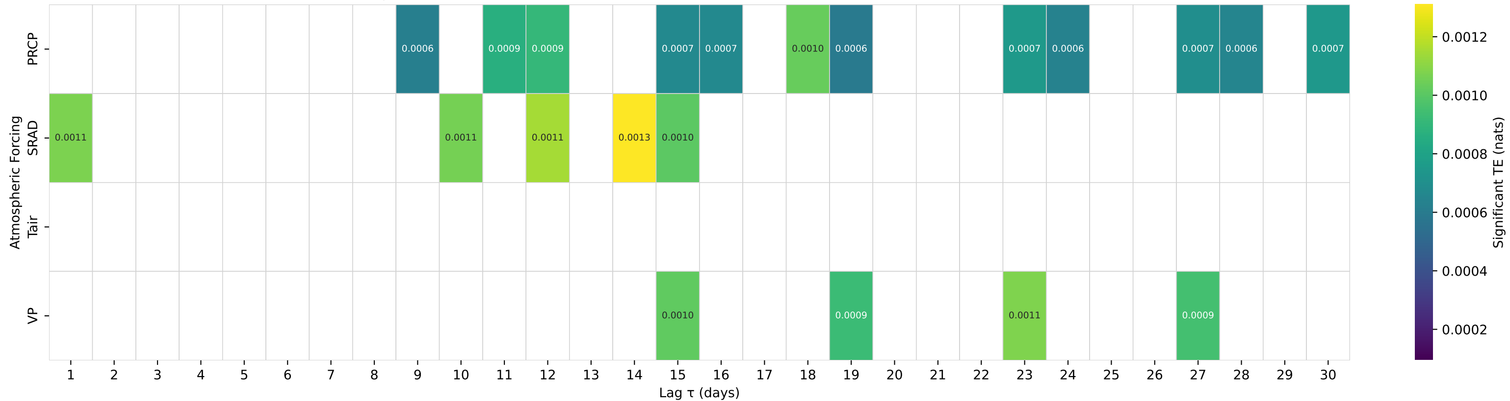
Shuffle-Test Significant TE to Streamflow — Basin 09306242 (HUC 14) — CORRAL GULCH NEAR RANGELY, CO.
