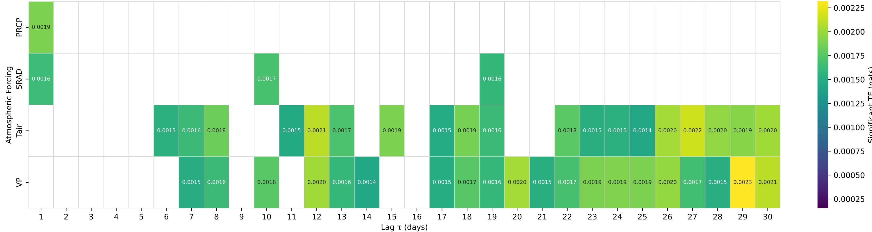
Shuffle-Test Significant TE to Streamflow — Basin 04213075 (HUC 04) — Brandy Run near Girard, PA
