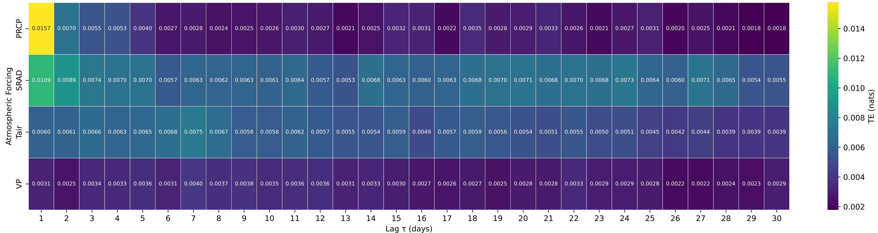
Shuffle-Test Significant TE to Streamflow — Basin 14154500 (HUC 17) — ROW RIVER ABOVE PITCHER CREEK NEAR, DORENA, OREG
