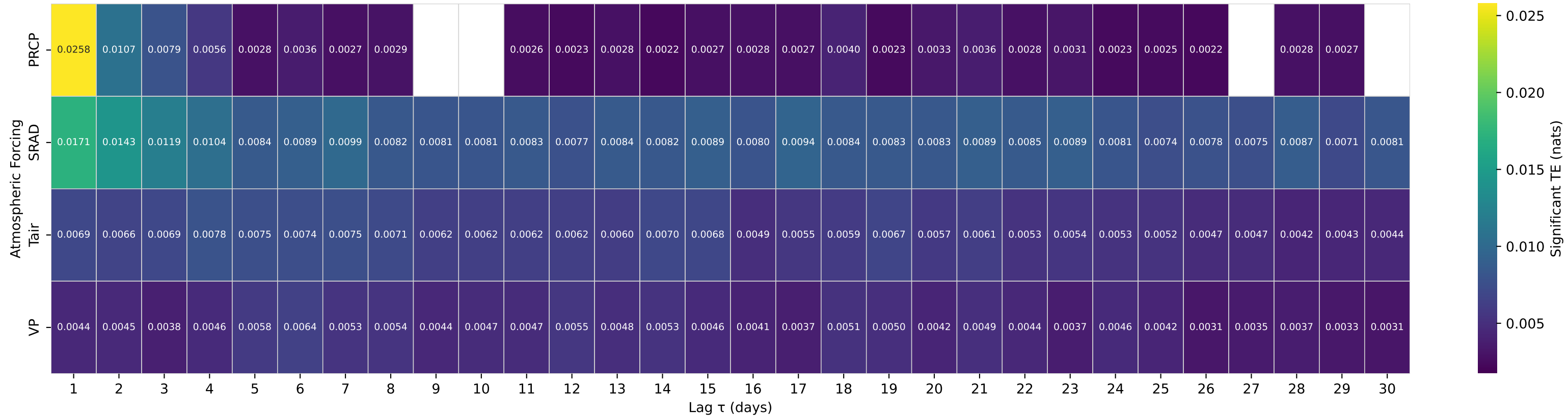
Shuffle-Test Significant TE to Streamflow — Basin 12040500 (HUC 17) — QUEETS RIVER NEAR CLEARWATER, WA
