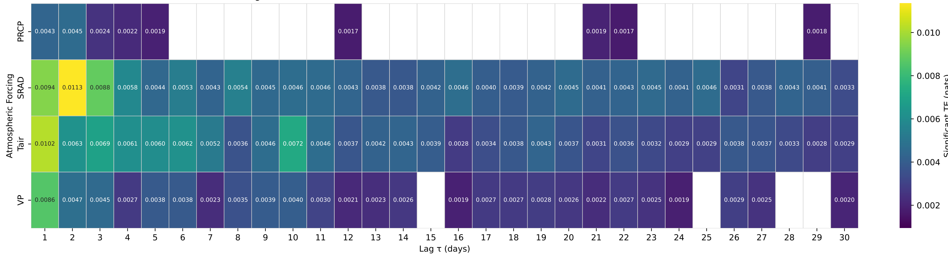
Shuffle-Test Significant TE to Streamflow — Basin 13331500 (HUC 17) — MINAM RIVER NEAR MINAM, OR
