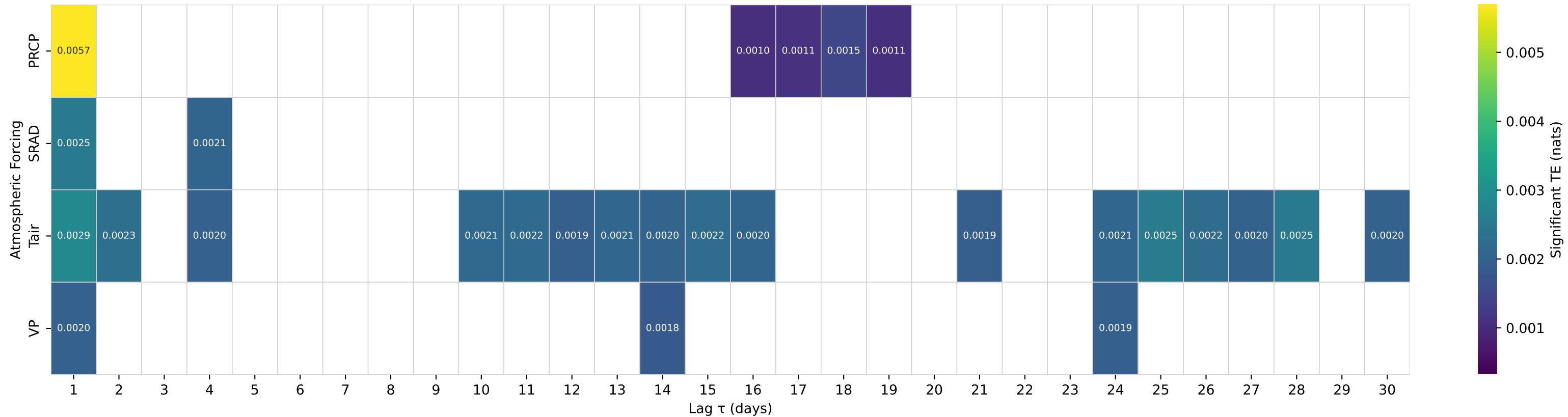
Shuffle-Test Significant TE to Streamflow — Basin 01073000 (HUC 01) — OYSTER RIVER NEAR DURHAM, NH
