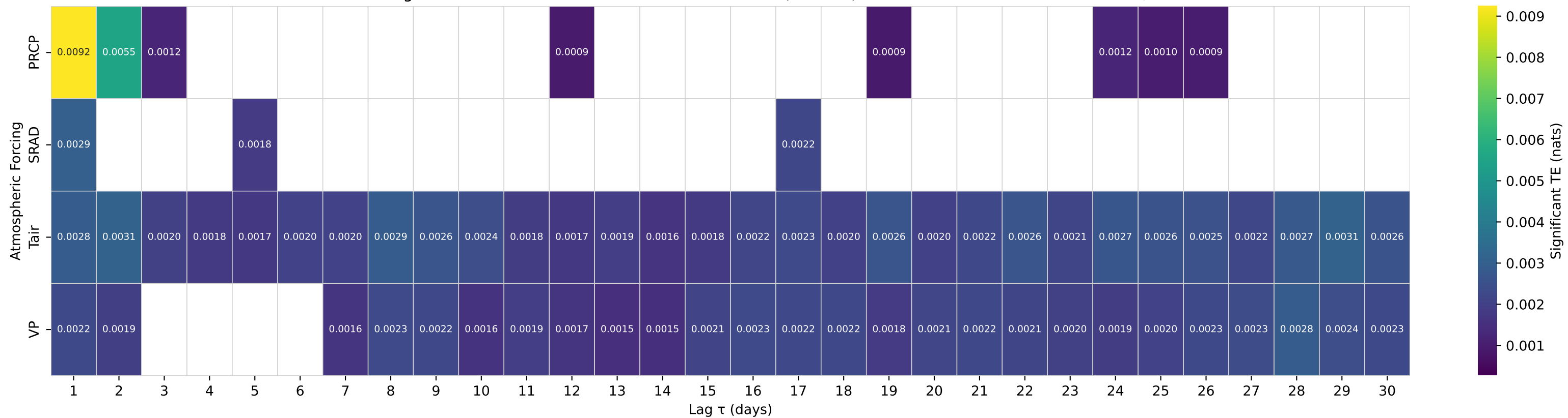
Shuffle-Test Significant TE to Streamflow — Basin 04122200 (HUC 04) — WHITE RIVER NEAR WHITEHALL, MI
