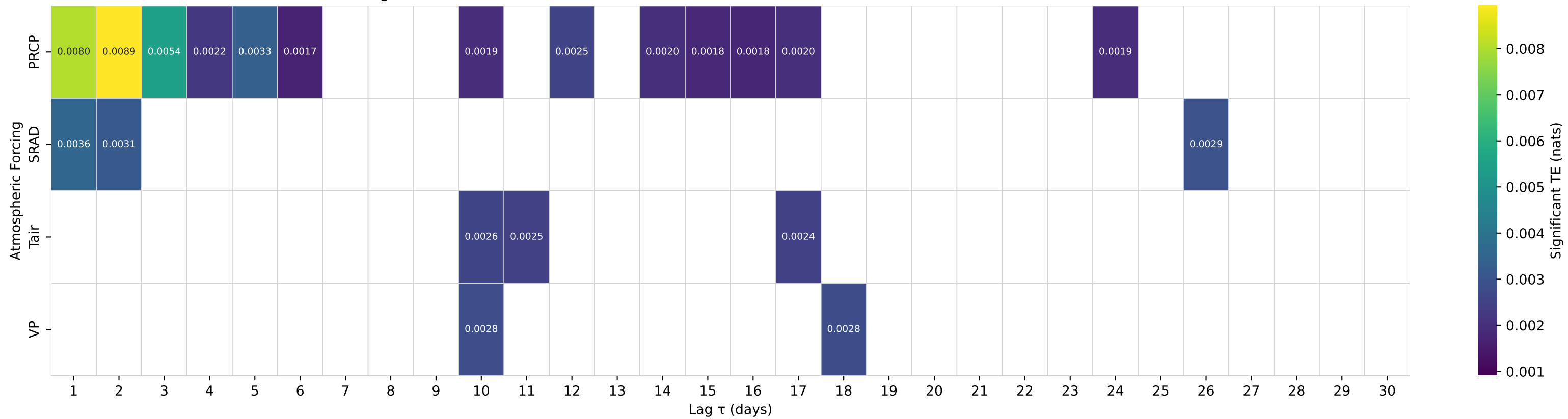
Shuffle-Test Significant TE to Streamflow — Basin 06934000 (HUC 10) — Gasconade River near Rich Fountain, MO
