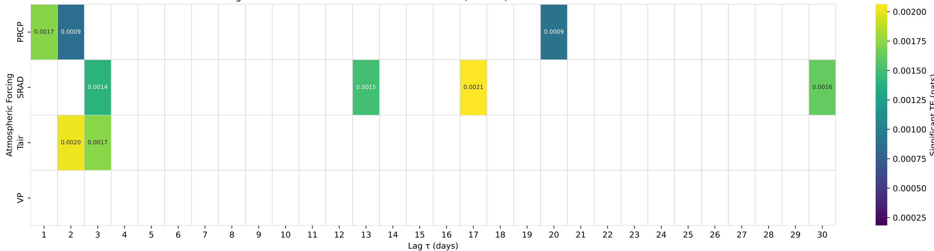
Shuffle-Test Significant TE to Streamflow — Basin 06479438 (HUC 10) — BIG SIOUX R NEAR WATERTOWN SD
