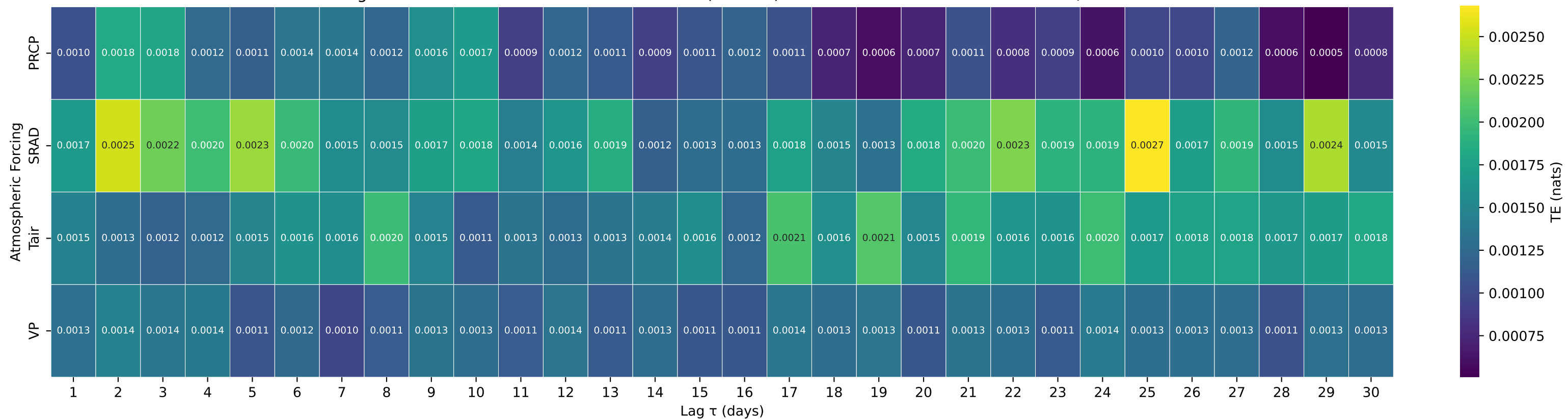
Shuffle-Test Significant TE to Streamflow — Basin 05123400 (HUC 09) — WILLOW CREEK NR WILLOW CITY, ND
