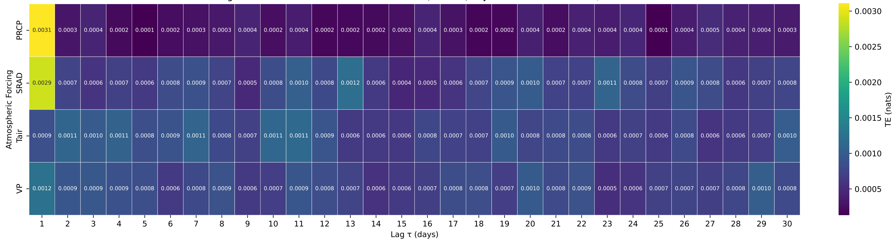
Shuffle-Test Significant TE to Streamflow — Basin 02143040 (HUC 03) — JACOB FORK AT RAMSEY, NC
