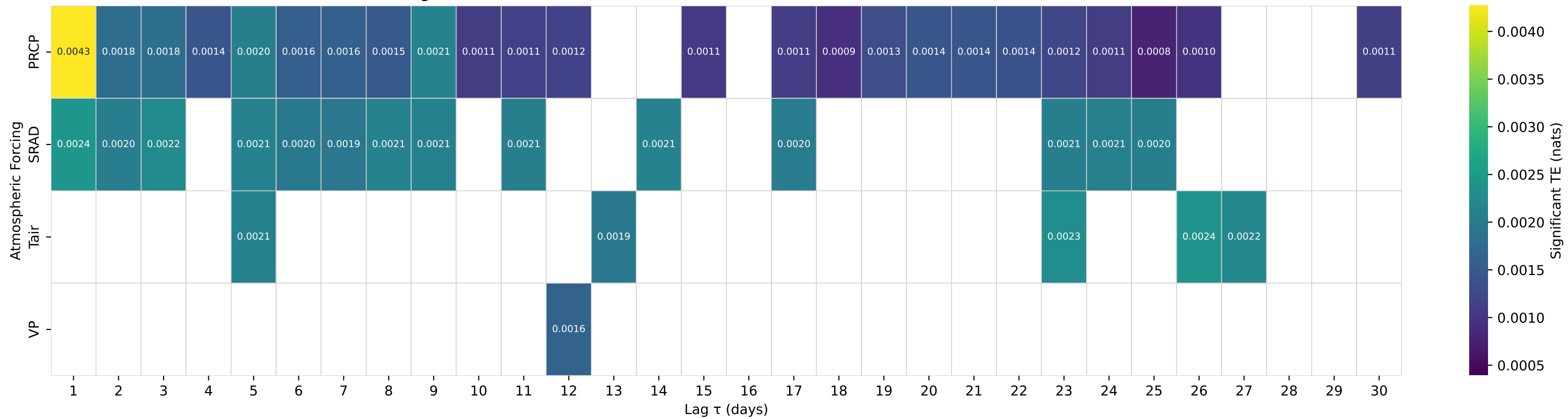
Shuffle-Test Significant TE to Streamflow — Basin 10263500 (HUC 18) — BIG ROCK C NR VALYERMO CA
