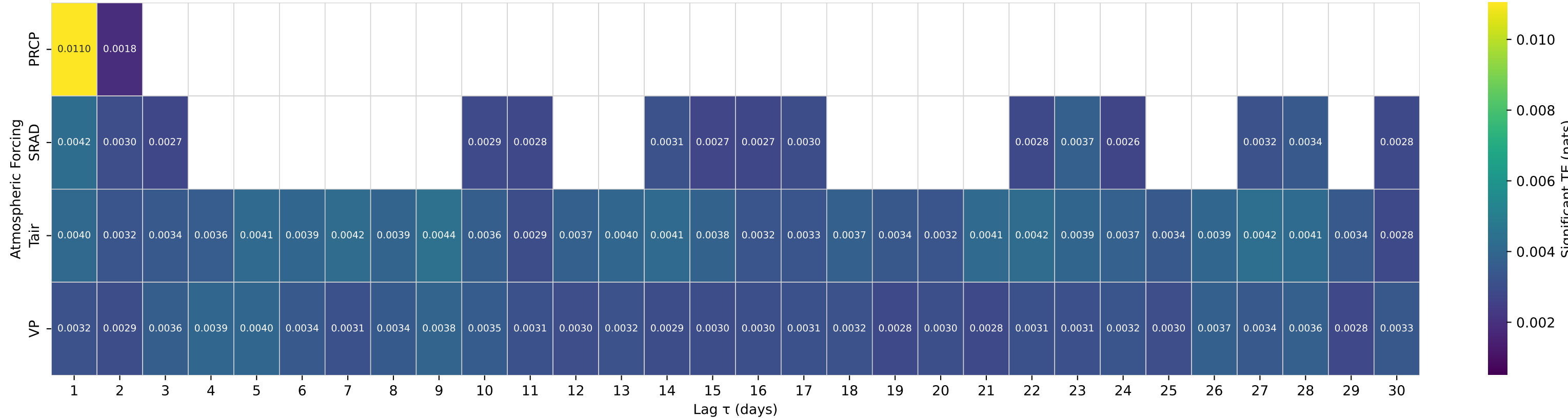
Shuffle-Test Significant TE to Streamflow — Basin 04213000 (HUC 04) — Conneaut Creek at Conneaut OH
