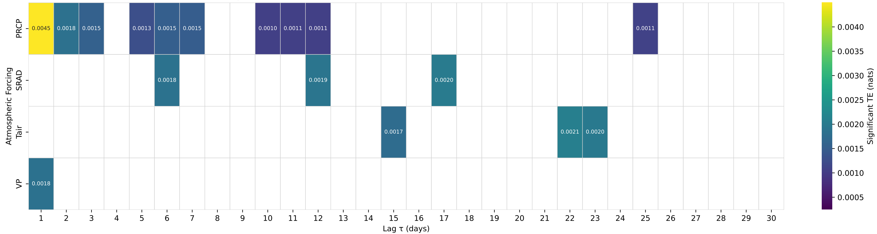
Shuffle-Test Significant TE to Streamflow — Basin 05503800 (HUC 07) — Crooked Creek near Paris, MO
