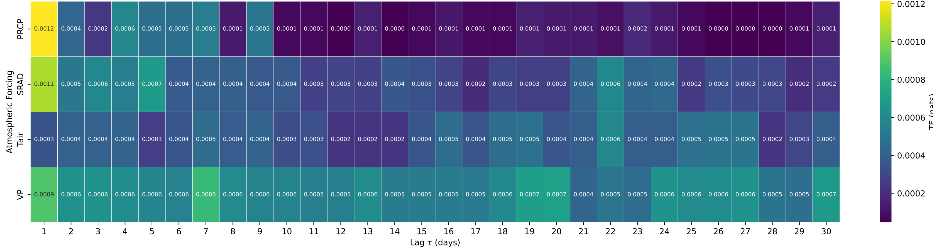
Shuffle-Test Significant TE to Streamflow — Basin 08190500 (HUC 12) — W Nueces Rv nr Brackettville, TX
