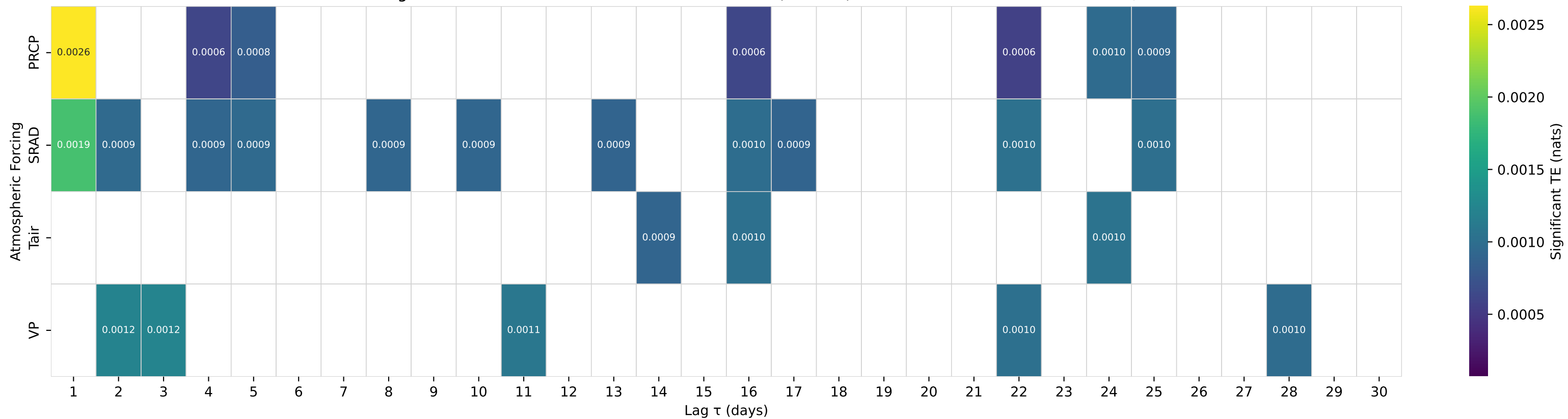
Shuffle-Test Significant TE to Streamflow — Basin 09430600 (HUC 15) — MOGOLLON CREEK NEAR CLIFF, NM
