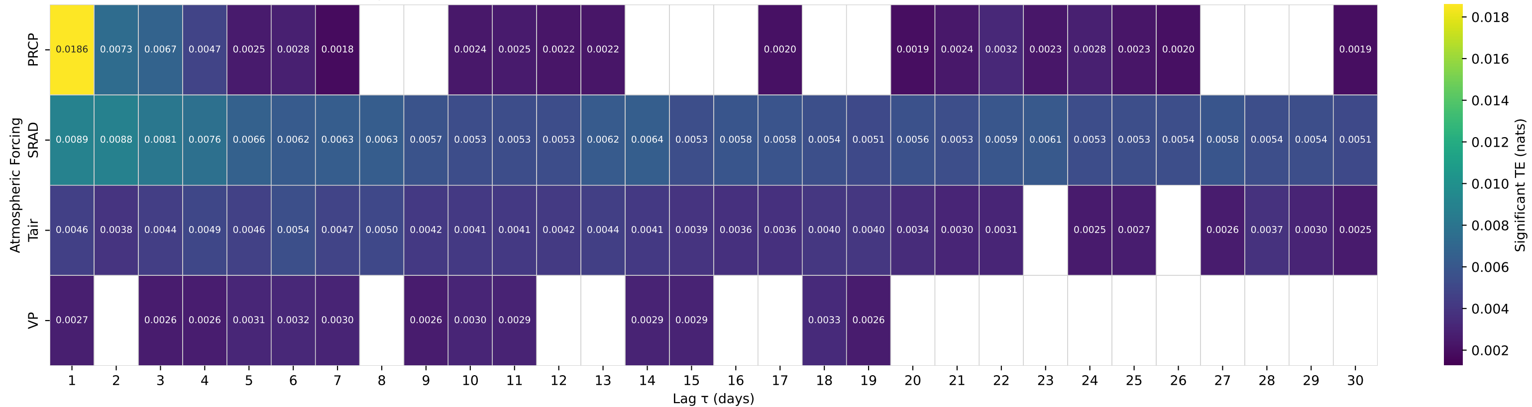
Shuffle-Test Significant TE to Streamflow — Basin 12054000 (HUC 17) — DUCKABUSH RIVER NEAR BRINNON, WA
