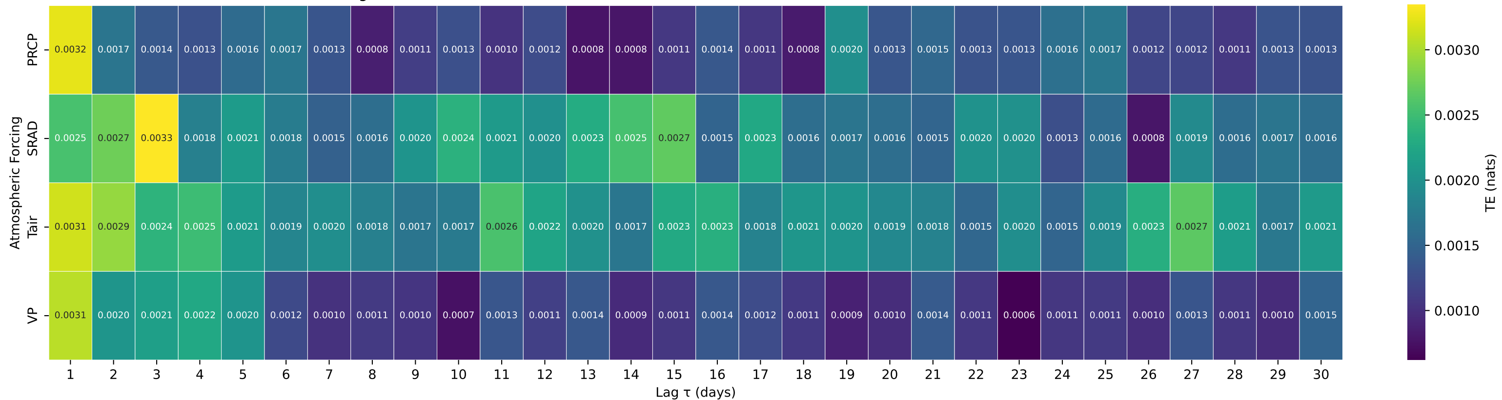
Shuffle-Test Significant TE to Streamflow — Basin 13161500 (HUC 17) — BRUNEAU RIVER AT ROWLAND NV
