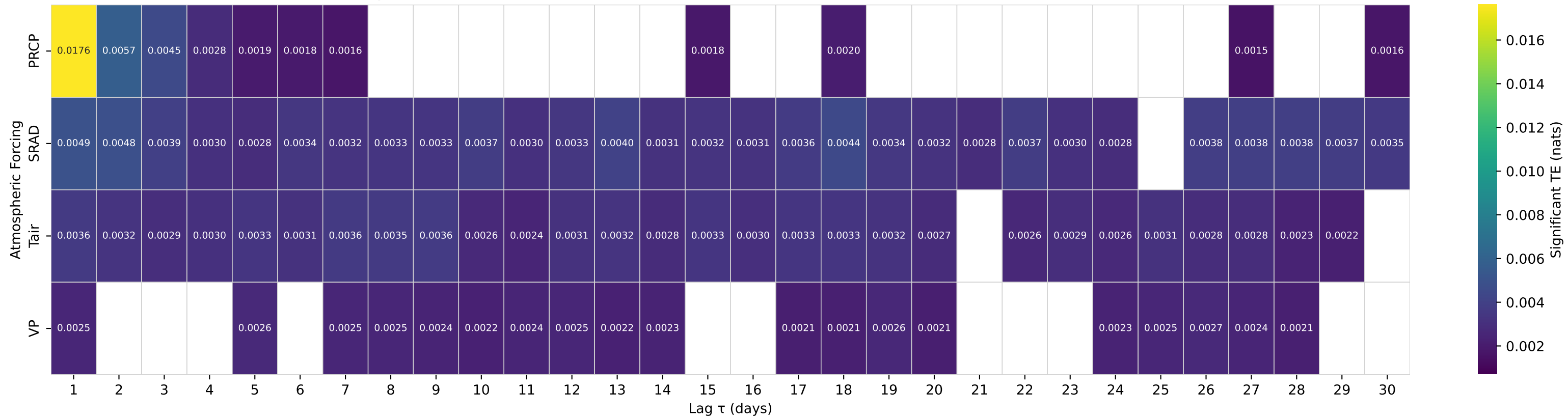
Shuffle-Test Significant TE to Streamflow — Basin 12143600 (HUC 17) — SF SNOQUALMIE RIVER AT EDGEWICK, WA
