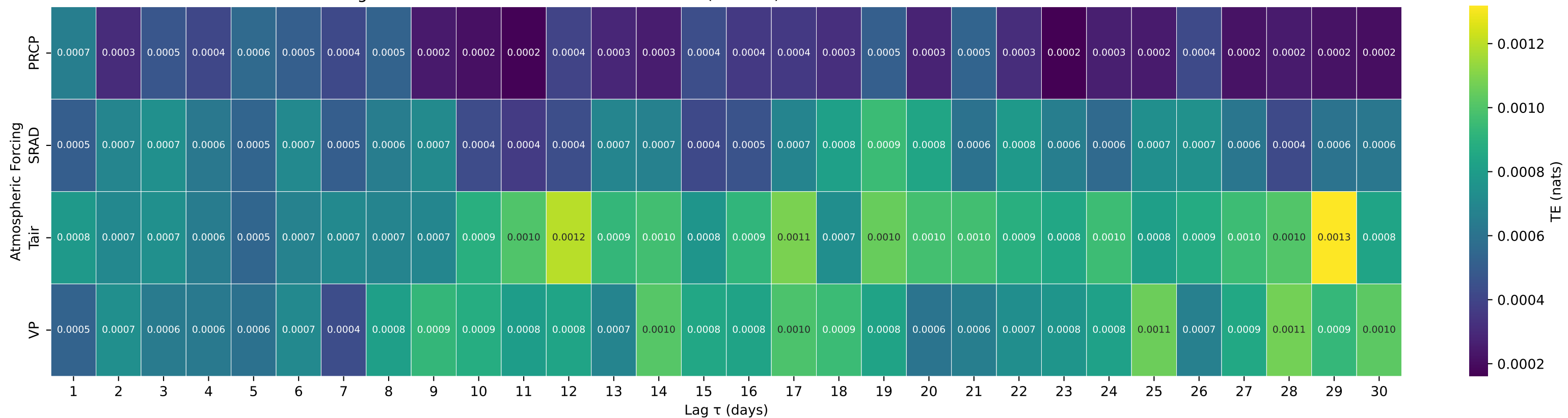
Shuffle-Test Significant TE to Streamflow — Basin 03237500 (HUC 05) — Ohio Brush Creek near West Union OH
