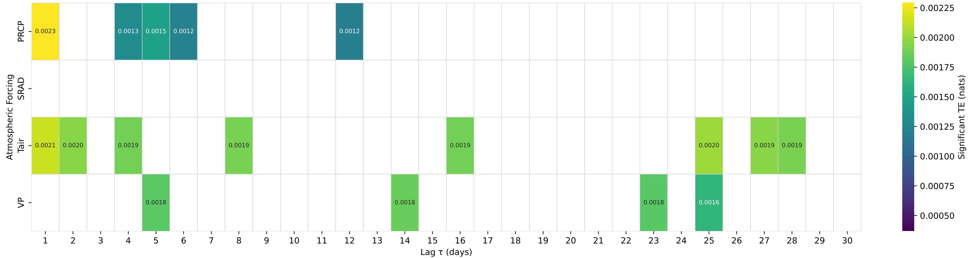
Shuffle-Test Significant TE to Streamflow — Basin 01365000 (HUC 02) — RONDOUT CREEK NEAR LOWES CORNERS NY
