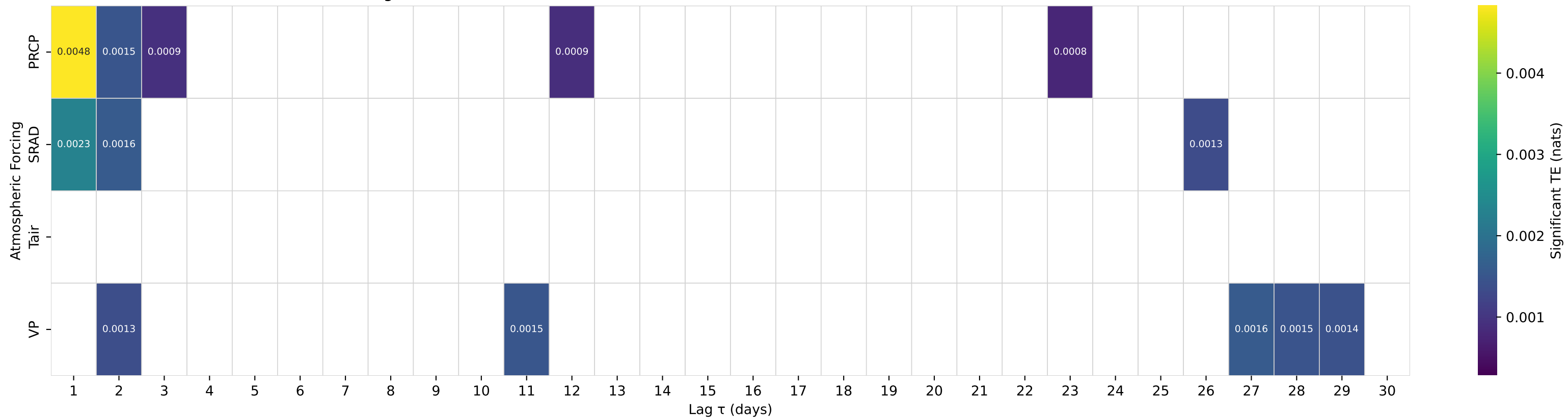
Shuffle-Test Significant TE to Streamflow — Basin 08176900 (HUC 12) — Coleta Ck at Arnold Rd nr Schroeder, TX
