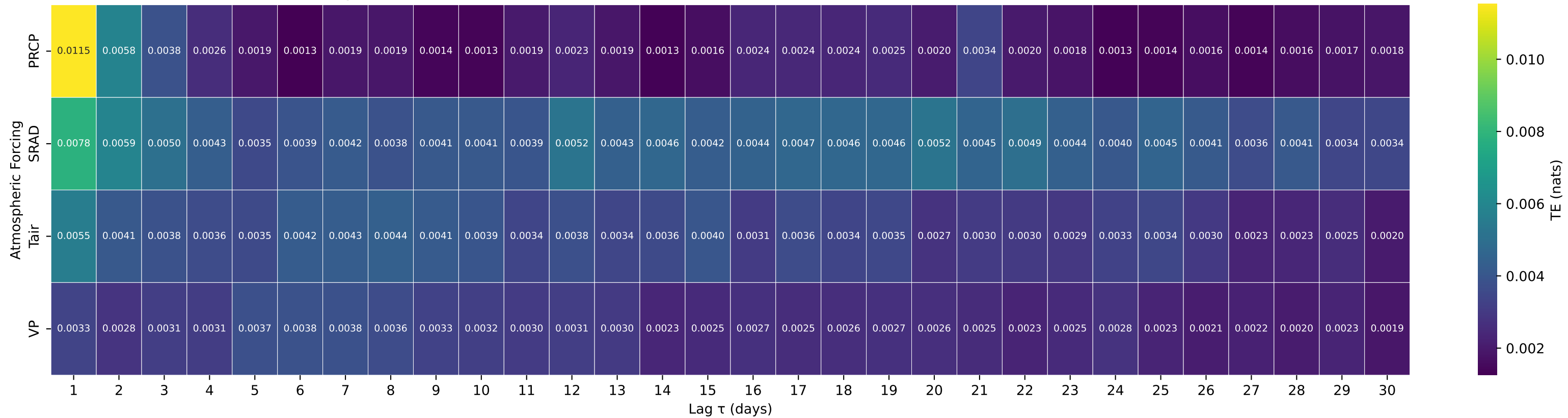
Shuffle-Test Significant TE to Streamflow — Basin 12147600 (HUC 17) — SOUTH FORK TOLT RIVER NEAR INDEX, WA
