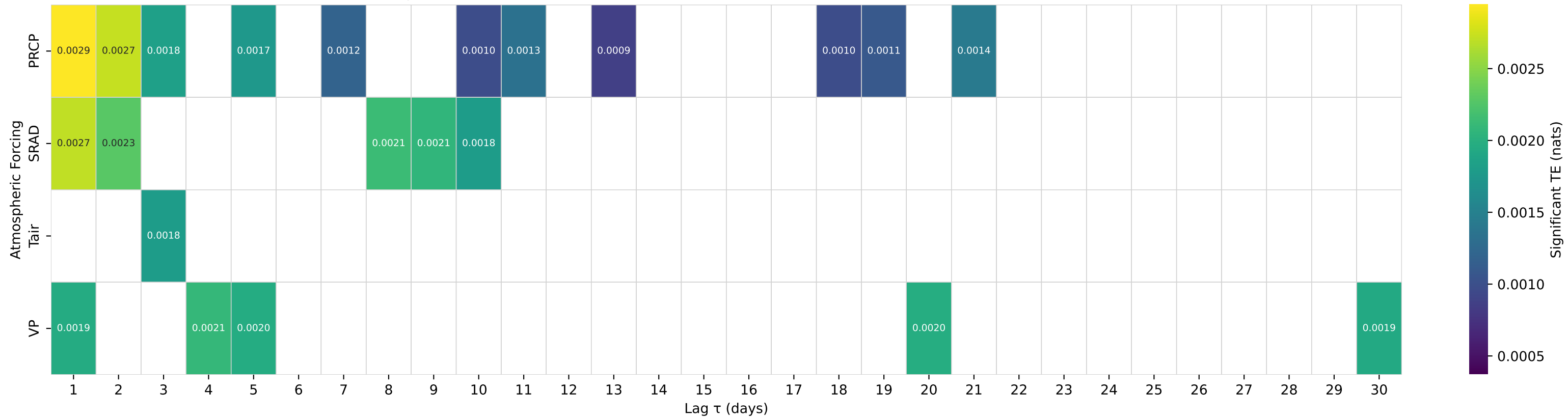
Shuffle-Test Significant TE to Streamflow — Basin 08155200 (HUC 12) — Barton Ck at SH 71 nr Oak Hill, TX
