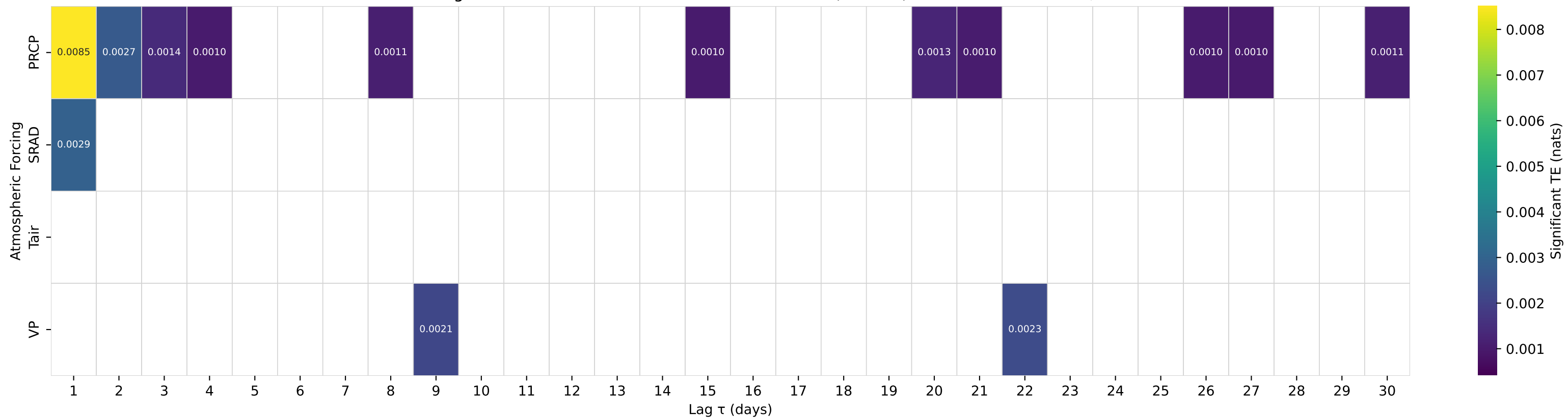
Shuffle-Test Significant TE to Streamflow — Basin 08164600 (HUC 12) — Garcitas Ck nr Inez, TX
