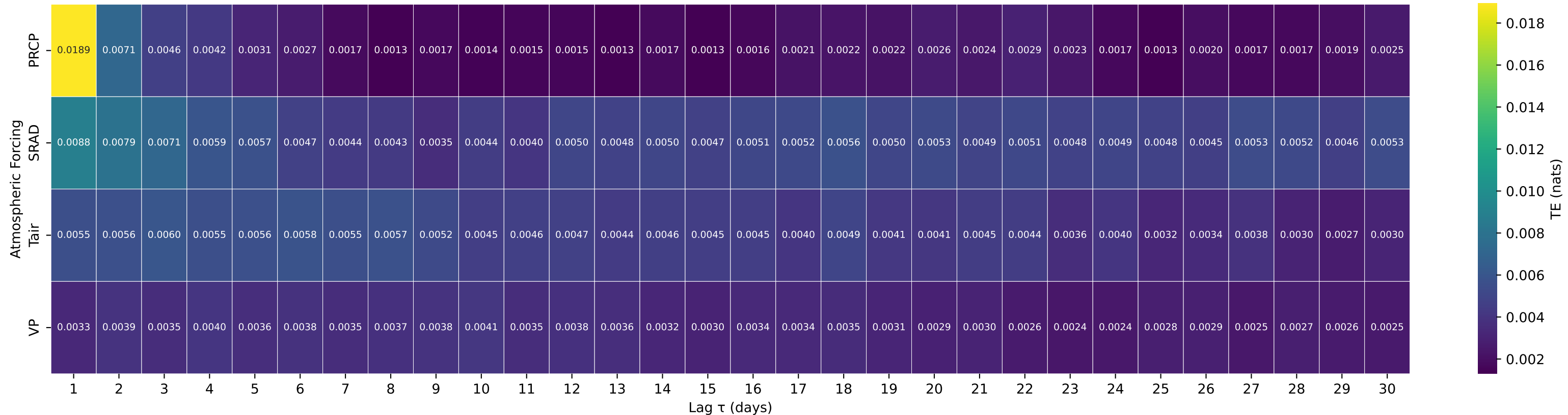
Shuffle-Test Significant TE to Streamflow — Basin 14138900 (HUC 17) — NORTH FORK BULL RUN RIVER NEAR MULTNOMAH FALLS, OR
