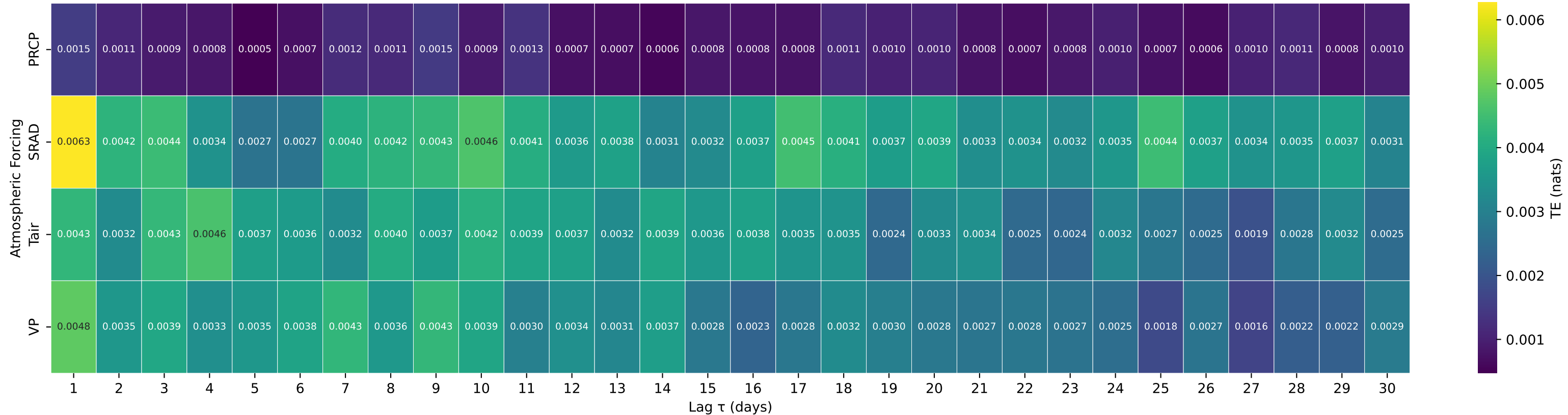
Shuffle-Test Significant TE to Streamflow — Basin 09034900 (HUC 14) — BOBTAIL CREEK NEAR JONES PASS, CO.
