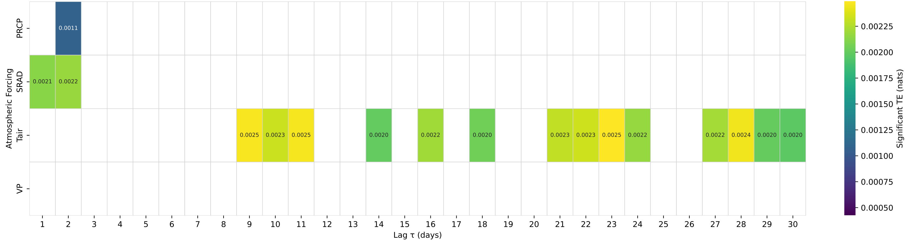
Shuffle-Test Significant TE to Streamflow — Basin 06354000 (HUC 10) — CANNONBALL RIVER AT BREIEN, ND
