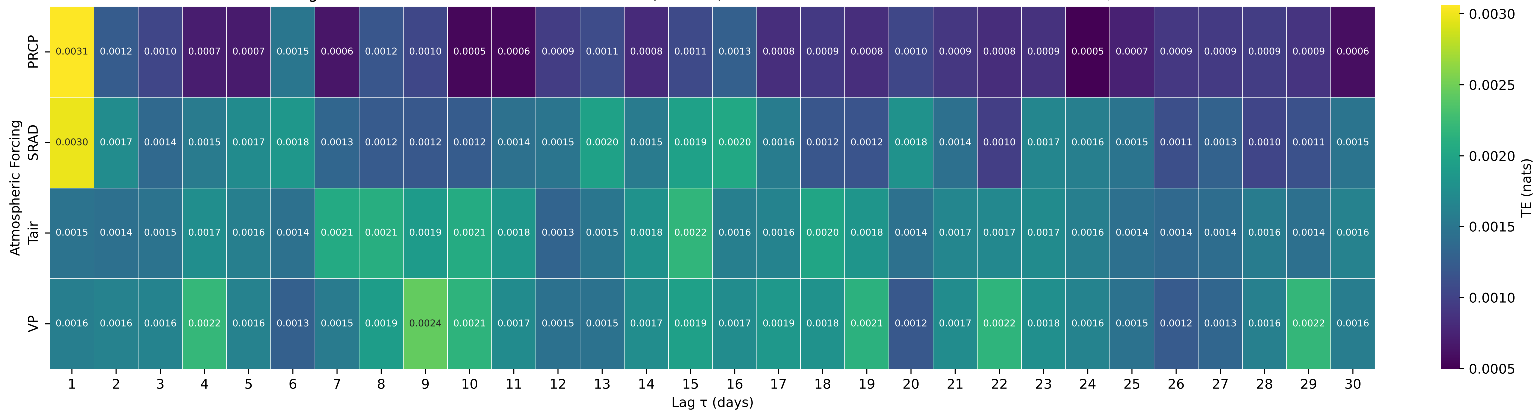
Shuffle-Test Significant TE to Streamflow — Basin 03504000 (HUC 06) — NANTAHALA RIVER NEAR RAINBOW SPRINGS, NC
