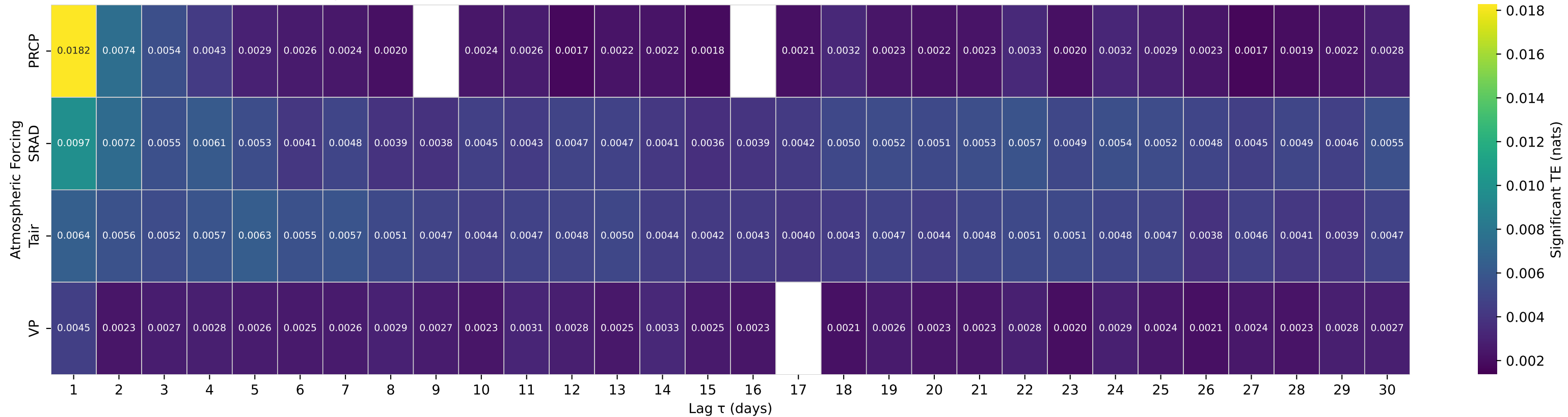
Shuffle-Test Significant TE to Streamflow — Basin 14158790 (HUC 17) — SMITH R AB SMITH R RES NR BELKNAP SPRGS,OREG.
