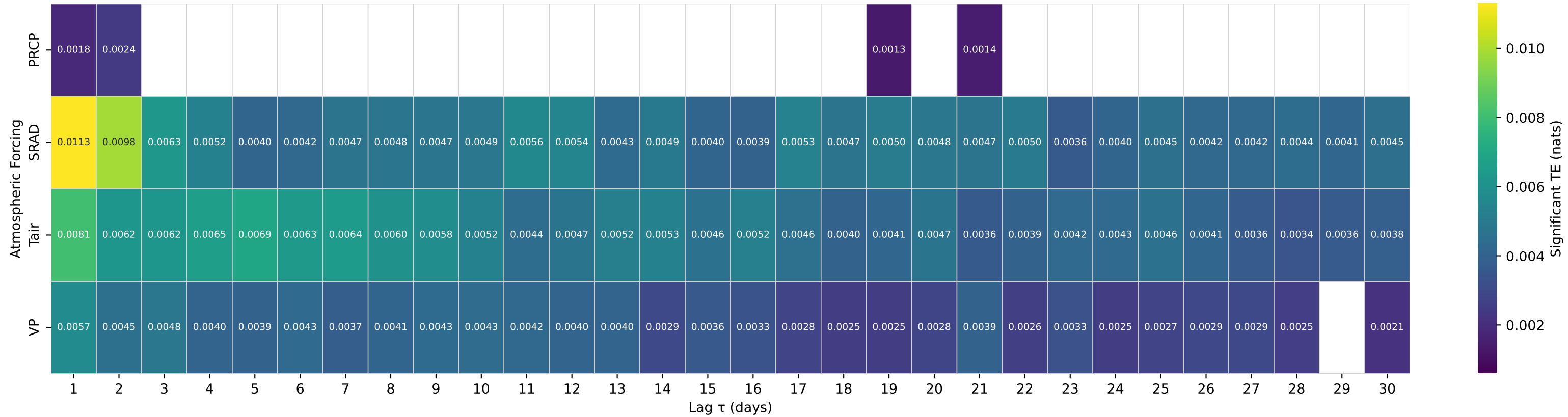
Shuffle-Test Significant TE to Streamflow — Basin 13011900 (HUC 17) — BUFFALO FORK AB LAVA CREEK NR MORAN WY
