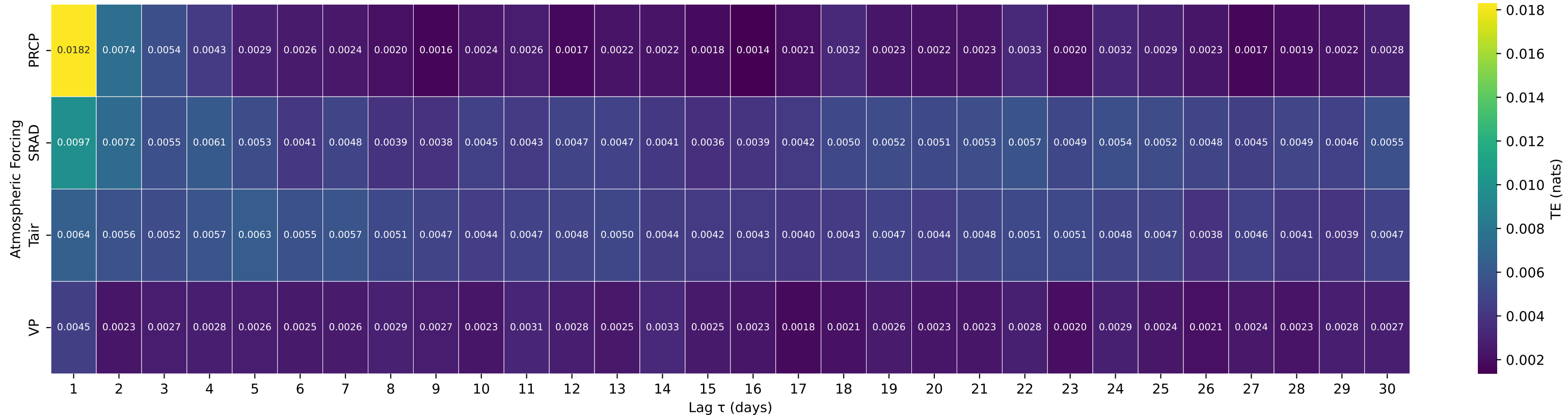
Shuffle-Test Significant TE to Streamflow — Basin 14158790 (HUC 17) — SMITH R AB SMITH R RES NR BELKNAP SPRGS,OREG.
