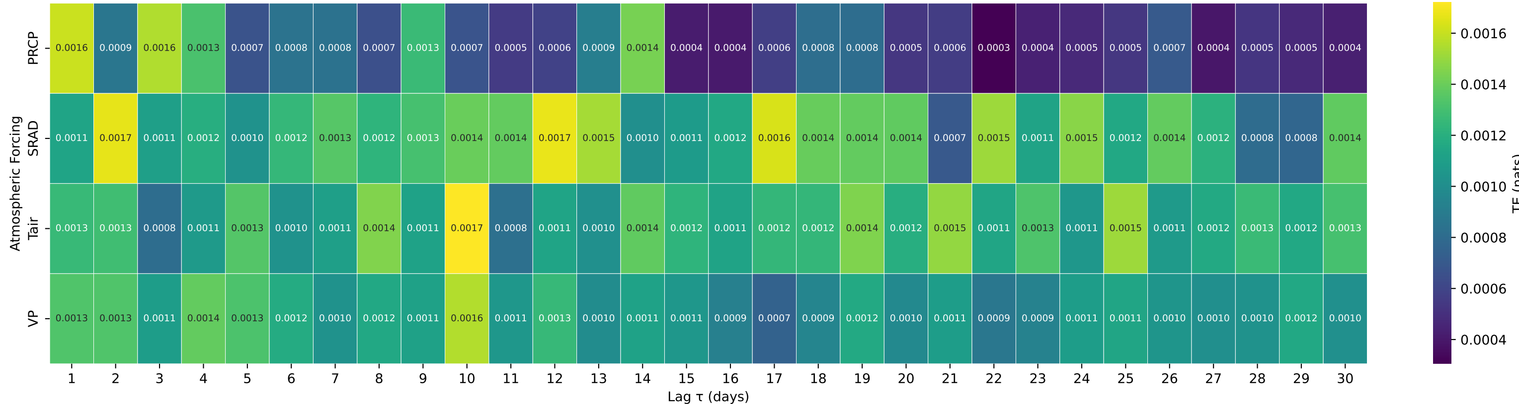
Shuffle-Test Significant TE to Streamflow — Basin 05413500 (HUC 07) — GRANT RIVER AT BURTON, WI
