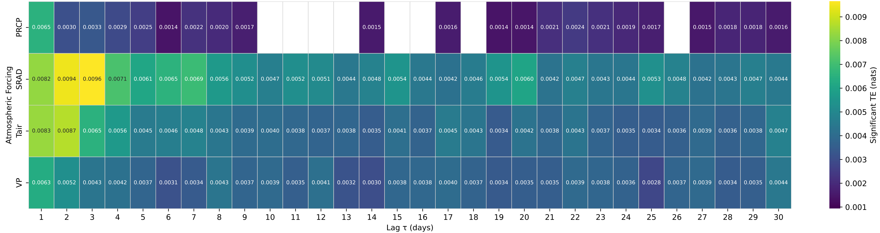
Shuffle-Test Significant TE to Streamflow — Basin 12414500 (HUC 17) — ST JOE RIVER AT CALDER ID
