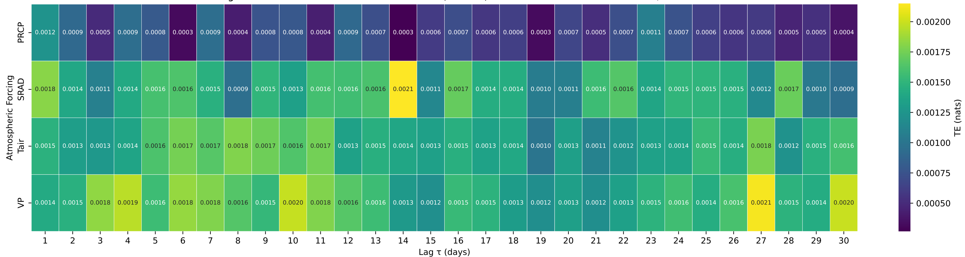
Shuffle-Test Significant TE to Streamflow — Basin 02027000 (HUC 02) — TYE RIVER NEAR LOVINGSTON, VA
