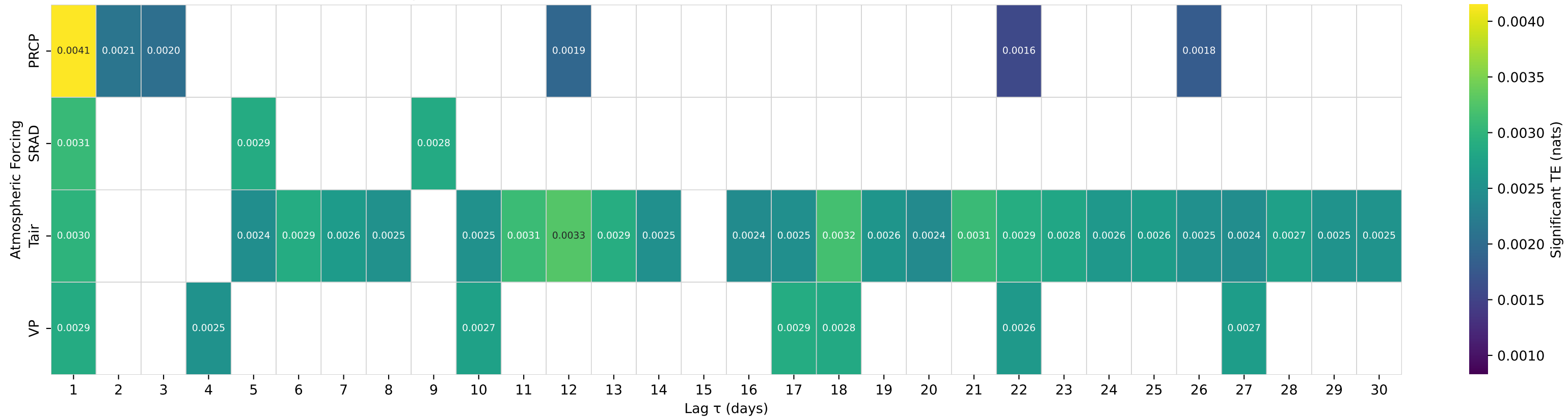
Shuffle-Test Significant TE to Streamflow — Basin 03241500 (HUC 05) — Massies Creek at Wilberforce OH
