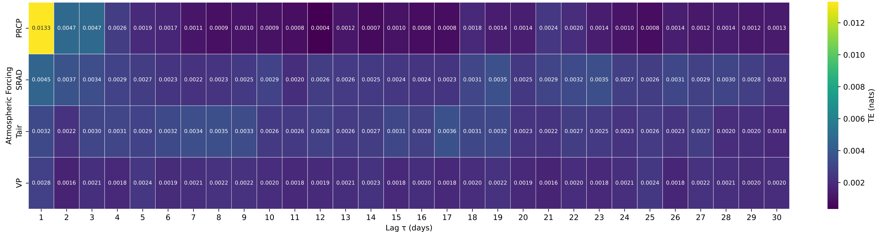
Shuffle-Test Significant TE to Streamflow — Basin 12114500 (HUC 17) — CEDAR RIVER BELOW BEAR CREEK NEAR CEDAR FALLS, WA
