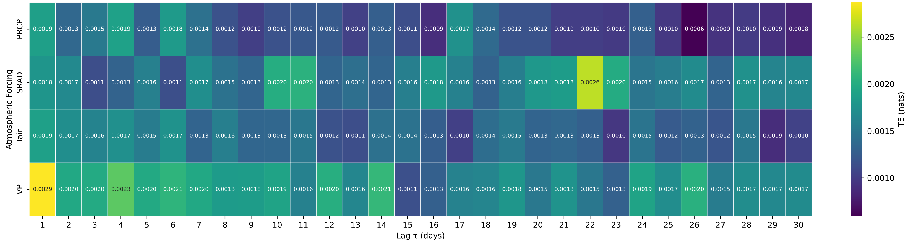
Shuffle-Test Significant TE to Streamflow — Basin 06888500 (HUC 10) — MILL C NR PAXICO, KS
