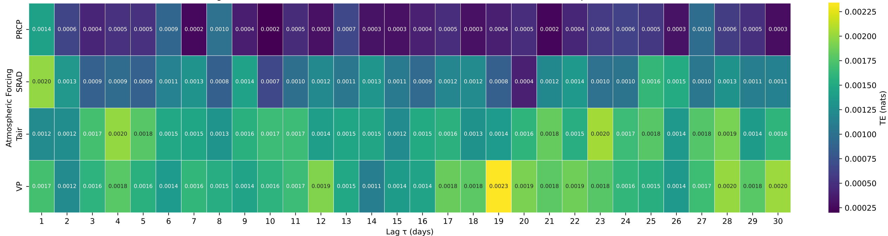
Shuffle-Test Significant TE to Streamflow — Basin 03049000 (HUC 05) — Buffalo Creek near Freeport, PA
