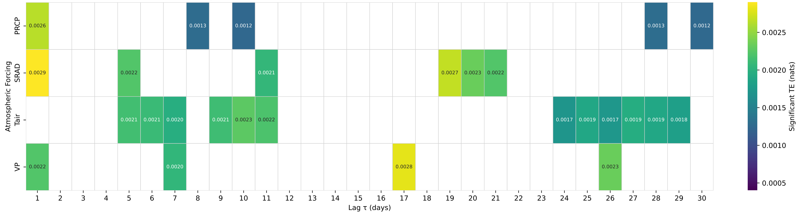
Shuffle-Test Significant TE to Streamflow — Basin 03165000 (HUC 05) — CHESTNUT CREEK AT GALAX, VA
