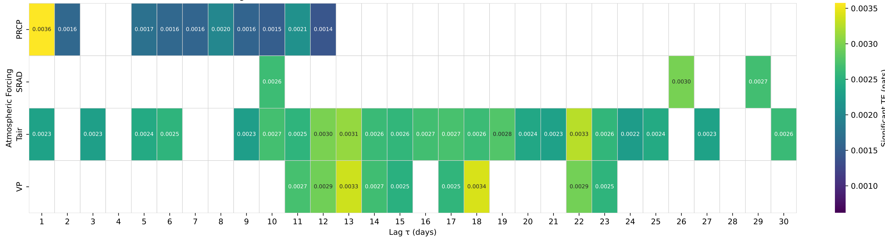
Shuffle-Test Significant TE to Streamflow — Basin 03140000 (HUC 05) — Mill Creek near Coshocton OH
