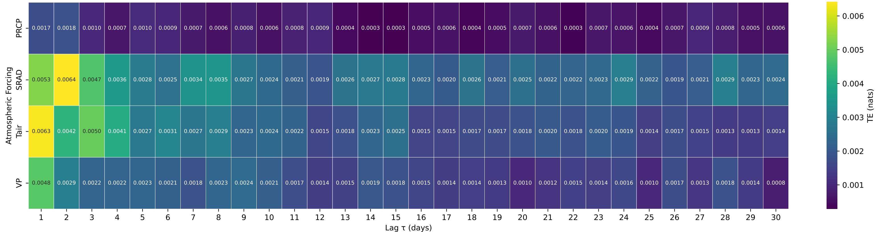
Shuffle-Test Significant TE to Streamflow — Basin 13240000 (HUC 17) — LAKE FORK PAYETTE RIVER AB JUMBO CR NR MCCALL ID
