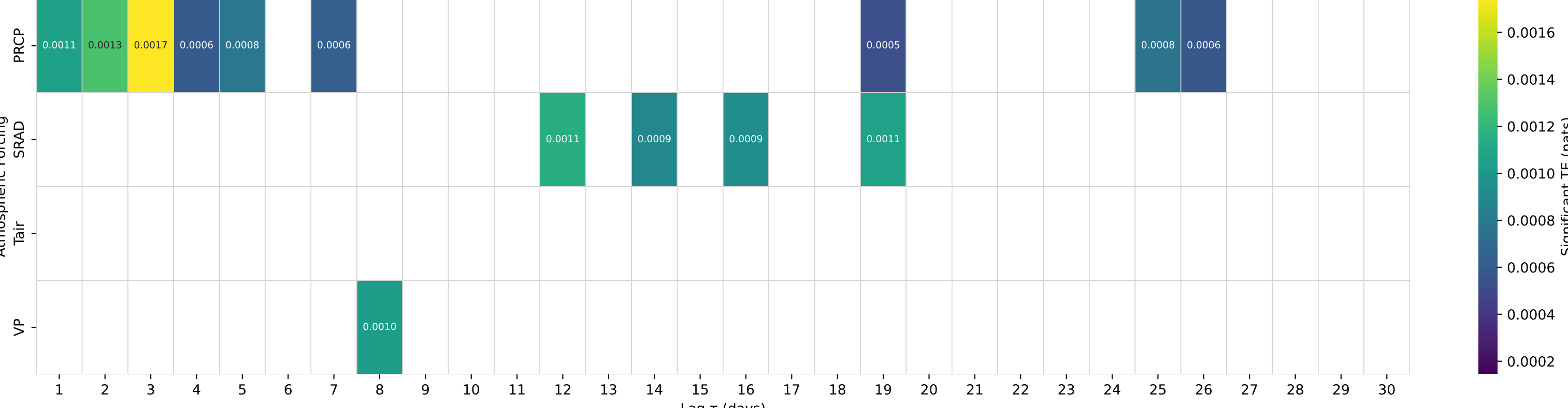
Shuffle-test Significant IE to Streamflow — Basin 07142300 (HUC 11) — RATTLESNAKE C NR MACKSVILLE, KS
