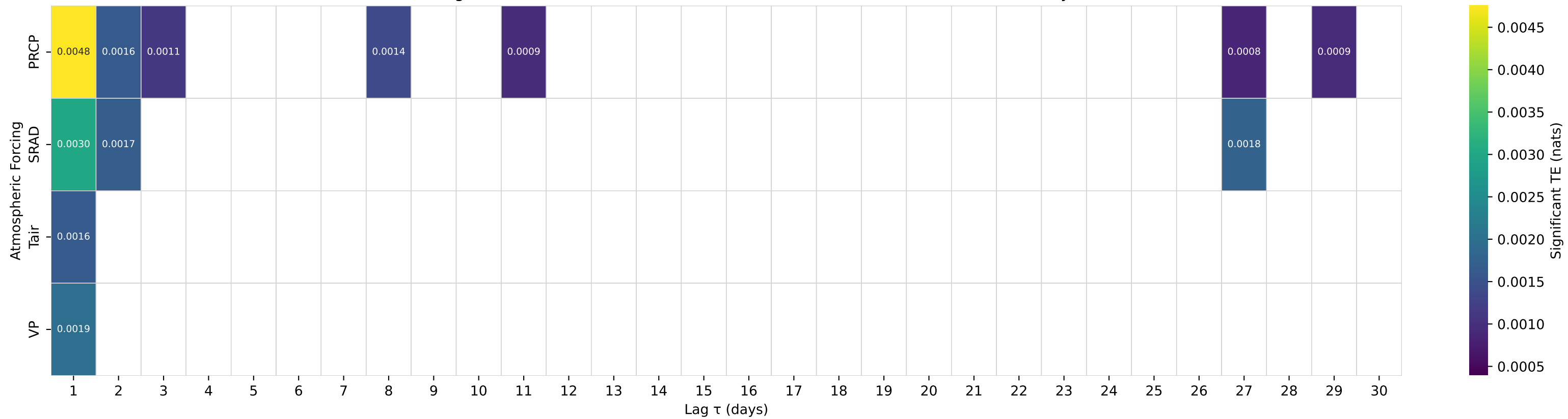
Shuffle-Test Significant TE to Streamflow — Basin 08066300 (HUC 12) — Menard Ck nr Rye, TX
