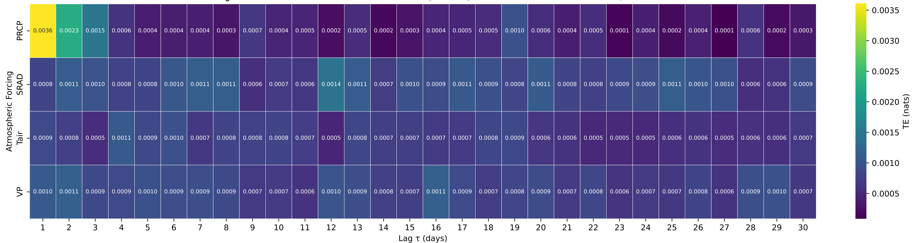
Shuffle-Test Significant TE to Streamflow — Basin 05458000 (HUC 07) — Little Cedar River near Ionia, IA
