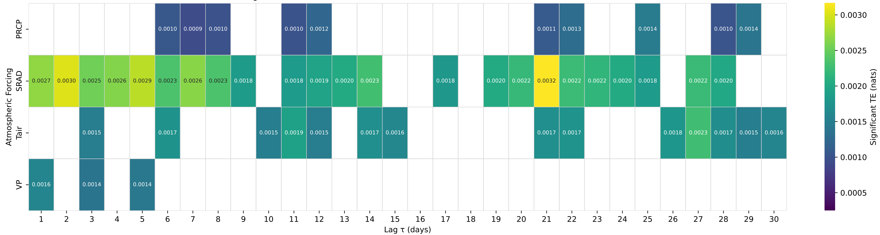
Shuffle-Test Significant TE to Streamflow — Basin 10244950 (HUC 16) — STEPTOE C NR ELY, NV
