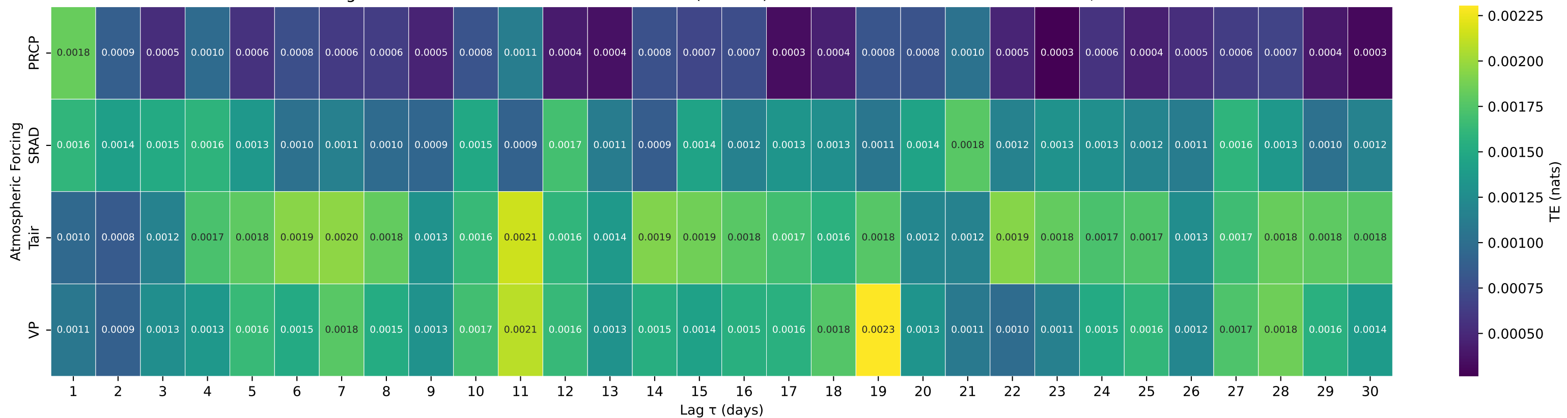
Shuffle-Test Significant TE to Streamflow — Basin 01638480 (HUC 02) — CATOCTIN CREEK AT TAYLORSTOWN, VA
