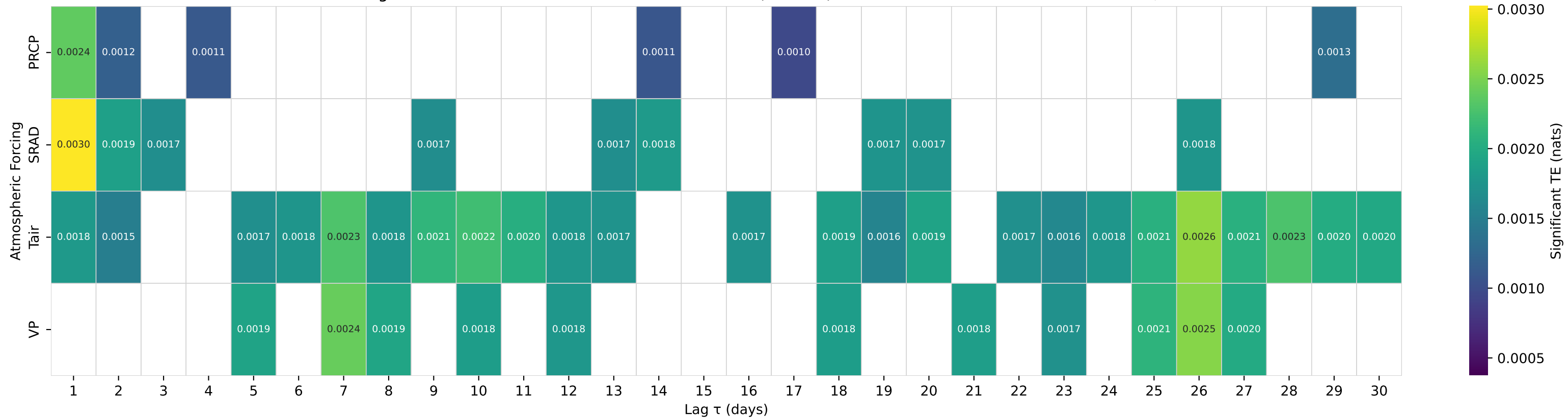
Shuffle-Test Significant TE to Streamflow — Basin 07291000 (HUC 08) — HOMOCHITTO RIVER AT EDDICETON, MS
