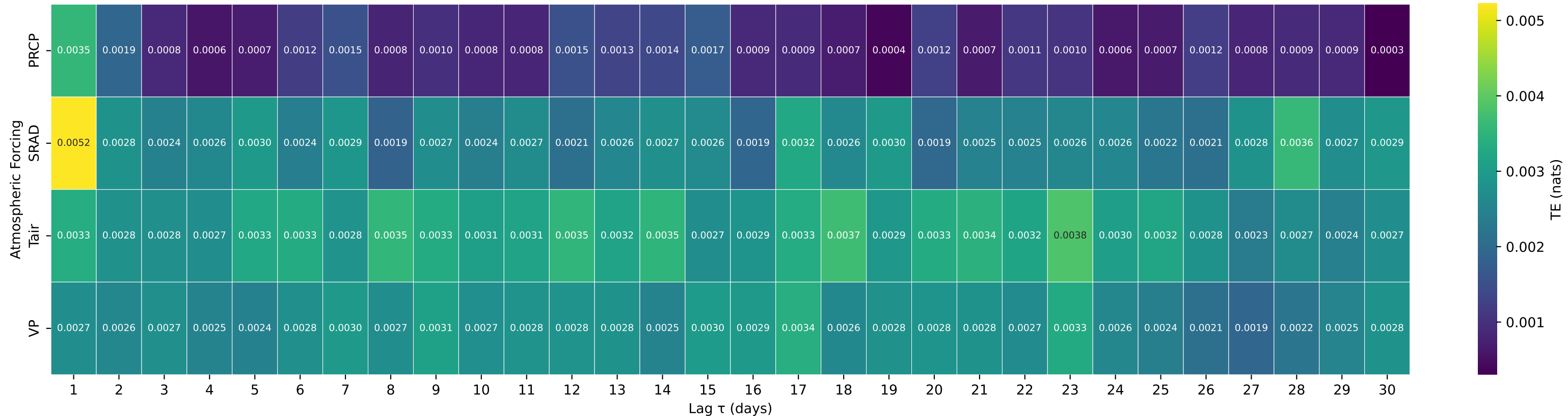
Shuffle-Test Significant TE to Streamflow — Basin 07261000 (HUC 11) — Cadron Creek near Guy, AR
