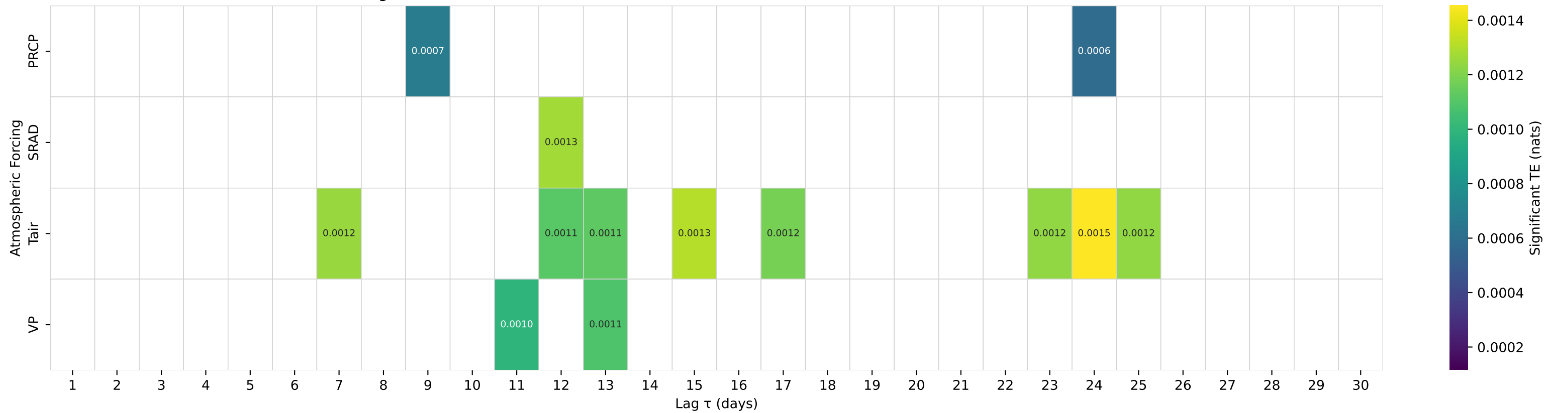
Shuffle-Test Significant TE to Streamflow — Basin 01350000 (HUC 02) — SCHOHARIE CREEK AT PRATTSVILLE NY
