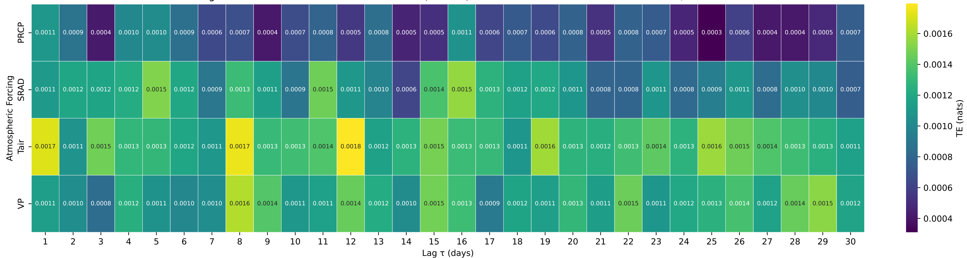
Shuffle-Test Significant TE to Streamflow — Basin 01187300 (HUC 01) — HUBBARD RIVER NR. WEST HARTLAND, CT.
