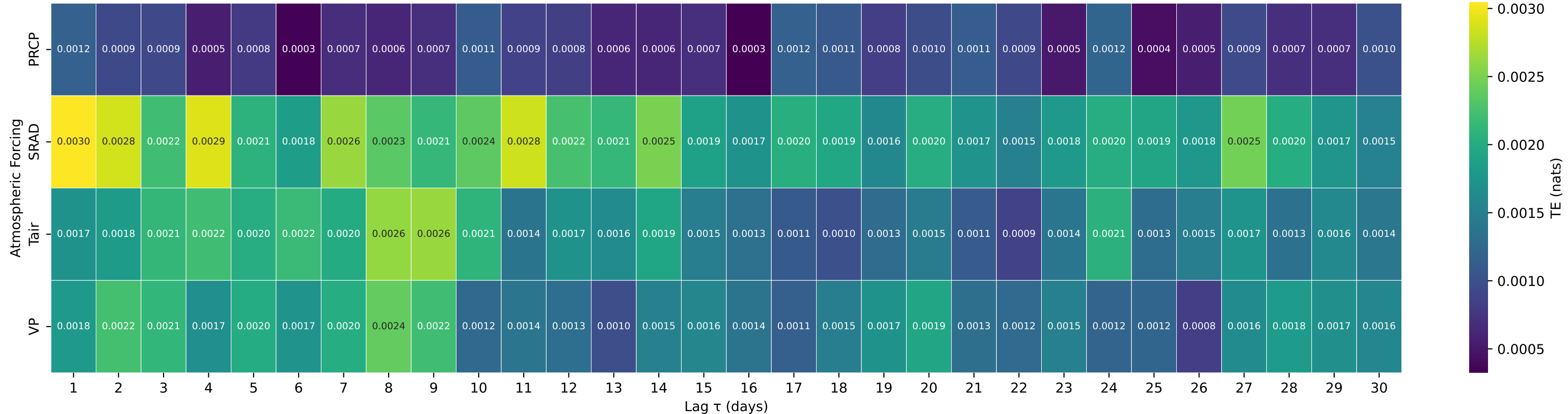
Shuffle-Test Significant TE to Streamflow — Basin 09047700 (HUC 14) — KEYSTONE GULCH NEAR DILLON, CO.
