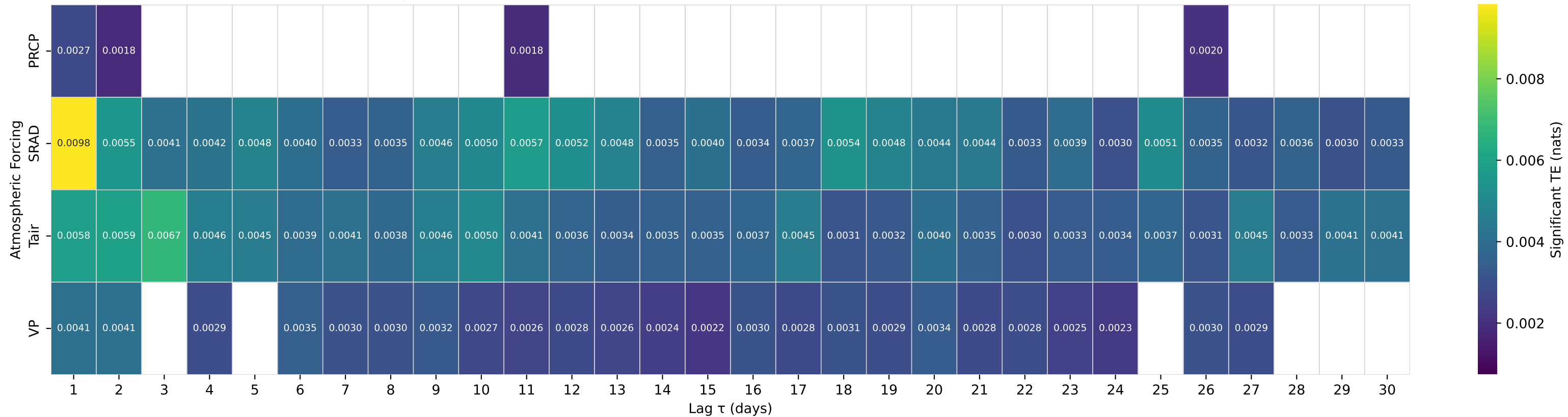
Shuffle-Test Significant TE to Streamflow — Basin 09107000 (HUC 14) — TAYLOR RIVER AT TAYLOR PARK, CO.
