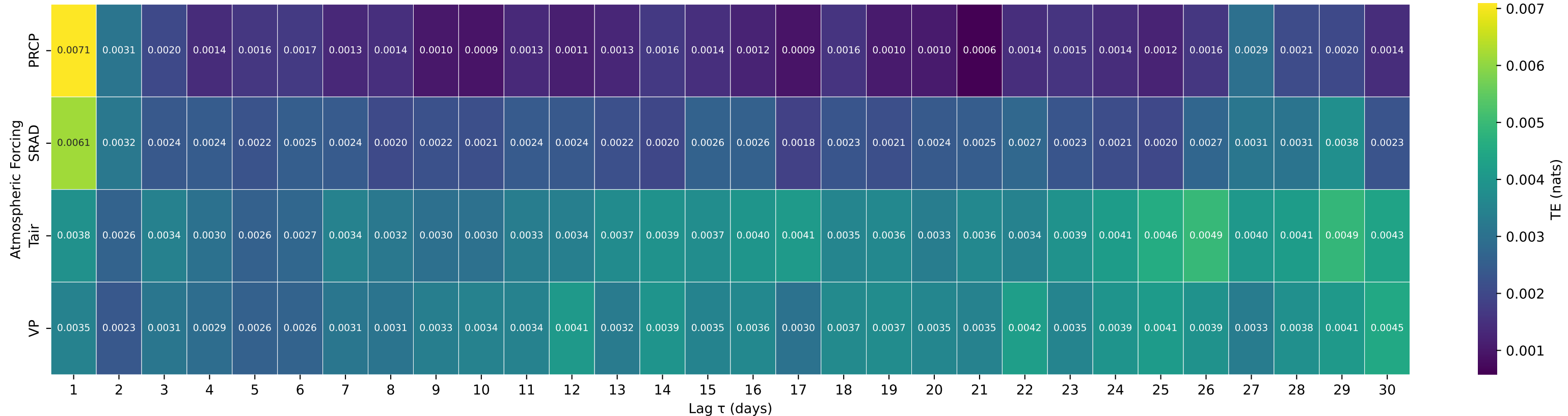
Shuffle-Test Significant TE to Streamflow — Basin 02464000 (HUC 03) — NORTH RIVER NEAR SAMANTHA AL
