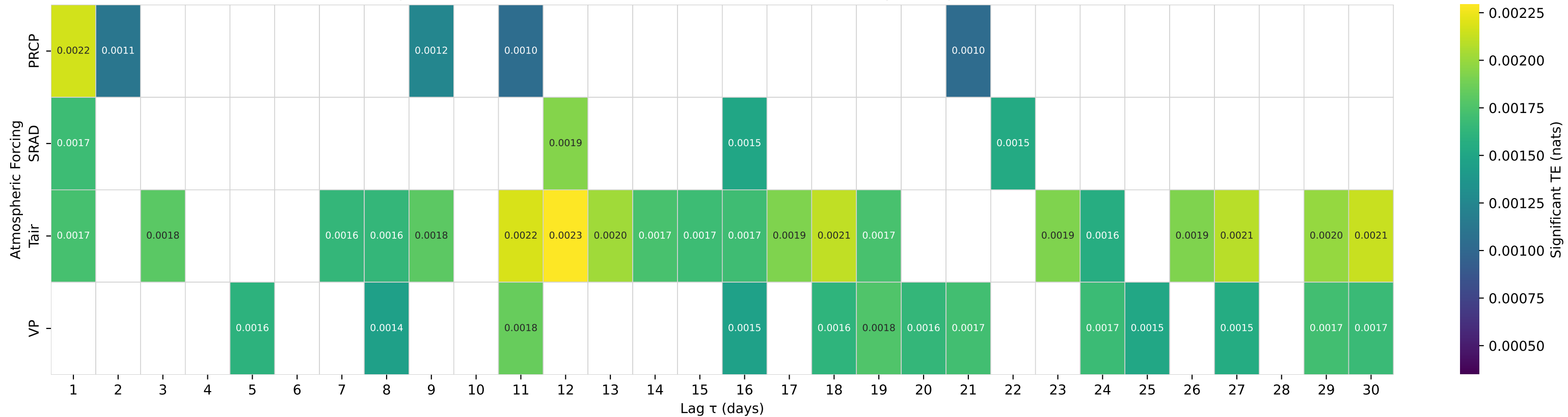
Shuffle-Test Significant TE to Streamflow — Basin 01550000 (HUC 02) — Lycoming Creek near Trout Run, PA
