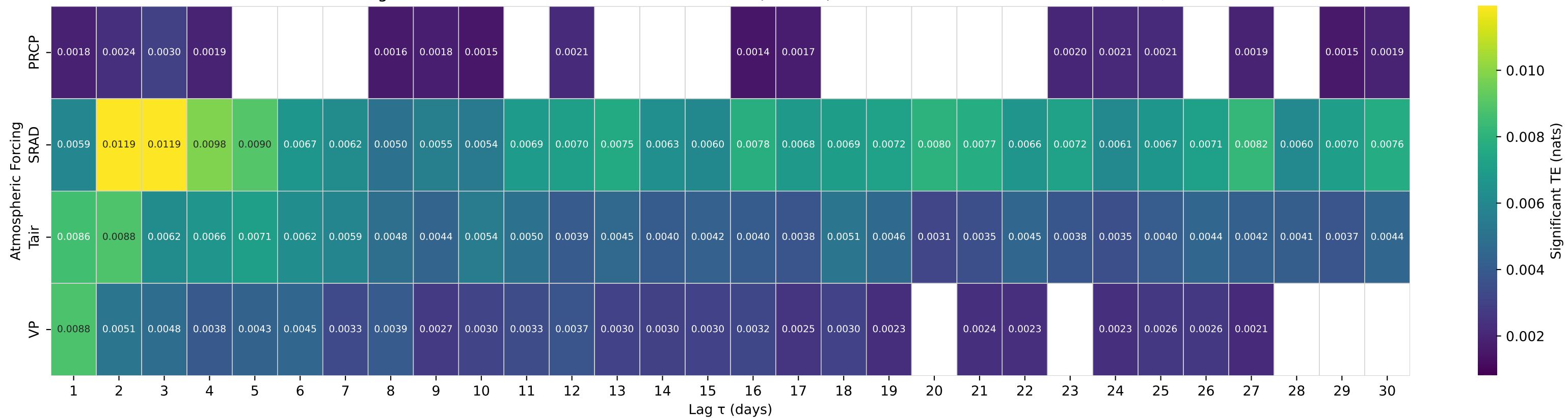
Shuffle-Test Significant TE to Streamflow — Basin 06224000 (HUC 10) — BULL LAKE CREEK ABOVE BULL LAKE, WY
