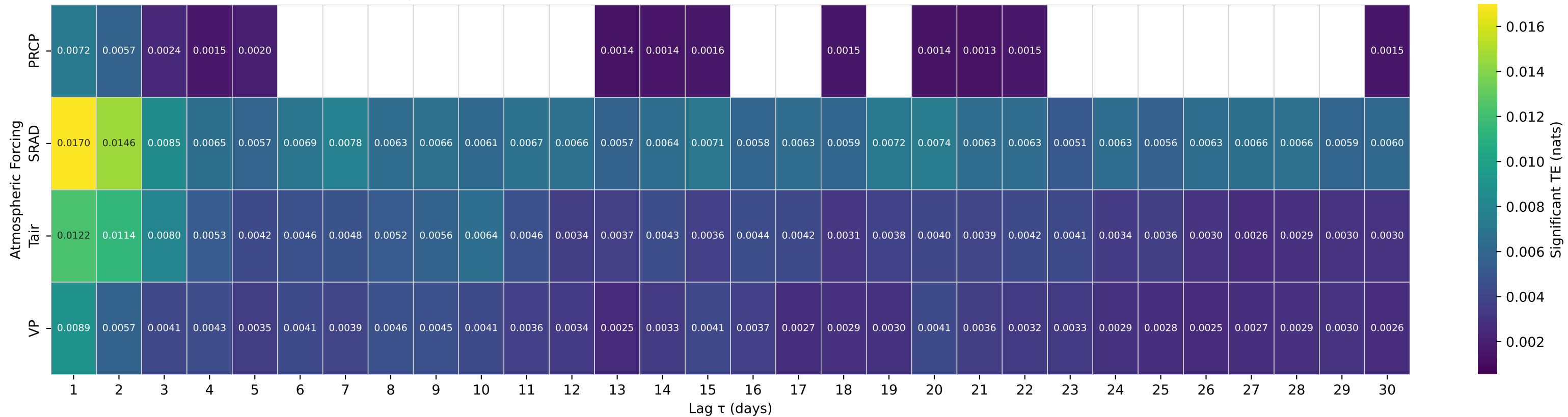
Shuffle-Test Significant TE to Streamflow — Basin 12451000 (HUC 17) — STEHEKIN RIVER AT STEHEKIN, WA
