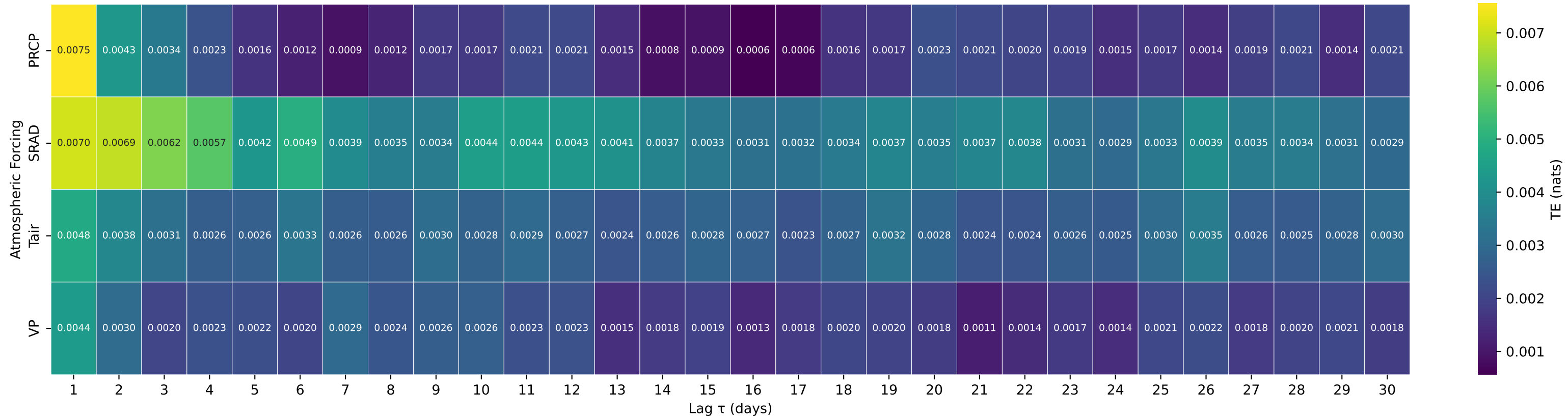
Shuffle-Test Significant TE to Streamflow — Basin 10336645 (HUC 16) — GENERAL C NR MEEKS BAY CA
