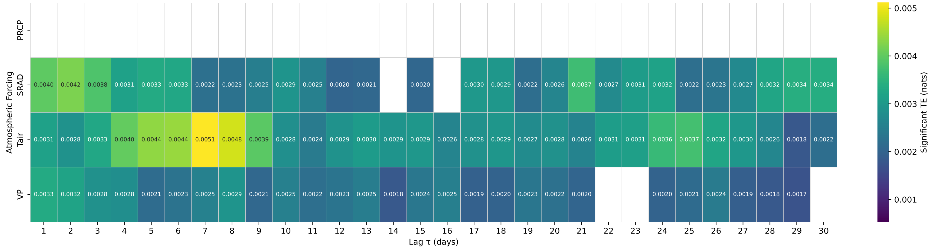
Shuffle-Test Significant TE to Streamflow — Basin 13018300 (HUC 17) — CACHE CREEK NEAR JACKSON, WY
