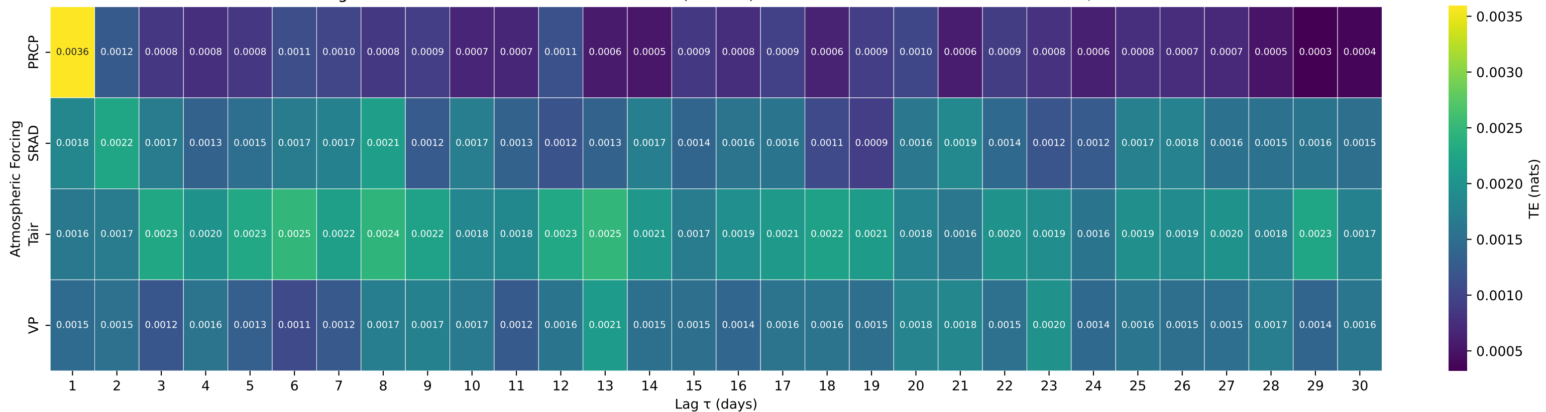
Shuffle-Test Significant TE to Streamflow — Basin 05399500 (HUC 07) — BIG EAU PLEINE RIVER AT STRATFORD, WI
