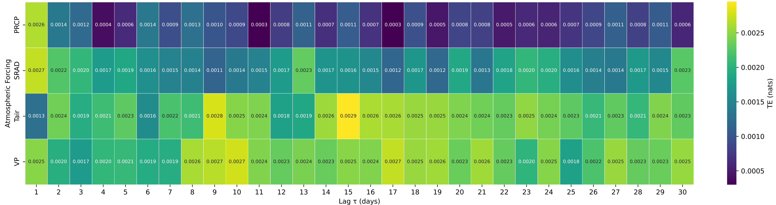
Shuffle-Test Significant TE to Streamflow — Basin 03500240 (HUC 06) — CARTOOGECHAYE CREEK NEAR FRANKLIN, NC
