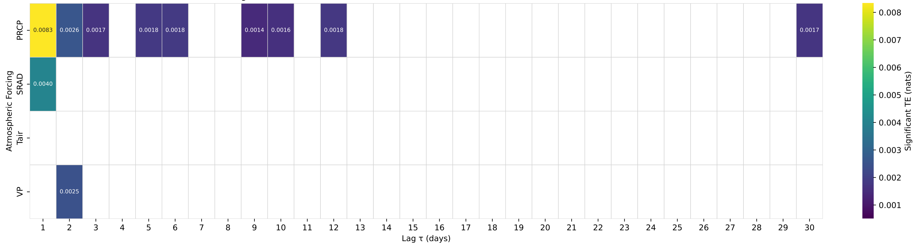
Shuffle-Test Significant TE to Streamflow — Basin 06906800 (HUC 10) — Lamine River near Otterville, MO
