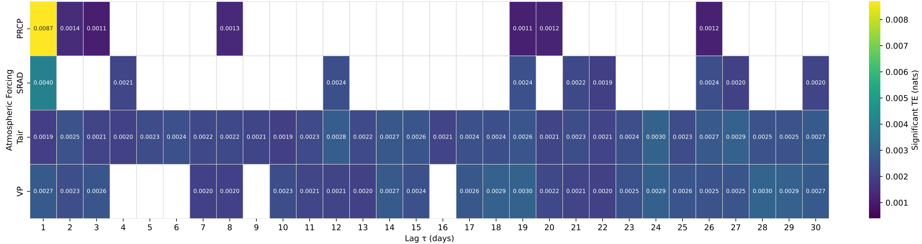
Shuffle-Test Significant TE to Streamflow — Basin 03300400 (HUC 05) — BEECH FORK AT MAUD, KY
