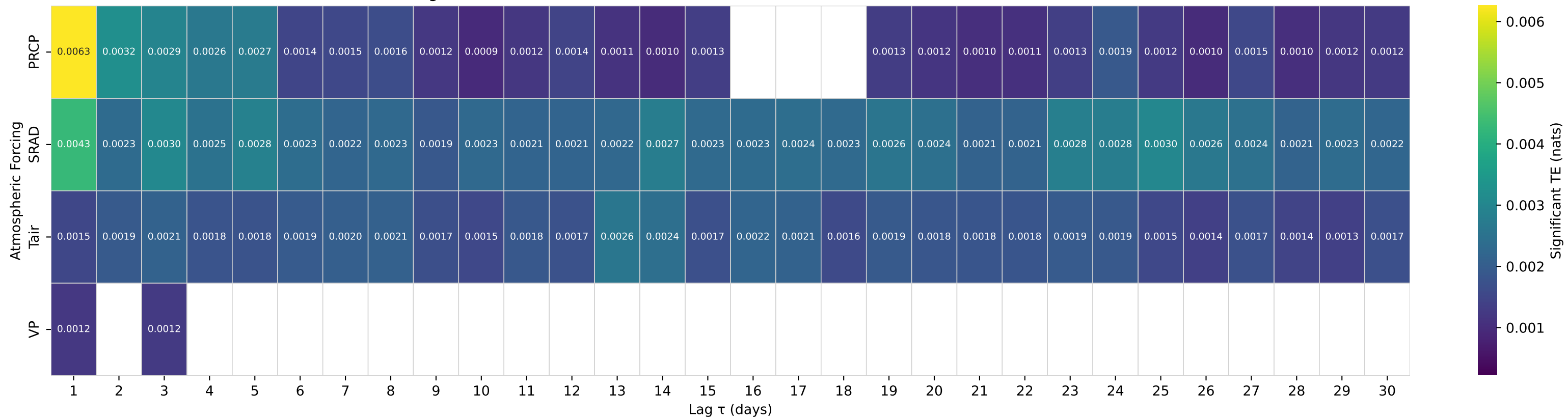
Shuffle-Test Significant TE to Streamflow — Basin 11475560 (HUC 18) — ELDER C NR BRANSCOMB CA
