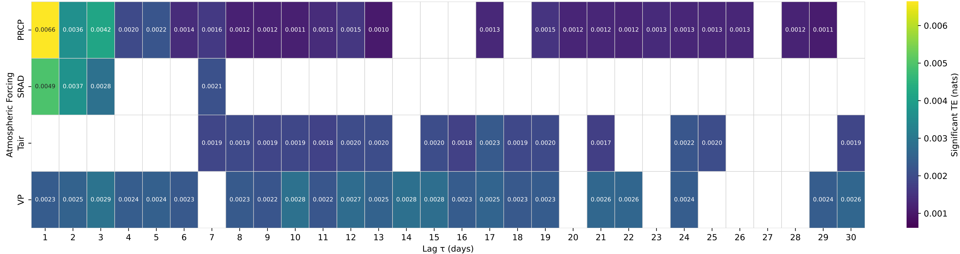
Shuffle-Test Significant TE to Streamflow — Basin 02296500 (HUC 03) — CHARLIE CREEK NEAR GARDNER FL
