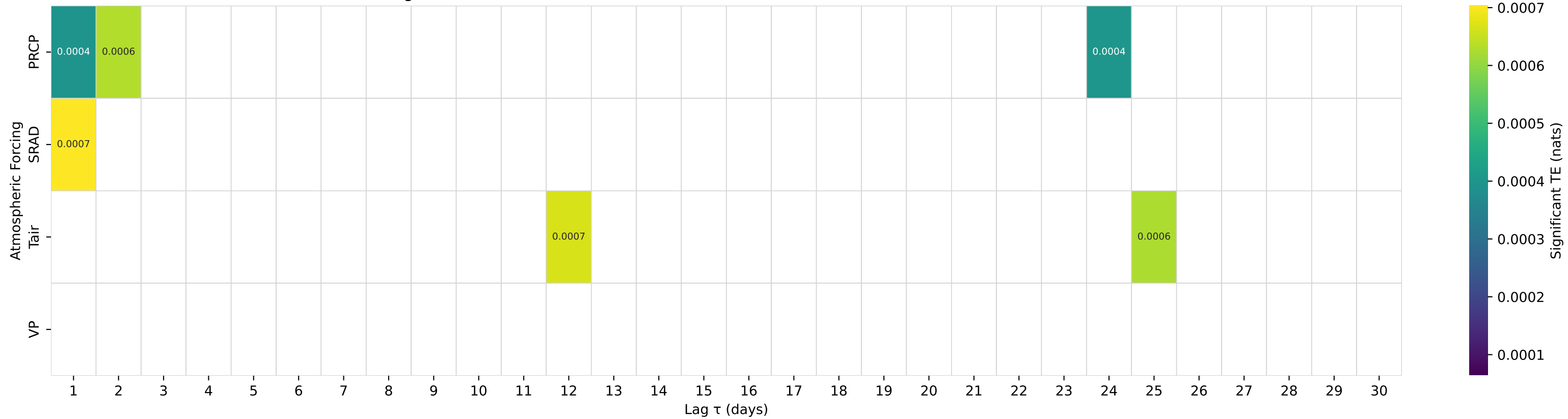
Shuffle-Test Significant TE to Streamflow — Basin 02064000 (HUC 03) — FALLING RIVER NEAR NARUNA, VA
