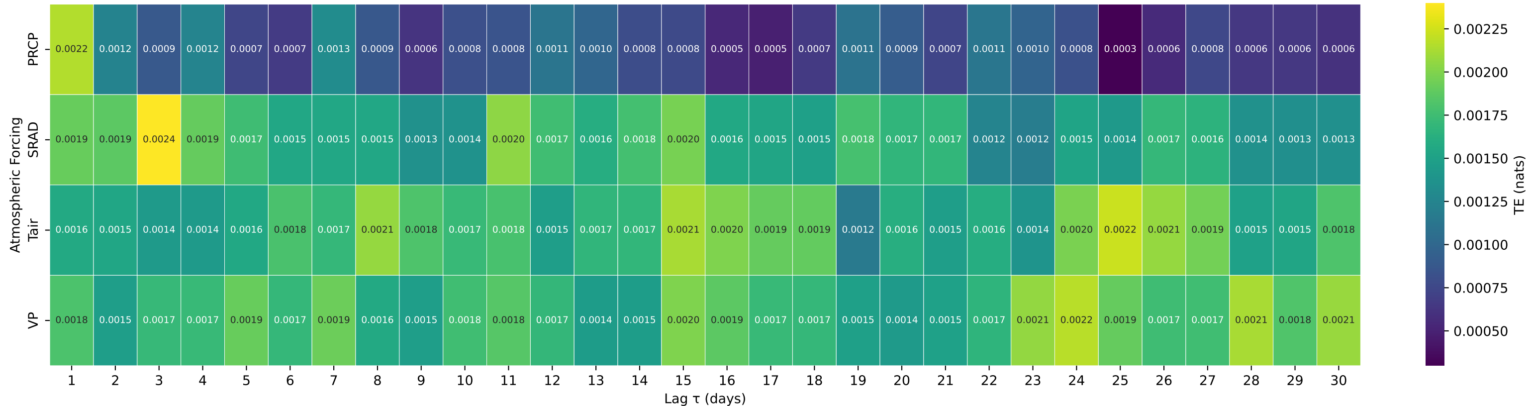
Shuffle-Test Significant TE to Streamflow — Basin 02028500 (HUC 02) — ROCKFISH RIVER NEAR GREENFIELD, VA
