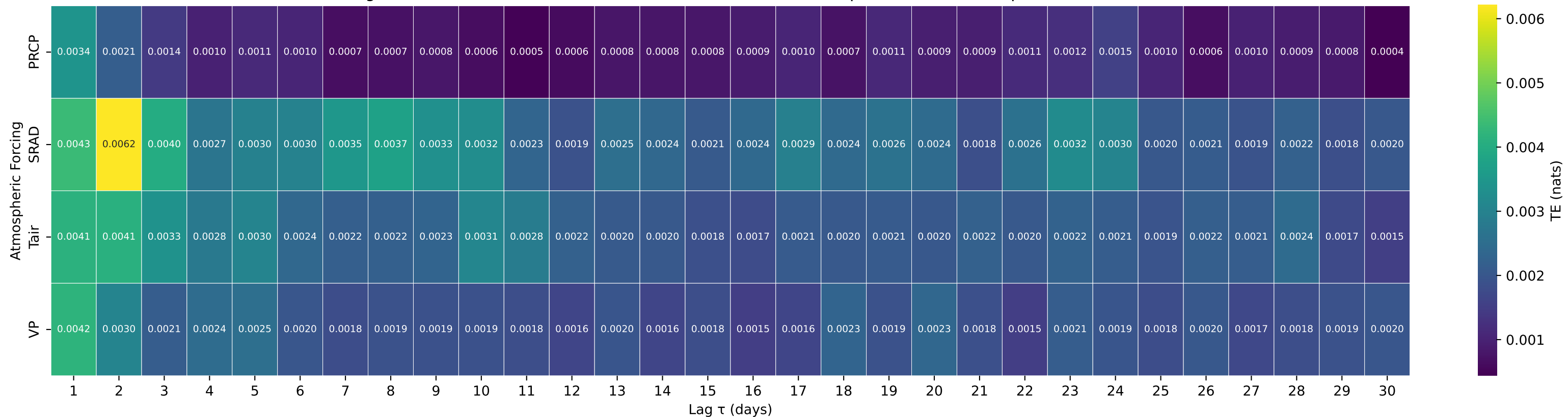
Shuffle-Test Significant TE to Streamflow — Basin 12390700 (HUC 17) — Prospect Creek at Thompson Falls MT
