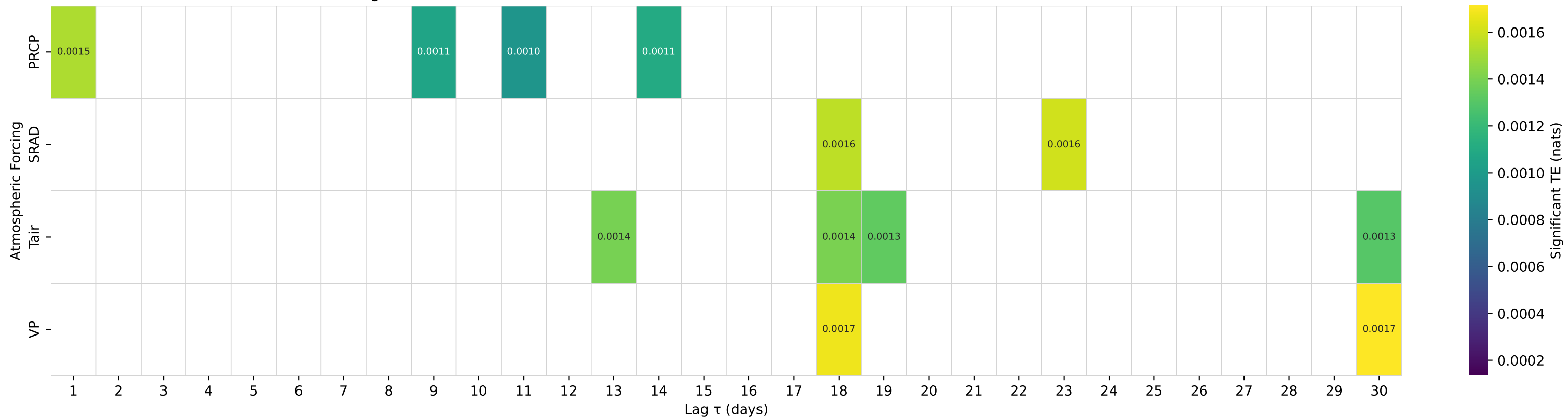
Shuffle-Test Significant TE to Streamflow — Basin 03479000 (HUC 06) — WATAUGA RIVER NEAR SUGAR GROVE, NC
