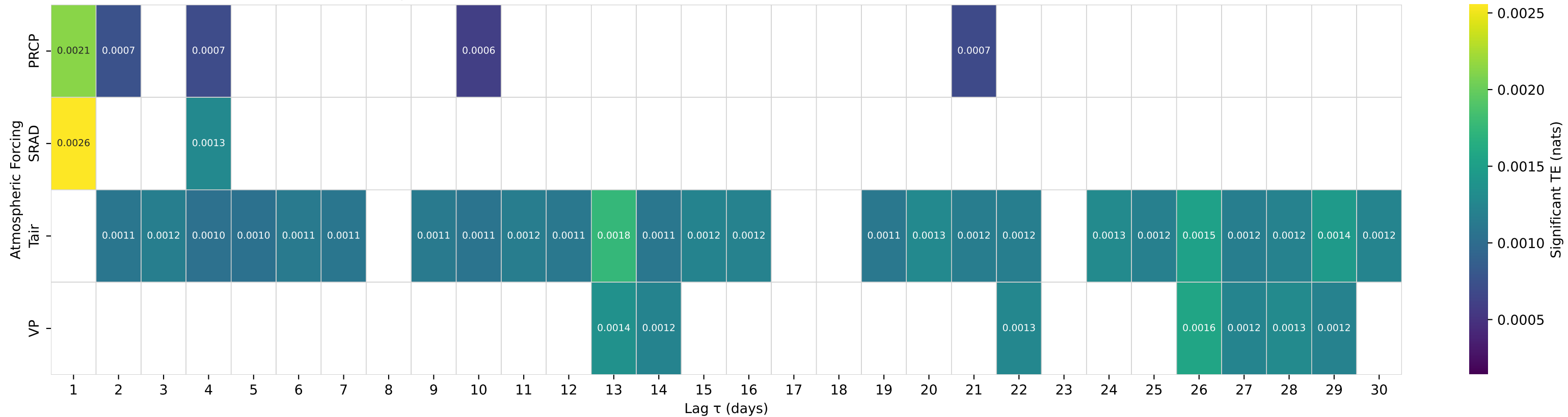
Shuffle-Test Significant TE to Streamflow — Basin 02349900 (HUC 03) — TURKEY CREEK AT BYROMVILLE, GA
