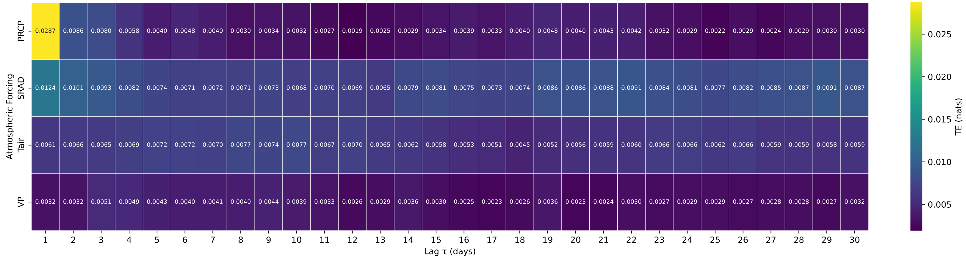
Shuffle-Test Significant TE to Streamflow — Basin 14166500 (HUC 17) — LONG TOM RIVER NEAR NOTI, OREG.
