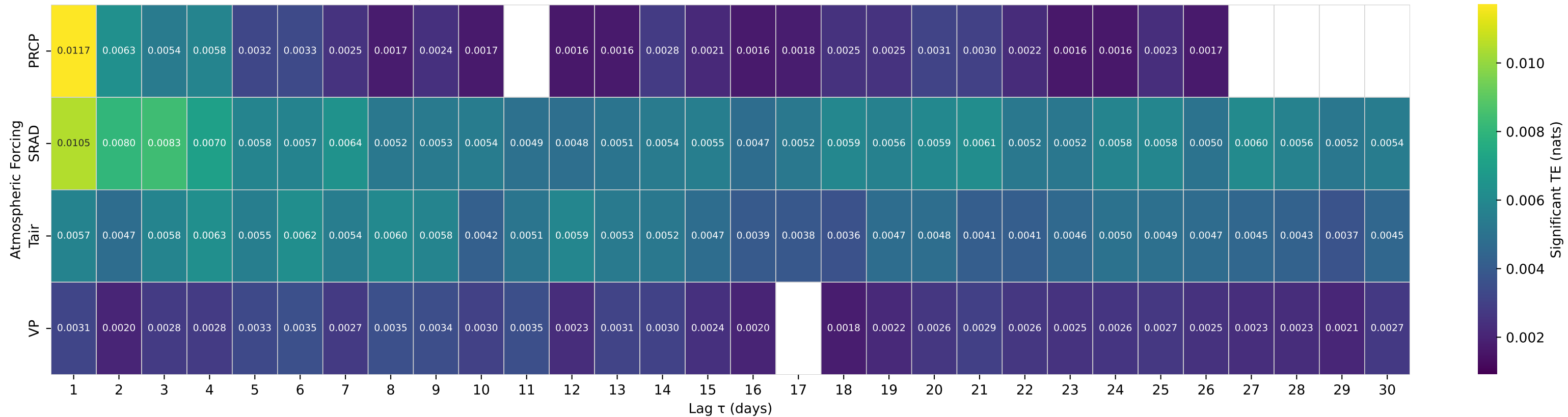
Shuffle-Test Significant TE to Streamflow — Basin 14187000 (HUC 17) — WILEY CREEK NEAR FOSTER, OR
