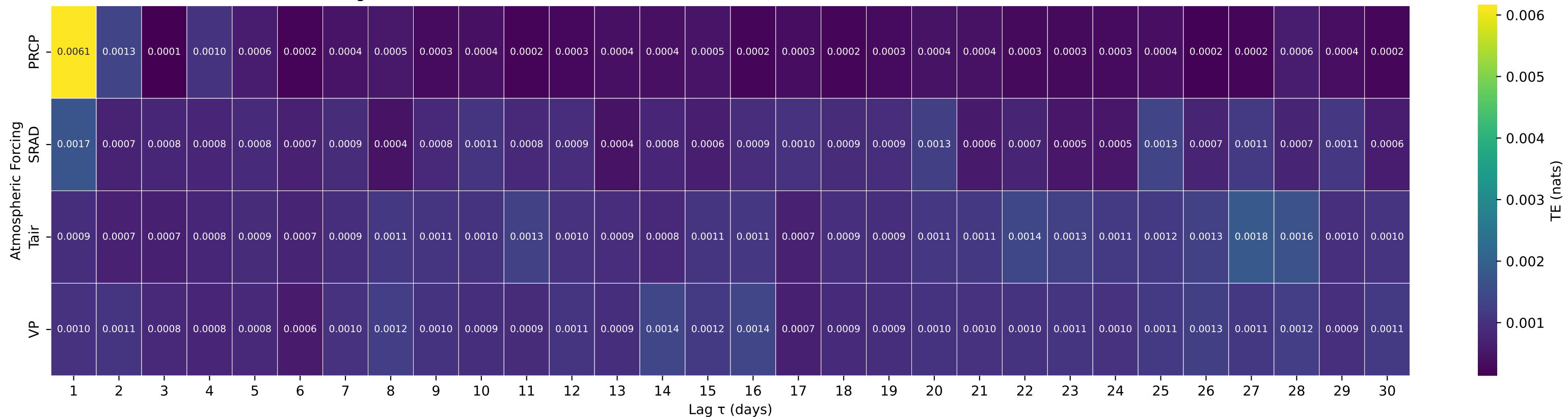
Shuffle-Test Significant TE to Streamflow — Basin 03604000 (HUC 06) — BUFFALO RIVER NEAR FLAT WOODS, TN
