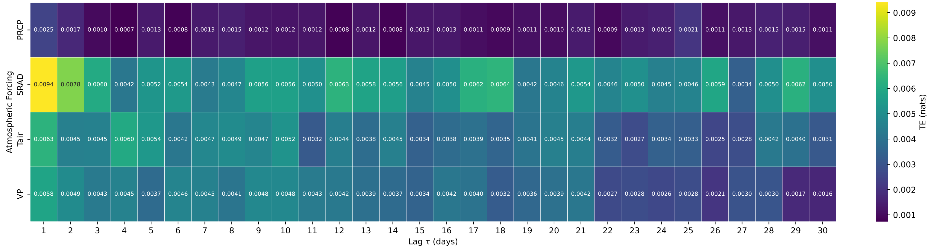
Shuffle-Test Significant TE to Streamflow — Basin 07083000 (HUC 11) — HALFMOON CREEK NEAR MALTA, CO.
