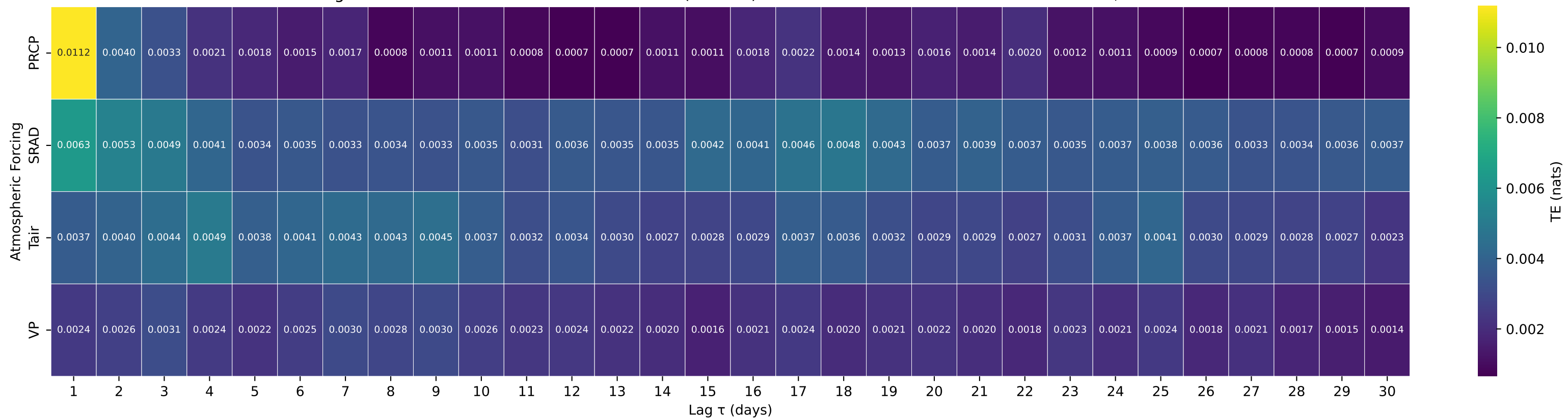
Shuffle-Test Significant TE to Streamflow — Basin 14222500 (HUC 17) — EAST FORK LEWIS RIVER NEAR HEISSON, WA
