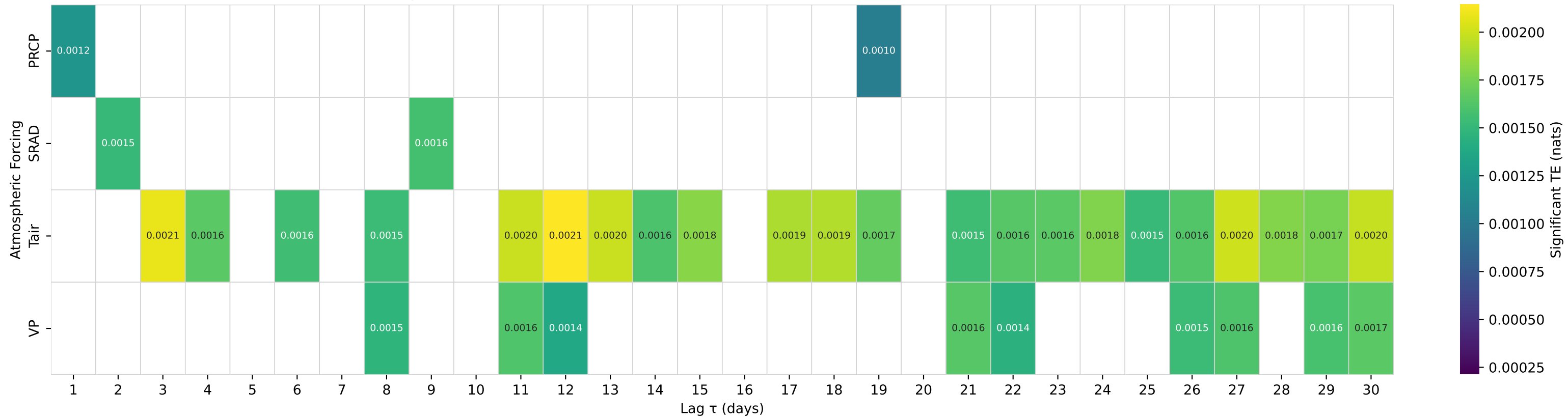
Shuffle-Test Significant TE to Streamflow — Basin 04233000 (HUC 04) — CAYUGA INLET NEAR ITHACA NY
