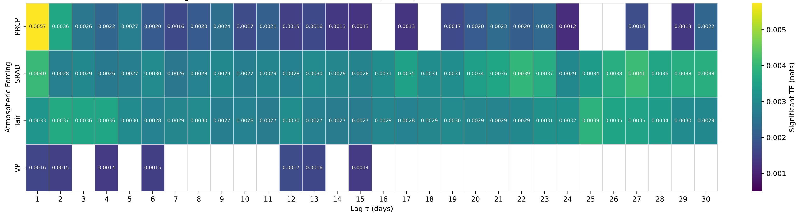
Shuffle-Test Significant TE to Streamflow — Basin 11284400 (HUC 18) — BIG C AB WHITES GULCH NR GROVELAND CA
