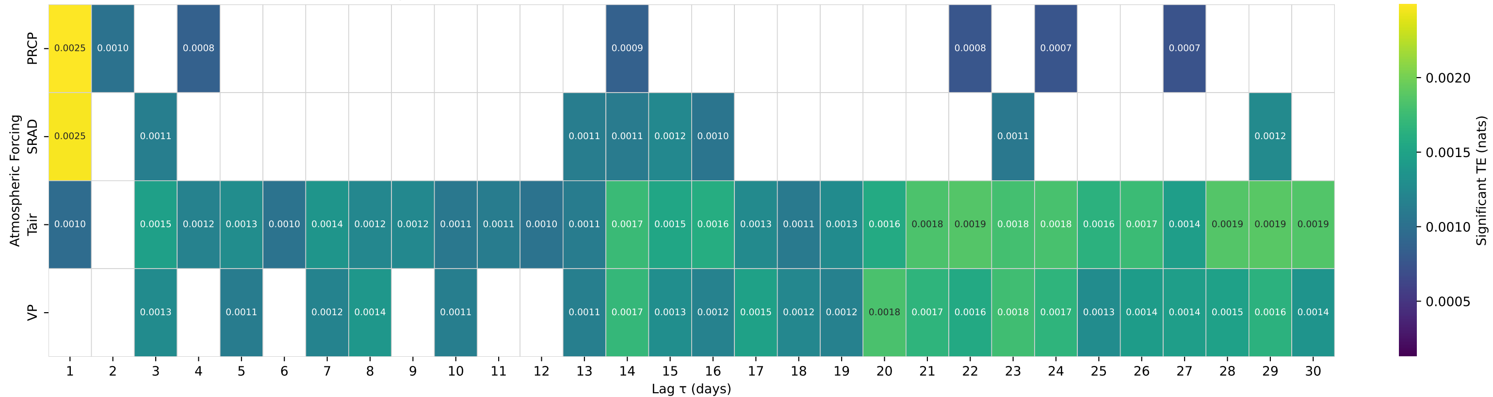
Shuffle-Test Significant TE to Streamflow — Basin 02422500 (HUC 03) — MULBERRY CREEK AT JONES AL
