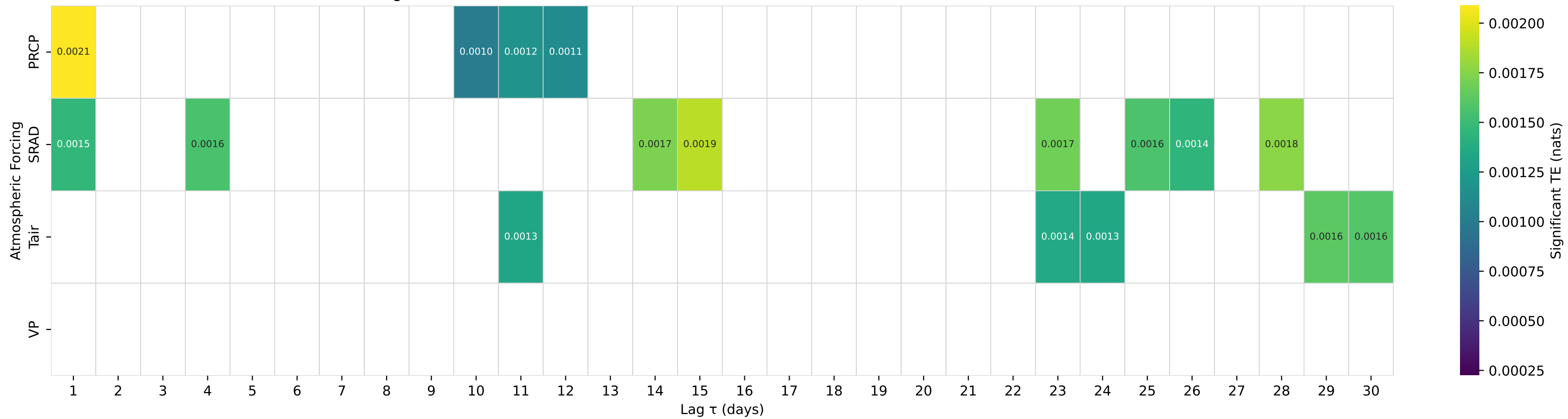
Shuffle-Test Significant TE to Streamflow — Basin 06344600 (HUC 10) — GREEN RIVER NR NEW HRADEC, ND
