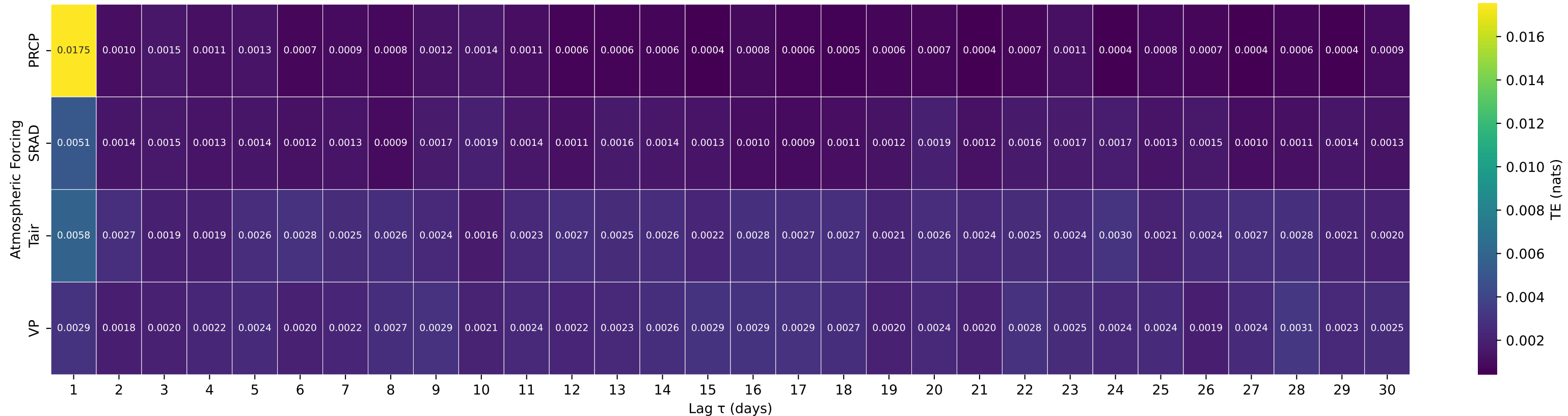
Shuffle-Test Significant TE to Streamflow — Basin 04105700 (HUC 04) — AUGUSTA CREEK NEAR AUGUSTA, MI
