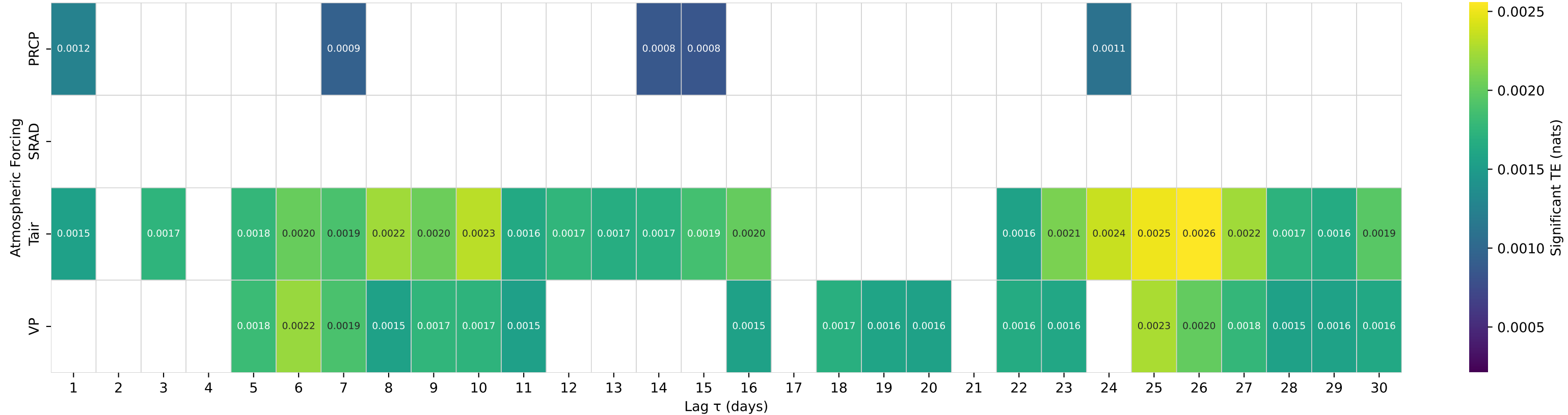
Shuffle-Test Significant TE to Streamflow — Basin 01634500 (HUC 02) — CEDAR CREEK NEAR WINCHESTER, VA
