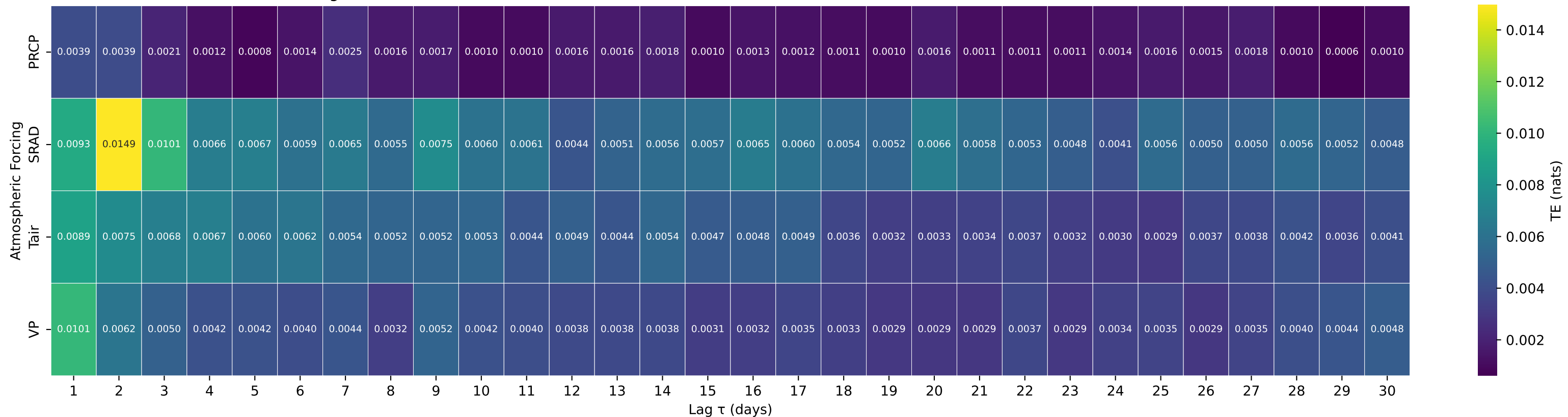
Shuffle-Test Significant TE to Streamflow — Basin 12358500 (HUC 17) — Middle Fork Flathead River nr West Glacier MT
