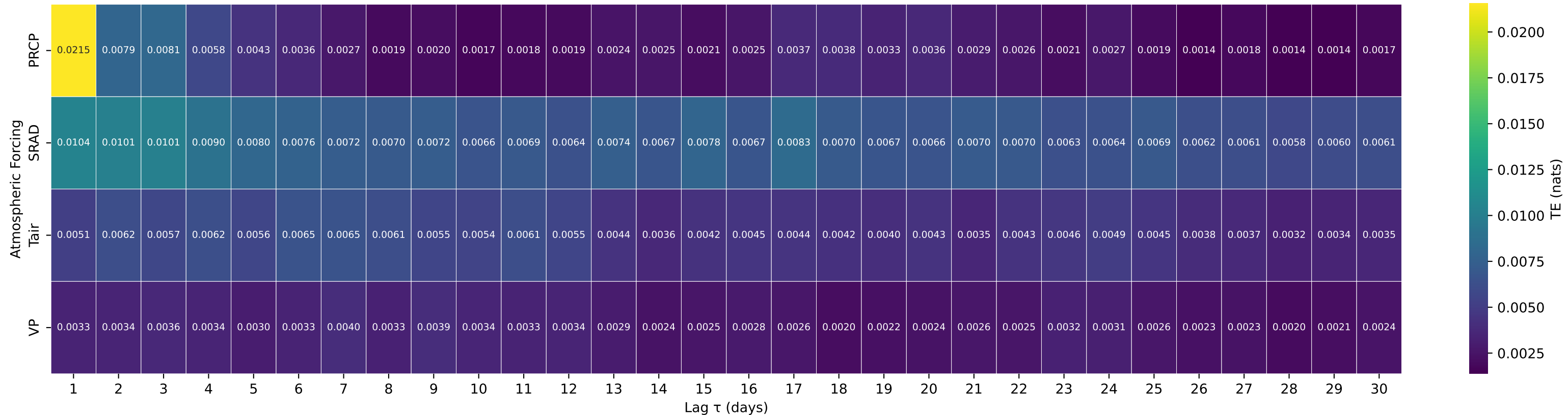
Shuffle-Test Significant TE to Streamflow — Basin 14303200 (HUC 17) — TUCCA CREEK NEAR BLAINE, OR.
