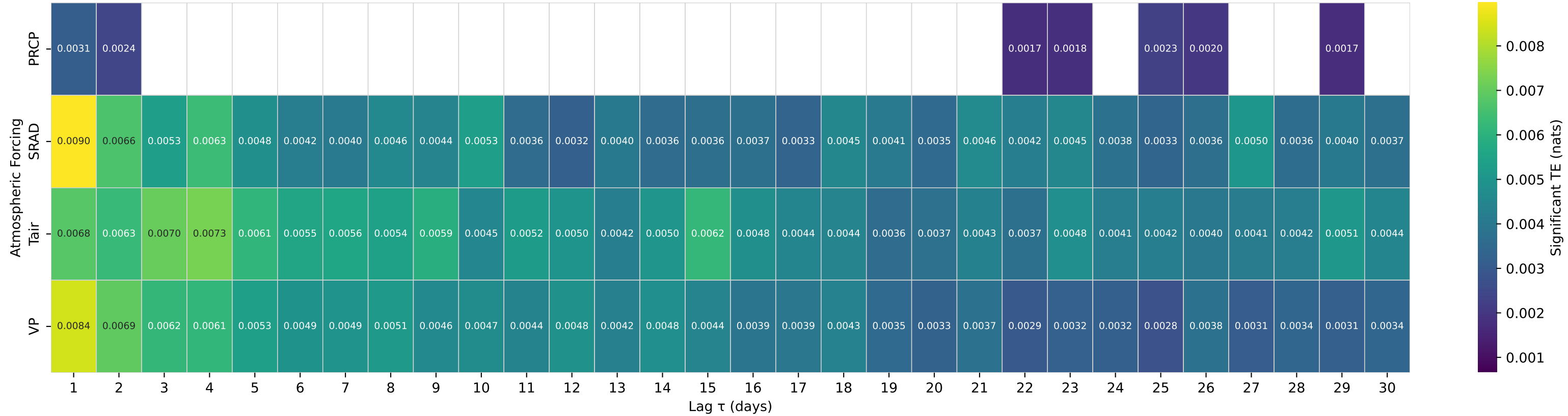
Shuffle-Test Significant TE to Streamflow — Basin 09066200 (HUC 14) — BOOTH CREEK NEAR MINTURN, CO.
