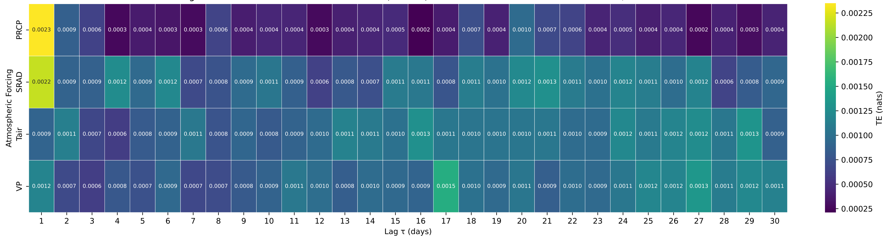
Shuffle-Test Significant TE to Streamflow — Basin 02112120 (HUC 03) — ROARING RIVER NEAR ROARING RIVER, NC
