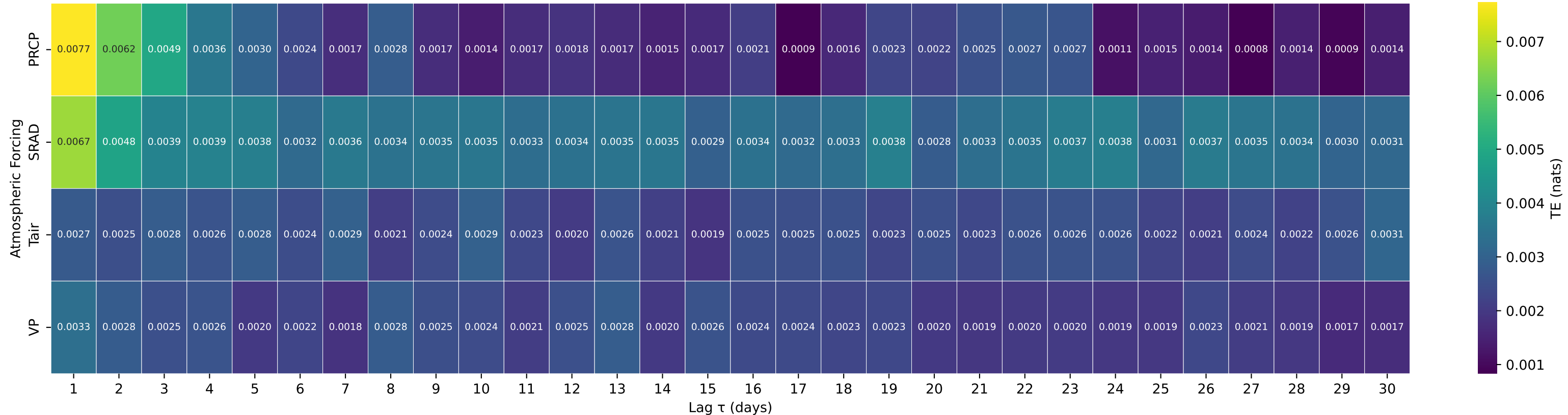
Shuffle-Test Significant TE to Streamflow — Basin 11162500 (HUC 18) — PESCADERO C NR PESCADERO CA
