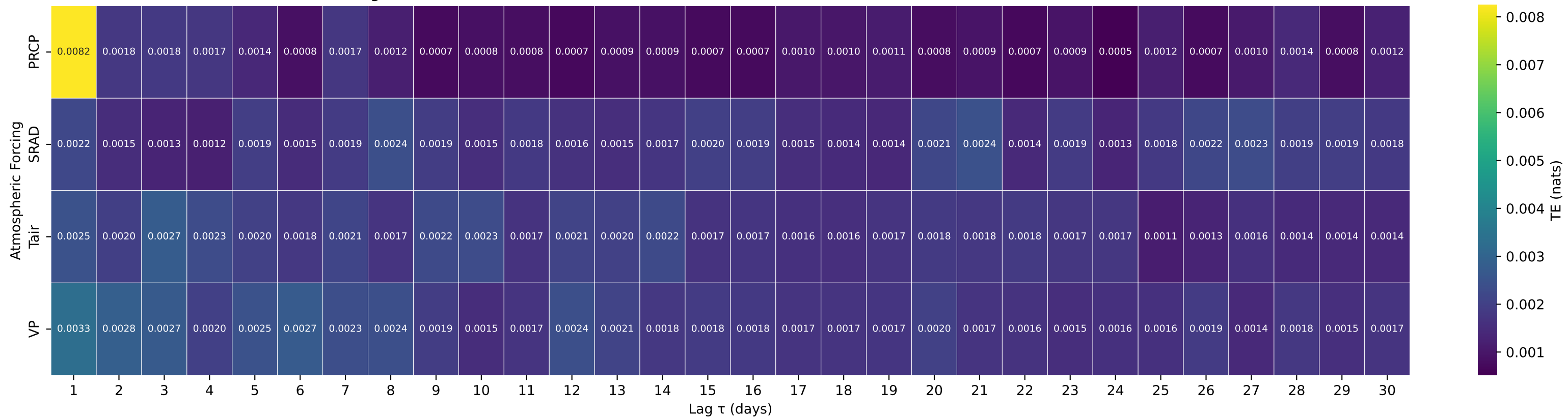
Shuffle-Test Significant TE to Streamflow — Basin 07148400 (HUC 11) — Salt Fork Arkansas River nr Alva, OK
