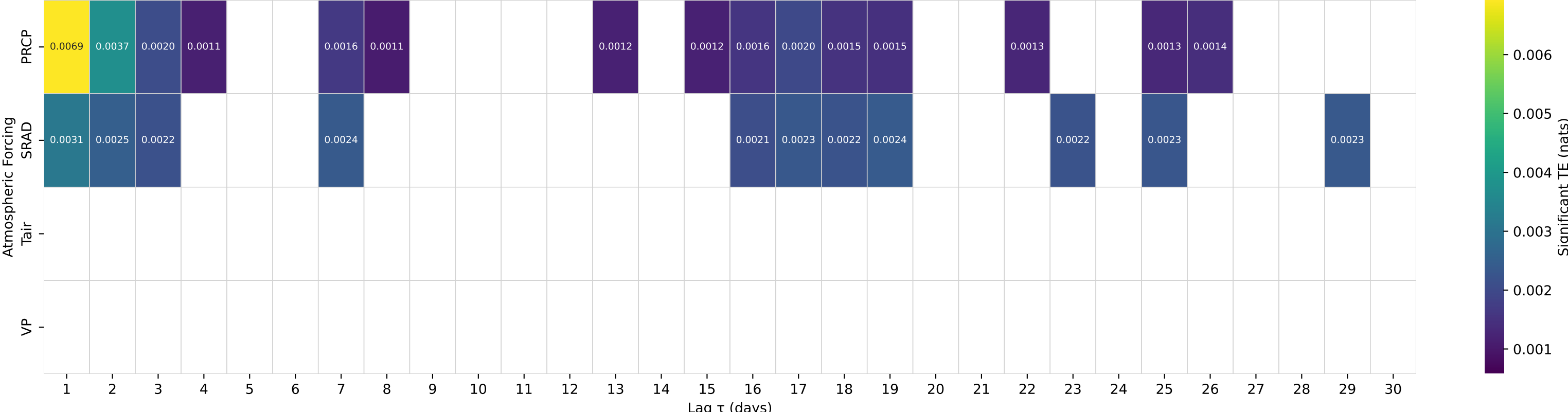
Shuffle-Test Significant TE to Streamflow — Basin 07362100 (HUC 08) — SMACKOVER CREEK NEAR SMACKOVER, ARK.
