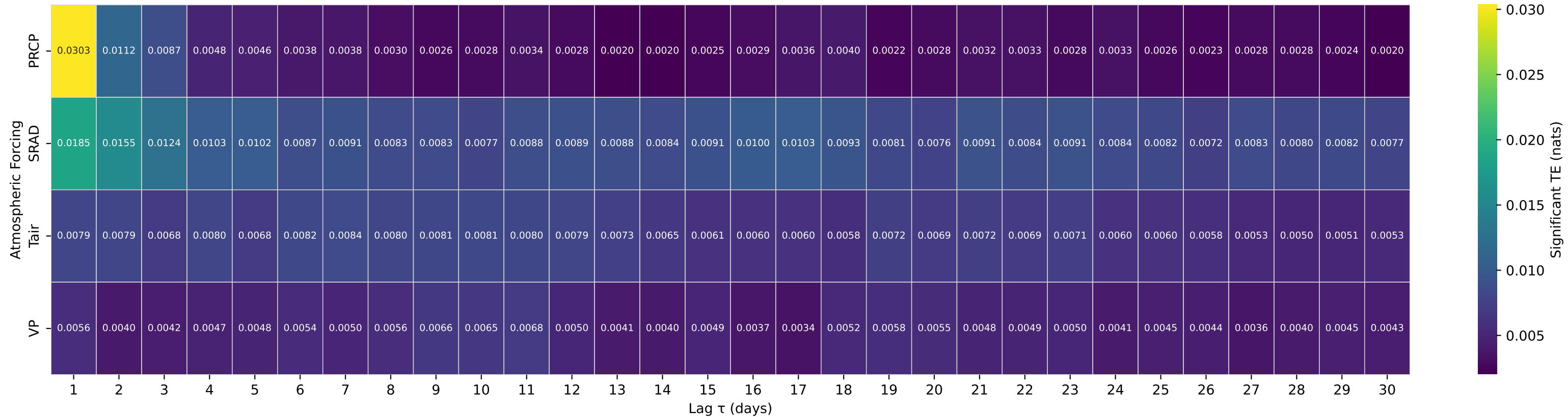
Shuffle-Test Significant TE to Streamflow — Basin 12013500 (HUC 17) — WILLAPA RIVER NEAR WILLAPA, WA
