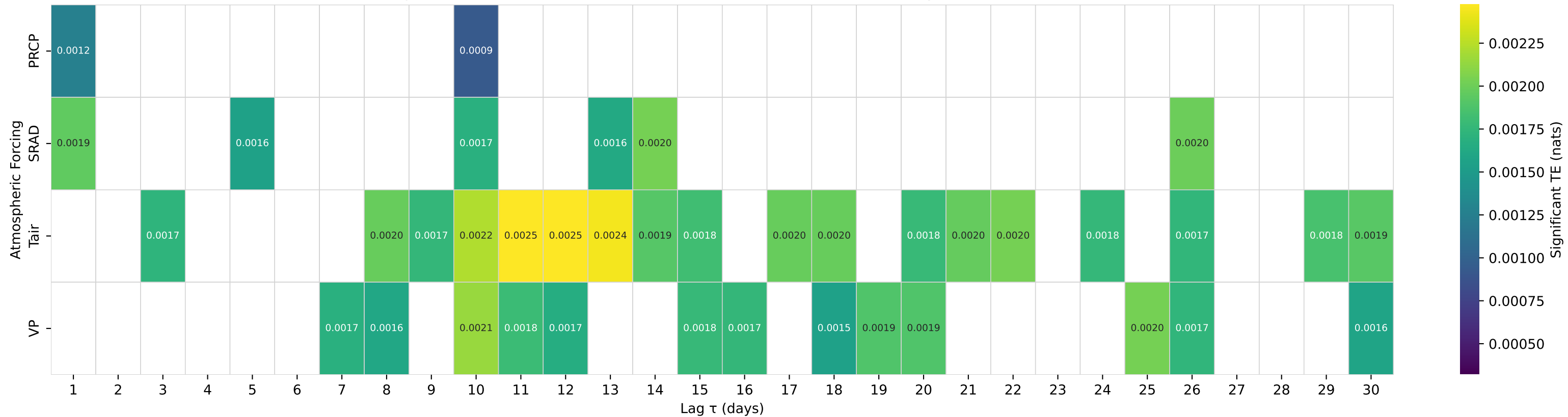
Shuffle-Test Significant TE to Streamflow — Basin 01552500 (HUC 02) — Muncy Creek near Sonestown, PA
