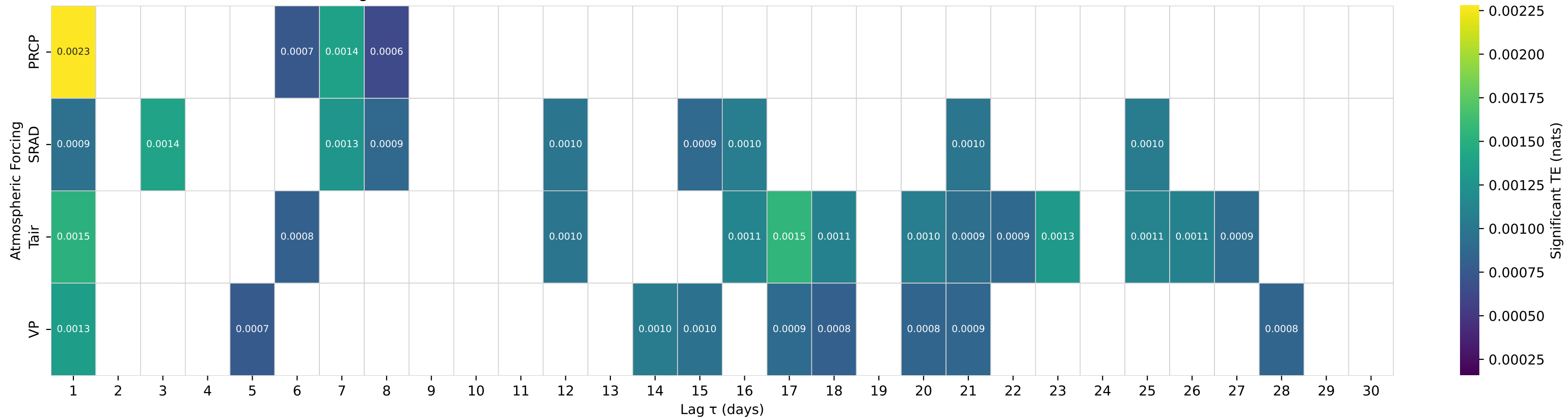
Shuffle-Test Significant TE to Streamflow — Basin 01047000 (HUC 01) — Carrabassett River near North Anson, Maine
