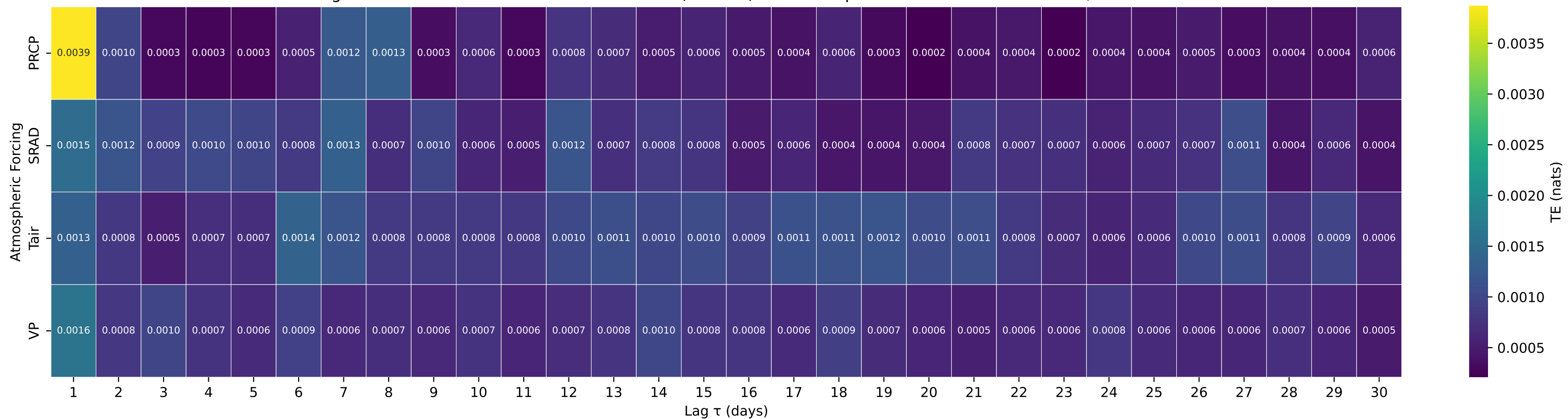
Shuffle-Test Significant TE to Streamflow — Basin 01031500 (HUC 01) — Piscataquis River near Dover-Foxcroft, Maine
