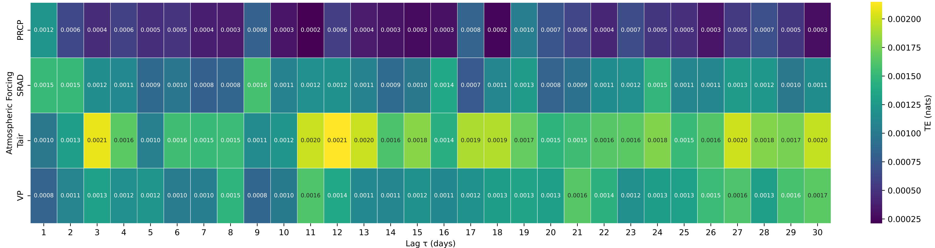
Shuffle-Test Significant TE to Streamflow — Basin 04233000 (HUC 04) — CAYUGA INLET NEAR ITHACA NY
