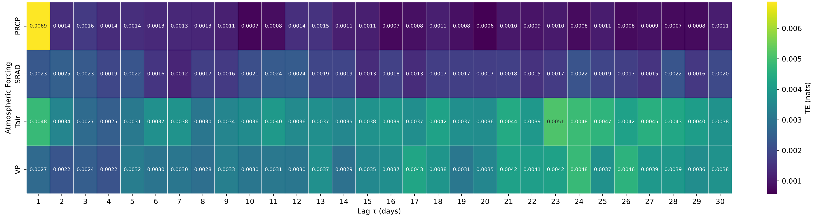
Shuffle-Test Significant TE to Streamflow — Basin 04161580 (HUC 04) — STONY CREEK NEAR ROMEO, MI
