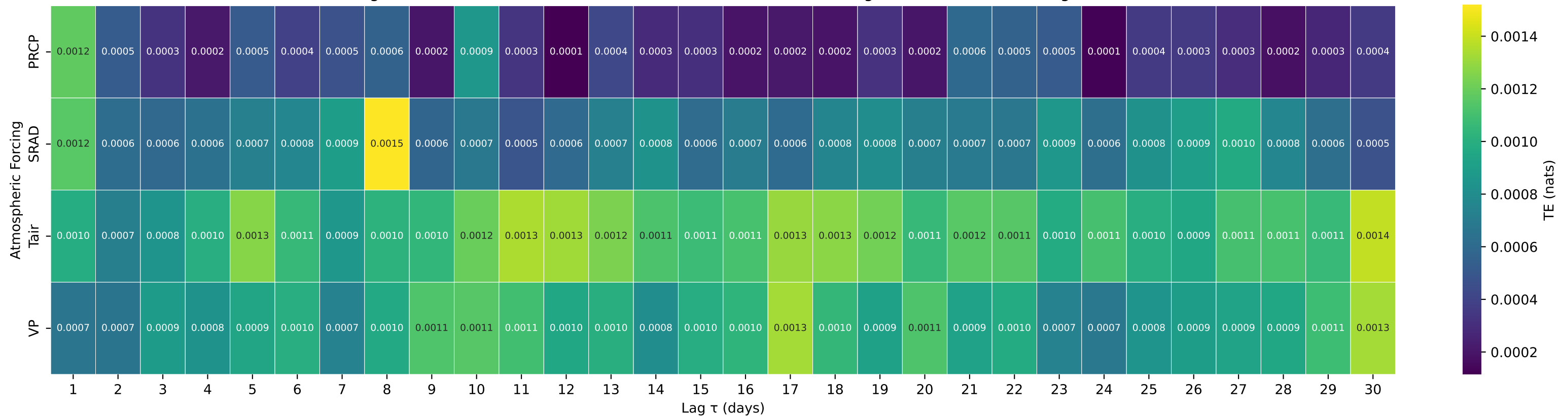
Shuffle-Test Significant TE to Streamflow — Basin 01539000 (HUC 02) — Fishing Creek near Bloomsburg, PA
