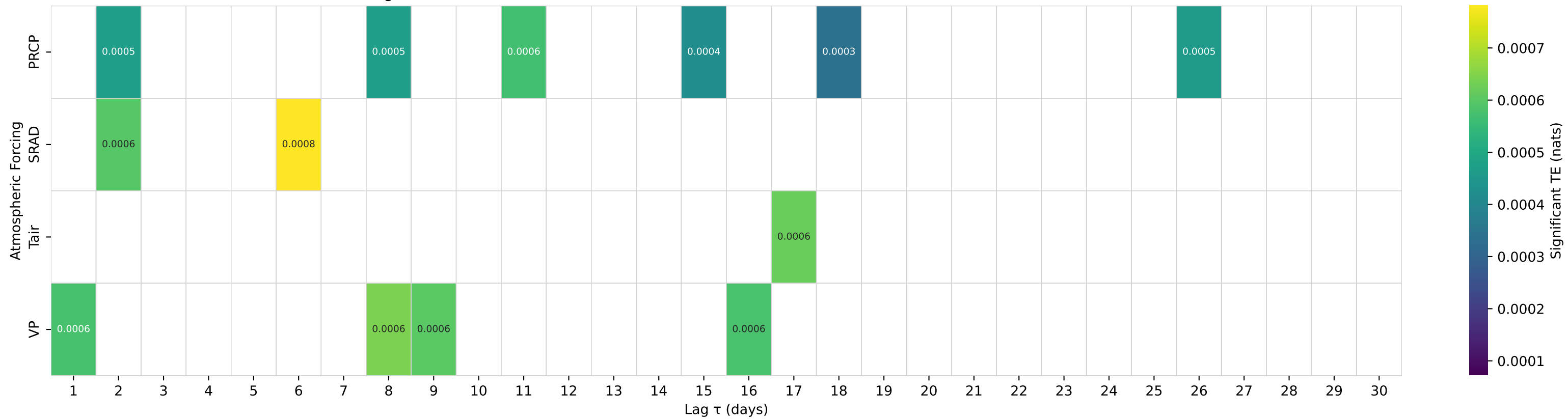
Shuffle-Test Significant TE to Streamflow — Basin 04015330 (HUC 04) — KNIFE RIVER NEAR TWO HARBORS, MN
