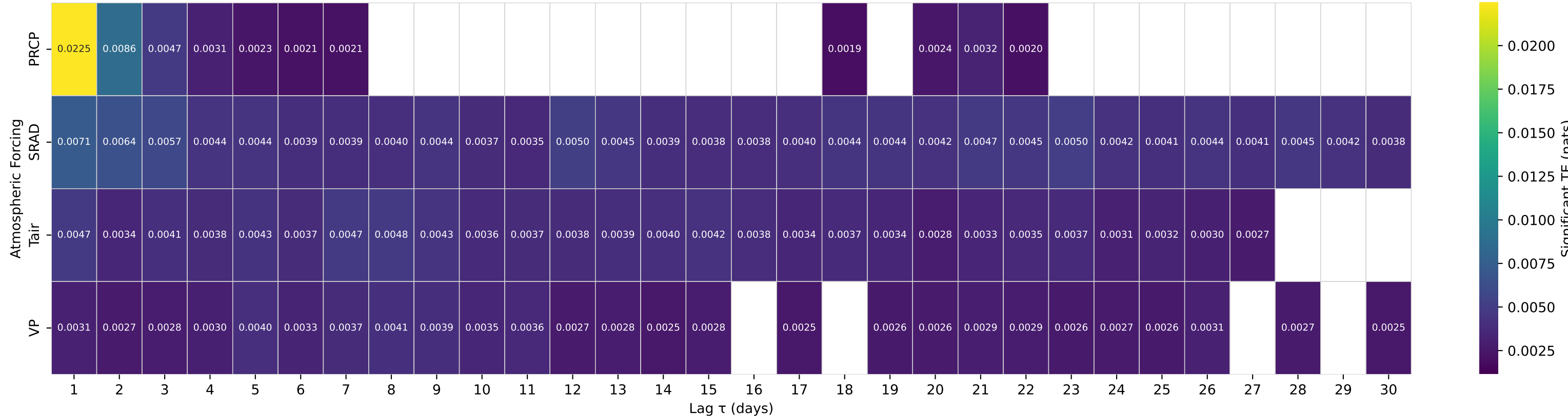
Shuffle-Test Significant TE to Streamflow — Basin 12141300 (HUC 17) — MIDDLE FORK SNOQUALMIE RIVER NEAR TANNER, WA
