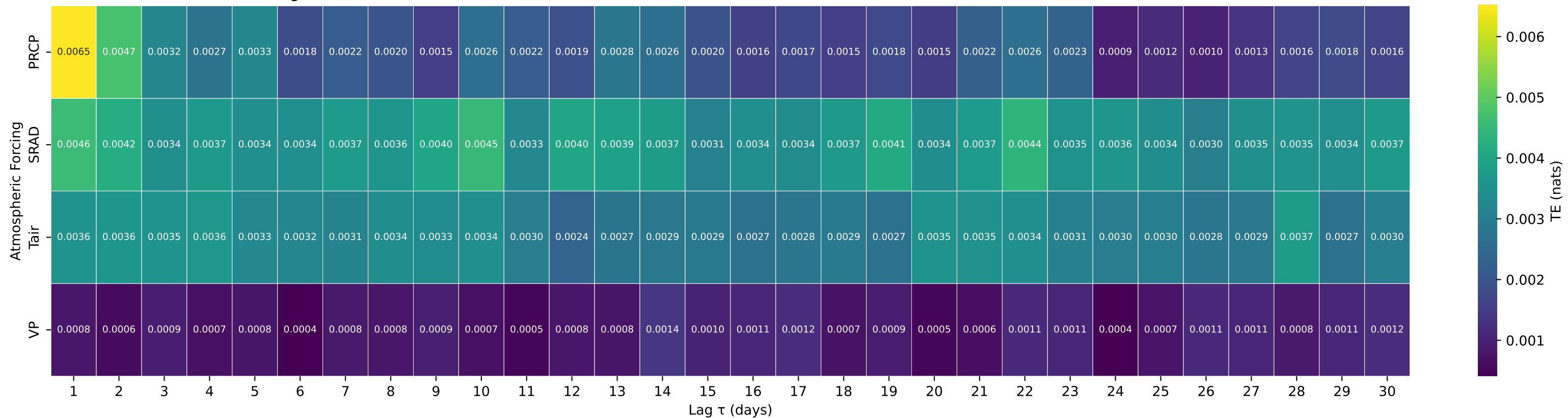
Shuffle-Test Significant TE to Streamflow — Basin 11451100 (HUC 18) — NF CACHE C A HOUGH SPRING NR CLEARLAKE OAKS CA
