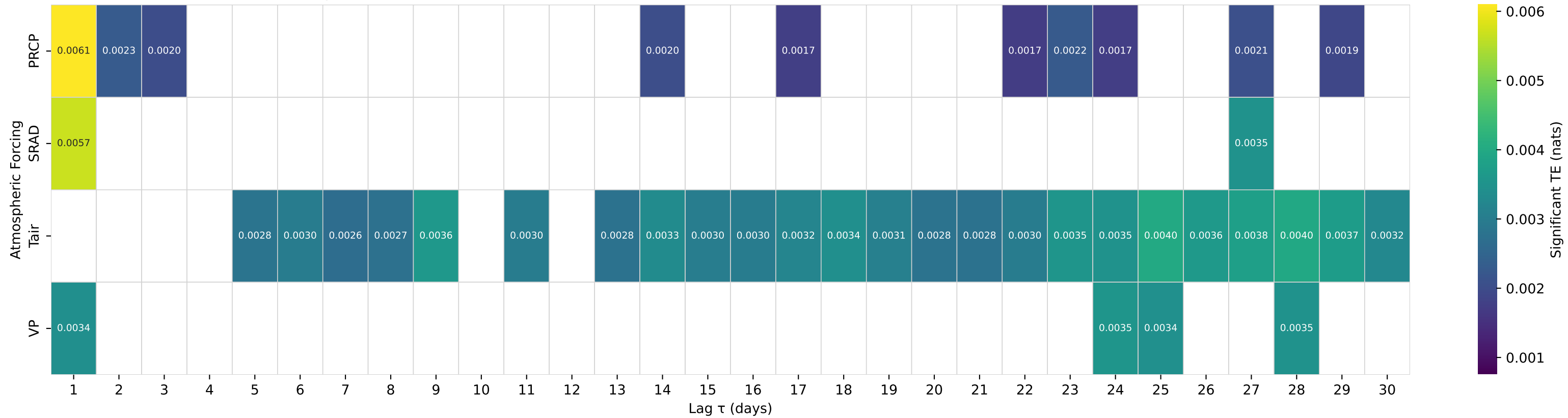
Shuffle-Test Significant TE to Streamflow — Basin 02464360 (HUC 03) — BINION CREEK BELOW GIN CREEK NEAR SAMANTHA AL
