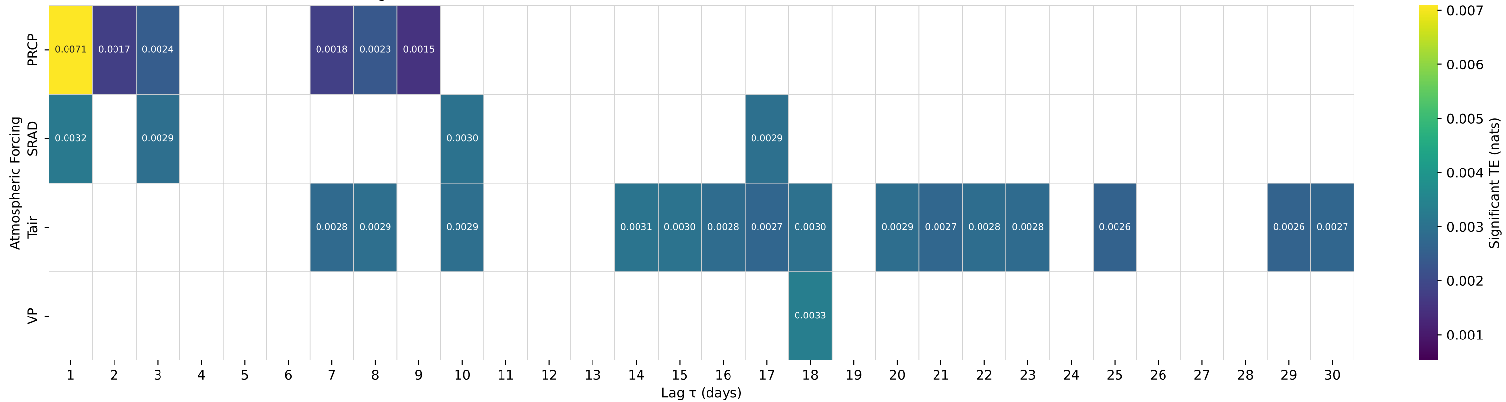
Shuffle-Test Significant TE to Streamflow — Basin 05591550 (HUC 07) — WHITLEY CREEK NEAR ALLENVILLE, IL
