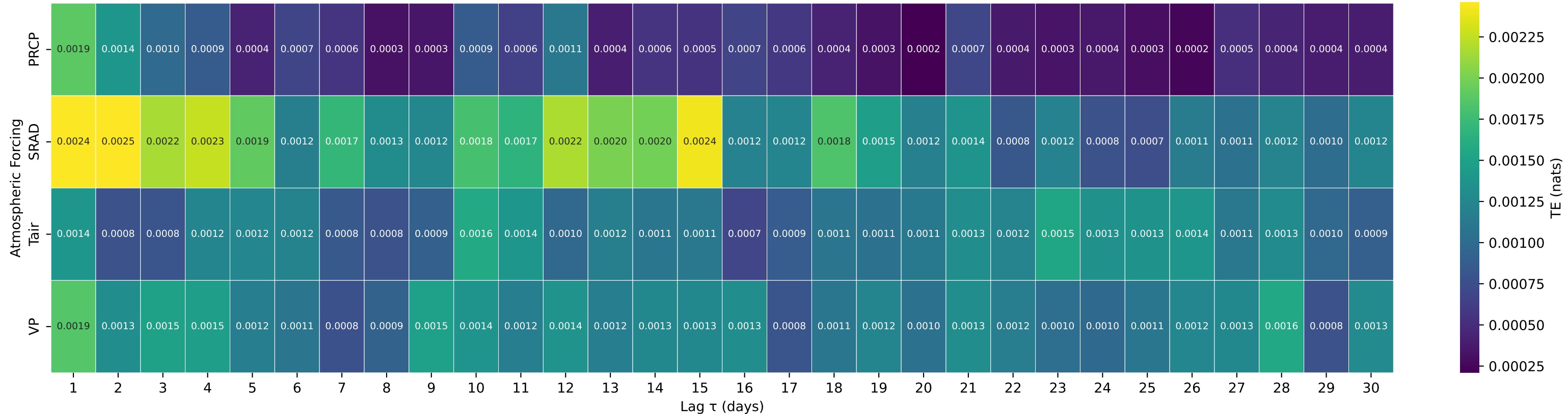
Shuffle-Test Significant TE to Streamflow — Basin 09492400 (HUC 15) — EAST FORK WHITE RIVER NEAR FORT APACHE, AZ.
