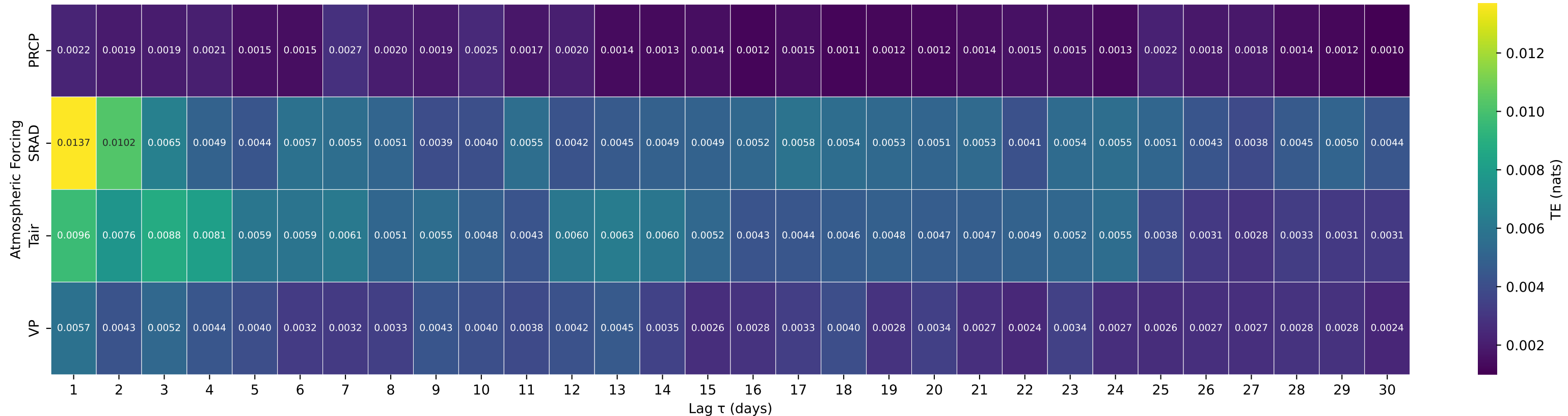
Shuffle-Test Significant TE to Streamflow — Basin 06188000 (HUC 10) — LAMAR RIVER NR TOWER FALLS RANGER STATION, YNP
