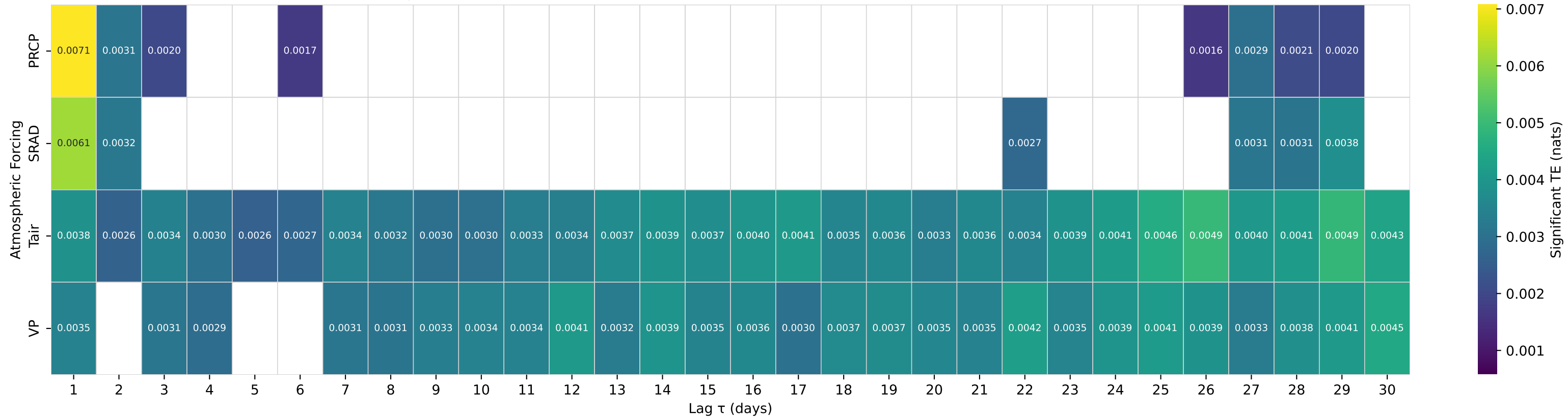
Shuffle-Test Significant TE to Streamflow — Basin 02464000 (HUC 03) — NORTH RIVER NEAR SAMANTHA AL
