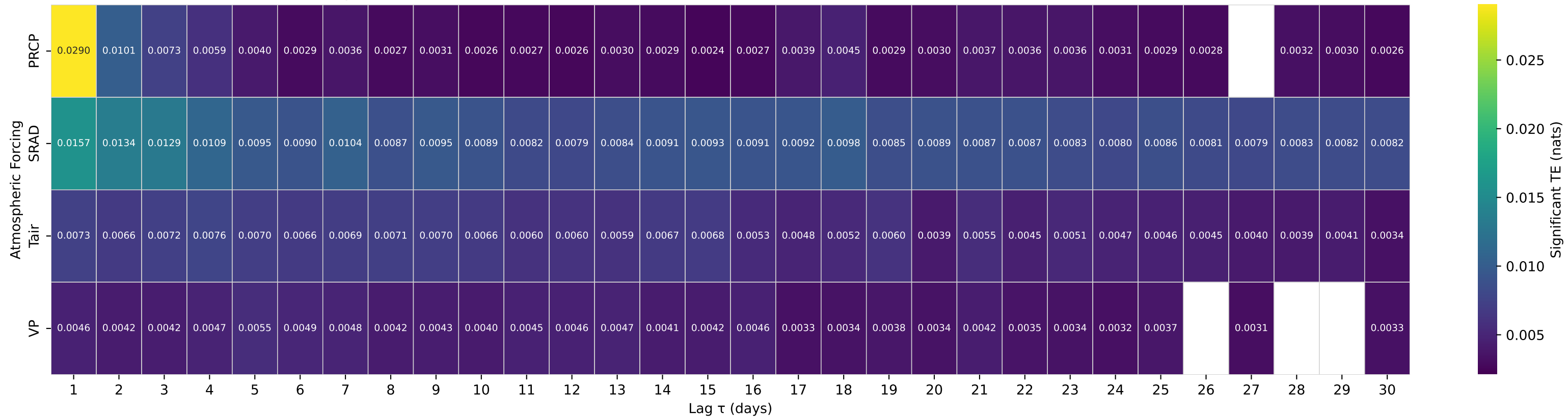
Shuffle-Test Significant TE to Streamflow — Basin 12041200 (HUC 17) — HOH RIVER AT US HIGHWAY 101 NEAR FORKS, WA
