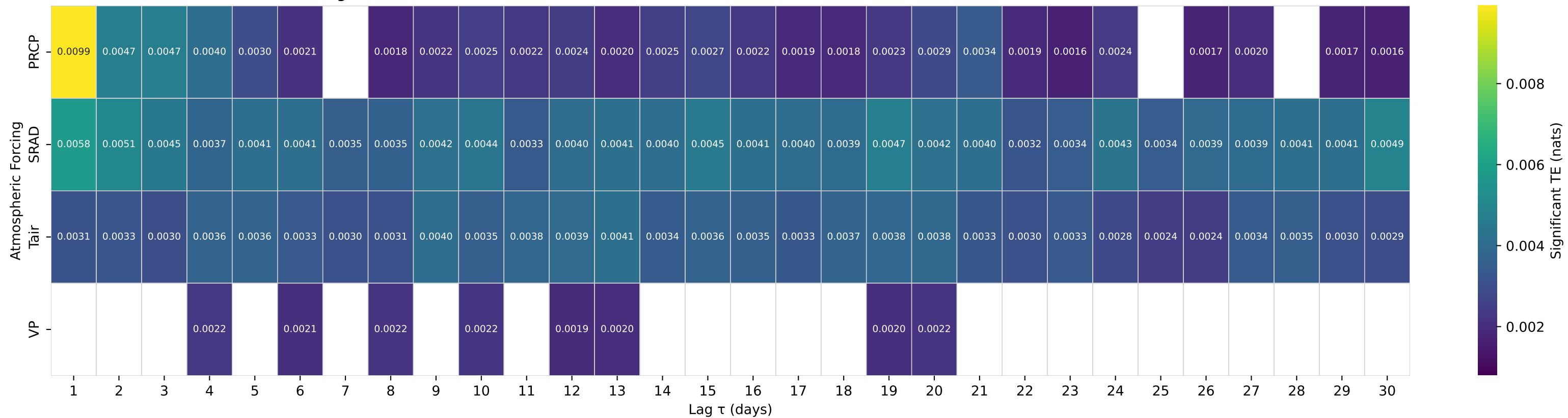
Shuffle-Test Significant TE to Streamflow — Basin 14308990 (HUC 17) — COW CREEK ABV GALESVILLE RES, NR AZALEA, OR.
