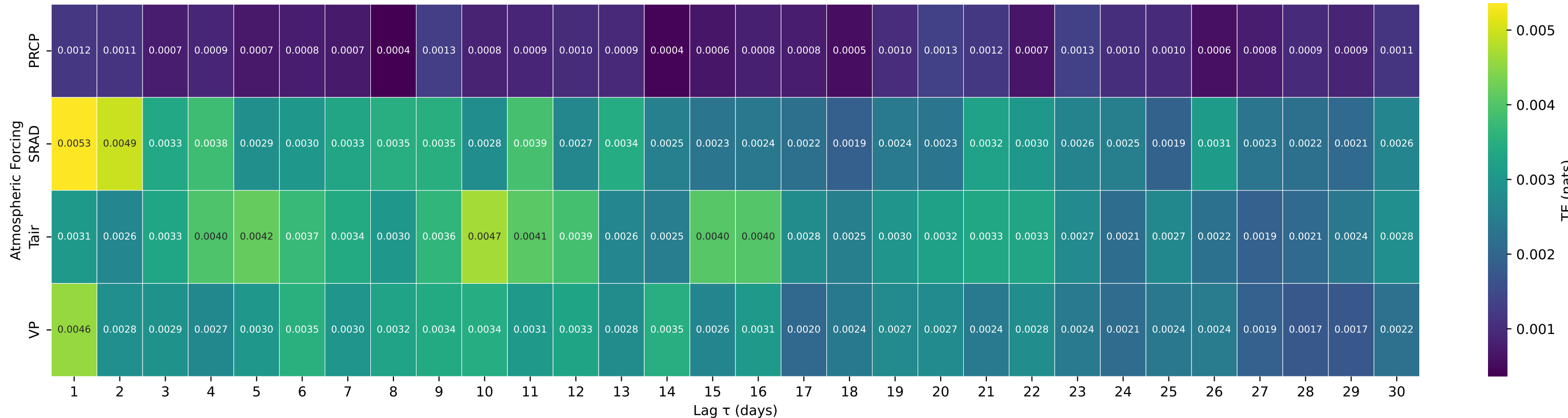
Shuffle-Test Significant TE to Streamflow — Basin 09035800 (HUC 14) — DARLING CREEK NEAR LEAL, CO.
