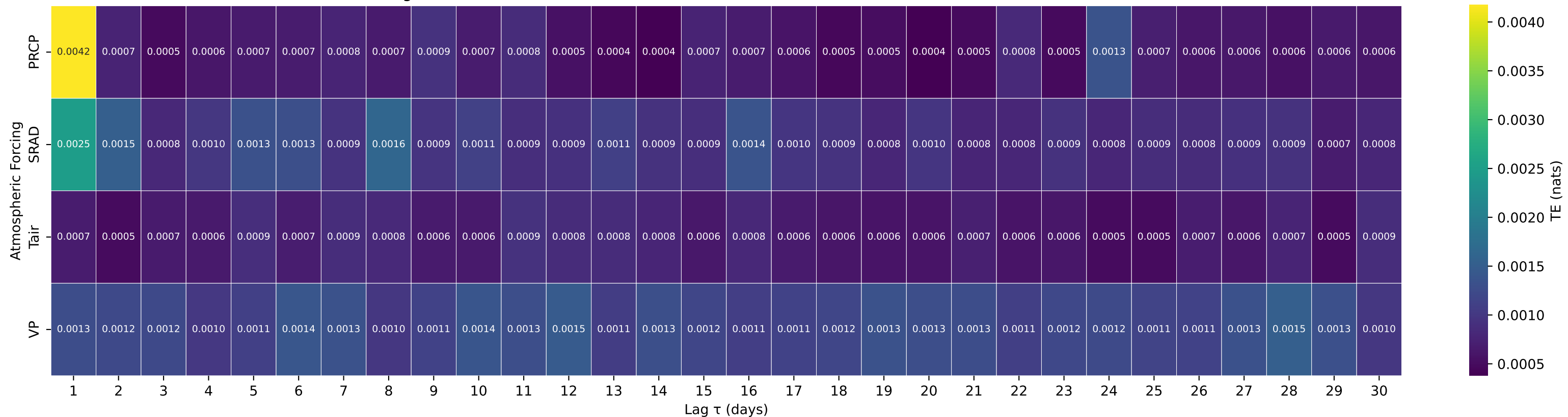
Shuffle-Test Significant TE to Streamflow — Basin 09430500 (HUC 15) — GILA RIVER NEAR GILA, NM
