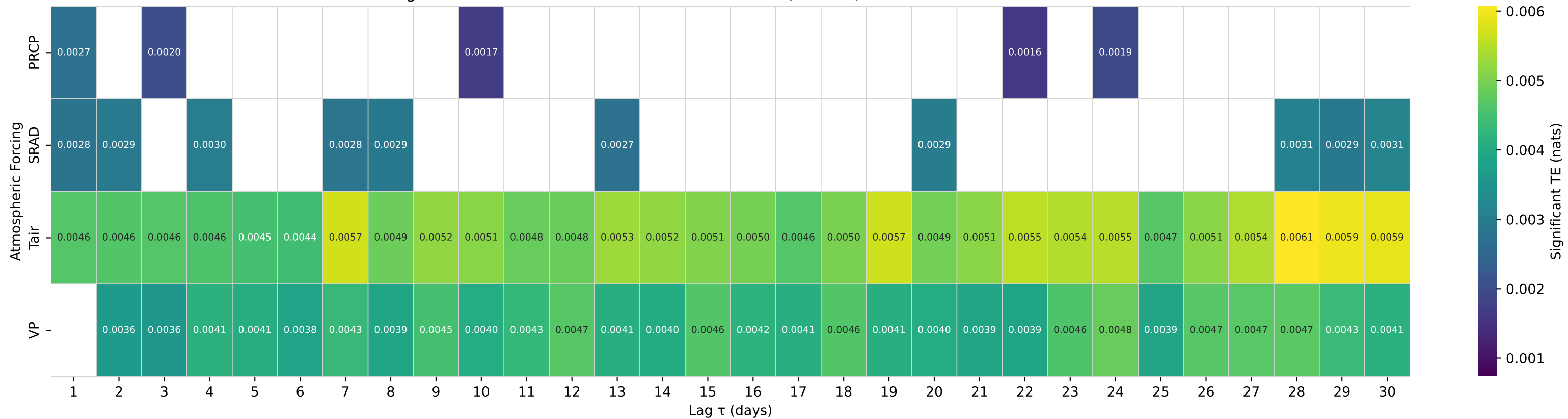
Shuffle-Test Significant TE to Streamflow — Basin 04216418 (HUC 04) — TONAWANDA CREEK AT ATTICA NY
