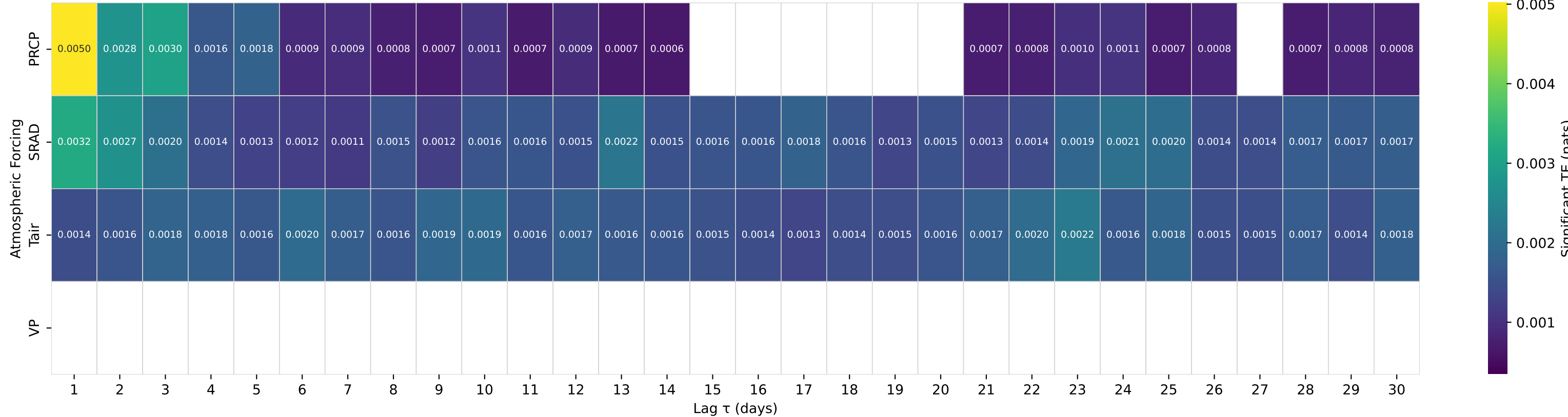
Shuffle-Test Significant TE to Streamflow — Basin 11383500 (HUC 18) — DEER C NR VINA CA
