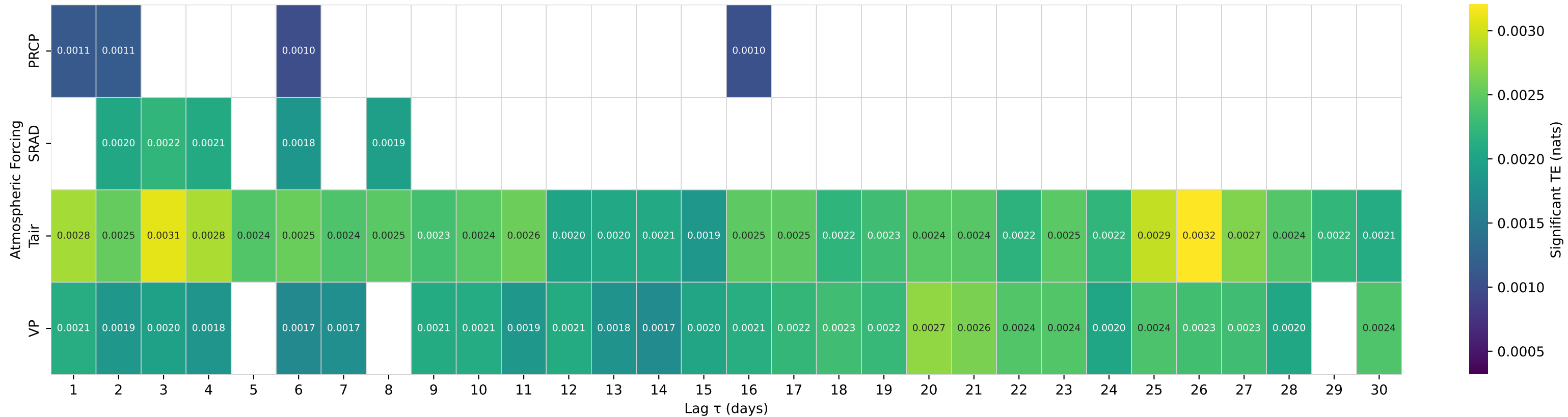
Shuffle-Test Significant TE to Streamflow — Basin 01170100 (HUC 01) — GREEN RIVER NEAR COLRAIN, MA
