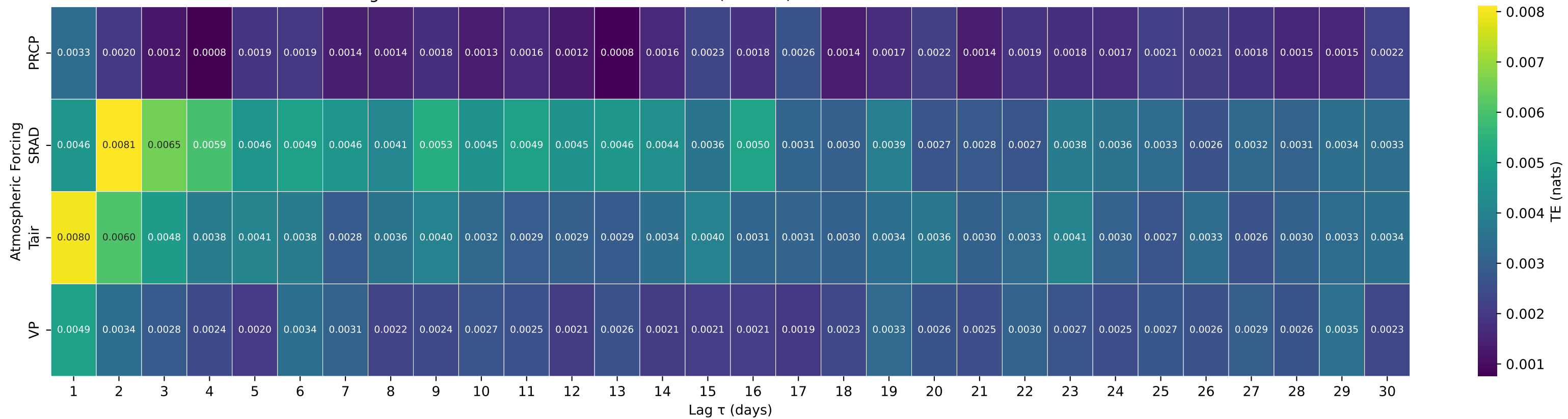
Shuffle-Test Significant TE to Streamflow — Basin 13338500 (HUC 17) — SF CLEARWATER RIVER AT STITES ID
