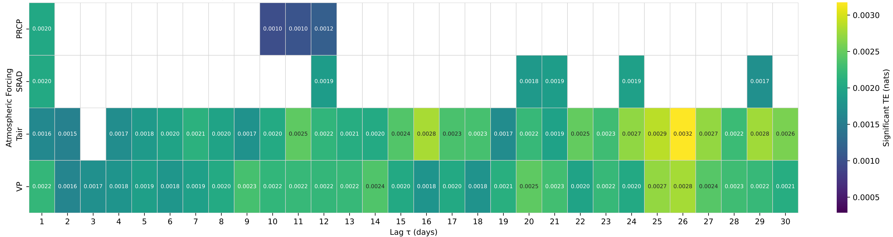
Shuffle-Test Significant TE to Streamflow — Basin 02013000 (HUC 02) — DUNLAP CREEK NEAR COVINGTON, VA
