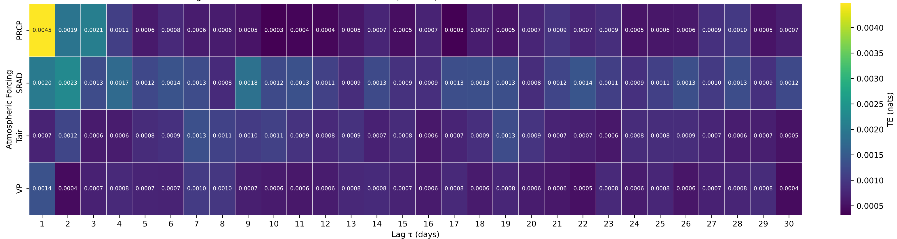
Shuffle-Test Significant TE to Streamflow — Basin 12178100 (HUC 17) — NEWHALEM CREEK NEAR NEWHALEM, WA
