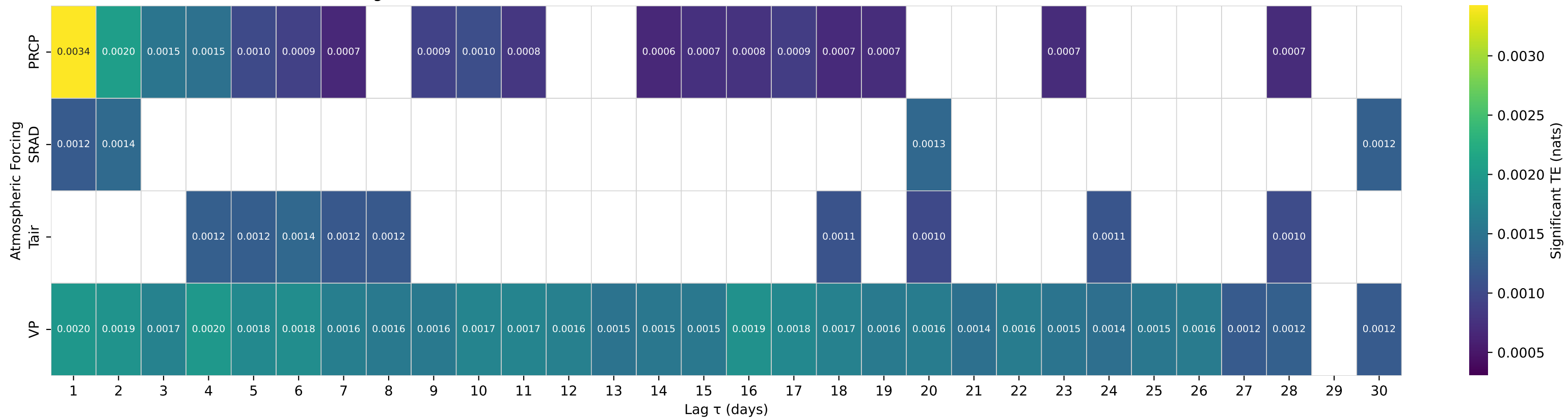
Shuffle-Test Significant TE to Streamflow — Basin 08380500 (HUC 13) — GALLINAS CREEK NEAR MONTEZUMA, NM
