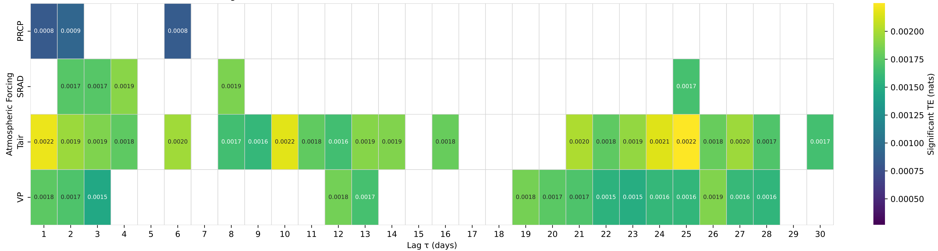
Shuffle-Test Significant TE to Streamflow — Basin 01169000 (HUC 01) — NORTH RIVER AT SHATTUCKVILLE, MA
