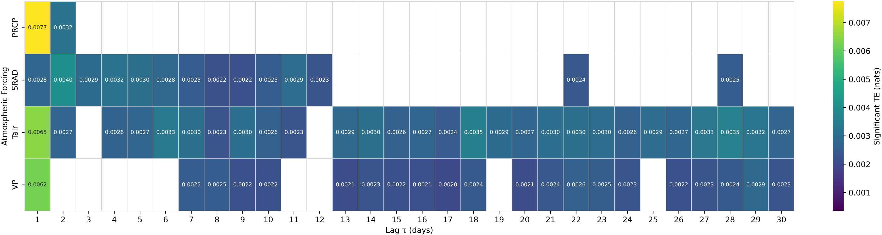
Shuffle-Test Significant TE to Streamflow — Basin 01134500 (HUC 01) — MOOSE RIVER AT VICTORY, VT
