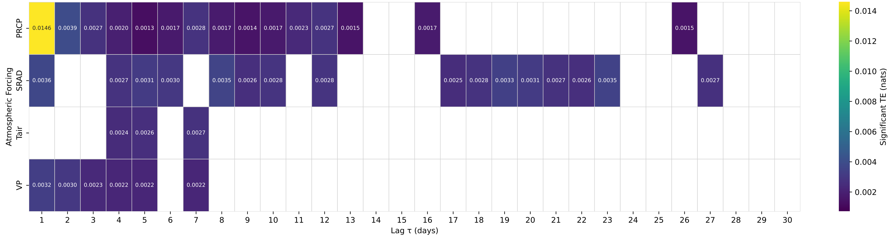
Shuffle-Test Significant TE to Streamflow — Basin 06447000 (HUC 10) — WHITE R NEAR KADOKA SD
