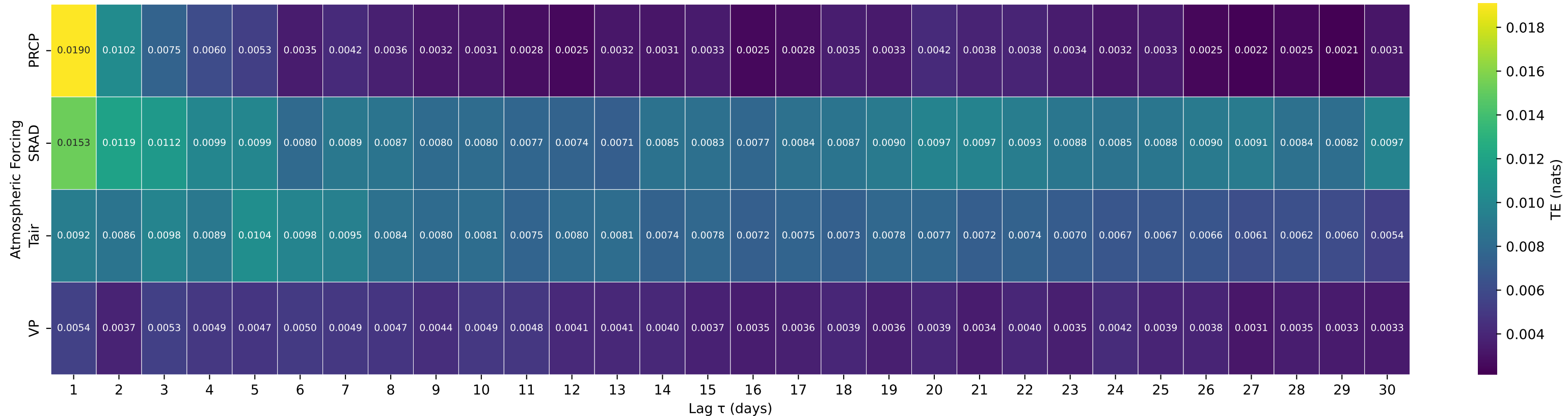
Shuffle-Test Significant TE to Streamflow — Basin 14316700 (HUC 17) — STEAMBOAT CREEK NEAR GLIDE, OR
