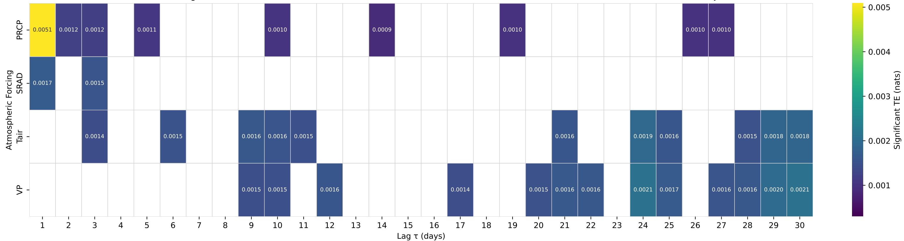
Shuffle-Test Significant TE to Streamflow — Basin 01466500 (HUC 02) — MCDONALDS BRANCH IN LEBANON STATE FOREST NJ
