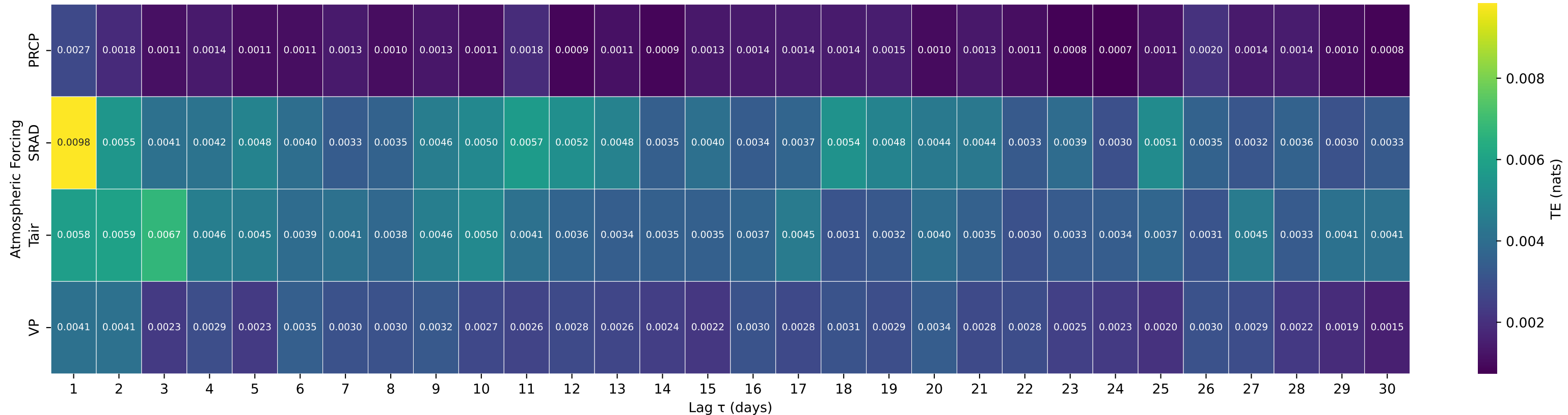
Shuffle-Test Significant TE to Streamflow — Basin 09107000 (HUC 14) — TAYLOR RIVER AT TAYLOR PARK, CO.
