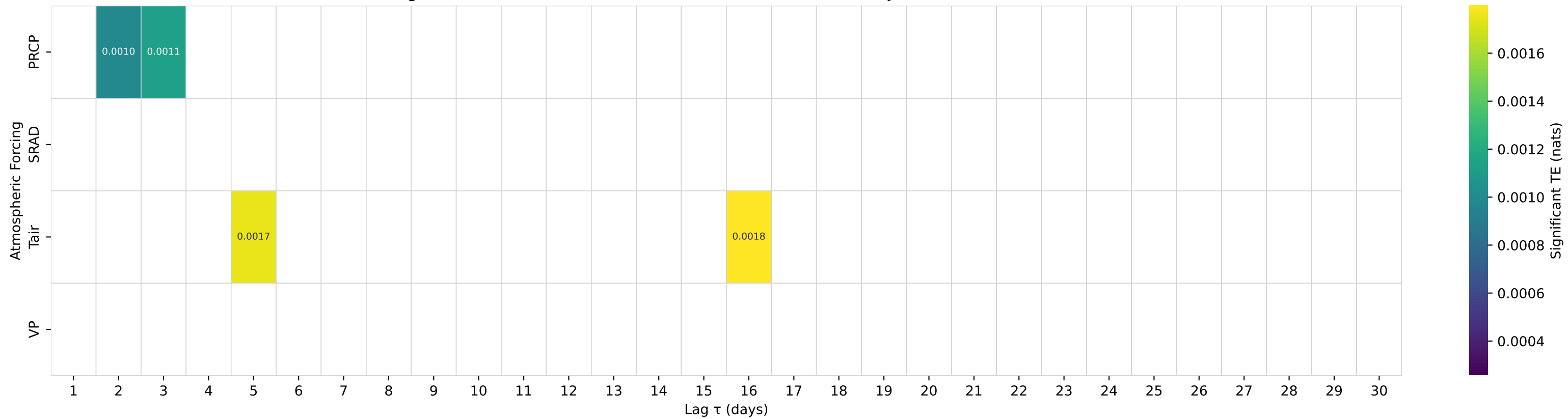
Shuffle-Test Significant TE to Streamflow — Basin 06468170 (HUC 10) — JAMES RIVER NR GRACE CITY, ND
