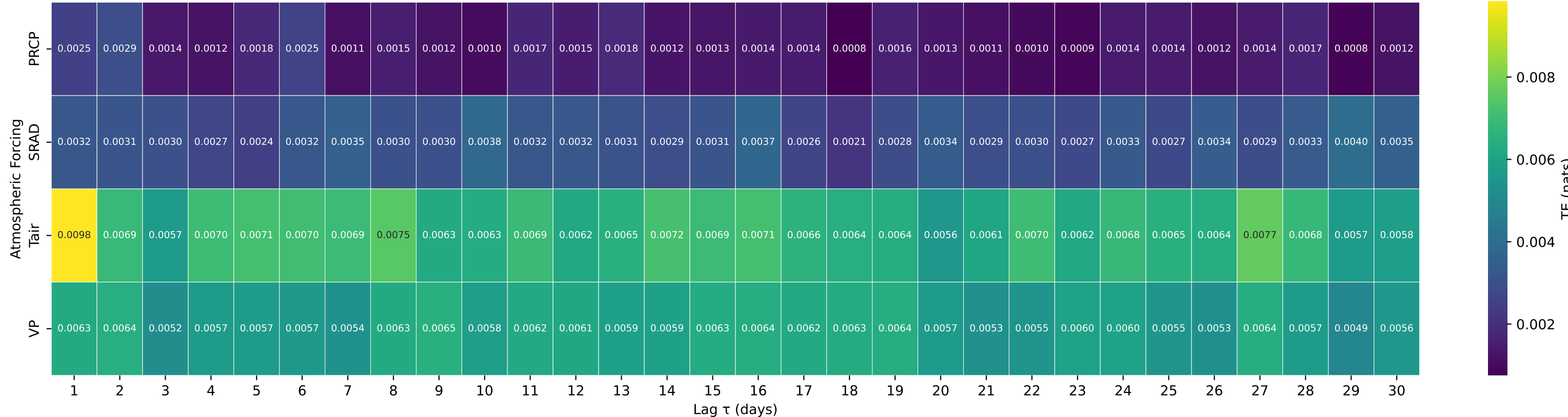
Shuffle-Test Significant TE to Streamflow — Basin 03021350 (HUC 05) — French Creek near Wattsburg, PA
