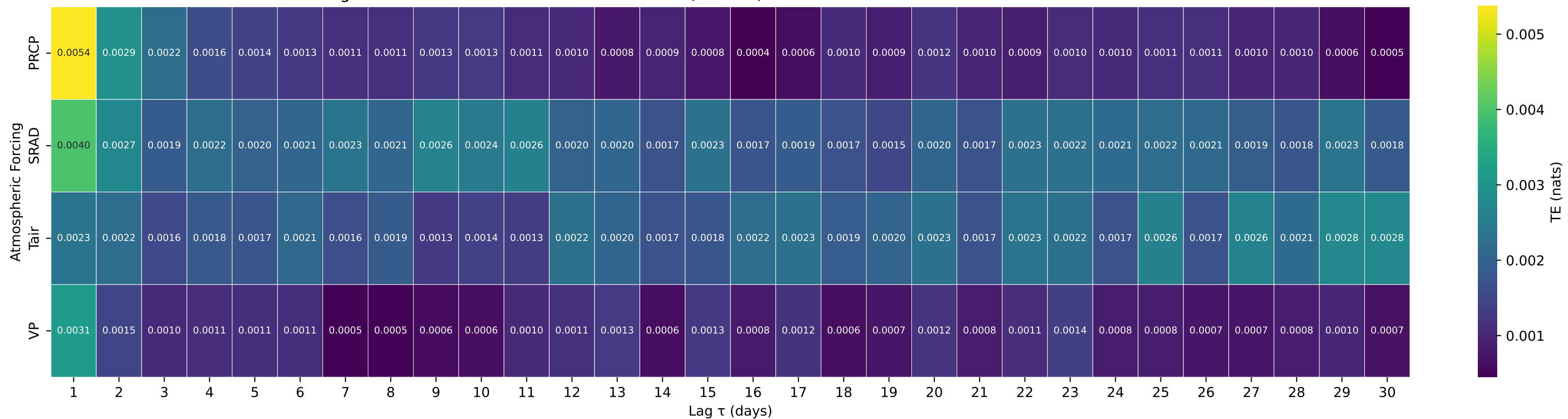
Shuffle-Test Significant TE to Streamflow — Basin 11523200 (HUC 18) — TRINITY R AB COFFEE C NR TRINITY CTR CA
