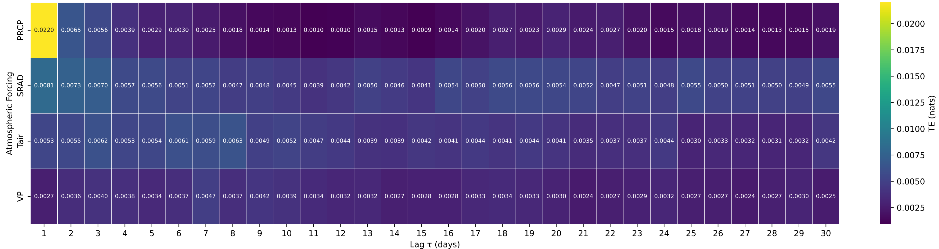
Shuffle-Test Significant TE to Streamflow — Basin 14139800 (HUC 17) — SOUTH FORK BULL RUN RIVER NEAR BULL RUN, OR
