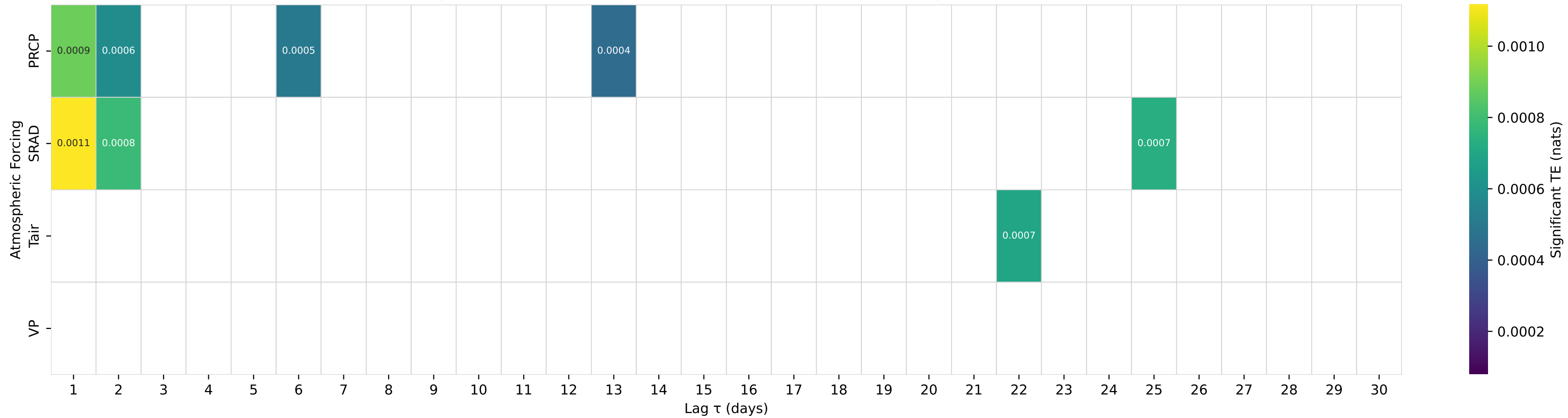
Shuffle-Test Significant TE to Streamflow — Basin 08029500 (HUC 12) — Big Cow Ck nr Newton, TX
