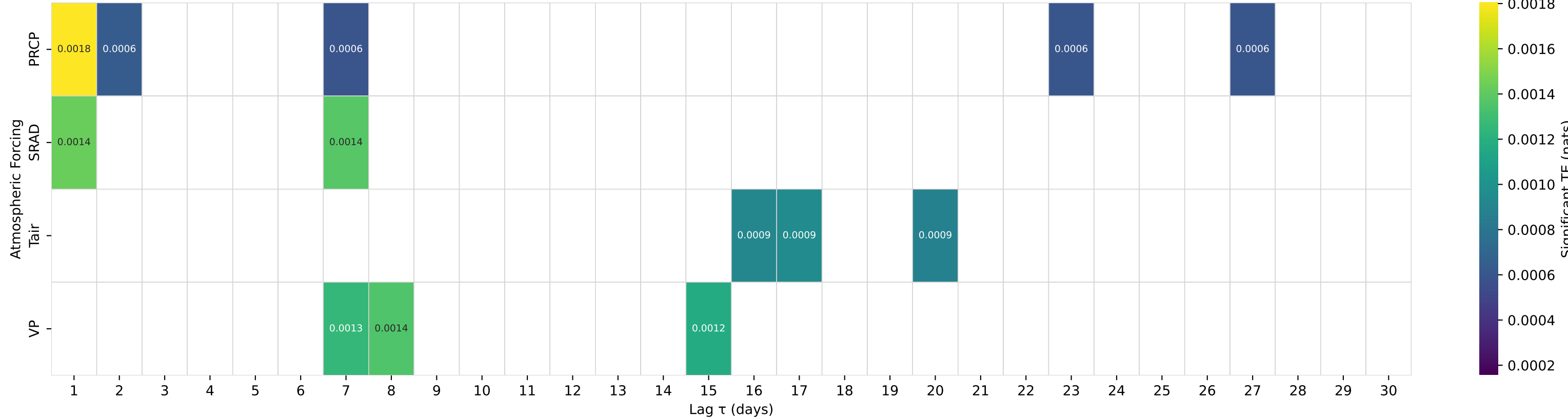
Shuffle-Test Significant TE to Streamflow — Basin 0211180 (HUC 03) — ELK CREEK AT ELKVILLE, NC
