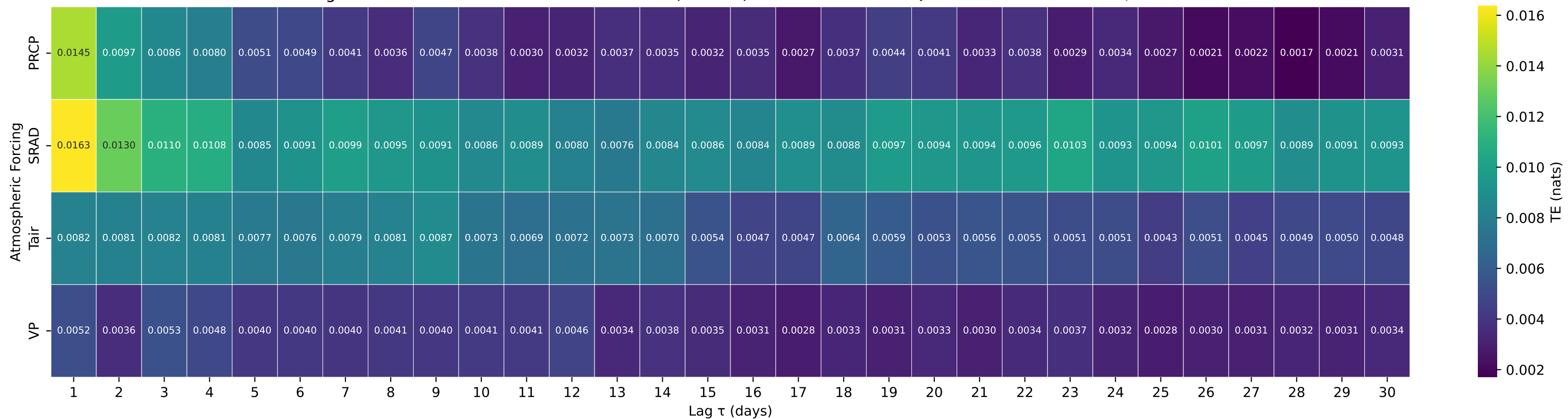
Shuffle-Test Significant TE to Streamflow — Basin 14325000 (HUC 17) — SOUTH FORK COQUILLE RIVER AT POWERS, OR
