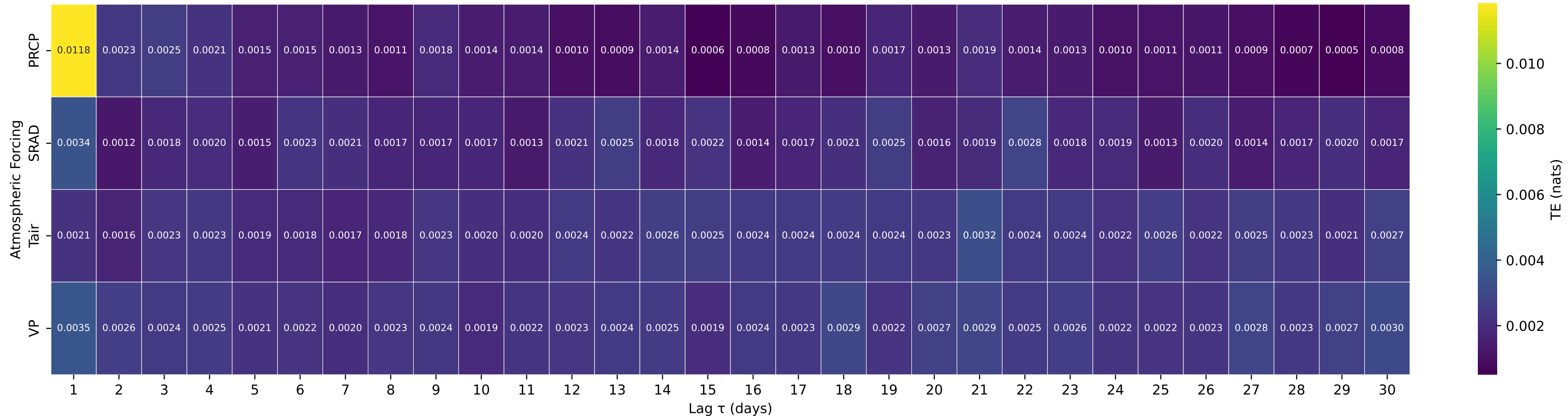
Shuffle-Test Significant TE to Streamflow — Basin 06919500 (HUC 10) — Cedar Creek near Pleasant View, MO
