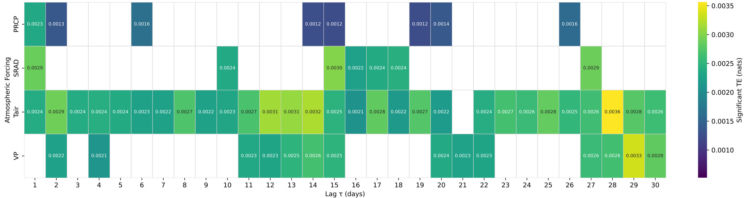
Shuffle-Test Significant TE to Streamflow — Basin 02193340 (HUC 03) — KETTLE CREEK NEAR WASHINGTON, GA
