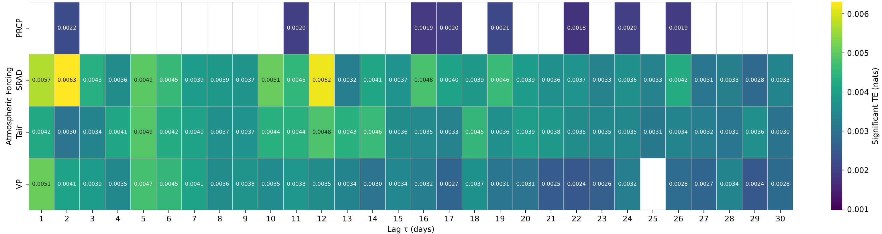
Shuffle-Test Significant TE to Streamflow — Basin 06746095 (HUC 10) — JOE WRIGHT CREEK ABOVE JOE WRIGHT RESERVOIR, CO.
