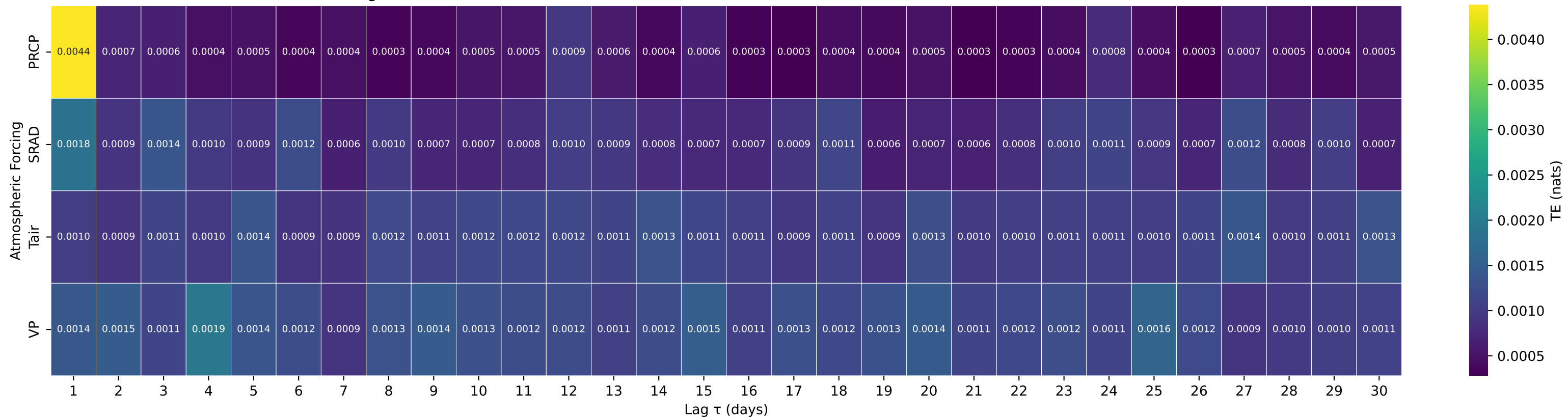
Shuffle-Test Significant TE to Streamflow — Basin 02046000 (HUC 03) — STONY CREEK NEAR DINWIDDIE, VA
