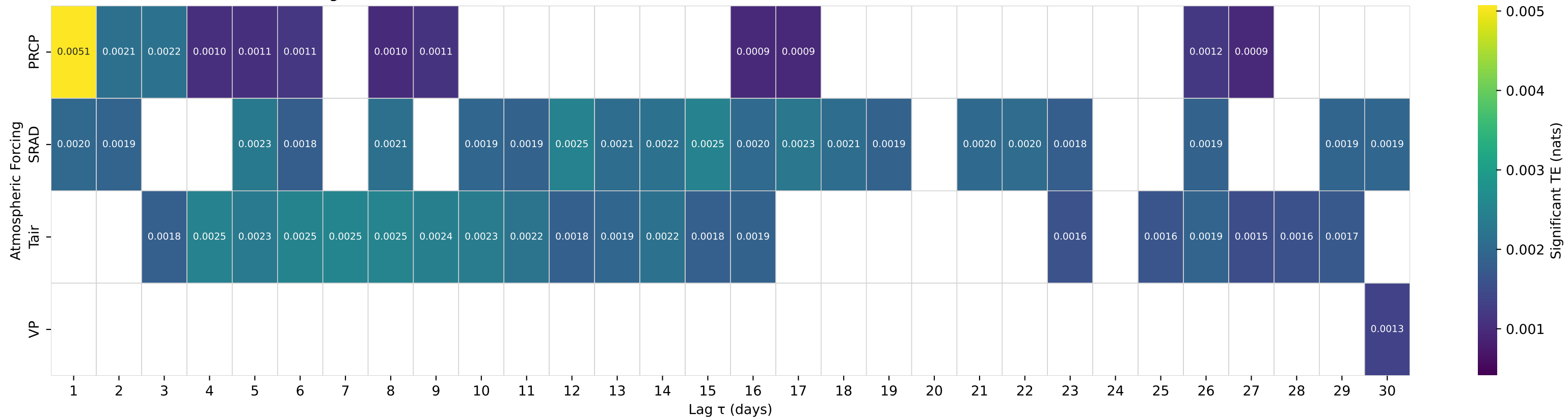
Shuffle-Test Significant TE to Streamflow — Basin 14096850 (HUC 17) — BEAVER CREEK, BLW QUARTZ CR, NR SIMNASHO, OR.
