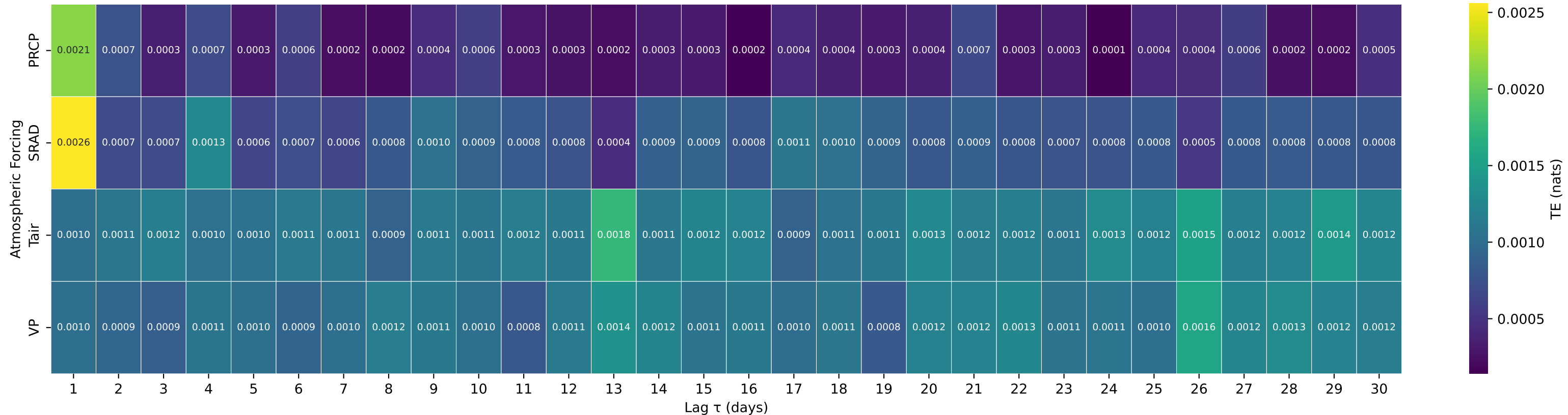
Shuffle-Test Significant TE to Streamflow — Basin 02349900 (HUC 03) — TURKEY CREEK AT BYROMVILLE, GA
