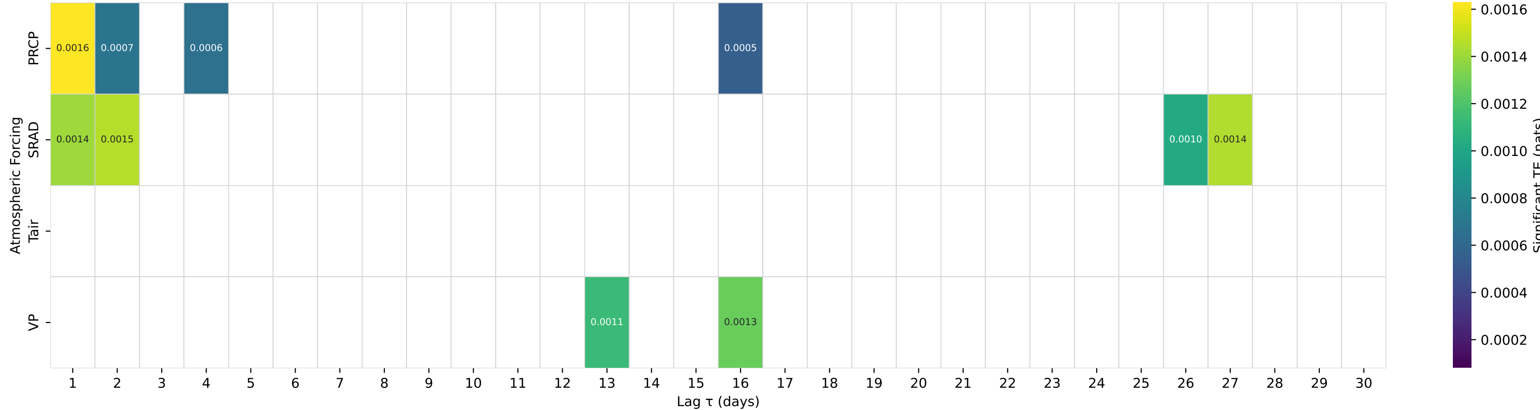
Shuffle-Test Significant TE to Streamflow — Basin 08066200 (HUC 12) — Long King Ck at Livingston, TX
