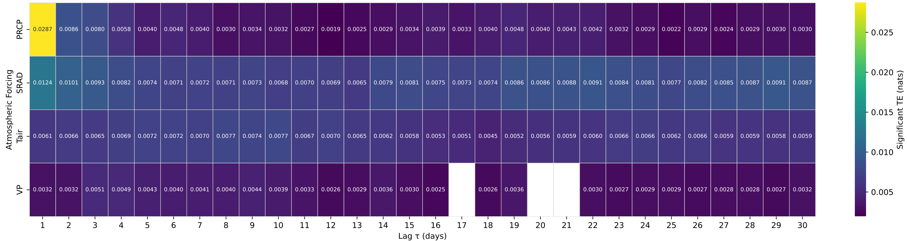
Shuffle-Test Significant TE to Streamflow — Basin 14166500 (HUC 17) — LONG TOM RIVER NEAR NOTI, OREG.
