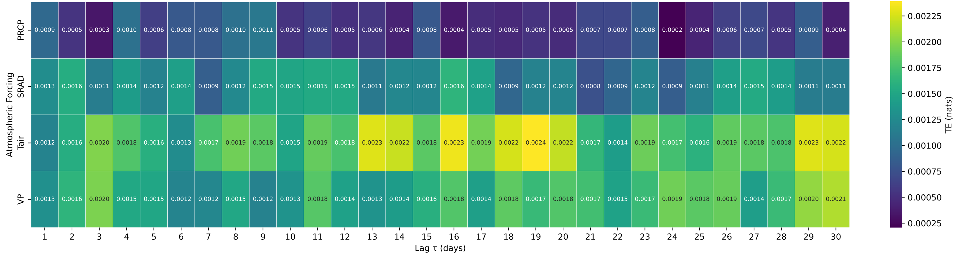
Shuffle-Test Significant TE to Streamflow — Basin 01516500 (HUC 02) — Corey Creek near Mainesburg, PA
