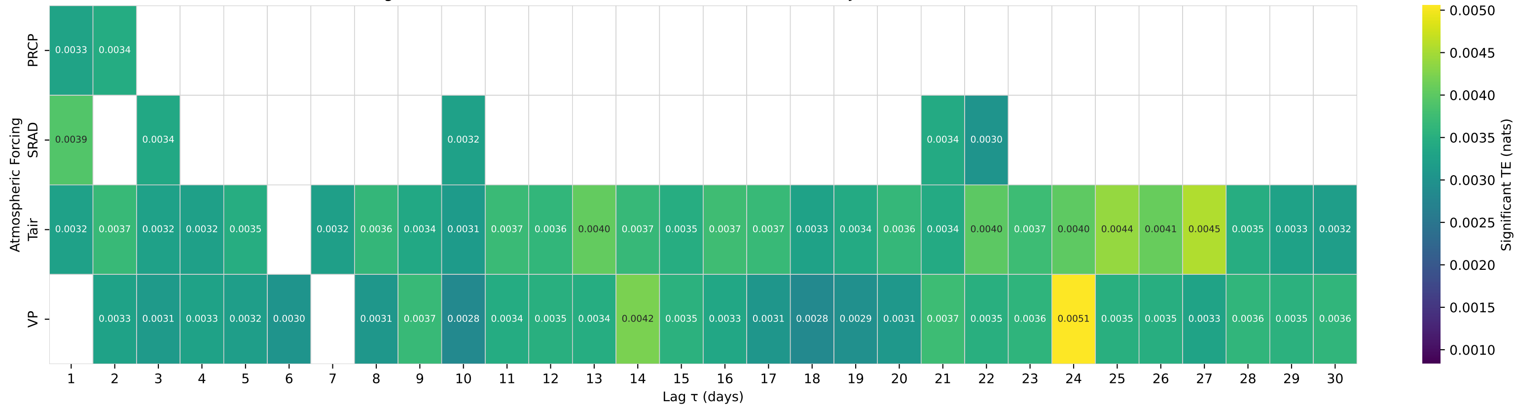
Shuffle-Test Significant TE to Streamflow — Basin 01451800 (HUC 02) — Jordan Creek near Schnecksville, PA
