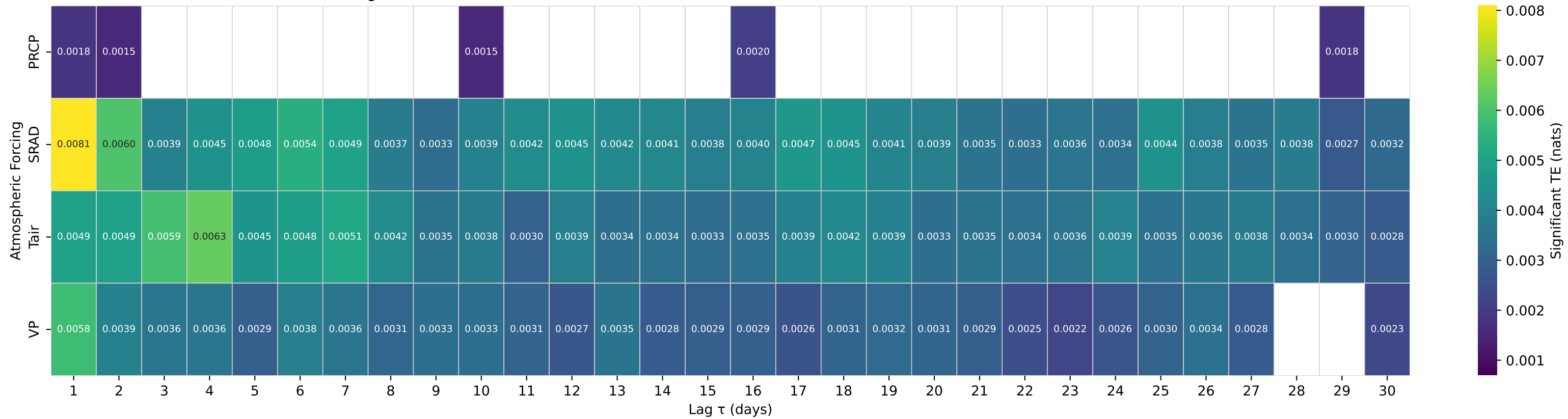
Shuffle-Test Significant TE to Streamflow — Basin 06622700 (HUC 10) — NORTH BRUSH CREEK NEAR SARATOGA, WY
