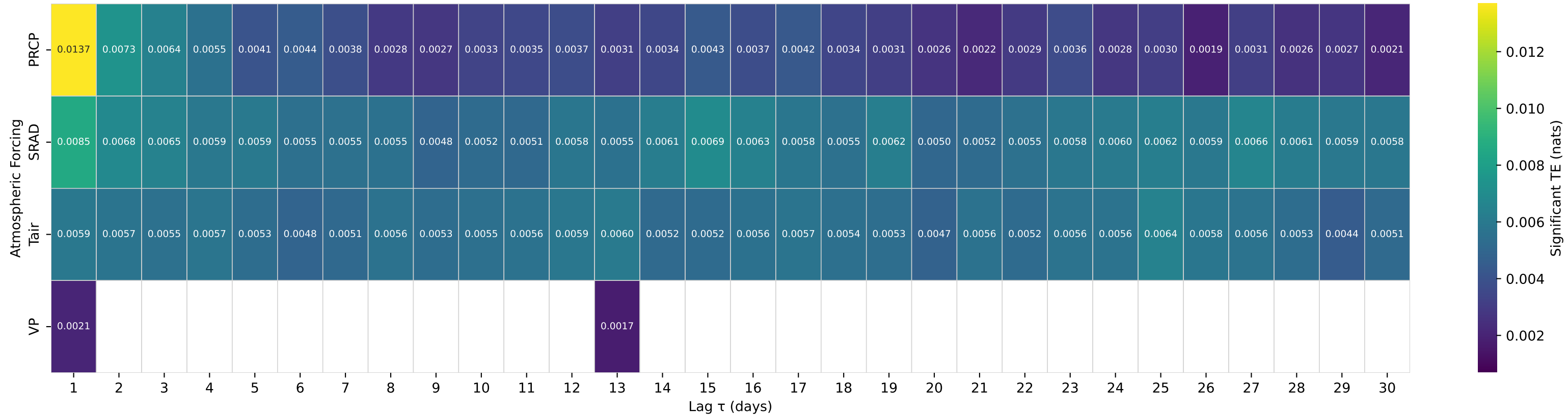
Shuffle-Test Significant TE to Streamflow — Basin 11480390 (HUC 18) — MAD R AB RUTH RES NR FOREST GLEN CA
