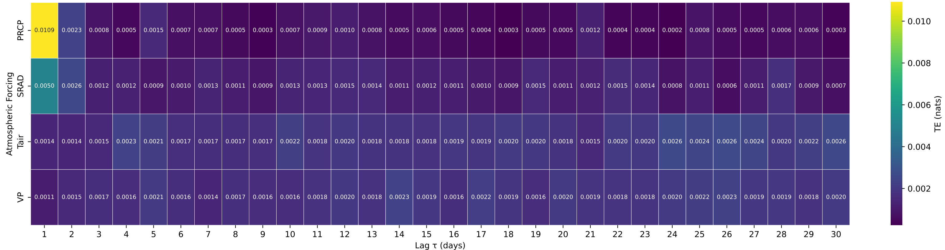
Shuffle-Test Significant TE to Streamflow — Basin 02215100 (HUC 03) — TUCSAWHATCHEE CREEK NEAR HAWKINSVILLE, GA
