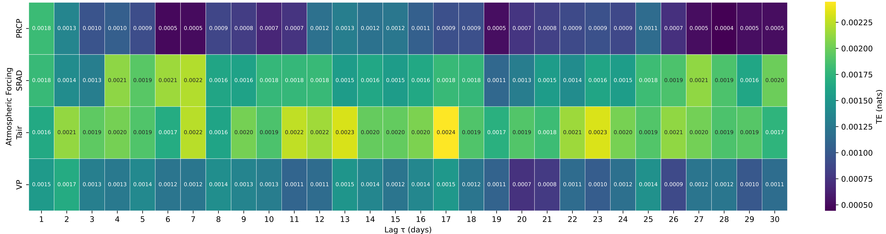
Shuffle-Test Significant TE to Streamflow — Basin 06350000 (HUC 10) — CANNONBALL RIVER AT REGENT, ND
