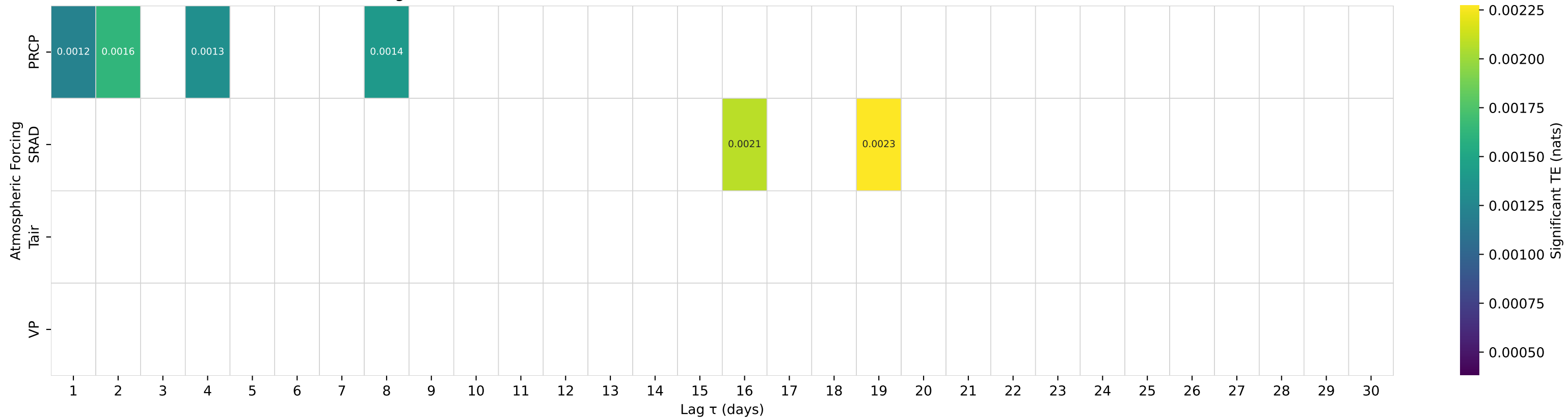
Shuffle-Test Significant TE to Streamflow — Basin 06479215 (HUC 10) — BIG SIOUX RIVER NR FLORENCE SD
