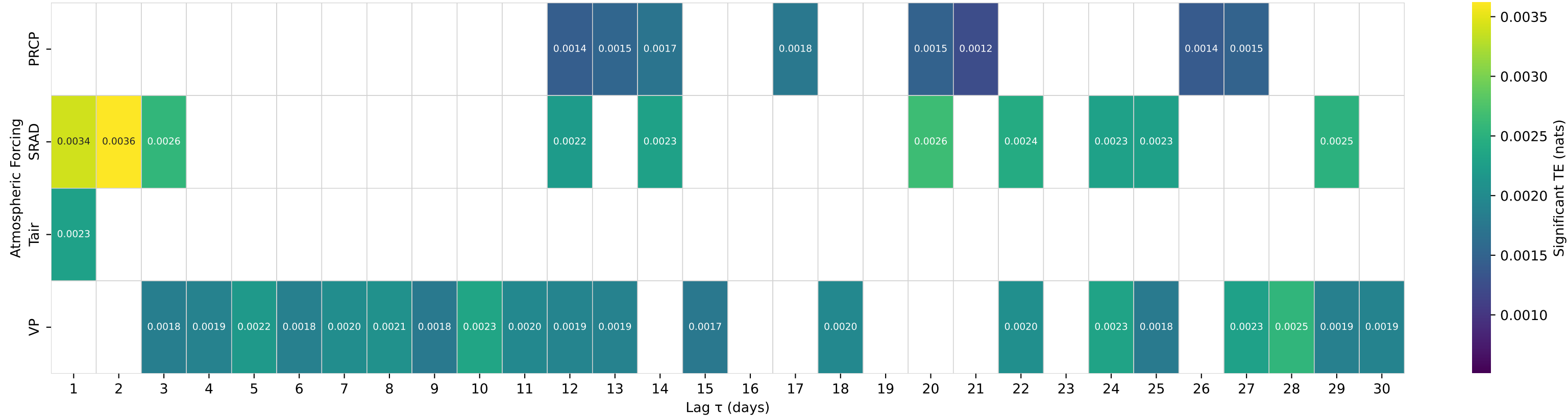
Shuffle-Test Significant TE to Streamflow — Basin 10023000 (HUC 16) — BIG CREEK NEAR RANDOLPH, UT
