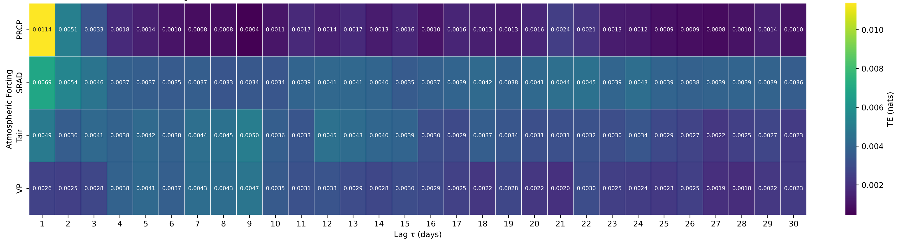
Shuffle-Test Significant TE to Streamflow — Basin 12147500 (HUC 17) — NORTH FORK TOLT RIVER NEAR CARNATION, WA
