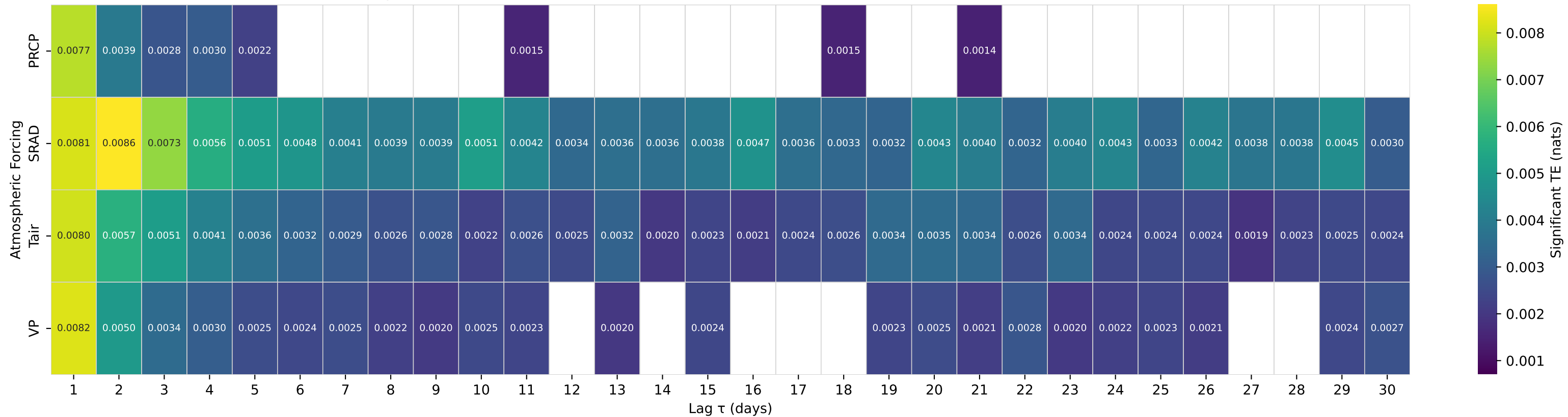
Shuffle-Test Significant TE to Streamflow — Basin 12175500 (HUC 17) — THUNDER CREEK NEAR NEWHALEM, WA
