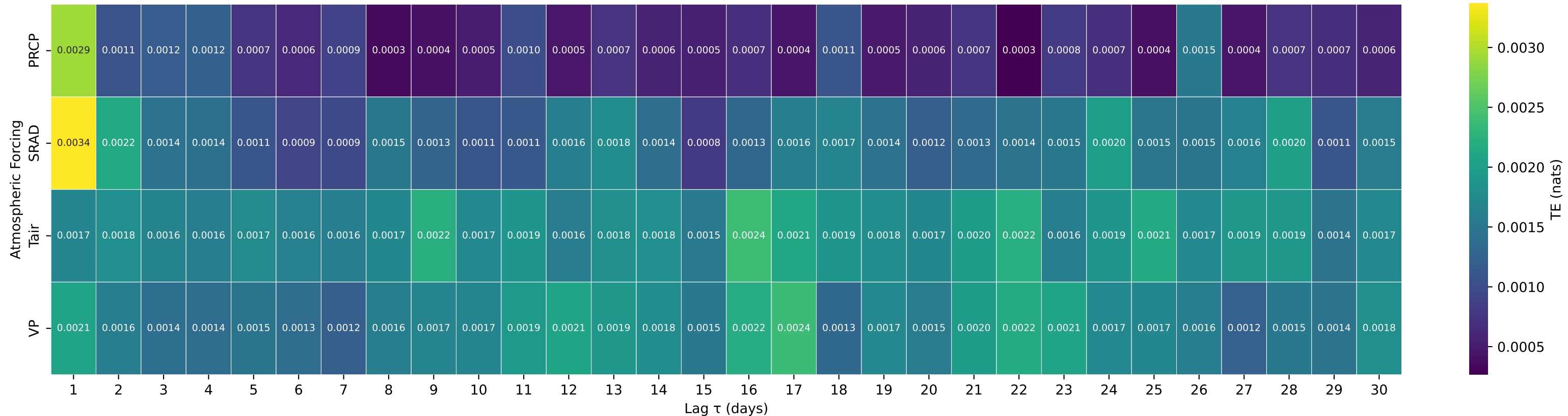
Shuffle-Test Significant TE to Streamflow — Basin 07263295 (HUC 11) — Maumelle River at Williams Junction, AR
