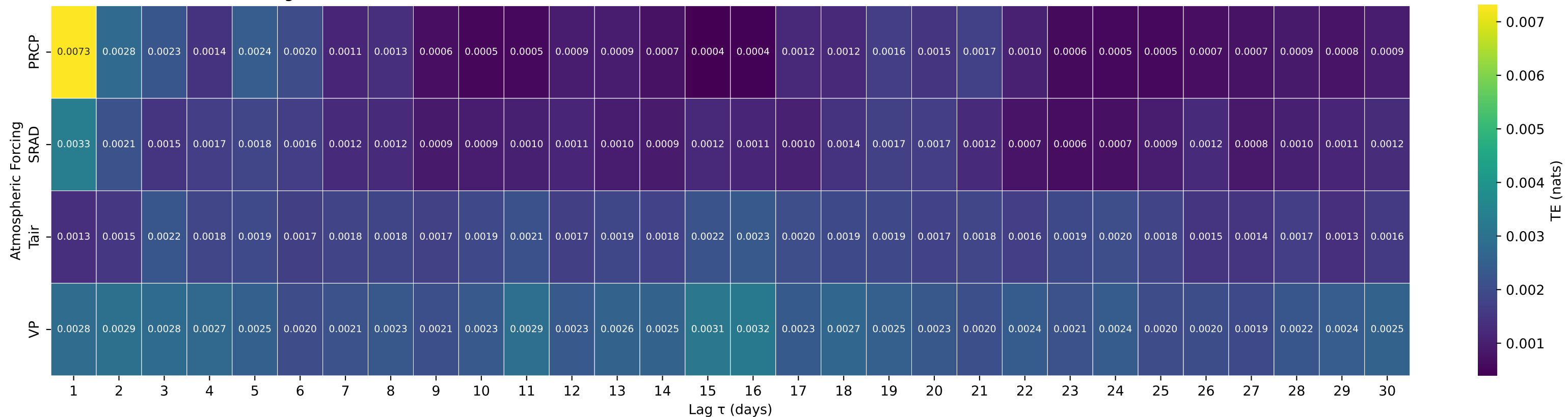
Shuffle-Test Significant TE to Streamflow — Basin 02231342 (HUC 03) — FT DRUM CREEK AT SUNSHINE ST PKY NEAR FT DRUM, FL
