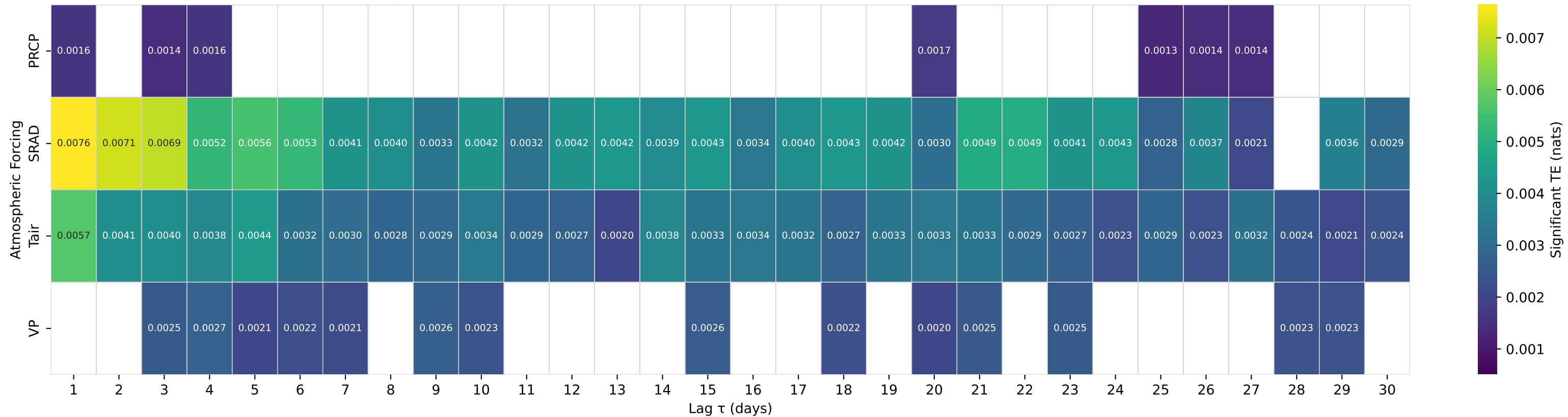
Shuffle-Test Significant TE to Streamflow — Basin 08271000 (HUC 13) — RIO LUCERO NEAR ARROYO SECO, NM
