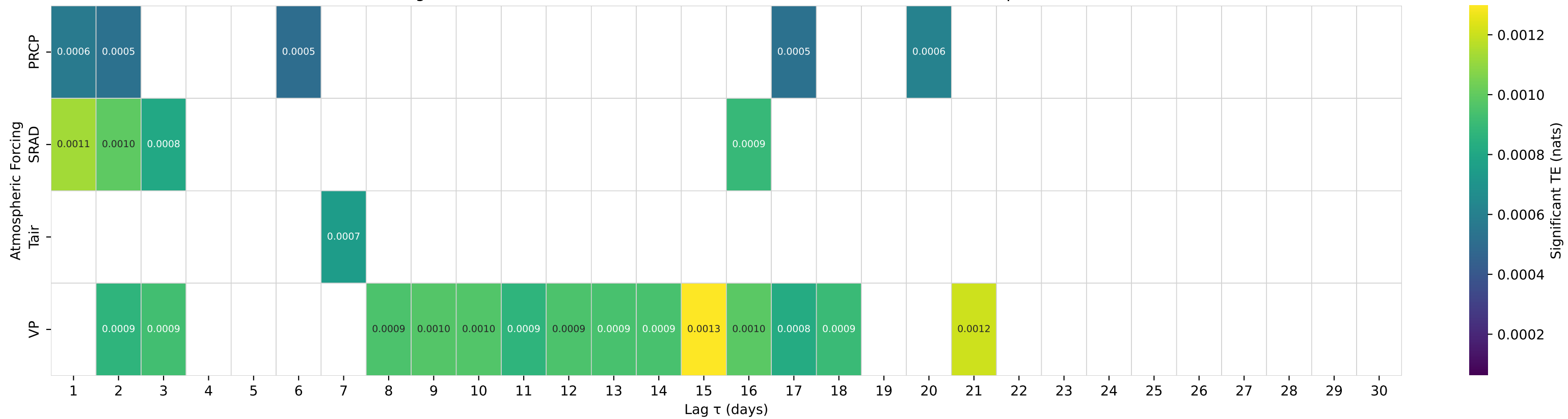
Shuffle-Test Significant TE to Streamflow — Basin 08165300 (HUC 12) — N Fk Guadalupe Rv nr Hunt, TX
