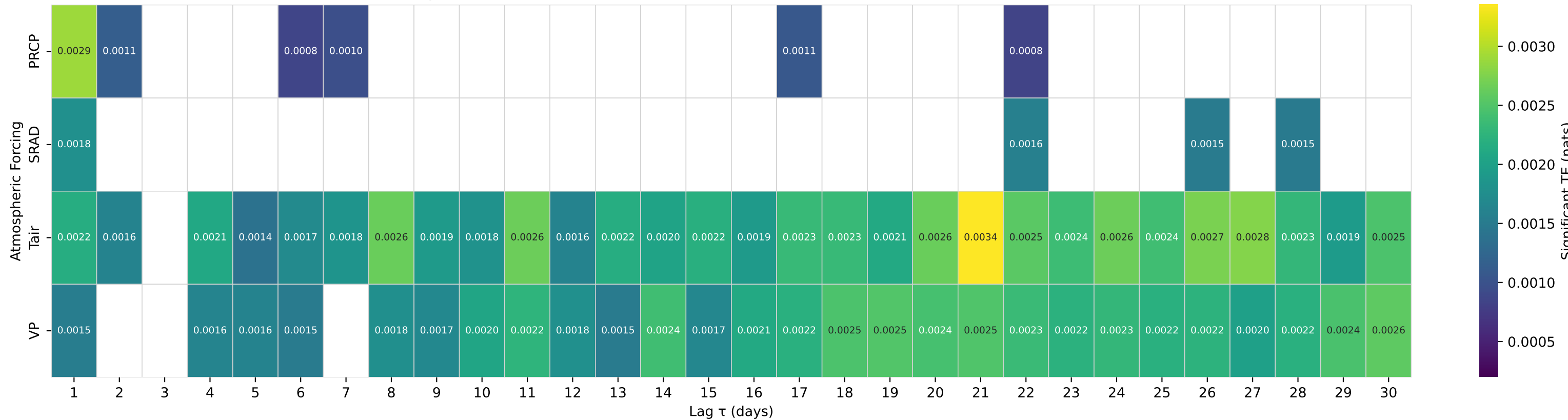
Shuffle-Test Significant TE to Streamflow — Basin 03159540 (HUC 05) — Shade River near Chester OH
