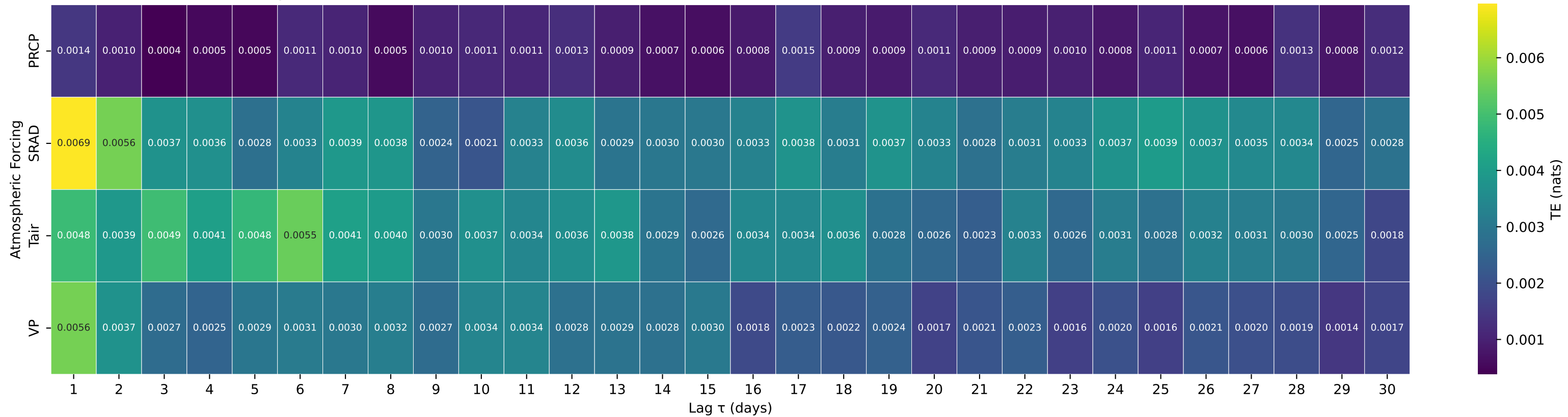
Shuffle-Test Significant TE to Streamflow — Basin 06632400 (HUC 10) — ROCK CREEK AB KING CANYON CANAL, NR ARLINGTON, WY
