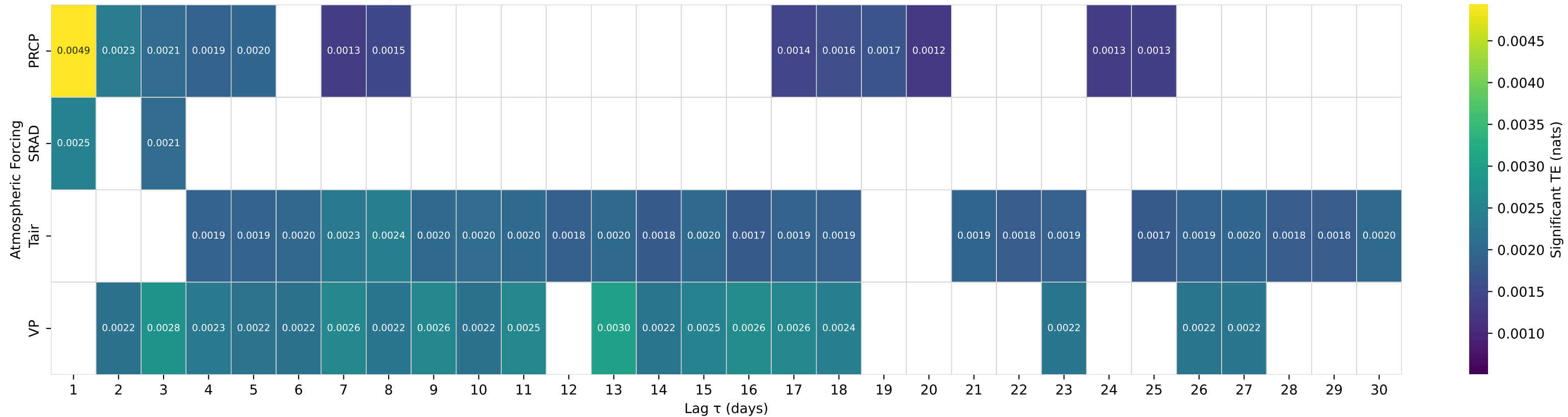
Shuffle-Test Significant TE to Streamflow — Basin 02297155 (HUC 03) — HORSE CREEK NEAR MYAKKA HEAD FL
