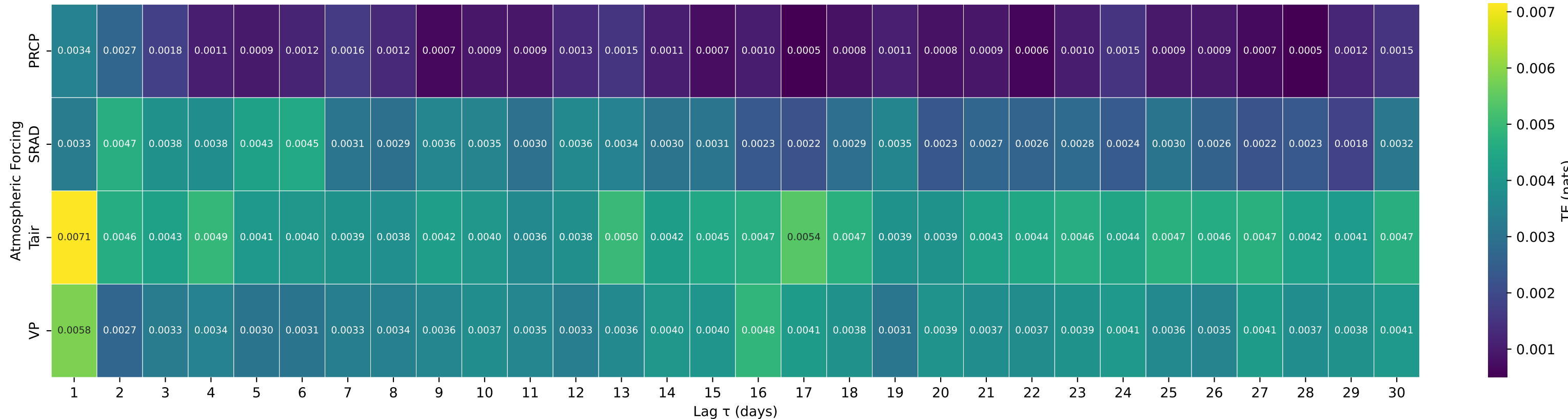
Shuffle-Test Significant TE to Streamflow — Basin 04296000 (HUC 01) — BLACK RIVER AT COVENTRY, VT
