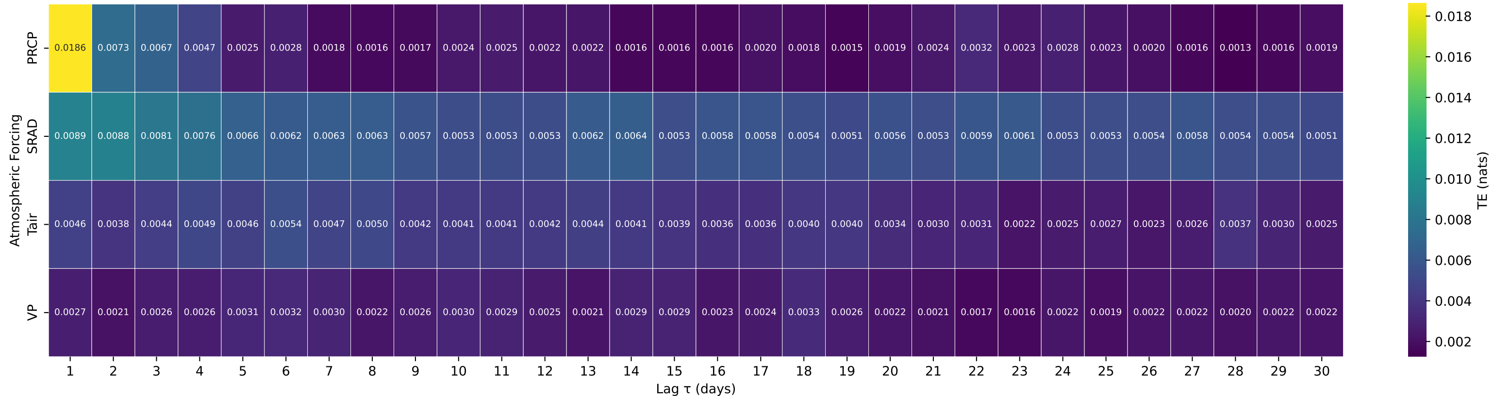
Shuffle-Test Significant TE to Streamflow — Basin 12054000 (HUC 17) — DUCKABUSH RIVER NEAR BRINNON, WA
