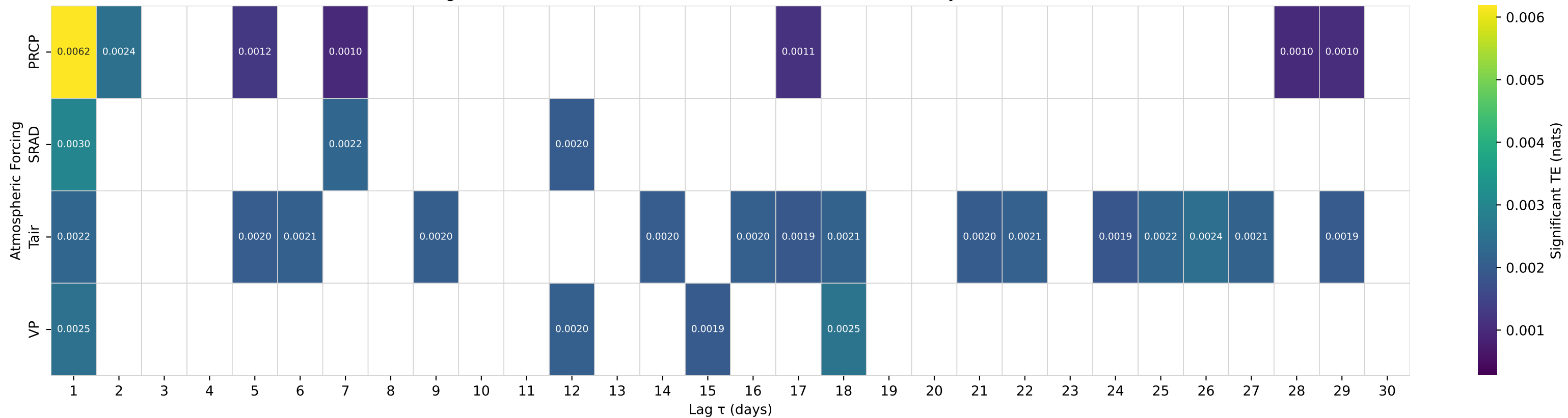
Shuffle-Test Significant TE to Streamflow — Basin 08025500 (HUC 12) — Bayou Toro near Toro, LA
