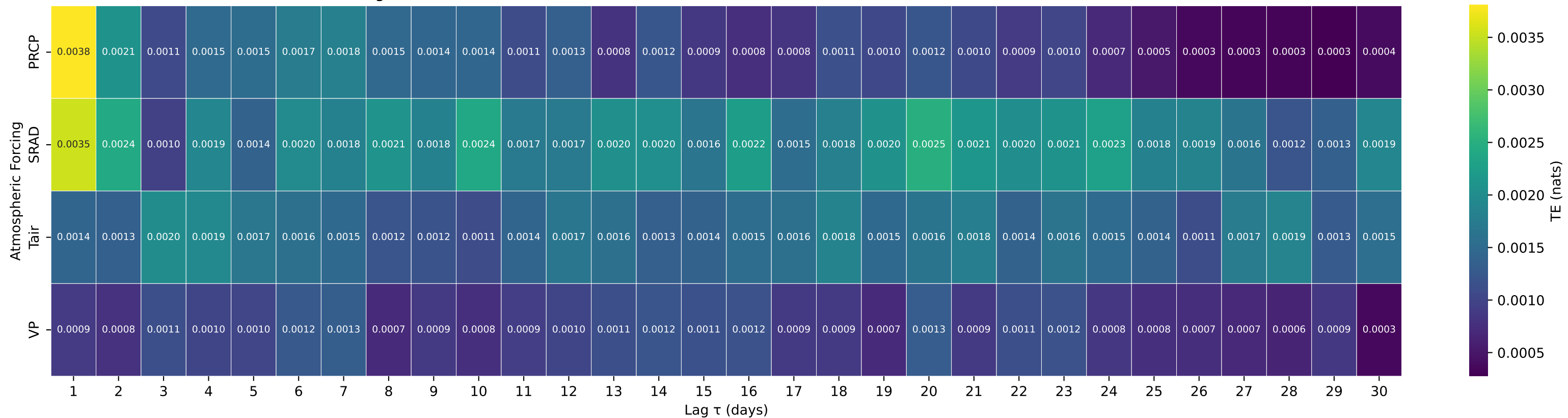
Shuffle-Test Significant TE to Streamflow — Basin 10259000 (HUC 18) — ANDREAS C NR PALM SPRINGS CA
