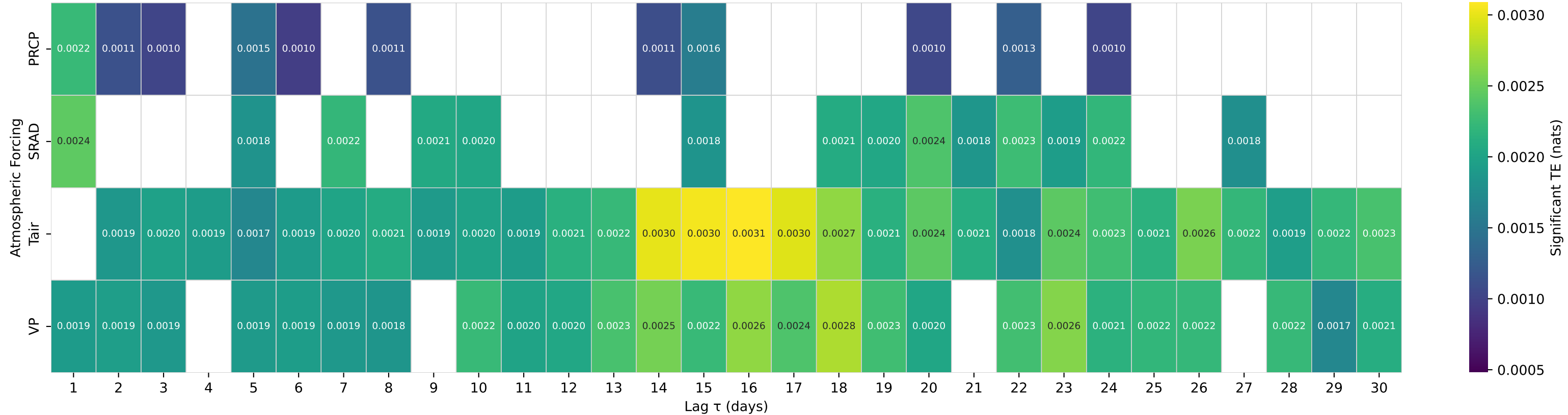
Shuffle-Test Significant TE to Streamflow — Basin 03384450 (HUC 05) — LUSK CREEK NEAR EDDYVILLE, IL
