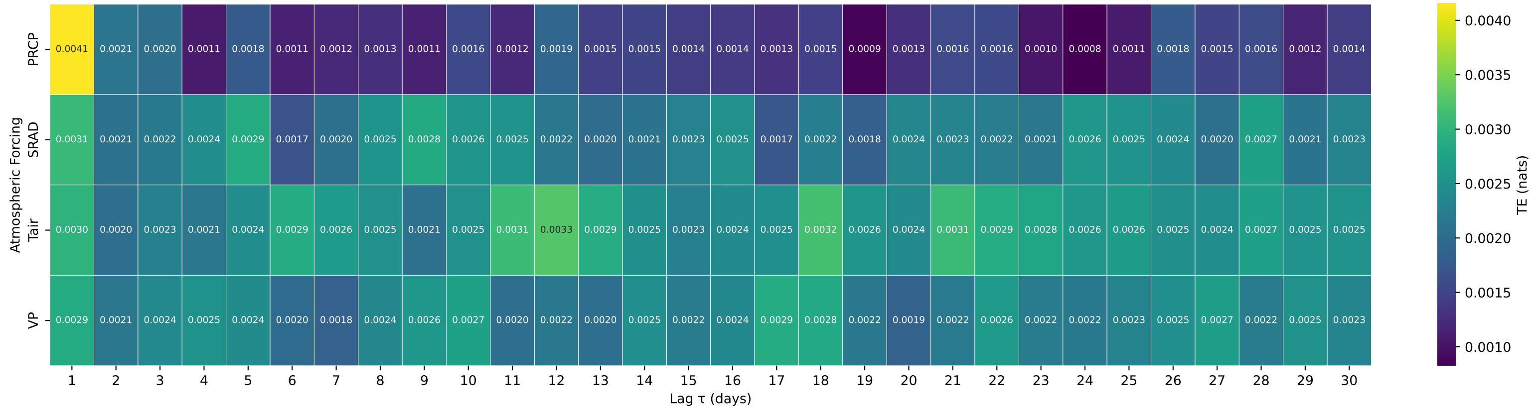
Shuffle-Test Significant TE to Streamflow — Basin 03241500 (HUC 05) — Massies Creek at Wilberforce OH
