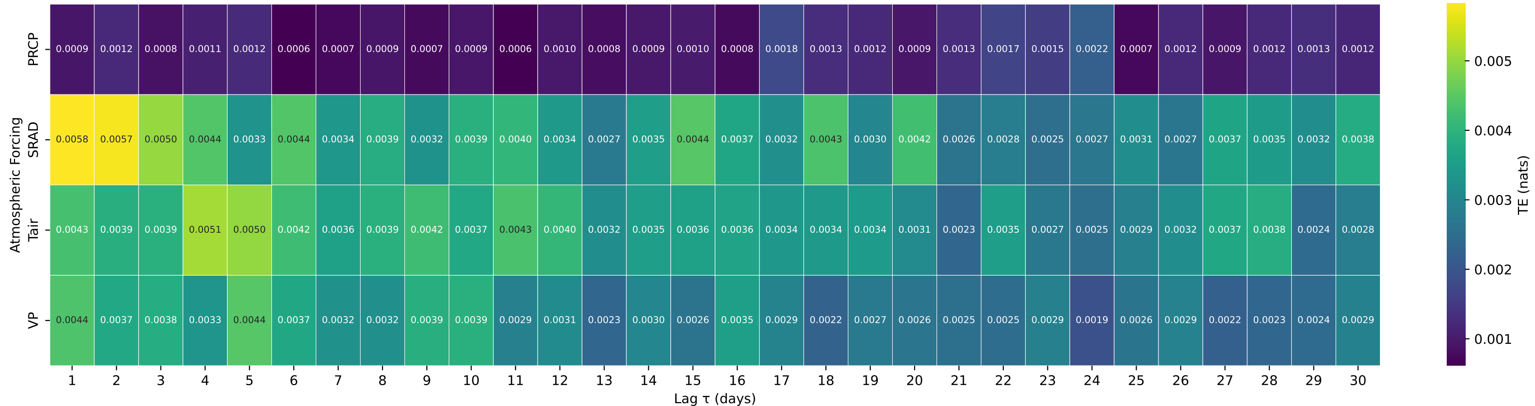
Shuffle-Test Significant TE to Streamflow — Basin 09035900 (HUC 14) — SOUTH FORK OF WILLIAMS FORK NEAR LEAL, CO.
