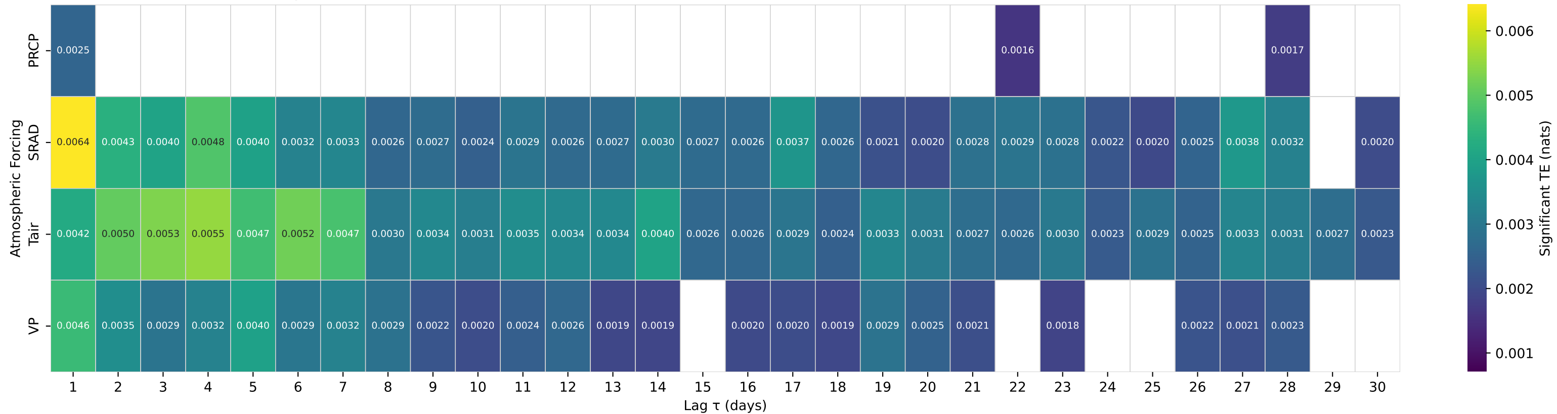
Shuffle-Test Significant TE to Streamflow — Basin 06623800 (HUC 10) — ENCAMPMENT RIVER AB HOG PARK CR, NR ENCAMPMENT, WY
