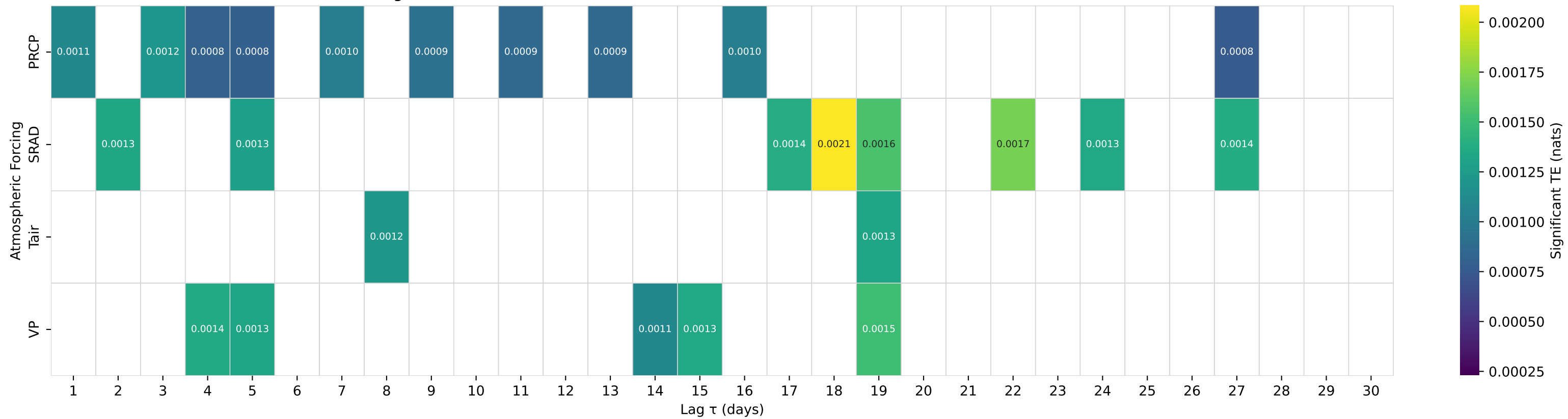
Shuffle-Test Significant TE to Streamflow — Basin 05414000 (HUC 07) — PLATTE RIVER NEAR ROCKVILLE, WI
