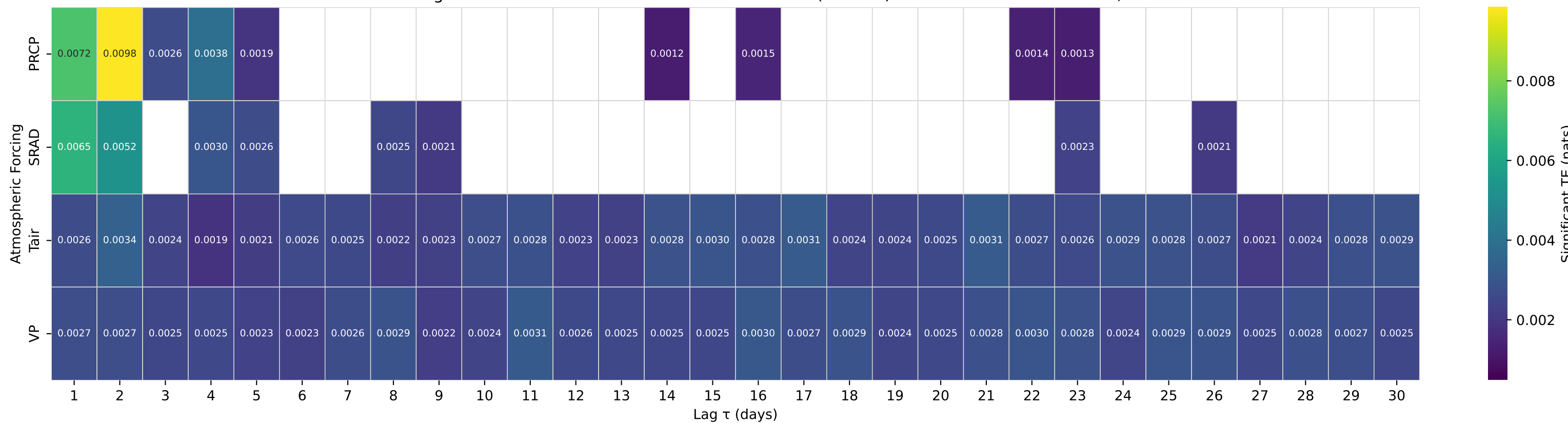
Shuffle-Test Significant TE to Streamflow — Basin 02472000 (HUC 03) — LEAF RIVER NR COLLINS, MS
