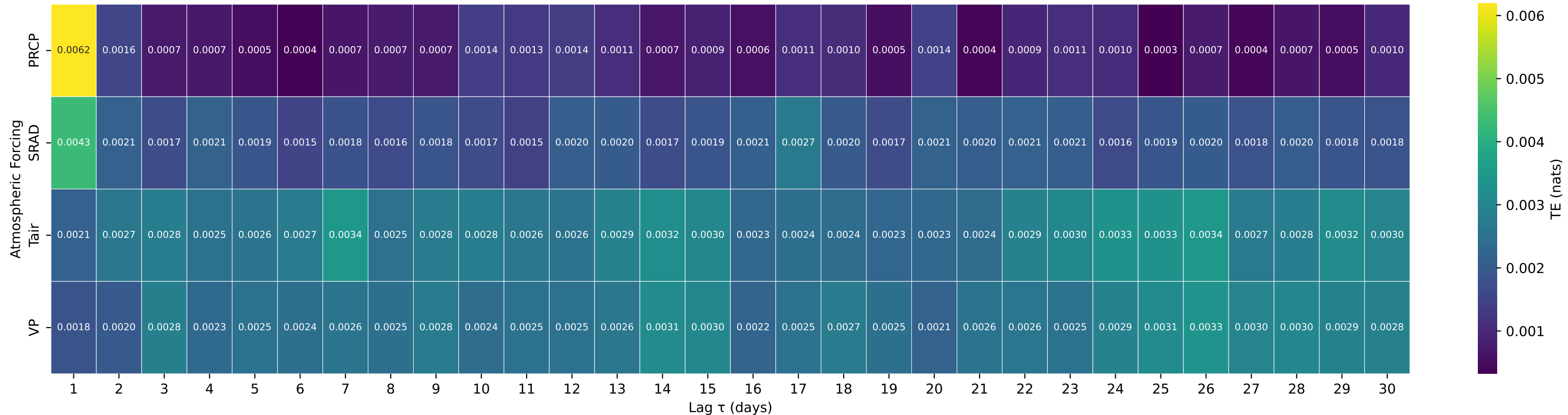
Shuffle-Test Significant TE to Streamflow — Basin 02081500 (HUC 03) — TAR RIVER NEAR TAR RIVER, NC
