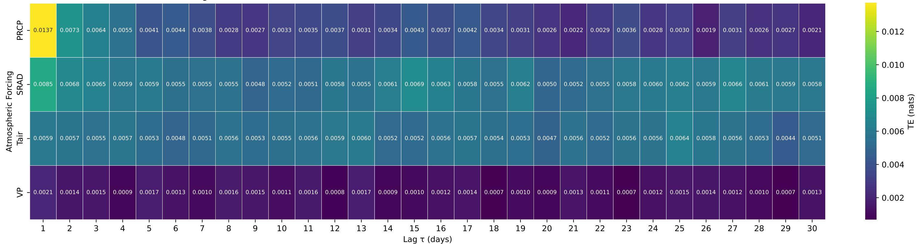
Shuffle-Test Significant TE to Streamflow — Basin 11480390 (HUC 18) — MAD R AB RUTH RES NR FOREST GLEN CA
