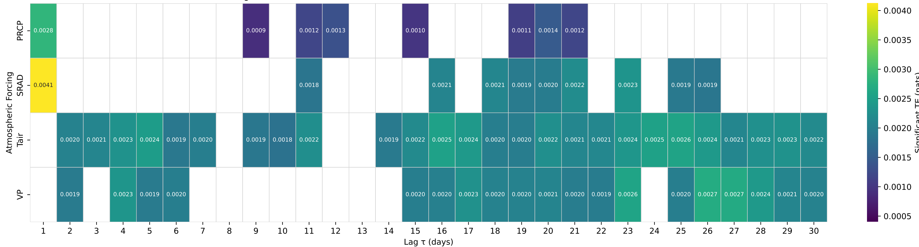
Shuffle-Test Significant TE to Streamflow — Basin 02125000 (HUC 03) — BIG BEAR CR NR RICHFIELD, NC
