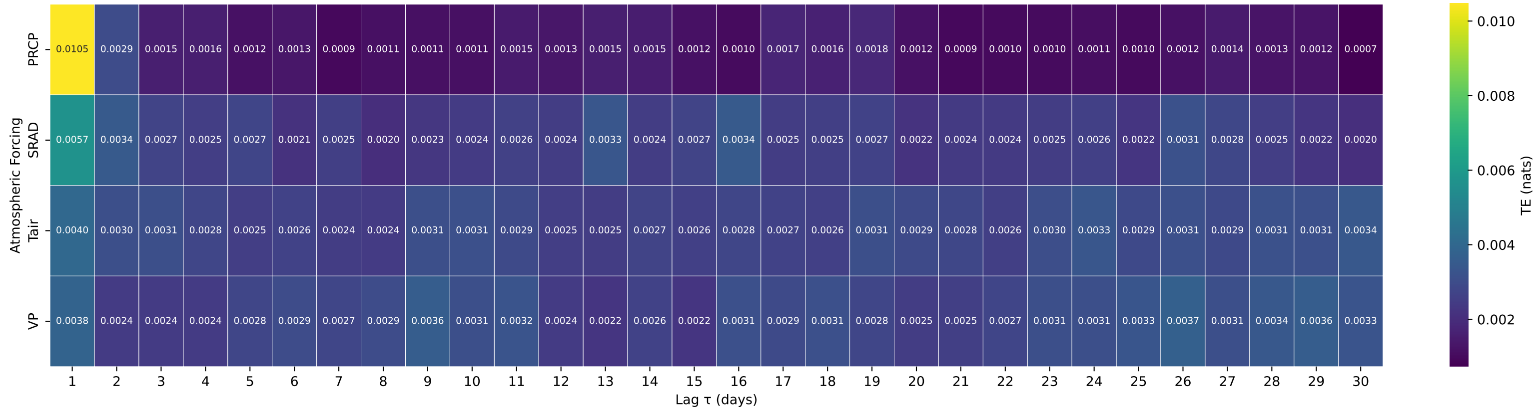
Shuffle-Test Significant TE to Streamflow — Basin 02481000 (HUC 03) — BILOXI RIVER AT WORTHAM, MS
