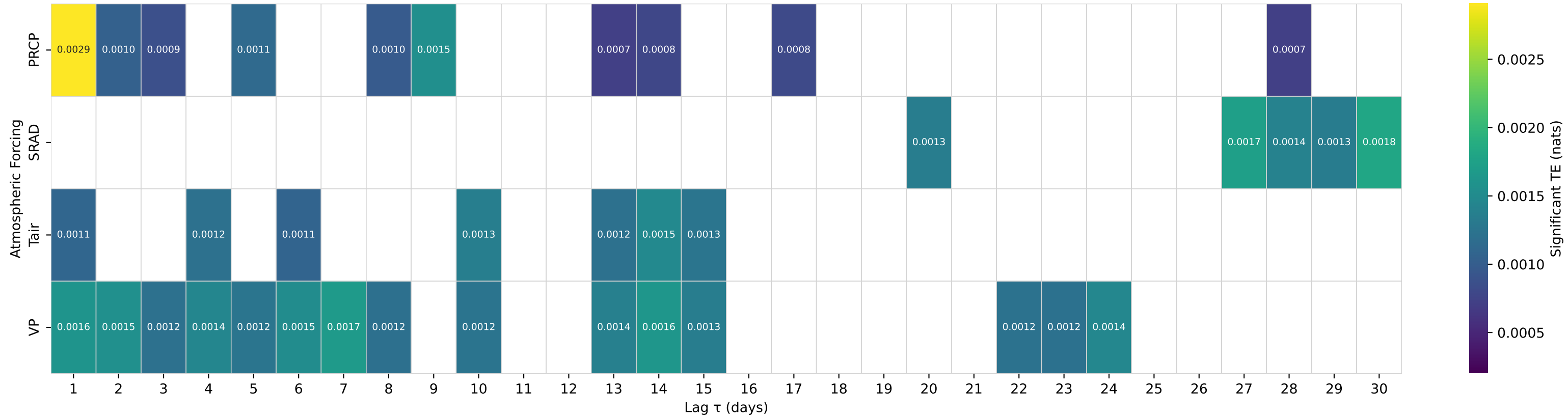
Shuffle-Test Significant TE to Streamflow — Basin 06889500 (HUC 10) — SOLDIER C NR TOPEKA, KS
