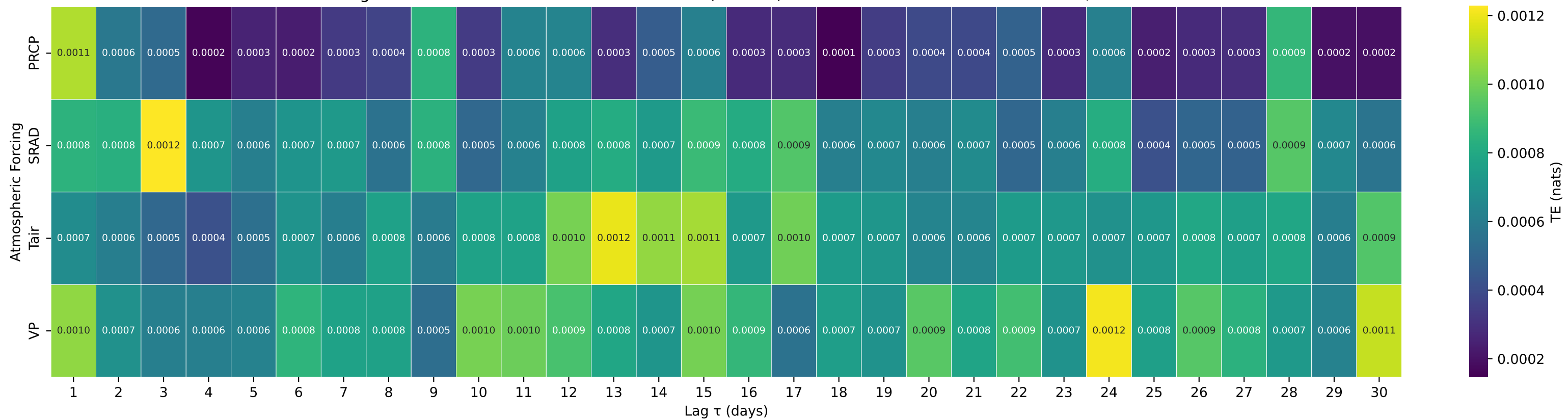
Shuffle-Test Significant TE to Streamflow — Basin 01620500 (HUC 02) — NORTH RIVER NEAR STOKESVILLE, VA
