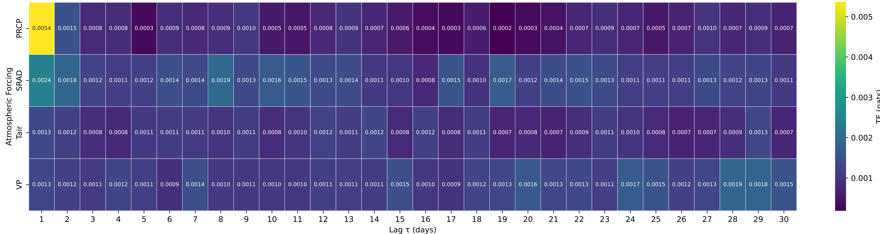
Shuffle-Test Significant TE to Streamflow — Basin 08164300 (HUC 12) — Navidad Rv nr Hallettsville, TX
