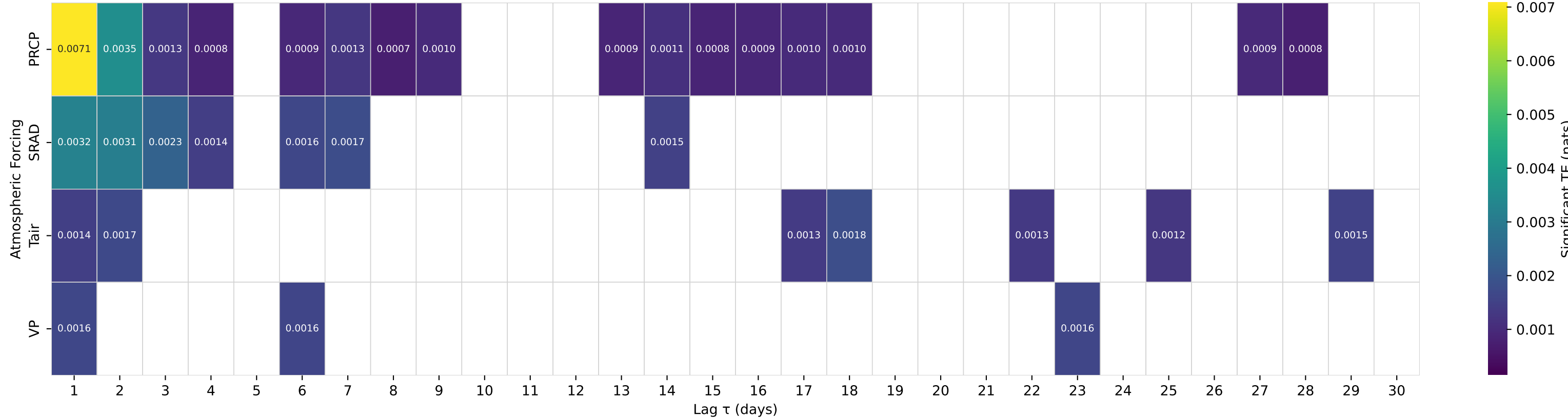
Shuffle-Test Significant TE to Streamflow — Basin 08109700 (HUC 12) — Middle Yegua Ck nr Dime Box, TX
