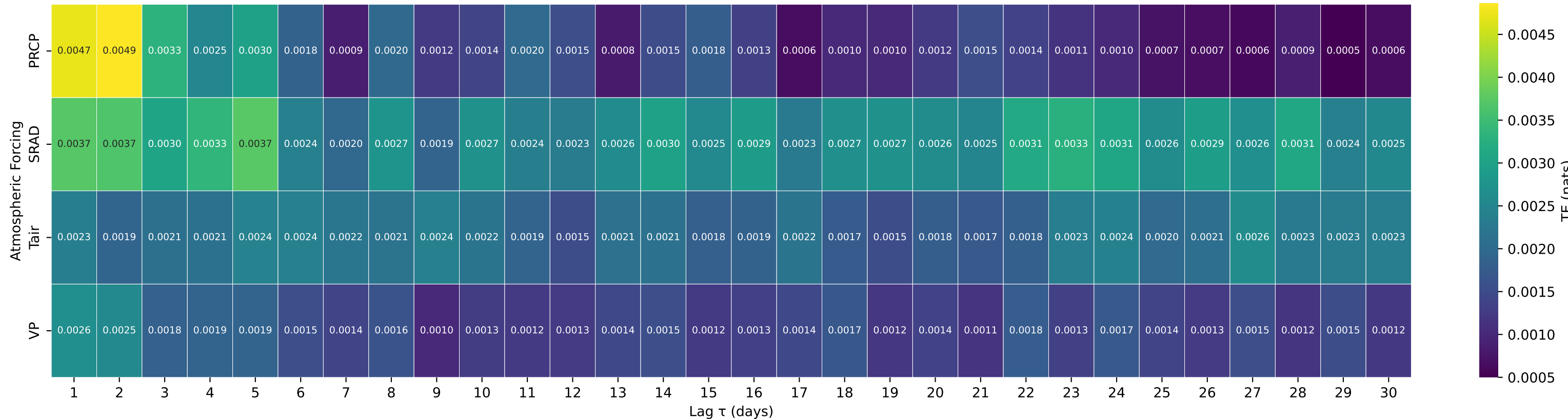
Shuffle-Test Significant TE to Streamflow — Basin 11180500 (HUC 18) — DRY C A UNION CITY CA
