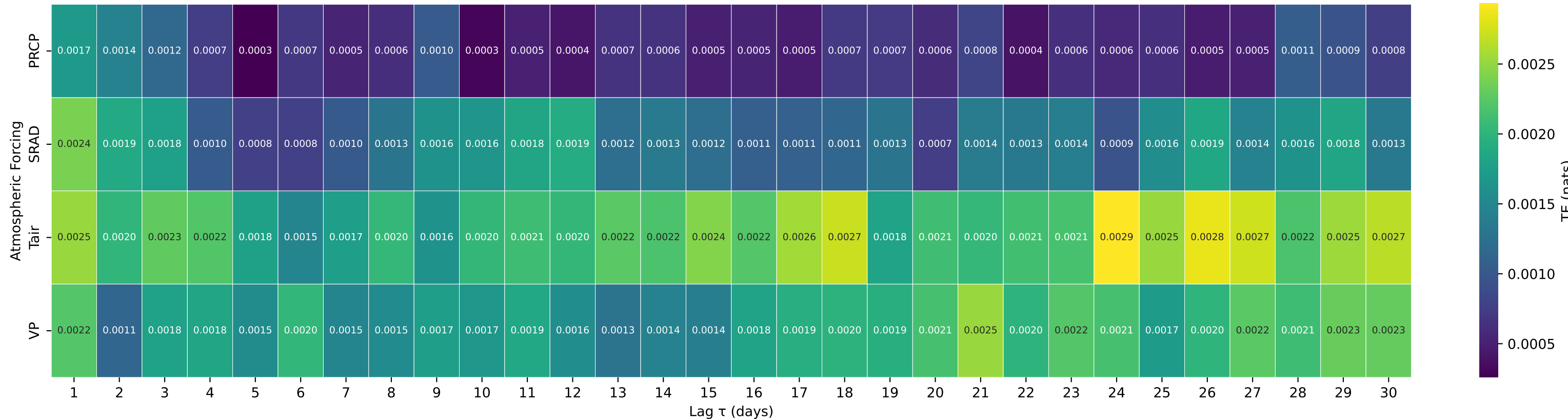
Shuffle-Test Significant TE to Streamflow — Basin 01548500 (HUC 02) — Pine Creek at Cedar Run, PA
