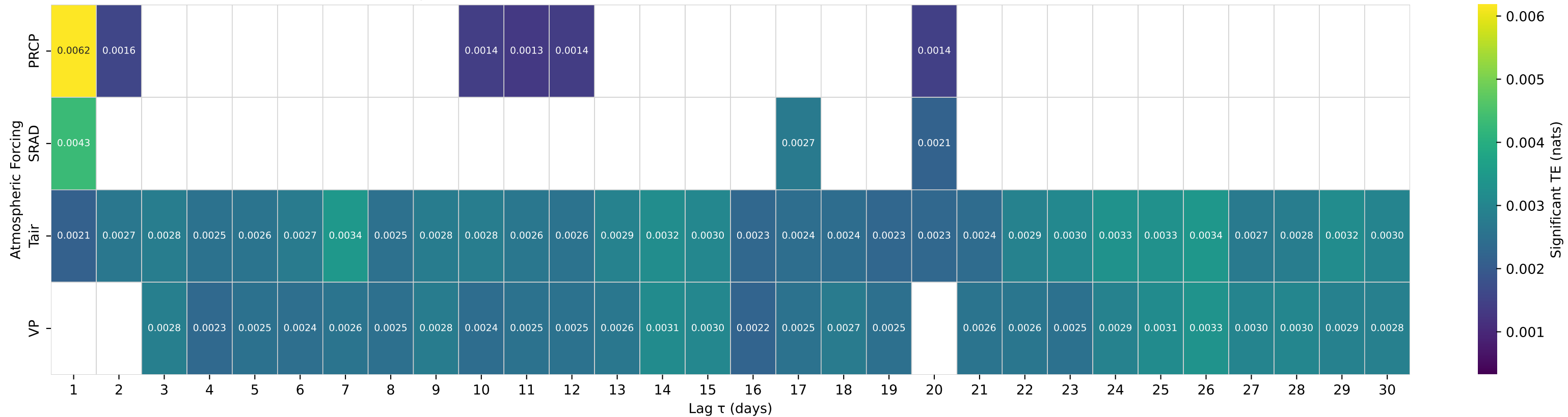
Shuffle-Test Significant TE to Streamflow — Basin 02081500 (HUC 03) — TAR RIVER NEAR TAR RIVER, NC
