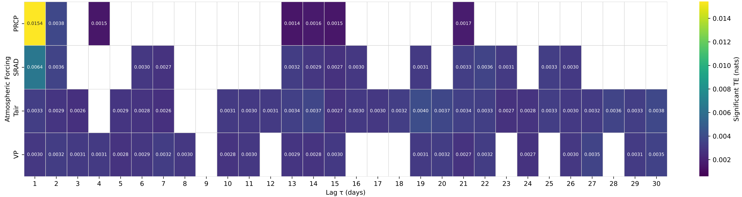
Shuffle-Test Significant TE to Streamflow — Basin 08023080 (HUC 12) — Bayou Grand Cane near Stanley, LA
