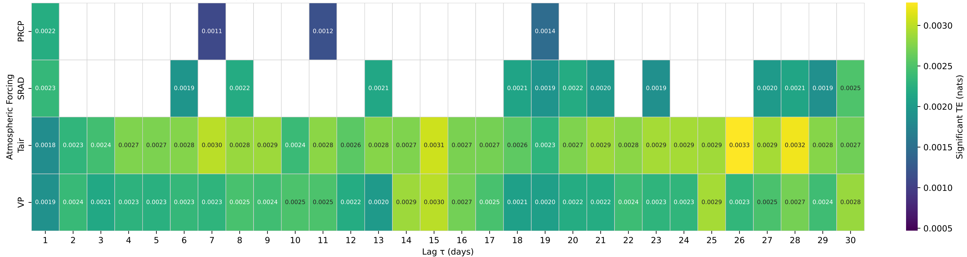
Shuffle-Test Significant TE to Streamflow — Basin 01639500 (HUC 02) — BIG PIPE CREEK AT BRUCEVILLE, MD
