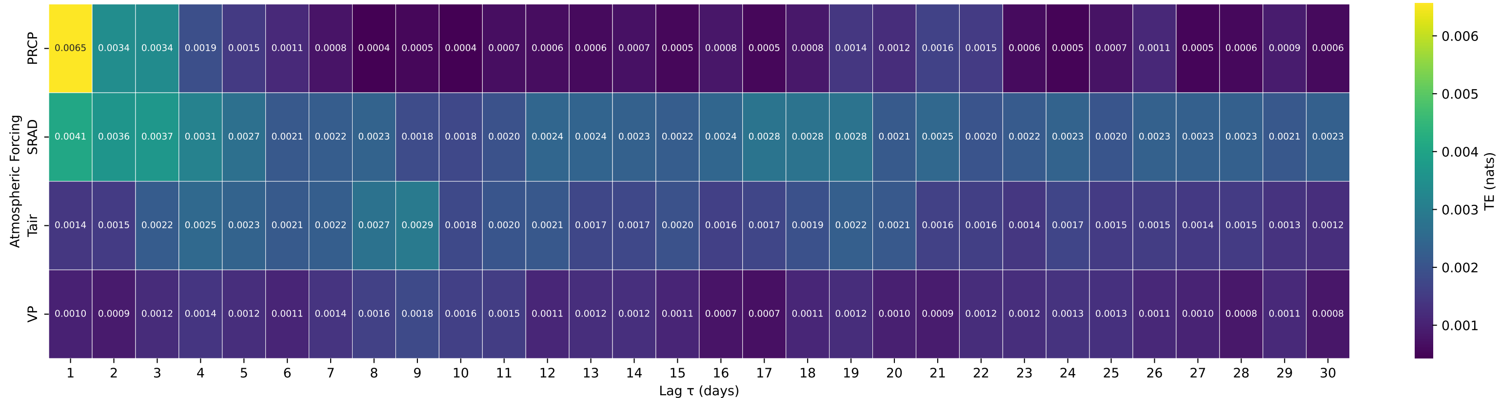
Shuffle-Test Significant TE to Streamflow — Basin 14182500 (HUC 17) — LITTLE NORTH SANTIAM RIVER NEAR MEHAMA, OR
