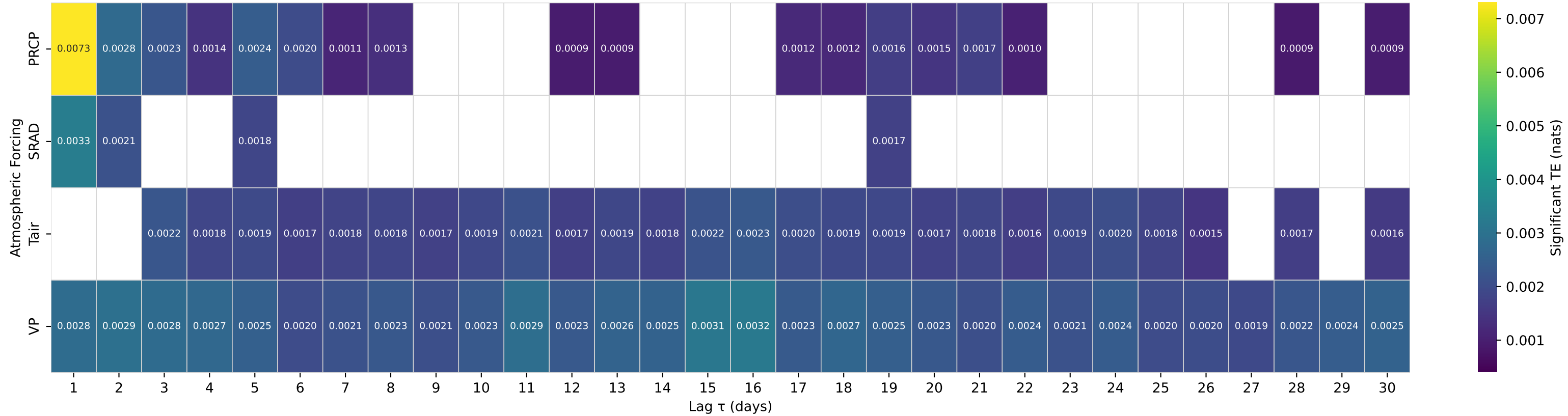
Shuffle-Test Significant TE to Streamflow — Basin 02231342 (HUC 03) — FT DRUM CREEK AT SUNSHINE ST PKY NEAR FT DRUM, FL
