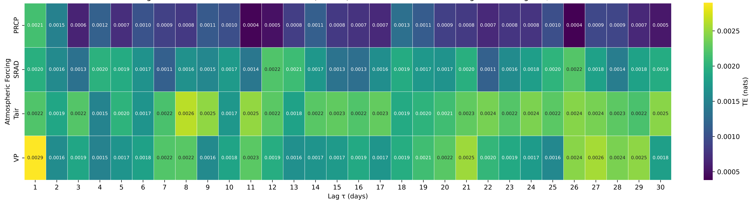
Shuffle-Test Significant TE to Streamflow — Basin 01543000 (HUC 02) — Driftwood Br Sinnemahoning Cr at Sterling Run, PA
