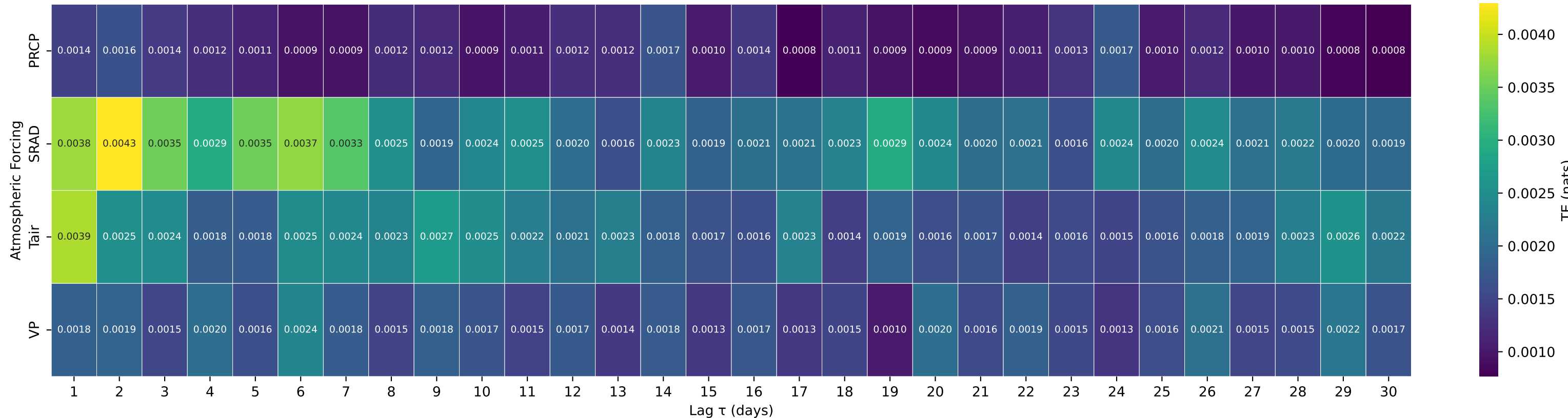
Shuffle-Test Significant TE to Streamflow — Basin 12374250 (HUC 17) — Mill Cr ab Bassoo Cr nr Niarada MT
