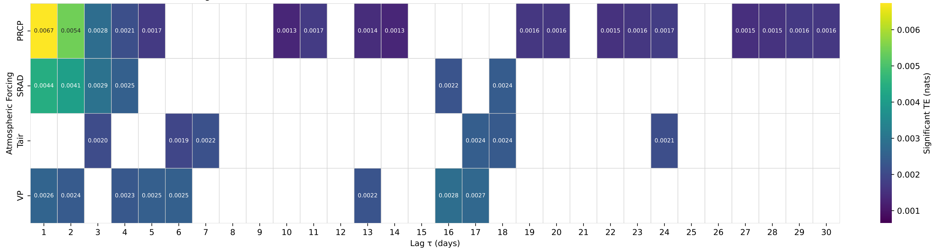
Shuffle-Test Significant TE to Streamflow — Basin 02312200 (HUC 03) — LITTLE WITHLACOOCHEE RIVER AT RERDELL, FLA.
