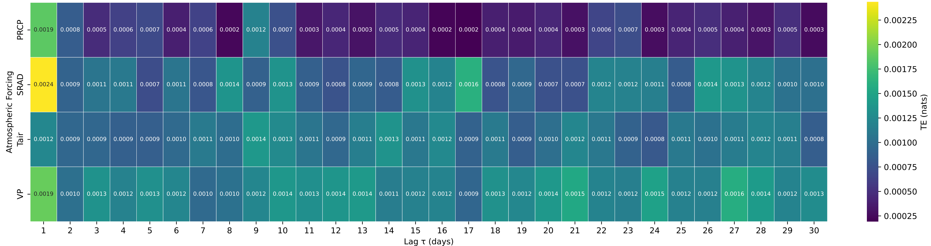
Shuffle-Test Significant TE to Streamflow — Basin 02140991 (HUC 03) — JOHNS RIVER AT ARNEYS STORE, NC
