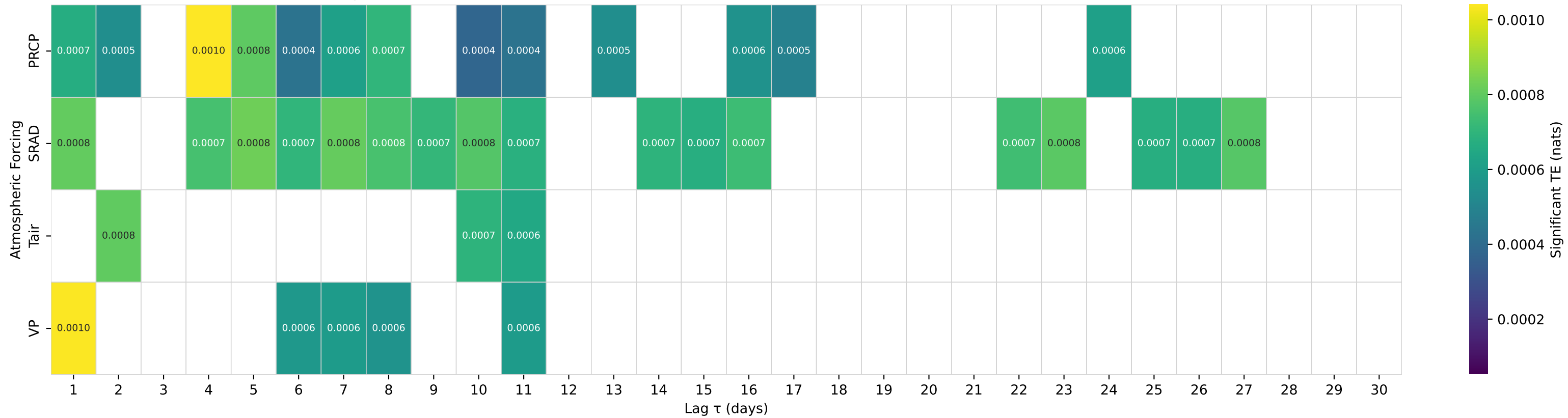
Shuffle-Test Significant TE to Streamflow — Basin 11224500 (HUC 18) — LOS GATOS C AB NUNEZ CYN NR COALINGA CA
