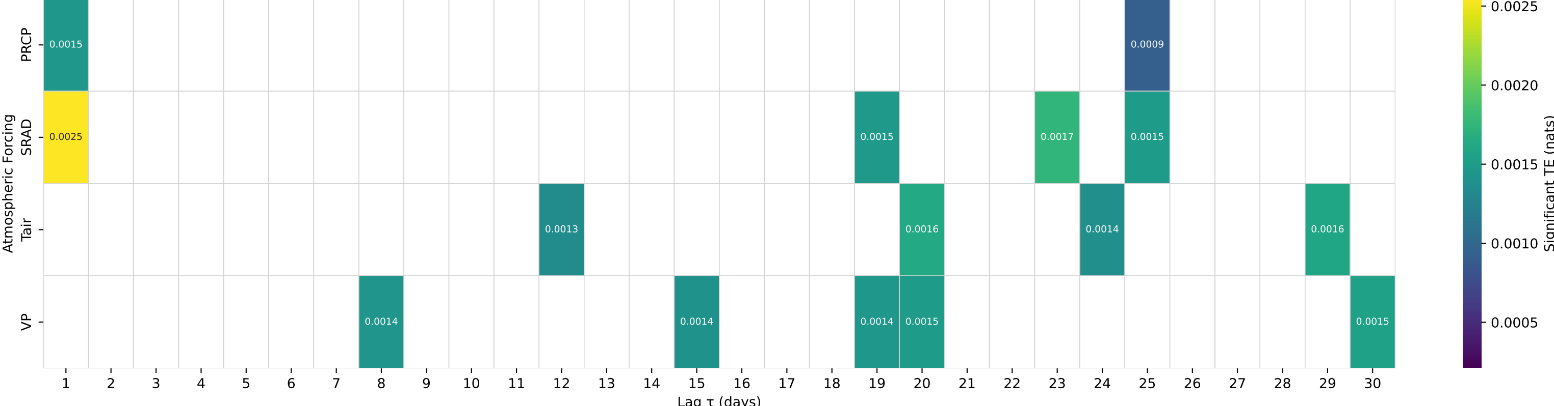
Shuffle-Test Significant TE to Streamflow — Basin 07362587 (HUC 08) — Alum Fork Saline River near Reform, AR
