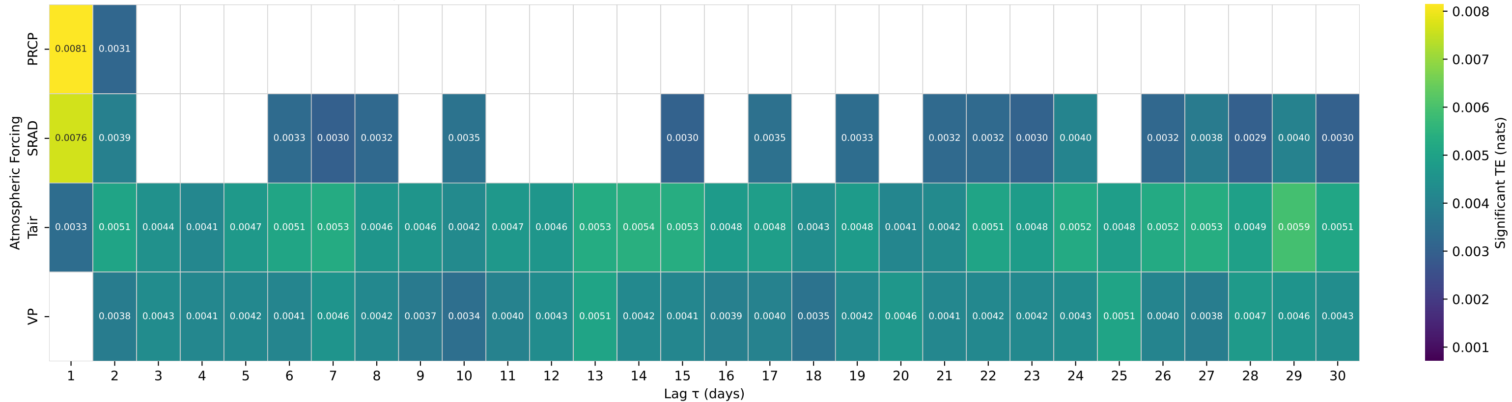
Shuffle-Test Significant TE to Streamflow — Basin 02196000 (HUC 03) — STEVENS CREEK NEAR MODOC, SC
