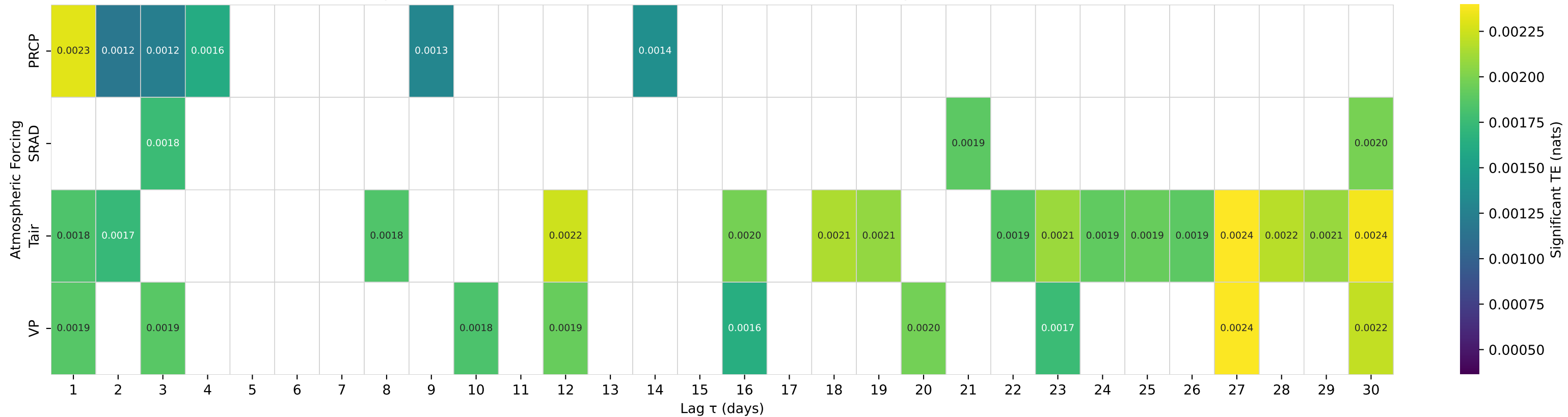
Shuffle-Test Significant TE to Streamflow — Basin 01545600 (HUC 02) — Young Womans Creek near Renovo, PA
