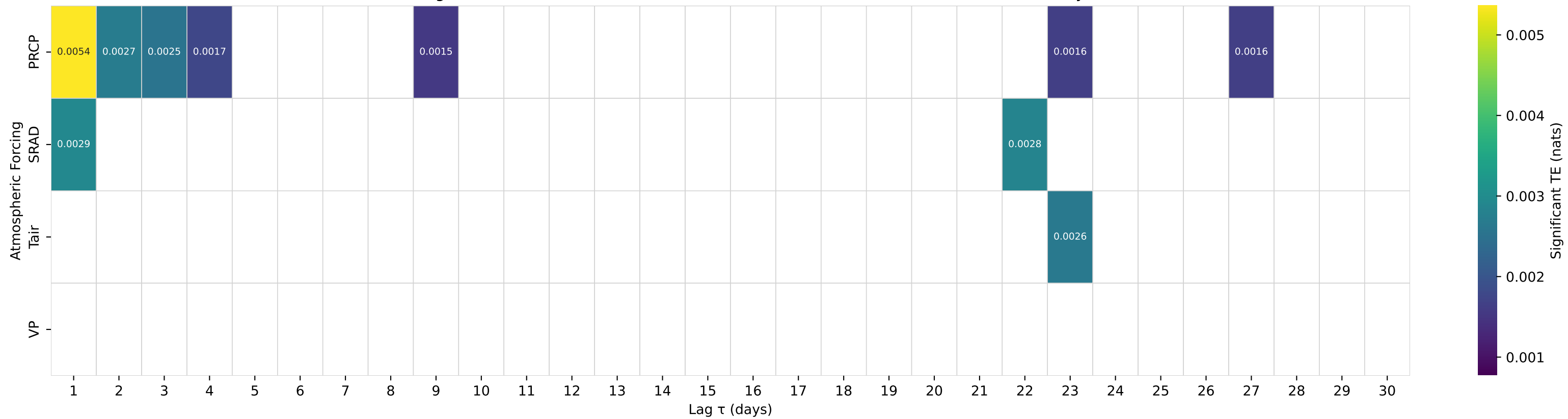
Shuffle-Test Significant TE to Streamflow — Basin 05501000 (HUC 07) — North River at Palmyra, MO
