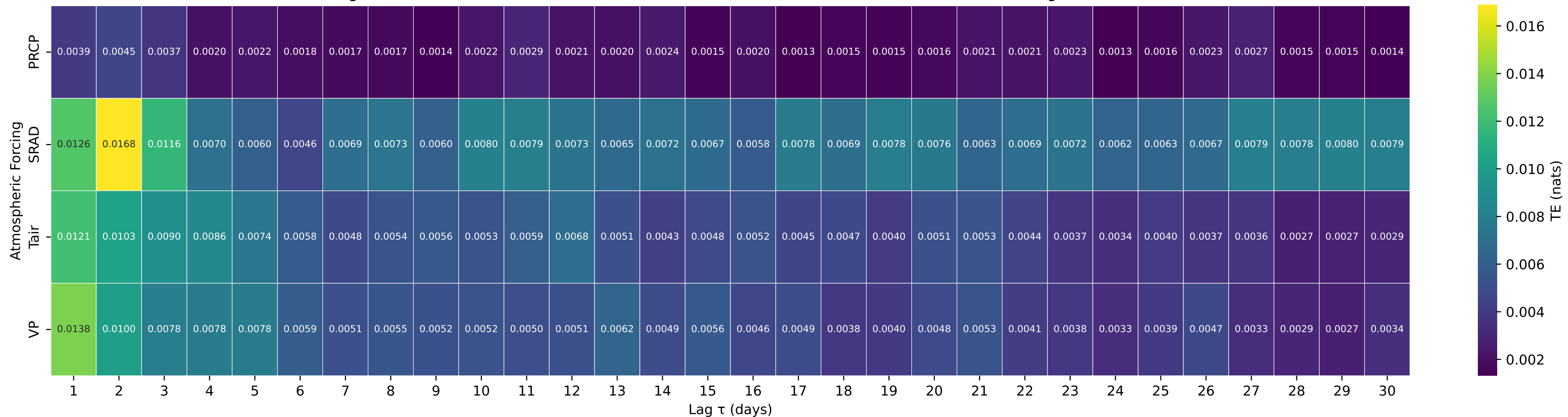
Shuffle-Test Significant TE to Streamflow — Basin 12377150 (HUC 17) — Mission Cr ab Reservoir nr ST Ignatius MT
