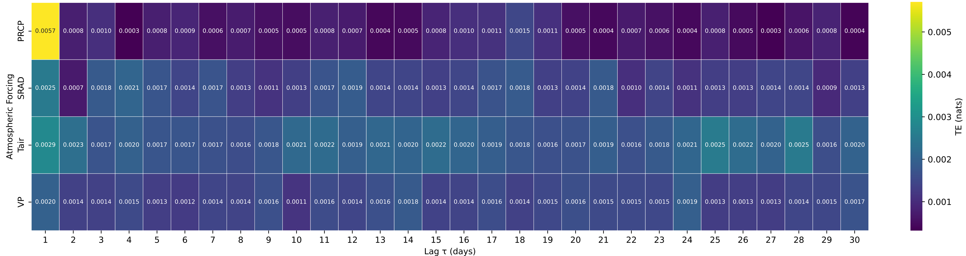
Shuffle-Test Significant TE to Streamflow — Basin 01073000 (HUC 01) — OYSTER RIVER NEAR DURHAM, NH
