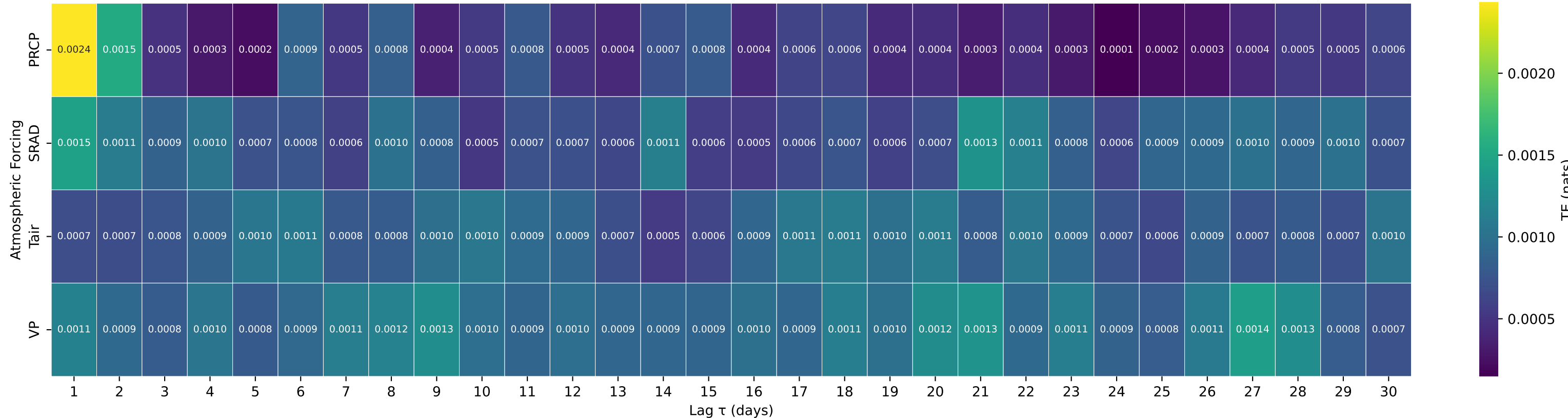
Shuffle-Test Significant TE to Streamflow — Basin 08086212 (HUC 12) — Hubbard Ck bl Albany, TX
