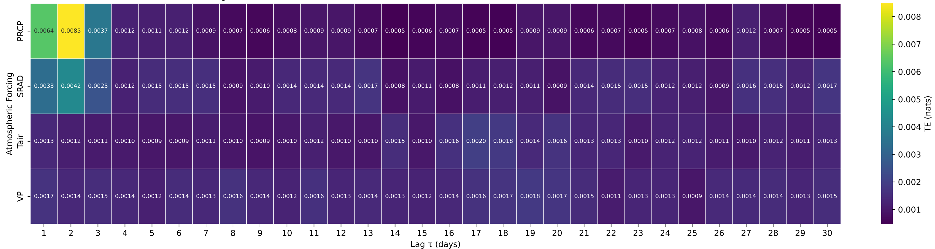
Shuffle-Test Significant TE to Streamflow — Basin 02202600 (HUC 03) — BLACK CREEK NEAR BLITCHTON, GA
