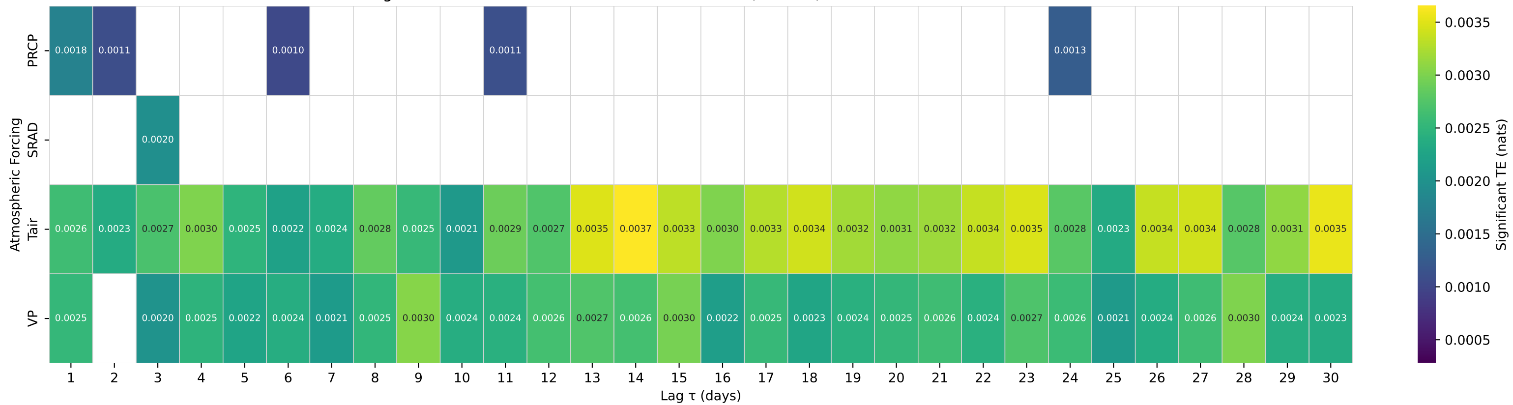
Shuffle-Test Significant TE to Streamflow — Basin 01510000 (HUC 02) — OTSELIC RIVER AT CINCINNATUS NY
