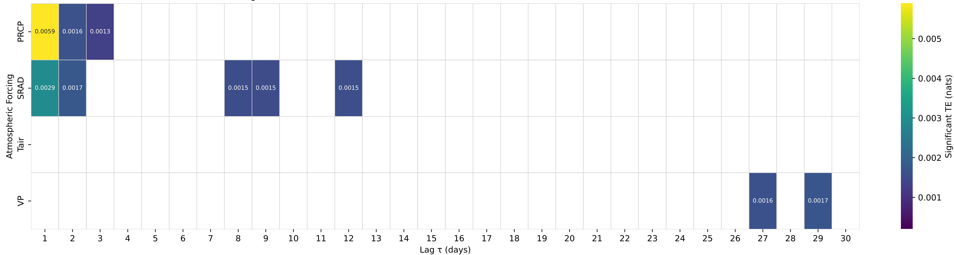
Shuffle-Test Significant TE to Streamflow — Basin 07375000 (HUC 08) — Tchefuncta River near Folsom, LA
