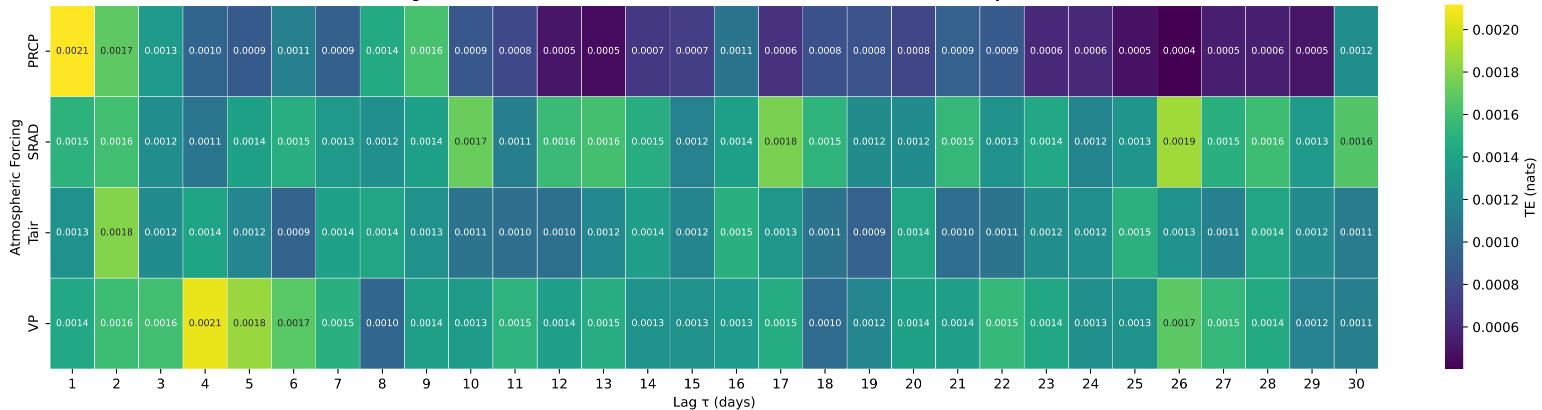
Shuffle-Test Significant TE to Streamflow — Basin 05507600 (HUC 07) — Lick Creek at Perry, MO
