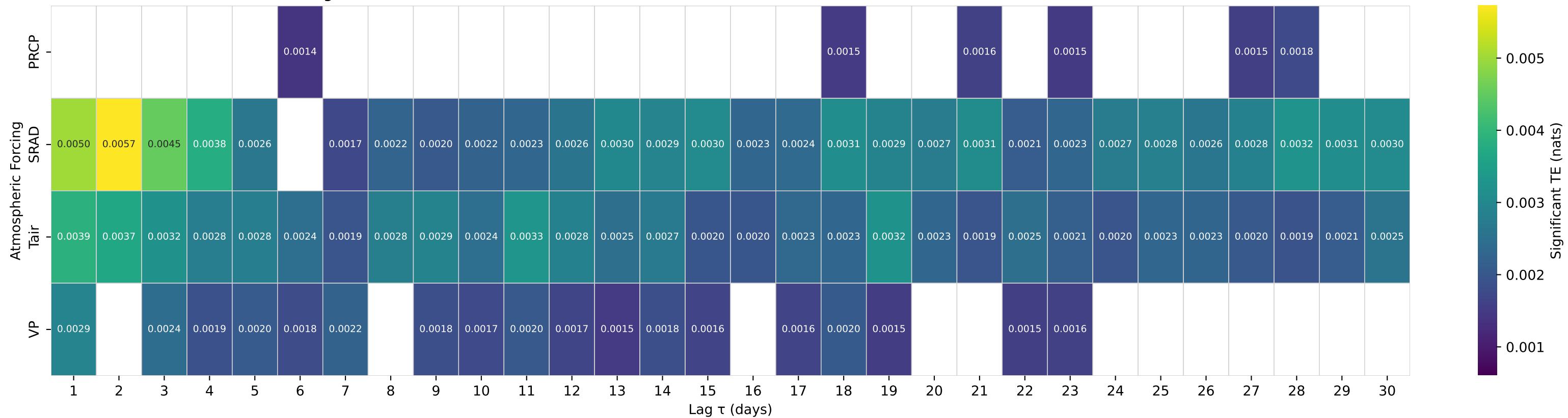
Shuffle-Test Significant TE to Streamflow — Basin 09223000 (HUC 14) — HAMS FORK BELOW POLE CREEK, NEAR FRONTIER, WY
