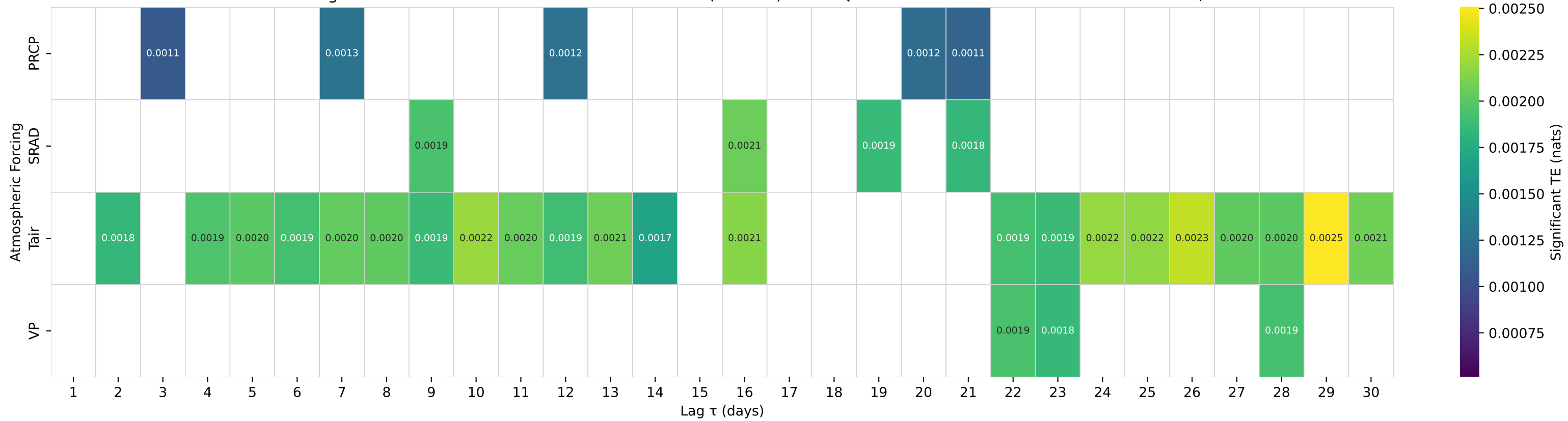
Shuffle-Test Significant TE to Streamflow — Basin 01658500 (HUC 02) — S F QUANTICO CREEK NEAR INDEPENDENT HILL, VA
