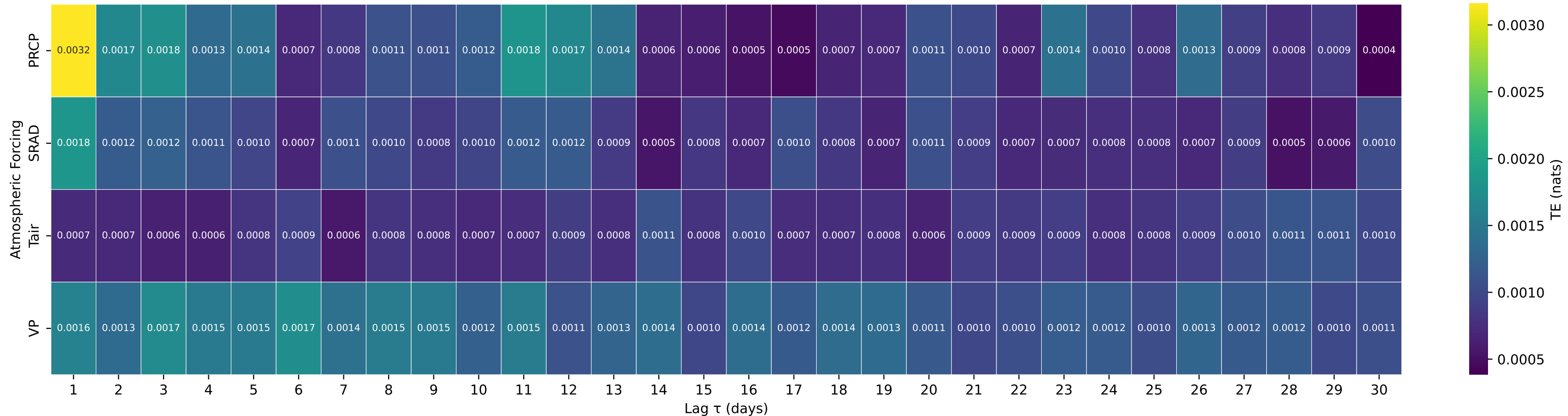
Shuffle-Test Significant TE to Streamflow — Basin 09480000 (HUC 15) — SANTA CRUZ RIVER NEAR LOCHIEL, AZ.
