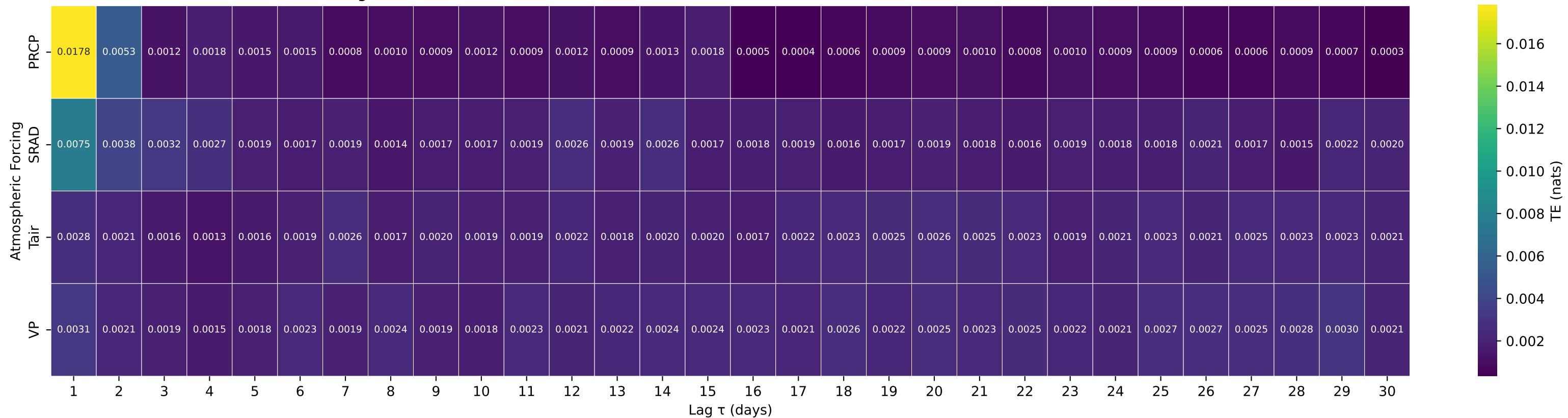
Shuffle-Test Significant TE to Streamflow — Basin 02479560 (HUC 03) — ESCATAWPA RIVER NEAR AGRICOLA MS
