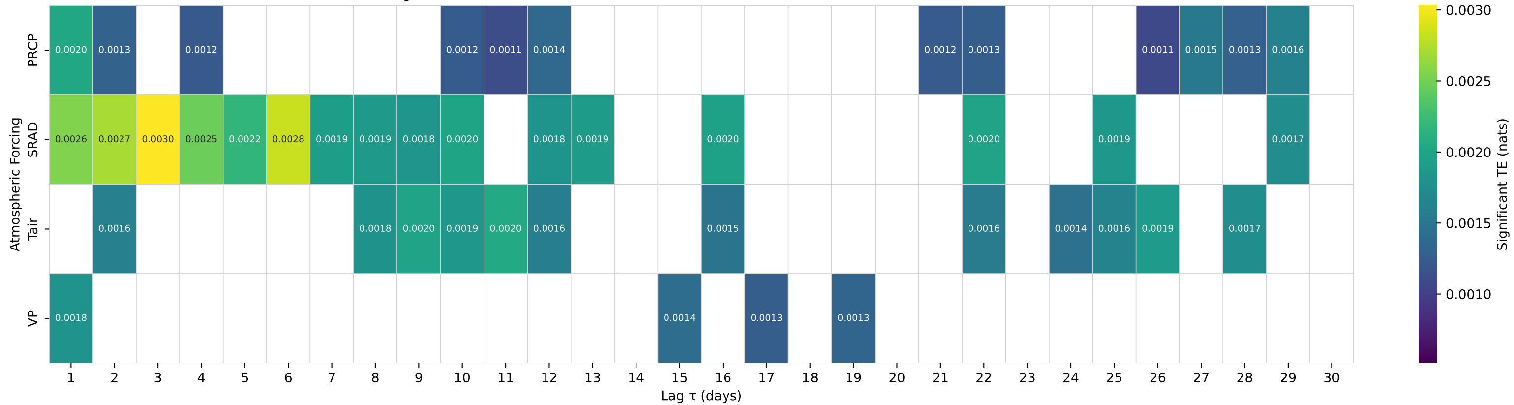
Shuffle-Test Significant TE to Streamflow — Basin 13083000 (HUC 17) — TRAPPER CREEK NR OAKLEY ID
