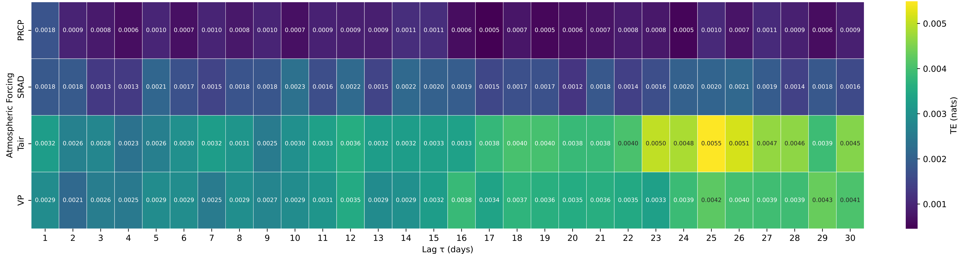
Shuffle-Test Significant TE to Streamflow — Basin 03078000 (HUC 05) — CASSELMAN RIVER AT GRANTSVILLE, MD
