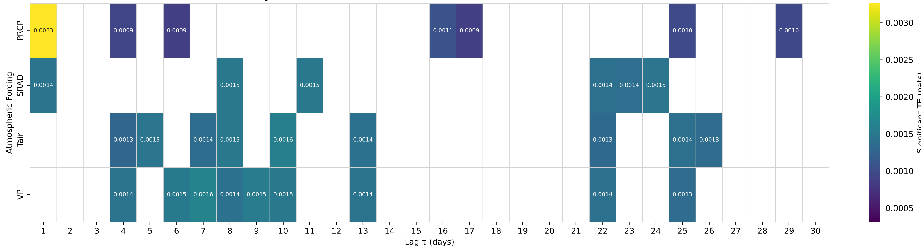
Shuffle-Test Significant TE to Streamflow — Basin 07197000 (HUC 11) — Baron Fork at Eldon, OK
