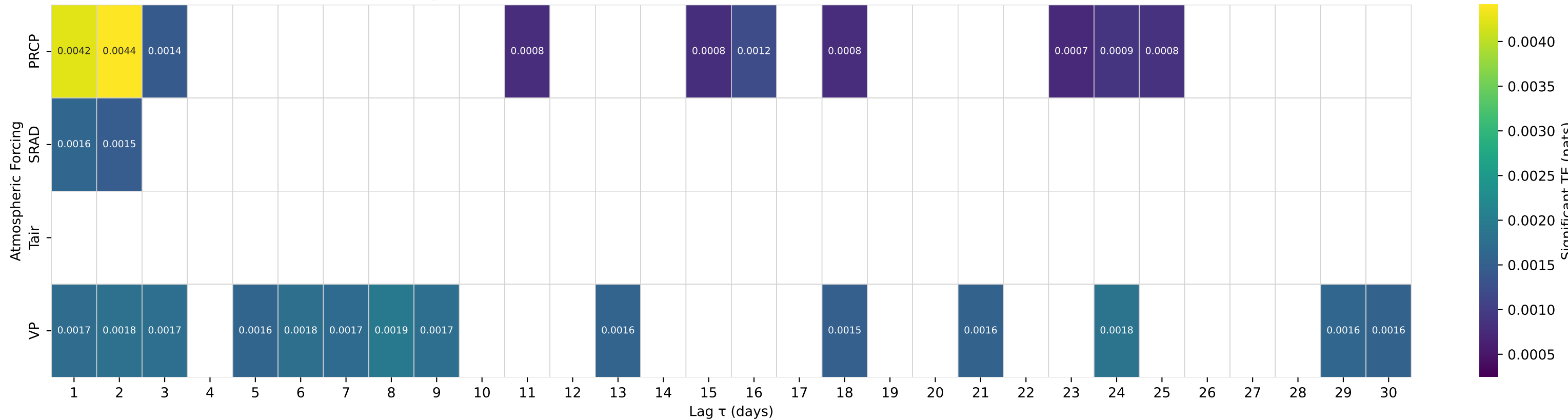
Shuffle-Test Significant TE to Streamflow — Basin 08194200 (HUC 12) — San Casimiro Ck nr Freer, TX
