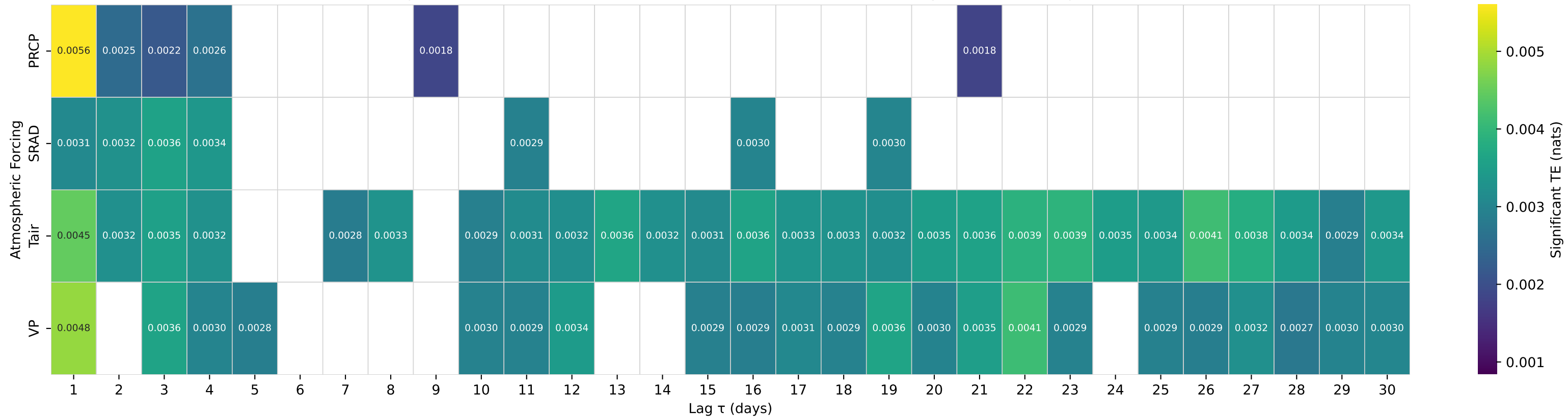
Shuffle-Test Significant TE to Streamflow — Basin 03010655 (HUC 05) — Oswayo Creek at Shinglehouse, PA
