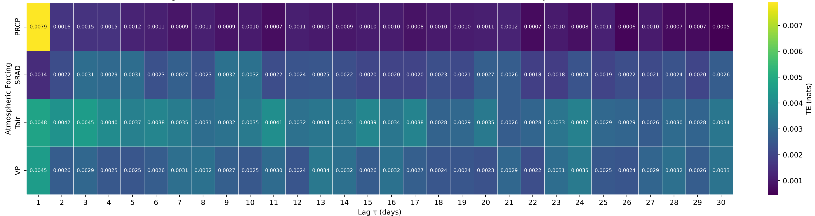
Shuffle-Test Significant TE to Streamflow — Basin 04057510 (HUC 04) — STURGEON RIVER NEAR NAHMA JUNCTION, MI
