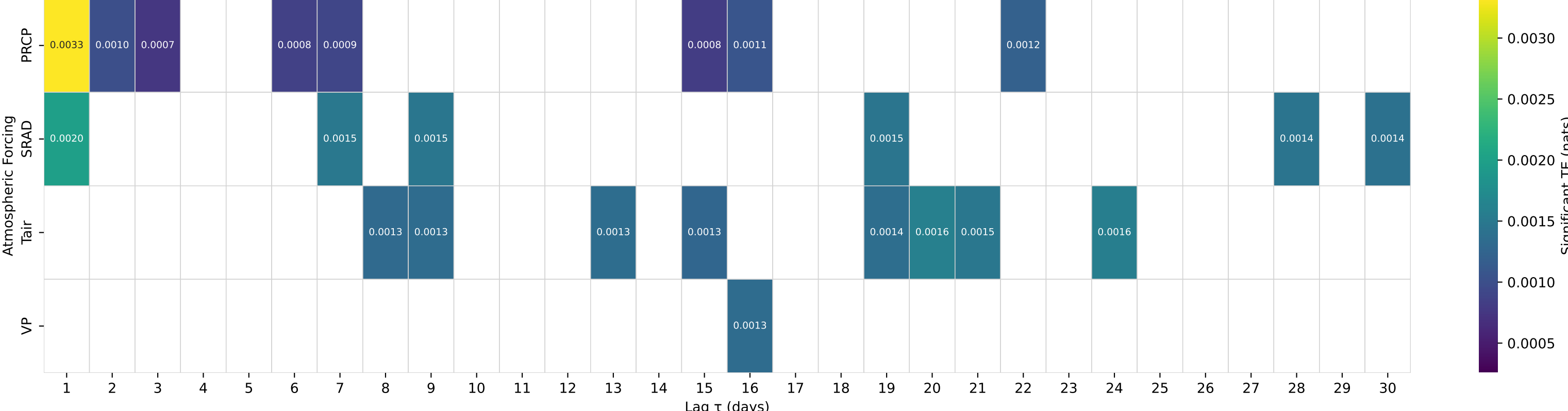
Shuffle-Test Significant TE to Streamflow — Basin 07056000 (HUC 11) — Buffalo River near St. Joe, AR
