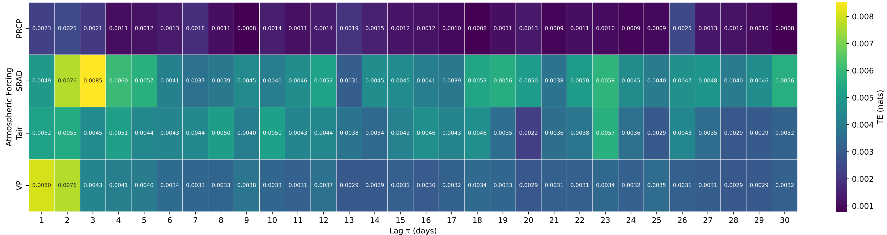
Shuffle-Test Significant TE to Streamflow — Basin 12375900 (HUC 17) — South Crow Creek near Ronan MT
