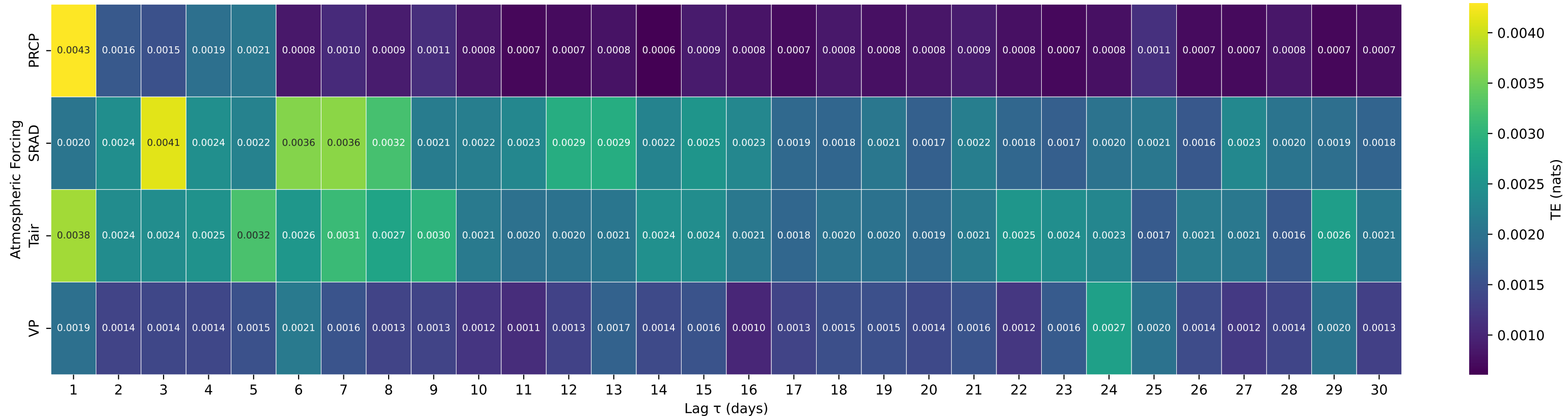
Shuffle-Test Significant TE to Streamflow — Basin 04040500 (HUC 04) — STURGEON RIVER NEAR SIDNAW, MI
