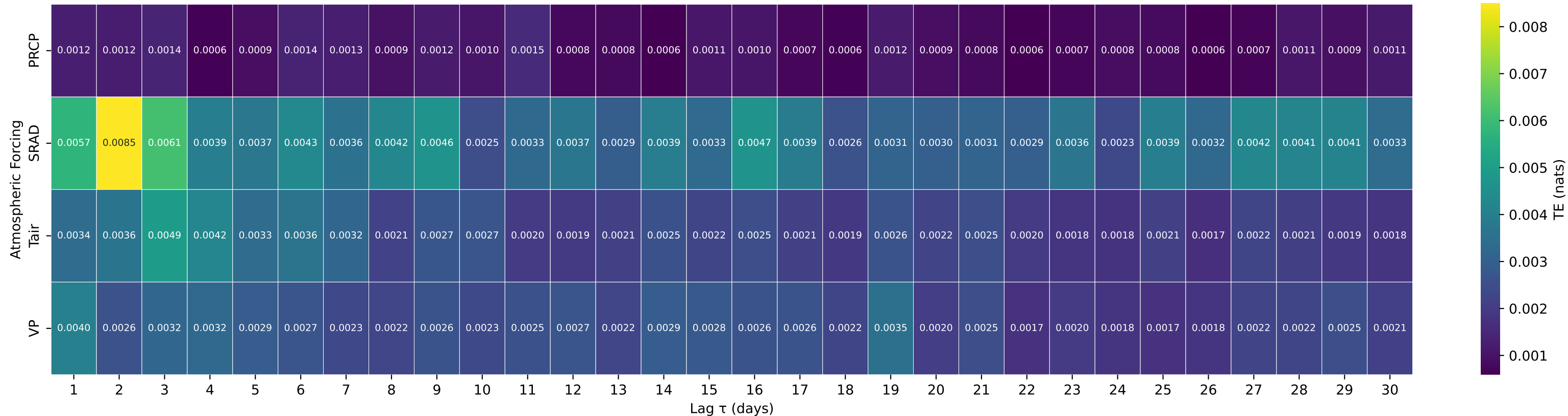
Shuffle-Test Significant TE to Streamflow — Basin 12381400 (HUC 17) — South Fork Jocko River near Arlee MT
