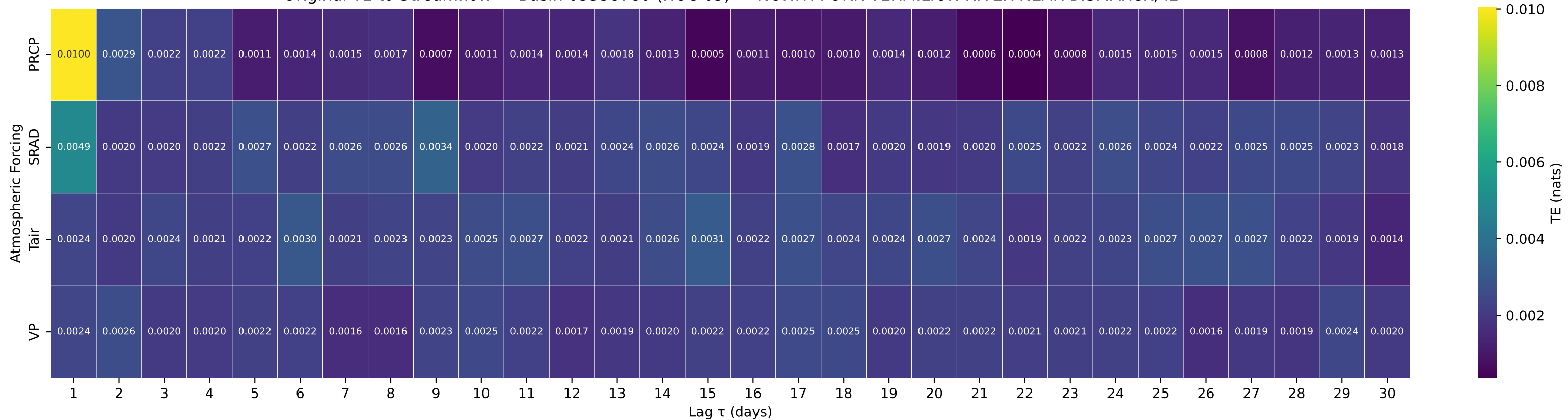
Shuffle-Test Significant TE to Streamflow — Basin 03338780 (HUC 05) — NORTH FORK VERMILION RIVER NEAR BISMARCK, IL
