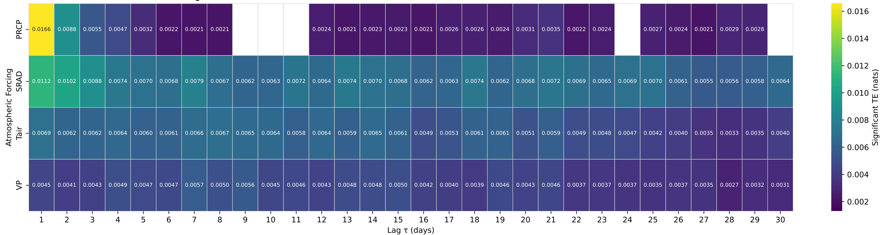
Shuffle-Test Significant TE to Streamflow — Basin 12167000 (HUC 17) — NF STILLAGUAMISH RIVER NEAR ARLINGTON, WA
