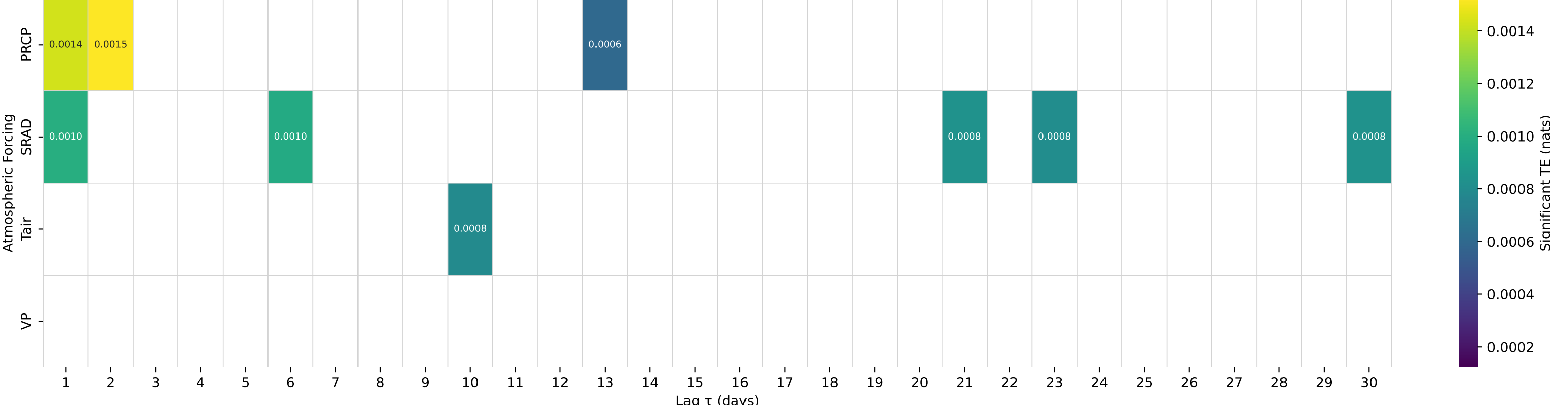
Shuffle-Test Significant TE to Streamflow — Basin 02361000 (HUC 03) — CHOCTAWHATCHEE RIVER NEAR NEWTON, AL.
