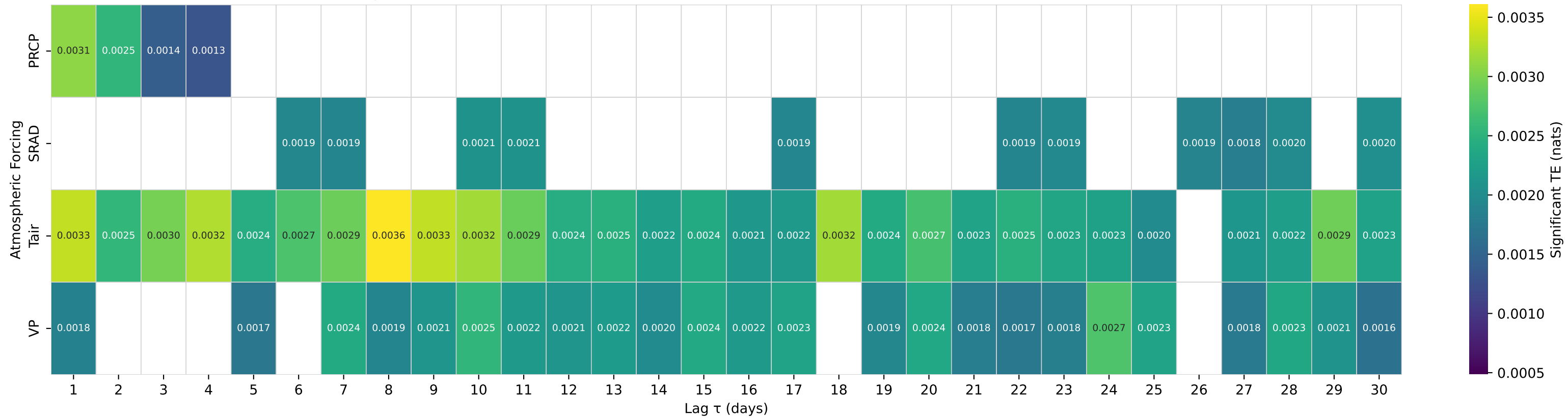
Shuffle-Test Significant TE to Streamflow — Basin 04056500 (HUC 04) — MANISTIQUE RIVER NEAR MANISTIQUE, MI
