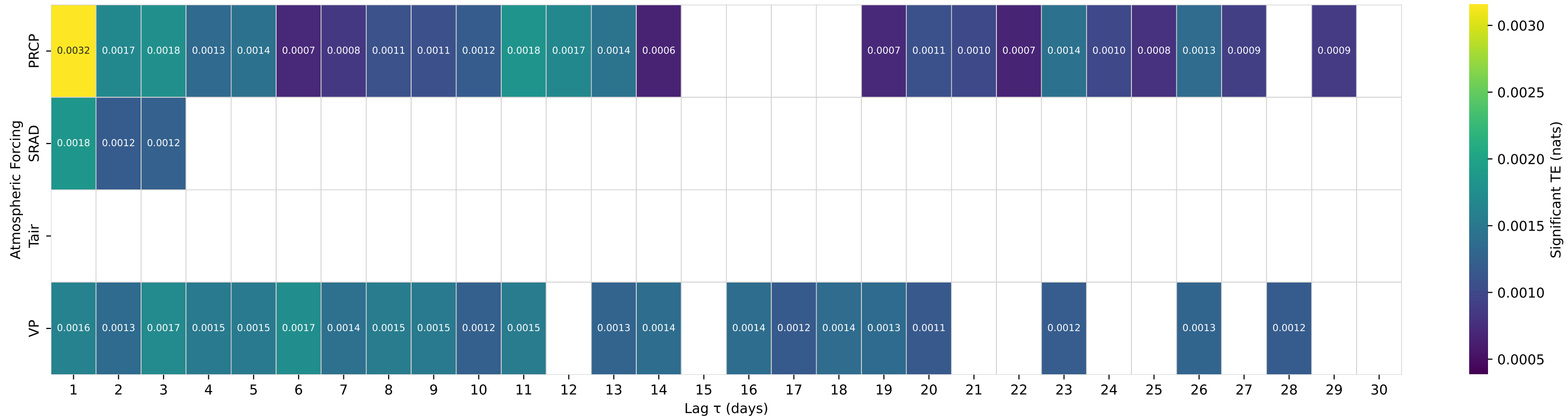
Shuffle-Test Significant TE to Streamflow — Basin 09480000 (HUC 15) — SANTA CRUZ RIVER NEAR LOCHIEL, AZ.
