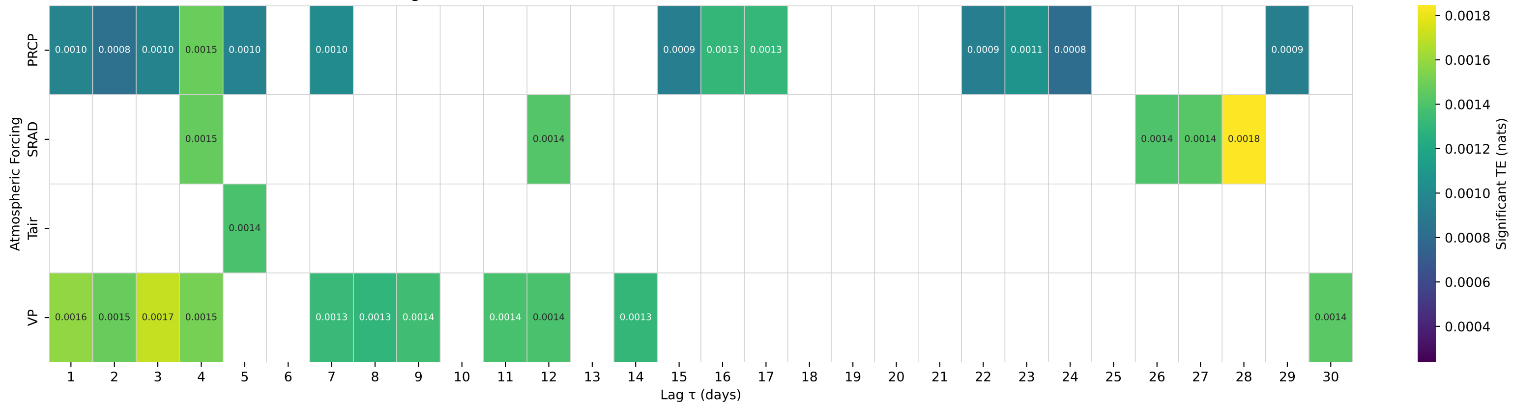
Shuffle-Test Significant TE to Streamflow — Basin 06879650 (HUC 10) — KINGS C NR MANHATTAN, KS
