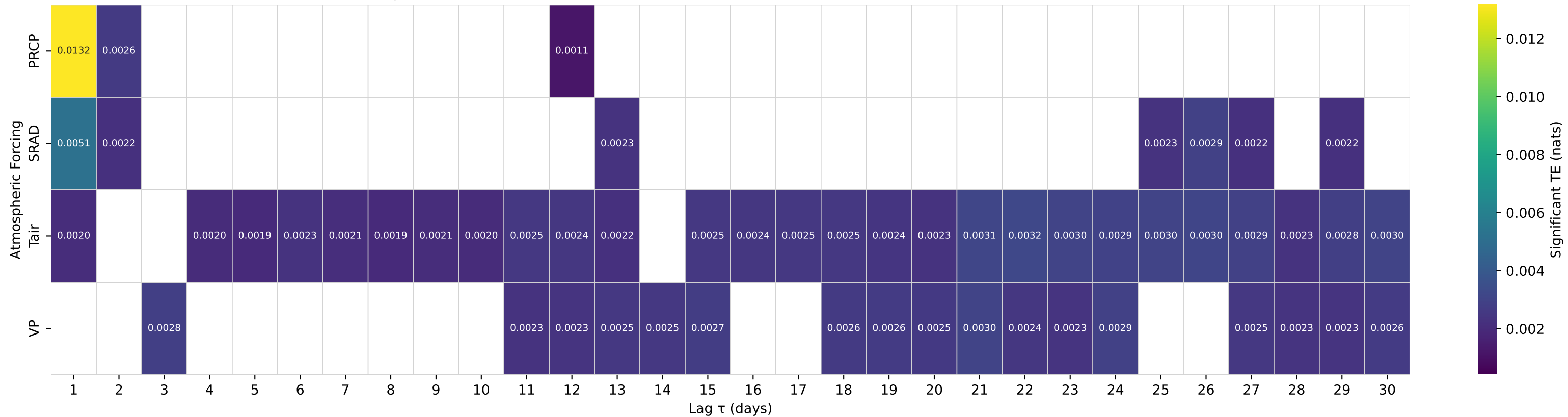
Shuffle-Test Significant TE to Streamflow — Basin 02469800 (HUC 03) — SATILPA CREEK NEAR COFFEEVILLE AL
