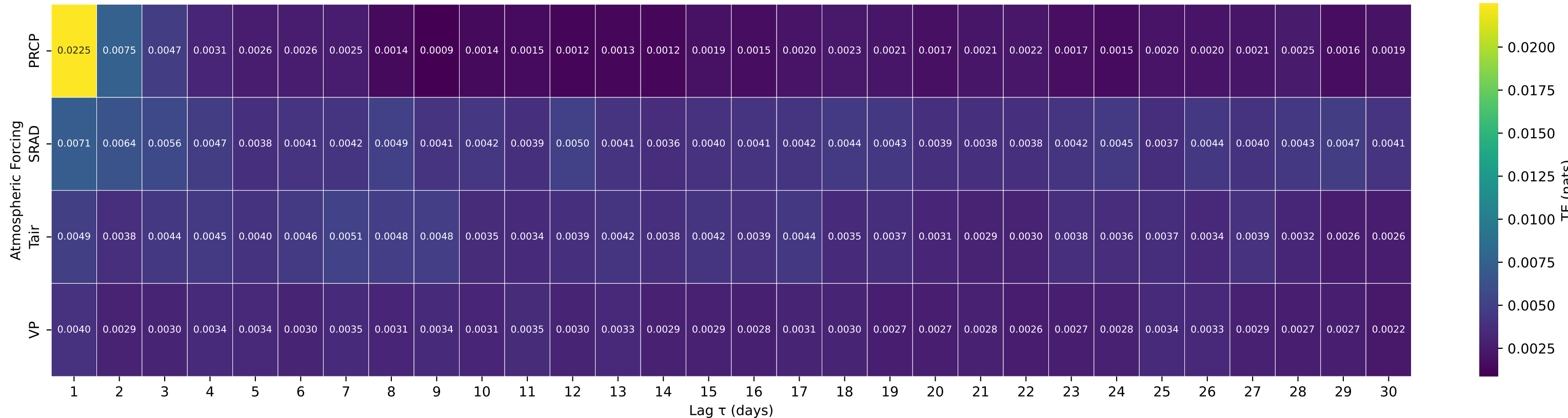
Shuffle-Test Significant TE to Streamflow — Basin 12144000 (HUC 17) — SF SNOQUALMIE RIVER AT NORTH BEND, WA
