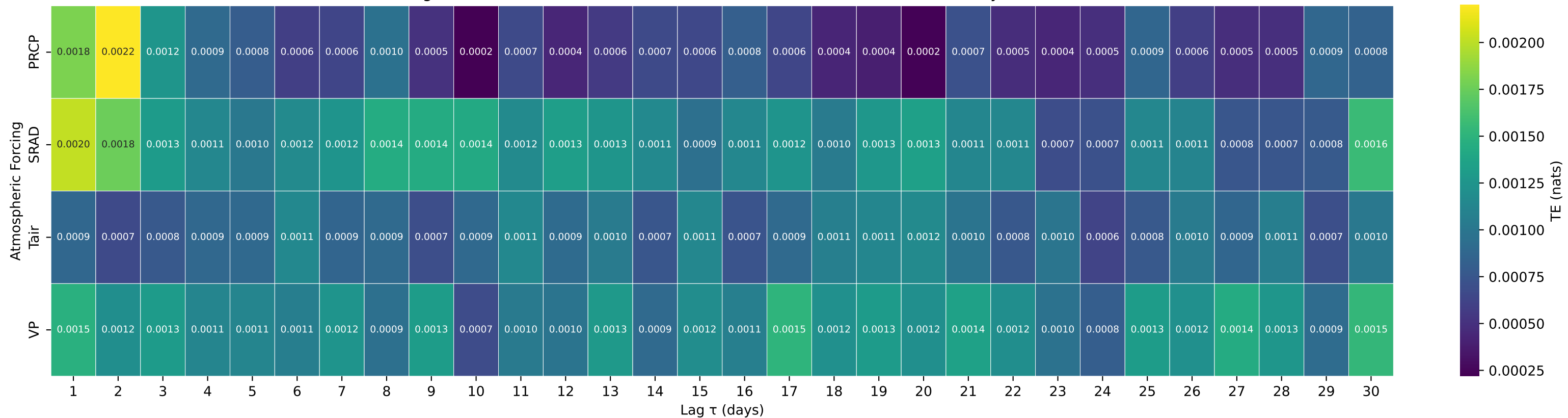
Shuffle-Test Significant TE to Streamflow — Basin 08171300 (HUC 12) — Blanco Rv nr Kyle, TX
