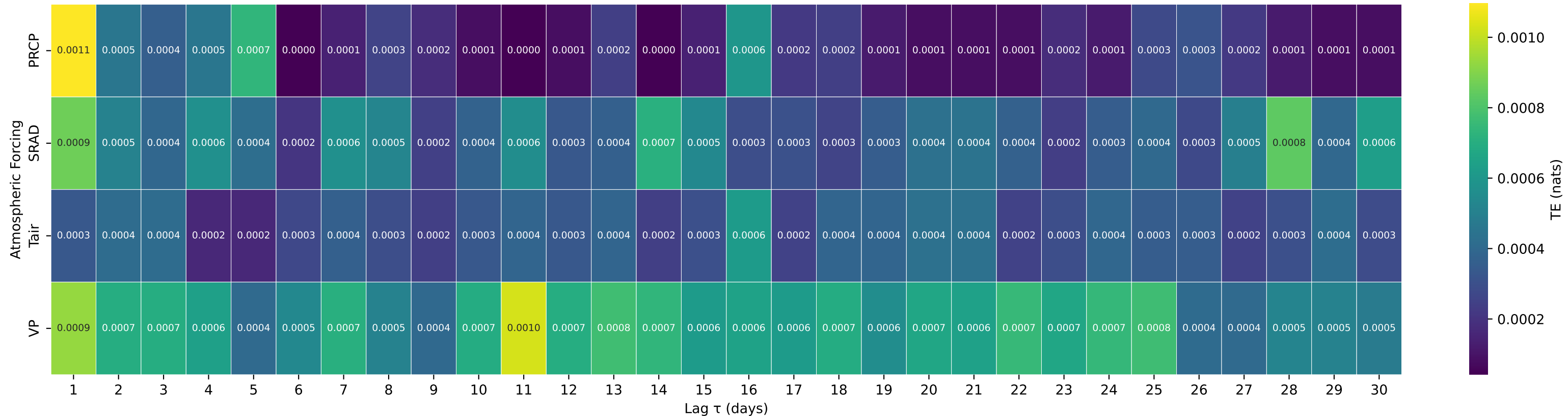
Shuffle-Test Significant TE to Streamflow — Basin 08196000 (HUC 12) — Dry Frio Rv nr Reagan Wells, TX
