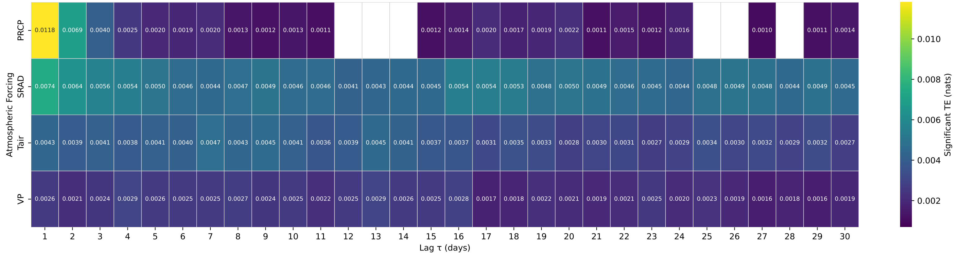
Shuffle-Test Significant TE to Streamflow — Basin 12025700 (HUC 17) — SKOOKUMCHUCK RIVER NEAR VAIL, WA
