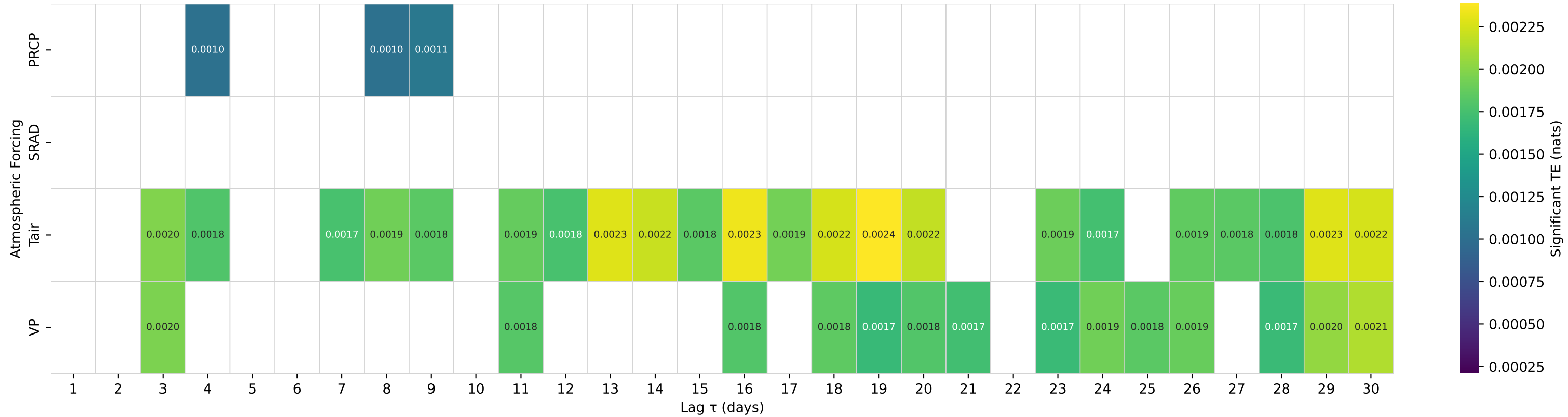
Shuffle-Test Significant TE to Streamflow — Basin 01516500 (HUC 02) — Corey Creek near Mainesburg, PA
