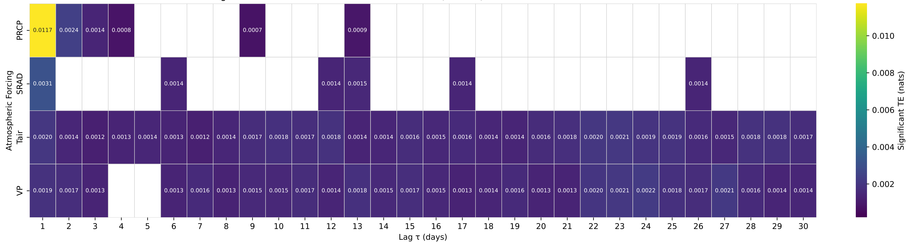
Shuffle-Test Significant TE to Streamflow — Basin 03574500 (HUC 06) — PAINT ROCK RIVER NEAR WOODVILLE AL
