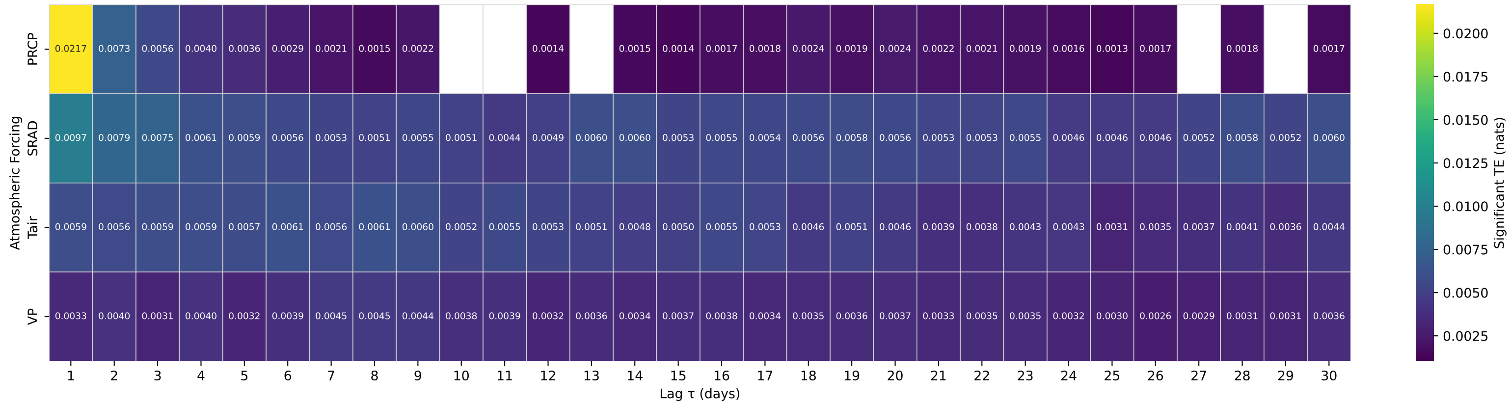
Shuffle-Test Significant TE to Streamflow — Basin 14141500 (HUC 17) — LITTLE SANDY RIVER NEAR BULL RUN, OREG.
