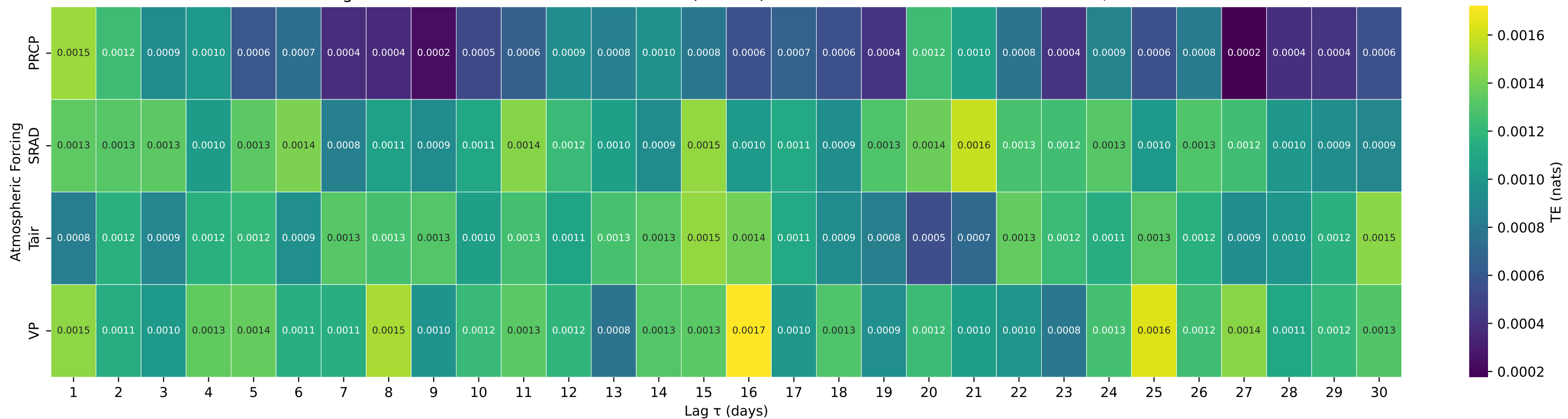
Shuffle-Test Significant TE to Streamflow — Basin 01666500 (HUC 02) — ROBINSON RIVER NEAR LOCUST DALE, VA
