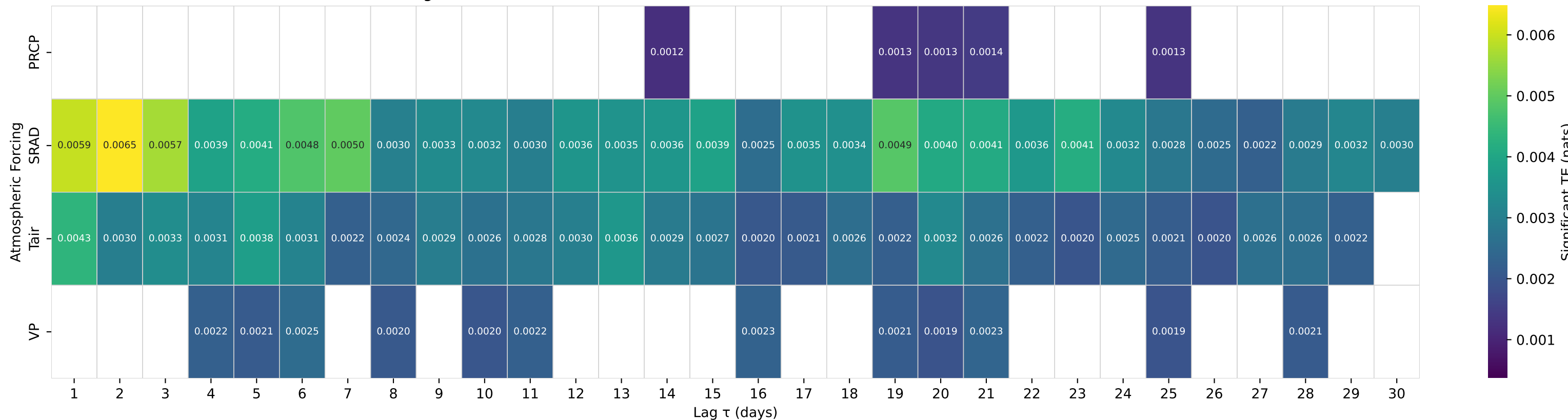
Shuffle-Test Significant TE to Streamflow — Basin 08267500 (HUC 13) — RIO HONDO NEAR VALDEZ, NM
