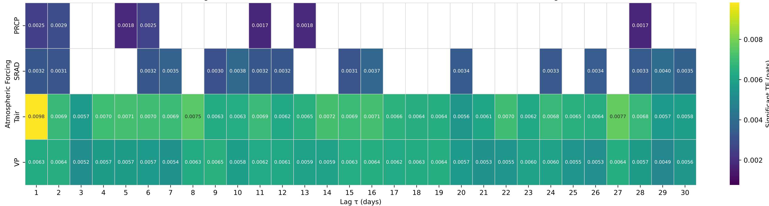
Shuffle-Test Significant TE to Streamflow — Basin 03021350 (HUC 05) — French Creek near Wattsburg, PA
