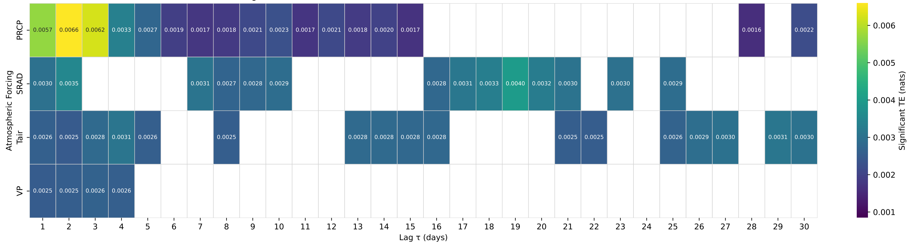
Shuffle-Test Significant TE to Streamflow — Basin 06452000 (HUC 10) — WHITE R NEAR OACOMA SD
