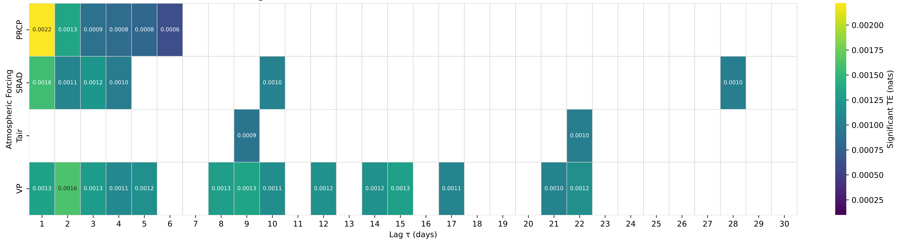
Shuffle-Test Significant TE to Streamflow — Basin 08195000 (HUC 12) — Frio Rv at Concan, TX
