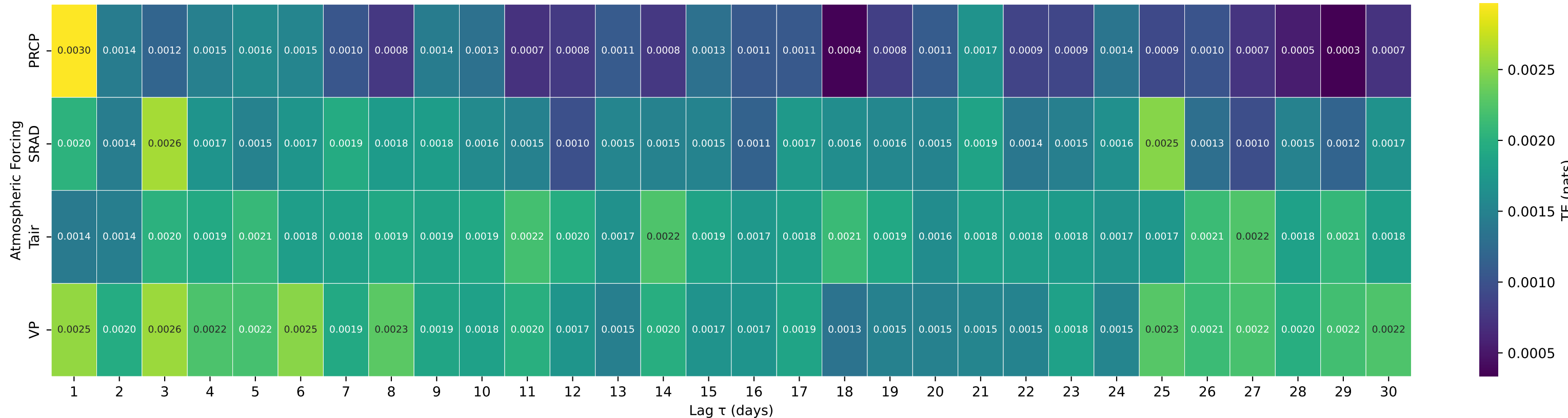
Shuffle-Test Significant TE to Streamflow — Basin 06921200 (HUC 10) — Lindley Creek near Polk, MO
