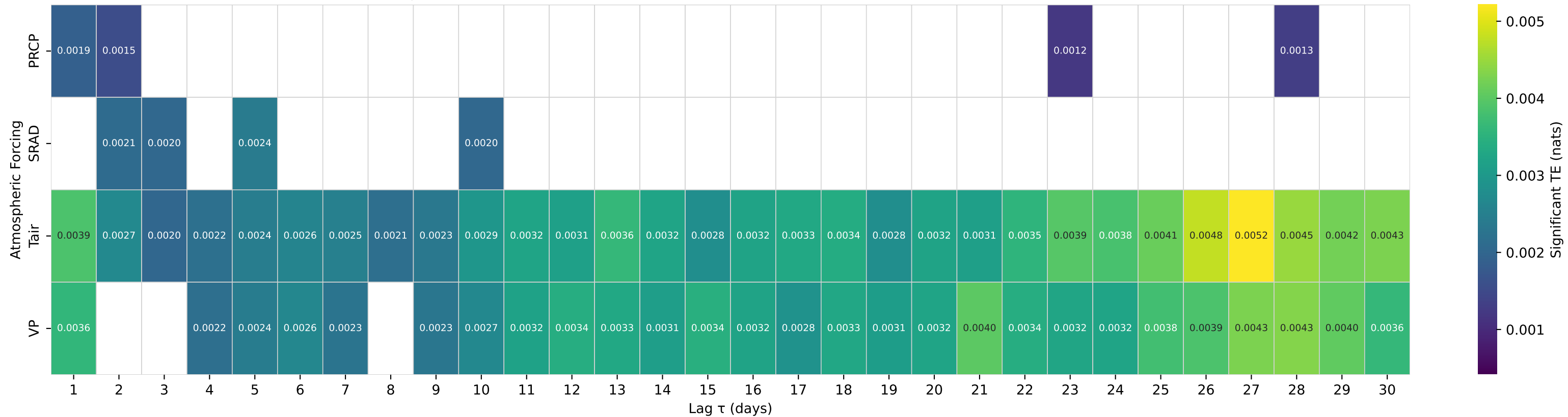
Shuffle-Test Significant TE to Streamflow — Basin 01596500 (HUC 02) — SAVAGE RIVER NEAR BARTON, MD
