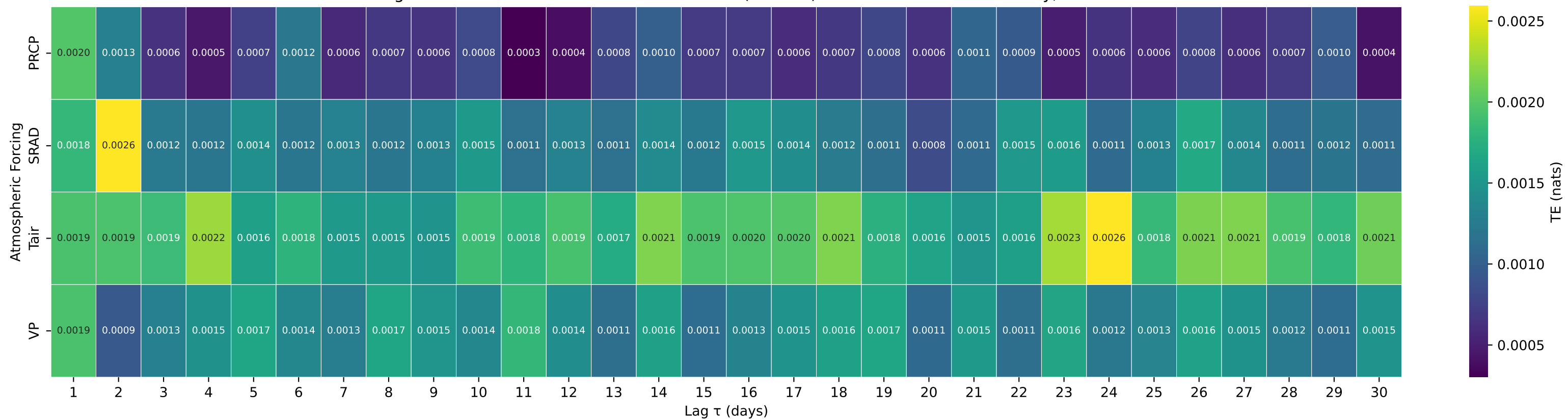
Shuffle-Test Significant TE to Streamflow — Basin 03011800 (HUC 05) — Kinzua Creek near Guffey, PA
