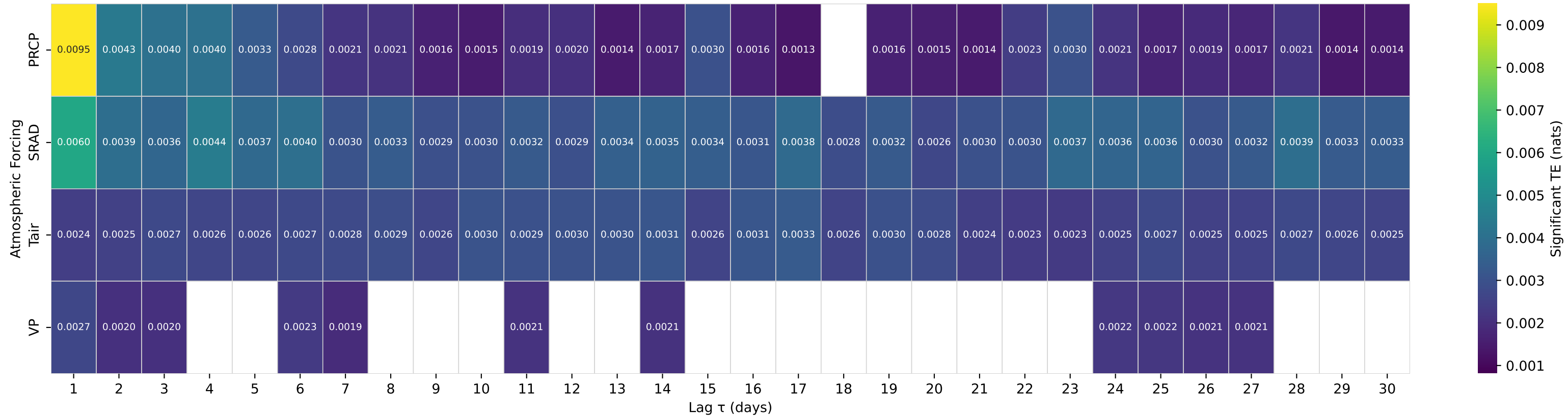
Shuffle-Test Significant TE to Streamflow — Basin 11468500 (HUC 18) — NOYO R NR FORT BRAGG CA
