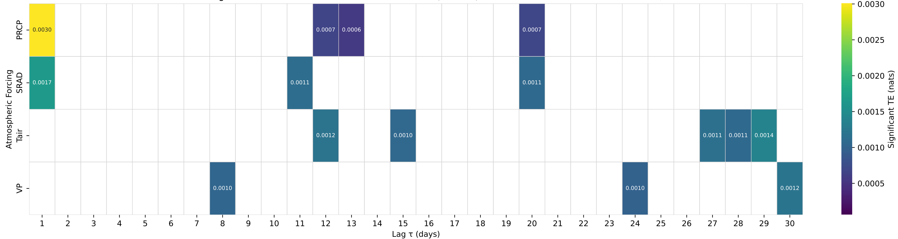
Shuffle-Test Significant TE to Streamflow — Basin 01484100 (HUC 02) — BEAVERDAM BRANCH AT HOUSTON, DE
