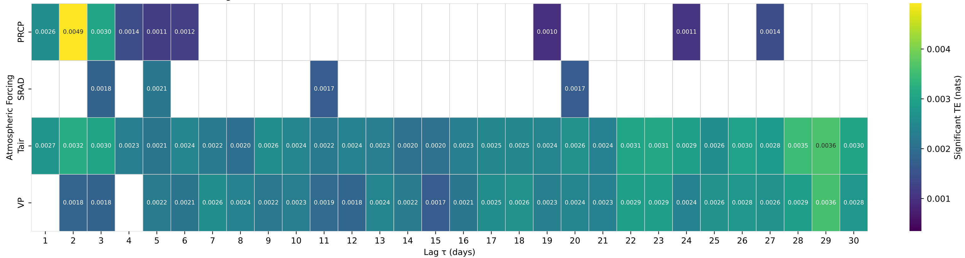
Shuffle-Test Significant TE to Streamflow — Basin 04122500 (HUC 04) — PERE MARQUETTE RIVER AT SCOTTVILLE, MI
