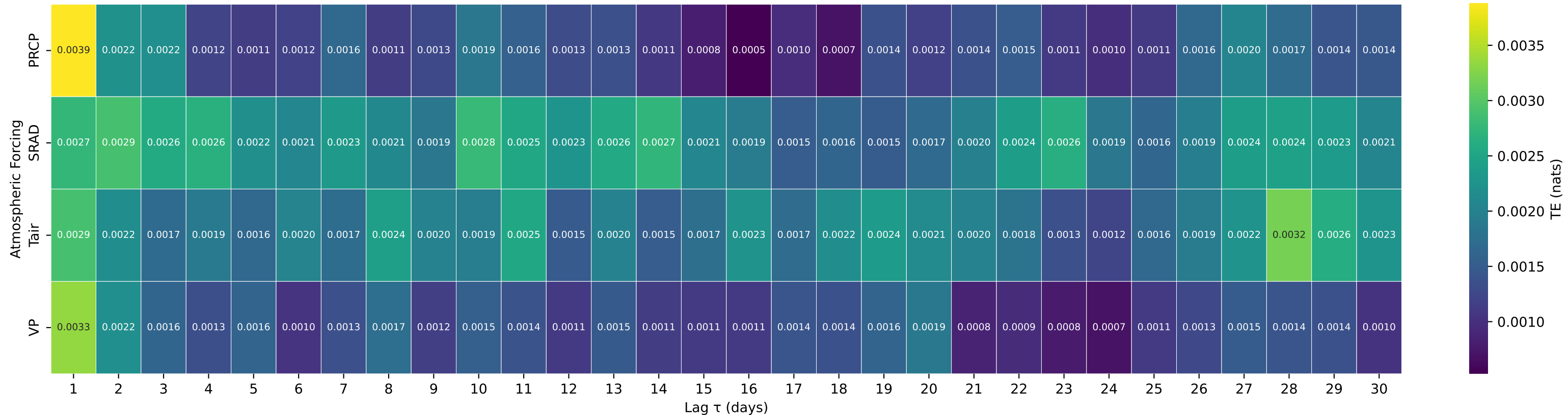
Shuffle-Test Significant TE to Streamflow — Basin 10329500 (HUC 16) — MARTIN C NR PARADISE VALLEY, NV
