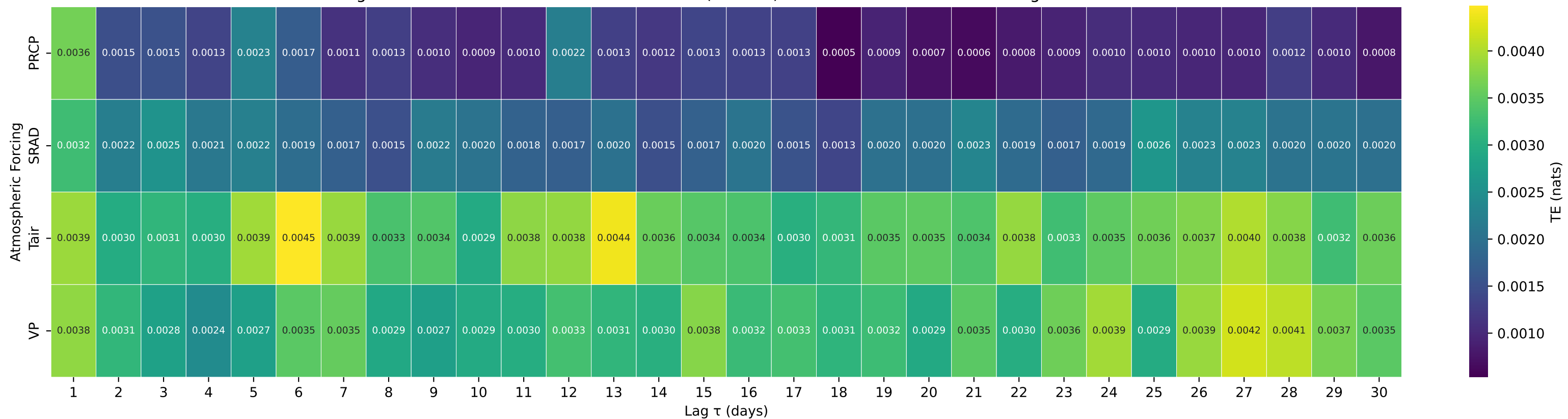
Shuffle-Test Significant TE to Streamflow — Basin 03238500 (HUC 05) — White Oak Creek near Georgetown OH
