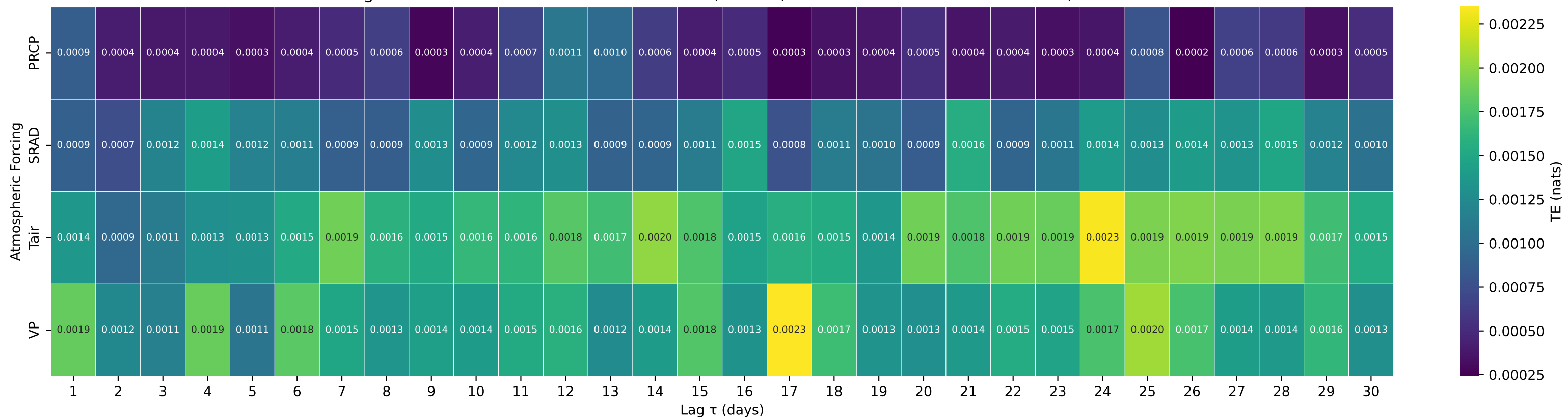
Shuffle-Test Significant TE to Streamflow — Basin 03180500 (HUC 05) — GREENBRIER RIVER AT DURBIN, WV
