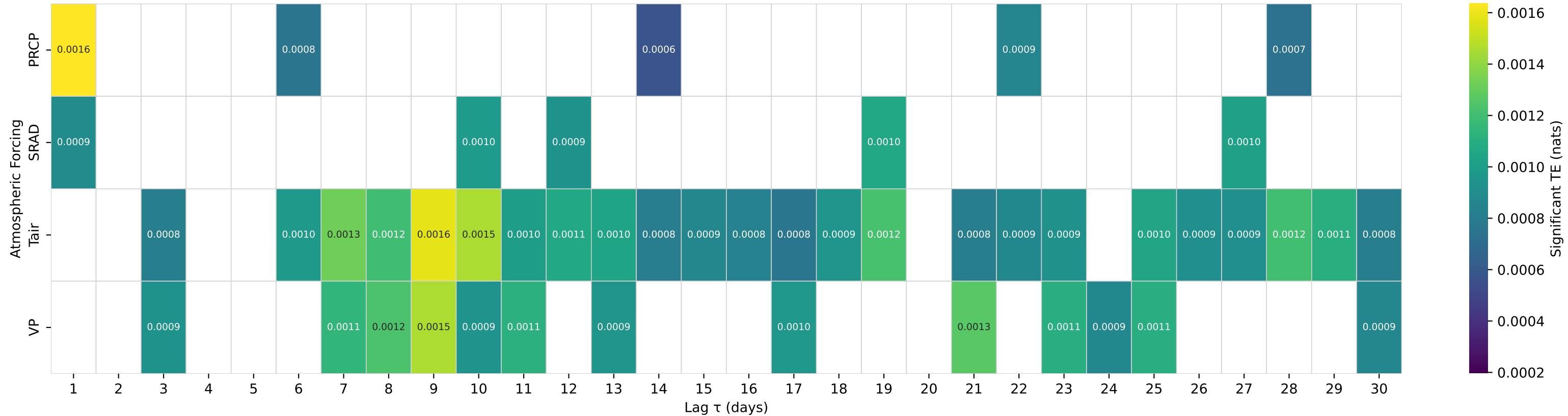
Shuffle-Test Significant TE to Streamflow — Basin 03592718 (HUC 06) — LITTLE YELLOW CREEK EAST NR BURNSVILLE, MS
