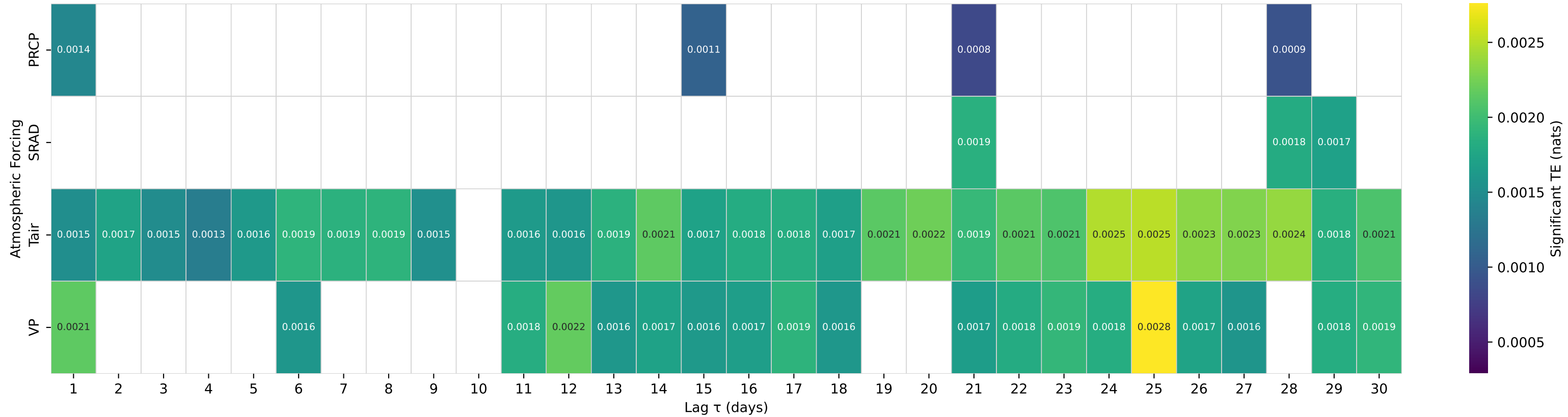
Shuffle-Test Significant TE to Streamflow — Basin 03069500 (HUC 05) — CHEAT RIVER NEAR PARSONS, WV
