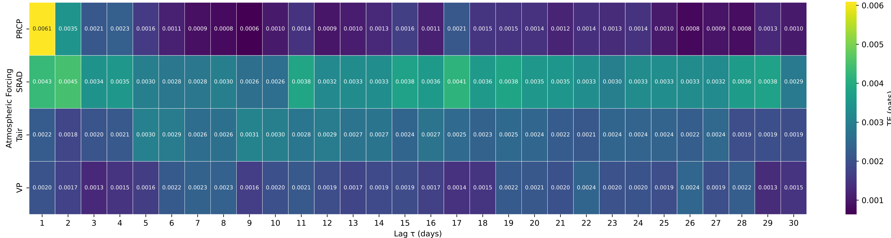
Shuffle-Test Significant TE to Streamflow — Basin 12073500 (HUC 17) — HUGE CREEK NEAR WAUNA, WA
