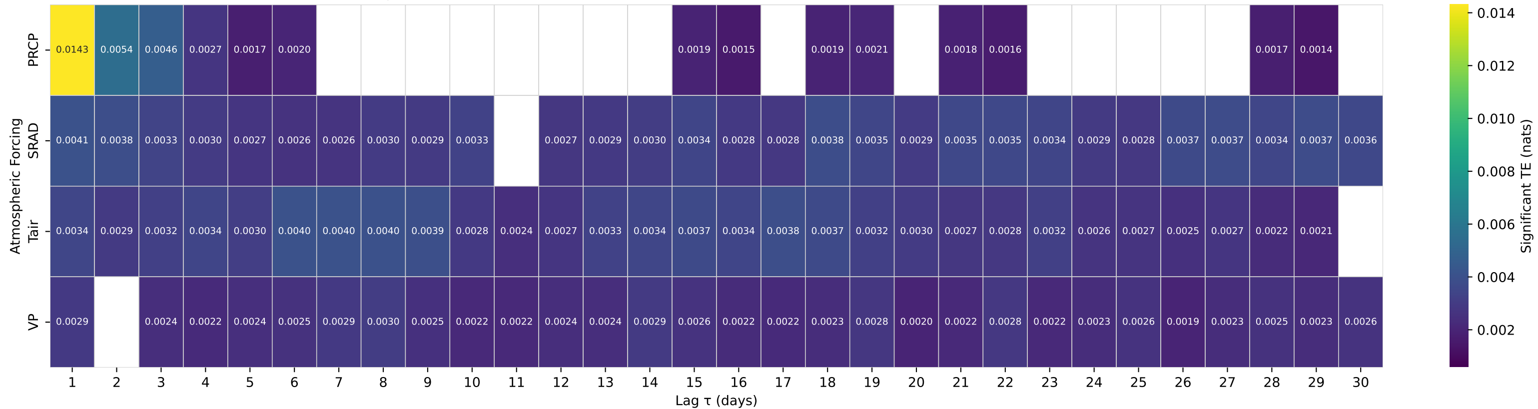
Shuffle-Test Significant TE to Streamflow — Basin 12115000 (HUC 17) — CEDAR RIVER NEAR CEDAR FALLS, WA
