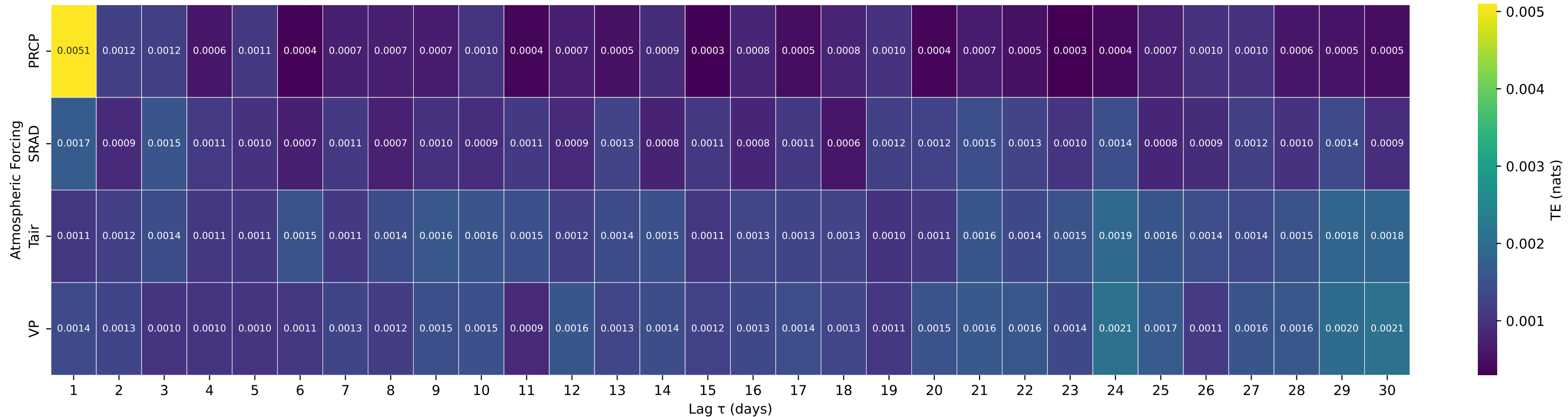
Shuffle-Test Significant TE to Streamflow — Basin 01466500 (HUC 02) — MCDONALDS BRANCH IN LEBANON STATE FOREST NJ
