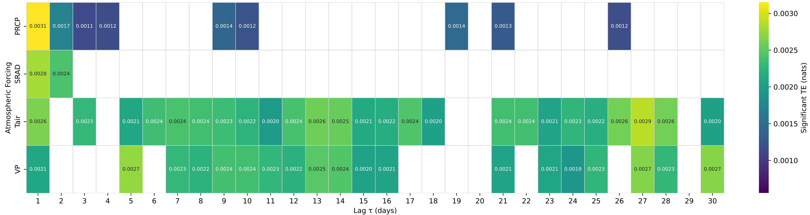
Shuffle-Test Significant TE to Streamflow — Basin 01568000 (HUC 02) — Sherman Creek at Shermans Dale, PA
