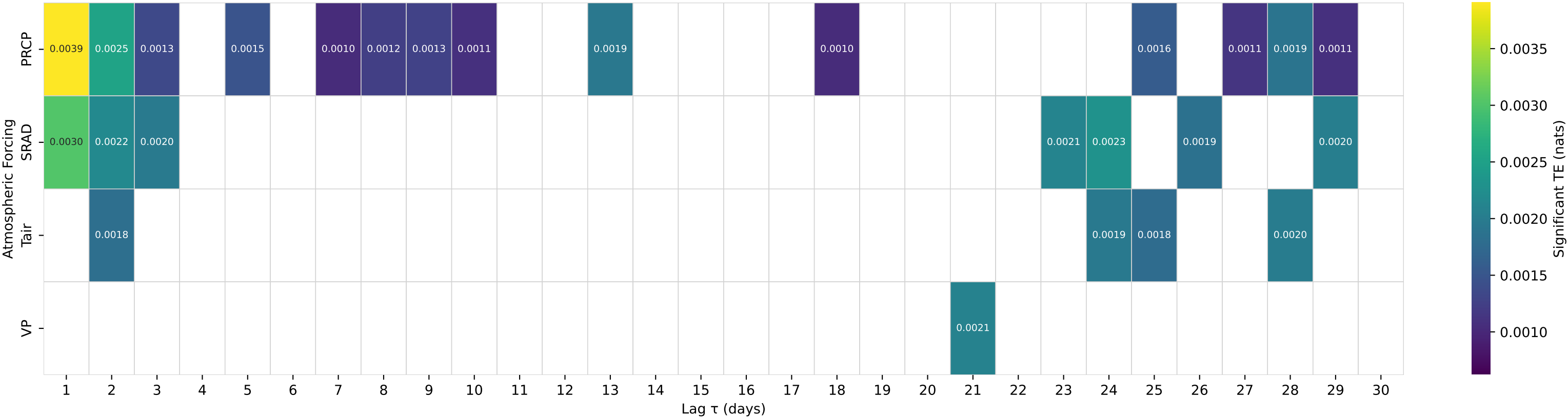
Original TE to Streamflow — Basin 02315500 (HUC 03) — SUWANNEE RIVER AT WHITE SPRINGS, FLA. Heatmap showing the relationship between atmospheric forcing (PRCP, SRAD, Tair, VP) and streamflow (TE) over a 30-day lag. The color scale ranges from 0.0010 (dark purple) to 0.0035 (yellow). Atmospheric Forcing 1 2 3 4 5 6 7 8 9 10 11 12 13 14 15 16 17 18 19 20 21 22 23 24 25 26 27 28 29 30 PRCP 0.0039 0.0025 0.0013 0.0010 0.0015 0.0010 0.0010 0.0012 0.0013 0.0011 0.0009 0.0009 0.0019 0.0010 0.0009 0.0009 0.0011 0.0010 0.0009 0.0006 0.0010 0.0009 0.0006 0.0009 0.0016 0.0009 0.0011 0.0019 0.0011 0.0008 SRAD 0.0030 0.0022 0.0020 0.0014 0.0012 0.0009 0.0015 0.0011 0.0015 0.0016 0.0018 0.0014 0.0020 0.0015 0.0011 0.0014 0.0016 0.0018 0.0015 0.0015 0.0017 0.0016 0.0021 0.0023 0.0017 0.0019 0.0019 0.0019 0.0020 0.0012 Tair 0.0012 0.0018 0.0013 0.0014 0.0017 0.0015 0.0015 0.0011 0.0010 0.0014 0.0011 0.0017 0.0016 0.0017 0.0014 0.0014 0.0014 0.0011 0.0012 0.0015 0.0016 0.0017 0.0017 0.0019 0.0018 0.0017 0.0017 0.0020 0.0016 0.0016 VP 0.0021 0.0020 0.0018 0.0014 0.0015 0.0016 0.0015 0.0013 0.0013 0.0013 0.0015 0.0017 0.0016 0.0016 0.0016 0.0017 0.0016 0.0015 0.0016 0.0013 0.0021 0.0021 0.0019 0.0014 0.0016 0.0017 0.0015 0.0021 0.0019 0.0019
