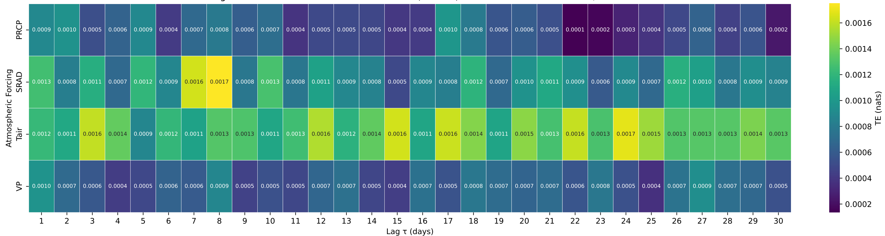
Shuffle-Test Significant TE to Streamflow — Basin 09386900 (HUC 15) — RIO NUTRIA NEAR RAMAH, NM
