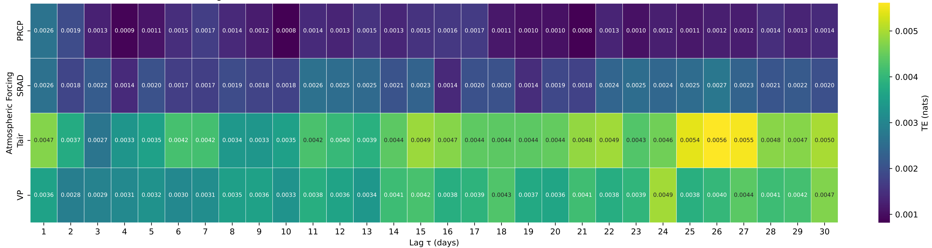
Shuffle-Test Significant TE to Streamflow — Basin 03070500 (HUC 05) — BIG SANDY CREEK AT ROCKVILLE, WV
