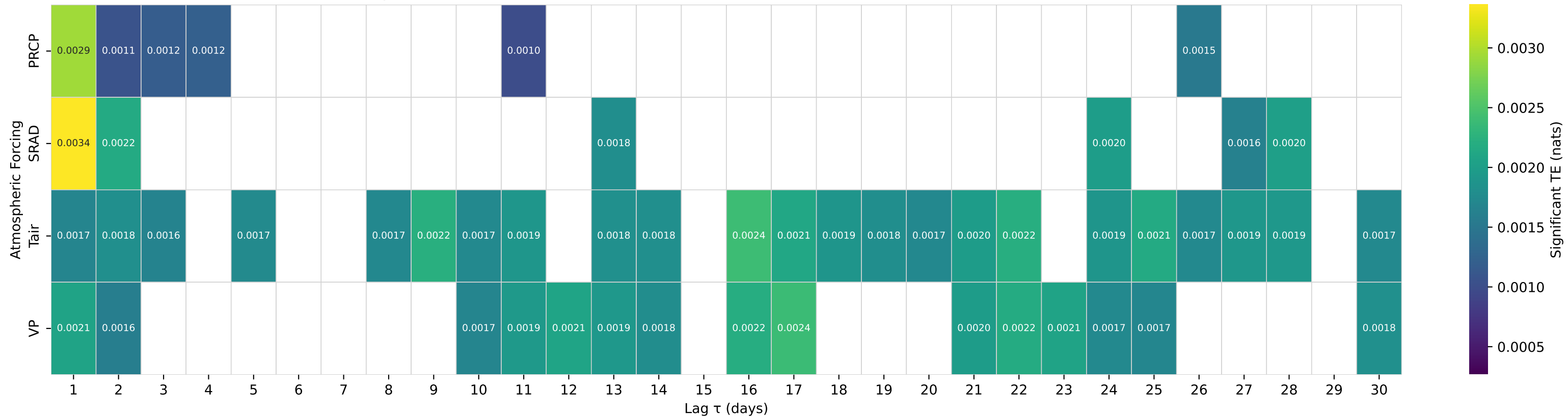
Shuffle-Test Significant TE to Streamflow — Basin 07263295 (HUC 11) — Maumelle River at Williams Junction, AR
