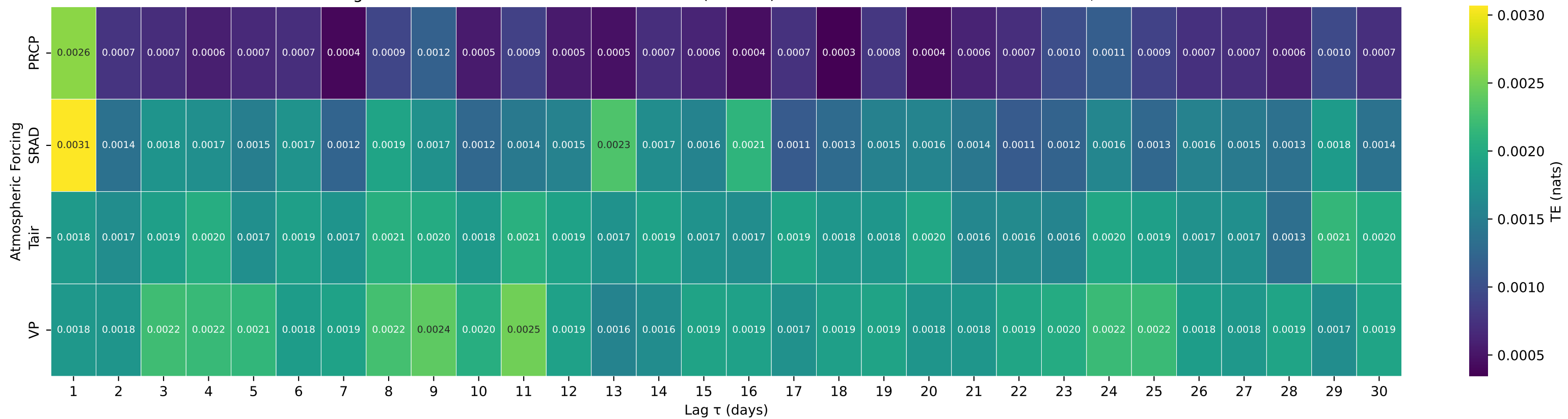
Shuffle-Test Significant TE to Streamflow — Basin 03439000 (HUC 06) — FRENCH BROAD RIVER AT ROSMAN, NC
