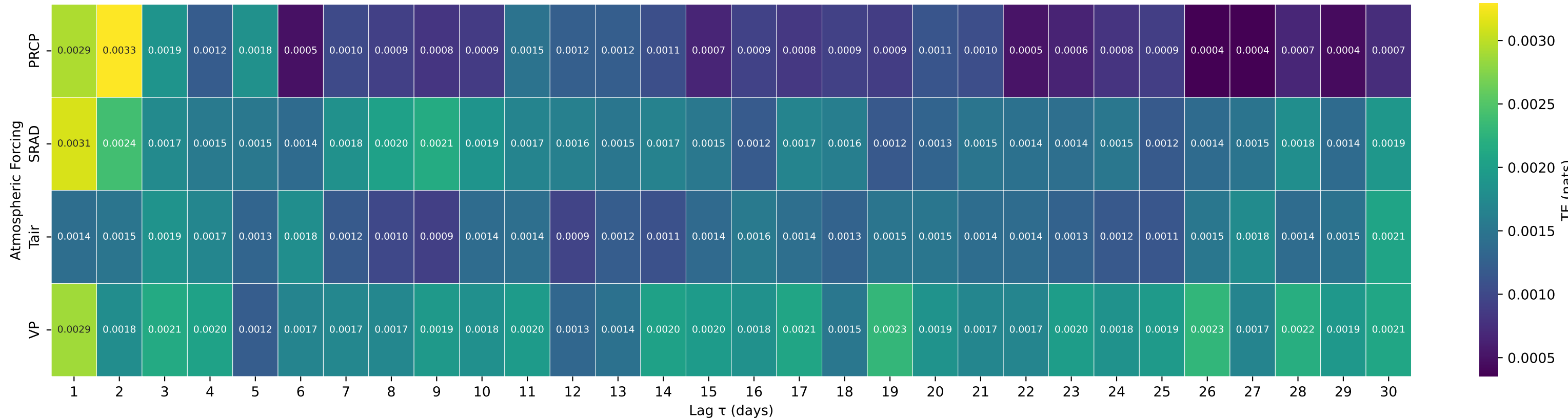
Shuffle-Test Significant TE to Streamflow — Basin 08158700 (HUC 12) — Onion Ck nr Driftwood, TX
