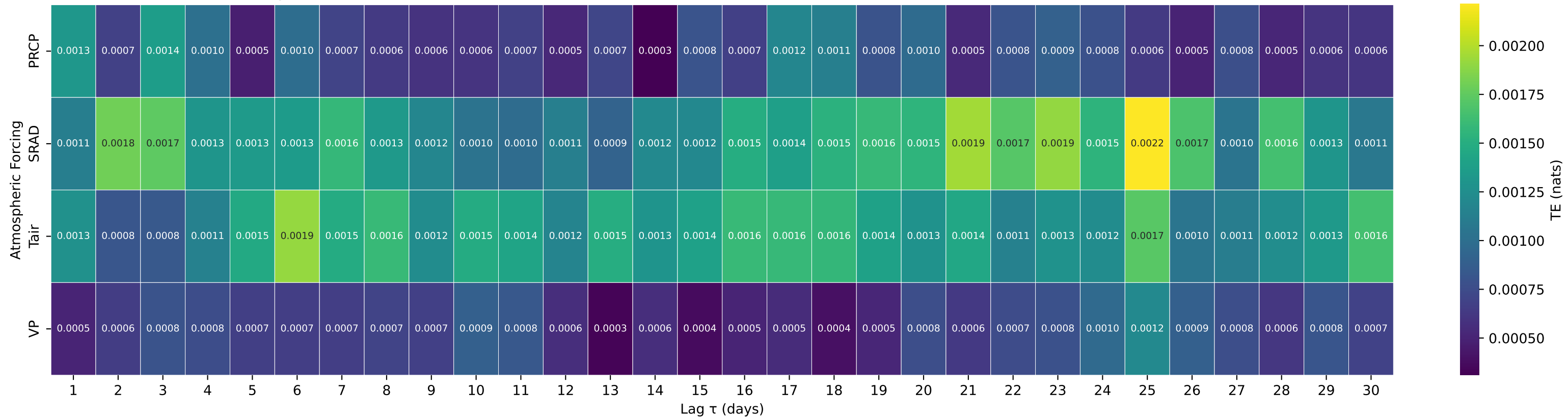
Shuffle-Test Significant TE to Streamflow — Basin 06468250 (HUC 10) — JAMES RIVER ABOVE ARROWWOOD LAKE NR KENSAL, ND
