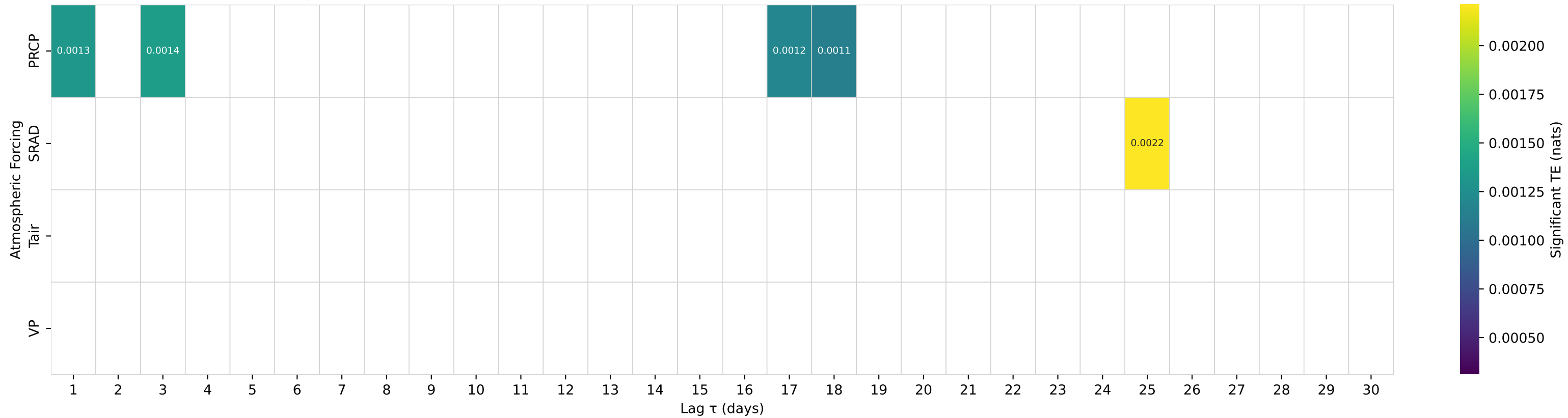
Shuffle-Test Significant TE to Streamflow — Basin 06468250 (HUC 10) — JAMES RIVER ABOVE ARROWWOOD LAKE NR KENSAL, ND
