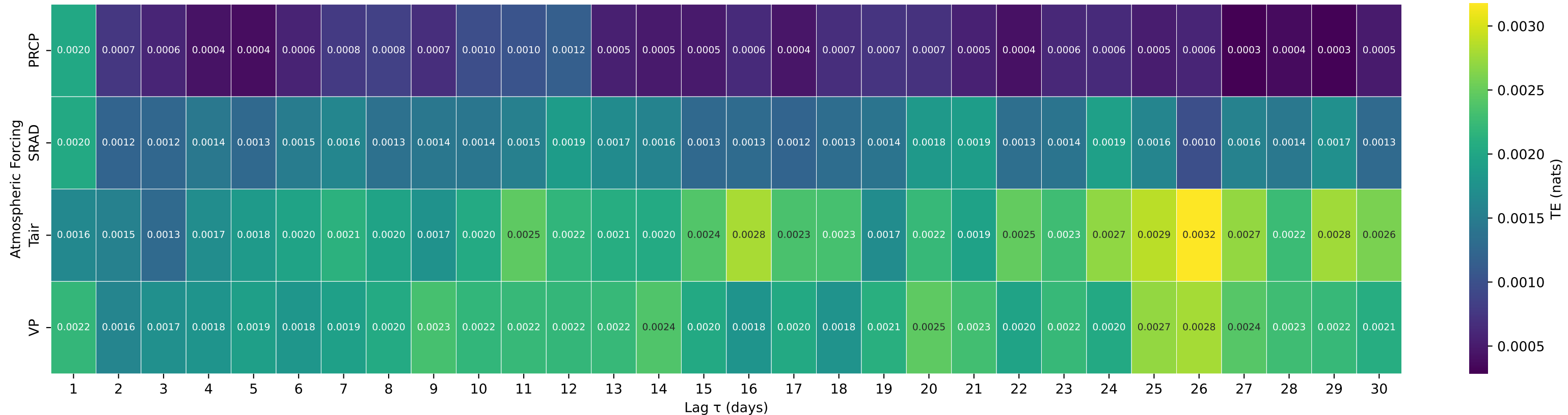
Shuffle-Test Significant TE to Streamflow — Basin 02013000 (HUC 02) — DUNLAP CREEK NEAR COVINGTON, VA
