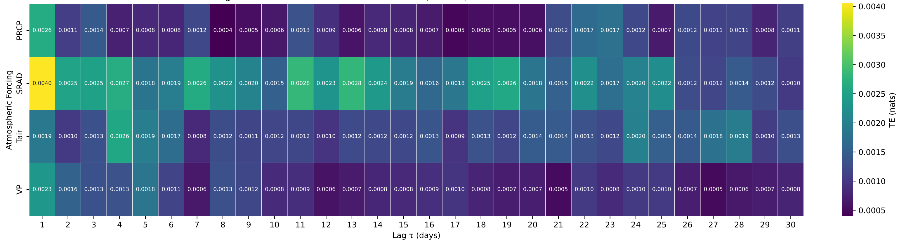
Shuffle-Test Significant TE to Streamflow — Basin 11237500 (HUC 18) — PITMAN C BL TAMARACK C CA
