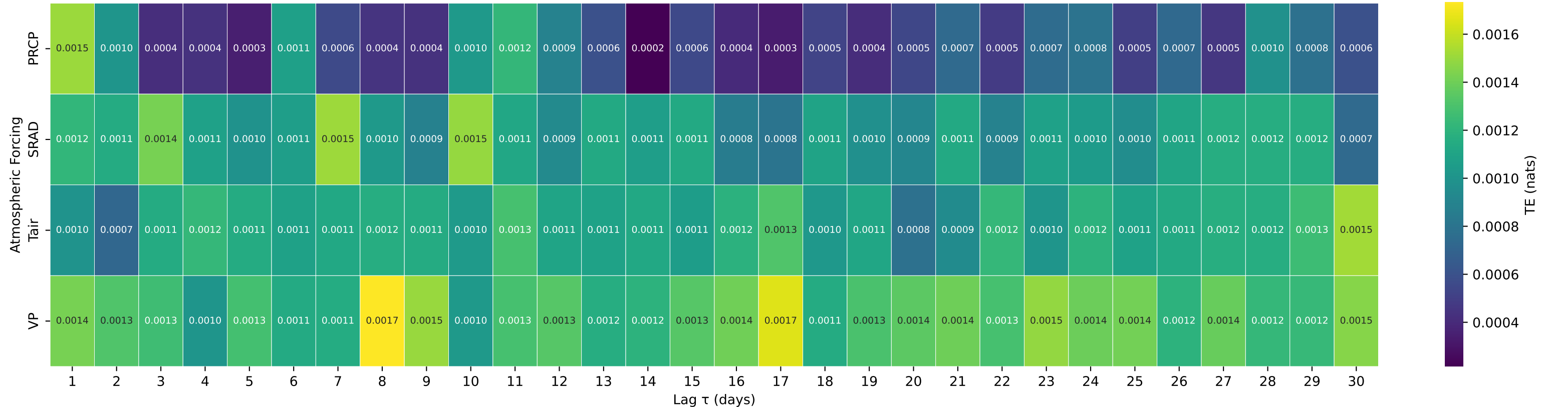
Shuffle-Test Significant TE to Streamflow — Basin 02074500 (HUC 03) — SANDY RIVER NEAR DANVILLE, VA
