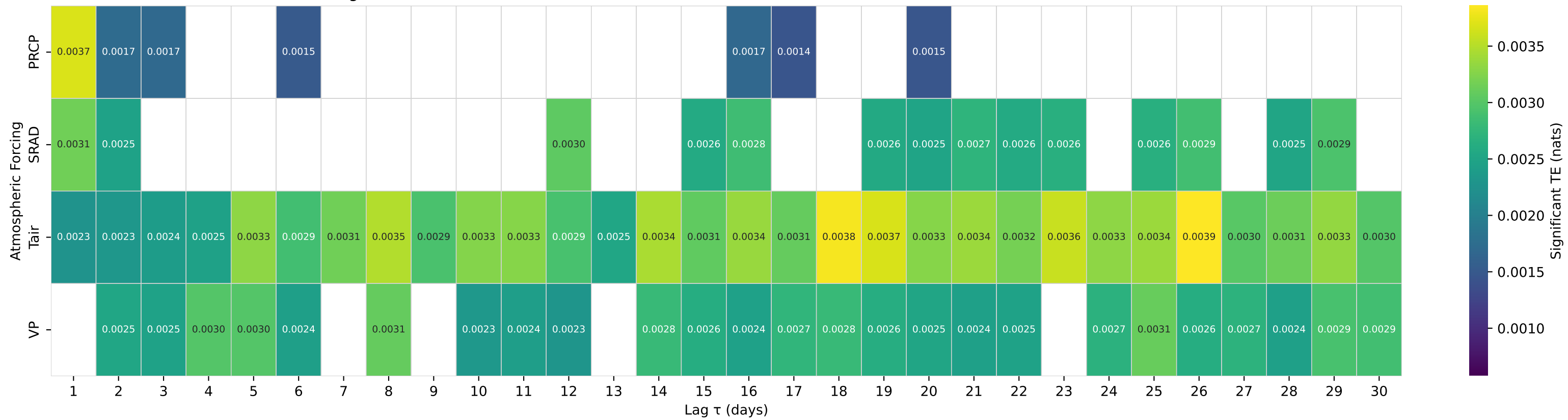
Shuffle-Test Significant TE to Streamflow — Basin 03460000 (HUC 06) — CATALOOCHEE CREEK NEAR CATALOOCHEE, NC
