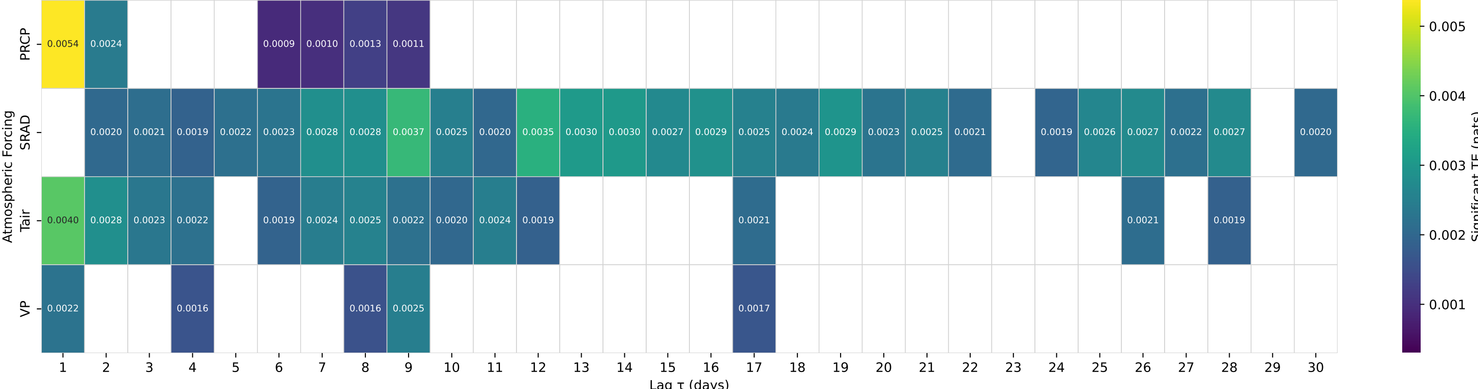
Shuffle-Test Significant TE to Streamflow — Basin 04063700 (HUC 04) — POPPLE RIVER NEAR FENCE, WI
