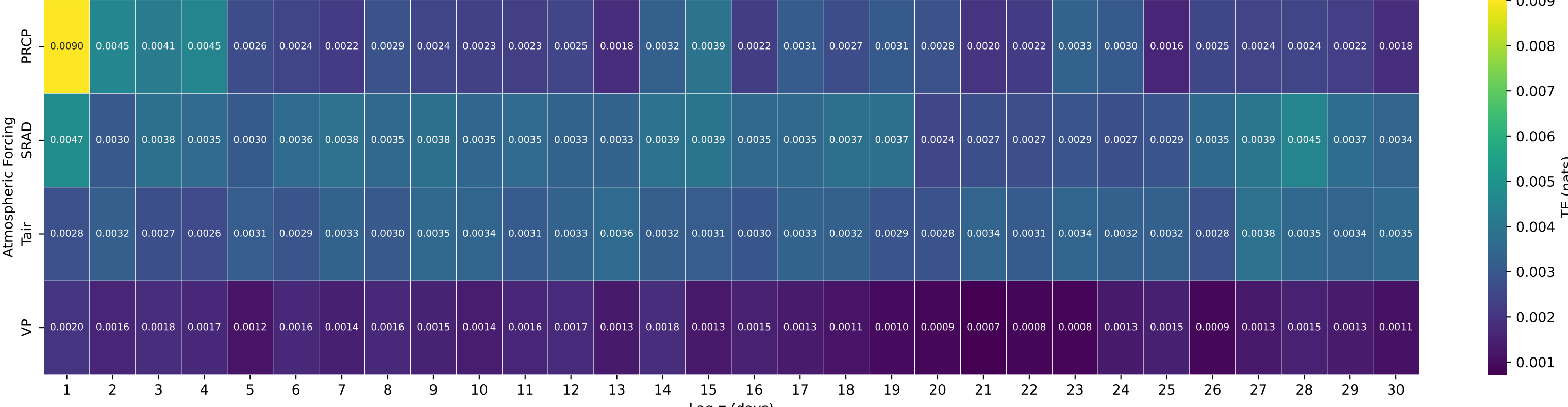
Shuffle-Test Significant TE to Streamflow — Basin 11528700 (HUC 18) — SF TRINITY R BL HYAMPOM CA
