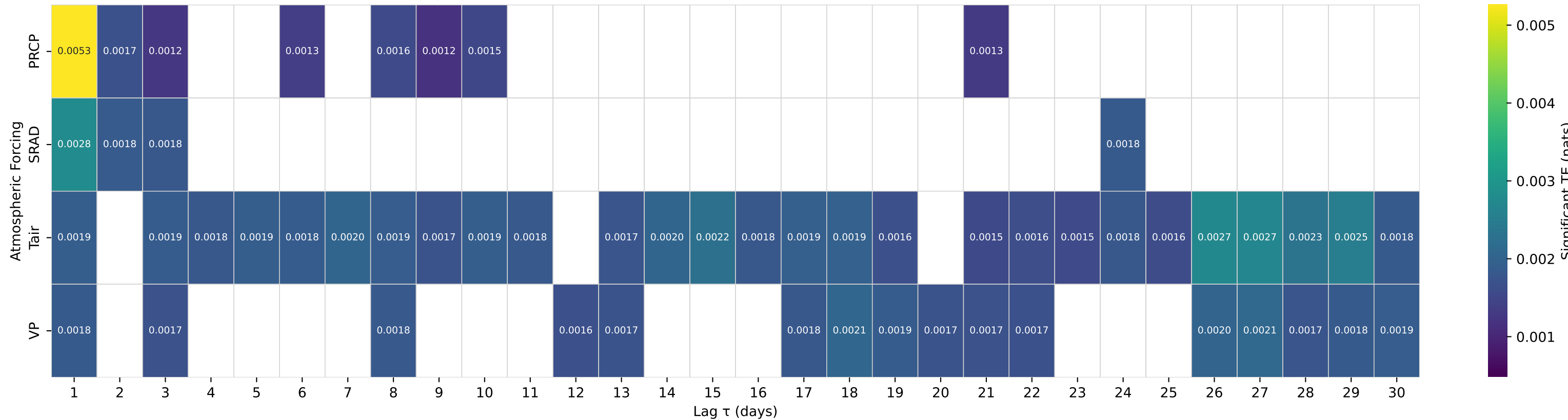
Shuffle-Test Significant TE to Streamflow — Basin 03173000 (HUC 05) — WALKER CREEK AT BANE, VA
