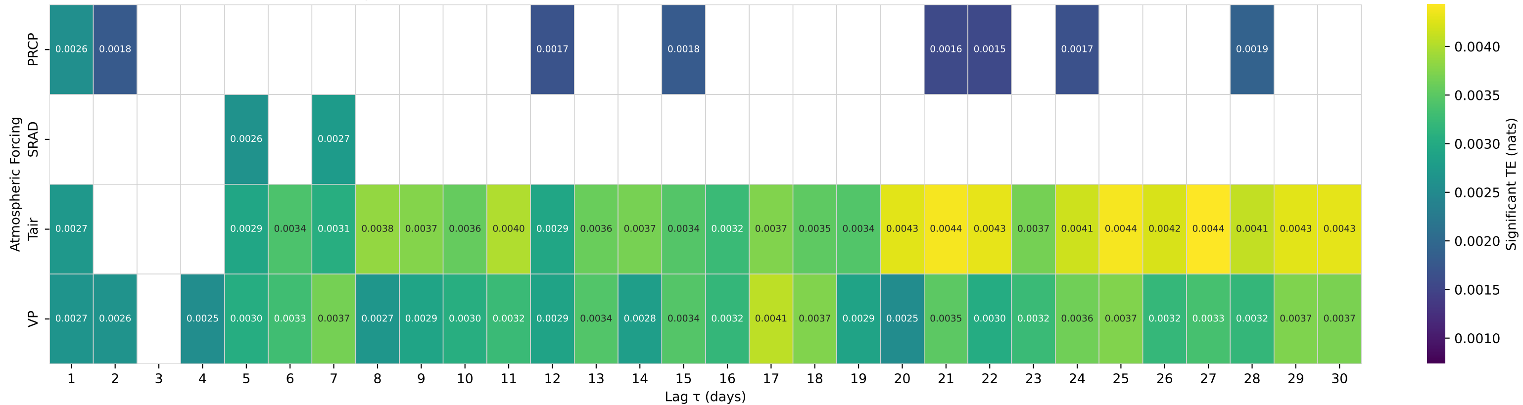
Shuffle-Test Significant TE to Streamflow — Basin 01594950 (HUC 02) — MCMILLAN F NEAR FORT PENDLETON, MD
