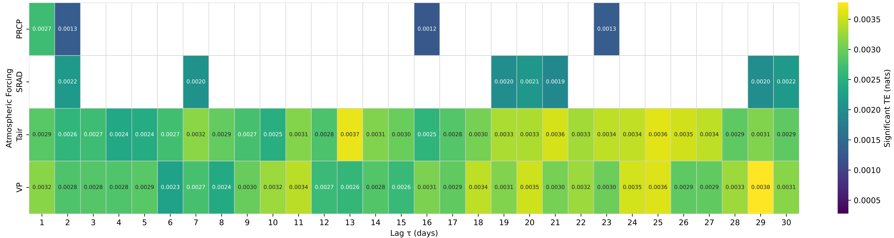
Shuffle-Test Significant TE to Streamflow — Basin 03187500 (HUC 05) — CRANBERRY RIVER NEAR RICHWOOD, WV
