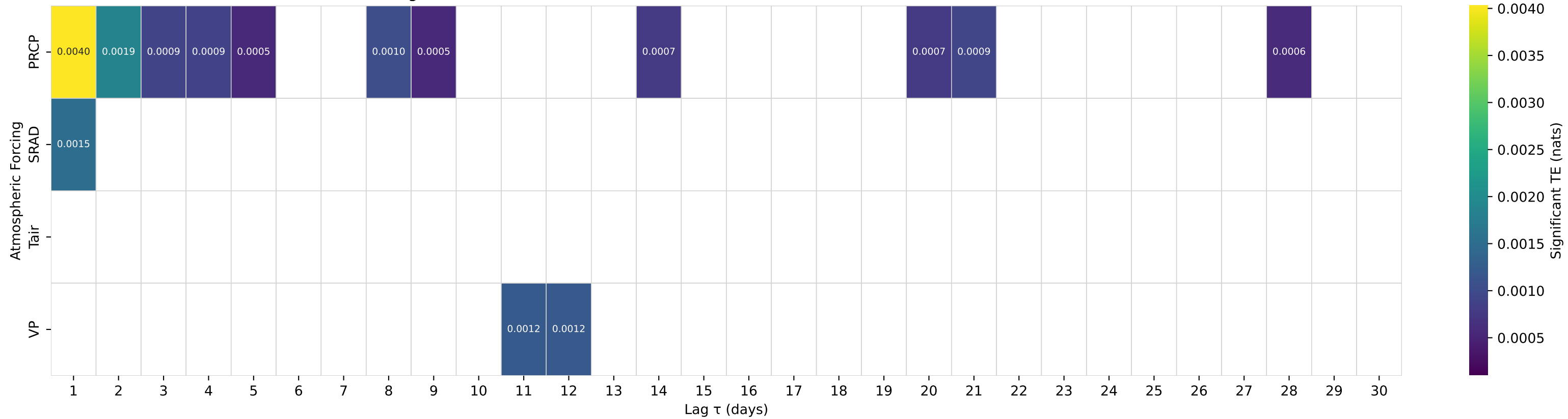
Shuffle-Test Significant TE to Streamflow — Basin 01669520 (HUC 02) — DRAGON SWAMP AT MASCOT, VA
