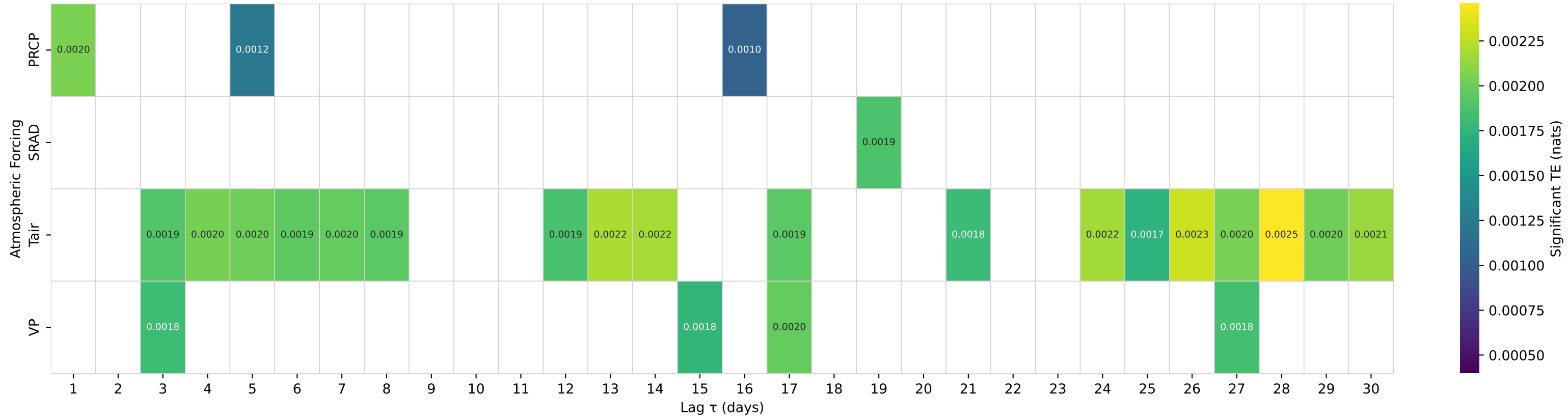
Shuffle-Test Significant TE to Streamflow — Basin 01586610 (HUC 02) — MORGAN RUN NEAR LOUISVILLE, MD
