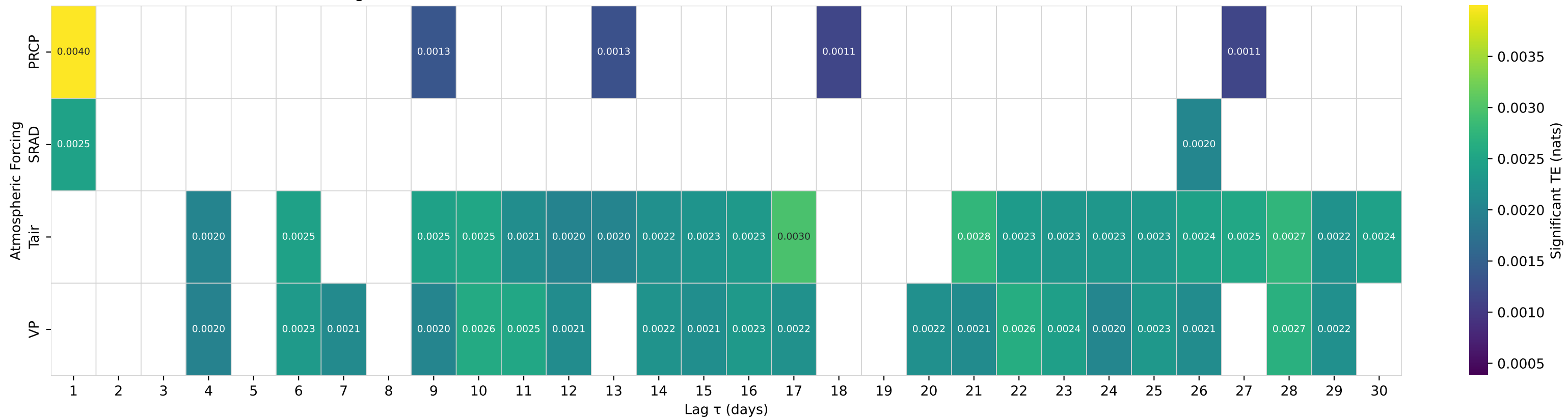
Shuffle-Test Significant TE to Streamflow — Basin 01486000 (HUC 02) — MANOKIN BRANCH NEAR PRINCESS ANNE, MD
