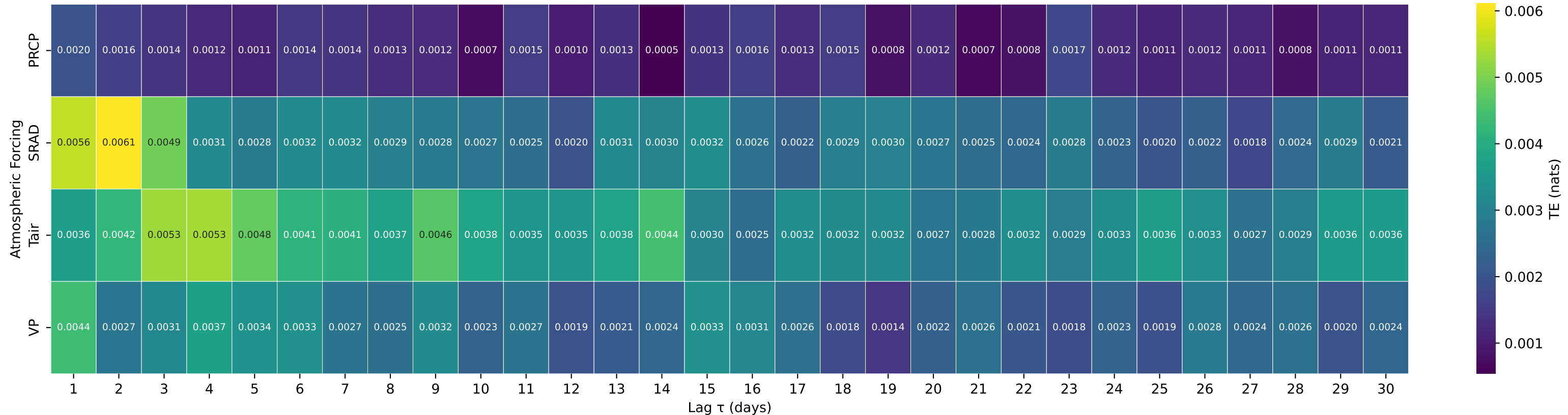
Shuffle-Test Significant TE to Streamflow — Basin 09066000 (HUC 14) — BLACK GORE CREEK NEAR MINTURN, CO.
