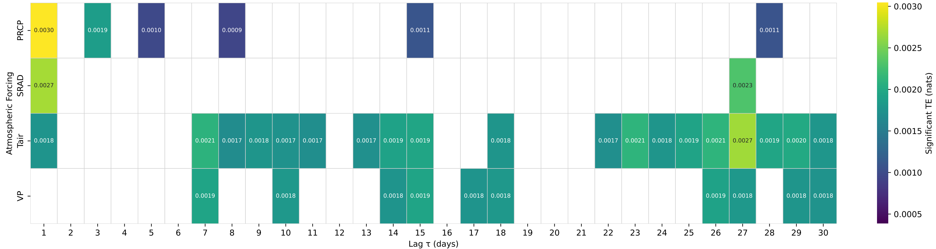
Shuffle-Test Significant TE to Streamflow — Basin 03357350 (HUC 05) — PLUM CREEK NEAR BAINBRIDGE, IND.
