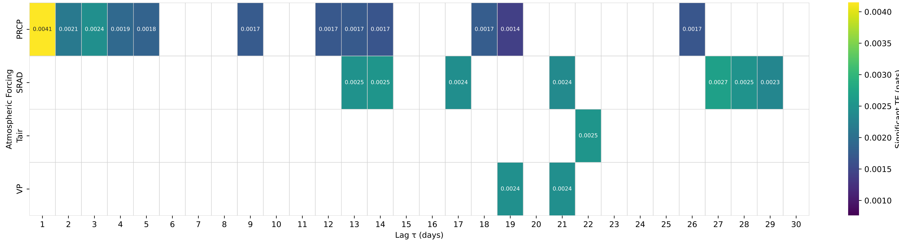
Shuffle-Test Significant TE to Streamflow — Basin 06453600 (HUC 10) — PONCA CREEK AT VERDEL, NEBR.
