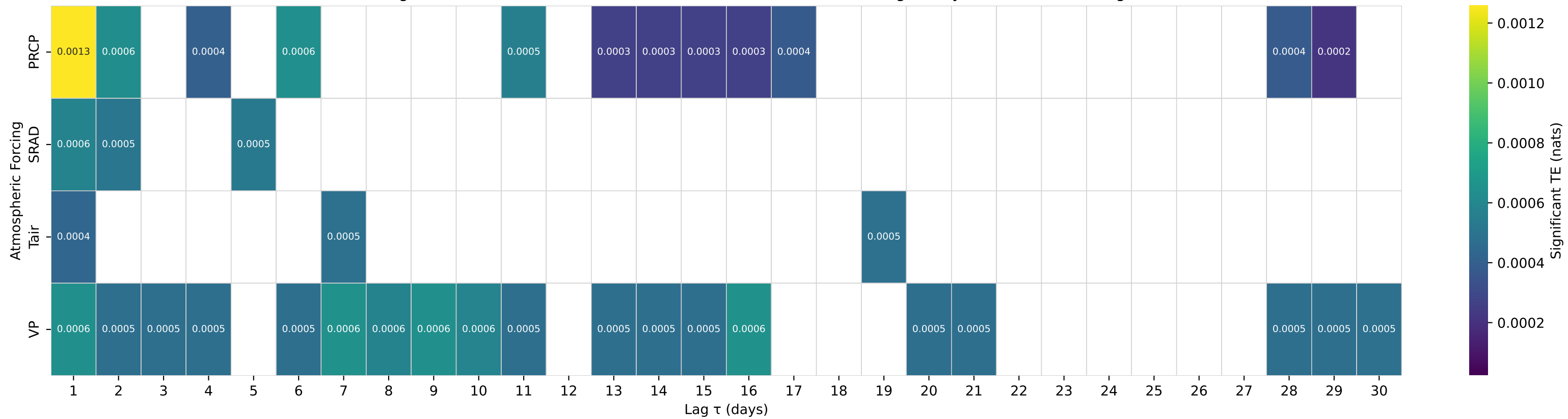
Shuffle-Test Significant TE to Streamflow — Basin 08086290 (HUC 12) — Big Sandy Ck abv Breckenridge, TX
