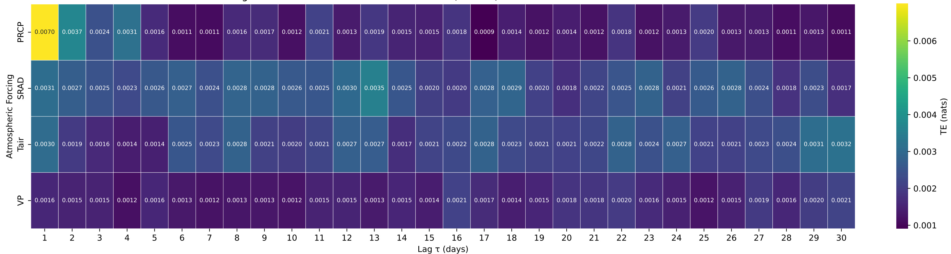
Shuffle-Test Significant TE to Streamflow — Basin 06464500 (HUC 10) — KEYA PAHA R AT WEWELA SD
