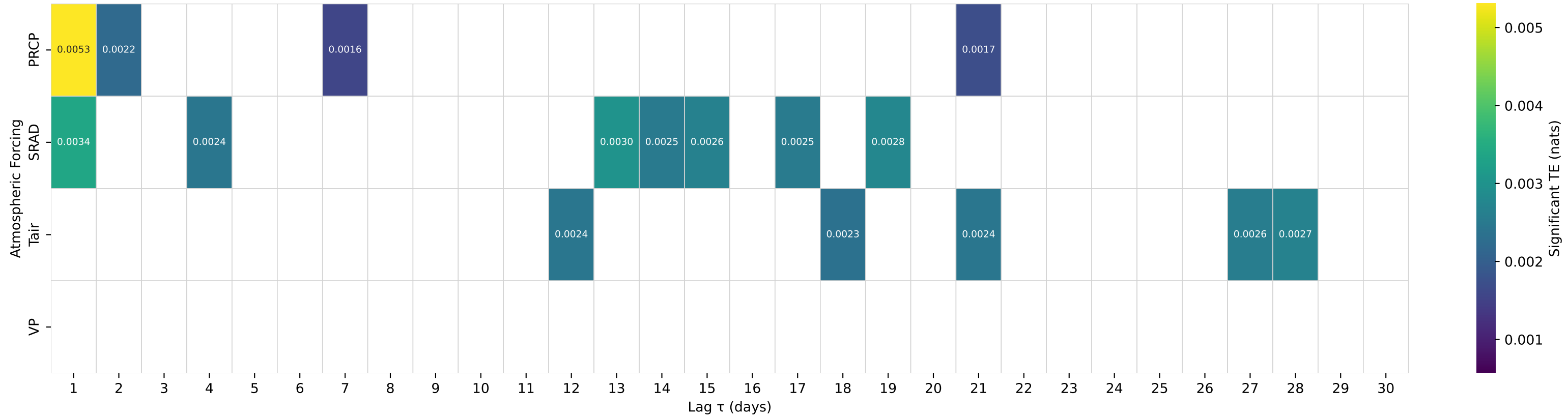
Shuffle-Test Significant TE to Streamflow — Basin 05593575 (HUC 07) — LITTLE CROOKED CREEK NEAR NEW MINDEN, IL
