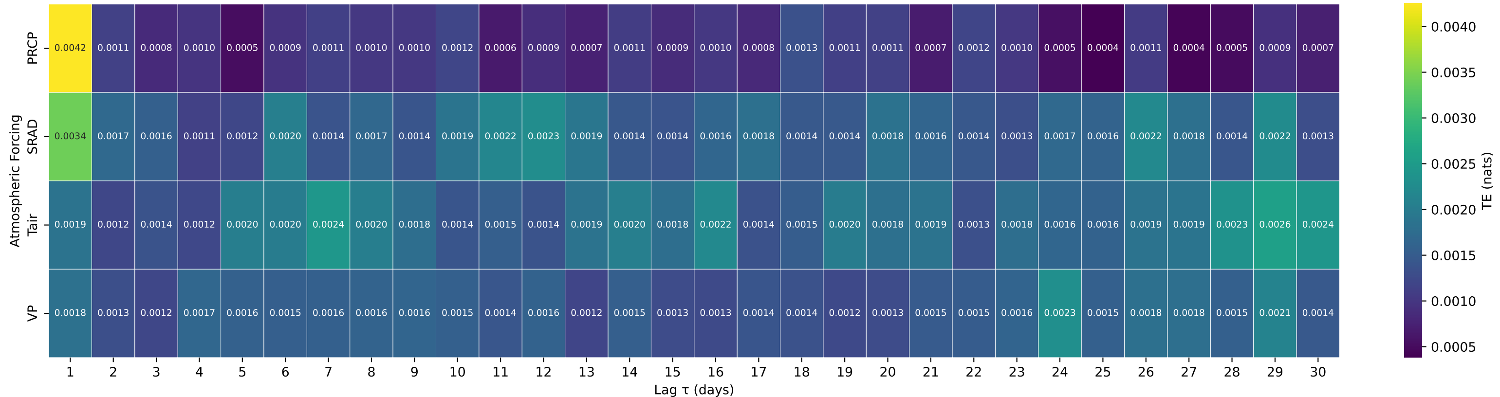
Shuffle-Test Significant TE to Streamflow — Basin 05592050 (HUC 07) — ROBINSON CREEK NEAR SHELBYVILLE, IL
