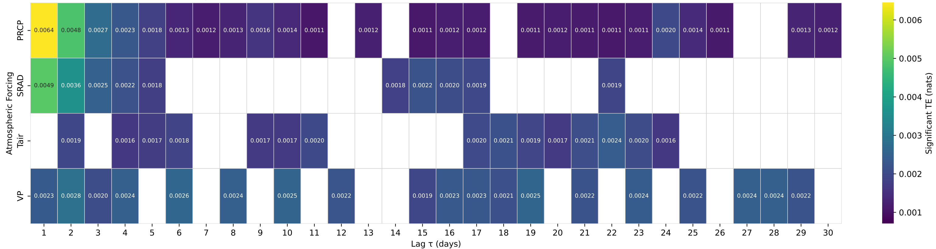
Shuffle-Test Significant TE to Streamflow — Basin 02310947 (HUC 03) — WITHLACOOCHEE RIVER NEAR CUMPRESSCO, FLA.
