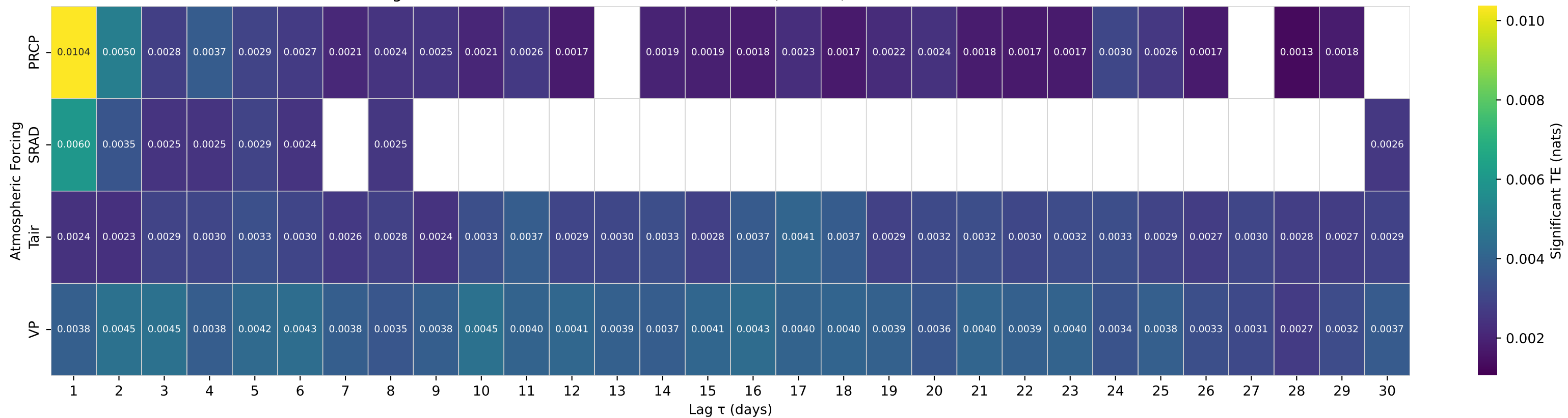
Shuffle-Test Significant TE to Streamflow — Basin 02298123 (HUC 03) — PRAIRIE CREEK NEAR FORT OGDEN FL
