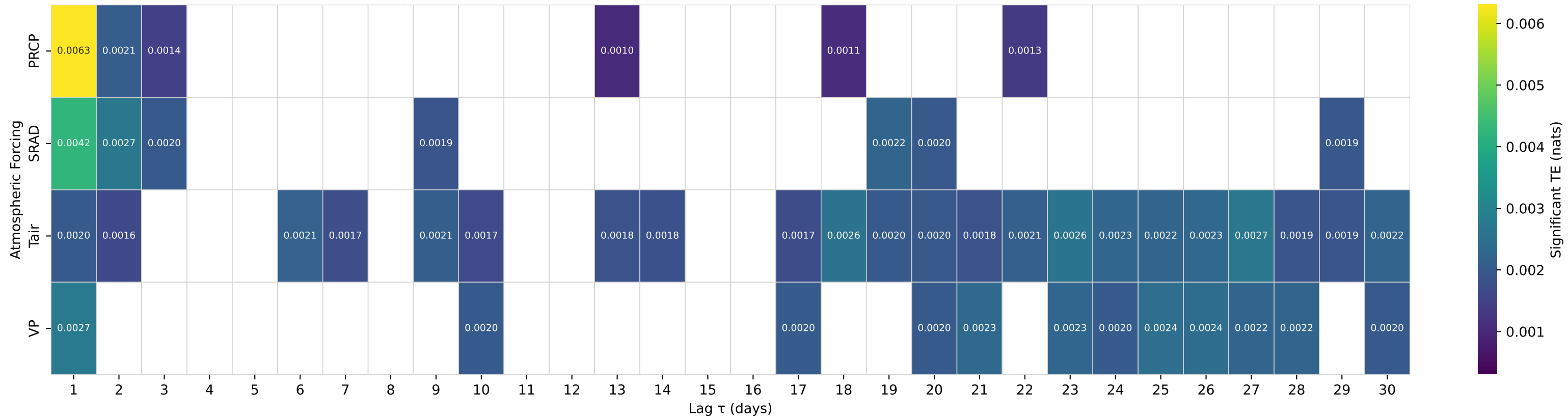
Shuffle-Test Significant TE to Streamflow — Basin 02472500 (HUC 03) — BOUIE CREEK NR HATTIESBURG, MS
