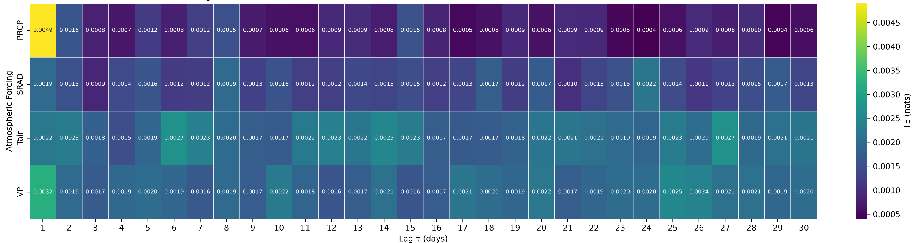
Shuffle-Test Significant TE to Streamflow — Basin 03366500 (HUC 05) — MUSCATATUCK RIVER NEAR DEPUTY, IN
