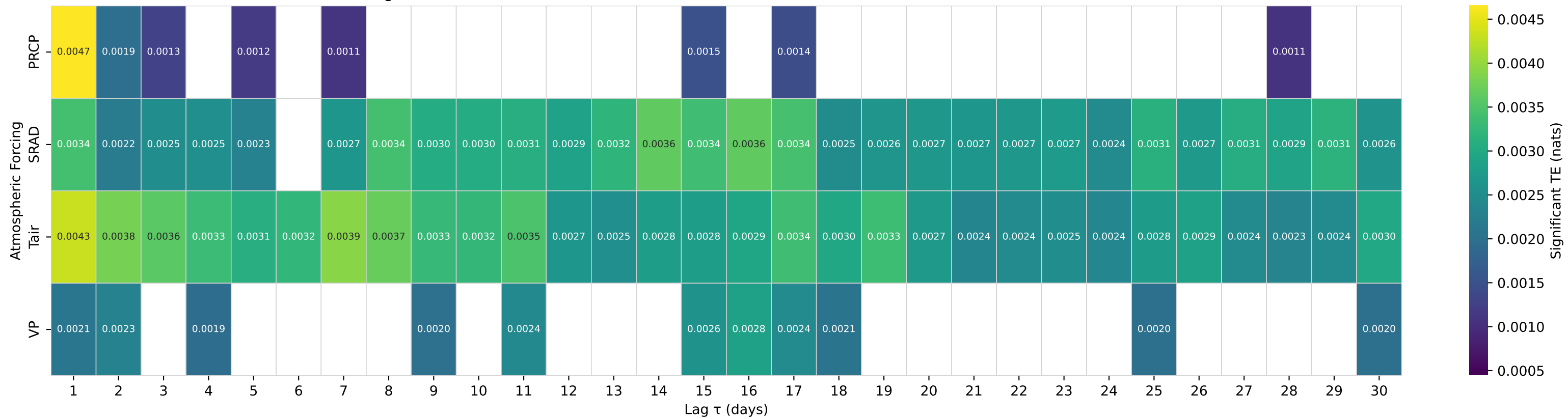
Shuffle-Test Significant TE to Streamflow — Basin 05129115 (HUC 09) — VERMILION RIVER NR CRANE LAKE, MN
