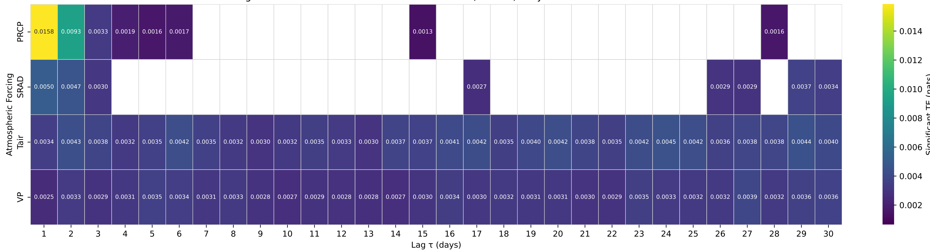
Shuffle-Test Significant TE to Streamflow — Basin 04196800 (HUC 04) — Tymochtee Creek at Crawford OH
