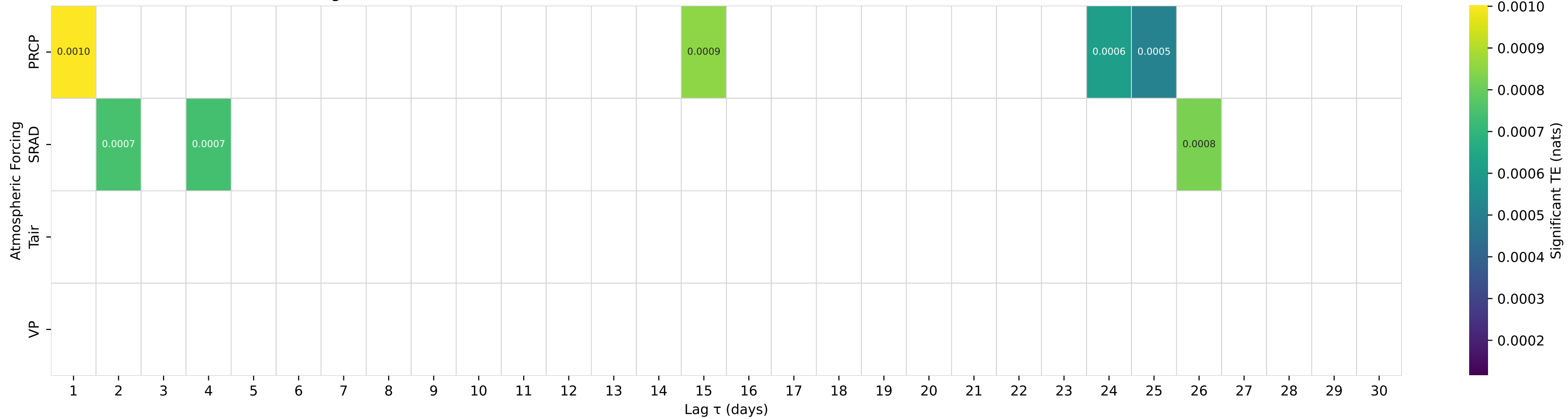
Shuffle-Test Significant TE to Streamflow — Basin 01606500 (HUC 02) — SO. BRANCH POTOMAC RIVER NR PETERSBURG, WV
