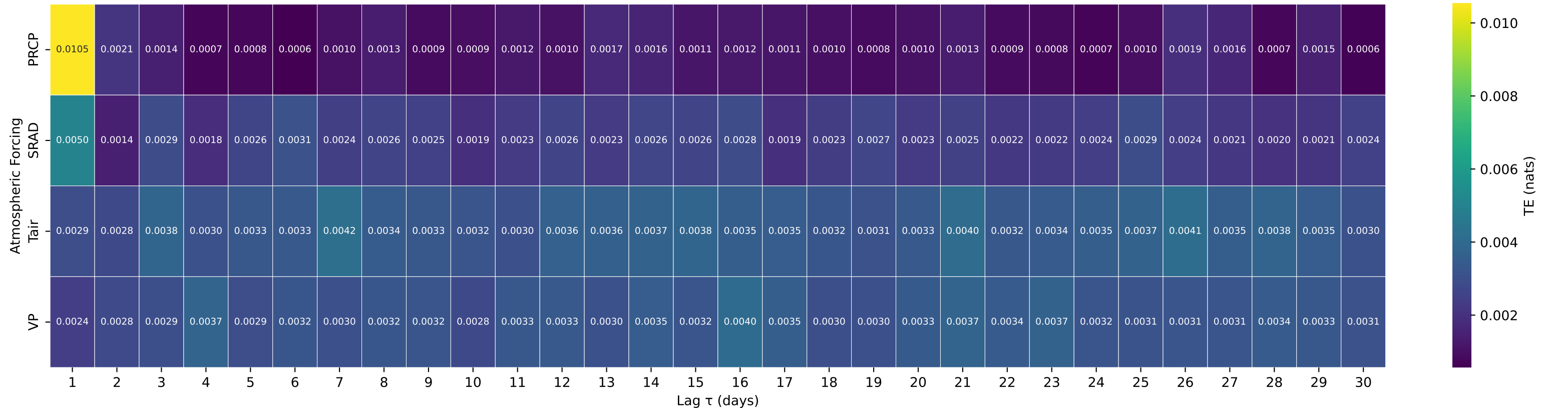
Shuffle-Test Significant TE to Streamflow — Basin 01487000 (HUC 02) — NANTICOKE RIVER NEAR BRIDGEVILLE, DE
