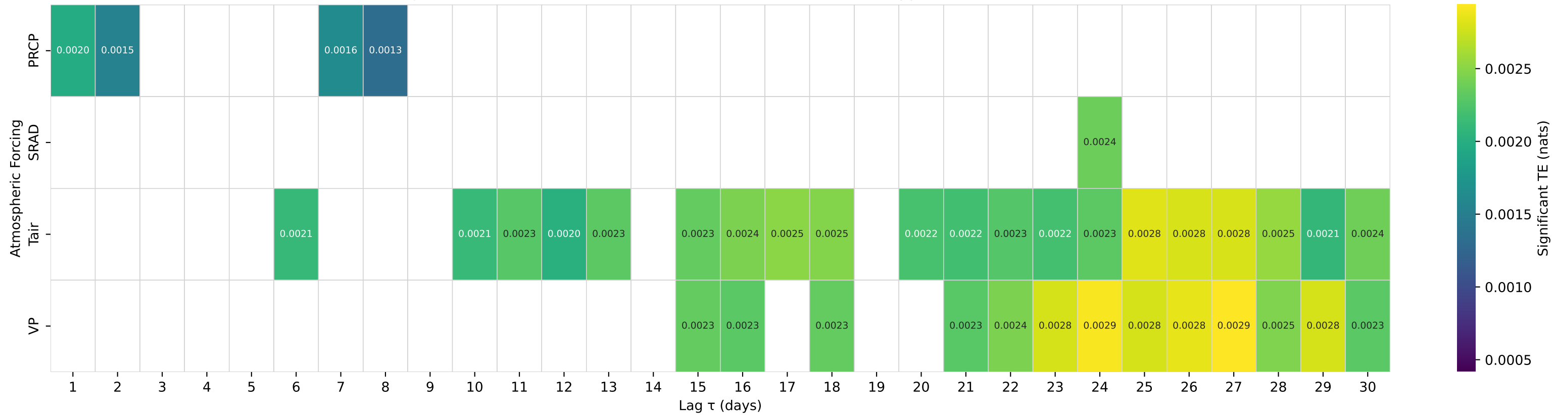
Shuffle-Test Significant TE to Streamflow — Basin 03237280 (HUC 05) — Upper Twin Creek at McGaw OH
