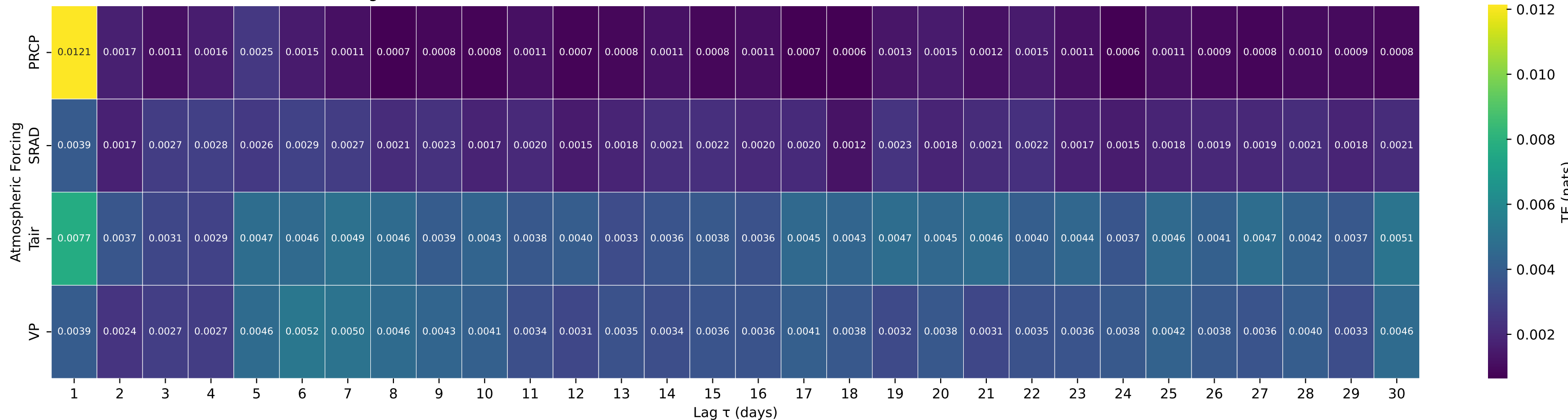
Shuffle-Test Significant TE to Streamflow — Basin 04124000 (HUC 04) — MANISTEE RIVER NEAR SHERMAN, MI
