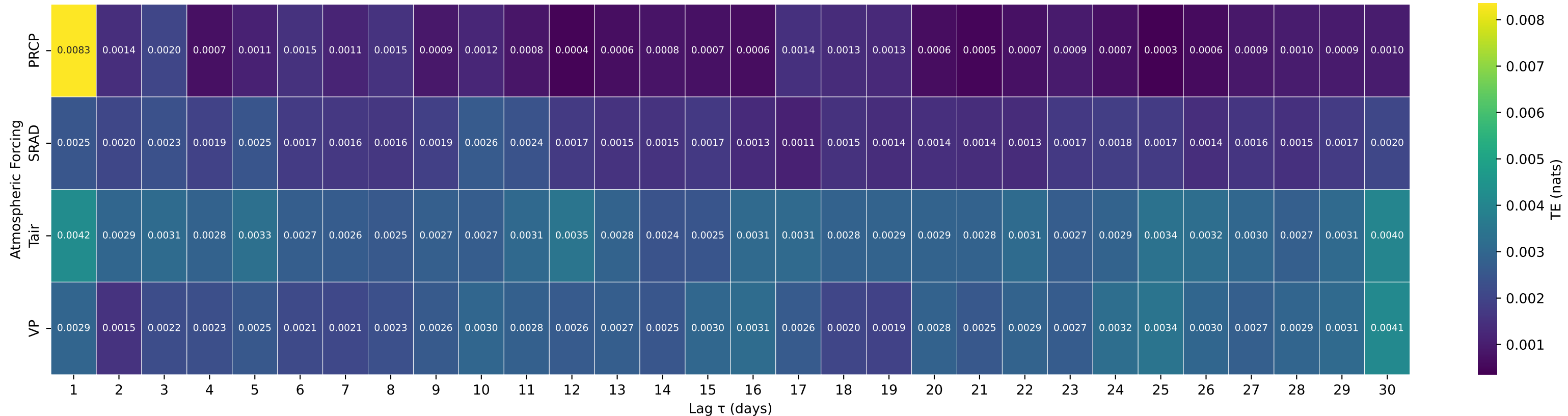
Shuffle-Test Significant TE to Streamflow — Basin 01162500 (HUC 01) — PRIEST BROOK NEAR WINCHENDON, MA
