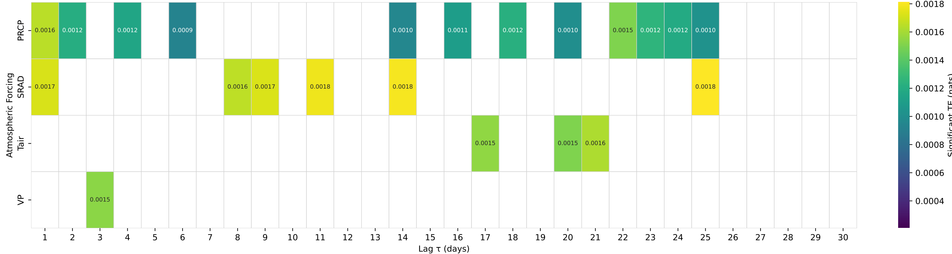
Shuffle-Test Significant TE to Streamflow — Basin 07195800 (HUC 11) — Flint Creek at Springtown, AR
