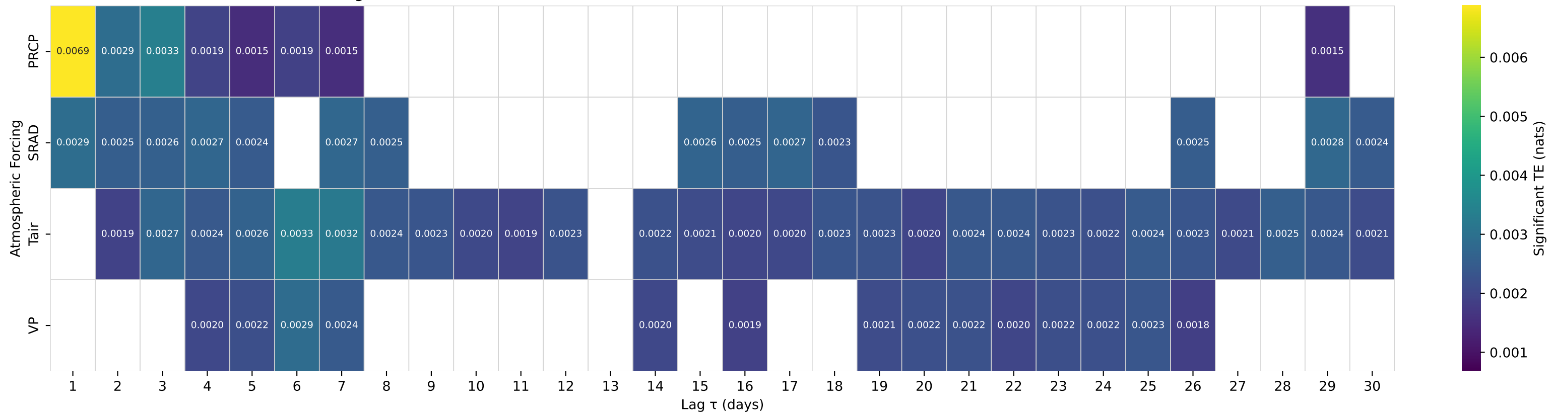
Shuffle-Test Significant TE to Streamflow — Basin 12095000 (HUC 17) — SOUTH PRAIRIE CREEK AT SOUTH PRAIRIE, WA
