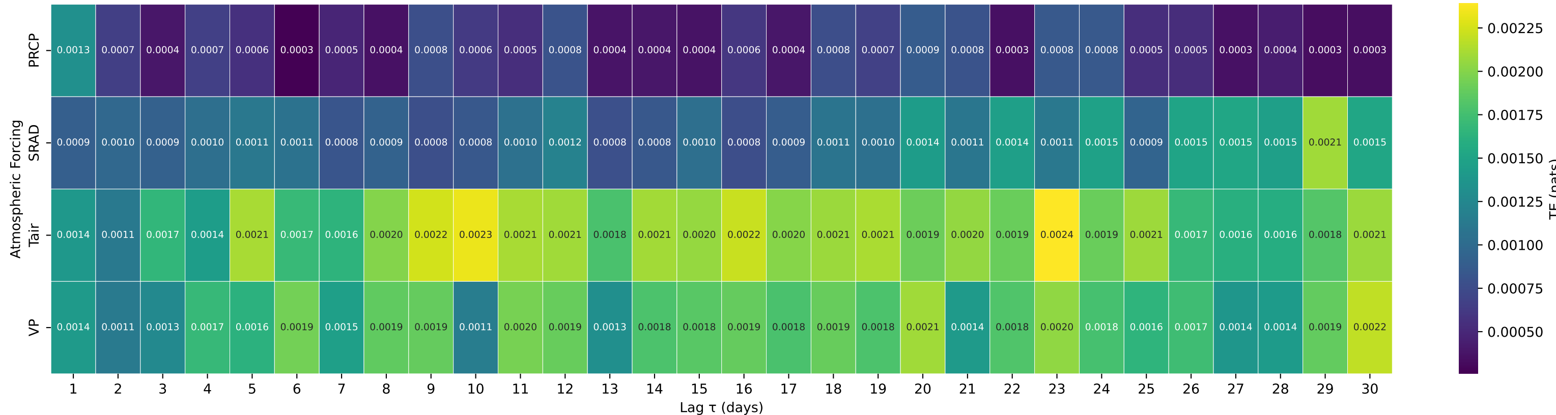
Shuffle-Test Significant TE to Streamflow — Basin 01415000 (HUC 02) — TREMPER KILL NEAR ANDES NY
