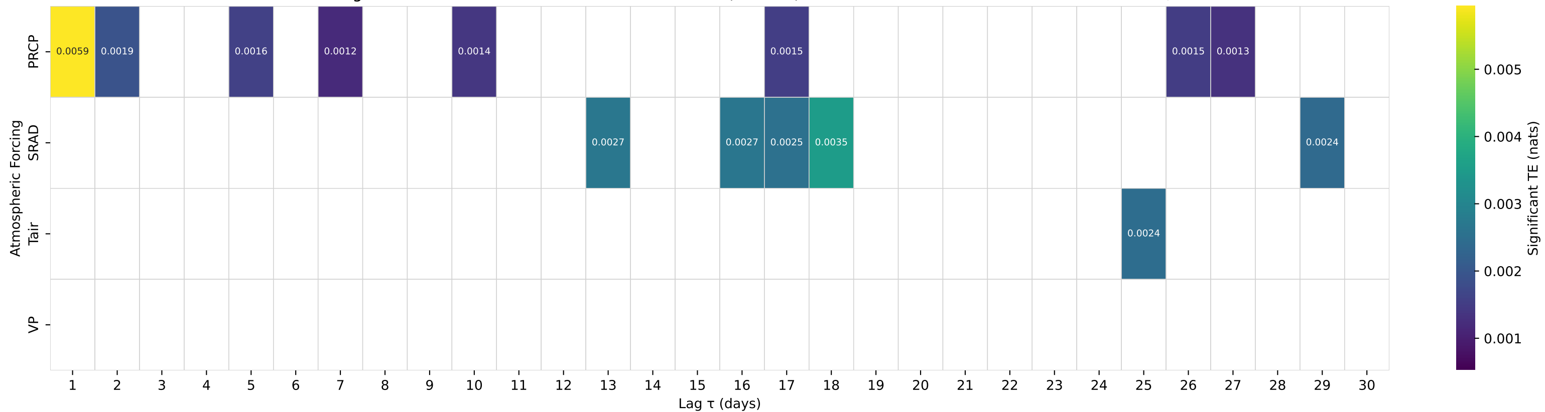
Shuffle-Test Significant TE to Streamflow — Basin 05291000 (HUC 07) — WHETSTONE RIVER NEAR BIG STONE CITY, SD
