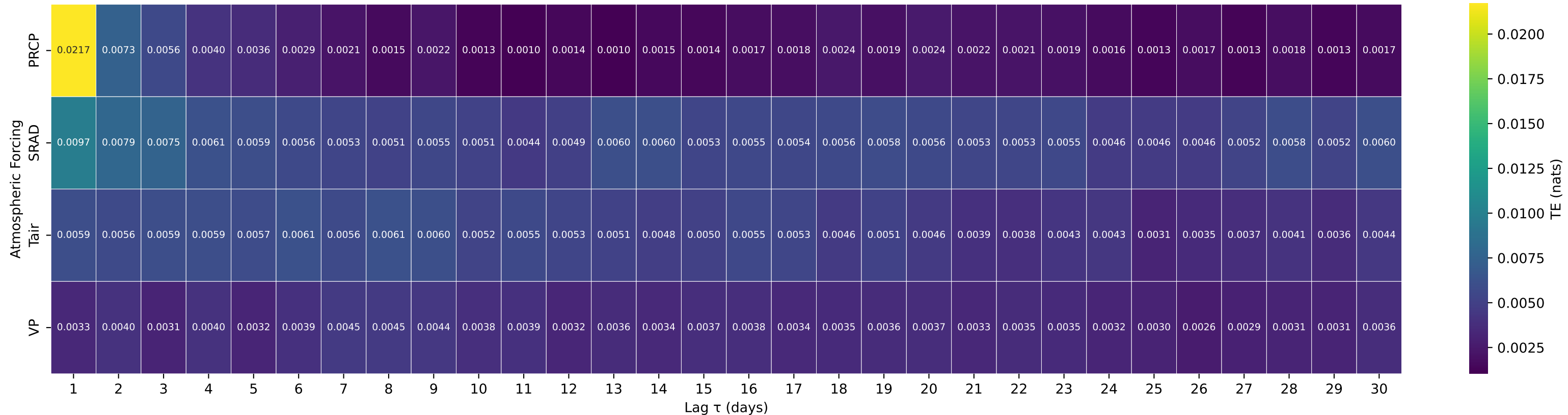
Shuffle-Test Significant TE to Streamflow — Basin 14141500 (HUC 17) — LITTLE SANDY RIVER NEAR BULL RUN, OREG.
