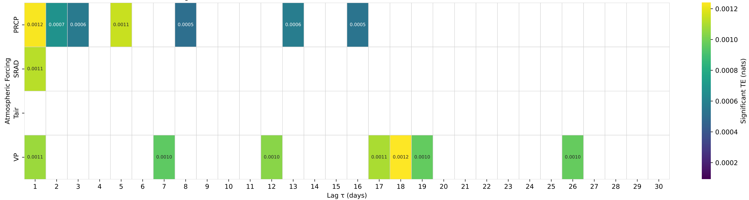
Shuffle-Test Significant TE to Streamflow — Basin 08202700 (HUC 12) — Seco Ck at Rowe Ranch nr D'Hanis, TX
