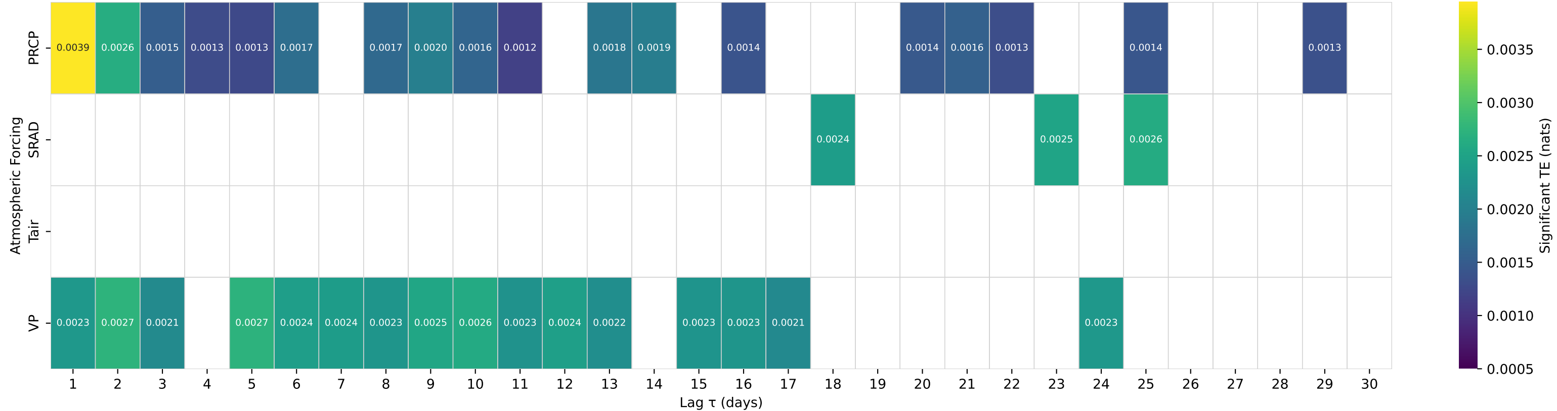
Shuffle-Test Significant TE to Streamflow — Basin 06853800 (HUC 10) — WHITE ROCK C NR BURR OAK, KS
