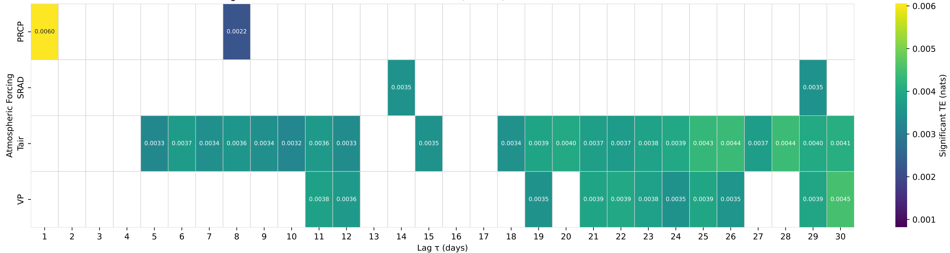
Shuffle-Test Significant TE to Streamflow — Basin 03050000 (HUC 05) — TYGART VALLEY RIVER NEAR DAILEY, WV
