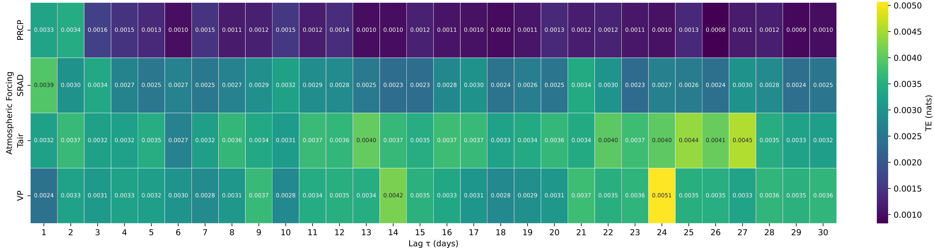
Shuffle-Test Significant TE to Streamflow — Basin 01451800 (HUC 02) — Jordan Creek near Schnecksville, PA
