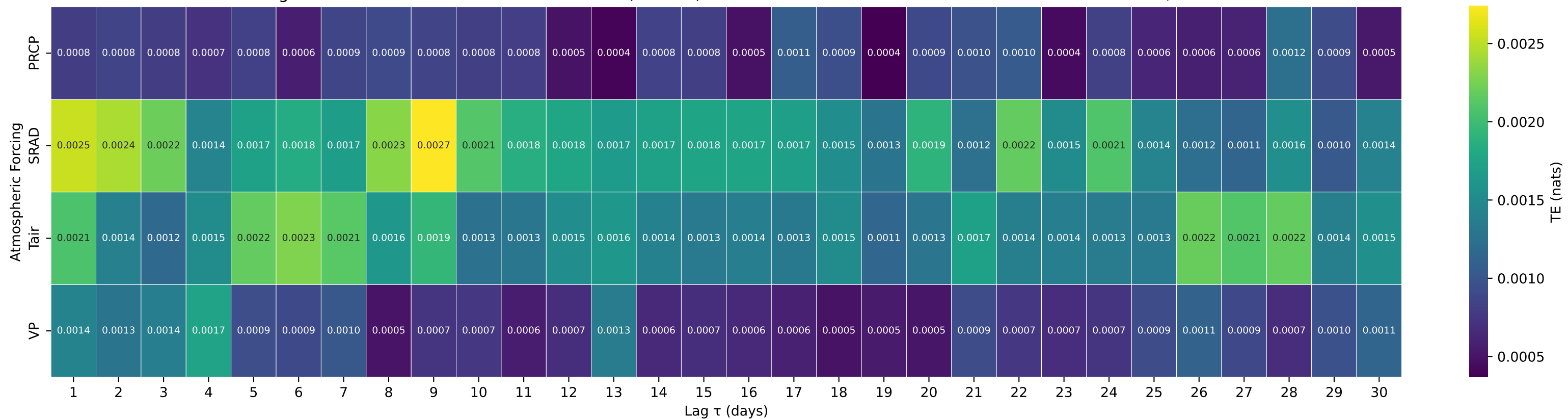
Shuffle-Test Significant TE to Streamflow — Basin 09312600 (HUC 14) — WHITE RIVER BL TABBYUNE C NEAR SOLDIER SUMMIT, UT
