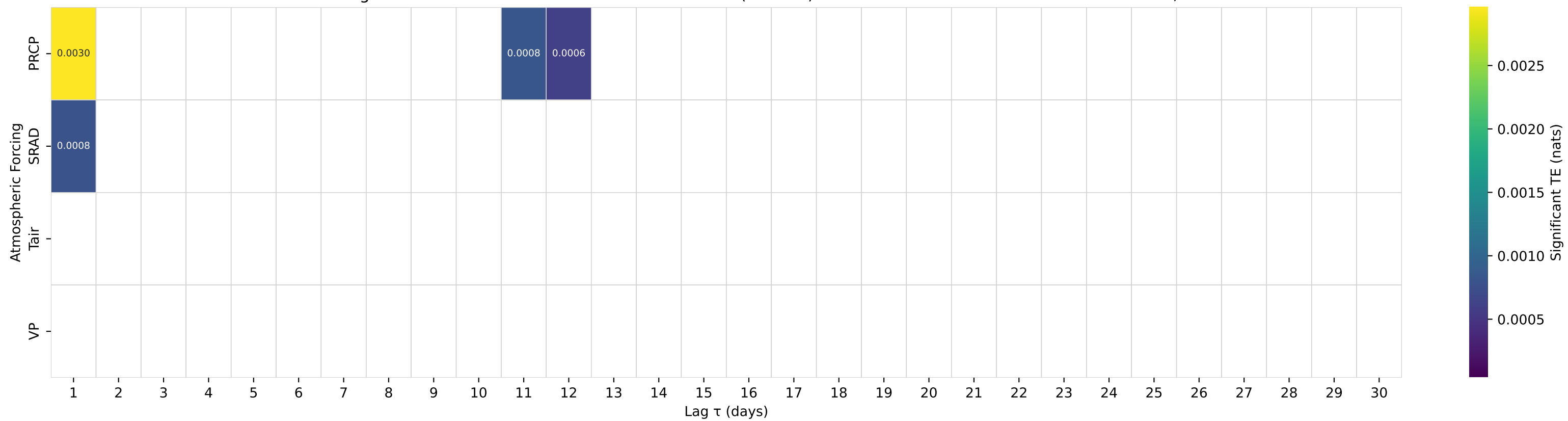
Shuffle-Test Significant TE to Streamflow — Basin 02082950 (HUC 03) — LITTLE FISHING CREEK NEAR WHITE OAK, NC
