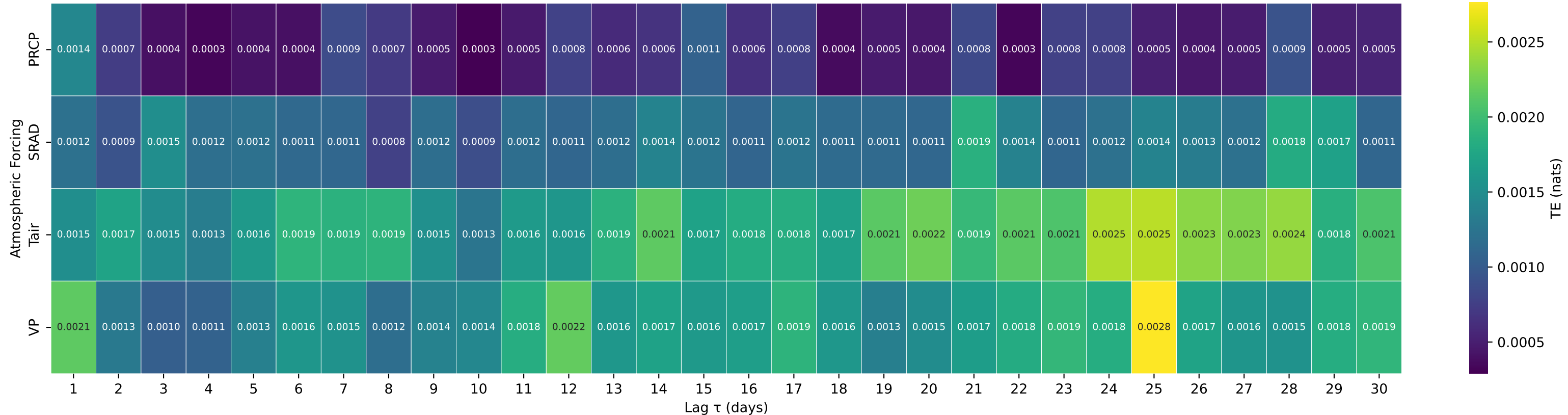
Shuffle-Test Significant TE to Streamflow — Basin 03069500 (HUC 05) — CHEAT RIVER NEAR PARSONS, WV
