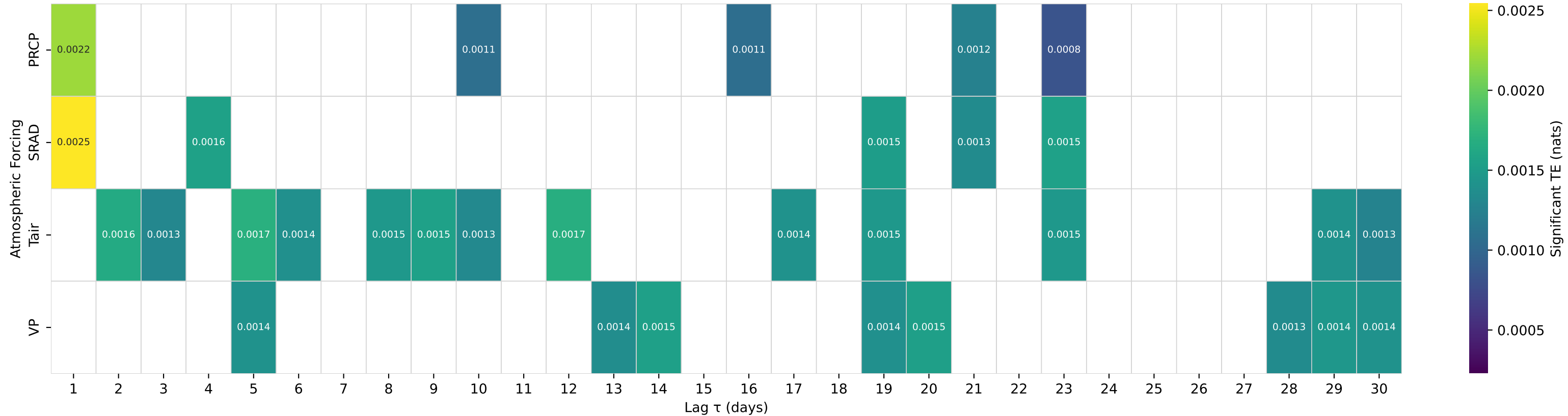
Shuffle-Test Significant TE to Streamflow — Basin 07359610 (HUC 08) — Caddo River near Caddo Gap, AR
