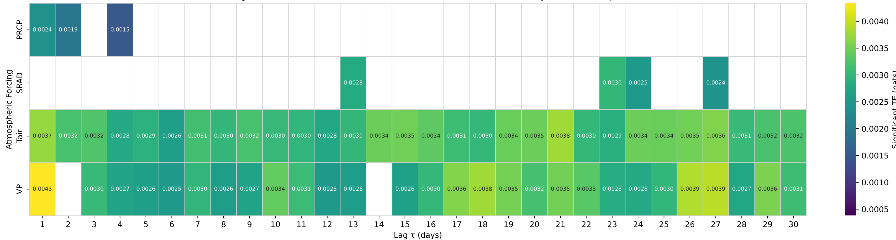
Shuffle-Test Significant TE to Streamflow — Basin 01542810 (HUC 02) — Waldy Run near Emporium, PA
