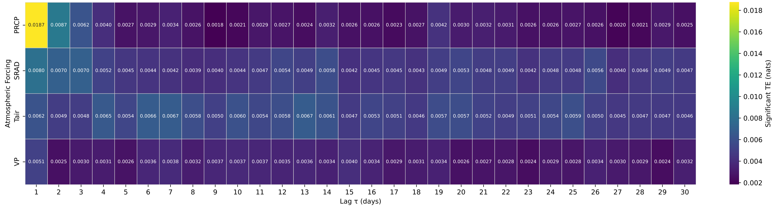
Shuffle-Test Significant TE to Streamflow — Basin 14158500 (HUC 17) — MCKENZIE RIVER AT OUTLET OF CLEAR LAKE, OR
