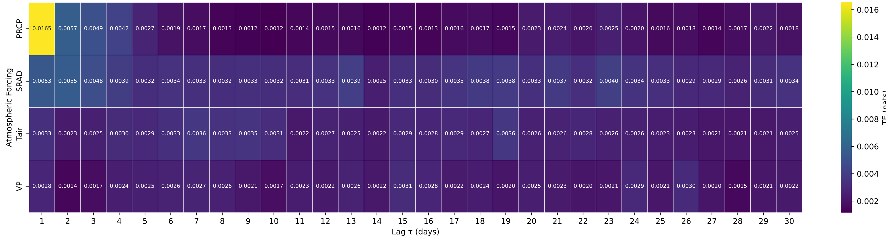
Shuffle-Test Significant TE to Streamflow — Basin 12189500 (HUC 17) — SAUK RIVER NEAR SAUK, WA
