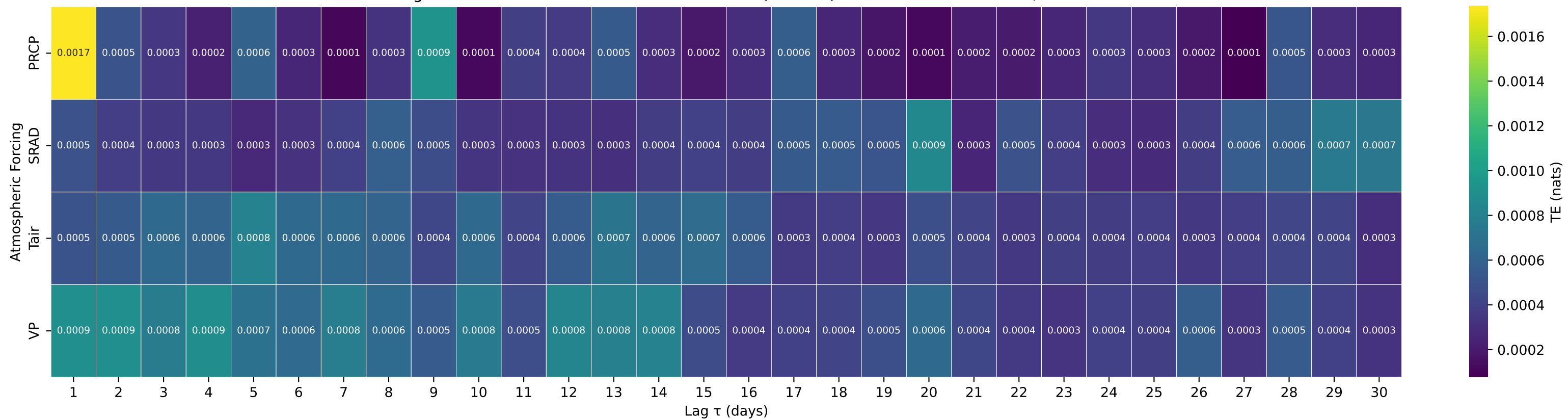
Shuffle-Test Significant TE to Streamflow — Basin 06889200 (HUC 10) — SOLDIER C NR DELIA, KS
