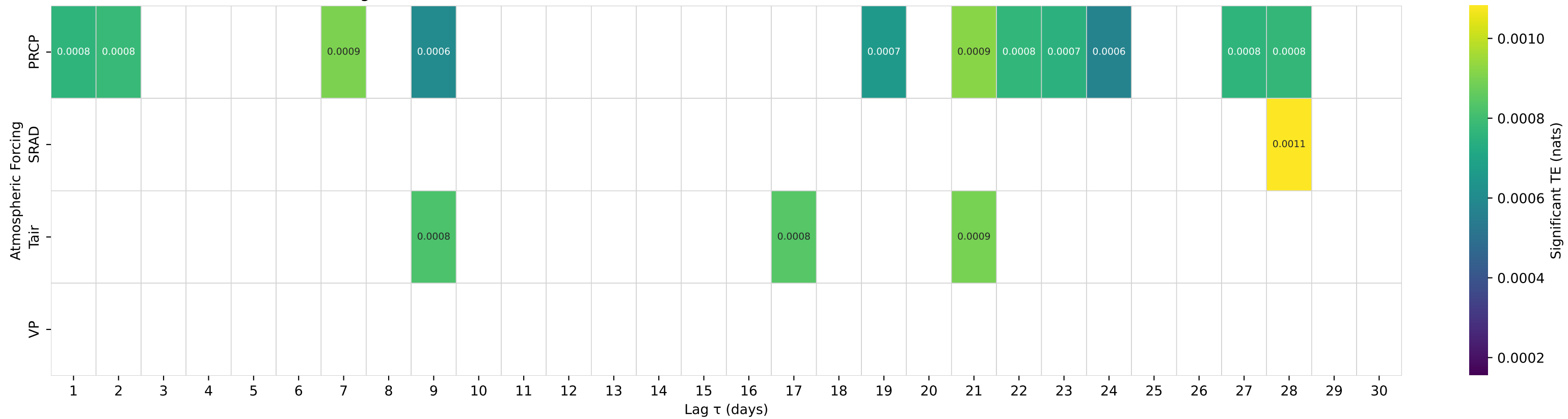
Shuffle-Test Significant TE to Streamflow — Basin 06847900 (HUC 10) — PRAIRIE DOG C AB KEITH SEBELIUS LAKE, KS
