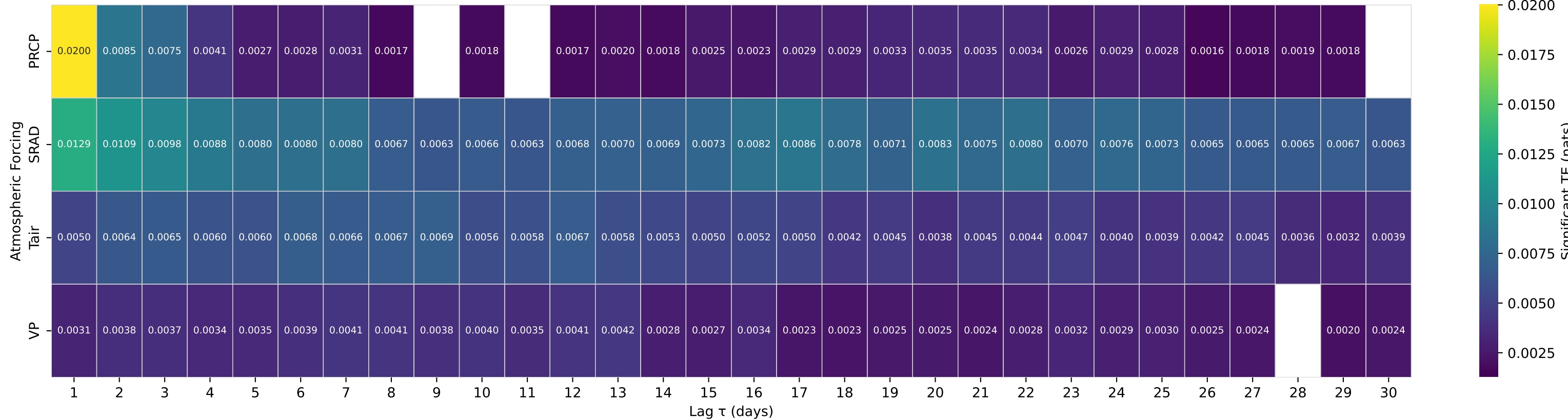
Shuffle-Test Significant TE to Streamflow — Basin 14305500 (HUC 17) — SILETZ RIVER AT SILETZ, OR
