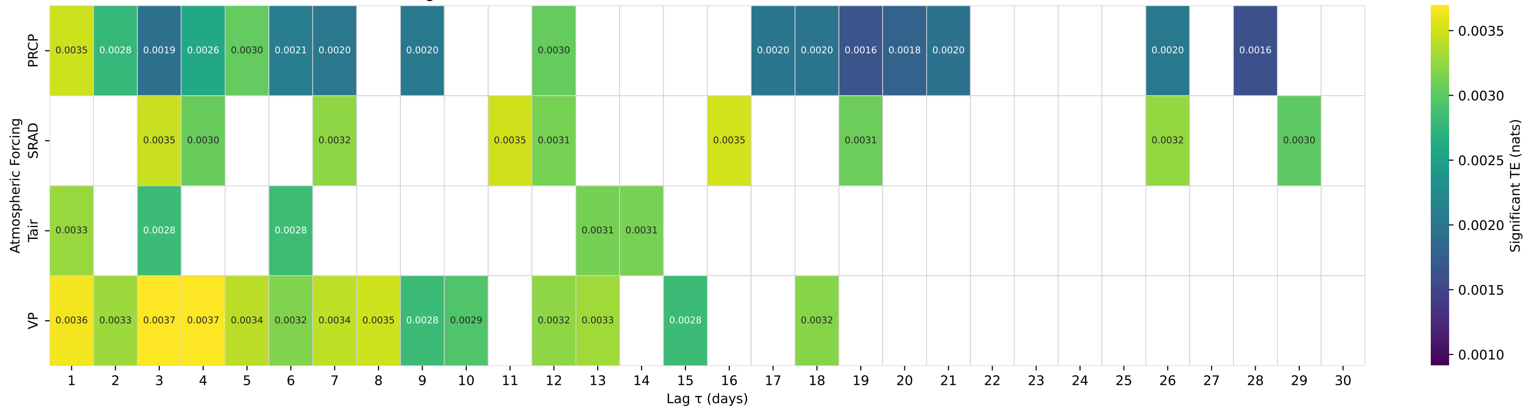
Shuffle-Test Significant TE to Streamflow — Basin 06814000 (HUC 10) — TURKEY C NR SENECA, KS
