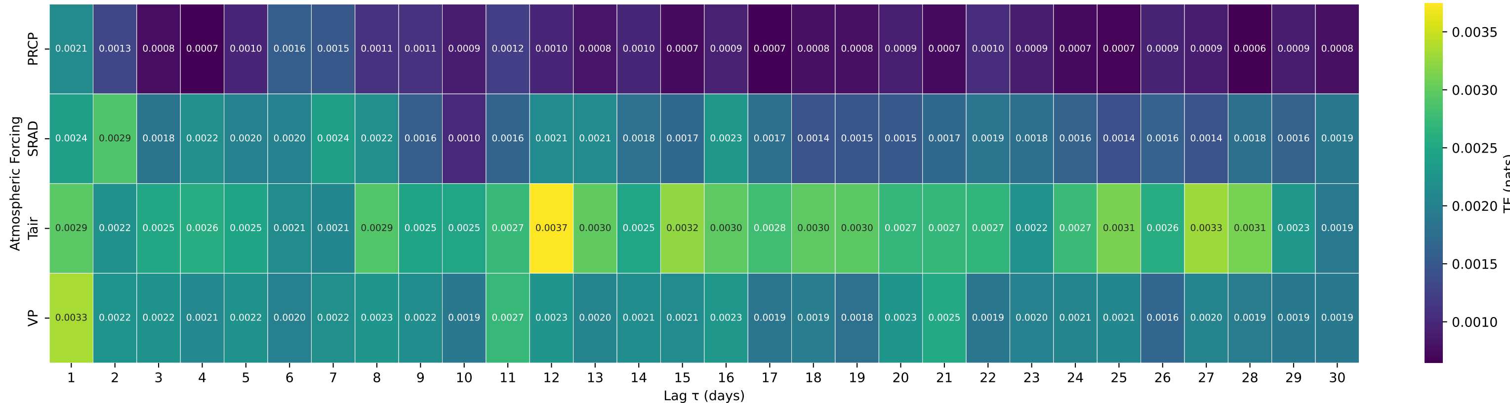
Shuffle-Test Significant TE to Streamflow — Basin 01054200 (HUC 01) — Wild River at Gilead, Maine
