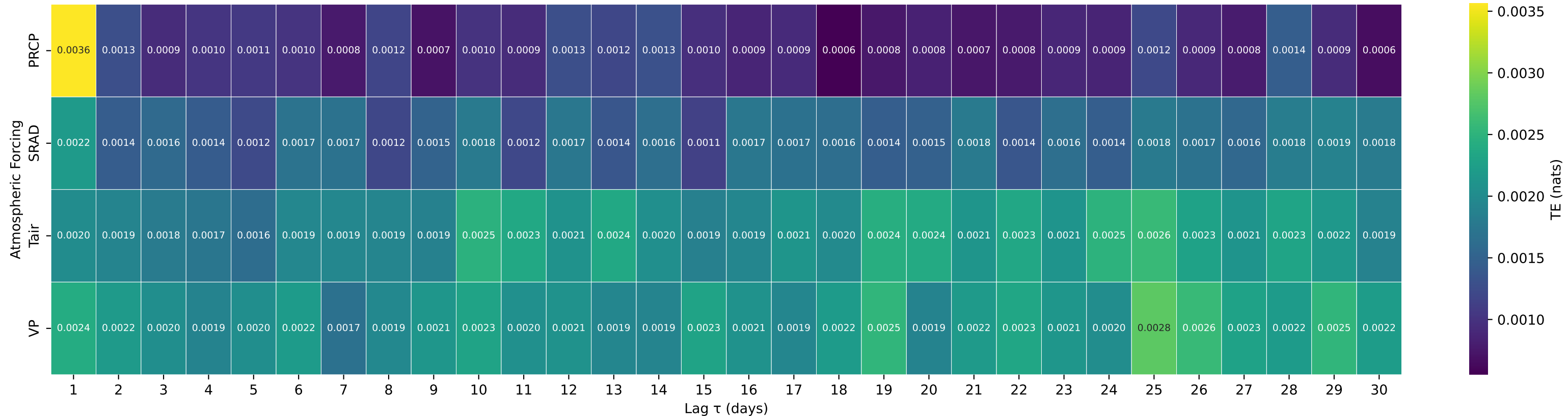
Shuffle-Test Significant TE to Streamflow — Basin 03144000 (HUC 05) — Wakatomika Creek near Frazzysburg OH
