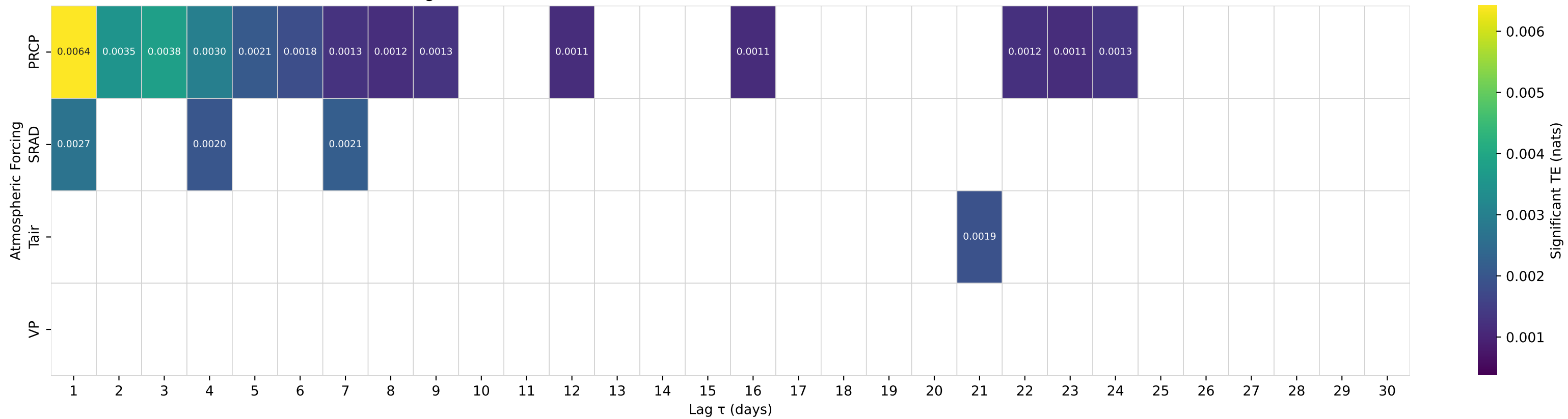
Shuffle-Test Significant TE to Streamflow — Basin 05585000 (HUC 07) — LA MOINE RIVER AT RIPLEY, IL
