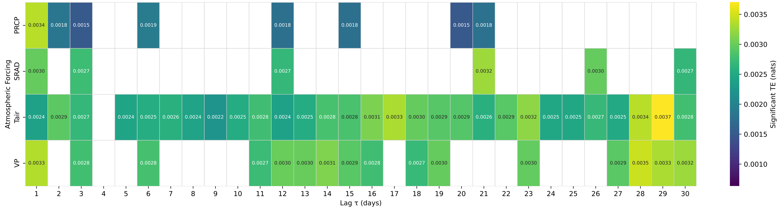
Shuffle-Test Significant TE to Streamflow — Basin 02395120 (HUC 03) — TWO RUN CREEK NEAR KINGSTON, GA
