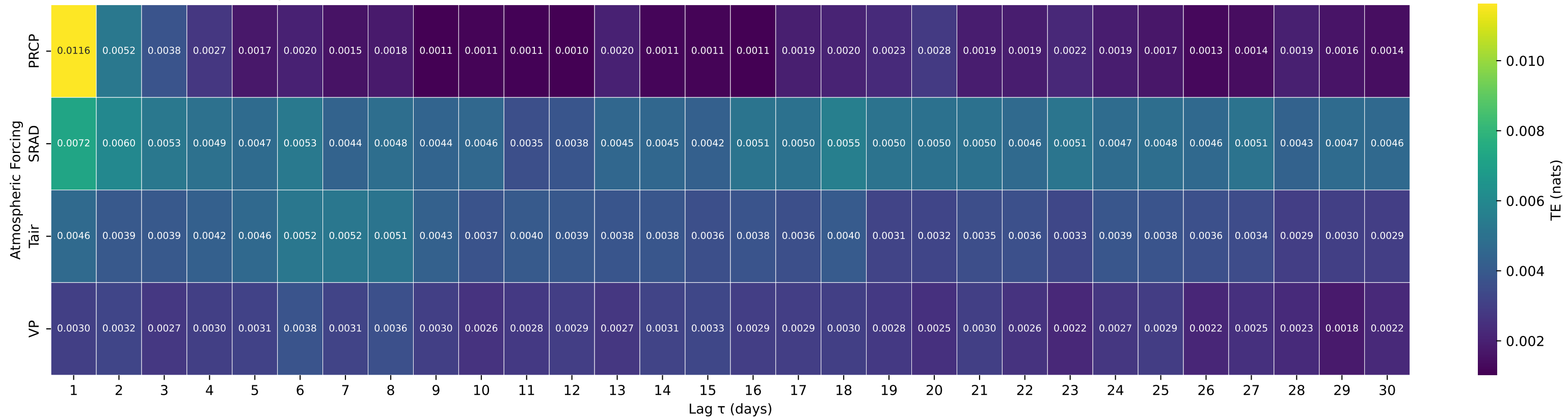
Shuffle-Test Significant TE to Streamflow — Basin 14236200 (HUC 17) — TILTON RIVER AB BEAR CANYON CREEK NEAR CINEBAR, WA
