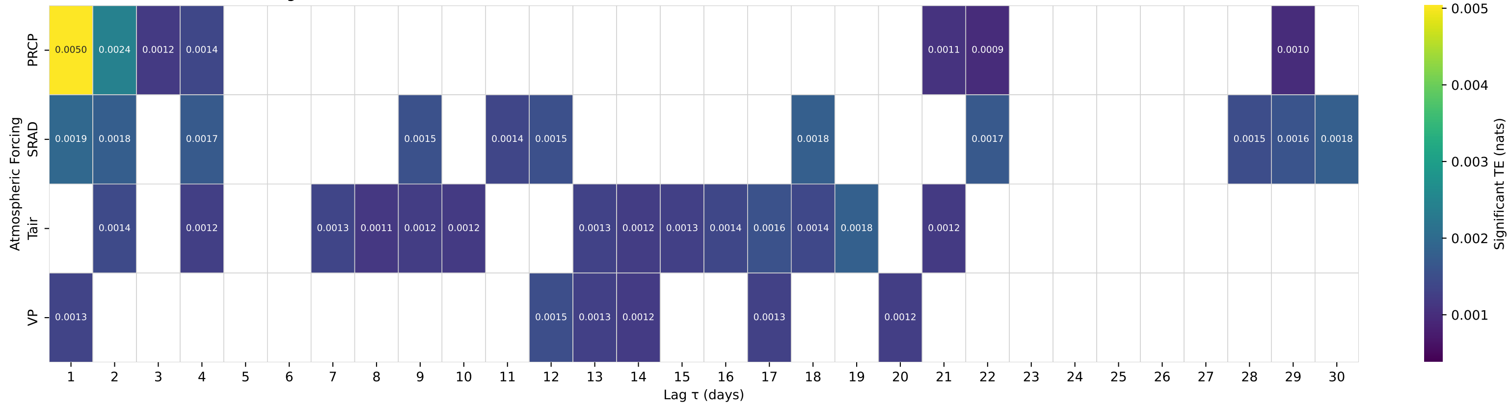
Shuffle-Test Significant TE to Streamflow — Basin 12186000 (HUC 17) — SAUK RIVER AB WHITECHUCK RIVER NEAR DARRINGTON, WA
