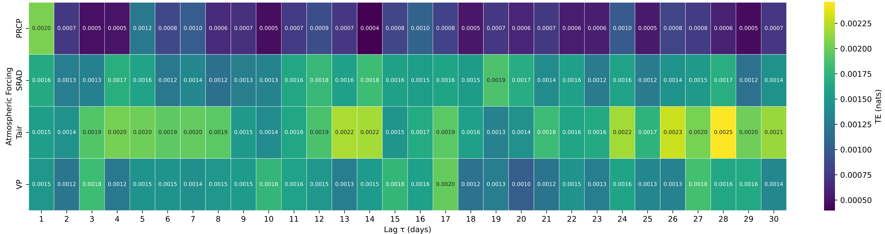
Shuffle-Test Significant TE to Streamflow — Basin 01586610 (HUC 02) — MORGAN RUN NEAR LOUISVILLE, MD
