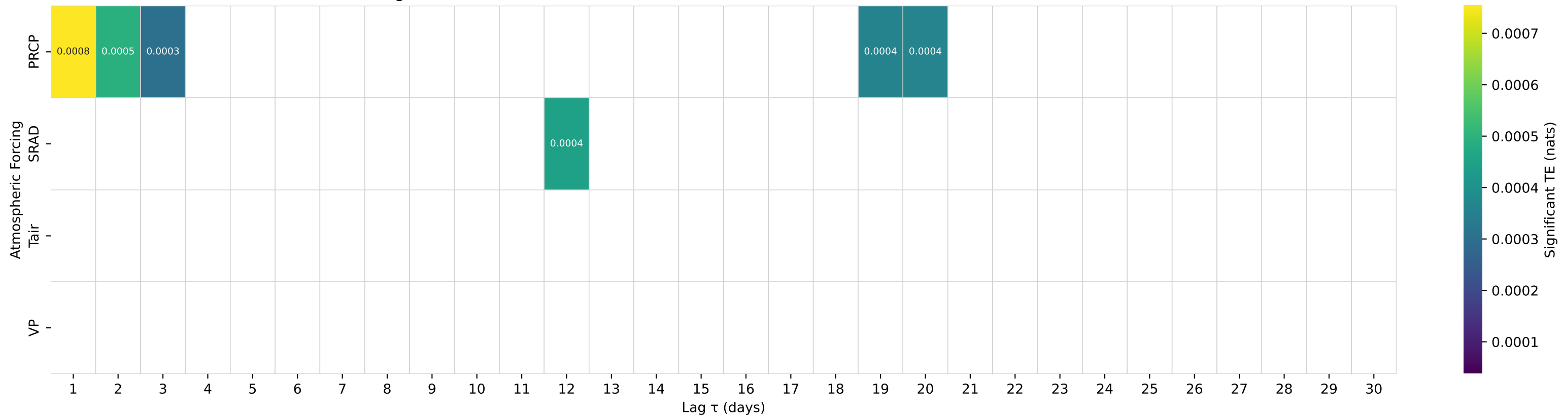
Shuffle-Test Significant TE to Streamflow — Basin 02055100 (HUC 03) — TINKER CREEK NEAR DALEVILLE, VA
