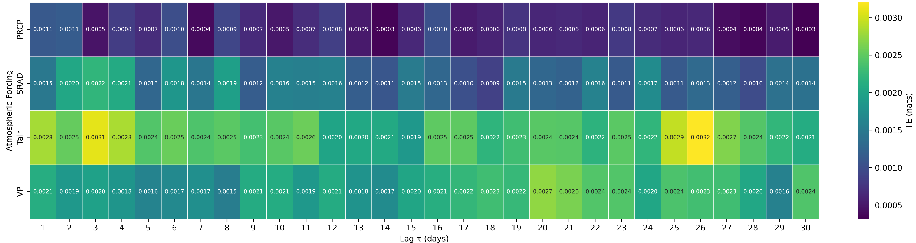
Shuffle-Test Significant TE to Streamflow — Basin 01170100 (HUC 01) — GREEN RIVER NEAR COLRAIN, MA
