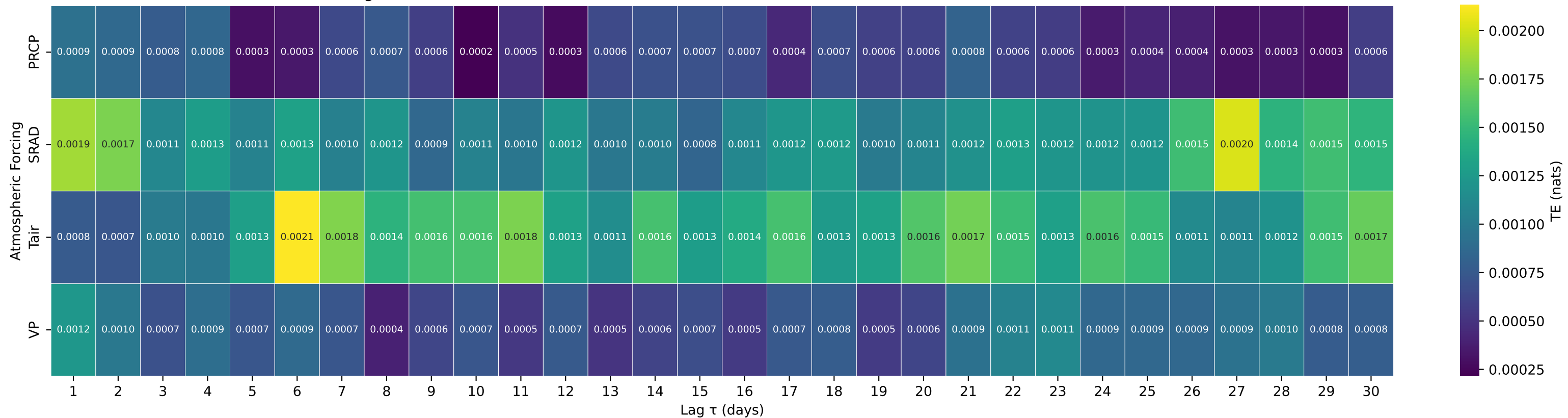
Shuffle-Test Significant TE to Streamflow — Basin 05056000 (HUC 09) — SHEYENNE RIVER NR WARWICK, ND
