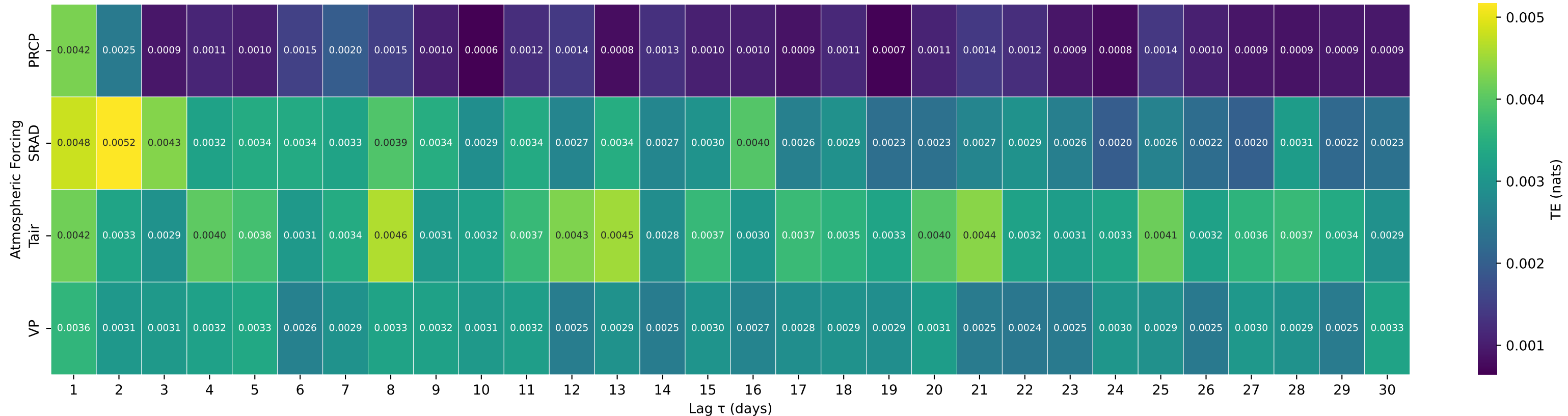
Shuffle-Test Significant TE to Streamflow — Basin 01137500 (HUC 01) — AMMONOOSUC RIVER AT BETHLEHEM JUNCTION, NH
