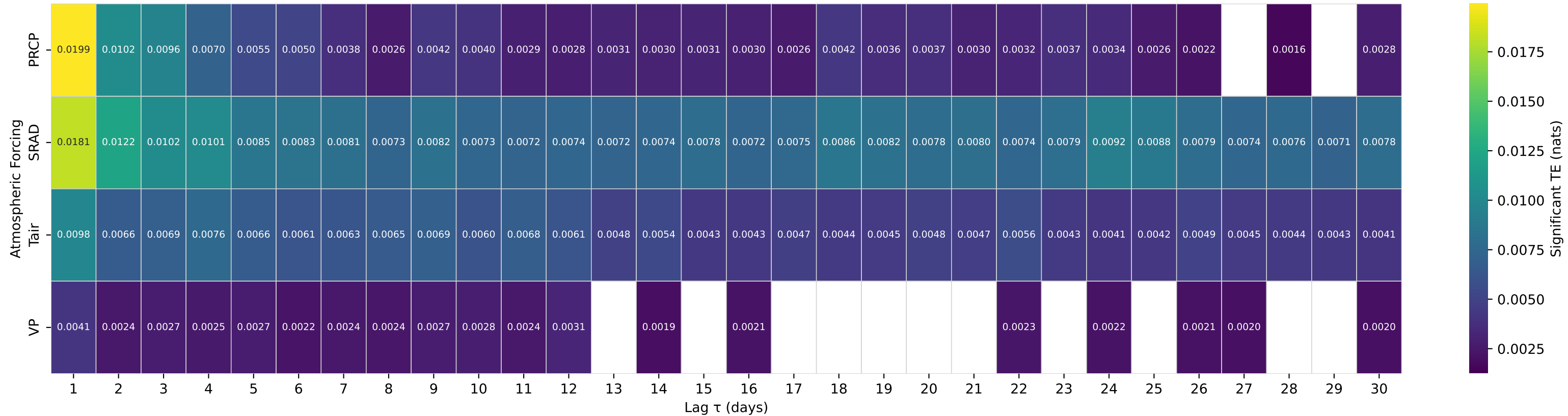
Shuffle-Test Significant TE to Streamflow — Basin 14400000 (HUC 17) — CHETCO RIVER NEAR BROOKINGS, OR
