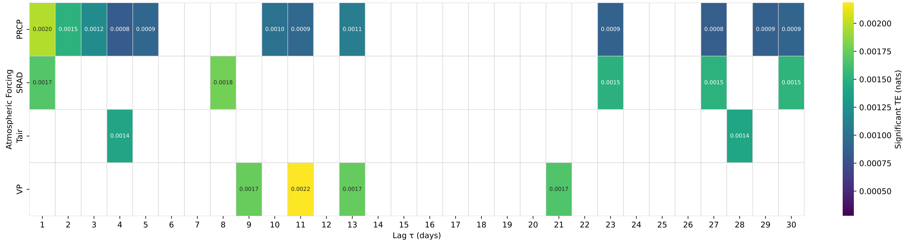
Shuffle-Test Significant TE to Streamflow — Basin 08103900 (HUC 12) — S Fk Rocky Ck nr Briggs, TX
