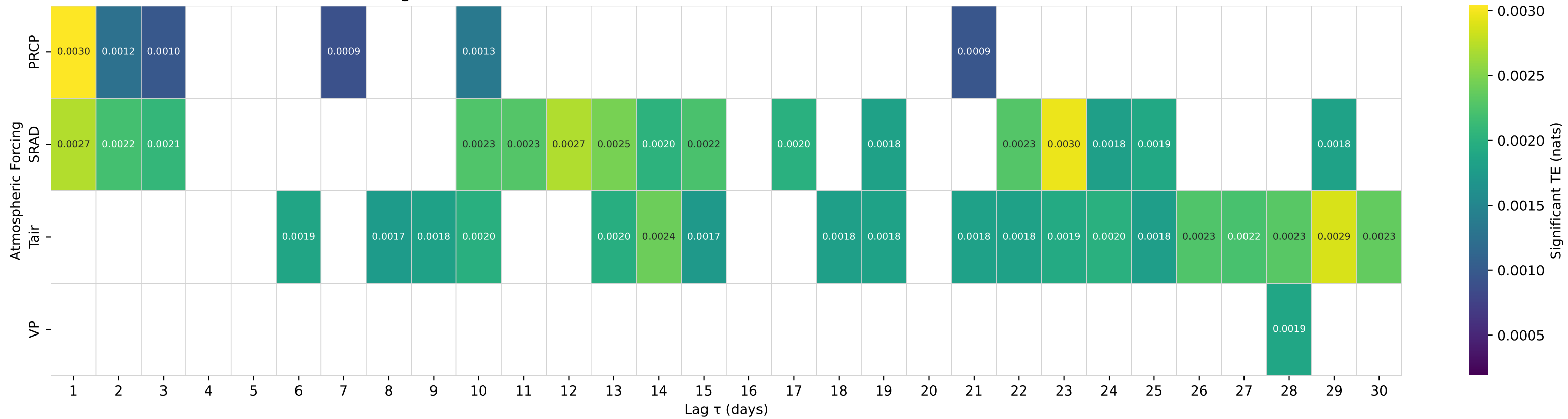
Shuffle-Test Significant TE to Streamflow — Basin 09484000 (HUC 15) — SABINO CREEK NEAR TUCSON, AZ.
