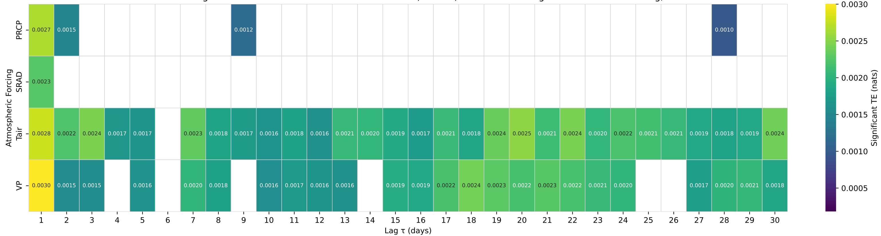
Shuffle-Test Significant TE to Streamflow — Basin 01543500 (HUC 02) — Sinnemahoning Creek at Sinnemahoning, PA
