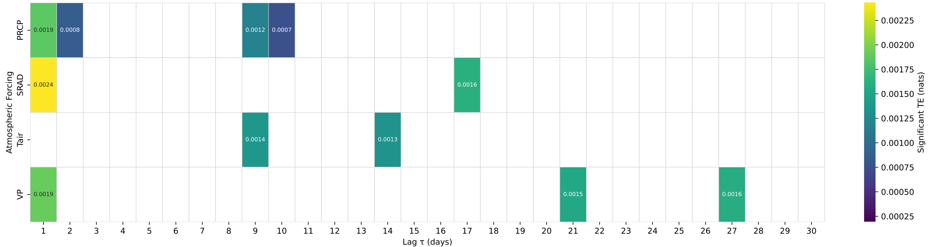
Shuffle-Test Significant TE to Streamflow — Basin 02140991 (HUC 03) — JOHNS RIVER AT ARNEYS STORE, NC
