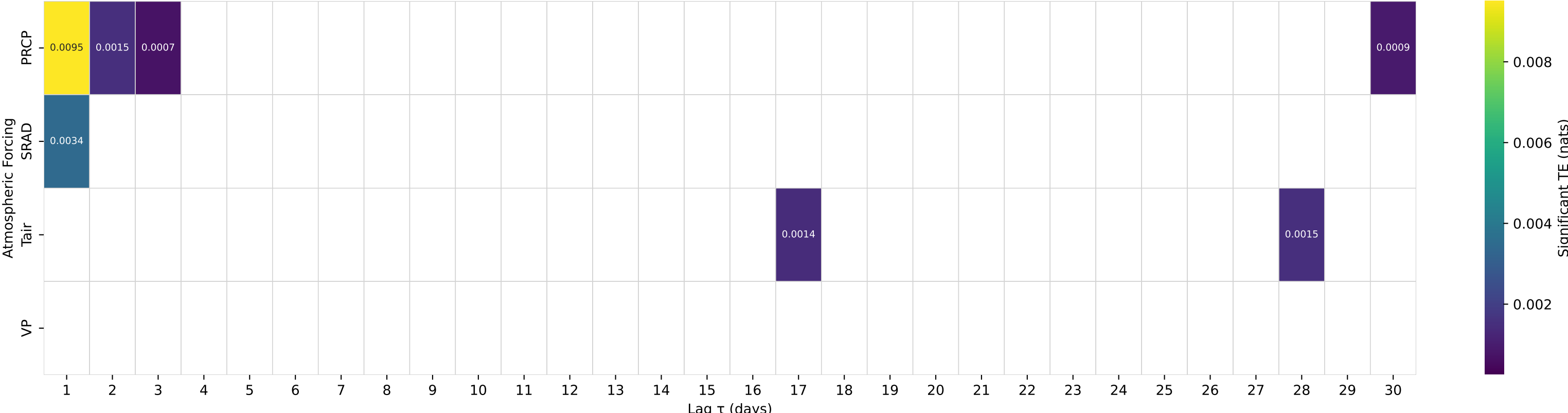
Shuffle-Test Significant TE to Streamflow — Basin 01411300 (HUC 02) — TUCKAHOE RIVER AT HEAD OF RIVER NJ
