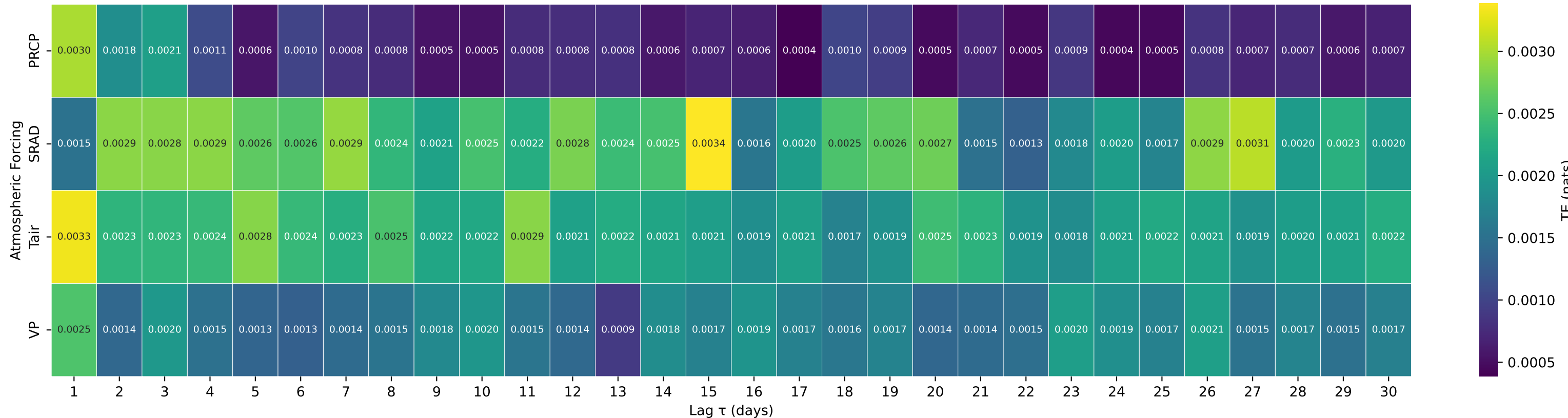
Shuffle-Test Significant TE to Streamflow — Basin 04027000 (HUC 04) — BAD RIVER NEAR ODANAH, WI
