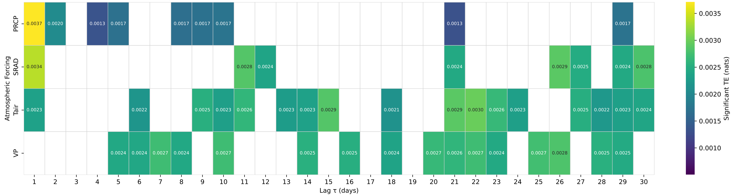
Shuffle-Test Significant TE to Streamflow — Basin 05593900 (HUC 07) — EAST FORK SHOAL CREEK NEAR COFFEEN, IL
