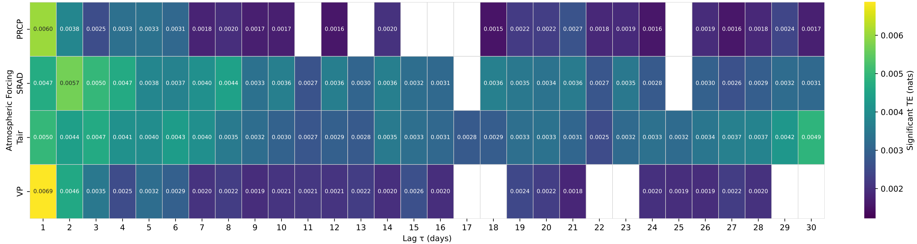
Shuffle-Test Significant TE to Streamflow — Basin 10396000 (HUC 17) — DONNER UND BLITZEN RIVER NR FRENCHGLEN OR
