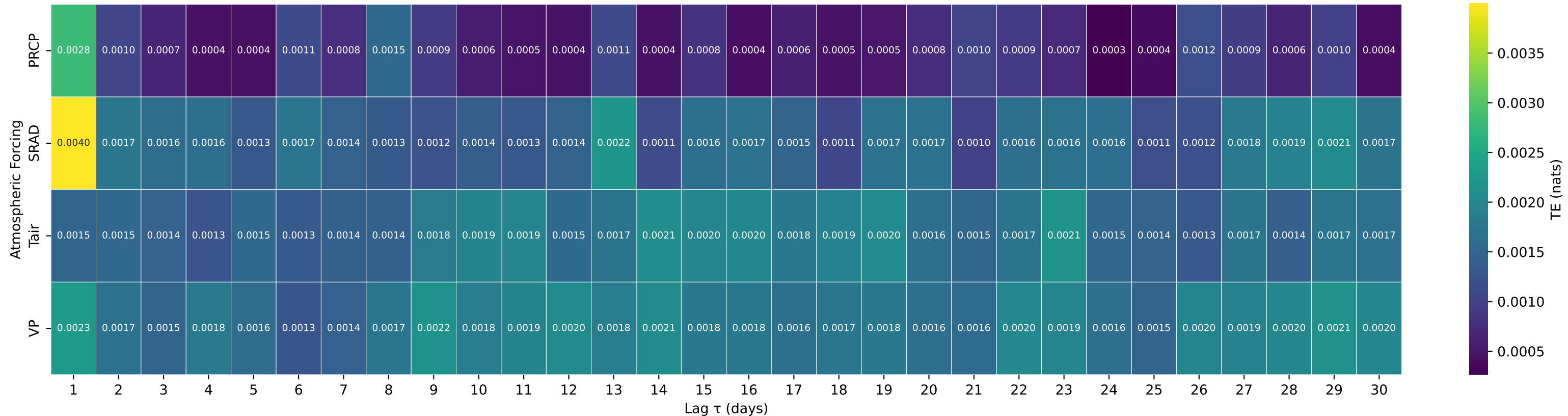
Shuffle-Test Significant TE to Streamflow — Basin 02178400 (HUC 03) — TALLULAH RIVER NEAR CLAYTON, GA
