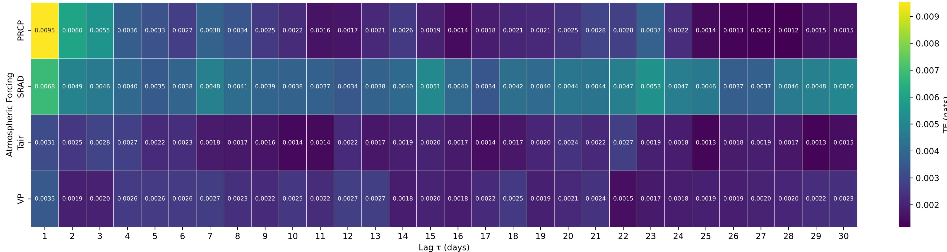
Shuffle-Test Significant TE to Streamflow — Basin 11143000 (HUC 18) — BIG SUR R NR BIG SUR CA
