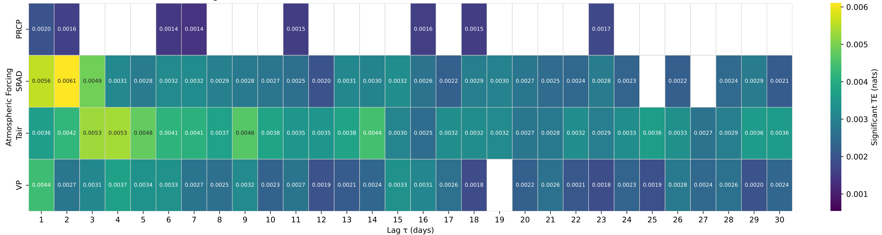
Shuffle-Test Significant TE to Streamflow — Basin 09066000 (HUC 14) — BLACK GORE CREEK NEAR MINTURN, CO.
