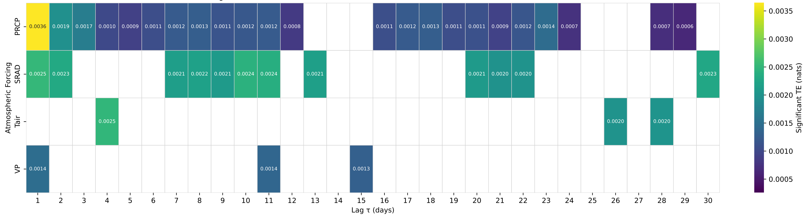
Shuffle-Test Significant TE to Streamflow — Basin 10259200 (HUC 18) — DEEP C NR PALM DESERT CA
