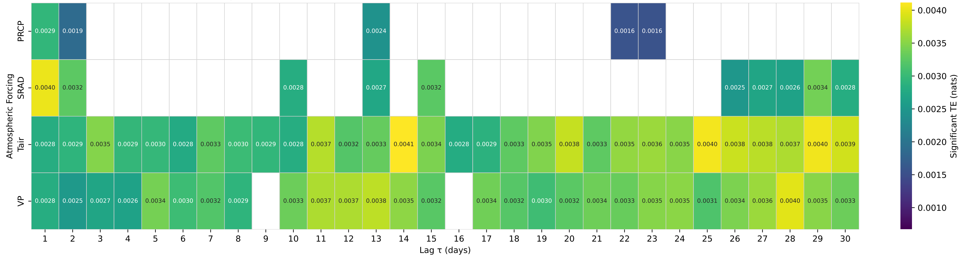
Shuffle-Test Significant TE to Streamflow — Basin 02415000 (HUC 03) — HILLABEE CREEK NEAR HACKNEYVILLE AL
