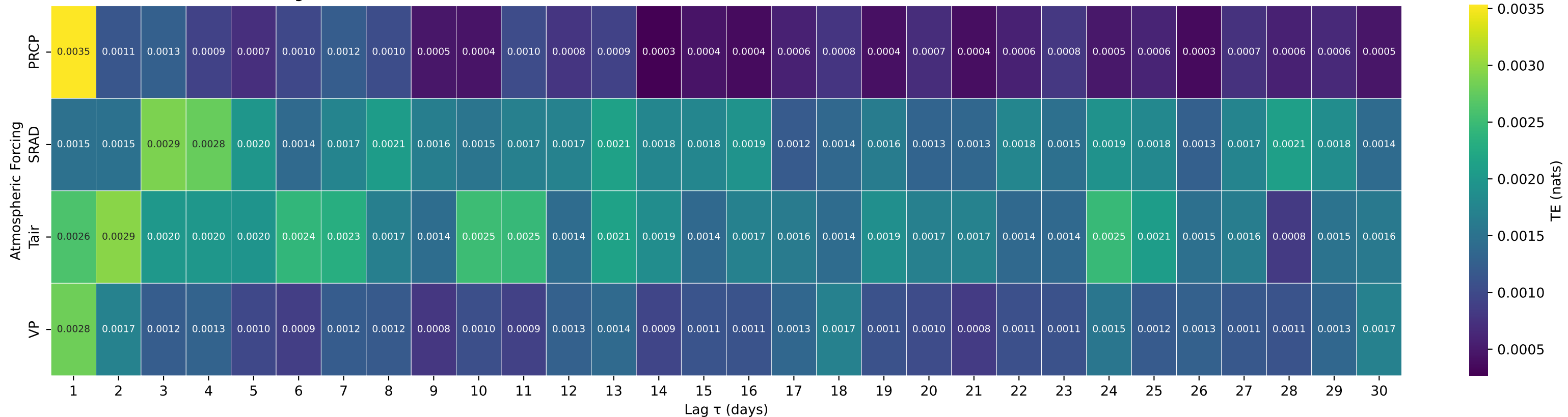
Shuffle-Test Significant TE to Streamflow — Basin 04057800 (HUC 04) — MIDDLE BRANCH ESCANABA RIVER AT HUMBOLDT, MI
