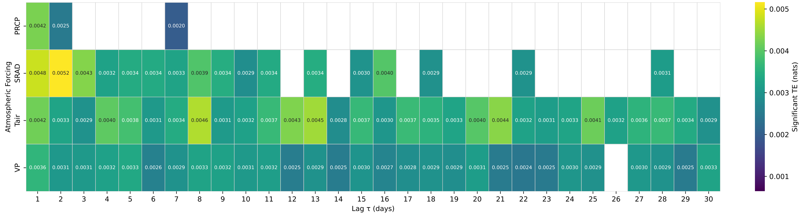
Shuffle-Test Significant TE to Streamflow — Basin 01137500 (HUC 01) — AMMONOOSUC RIVER AT BETHLEHEM JUNCTION, NH
