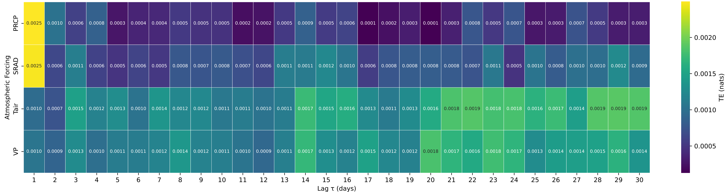
Shuffle-Test Significant TE to Streamflow — Basin 02422500 (HUC 03) — MULBERRY CREEK AT JONES AL
