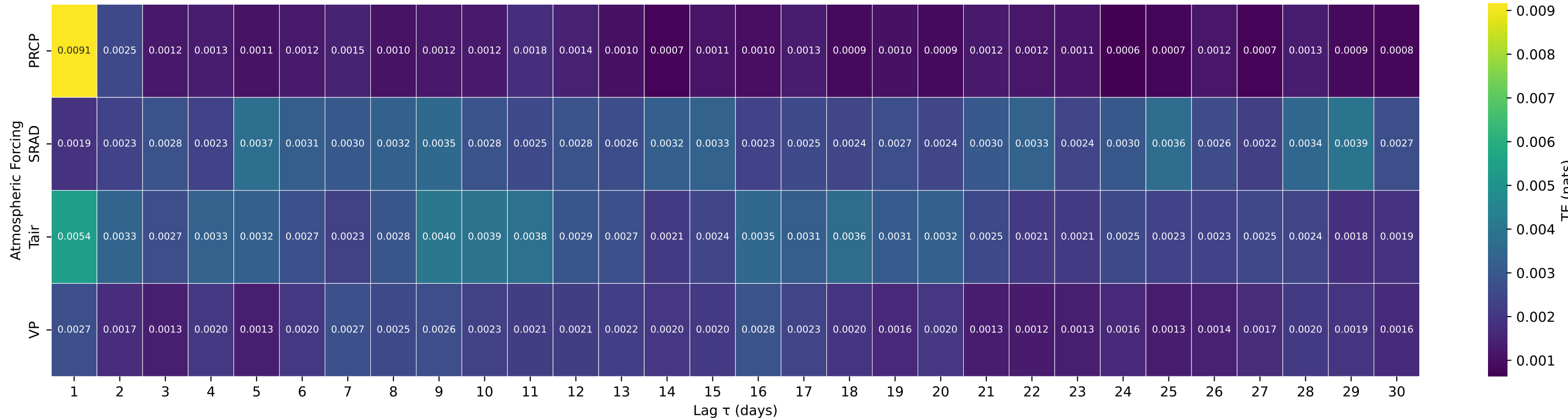
Shuffle-Test Significant TE to Streamflow — Basin 04074950 (HUC 04) — WOLF RIVER AT LANGLADE, WI
