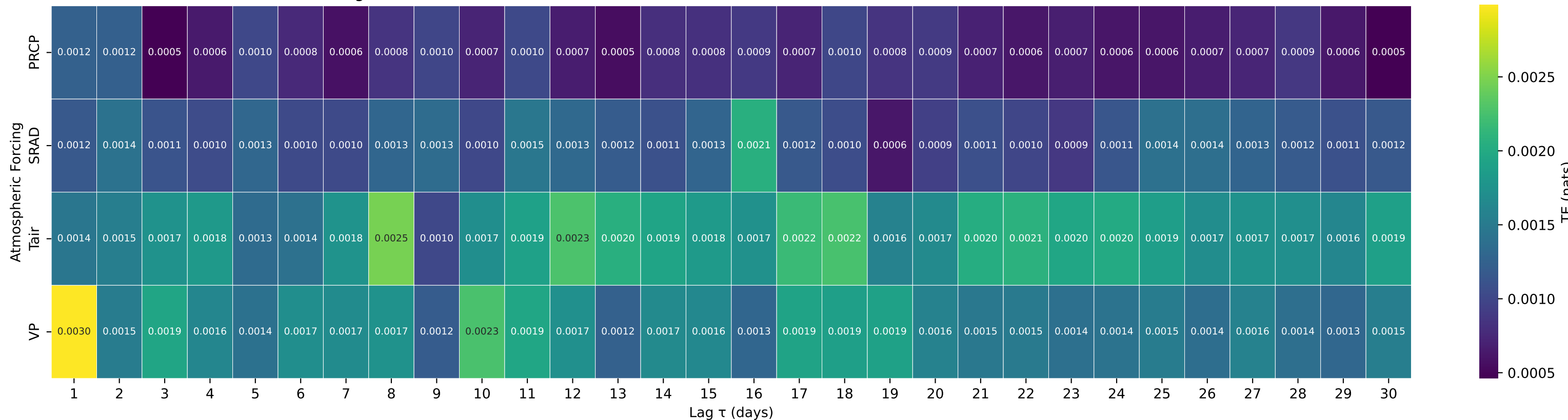
Shuffle-Test Significant TE to Streamflow — Basin 03028000 (HUC 05) — West Branch Clarion River at Wilcox, PA
