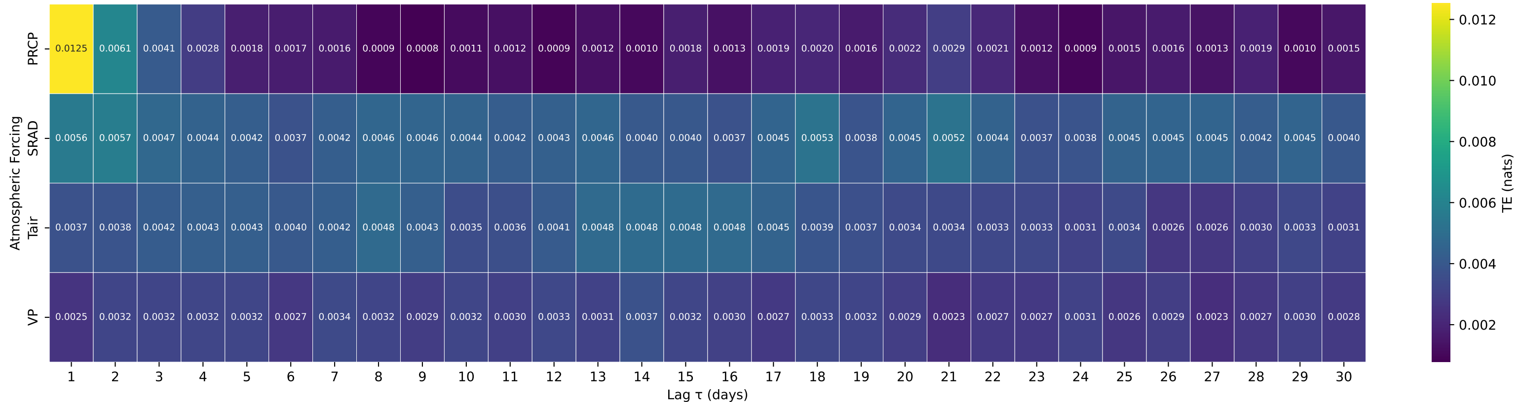
Shuffle-Test Significant TE to Streamflow — Basin 12115500 (HUC 17) — REX RIVER NEAR CEDAR FALLS, WA
