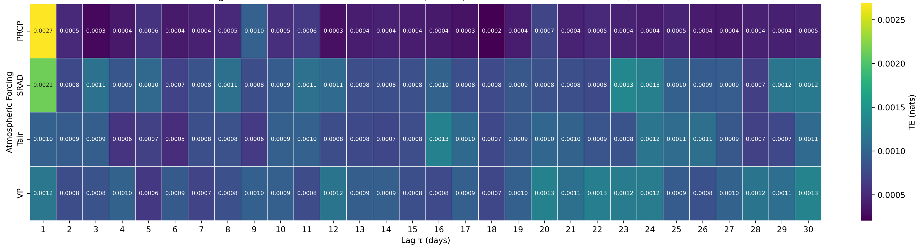
Shuffle-Test Significant TE to Streamflow — Basin 02149000 (HUC 03) — COVE CREEK NEAR LAKE LURE, NC
