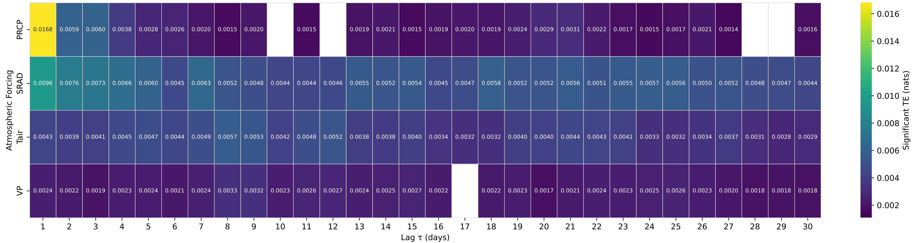
Shuffle-Test Significant TE to Streamflow — Basin 14185000 (HUC 17) — SOUTH SANTIAM RIVER BELOW CASCADIA, OR
