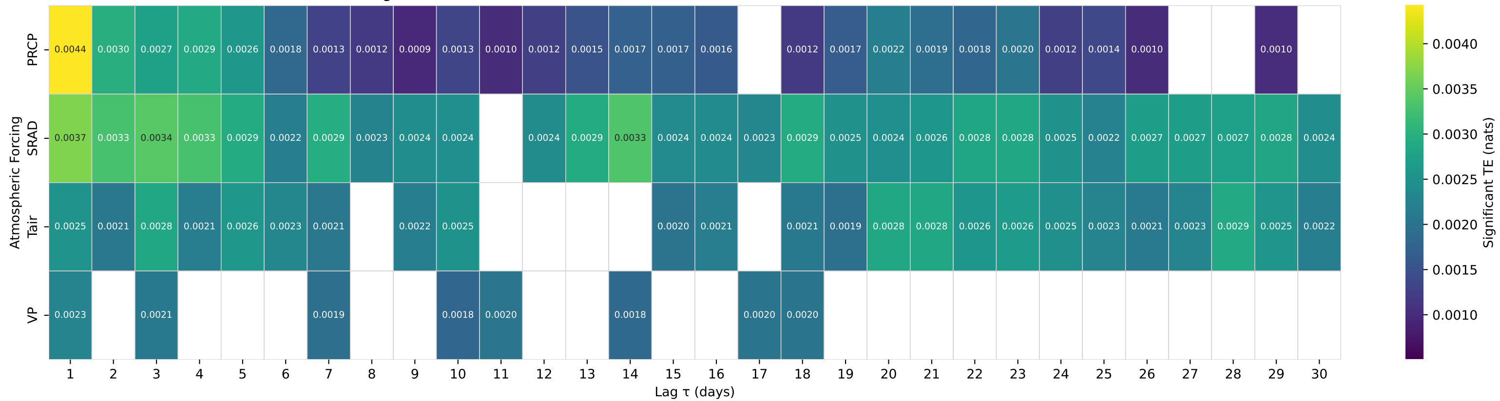
Shuffle-Test Significant TE to Streamflow — Basin 11124500 (HUC 18) — SANTA CRUZ C NR SANTA YNEZ CA
