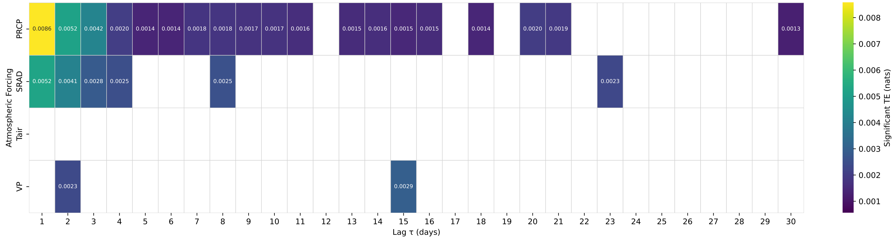
Shuffle-Test Significant TE to Streamflow — Basin 02235200 (HUC 03) — BLACKWATER CREEK NEAR CASSIA, FL
