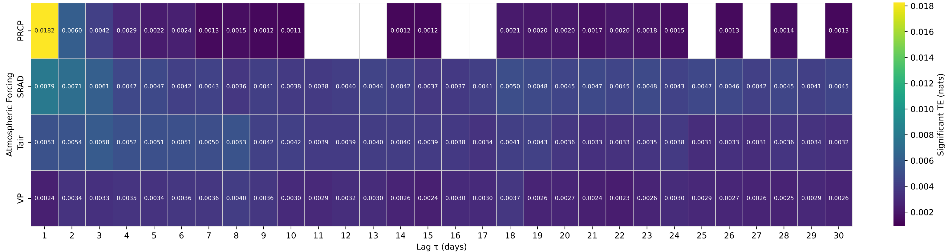
Shuffle-Test Significant TE to Streamflow — Basin 14138800 (HUC 17) — BLAZED ALDER CREEK NEAR RHODODENDRON, OREG.
