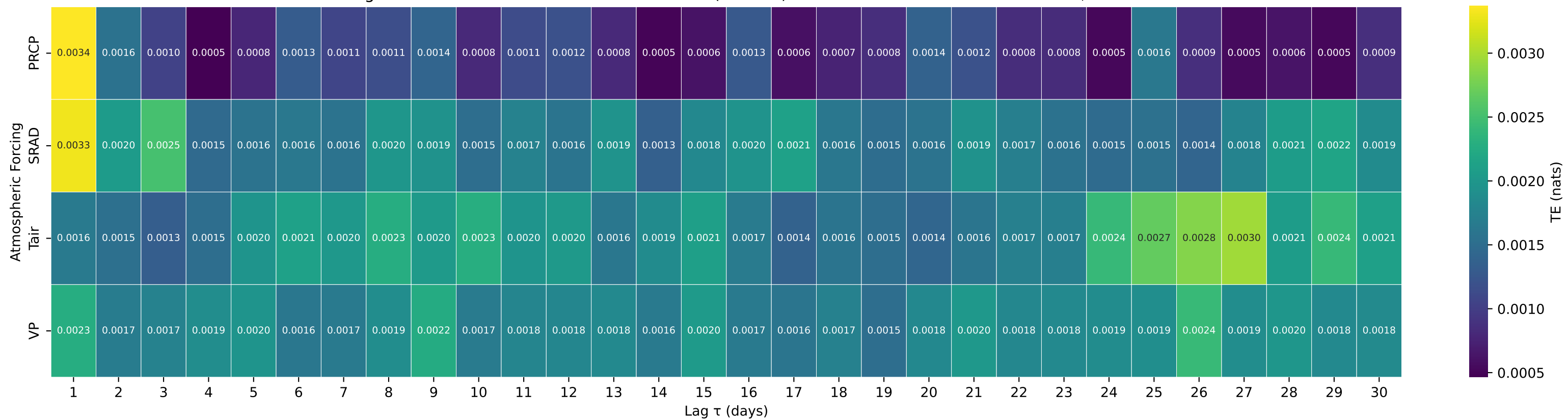
Shuffle-Test Significant TE to Streamflow — Basin 02014000 (HUC 02) — POTTS CREEK NEAR COVINGTON, VA
