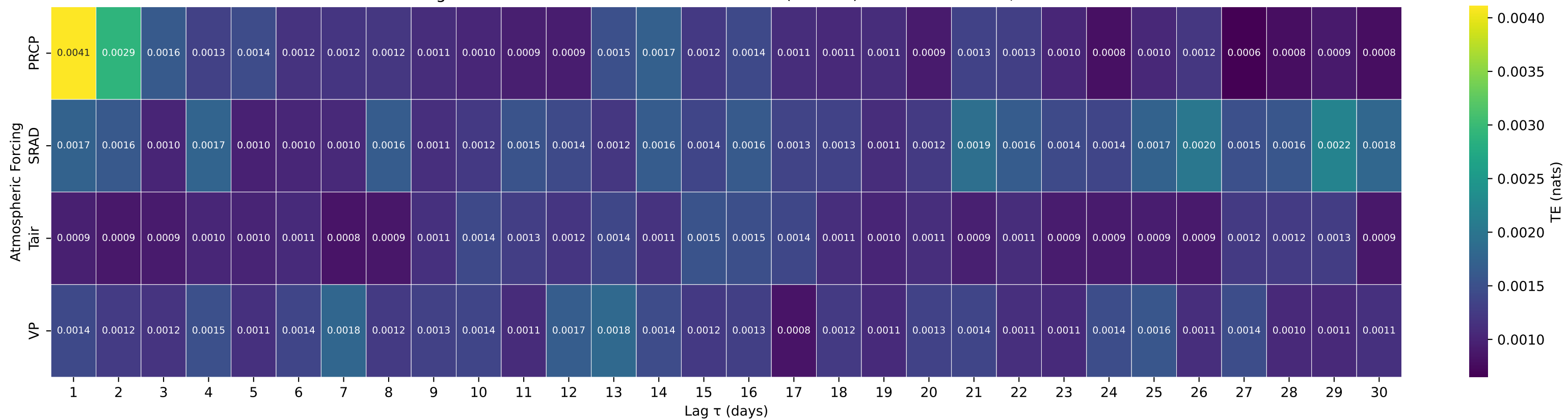
Shuffle-Test Significant TE to Streamflow — Basin 06876700 (HUC 10) — SALT C NR ADA, KS
