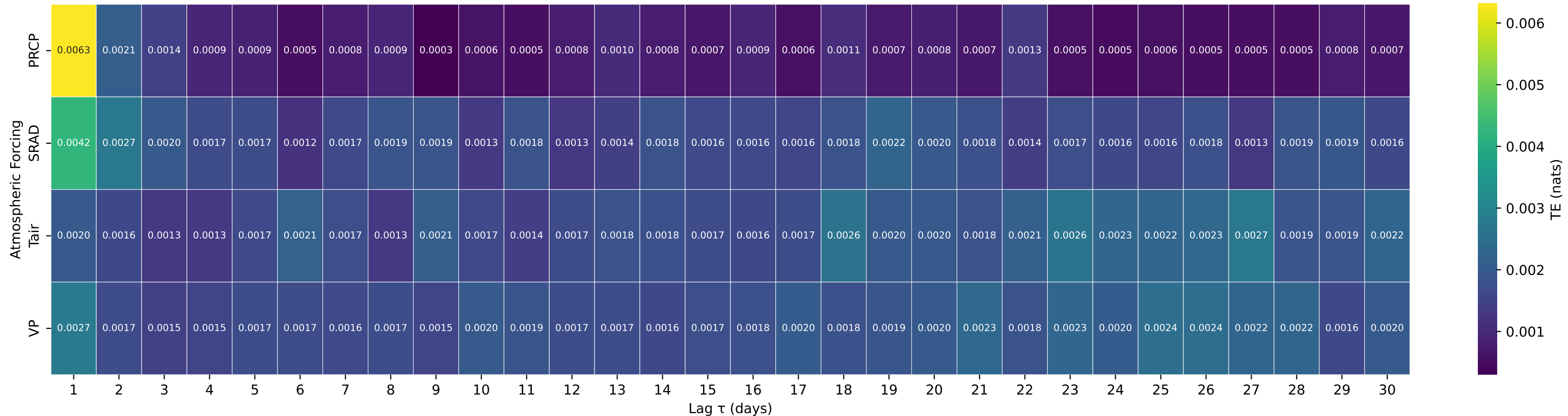
Shuffle-Test Significant TE to Streamflow — Basin 02472500 (HUC 03) — BOUIE CREEK NR HATTIESBURG, MS
