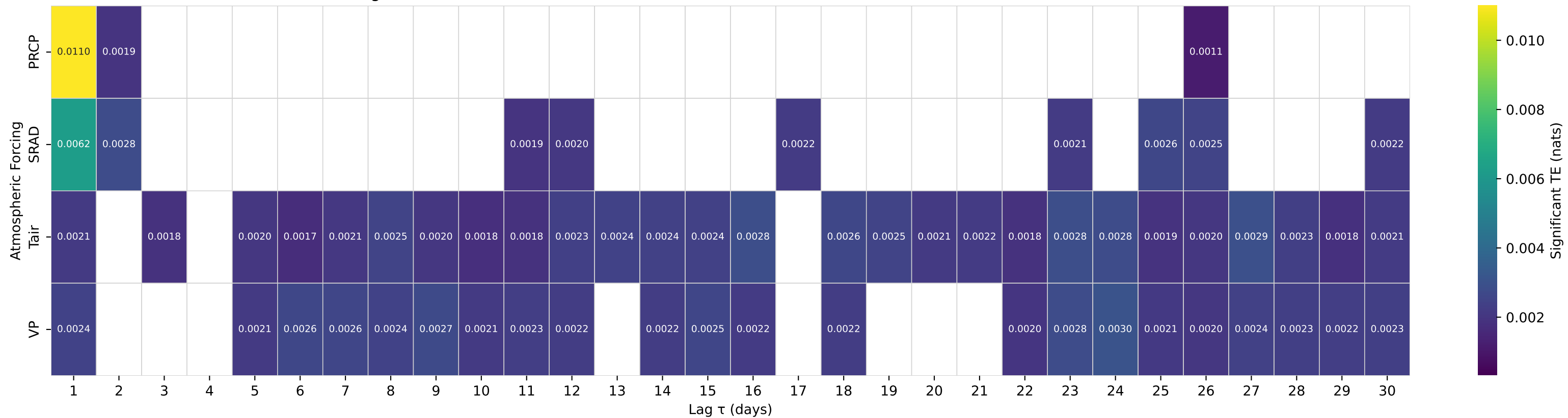
Shuffle-Test Significant TE to Streamflow — Basin 02427250 (HUC 03) — PINE BARREN CREEK NEAR SNOW HILL, AL.
