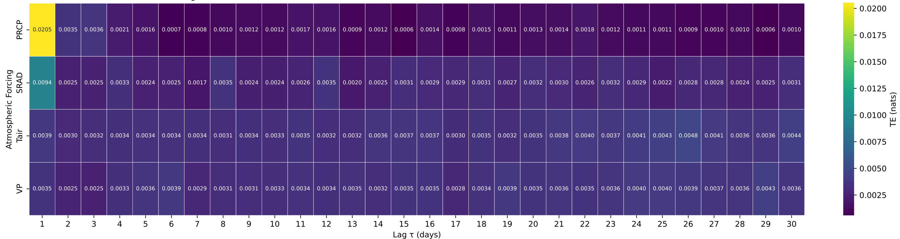
Shuffle-Test Significant TE to Streamflow — Basin 02051500 (HUC 03) — MEHERRIN RIVER NEAR LAWRENCEVILLE, VA
