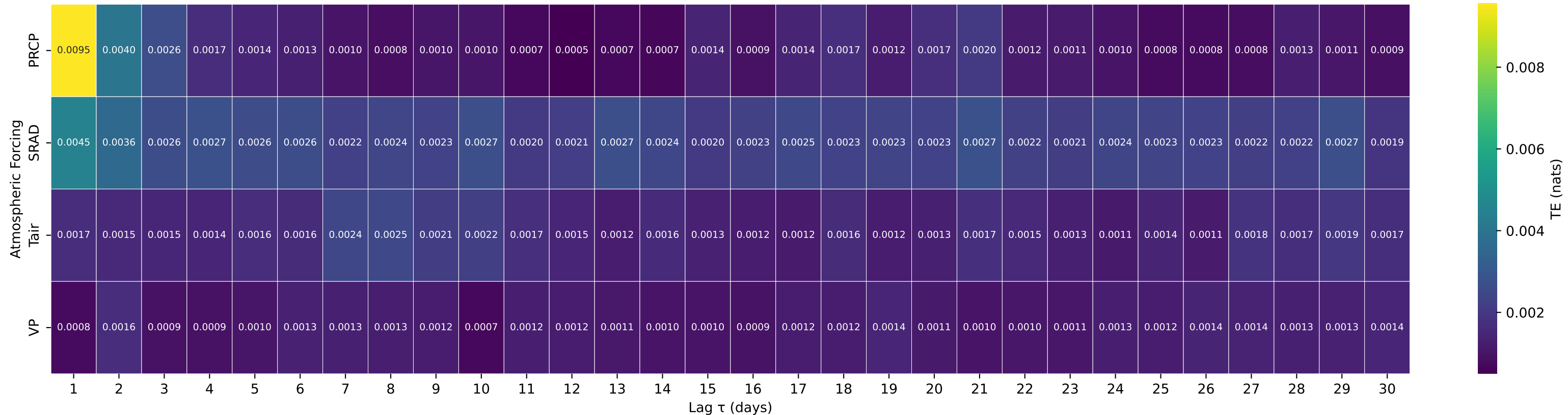
Shuffle-Test Significant TE to Streamflow — Basin 12092000 (HUC 17) — PUYALLUP RIVER NEAR ELECTRON, WA
