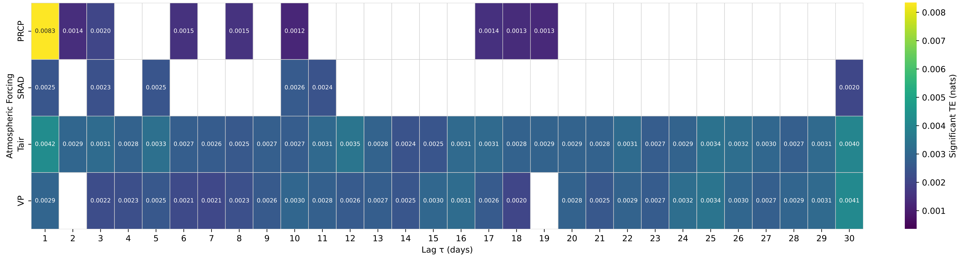
Shuffle-Test Significant TE to Streamflow — Basin 01162500 (HUC 01) — PRIEST BROOK NEAR WINCHENDON, MA
