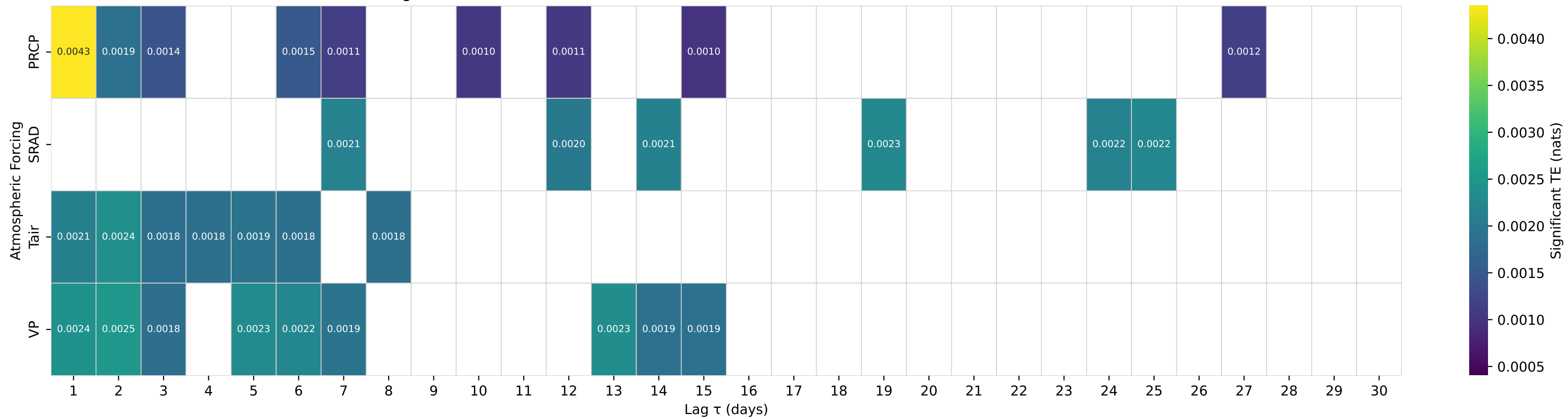
Shuffle-Test Significant TE to Streamflow — Basin 05487980 (HUC 07) — White Breast Creek near Dallas, IA
