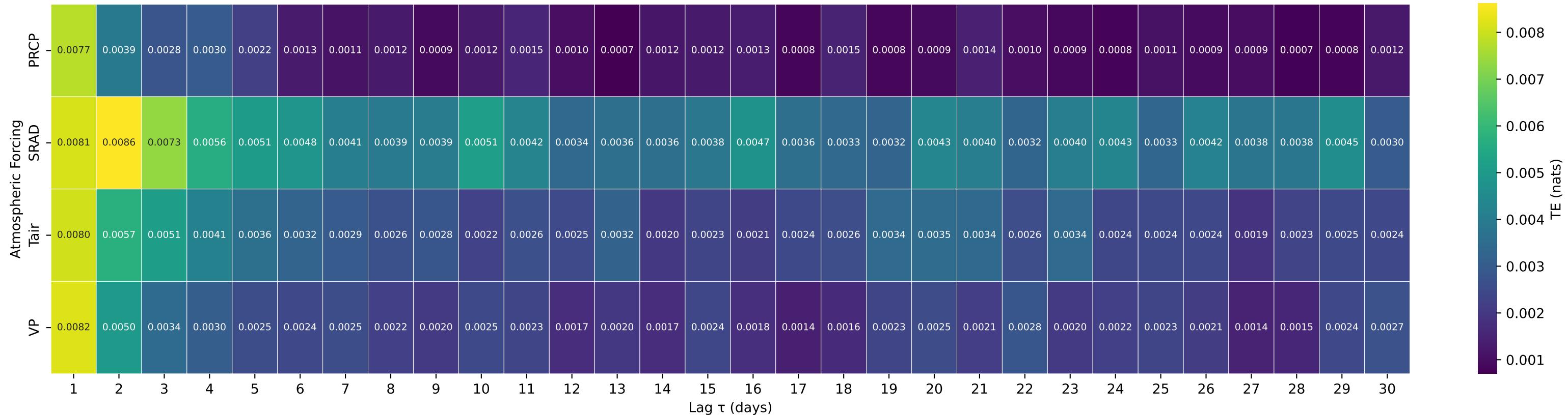
Shuffle-Test Significant TE to Streamflow — Basin 12175500 (HUC 17) — THUNDER CREEK NEAR NEWHALEM, WA
