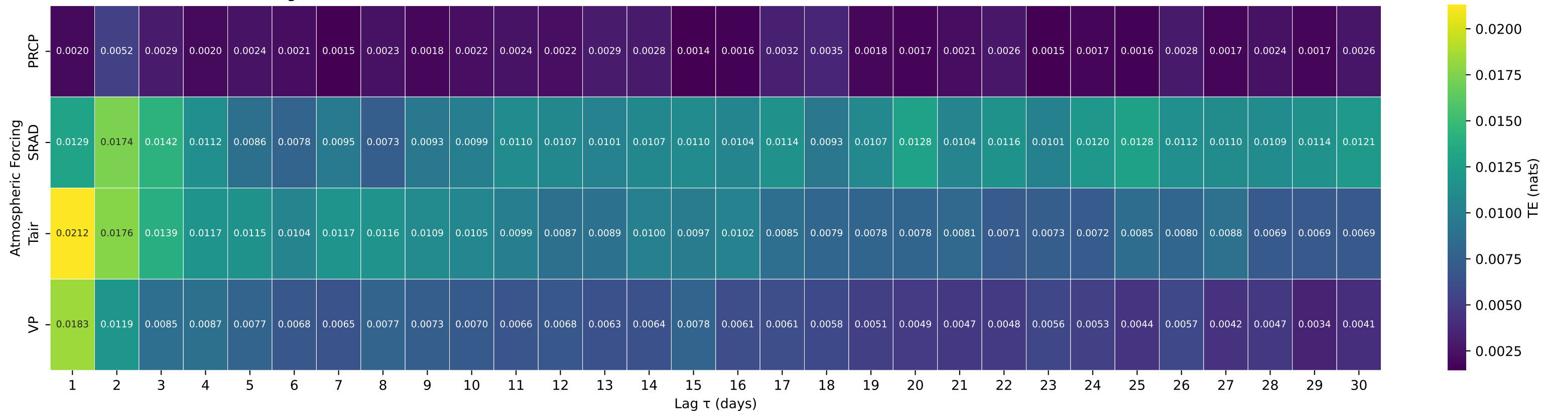
Shuffle-Test Significant TE to Streamflow — Basin 06221400 (HUC 10) — DINWOODY CREEK ABOVE LAKES, NEAR BURRIS, WYO.
