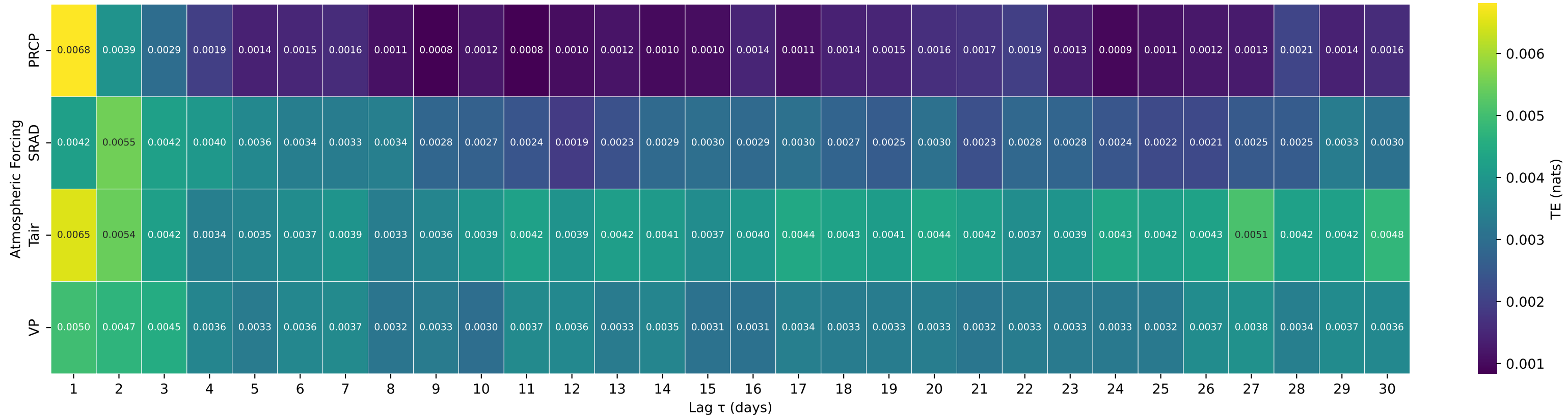
Shuffle-Test Significant TE to Streamflow — Basin 12411000 (HUC 17) — NF COEUR D ALENE R AB SHOSHONE CK NR PRICHARD ID
