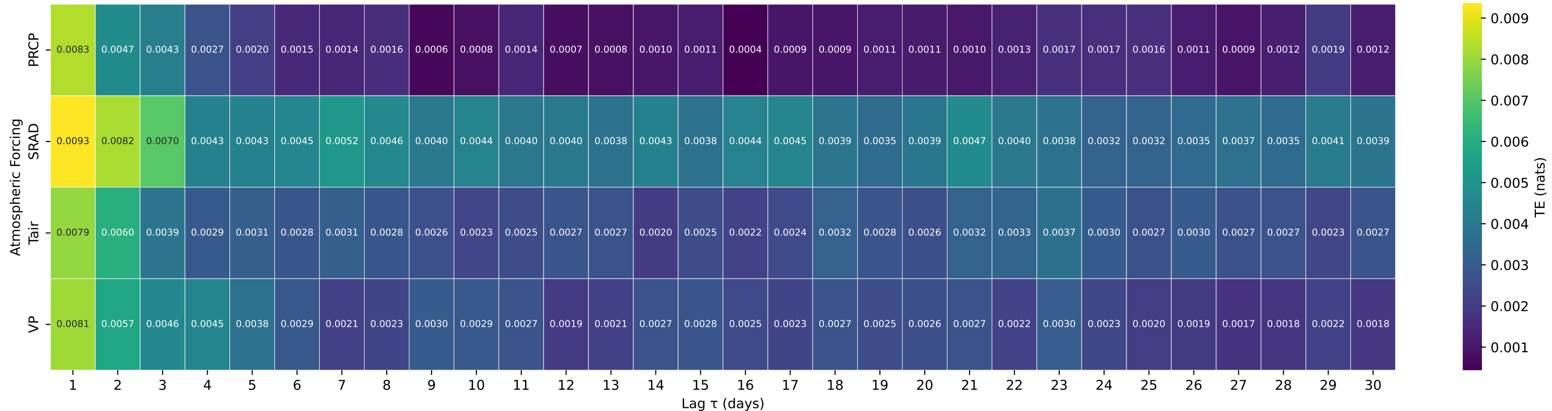
Shuffle-Test Significant TE to Streamflow — Basin 12488500 (HUC 17) — AMERICAN RIVER NEAR NILE, WA
