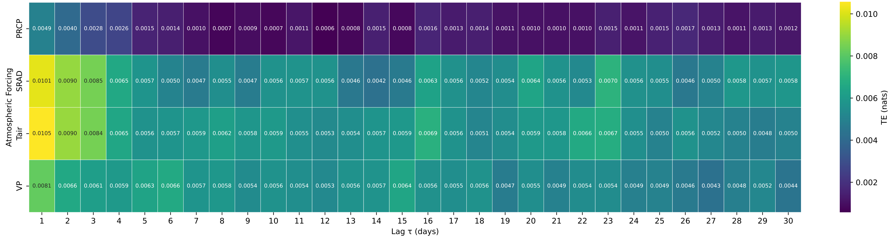
Shuffle-Test Significant TE to Streamflow — Basin 09352900 (HUC 14) — VALLECITO CREEK NEAR BAYFIELD, CO.
