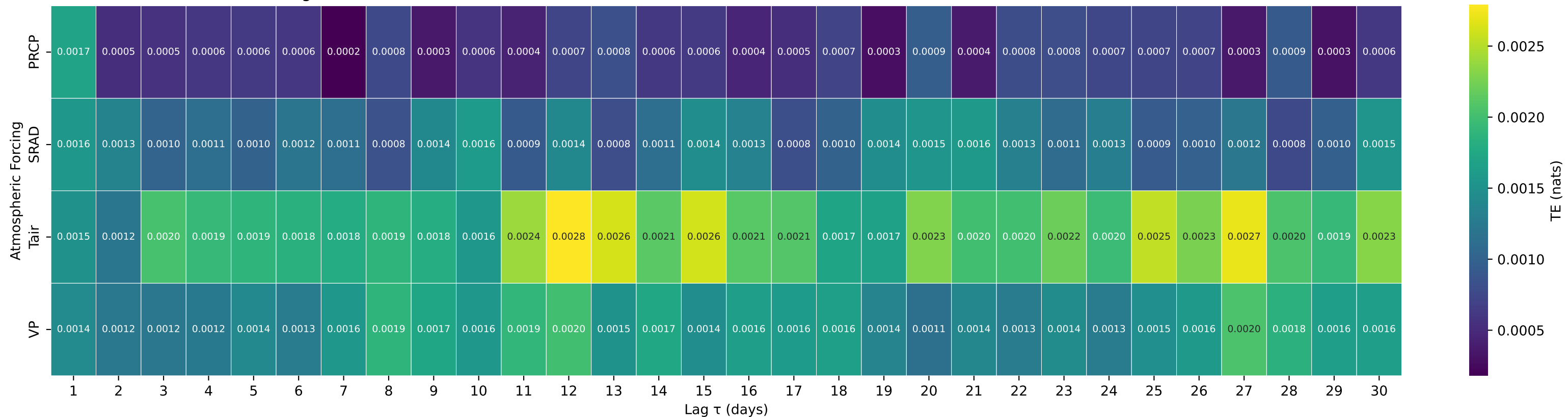
Shuffle-Test Significant TE to Streamflow — Basin 01434025 (HUC 02) — BISCUIT BK ABOVE PIGEON BK AT FROST VALLEY NY
