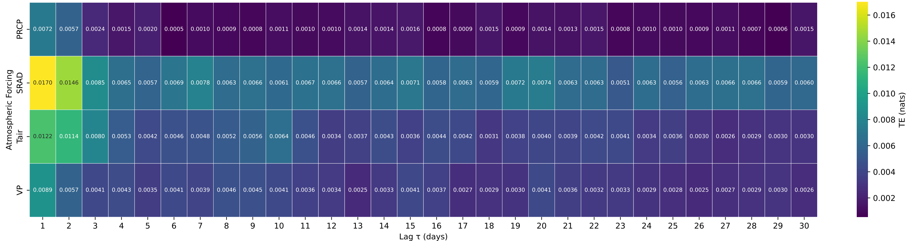
Shuffle-Test Significant TE to Streamflow — Basin 12451000 (HUC 17) — STEHEKIN RIVER AT STEHEKIN, WA
