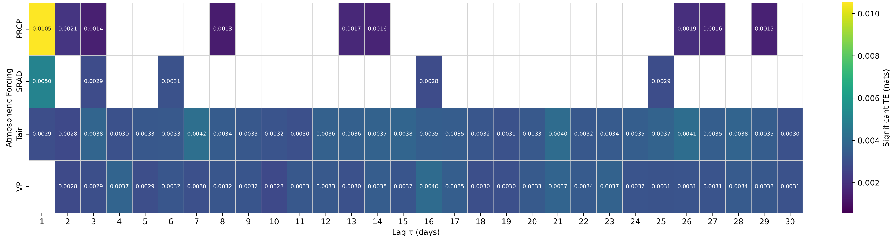
Shuffle-Test Significant TE to Streamflow — Basin 01487000 (HUC 02) — NANTICOKE RIVER NEAR BRIDGEVILLE, DE
