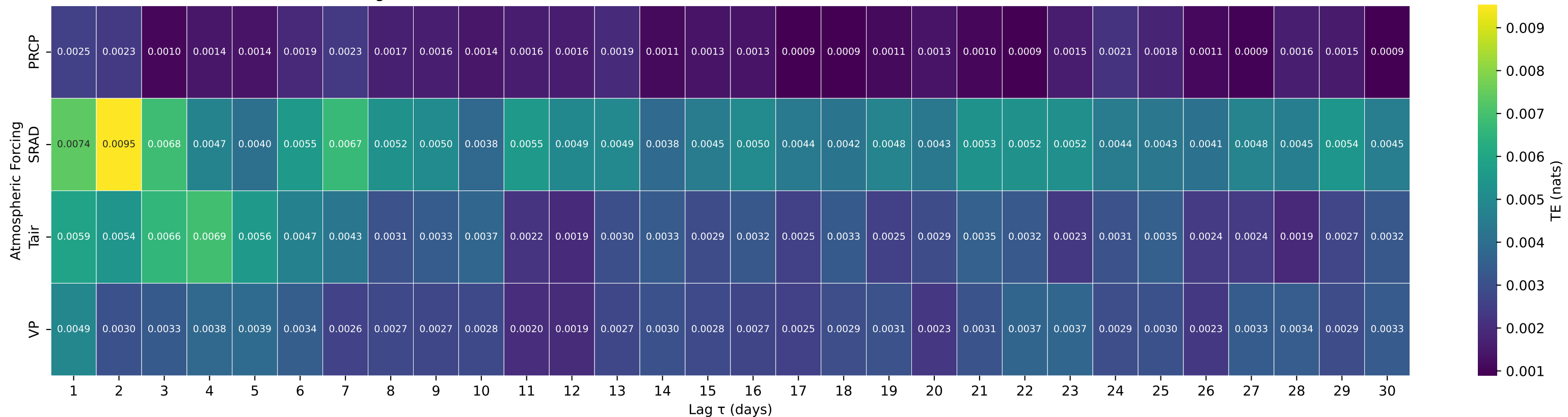
Shuffle-Test Significant TE to Streamflow — Basin 12388400 (HUC 17) — Revais Cr bl West Fork nr Dixon MT
