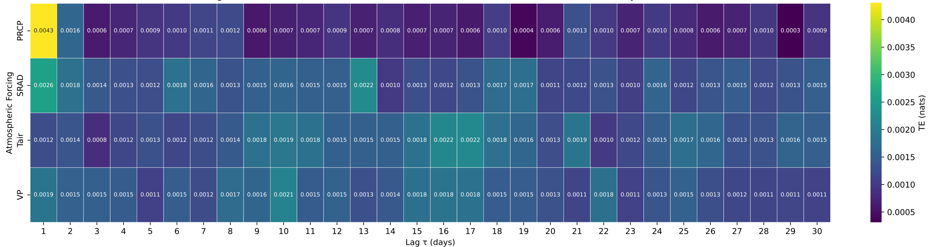
Shuffle-Test Significant TE to Streamflow — Basin 07071500 (HUC 11) — Eleven Point River near Bardley, MO
