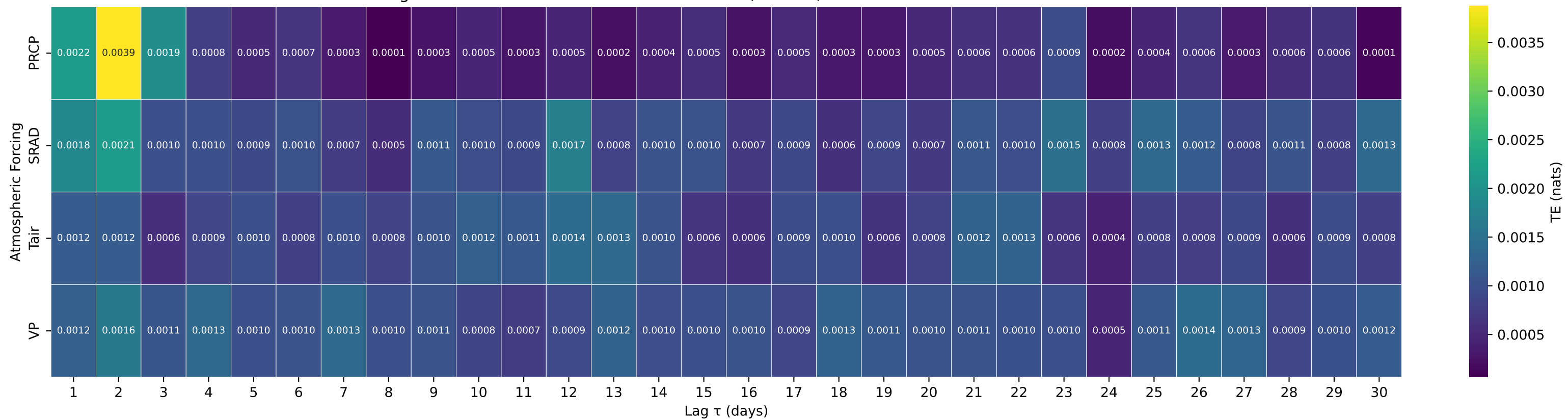
Shuffle-Test Significant TE to Streamflow — Basin 02363000 (HUC 03) — PEA RIVER NEAR ARITON AL
