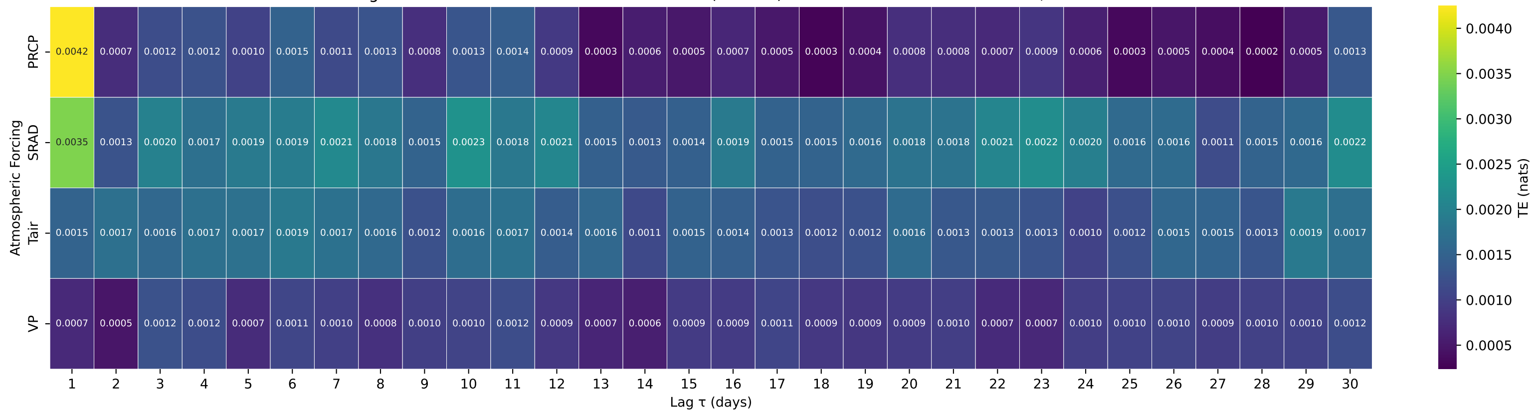
Shuffle-Test Significant TE to Streamflow — Basin 09497980 (HUC 15) — CHERRY CREEK NEAR GLOBE, AZ.
