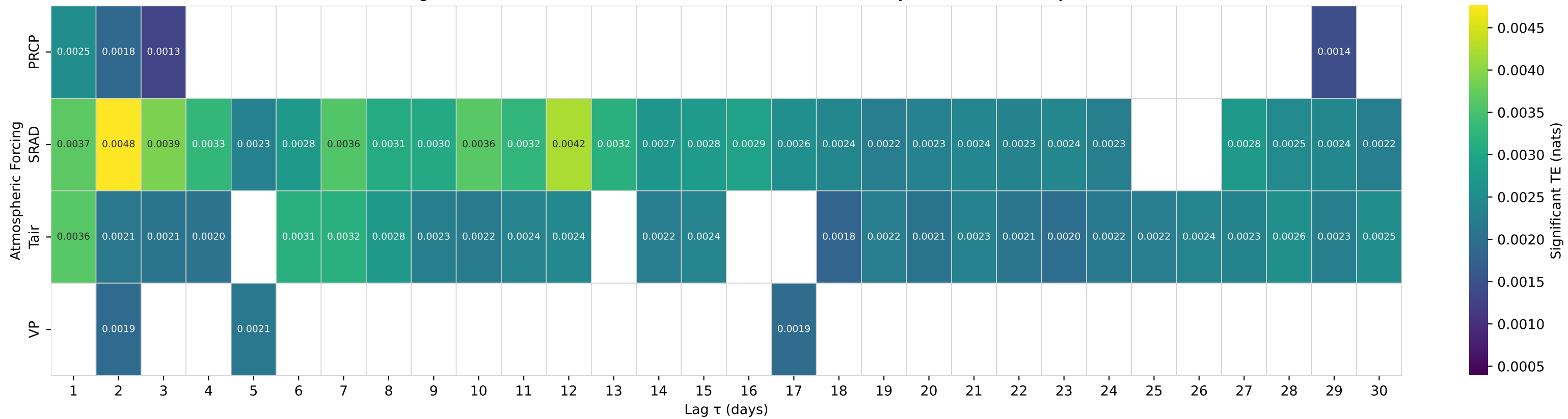
Shuffle-Test Significant TE to Streamflow — Basin 08324000 (HUC 13) — JEMEZ RIVER NEAR JEMEZ, NM
