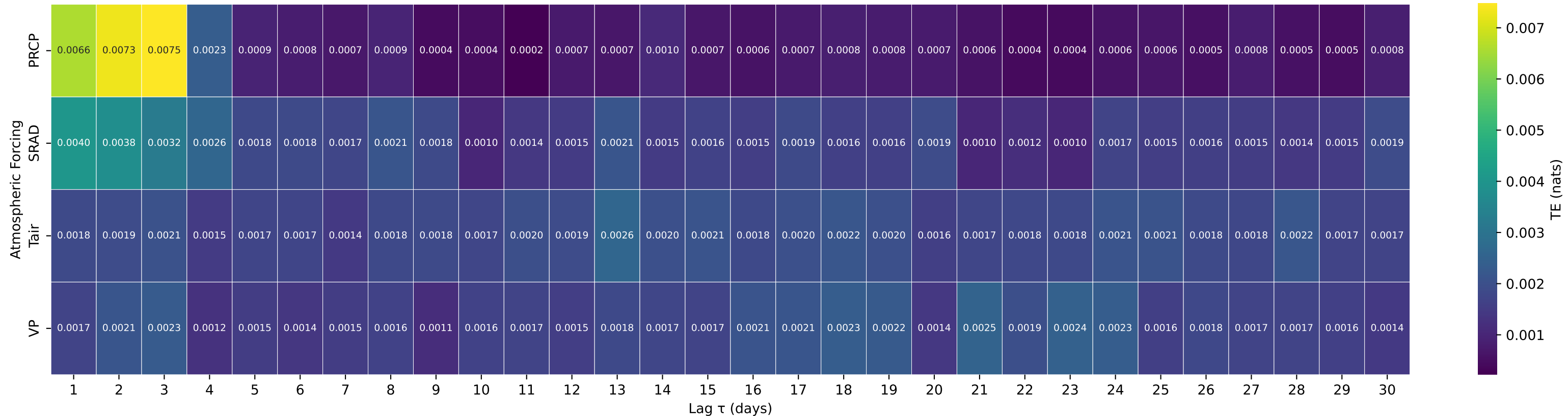
Shuffle-Test Significant TE to Streamflow — Basin 08013000 (HUC 08) — CALCASIEU RIVER NR GLENMORA, LA
