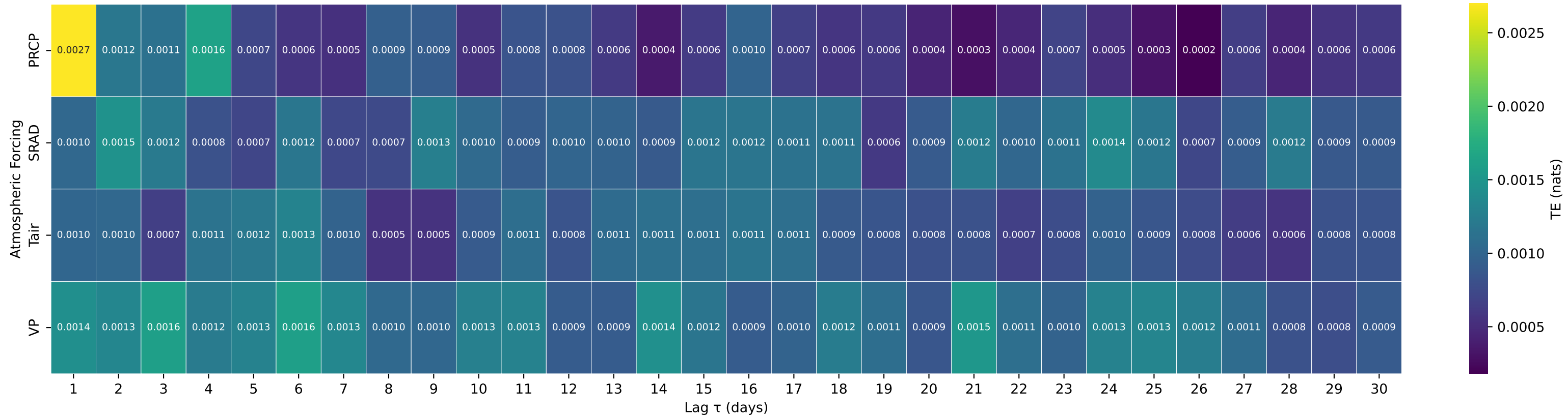
Shuffle-Test Significant TE to Streamflow — Basin 07301500 (HUC 11) — North Fork Red River near Carter, OK
