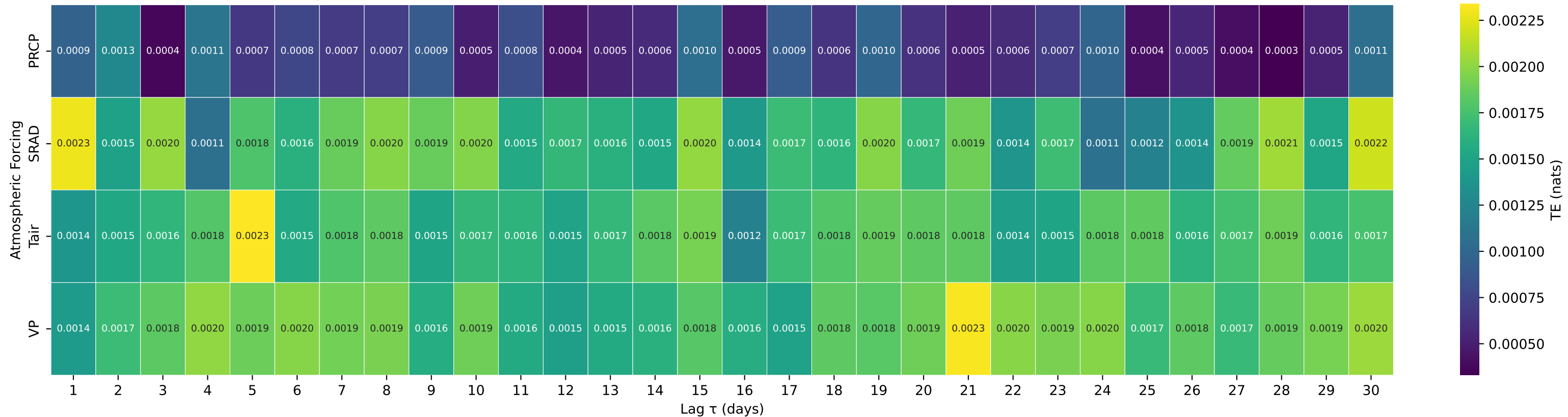
Shuffle-Test Significant TE to Streamflow — Basin 02051000 (HUC 03) — NORTH MEHERRIN RIVER NEAR LUNENBURG, VA
