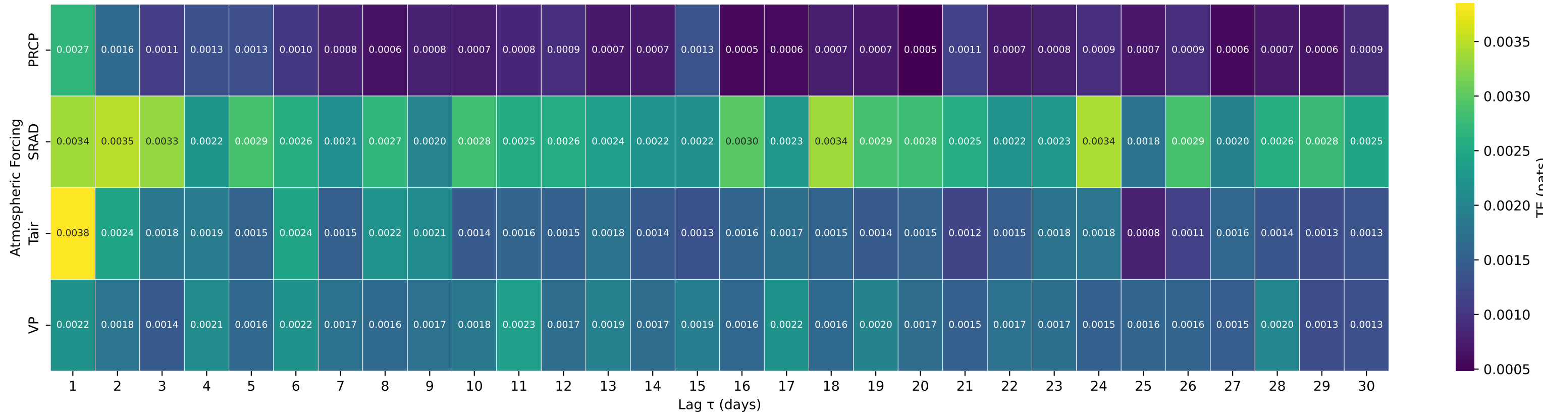
Shuffle-Test Significant TE to Streamflow — Basin 08377900 (HUC 13) — RIO MORA NEAR TERRERO, NM
