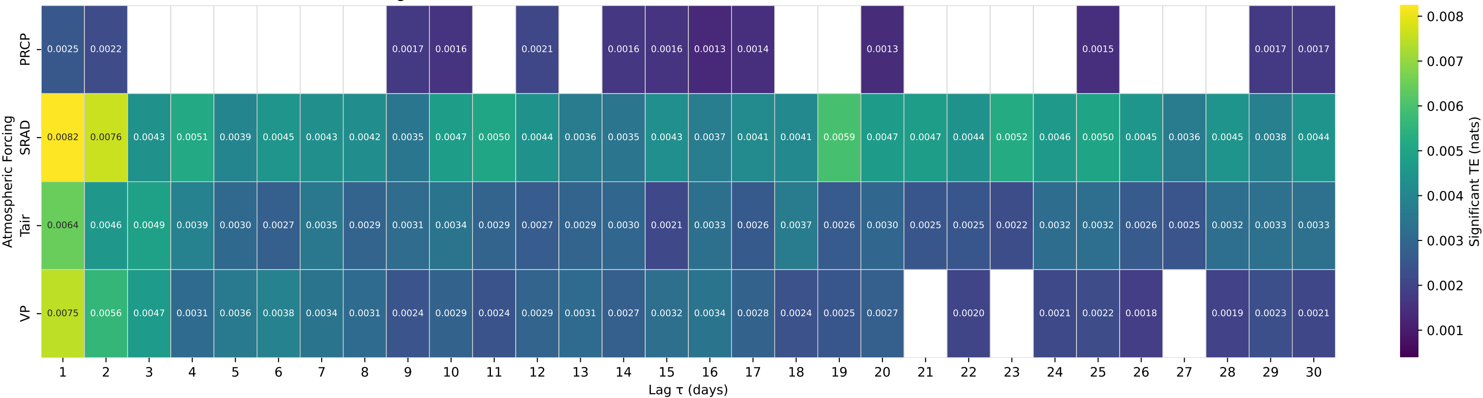
Shuffle-Test Significant TE to Streamflow — Basin 10316500 (HUC 16) — LAMOILLE C NR LAMOILLE, NV
