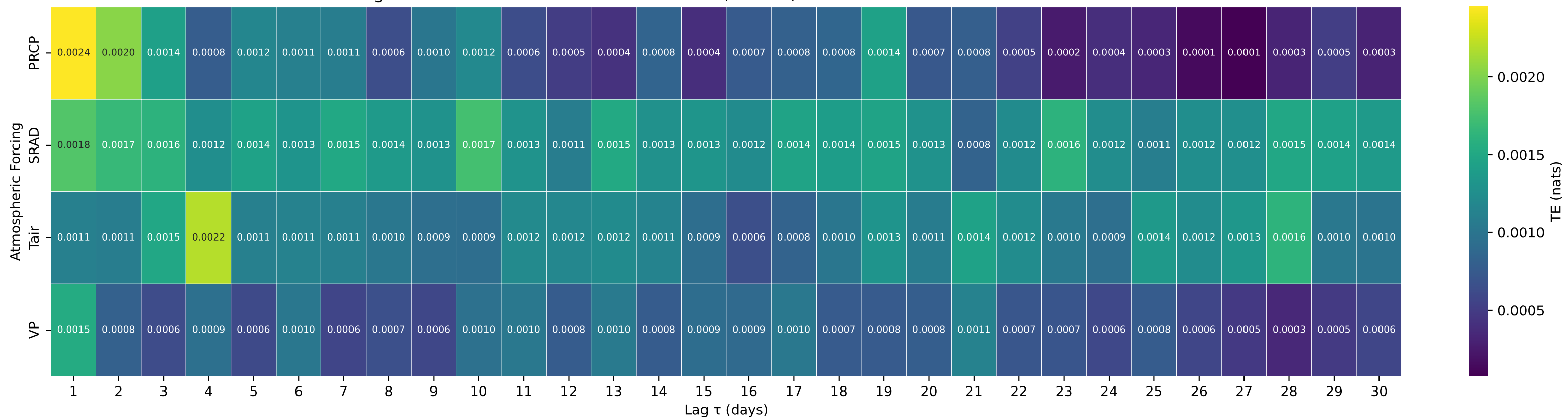
Shuffle-Test Significant TE to Streamflow — Basin 10258500 (HUC 18) — PALM CYN C NR PALM SPRINGS CA
