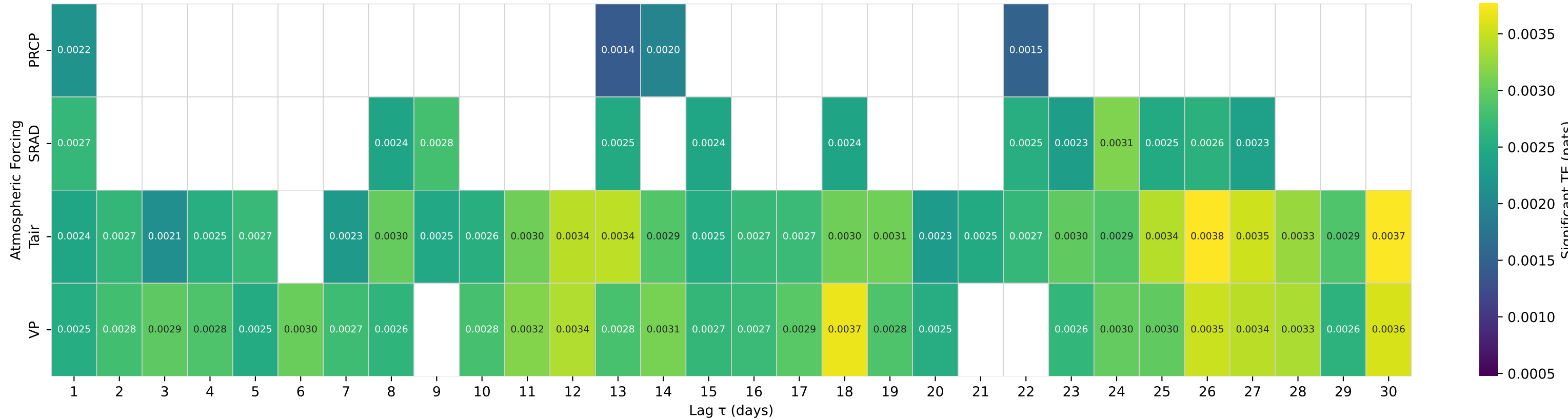
Shuffle-Test Significant TE to Streamflow — Basin 07295000 (HUC 08) — BUFFALO RIVER NR WOODVILLE, MS
