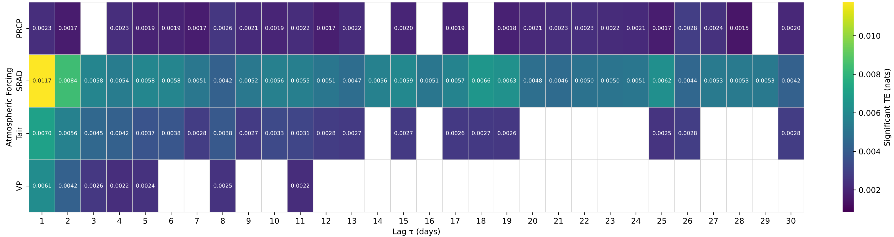
Shuffle-Test Significant TE to Streamflow — Basin 06278300 (HUC 10) — SHELL CREEK ABOVE SHELL CREEK RESERVOIR, WY
