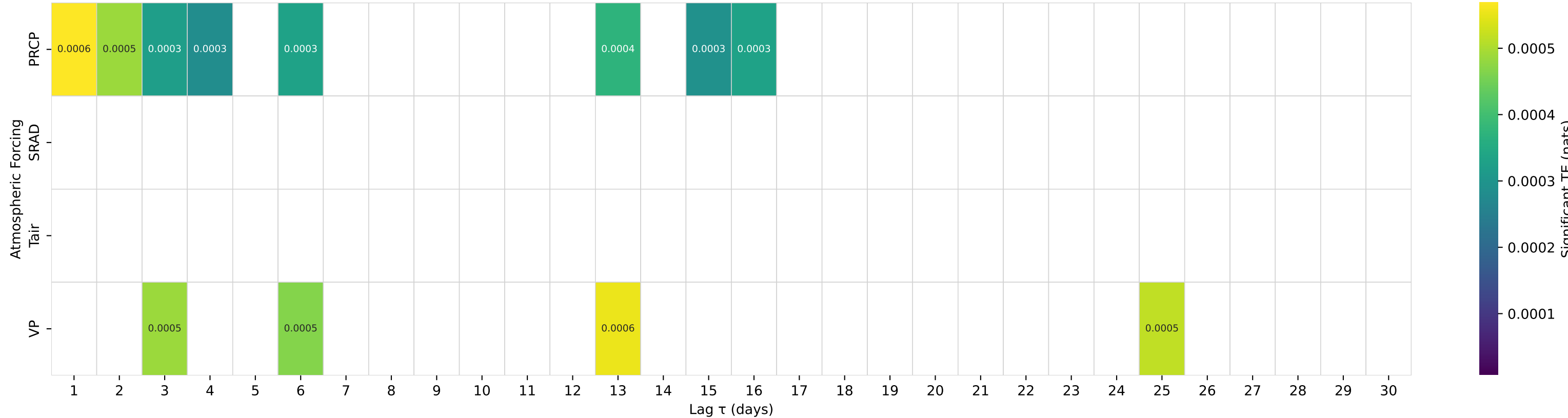
Shuffle-Test Significant TE to Streamflow — Basin 08200000 (HUC 12) — Hondo Ck nr Tarpley, TX
