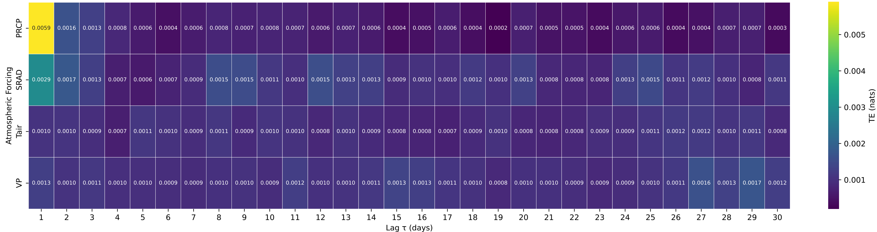
Shuffle-Test Significant TE to Streamflow — Basin 07375000 (HUC 08) — Tchefuncta River near Folsom, LA
