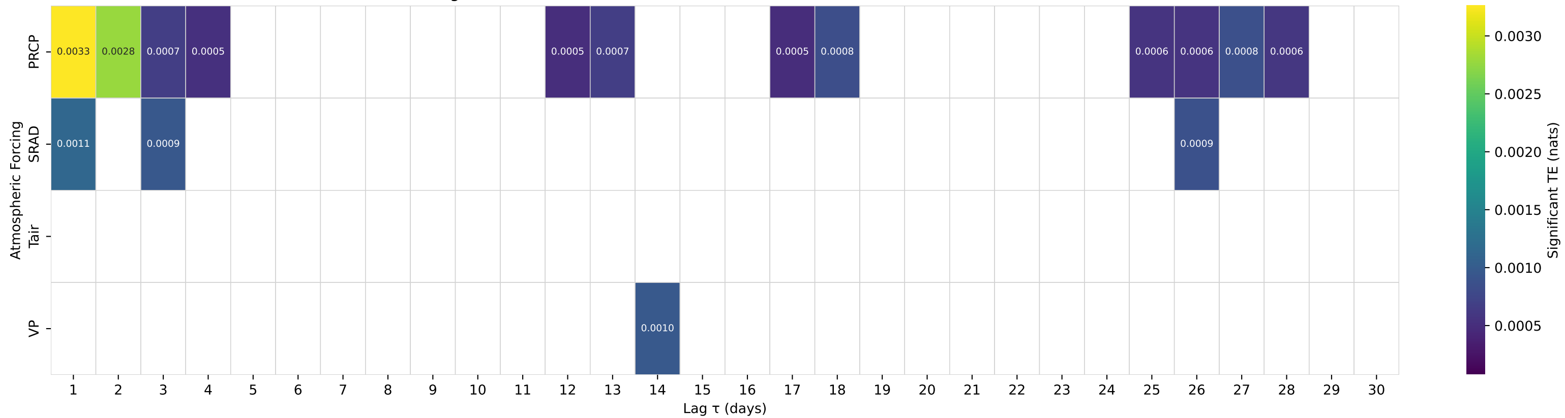
Shuffle-Test Significant TE to Streamflow — Basin 08164000 (HUC 12) — Lavaca Rv nr Edna, TX
