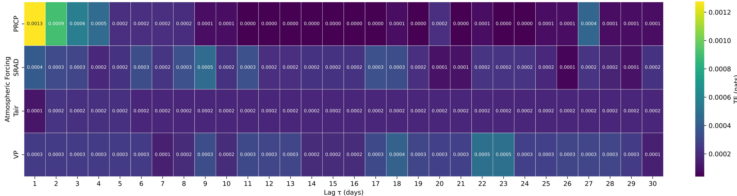
Shuffle-Test Significant TE to Streamflow — Basin 08178880 (HUC 12) — Medina Rv at Bandera, TX
