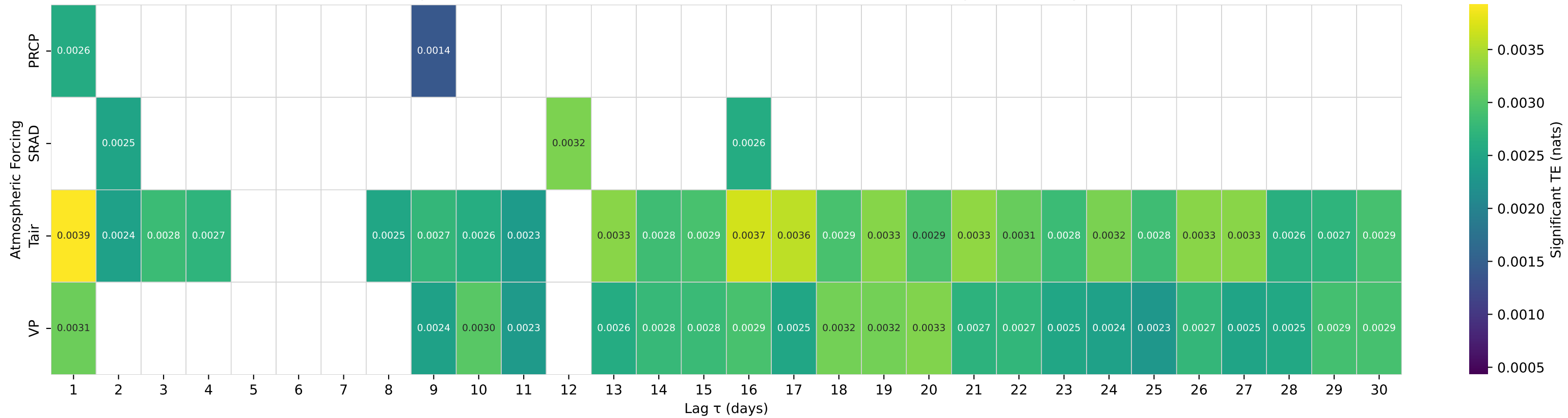
Shuffle-Test Significant TE to Streamflow — Basin 01557500 (HUC 02) — Bald Eagle Creek at Tyrone, PA
