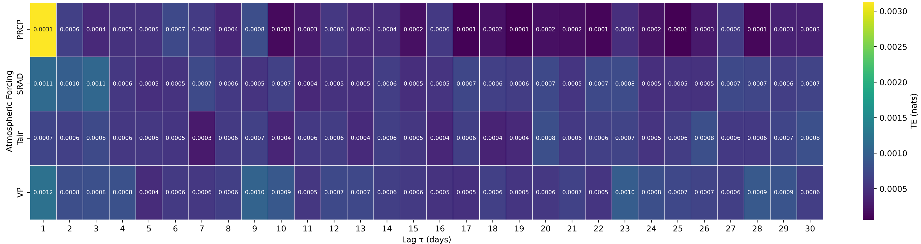
Shuffle-Test Significant TE to Streamflow — Basin 07315200 (HUC 11) — E Fk Little Wichita Rv nr Henrietta, TX
