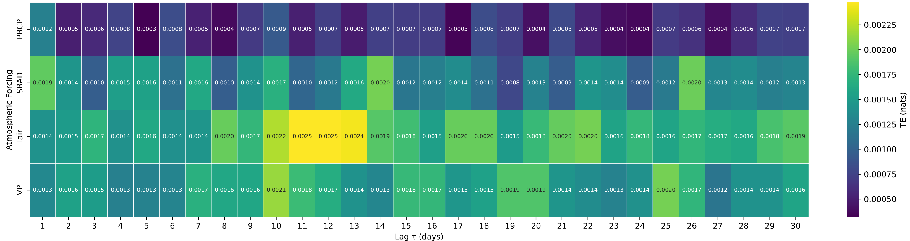
Shuffle-Test Significant TE to Streamflow — Basin 01552500 (HUC 02) — Muncy Creek near Sonestown, PA
