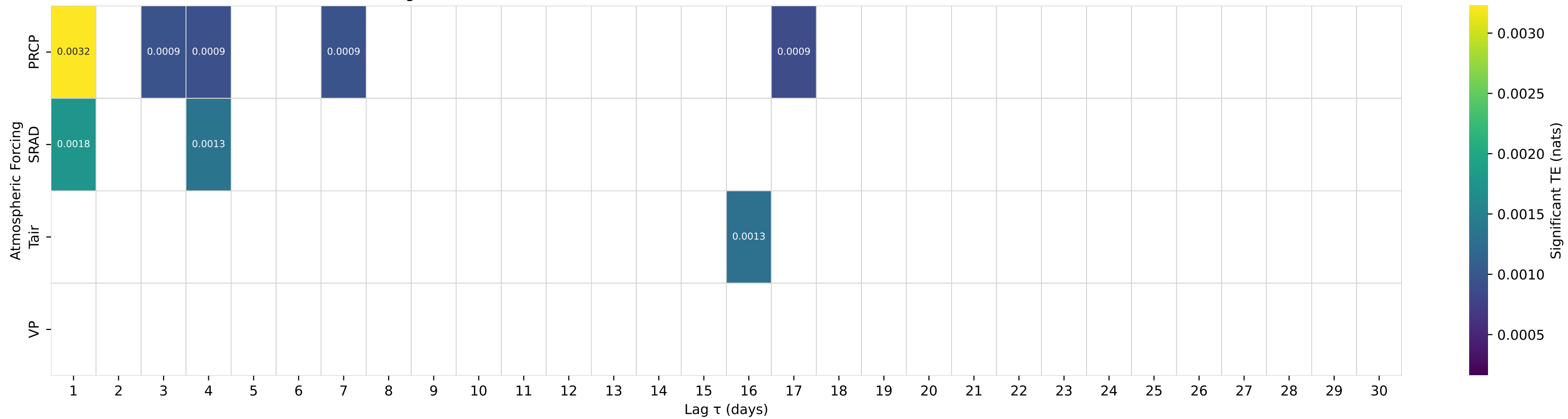
Shuffle-Test Significant TE to Streamflow — Basin 01195100 (HUC 01) — INDIAN RIVER NEAR CLINTON, CT.
