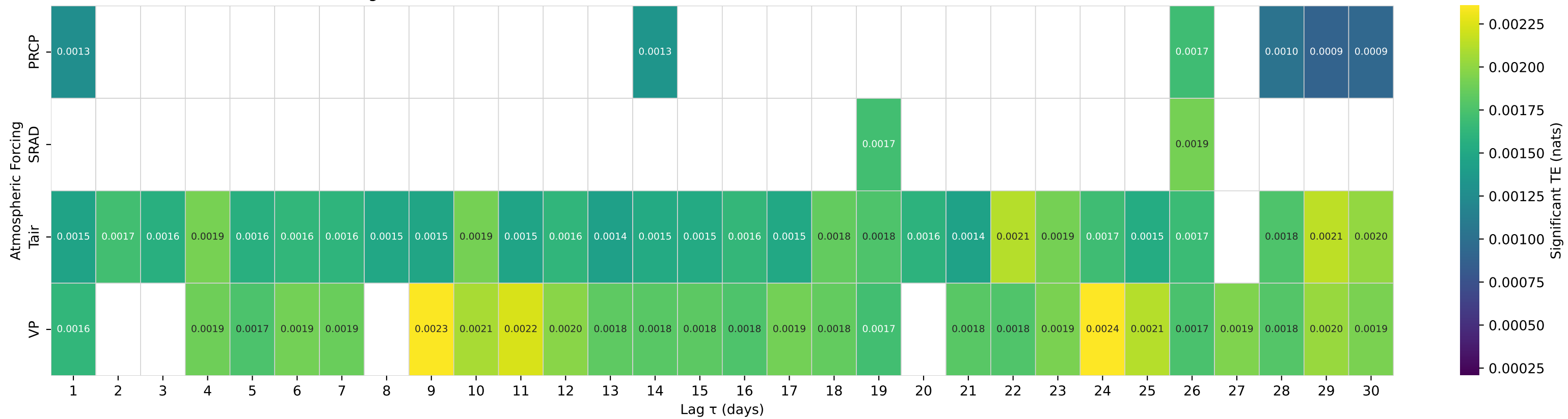
Shuffle-Test Significant TE to Streamflow — Basin 02381600 (HUC 03) — FAUSETT CREEK NEAR TALKING ROCK, GA
