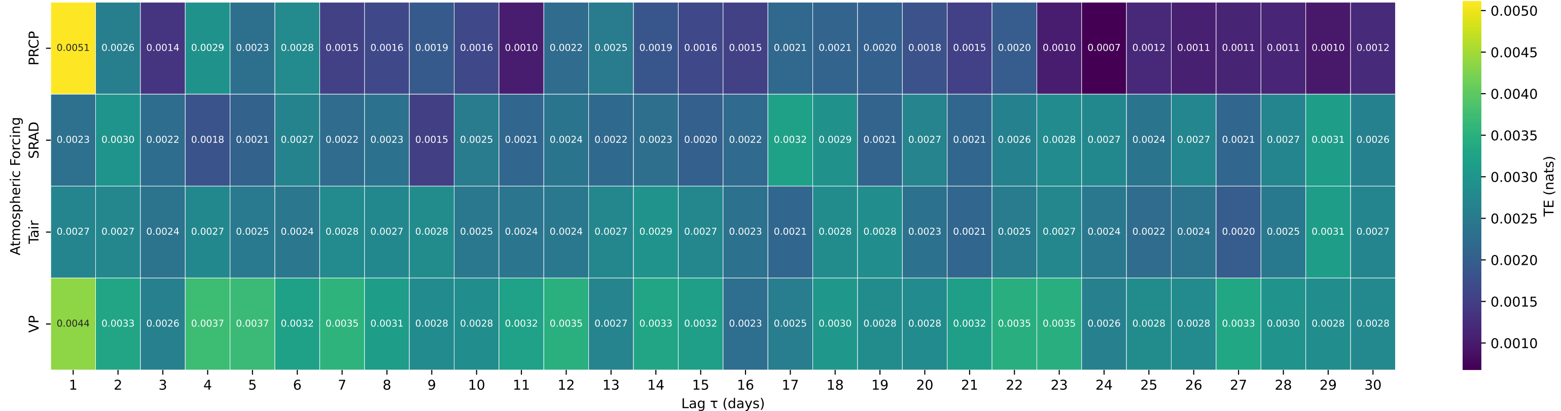
Shuffle-Test Significant TE to Streamflow — Basin 06885500 (HUC 10) — BLACK VERMILLION R NR FRANKFORT, KS
