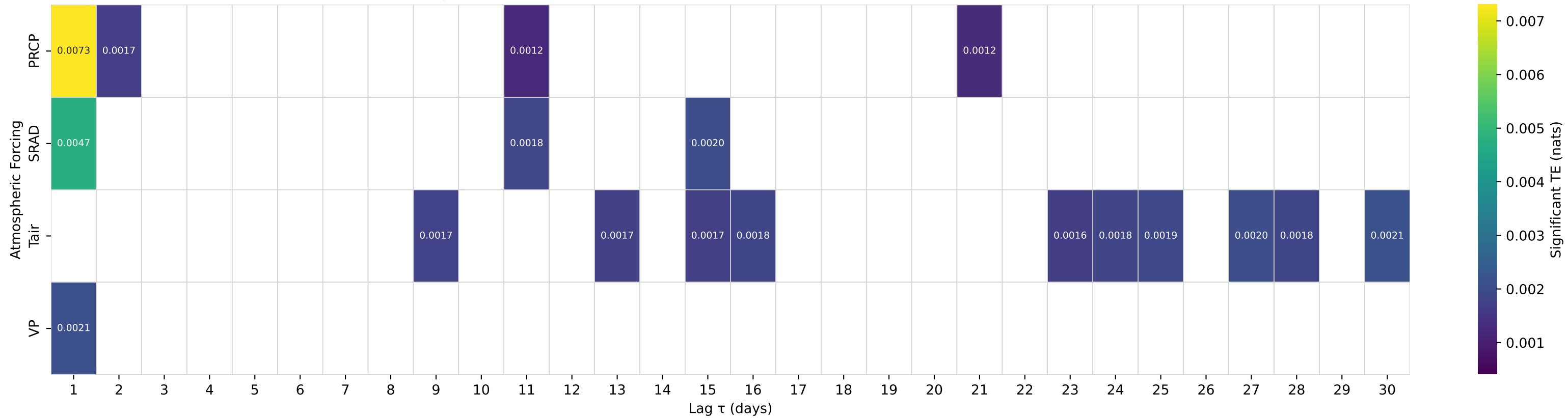
Shuffle-Test Significant TE to Streamflow — Basin 02018000 (HUC 02) — CRAIG CREEK AT PARR, VA
