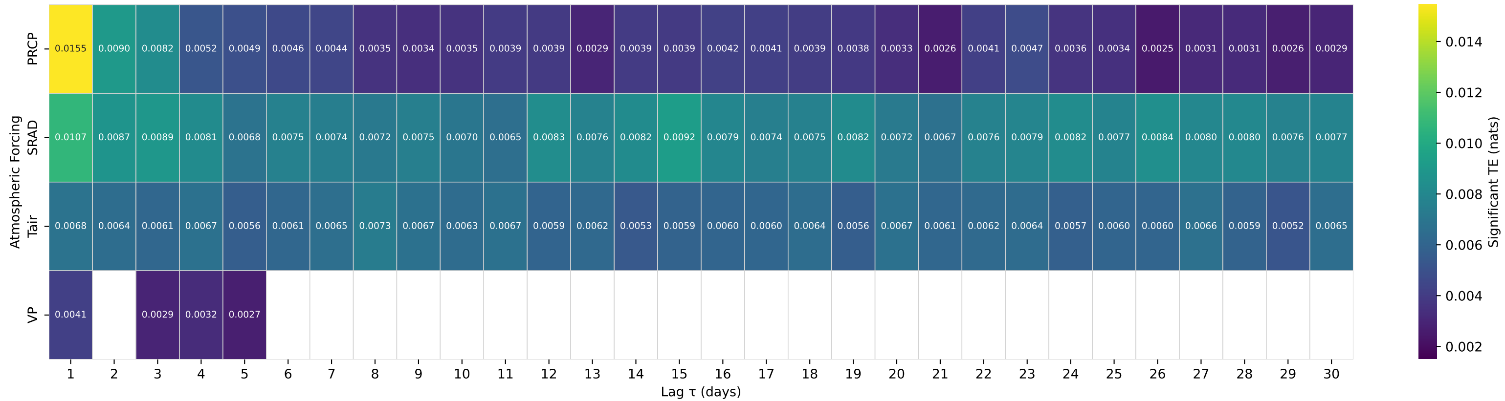
Shuffle-Test Significant TE to Streamflow — Basin 11478500 (HUC 18) — VAN DUZEN R NR BRIDGEVILLE CA
