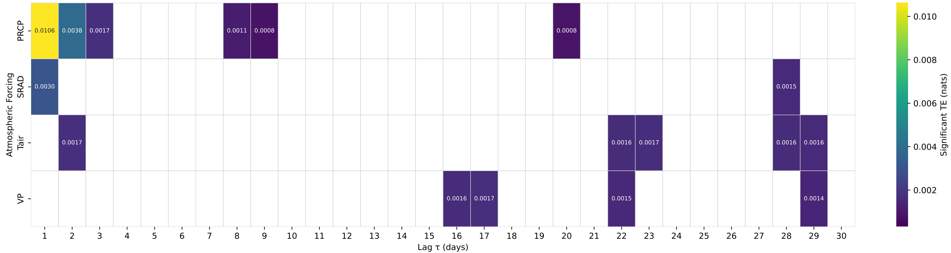
Shuffle-Test Significant TE to Streamflow — Basin 01485500 (HUC 02) — NASSAWANGO CREEK NEAR SNOW HILL, MD
