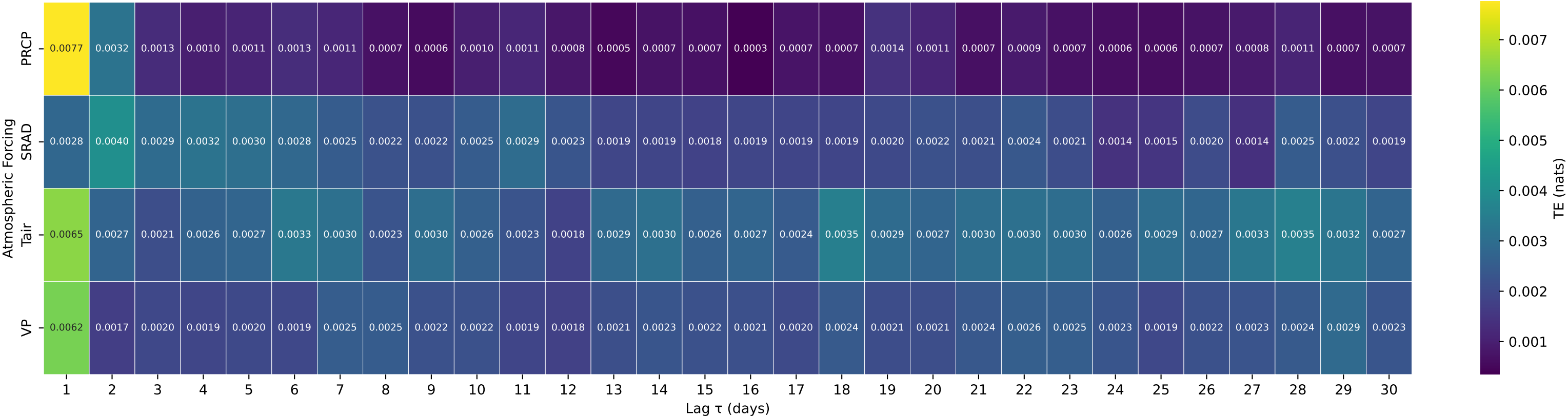
Shuffle-Test Significant TE to Streamflow — Basin 01134500 (HUC 01) — MOOSE RIVER AT VICTORY, VT
