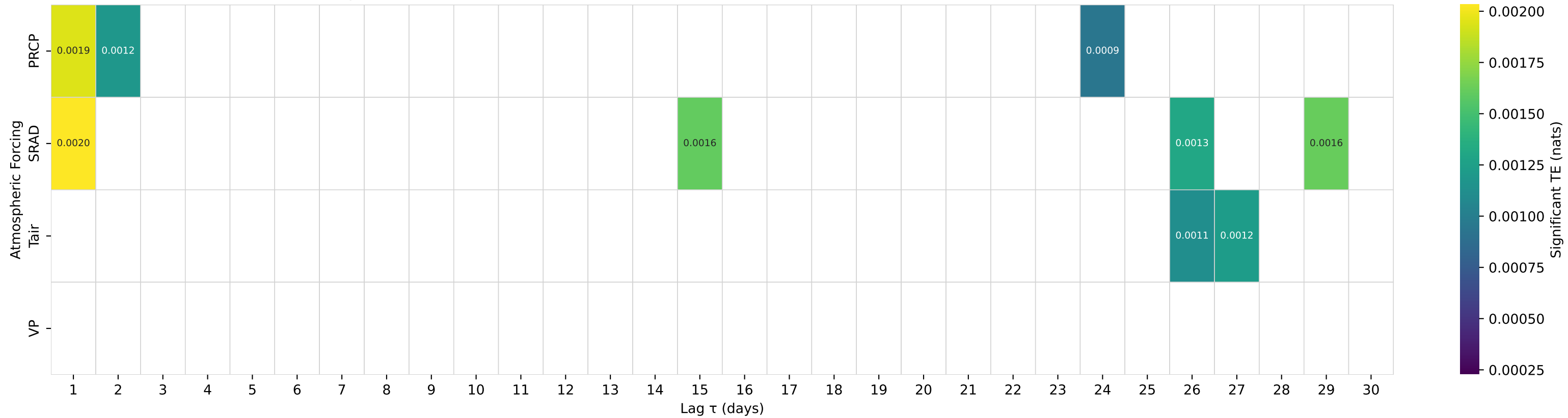
Shuffle-Test Significant TE to Streamflow — Basin 03161000 (HUC 05) — SOUTH FORK NEW RIVER NEAR JEFFERSON, NC
