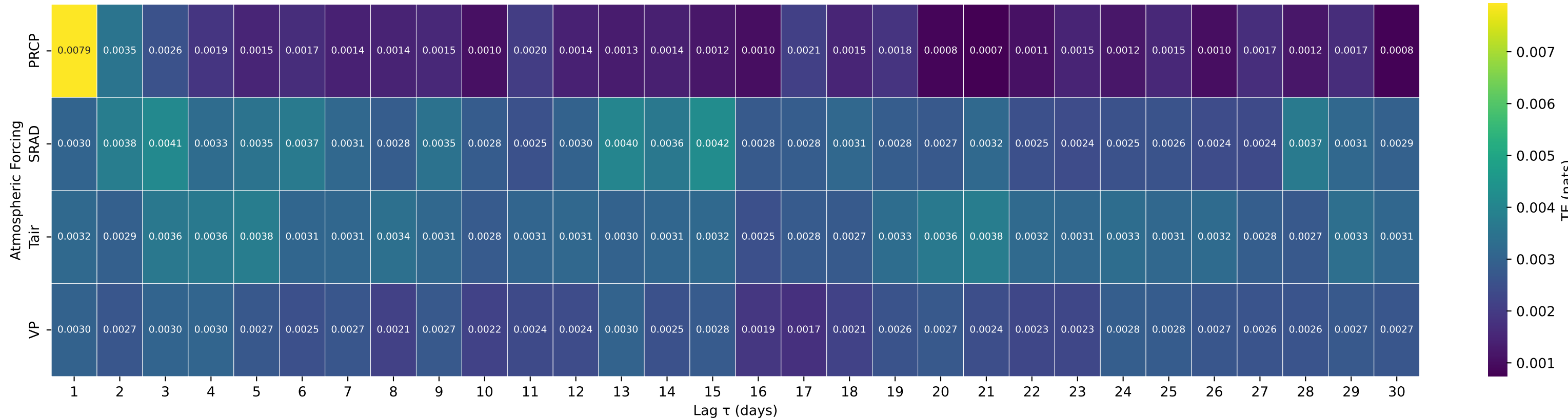
Shuffle-Test Significant TE to Streamflow — Basin 05393500 (HUC 07) — SPIRIT RIVER AT SPIRIT FALLS, WI
