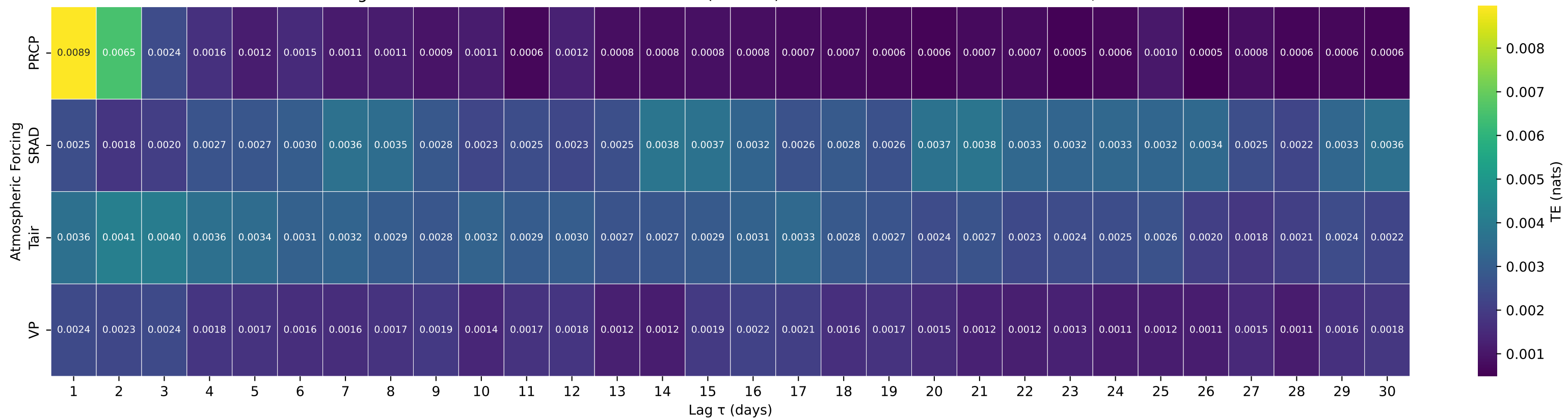
Shuffle-Test Significant TE to Streamflow — Basin 05131500 (HUC 09) — LITTLE FORK RIVER AT LITTLEFORK, MN
