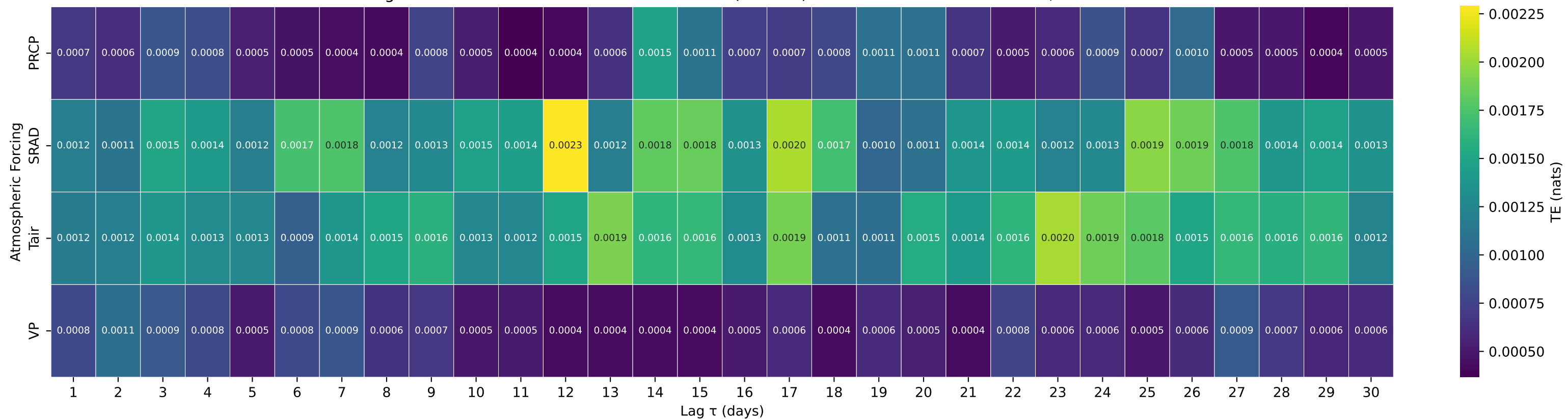
Shuffle-Test Significant TE to Streamflow — Basin 06352000 (HUC 10) — CEDAR CREEK NR HAYNES, ND
