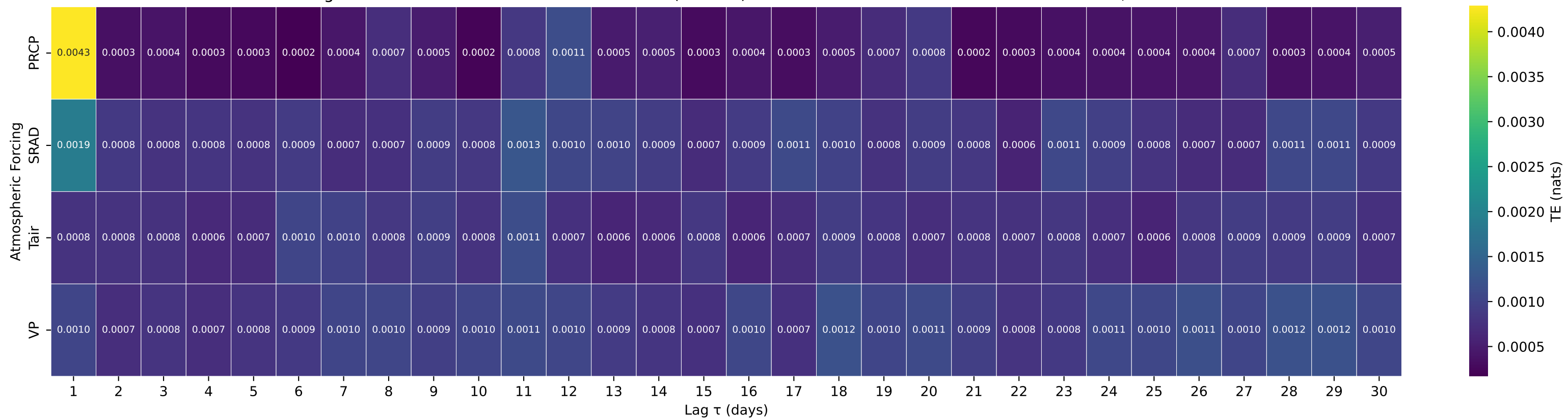
Shuffle-Test Significant TE to Streamflow — Basin 01669000 (HUC 02) — PISCATAWAY CREEK NEAR TAPPAHANNOCK, VA
