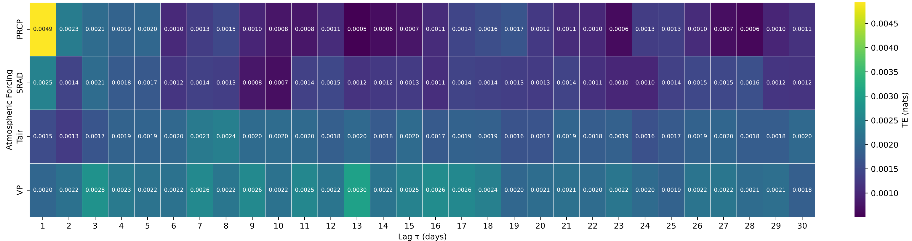
Shuffle-Test Significant TE to Streamflow — Basin 02297155 (HUC 03) — HORSE CREEK NEAR MYAKKA HEAD FL
