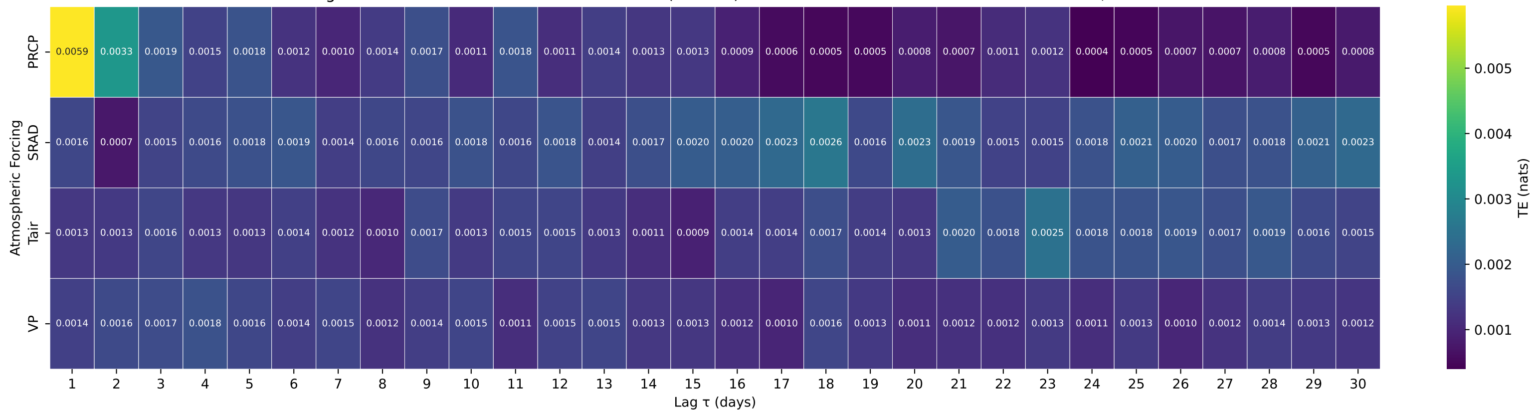
Shuffle-Test Significant TE to Streamflow — Basin 06440200 (HUC 10) — SOUTH FORK BAD R NEAR COTTONWOOD,SD
