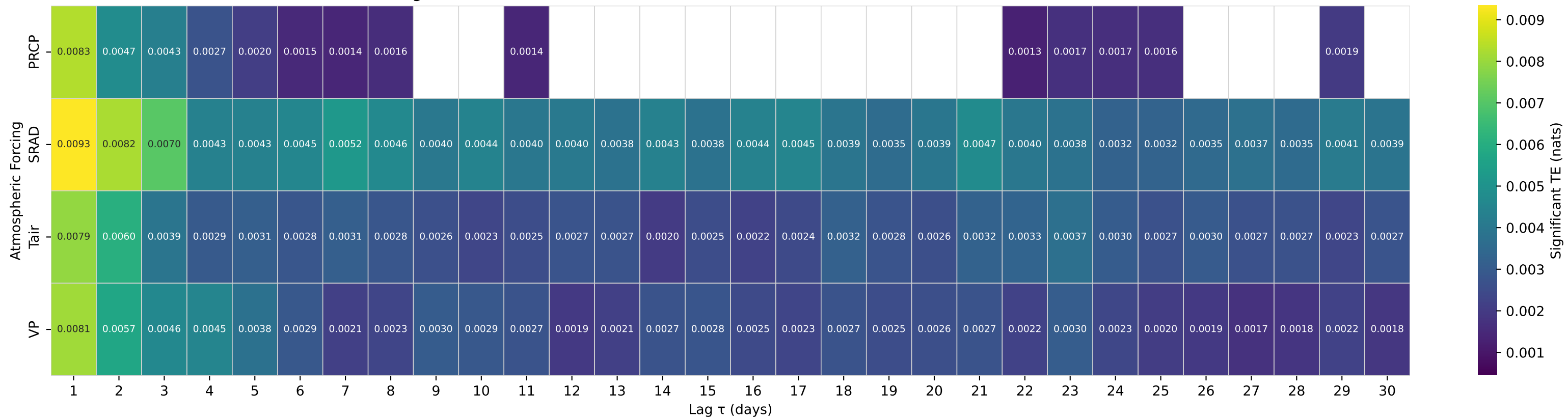
Shuffle-Test Significant TE to Streamflow — Basin 12488500 (HUC 17) — AMERICAN RIVER NEAR NILE, WA
