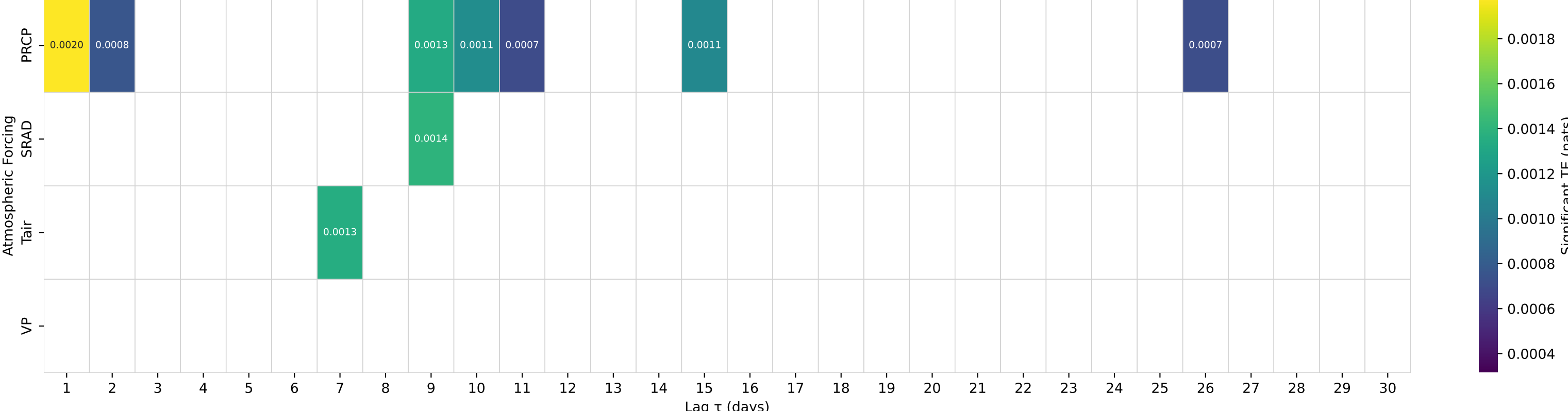
Shuffle-Test Significant TE to Streamflow — Basin 03450000 (HUC 06) — BEETREE CREEK NEAR SWANNANOA, NC
