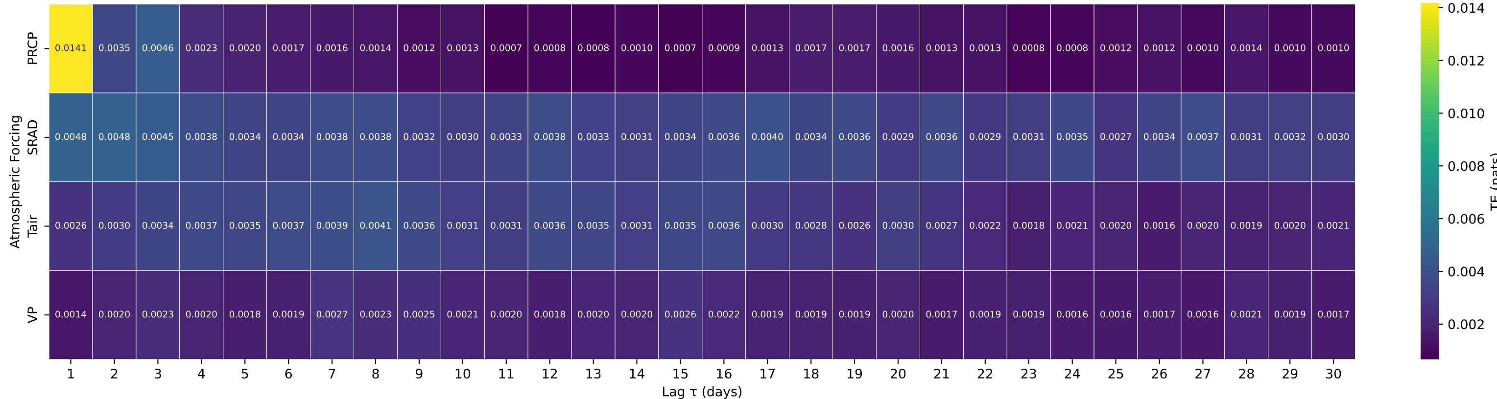
Shuffle-Test Significant TE to Streamflow — Basin 14137000 (HUC 17) — SANDY RIVER NEAR MARMOT, OR
