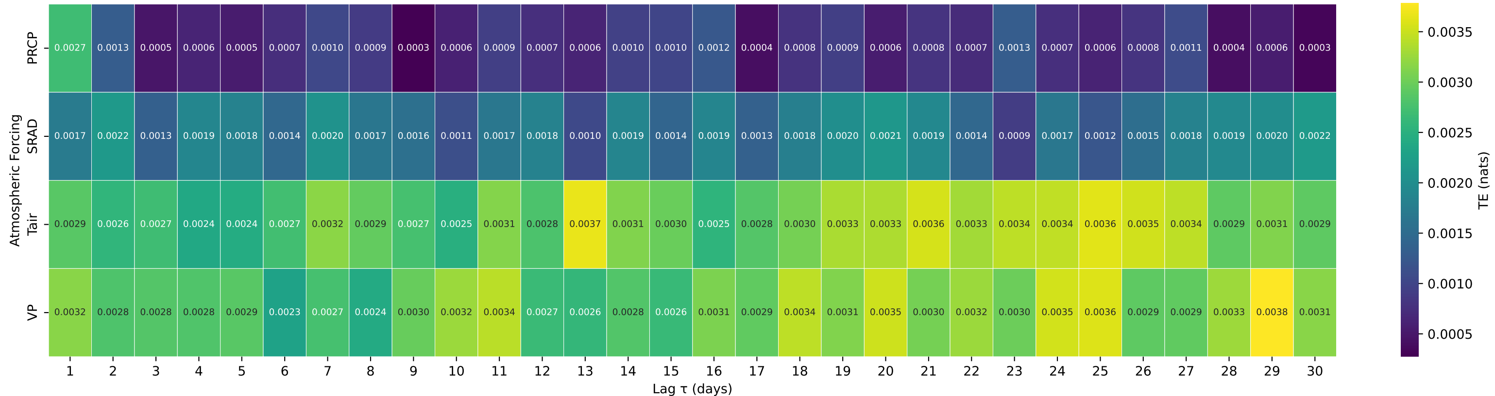
Shuffle-Test Significant TE to Streamflow — Basin 03187500 (HUC 05) — CRANBERRY RIVER NEAR RICHWOOD, WV
