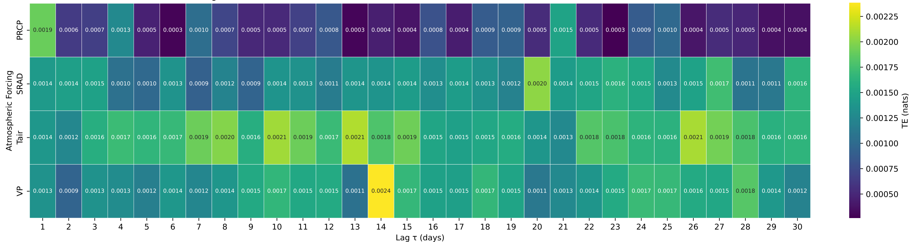
Shuffle-Test Significant TE to Streamflow — Basin 01644000 (HUC 02) — GOOSE CREEK NEAR LEESBURG, VA
