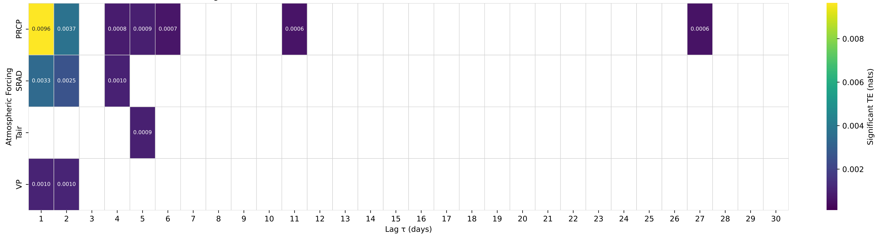
Shuffle-Test Significant TE to Streamflow — Basin 02327100 (HUC 03) — SOPCHOPPY RIVER NR SOPCHOPPY, FLA.
