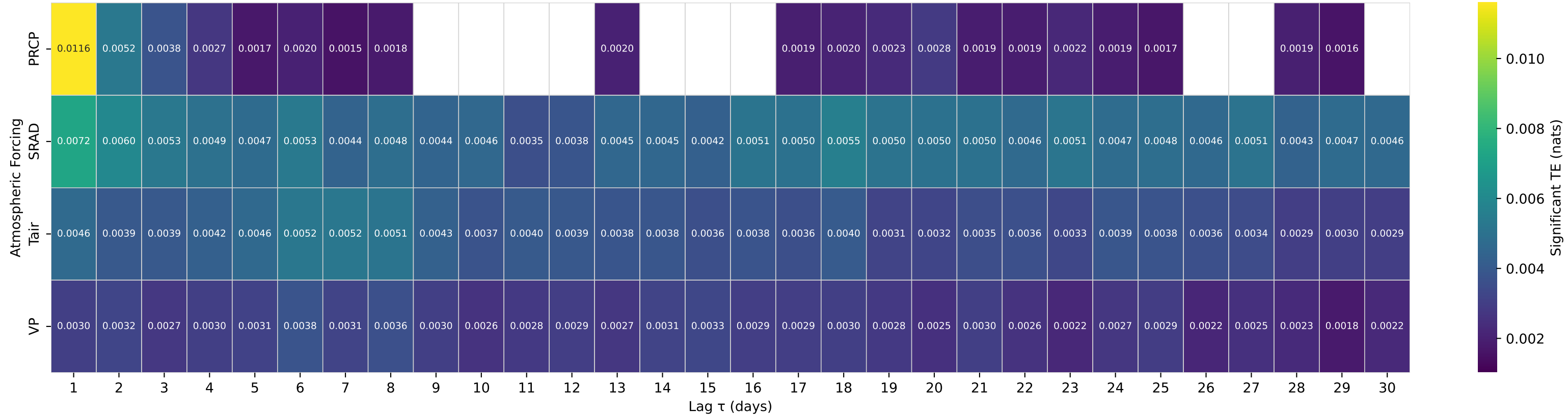
Shuffle-Test Significant TE to Streamflow — Basin 14236200 (HUC 17) — TILTON RIVER AB BEAR CANYON CREEK NEAR CINEBAR, WA
