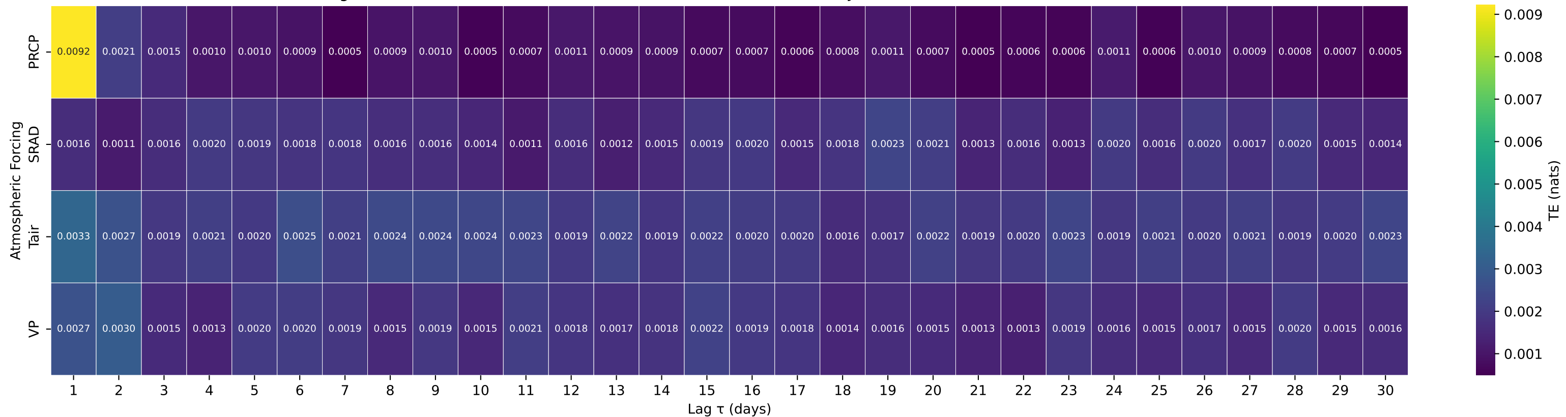
Shuffle-Test Significant TE to Streamflow — Basin 04024430 (HUC 04) — NEMADJI RIVER NEAR SOUTH SUPERIOR, WI
