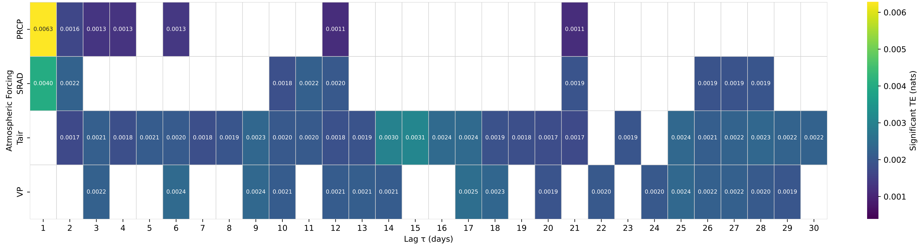
Shuffle-Test Significant TE to Streamflow — Basin 02216180 (HUC 03) — TURNPIKE CREEK NEAR MCRAE, GA
