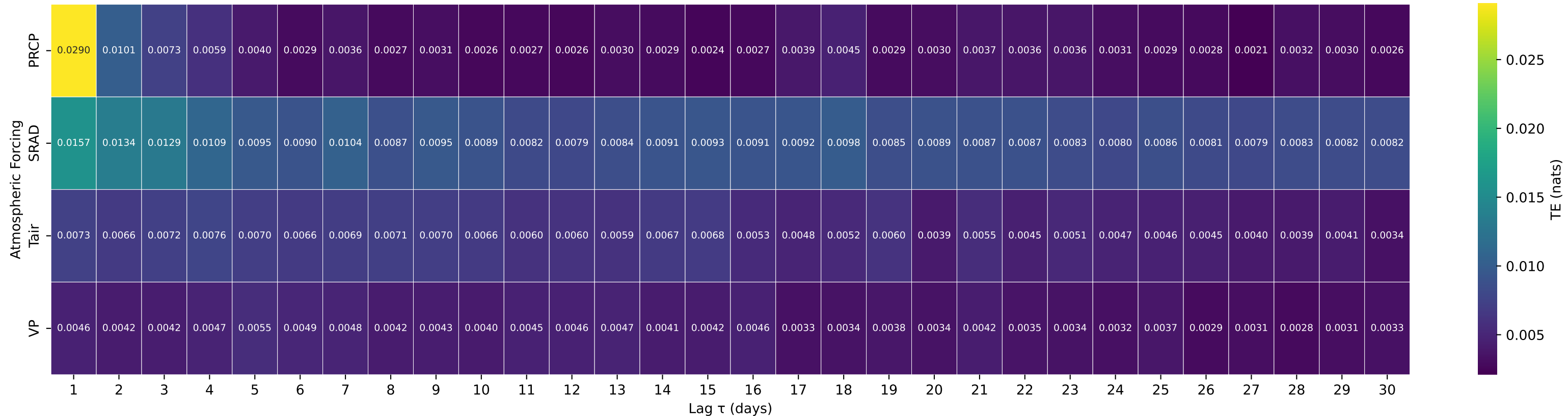
Shuffle-Test Significant TE to Streamflow — Basin 12041200 (HUC 17) — HOH RIVER AT US HIGHWAY 101 NEAR FORKS, WA
