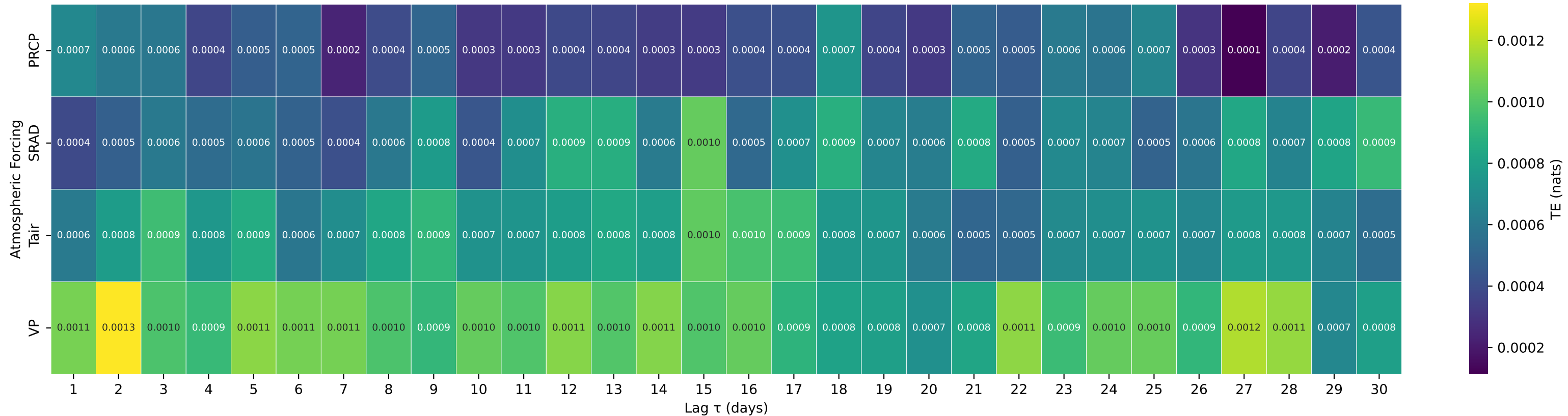
Shuffle-Test Significant TE to Streamflow — Basin 06803510 (HUC 10) — LITTLE SALT CREEK NEAR LINCOLN, NEBR.
