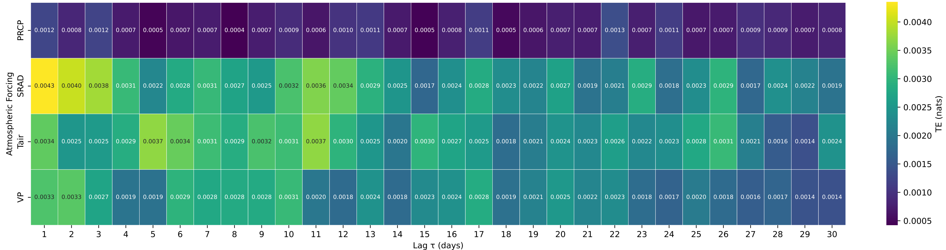
Shuffle-Test Significant TE to Streamflow — Basin 09066300 (HUC 14) — MIDDLE CREEK NEAR MINTURN, CO.
