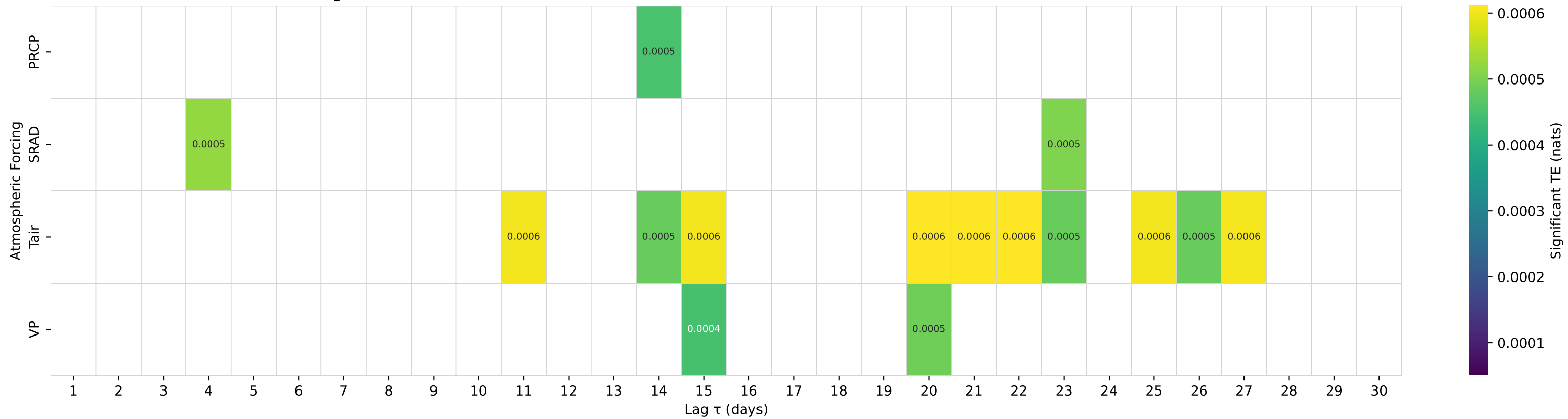
Shuffle-Test Significant TE to Streamflow — Basin 01605500 (HUC 02) — SOUTH BRANCH POTOMAC RIVER AT FRANKLIN, WV
