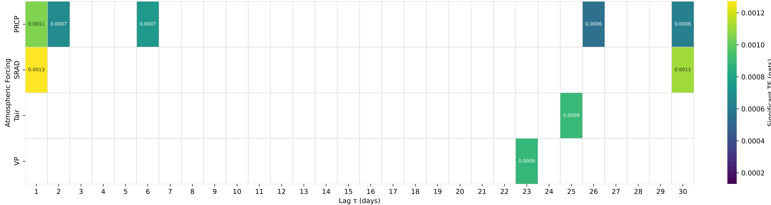
Shuffle-Test Significant TE to Streamflow — Basin 02077200 (HUC 03) — HYCO CREEK NEAR LEASBURG, NC
