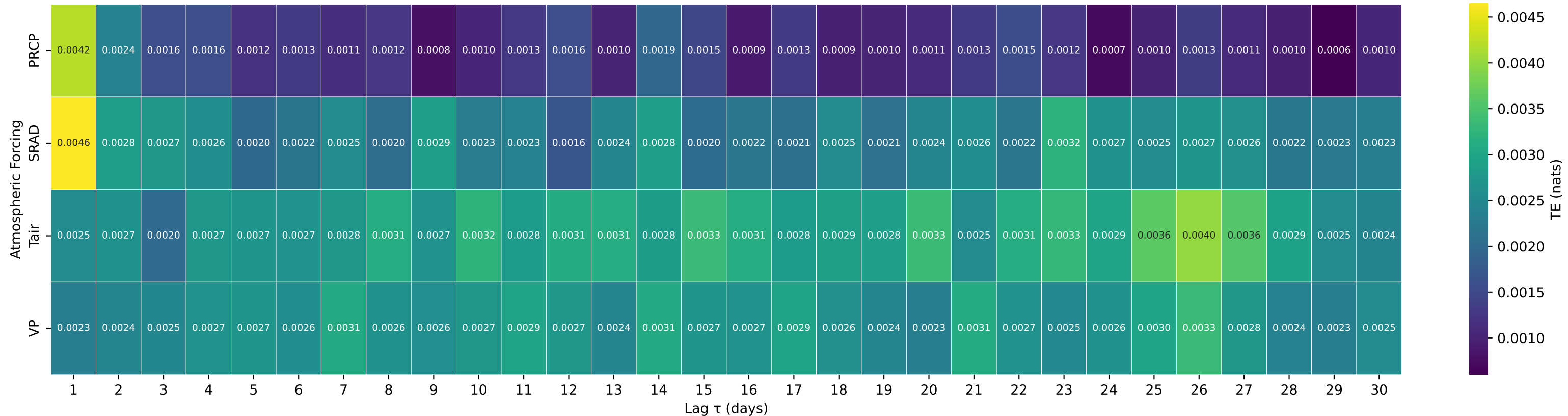
Shuffle-Test Significant TE to Streamflow — Basin 07292500 (HUC 08) — HOMOCHITTO RIVER AT ROSETTA, MS
