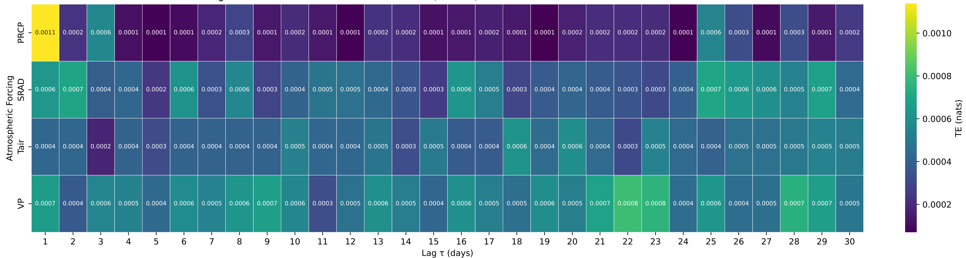
Shuffle-Test Significant TE to Streamflow — Basin 02369800 (HUC 03) — BLACKWATER RIVER NEAR BRADLEY AL
