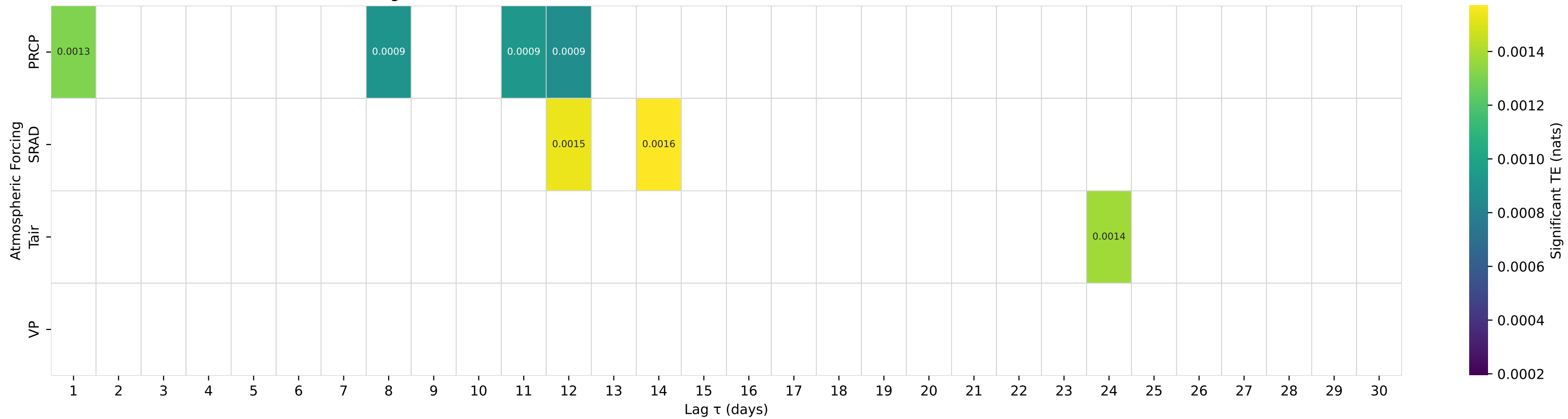
Shuffle-Test Significant TE to Streamflow — Basin 06339500 (HUC 10) — KNIFE RIVER NR GOLDEN VALLEY, ND
