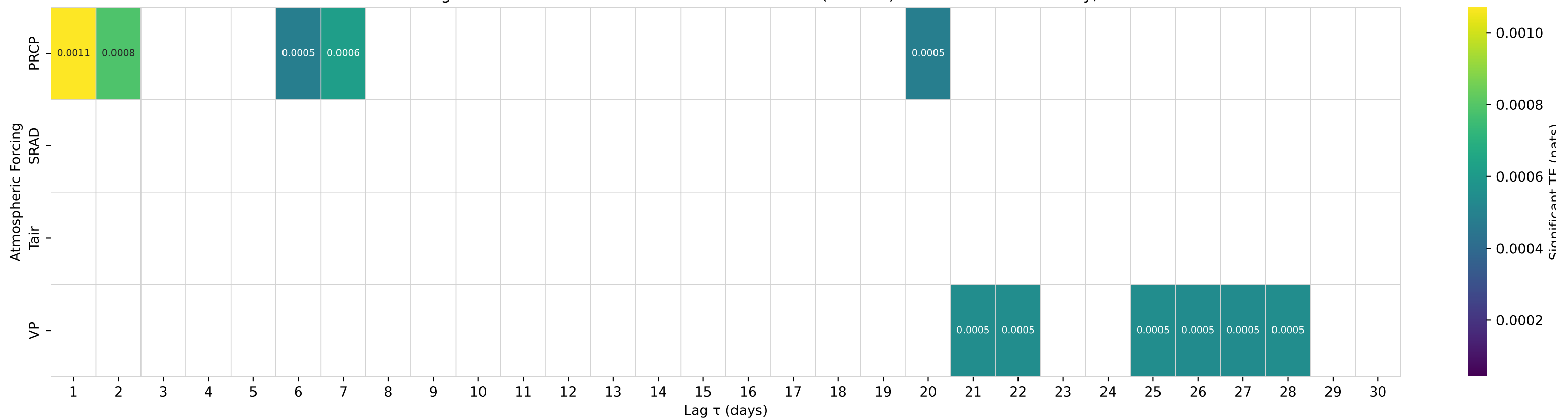
Shuffle-Test Significant TE to Streamflow — Basin 08082700 (HUC 12) — Millers Ck nr Munday, TX
