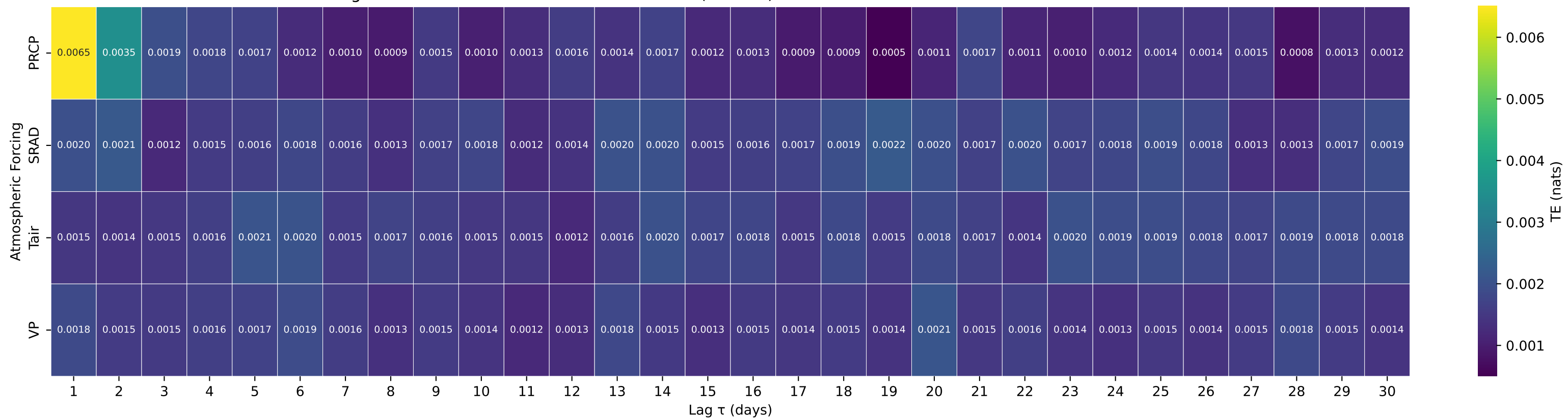
Shuffle-Test Significant TE to Streamflow — Basin 06477500 (HUC 10) — FIRESTEEL CR NEAR MOUNT VERNON SD
