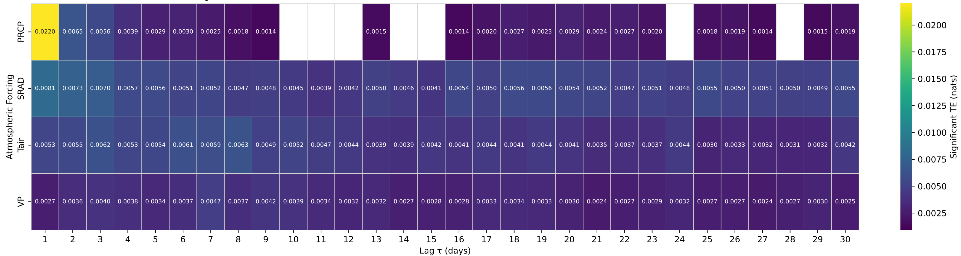
Shuffle-Test Significant TE to Streamflow — Basin 14139800 (HUC 17) — SOUTH FORK BULL RUN RIVER NEAR BULL RUN, OR
