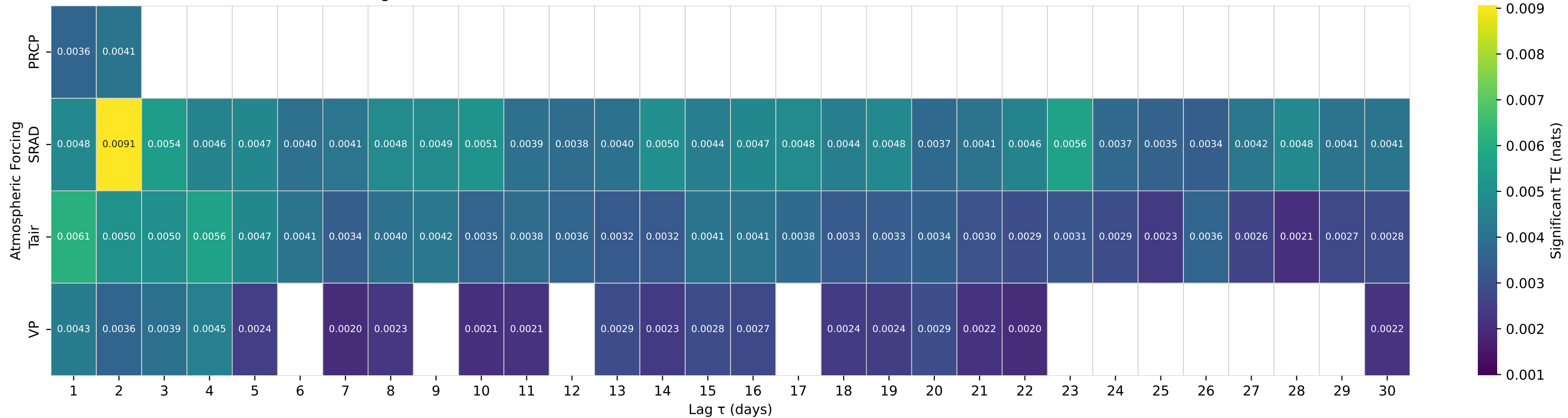
Shuffle-Test Significant TE to Streamflow — Basin 06037500 (HUC 10) — Madison River near West Yellowstone MT
