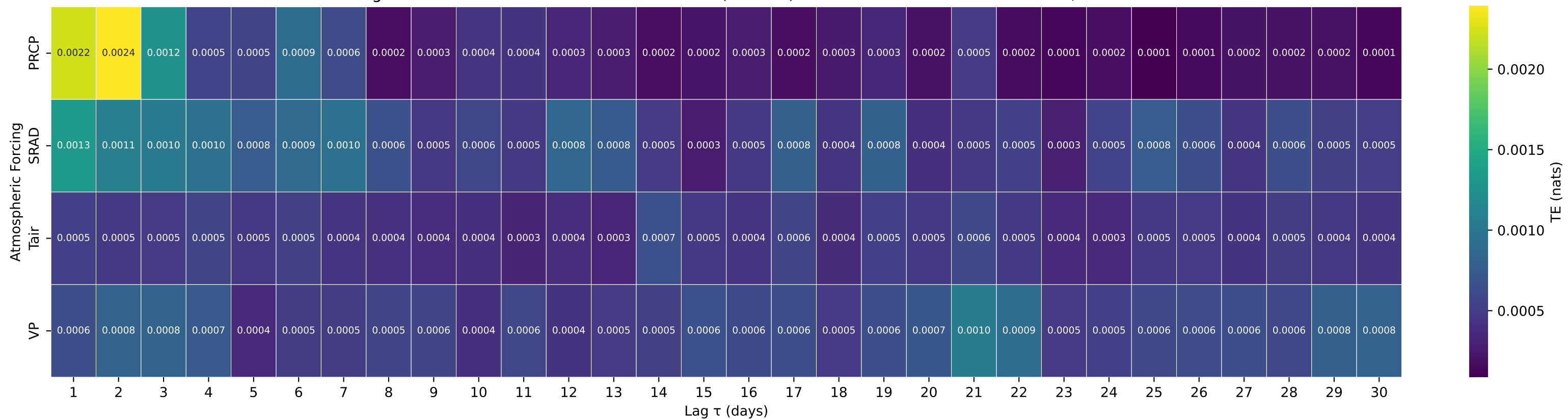
Shuffle-Test Significant TE to Streamflow — Basin 02053200 (HUC 03) — POTECA SI CREEK NEAR UNION, NC
