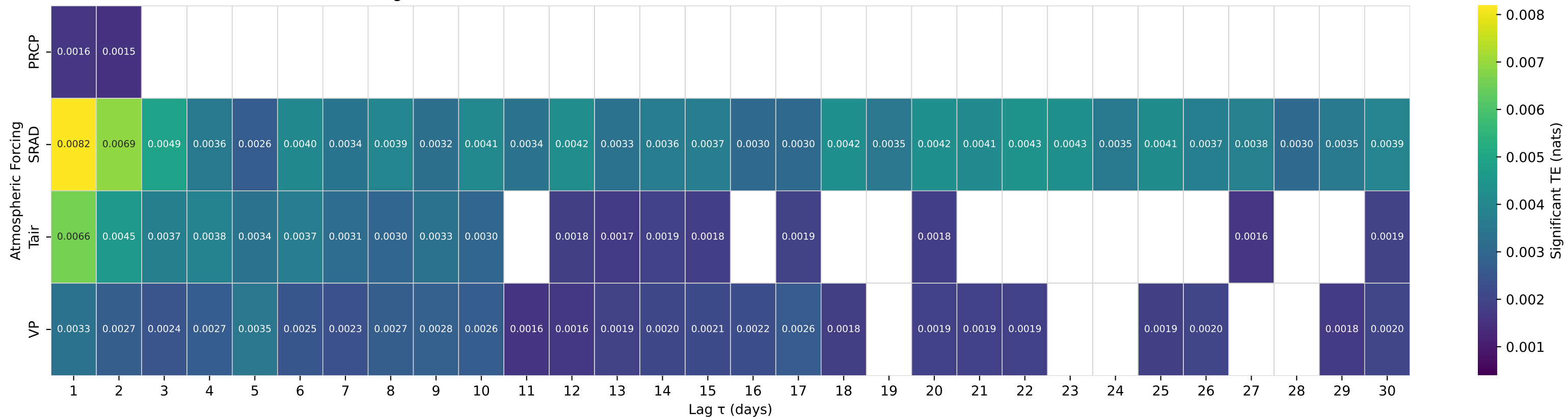
Shuffle-Test Significant TE to Streamflow — Basin 12447390 (HUC 17) — ANDREWS CREEK NEAR MAZAMA, WA
