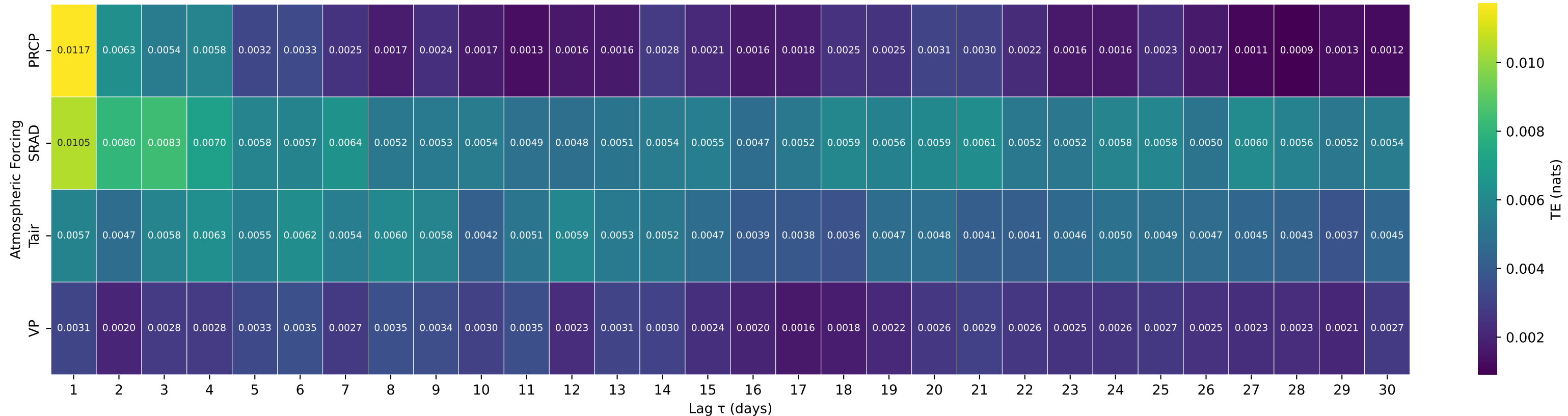
Shuffle-Test Significant TE to Streamflow — Basin 14187000 (HUC 17) — WILEY CREEK NEAR FOSTER, OR
