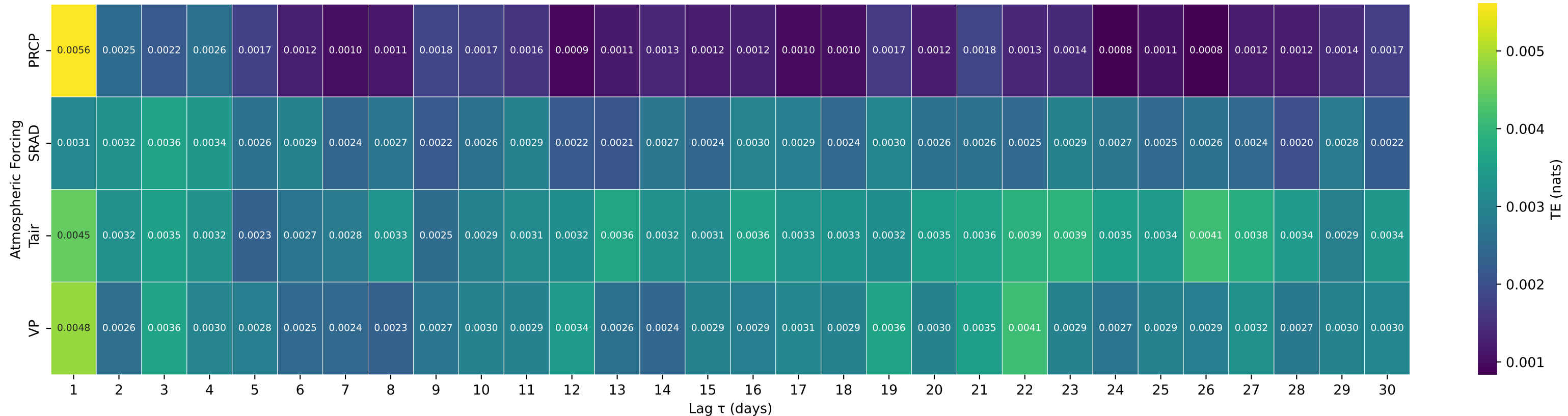
Shuffle-Test Significant TE to Streamflow — Basin 03010655 (HUC 05) — Oswayo Creek at Shinglehouse, PA
