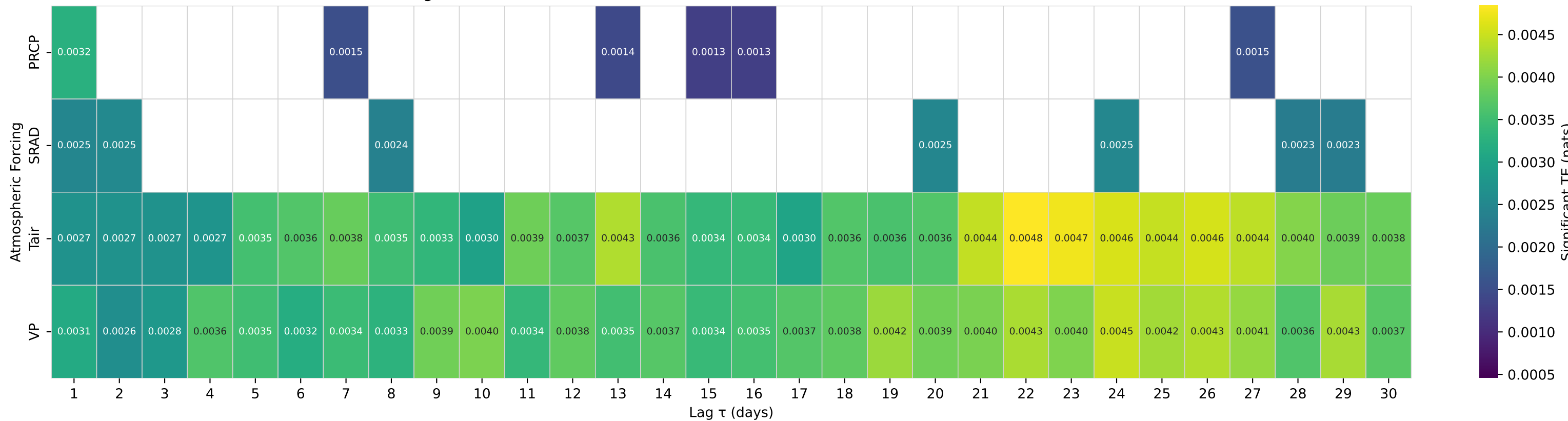
Shuffle-Test Significant TE to Streamflow — Basin 03186500 (HUC 05) — WILLIAMS RIVER AT DYER, WV
