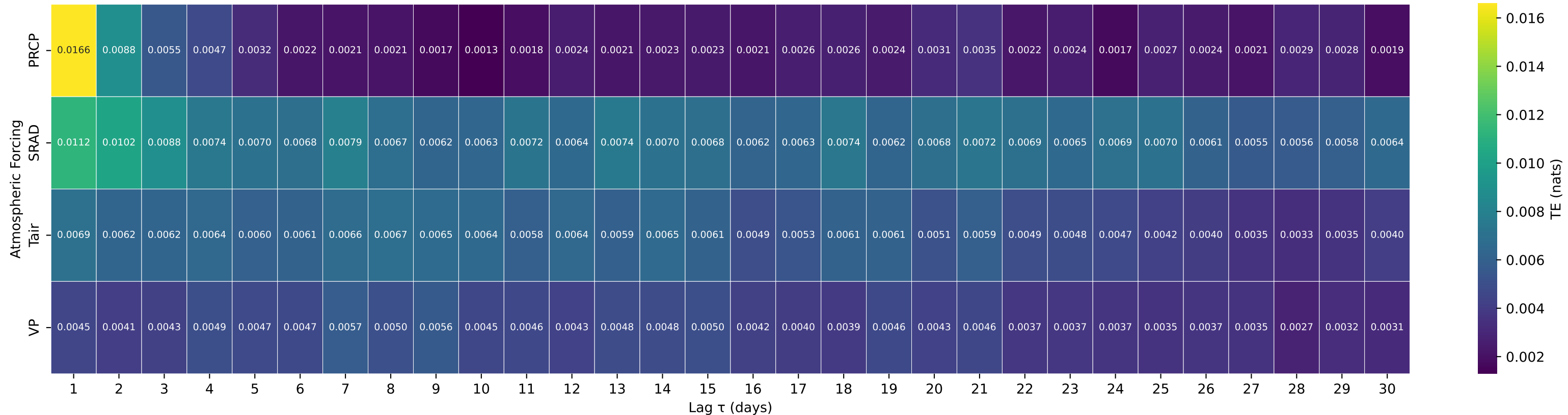
Shuffle-Test Significant TE to Streamflow — Basin 12167000 (HUC 17) — NF STILLAGUAMISH RIVER NEAR ARLINGTON, WA
