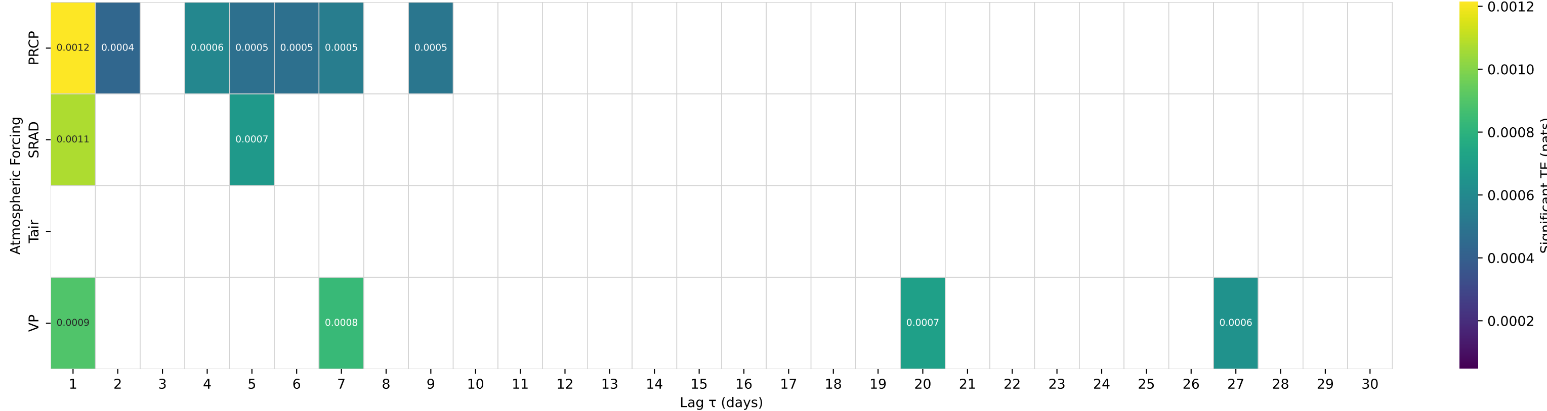
Shuffle-Test Significant TE to Streamflow — Basin 08190500 (HUC 12) — W Nueces Rv nr Brackettville, TX
