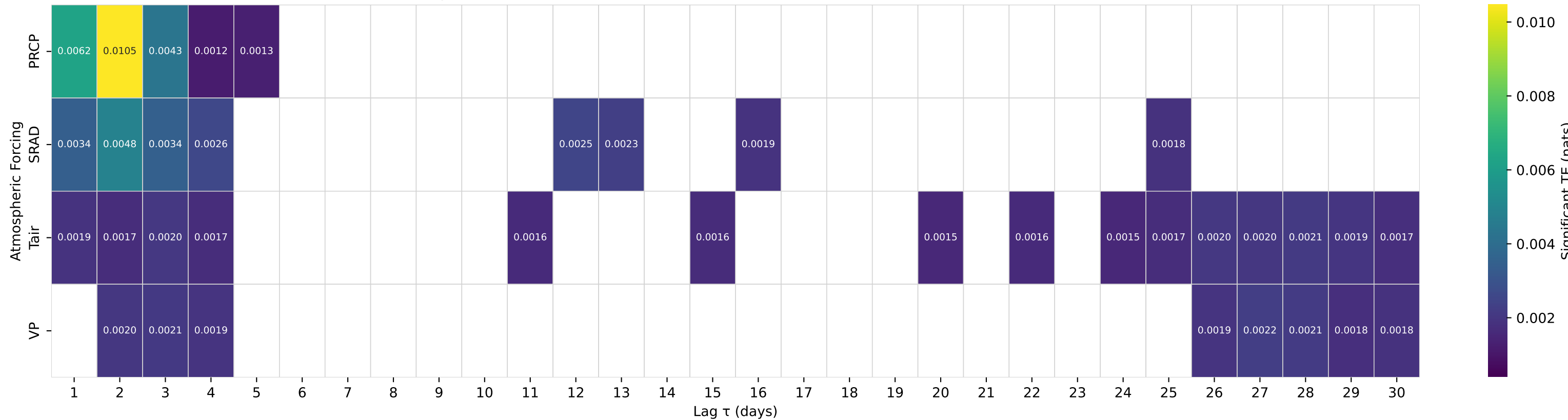
Shuffle-Test Significant TE to Streamflow — Basin 07376000 (HUC 08) — Tickfaw River at Holden, LA
