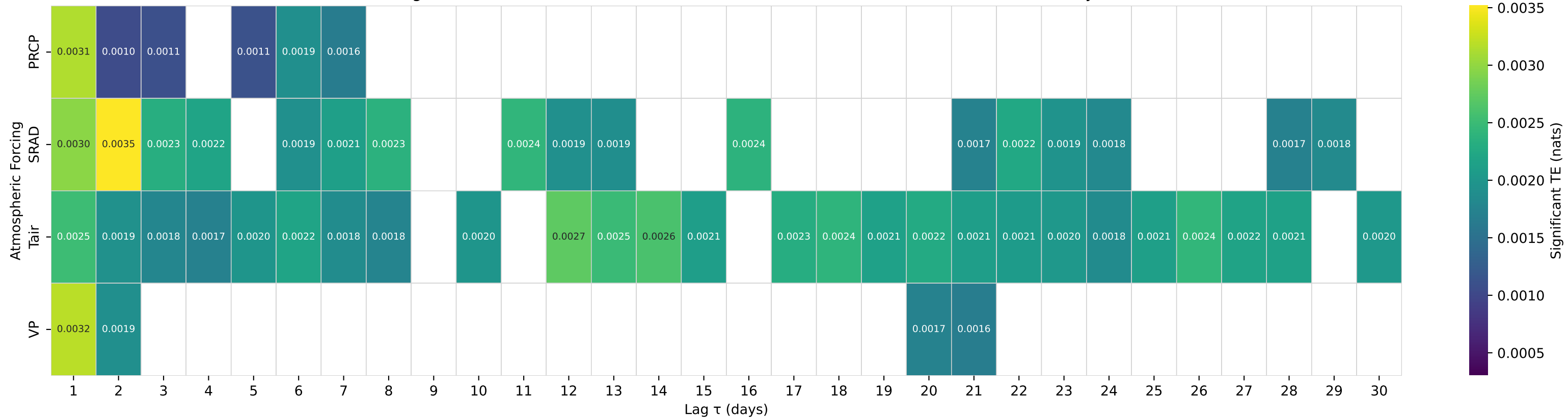
Shuffle-Test Significant TE to Streamflow — Basin 01055000 (HUC 01) — Swift River near Roxbury, Maine
