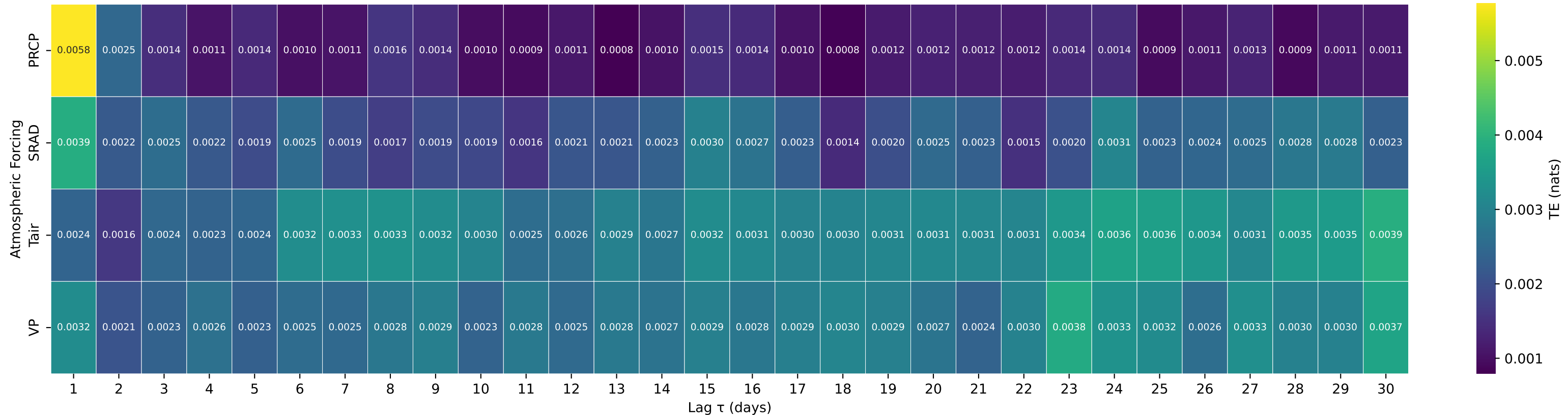
Shuffle-Test Significant TE to Streamflow — Basin 03473000 (HUC 06) — S F HOLSTON RIVER NEAR DAMASCUS, VA
