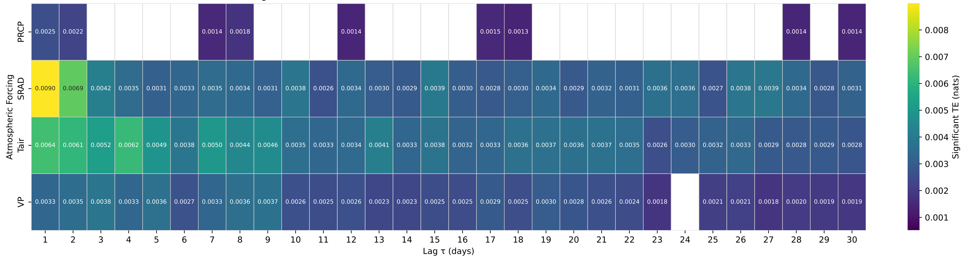
Shuffle-Test Significant TE to Streamflow — Basin 13011500 (HUC 17) — PACIFIC CREEK AT MORAN WY
