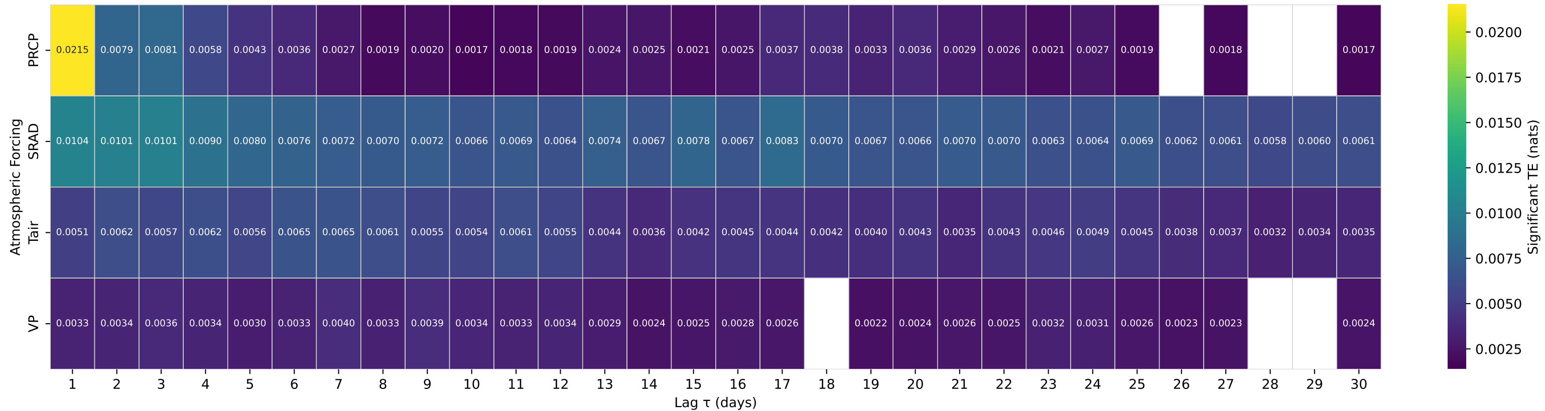
Shuffle-Test Significant TE to Streamflow — Basin 14303200 (HUC 17) — TUCCA CREEK NEAR BLAINE, OR.
