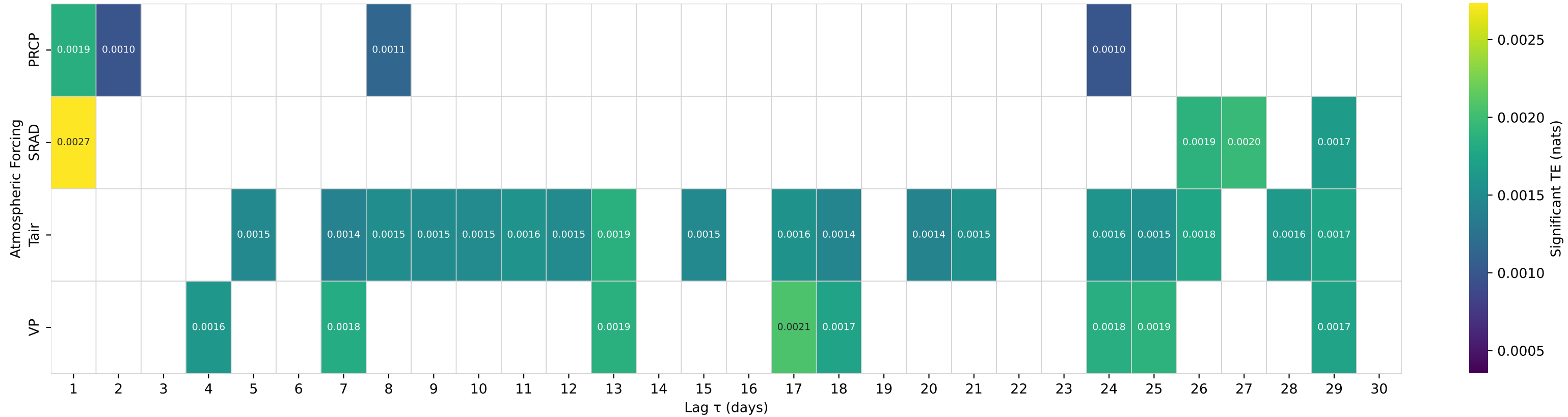
Shuffle-Test Significant TE to Streamflow — Basin 02111500 (HUC 03) — REDDIES RIVER AT NORTH WILKESBORO, NC
