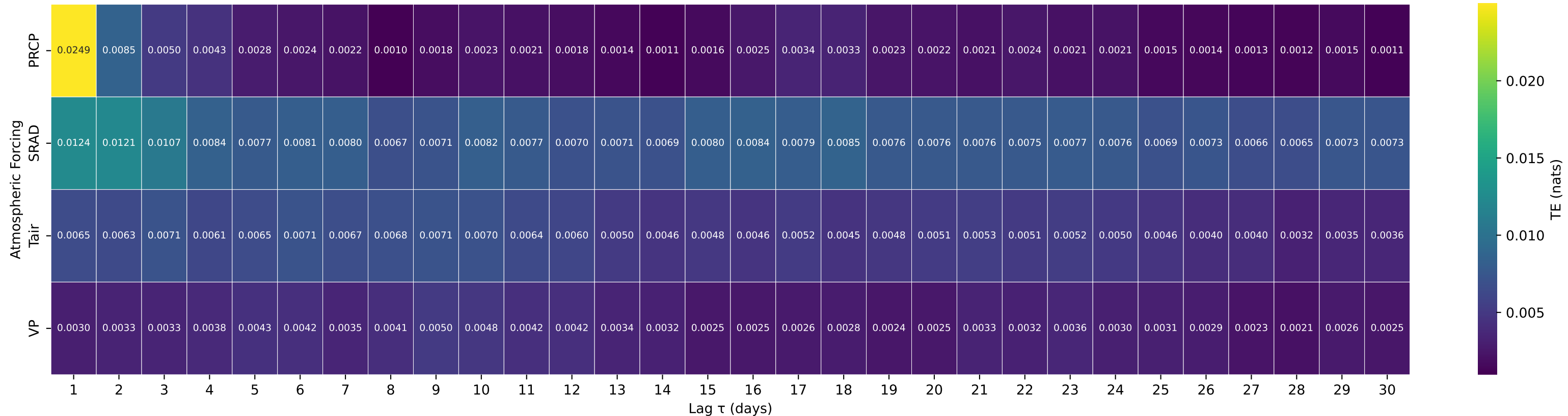
Shuffle-Test Significant TE to Streamflow — Basin 14301000 (HUC 17) — NEHALEM RIVER NEAR FOSS, OR
