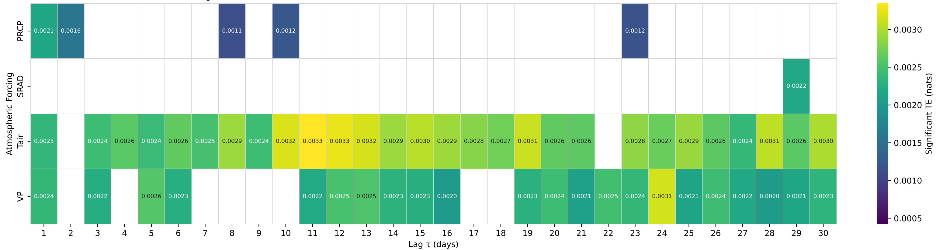
Shuffle-Test Significant TE to Streamflow — Basin 01423000 (HUC 02) — WEST BRANCH DELAWARE RIVER AT WALTON NY
