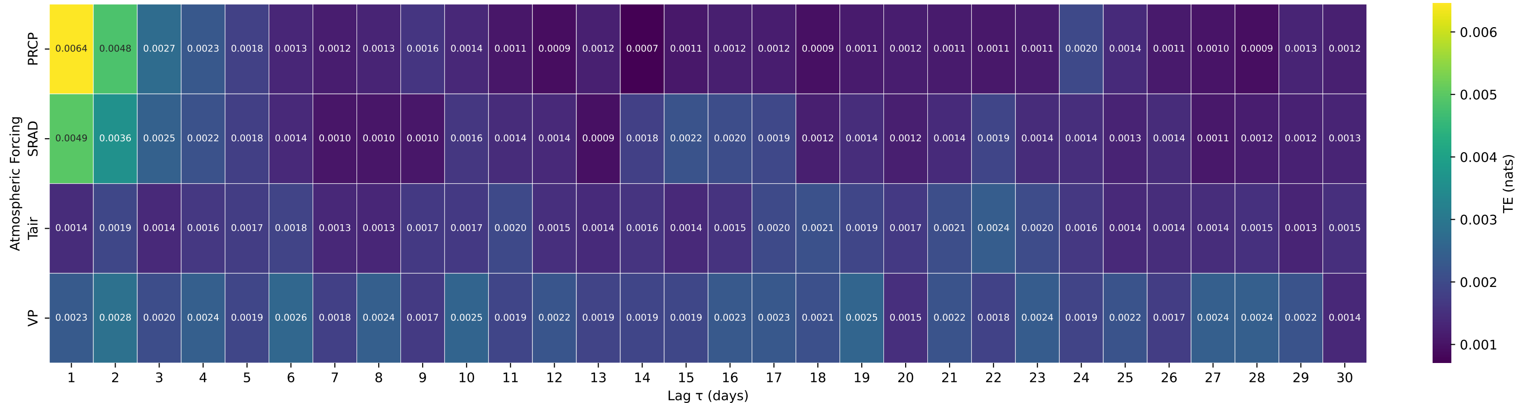
Shuffle-Test Significant TE to Streamflow — Basin 02310947 (HUC 03) — WITHLACOOCHEE RIVER NEAR CUMPRESSCO, FLA.
