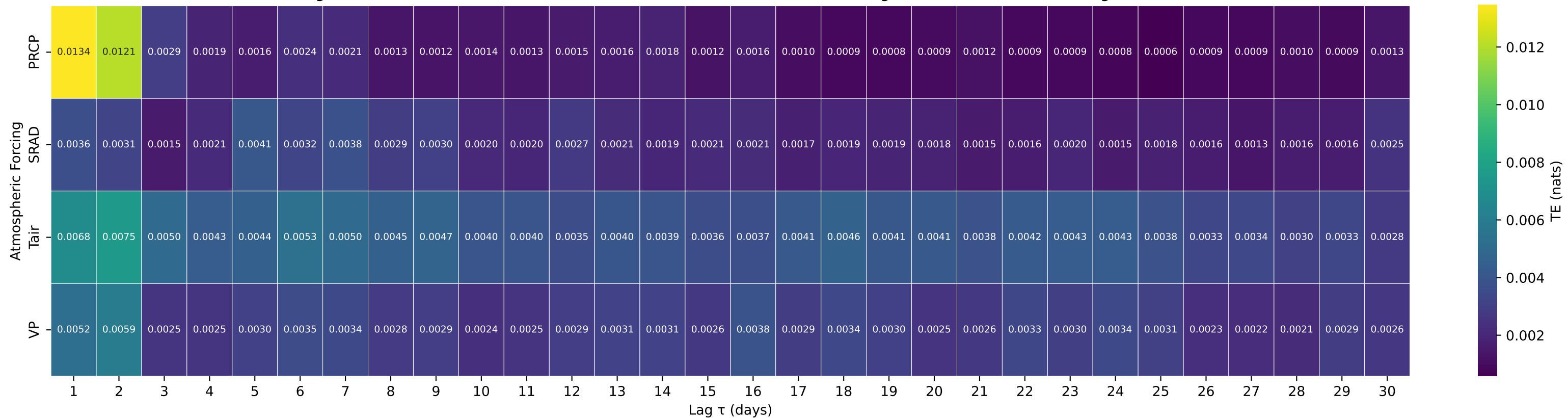
Shuffle-Test Significant TE to Streamflow — Basin 01030500 (HUC 01) — Mattawamkeag River near Mattawamkeag, Maine
