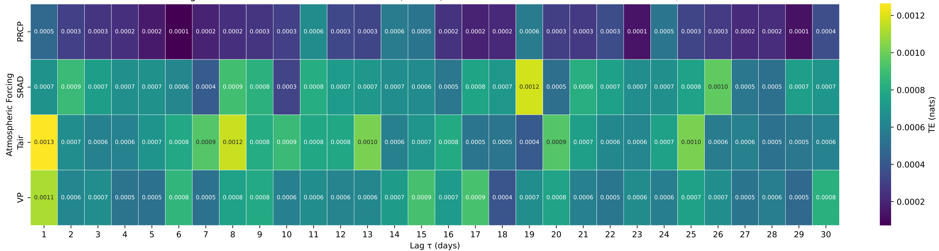
Shuffle-Test Significant TE to Streamflow — Basin 01632000 (HUC 02) — N F SHENANDOAH RIVER AT COOTES STORE, VA
