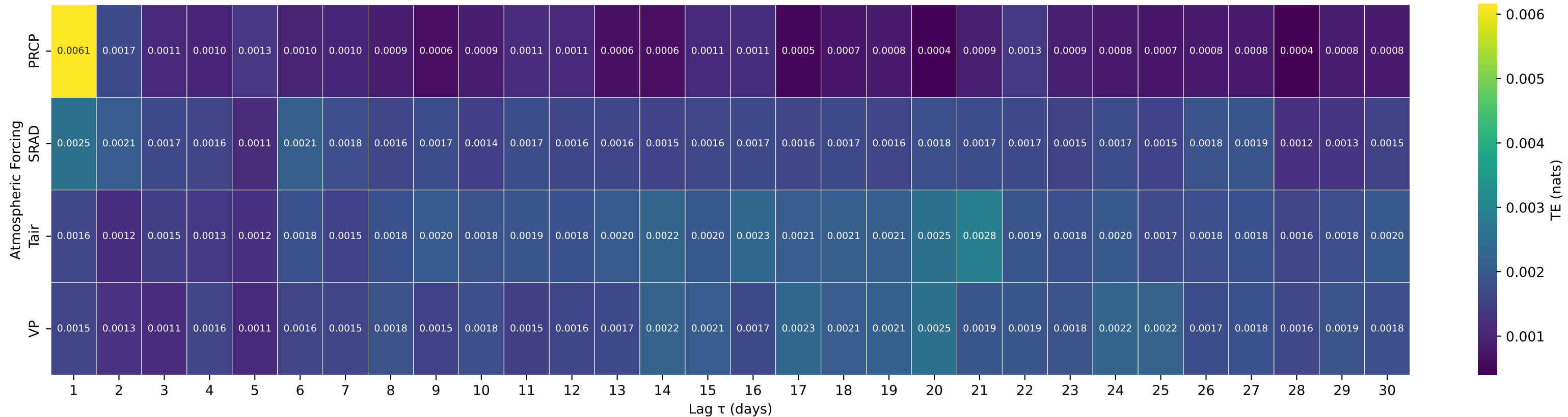
Shuffle-Test Significant TE to Streamflow — Basin 07066000 (HUC 11) — Jacks Fork at Eminence, MO
