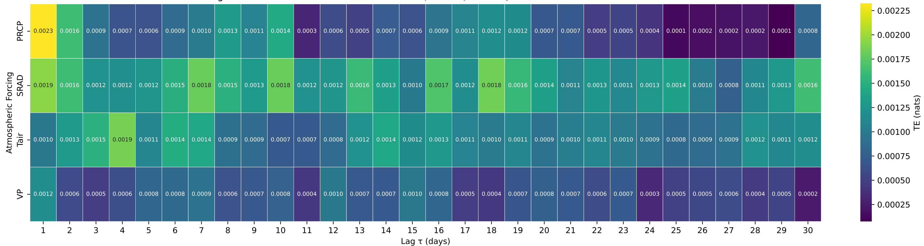
Shuffle-Test Significant TE to Streamflow — Basin 10258000 (HUC 18) — TAHQUITZ C NR PALM SPRINGS CA
