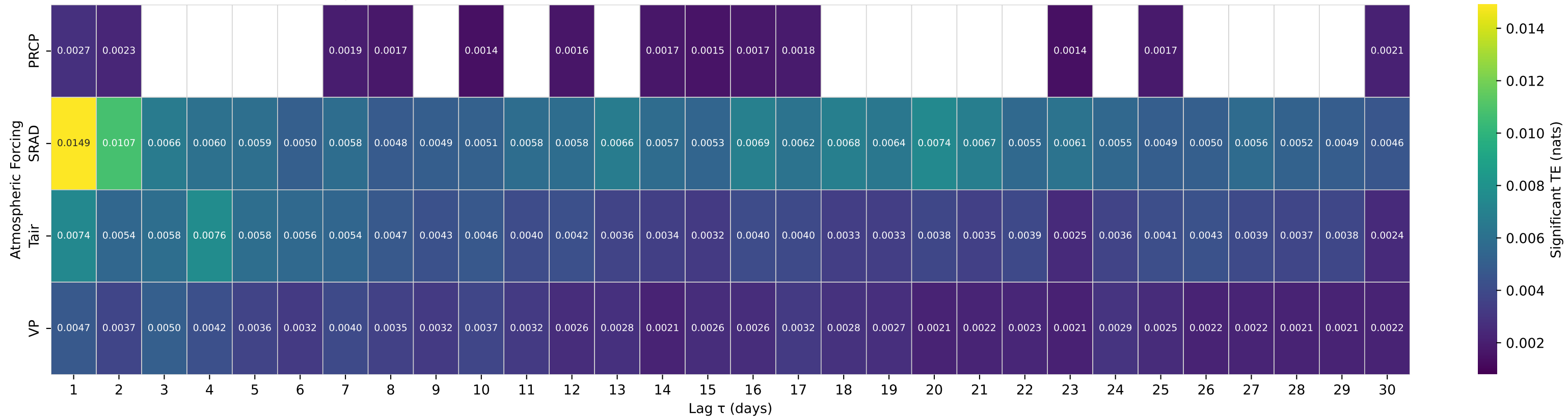
Shuffle-Test Significant TE to Streamflow — Basin 06280300 (HUC 10) — SOUTH FORK SHOSHONE RIVER NEAR VALLEY, WY
