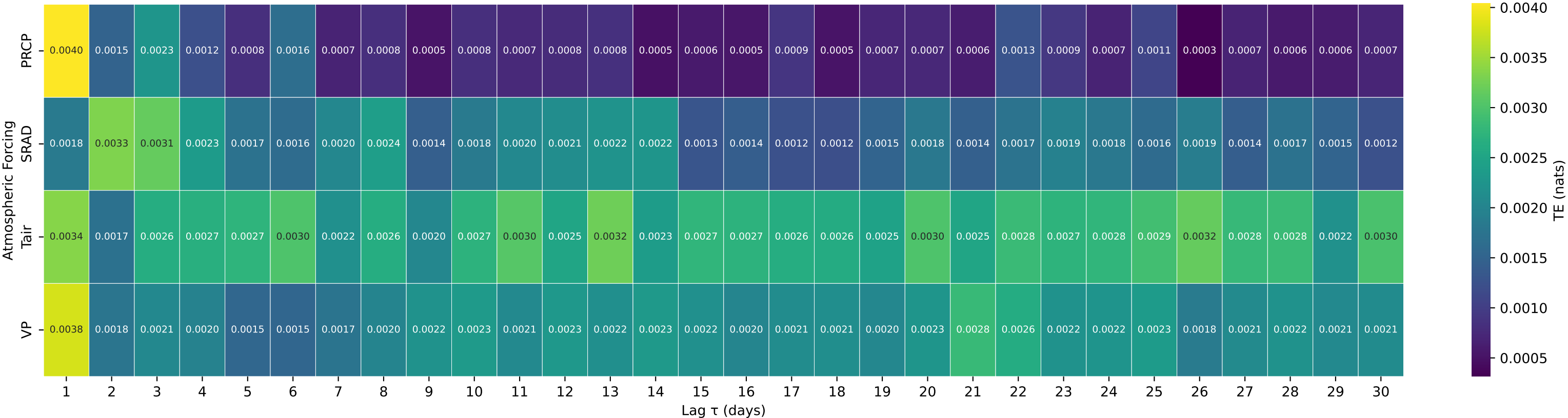
Shuffle-Test Significant TE to Streamflow — Basin 01078000 (HUC 01) — SMITH RIVER NEAR BRISTOL, NH
