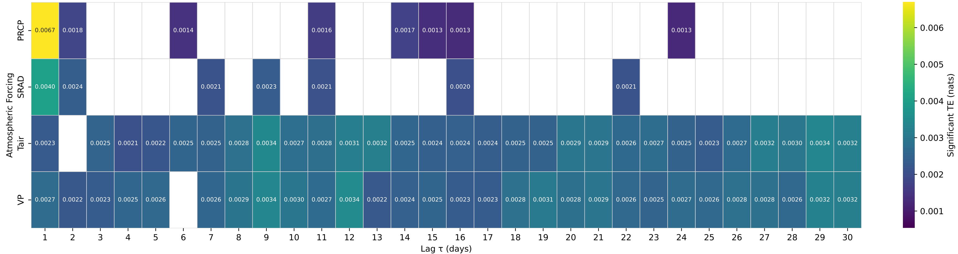
Shuffle-Test Significant TE to Streamflow — Basin 07290650 (HUC 08) — BAYOU PIERRE NR WILLOWS, MS
