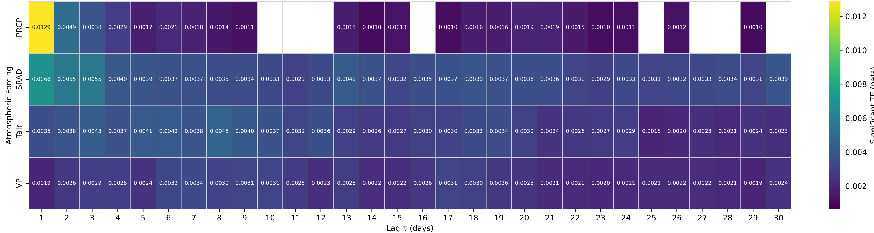
Shuffle-Test Significant TE to Streamflow — Basin 14138870 (HUC 17) — FIR CREEK NEAR BRIGHTWOOD, OR
