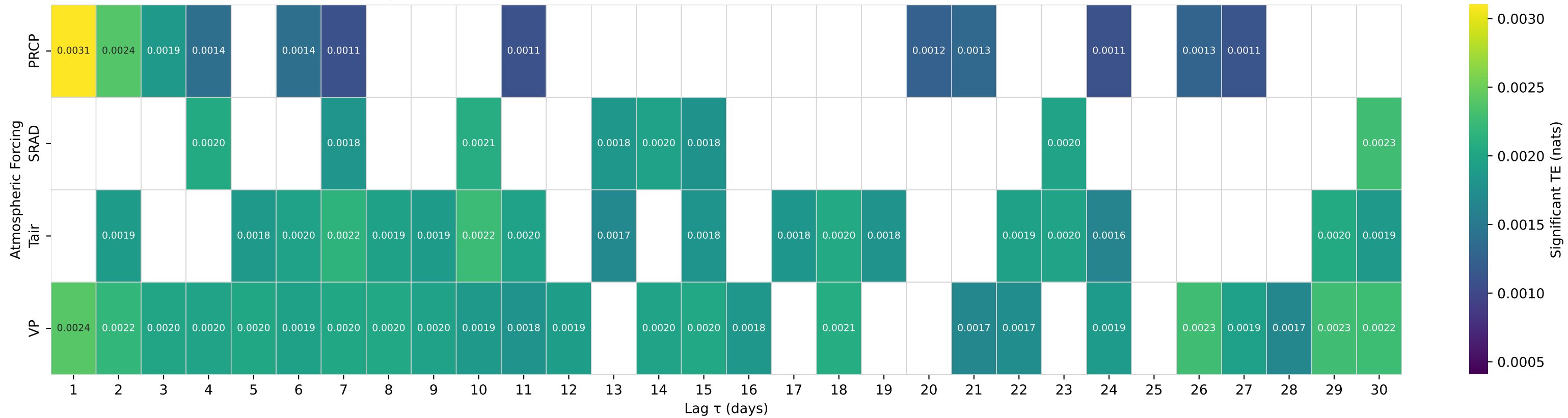
Shuffle-Test Significant TE to Streamflow — Basin 06784000 (HUC 10) — SOUTH LOUP R AT ST. MICHAEL, NEBR.
