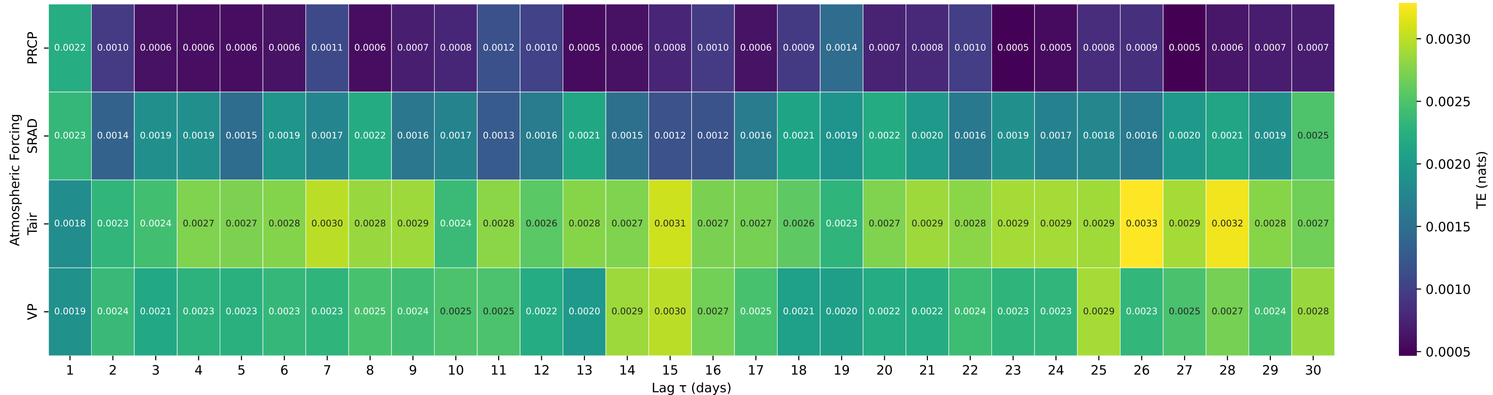
Shuffle-Test Significant TE to Streamflow — Basin 01639500 (HUC 02) — BIG PIPE CREEK AT BRUCEVILLE, MD
