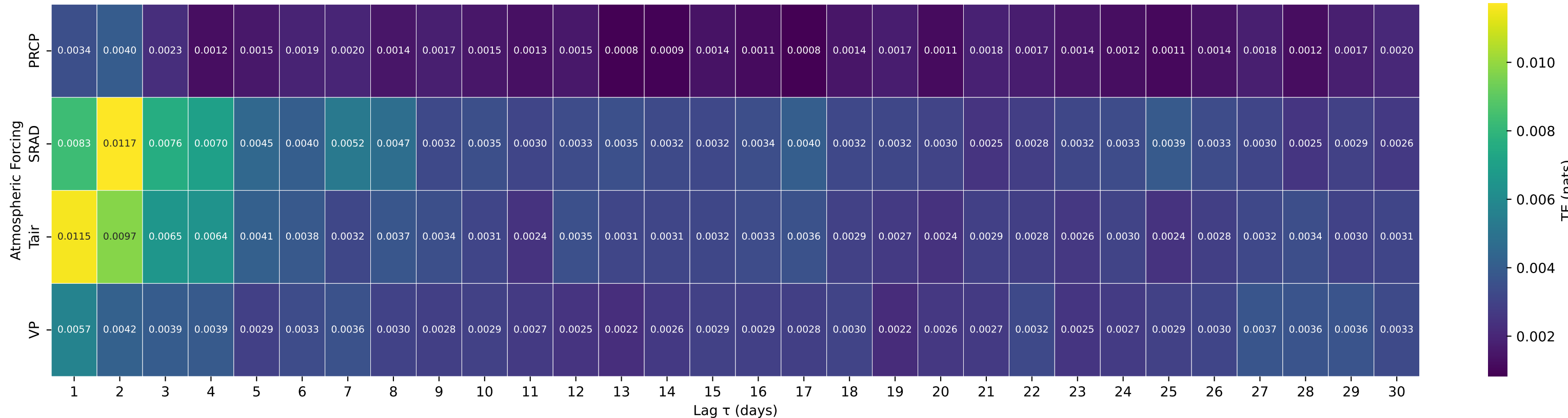
Shuffle-Test Significant TE to Streamflow — Basin 13337000 (HUC 17) — LOCHSA RIVER NR LOWELL ID
