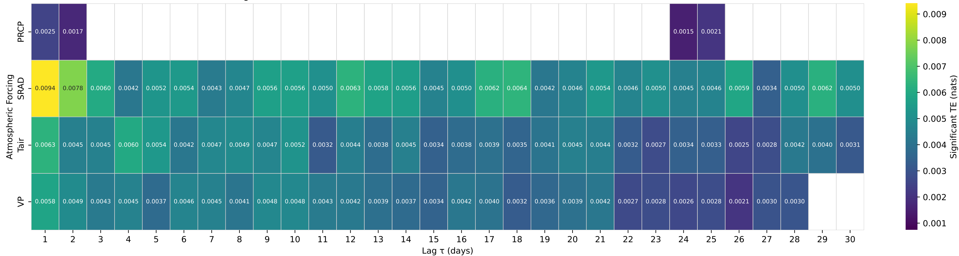
Shuffle-Test Significant TE to Streamflow — Basin 07083000 (HUC 11) — HALFMOON CREEK NEAR MALTA, CO.
