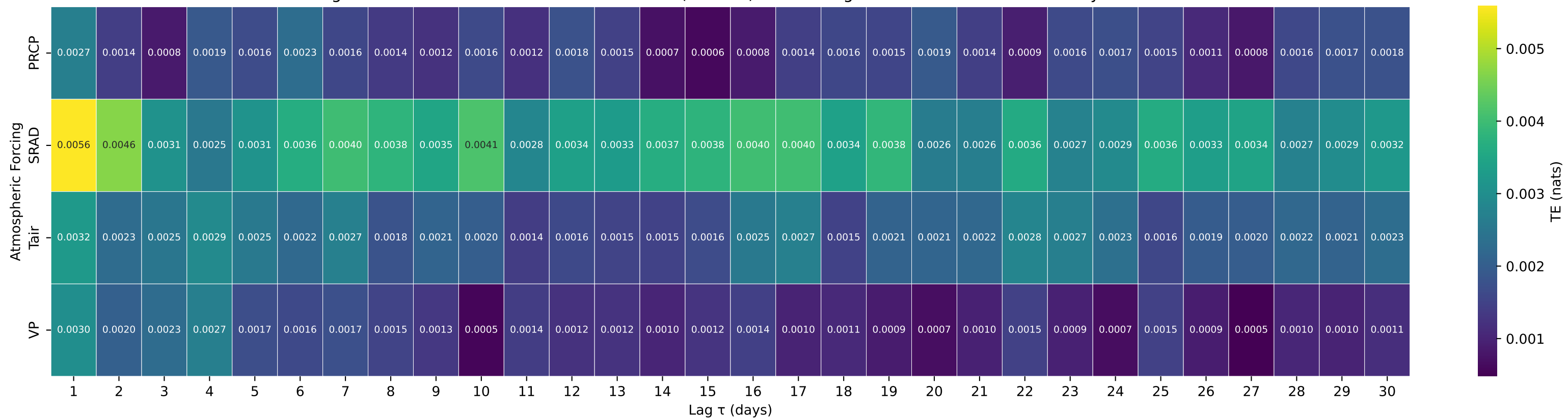
Shuffle-Test Significant TE to Streamflow — Basin 06289000 (HUC 10) — Little Bighorn River at State Line nr Wyola MT
