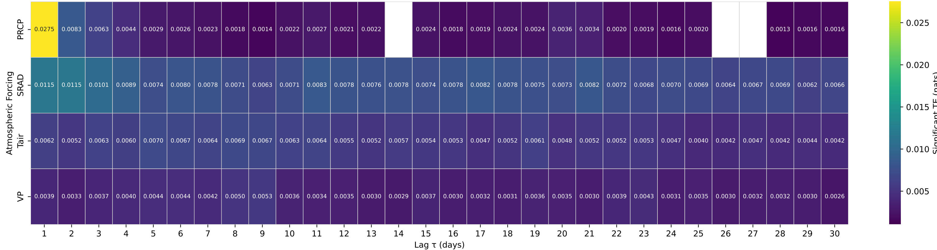
Shuffle-Test Significant TE to Streamflow — Basin 12035000 (HUC 17) — SATSOP RIVER NEAR SATSOP, WA
