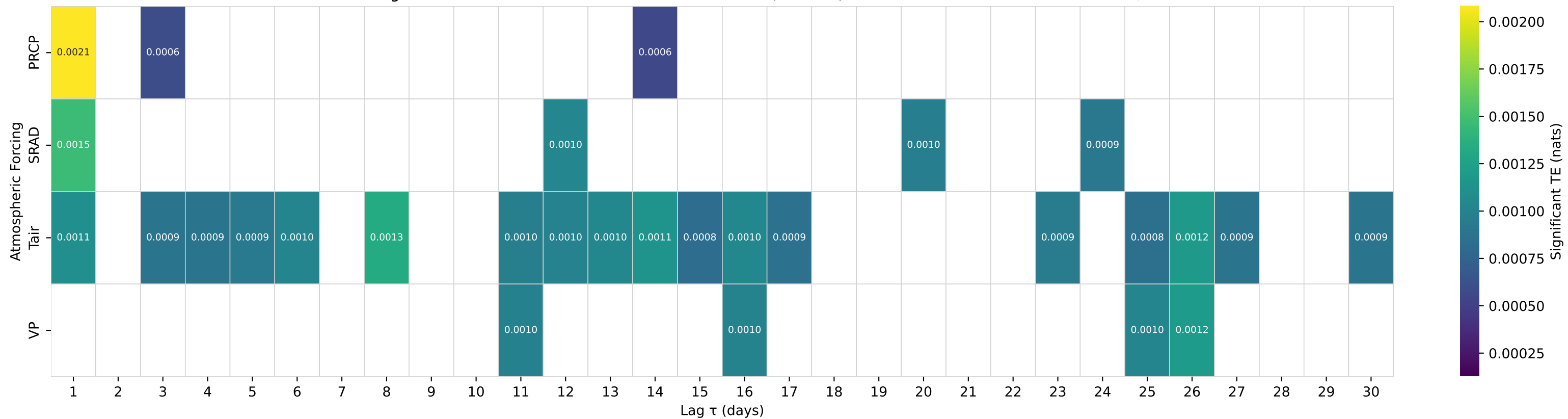
Shuffle-Test Significant TE to Streamflow — Basin 01667500 (HUC 02) — RAPIDAN RIVER NEAR CULPEPER, VA
