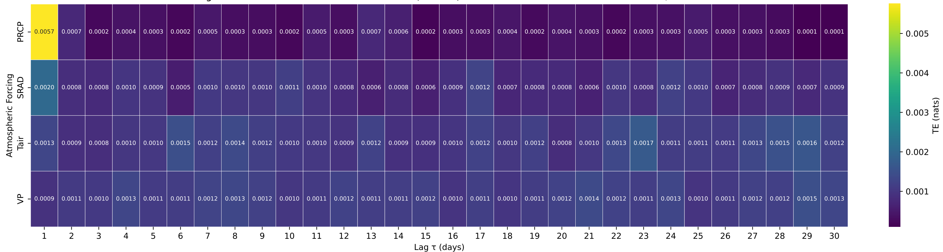
Shuffle-Test Significant TE to Streamflow — Basin 01491000 (HUC 02) — CHOPTANK RIVER NEAR GREENSBORO, MD
