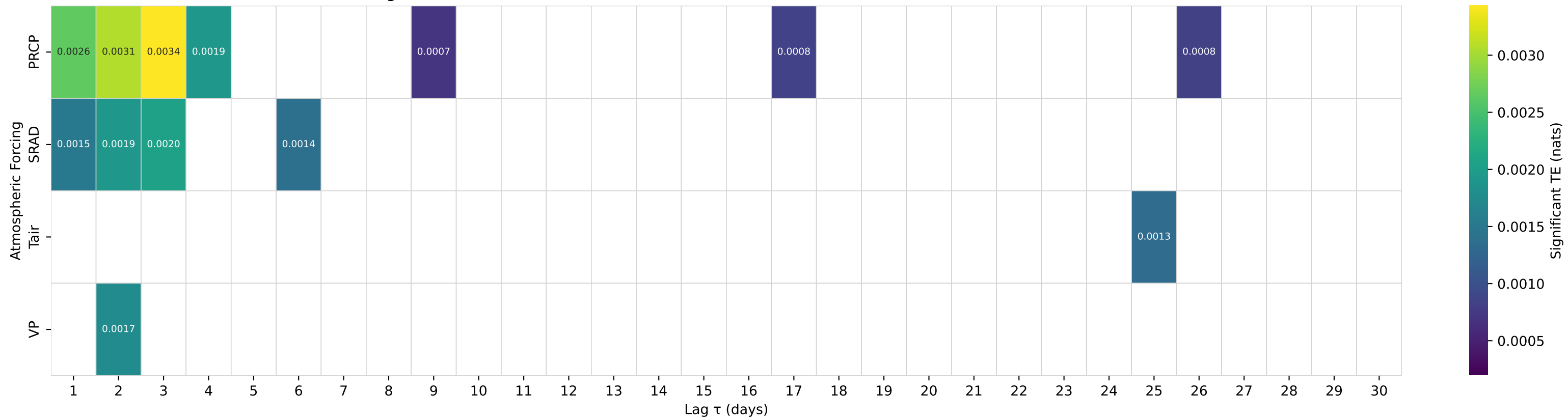
Shuffle-Test Significant TE to Streamflow — Basin 02372250 (HUC 03) — PATSALIGA CREEK NEAR BRANTLEY AL
