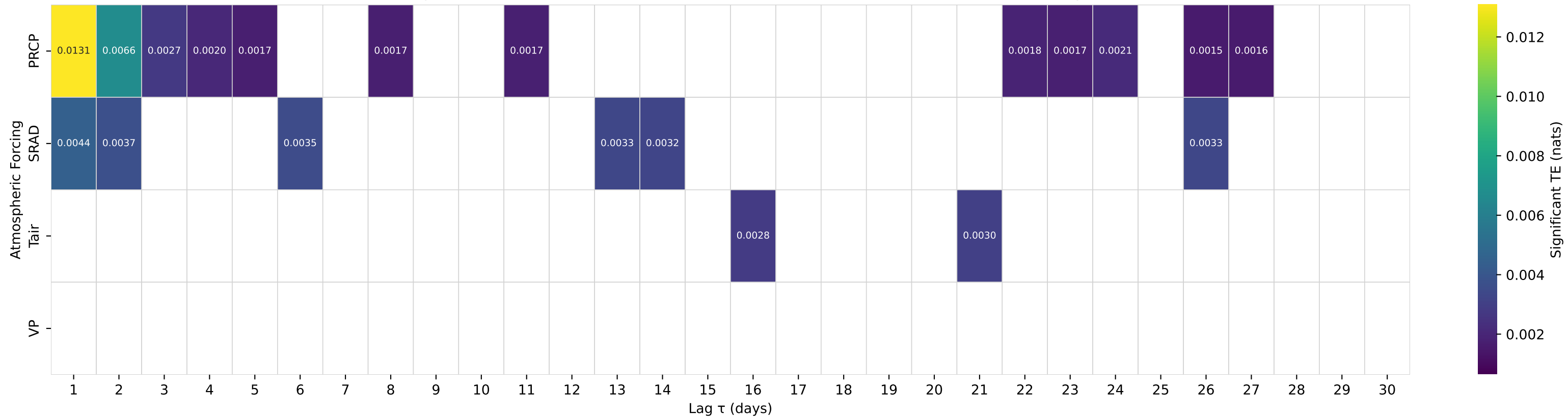
Shuffle-Test Significant TE to Streamflow — Basin 07068000 (HUC 11) — Current River at Doniphan, MO
