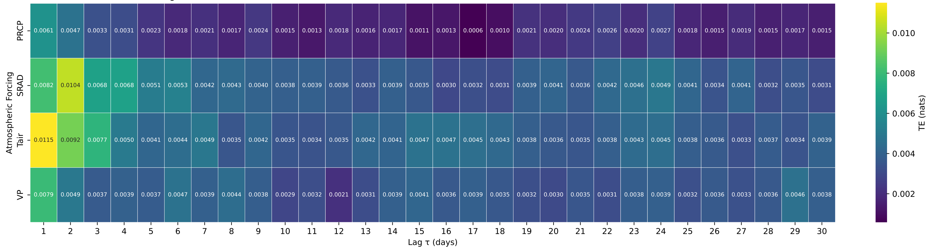
Shuffle-Test Significant TE to Streamflow — Basin 13340600 (HUC 17) — NF CLEARWATER RIVER NR CANYON RANGER STATION ID
