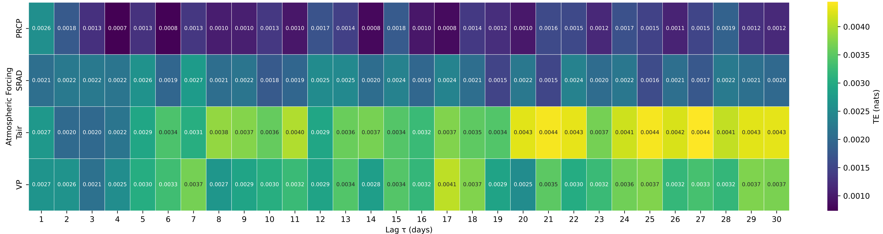
Shuffle-Test Significant TE to Streamflow — Basin 01594950 (HUC 02) — MCMILLAN F NEAR FORT PENDLETON, MD
