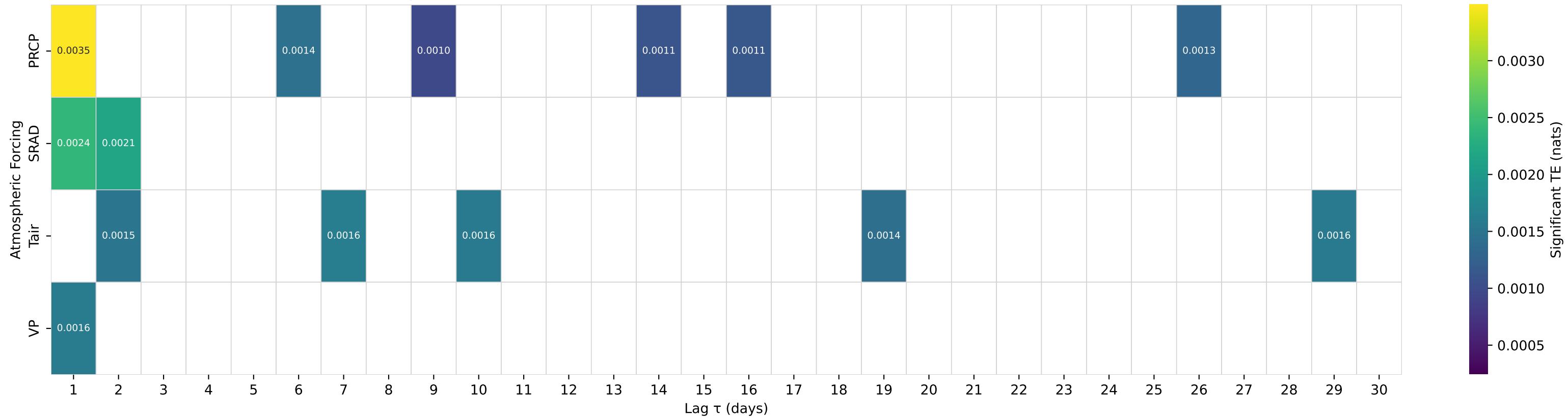
Shuffle-Test Significant TE to Streamflow — Basin 02384540 (HUC 03) — MILL CREEK NEAR CRANDALL, GA
