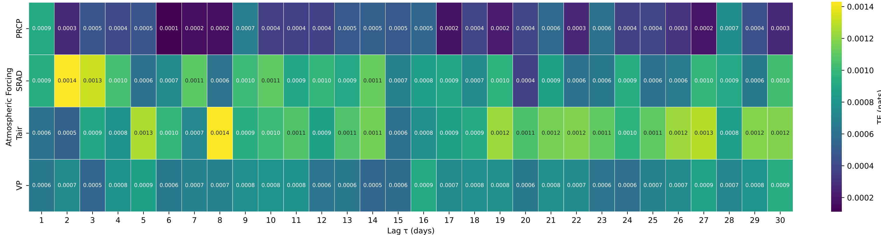
Shuffle-Test Significant TE to Streamflow — Basin 01547700 (HUC 02) — Marsh Creek at Blanchard, PA
