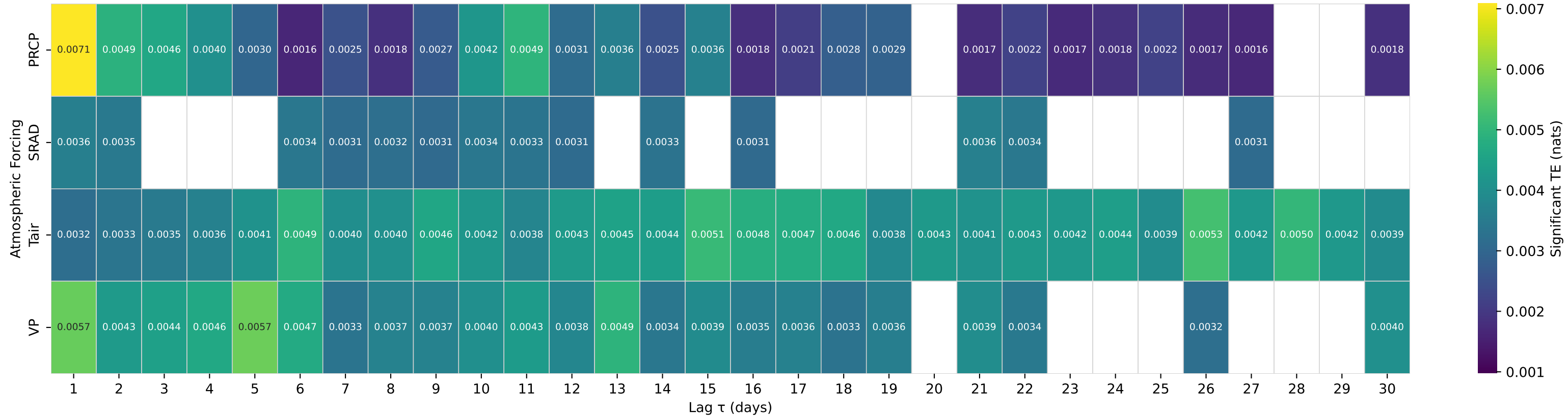
Shuffle-Test Significant TE to Streamflow — Basin 09484600 (HUC 15) — PANTANO WASH NEAR VAIL, AZ.
