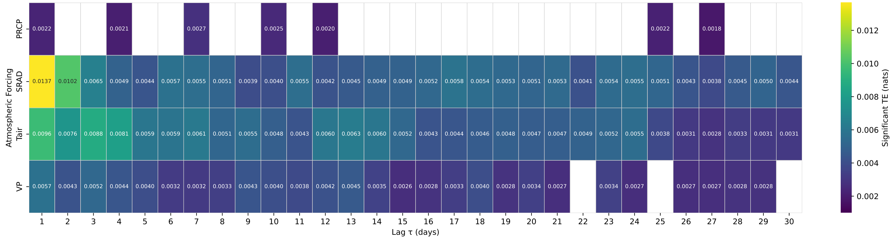
Shuffle-Test Significant TE to Streamflow — Basin 06188000 (HUC 10) — LAMAR RIVER NR TOWER FALLS RANGER STATION, YNP
