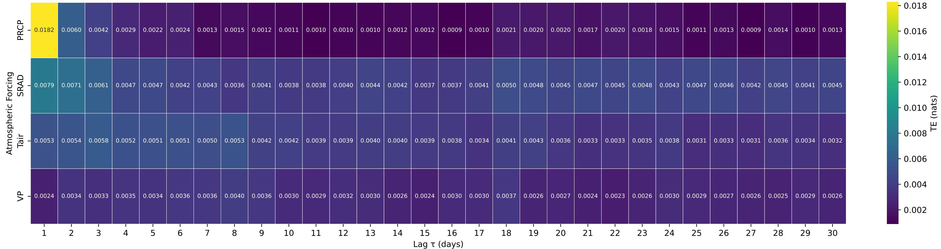
Shuffle-Test Significant TE to Streamflow — Basin 14138800 (HUC 17) — BLAZED ALDER CREEK NEAR RHODODENDRON, OREG.
