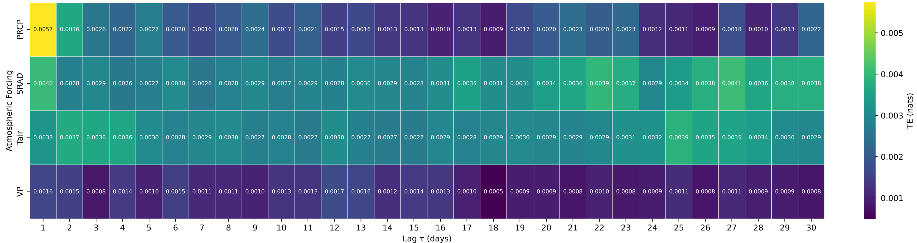
Shuffle-Test Significant TE to Streamflow — Basin 11284400 (HUC 18) — BIG C AB WHITES GULCH NR GROVELAND CA
