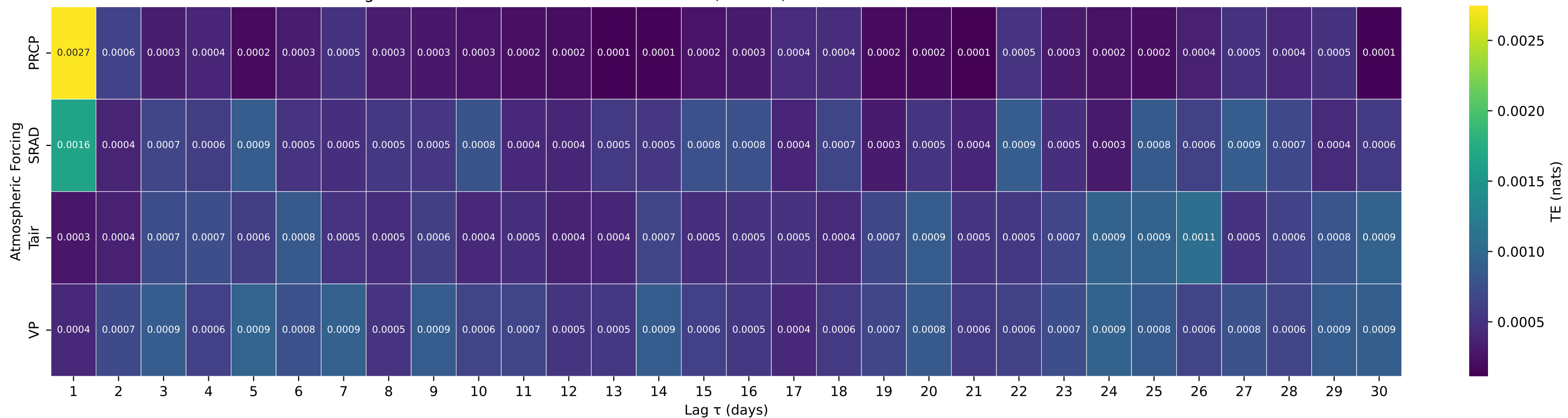
Shuffle-Test Significant TE to Streamflow — Basin 02465493 (HUC 03) — ELLIOTTS CREEK AT MOUNDVILLE AL
