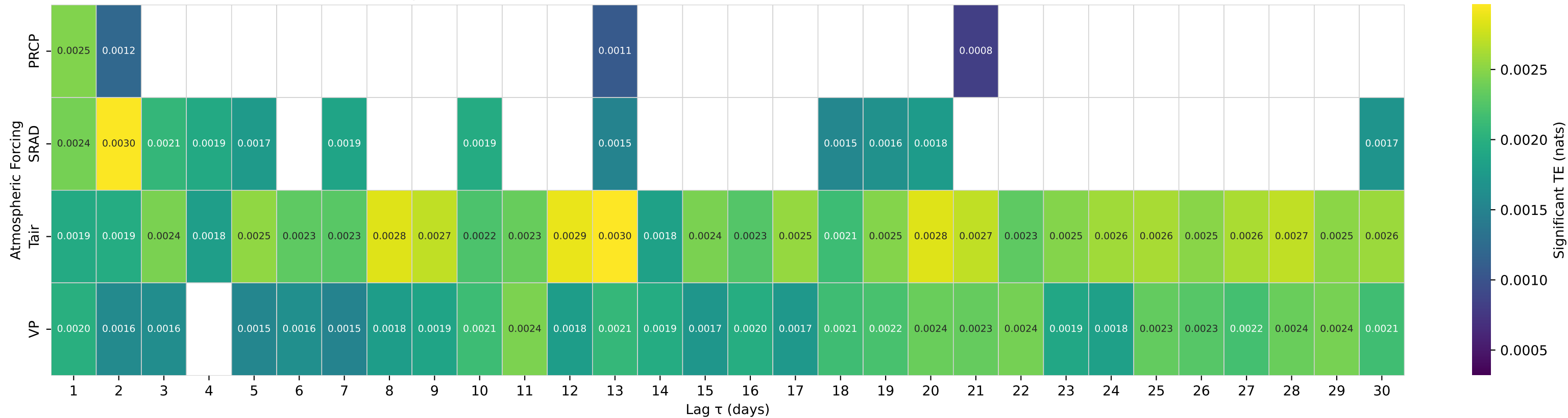
Shuffle-Test Significant TE to Streamflow — Basin 01142500 (HUC 01) — AYERS BROOK AT RANDOLPH, VT
