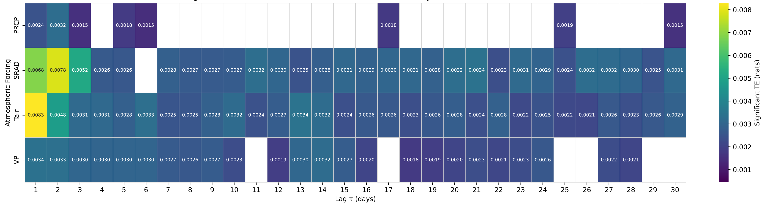
Shuffle-Test Significant TE to Streamflow — Basin 13313000 (HUC 17) — JOHNSON CREEK AT YELLOW PINE ID
