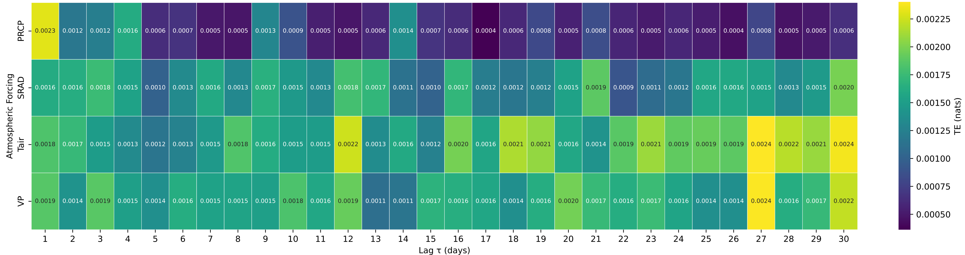
Shuffle-Test Significant TE to Streamflow — Basin 01545600 (HUC 02) — Young Womans Creek near Renovo, PA
