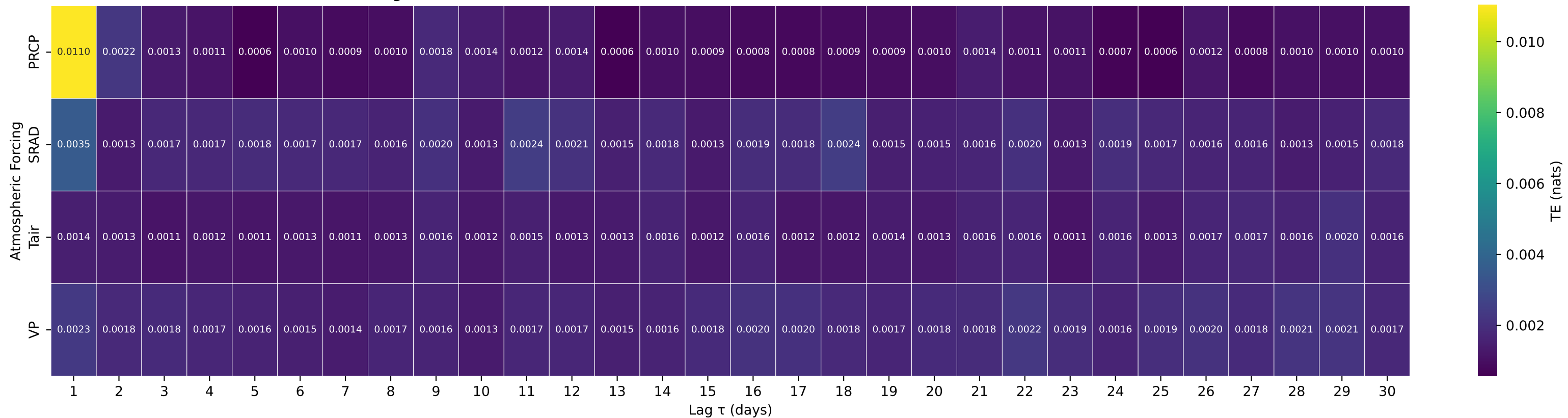
Shuffle-Test Significant TE to Streamflow — Basin 05514500 (HUC 07) — CUIVRE RIVER NEAR TROY, MO
