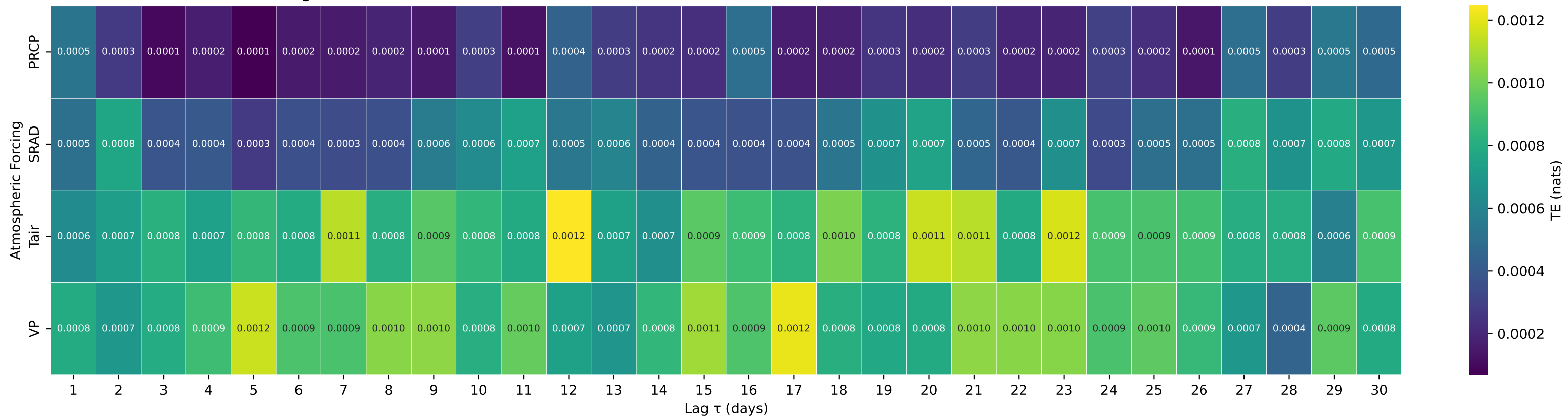
Shuffle-Test Significant TE to Streamflow — Basin 02342933 (HUC 03) — SOUTH FORK COWIKEE CREEK NEAR BATESVILLE AL
