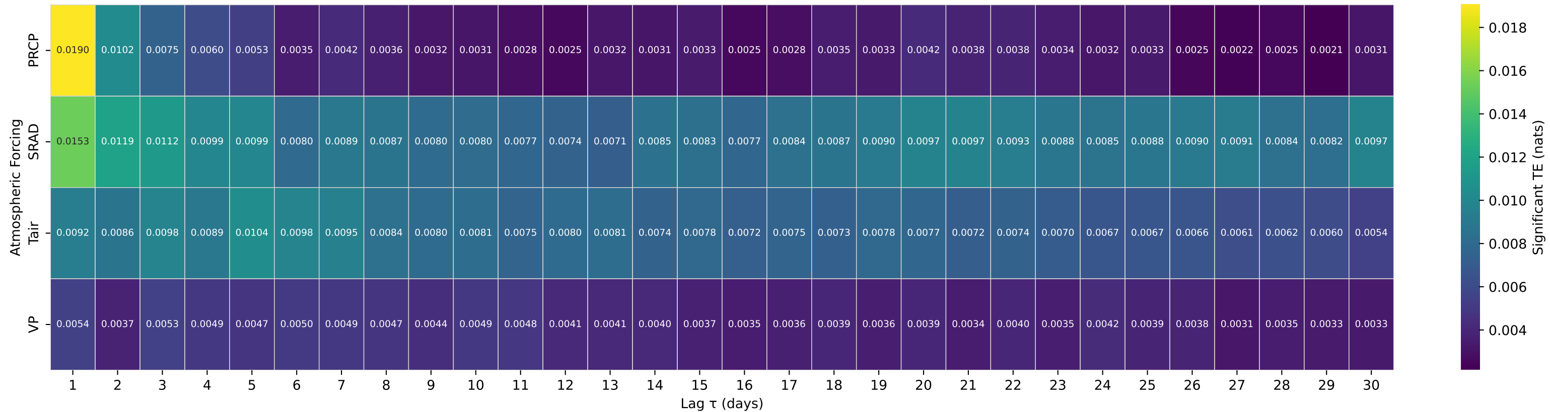
Shuffle-Test Significant TE to Streamflow — Basin 14316700 (HUC 17) — STEAMBOAT CREEK NEAR GLIDE, OR
