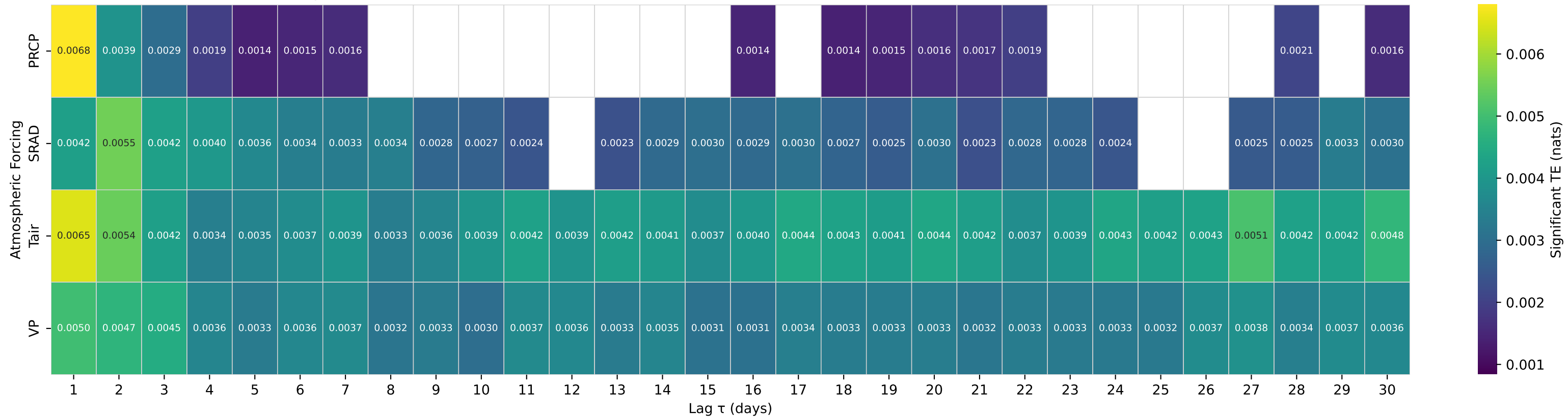
Shuffle-Test Significant TE to Streamflow — Basin 12411000 (HUC 17) — NF COEUR D ALENE R AB SHOSHONE CK NR PRICHARD ID
