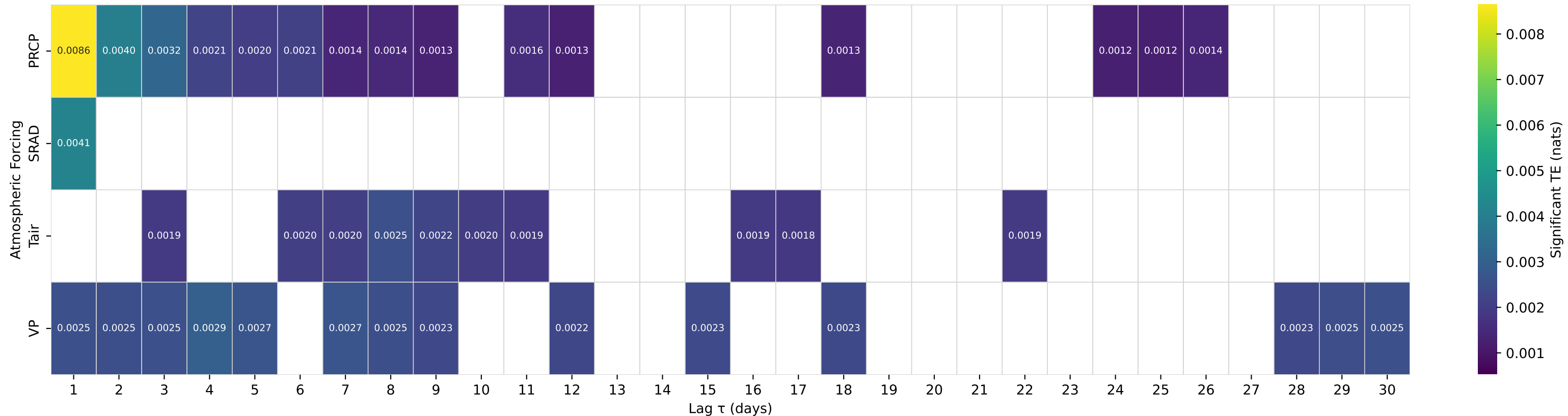
Shuffle-Test Significant TE to Streamflow — Basin 02298608 (HUC 03) — MYAKKA RIVER AT MYAKKA CITY FL
