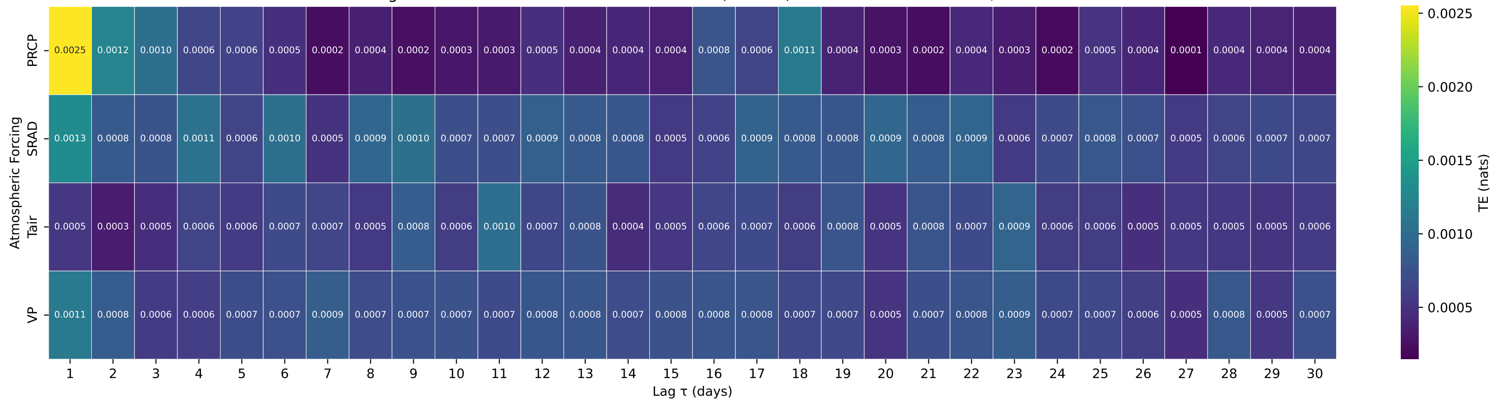
Shuffle-Test Significant TE to Streamflow — Basin 06917000 (HUC 10) — L OSAGE R AT FULTON, KS
