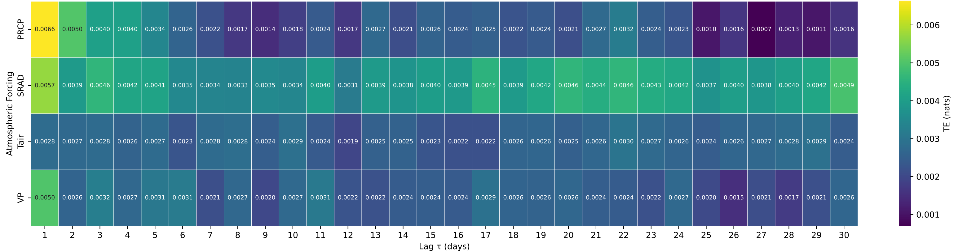
Shuffle-Test Significant TE to Streamflow — Basin 11141280 (HUC 18) — LOPEZ C NR ARROYO GRANDE CA
