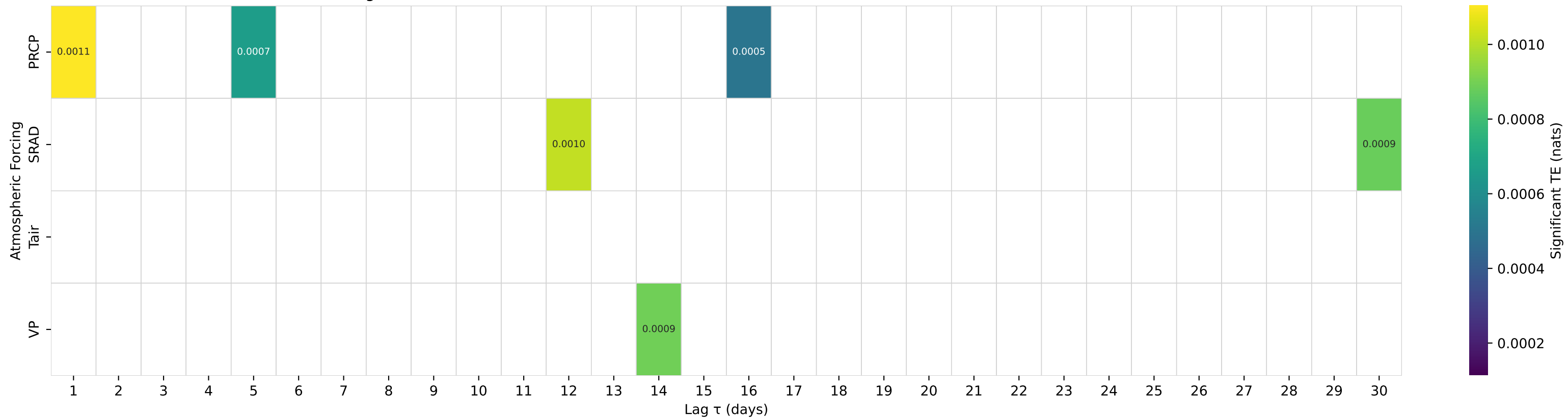
Shuffle-Test Significant TE to Streamflow — Basin 02038850 (HUC 02) — HOLIDAY CREEK NEAR ANDERSONVILLE, VA
