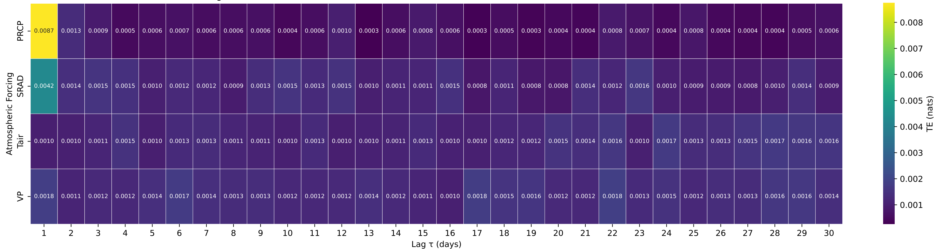
Shuffle-Test Significant TE to Streamflow — Basin 02374500 (HUC 03) — MURDER CREEK NEAR EVERGREEN AL
