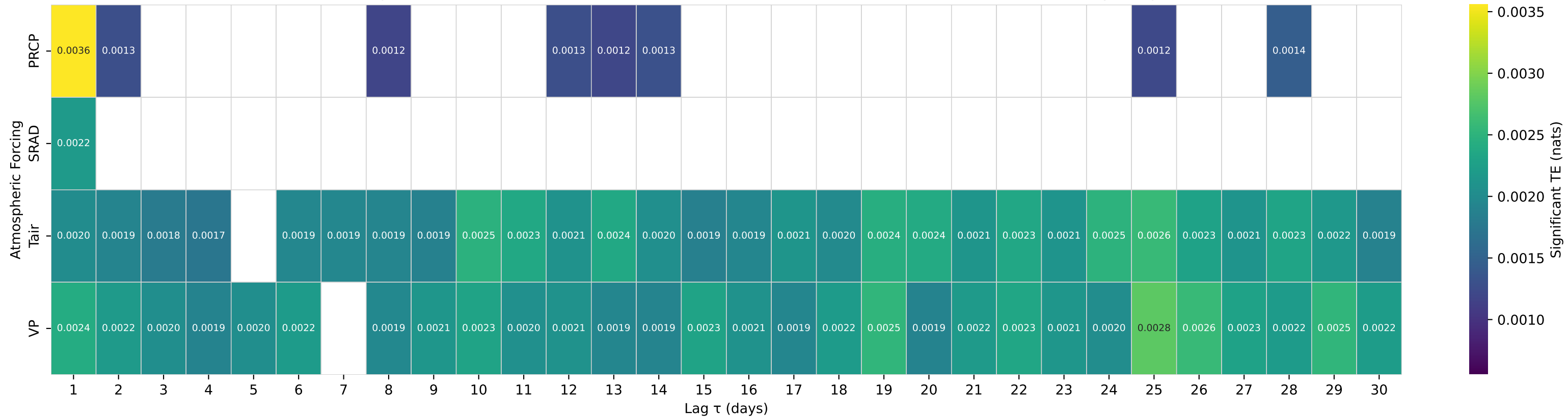
Shuffle-Test Significant TE to Streamflow — Basin 03144000 (HUC 05) — Wakatomika Creek near Frazzysburg OH
