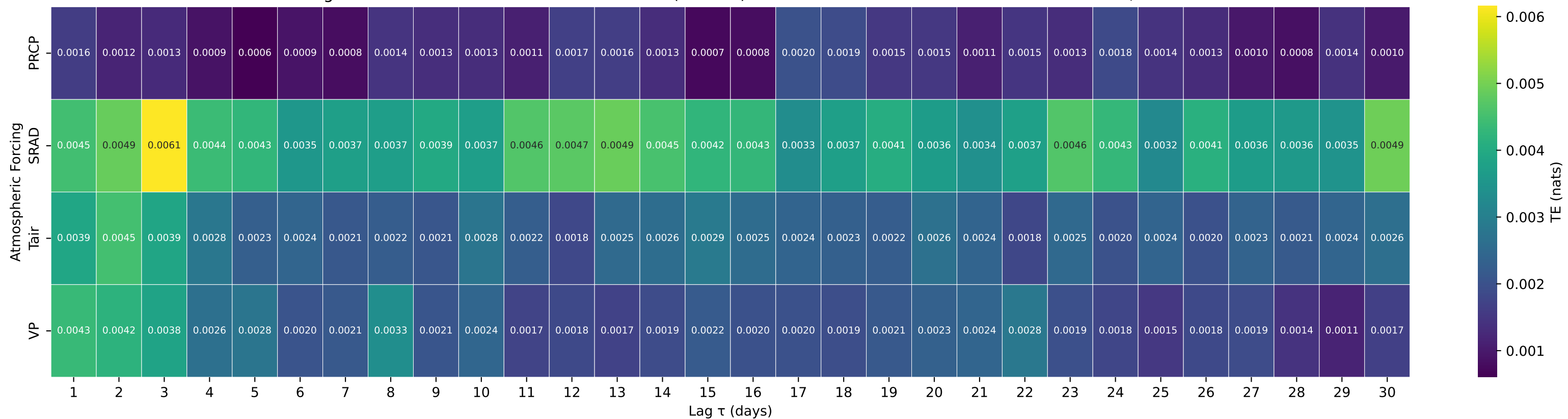
Shuffle-Test Significant TE to Streamflow — Basin 10172800 (HUC 16) — SOUTH WILLOW CREEK NEAR GRANTSVILLE, UT
