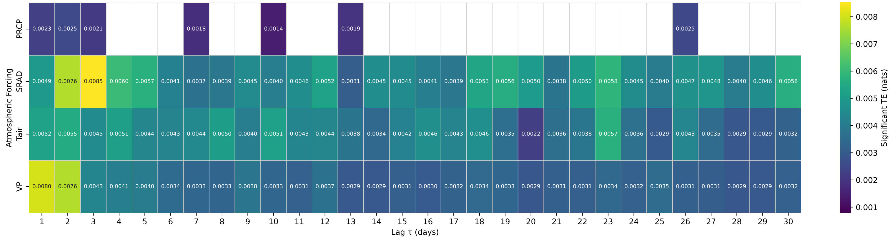
Shuffle-Test Significant TE to Streamflow — Basin 12375900 (HUC 17) — South Crow Creek near Ronan MT
