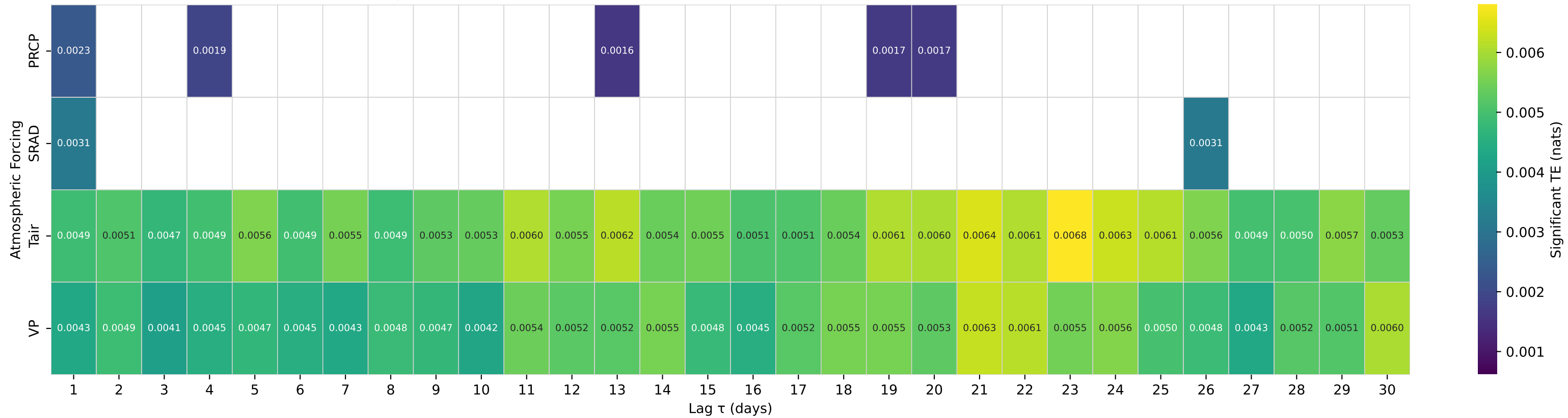
Shuffle-Test Significant TE to Streamflow — Basin 01333000 (HUC 02) — GREEN RIVER AT WILLIAMSTOWN, MA
