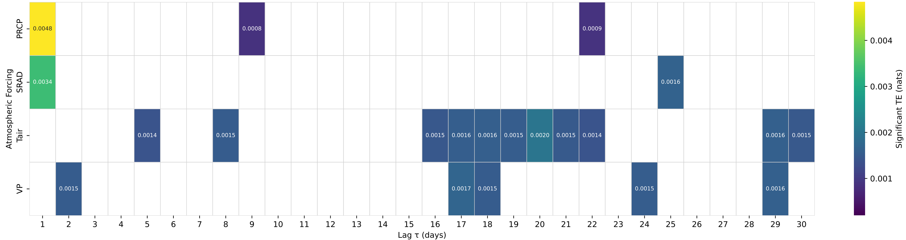
Shuffle-Test Significant TE to Streamflow — Basin 02143000 (HUC 03) — HENRY FORK NEAR HENRY RIVER, NC
