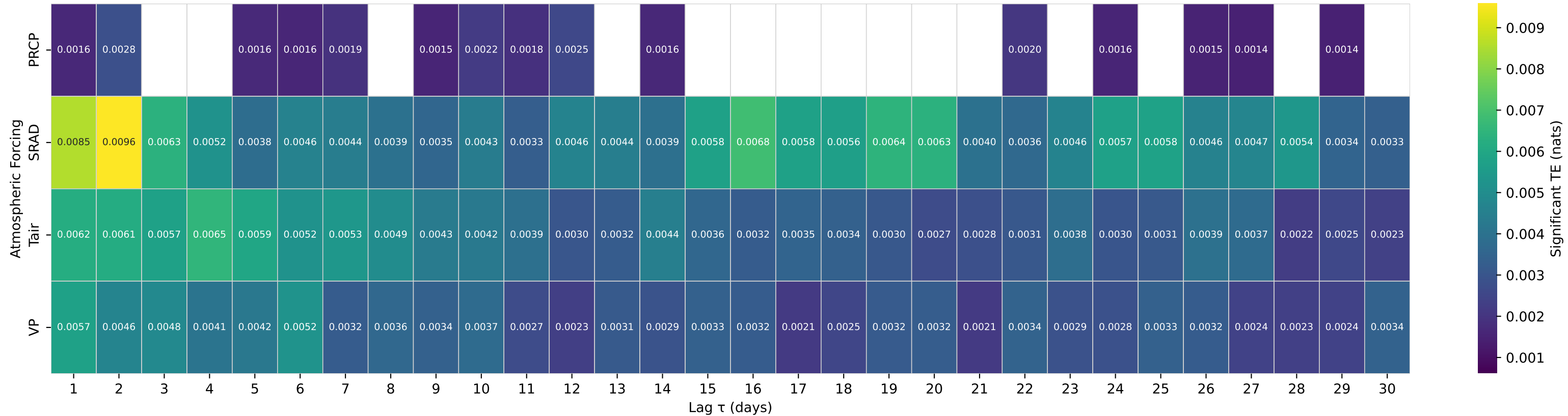
Shuffle-Test Significant TE to Streamflow — Basin 06043500 (HUC 10) — Gallatin River near Gallatin Gateway MT
