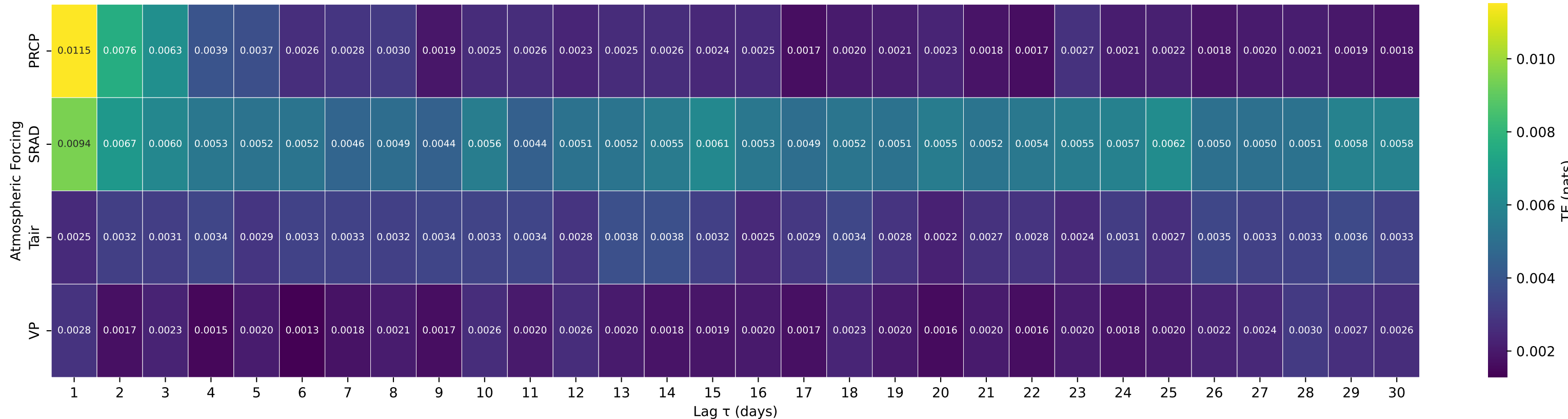
Shuffle-Test Significant TE to Streamflow — Basin 11481200 (HUC 18) — LITTLE R NR TRINIDAD CA
