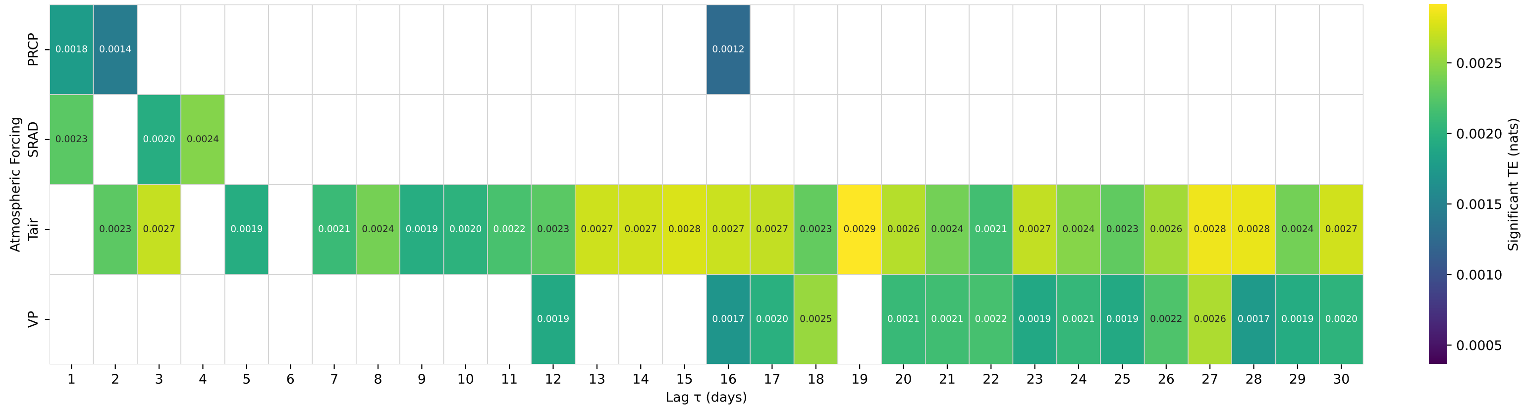
Shuffle-Test Significant TE to Streamflow — Basin 04224775 (HUC 04) — CANASERAGA CREEK ABOVE DANSVILLE NY
