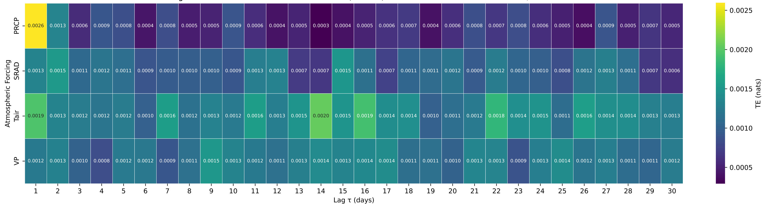
Shuffle-Test Significant TE to Streamflow — Basin 01440400 (HUC 02) — Brodhead Creek near Analomink, PA
