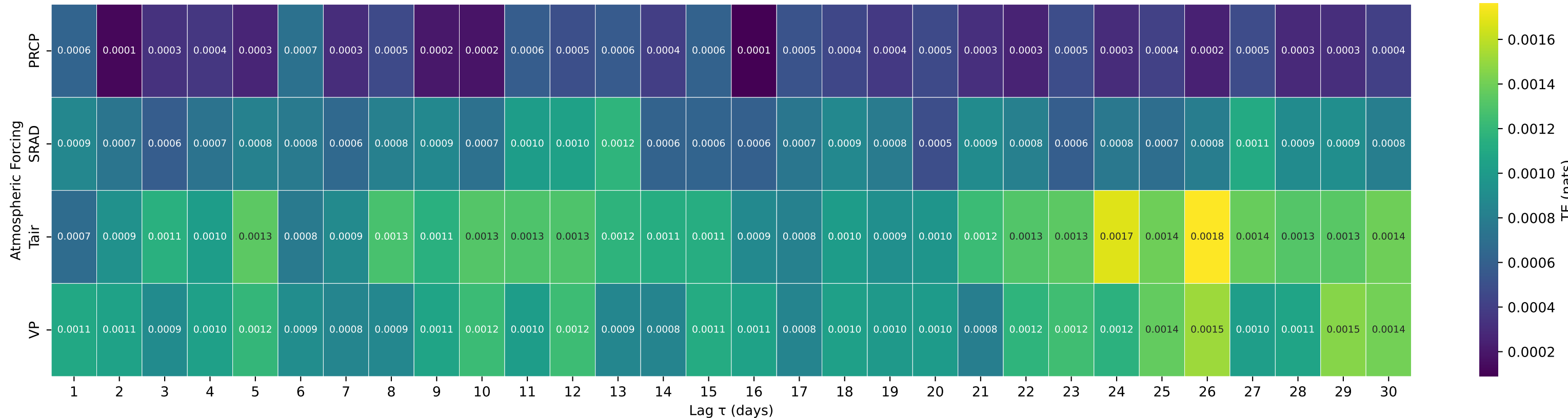
Shuffle-Test Significant TE to Streamflow — Basin 02011460 (HUC 02) — BACK CREEK NEAR SUNRISE, VA
