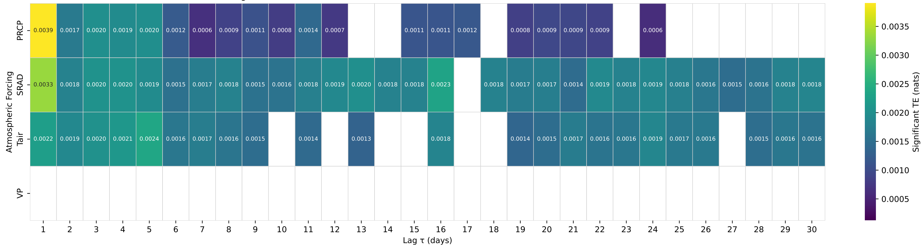
Shuffle-Test Significant TE to Streamflow — Basin 11098000 (HUC 18) — ARROYO SECO NR PASADENA CA
