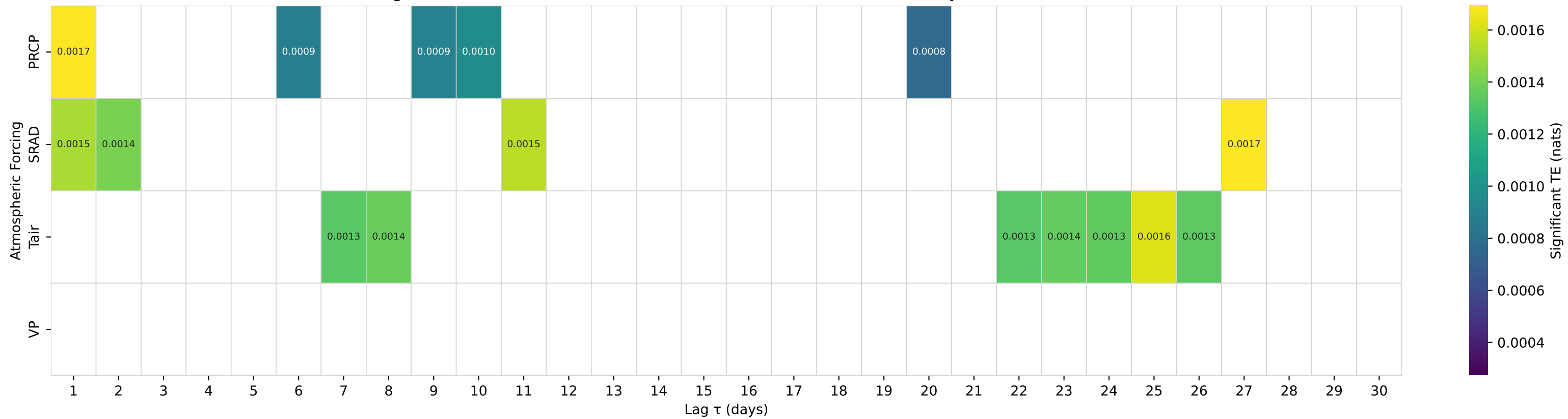
Shuffle-Test Significant TE to Streamflow — Basin 01613050 (HUC 02) — Tonoloway Creek near Needmore, PA
