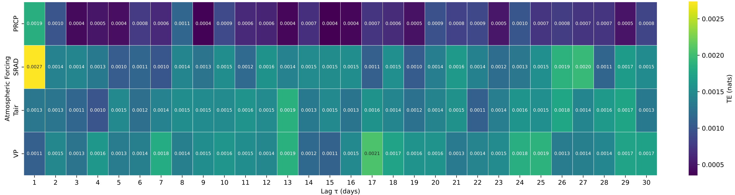
Shuffle-Test Significant TE to Streamflow — Basin 02111500 (HUC 03) — REDDIES RIVER AT NORTH WILKESBORO, NC
