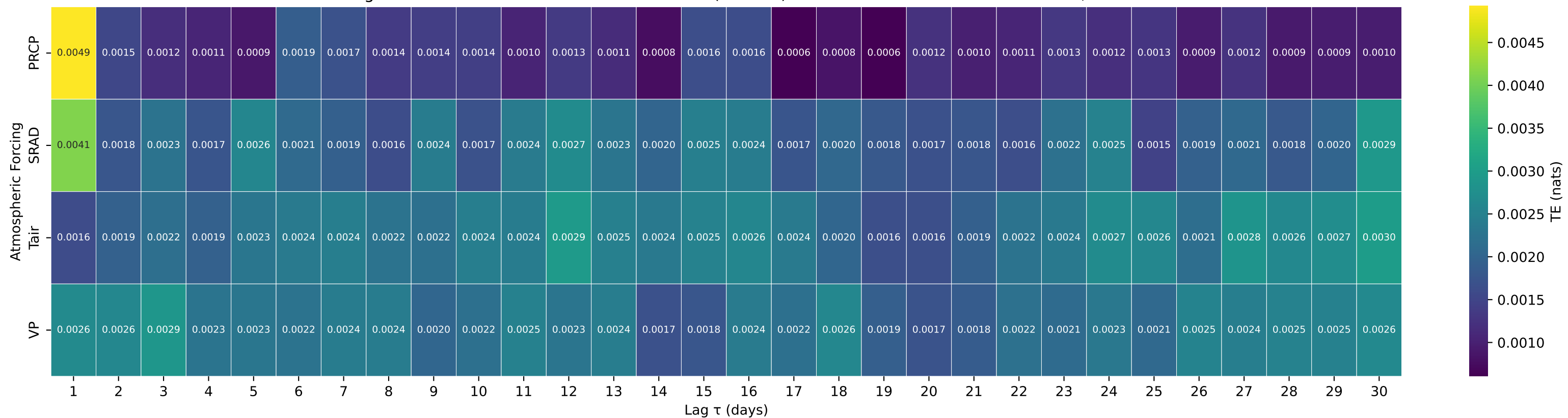
Shuffle-Test Significant TE to Streamflow — Basin 03170000 (HUC 05) — LITTLE RIVER AT GRAYSONTOWN, VA
