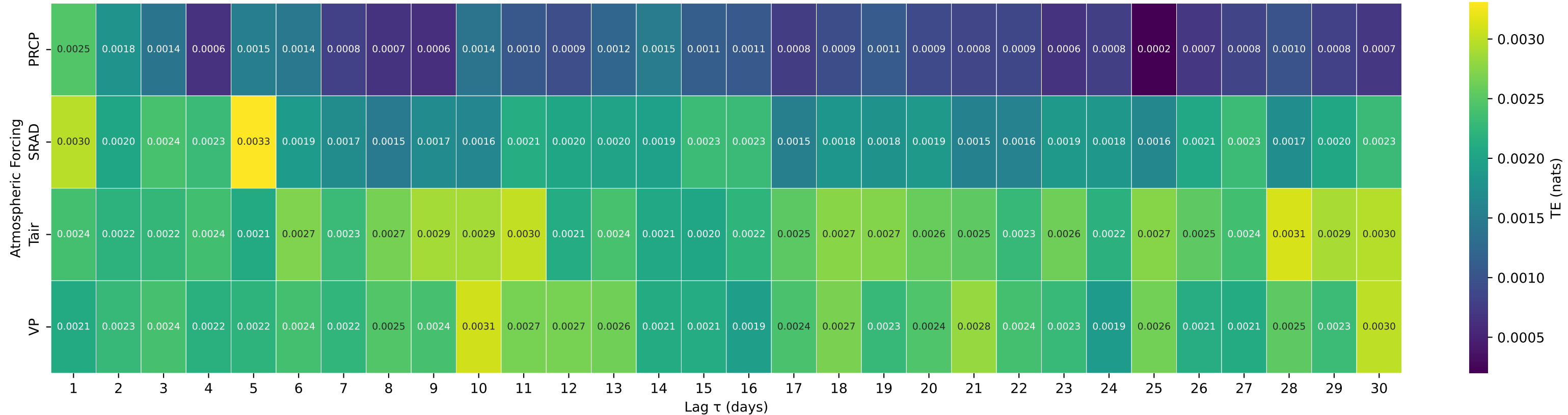
Shuffle-Test Significant TE to Streamflow — Basin 02430085 (HUC 03) — RED BUD CREEK NR MOORES MILL, MS
