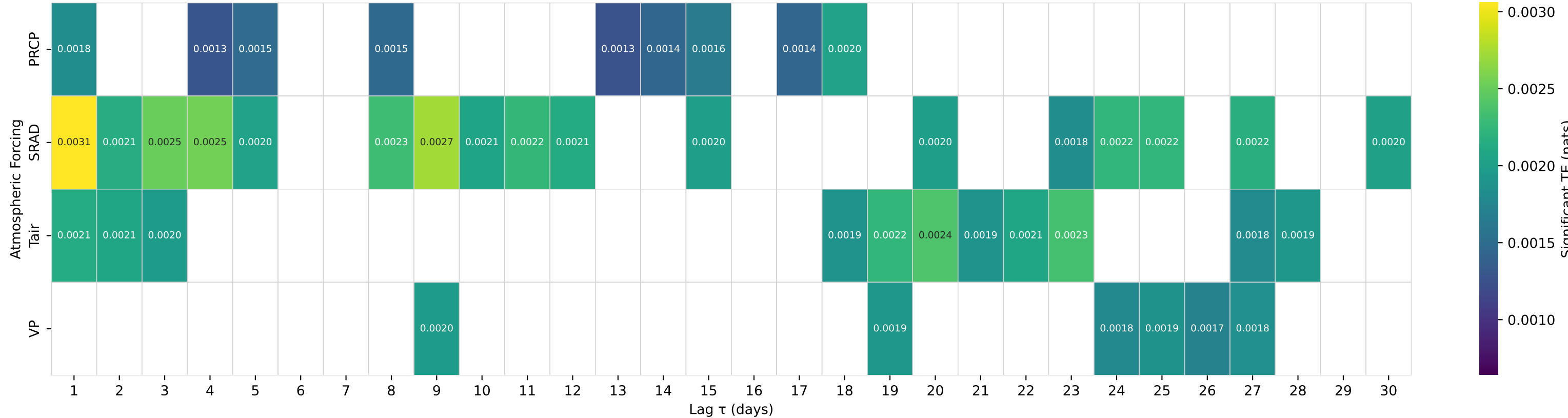
Shuffle-Test Significant TE to Streamflow — Basin 06408700 (HUC 10) — RHOADS FORK NEAR ROCHFORD SD
