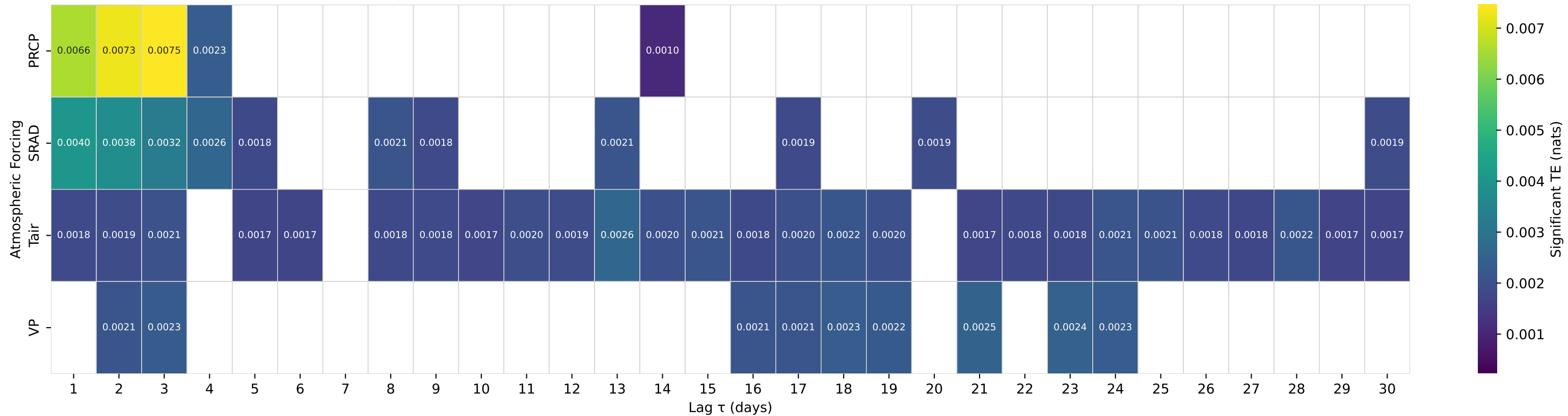
Shuffle-Test Significant TE to Streamflow — Basin 08013000 (HUC 08) — CALCASIEU RIVER NR GLENMORA, LA
