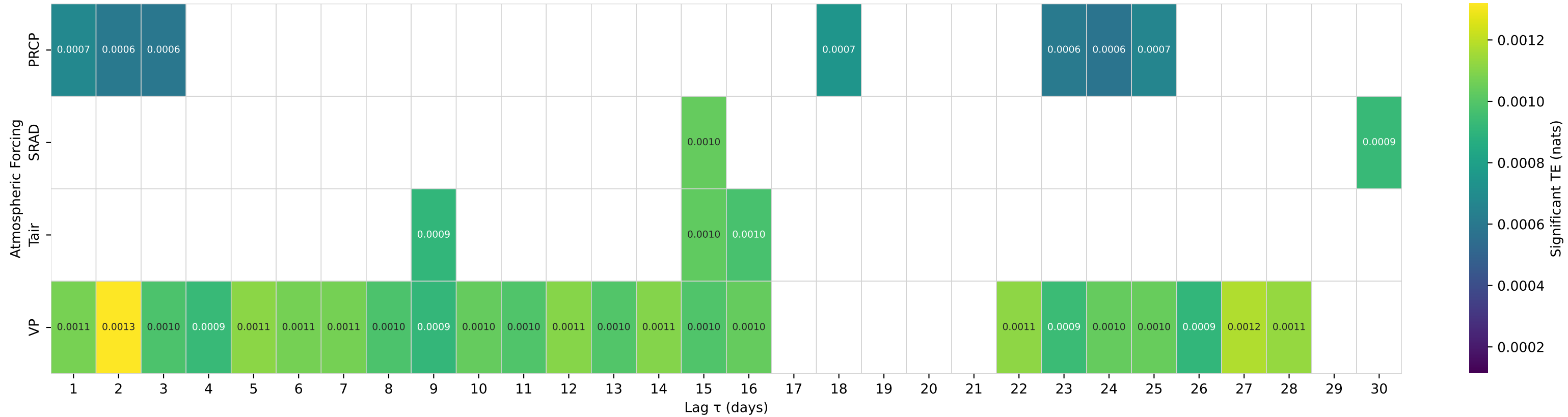
Shuffle-Test Significant TE to Streamflow — Basin 06803510 (HUC 10) — LITTLE SALT CREEK NEAR LINCOLN, NEBR.
