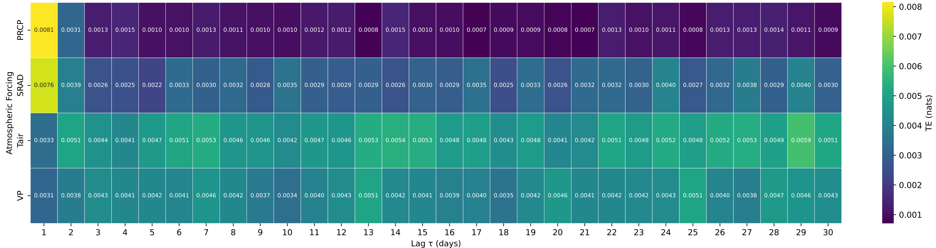
Shuffle-Test Significant TE to Streamflow — Basin 02196000 (HUC 03) — STEVENS CREEK NEAR MODOC, SC
