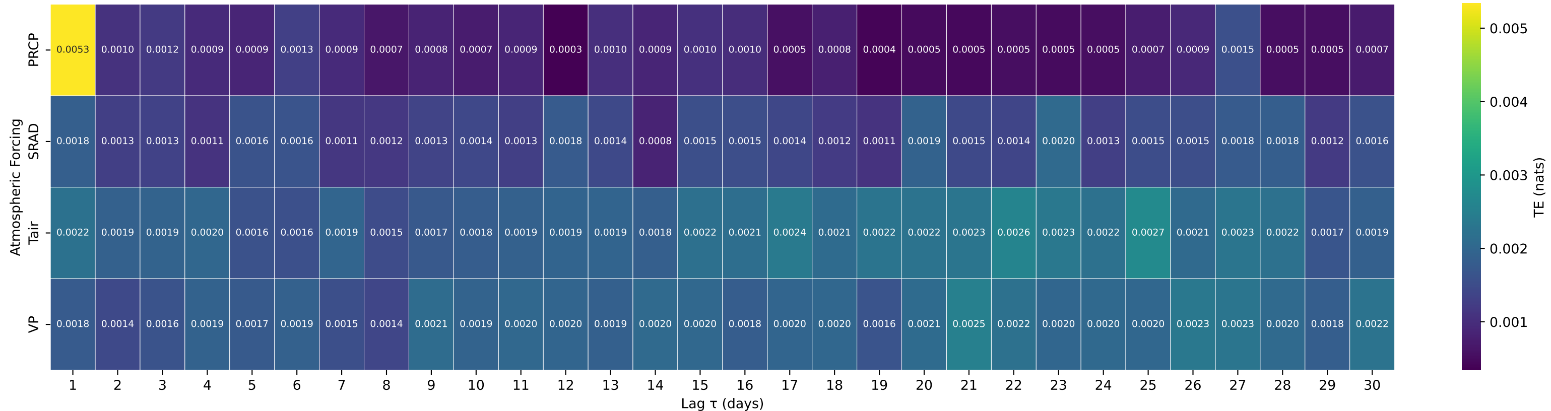
Shuffle-Test Significant TE to Streamflow — Basin 01123000 (HUC 01) — LITTLE RIVER NEAR HANOVER, CT.
