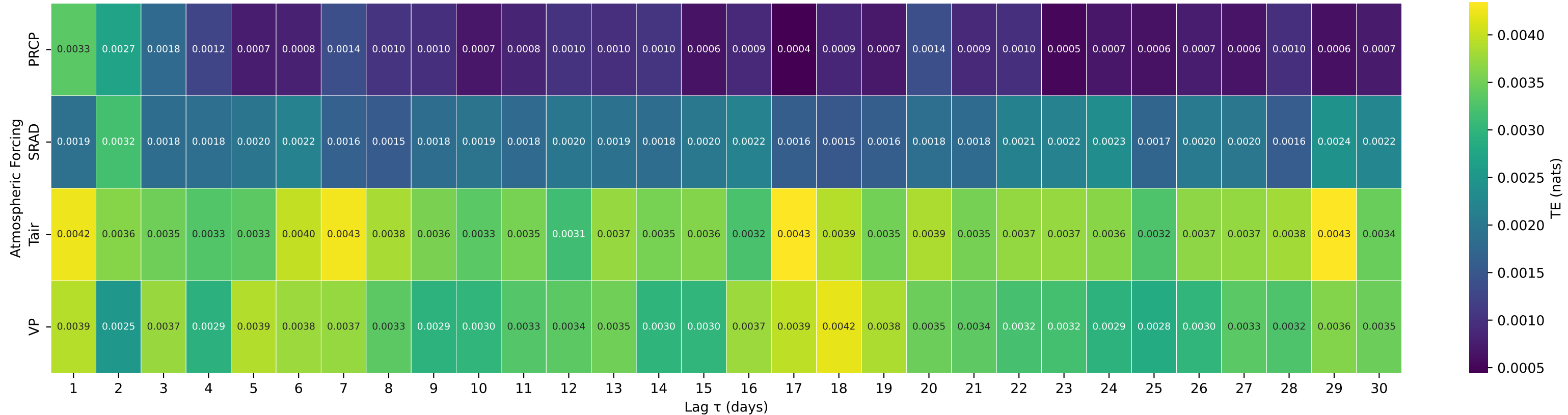
Shuffle-Test Significant TE to Streamflow — Basin 03015500 (HUC 05) — Brokenstraw Creek at Youngsville, PA
