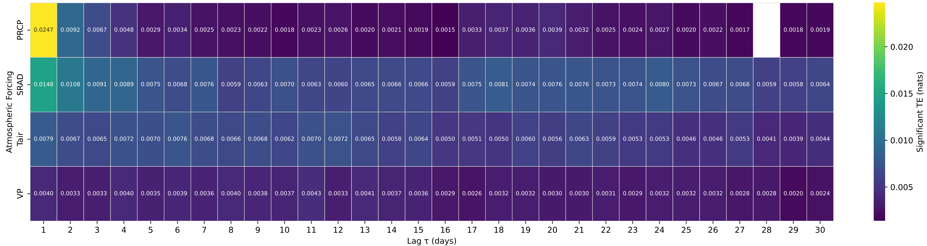
Shuffle-Test Significant TE to Streamflow — Basin 14185900 (HUC 17) — QUARTZVILLE CREEK NEAR CASCADIA, OREG.
