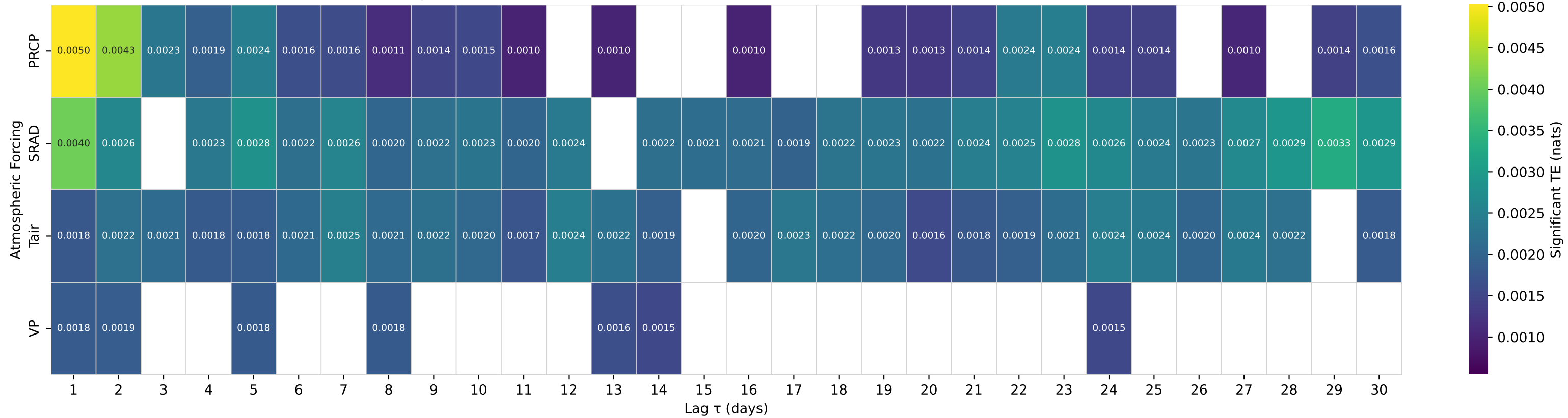
Shuffle-Test Significant TE to Streamflow — Basin 11274500 (HUC 18) — ORESTIMBA C NR NEWMAN CA
