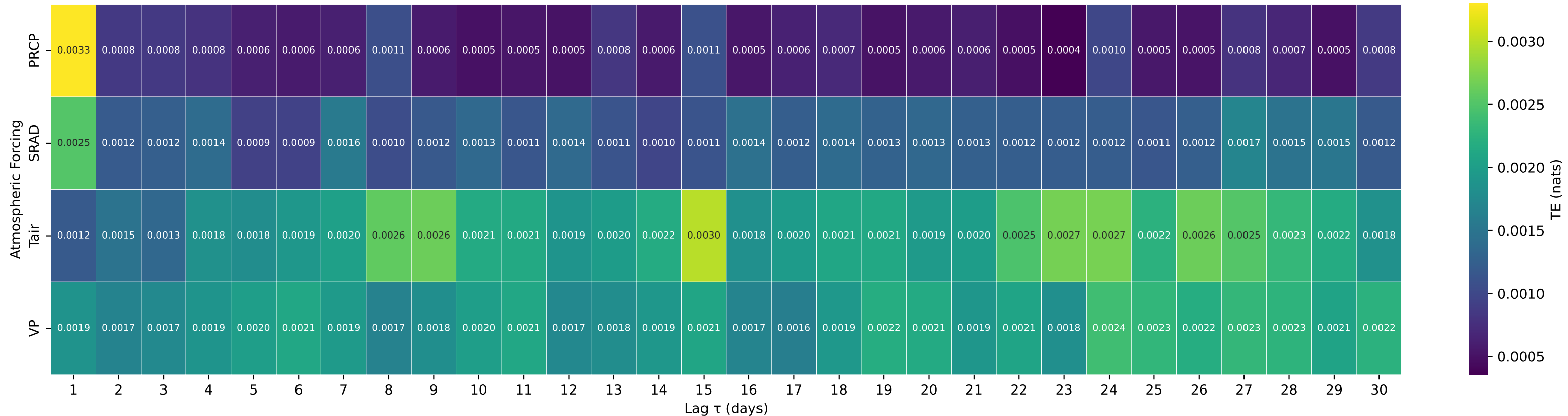
Shuffle-Test Significant TE to Streamflow — Basin 03488000 (HUC 06) — N F HOLSTON RIVER NEAR SALTVILLE, VA
