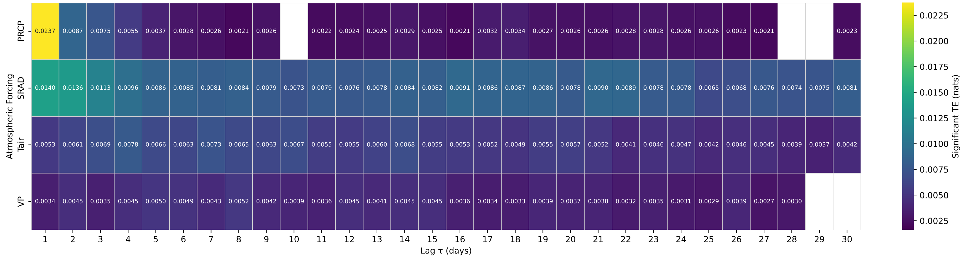
Shuffle-Test Significant TE to Streamflow — Basin 12043000 (HUC 17) — CALAWAH RIVER NEAR FORKS, WA
