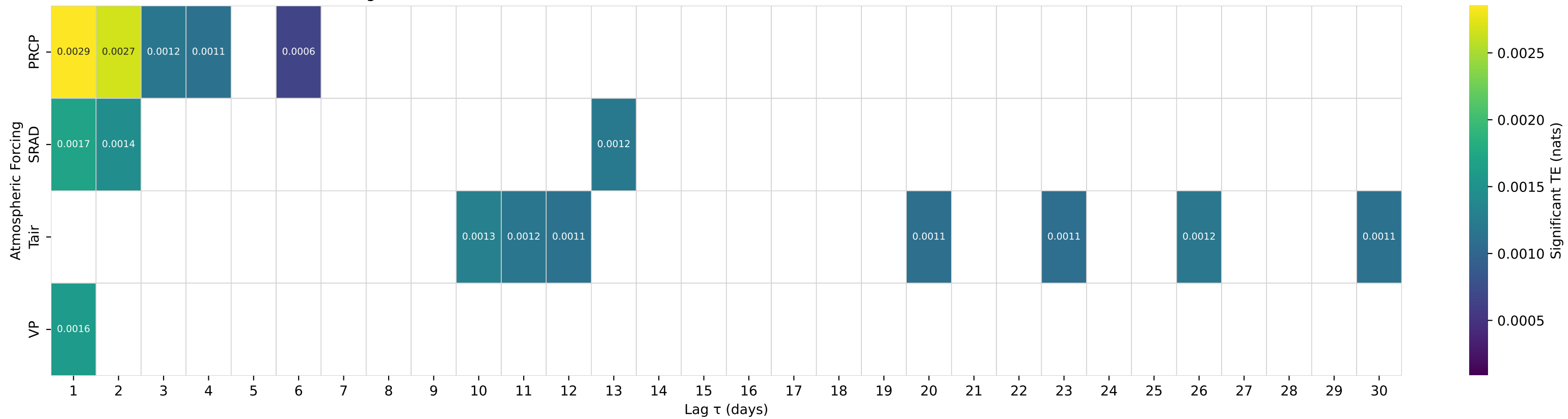
Shuffle-Test Significant TE to Streamflow — Basin 02350900 (HUC 03) — KINCHAFOONEE CREEK NEAR DAWSON, GA
