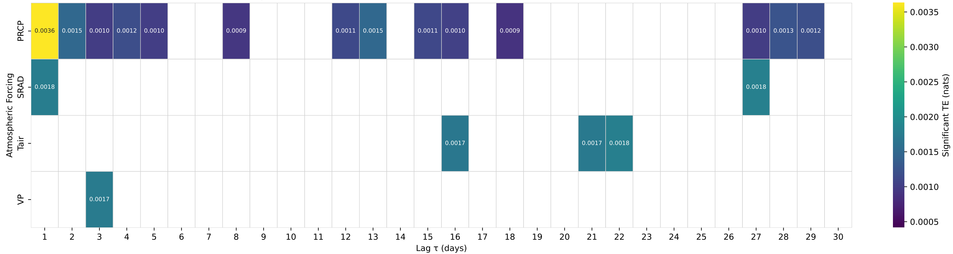
Shuffle-Test Significant TE to Streamflow — Basin 07301410 (HUC 11) — Sweetwater Ck nr Kelton, TX
