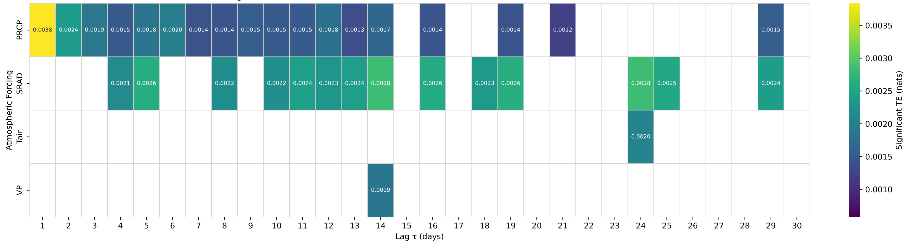
Shuffle-Test Significant TE to Streamflow — Basin 06431500 (HUC 10) — SPEARFISH CR AT SPEARFISH SD
