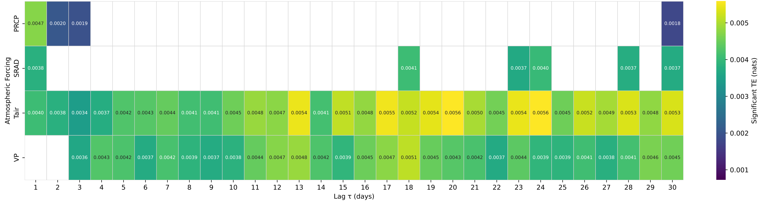
Shuffle-Test Significant TE to Streamflow — Basin 04197170 (HUC 04) — Rock Creek at Tiffin OH
