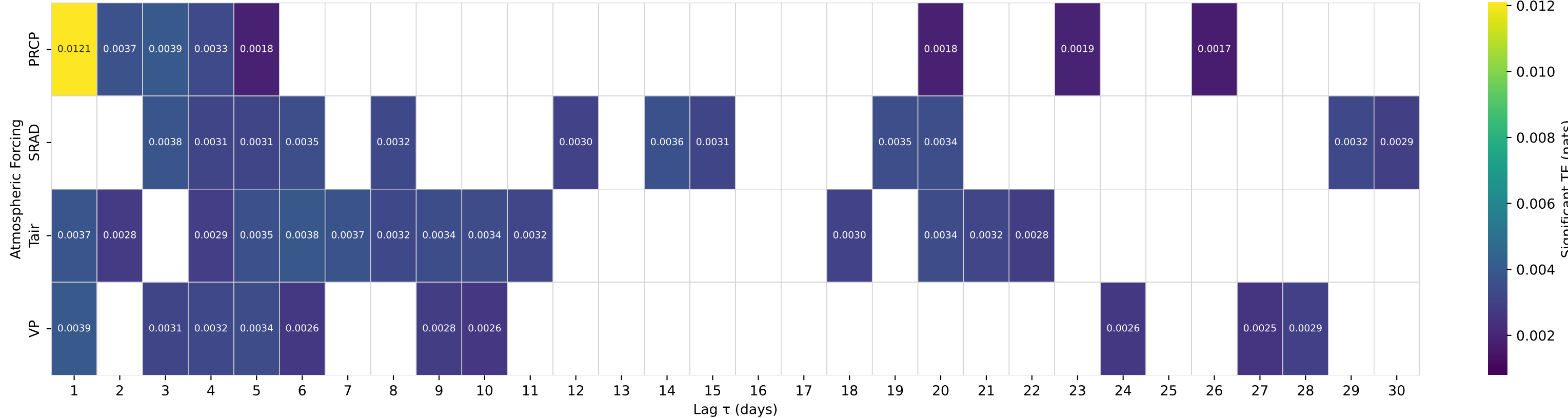
Shuffle-Test Significant TE to Streamflow — Basin 05362000 (HUC 07) — JUMP RIVER AT SHELDON, WI
