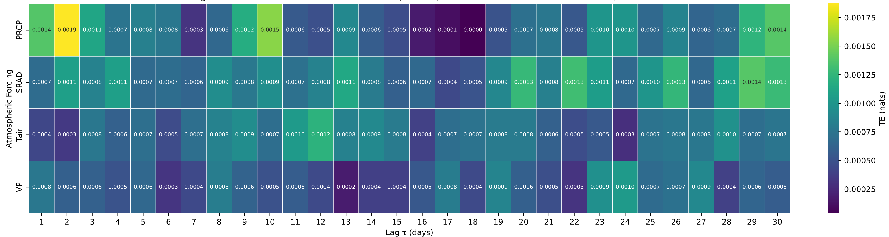
Shuffle-Test Significant TE to Streamflow — Basin 10310500 (HUC 16) — CLEAR CREEK NEAR CARSON CITY, NV
