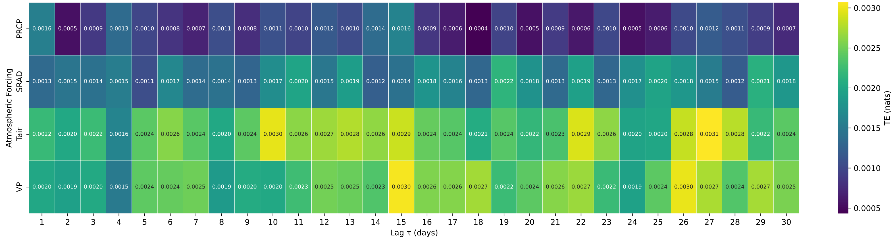
Shuffle-Test Significant TE to Streamflow — Basin 03368000 (HUC 05) — BRUSH CREEK NEAR NEBRASKA, IN
