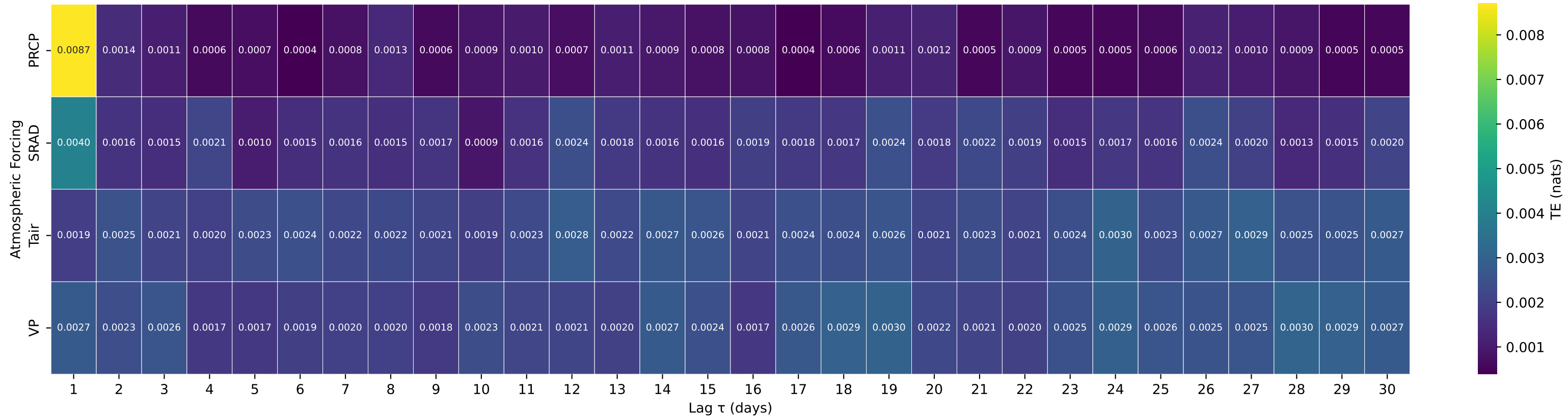
Shuffle-Test Significant TE to Streamflow — Basin 03300400 (HUC 05) — BEECH FORK AT MAUD, KY
