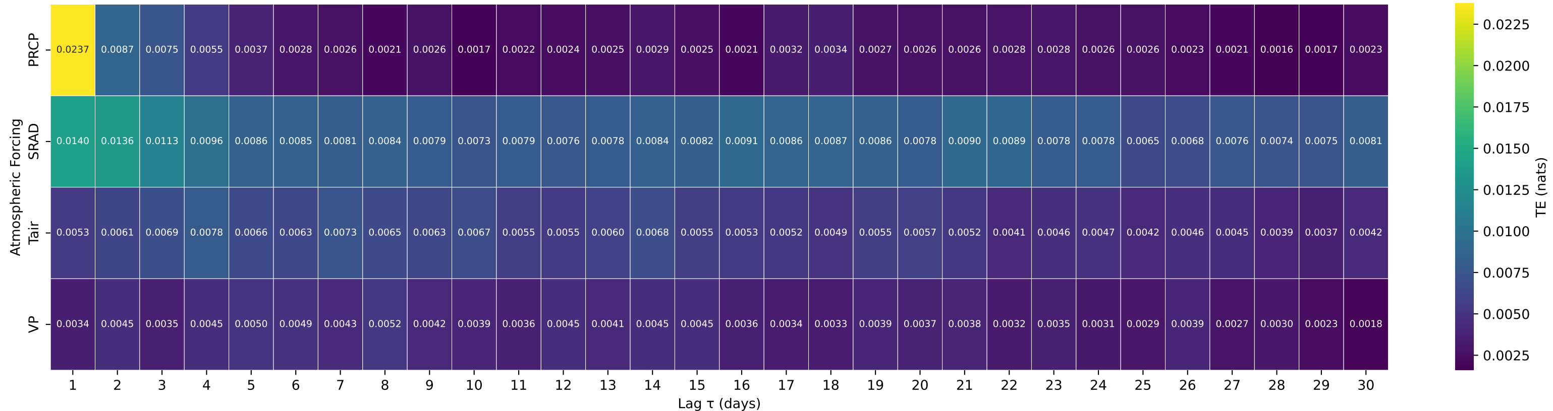
Shuffle-Test Significant TE to Streamflow — Basin 12043000 (HUC 17) — CALAWAH RIVER NEAR FORKS, WA
