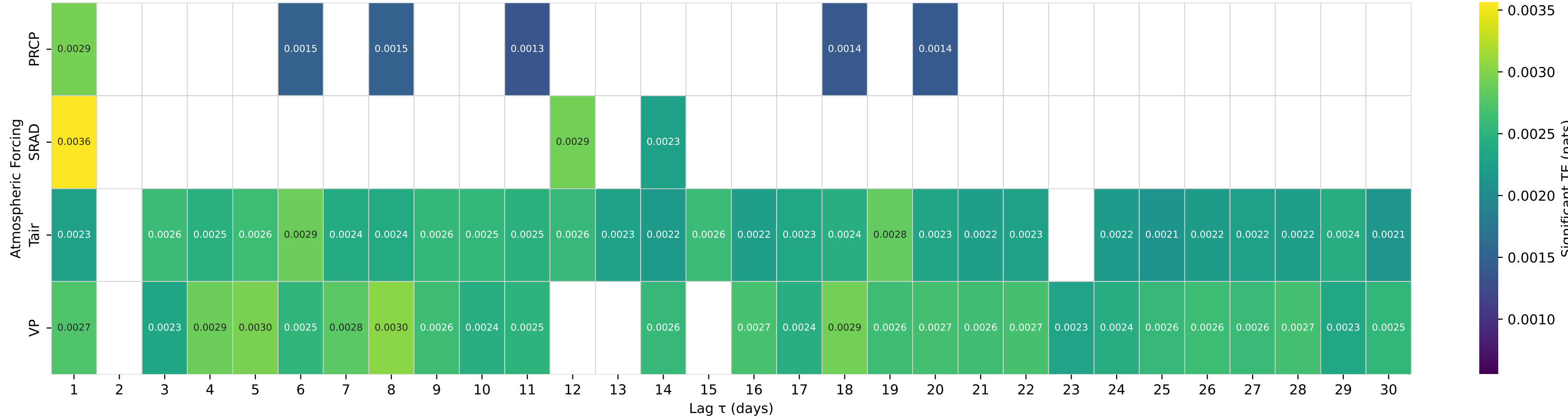
Shuffle-Test Significant TE to Streamflow — Basin 03455500 (HUC 06) — W F PIGEON R ABOVE LAKE LOGAN NR HAZELWOOD, NC
