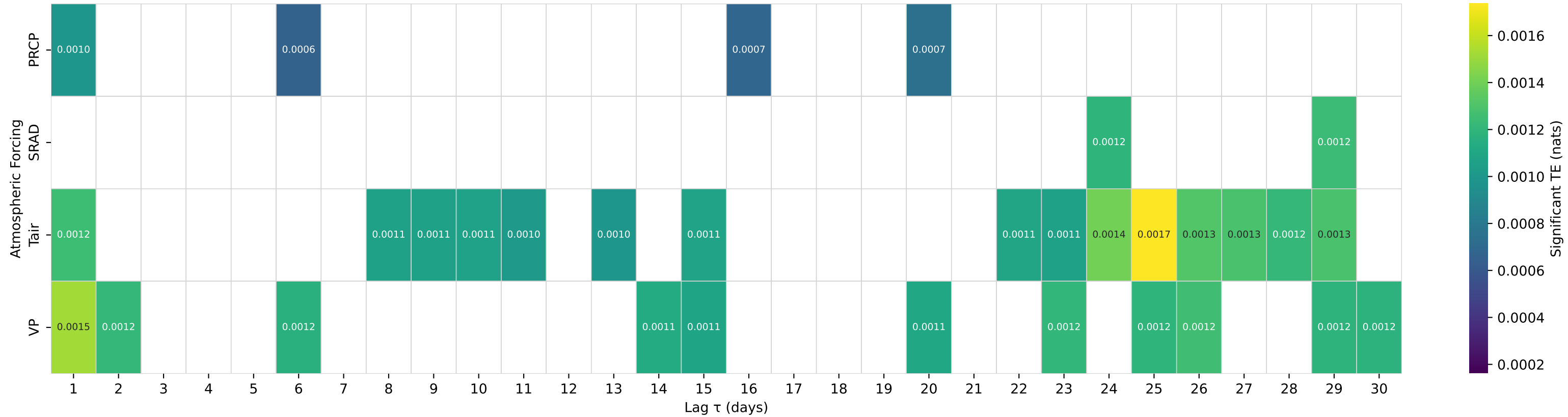
Shuffle-Test Significant TE to Streamflow — Basin 02011400 (HUC 02) — JACKSON RIVER NEAR BACOVA, VA
