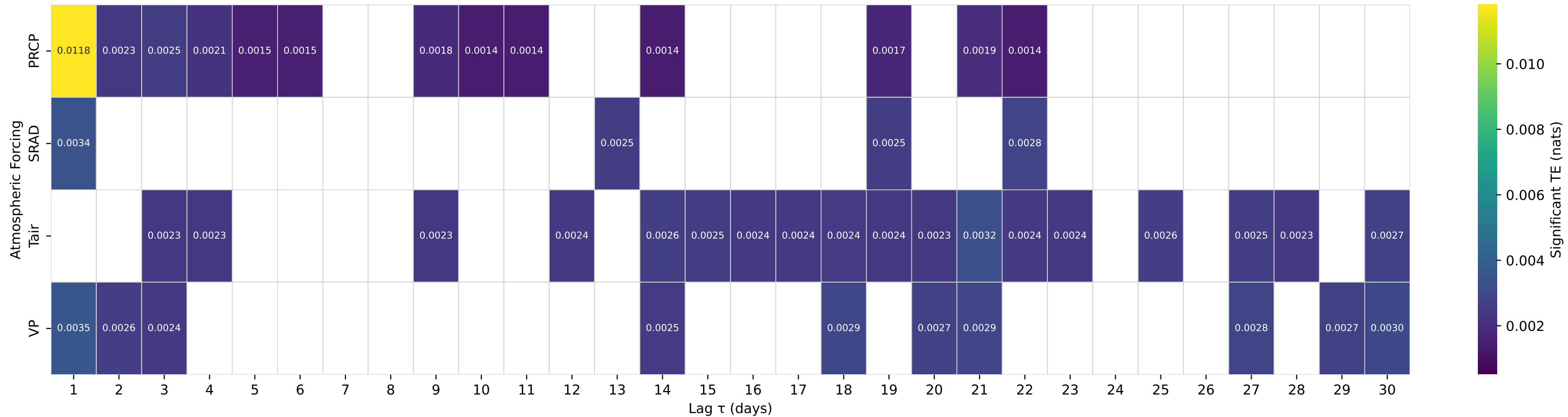
Shuffle-Test Significant TE to Streamflow — Basin 06919500 (HUC 10) — Cedar Creek near Pleasant View, MO
