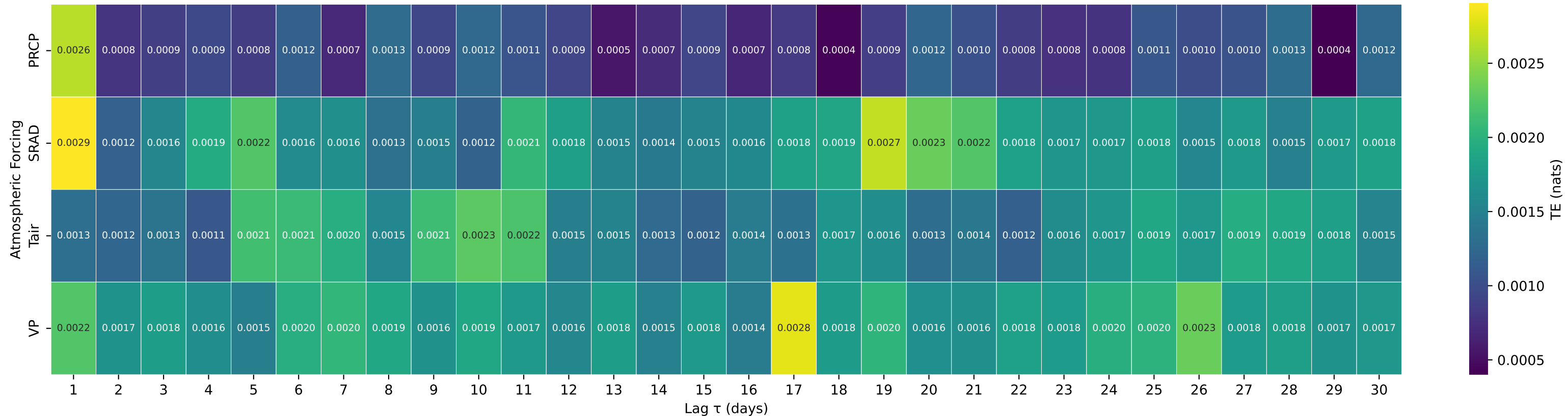
Shuffle-Test Significant TE to Streamflow — Basin 03165000 (HUC 05) — CHESTNUT CREEK AT GALAX, VA
