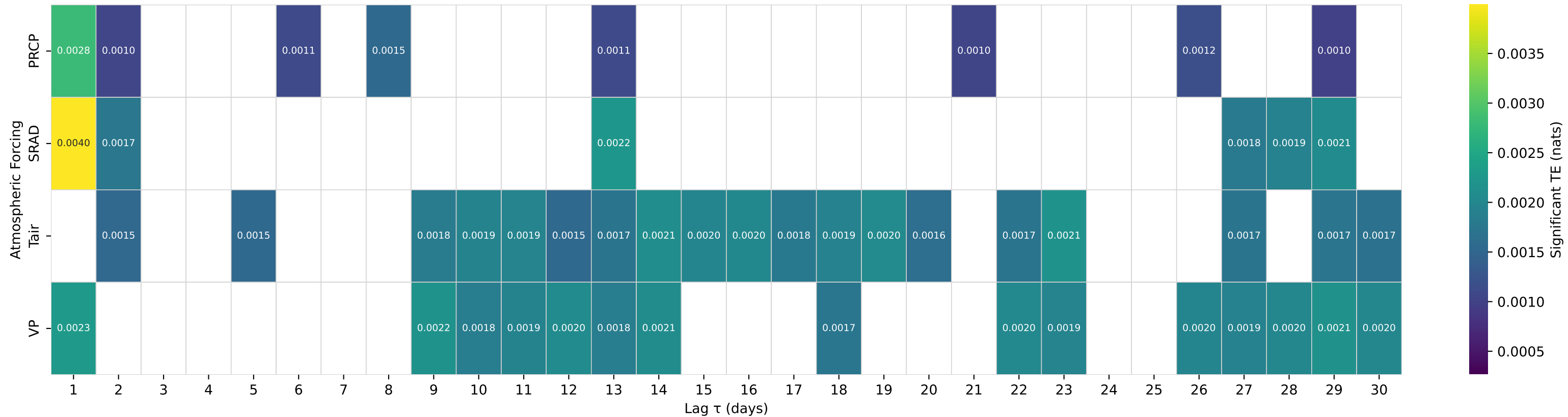
Shuffle-Test Significant TE to Streamflow — Basin 02178400 (HUC 03) — TALLULAH RIVER NEAR CLAYTON, GA
