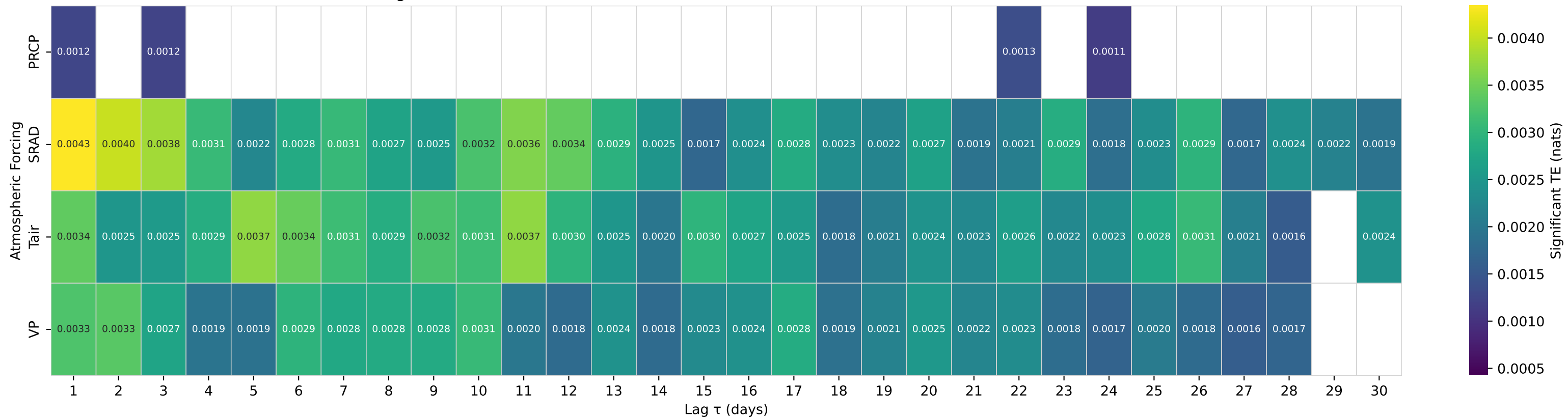
Shuffle-Test Significant TE to Streamflow — Basin 09066300 (HUC 14) — MIDDLE CREEK NEAR MINTURN, CO.
