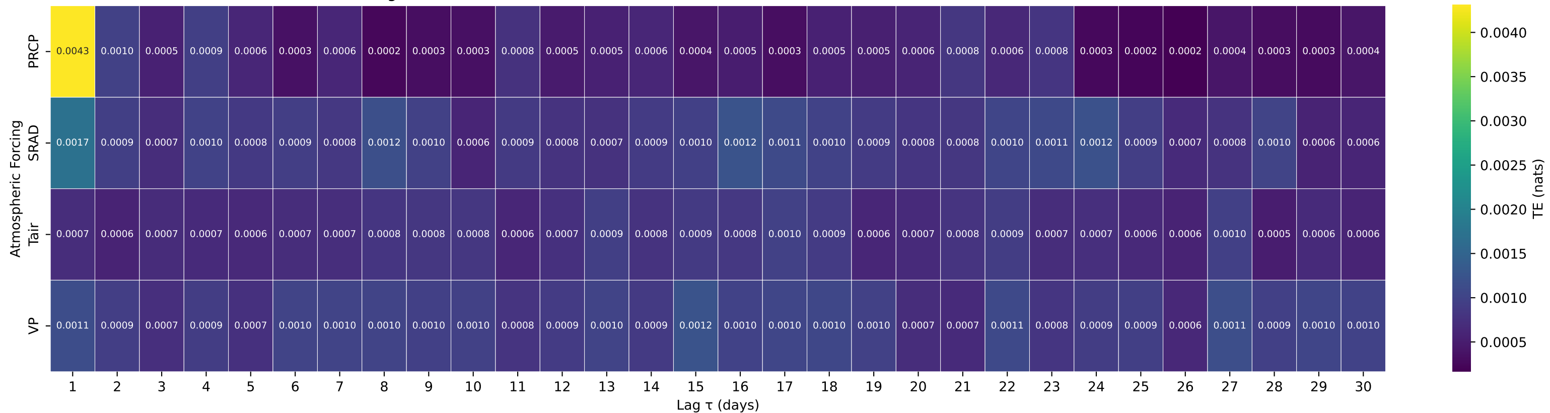
Shuffle-Test Significant TE to Streamflow — Basin 07184000 (HUC 11) — LIGHTNING C NR MCCUNE, KS
