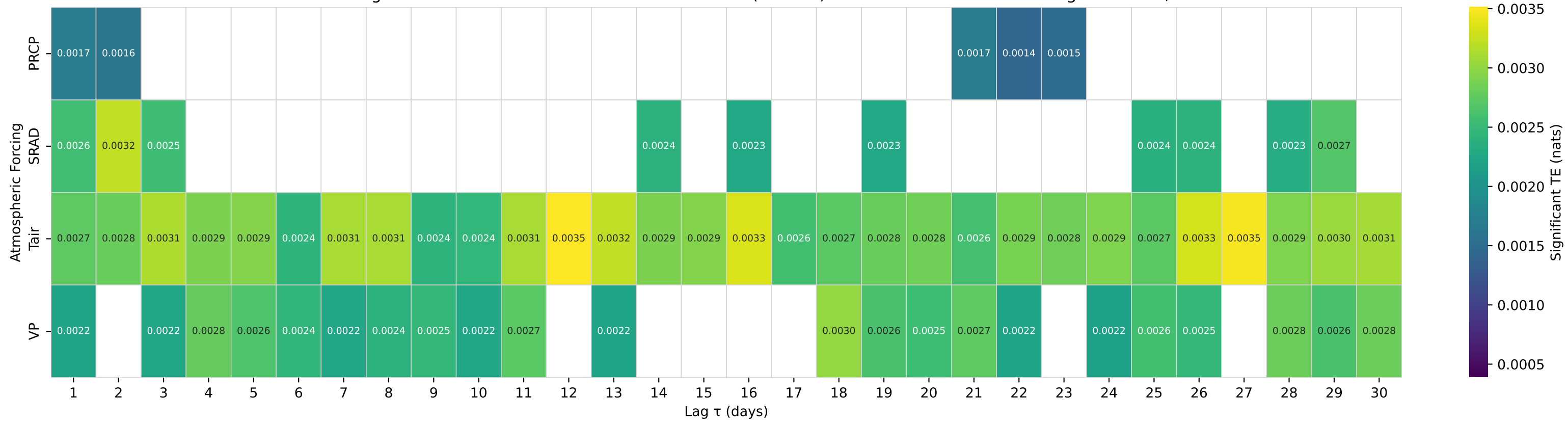
Shuffle-Test Significant TE to Streamflow — Basin 01549500 (HUC 02) — Blockhouse Creek near English Center, PA
