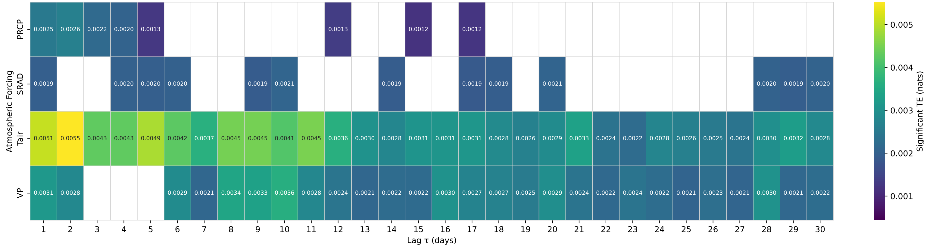
Shuffle-Test Significant TE to Streamflow — Basin 04045500 (HUC 04) — TAHQUAMENON RIVER NEAR PARADISE, MI
