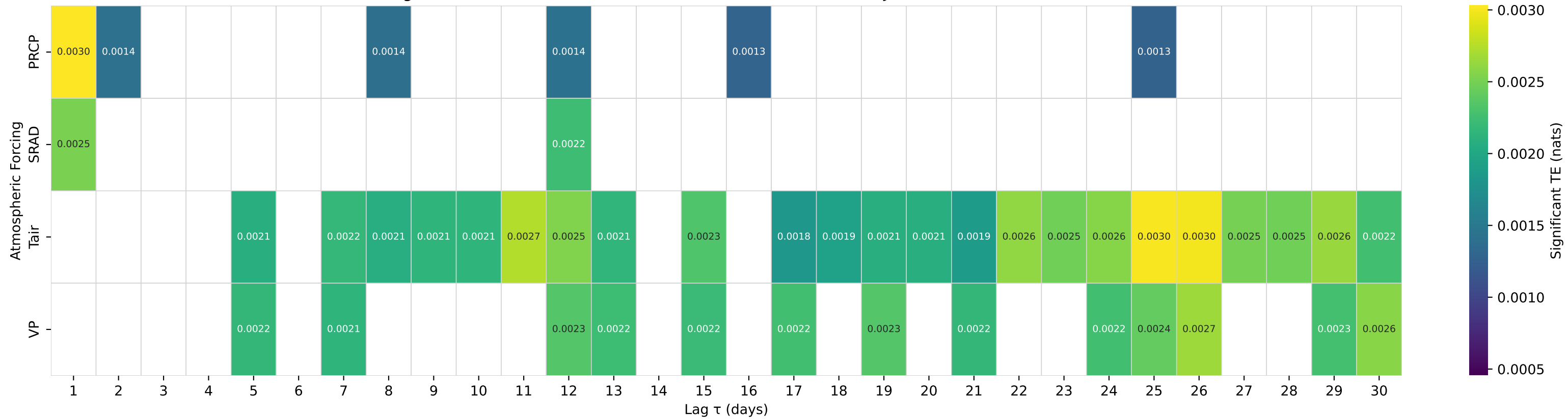
Shuffle-Test Significant TE to Streamflow — Basin 02017500 (HUC 02) — JOHNS CREEK AT NEW CASTLE, VA
