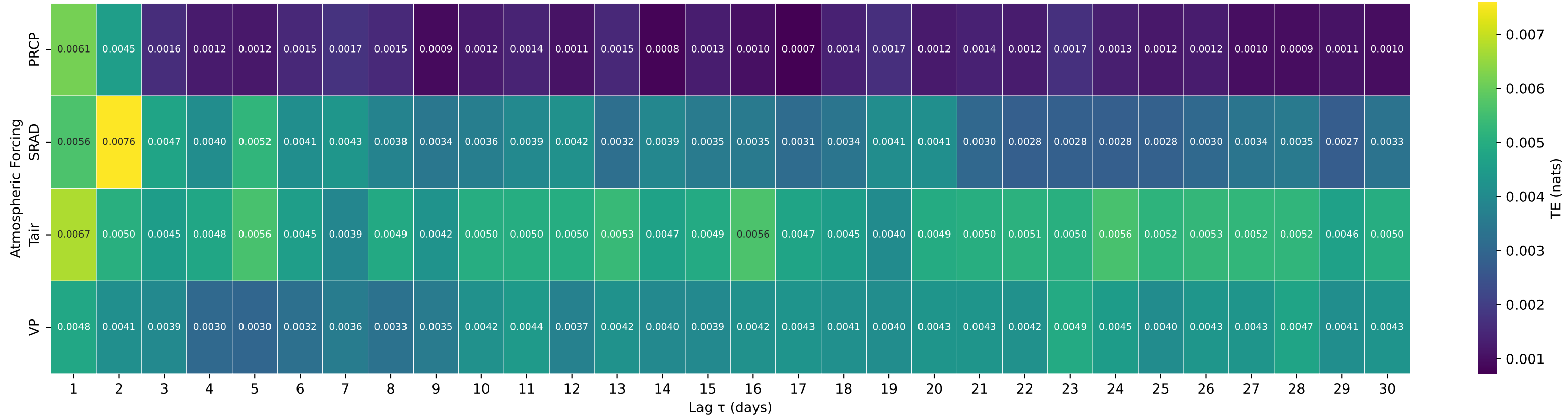
Shuffle-Test Significant TE to Streamflow — Basin 01139000 (HUC 01) — WELLS RIVER AT WELLS RIVER, VT
