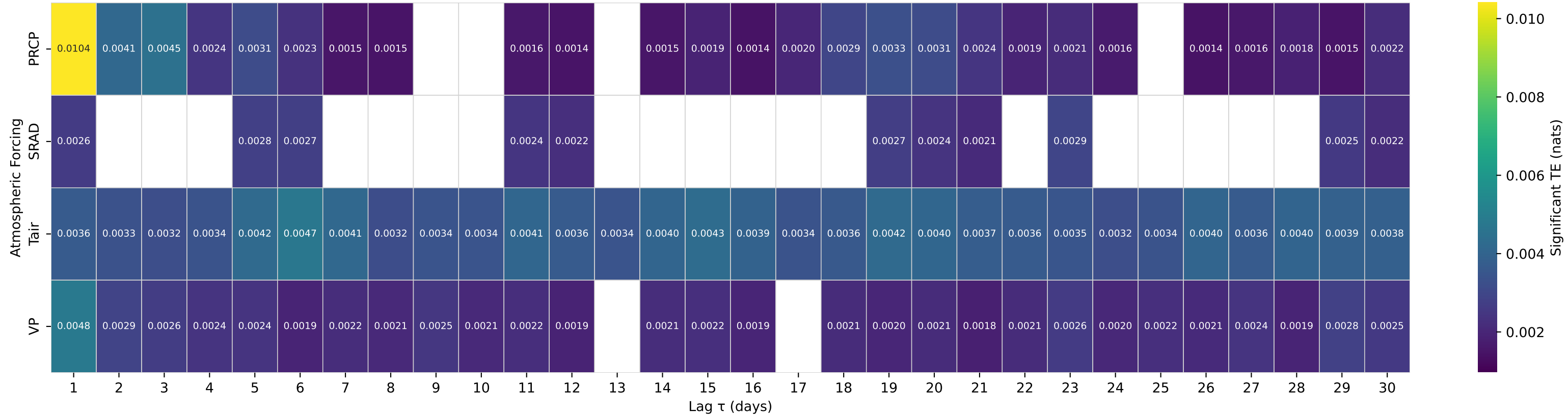
Shuffle-Test Significant TE to Streamflow — Basin 14020000 (HUC 17) — UMATILLA RIVER ABOVE MEACHAM CREEK, NR GIBBON, OR
