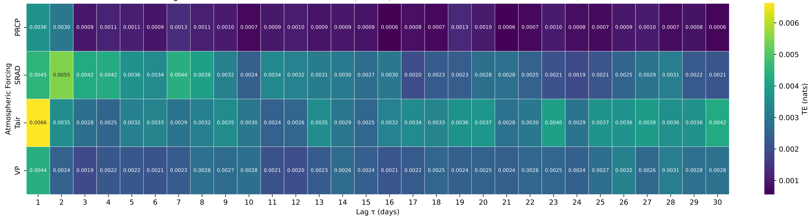
Shuffle-Test Significant TE to Streamflow — Basin 01052500 (HUC 01) — Diamond River near Wentworth Location, NH
