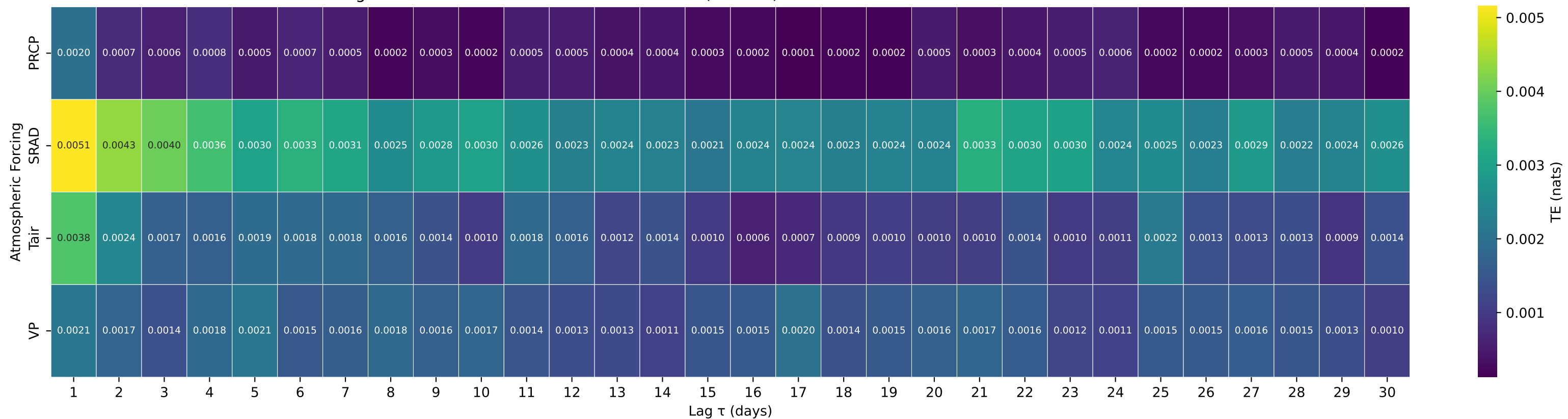
Shuffle-Test Significant TE to Streamflow — Basin 11230500 (HUC 18) — BEAR C NR LAKE THOMAS A EDISON CA
