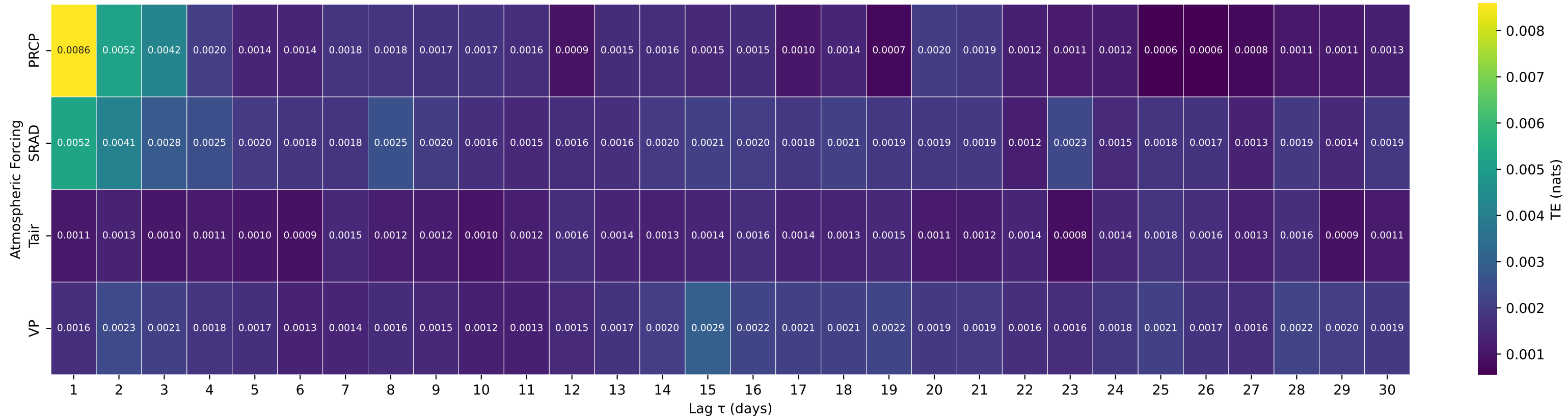
Shuffle-Test Significant TE to Streamflow — Basin 02235200 (HUC 03) — BLACKWATER CREEK NEAR CASSIA, FL
