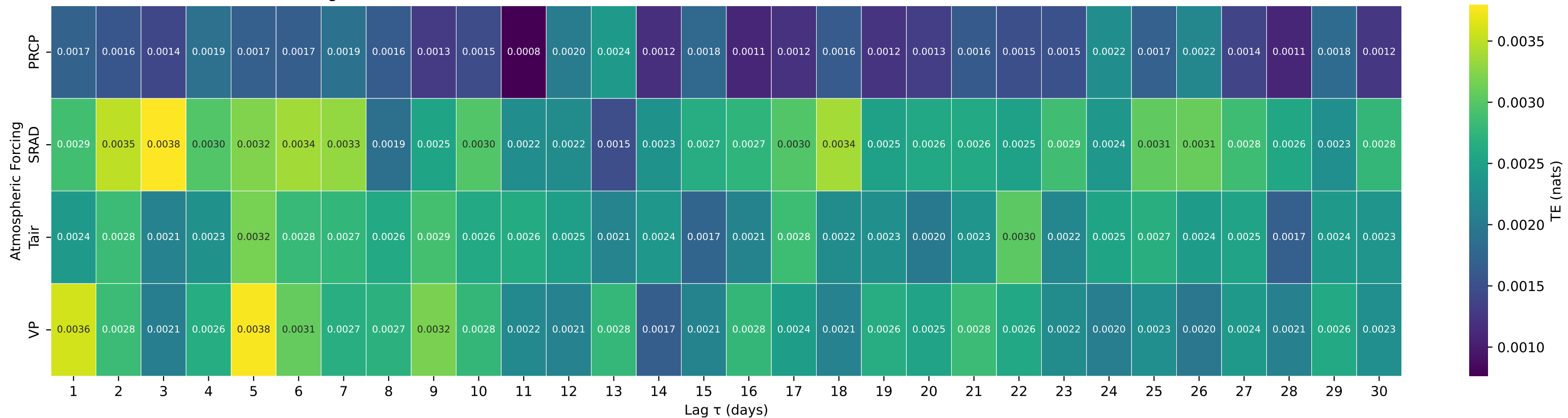
Shuffle-Test Significant TE to Streamflow — Basin 10166430 (HUC 16) — WEST CANYON CREEK NEAR CEDAR FORT, UT
