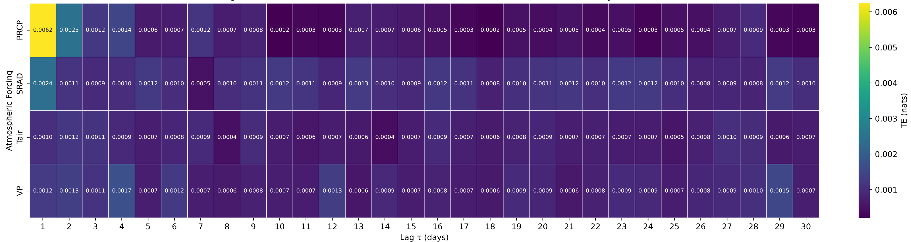
Shuffle-Test Significant TE to Streamflow — Basin 07315700 (HUC 11) — Mud Creek near Courtney, OK
