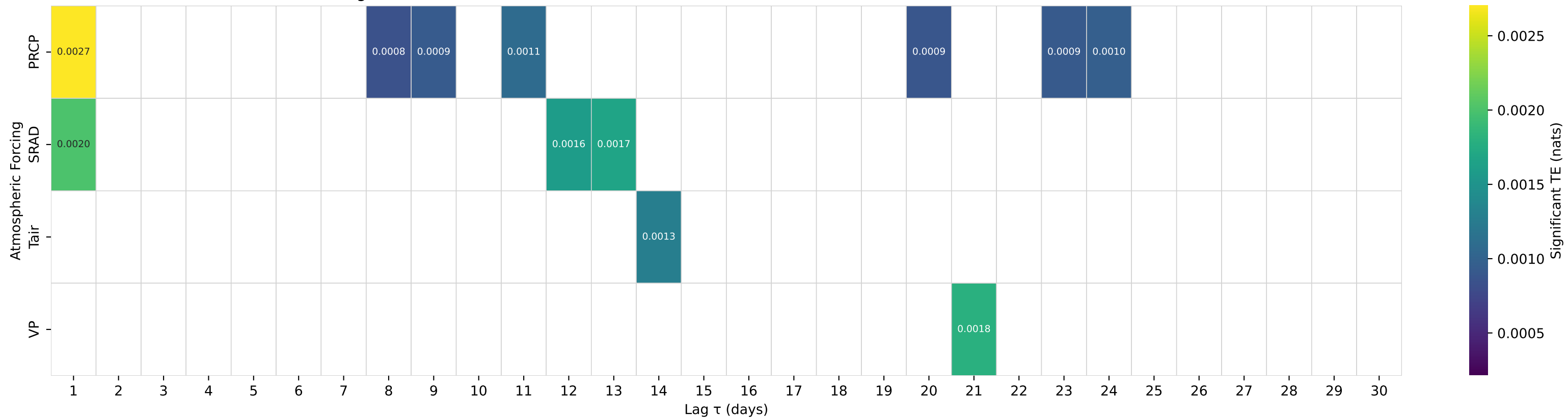
Shuffle-Test Significant TE to Streamflow — Basin 03456500 (HUC 06) — EAST FORK PIGEON RIVER NEAR CANTON, NC
