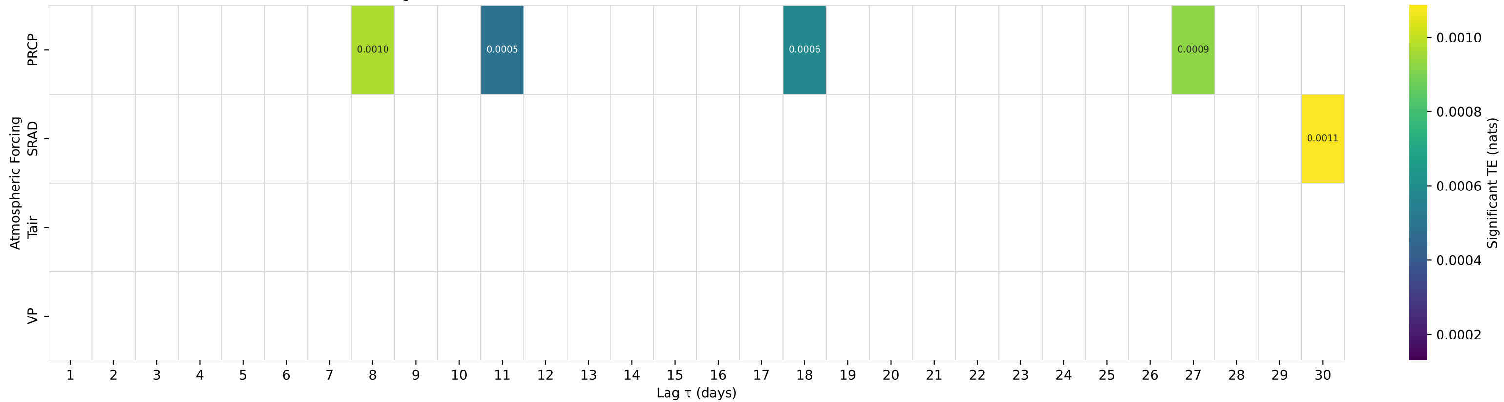
Shuffle-Test Significant TE to Streamflow — Basin 03049800 (HUC 05) — Little Pine Creek near Etna, PA
