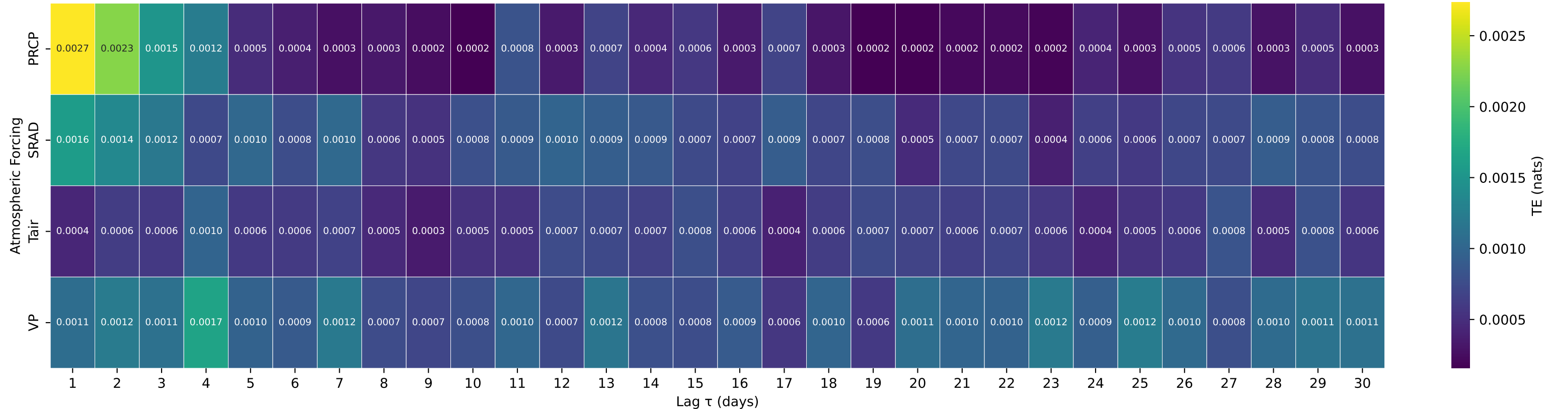
Shuffle-Test Significant TE to Streamflow — Basin 02092500 (HUC 03) — TRENT RIVER NEAR TRENTON, NC
