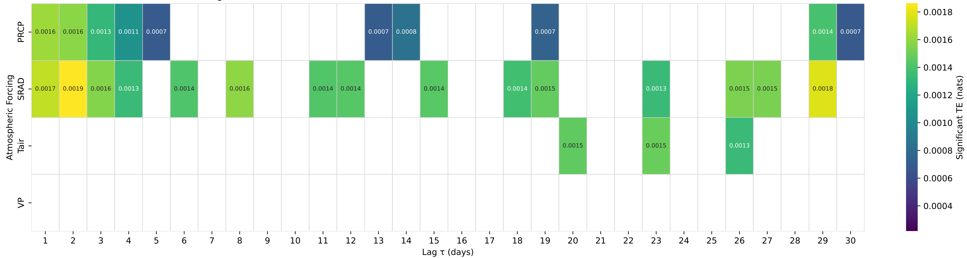
Shuffle-Test Significant TE to Streamflow — Basin 09404450 (HUC 15) — EAST FORK VIRGIN RIVER NEAR GLENDALE, UT
