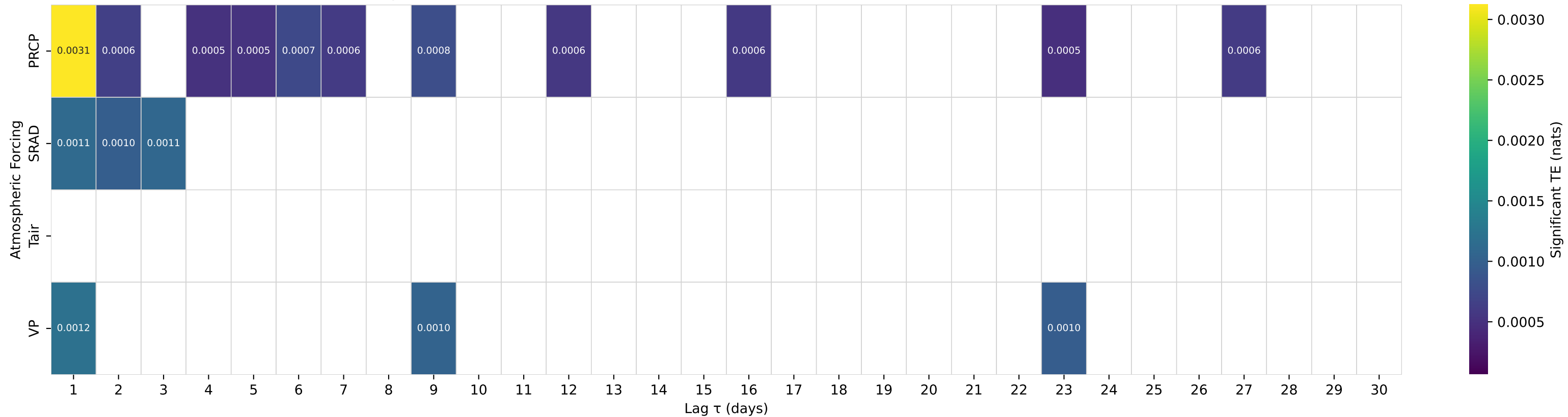
Shuffle-Test Significant TE to Streamflow — Basin 07315200 (HUC 11) — E Fk Little Wichita Rv nr Henrietta, TX
