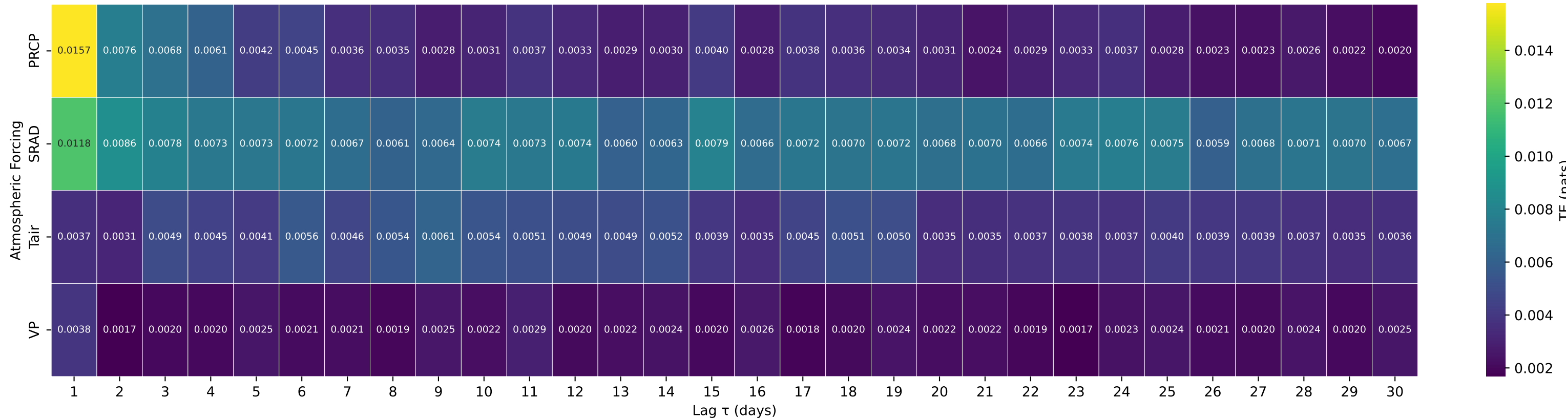
Shuffle-Test Significant TE to Streamflow — Basin 11482500 (HUC 18) — REDWOOD C A ORICK CA
