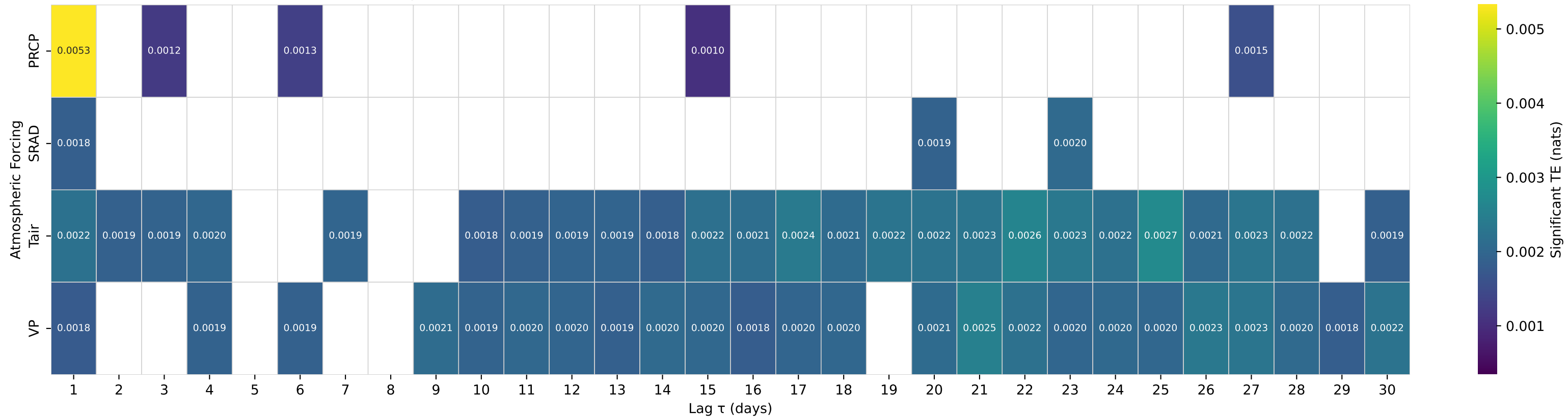
Shuffle-Test Significant TE to Streamflow — Basin 01123000 (HUC 01) — LITTLE RIVER NEAR HANOVER, CT.
