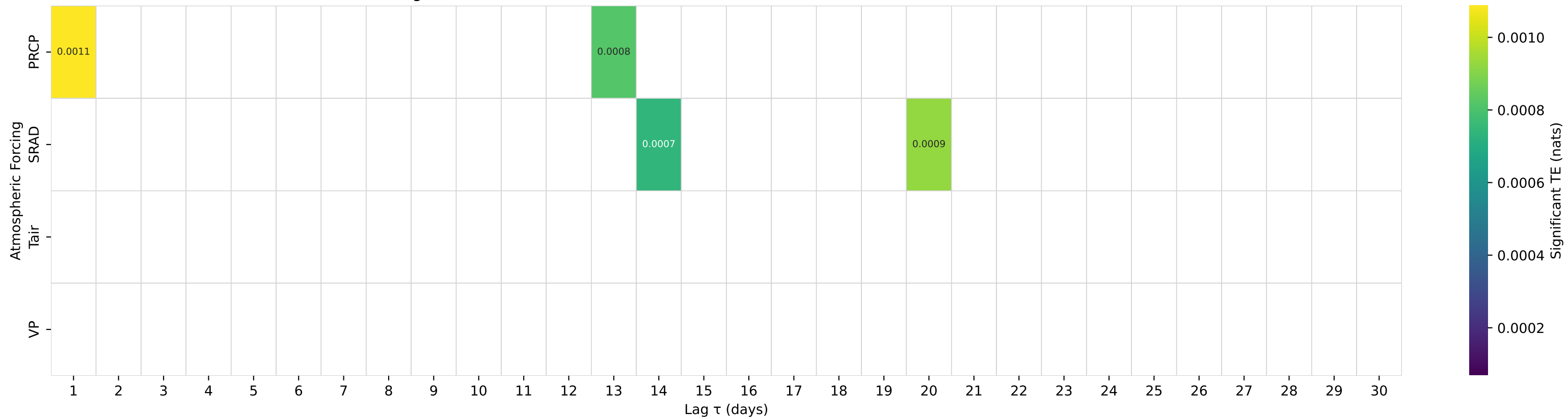
Shuffle-Test Significant TE to Streamflow — Basin 06903400 (HUC 10) — Chariton River near Chariton, IA
