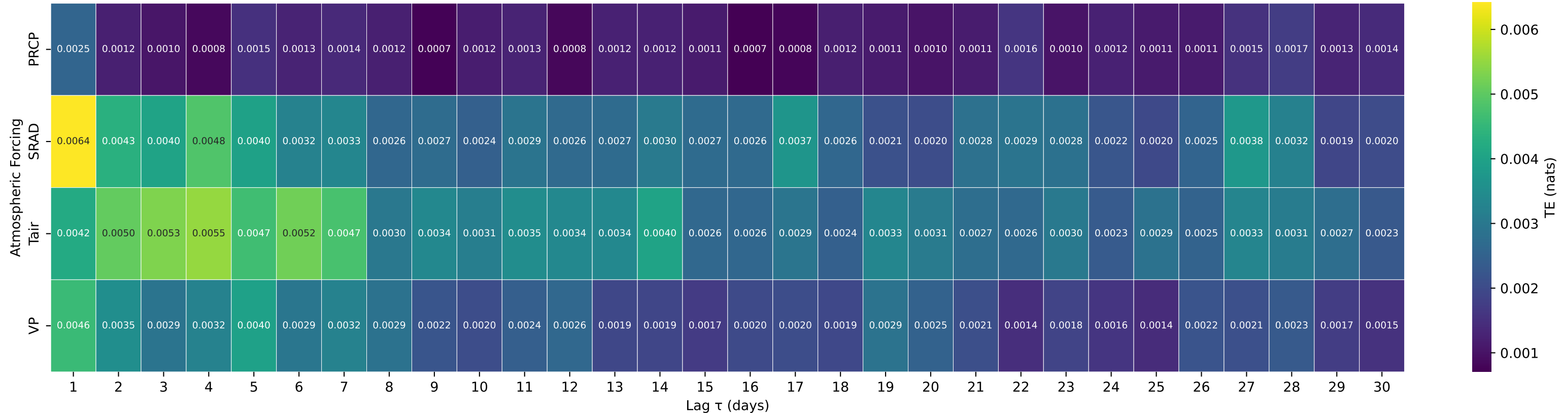
Shuffle-Test Significant TE to Streamflow — Basin 06623800 (HUC 10) — ENCAMPMENT RIVER AB HOG PARK CR, NR ENCAMPMENT, WY
