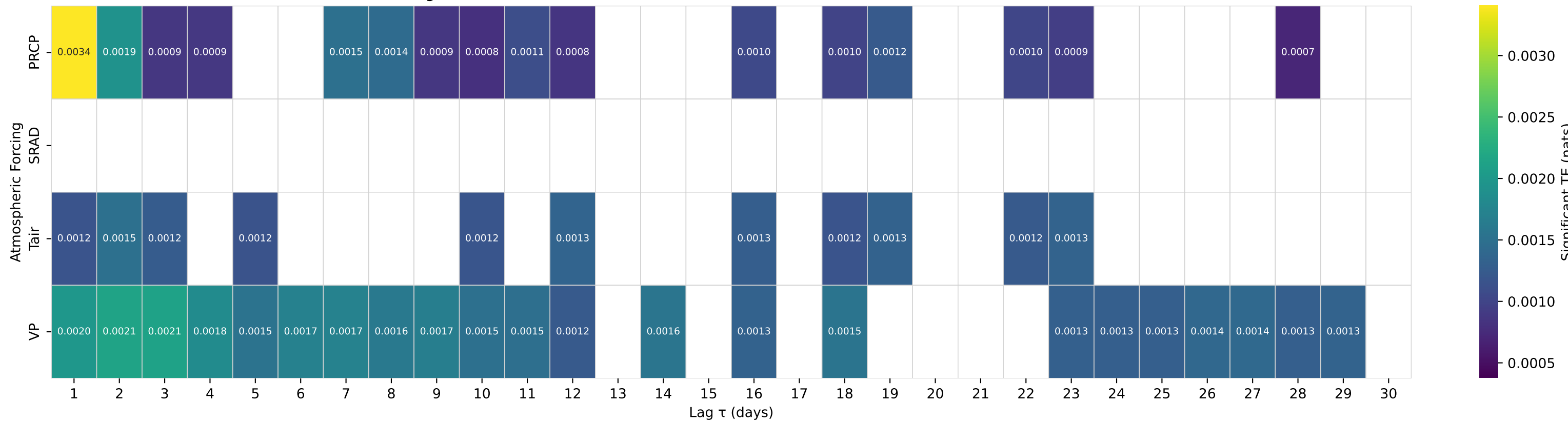
Shuffle-Test Significant TE to Streamflow — Basin 07226500 (HUC 11) — UTE CREEK NEAR LOGAN, NM
