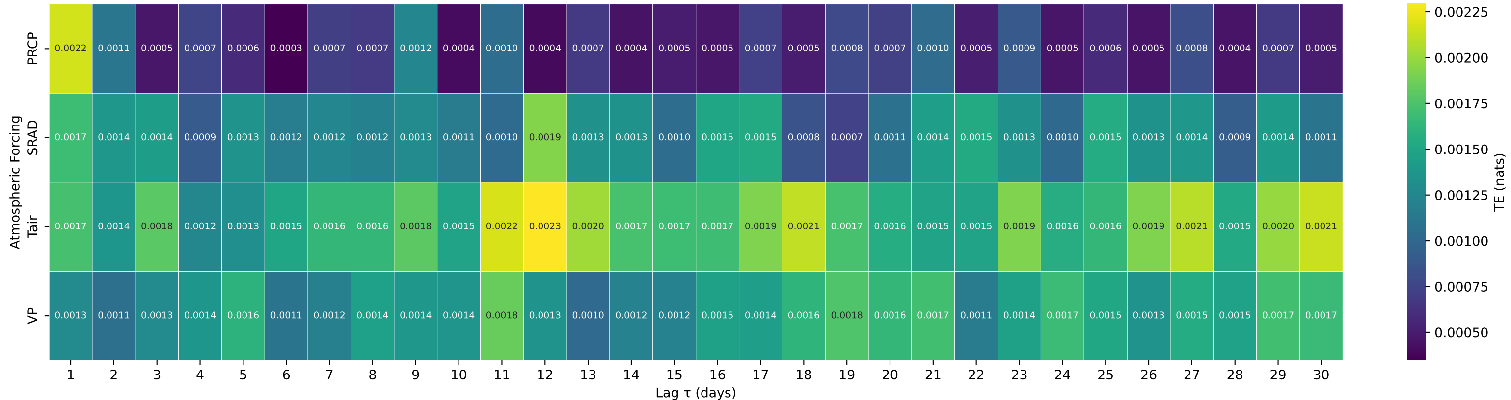
Shuffle-Test Significant TE to Streamflow — Basin 01550000 (HUC 02) — Lycoming Creek near Trout Run, PA
