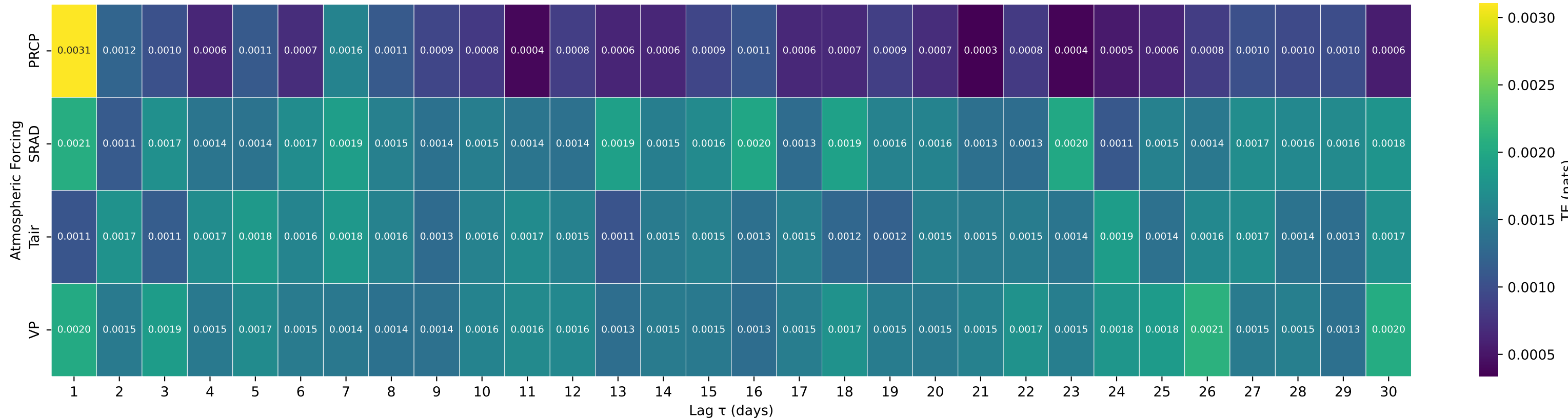
Shuffle-Test Significant TE to Streamflow — Basin 03285000 (HUC 05) — DIX RIVER NEAR DANVILLE, KY
