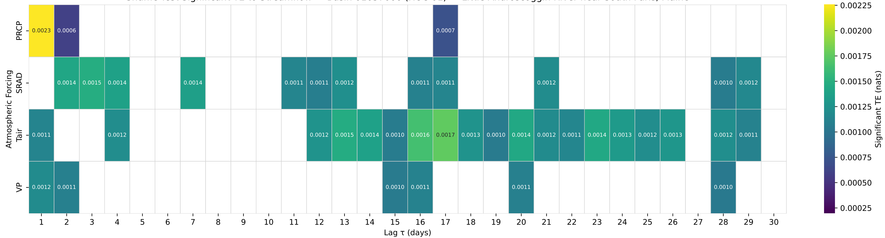
Shuffle-Test Significant TE to Streamflow — Basin 01057000 (HUC 01) — Little Androscoggin River near South Paris, Maine
