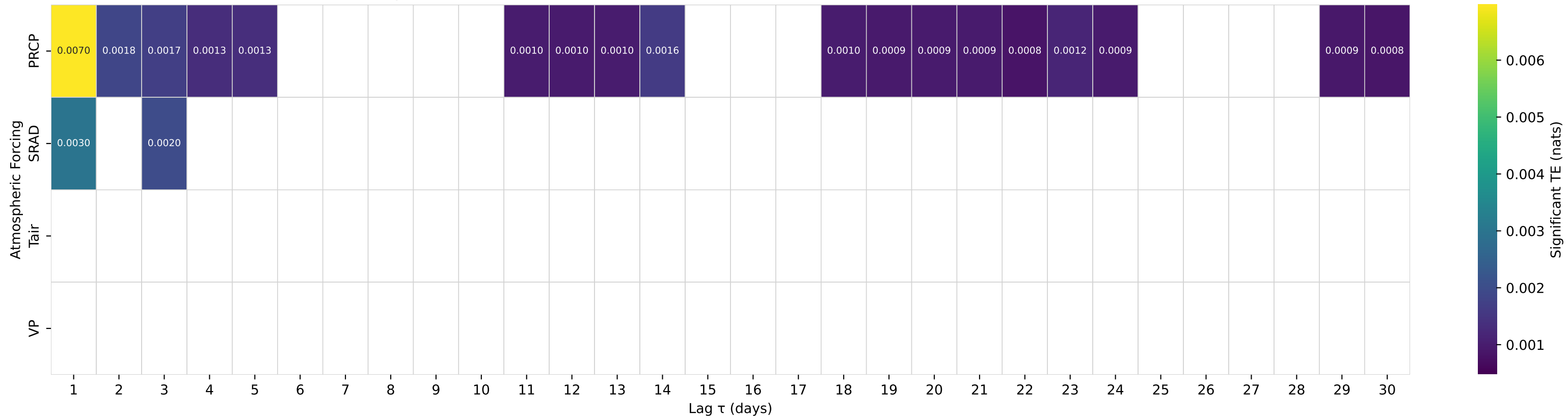
Shuffle-Test Significant TE to Streamflow — Basin 02300700 (HUC 03) — BULLFROG CREEK NEAR WIMAUMA FL
