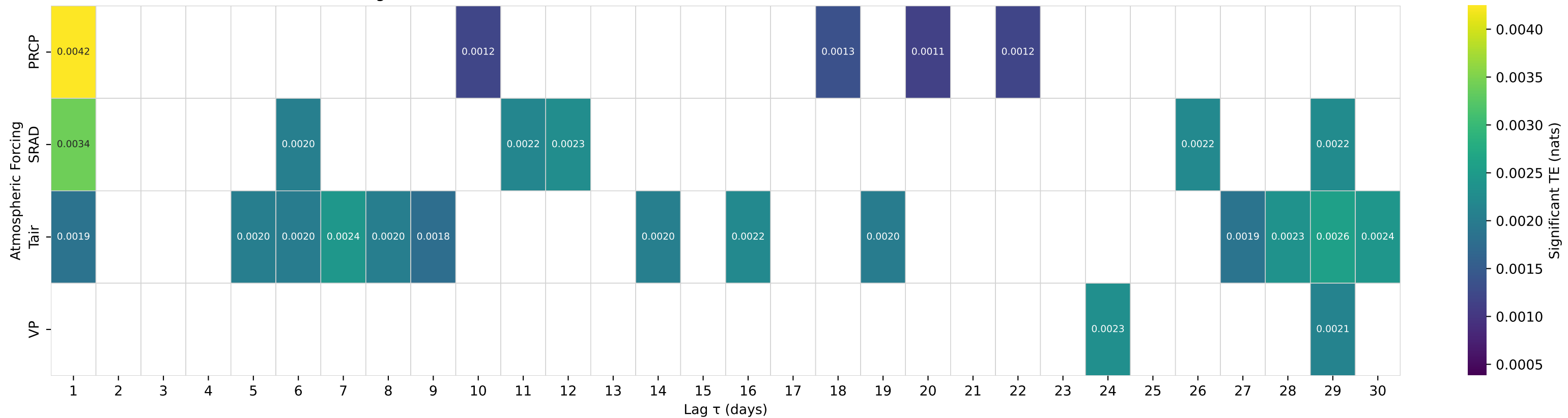
Shuffle-Test Significant TE to Streamflow — Basin 05592050 (HUC 07) — ROBINSON CREEK NEAR SHELBYVILLE, IL
