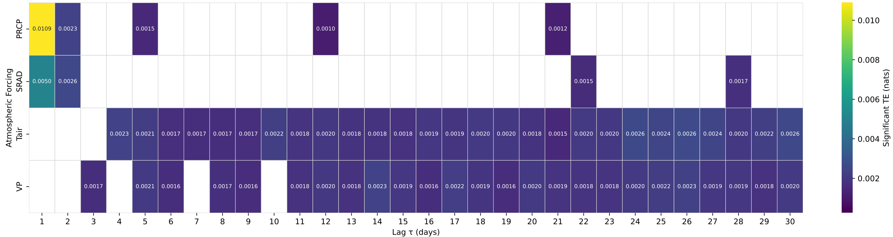
Shuffle-Test Significant TE to Streamflow — Basin 02215100 (HUC 03) — TUCSAWHATCHEE CREEK NEAR HAWKINSVILLE, GA
