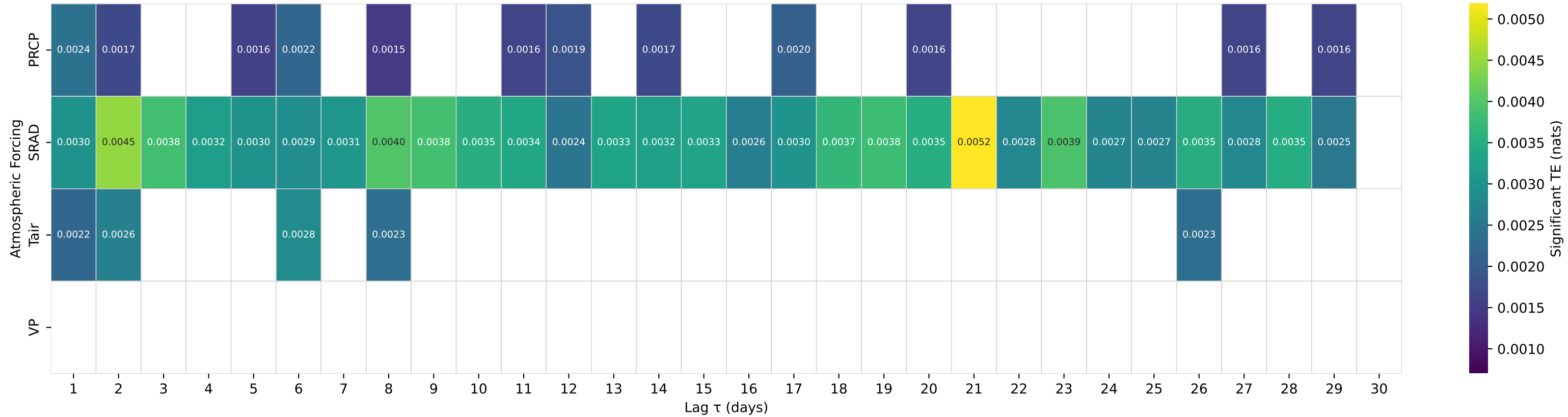
Shuffle-Test Significant TE to Streamflow — Basin 06409000 (HUC 10) — CASTLE CR ABOVE DEERFIELD RES NEAR HILL CITY SD
