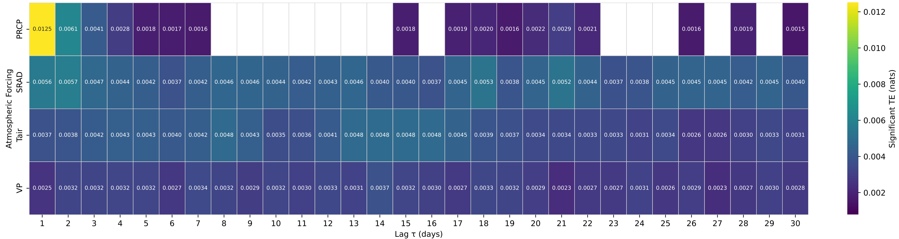
Shuffle-Test Significant TE to Streamflow — Basin 12115500 (HUC 17) — REX RIVER NEAR CEDAR FALLS, WA
