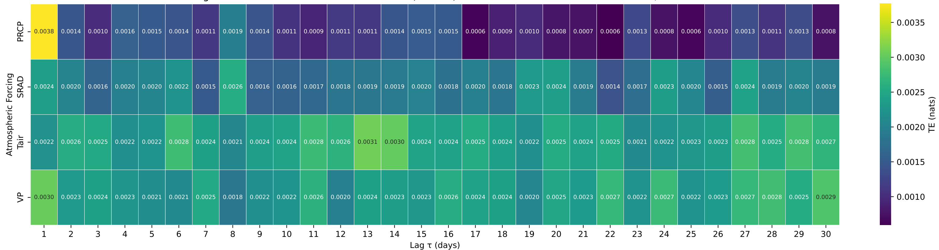
Shuffle-Test Significant TE to Streamflow — Basin 03291780 (HUC 05) — INDIAN-KENTUCK CREEK NR CANAAN, IND.
