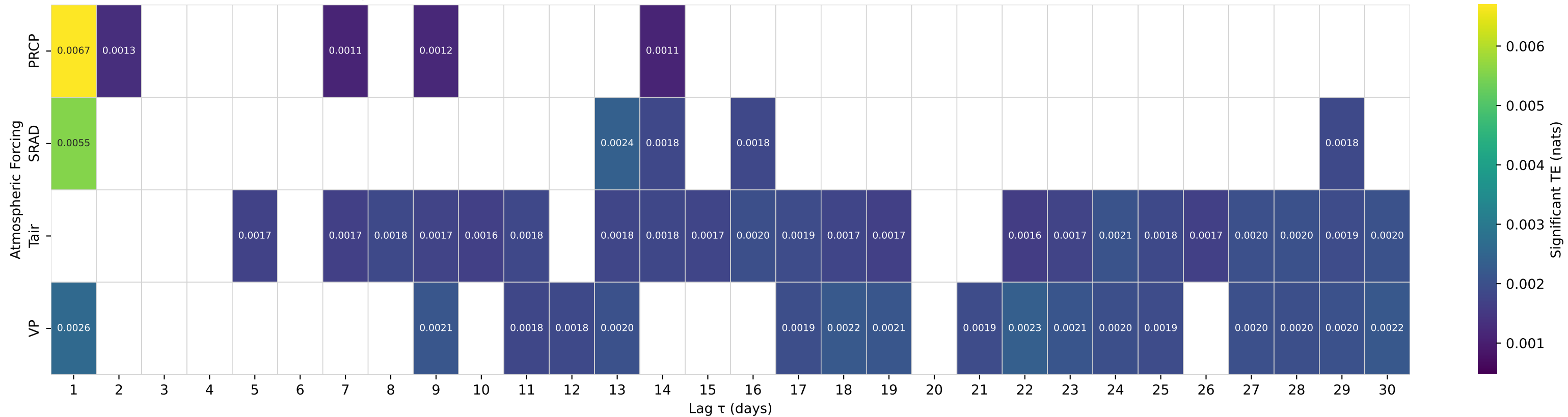
Shuffle-Test Significant TE to Streamflow — Basin 03500000 (HUC 06) — LITTLE TENNESSEE RIVER NEAR PRENTISS, NC
