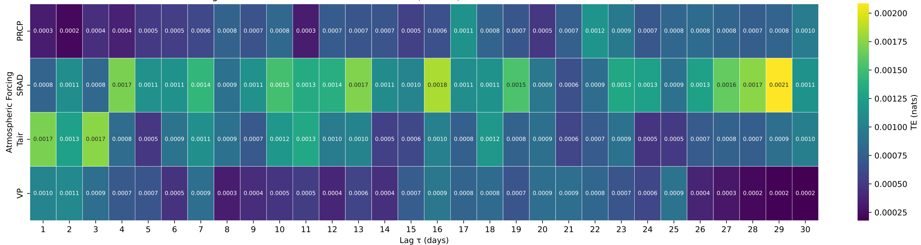
Shuffle-Test Significant TE to Streamflow — Basin 10249300 (HUC 16) — S TWIN R NR ROUND MOUNTAIN, NV
