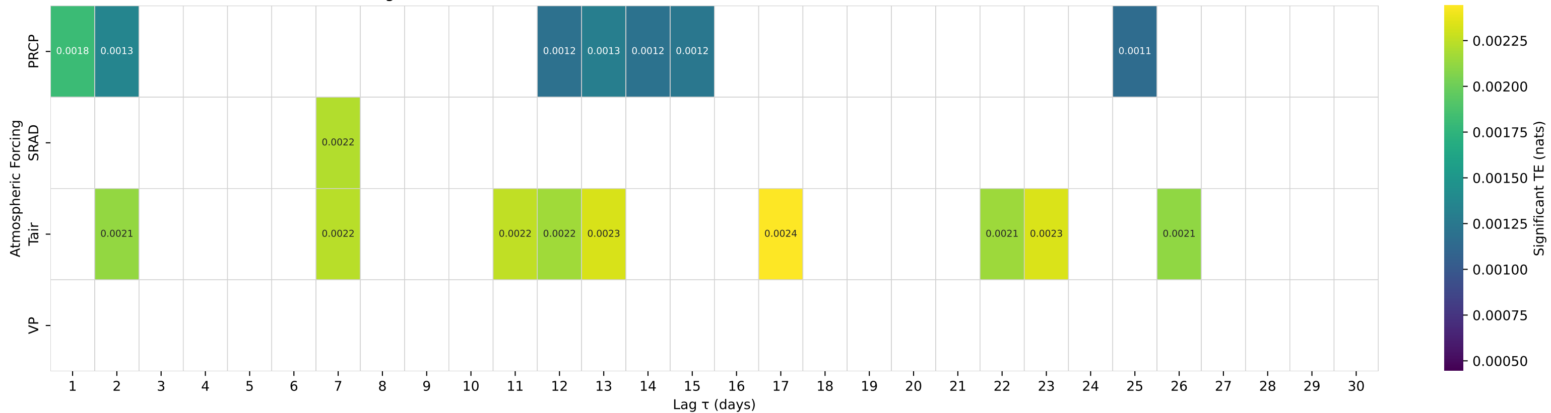
Shuffle-Test Significant TE to Streamflow — Basin 06350000 (HUC 10) — CANNONBALL RIVER AT REGENT, ND
