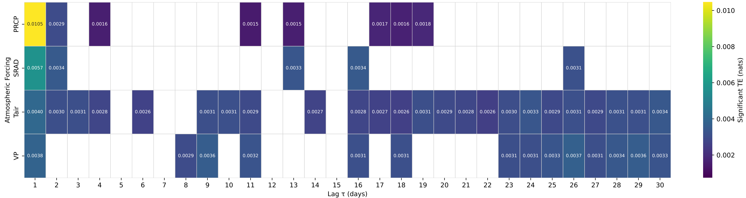
Shuffle-Test Significant TE to Streamflow — Basin 02481000 (HUC 03) — BILOXI RIVER AT WORTHAM, MS
