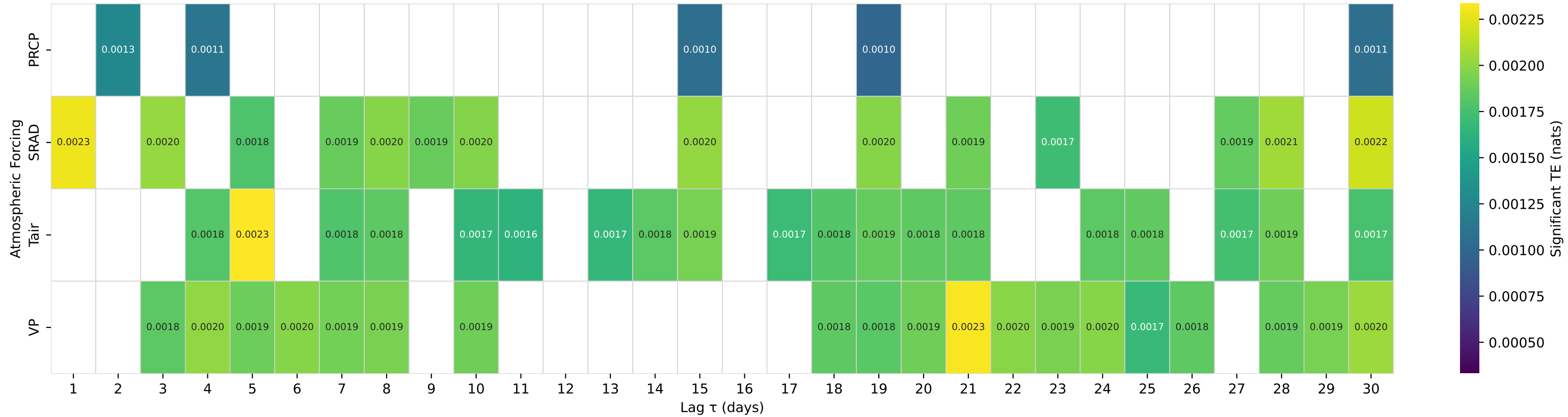
Shuffle-Test Significant TE to Streamflow — Basin 02051000 (HUC 03) — NORTH MEHERRIN RIVER NEAR LUNENBURG, VA
