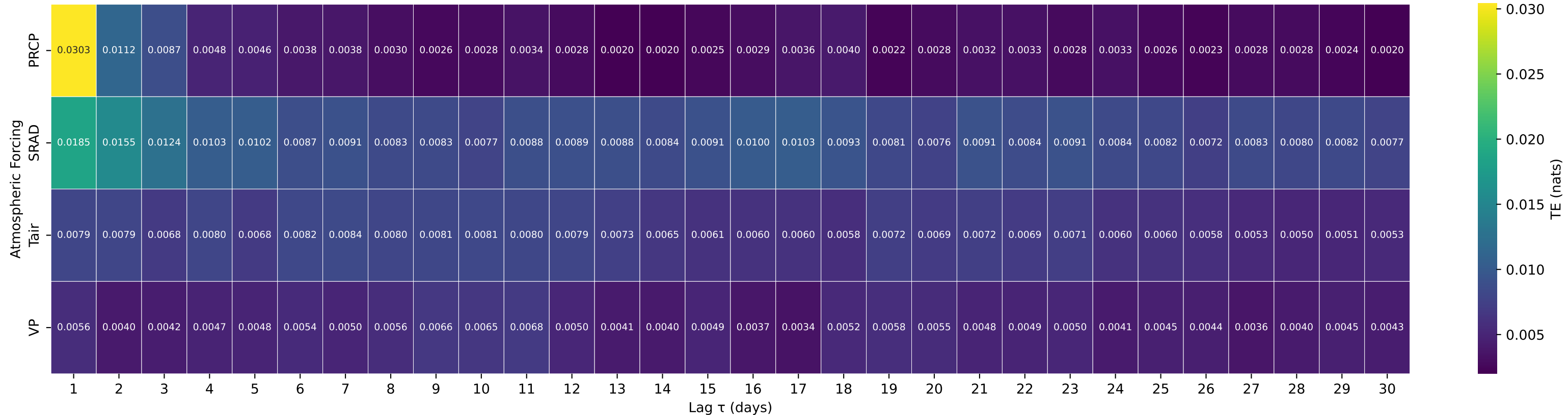
Shuffle-Test Significant TE to Streamflow — Basin 12013500 (HUC 17) — WILLAPA RIVER NEAR WILLAPA, WA
