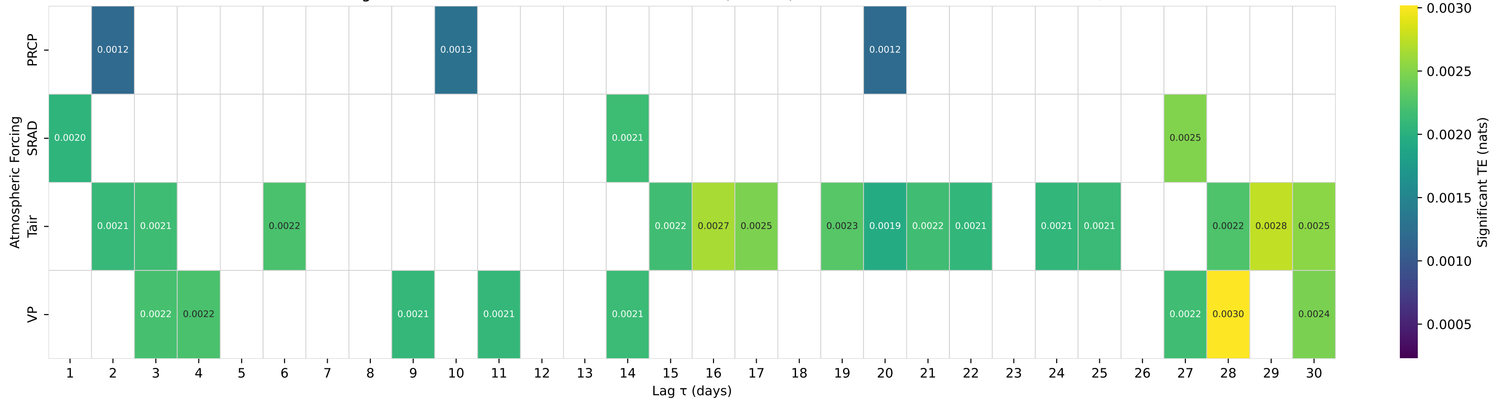
Shuffle-Test Significant TE to Streamflow — Basin 02096846 (HUC 03) — CANE CREEK NEAR ORANGE GROVE, NC
