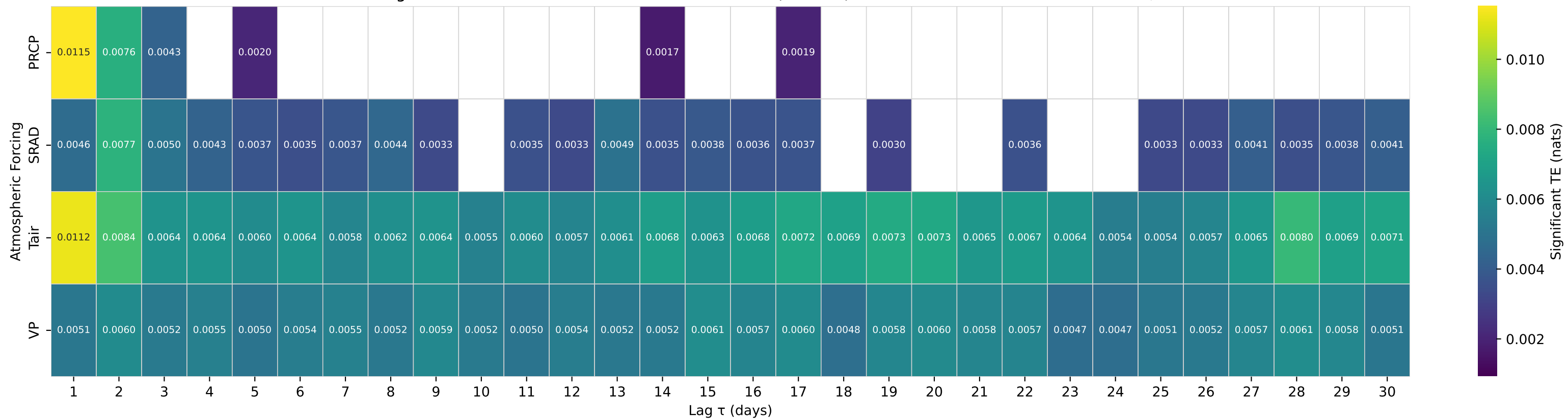
Shuffle-Test Significant TE to Streamflow — Basin 04127997 (HUC 04) — STURGEON RIVER AT WOLVERINE, MI
