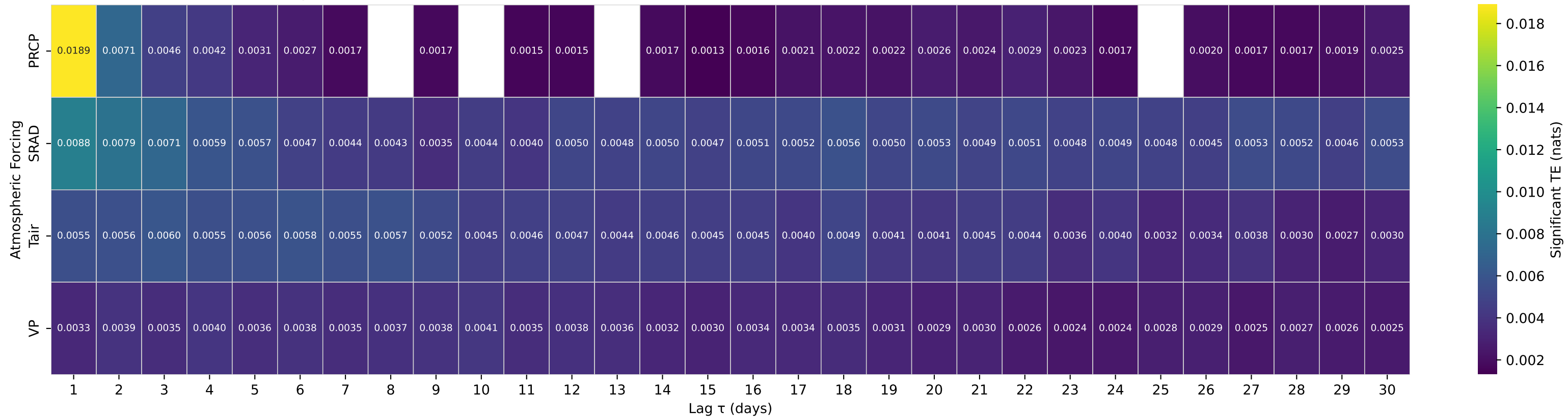
Shuffle-Test Significant TE to Streamflow — Basin 14138900 (HUC 17) — NORTH FORK BULL RUN RIVER NEAR MULTNOMAH FALLS, OR
