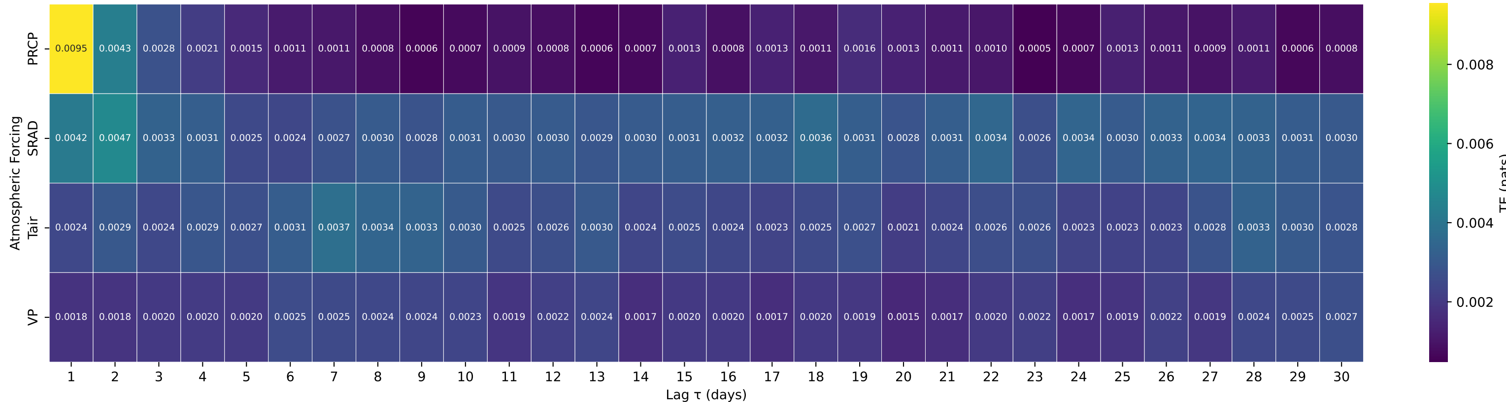
Shuffle-Test Significant TE to Streamflow — Basin 12117000 (HUC 17) — TAYLOR CREEK NEAR SELLECK, WA
