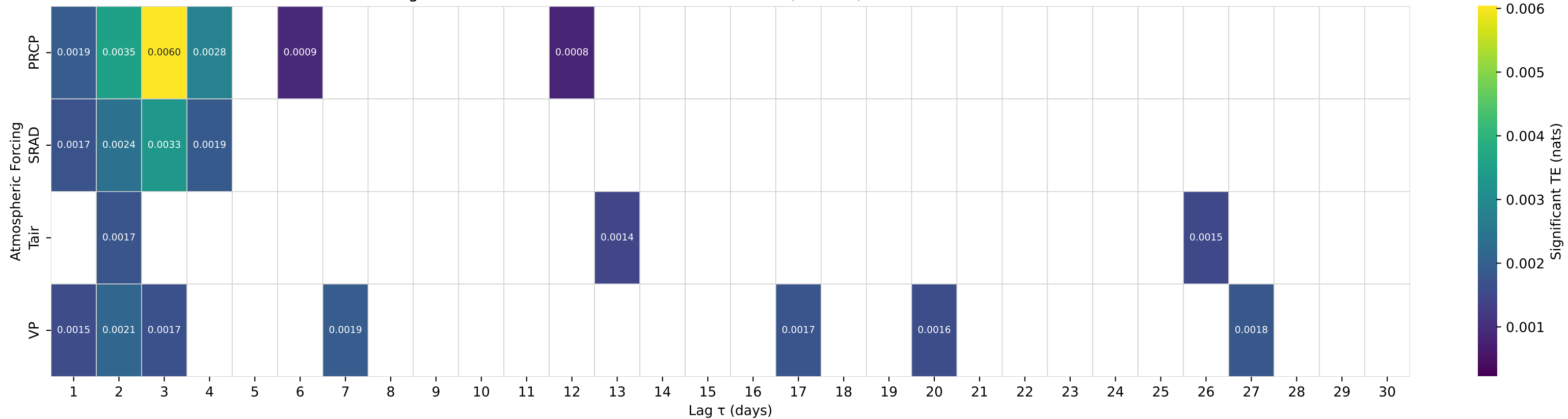
Shuffle-Test Significant TE to Streamflow — Basin 02371500 (HUC 03) — CONECUH RIVER AT BRANTLEY AL
