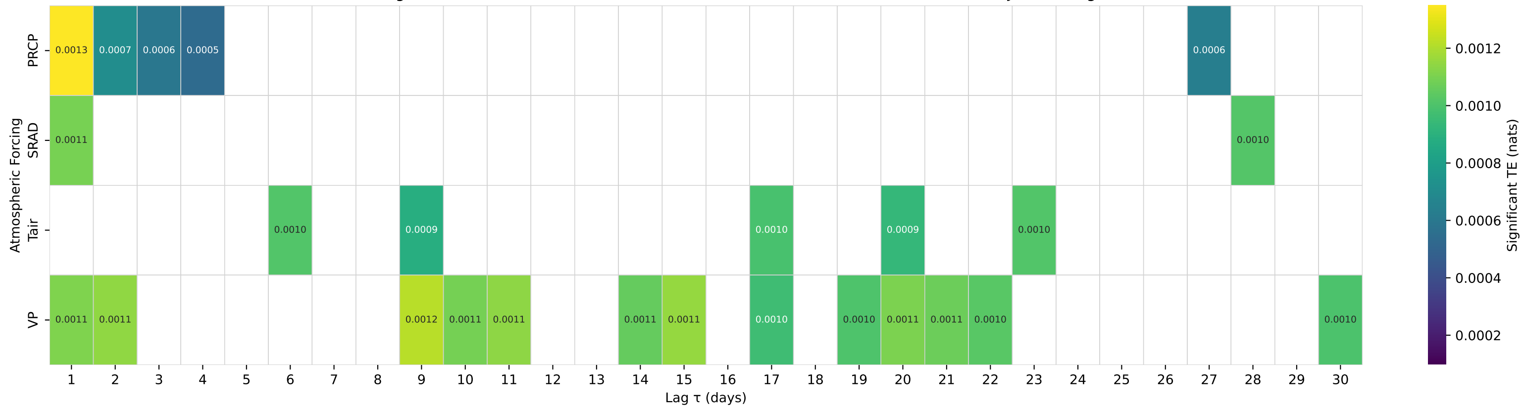
Shuffle-Test Significant TE to Streamflow — Basin 08079600 (HUC 12) — DMF Brazos Rv at Justiceburg, TX
