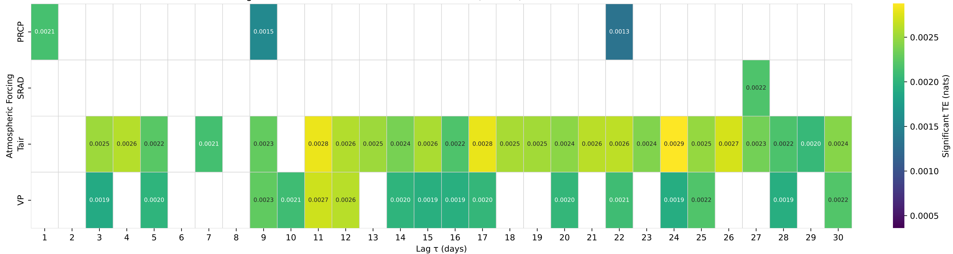
Shuffle-Test Significant TE to Streamflow — Basin 01414500 (HUC 02) — MILL BROOK NEAR DUNRAVEN NY
