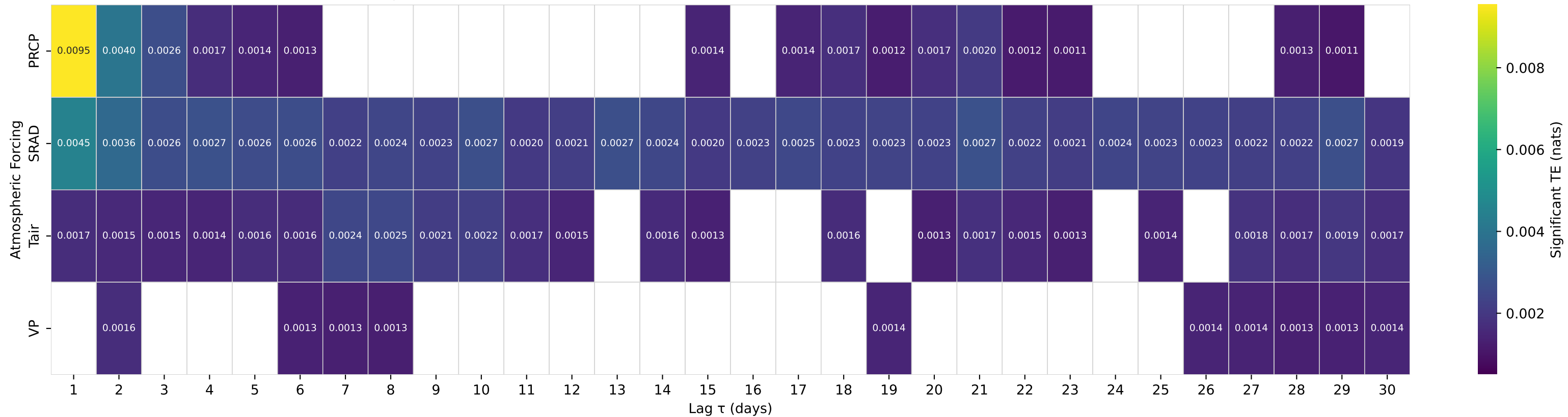
Shuffle-Test Significant TE to Streamflow — Basin 12092000 (HUC 17) — PUYALLUP RIVER NEAR ELECTRON, WA
