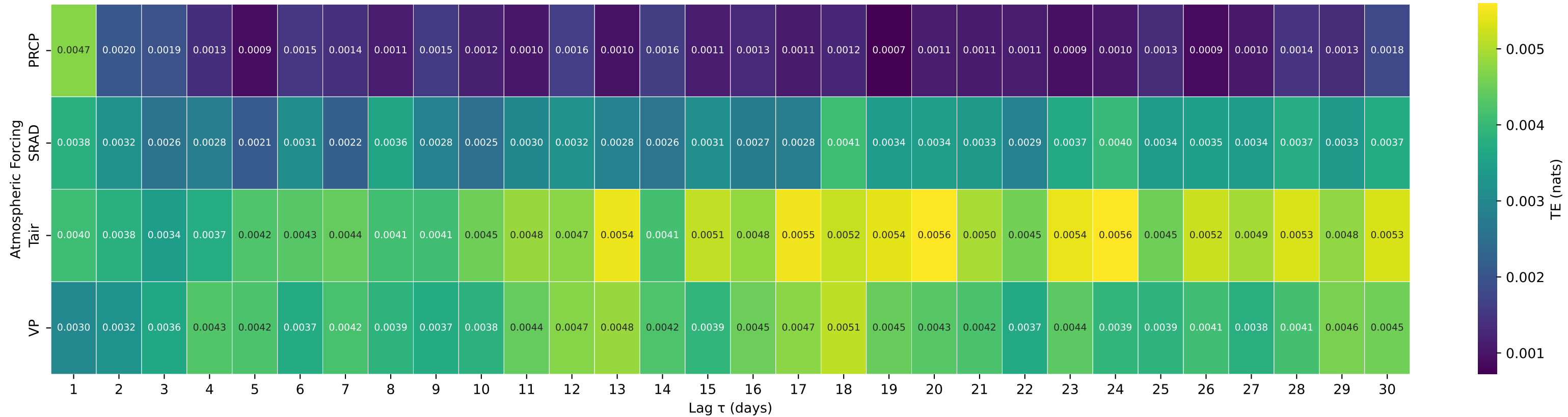
Shuffle-Test Significant TE to Streamflow — Basin 04197170 (HUC 04) — Rock Creek at Tiffin OH
