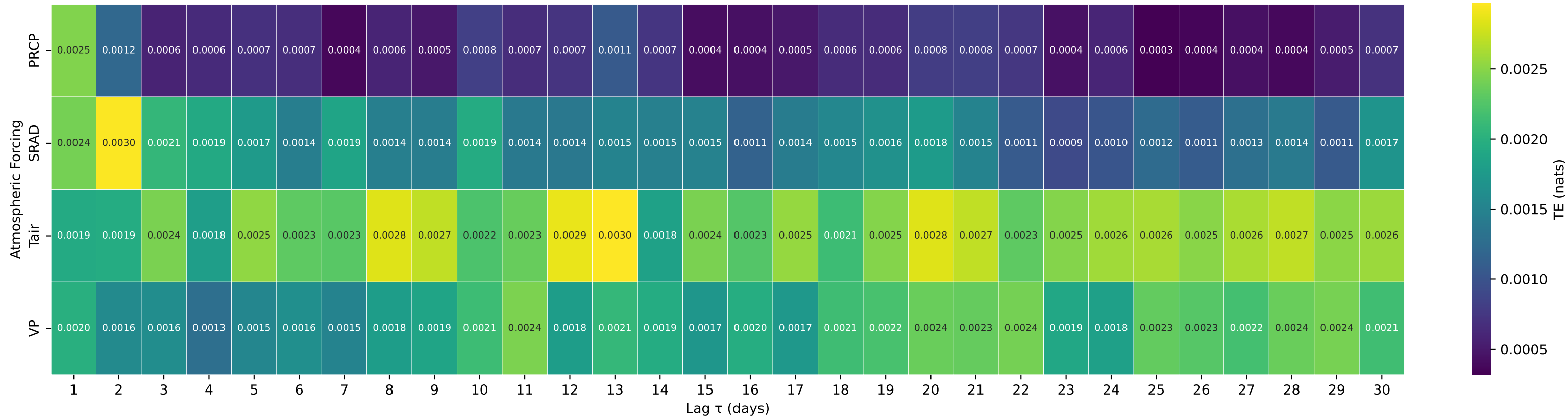
Shuffle-Test Significant TE to Streamflow — Basin 01142500 (HUC 01) — AYERS BROOK AT RANDOLPH, VT
