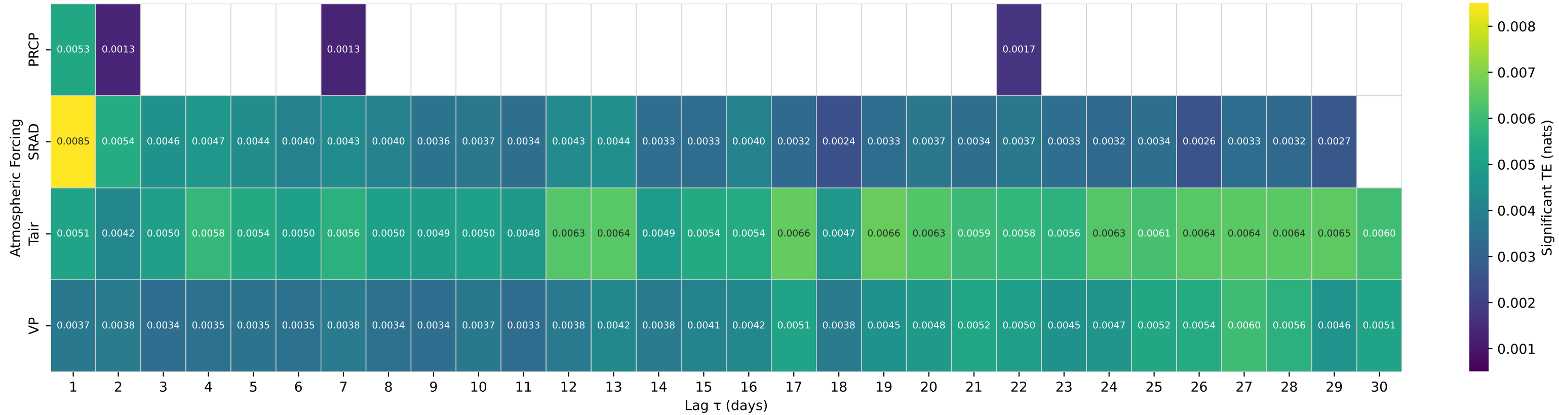
Shuffle-Test Significant TE to Streamflow — Basin 01139800 (HUC 01) — EAST ORANGE BRANCH AT EAST ORANGE, VT
