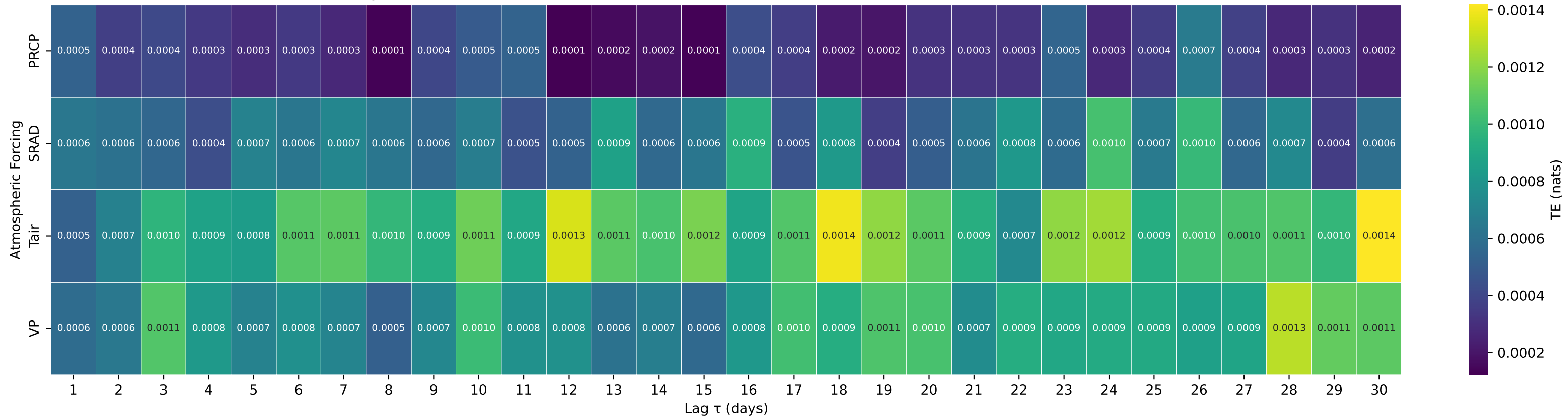
Shuffle-Test Significant TE to Streamflow — Basin 01532000 (HUC 02) — Towanda Creek near Monroeton, PA
