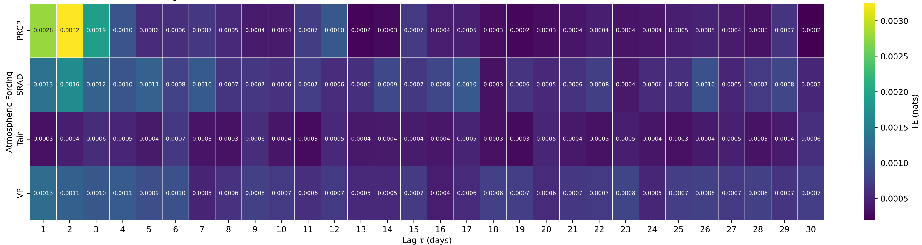
Shuffle-Test Significant TE to Streamflow — Basin 02108000 (HUC 03) — NORTHEAST CAPE FEAR RIVER NEAR CHINQUAPIN, NC
