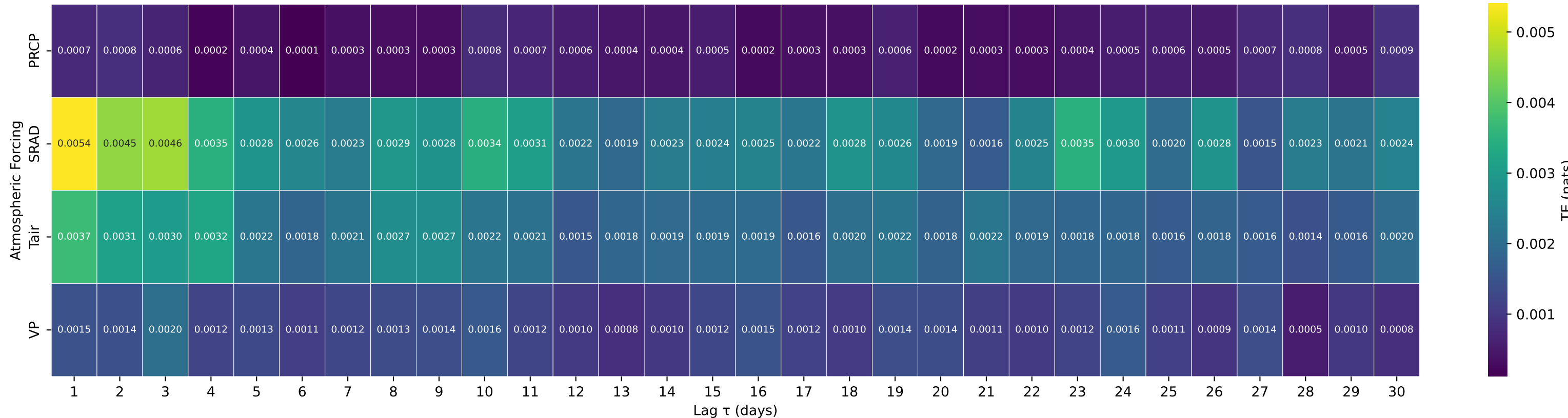
Shuffle-Test Significant TE to Streamflow — Basin 10173450 (HUC 16) — MAMMOTH CREEK ABV WEST HATCH DITCH, NEAR HATCH, UT
