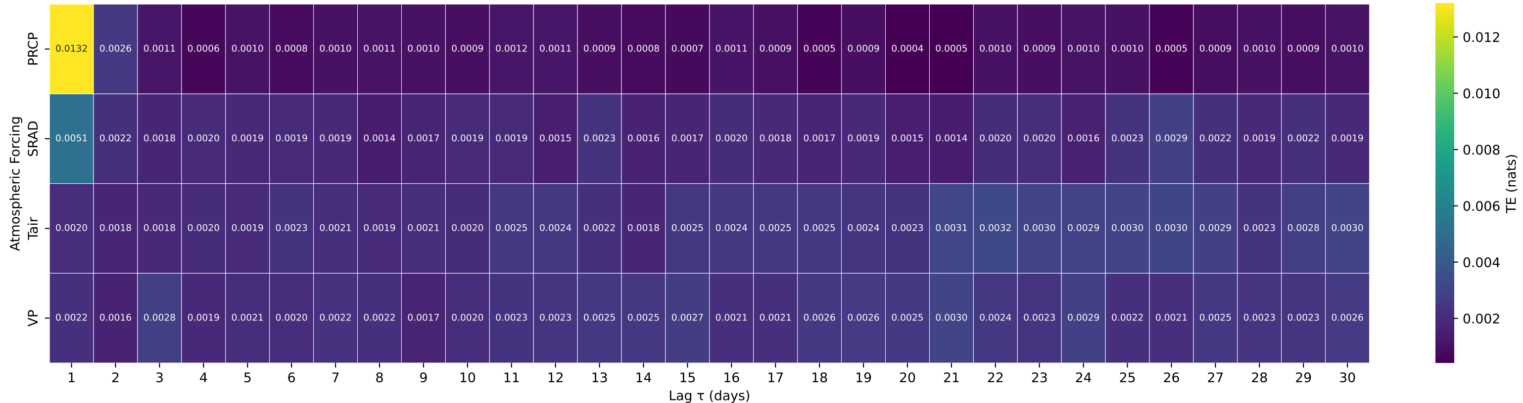
Shuffle-Test Significant TE to Streamflow — Basin 02469800 (HUC 03) — SATILPA CREEK NEAR COFFEEVILLE AL
