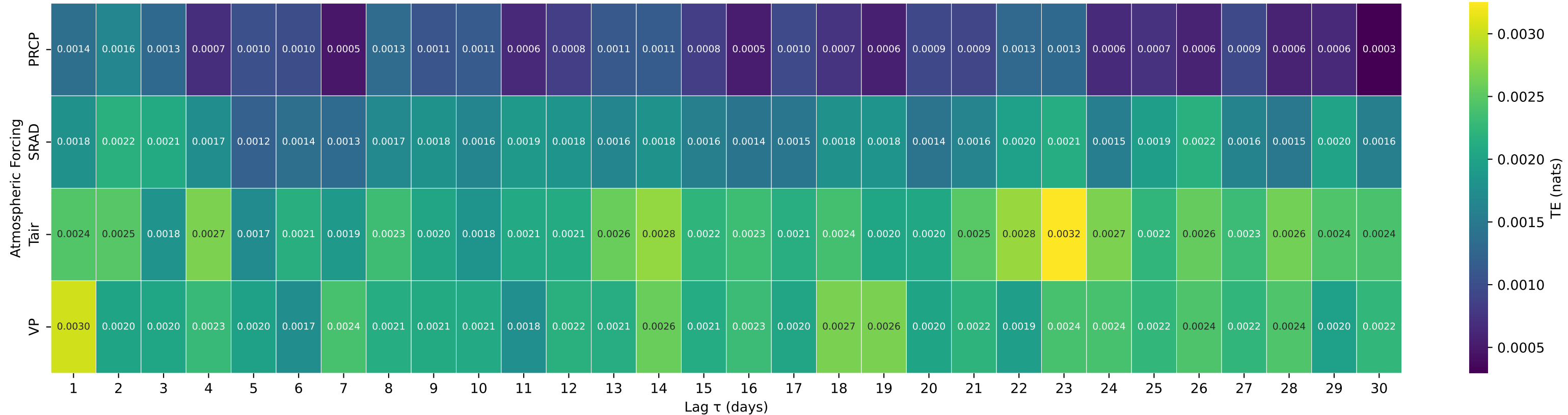
Shuffle-Test Significant TE to Streamflow — Basin 03026500 (HUC 05) — Sevenmile Run near Rasselas, PA
