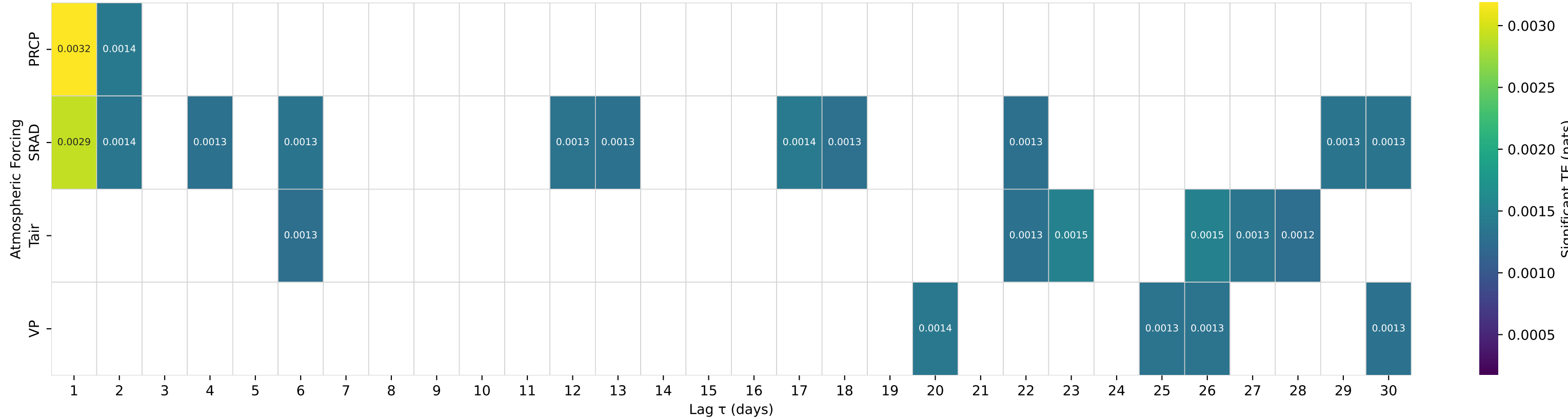
Shuffle-Test Significant TE to Streamflow — Basin 07373000 (HUC 08) — Big Creek at Pollock, LA
