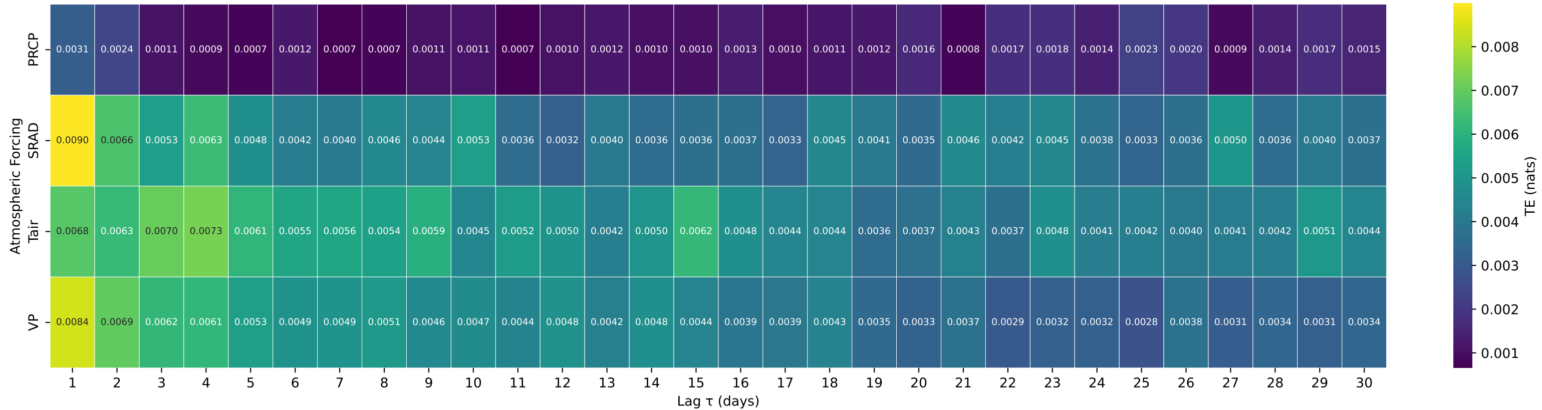
Shuffle-Test Significant TE to Streamflow — Basin 09066200 (HUC 14) — BOOTH CREEK NEAR MINTURN, CO.
