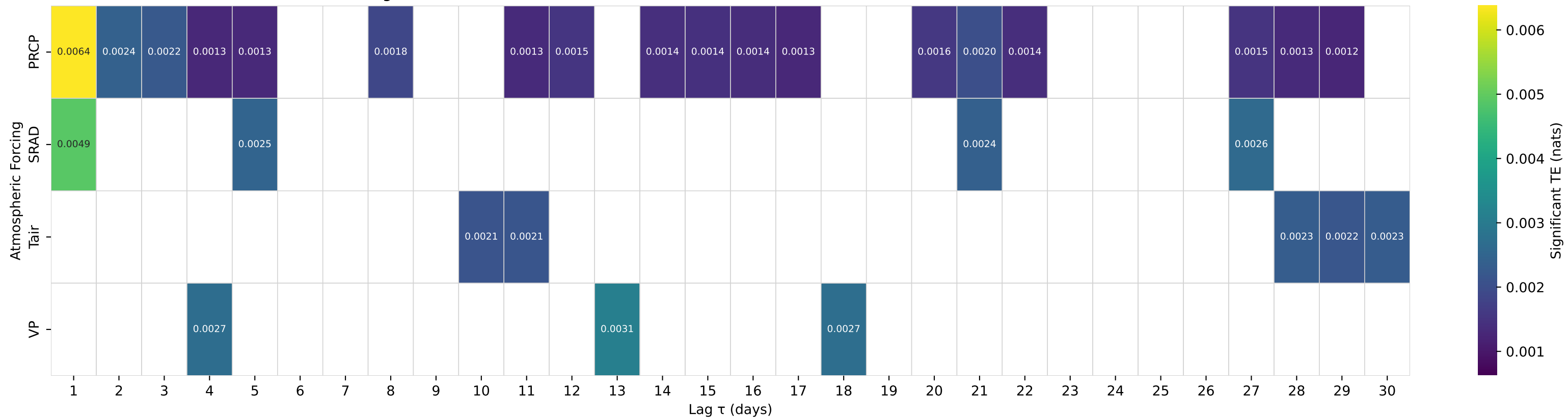
Shuffle-Test Significant TE to Streamflow — Basin 02324400 (HUC 03) — FENHOLLOWAY RIVER NEAR FOLEY, FLA.
