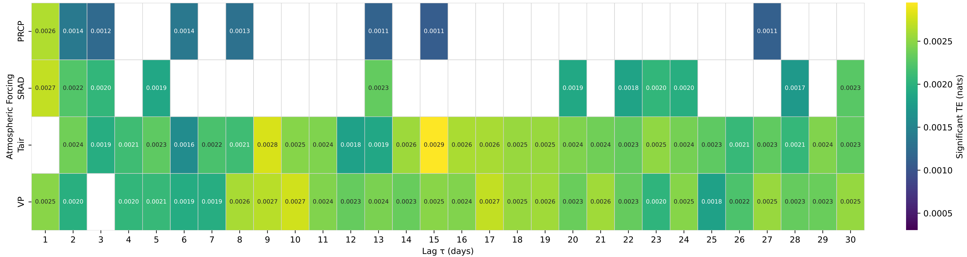
Shuffle-Test Significant TE to Streamflow — Basin 03500240 (HUC 06) — CARTOOGECHAYE CREEK NEAR FRANKLIN, NC
