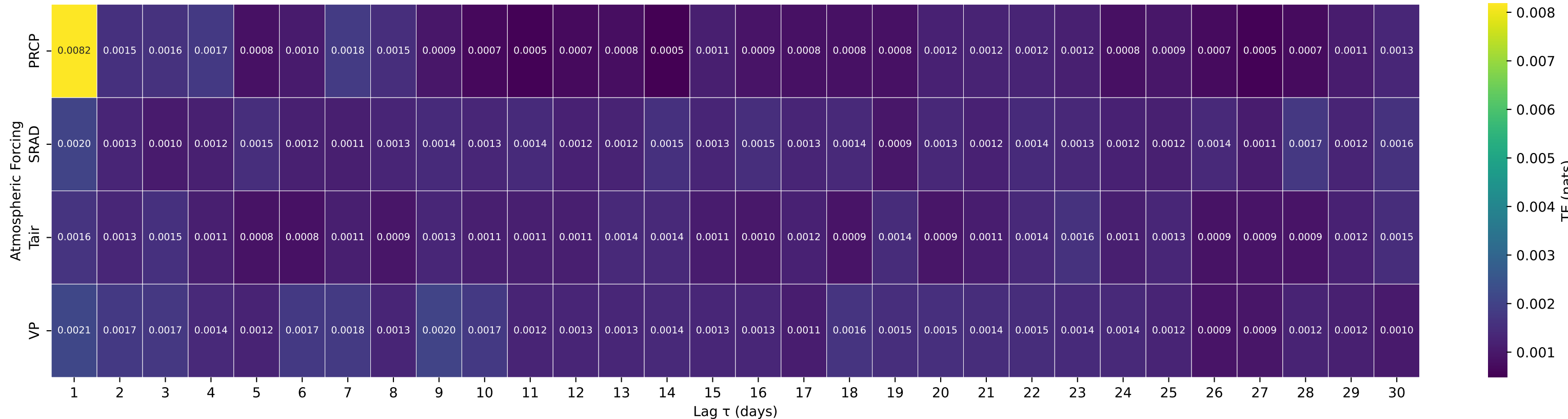
Shuffle-Test Significant TE to Streamflow — Basin 07145700 (HUC 11) — SLATE C AT WELLINGTON, KS
