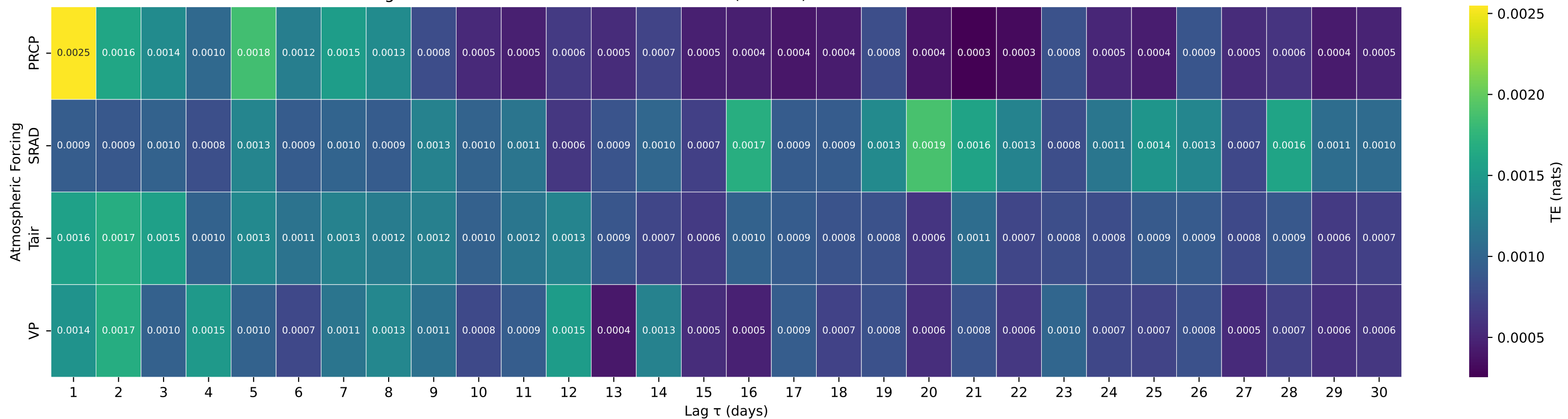
Shuffle-Test Significant TE to Streamflow — Basin 06404000 (HUC 10) — BATTLE CR NEAR KEYSTONE SD
