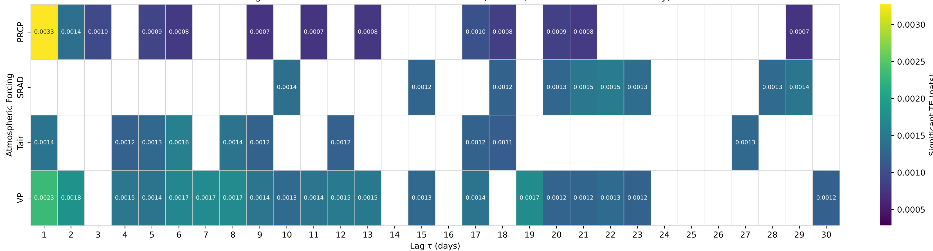
Shuffle-Test Significant TE to Streamflow — Basin 05489000 (HUC 07) — Cedar Creek near Bussey, IA
