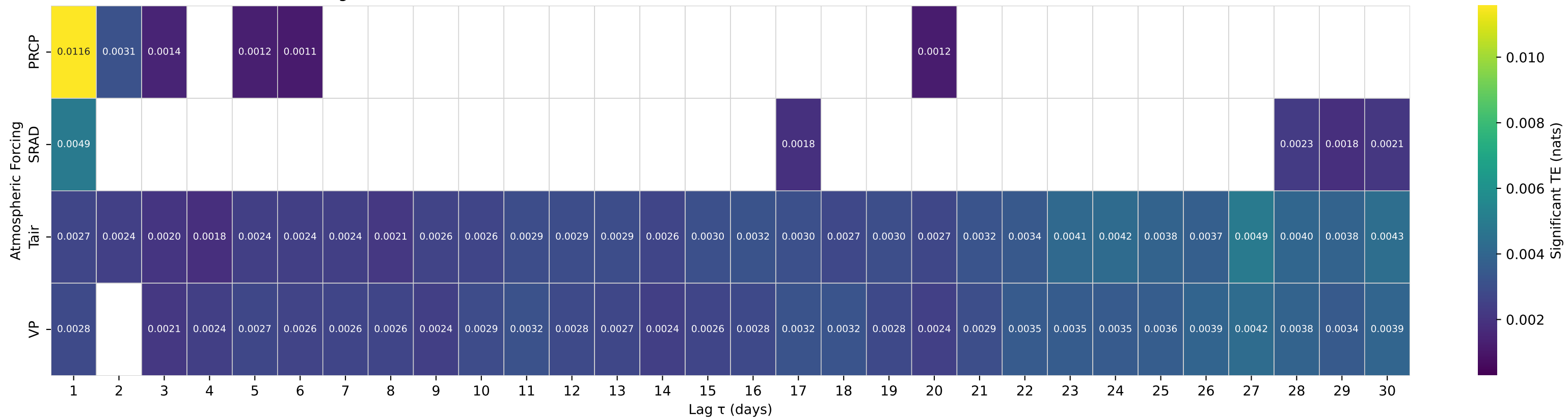
Shuffle-Test Significant TE to Streamflow — Basin 03281500 (HUC 05) — SOUTH FORK KENTUCKY RIVER AT BOONEVILLE, KY
