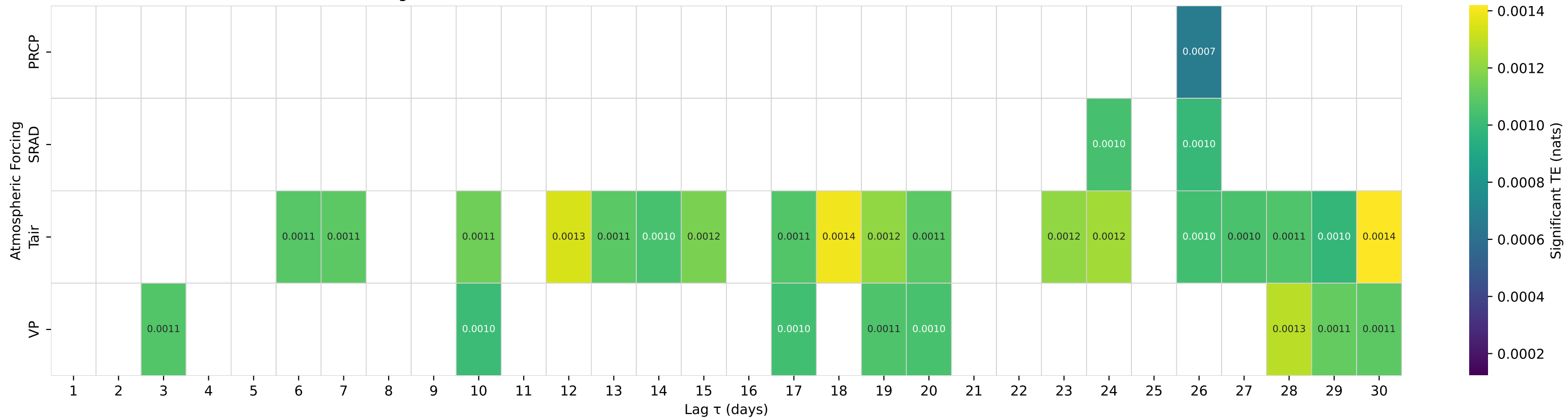
Shuffle-Test Significant TE to Streamflow — Basin 01532000 (HUC 02) — Towanda Creek near Monroeton, PA
