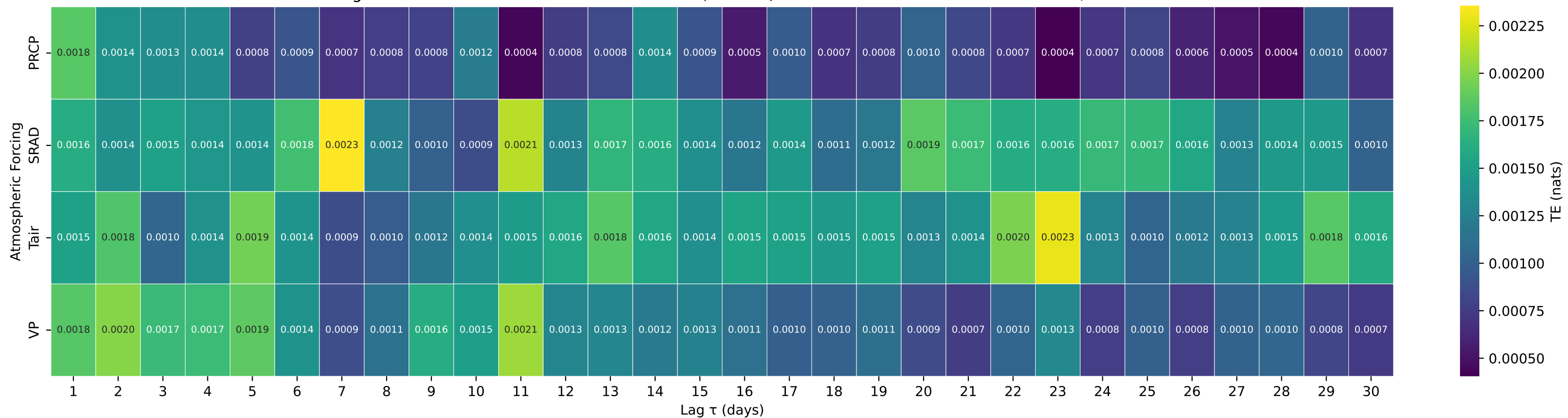
Shuffle-Test Significant TE to Streamflow — Basin 05062500 (HUC 09) — WILD RICE RIVER AT TWIN VALLEY, MN
