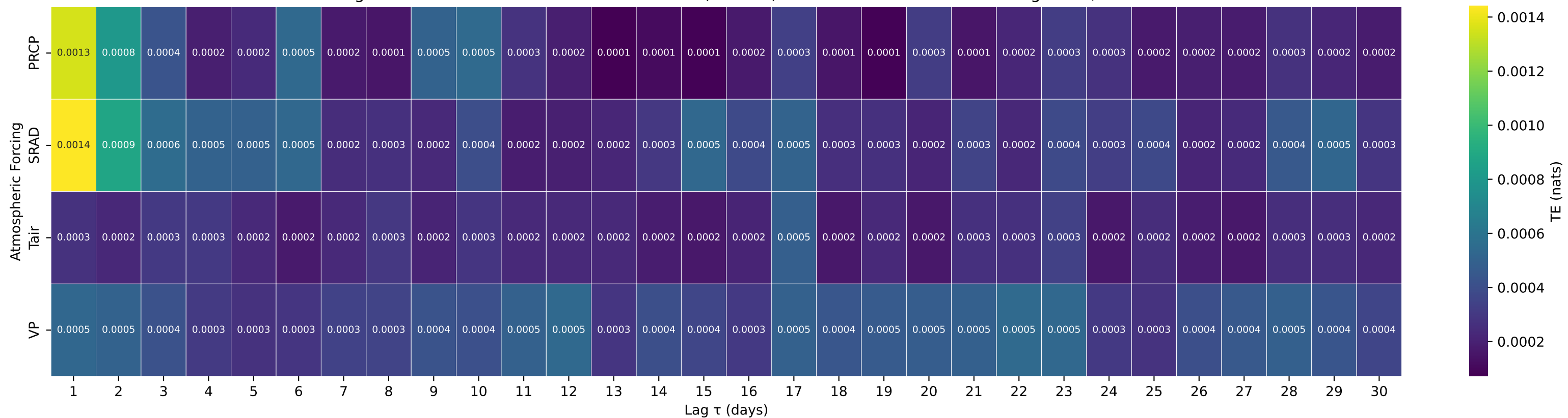
Shuffle-Test Significant TE to Streamflow — Basin 08104900 (HUC 12) — S Fk San Gabriel Rv at Georgetown, TX
