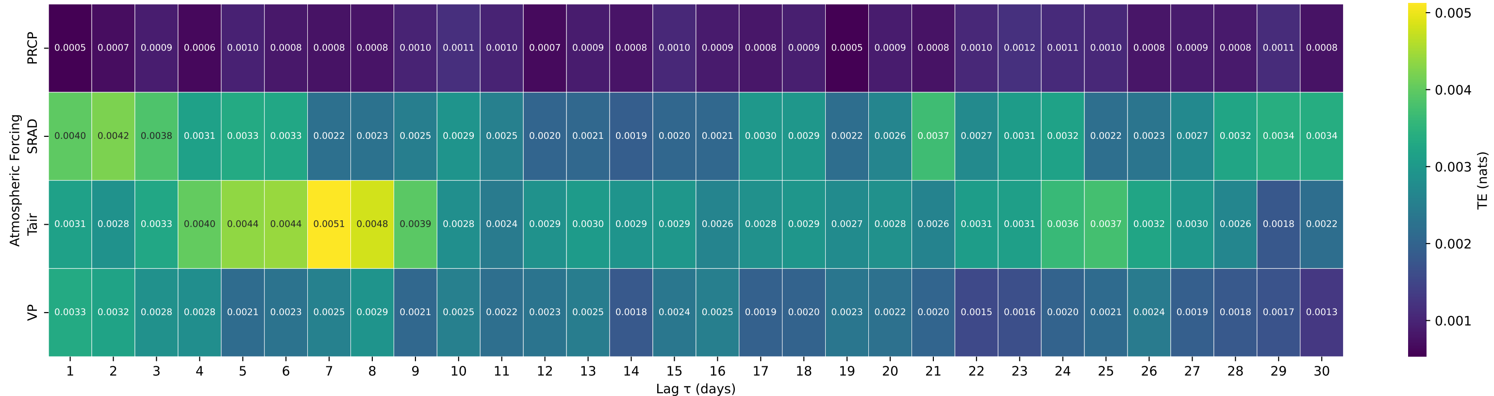
Shuffle-Test Significant TE to Streamflow — Basin 13018300 (HUC 17) — CACHE CREEK NEAR JACKSON, WY
