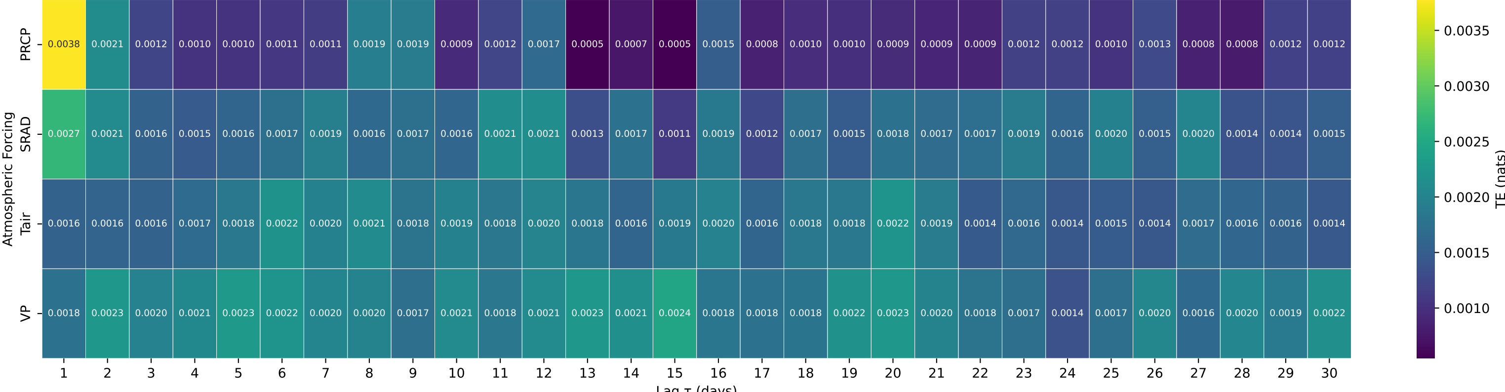
Shuffle-Test Significant TE to Streamflow — Basin 05508805 (HUC 07) — Spencer Cr. bl Plum Cr. nr Frankford, MC
