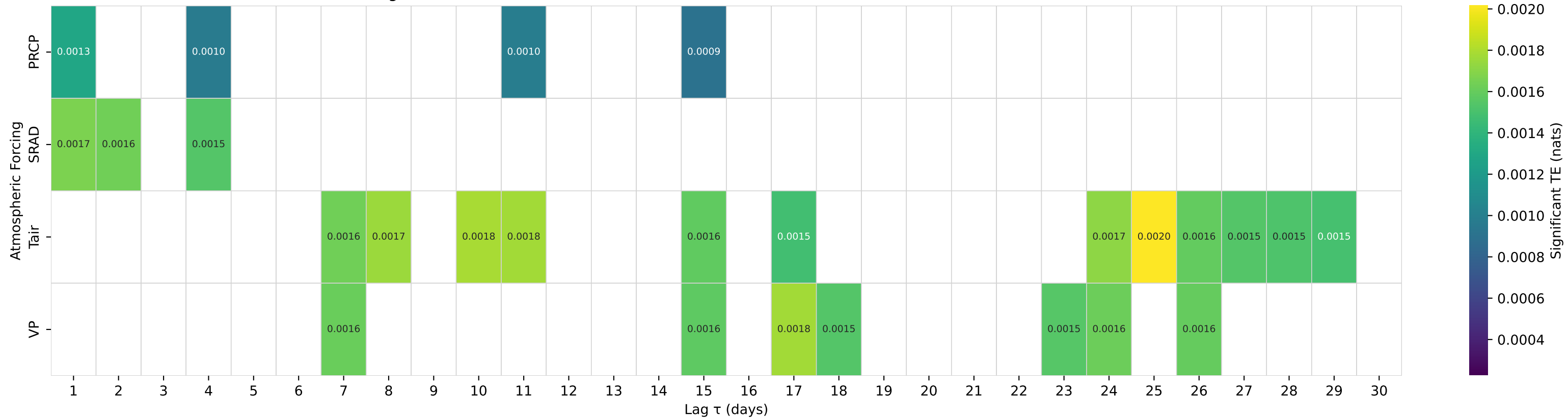
Shuffle-Test Significant TE to Streamflow — Basin 01632900 (HUC 02) — SMITH CREEK NEAR NEW MARKET, VA
