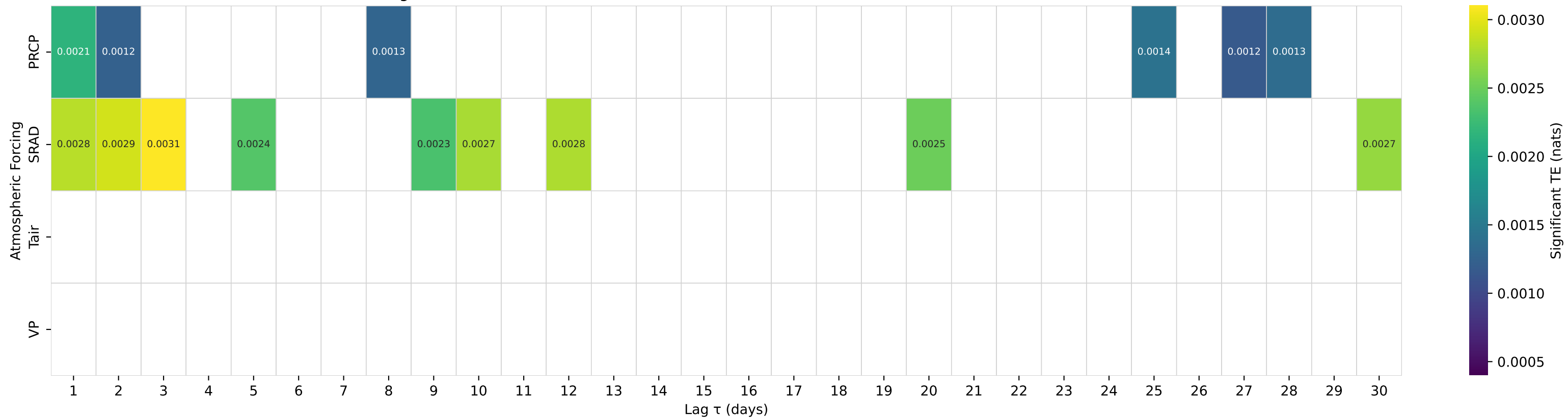
Shuffle-Test Significant TE to Streamflow — Basin 10172700 (HUC 16) — VERNON CREEK NEAR VERNON, UT
