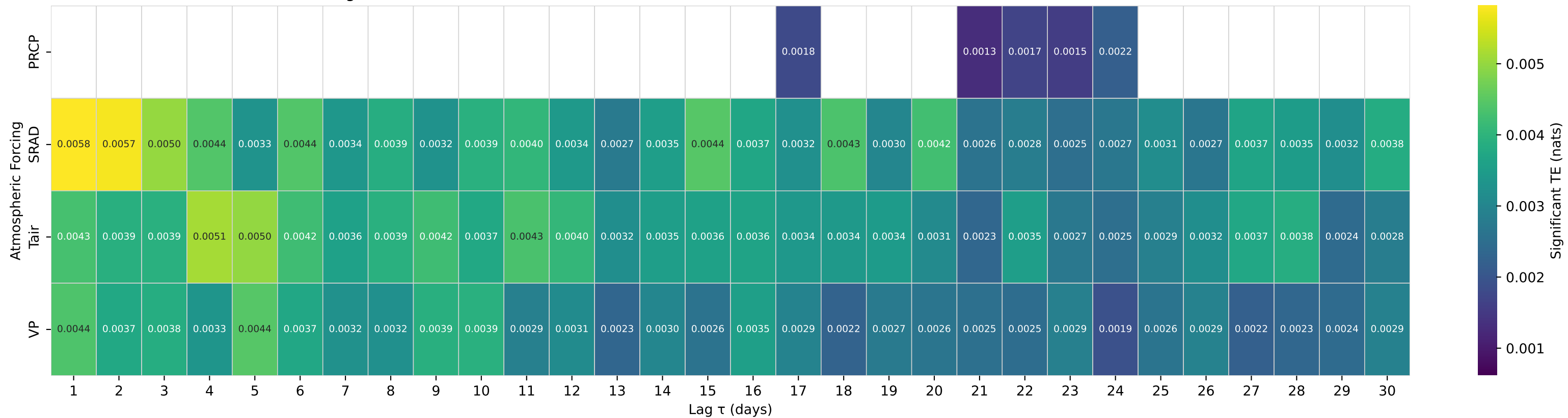
Shuffle-Test Significant TE to Streamflow — Basin 09035900 (HUC 14) — SOUTH FORK OF WILLIAMS FORK NEAR LEAL, CO.
