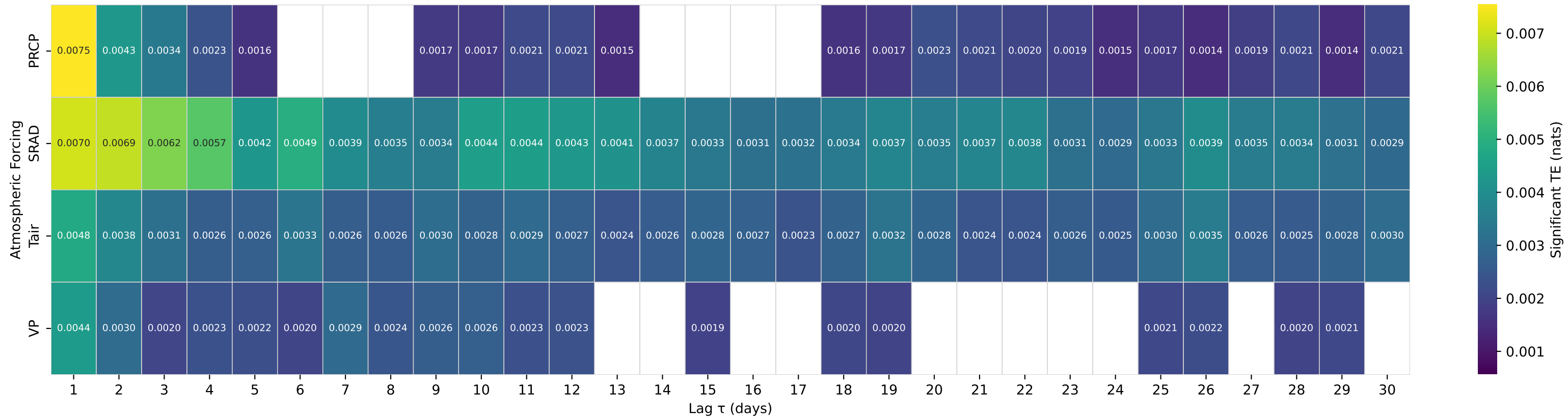
Shuffle-Test Significant TE to Streamflow — Basin 10336645 (HUC 16) — GENERAL C NR MEEKS BAY CA
