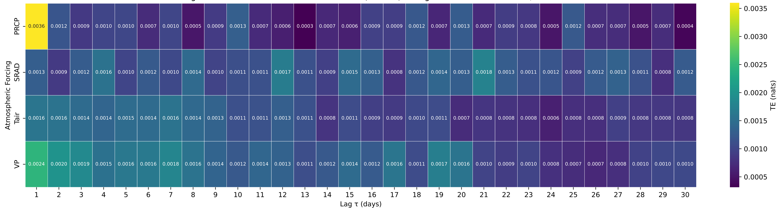
Shuffle-Test Significant TE to Streamflow — Basin 05488200 (HUC 07) — English Creek near Knoxville, IA
