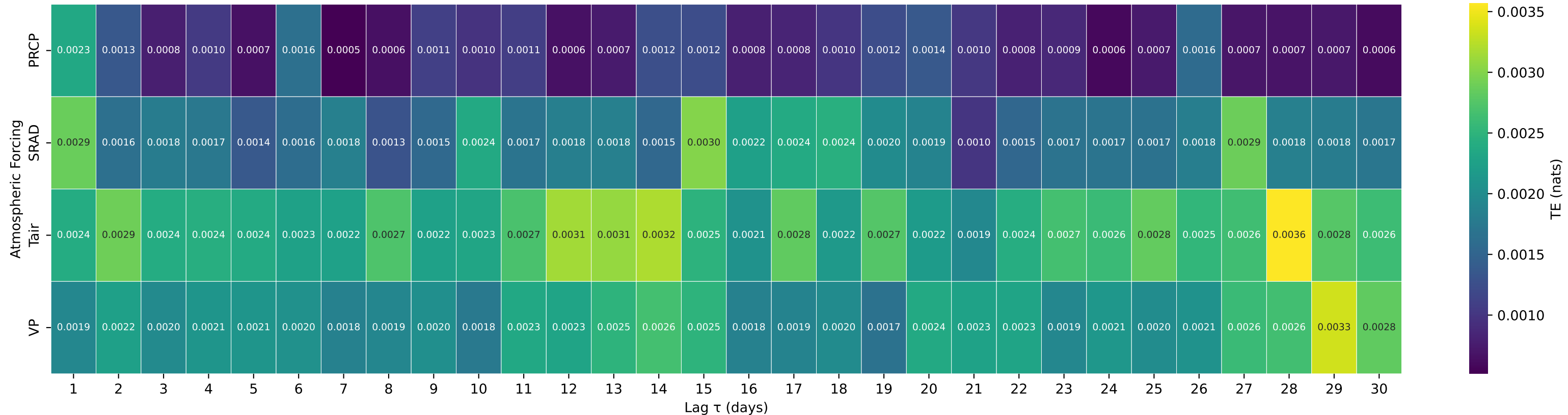
Shuffle-Test Significant TE to Streamflow — Basin 02193340 (HUC 03) — KETTLE CREEK NEAR WASHINGTON, GA
