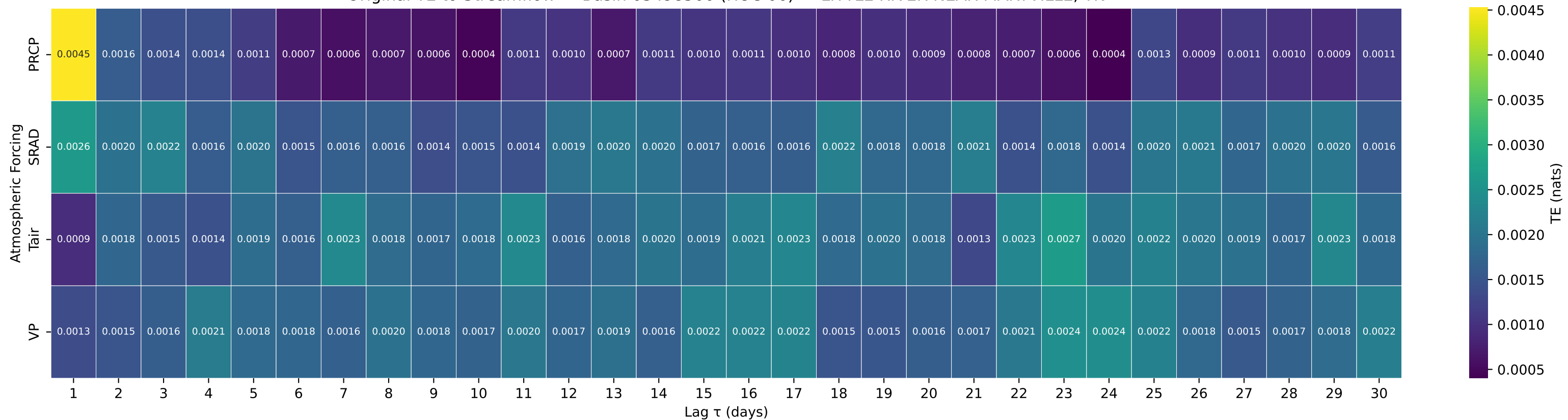
Shuffle-Test Significant TE to Streamflow — Basin 03498500 (HUC 06) — LITTLE RIVER NEAR MARYVILLE, TN
