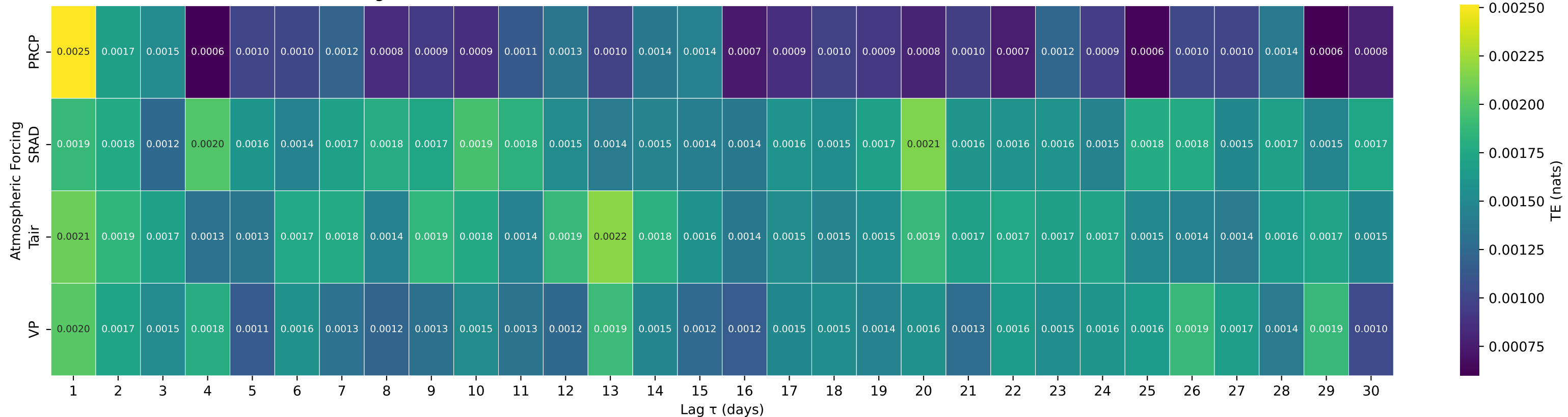
Shuffle-Test Significant TE to Streamflow — Basin 03364500 (HUC 05) — CLIFTY CREEK AT HARTSVILLE, IN
