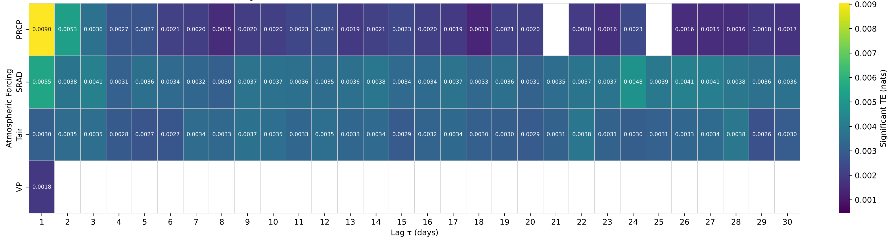
Shuffle-Test Significant TE to Streamflow — Basin 11473900 (HUC 18) — MF EEL R NR DOS RIOS CA
