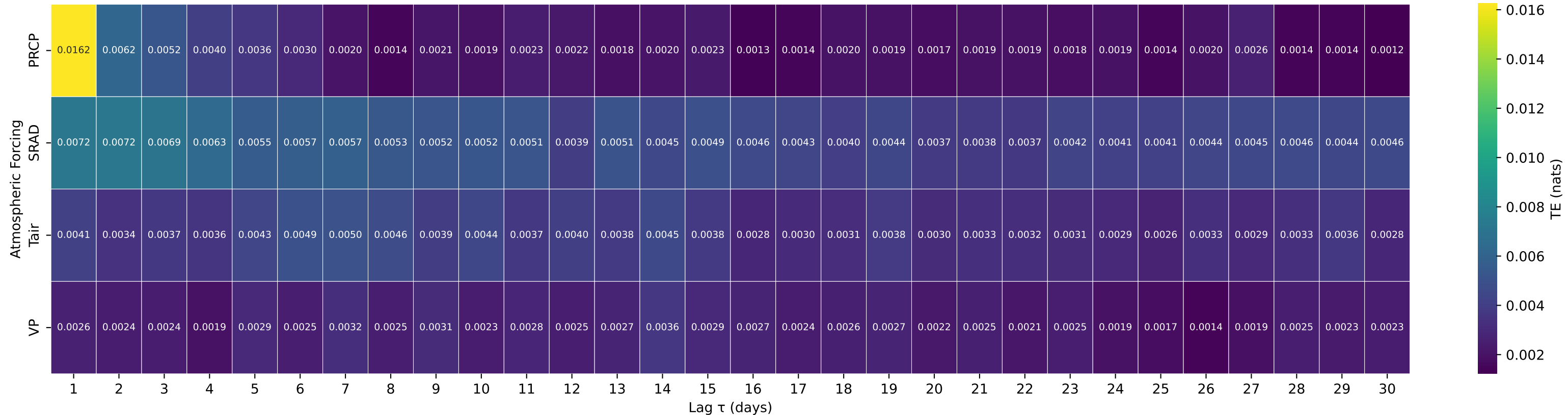
Shuffle-Test Significant TE to Streamflow — Basin 12048000 (HUC 17) — DUNGENESS RIVER NEAR SEQUIM, WA
