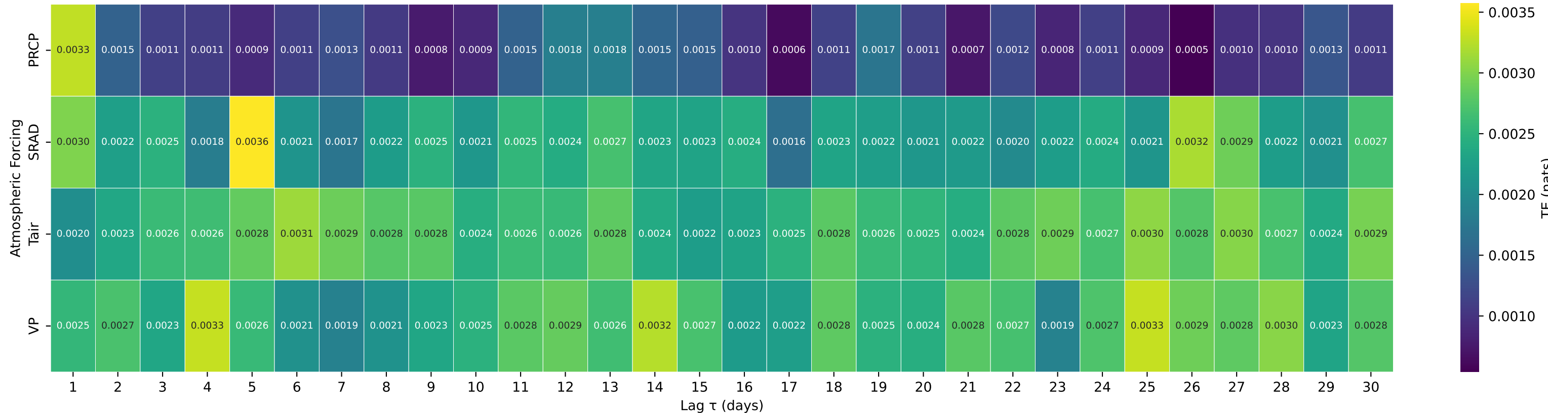
Shuffle-Test Significant TE to Streamflow — Basin 02430615 (HUC 03) — MUD CREEK NR FAIRVIEW, MS
