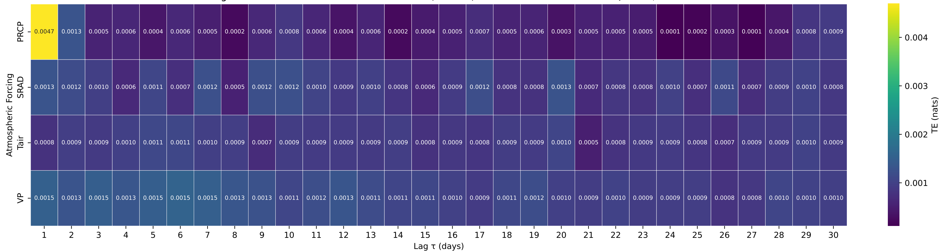
Shuffle-Test Significant TE to Streamflow — Basin 07299670 (HUC 11) — Groesbeck Ck at SH 6 nr Quanah, TX
