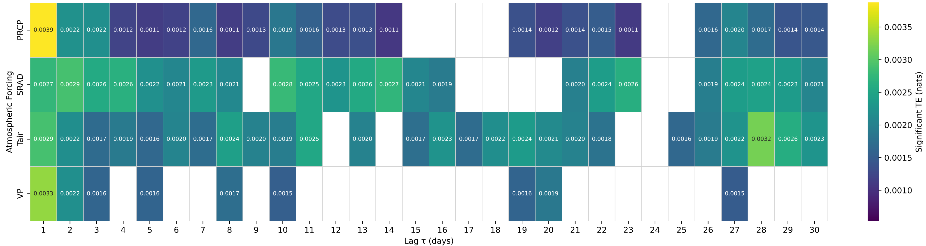
Shuffle-Test Significant TE to Streamflow — Basin 10329500 (HUC 16) — MARTIN C NR PARADISE VALLEY, NV
