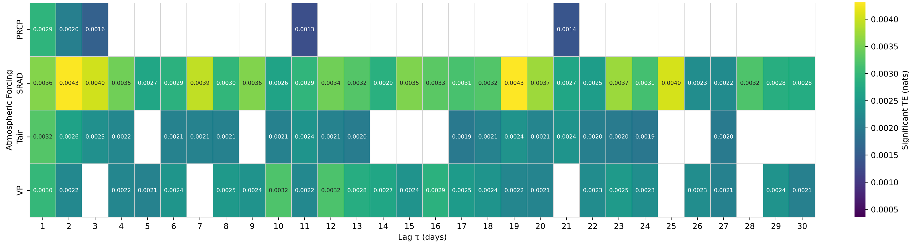
Shuffle-Test Significant TE to Streamflow — Basin 08378500 (HUC 13) — PECOS RIVER NEAR PECOS, NM
