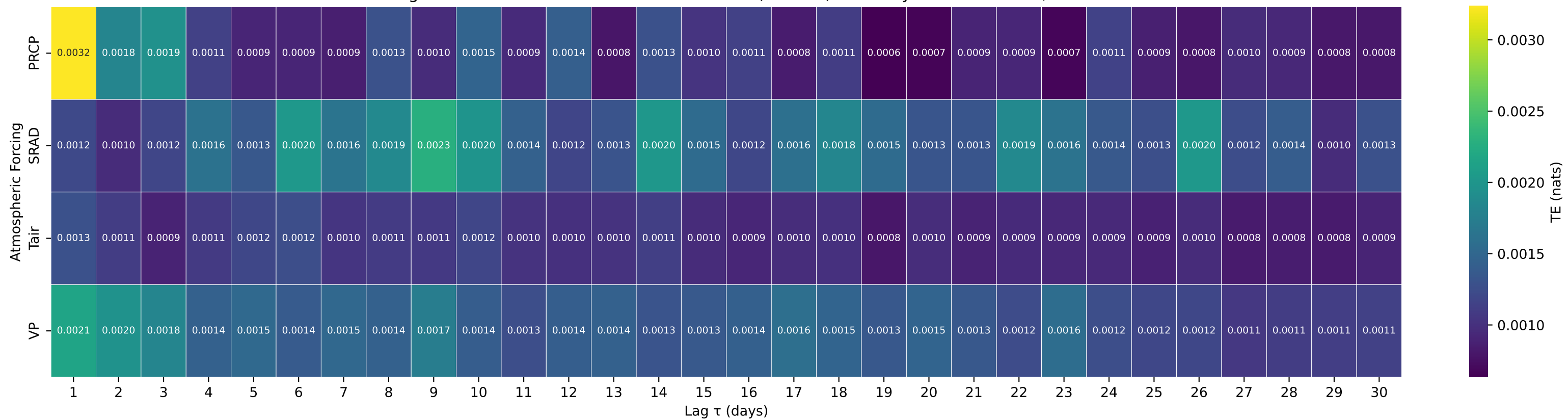
Shuffle-Test Significant TE to Streamflow — Basin 05412500 (HUC 07) — Turkey River at Garber, IA
