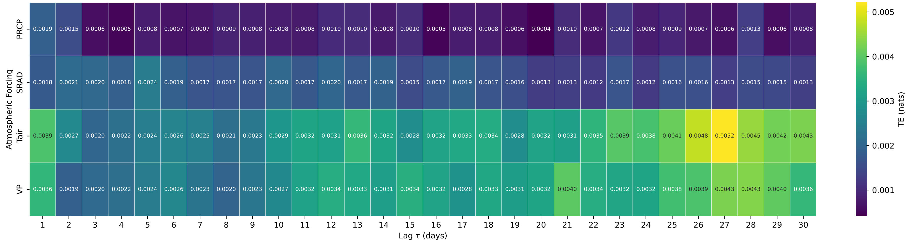
Shuffle-Test Significant TE to Streamflow — Basin 01596500 (HUC 02) — SAVAGE RIVER NEAR BARTON, MD
