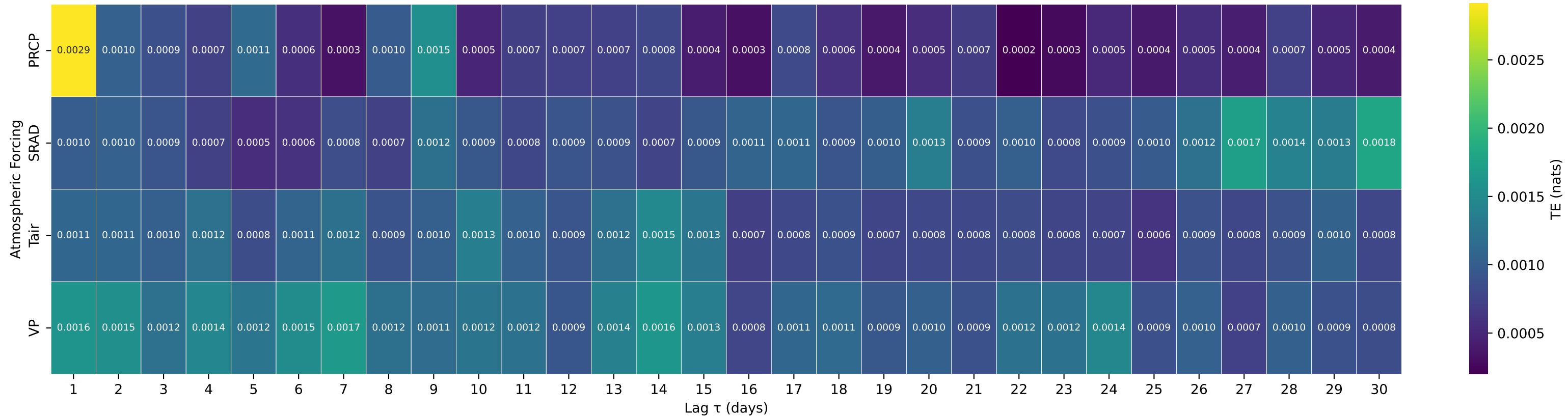
Shuffle-Test Significant TE to Streamflow — Basin 06889500 (HUC 10) — SOLDIER C NR TOPEKA, KS
