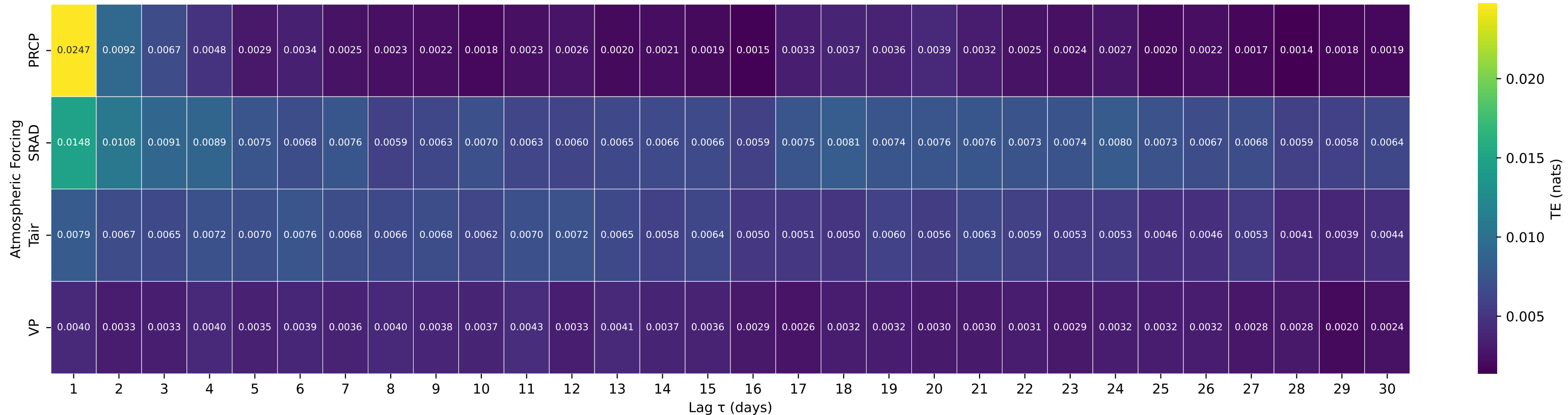
Shuffle-Test Significant TE to Streamflow — Basin 14185900 (HUC 17) — QUARTZVILLE CREEK NEAR CASCADIA, OREG.
