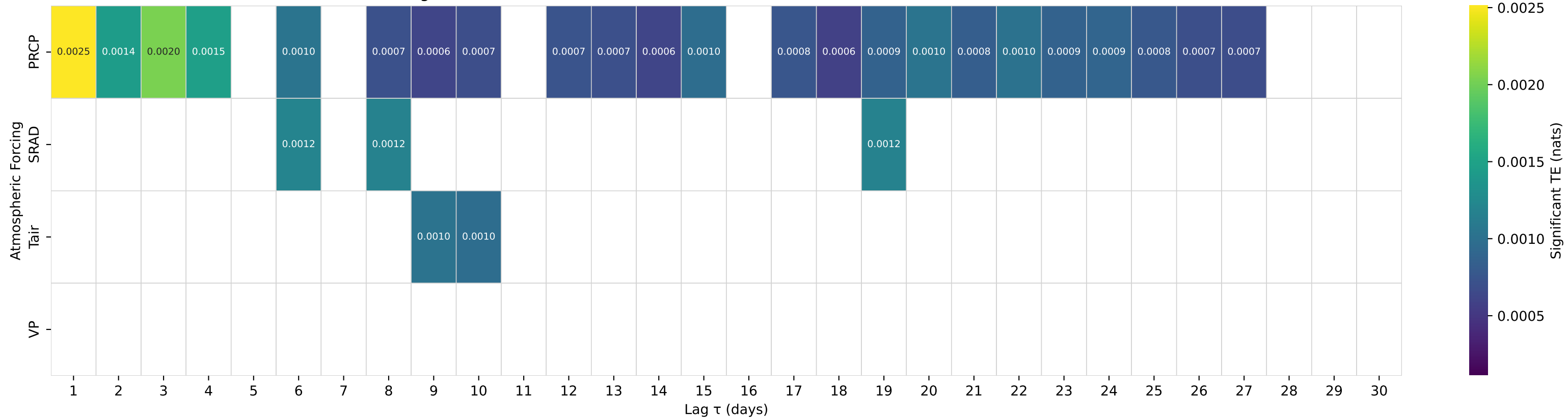
Shuffle-Test Significant TE to Streamflow — Basin 14362250 (HUC 17) — STAR GULCH NEAR RUCH, OR.
