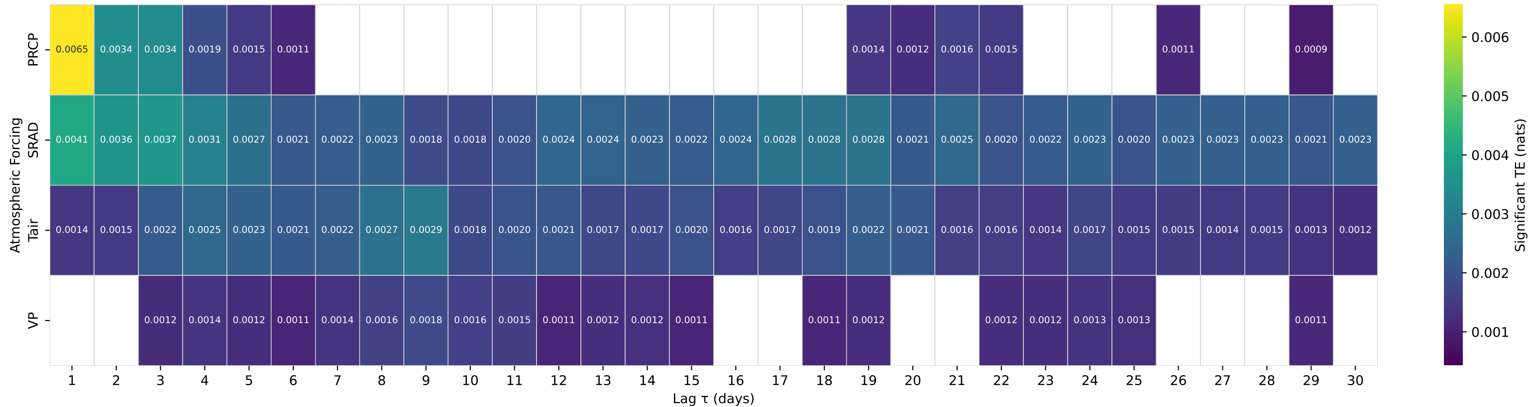
Shuffle-Test Significant TE to Streamflow — Basin 14182500 (HUC 17) — LITTLE NORTH SANTIAM RIVER NEAR MEHAMA, OR
