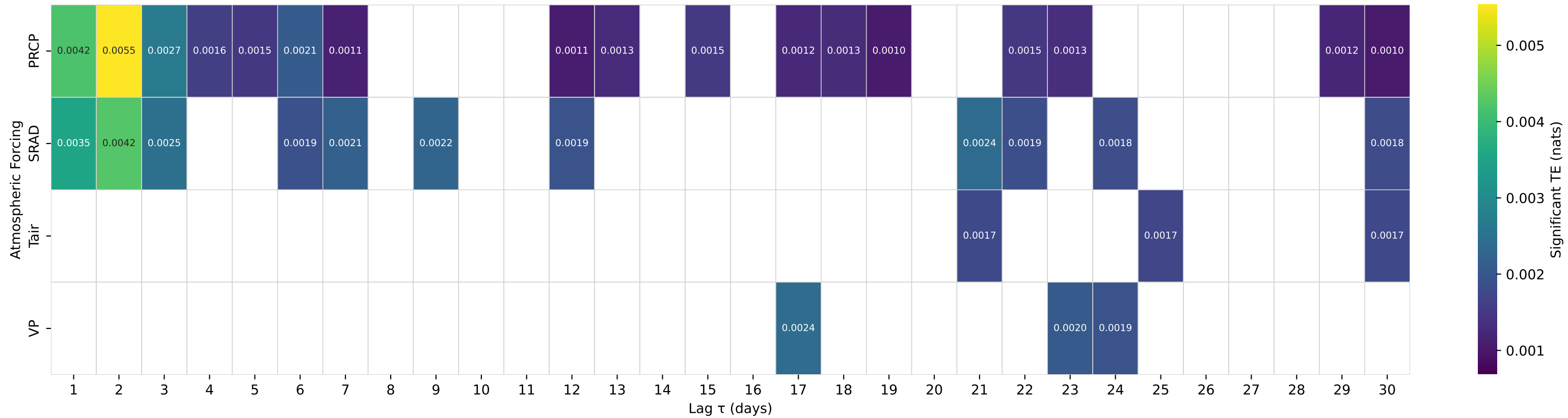
Shuffle-Test Significant TE to Streamflow — Basin 02314500 (HUC 03) — SUWANNEE RIVER AT US 441, AT FARGO, GA
