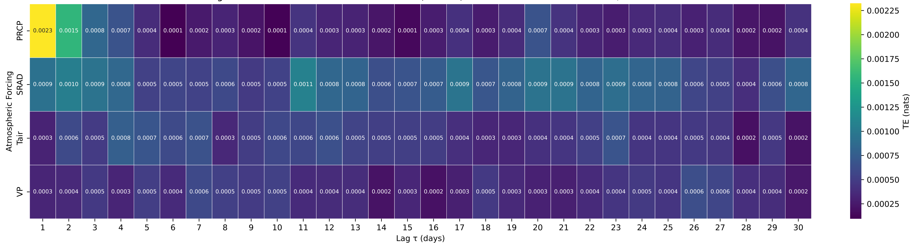
Shuffle-Test Significant TE to Streamflow — Basin 12020000 (HUC 17) — CHEHALIS RIVER NEAR DOTY, WA
