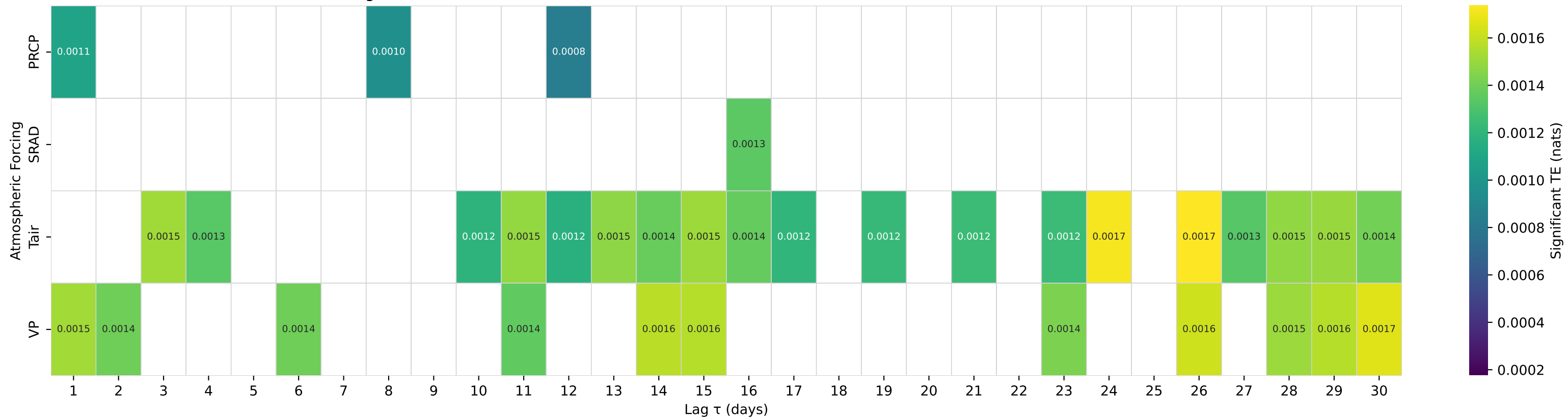
Shuffle-Test Significant TE to Streamflow — Basin 02015700 (HUC 02) — BULLPASTURE RIVER AT WILLIAMSVILLE, VA
