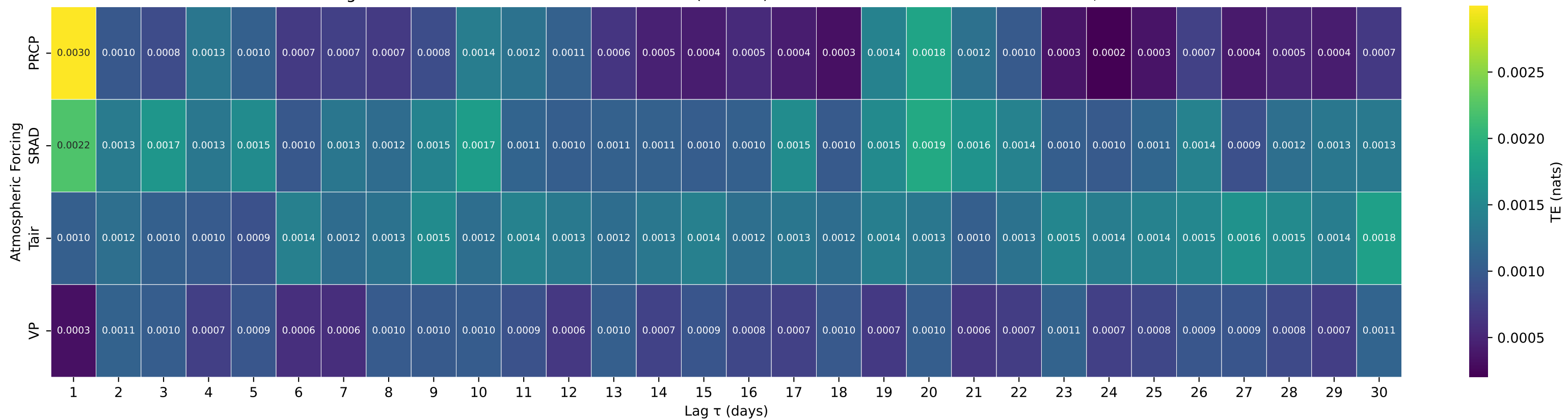
Shuffle-Test Significant TE to Streamflow — Basin 09505200 (HUC 15) — WET BEAVER CREEK NEAR RIMROCK, AZ.
