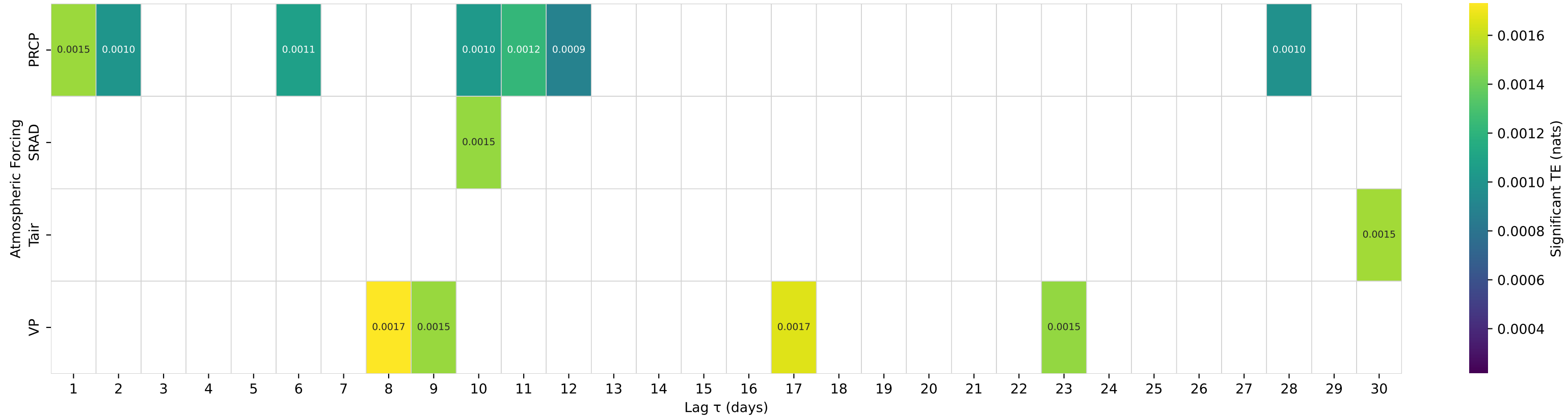
Shuffle-Test Significant TE to Streamflow — Basin 02074500 (HUC 03) — SANDY RIVER NEAR DANVILLE, VA
