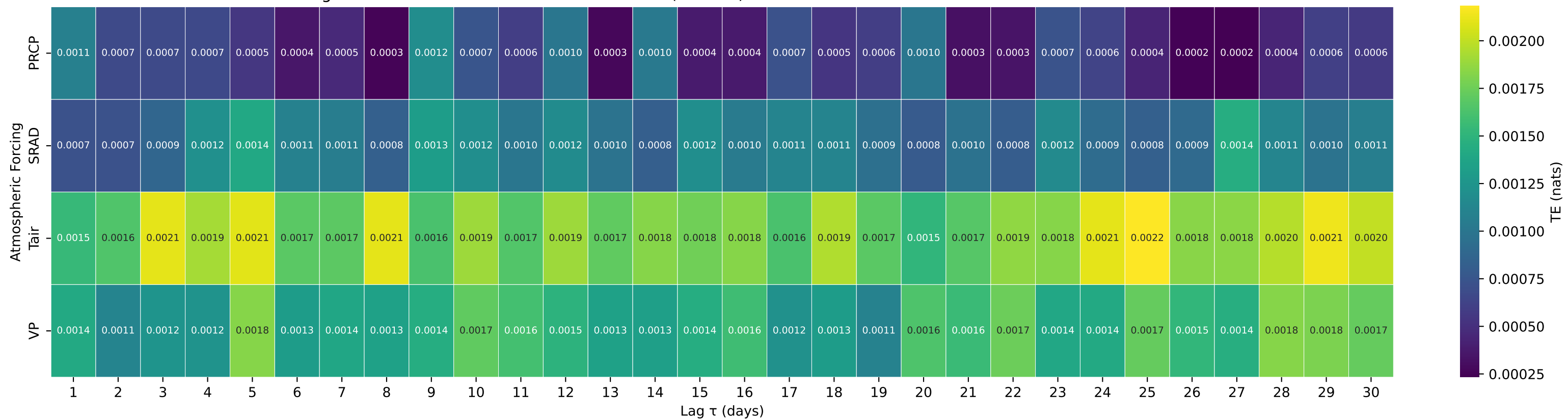
Shuffle-Test Significant TE to Streamflow — Basin 01413500 (HUC 02) — EAST BR DELAWARE R AT MARGARETVILLE NY
