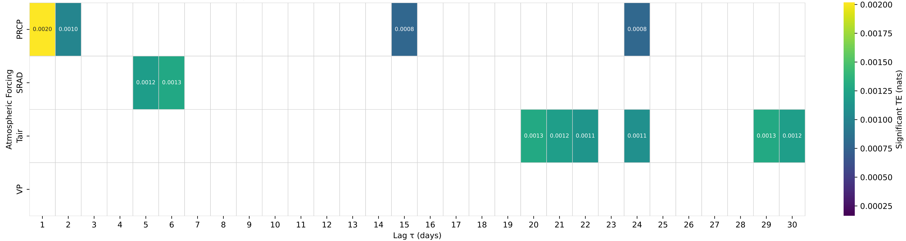
Shuffle-Test Significant TE to Streamflow — Basin 03066000 (HUC 05) — BLACKWATER R AT DAVIS, WV
