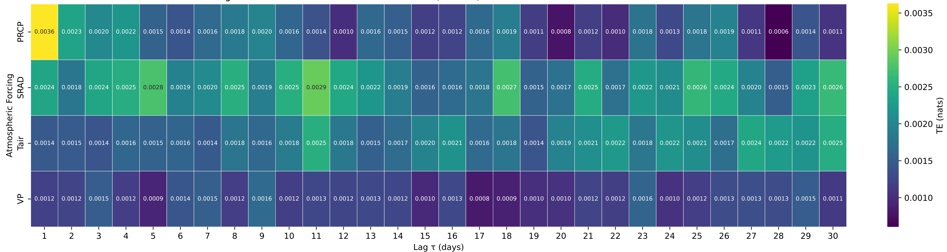
Shuffle-Test Significant TE to Streamflow — Basin 06360500 (HUC 10) — MOREAU R NEAR WHITEHORSE SD
