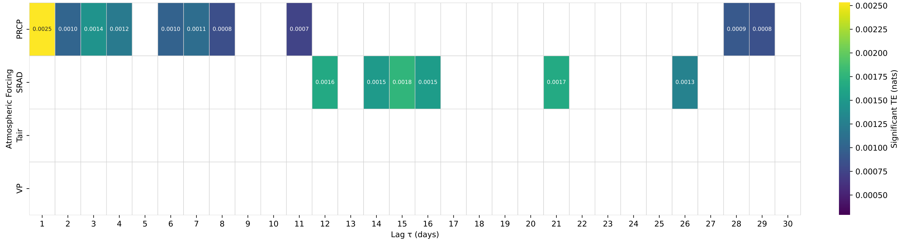
Shuffle-Test Significant TE to Streamflow — Basin 06450500 (HUC 10) — LITTLE WHITE R BELOW WHITE RIVER SD
