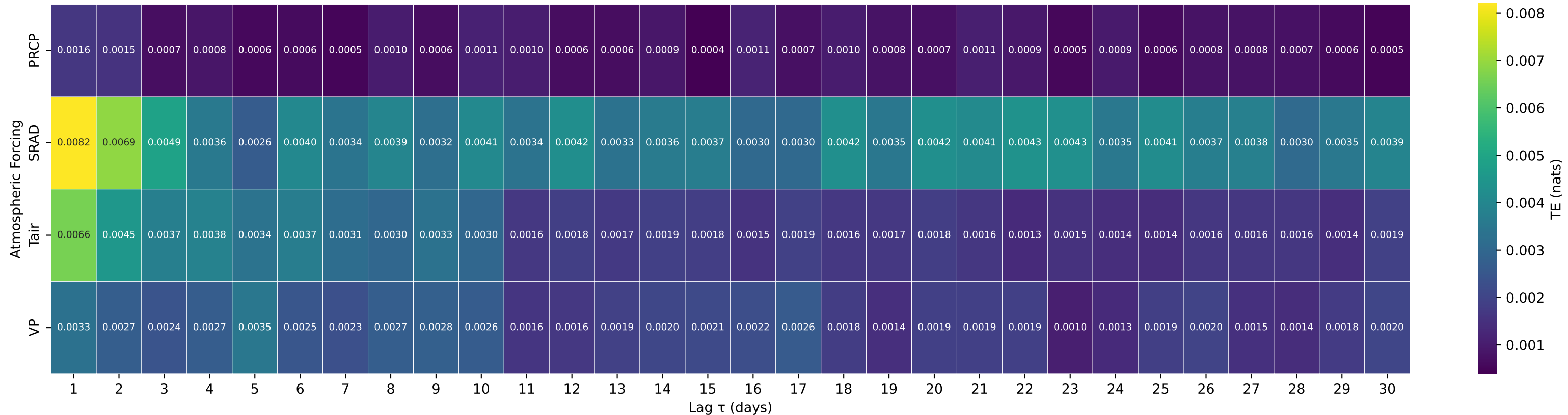
Shuffle-Test Significant TE to Streamflow — Basin 12447390 (HUC 17) — ANDREWS CREEK NEAR MAZAMA, WA
