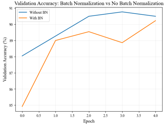
Plot 5 & 6: Validation accuracy (left) and training loss (right) — with vs. without Batch Normalization
