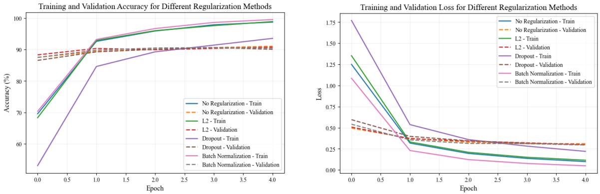
Plot 3: Training/validation accuracy (left) and Plot 4: Training/validation loss (right), for different regularization methods
