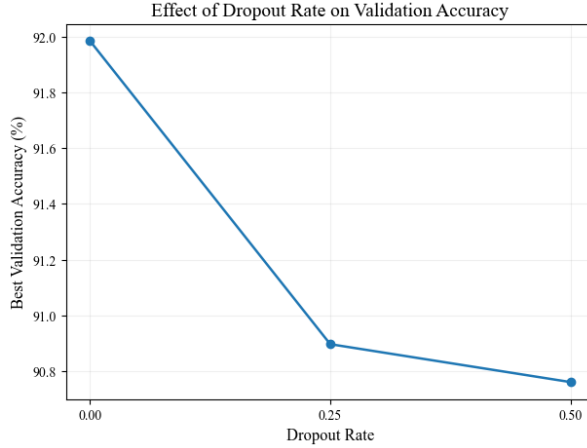
Plot 10: Effect of dropout rate on validation accuracy
