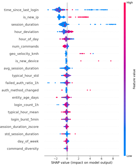
SHAP Global Feature Attribution
