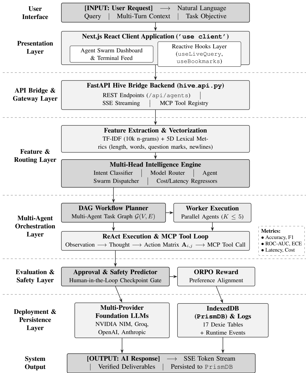
Figure 4.2: Different Layers.
