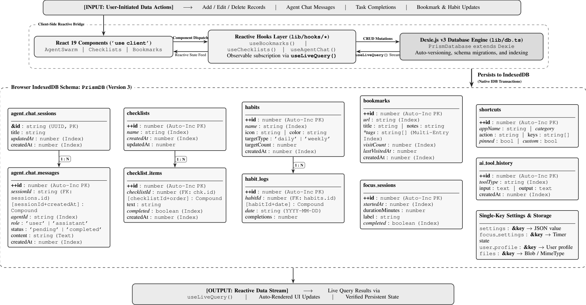
Figure 4.4: Browser IndexedDB Database Schema and Reactive Data Architecture (PrismDB)
