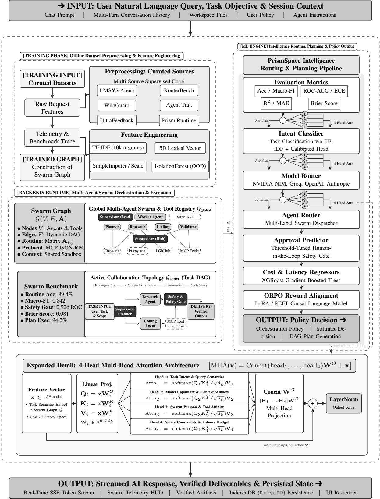
Figure 4.1: Framework of PrismSpace Multi-Agent System
