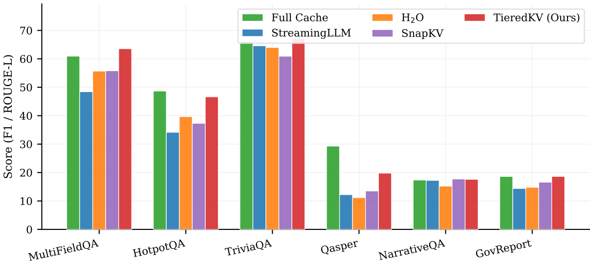
LongBench Benchmark Accuracy — Equal-VRAM Setting
