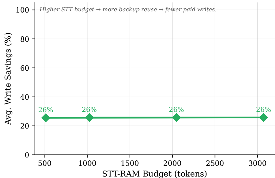
Write Savings vs. STT Budget (Ablation)
