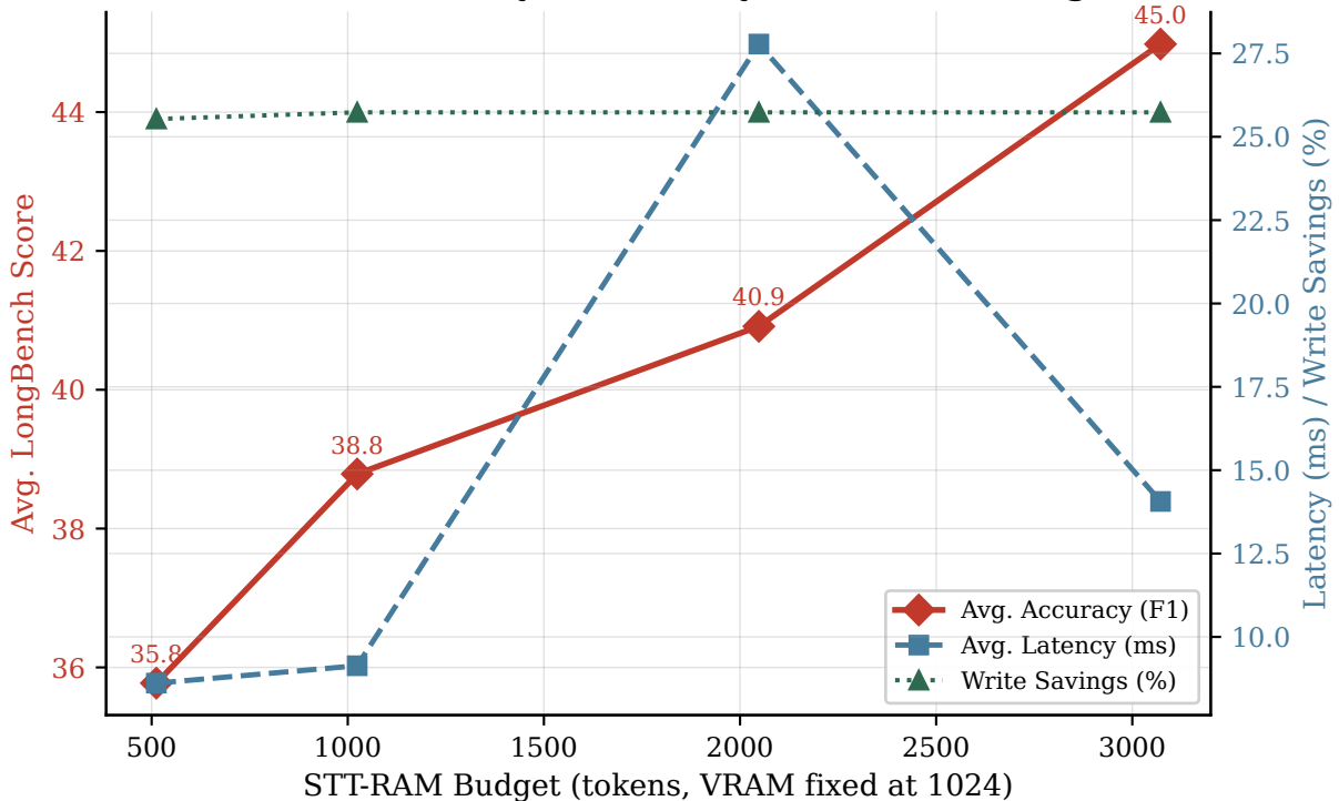
TieredKV: Accuracy & Efficiency vs. STT-RAM Budget
