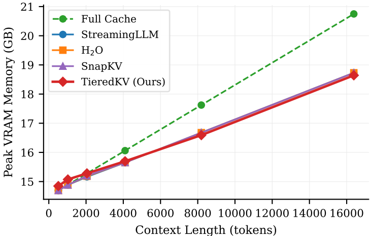
Peak VRAM Footprint vs. Context Length
