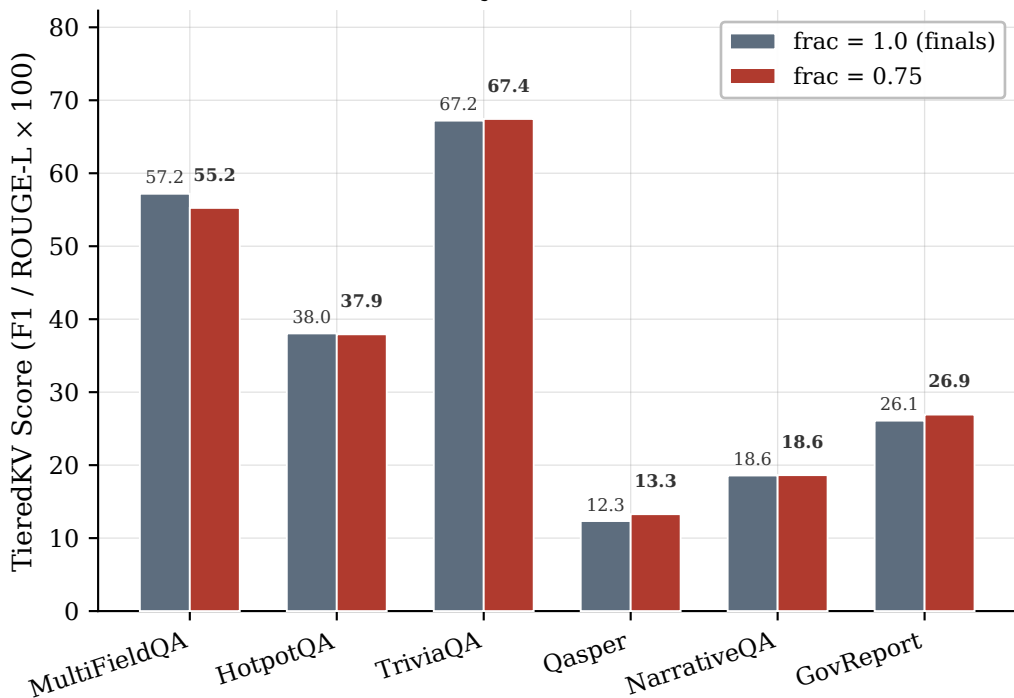
(a) Accuracy holds at frac = 0.75
