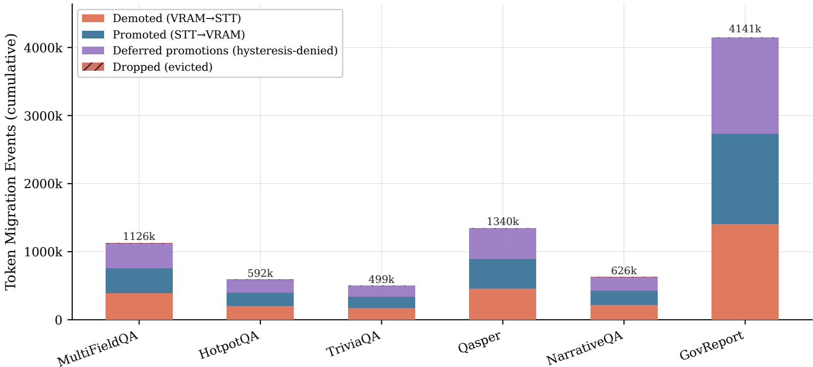
TieredKV Migration Profile per Task (Equal-VRAM Setting)
