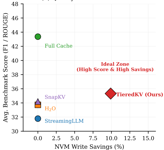
(b) Quality vs. Write Reduction
