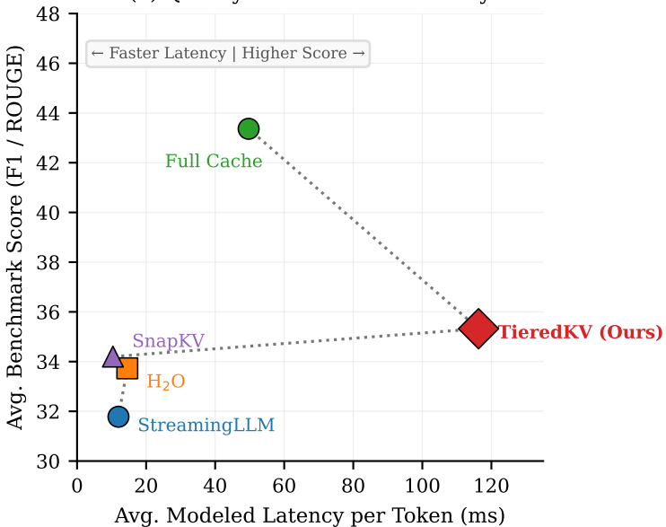
(a) Quality vs. Hardware Latency
