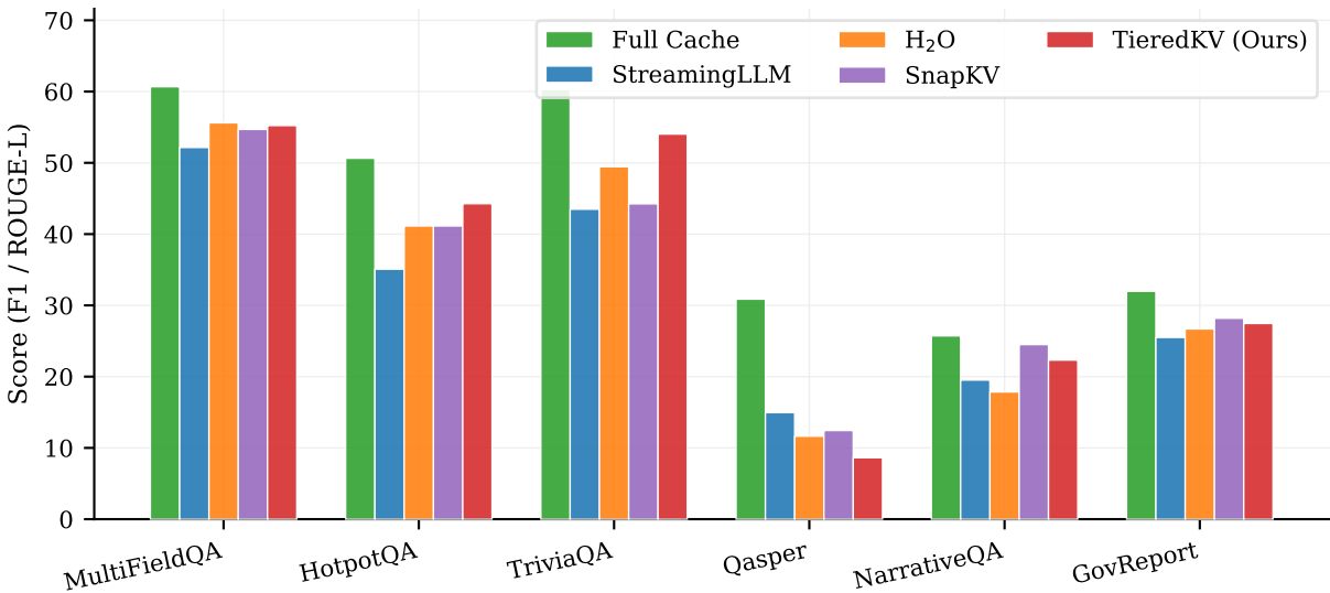
LongBench Benchmark Accuracy — Iso-VRAM Setting
