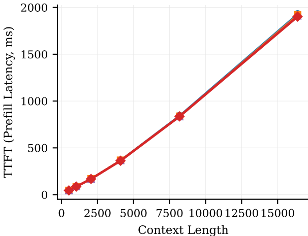
(a) Time-To-First-Token (TTFT)
