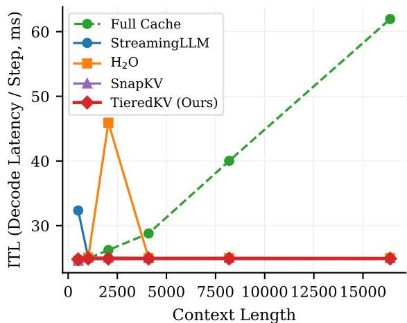
(b) Inter-Token Latency (ITL)
