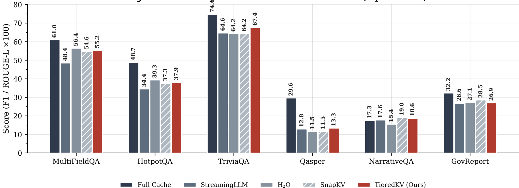
LongBench Accuracy — TieredKV vs. SOTA Baselines (Equal-VRAM)
