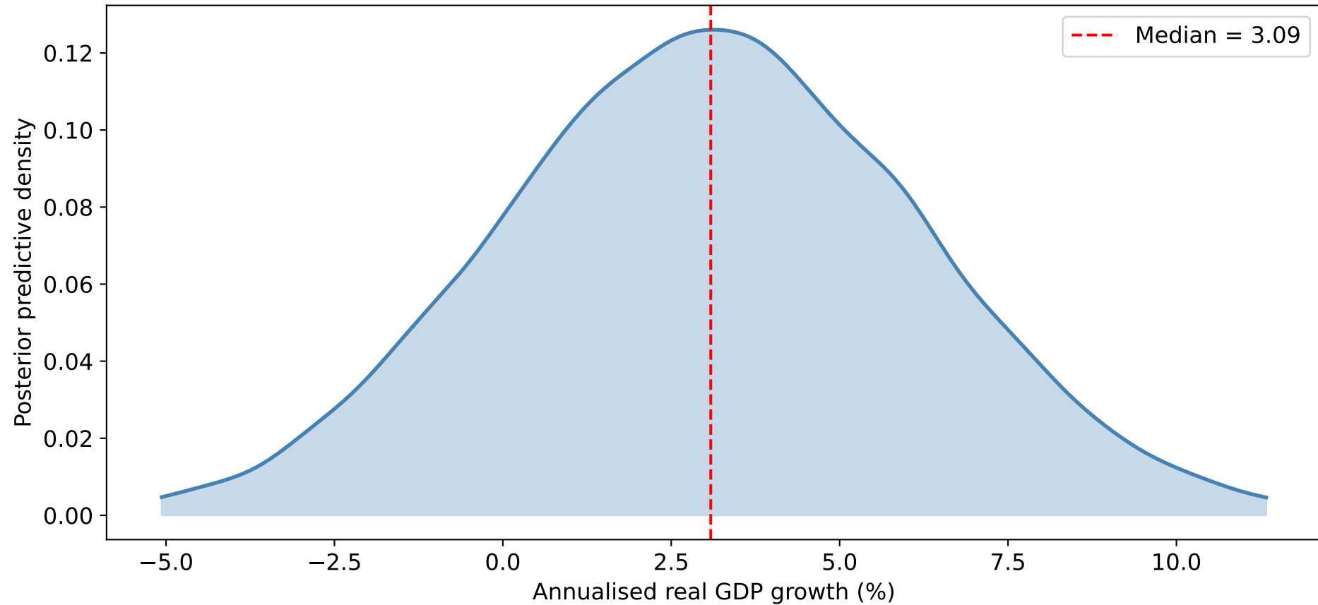
Posterior Predictive Density of Real GDP Growth in 2020-Q2 ( p = 20 )
