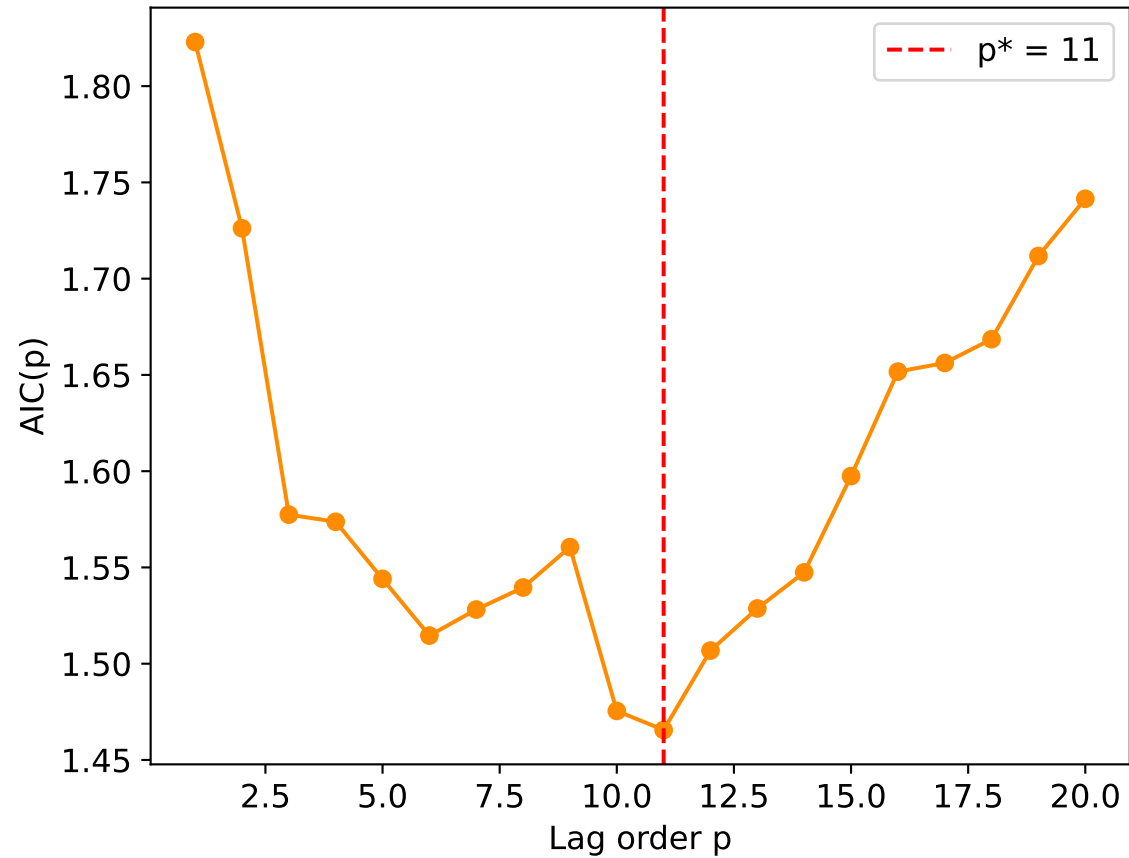
AIC
