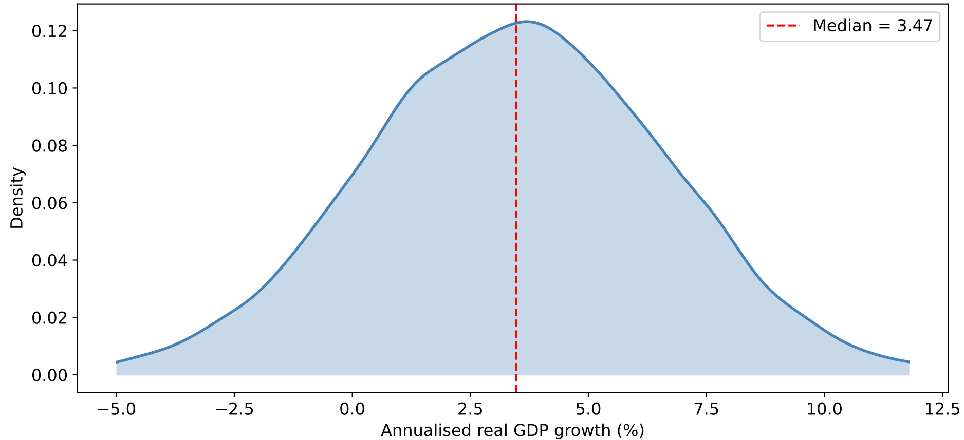
Predictive Density of Real GDP Growth, 2020-Q2 ( p = 1 )
