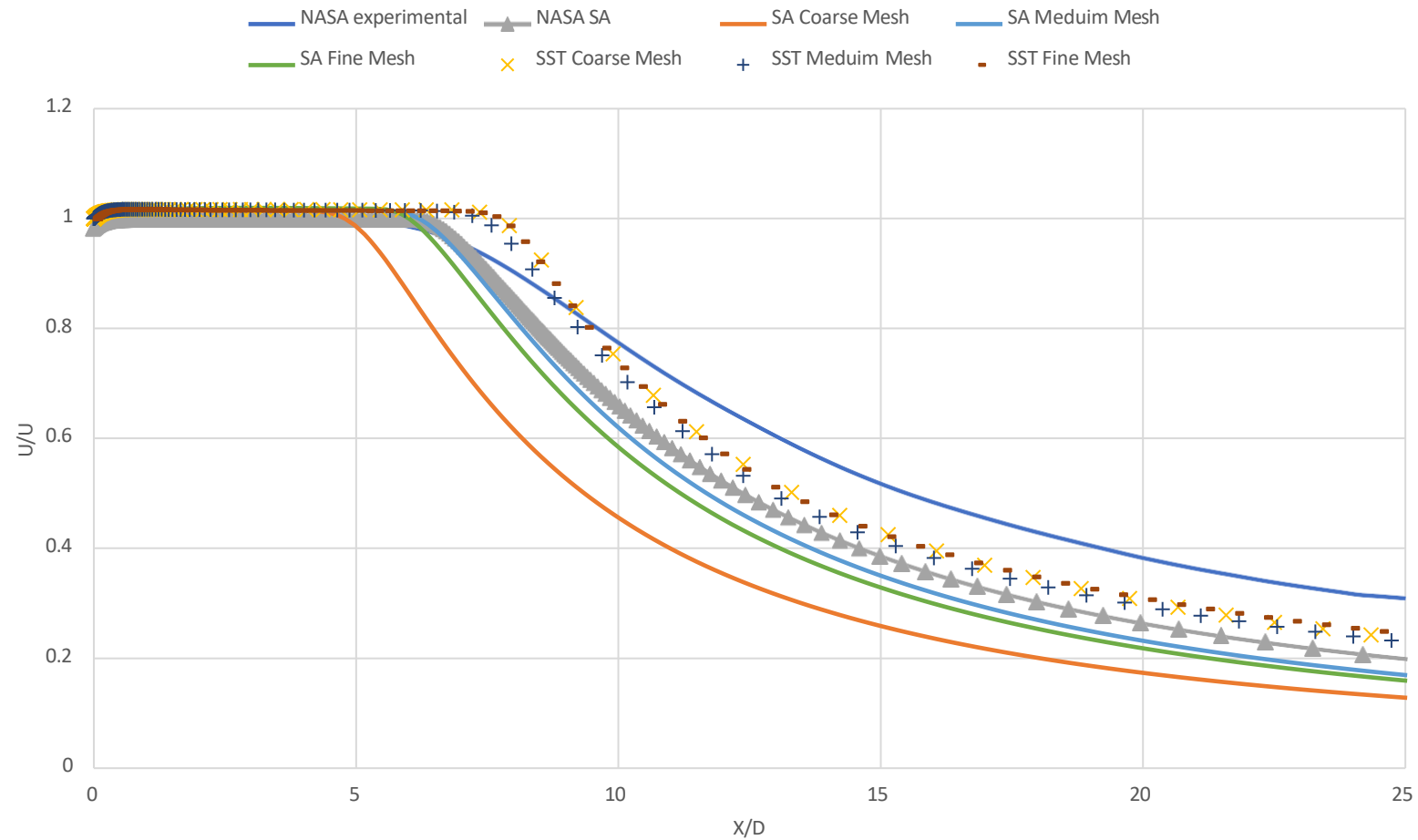
AXIAL VELOCITY VS AXIAL DISTANCE PRESENT CFD VS NASA'S DATA
