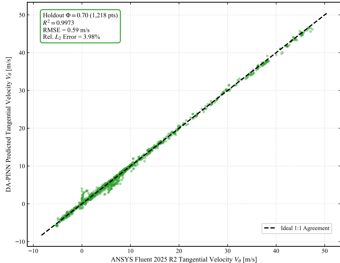
(e) Overall Tangential Swirl Velocity Parity Scatter
