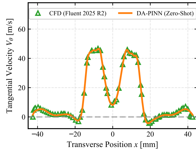
(c) Station z = 25 mm (Flame Core)
