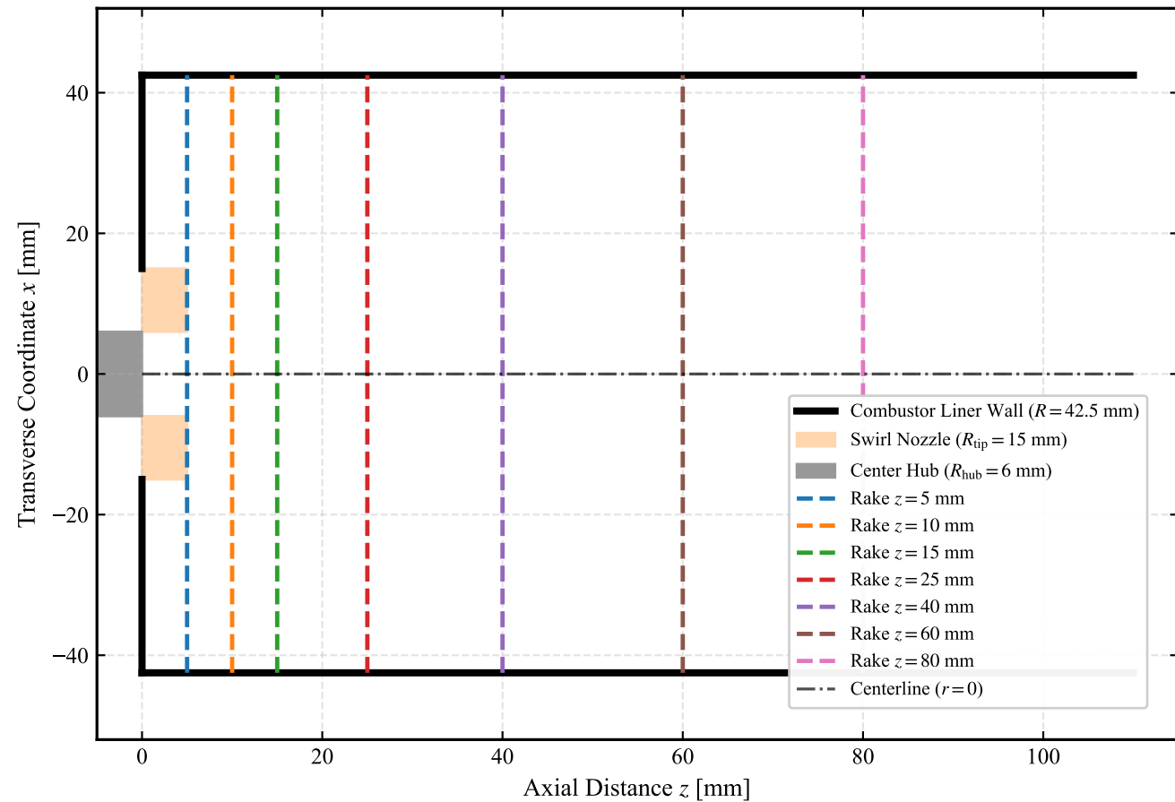
(a) Combustor Domain &amp; 7 Measurement Stations
