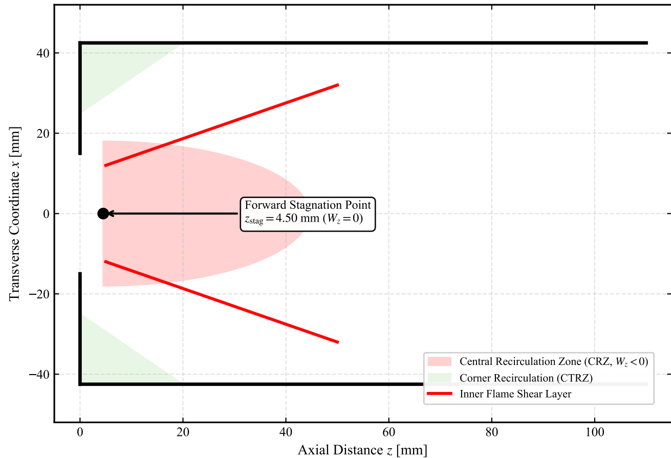
(b) Swirl Flow Aerodynamic Topology &amp; Recirculation
