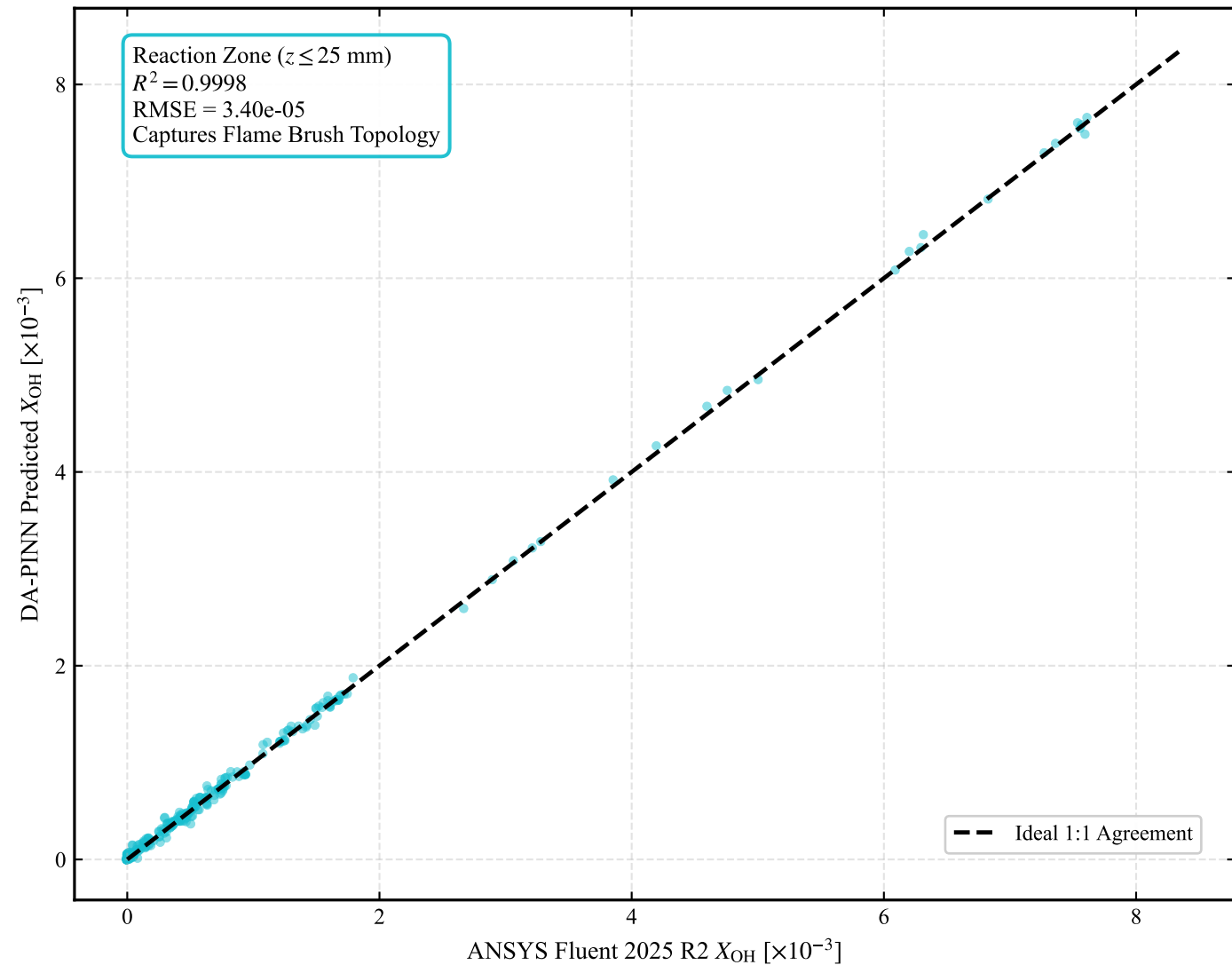
(e) Reaction Zone OH Radical Parity Scatter
