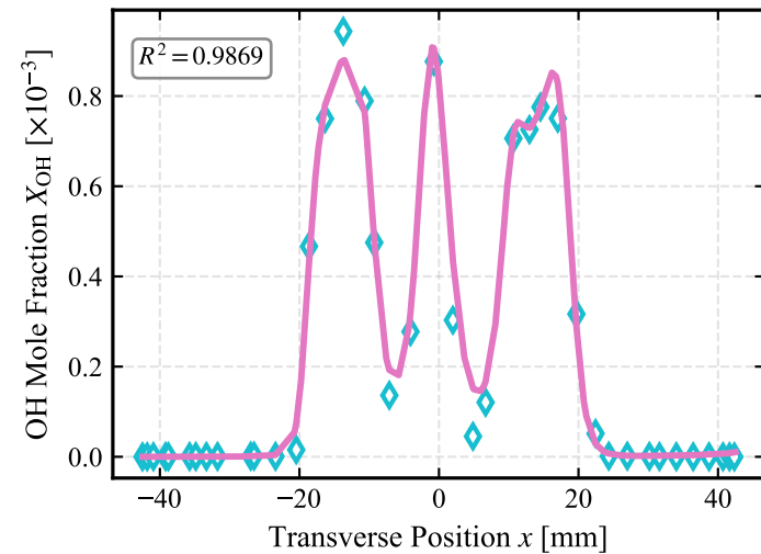
(c) Station z = 15 mm (Inner Flame Core)
