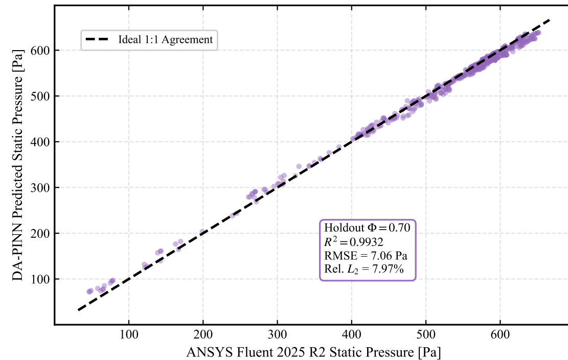
(b) Static Pressure Parity Scatter
