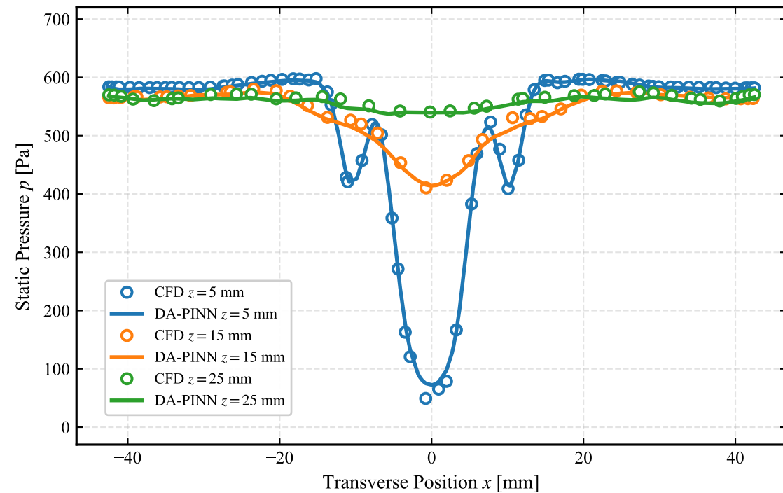
(a) Radial Pressure Traverses \partial p / \partial r = \rho V_\theta^2 / r
