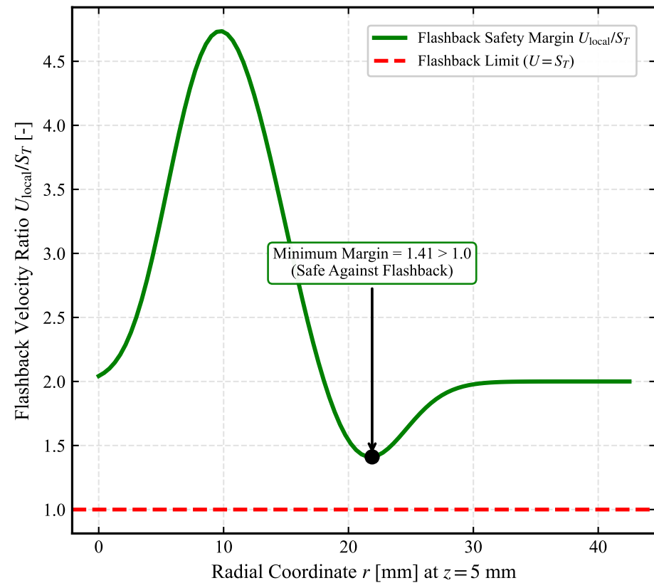
(c) Localized Aerodynamic Flashback Safety Margin
