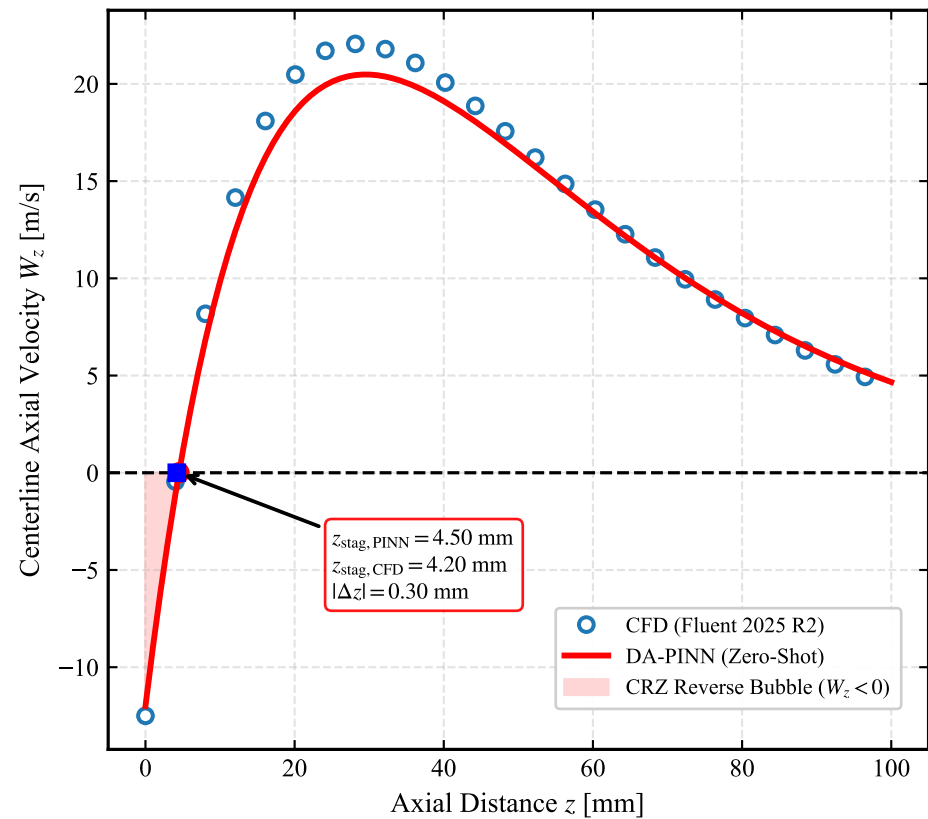
(a) Centerline CRZ Aerodynamics &amp; Stagnation
