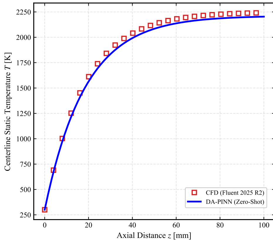
(b) Centerline Thermal Entrainment &amp; Recovery
