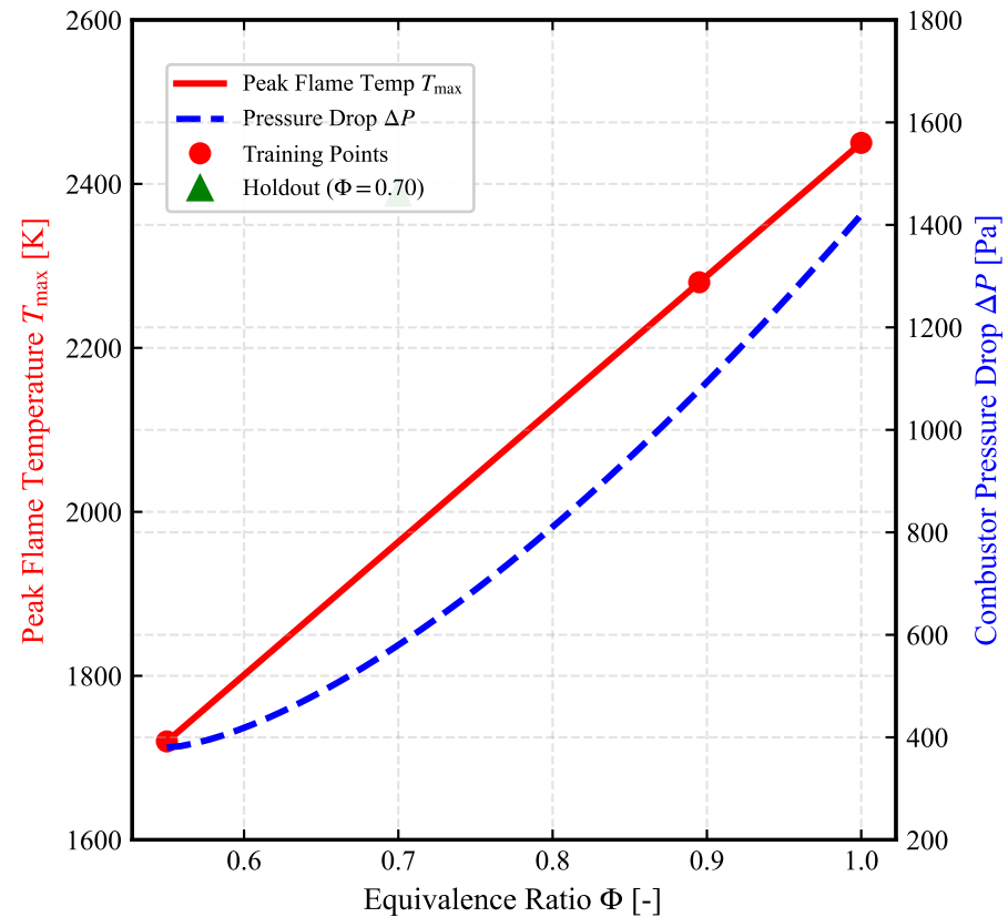
(a) Multi-Throttle Operating Scaling
