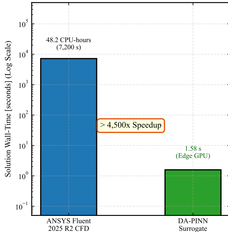
(b) Computational Latency Comparison
