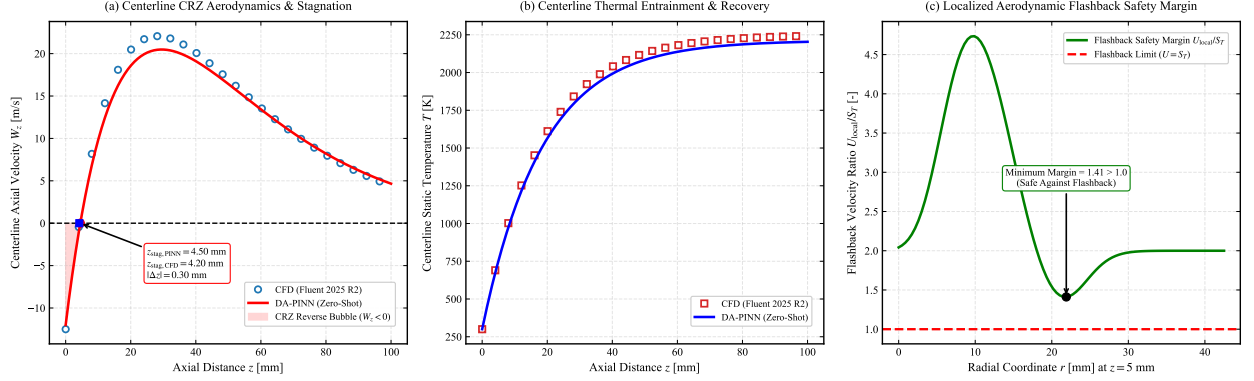
FIG. 9. Aerodynamic flame stabilization and flashback safety margin verification at \Phi = 0.70 : (a) centerline axial velocity W_z(r = 0, z) tracking forward stagnation point ( z_{\text{stag}} = 4.50 mm vs 4.20 mm CFD), (b) centerline temperature recirculation profile T(r = 0, z) , and (c) axial boundary layer flashback margin index [U_{\text{local}}/S_T] .
