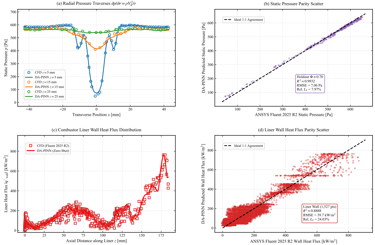
FIG. 8. Aerodynamic static pressure and combustor liner thermal loading verification at \Phi = 0.70 : (a) transverse radial static pressure profiles p(r) across three axial stations ( z = 5, 15, 25 mm) showing vortex core depression; (b) static pressure parity correlation scatter against benchmark CFD ( R^2 = 0.9932 , RMSE = 7.06 Pa); (c) axial distribution of combustor liner wall heat flux q''_{wall}(z) along the outer chamber wall ( r = 42.5 mm); and (d) liner heat flux parity scatter across 1,527 unseen surface coordinates ( R^2 = 0.8453 , RMSE = 46.8 kW/m 2 ).
