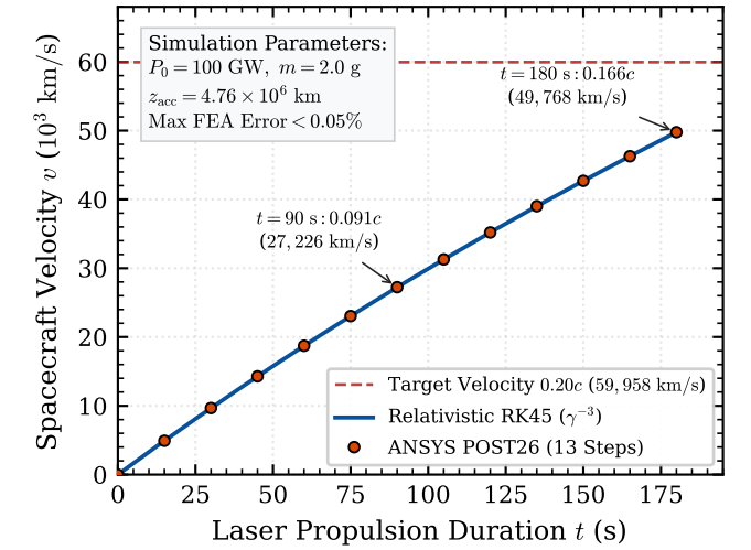
FIG. 5. Relativistic velocity trajectory v(t) over 180 seconds under 100 GW laser thrust, showing theoretical continuum RK45 integration verified against 13 ANSYS Mechanical APDL POST26 discrete finite element load steps (deviation < 0.05\% ).
