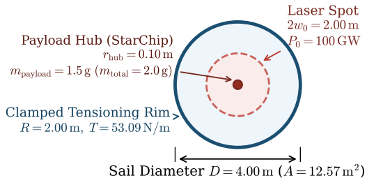
(a) Top-Down Geometric Layout
