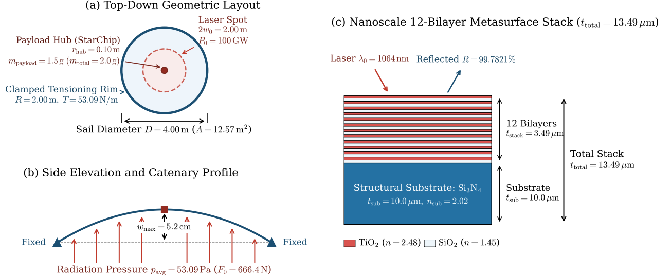
FIG. 1. Dimensioned 2D engineering schematic of the Project Setu 4.0 m circular lightsail showing payload hub ( r_{\text{hub}} = 0.10 m), clamped perimeter ring ( R = 2.00 m), and 12-bilayer \text{TiO}_2/\text{SiO}_2 dielectric metasurface on 10.0\ \mu\text{m} \text{Si}_3\text{N}_4 substrate.
