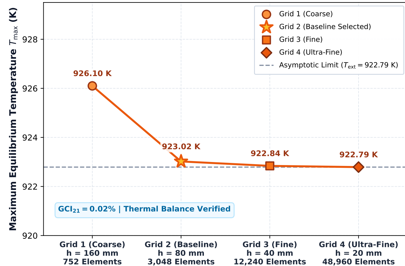
B. 3D Steady-State Thermal Convergence (ANSYS MAPDL)
