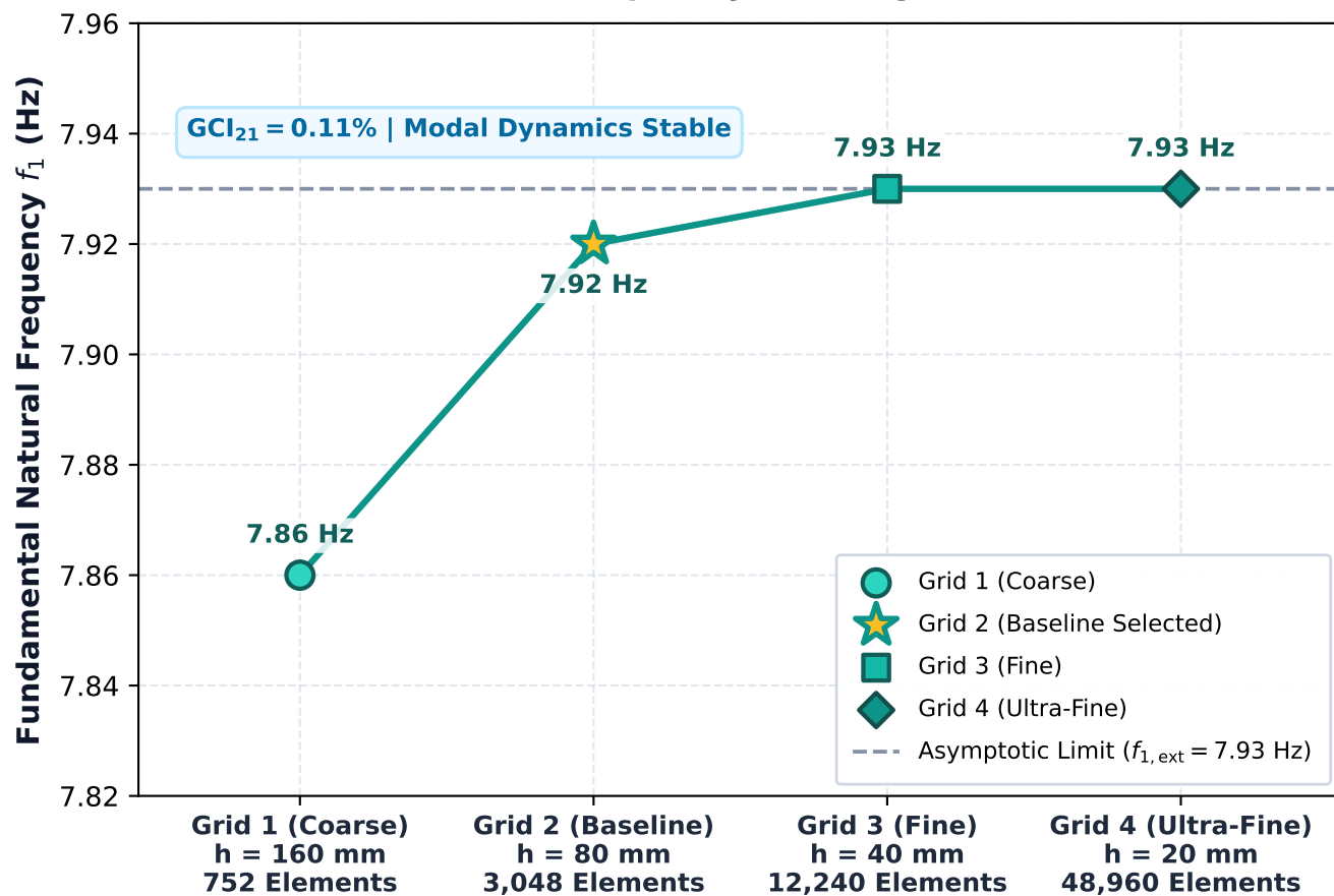
C. 3D Modal Natural Frequency Convergence (ANSYS MAPDL)
