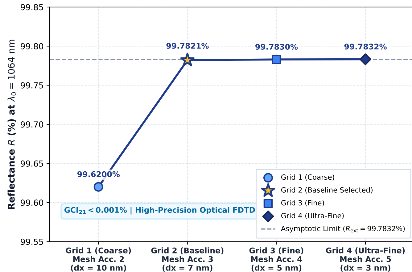
D. 3D Wave Optics FDTD Mesh Convergence (Ansys Lumerical)
