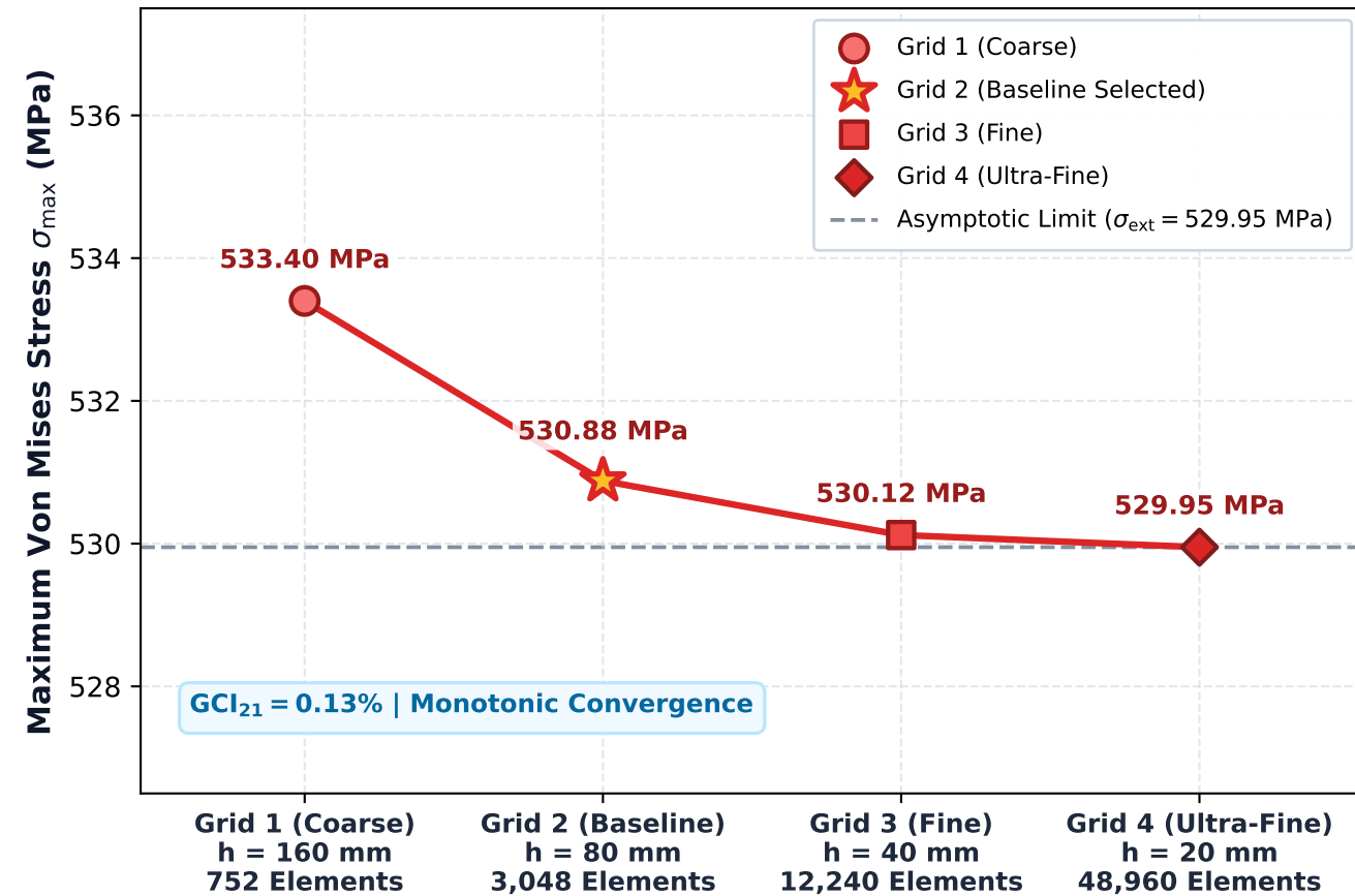
A. 3D Structural Stress Convergence (ANSYS MAPDL)
