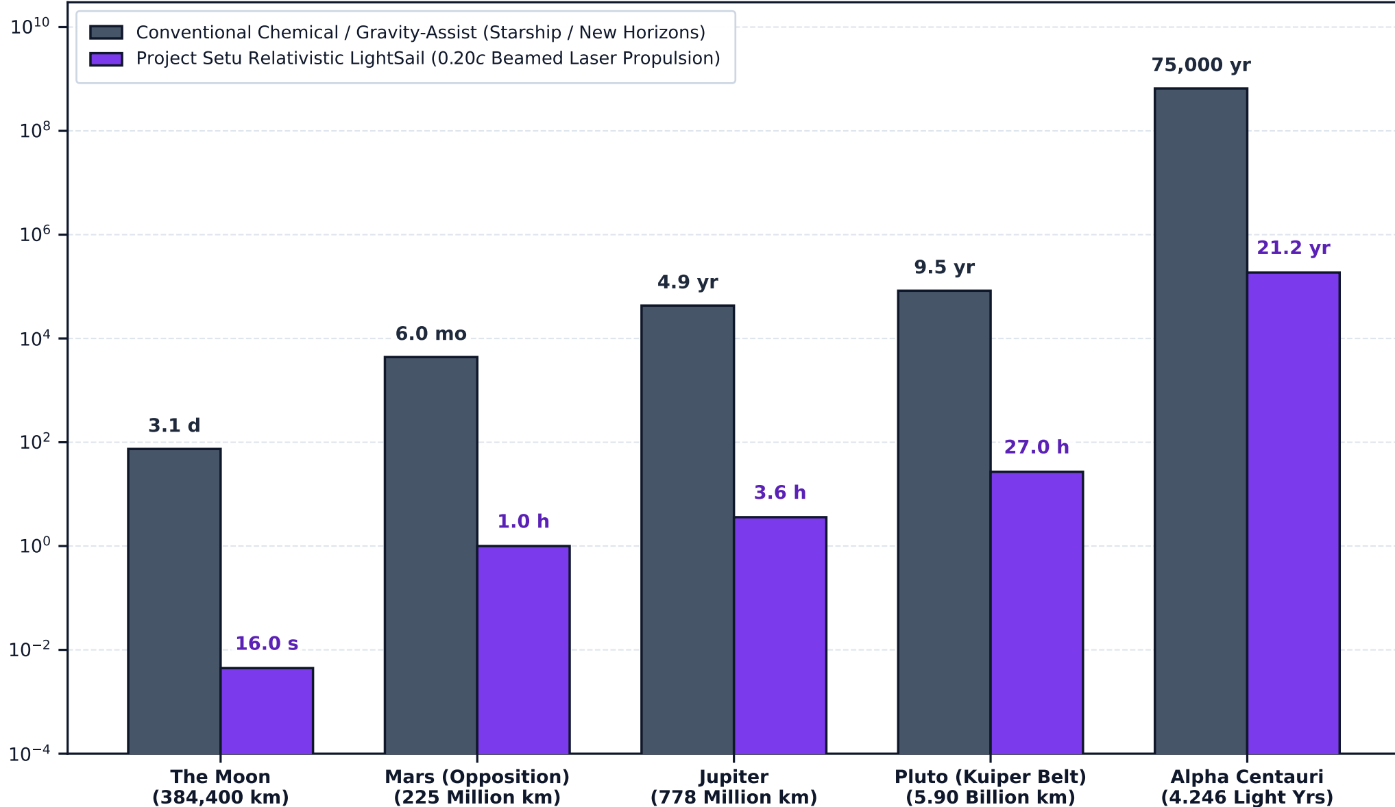
Mission Transit Time (Hours — Logarithmic Scale)
