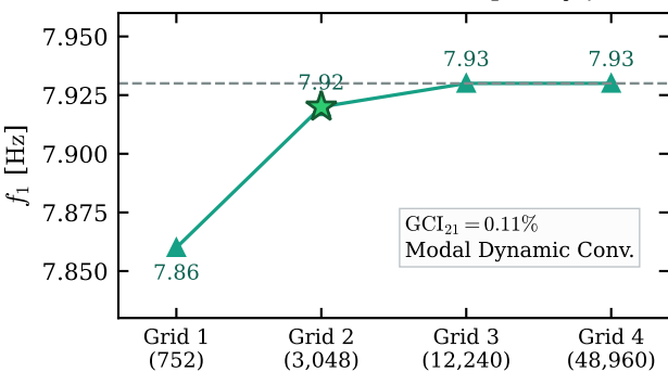
(c) Fundamental Modal Frequency f_1
