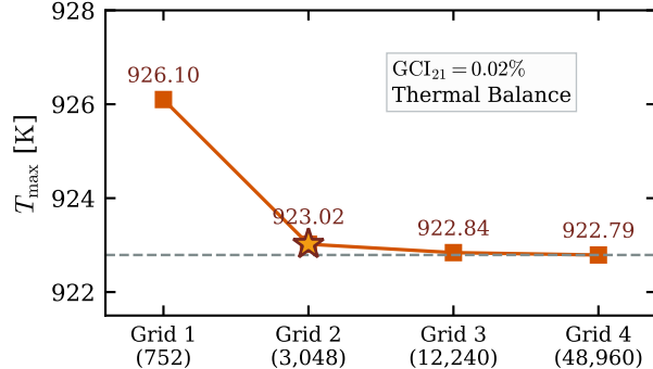
(b) Peak Core Temperature T_{\max}
