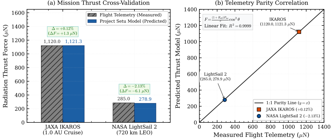
FIG. 12. Empirical cross-validation of radiation pressure propulsion against in-flight telemetry from JAXA IKAROS and NASA LightSail 2 missions.
