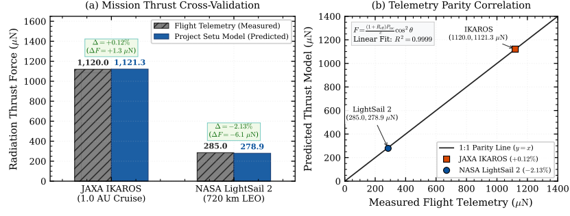
FIG. 12. Empirical cross-validation of radiation pressure propulsion against in-flight telemetry from JAXA IKAROS and NASA LightSail 2 missions.
