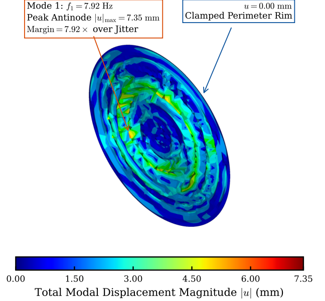
FIG. 11. Fundamental drumhead modal vibration mode shape ( f_1 = 7.92 \text{ Hz} ) extracted via Block Lanczos eigensolver under radiation stress stiffening.
