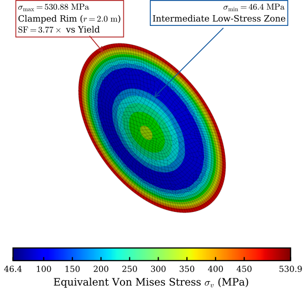
FIG. 10. 3D Structural Stress FEA on ANSYS Mechanical APDL 2025 R2 (SHELL181) displaying peak Von Mises stress of 530.88 MPa at the clamped perimeter.
